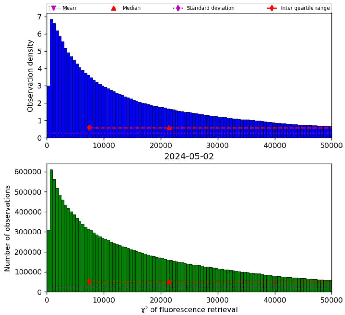
Figure 42: Histogram of “ \chi^2 of fluorescence retrieval” for 2024-05-02 to 2024-05-03
