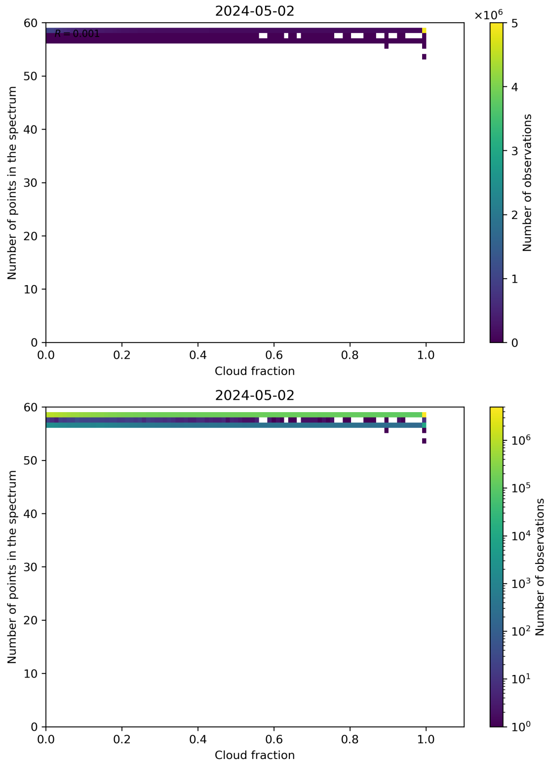
Figure 74: Scatter density plot of “Cloud fraction” against “Number of points in the spectrum” for 2024-05-02 to 2024-05-03.
