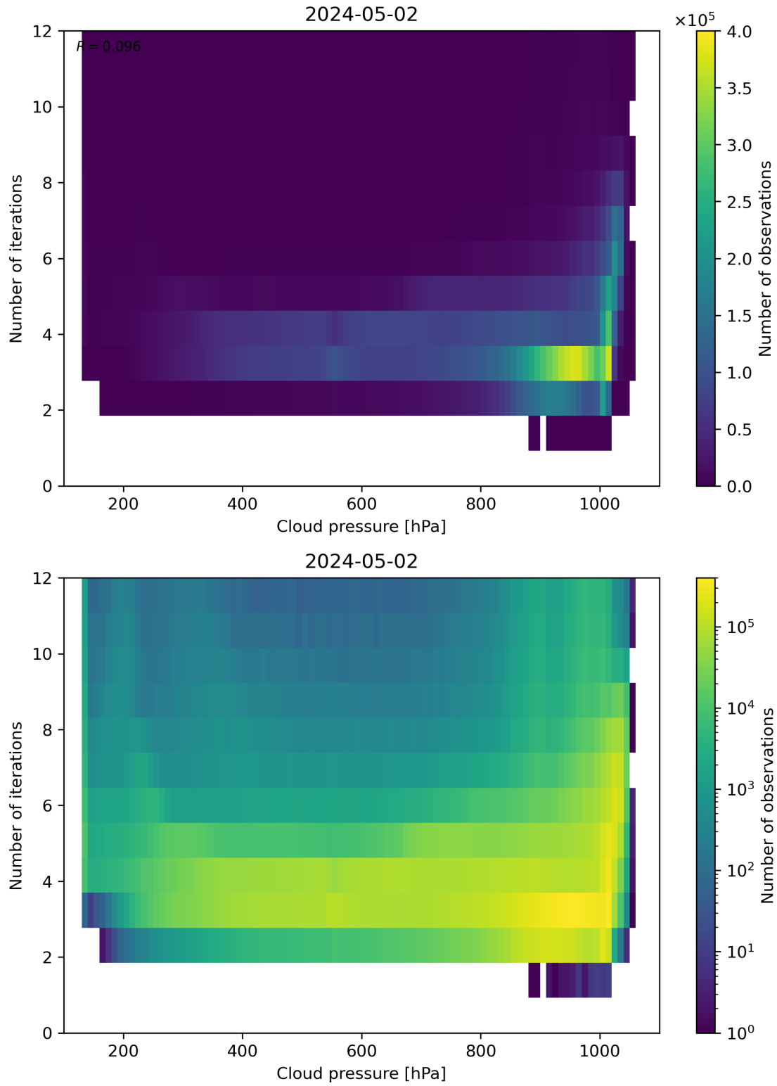
Figure 81: Scatter density plot of “Cloud pressure” against “Number of iterations” for 2024-05-02 to 2024-05-03.
