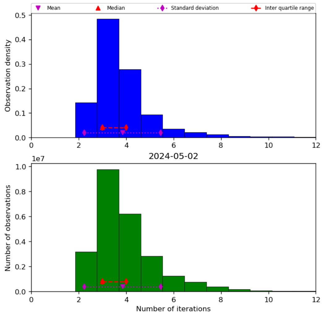
Figure 39: Histogram of “Number of iterations” for 2024-05-02 to 2024-05-03
