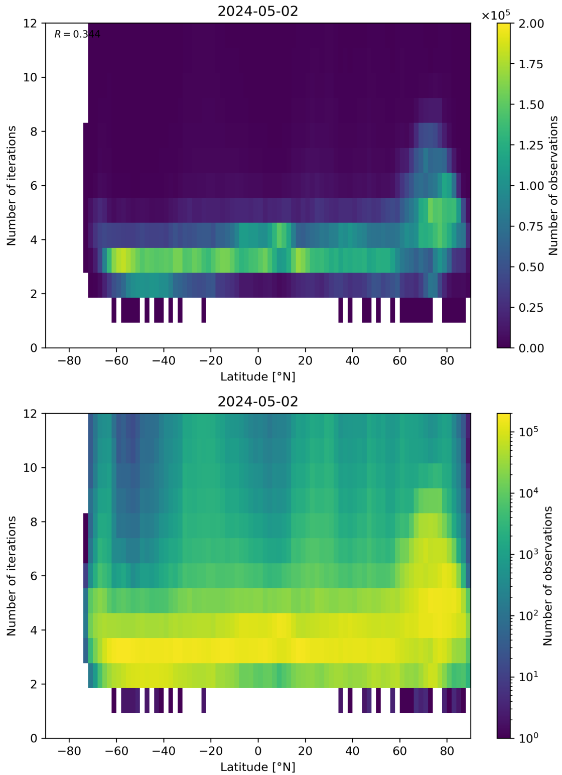
Figure 93: Scatter density plot of “Latitude” against “Number of iterations” for 2024-05-02 to 2024-05-03.
