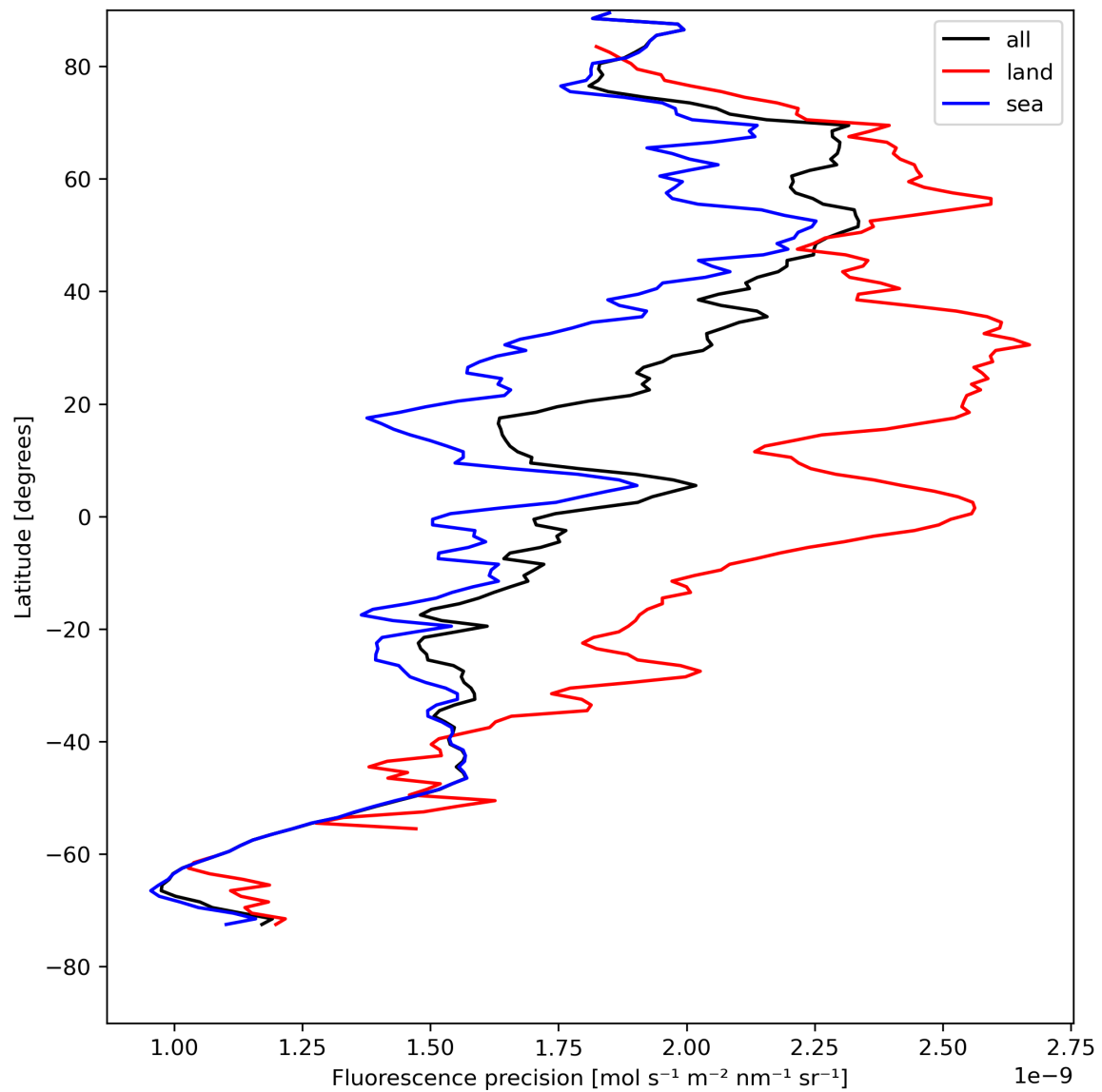
Figure 24: Zonal average of “Fluorescence precision” for 2024-05-02 to 2024-05-03.
