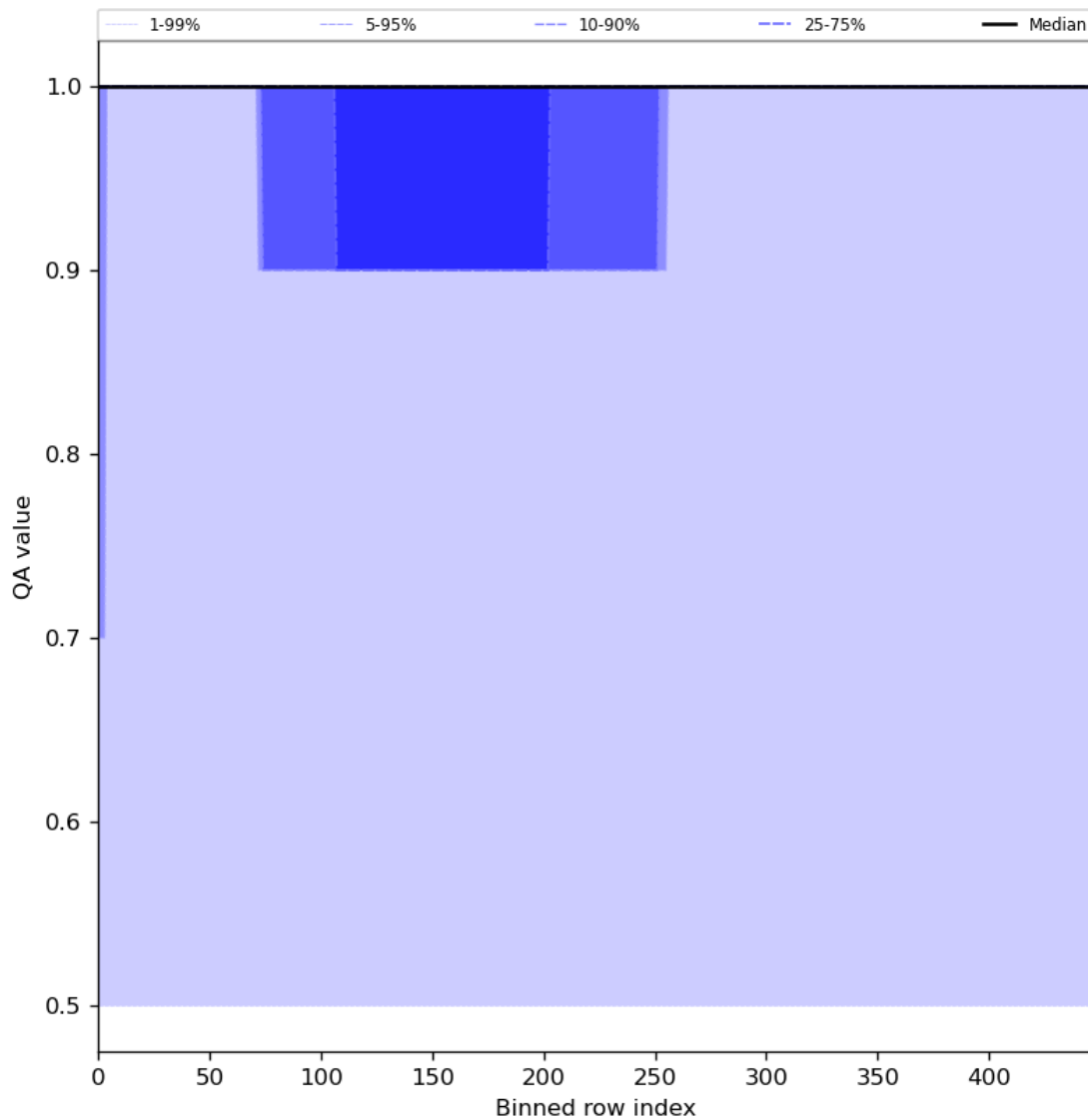
Figure 46: Along track statistics of “QA value” for 2024-05-02 to 2024-05-03
