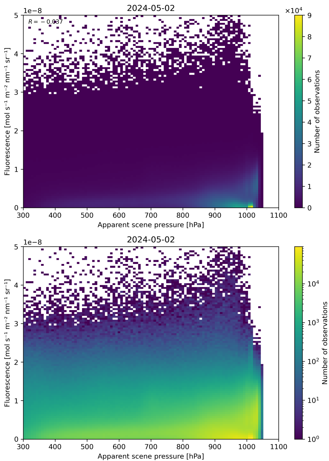
Figure 64: Scatter density plot of “Apparent scene pressure” against “Fluorescence” for 2024-05-02 to 2024-05-03.
