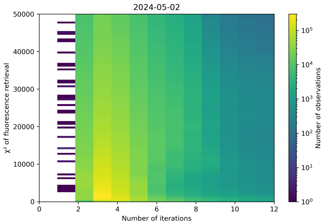
Figure 97: Scatter density plot of “Number of iterations” against “ \chi^2 of fluorescence retrieval” for 2024-05-02 to 2024-05-03.
