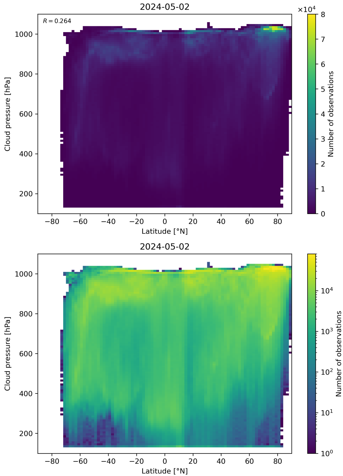
Figure 91: Scatter density plot of “Latitude” against “Cloud pressure” for 2024-05-02 to 2024-05-03.
