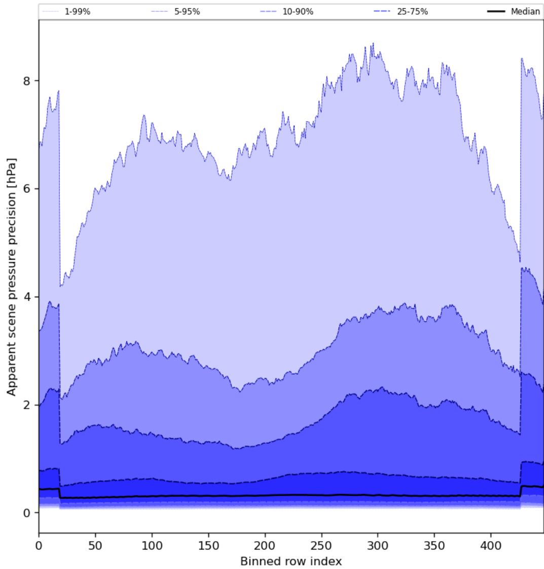
Figure 54: Along track statistics of “Apparent scene pressure precision” for 2024-05-02 to 2024-05-03
