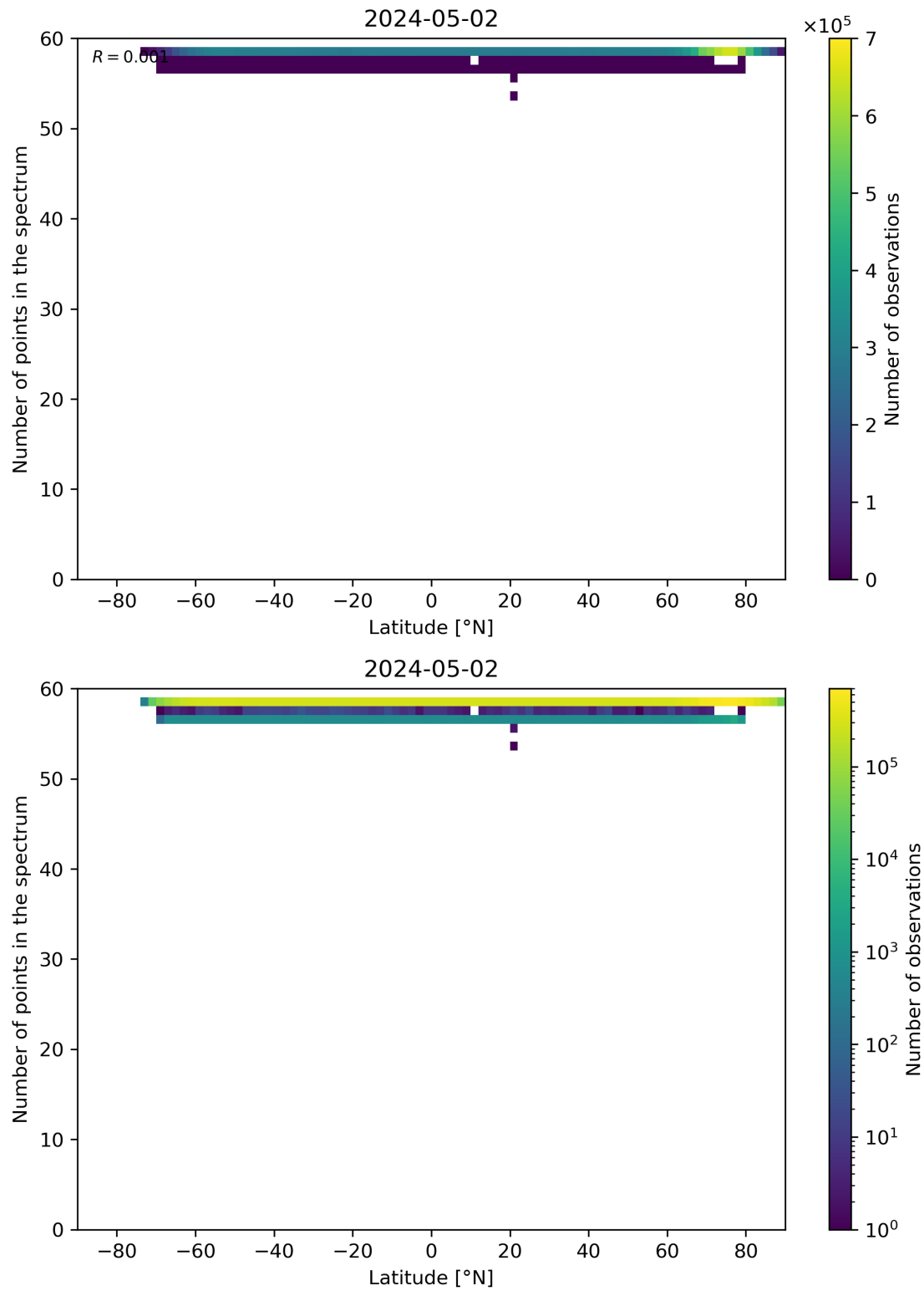
Figure 94: Scatter density plot of “Latitude” against “Number of points in the spectrum” for 2024-05-02 to 2024-05-03.
