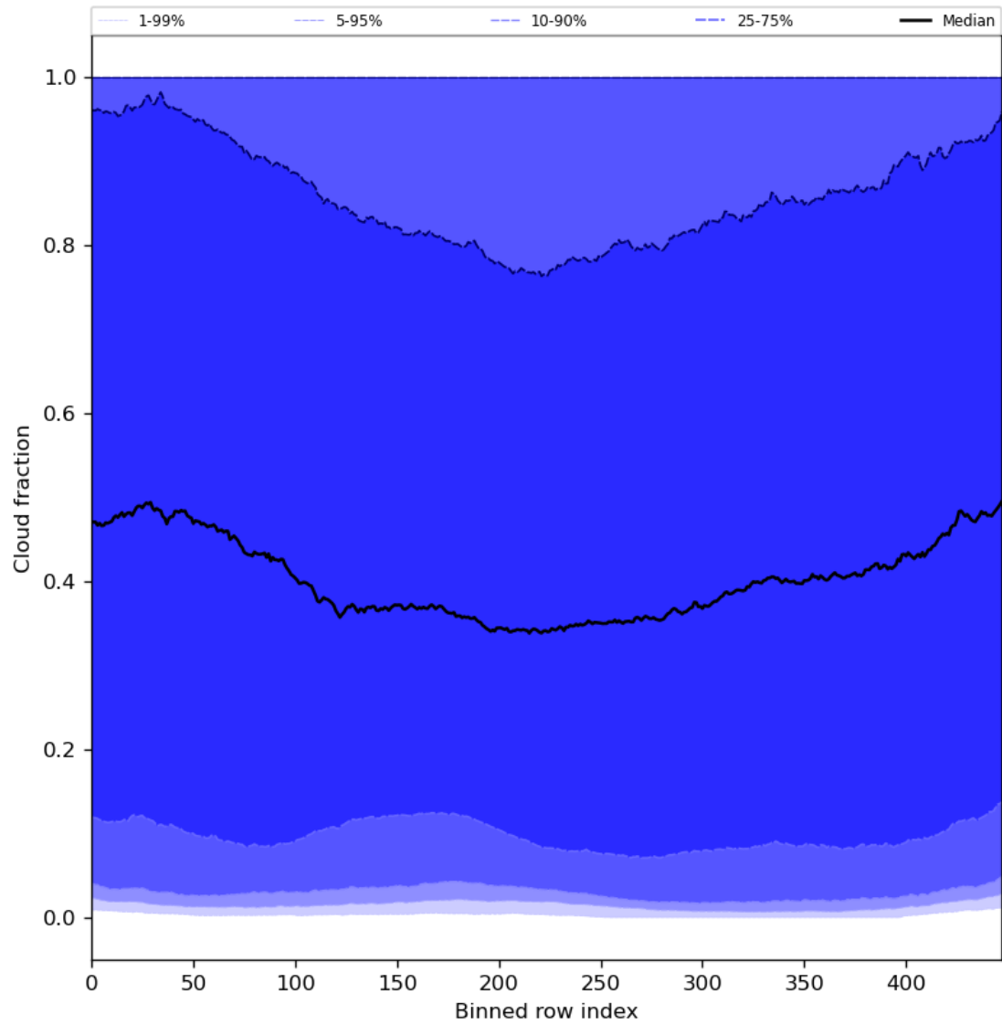
Figure 49: Along track statistics of “Cloud fraction” for 2024-05-02 to 2024-05-03
