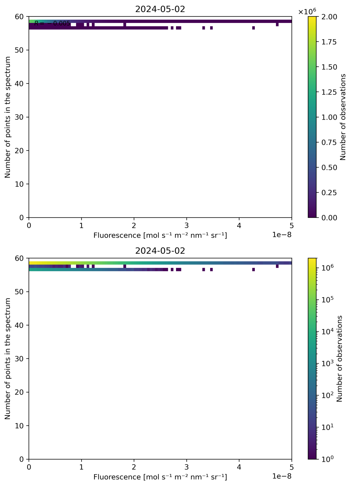
Figure 86: Scatter density plot of “Fluorescence” against “Number of points in the spectrum” for 2024-05-02 to 2024-05-03.
