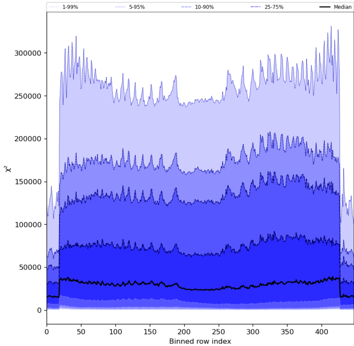
Figure 55: Along track statistics of “ \chi^2 ” for 2024-05-02 to 2024-05-03
