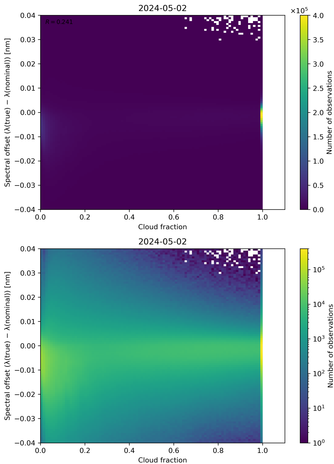
Figure 76: Scatter density plot of “Cloud fraction” against “Spectral offset ( \lambda(\text{true}) - \lambda(\text{nominal}) )” for 2024-05-02 to 2024-05-03.
