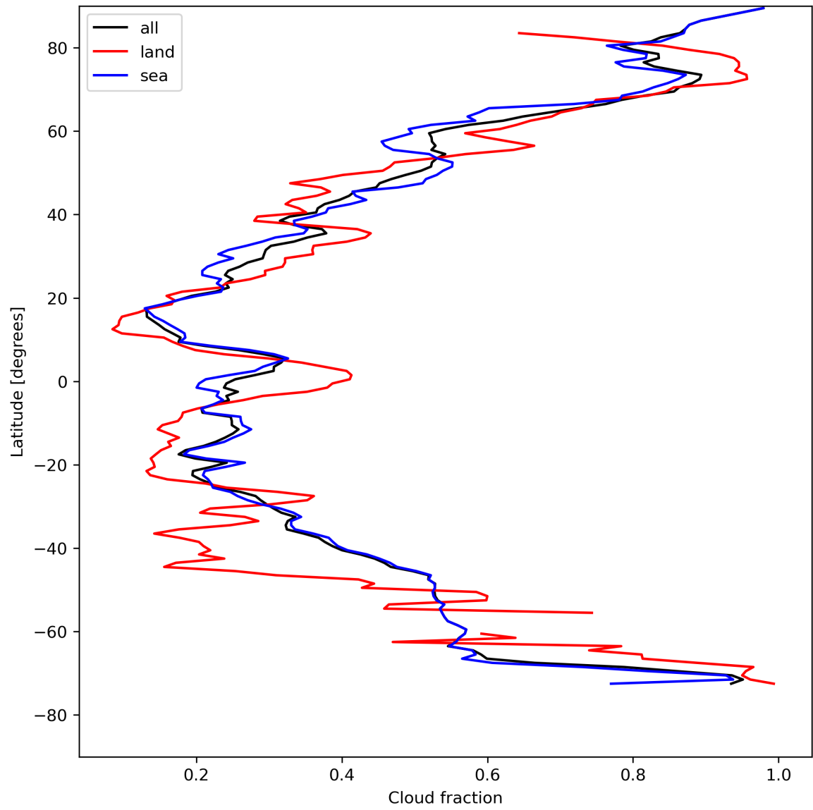
Figure 15: Zonal average of “Cloud fraction” for 2024-05-02 to 2024-05-03.
