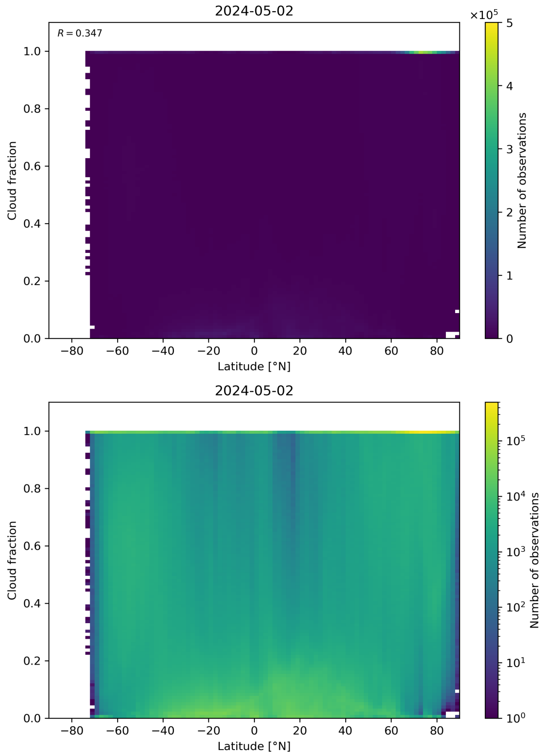
Figure 90: Scatter density plot of “Latitude” against “Cloud fraction” for 2024-05-02 to 2024-05-03.
