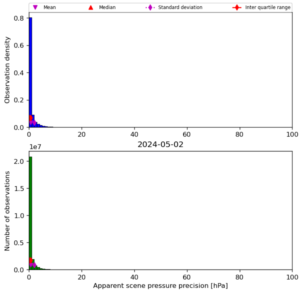
Figure 37: Histogram of “Apparent scene pressure precision” for 2024-05-02 to 2024-05-03
