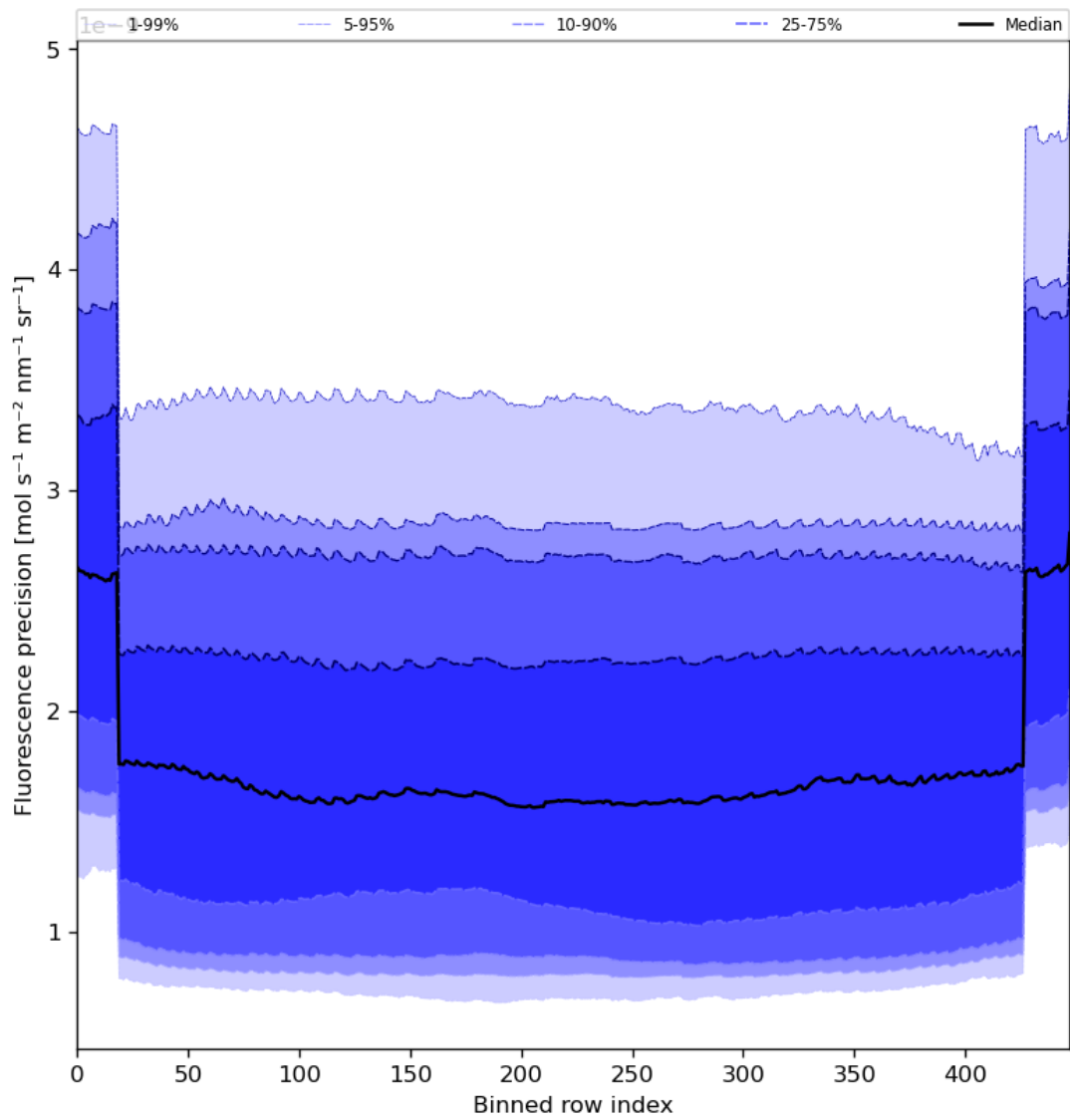
Figure 58: Along track statistics of "Fluorescence precision" for 2024-05-02 to 2024-05-03
