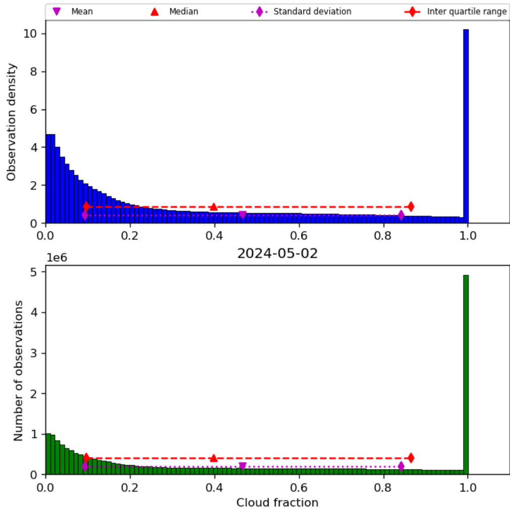
Figure 32: Histogram of "Cloud fraction" for 2024-05-02 to 2024-05-03
