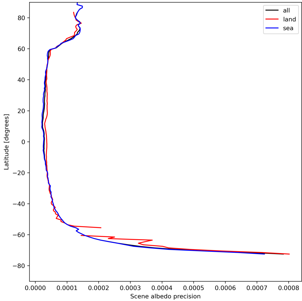
Figure 18: Zonal average of “Scene albedo precision” for 2024-05-02 to 2024-05-03.
