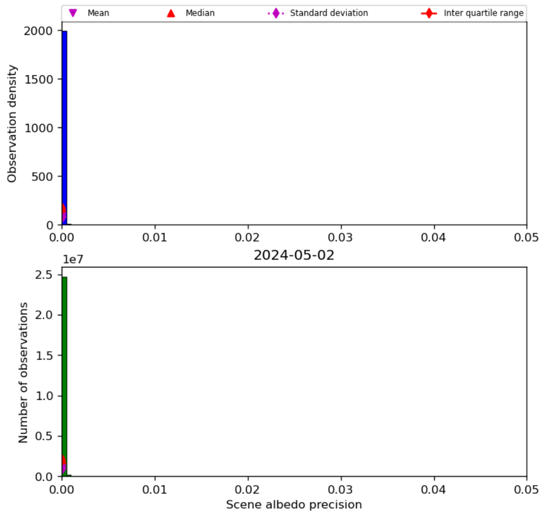
Figure 35: Histogram of “Scene albedo precision” for 2024-05-02 to 2024-05-03
