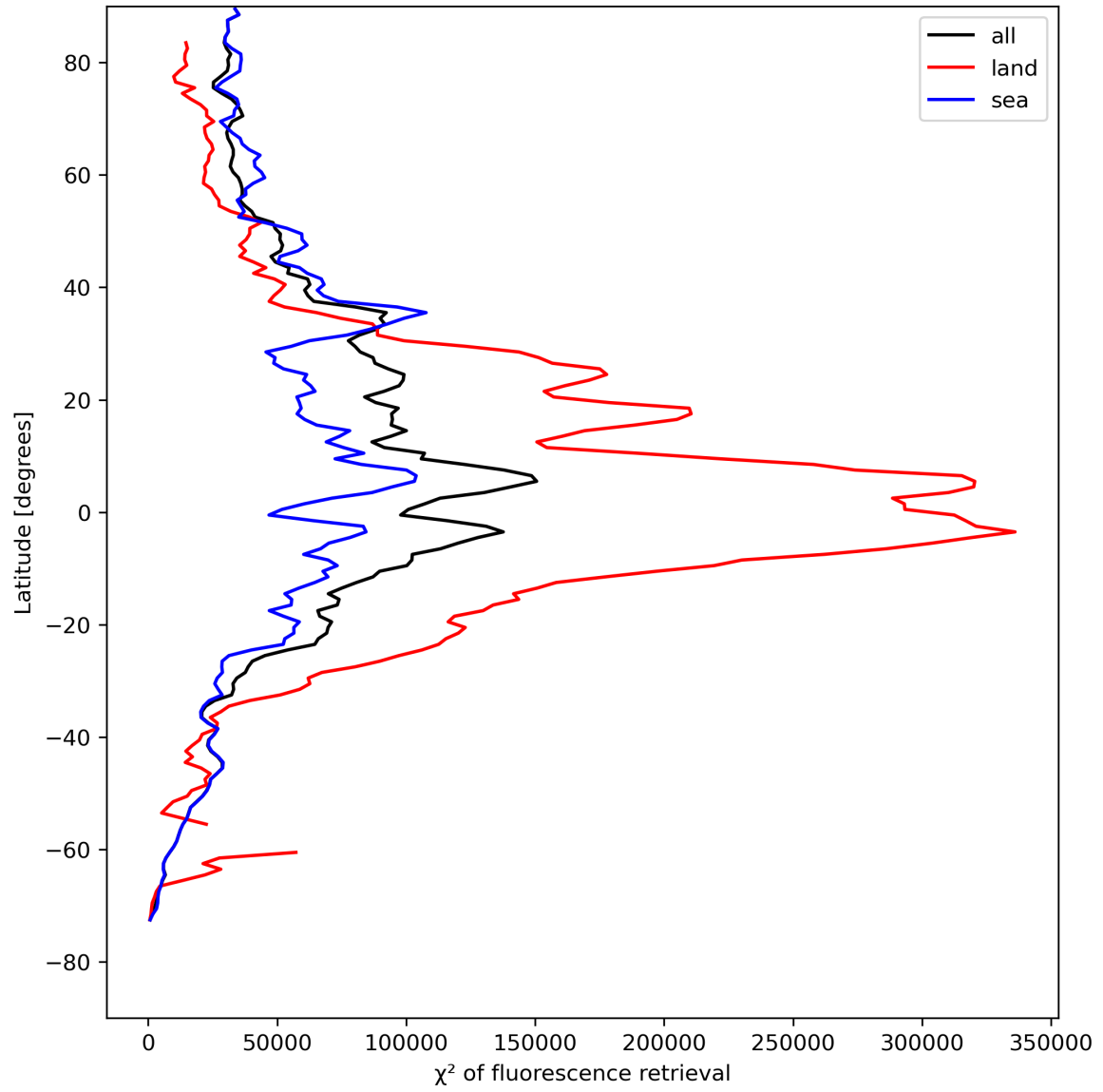
Figure 25: Zonal average of “ \chi^2 of fluorescence retrieval” for 2024-05-02 to 2024-05-03.
