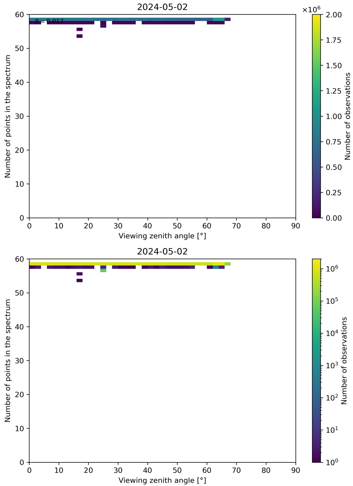
Figure 125: Scatter density plot of “Viewing zenith angle” against “Number of points in the spectrum” for 2024-05-02 to 2024-05-03.
