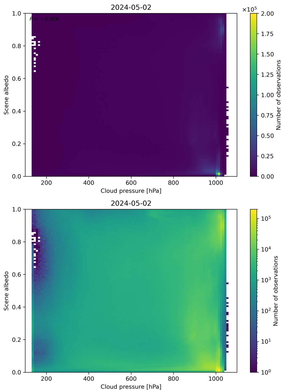
Figure 83: Scatter density plot of “Cloud pressure” against “Scene albedo” for 2024-05-02 to 2024-05-03.
