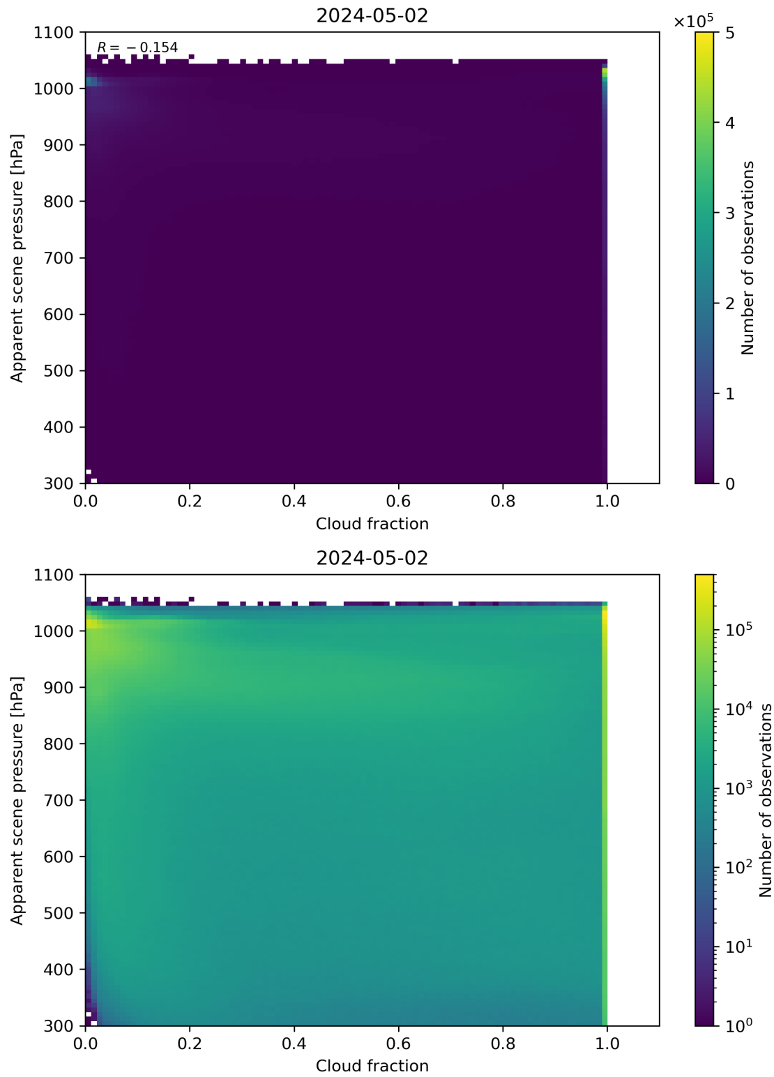
Figure 70: Scatter density plot of “Cloud fraction” against “Apparent scene pressure” for 2024-05-02 to 2024-05-03.
