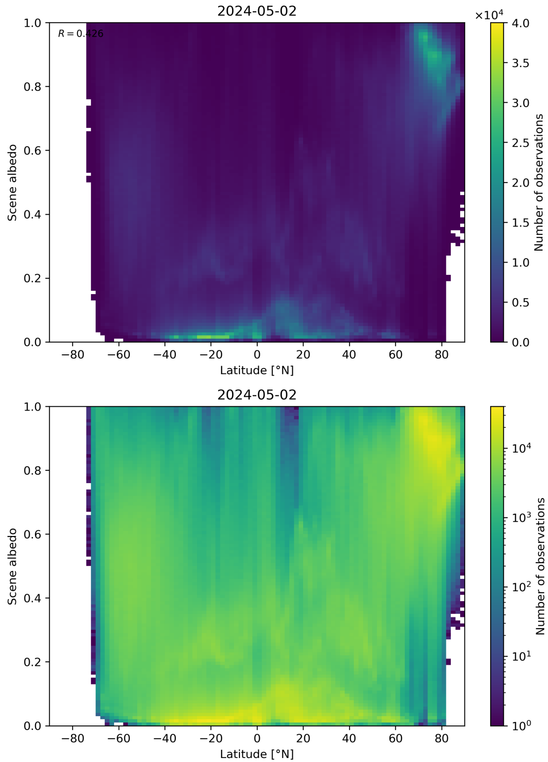
Figure 95: Scatter density plot of “Latitude” against “Scene albedo” for 2024-05-02 to 2024-05-03.
