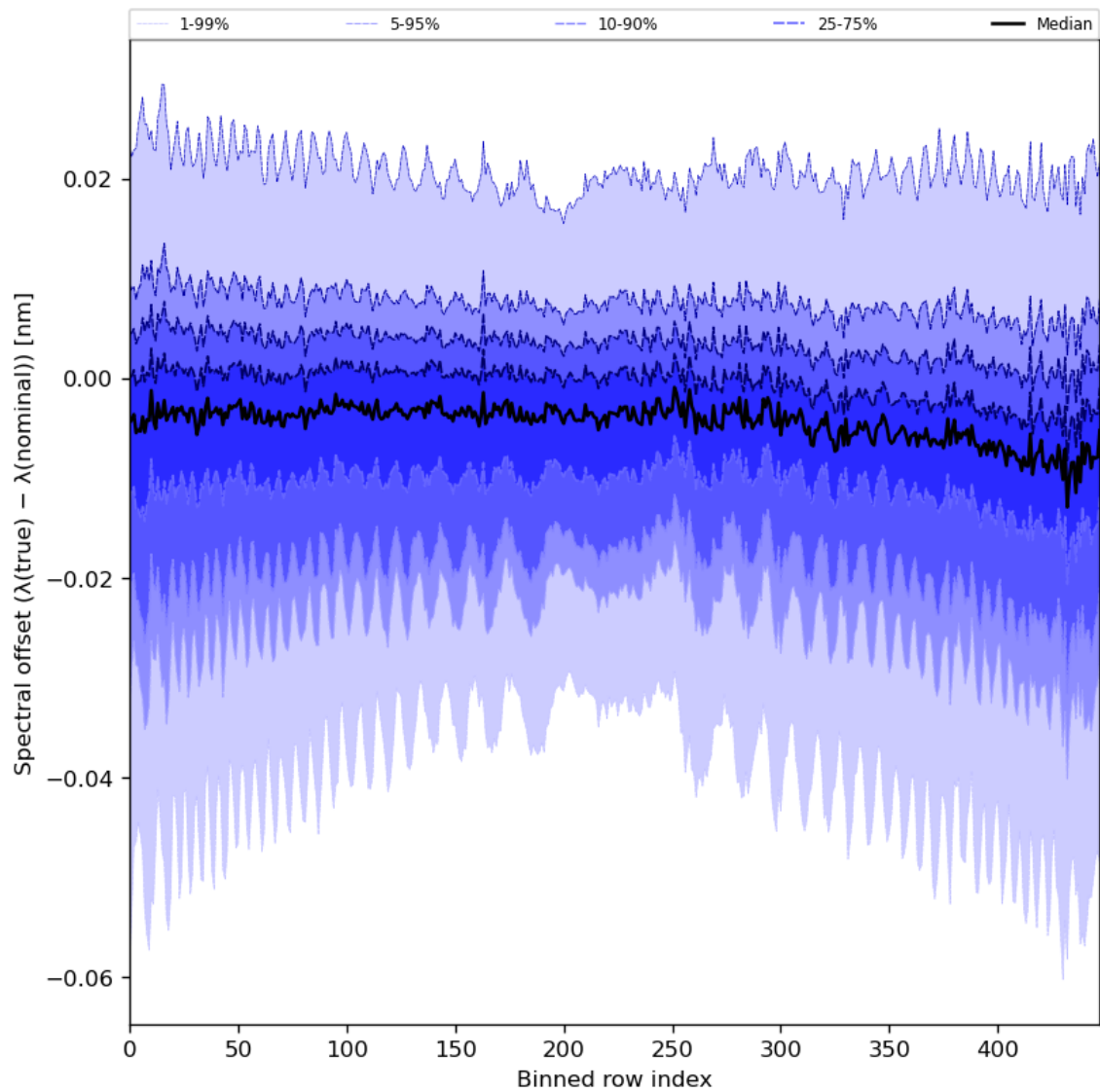
Figure 62: Along track statistics of “Spectral offset ( \lambda(\text{true}) - \lambda(\text{nominal}) )” for 2024-05-02 to 2024-05-03
