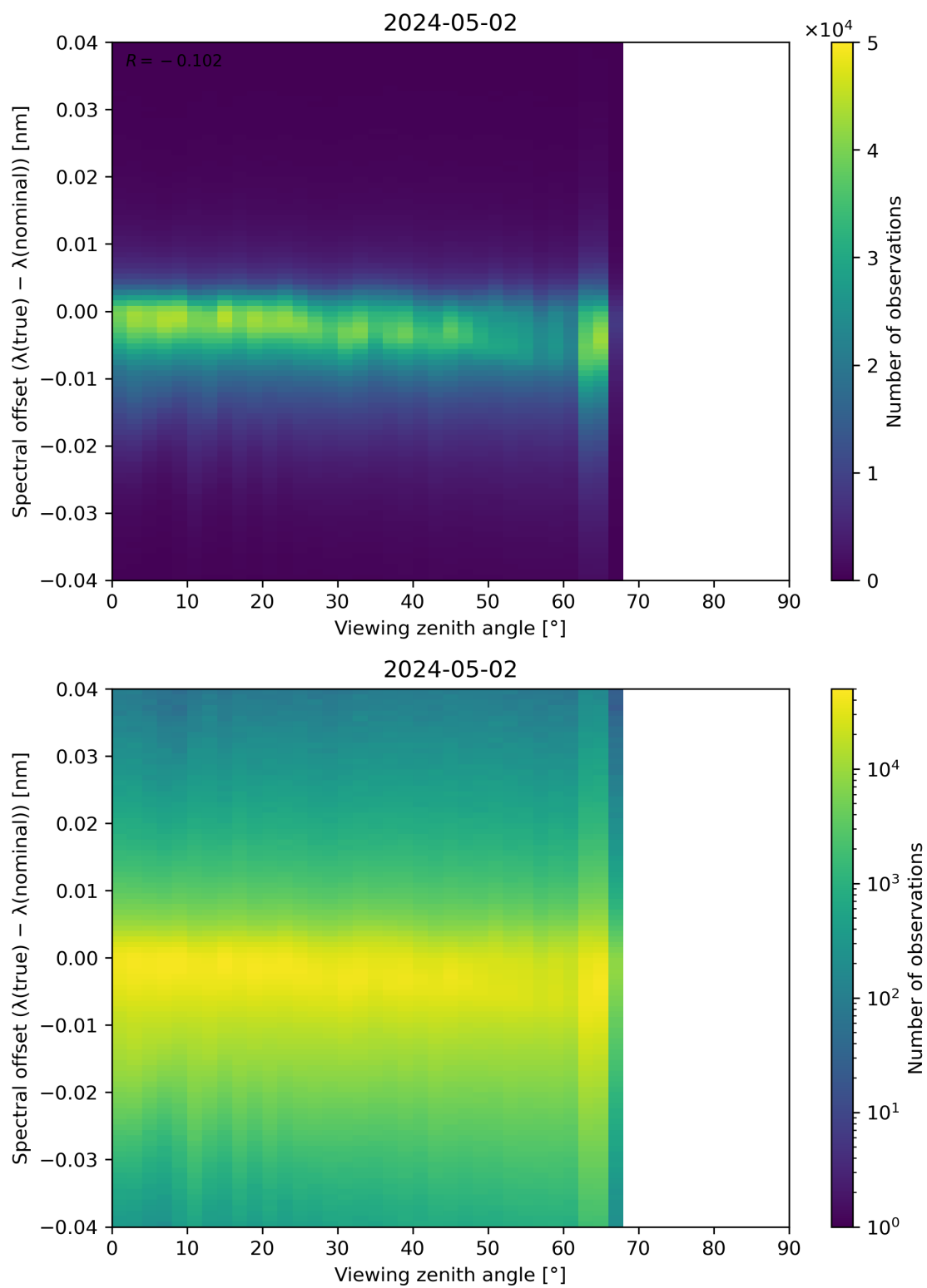
Figure 128: Scatter density plot of “Viewing zenith angle” against “Spectral offset ( \lambda(\text{true}) - \lambda(\text{nominal}) )” for 2024-05-02 to 2024-05-03.
