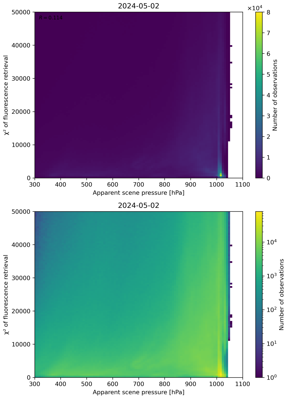
Figure 63: Scatter density plot of “Apparent scene pressure” against “ \chi^2 of fluorescence retrieval” for 2024-05-02 to 2024-05-03.
