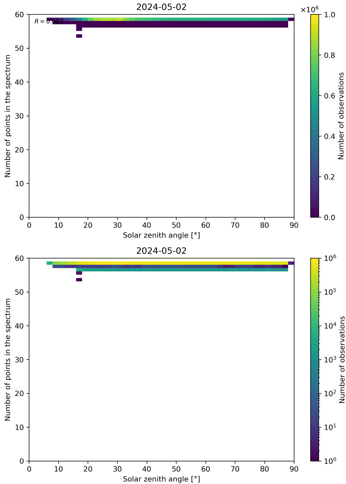
Figure 115: Scatter density plot of “Solar zenith angle” against “Number of points in the spectrum” for 2024-05-02 to 2024-05-03.
