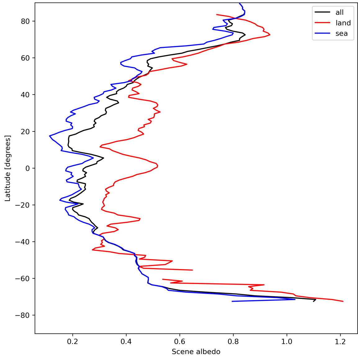
Figure 17: Zonal average of “Scene albedo” for 2024-05-02 to 2024-05-03.
