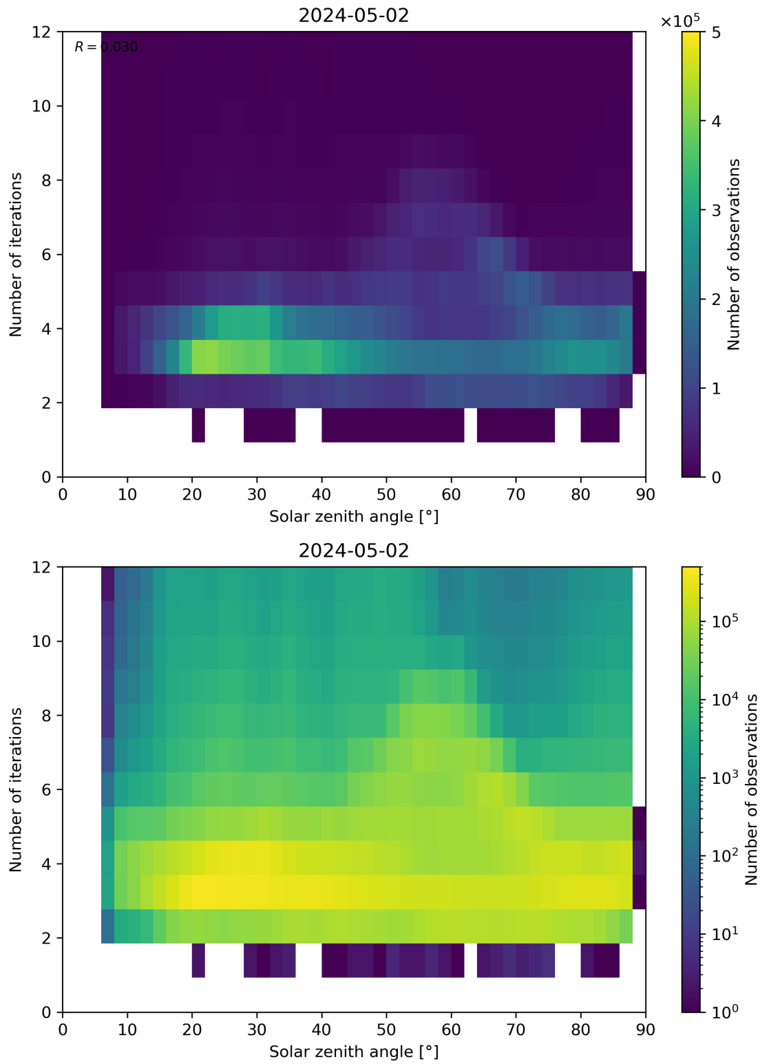
Figure 114: Scatter density plot of “Solar zenith angle” against “Number of iterations” for 2024-05-02 to 2024-05-03.
