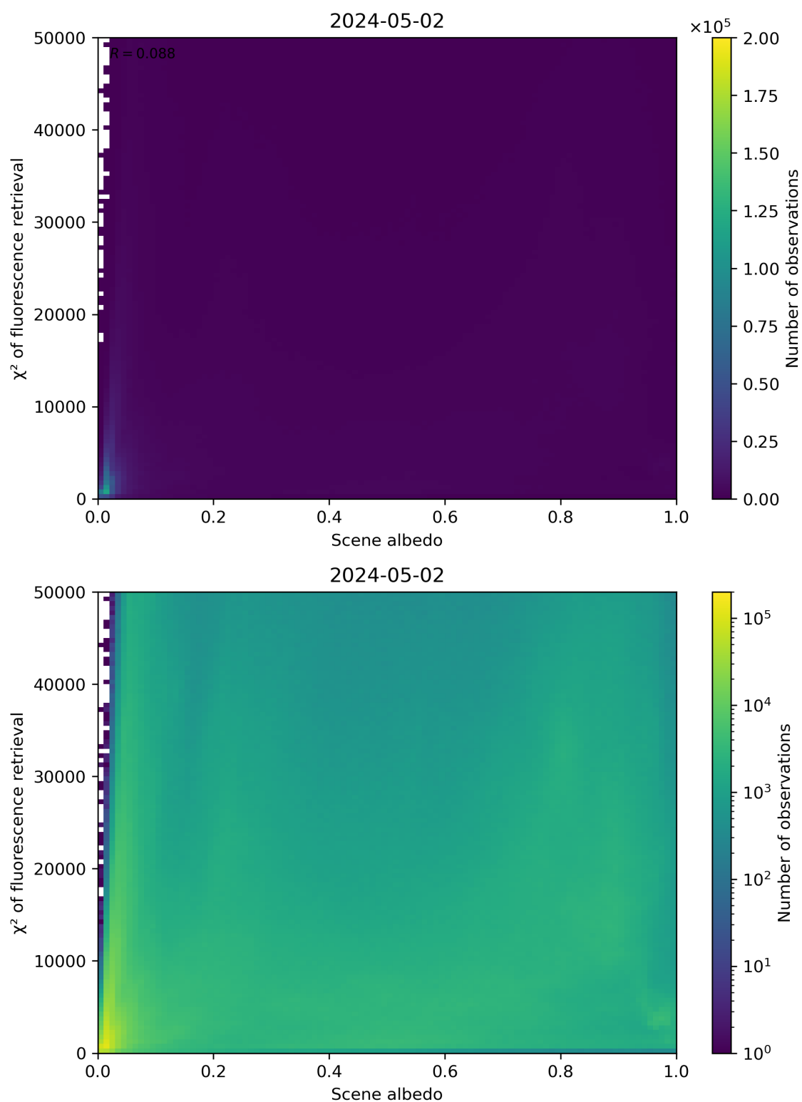
Figure 103: Scatter density plot of “Scene albedo” against “ \chi^2 of fluorescence retrieval” for 2024-05-02 to 2024-05-03.
