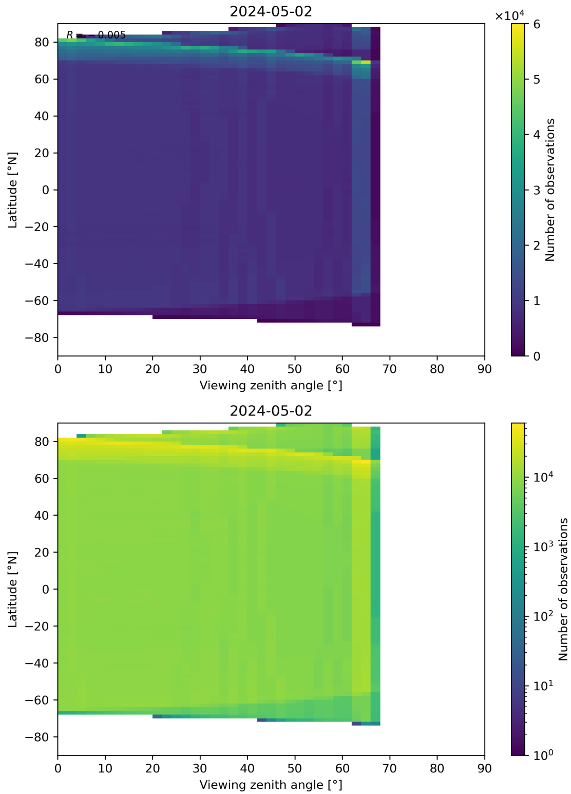
Figure 123: Scatter density plot of “Viewing zenith angle” against “Latitude” for 2024-05-02 to 2024-05-03.
