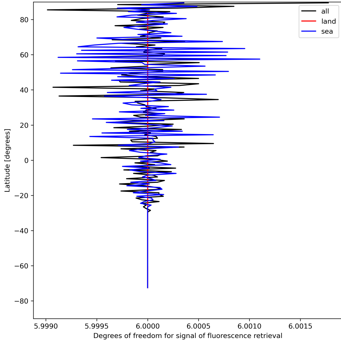
Figure 26: Zonal average of “Degrees of freedom for signal of fluorescence retrieval” for 2024-05-02 to 2024-05-03.
