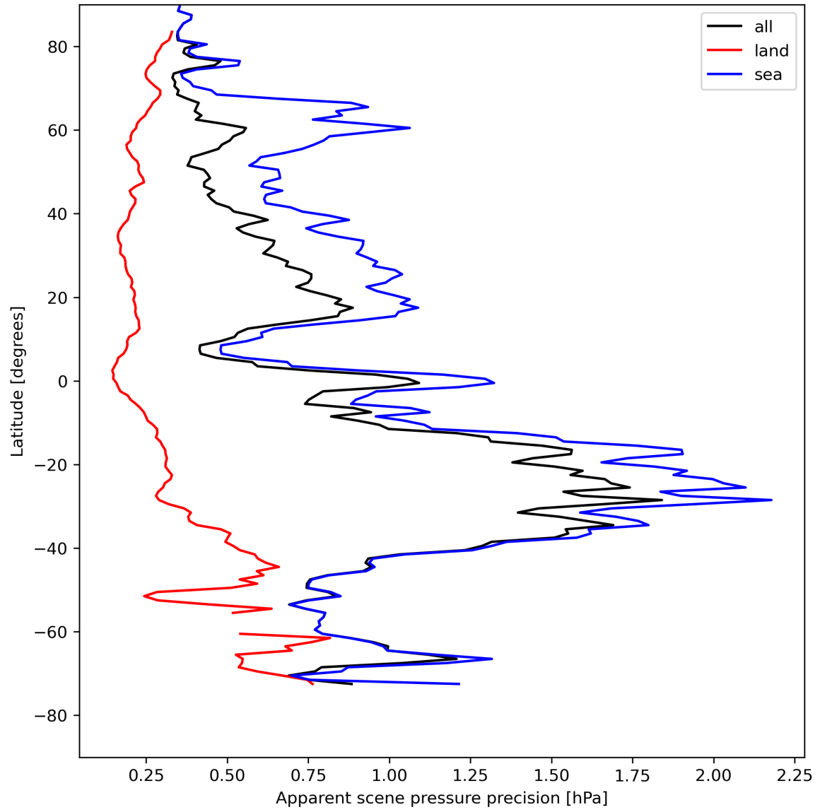
Figure 20: Zonal average of “Apparent scene pressure precision” for 2024-05-02 to 2024-05-03.
