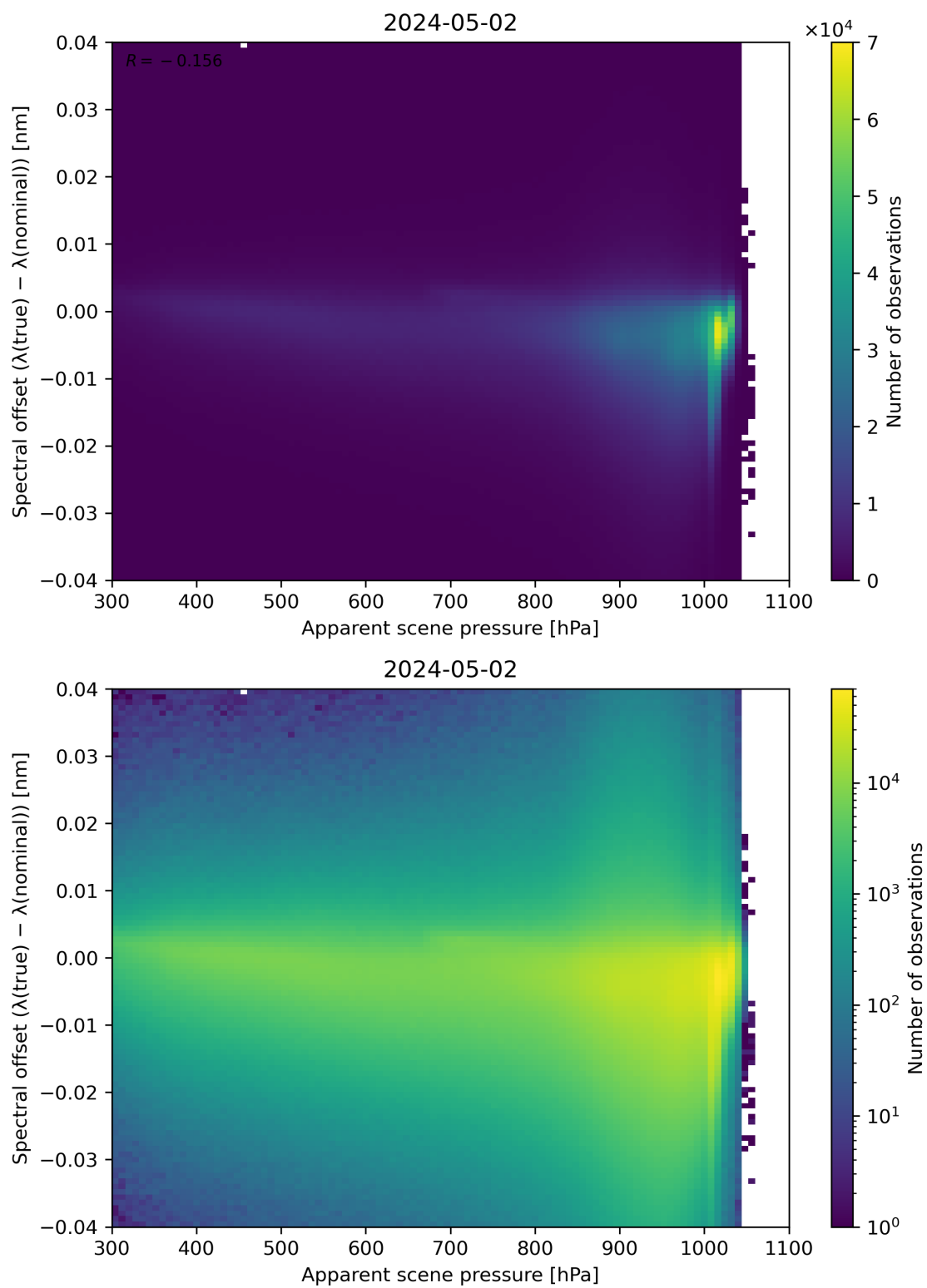
Figure 67: Scatter density plot of “Apparent scene pressure” against “Spectral offset ( \lambda(\text{true}) - \lambda(\text{nominal}) )” for 2024-05-02 to 2024-05-03.
