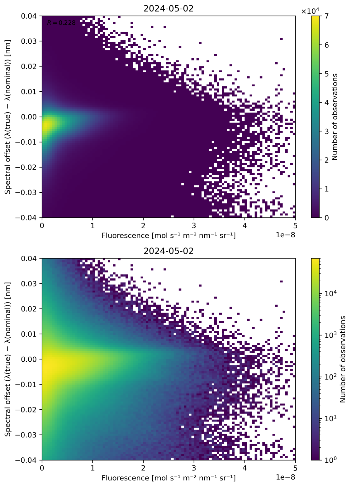
Figure 87: Scatter density plot of “Fluorescence” against “Spectral offset ( \lambda(\text{true}) - \lambda(\text{nominal}) )” for 2024-05-02 to 2024-05-03.
