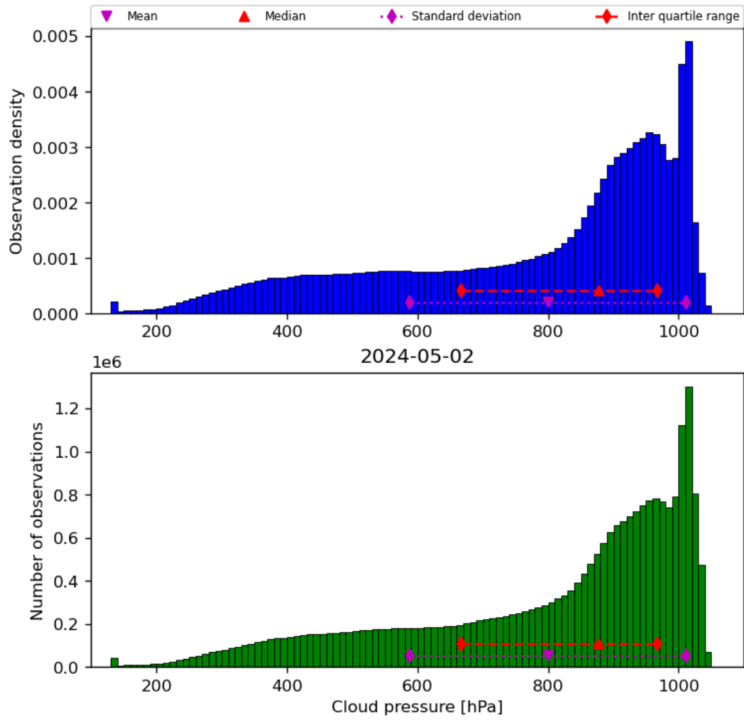
Figure 30: Histogram of “Cloud pressure” for 2024-05-02 to 2024-05-03
