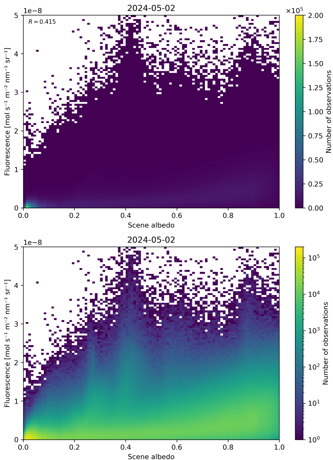
Figure 104: Scatter density plot of “Scene albedo” against “Fluorescence” for 2024-05-02 to 2024-05-03.
