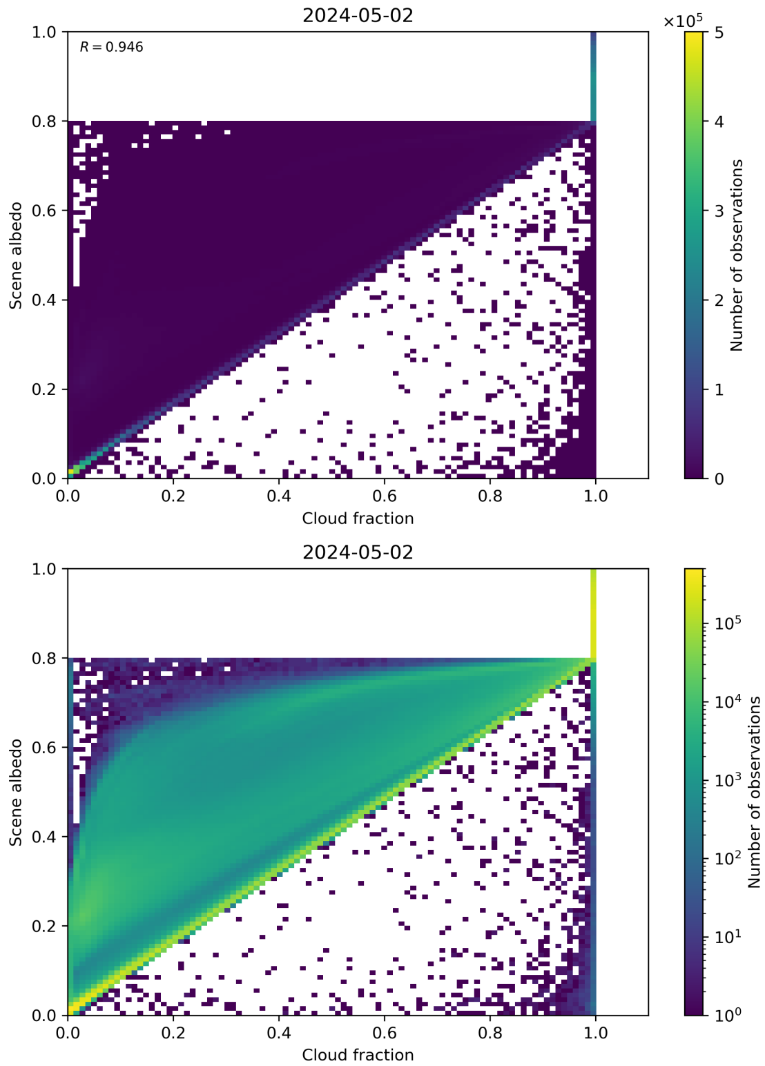
Figure 75: Scatter density plot of “Cloud fraction” against “Scene albedo” for 2024-05-02 to 2024-05-03.
