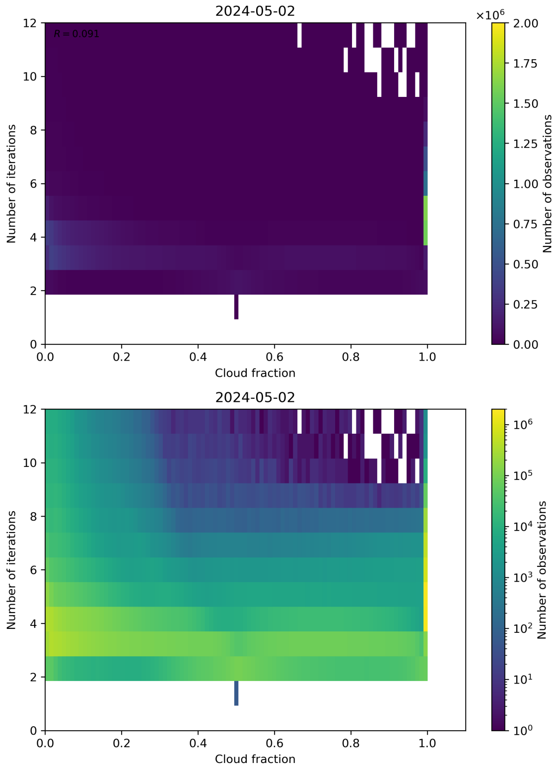
Figure 73: Scatter density plot of “Cloud fraction” against “Number of iterations” for 2024-05-02 to 2024-05-03.
