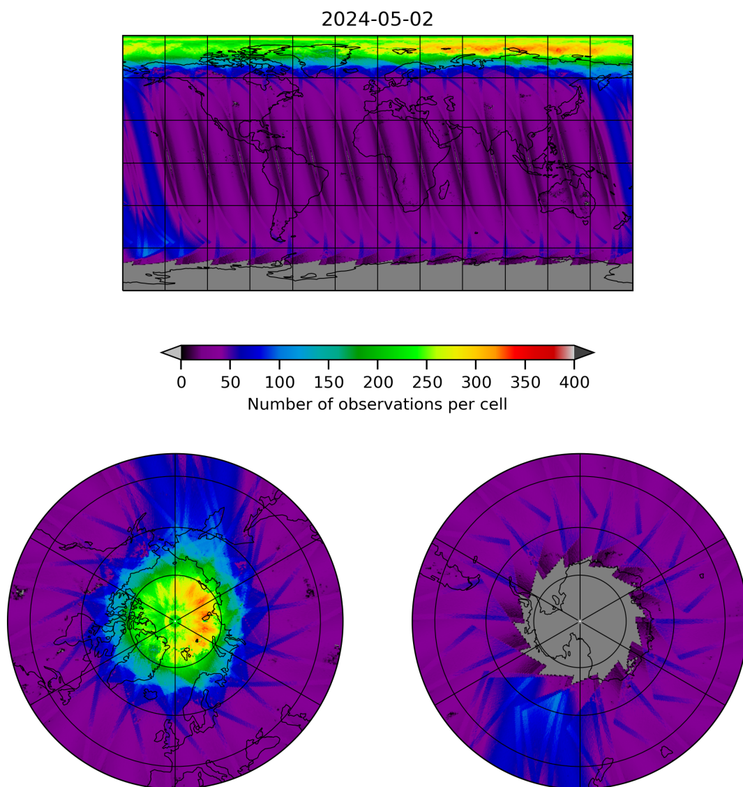
Figure 11: Map of the number of observations for 2024-05-02 to 2024-05-03
