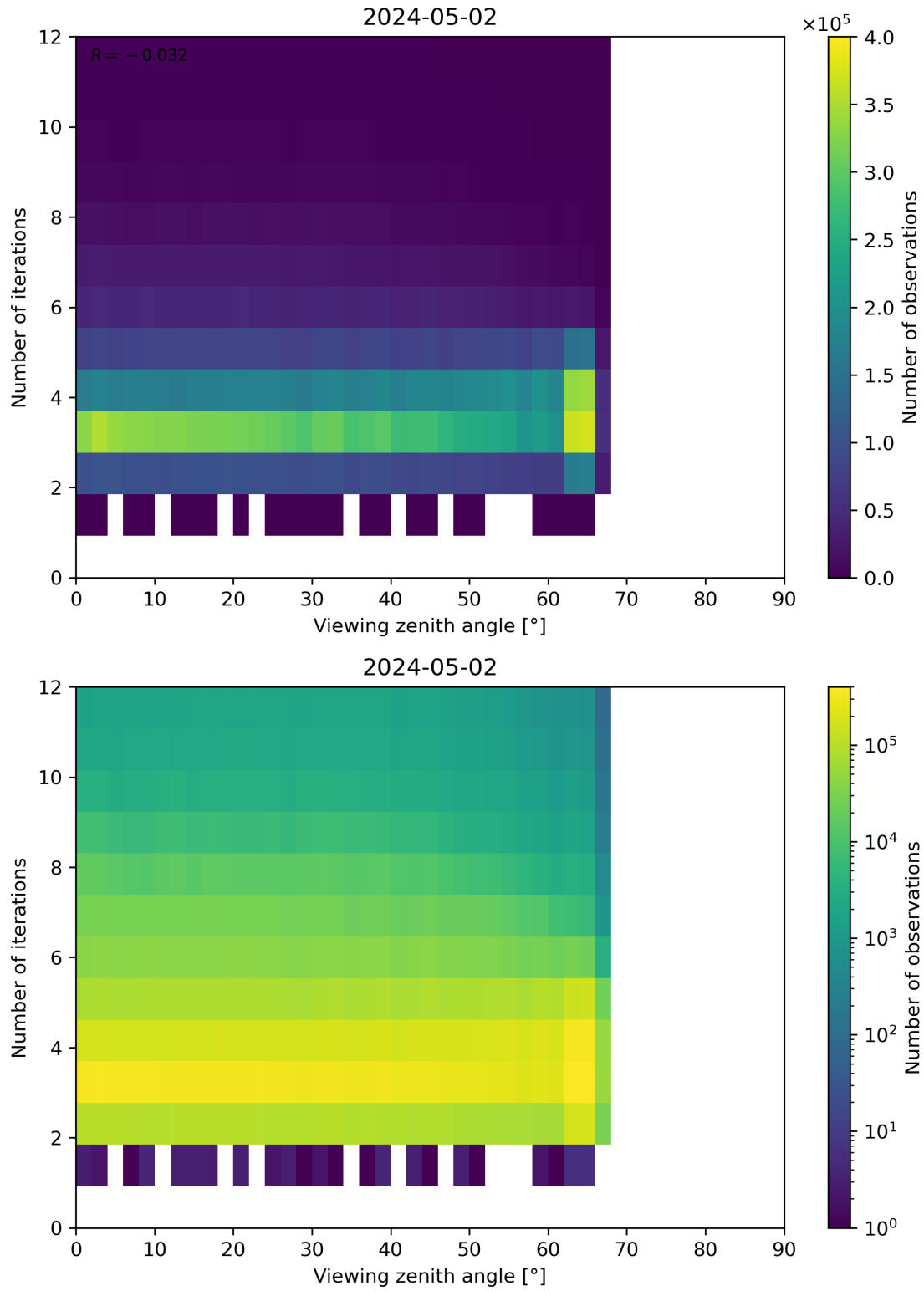
Figure 124: Scatter density plot of “Viewing zenith angle” against “Number of iterations” for 2024-05-02 to 2024-05-03.
