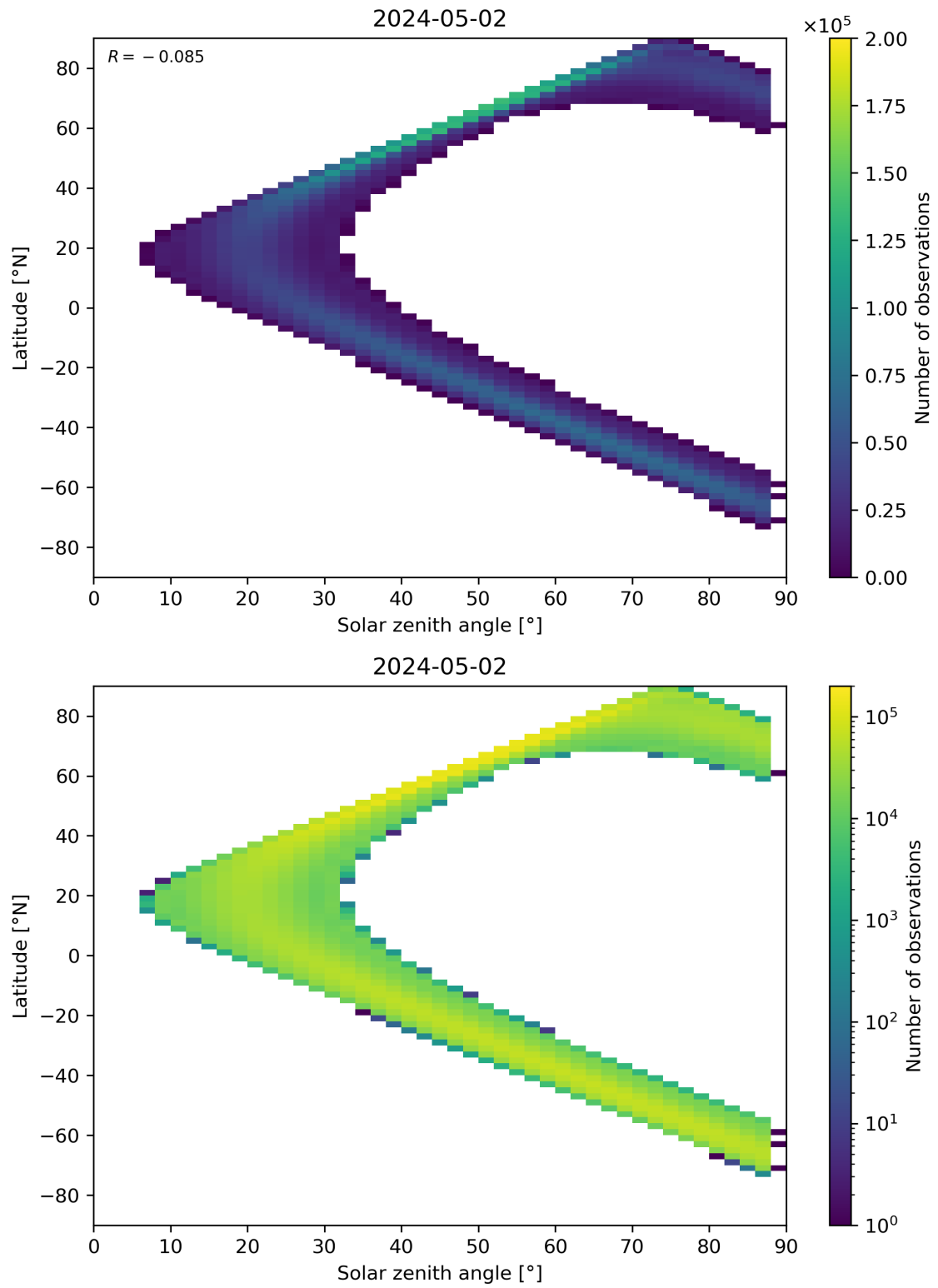
Figure 113: Scatter density plot of “Solar zenith angle” against “Latitude” for 2024-05-02 to 2024-05-03.
