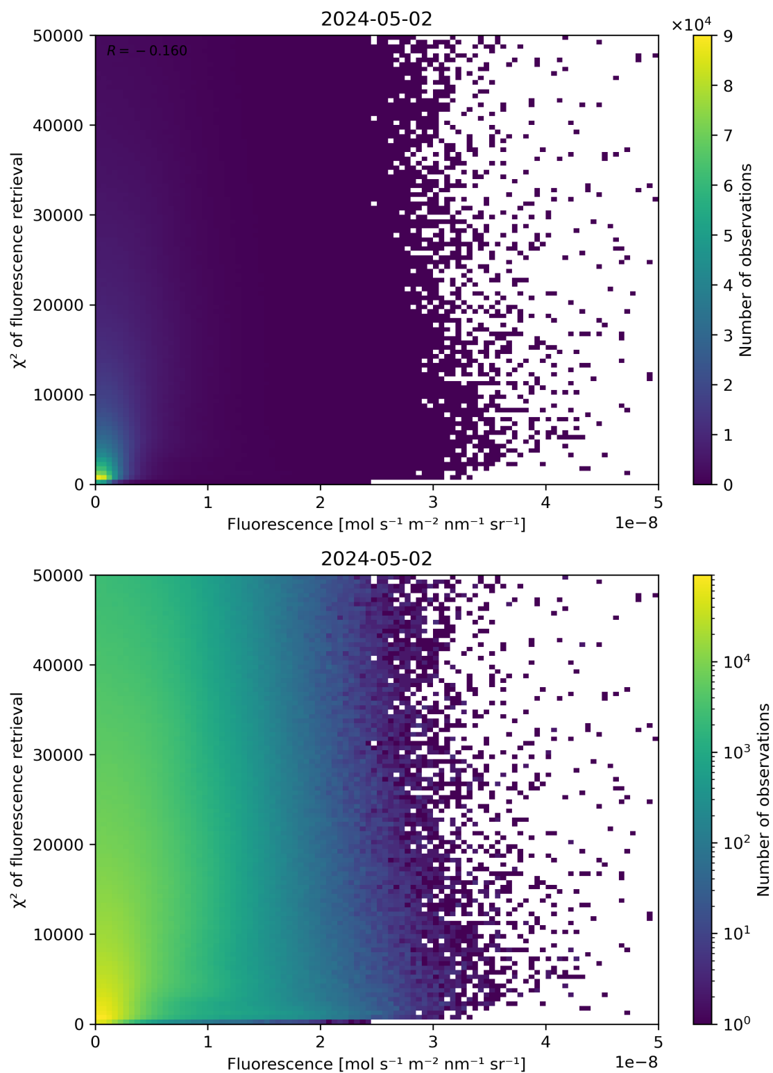
Figure 85: Scatter density plot of “Fluorescence” against “ \chi^2 of fluorescence retrieval” for 2024-05-02 to 2024-05-03.
