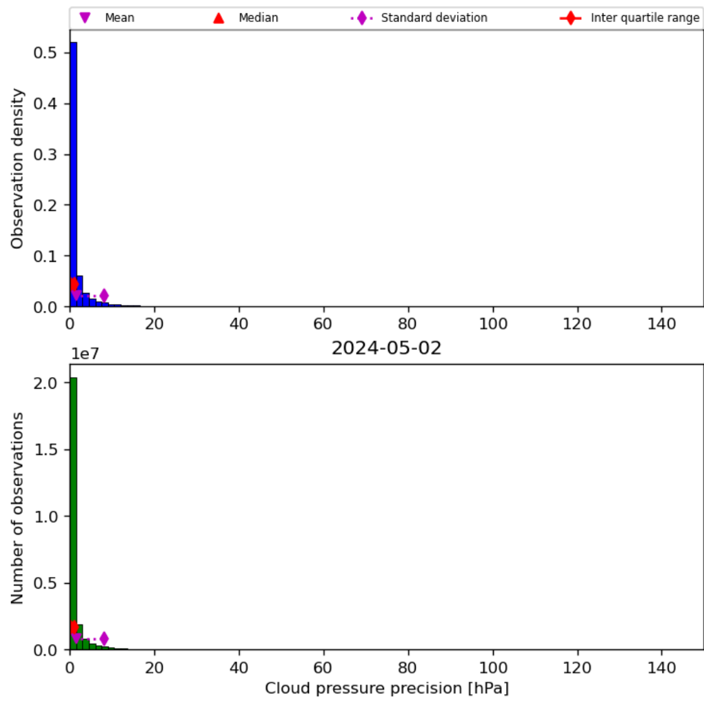
Figure 31: Histogram of “Cloud pressure precision” for 2024-05-02 to 2024-05-03
