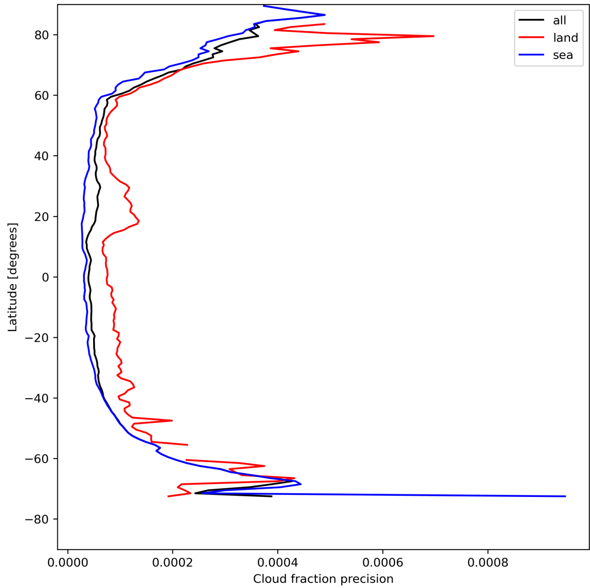
Figure 16: Zonal average of “Cloud fraction precision” for 2024-05-02 to 2024-05-03.
