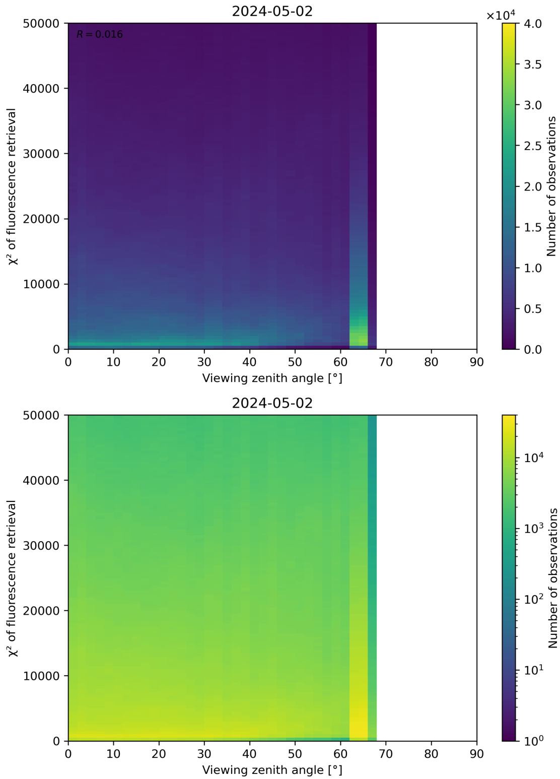
Figure 119: Scatter density plot of “Viewing zenith angle” against “ \chi^2 of fluorescence retrieval” for 2024-05-02 to 2024-05-03.
