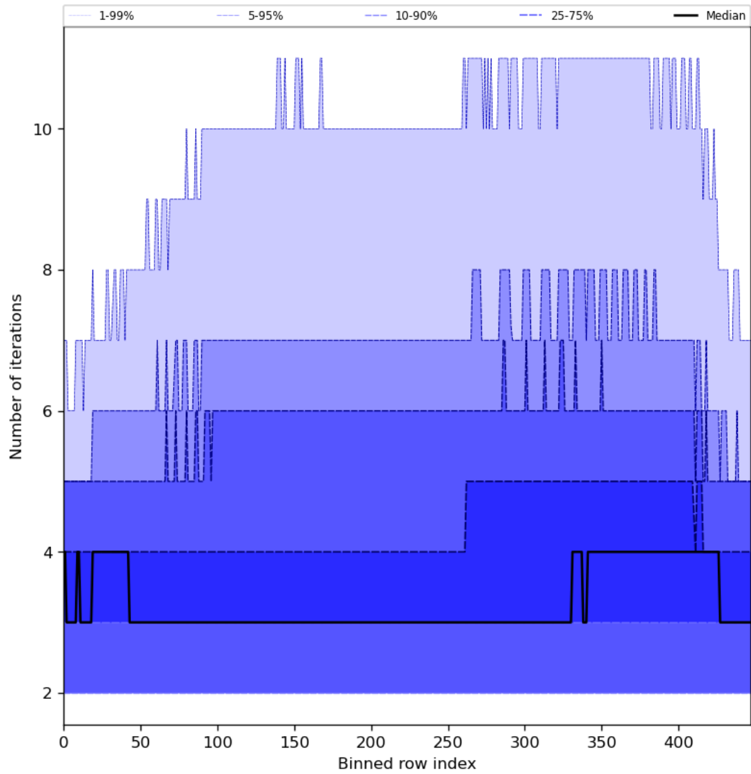
Figure 56: Along track statistics of “Number of iterations” for 2024-05-02 to 2024-05-03
