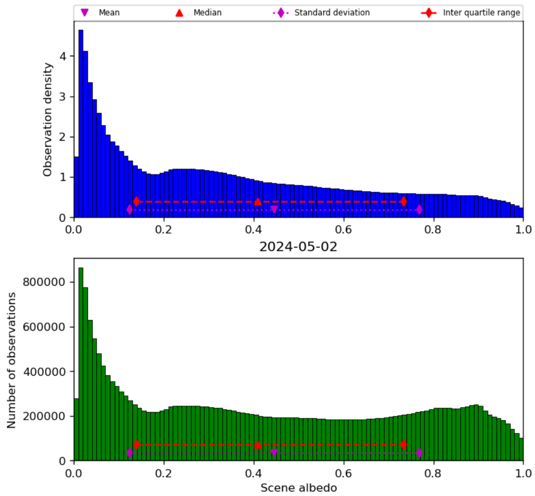
Figure 34: Histogram of “Scene albedo” for 2024-05-02 to 2024-05-03
