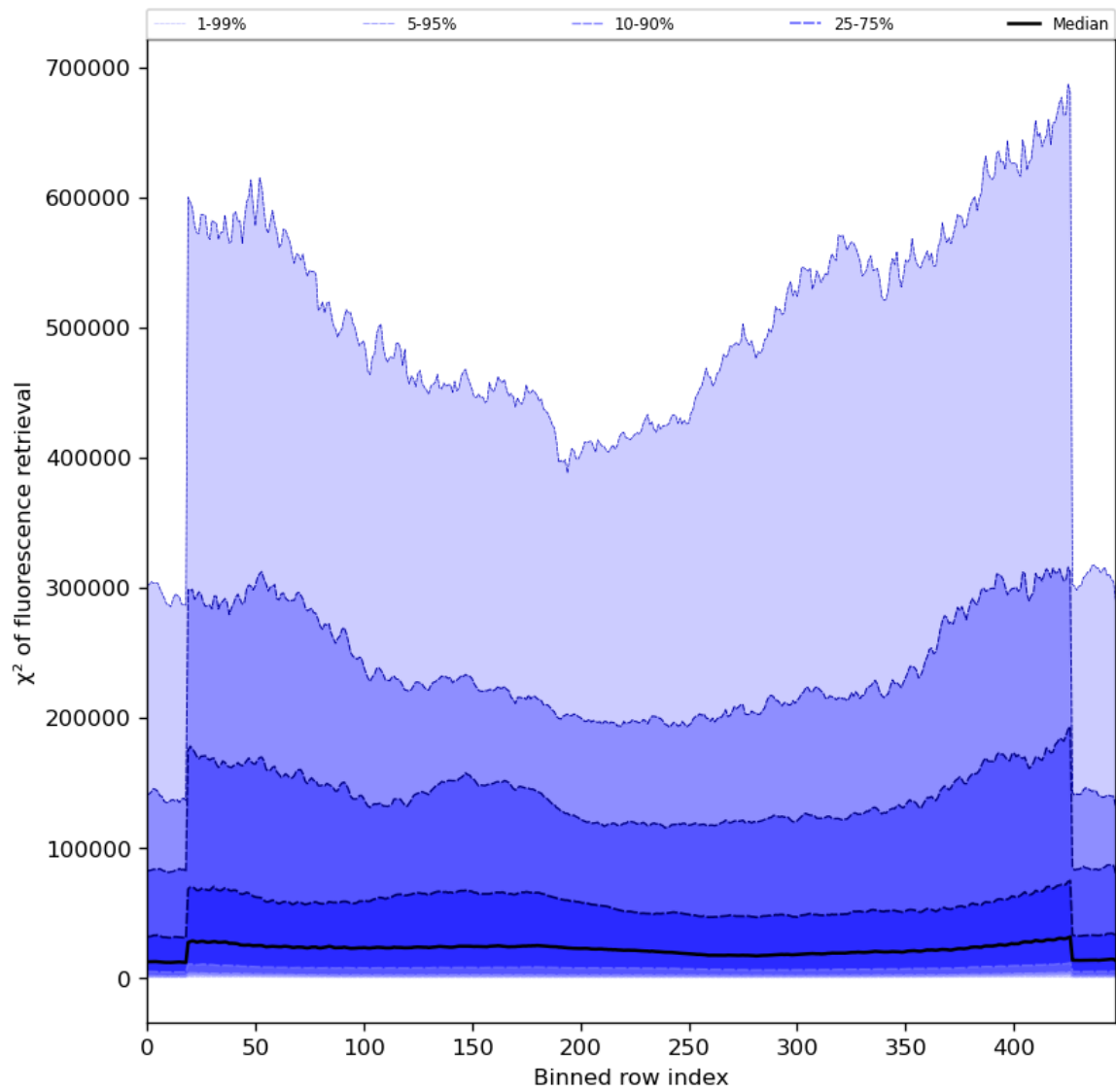
Figure 59: Along track statistics of “ \chi^2 of fluorescence retrieval” for 2024-05-02 to 2024-05-03
