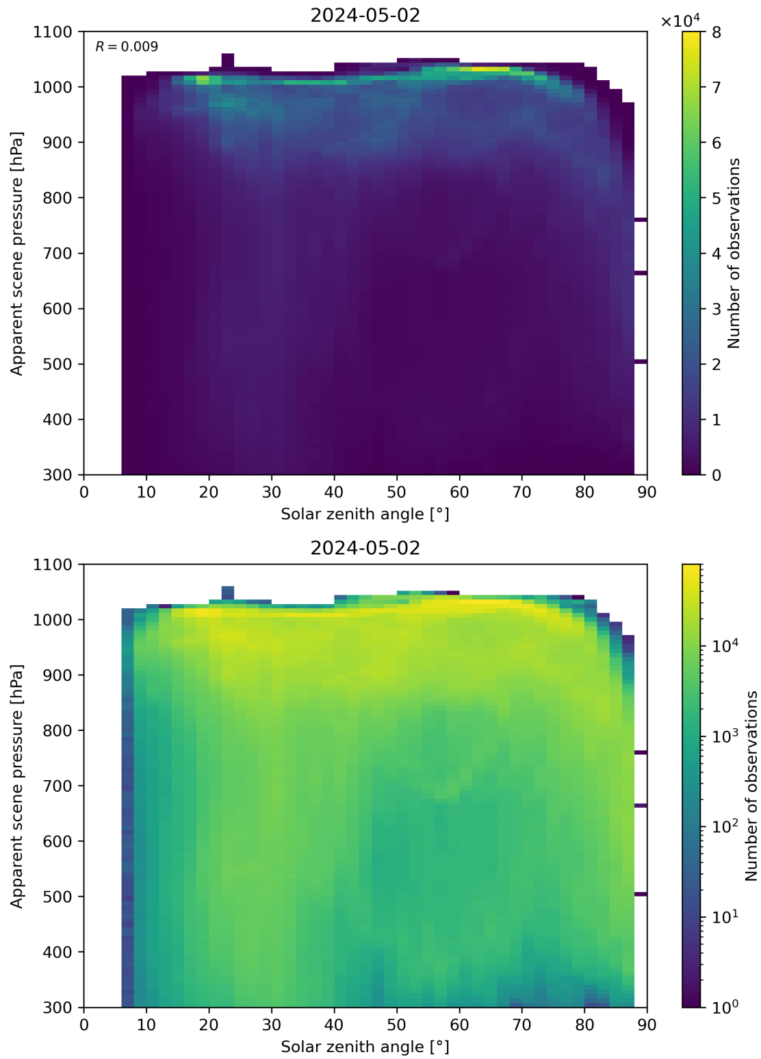
Figure 108: Scatter density plot of “Solar zenith angle” against “Apparent scene pressure” for 2024-05-02 to 2024-05-03.
