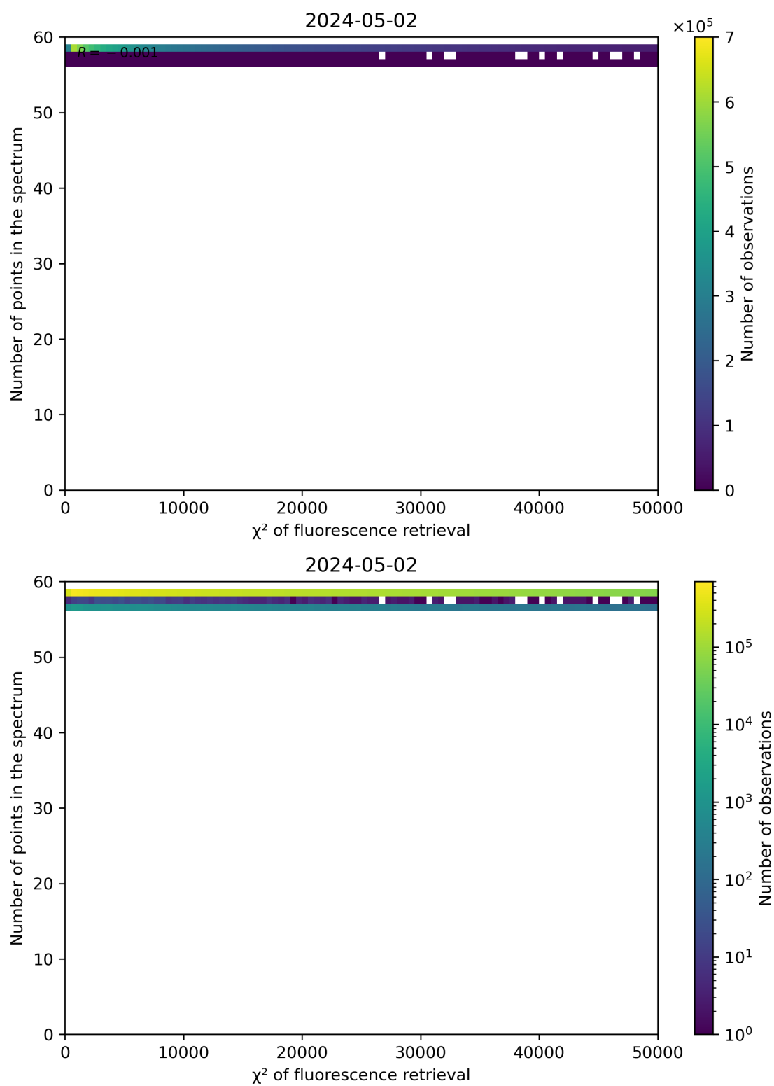
Figure 68: Scatter density plot of " \chi^2 of fluorescence retrieval" against "Number of points in the spectrum" for 2024-05-02 to 2024-05-03.
