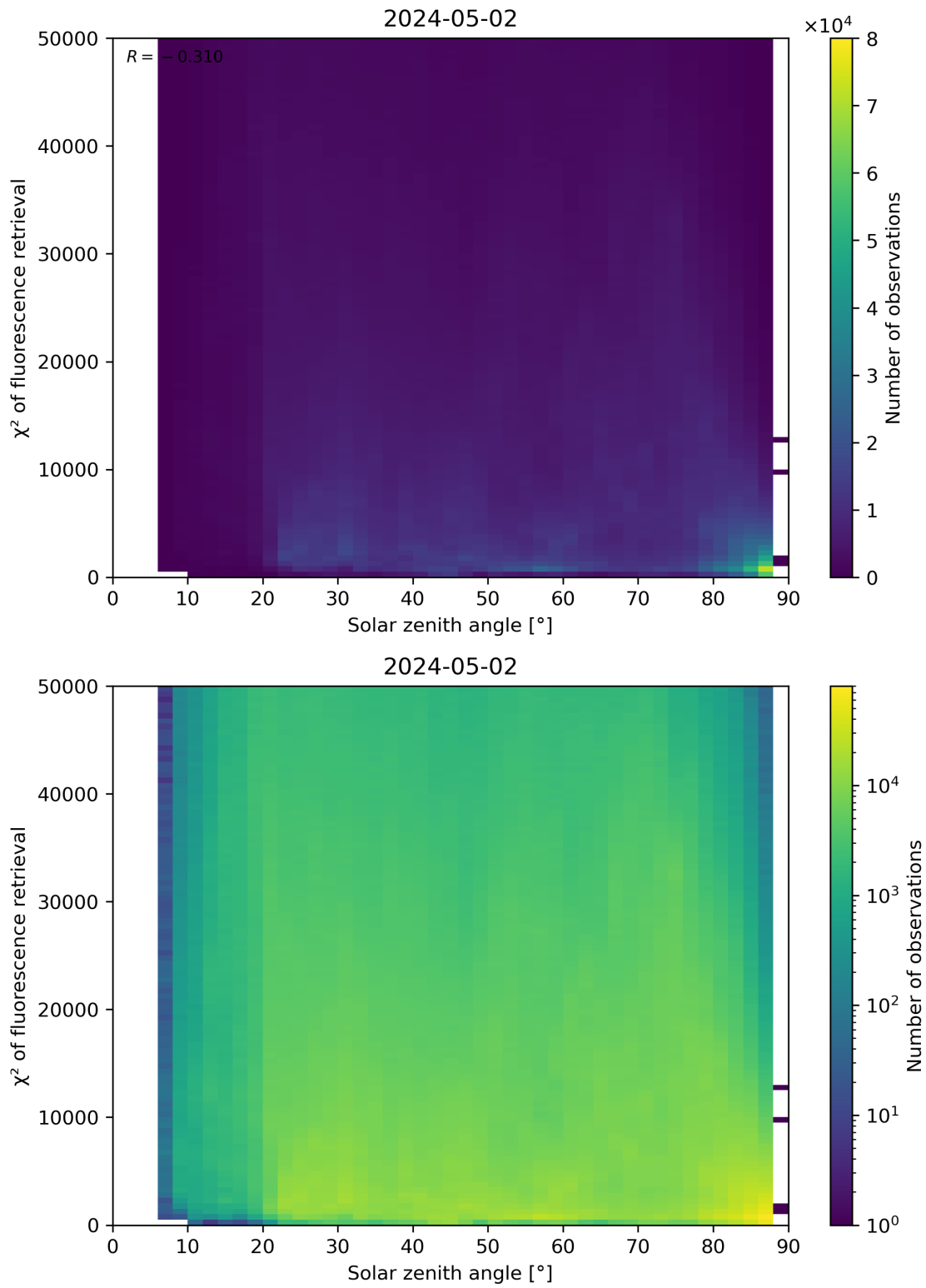
Figure 109: Scatter density plot of “Solar zenith angle” against “ \chi^2 of fluorescence retrieval” for 2024-05-02 to 2024-05-03.
