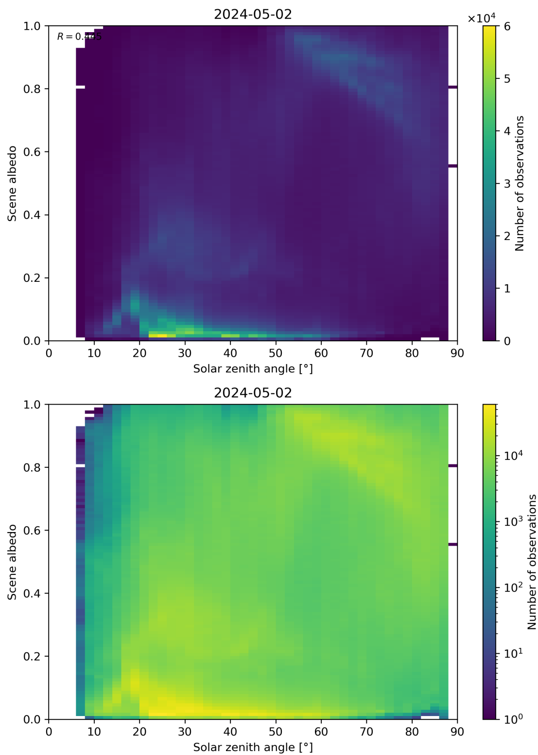
Figure 116: Scatter density plot of “Solar zenith angle” against “Scene albedo” for 2024-05-02 to 2024-05-03.
