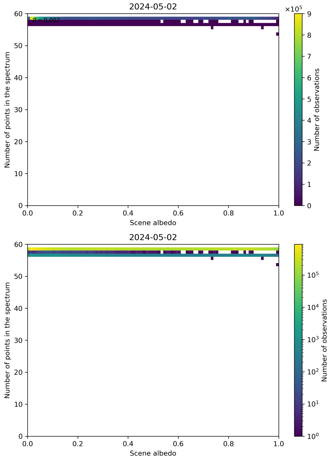
Figure 106: Scatter density plot of “Scene albedo” against “Number of points in the spectrum” for 2024-05-02 to 2024-05-03.
