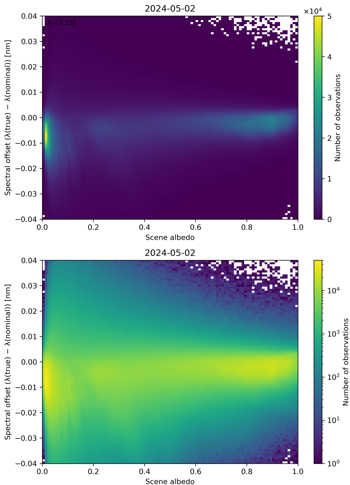
Figure 107: Scatter density plot of “Scene albedo” against “Spectral offset ( \lambda(\text{true}) - \lambda(\text{nominal}) )” for 2024-05-02 to 2024-05-03.
