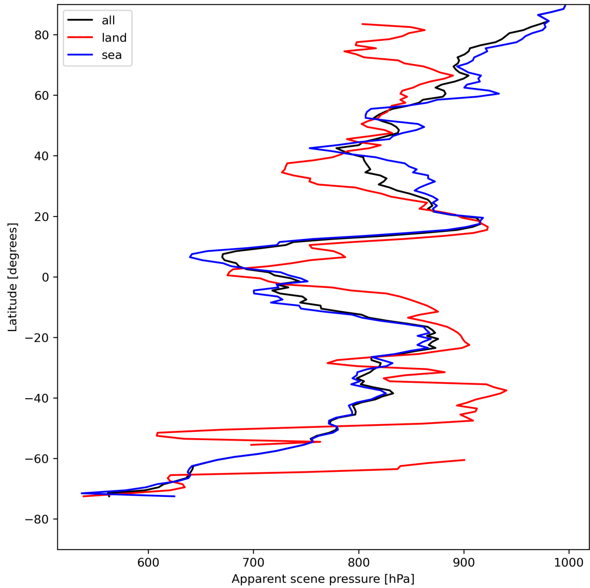
Figure 19: Zonal average of “Apparent scene pressure” for 2024-05-02 to 2024-05-03.
