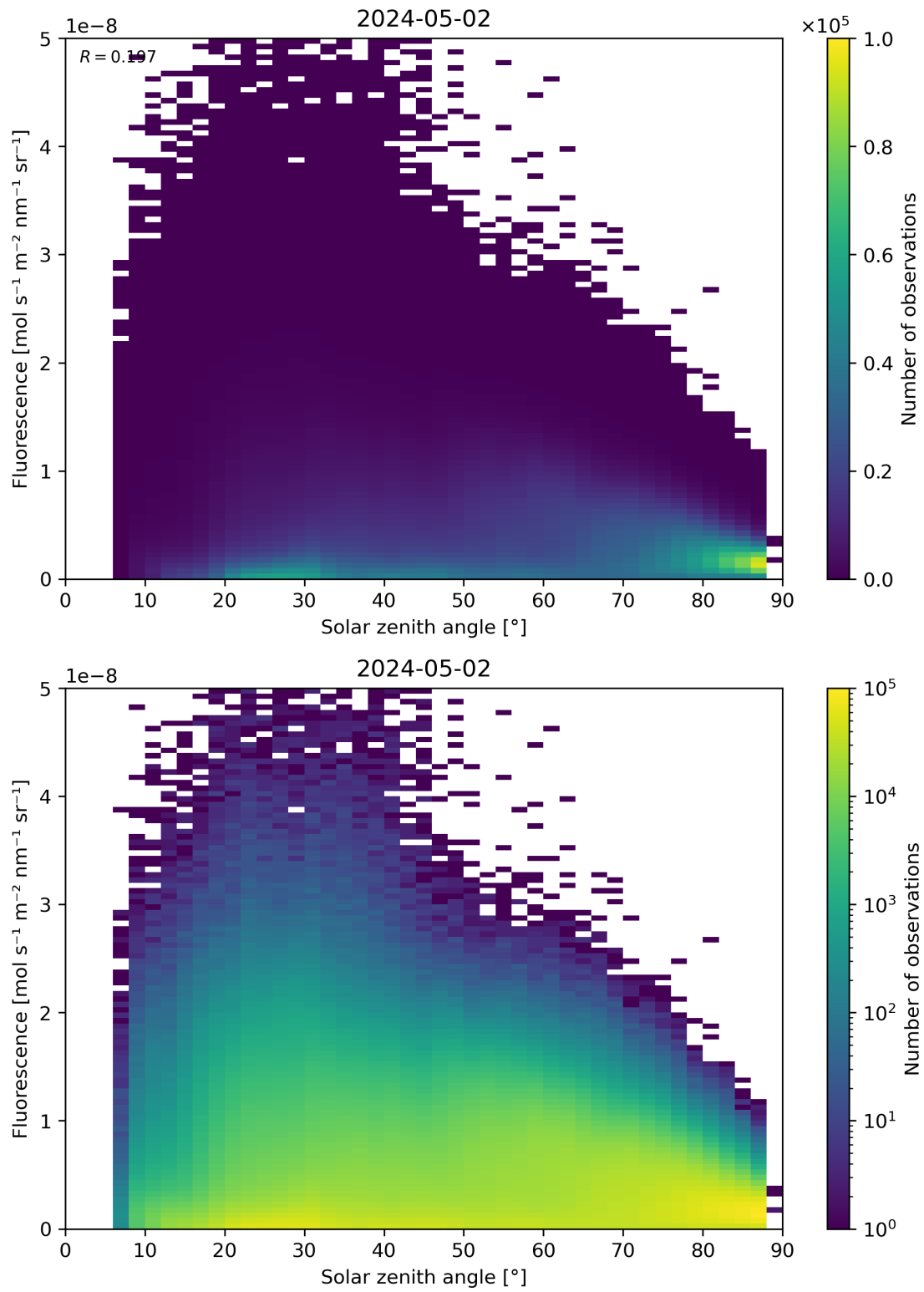
Figure 112: Scatter density plot of “Solar zenith angle” against “Fluorescence” for 2024-05-02 to 2024-05-03.
