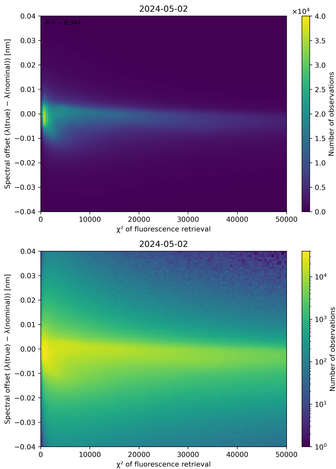
Figure 69: Scatter density plot of " \chi^2 of fluorescence retrieval" against "Spectral offset ( \lambda(\text{true}) - \lambda(\text{nominal}) )" for 2024-05-02 to 2024-05-03.
