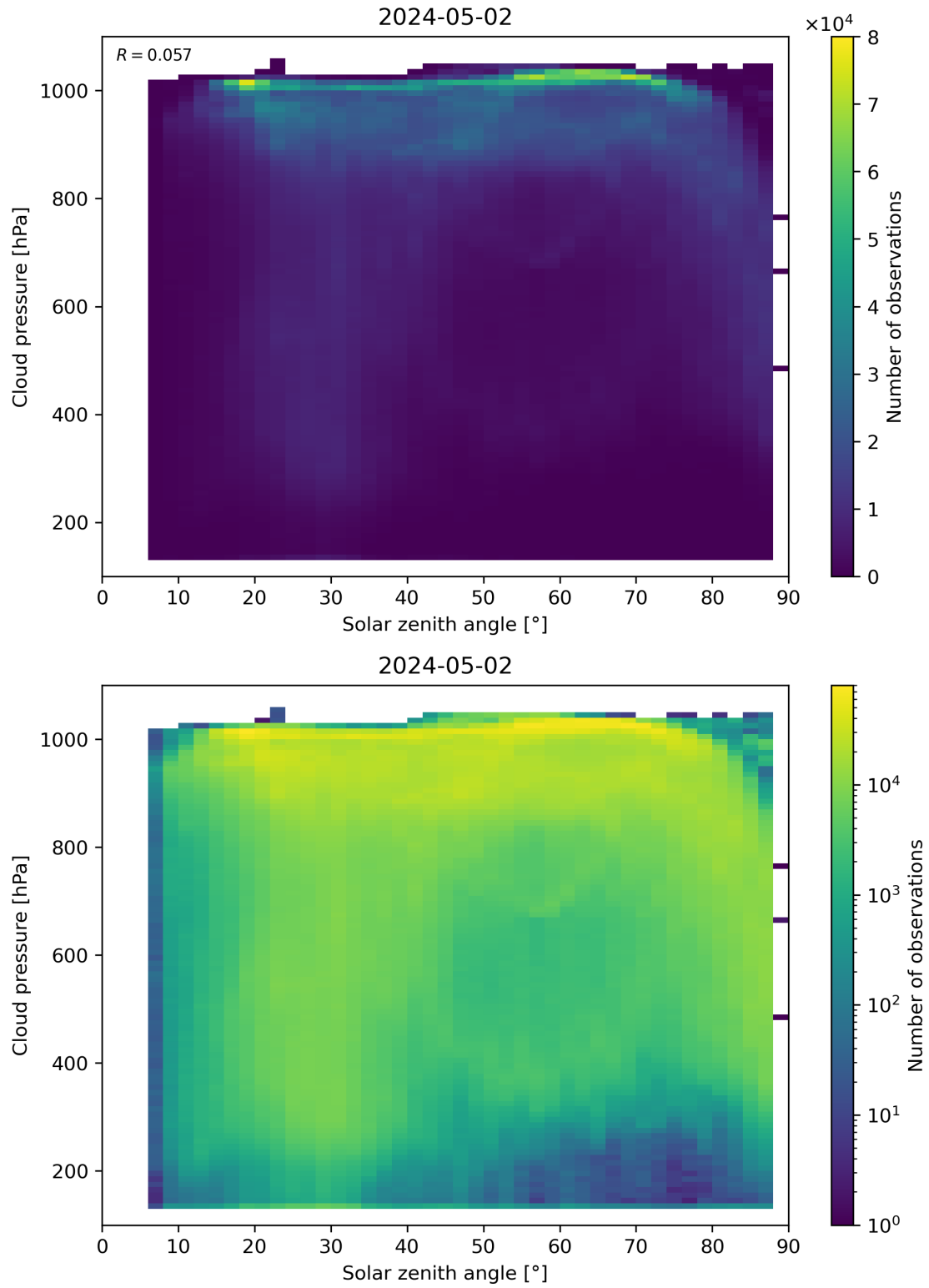
Figure 111: Scatter density plot of “Solar zenith angle” against “Cloud pressure” for 2024-05-02 to 2024-05-03.
