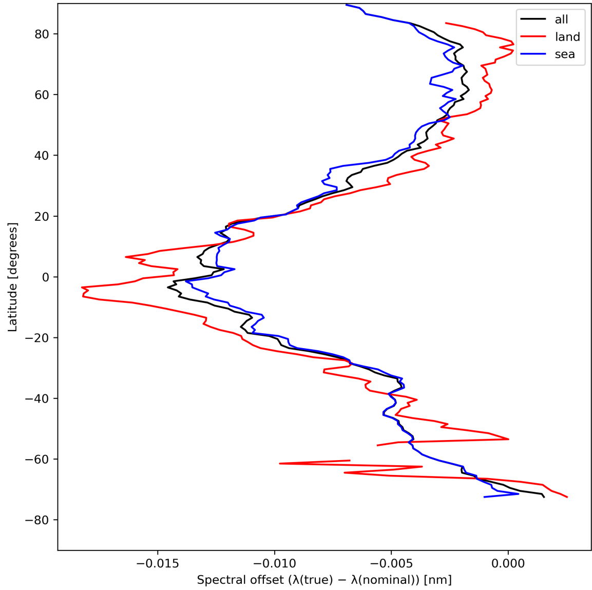
Figure 28: Zonal average of “Spectral offset ( \lambda(\text{true}) - \lambda(\text{nominal}) )” for 2024-05-02 to 2024-05-03.
