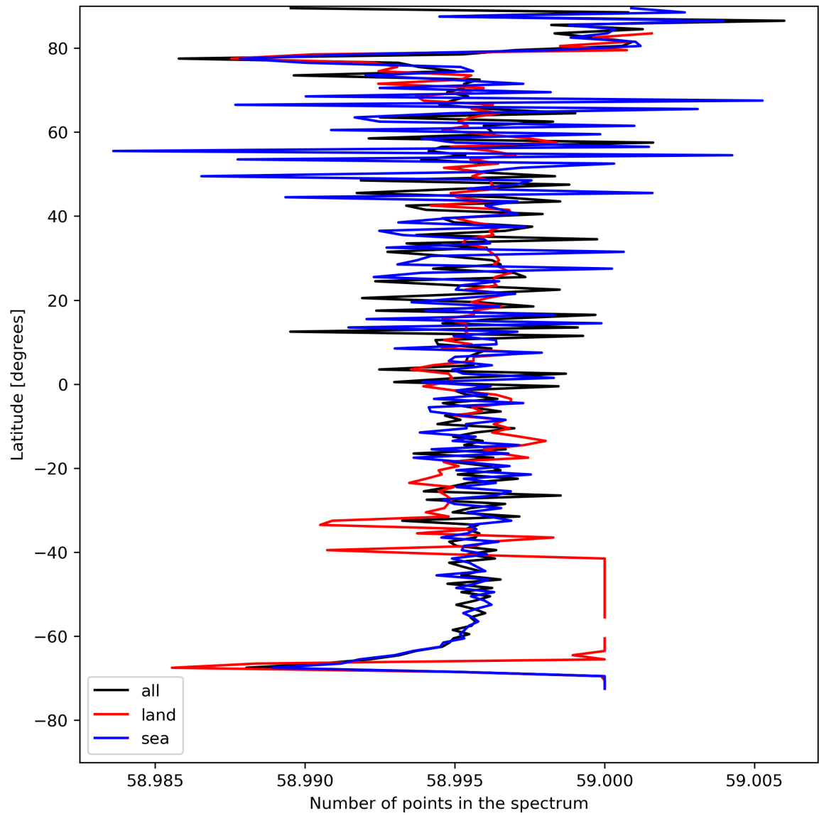
Figure 27: Zonal average of “Number of points in the spectrum” for 2024-05-02 to 2024-05-03.
