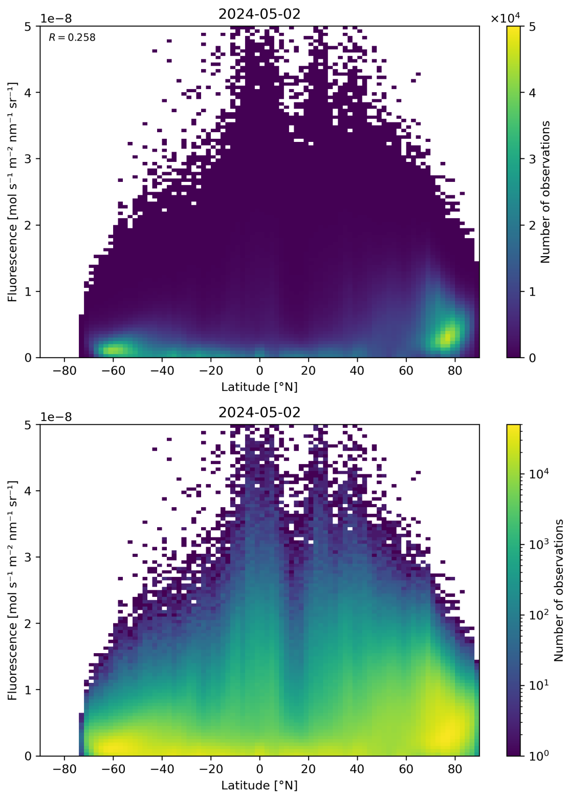
Figure 92: Scatter density plot of “Latitude” against “Fluorescence” for 2024-05-02 to 2024-05-03.
