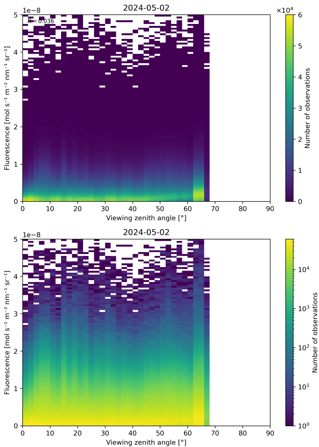
Figure 122: Scatter density plot of “Viewing zenith angle” against “Fluorescence” for 2024-05-02 to 2024-05-03.
