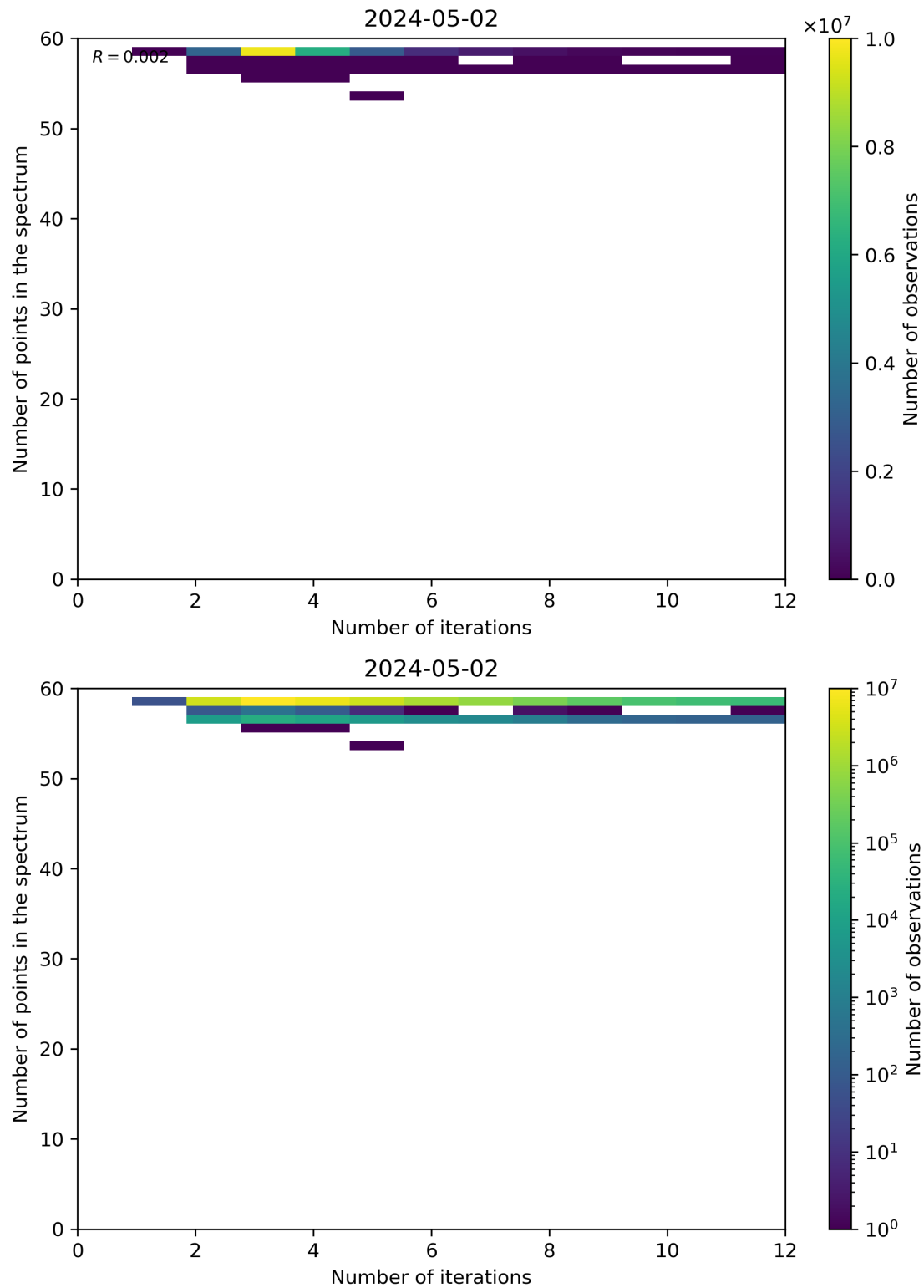
Figure 99: Scatter density plot of “Number of iterations” against “Number of points in the spectrum” for 2024-05-02 to 2024-05-03.
