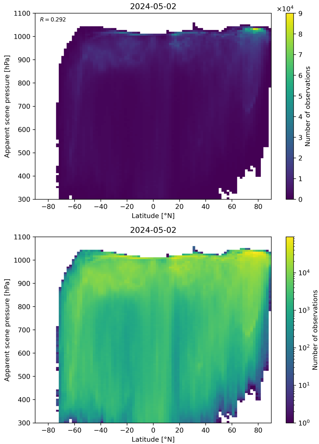
Figure 88: Scatter density plot of “Latitude” against “Apparent scene pressure” for 2024-05-02 to 2024-05-03.
