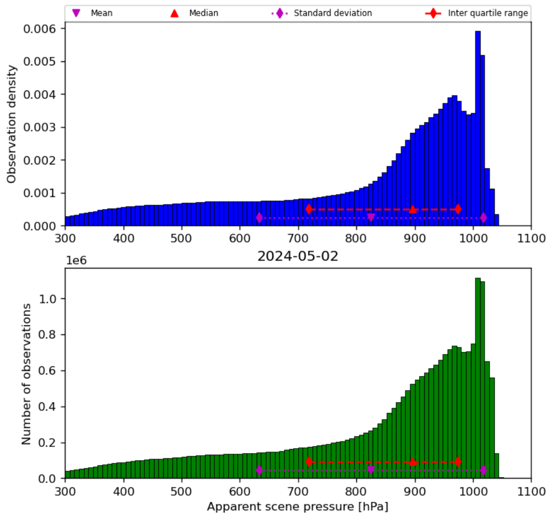
Figure 36: Histogram of “Apparent scene pressure” for 2024-05-02 to 2024-05-03
