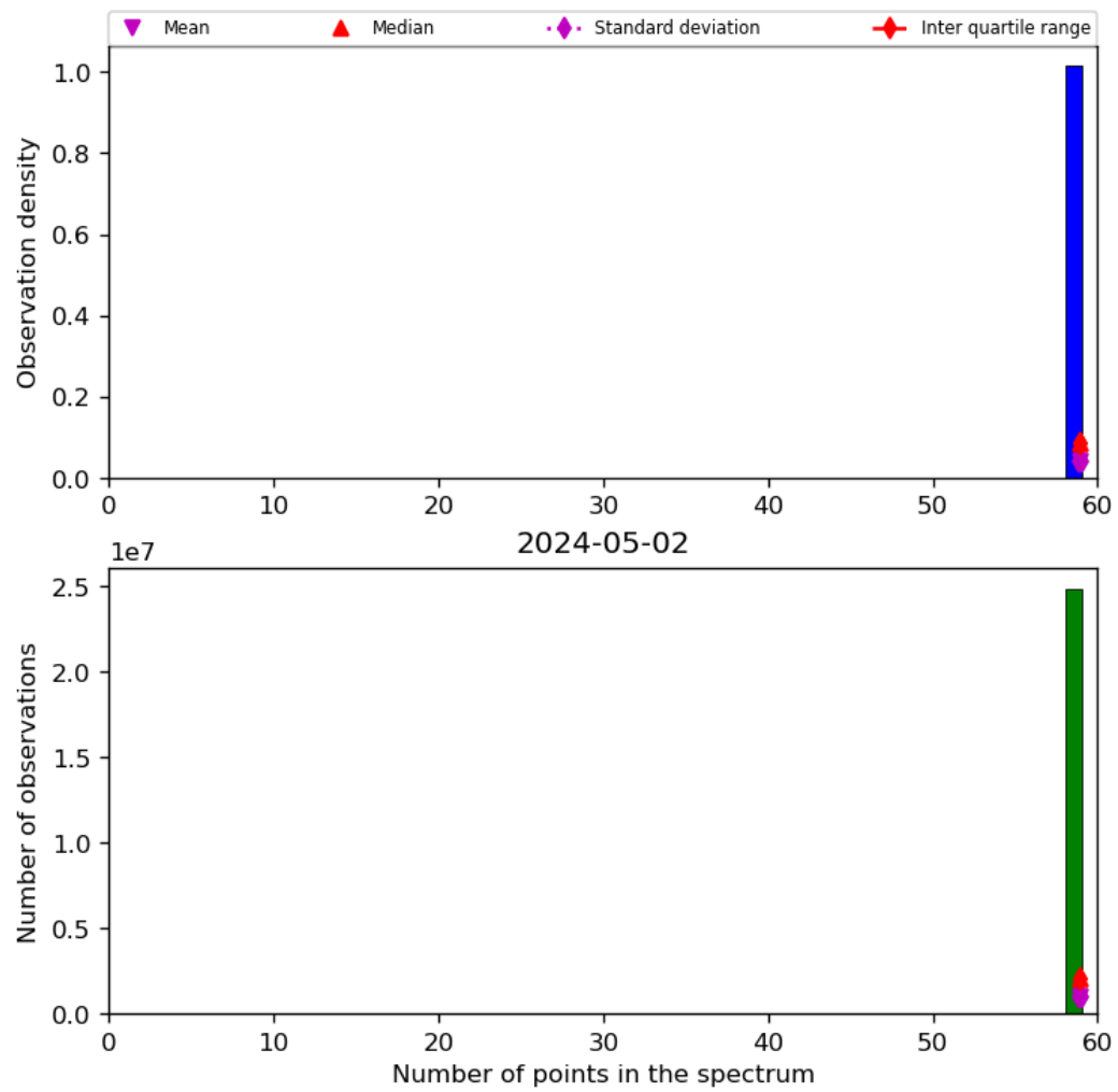
Figure 44: Histogram of “Number of points in the spectrum” for 2024-05-02 to 2024-05-03
