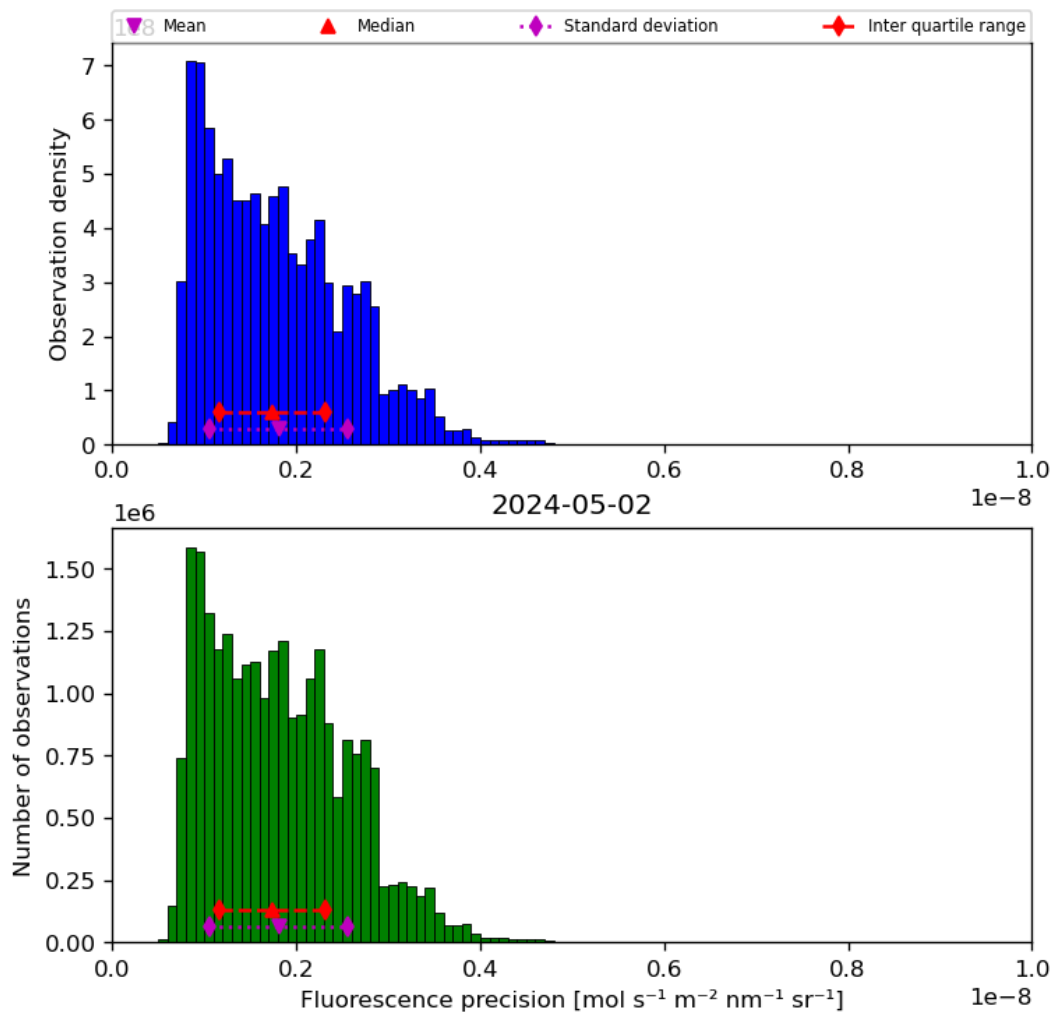
Figure 41: Histogram of “Fluorescence precision” for 2024-05-02 to 2024-05-03
