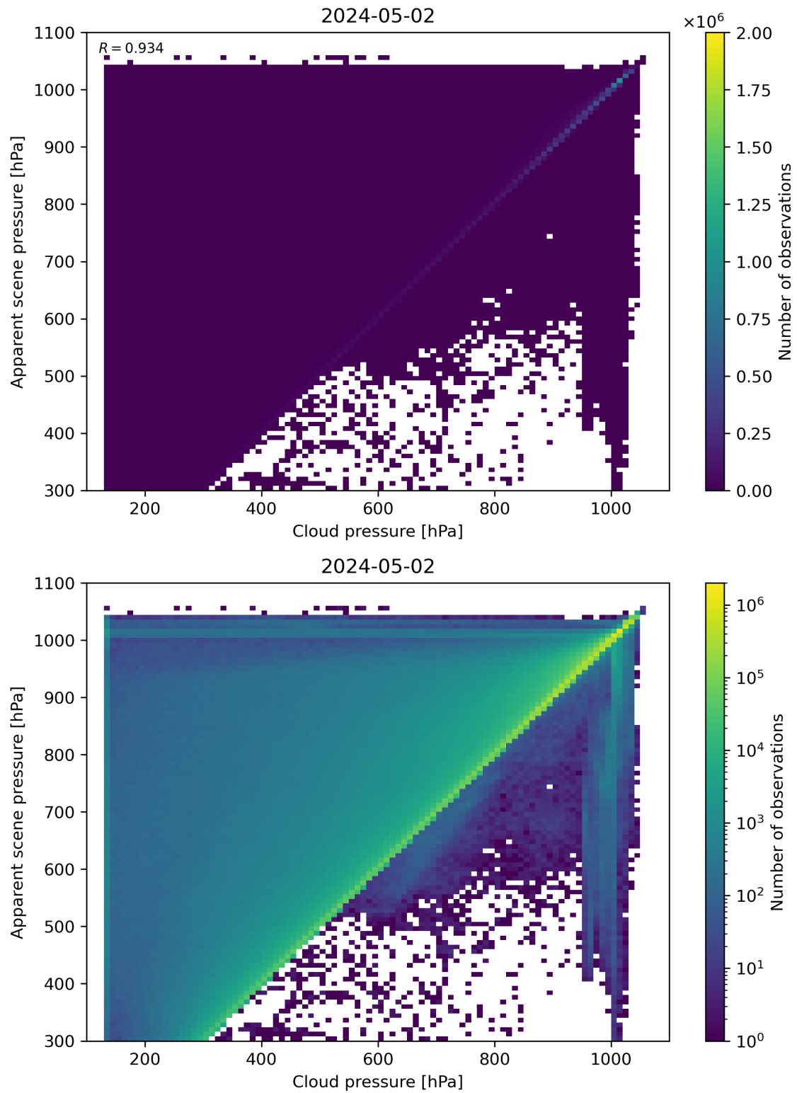
Figure 77: Scatter density plot of “Cloud pressure” against “Apparent scene pressure” for 2024-05-02 to 2024-05-03.
