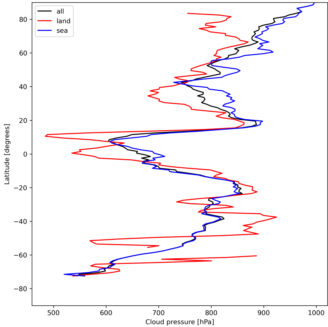
Figure 13: Zonal average of “Cloud pressure” for 2024-05-02 to 2024-05-03.
