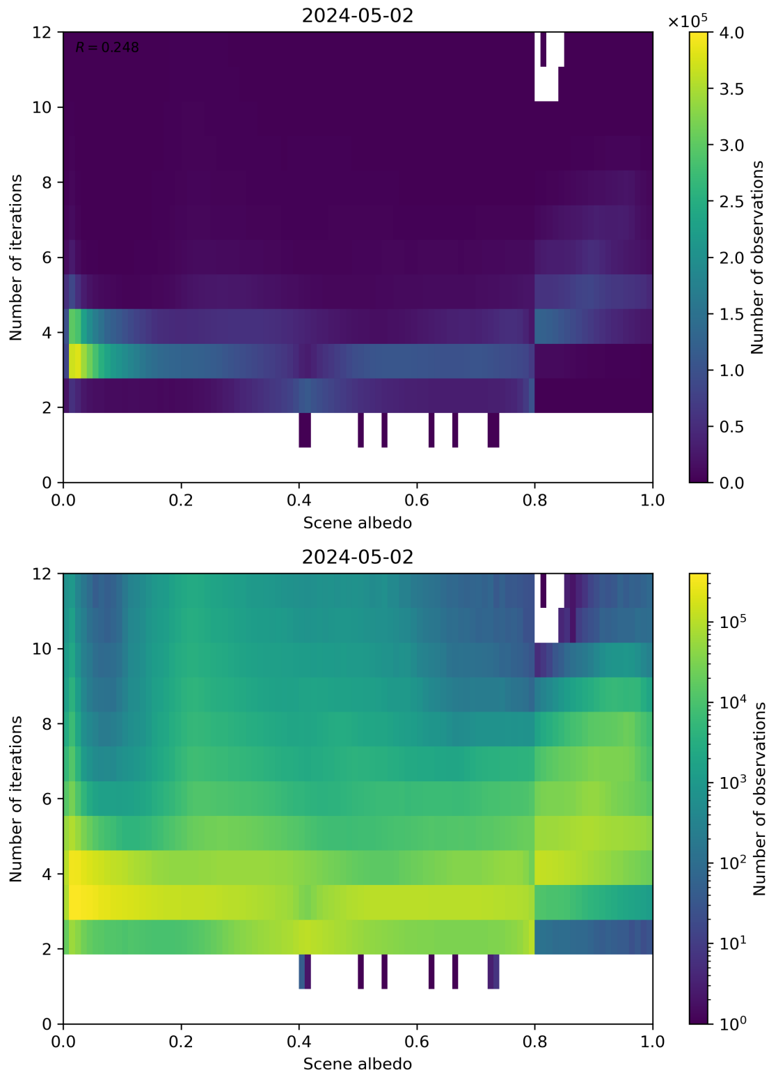
Figure 105: Scatter density plot of “Scene albedo” against “Number of iterations” for 2024-05-02 to 2024-05-03.
