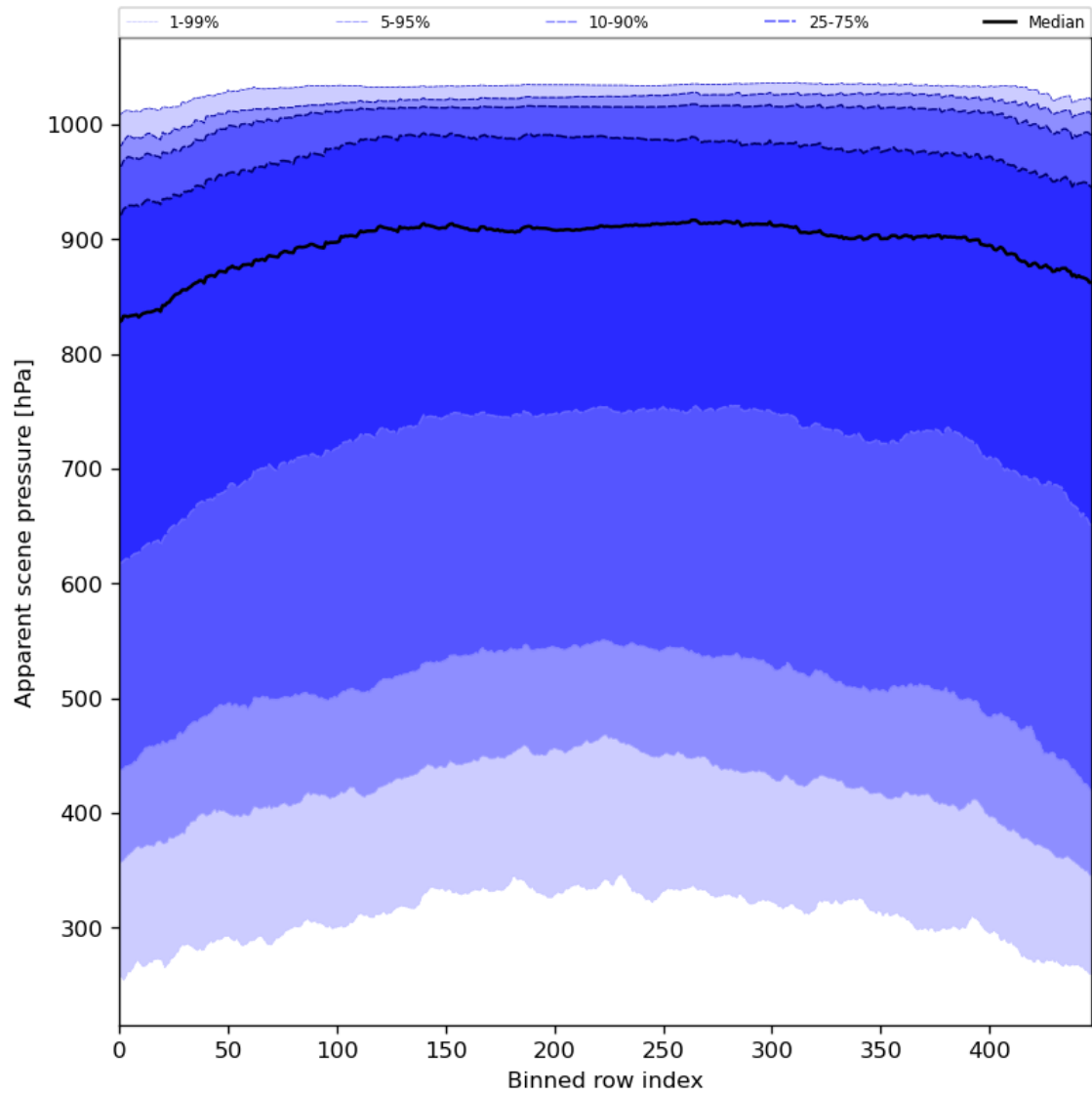
Figure 53: Along track statistics of “Apparent scene pressure” for 2024-05-02 to 2024-05-03
