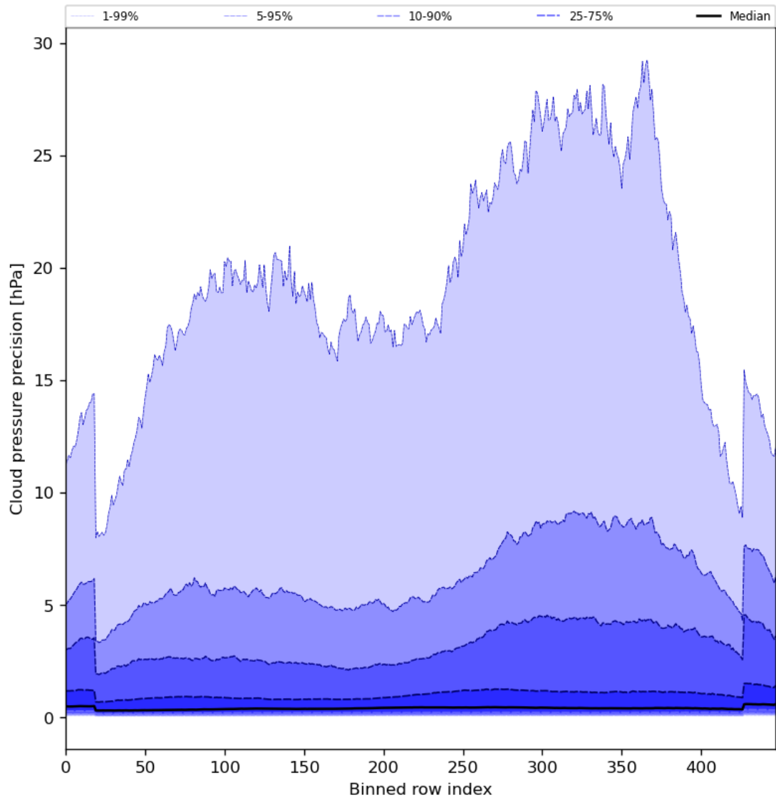
Figure 48: Along track statistics of “Cloud pressure precision” for 2024-05-02 to 2024-05-03
