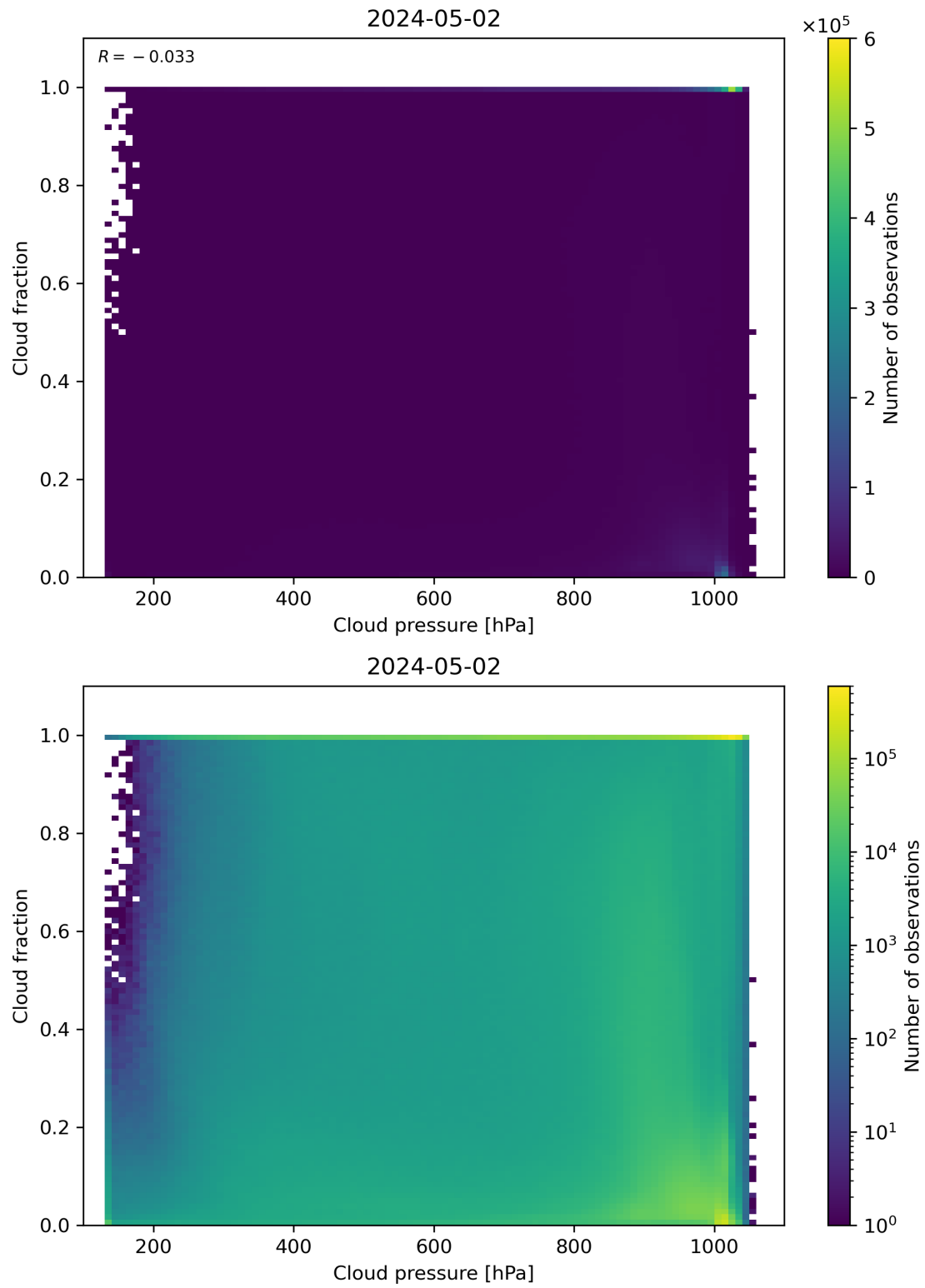
Figure 79: Scatter density plot of “Cloud pressure” against “Cloud fraction” for 2024-05-02 to 2024-05-03.
