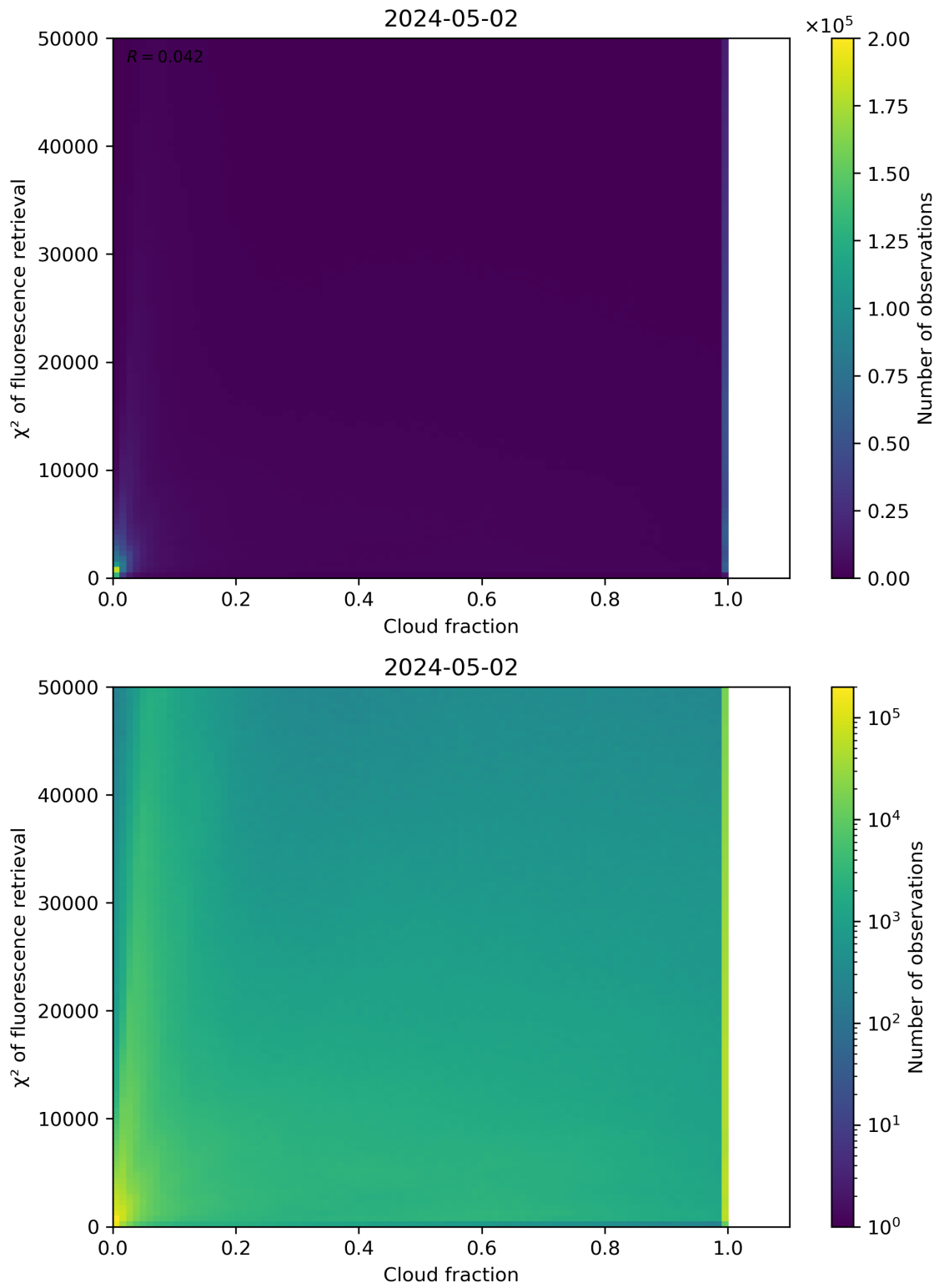
Figure 71: Scatter density plot of “Cloud fraction” against “ \chi^2 of fluorescence retrieval” for 2024-05-02 to 2024-05-03.
