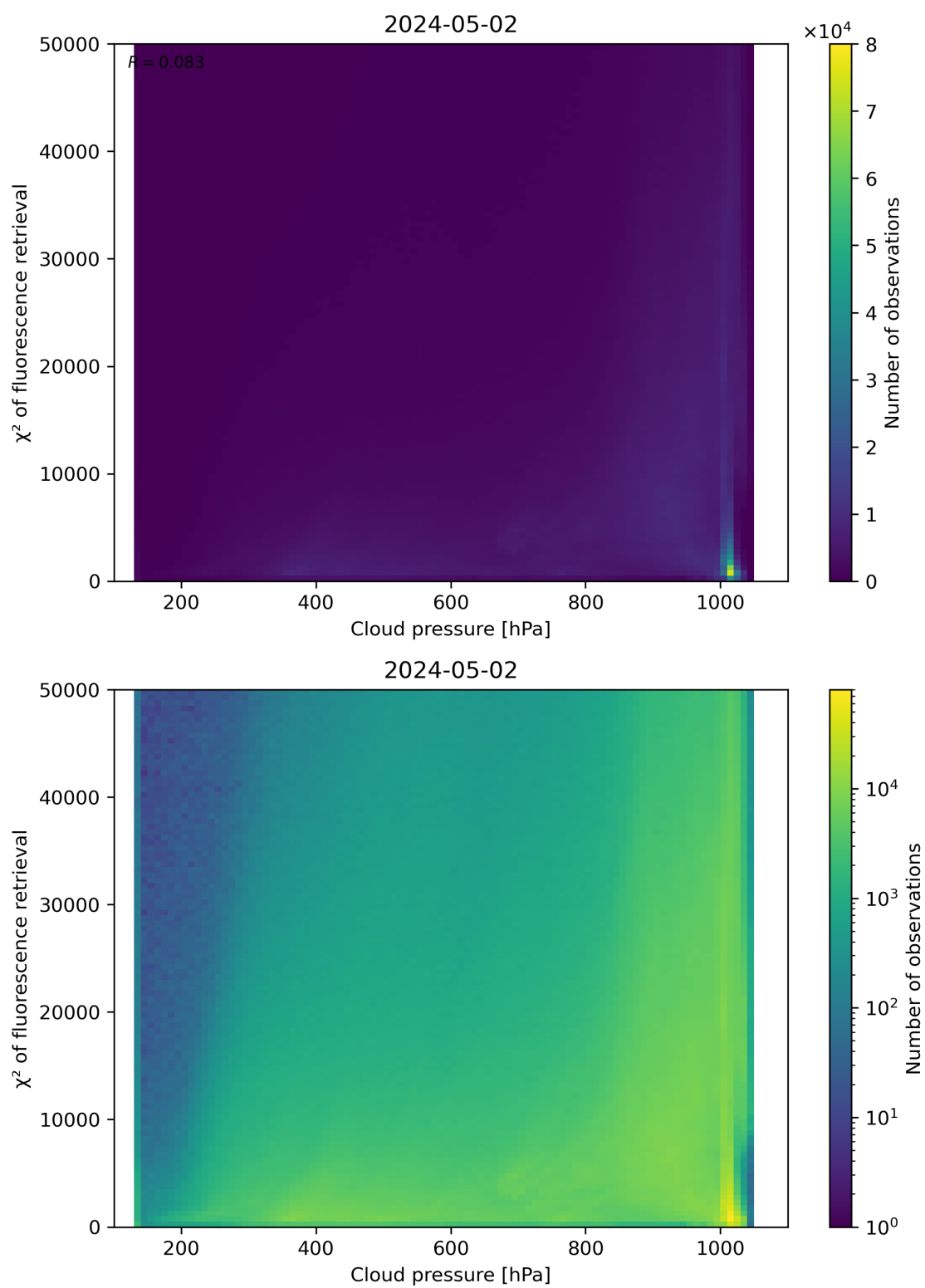
Figure 78: Scatter density plot of “Cloud pressure” against “ \chi^2 of fluorescence retrieval” for 2024-05-02 to 2024-05-03.
