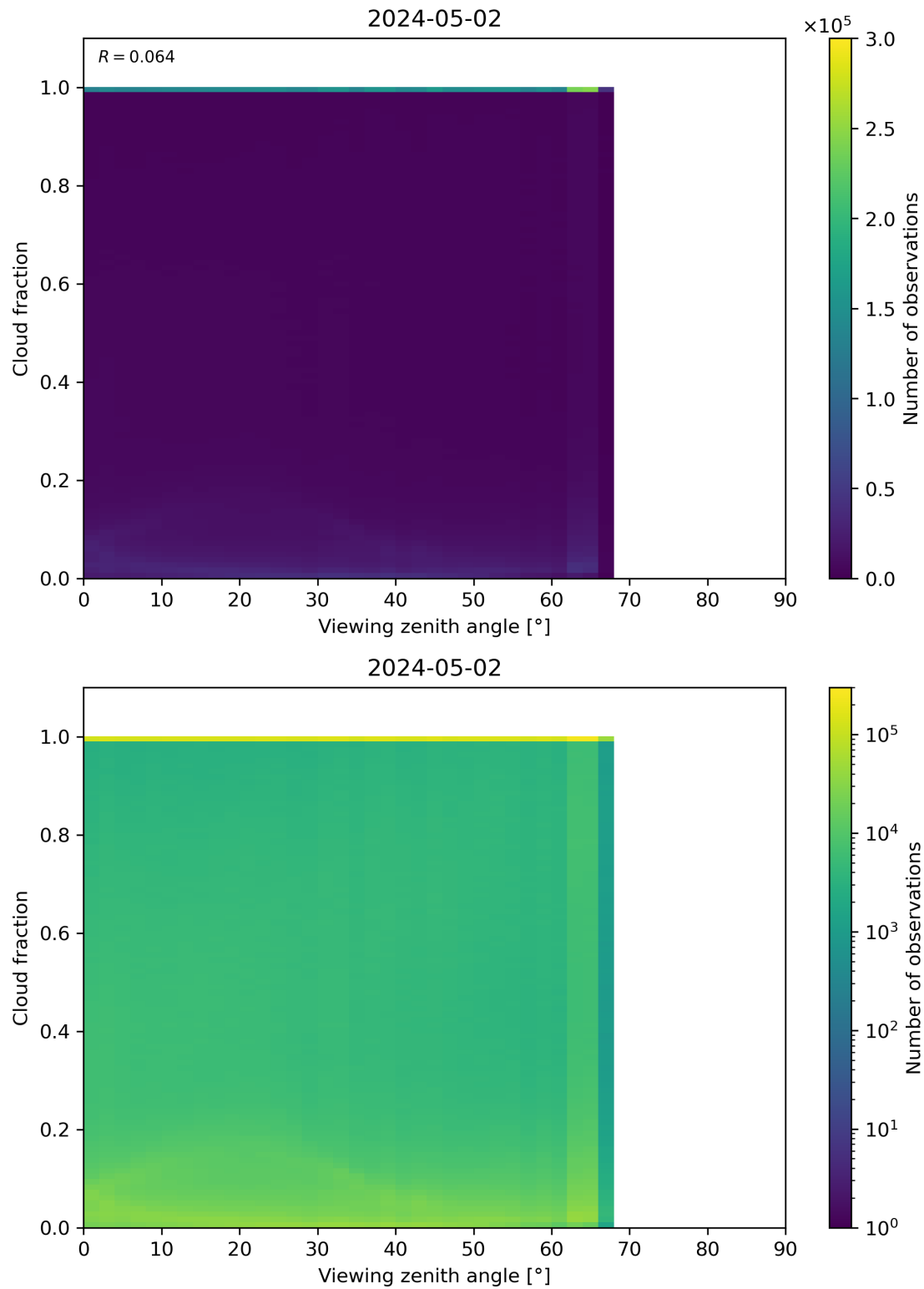
Figure 120: Scatter density plot of “Viewing zenith angle” against “Cloud fraction” for 2024-05-02 to 2024-05-03.
