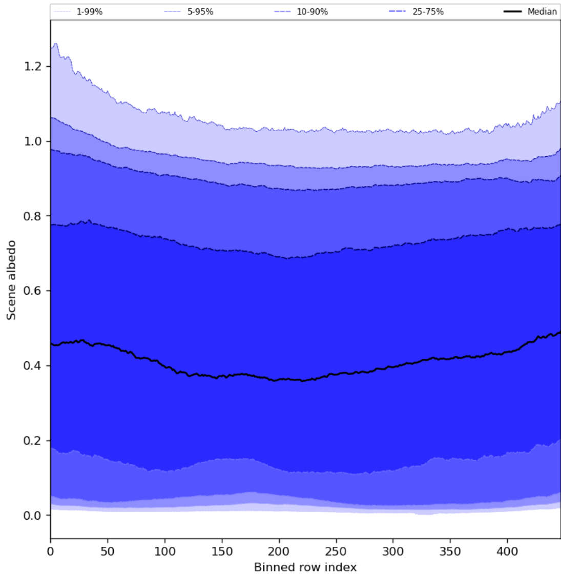
Figure 51: Along track statistics of “Scene albedo” for 2024-05-02 to 2024-05-03
