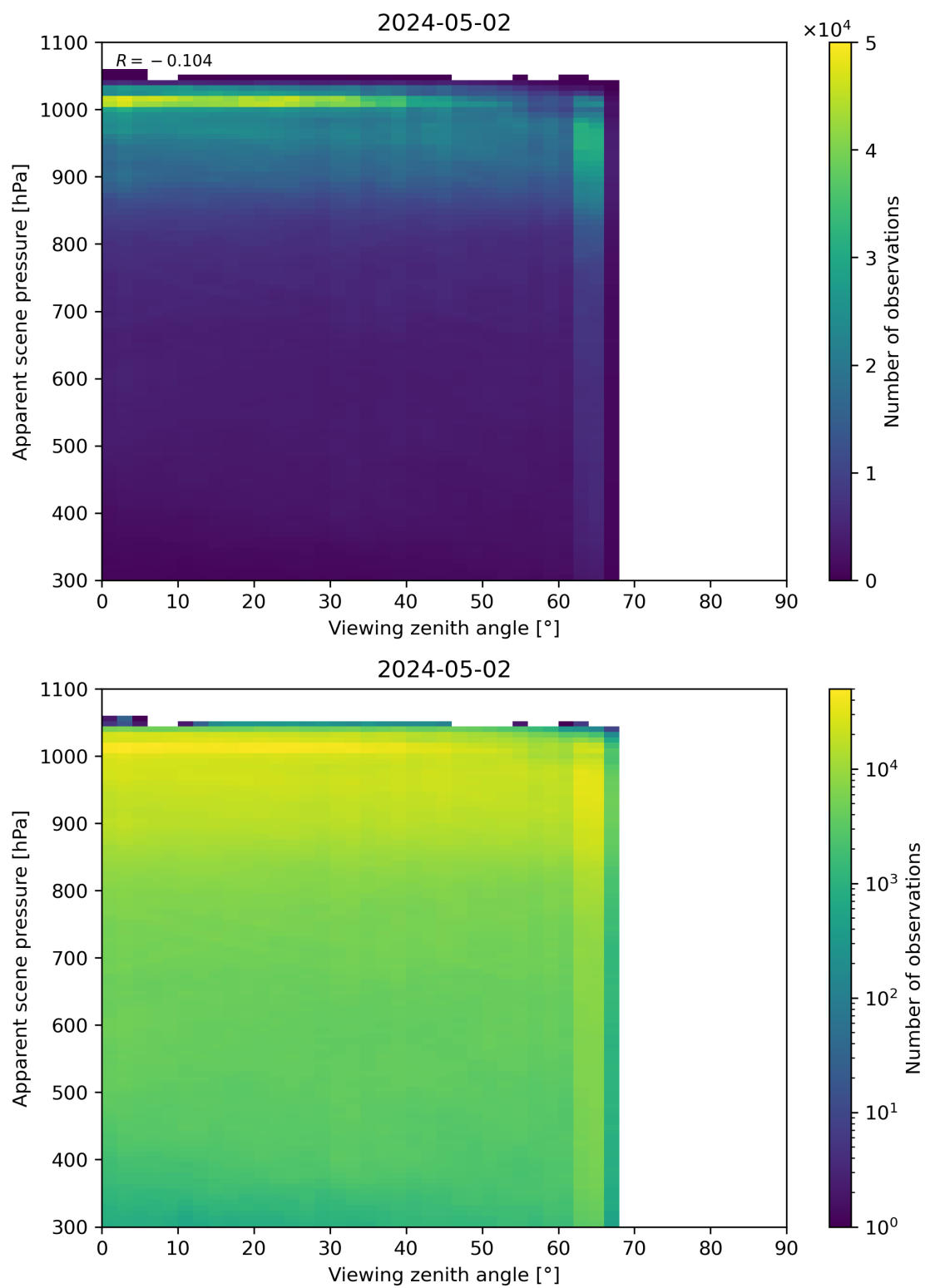
Figure 118: Scatter density plot of “Viewing zenith angle” against “Apparent scene pressure” for 2024-05-02 to 2024-05-03.
