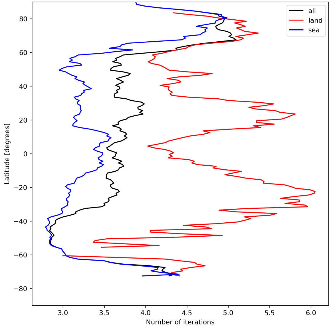
Figure 22: Zonal average of “Number of iterations” for 2024-05-02 to 2024-05-03.
