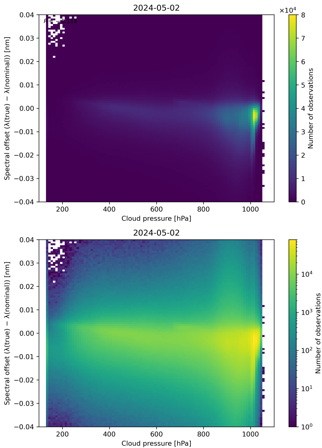
Figure 84: Scatter density plot of “Cloud pressure” against “Spectral offset ( \lambda(\text{true}) - \lambda(\text{nominal}) )” for 2024-05-02 to 2024-05-03.
