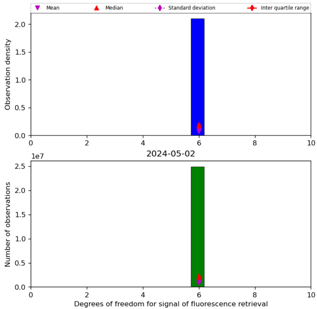
Figure 43: Histogram of “Degrees of freedom for signal of fluorescence retrieval” for 2024-05-02 to 2024-05-03
