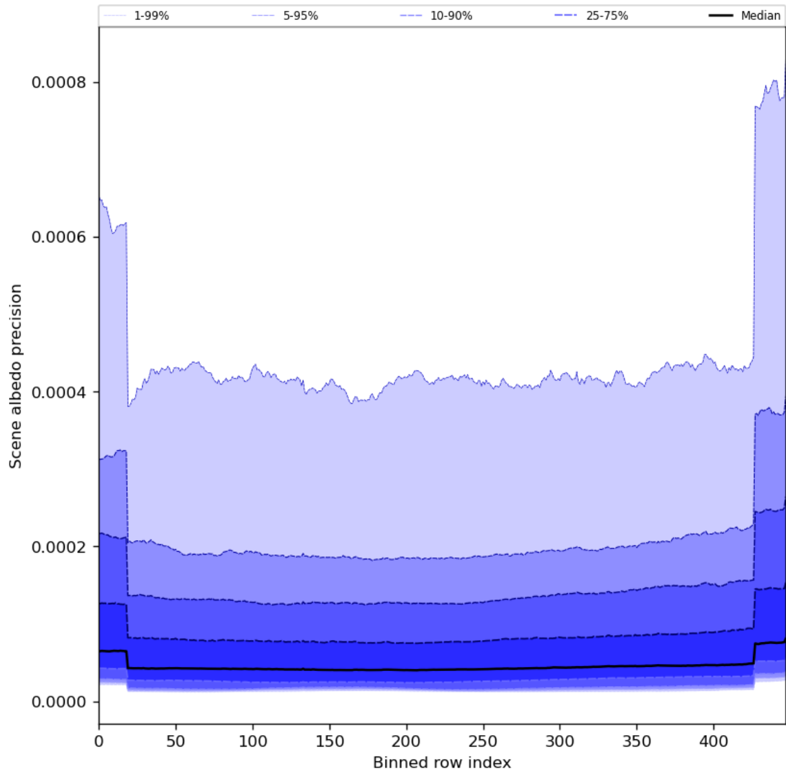
Figure 52: Along track statistics of “Scene albedo precision” for 2024-05-02 to 2024-05-03
