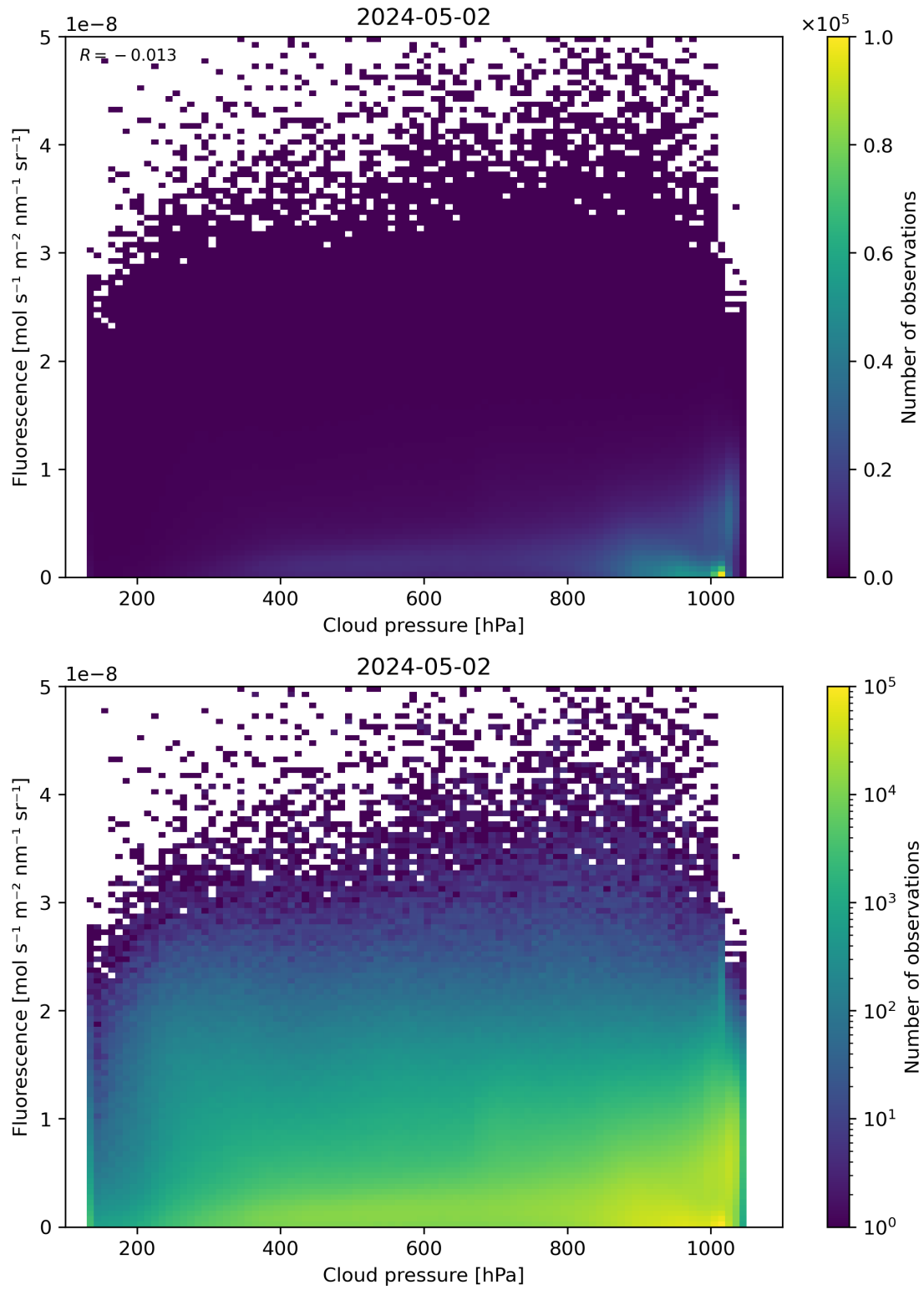
Figure 80: Scatter density plot of “Cloud pressure” against “Fluorescence” for 2024-05-02 to 2024-05-03.
