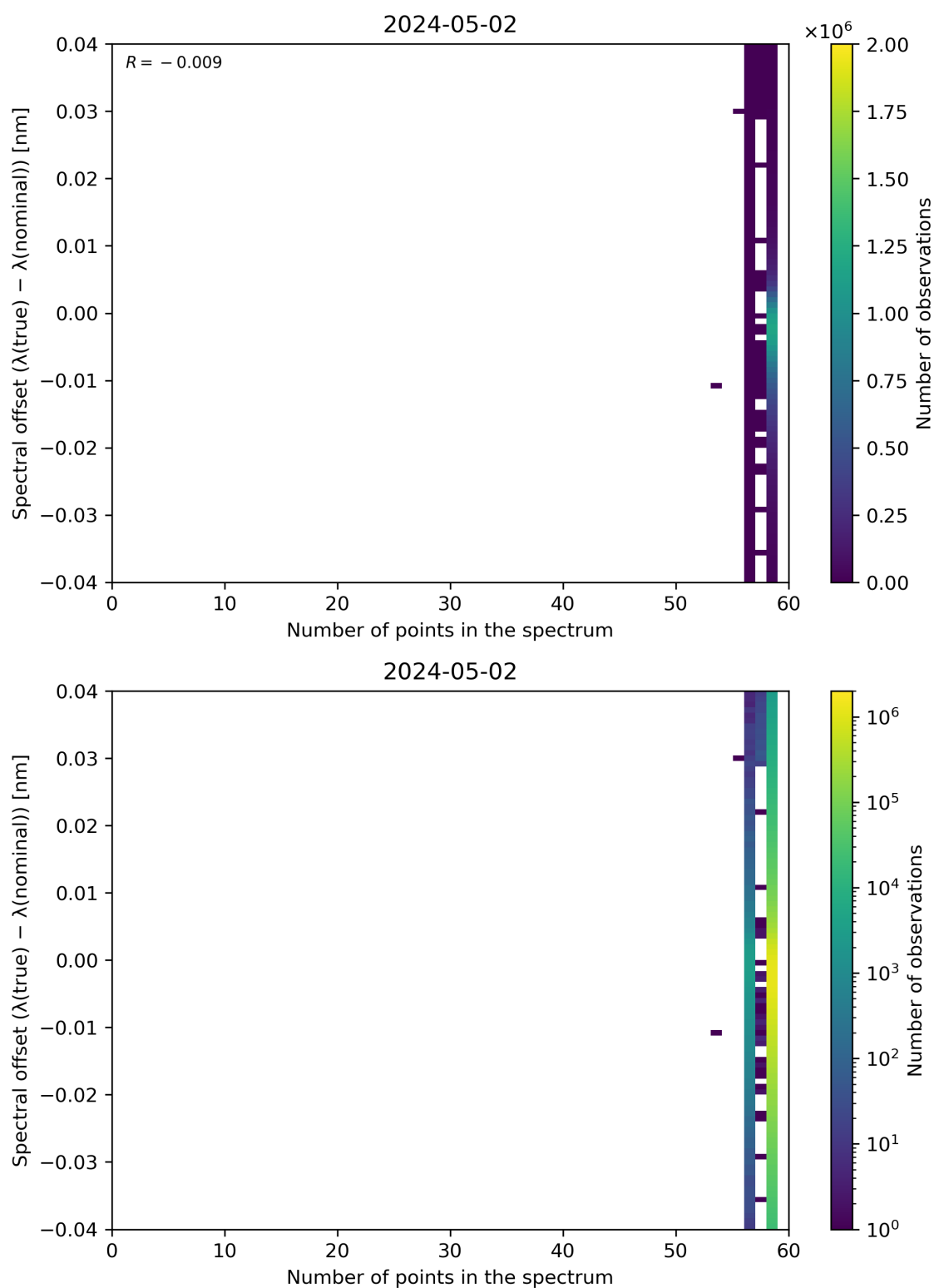
Figure 101: Scatter density plot of “Number of points in the spectrum” against “Spectral offset ( \lambda(\text{true}) - \lambda(\text{nominal}) )” for 2024-05-02 to 2024-05-03.
