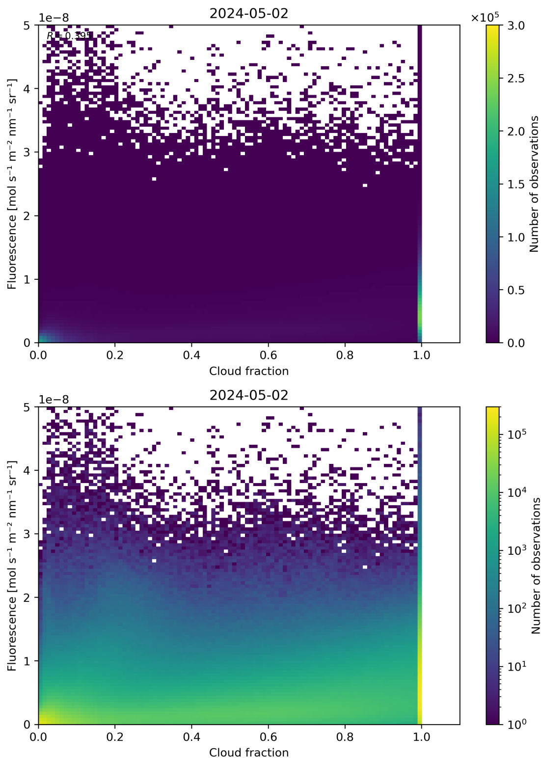
Figure 72: Scatter density plot of “Cloud fraction” against “Fluorescence” for 2024-05-02 to 2024-05-03.
