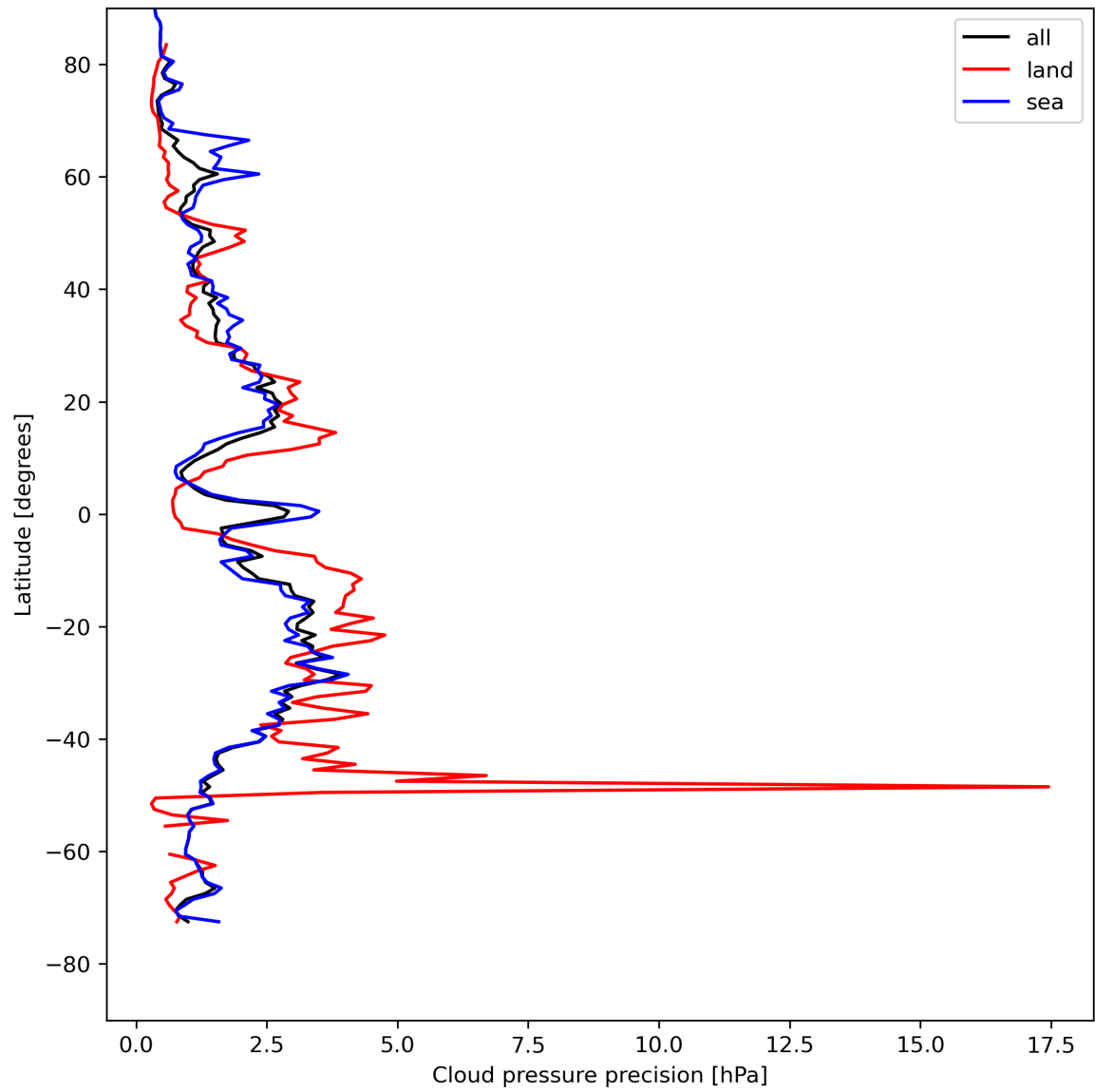
Figure 14: Zonal average of “Cloud pressure precision” for 2024-05-02 to 2024-05-03.
