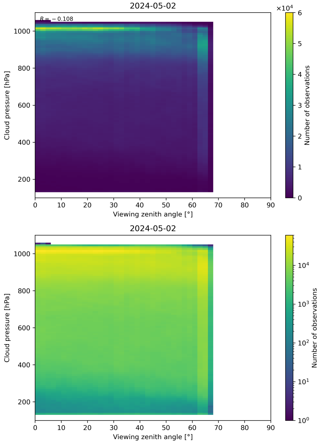
Figure 121: Scatter density plot of “Viewing zenith angle” against “Cloud pressure” for 2024-05-02 to 2024-05-03.
