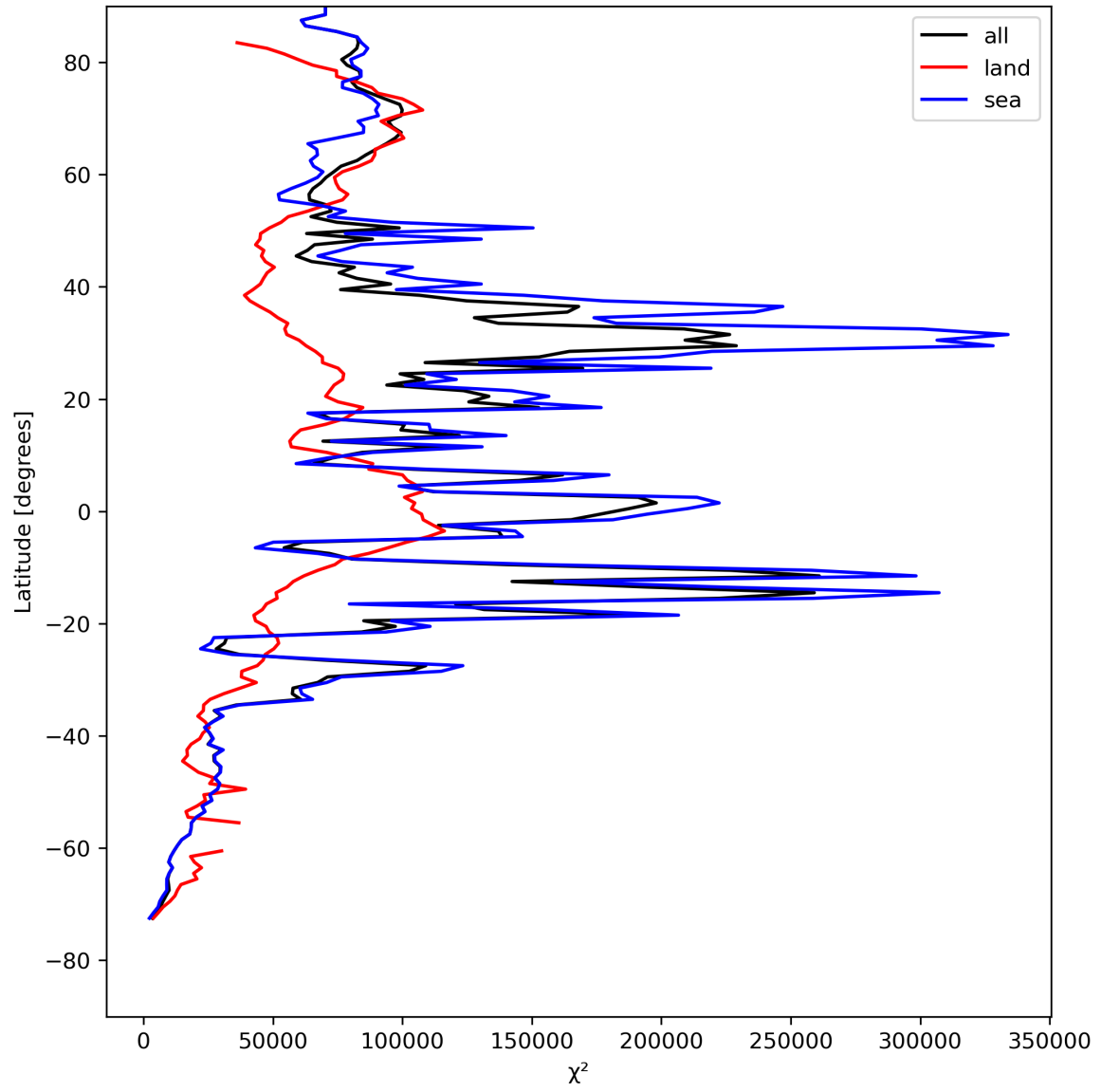
Figure 21: Zonal average of “ \chi^2 ” for 2024-05-02 to 2024-05-03.
