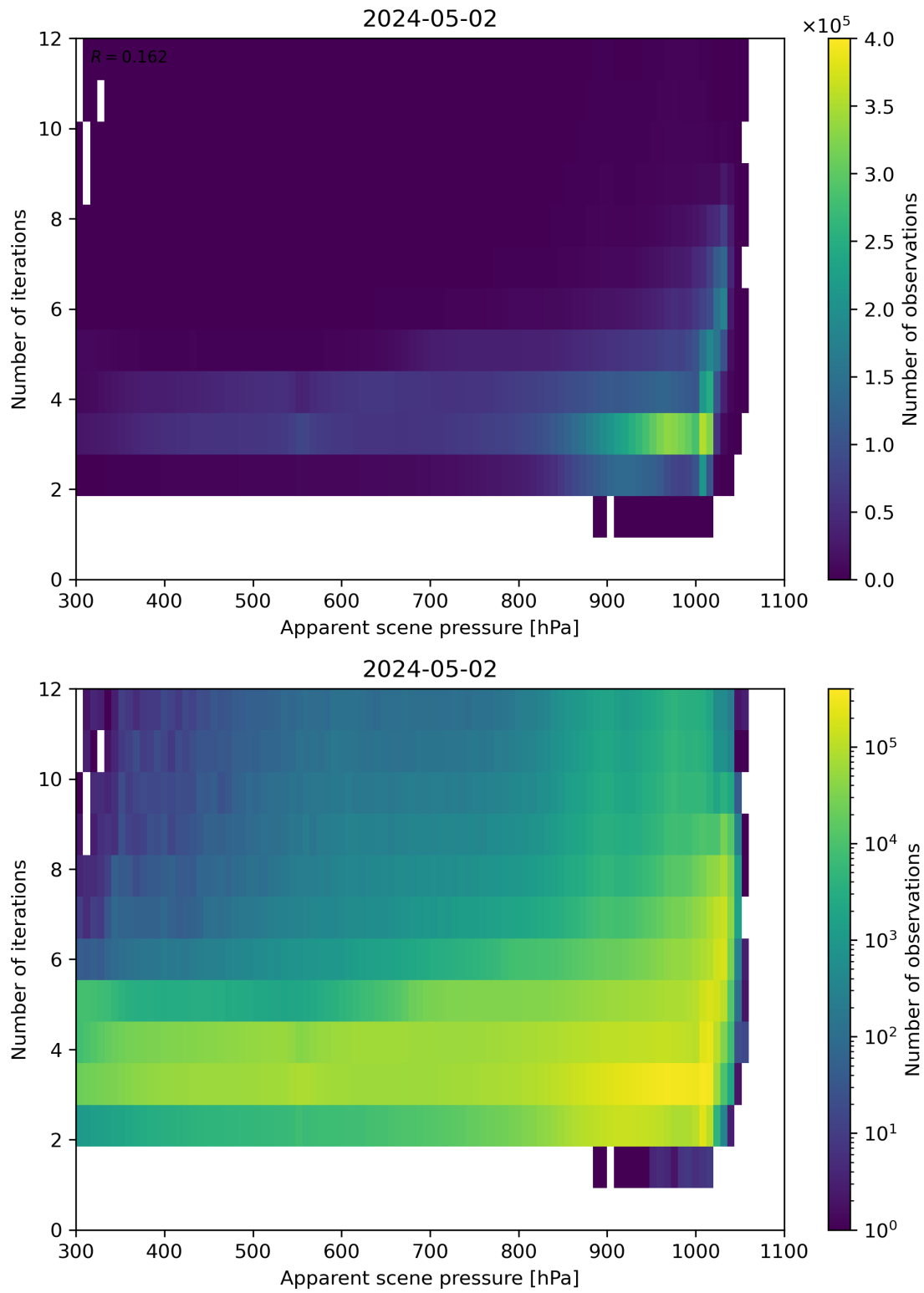
Figure 65: Scatter density plot of “Apparent scene pressure” against “Number of iterations” for 2024-05-02 to 2024-05-03.
