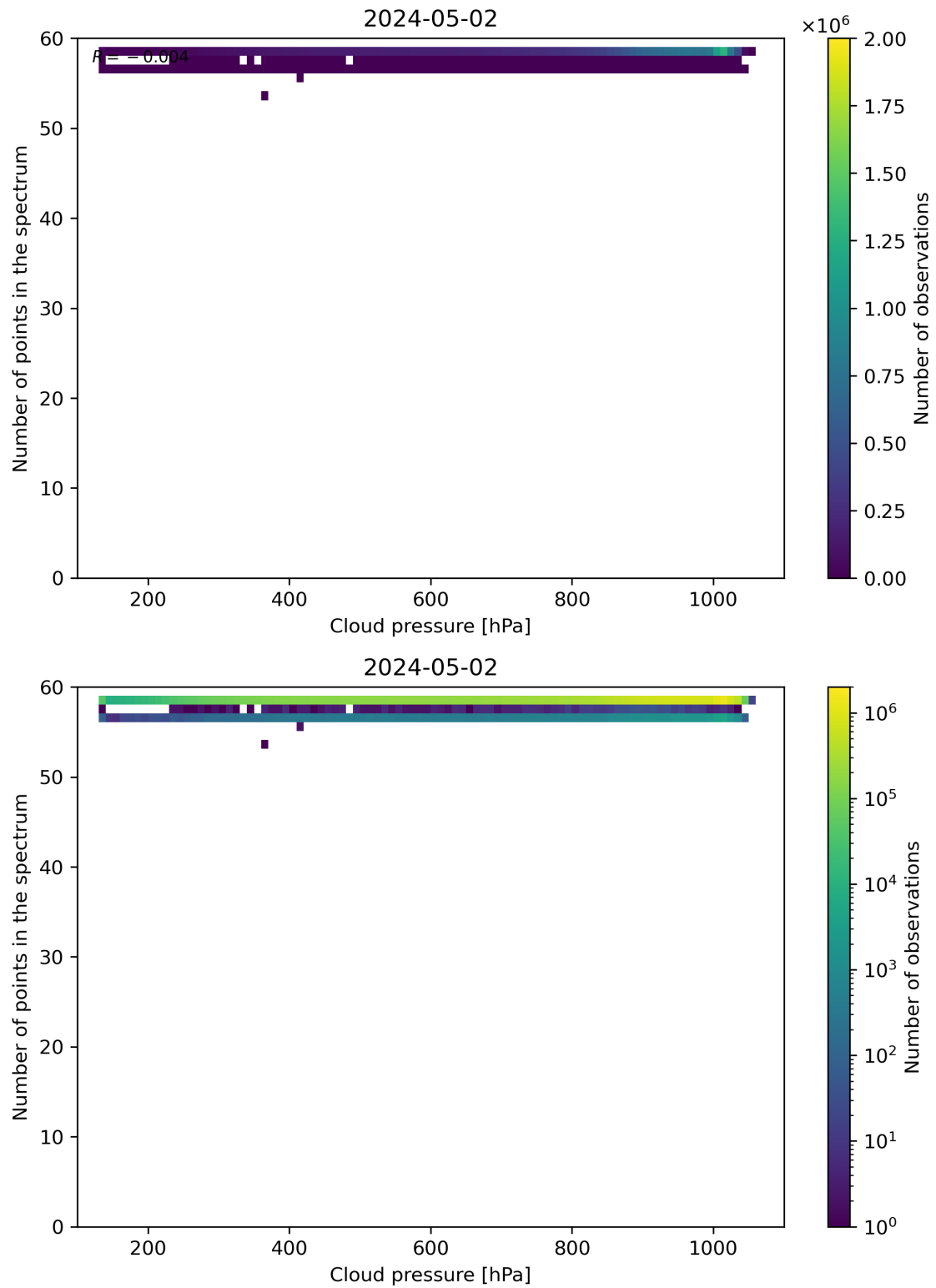
Figure 82: Scatter density plot of “Cloud pressure” against “Number of points in the spectrum” for 2024-05-02 to 2024-05-03.
