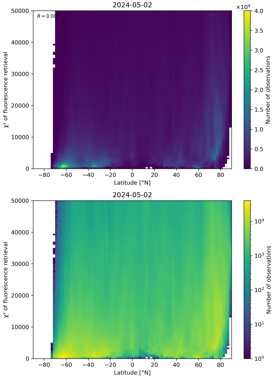
Figure 89: Scatter density plot of “Latitude” against “ \chi^2 of fluorescence retrieval” for 2024-05-02 to 2024-05-03.
