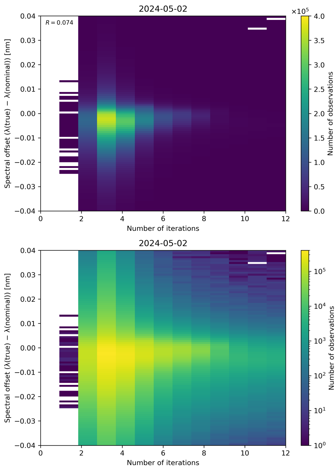
Figure 100: Scatter density plot of “Number of iterations” against “Spectral offset ( \lambda(\text{true}) - \lambda(\text{nominal}) )” for 2024-05-02 to 2024-05-03.
