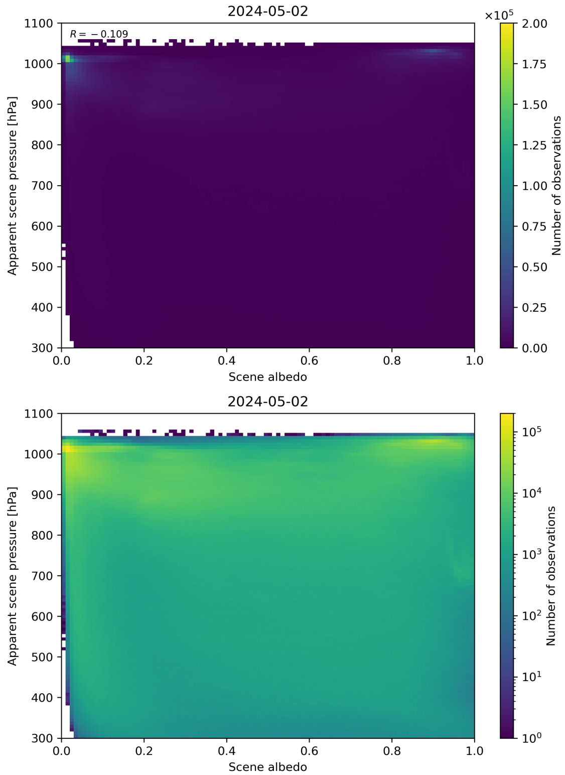
Figure 102: Scatter density plot of “Scene albedo” against “Apparent scene pressure” for 2024-05-02 to 2024-05-03.
