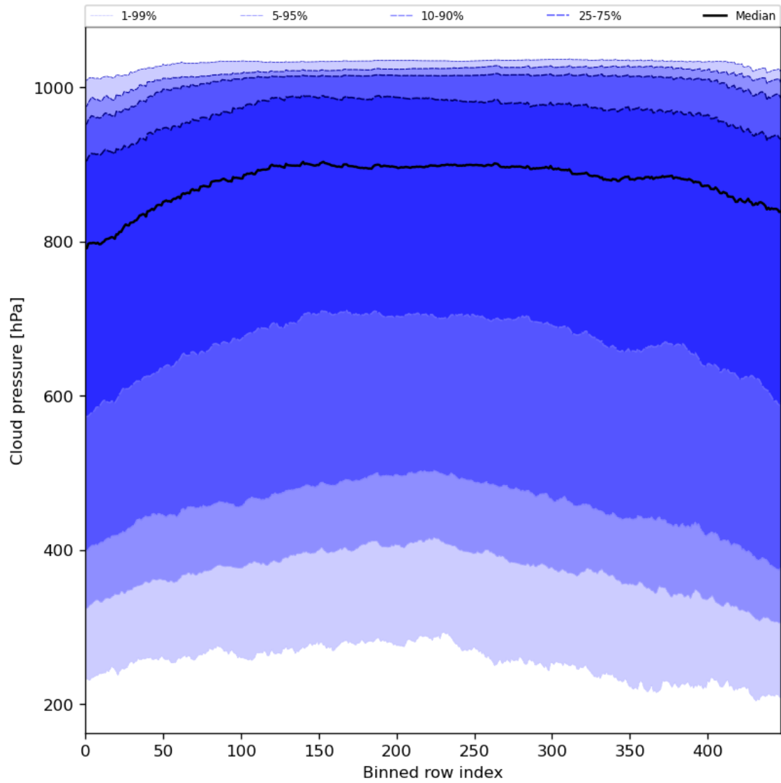
Figure 47: Along track statistics of “Cloud pressure” for 2024-05-02 to 2024-05-03
