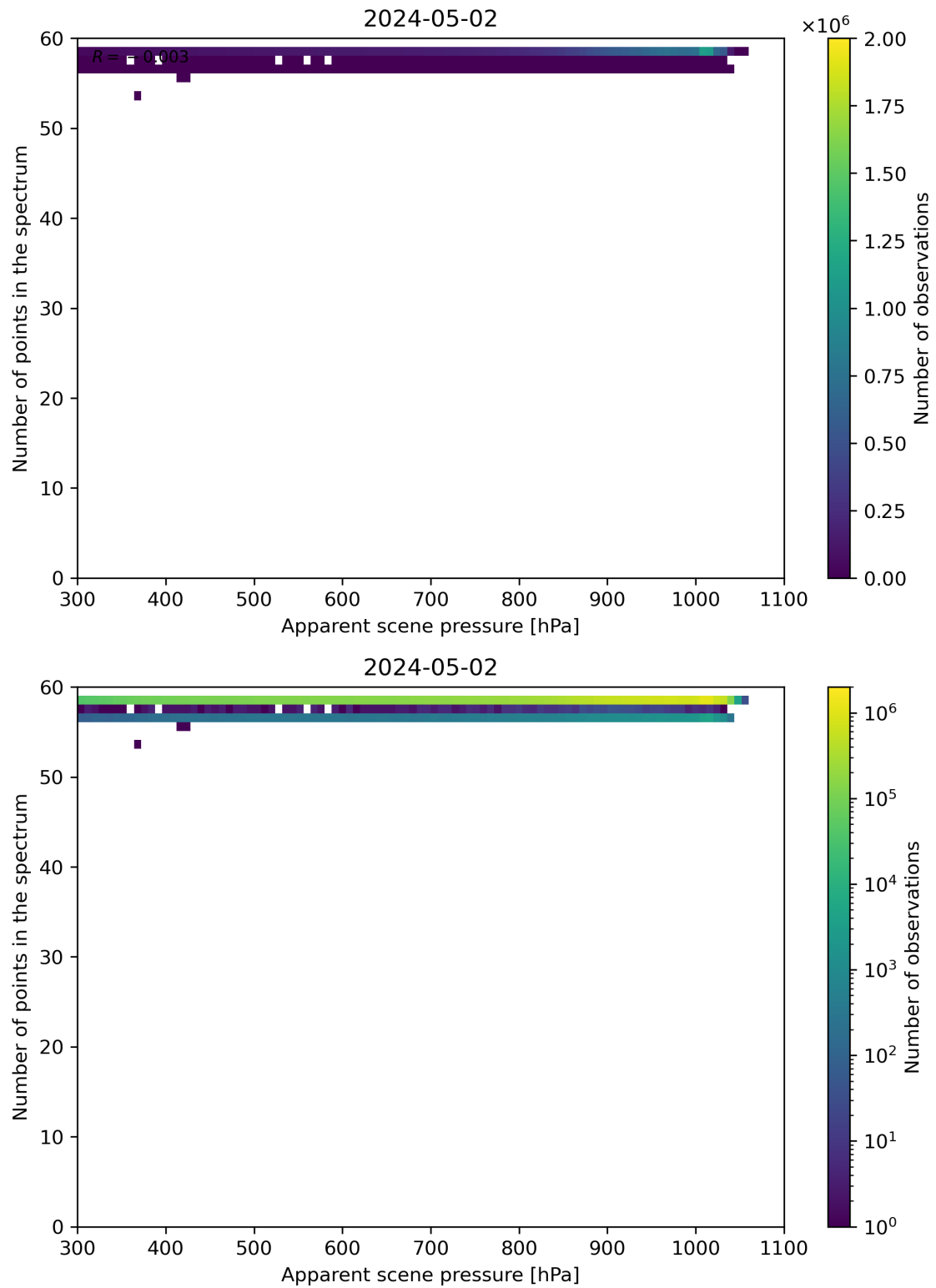
Figure 66: Scatter density plot of “Apparent scene pressure” against “Number of points in the spectrum” for 2024-05-02 to 2024-05-03.
