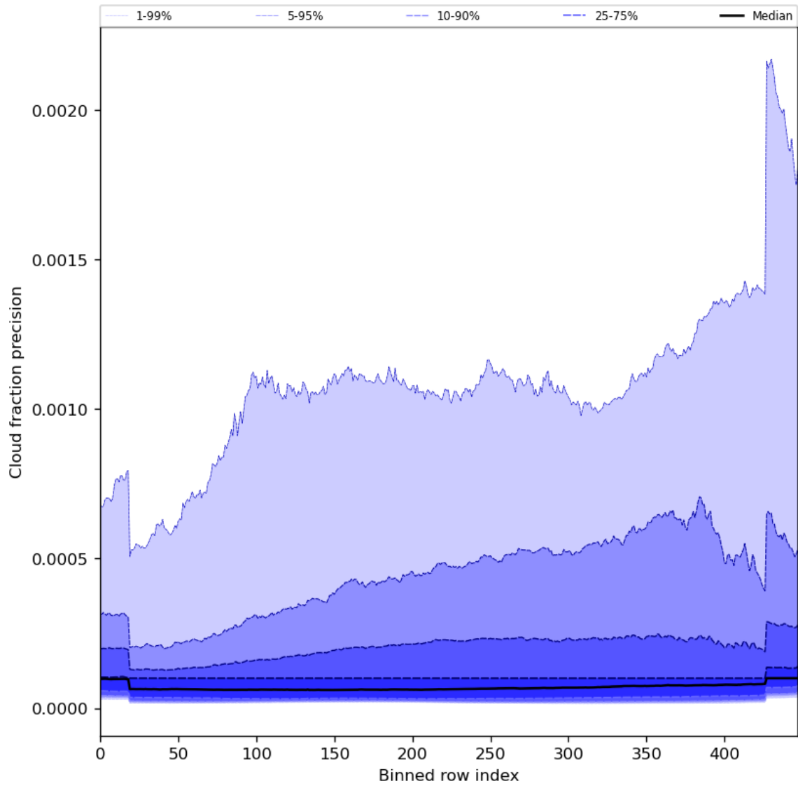
Figure 50: Along track statistics of “Cloud fraction precision” for 2024-05-02 to 2024-05-03
