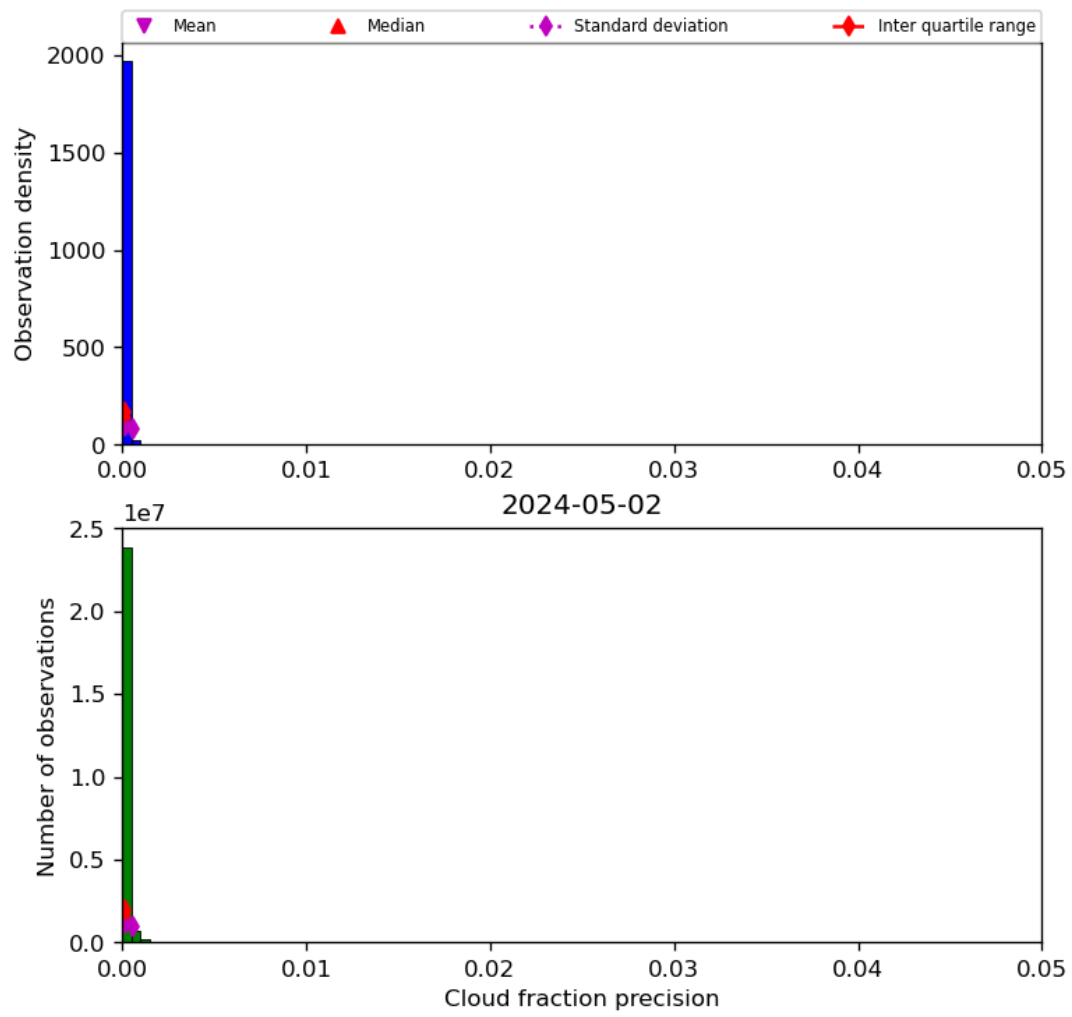
Figure 33: Histogram of “Cloud fraction precision” for 2024-05-02 to 2024-05-03
