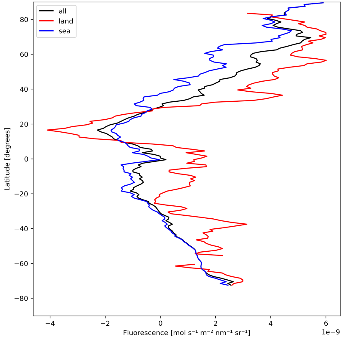
Figure 23: Zonal average of “Fluorescence” for 2024-05-02 to 2024-05-03.
