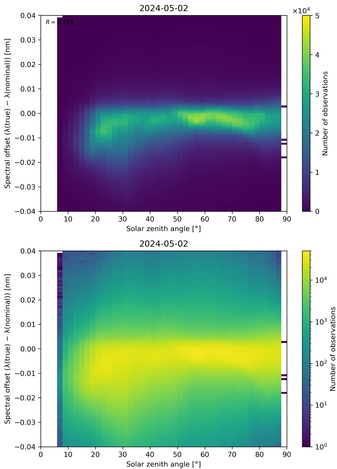
Figure 117: Scatter density plot of “Solar zenith angle” against “Spectral offset ( \lambda(\text{true}) - \lambda(\text{nominal}) )” for 2024-05-02 to 2024-05-03.
