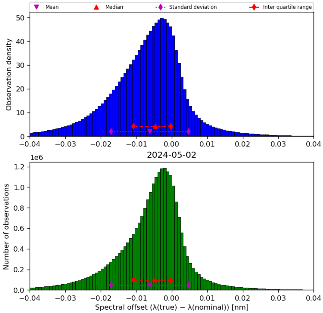
Figure 45: Histogram of “Spectral offset ( \lambda(\text{true}) - \lambda(\text{nominal}) )” for 2024-05-02 to 2024-05-03
