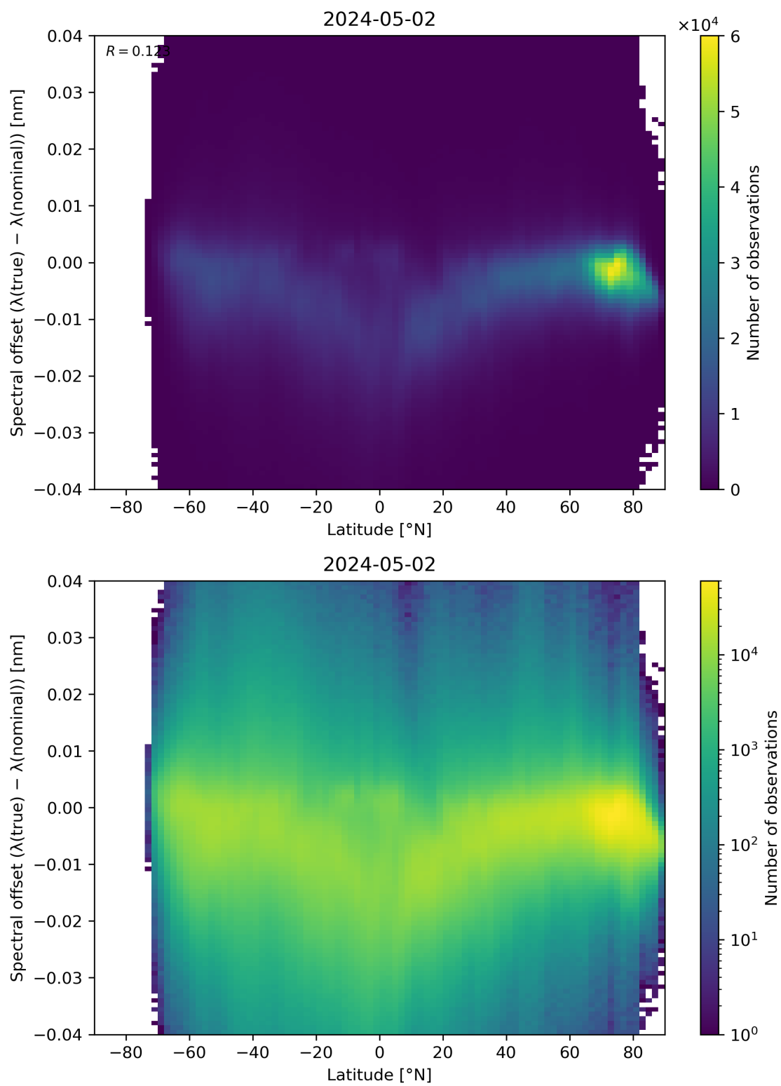
Figure 96: Scatter density plot of “Latitude” against “Spectral offset ( \lambda(\text{true}) - \lambda(\text{nominal}) )” for 2024-05-02 to 2024-05-03.
