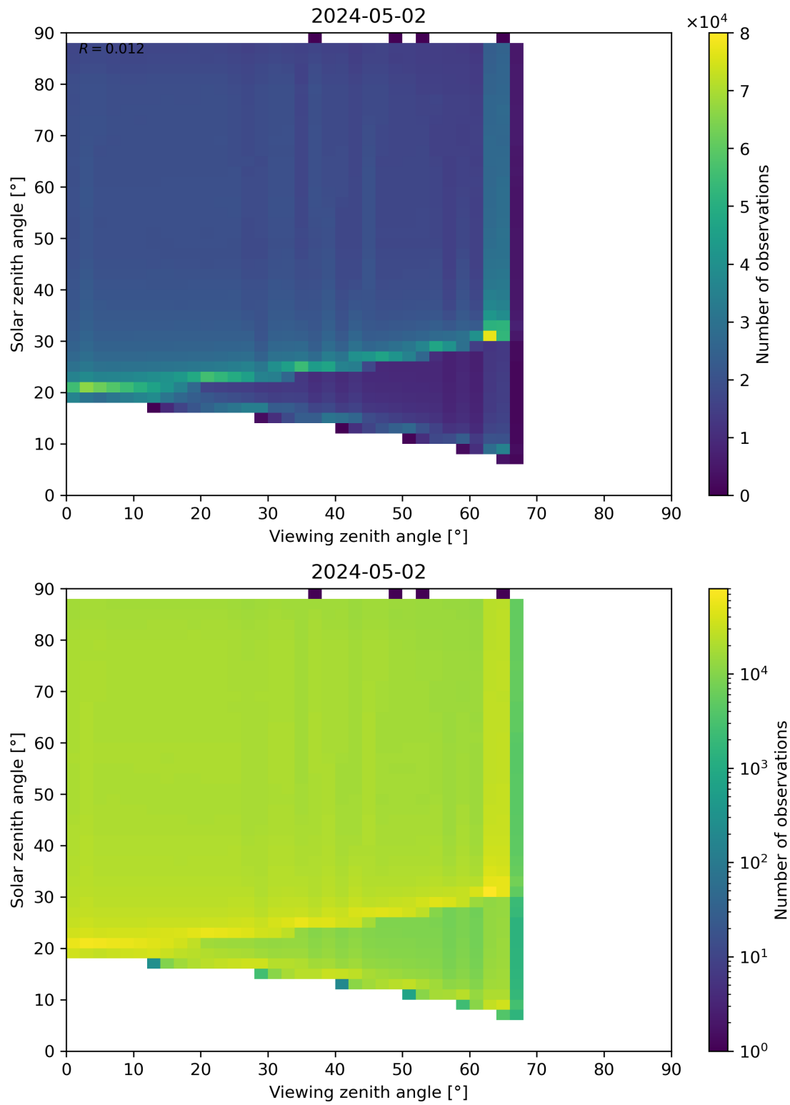
Figure 127: Scatter density plot of “Viewing zenith angle” against “Solar zenith angle” for 2024-05-02 to 2024-05-03.
