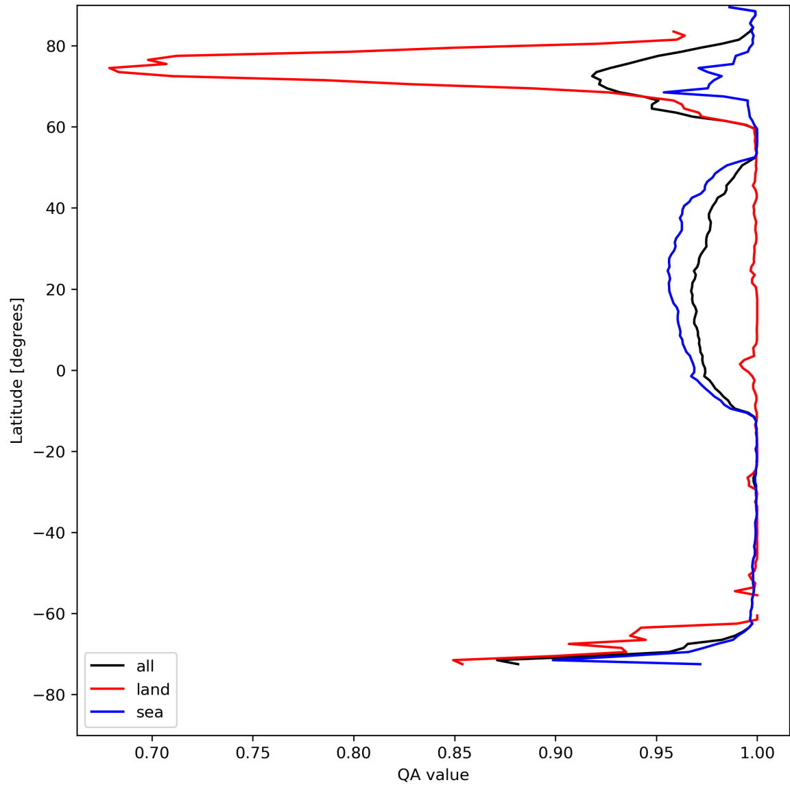
Figure 12: Zonal average of “QA value” for 2024-05-02 to 2024-05-03.
