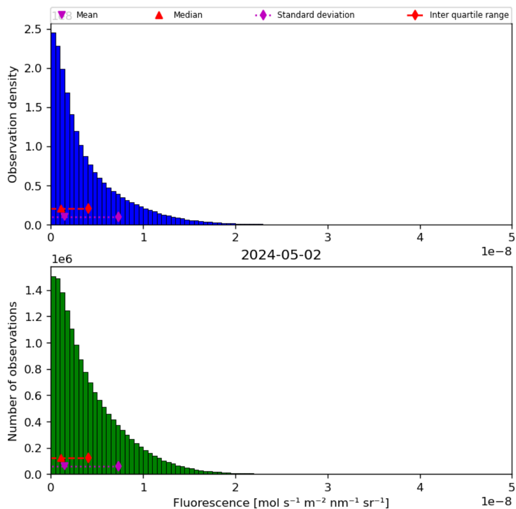
Figure 40: Histogram of “Fluorescence” for 2024-05-02 to 2024-05-03
