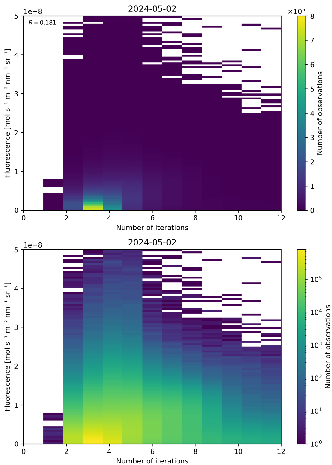
Figure 98: Scatter density plot of “Number of iterations” against “Fluorescence” for 2024-05-02 to 2024-05-03.
