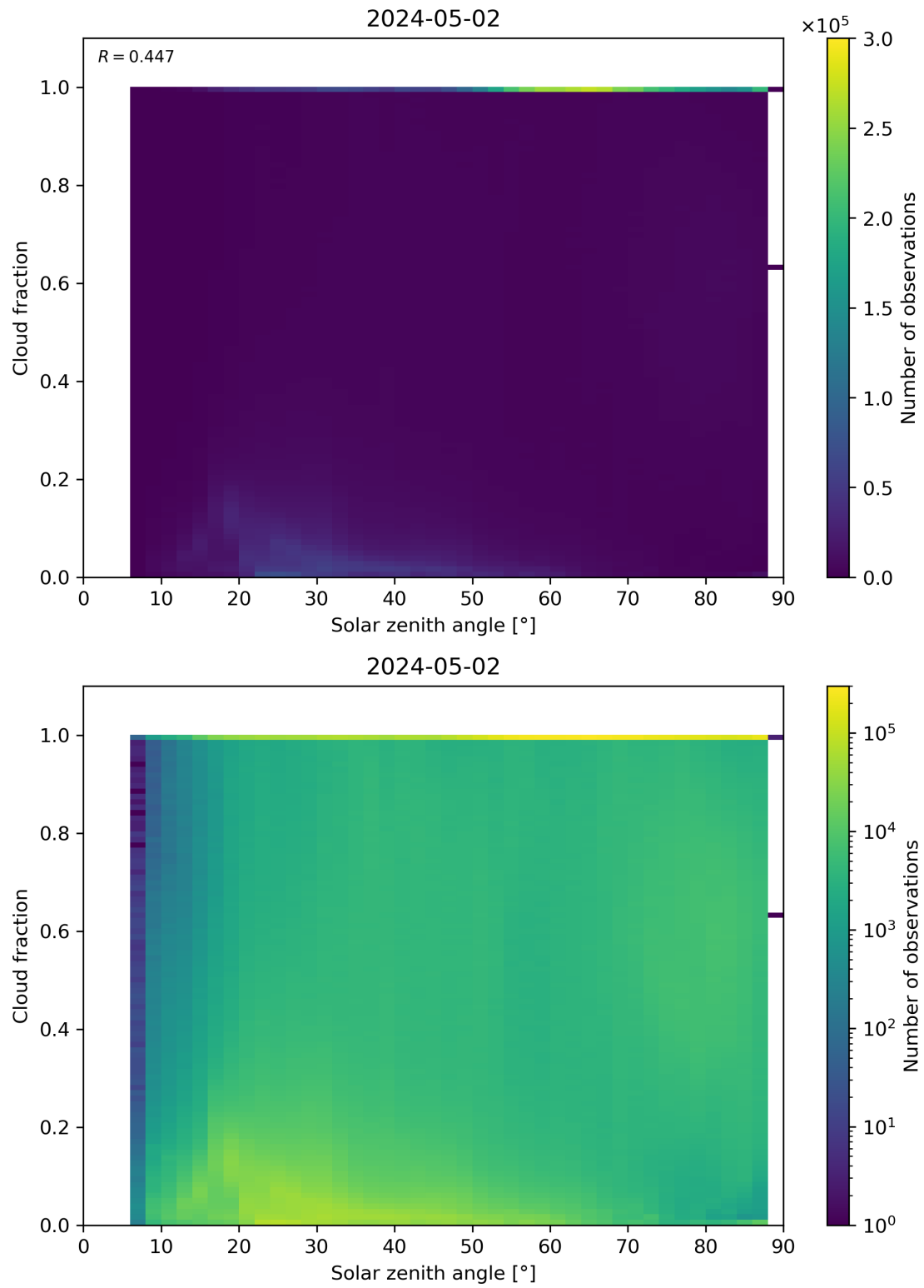
Figure 110: Scatter density plot of “Solar zenith angle” against “Cloud fraction” for 2024-05-02 to 2024-05-03.
