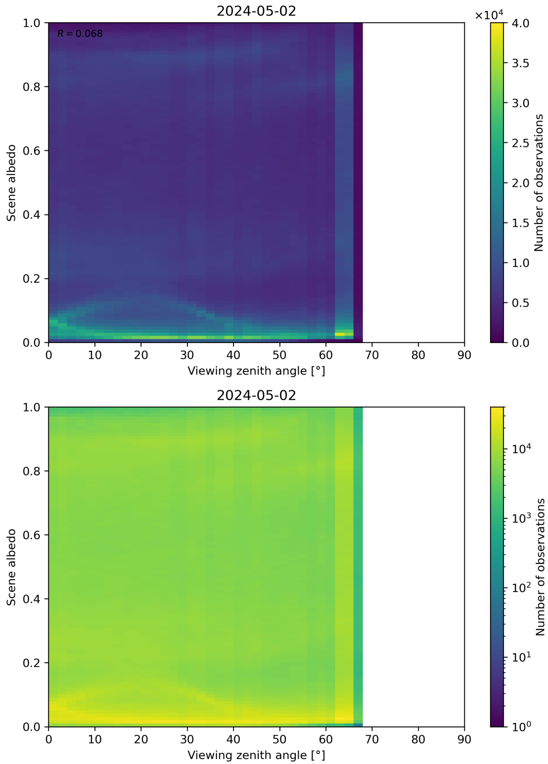
Figure 126: Scatter density plot of “Viewing zenith angle” against “Scene albedo” for 2024-05-02 to 2024-05-03.
