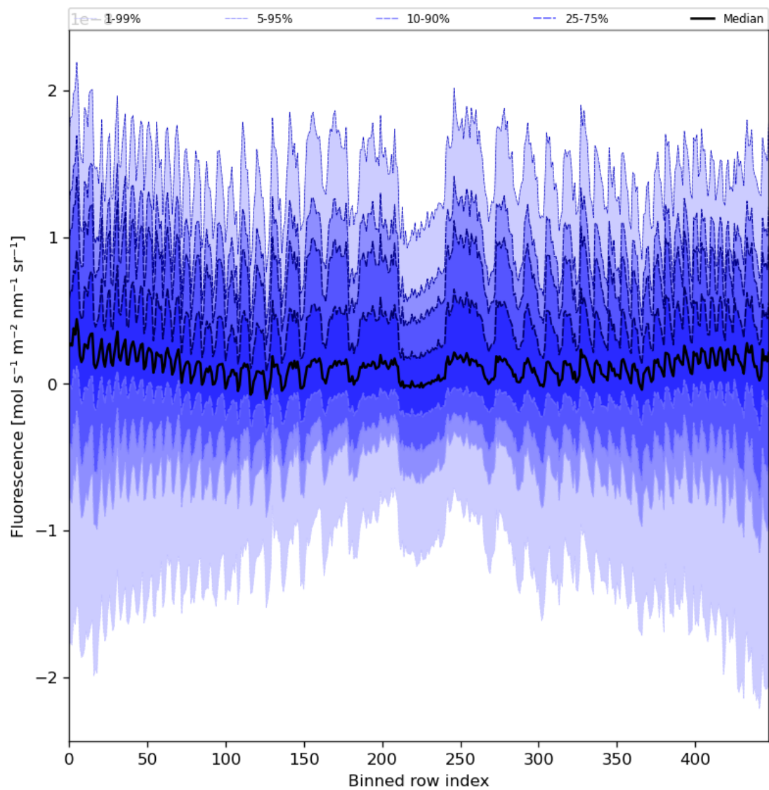
Figure 57: Along track statistics of “Fluorescence” for 2024-05-02 to 2024-05-03
