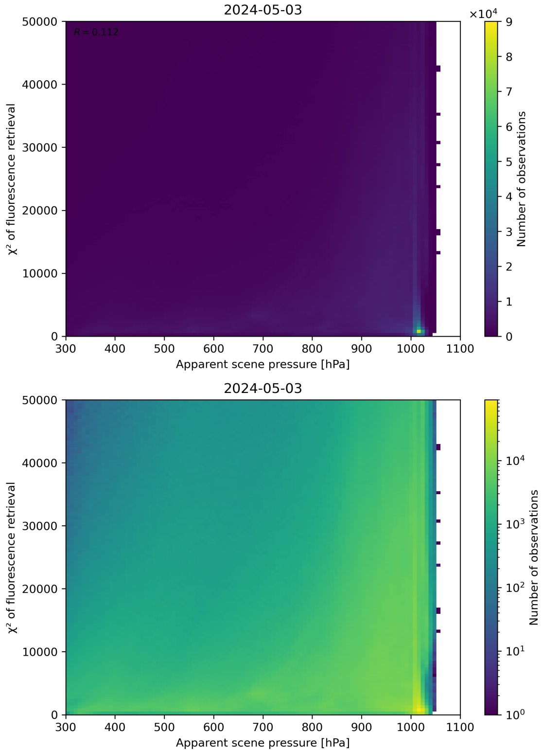
Figure 63: Scatter density plot of “Apparent scene pressure” against “ \chi^2 of fluorescence retrieval” for 2024-05-02 to 2024-05-04.
