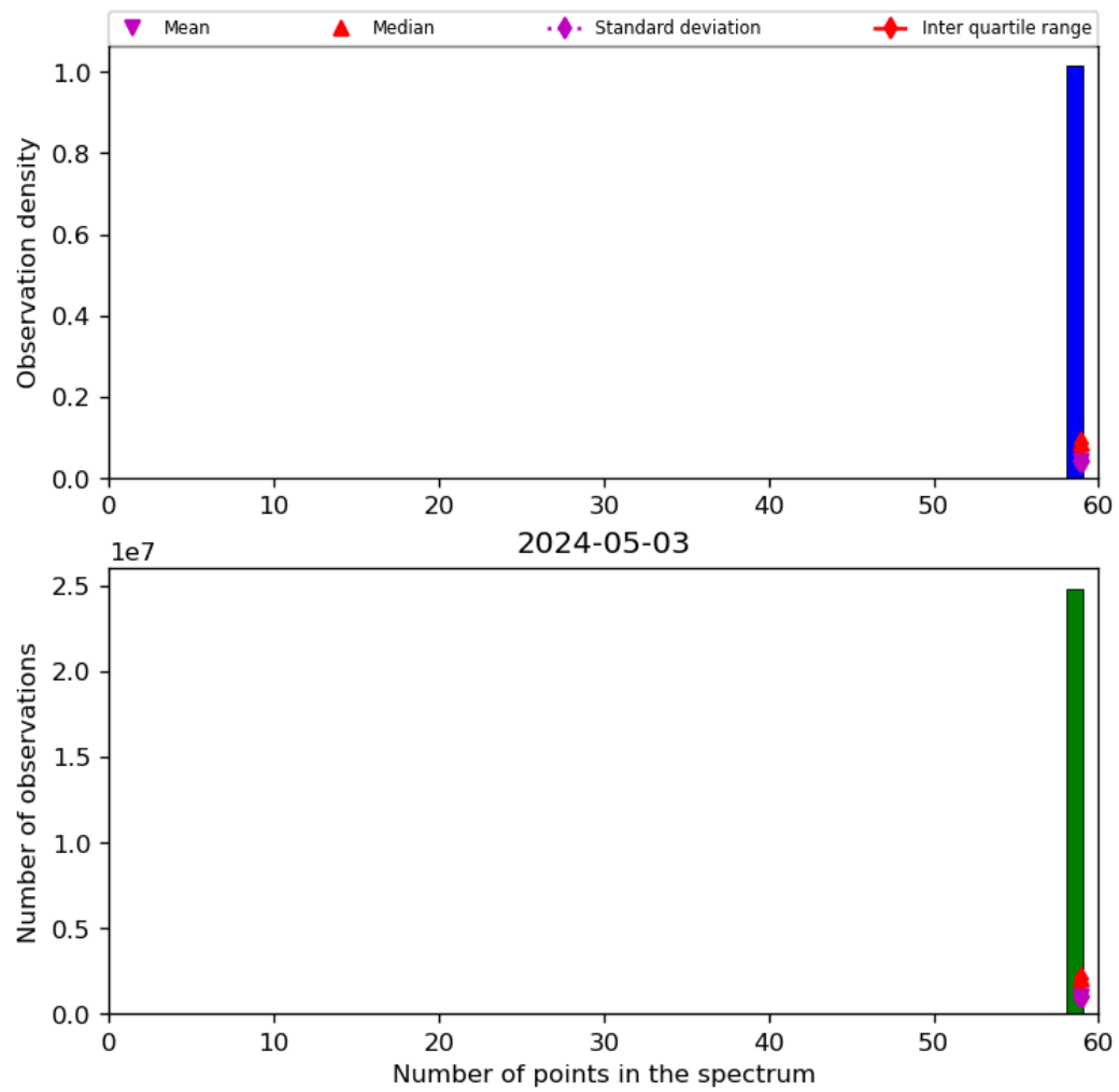
Figure 44: Histogram of “Number of points in the spectrum” for 2024-05-02 to 2024-05-04
