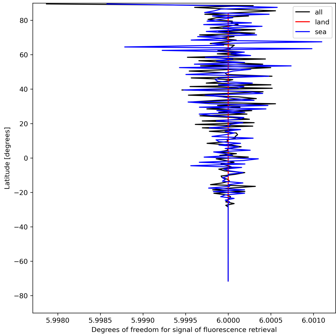
Figure 26: Zonal average of “Degrees of freedom for signal of fluorescence retrieval” for 2024-05-02 to 2024-05-04.
