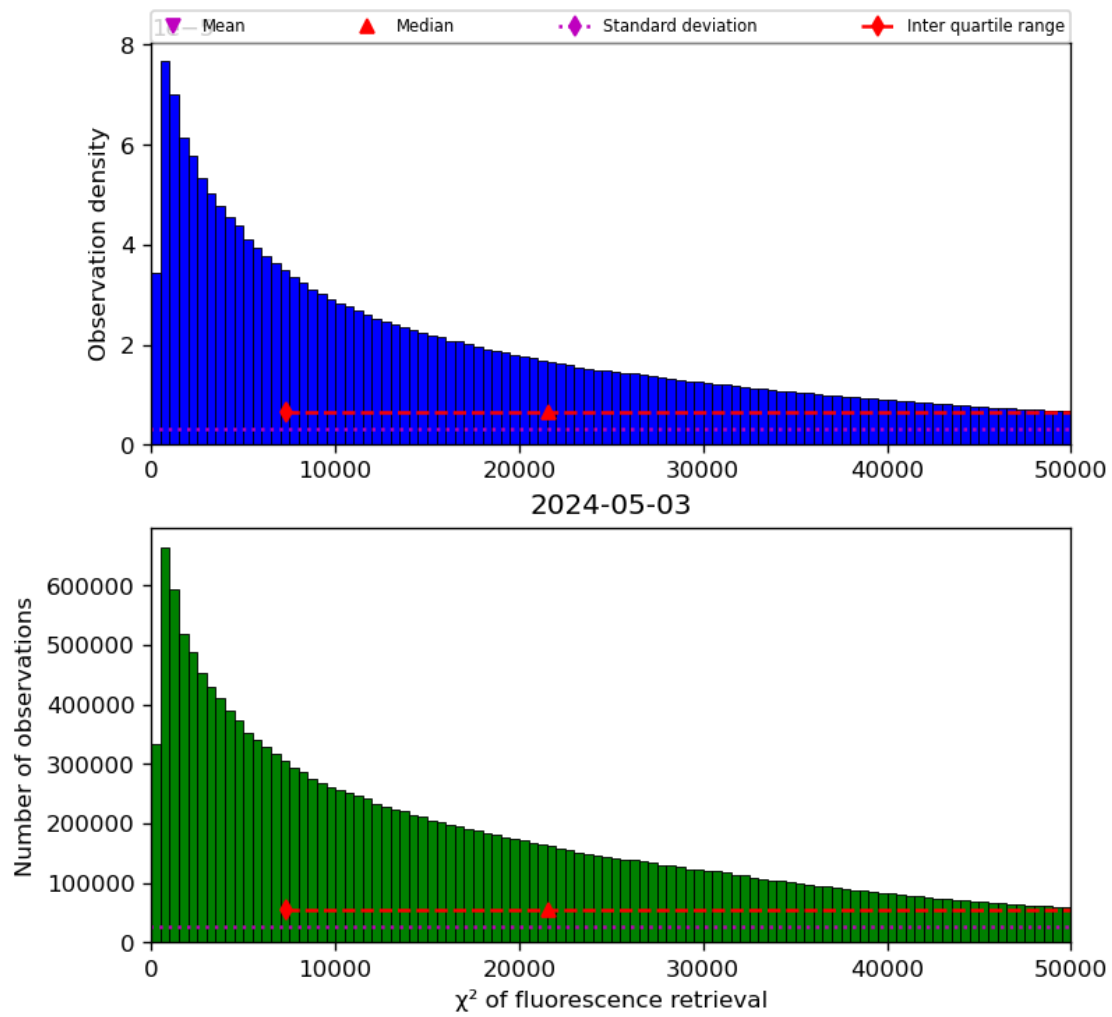
Figure 42: Histogram of “ \chi^2 of fluorescence retrieval” for 2024-05-02 to 2024-05-04
