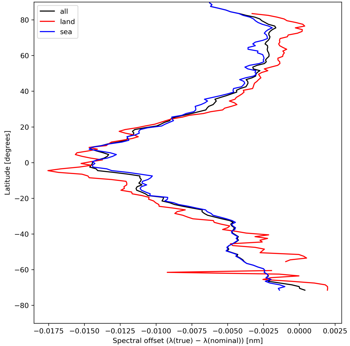
Figure 28: Zonal average of “Spectral offset ( \lambda(\text{true}) - \lambda(\text{nominal}) )” for 2024-05-02 to 2024-05-04.
