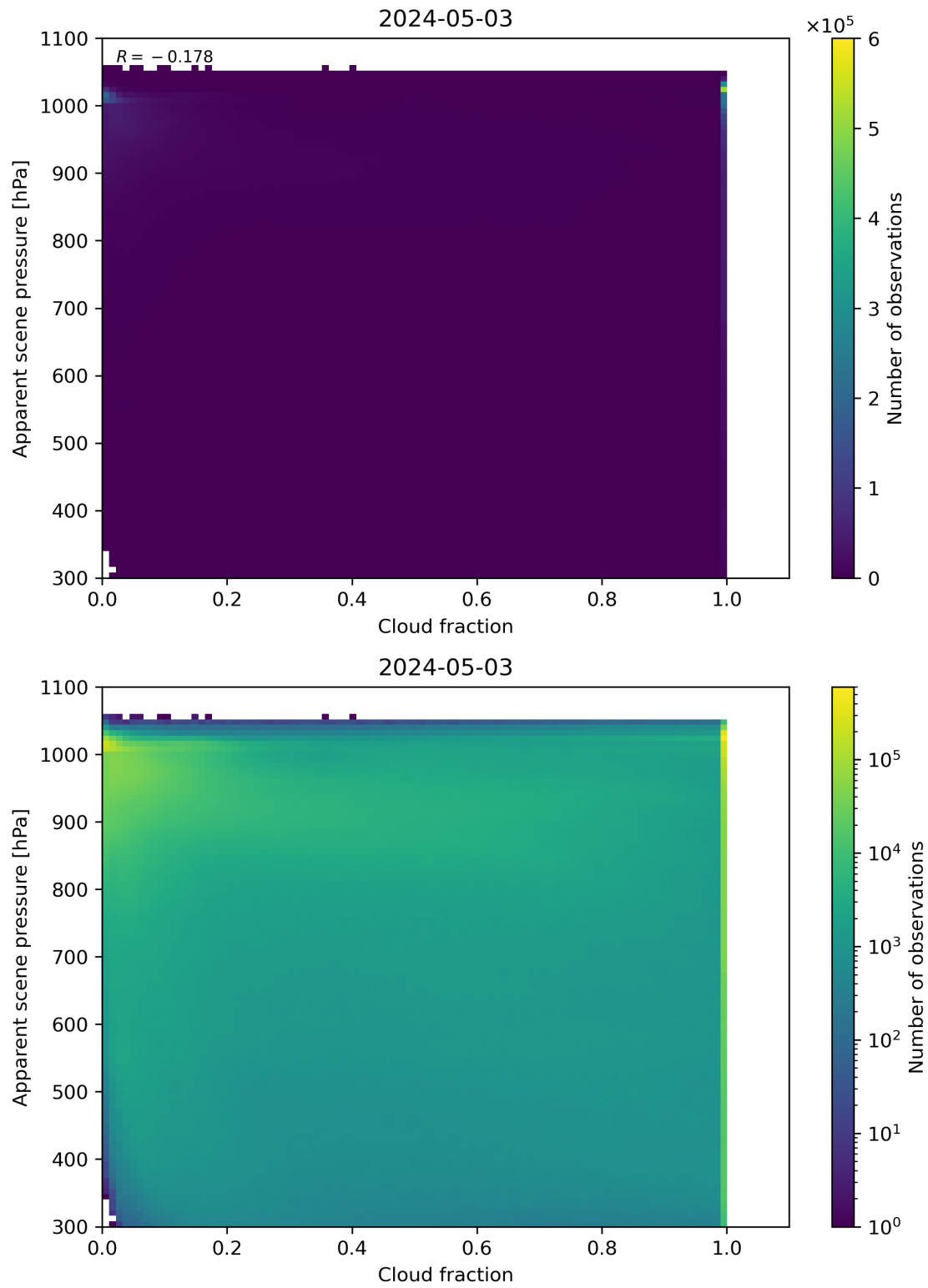
Figure 70: Scatter density plot of “Cloud fraction” against “Apparent scene pressure” for 2024-05-02 to 2024-05-04.
