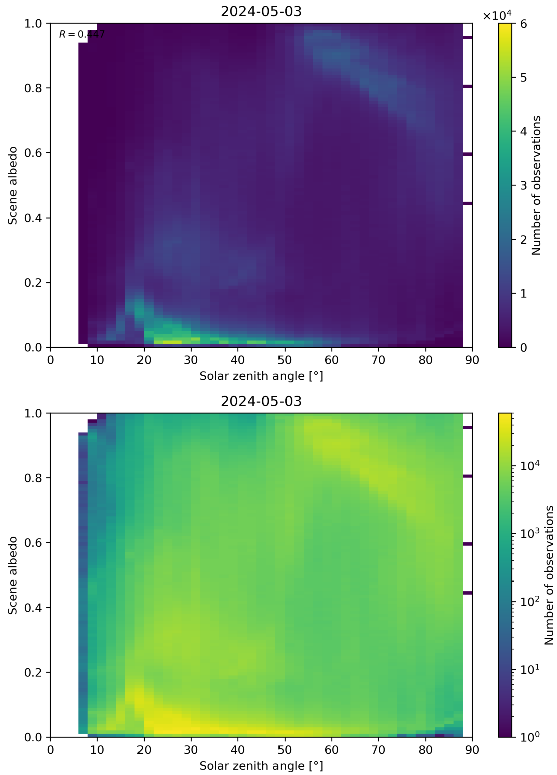
Figure 116: Scatter density plot of “Solar zenith angle” against “Scene albedo” for 2024-05-02 to 2024-05-04.
