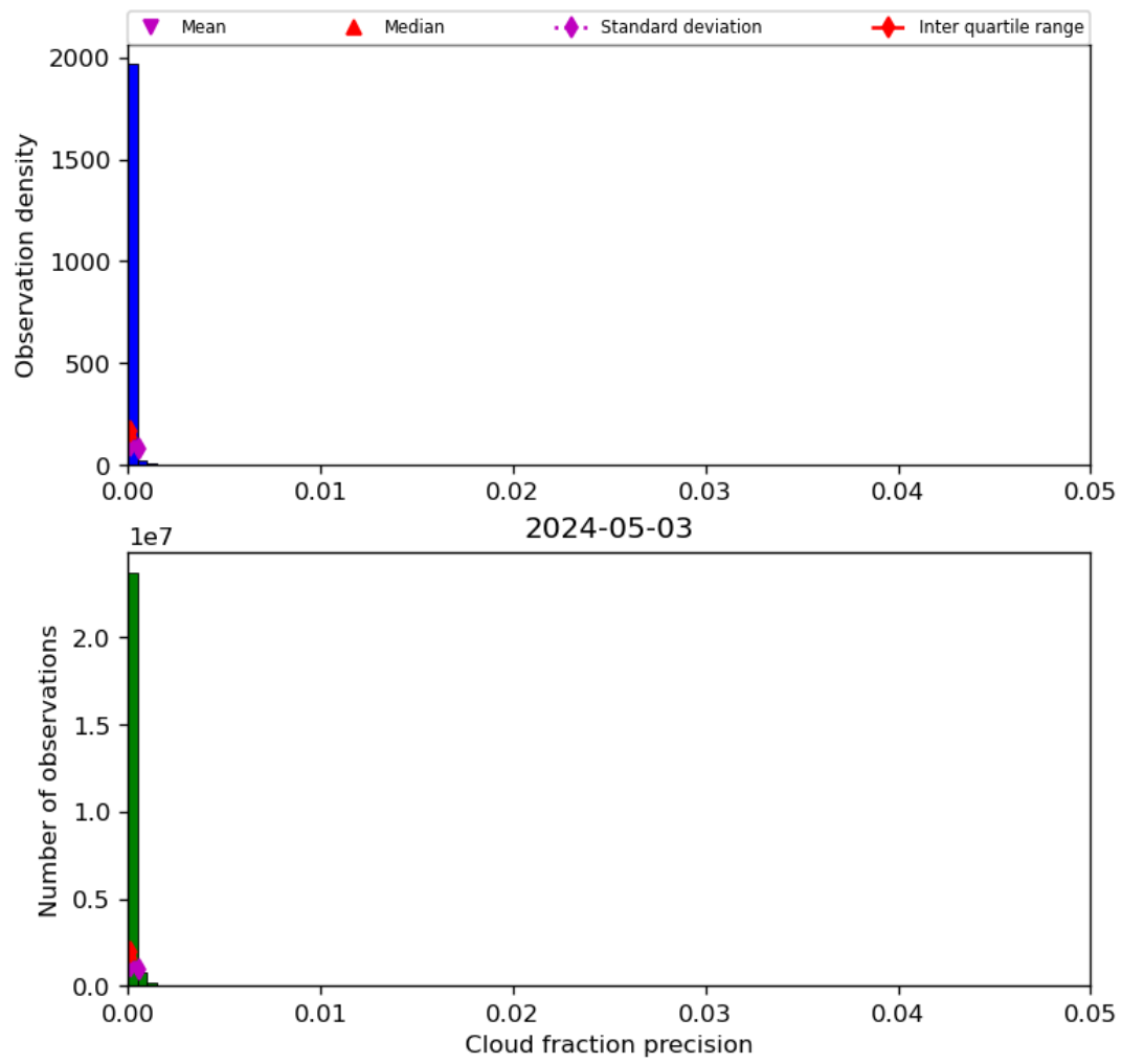
Figure 33: Histogram of “Cloud fraction precision” for 2024-05-02 to 2024-05-04
