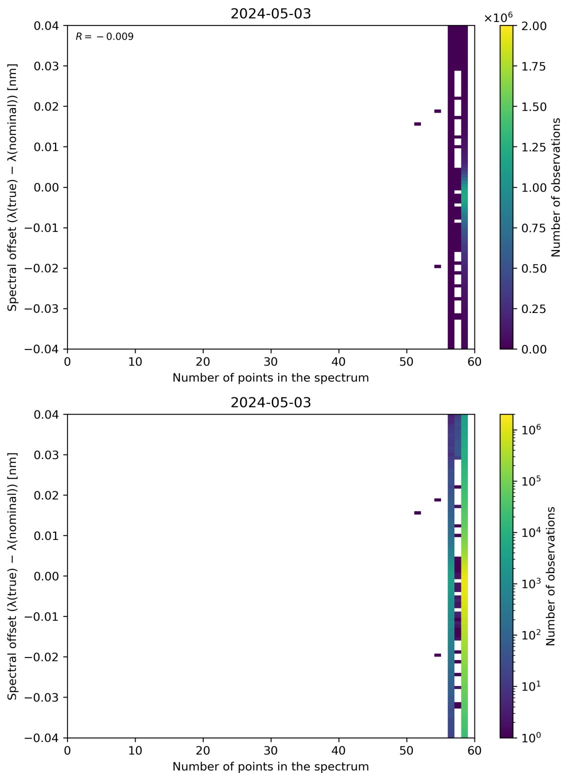
Figure 101: Scatter density plot of “Number of points in the spectrum” against “Spectral offset ( \lambda(\text{true}) - \lambda(\text{nominal}) )” for 2024-05-02 to 2024-05-04.
