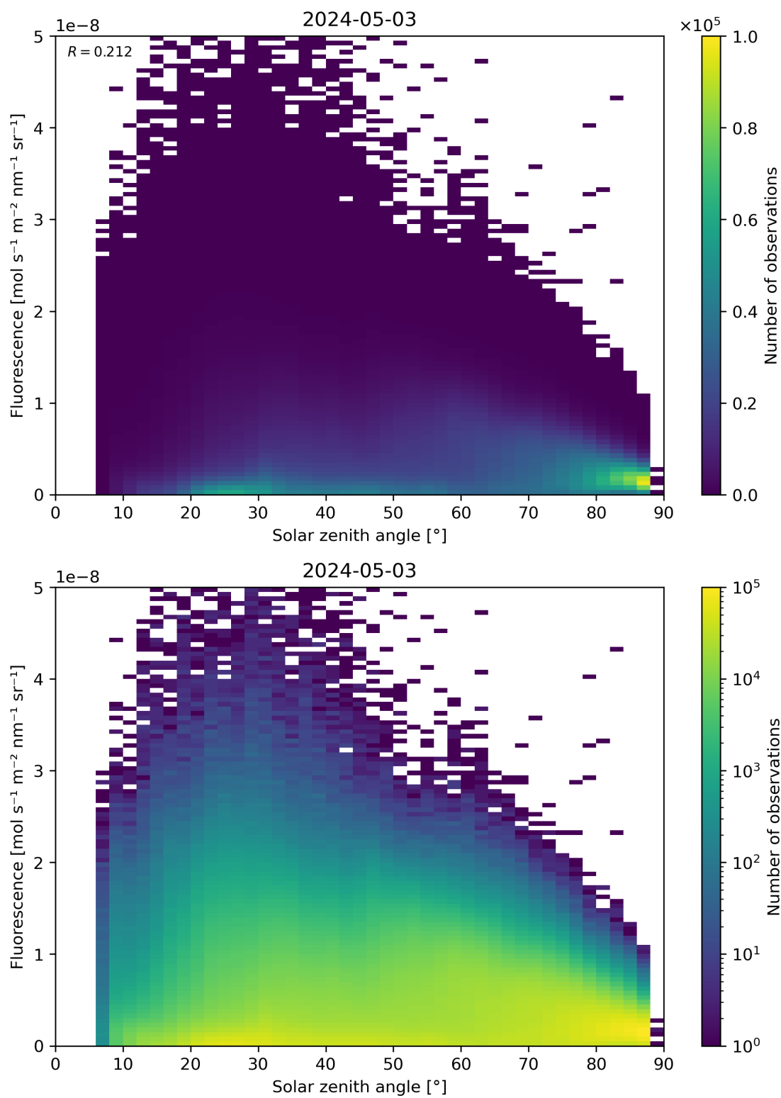
Figure 112: Scatter density plot of “Solar zenith angle” against “Fluorescence” for 2024-05-02 to 2024-05-04.
