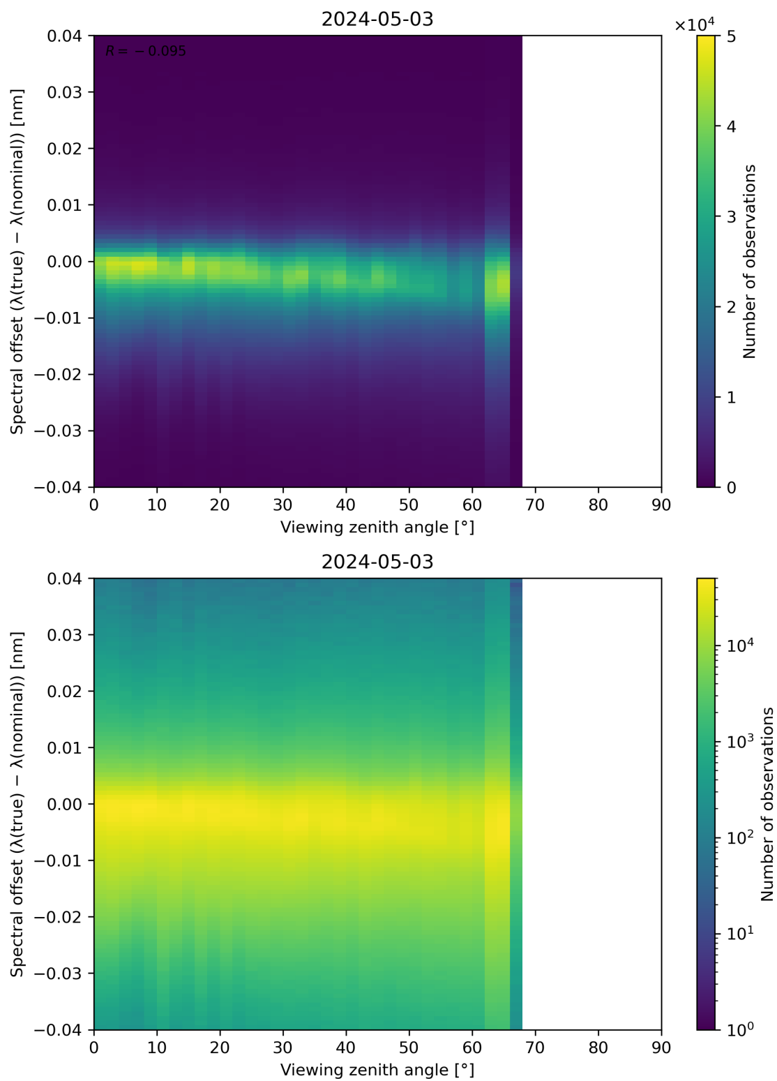
Figure 128: Scatter density plot of “Viewing zenith angle” against “Spectral offset ( \lambda(\text{true}) - \lambda(\text{nominal}) )” for 2024-05-02 to 2024-05-04.
