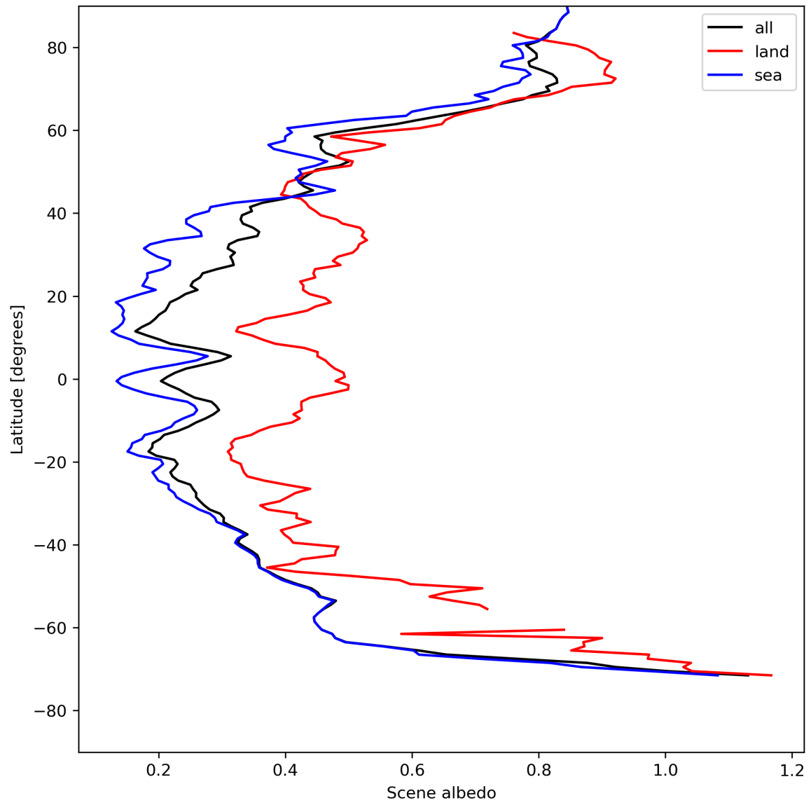
Figure 17: Zonal average of “Scene albedo” for 2024-05-02 to 2024-05-04.
