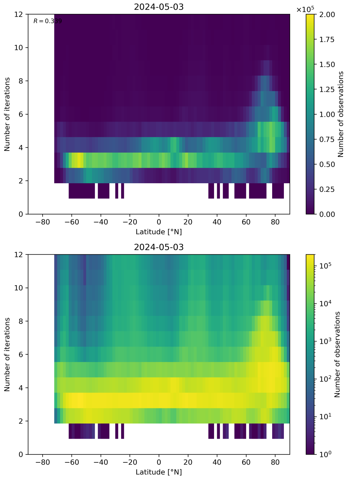
Figure 93: Scatter density plot of “Latitude” against “Number of iterations” for 2024-05-02 to 2024-05-04.
