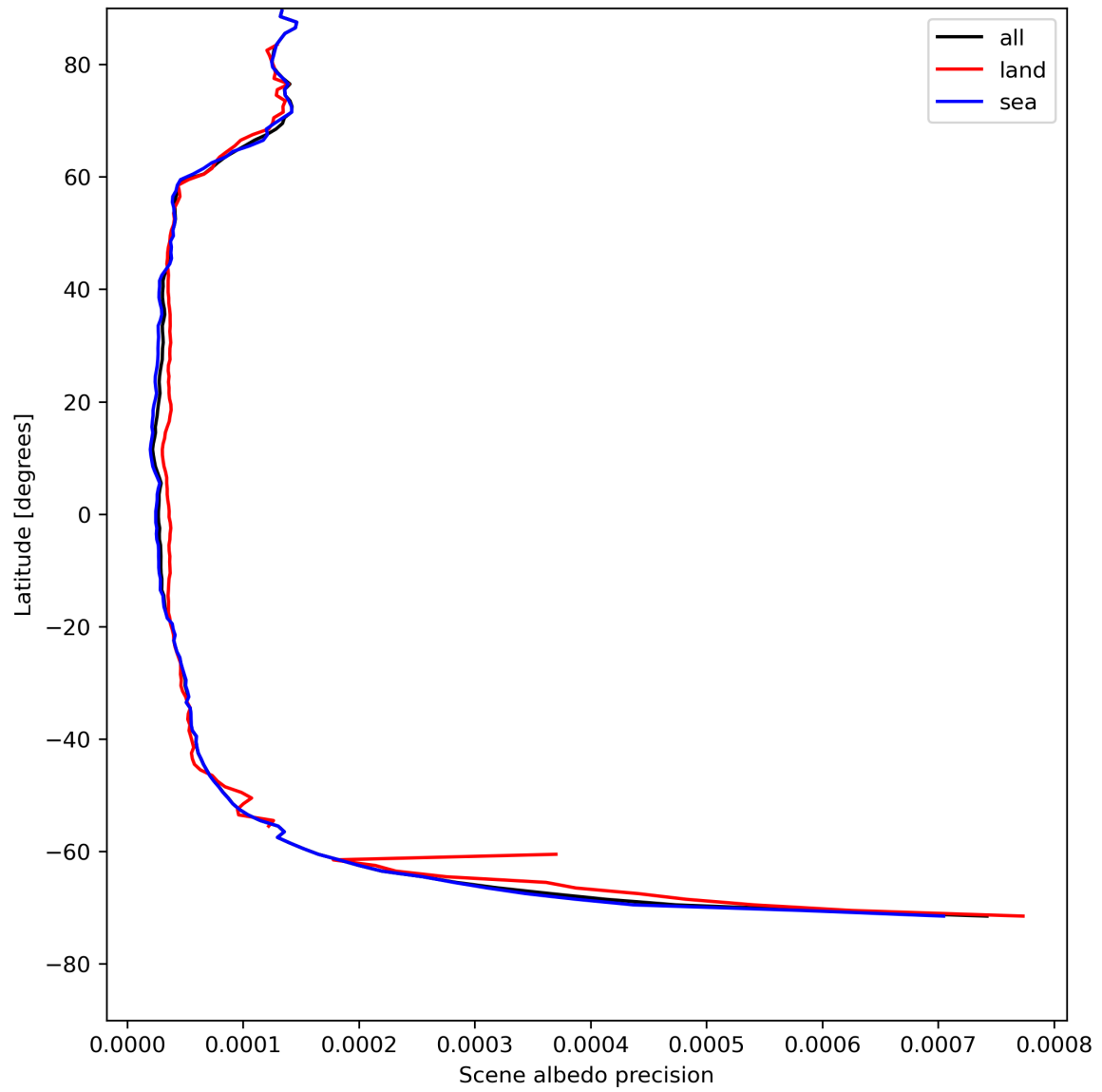
Figure 18: Zonal average of “Scene albedo precision” for 2024-05-02 to 2024-05-04.
