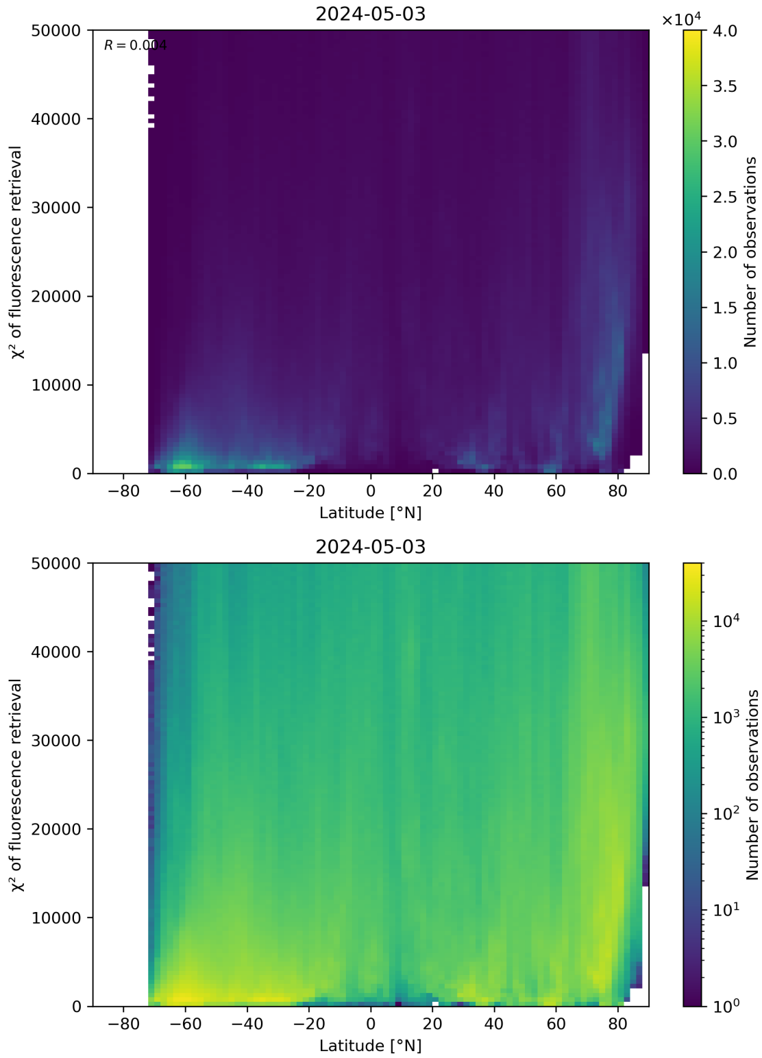
Figure 89: Scatter density plot of “Latitude” against “ \chi^2 of fluorescence retrieval” for 2024-05-02 to 2024-05-04.
