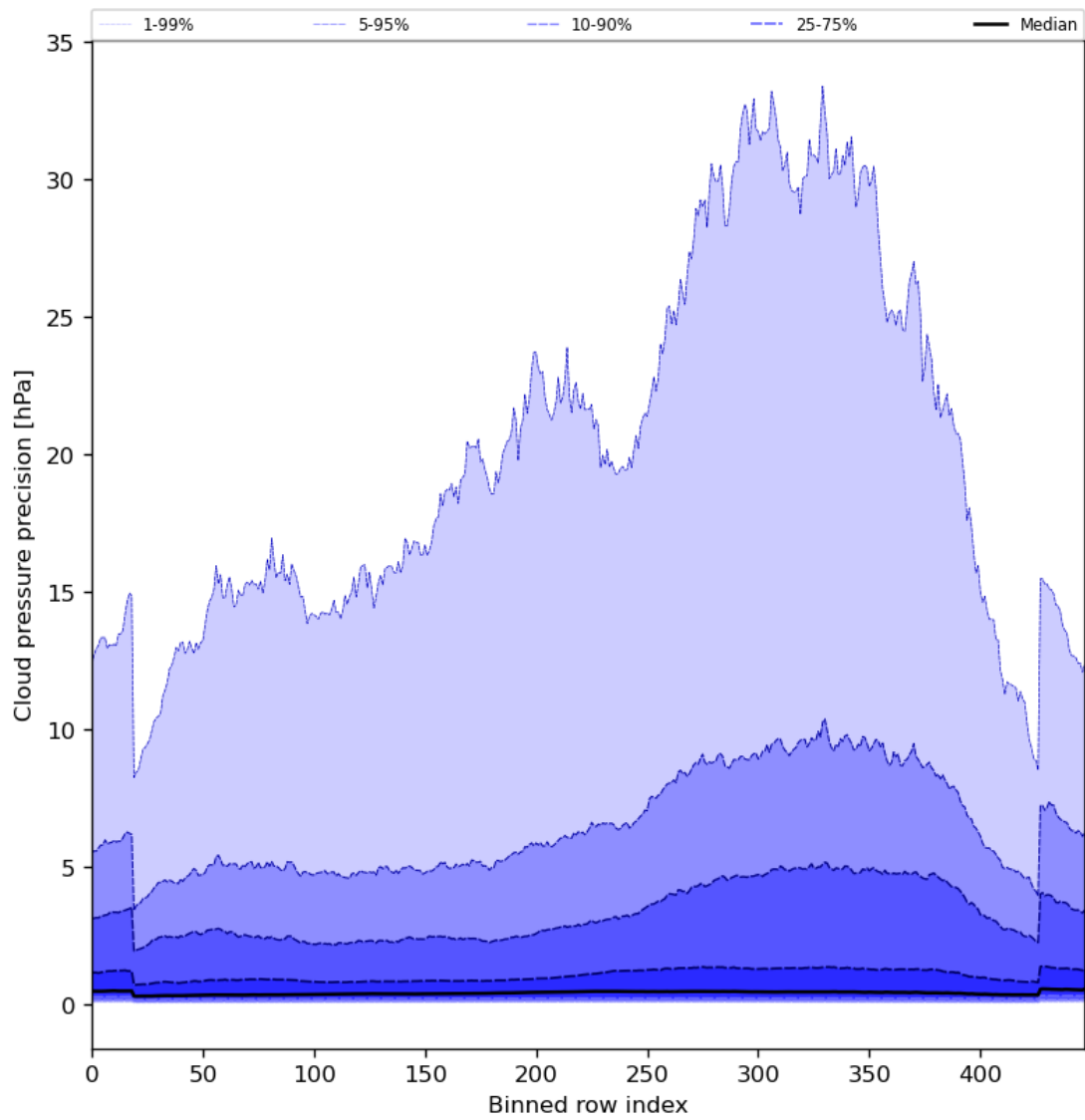
Figure 48: Along track statistics of “Cloud pressure precision” for 2024-05-02 to 2024-05-04
