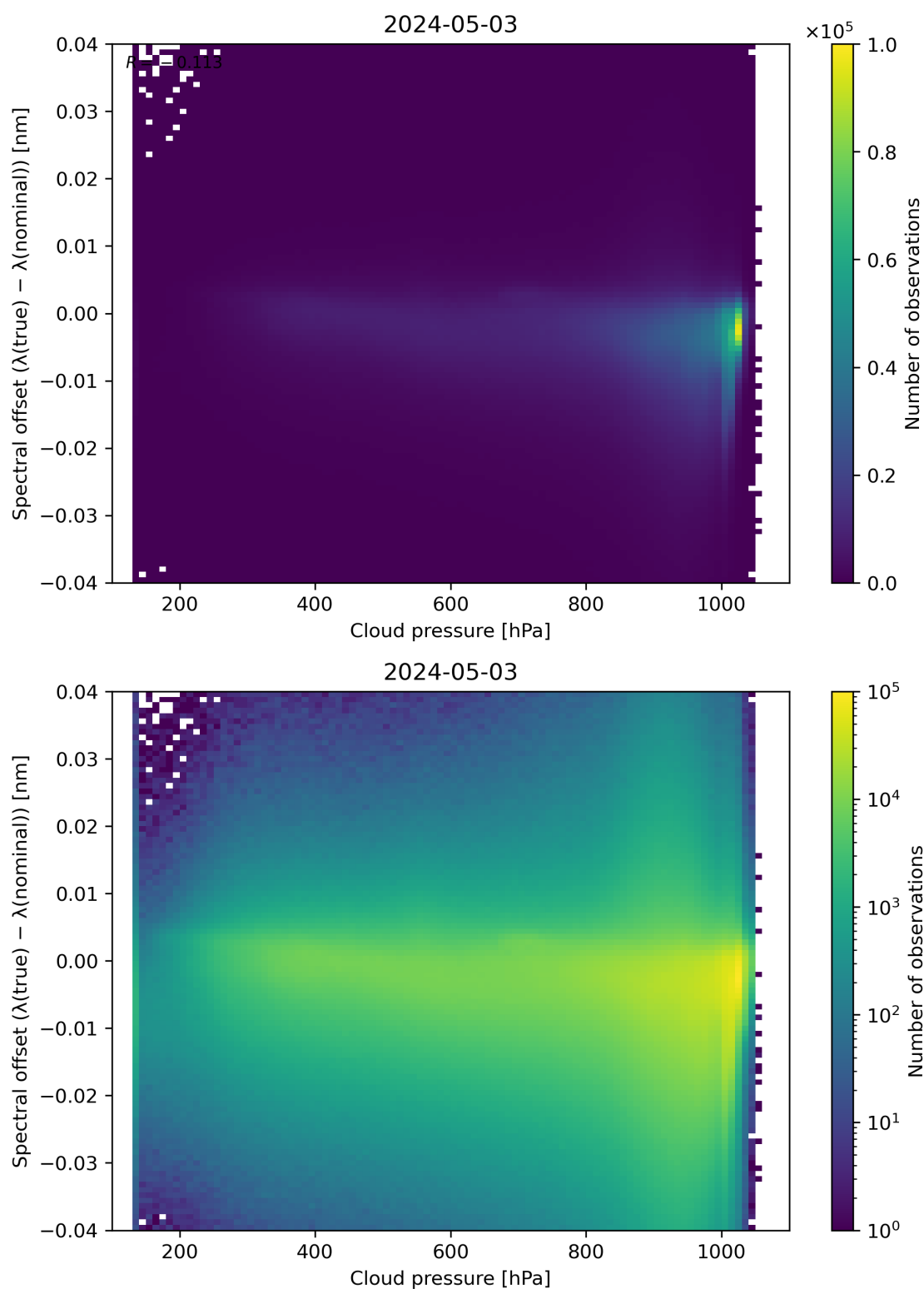
Figure 84: Scatter density plot of “Cloud pressure” against “Spectral offset ( \lambda(\text{true}) - \lambda(\text{nominal}) )” for 2024-05-02 to 2024-05-04.
