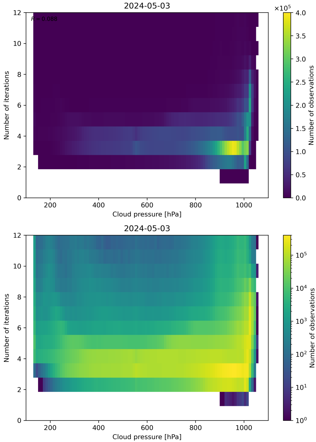
Figure 81: Scatter density plot of “Cloud pressure” against “Number of iterations” for 2024-05-02 to 2024-05-04.
