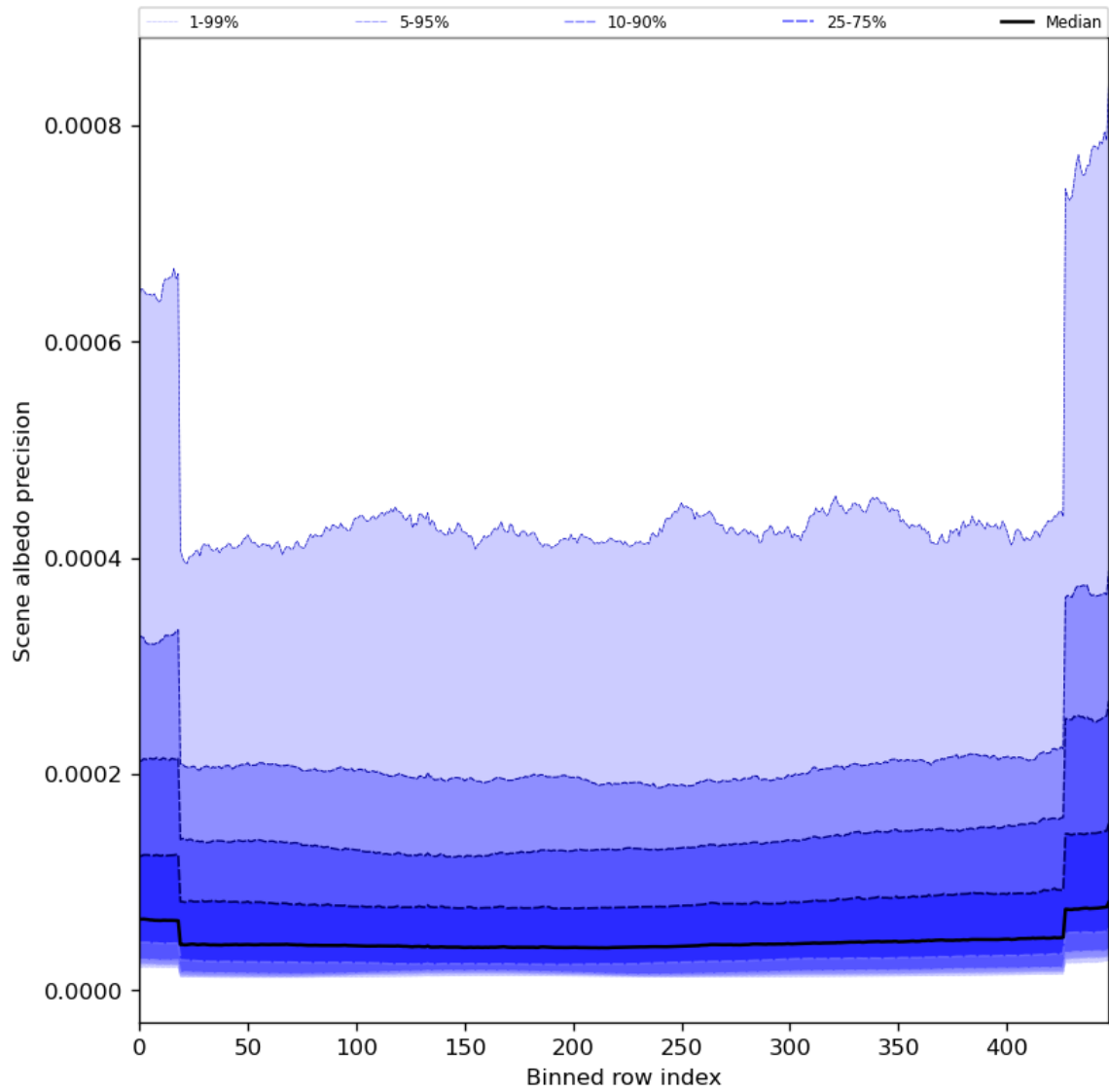
Figure 52: Along track statistics of “Scene albedo precision” for 2024-05-02 to 2024-05-04
