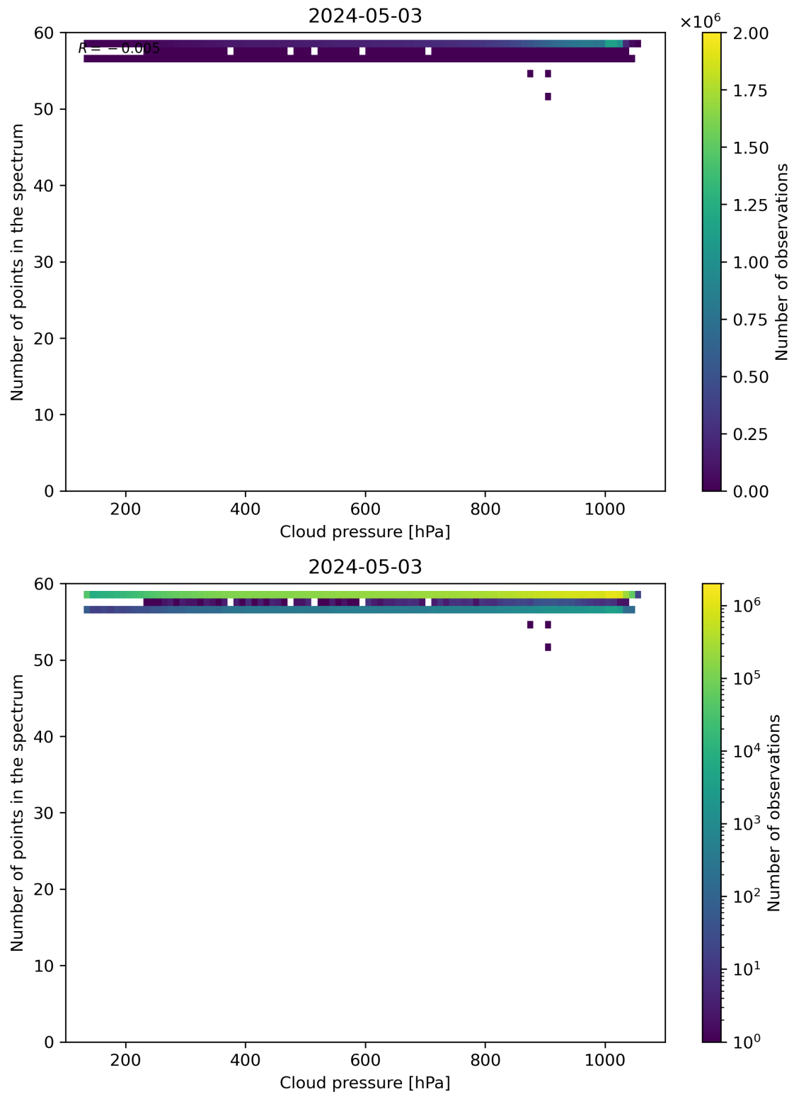
Figure 82: Scatter density plot of “Cloud pressure” against “Number of points in the spectrum” for 2024-05-02 to 2024-05-04.
