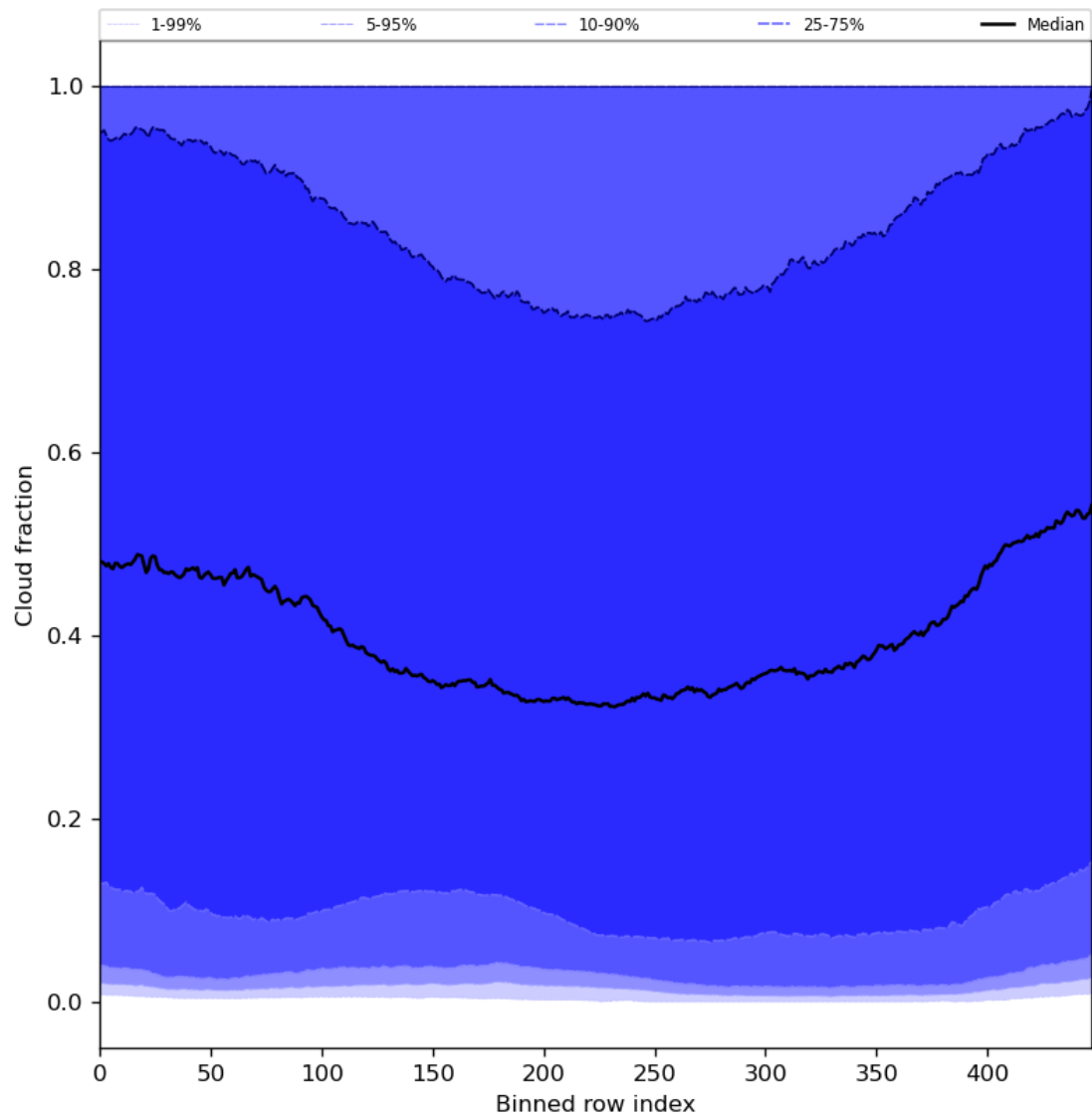
Figure 49: Along track statistics of “Cloud fraction” for 2024-05-02 to 2024-05-04
