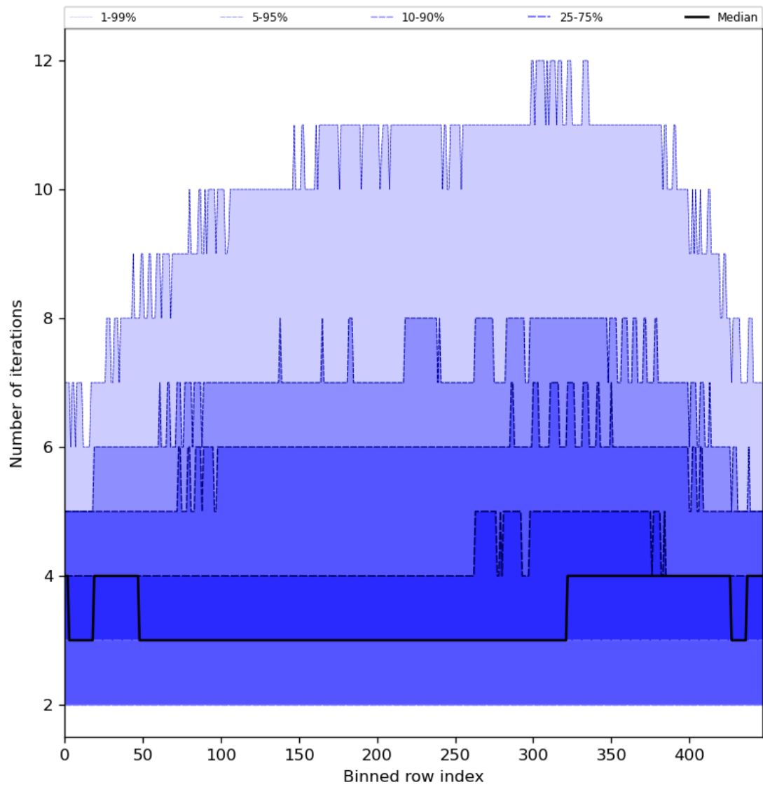
Figure 56: Along track statistics of “Number of iterations” for 2024-05-02 to 2024-05-04
