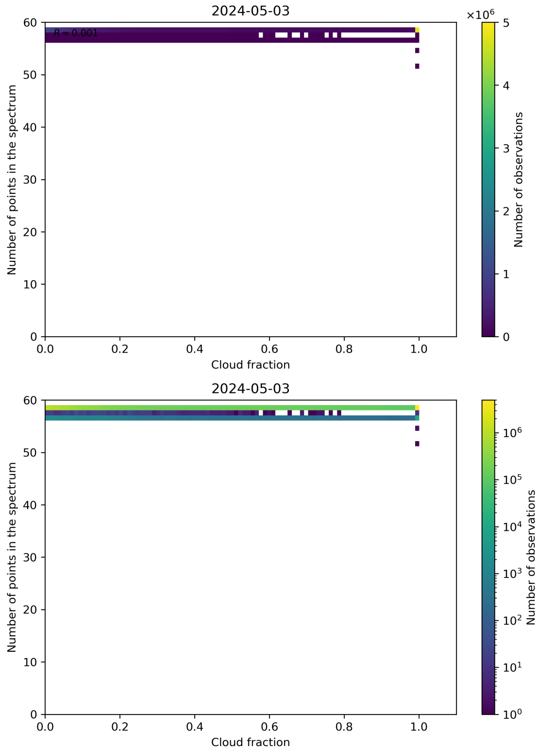
Figure 74: Scatter density plot of “Cloud fraction” against “Number of points in the spectrum” for 2024-05-02 to 2024-05-04.
