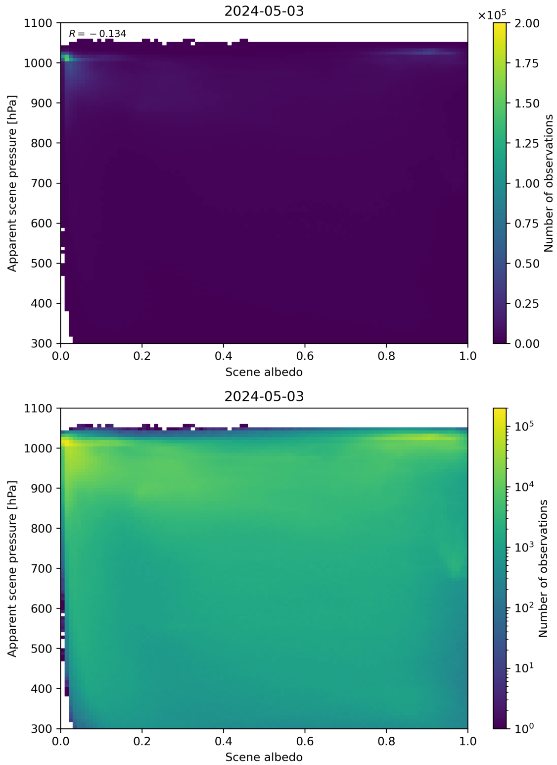
Figure 102: Scatter density plot of “Scene albedo” against “Apparent scene pressure” for 2024-05-02 to 2024-05-04.
