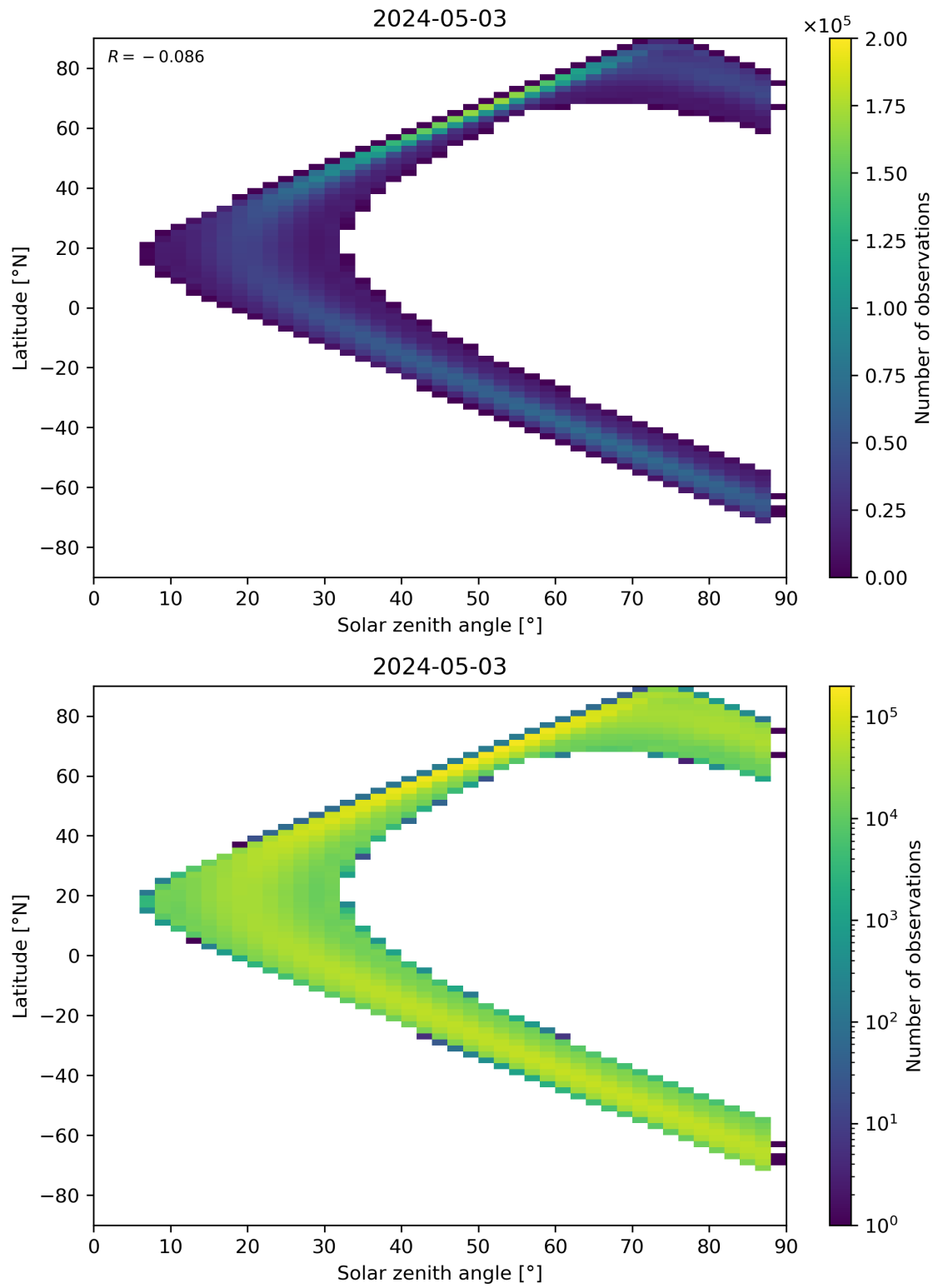
Figure 113: Scatter density plot of “Solar zenith angle” against “Latitude” for 2024-05-02 to 2024-05-04.
