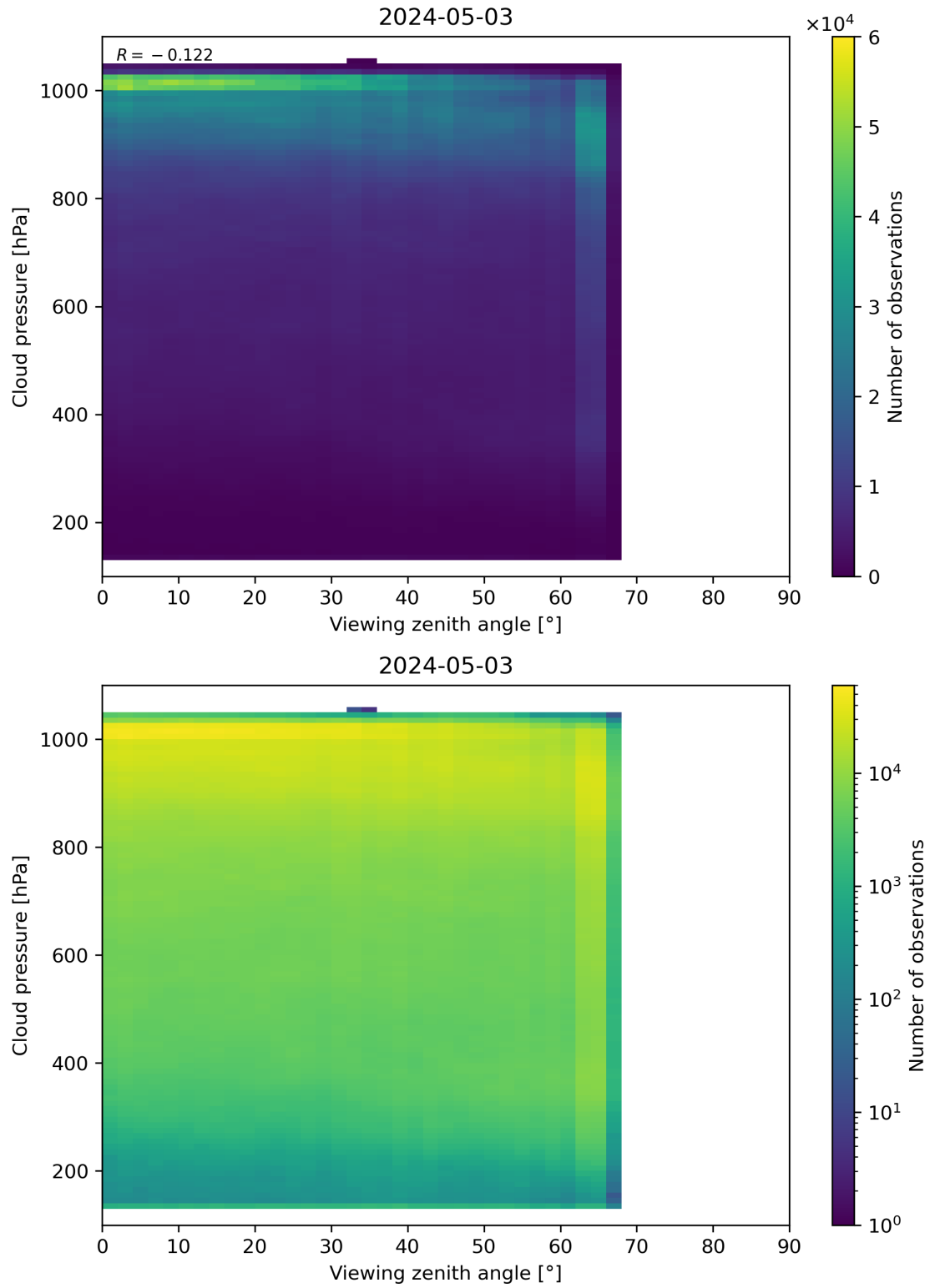
Figure 121: Scatter density plot of “Viewing zenith angle” against “Cloud pressure” for 2024-05-02 to 2024-05-04.
