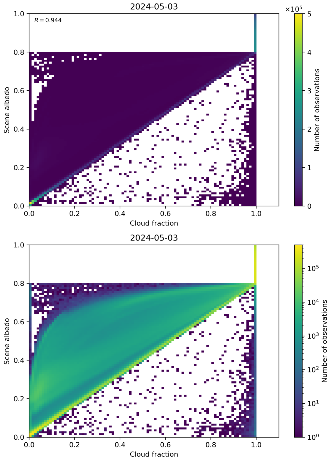
Figure 75: Scatter density plot of “Cloud fraction” against “Scene albedo” for 2024-05-02 to 2024-05-04.
