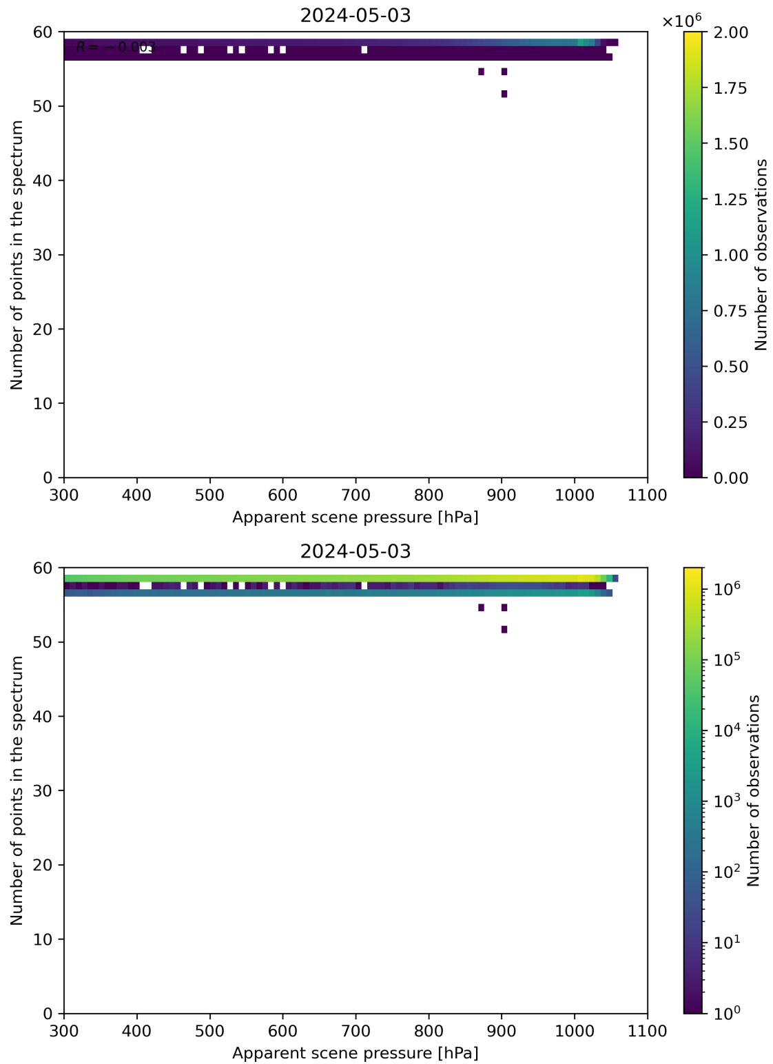
Figure 66: Scatter density plot of “Apparent scene pressure” against “Number of points in the spectrum” for 2024-05-02 to 2024-05-04.
