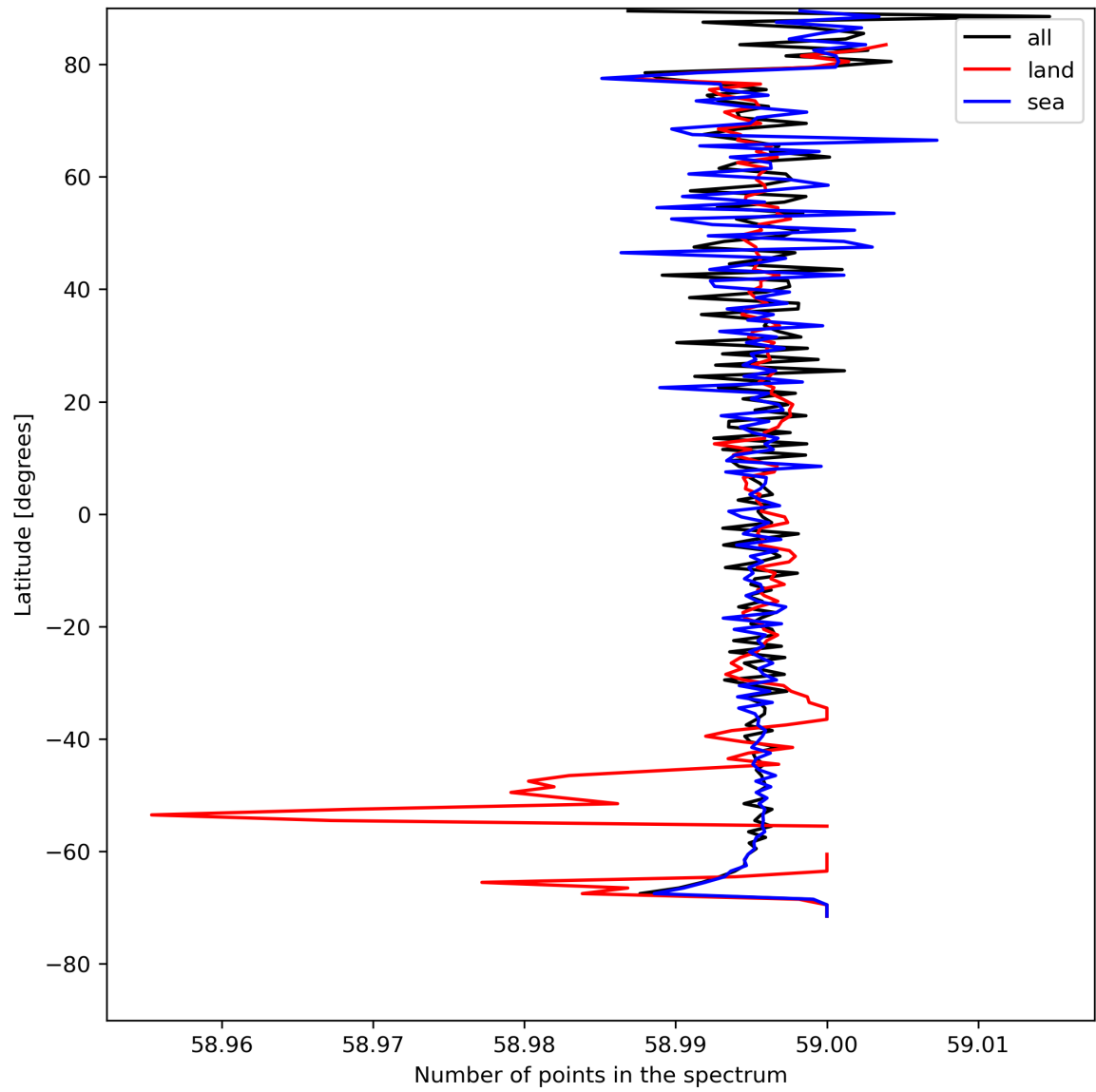
Figure 27: Zonal average of “Number of points in the spectrum” for 2024-05-02 to 2024-05-04.
