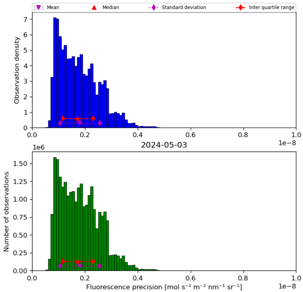
Figure 41: Histogram of “Fluorescence precision” for 2024-05-02 to 2024-05-04
