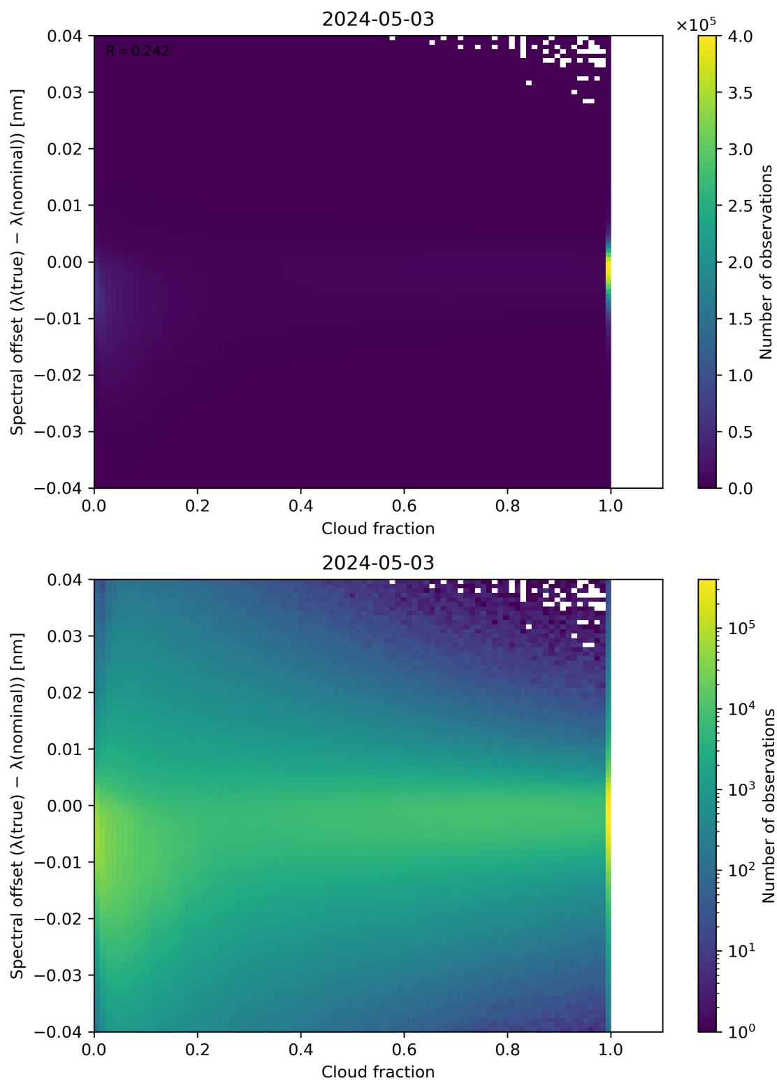
Figure 76: Scatter density plot of “Cloud fraction” against “Spectral offset ( \lambda(\text{true}) - \lambda(\text{nominal}) )” for 2024-05-02 to 2024-05-04.
