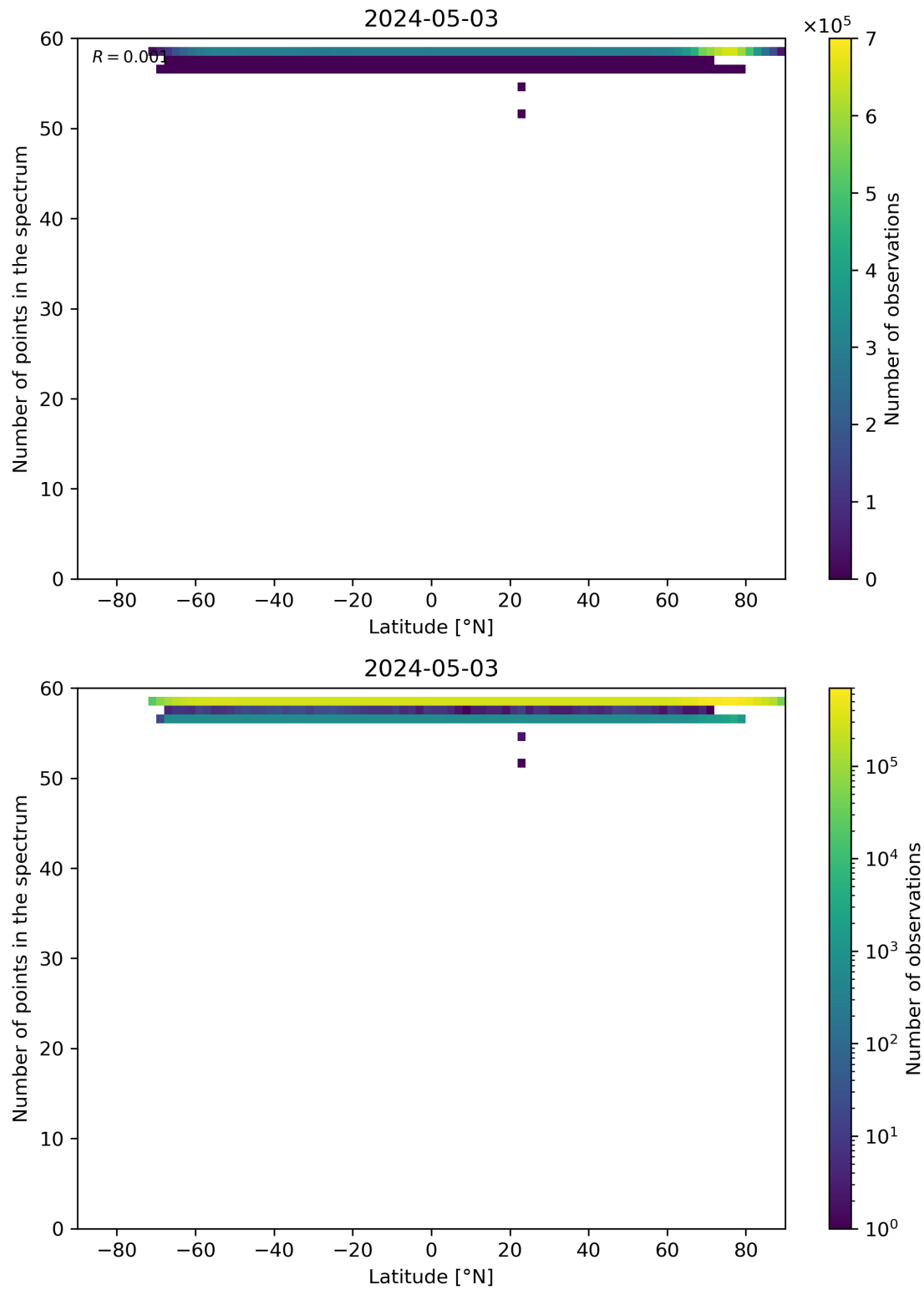
Figure 94: Scatter density plot of “Latitude” against “Number of points in the spectrum” for 2024-05-02 to 2024-05-04.
