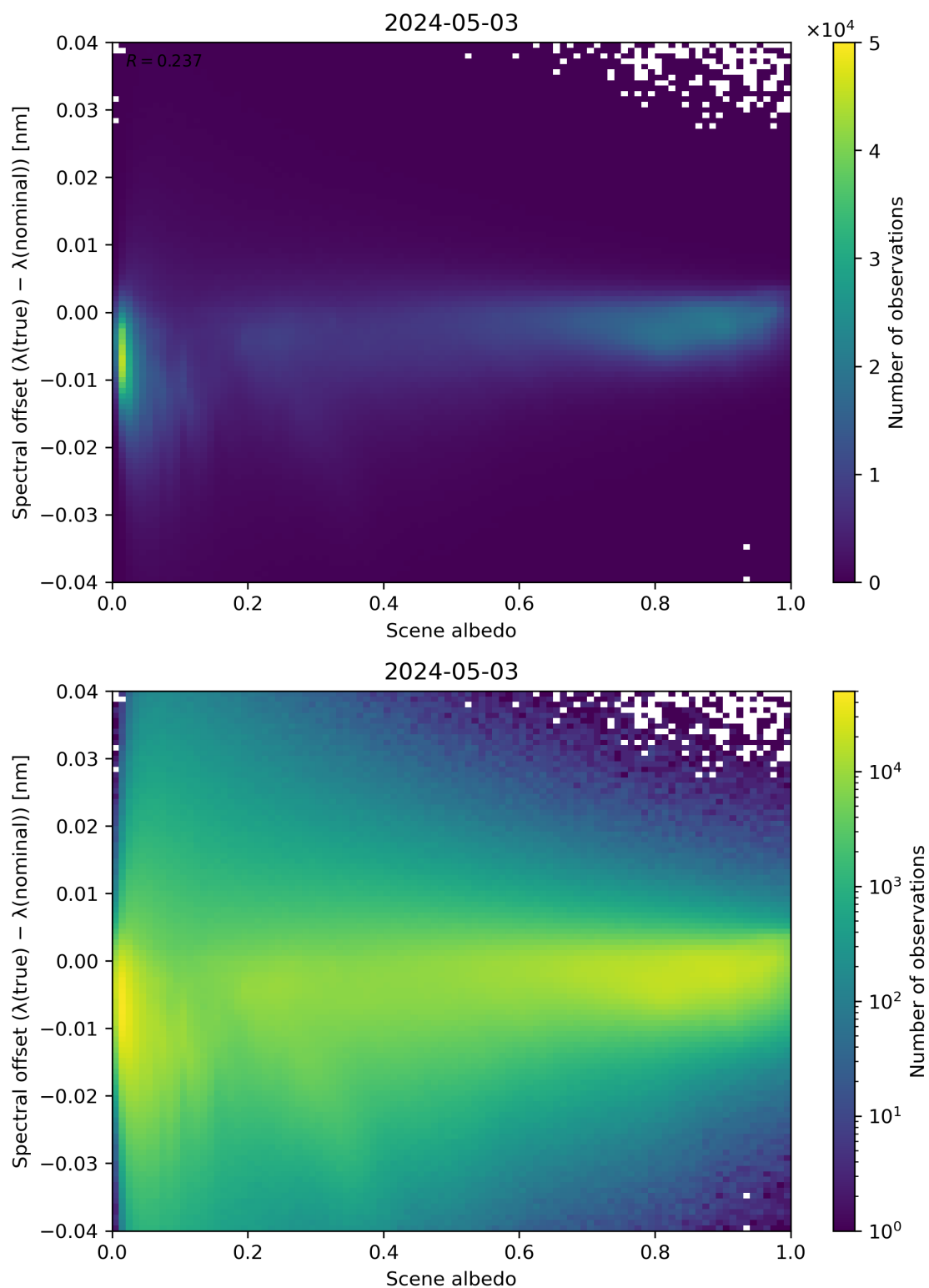
Figure 107: Scatter density plot of “Scene albedo” against “Spectral offset ( \lambda(\text{true}) - \lambda(\text{nominal}) )” for 2024-05-02 to 2024-05-04.
