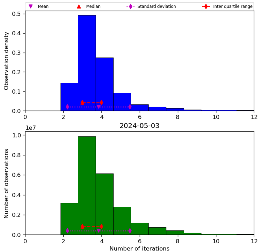
Figure 39: Histogram of “Number of iterations” for 2024-05-02 to 2024-05-04
