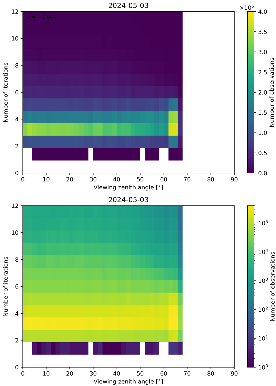
Figure 124: Scatter density plot of “Viewing zenith angle” against “Number of iterations” for 2024-05-02 to 2024-05-04.
