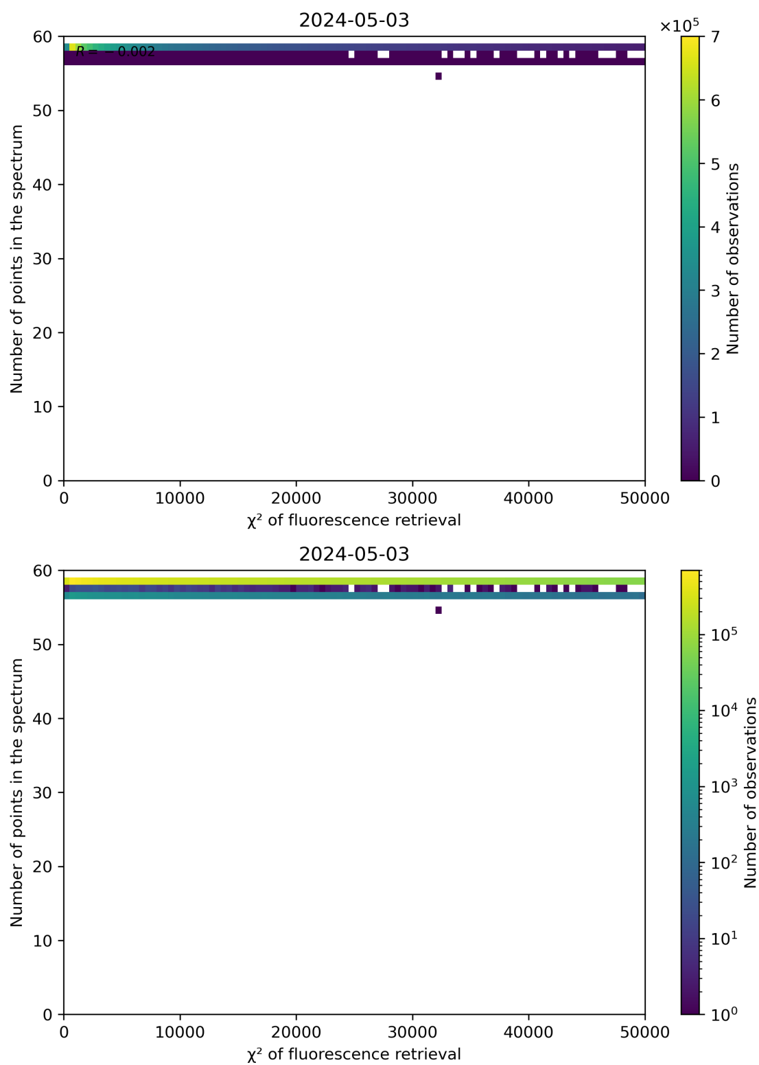
Figure 68: Scatter density plot of " \chi^2 of fluorescence retrieval" against "Number of points in the spectrum" for 2024-05-02 to 2024-05-04.
