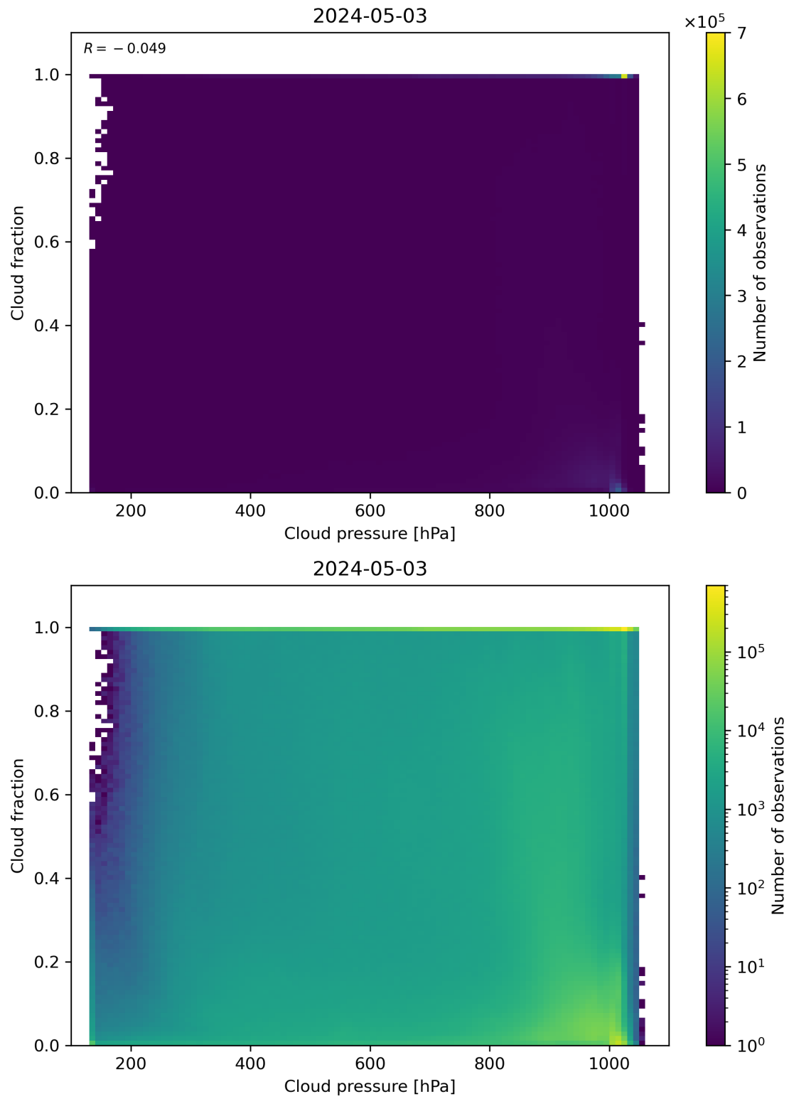
Figure 79: Scatter density plot of “Cloud pressure” against “Cloud fraction” for 2024-05-02 to 2024-05-04.
