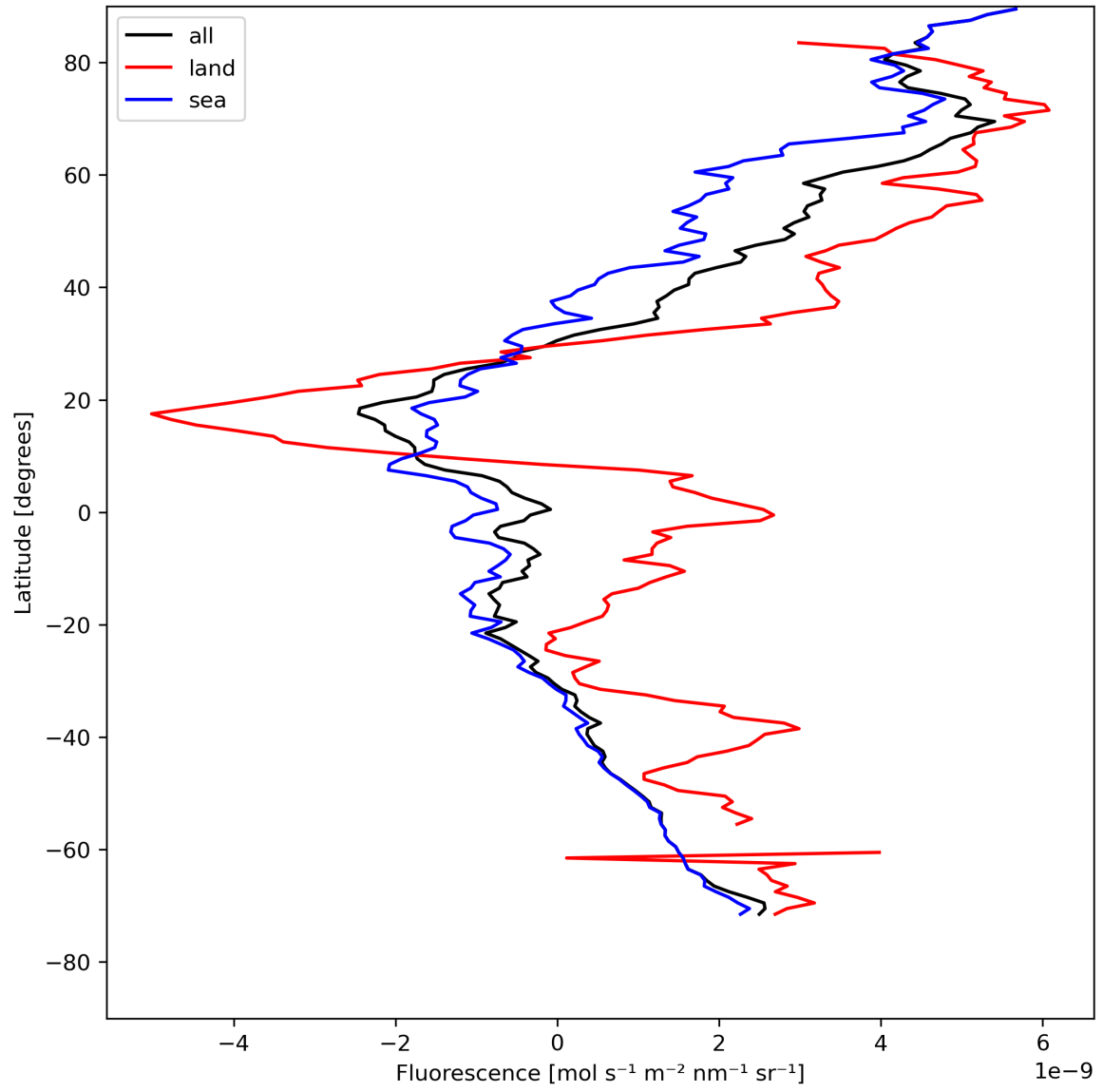
Figure 23: Zonal average of “Fluorescence” for 2024-05-02 to 2024-05-04.
