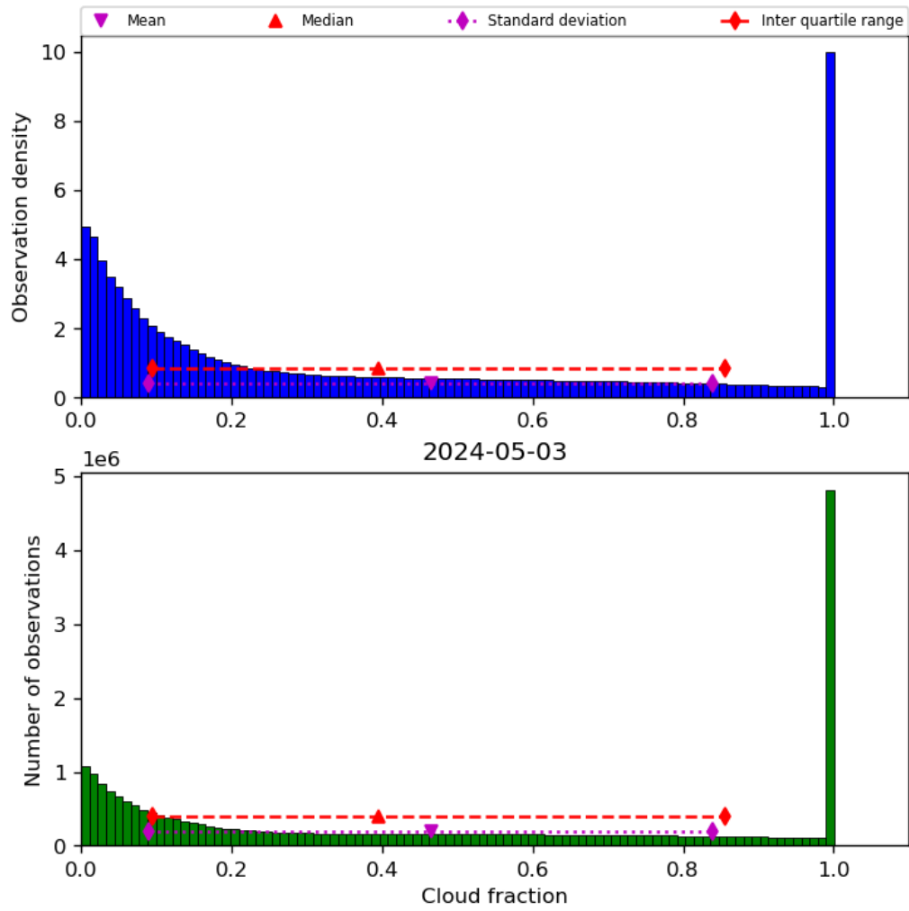
Figure 32: Histogram of “Cloud fraction” for 2024-05-02 to 2024-05-04
