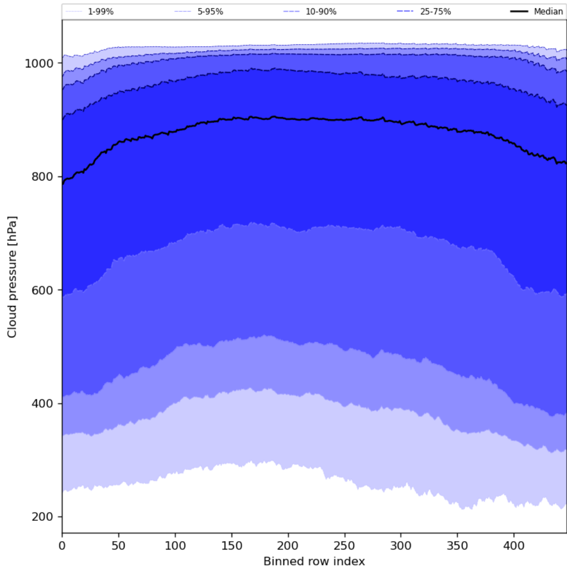
Figure 47: Along track statistics of “Cloud pressure” for 2024-05-02 to 2024-05-04
