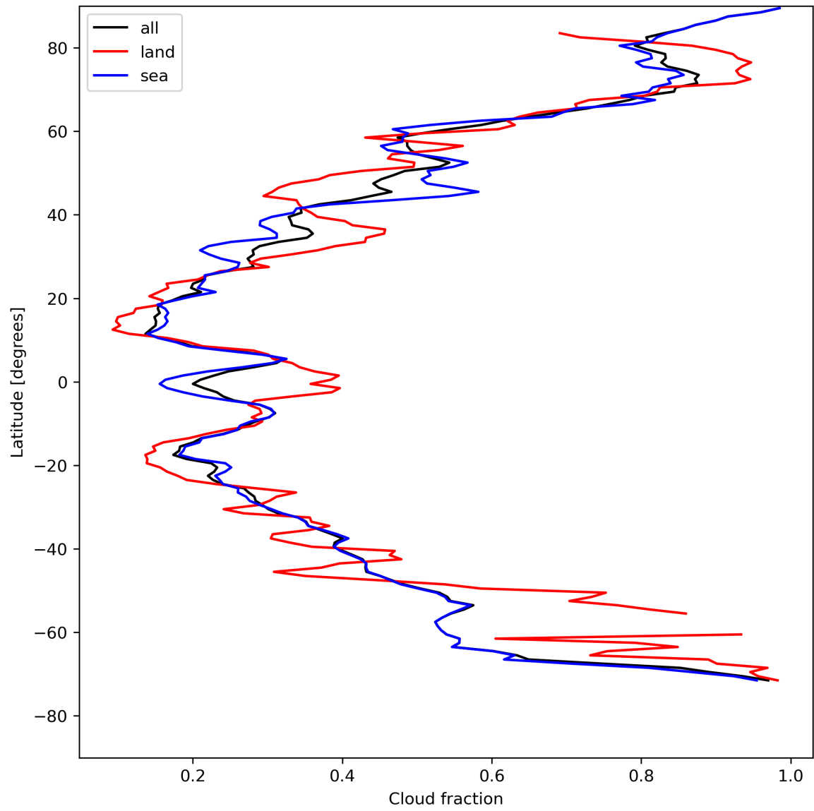
Figure 15: Zonal average of “Cloud fraction” for 2024-05-02 to 2024-05-04.
