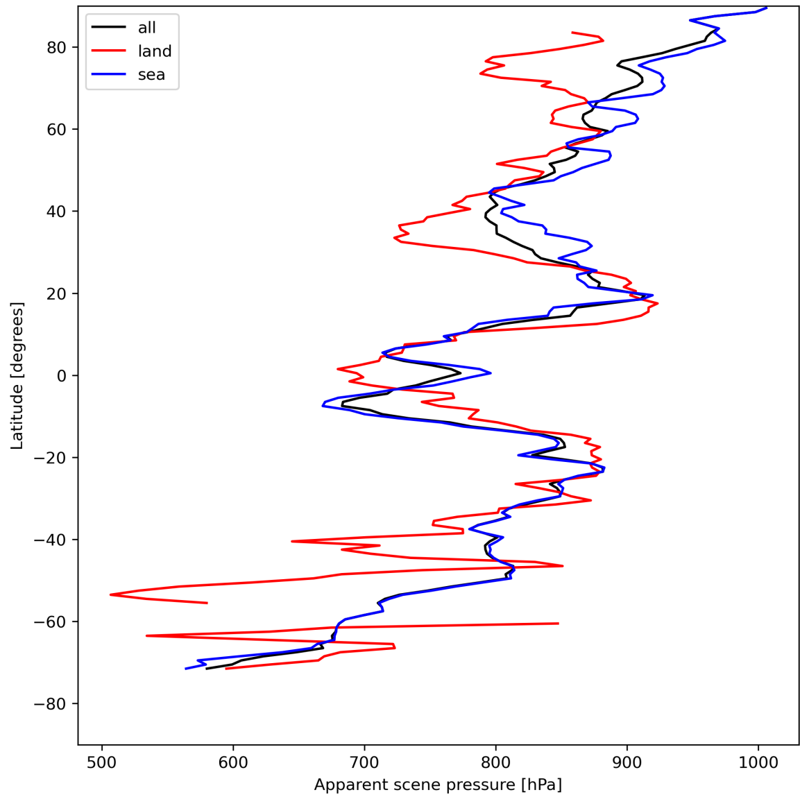
Figure 19: Zonal average of “Apparent scene pressure” for 2024-05-02 to 2024-05-04.
