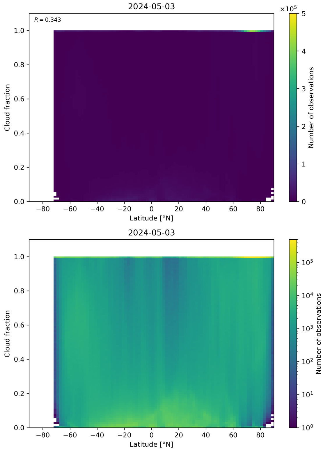
Figure 90: Scatter density plot of “Latitude” against “Cloud fraction” for 2024-05-02 to 2024-05-04.
