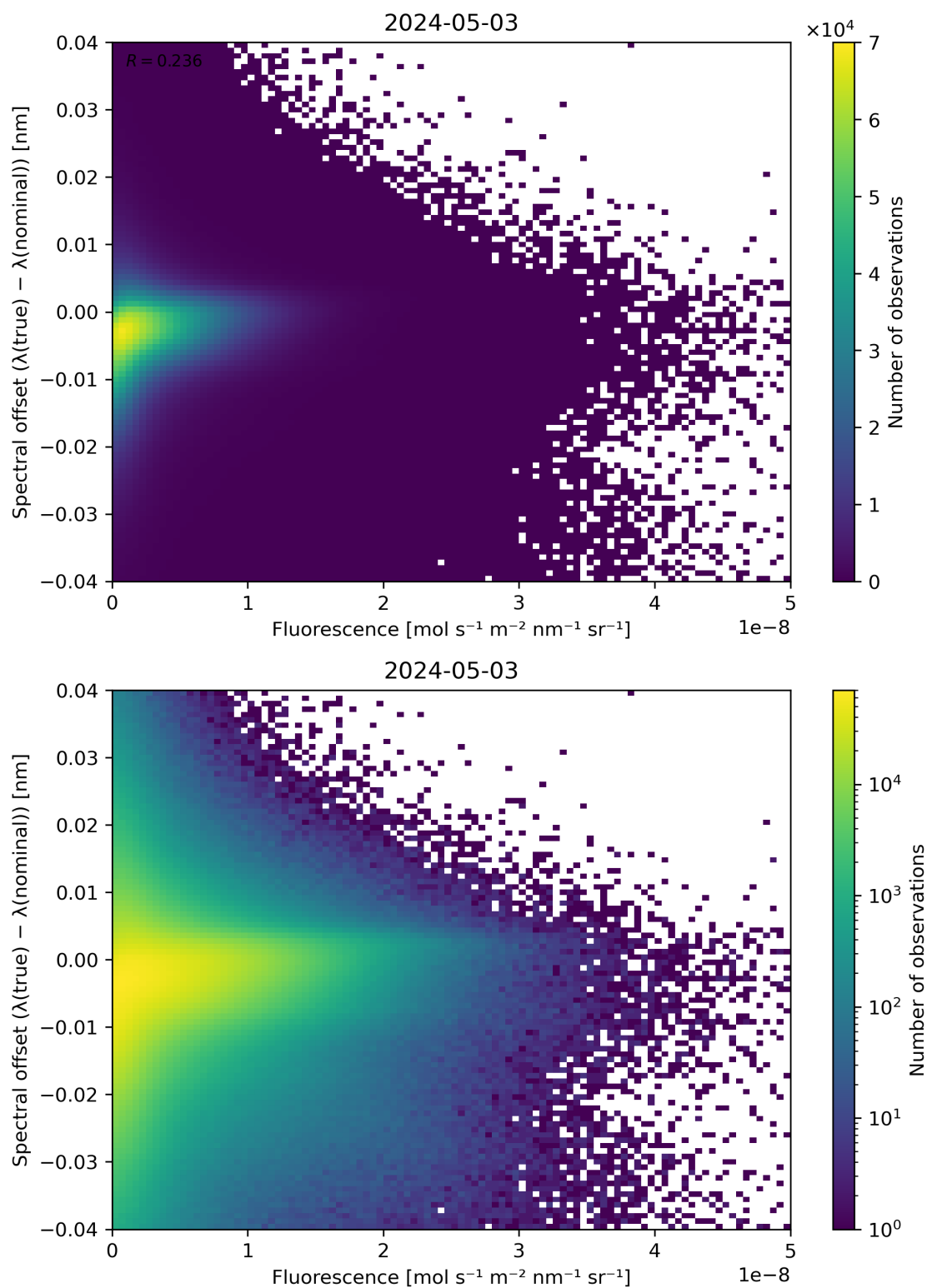
Figure 87: Scatter density plot of “Fluorescence” against “Spectral offset ( \lambda(\text{true}) - \lambda(\text{nominal}) )” for 2024-05-02 to 2024-05-04.
