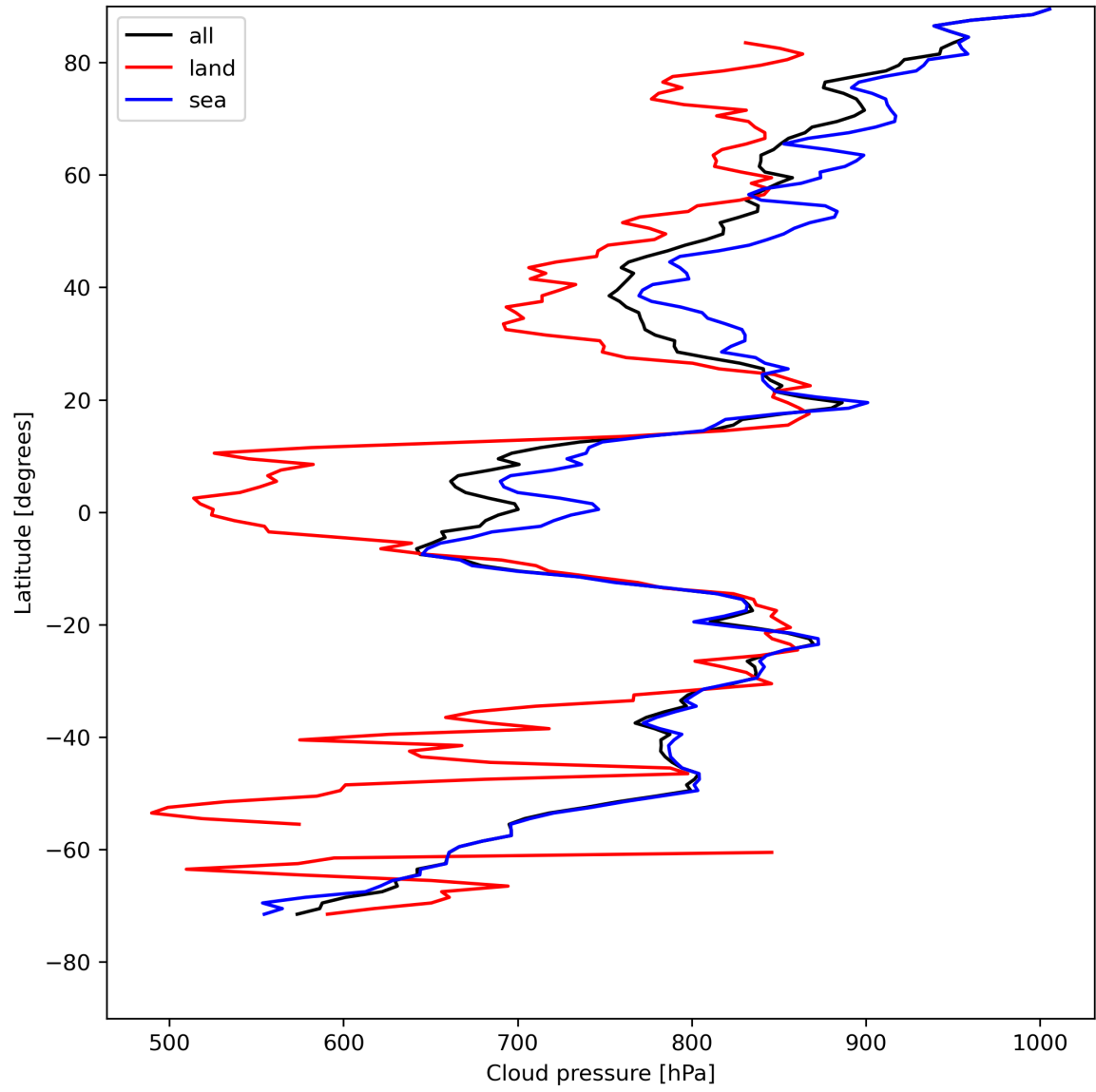
Figure 13: Zonal average of “Cloud pressure” for 2024-05-02 to 2024-05-04.
