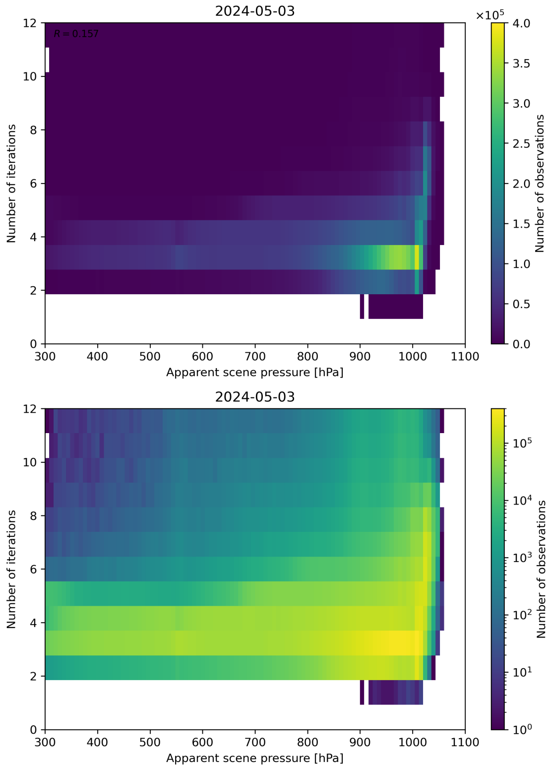
Figure 65: Scatter density plot of “Apparent scene pressure” against “Number of iterations” for 2024-05-02 to 2024-05-04.
