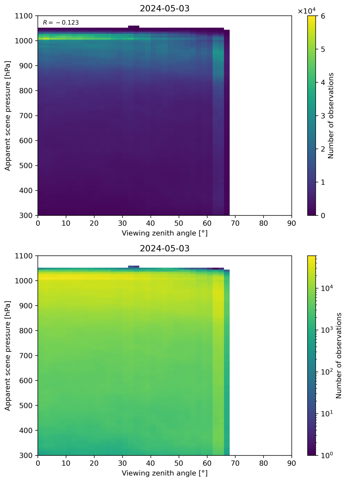
Figure 118: Scatter density plot of “Viewing zenith angle” against “Apparent scene pressure” for 2024-05-02 to 2024-05-04.
