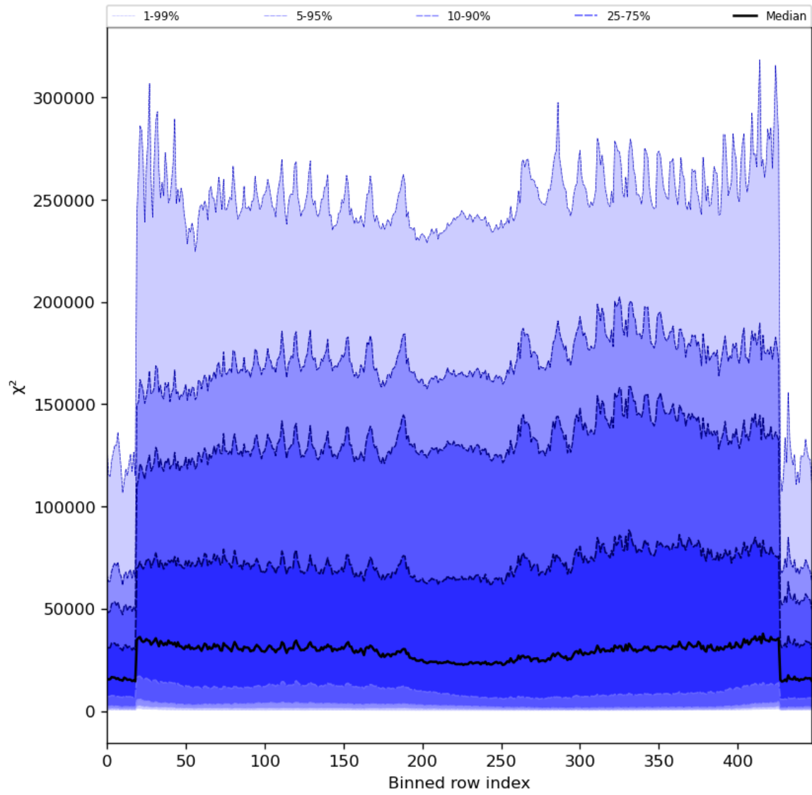
Figure 55: Along track statistics of “ \chi^2 ” for 2024-05-02 to 2024-05-04
