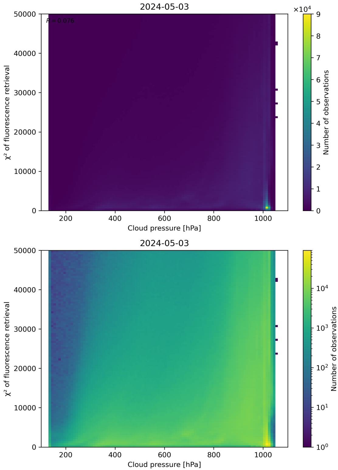
Figure 78: Scatter density plot of “Cloud pressure” against “ \chi^2 of fluorescence retrieval” for 2024-05-02 to 2024-05-04.
