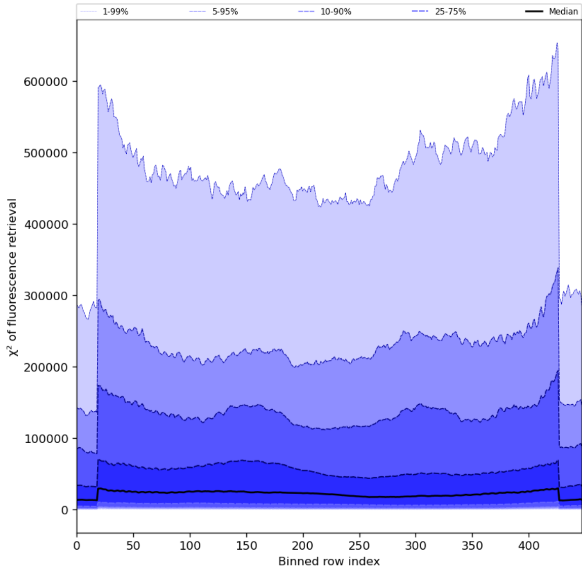
Figure 59: Along track statistics of “ \chi^2 of fluorescence retrieval” for 2024-05-02 to 2024-05-04
