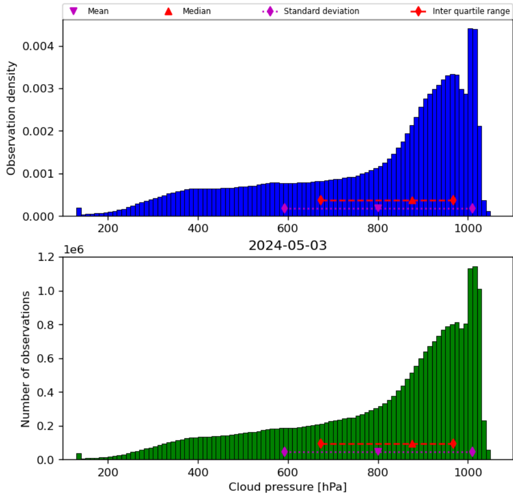
Figure 30: Histogram of “Cloud pressure” for 2024-05-02 to 2024-05-04
