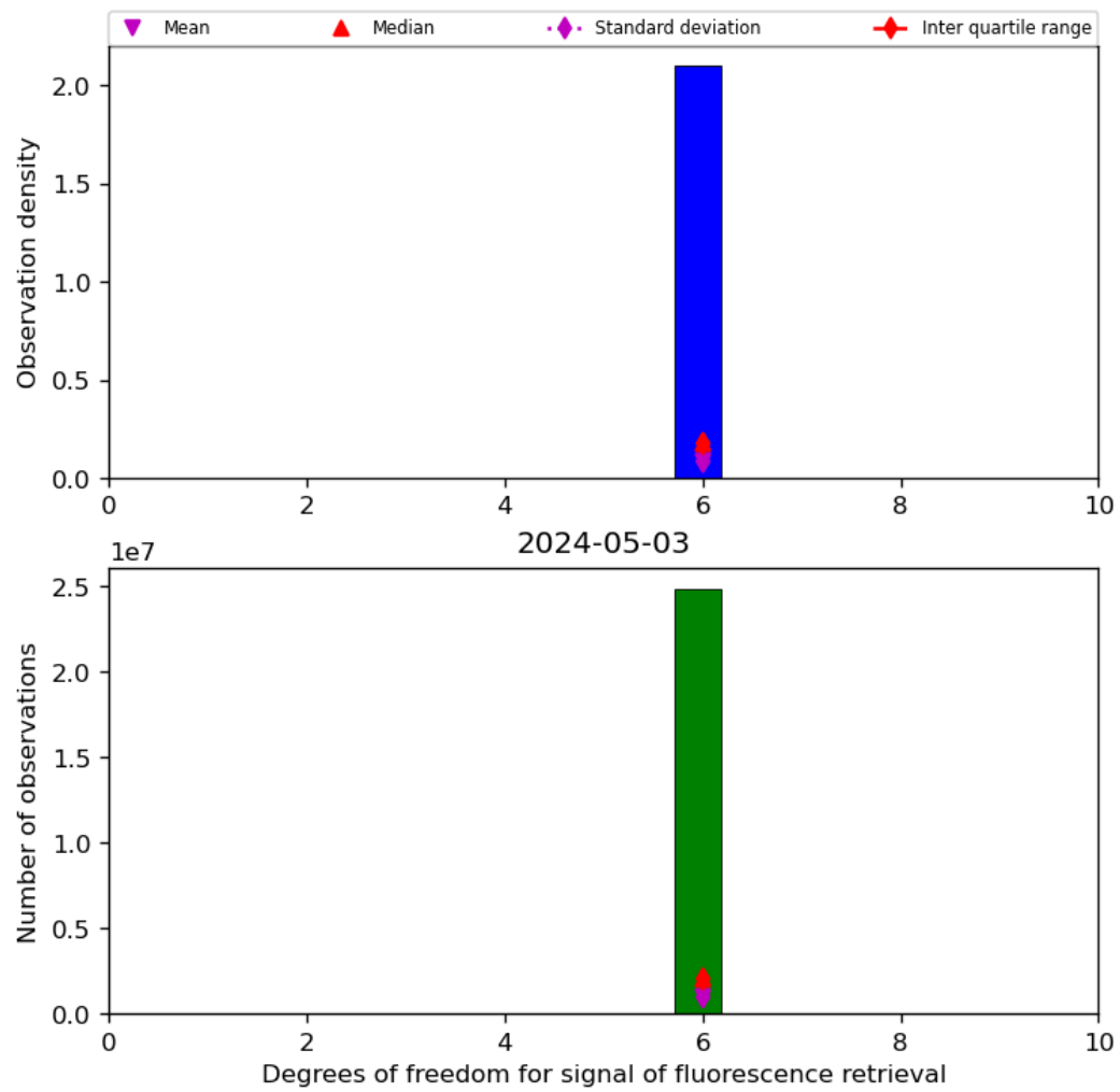
Figure 43: Histogram of “Degrees of freedom for signal of fluorescence retrieval” for 2024-05-02 to 2024-05-04
