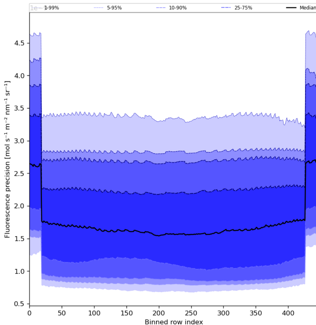
Figure 58: Along track statistics of “Fluorescence precision” for 2024-05-02 to 2024-05-04
