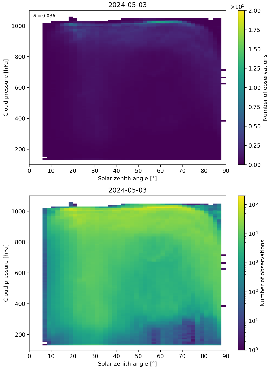
Figure 111: Scatter density plot of “Solar zenith angle” against “Cloud pressure” for 2024-05-02 to 2024-05-04.
