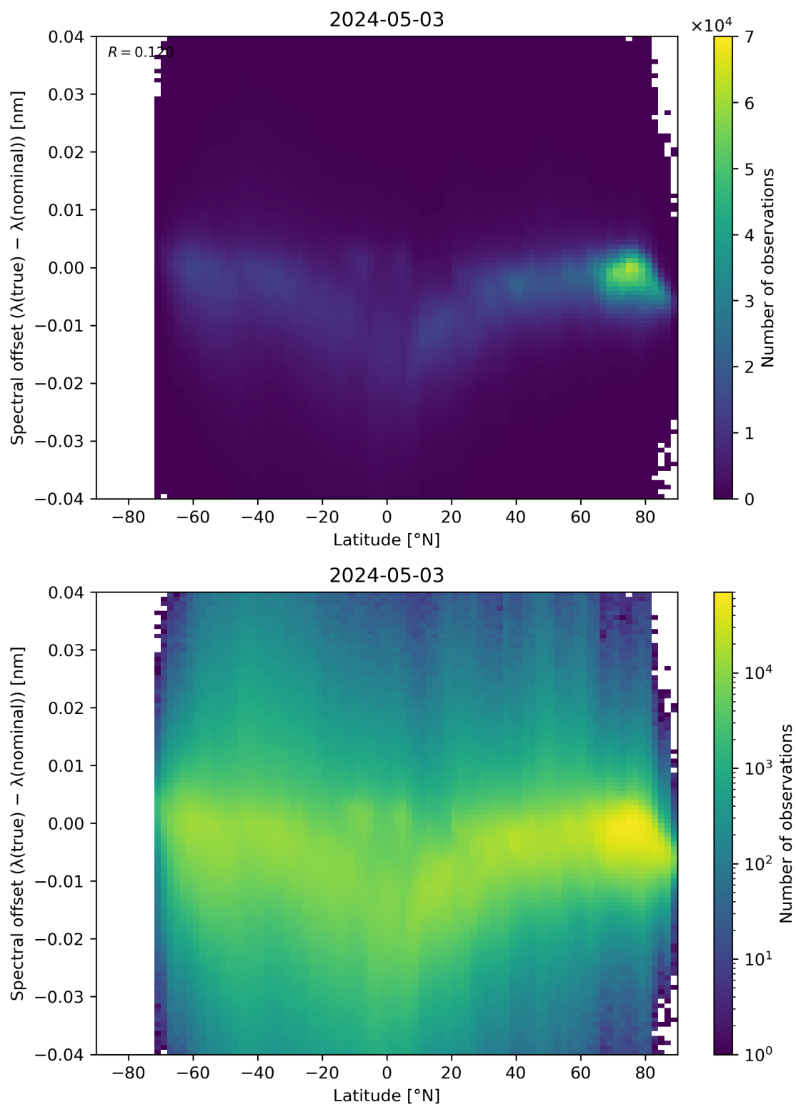
Figure 96: Scatter density plot of “Latitude” against “Spectral offset ( \lambda(\text{true}) - \lambda(\text{nominal}) )” for 2024-05-02 to 2024-05-04.
