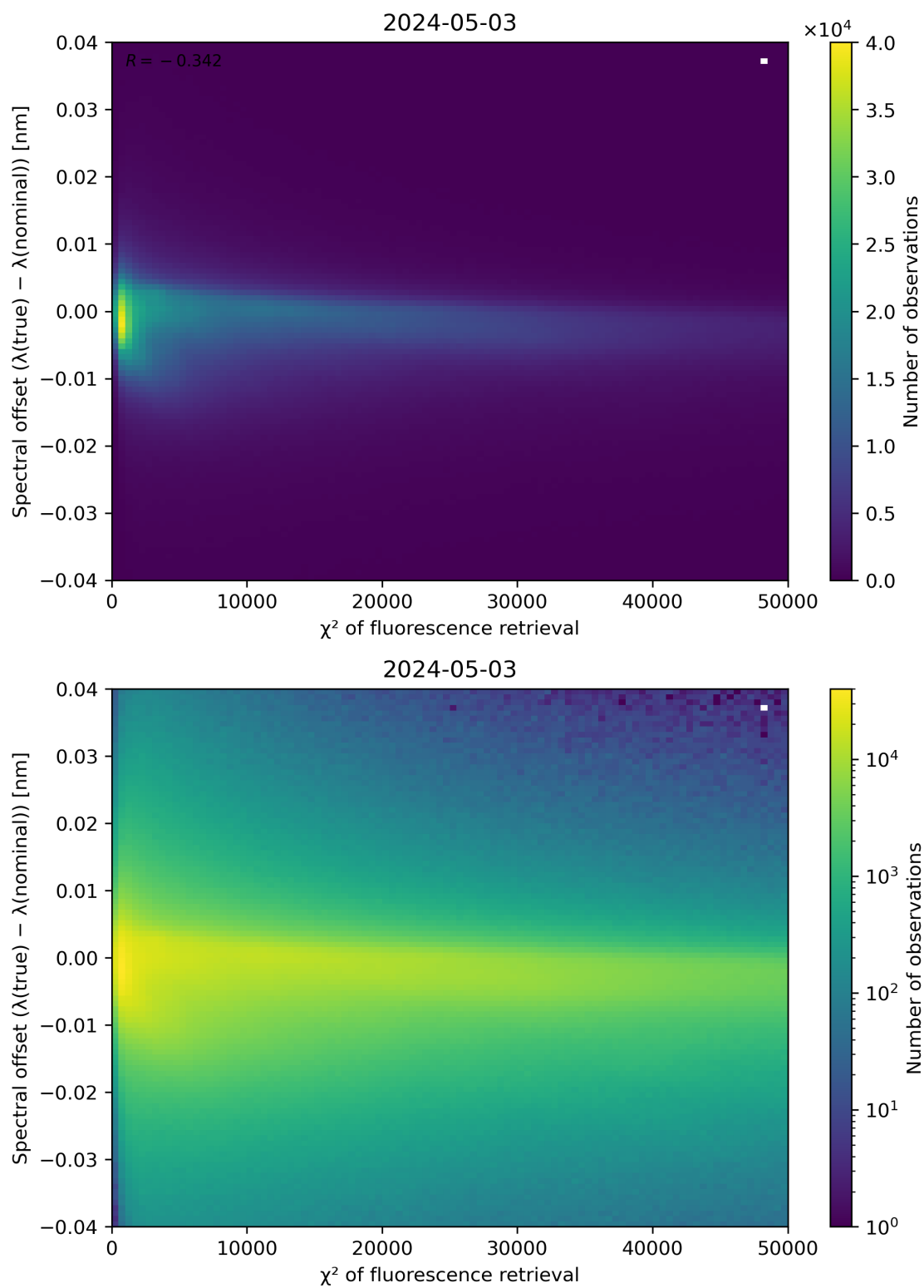
Figure 69: Scatter density plot of " \chi^2 of fluorescence retrieval" against "Spectral offset ( \lambda(\text{true}) - \lambda(\text{nominal})) " for 2024-05-02 to 2024-05-04.
