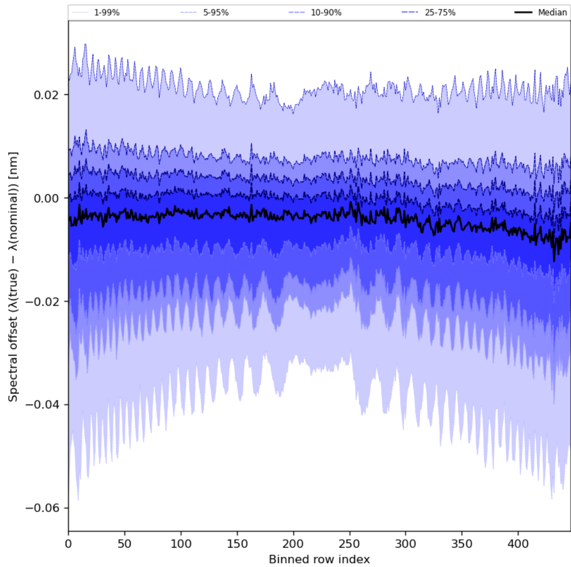
Figure 62: Along track statistics of “Spectral offset ( \lambda(\text{true}) - \lambda(\text{nominal}) )” for 2024-05-02 to 2024-05-04
