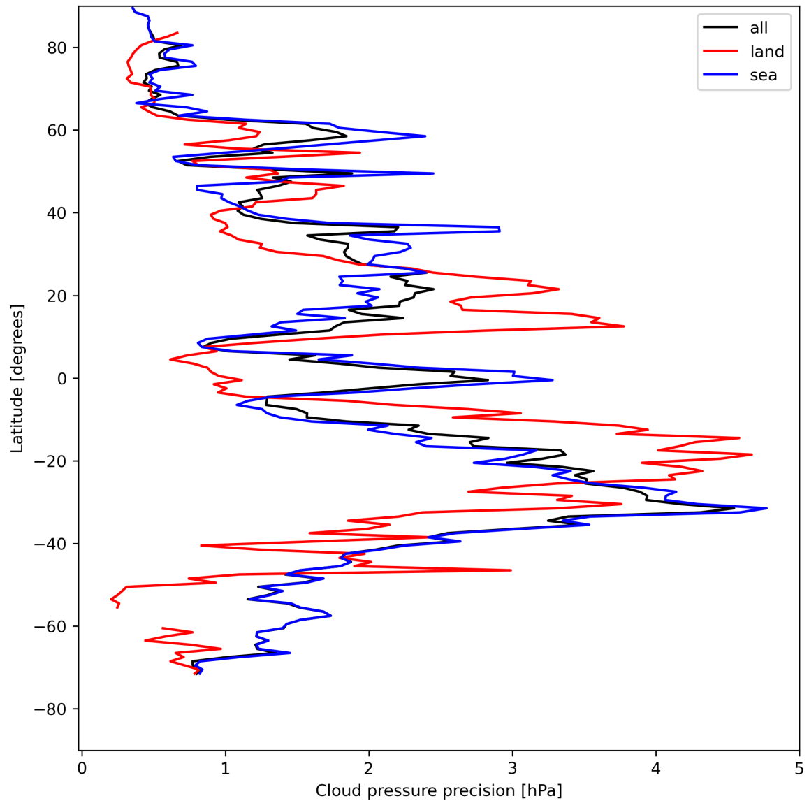
Figure 14: Zonal average of “Cloud pressure precision” for 2024-05-02 to 2024-05-04.
