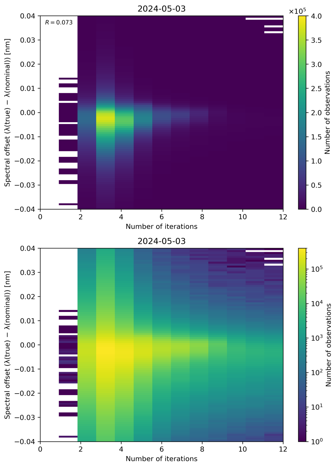
Figure 100: Scatter density plot of “Number of iterations” against “Spectral offset ( \lambda(\text{true}) - \lambda(\text{nominal}) )” for 2024-05-02 to 2024-05-04.
