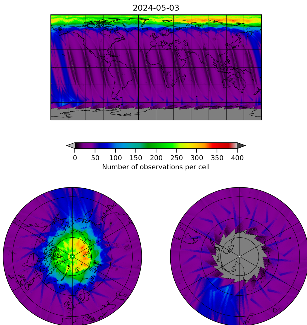
Figure 11: Map of the number of observations for 2024-05-02 to 2024-05-04
