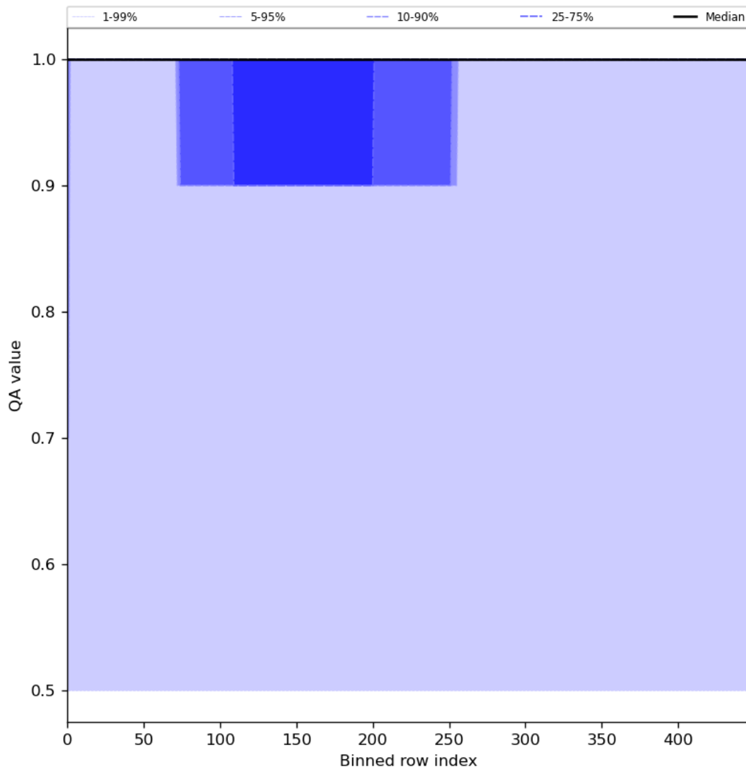
Figure 46: Along track statistics of “QA value” for 2024-05-02 to 2024-05-04
