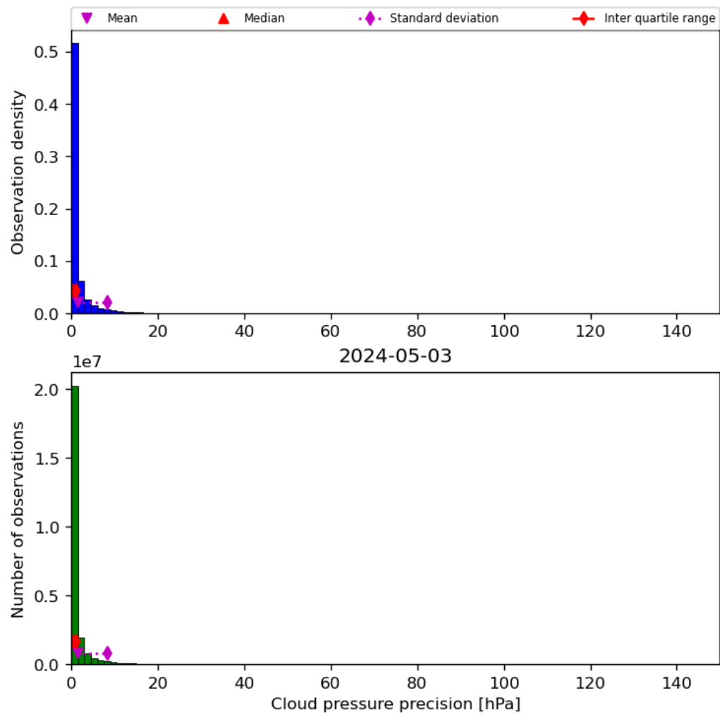
Figure 31: Histogram of “Cloud pressure precision” for 2024-05-02 to 2024-05-04
