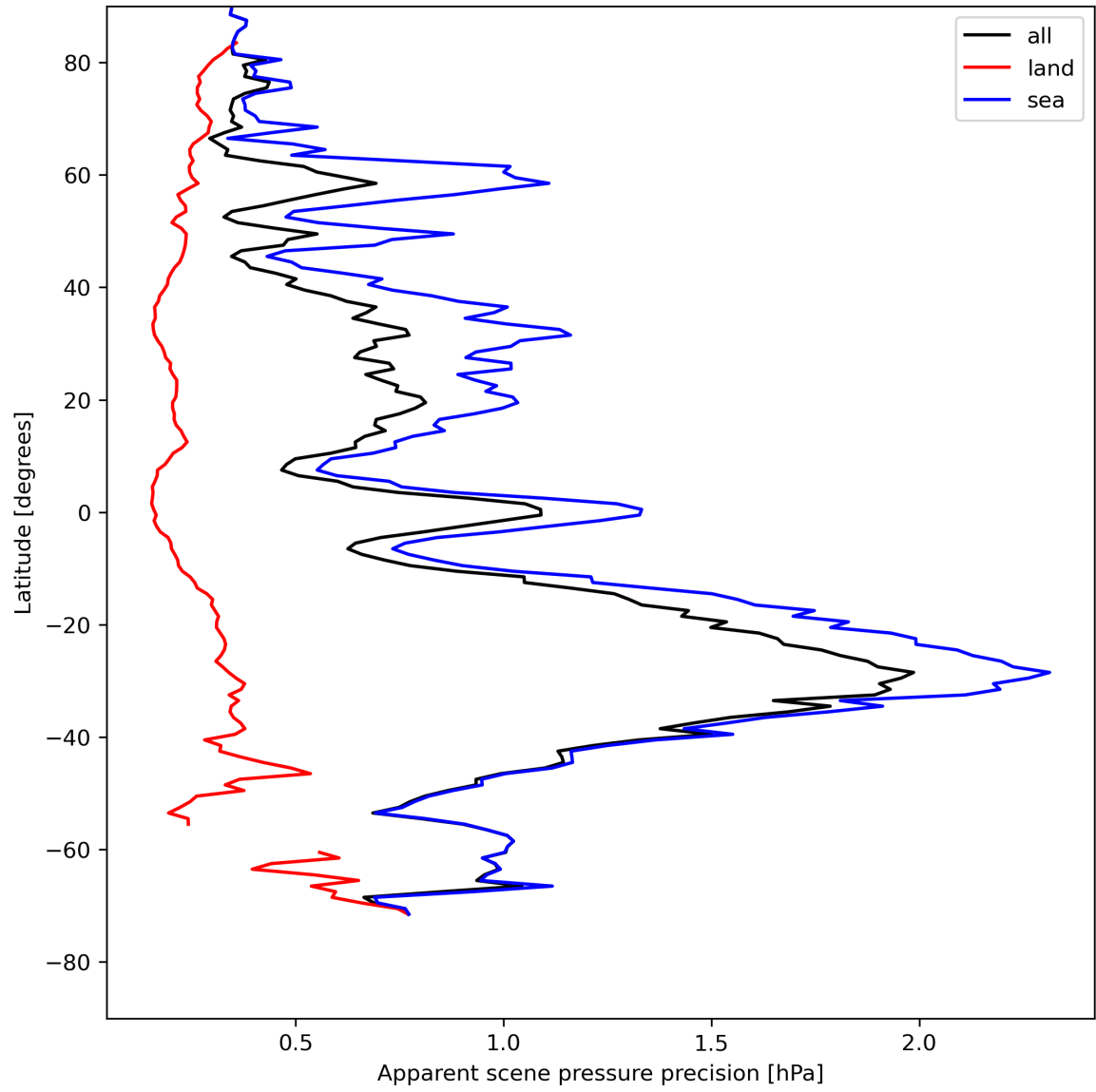
Figure 20: Zonal average of “Apparent scene pressure precision” for 2024-05-02 to 2024-05-04.
