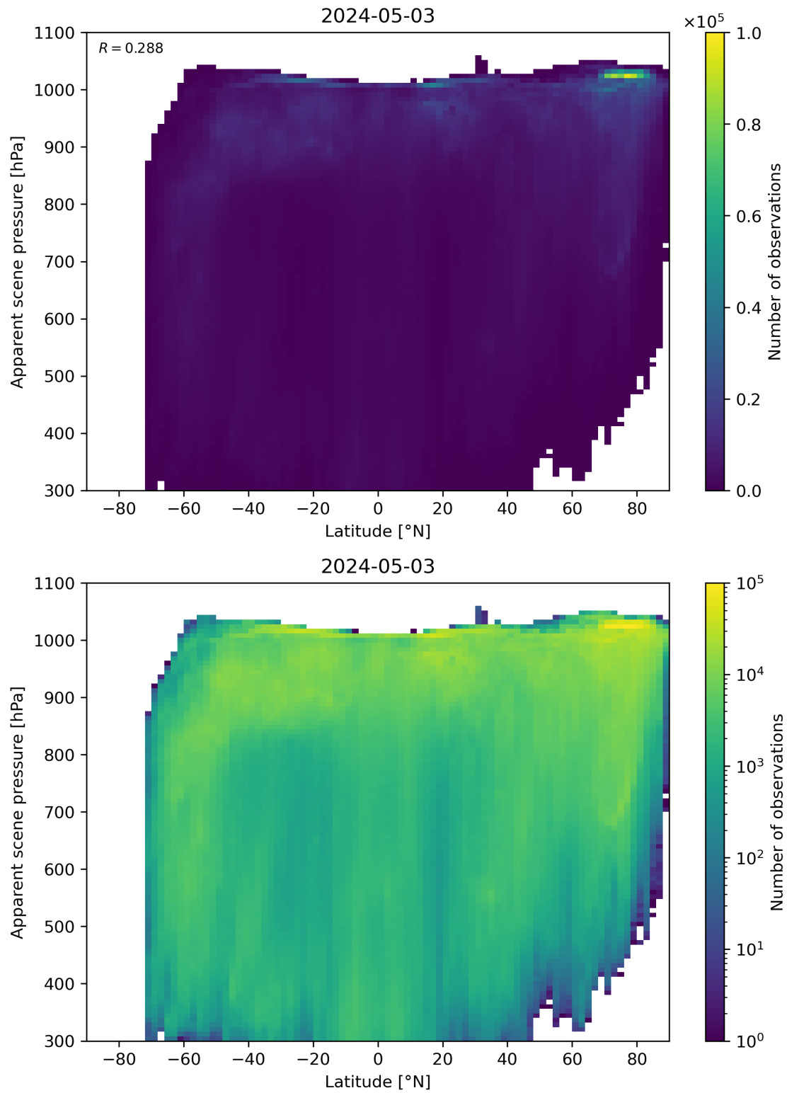
Figure 88: Scatter density plot of “Latitude” against “Apparent scene pressure” for 2024-05-02 to 2024-05-04.
