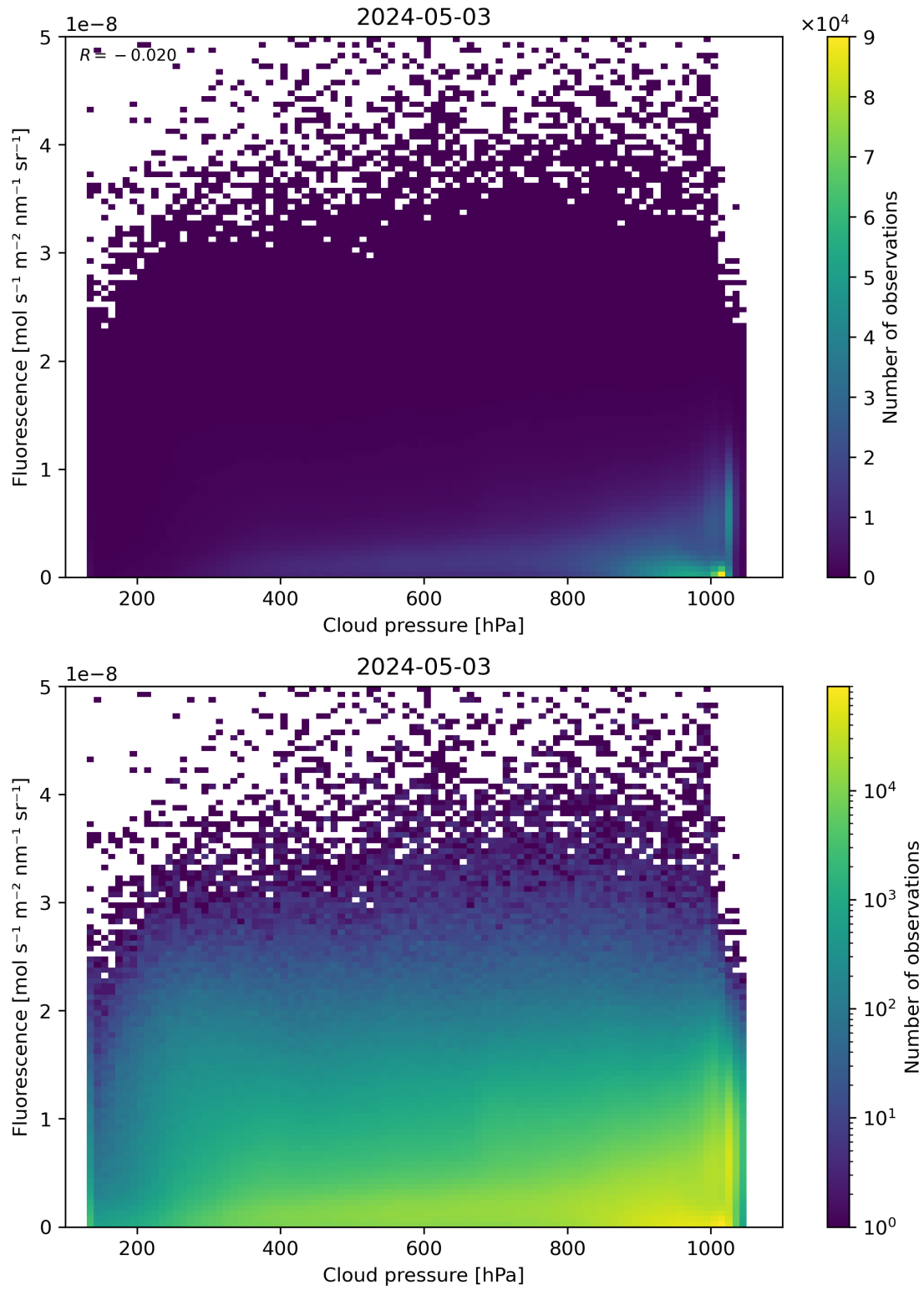
Figure 80: Scatter density plot of “Cloud pressure” against “Fluorescence” for 2024-05-02 to 2024-05-04.
