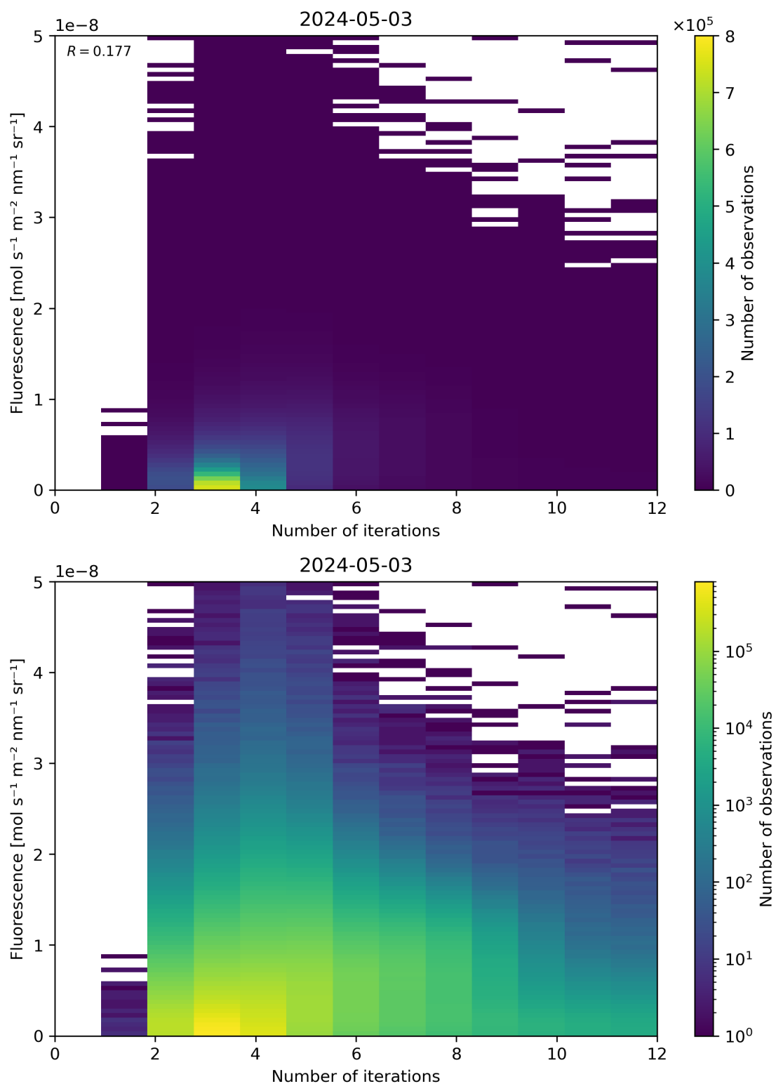
Figure 98: Scatter density plot of “Number of iterations” against “Fluorescence” for 2024-05-02 to 2024-05-04.
