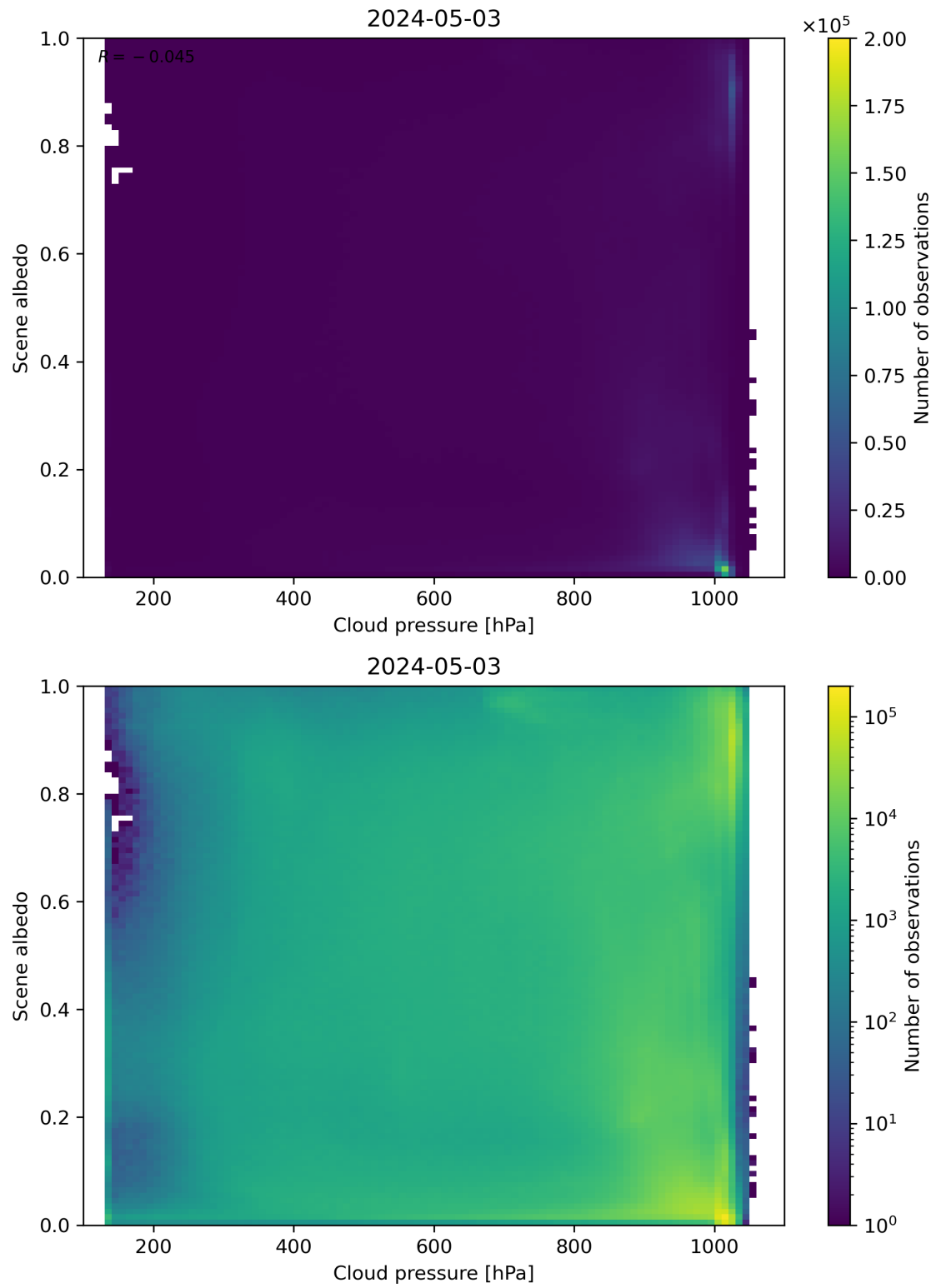
Figure 83: Scatter density plot of “Cloud pressure” against “Scene albedo” for 2024-05-02 to 2024-05-04.
