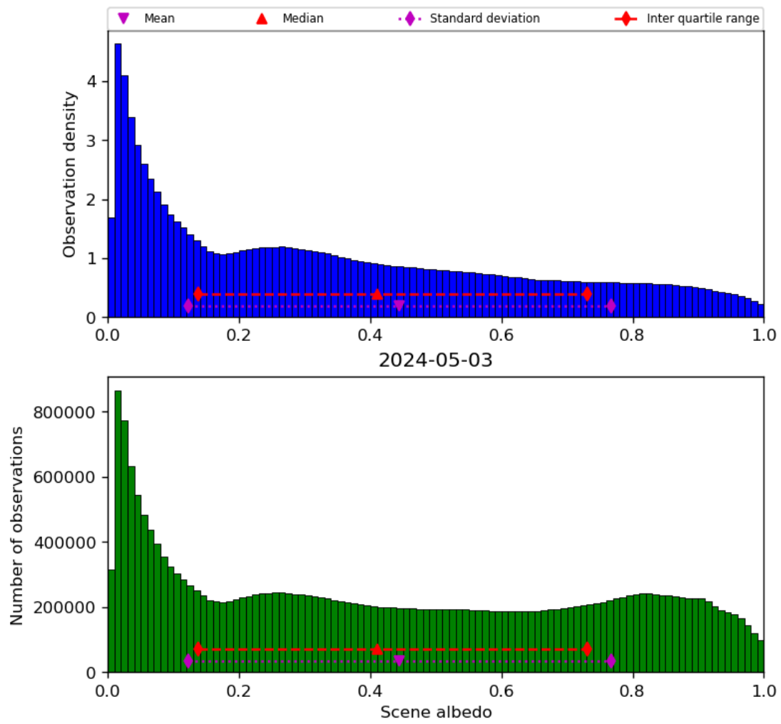
Figure 34: Histogram of “Scene albedo” for 2024-05-02 to 2024-05-04
