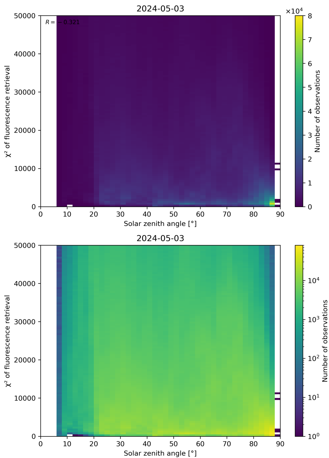
Figure 109: Scatter density plot of “Solar zenith angle” against “ \chi^2 of fluorescence retrieval” for 2024-05-02 to 2024-05-04.
