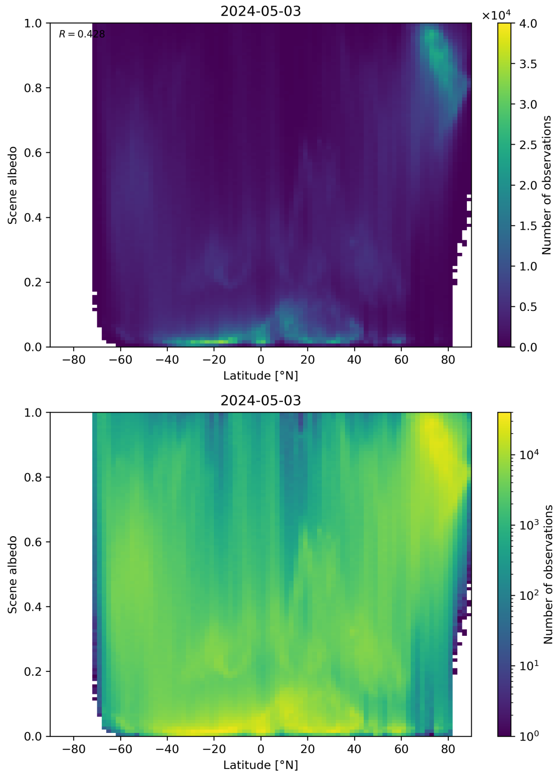
Figure 95: Scatter density plot of “Latitude” against “Scene albedo” for 2024-05-02 to 2024-05-04.
