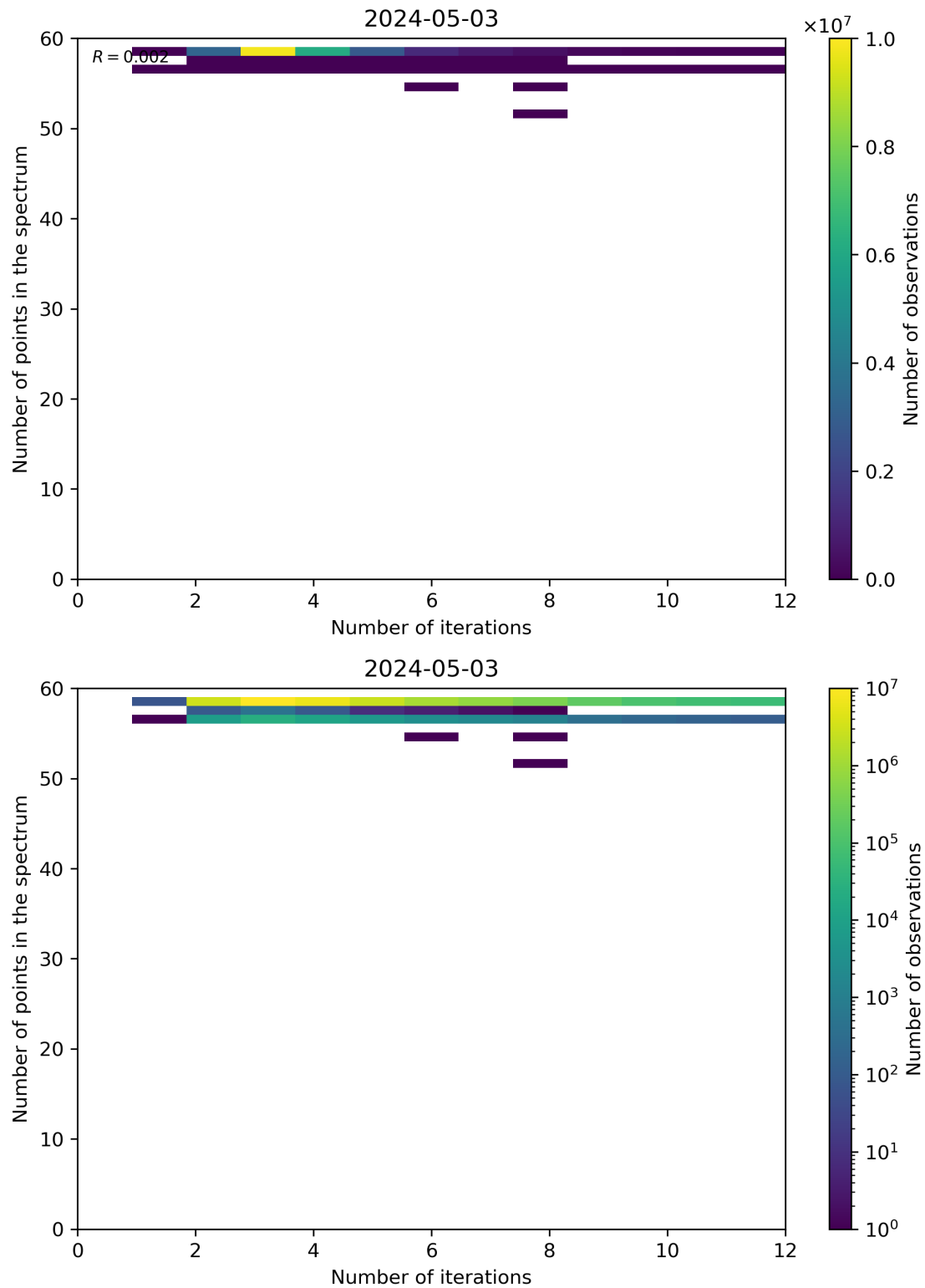
Figure 99: Scatter density plot of “Number of iterations” against “Number of points in the spectrum” for 2024-05-02 to 2024-05-04.
