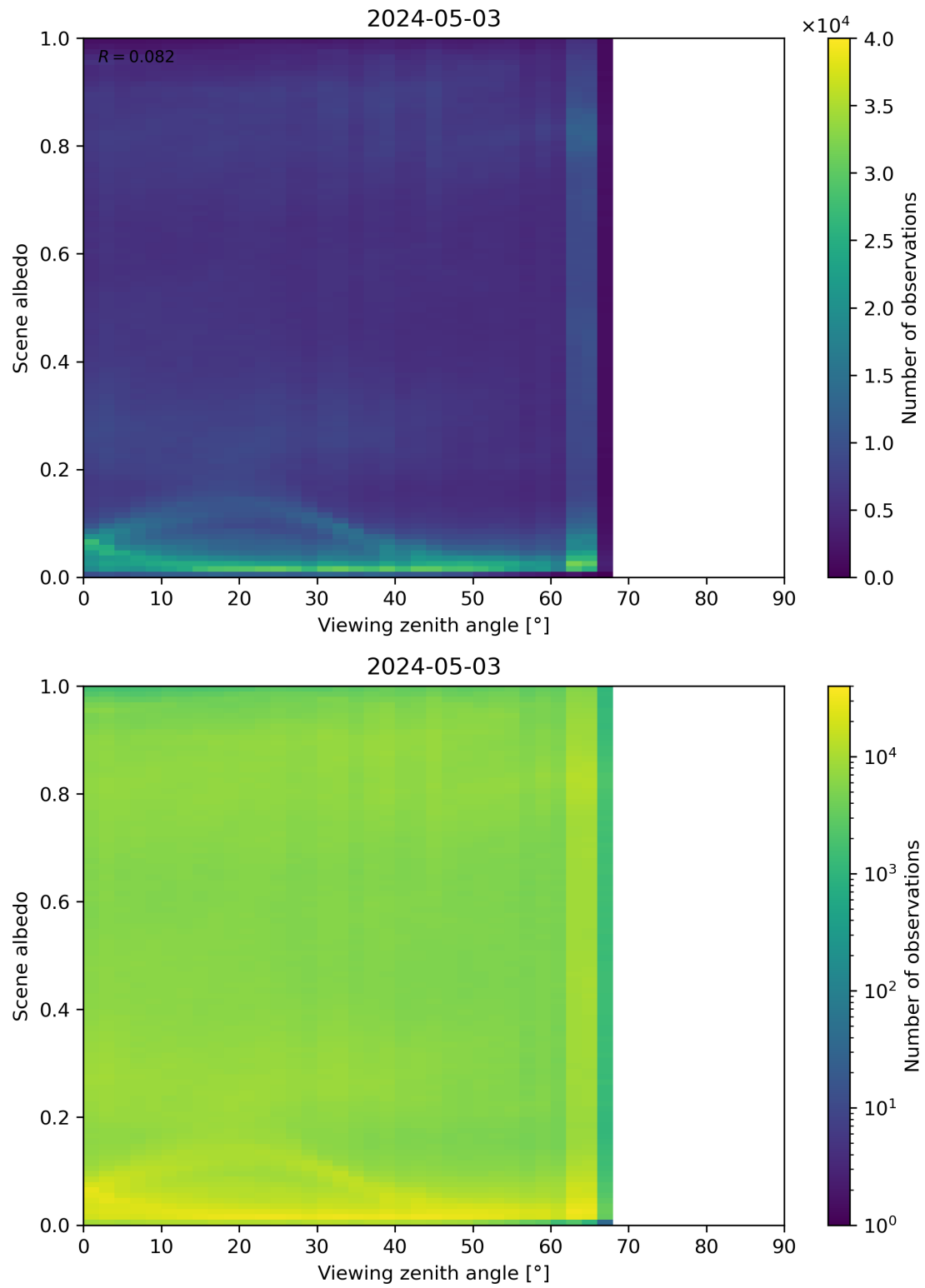
Figure 126: Scatter density plot of “Viewing zenith angle” against “Scene albedo” for 2024-05-02 to 2024-05-04.
