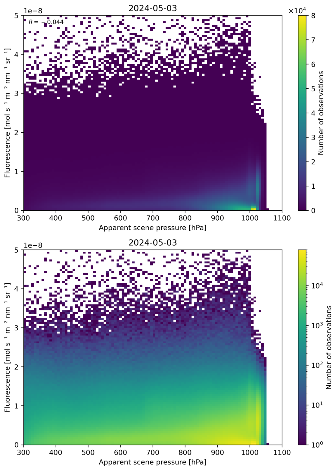
Figure 64: Scatter density plot of “Apparent scene pressure” against “Fluorescence” for 2024-05-02 to 2024-05-04.
