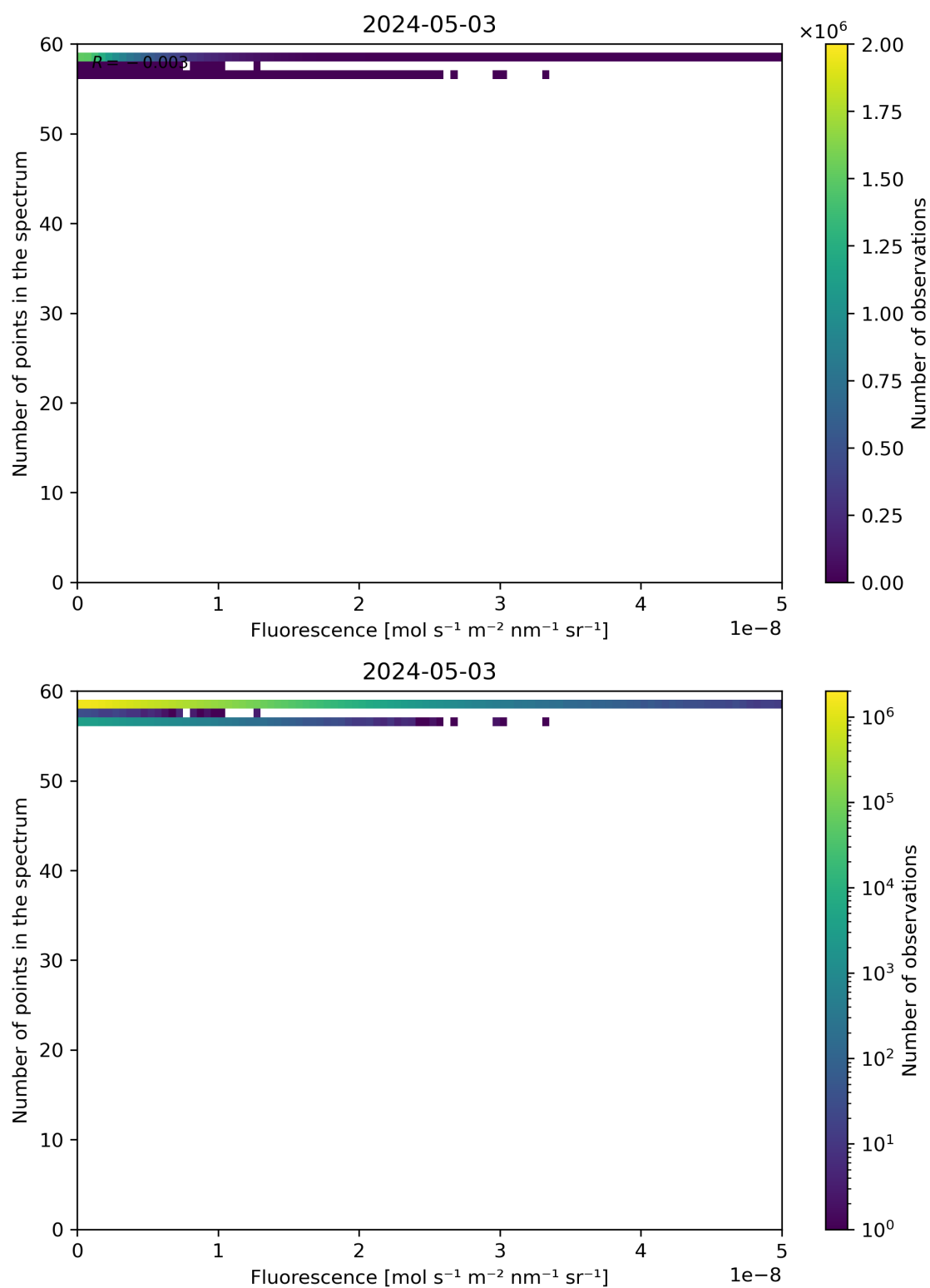
Figure 86: Scatter density plot of “Fluorescence” against “Number of points in the spectrum” for 2024-05-02 to 2024-05-04.
