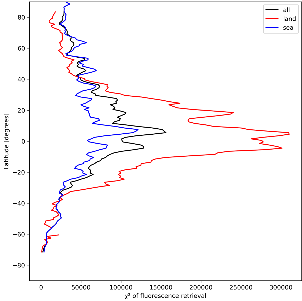
Figure 25: Zonal average of “ \chi^2 of fluorescence retrieval” for 2024-05-02 to 2024-05-04.
