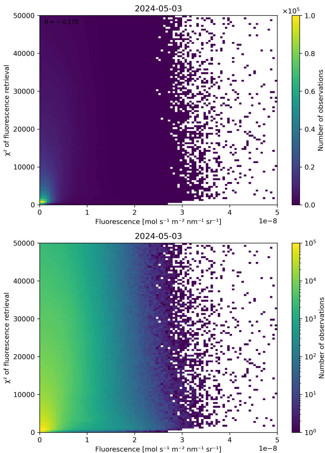
Figure 85: Scatter density plot of “Fluorescence” against “ \chi^2 of fluorescence retrieval” for 2024-05-02 to 2024-05-04.
