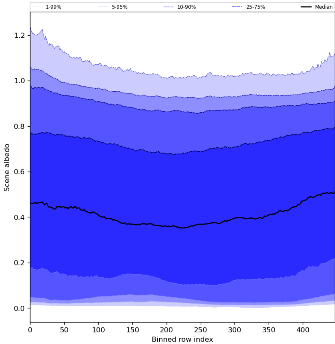
Figure 51: Along track statistics of “Scene albedo” for 2024-05-02 to 2024-05-04
