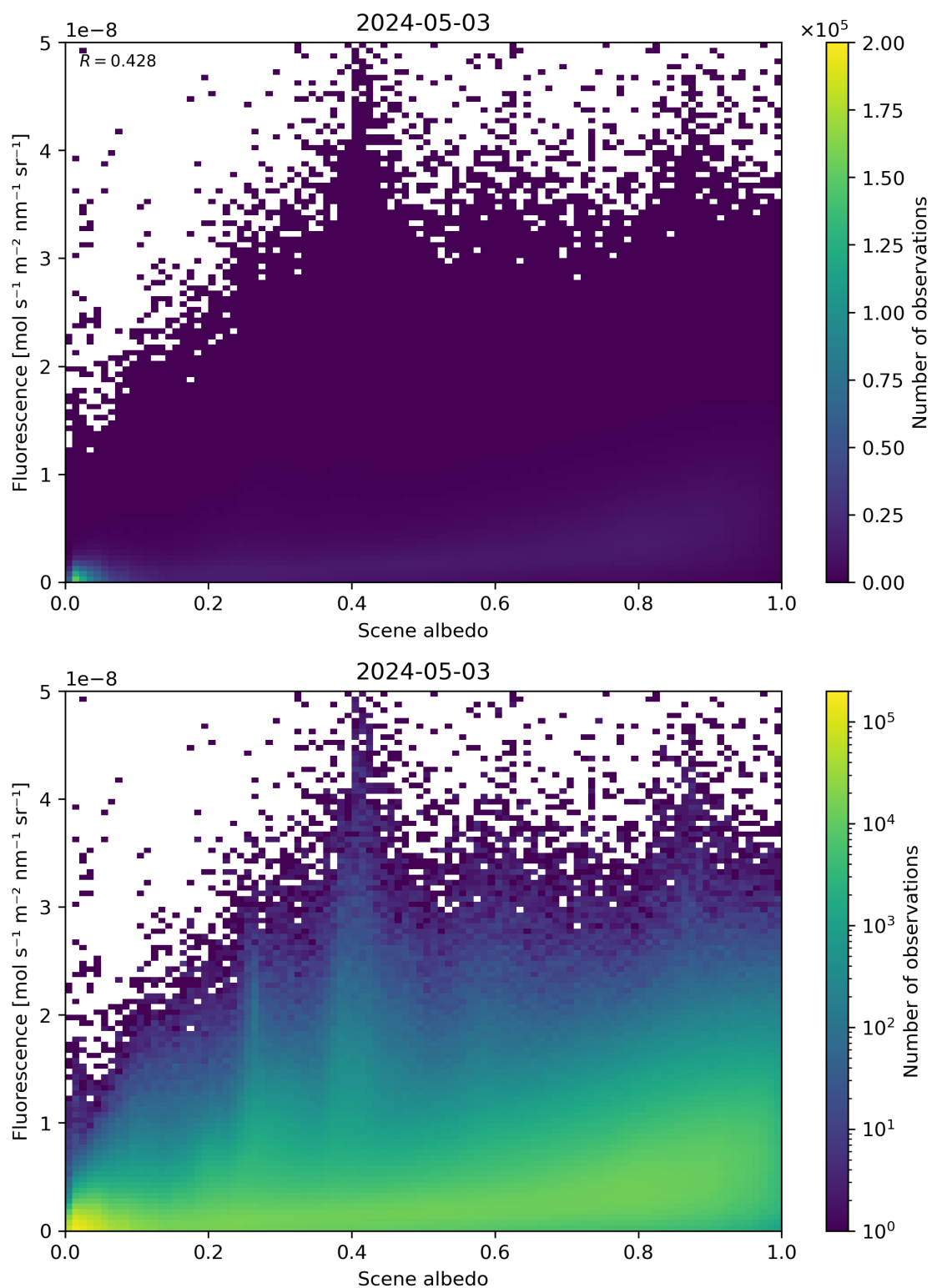
Figure 104: Scatter density plot of “Scene albedo” against “Fluorescence” for 2024-05-02 to 2024-05-04.
