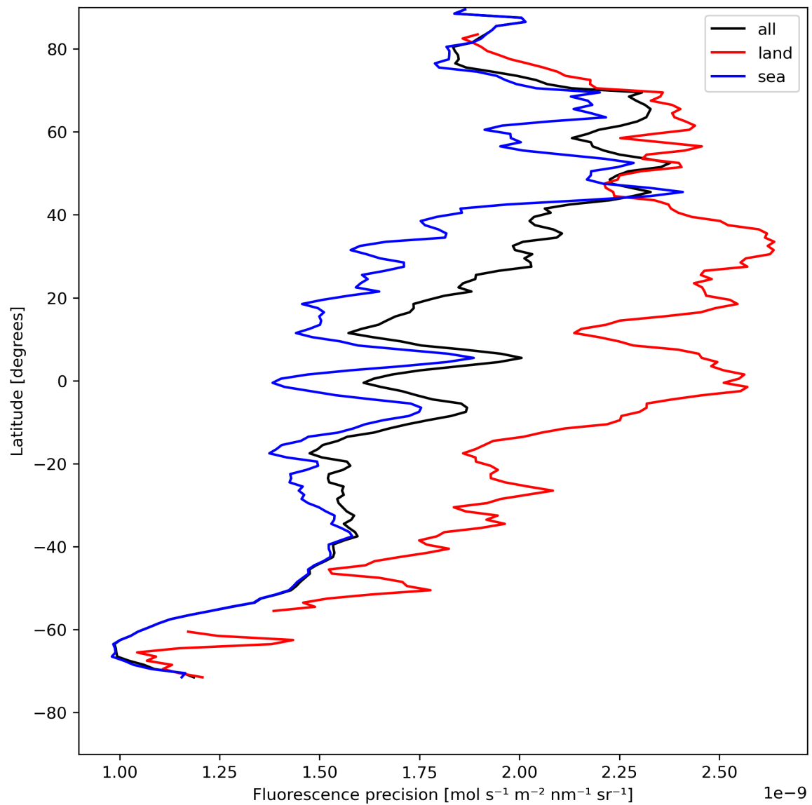
Figure 24: Zonal average of “Fluorescence precision” for 2024-05-02 to 2024-05-04.
