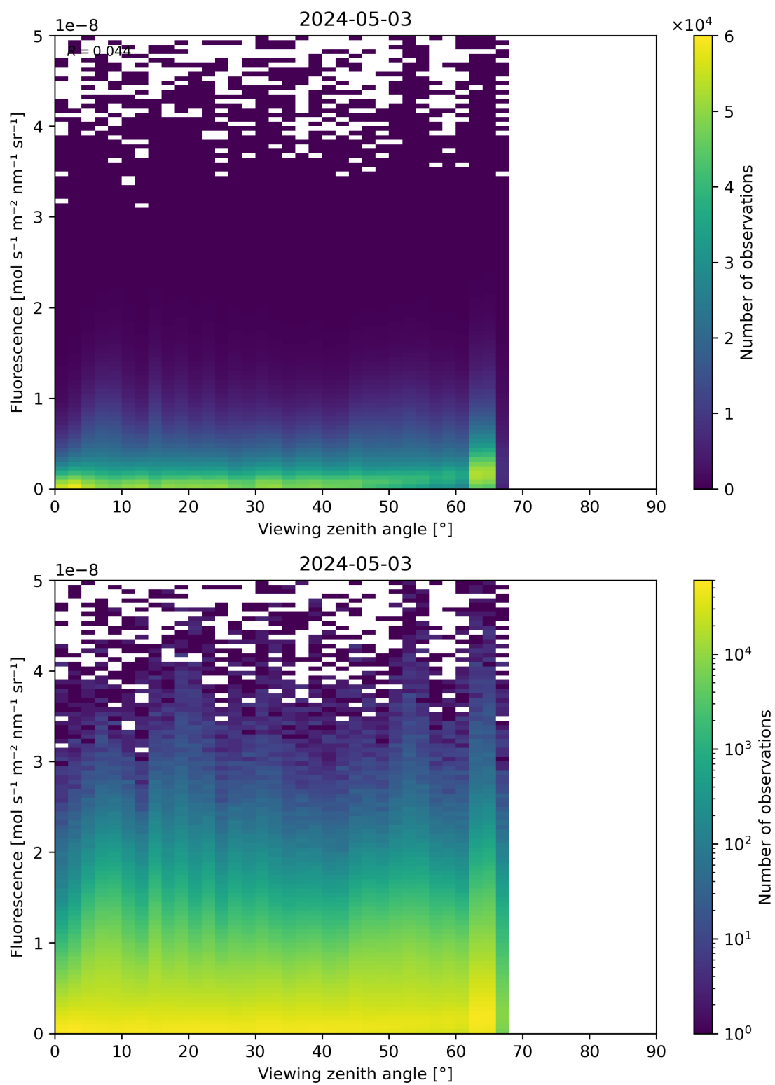
Figure 122: Scatter density plot of “Viewing zenith angle” against “Fluorescence” for 2024-05-02 to 2024-05-04.
