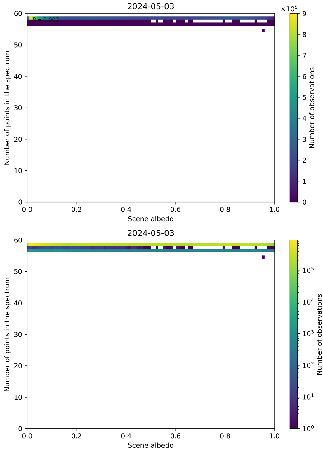
Figure 106: Scatter density plot of “Scene albedo” against “Number of points in the spectrum” for 2024-05-02 to 2024-05-04.
