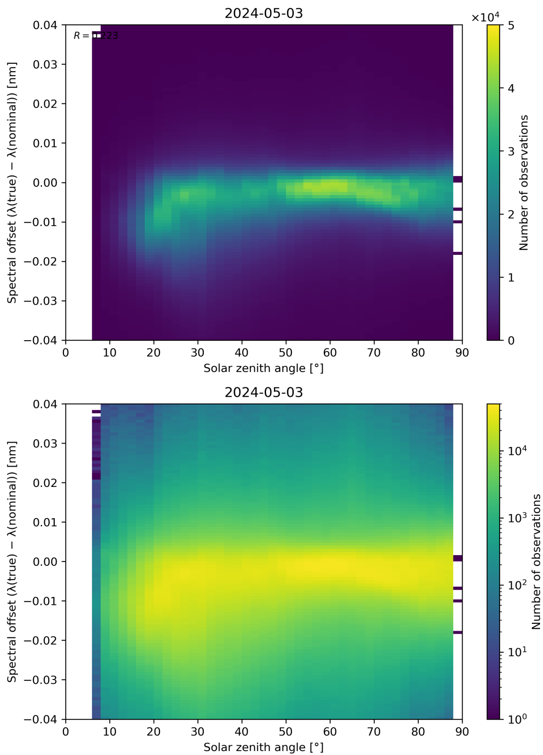
Figure 117: Scatter density plot of “Solar zenith angle” against “Spectral offset ( \lambda(\text{true}) - \lambda(\text{nominal}) )” for 2024-05-02 to 2024-05-04.
