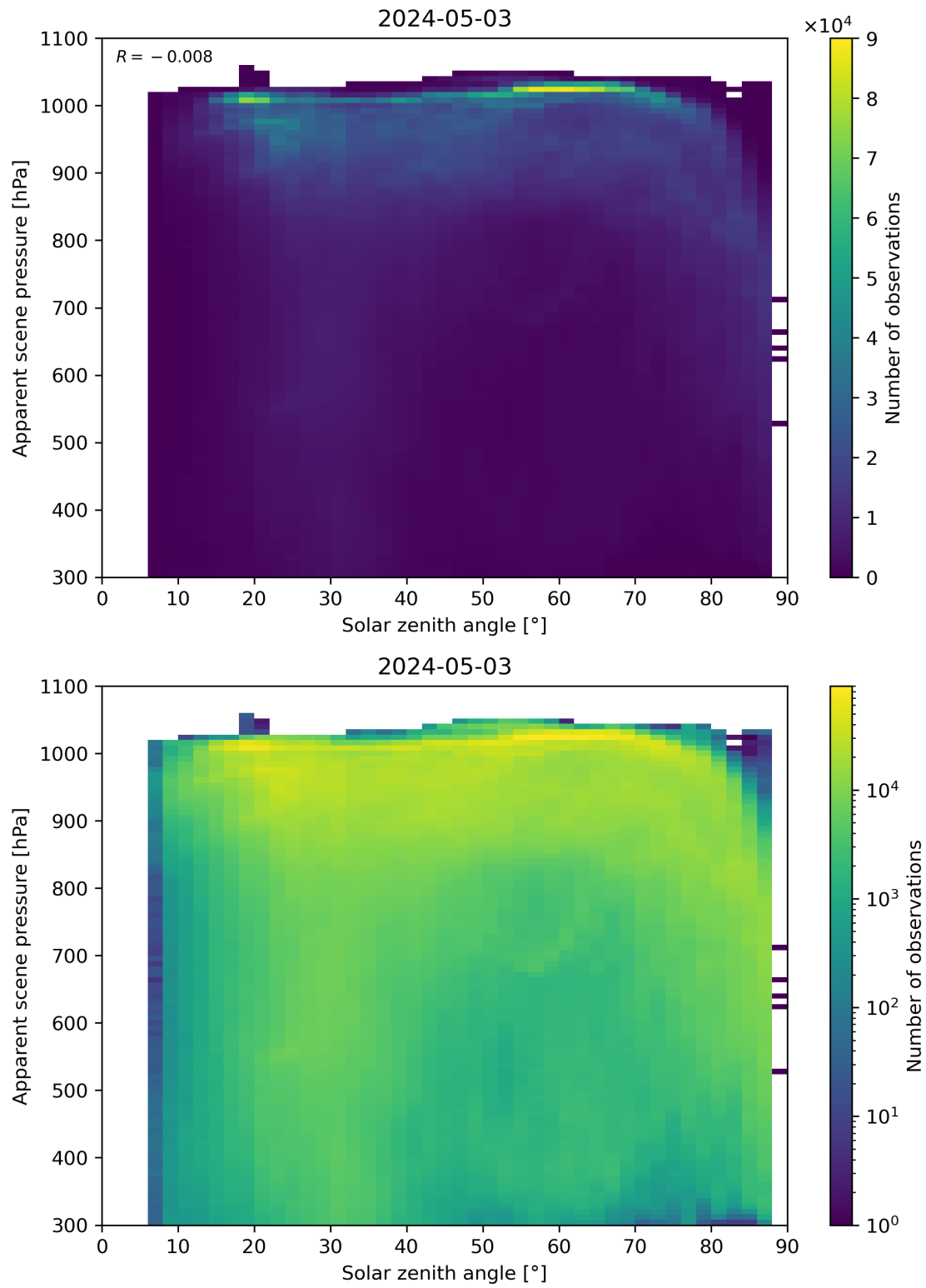
Figure 108: Scatter density plot of “Solar zenith angle” against “Apparent scene pressure” for 2024-05-02 to 2024-05-04.
