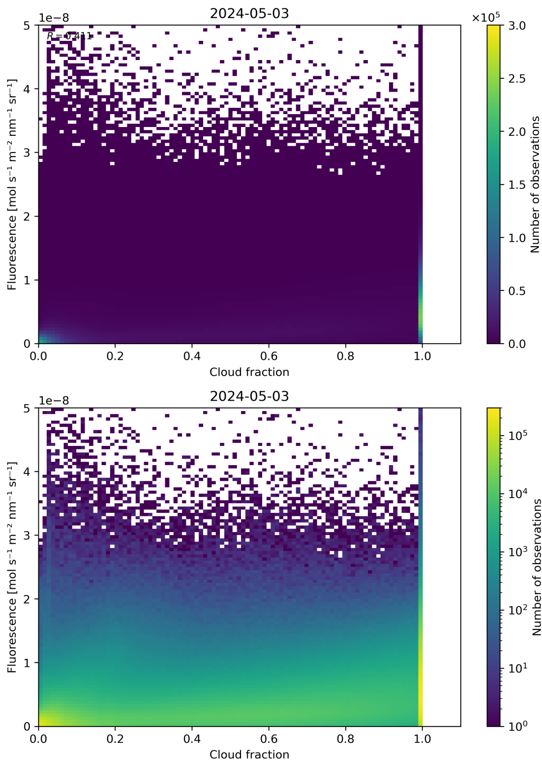
Figure 72: Scatter density plot of "Cloud fraction" against "Fluorescence" for 2024-05-02 to 2024-05-04.
