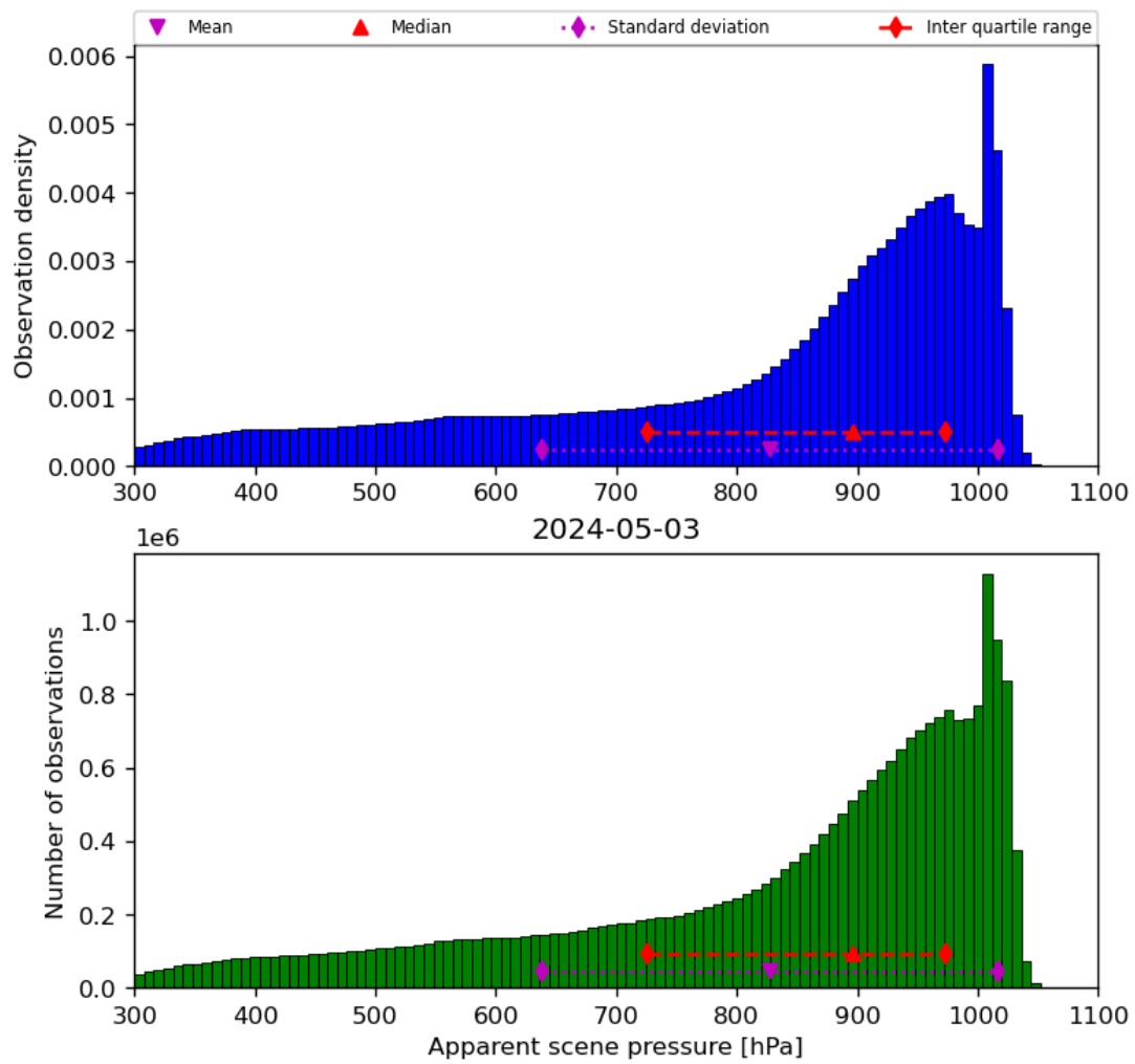
Figure 36: Histogram of “Apparent scene pressure” for 2024-05-02 to 2024-05-04
