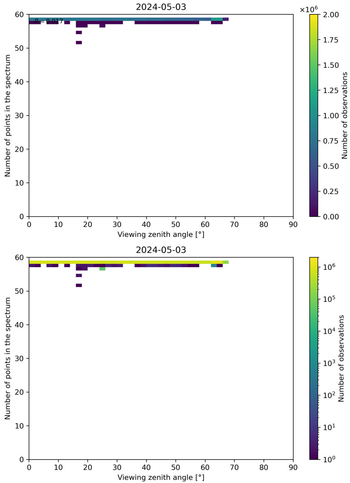
Figure 125: Scatter density plot of “Viewing zenith angle” against “Number of points in the spectrum” for 2024-05-02 to 2024-05-04.
