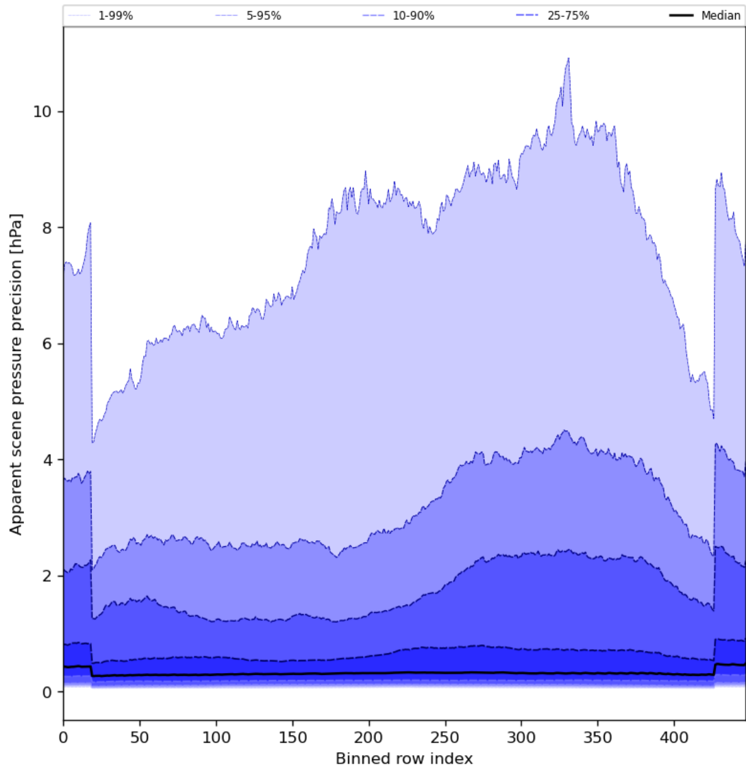
Figure 54: Along track statistics of “Apparent scene pressure precision” for 2024-05-02 to 2024-05-04
