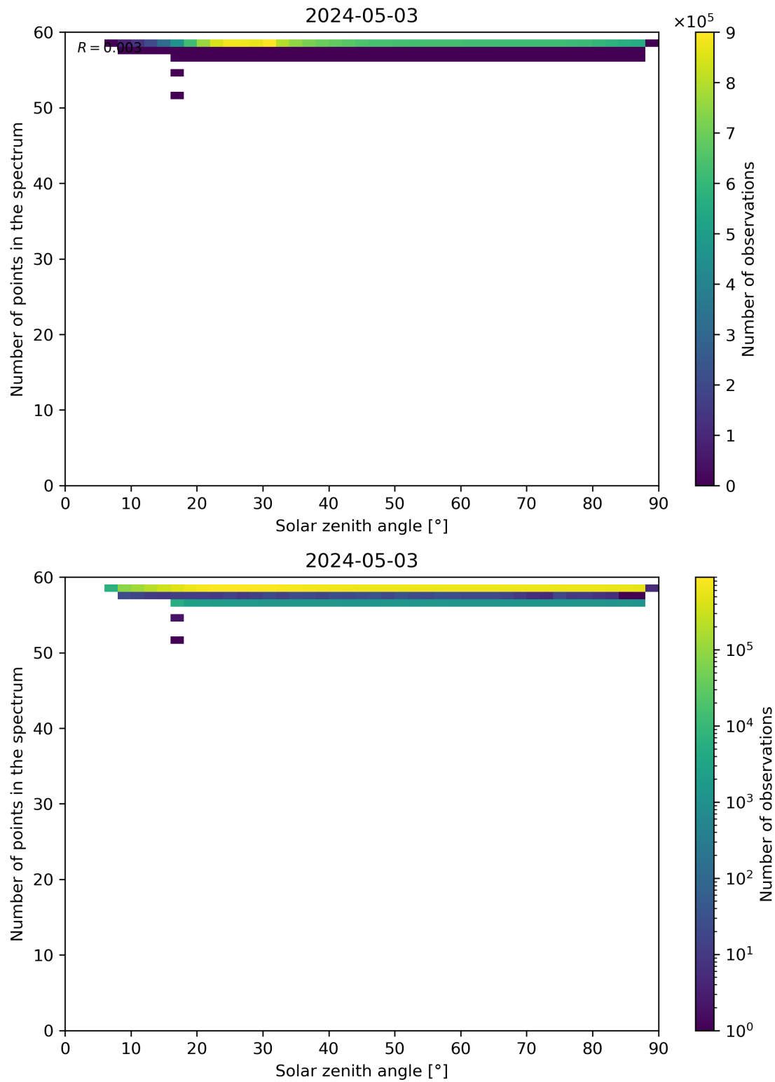
Figure 115: Scatter density plot of “Solar zenith angle” against “Number of points in the spectrum” for 2024-05-02 to 2024-05-04.
