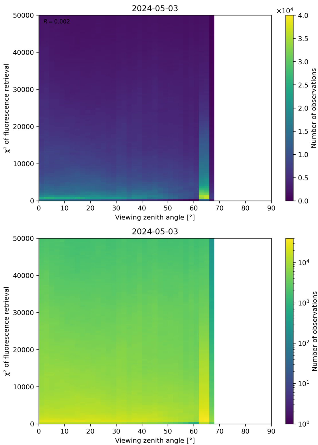
Figure 119: Scatter density plot of “Viewing zenith angle” against “ \chi^2 of fluorescence retrieval” for 2024-05-02 to 2024-05-04.
