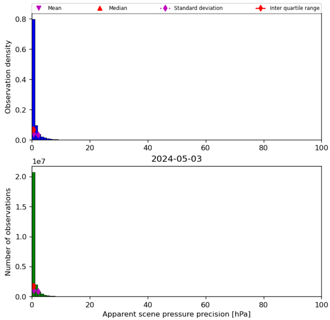
Figure 37: Histogram of “Apparent scene pressure precision” for 2024-05-02 to 2024-05-04
