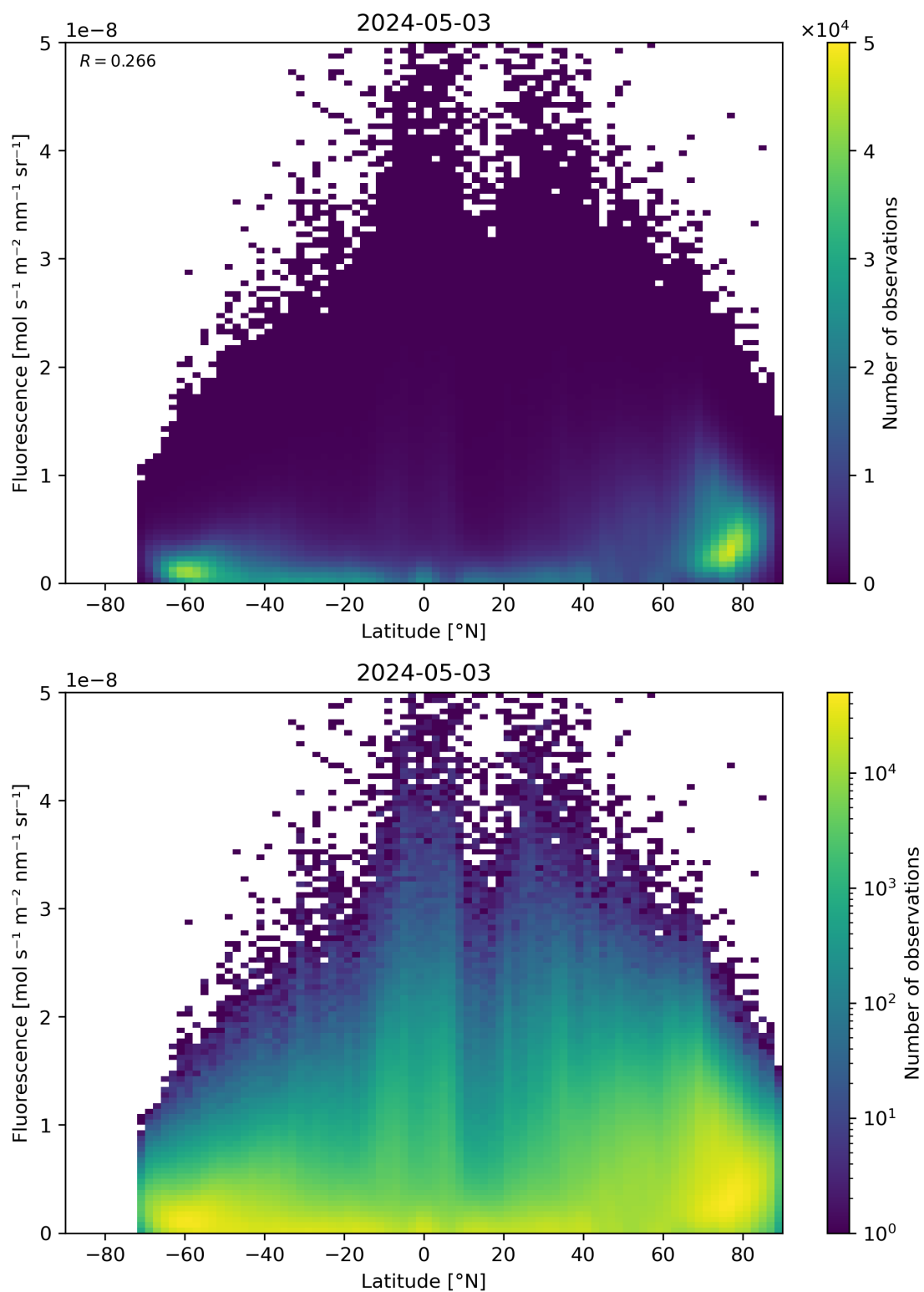
Figure 92: Scatter density plot of “Latitude” against “Fluorescence” for 2024-05-02 to 2024-05-04.
