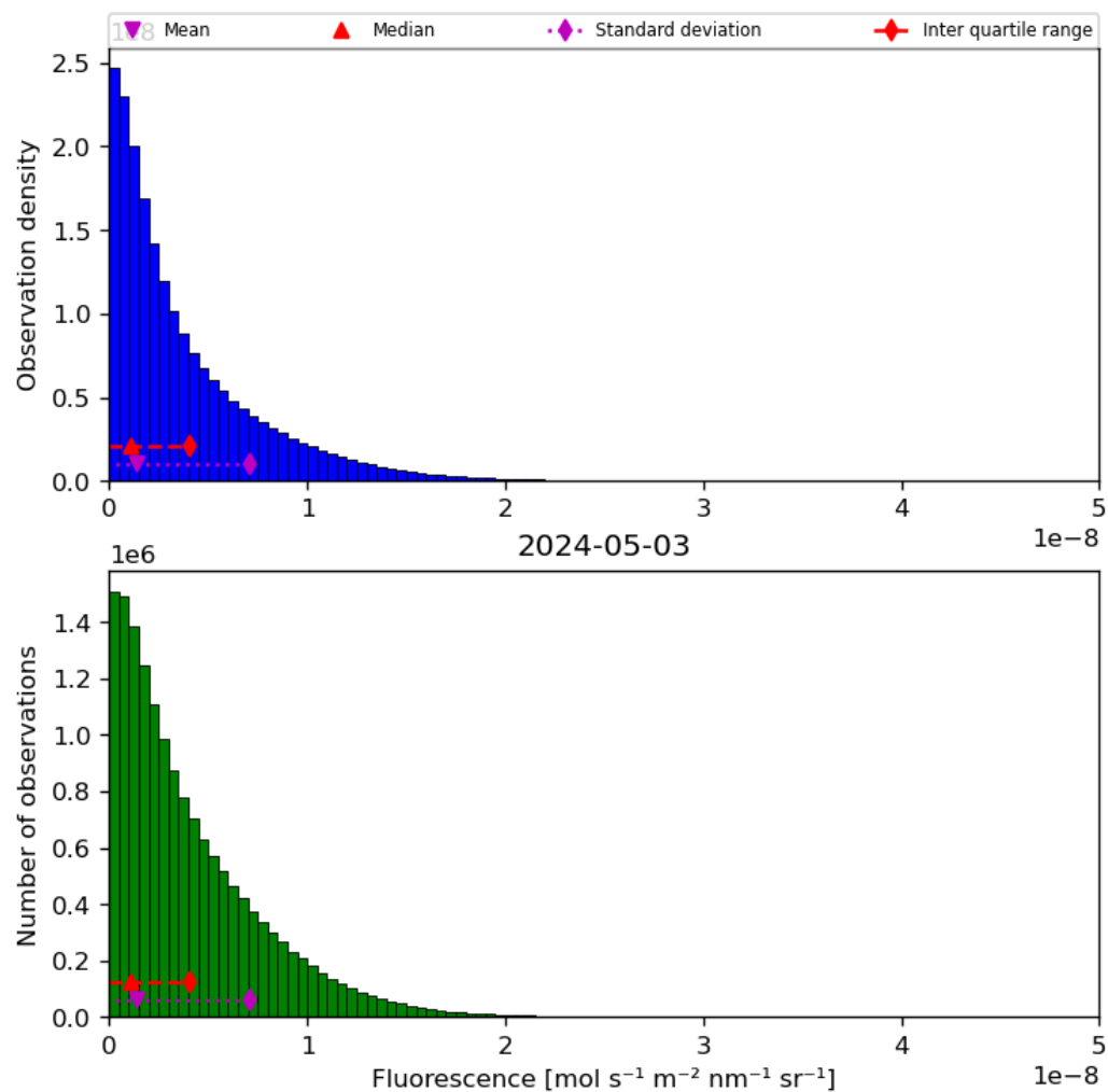
Figure 40: Histogram of “Fluorescence” for 2024-05-02 to 2024-05-04
