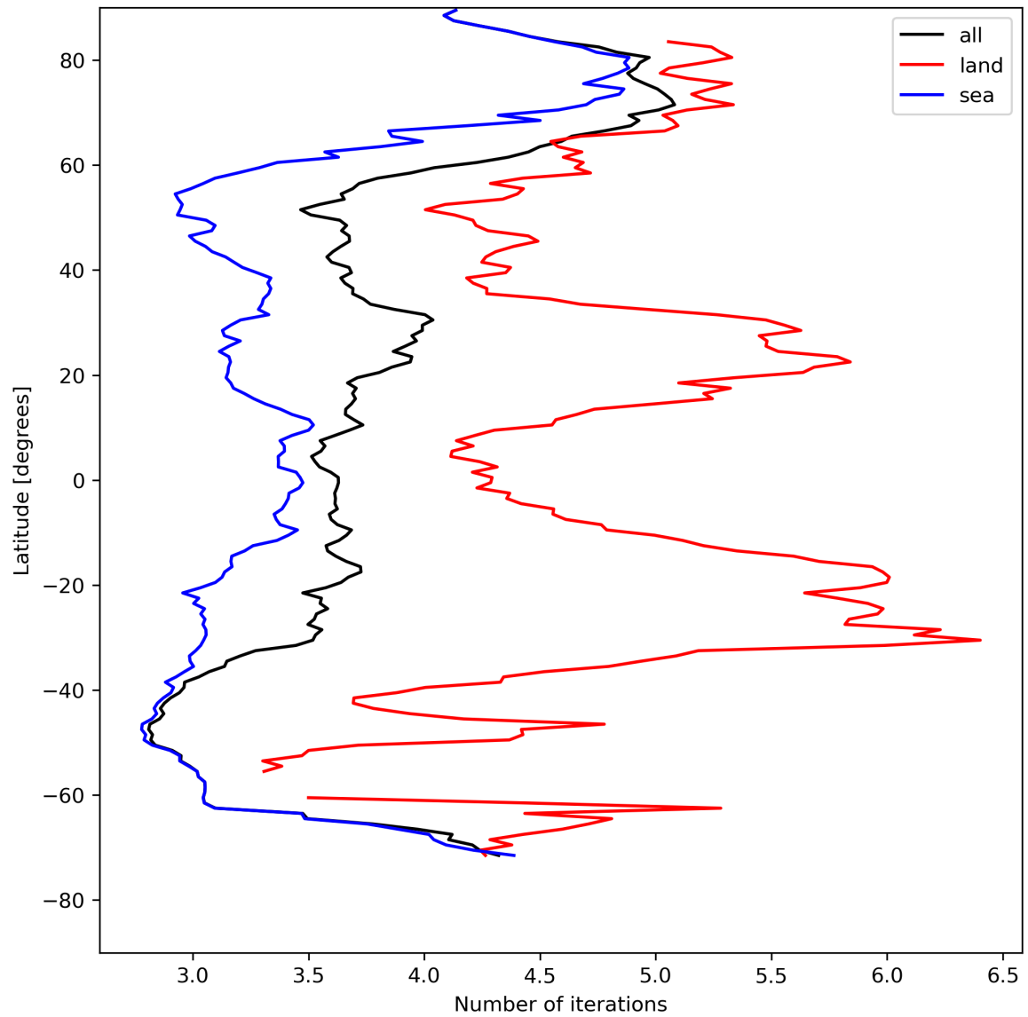
Figure 22: Zonal average of “Number of iterations” for 2024-05-02 to 2024-05-04.
