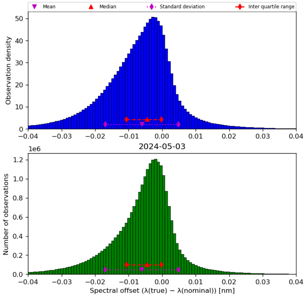
Figure 45: Histogram of “Spectral offset ( \lambda(\text{true}) - \lambda(\text{nominal}) )” for 2024-05-02 to 2024-05-04
