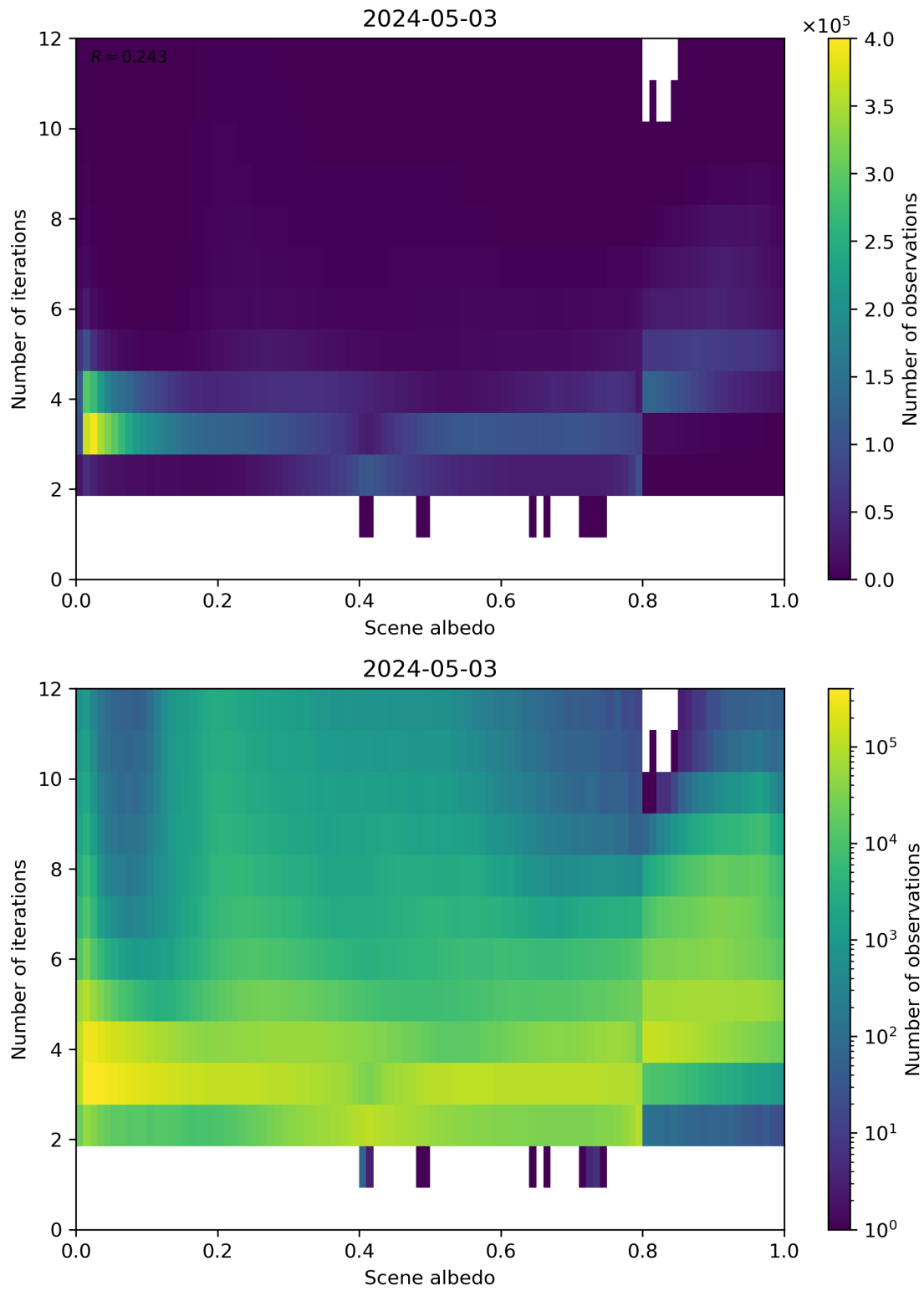
Figure 105: Scatter density plot of “Scene albedo” against “Number of iterations” for 2024-05-02 to 2024-05-04.
