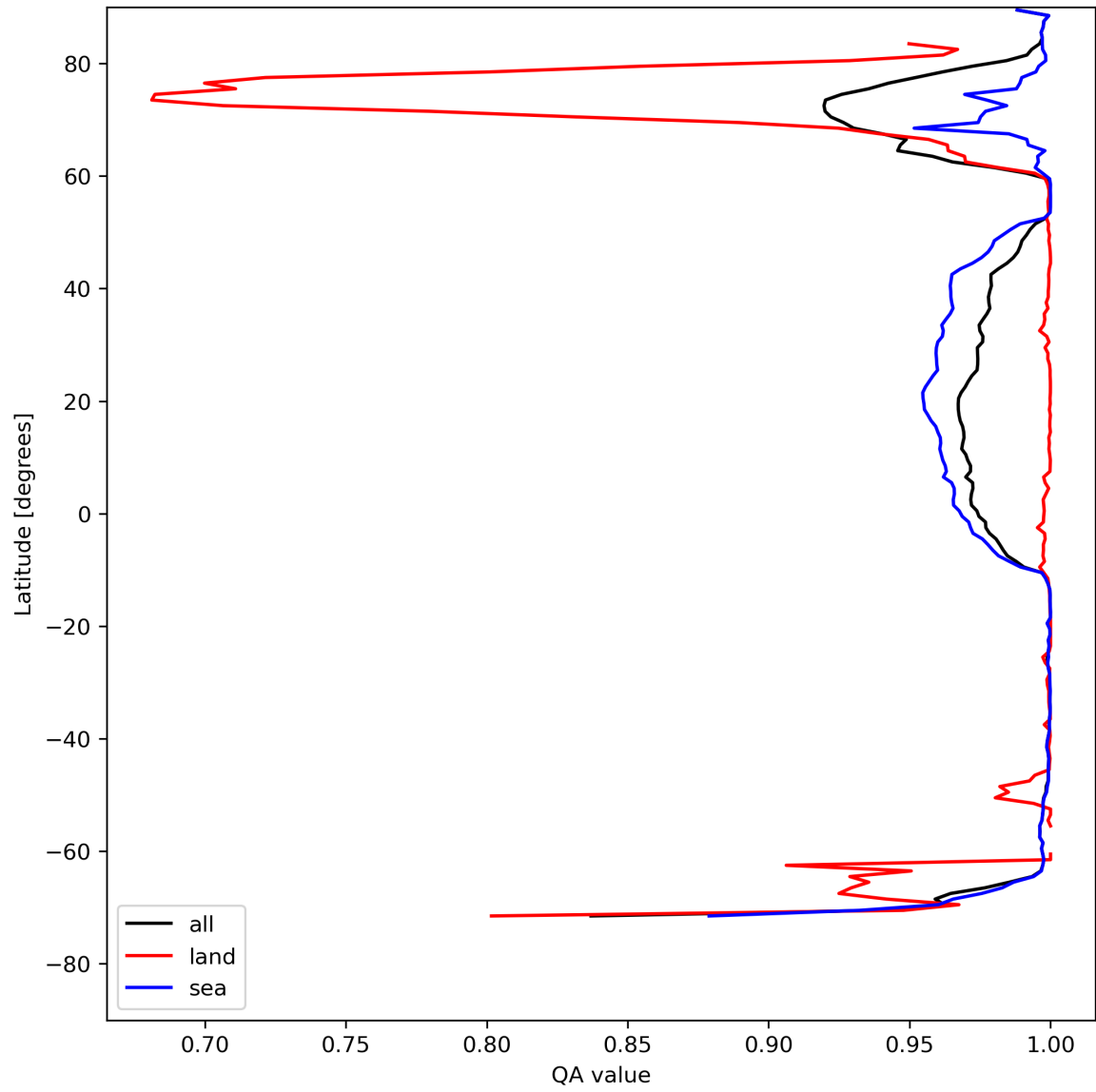
Figure 12: Zonal average of “QA value” for 2024-05-02 to 2024-05-04.
