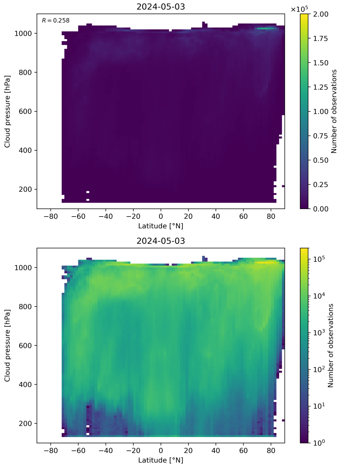
Figure 91: Scatter density plot of “Latitude” against “Cloud pressure” for 2024-05-02 to 2024-05-04.
