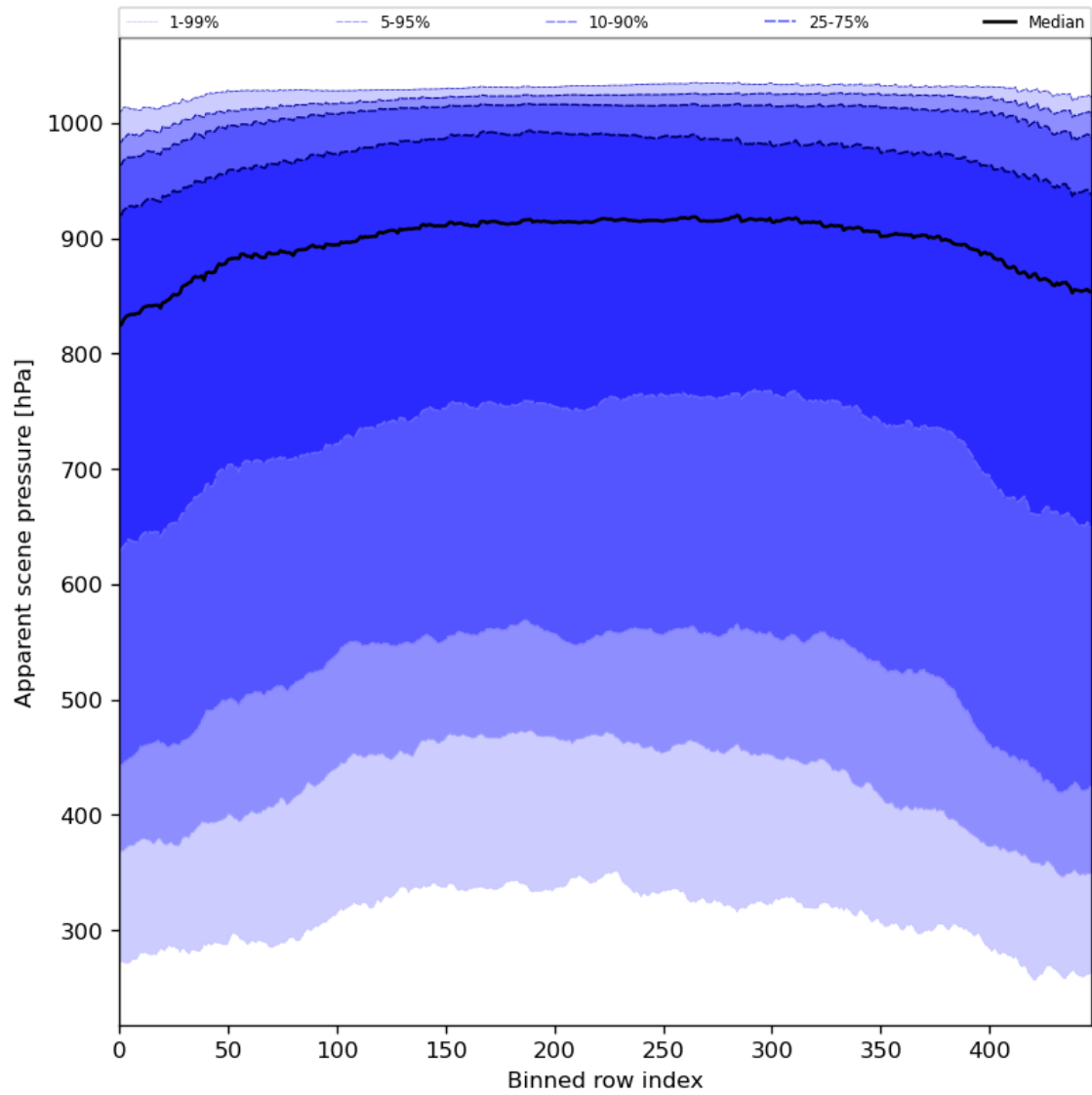
Figure 53: Along track statistics of “Apparent scene pressure” for 2024-05-02 to 2024-05-04
