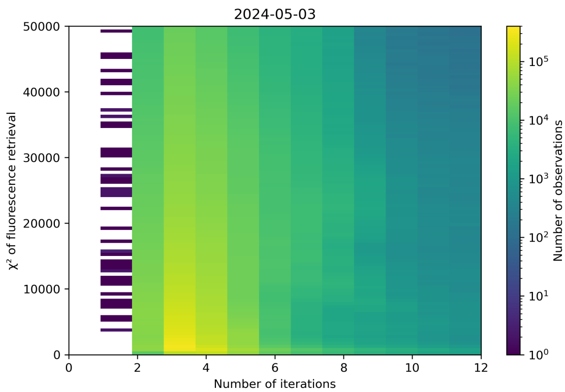
Figure 97: Scatter density plot of “Number of iterations” against “ \chi^2 of fluorescence retrieval” for 2024-05-02 to 2024-05-04.
