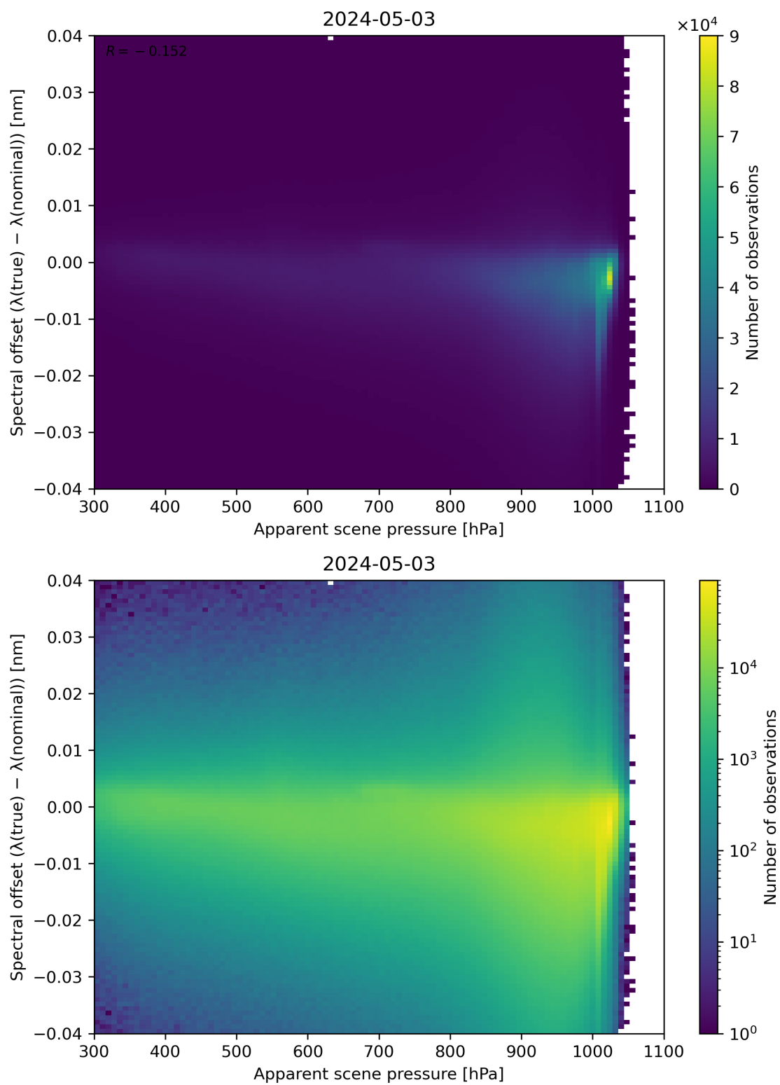
Figure 67: Scatter density plot of “Apparent scene pressure” against “Spectral offset ( \lambda(\text{true}) - \lambda(\text{nominal}) )” for 2024-05-02 to 2024-05-04.
