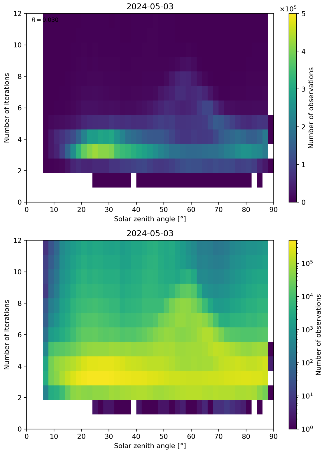
Figure 114: Scatter density plot of “Solar zenith angle” against “Number of iterations” for 2024-05-02 to 2024-05-04.
