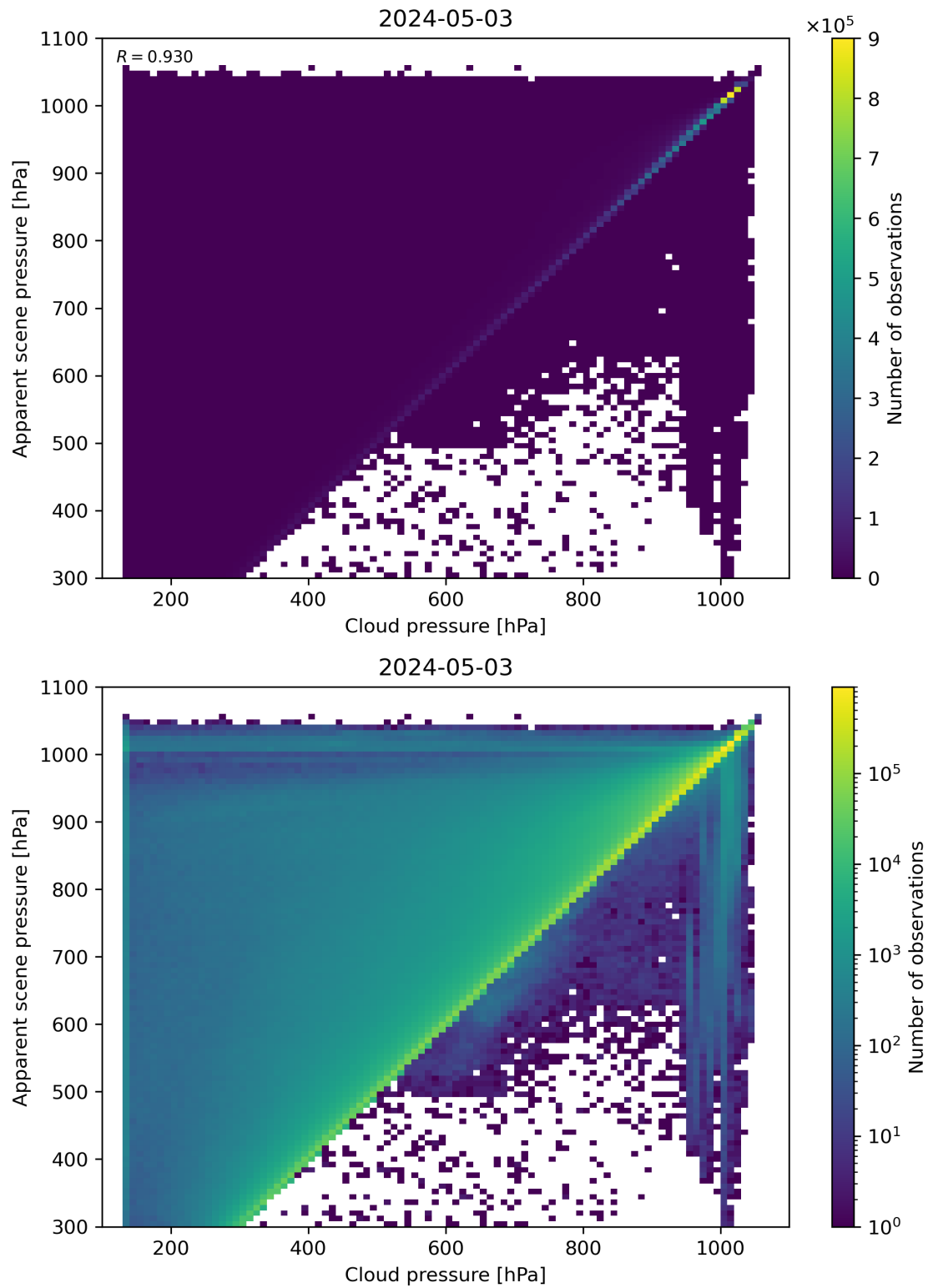
Figure 77: Scatter density plot of “Cloud pressure” against “Apparent scene pressure” for 2024-05-02 to 2024-05-04.
