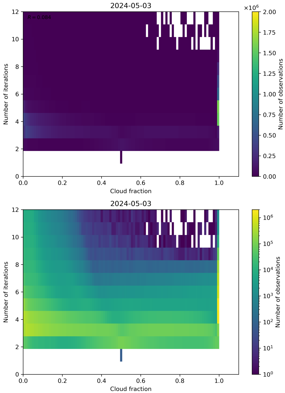
Figure 73: Scatter density plot of “Cloud fraction” against “Number of iterations” for 2024-05-02 to 2024-05-04.
