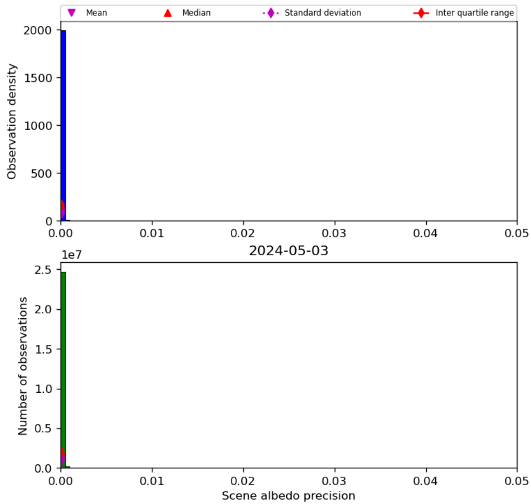
Figure 35: Histogram of “Scene albedo precision” for 2024-05-02 to 2024-05-04
