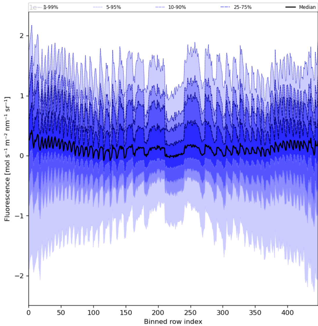
Figure 57: Along track statistics of “Fluorescence” for 2024-05-02 to 2024-05-04
