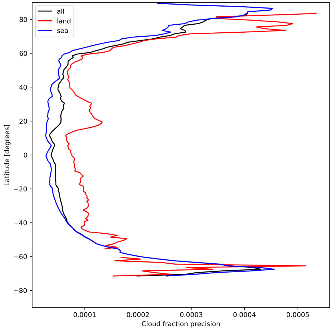
Figure 16: Zonal average of “Cloud fraction precision” for 2024-05-02 to 2024-05-04.
