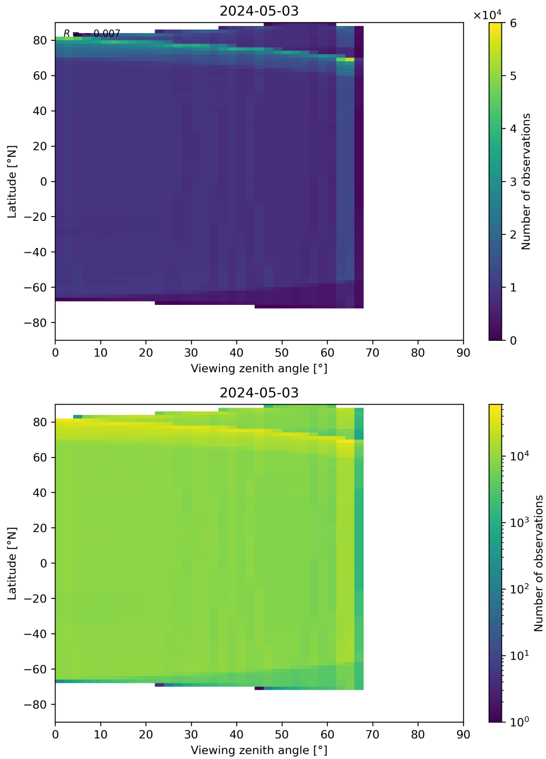
Figure 123: Scatter density plot of “Viewing zenith angle” against “Latitude” for 2024-05-02 to 2024-05-04.
