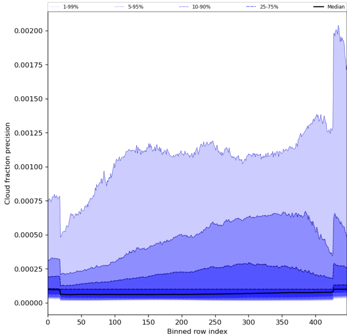
Figure 50: Along track statistics of “Cloud fraction precision” for 2024-05-02 to 2024-05-04
