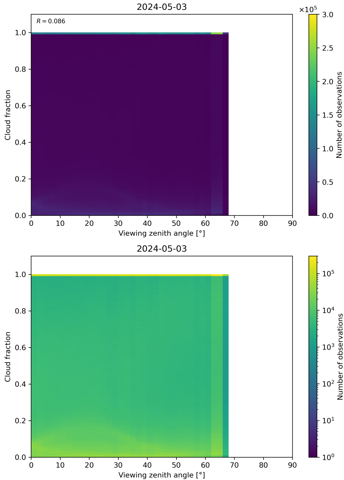
Figure 120: Scatter density plot of “Viewing zenith angle” against “Cloud fraction” for 2024-05-02 to 2024-05-04.
