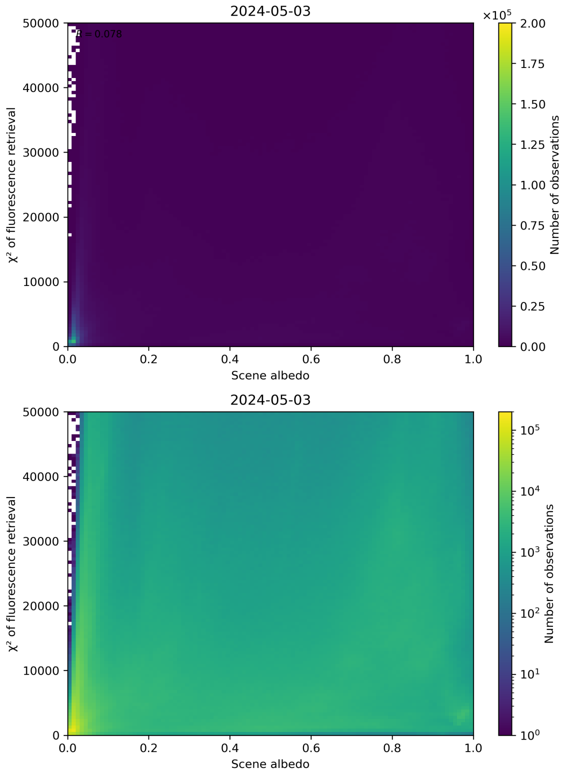
Figure 103: Scatter density plot of “Scene albedo” against “ \chi^2 of fluorescence retrieval” for 2024-05-02 to 2024-05-04.
