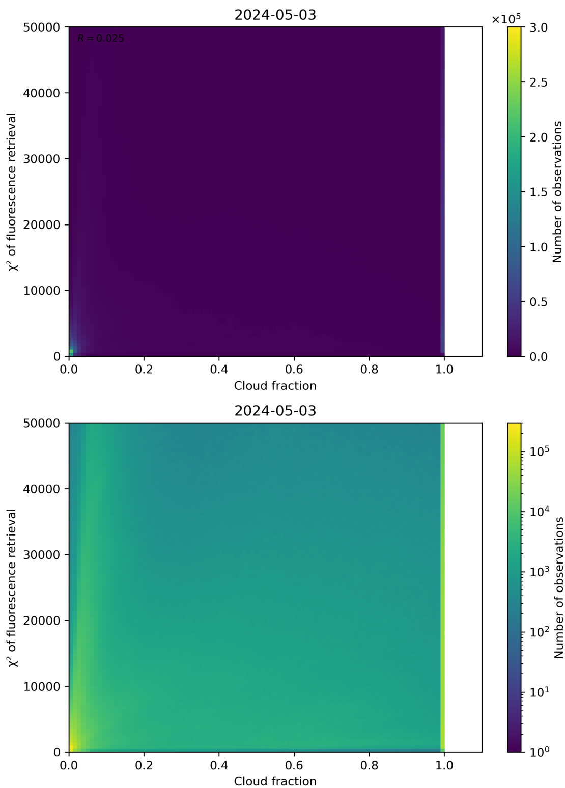
Figure 71: Scatter density plot of “Cloud fraction” against “ \chi^2 of fluorescence retrieval” for 2024-05-02 to 2024-05-04.
