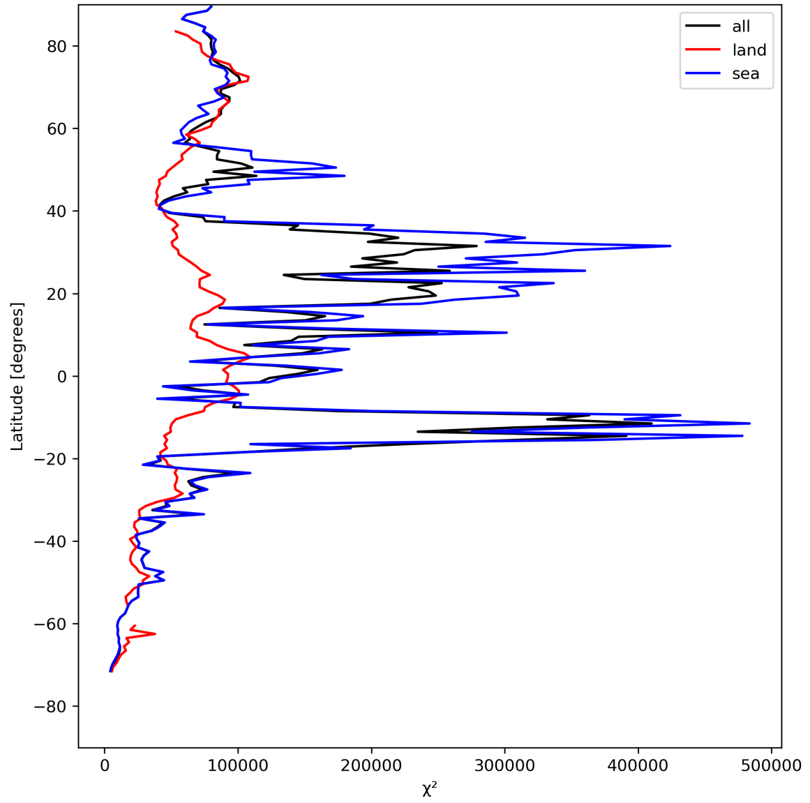
Figure 21: Zonal average of “ \chi^2 ” for 2024-05-02 to 2024-05-04.
