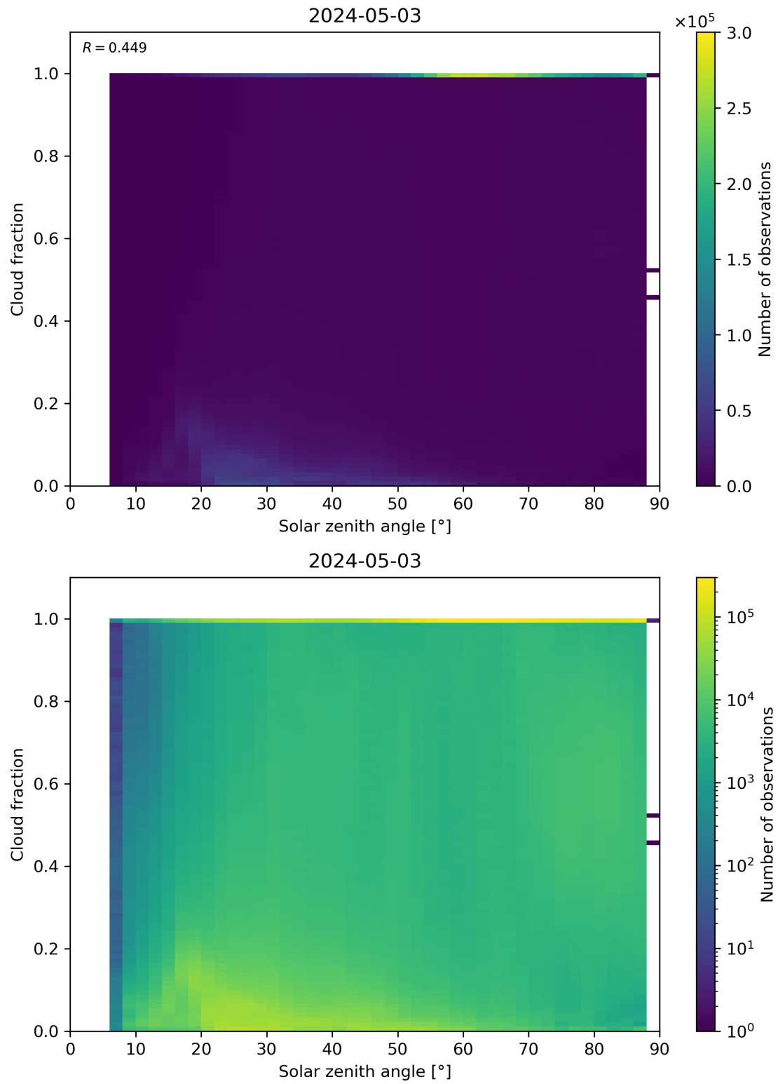
Figure 110: Scatter density plot of “Solar zenith angle” against “Cloud fraction” for 2024-05-02 to 2024-05-04.
