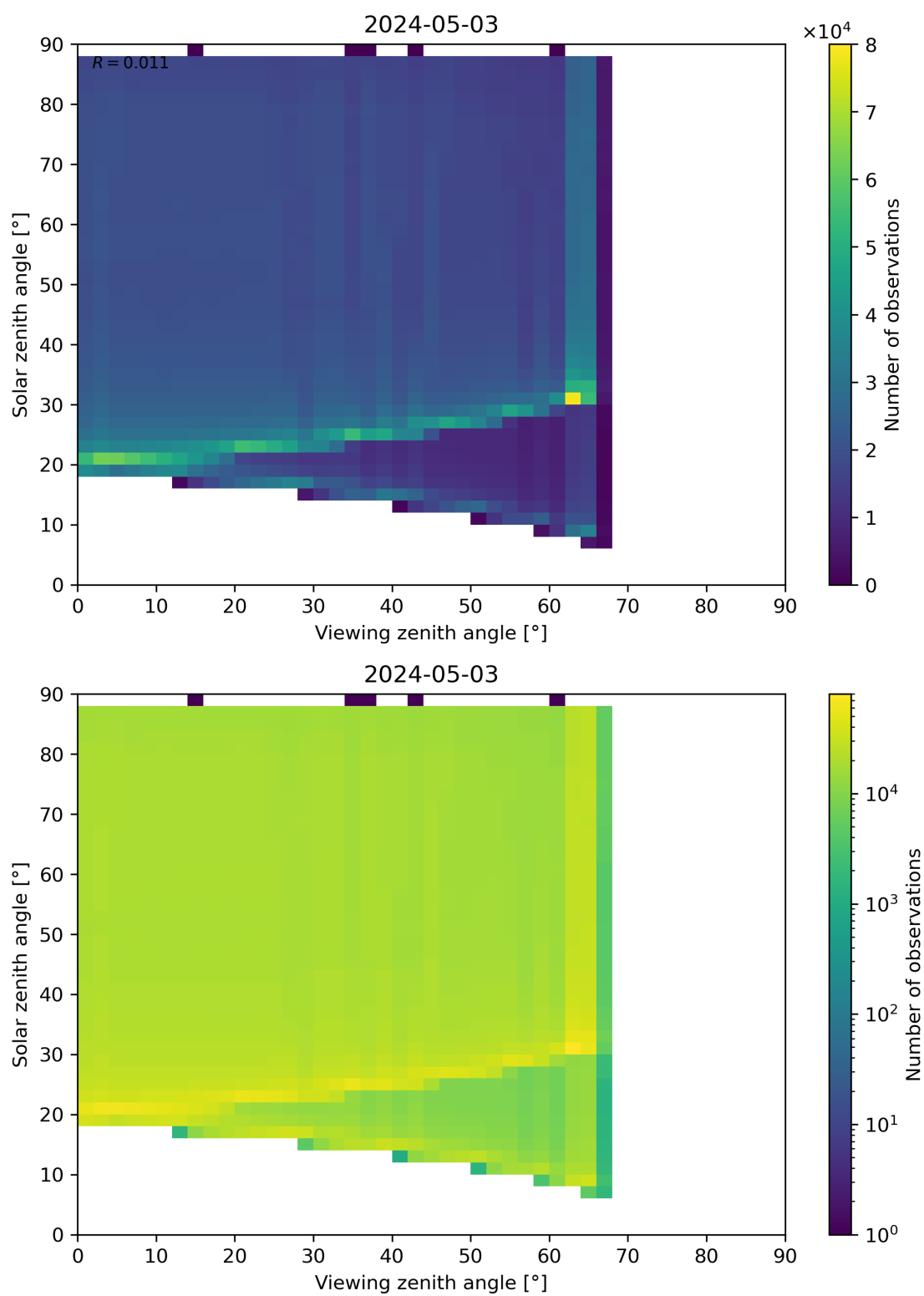
Figure 127: Scatter density plot of “Viewing zenith angle” against “Solar zenith angle” for 2024-05-02 to 2024-05-04.
