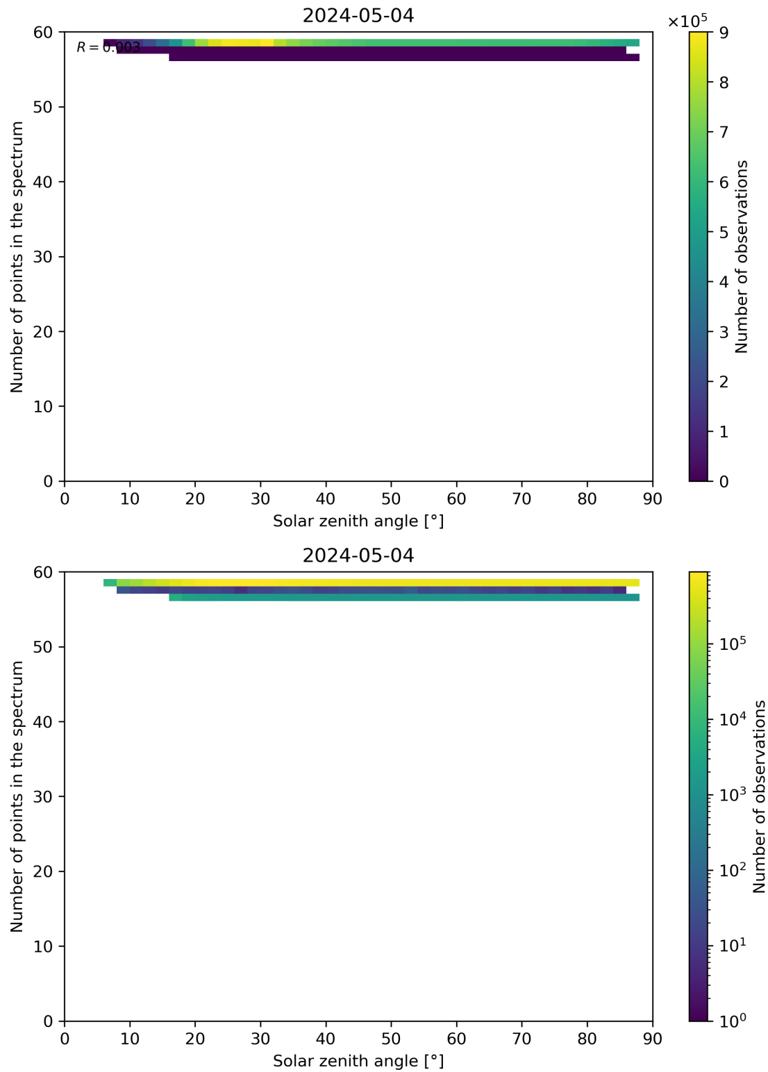
Figure 115: Scatter density plot of “Solar zenith angle” against “Number of points in the spectrum” for 2024-05-03 to 2024-05-05.
