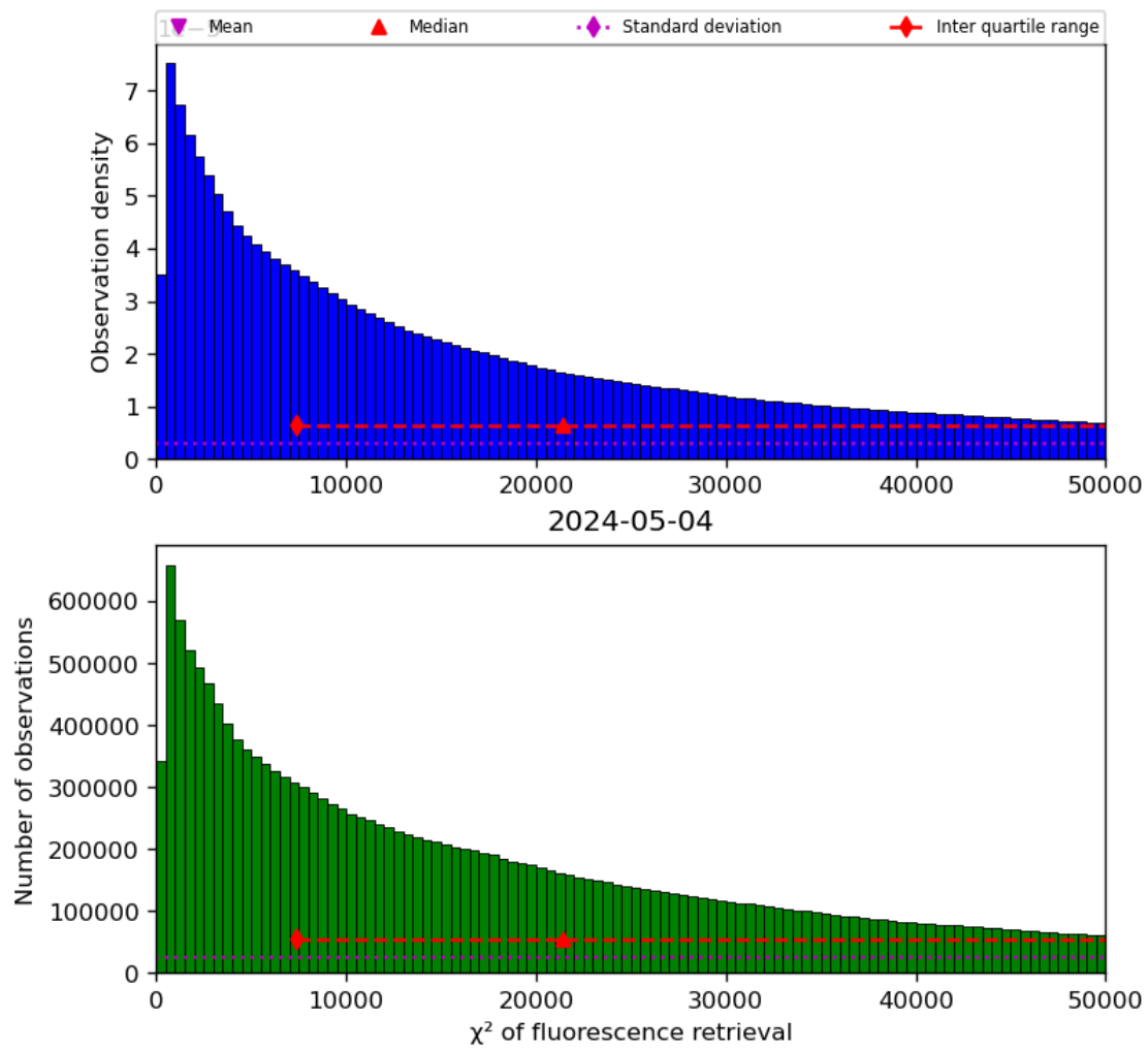
Figure 42: Histogram of “ \chi^2 of fluorescence retrieval” for 2024-05-03 to 2024-05-05
