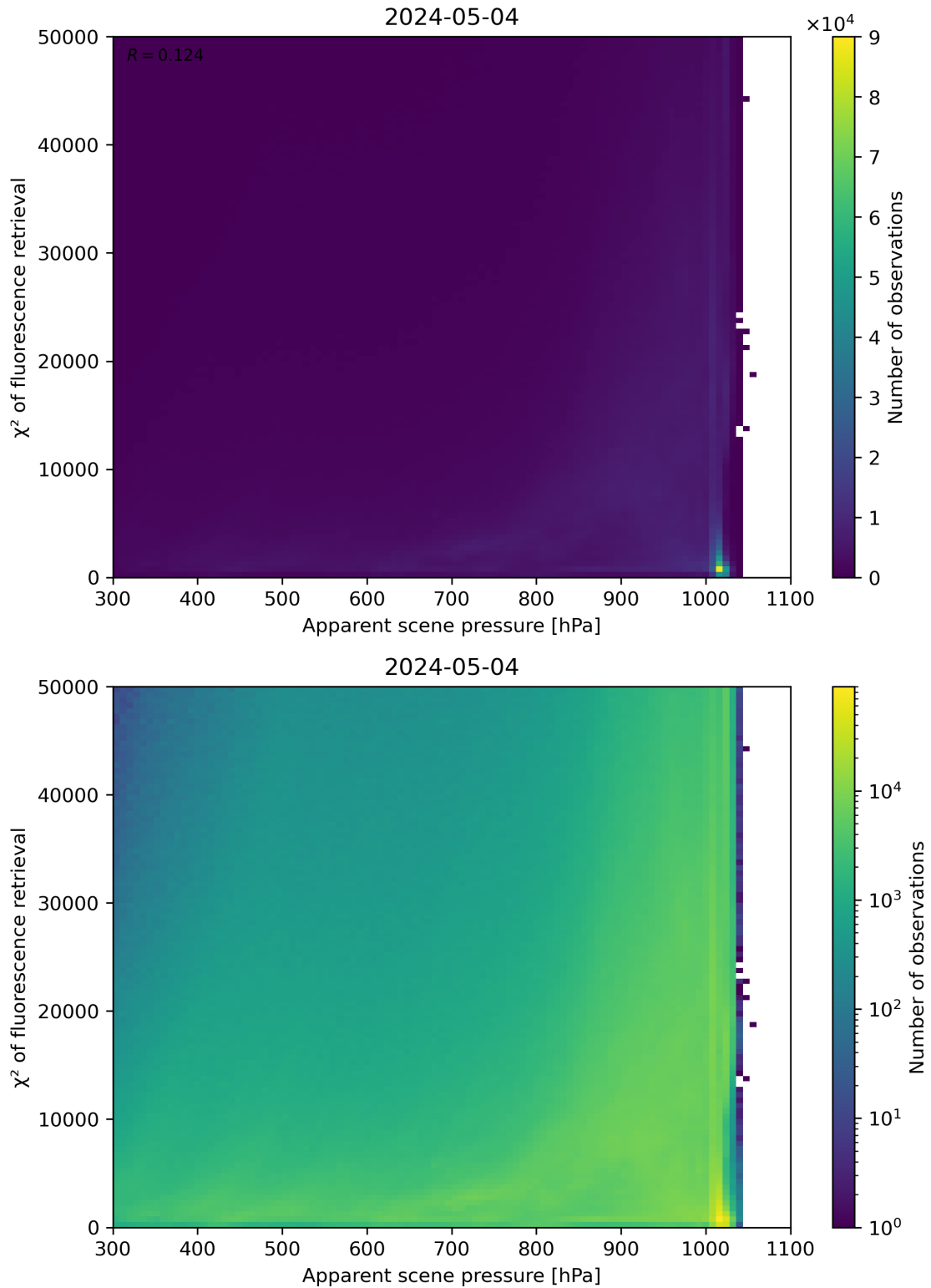
Figure 63: Scatter density plot of “Apparent scene pressure” against “ \chi^2 of fluorescence retrieval” for 2024-05-03 to 2024-05-05.
