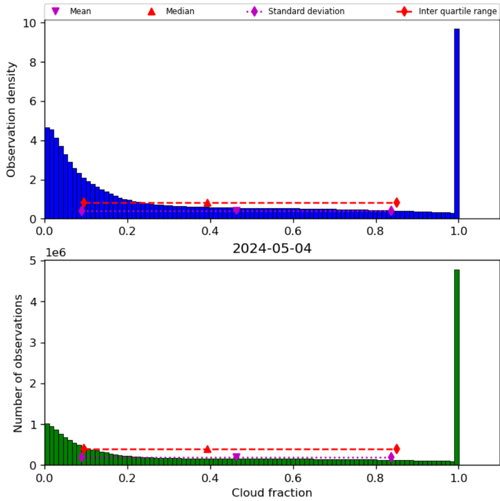
Figure 32: Histogram of “Cloud fraction” for 2024-05-03 to 2024-05-05
