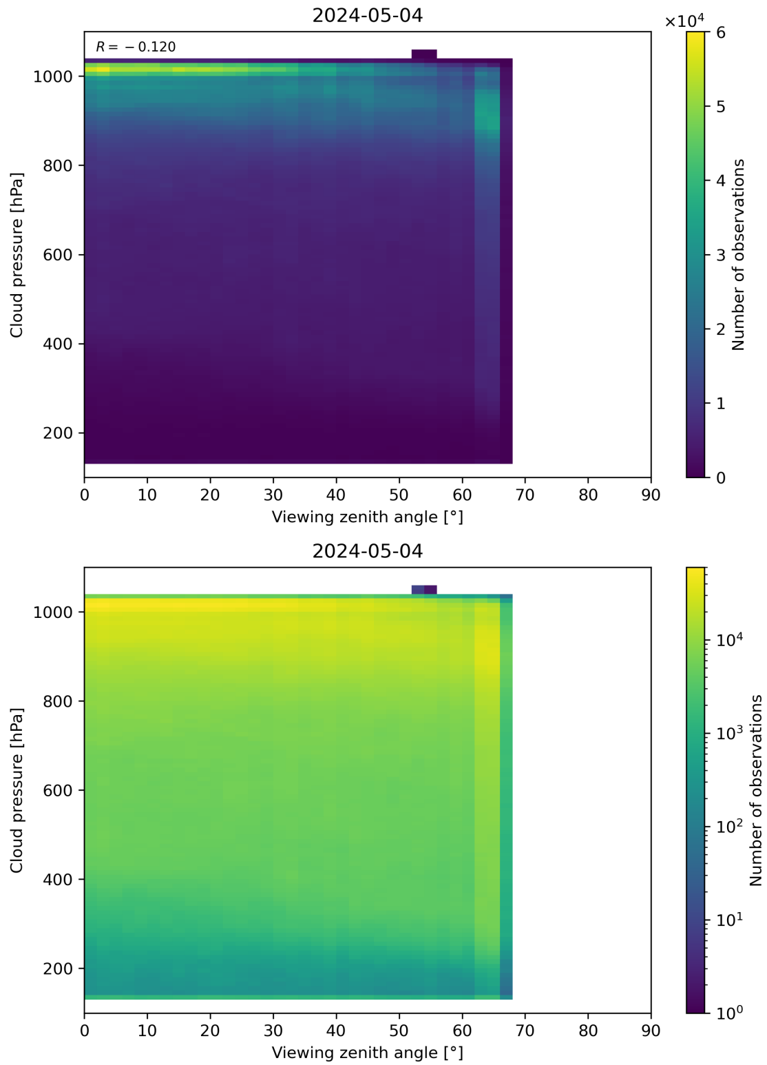
Figure 121: Scatter density plot of “Viewing zenith angle” against “Cloud pressure” for 2024-05-03 to 2024-05-05.
