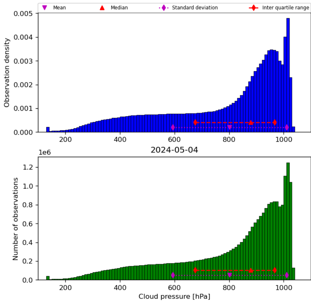
Figure 30: Histogram of “Cloud pressure” for 2024-05-03 to 2024-05-05
