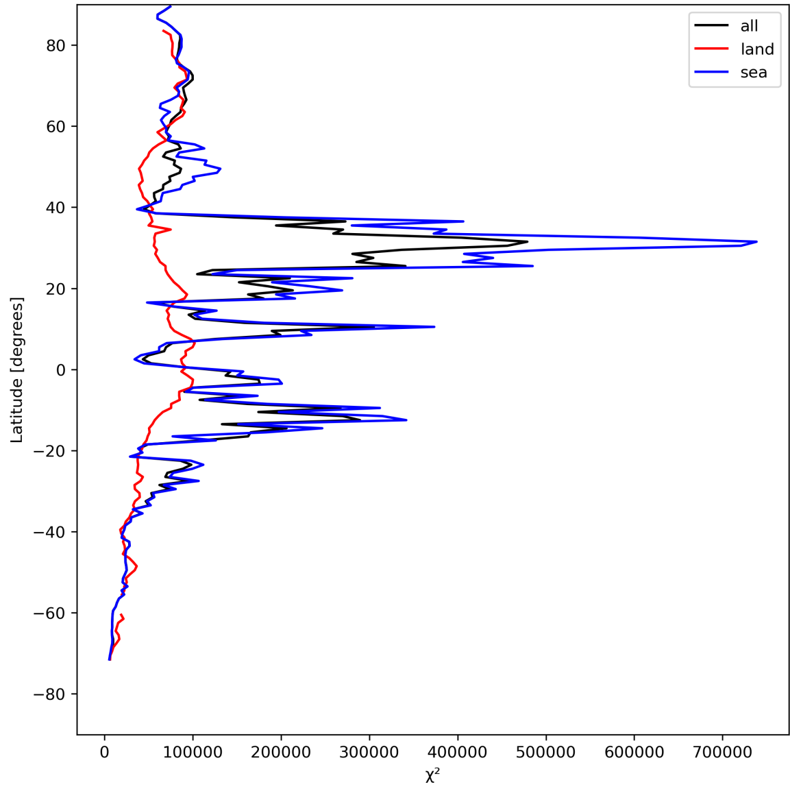
Figure 21: Zonal average of “ \chi^2 ” for 2024-05-03 to 2024-05-05.
