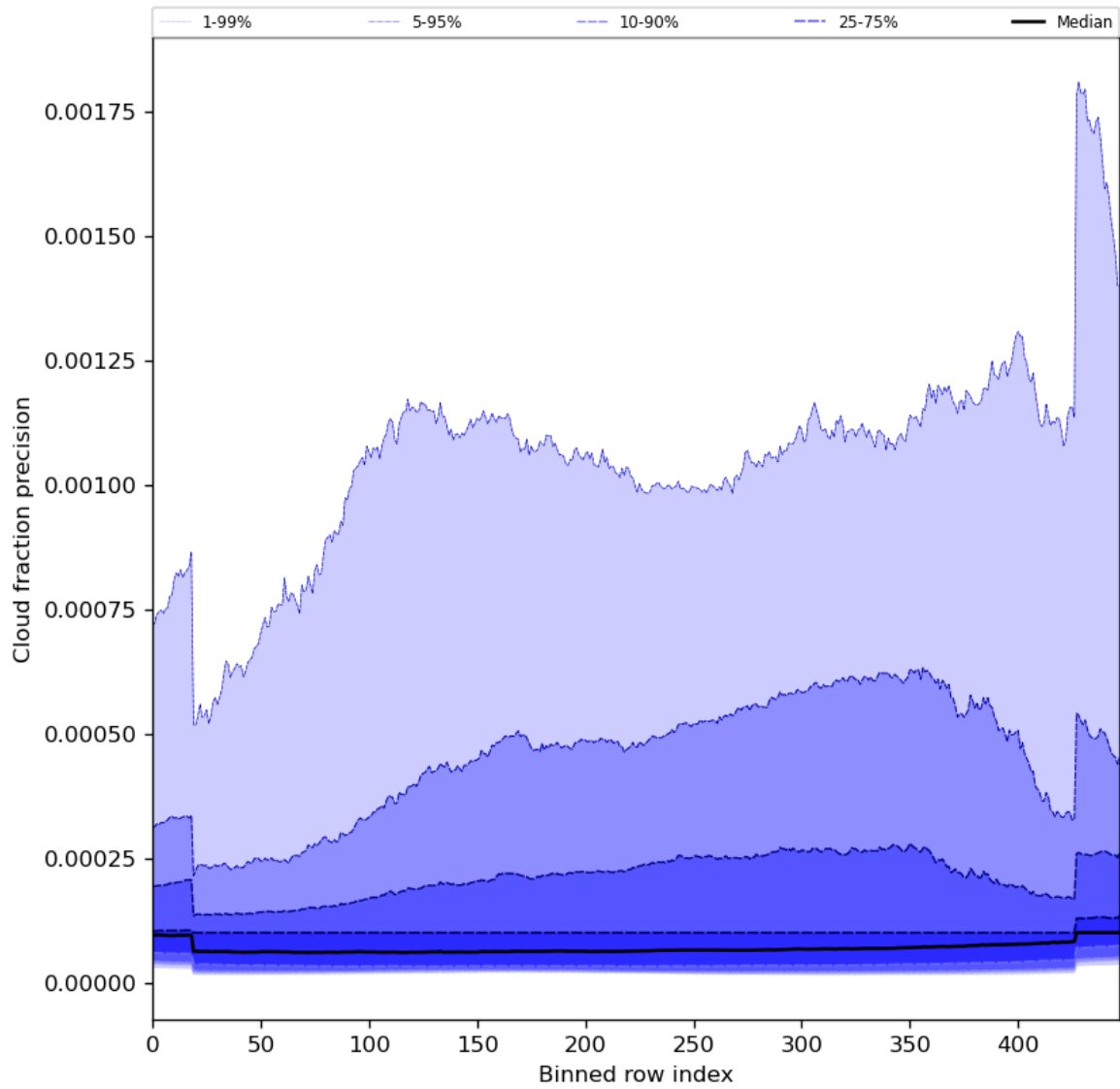
Figure 50: Along track statistics of “Cloud fraction precision” for 2024-05-03 to 2024-05-05
