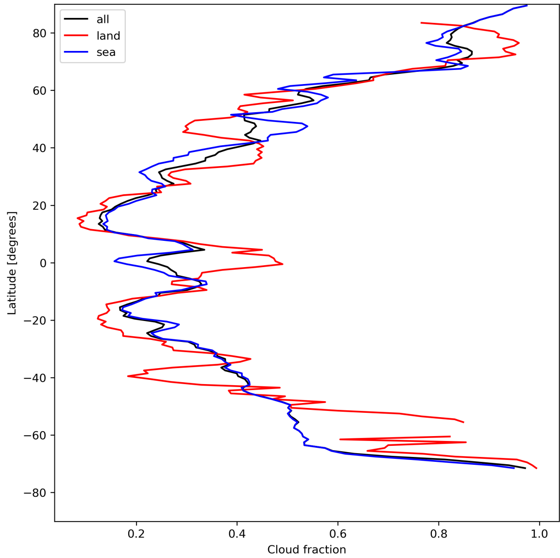
Figure 15: Zonal average of “Cloud fraction” for 2024-05-03 to 2024-05-05.
