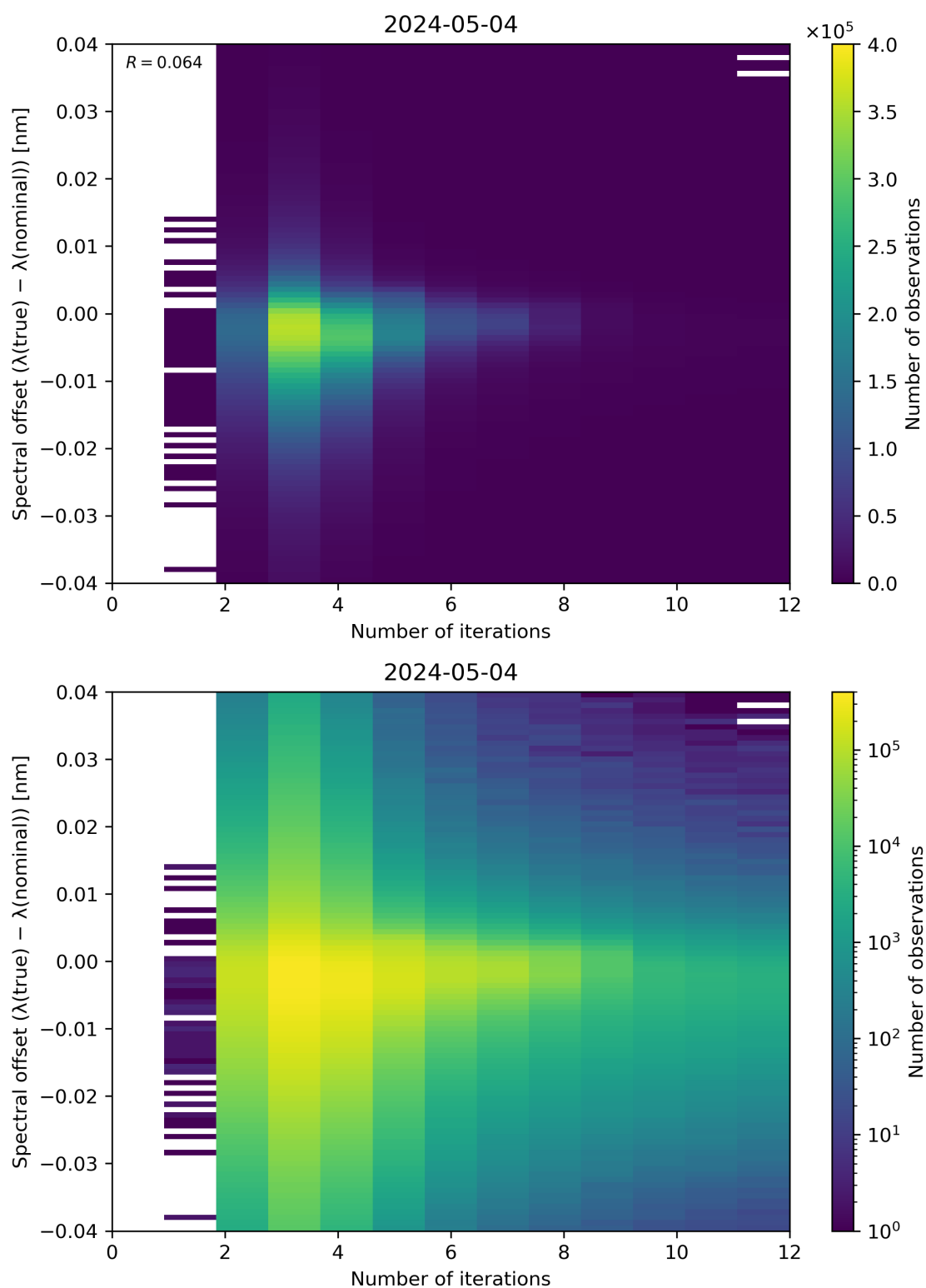
Figure 100: Scatter density plot of “Number of iterations” against “Spectral offset ( \lambda(\text{true}) - \lambda(\text{nominal}) )” for 2024-05-03 to 2024-05-05.
