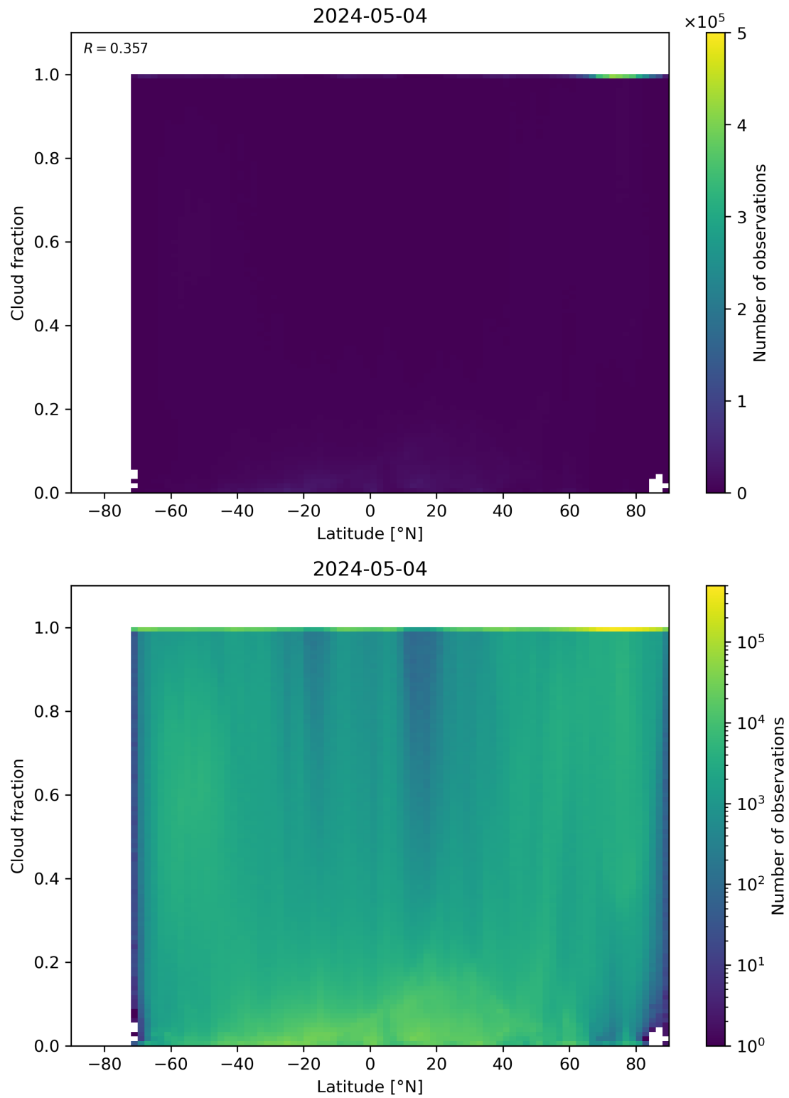
Figure 90: Scatter density plot of “Latitude” against “Cloud fraction” for 2024-05-03 to 2024-05-05.
