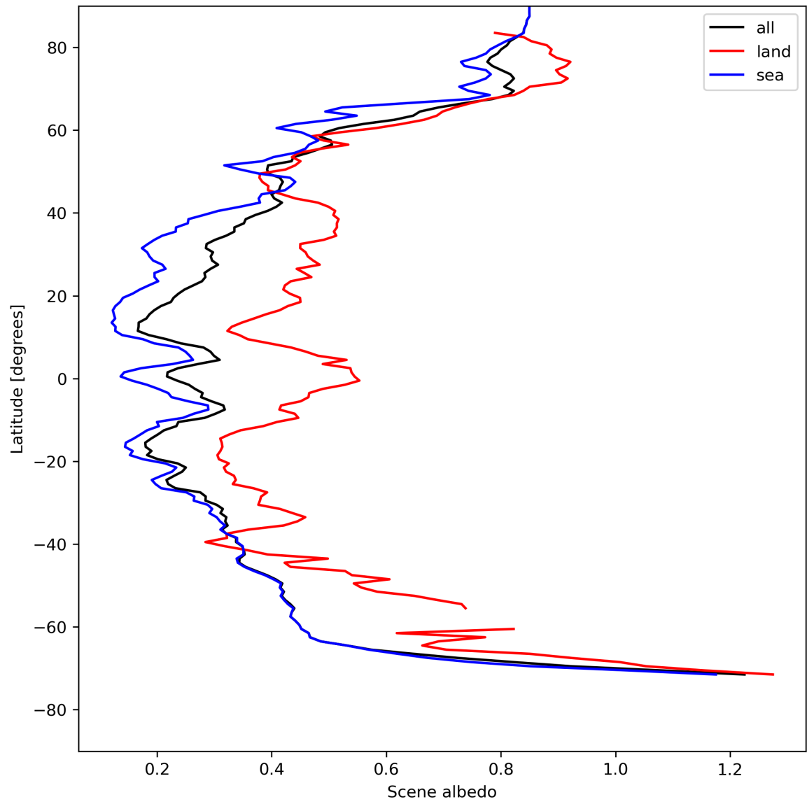
Figure 17: Zonal average of “Scene albedo” for 2024-05-03 to 2024-05-05.
