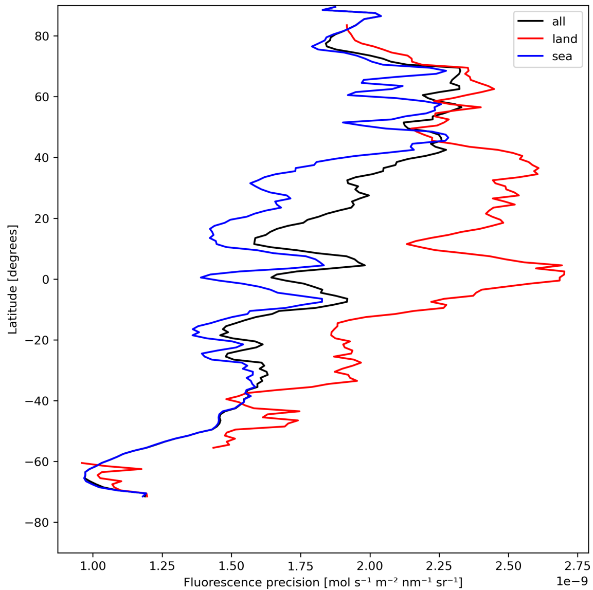
Figure 24: Zonal average of “Fluorescence precision” for 2024-05-03 to 2024-05-05.
