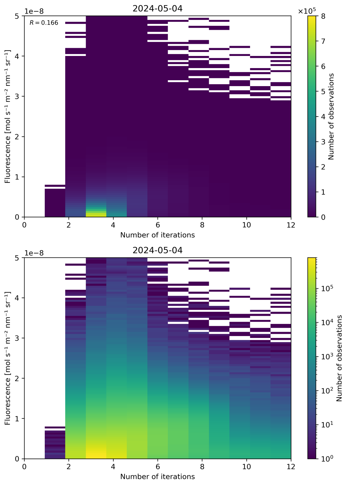
Figure 98: Scatter density plot of “Number of iterations” against “Fluorescence” for 2024-05-03 to 2024-05-05.
