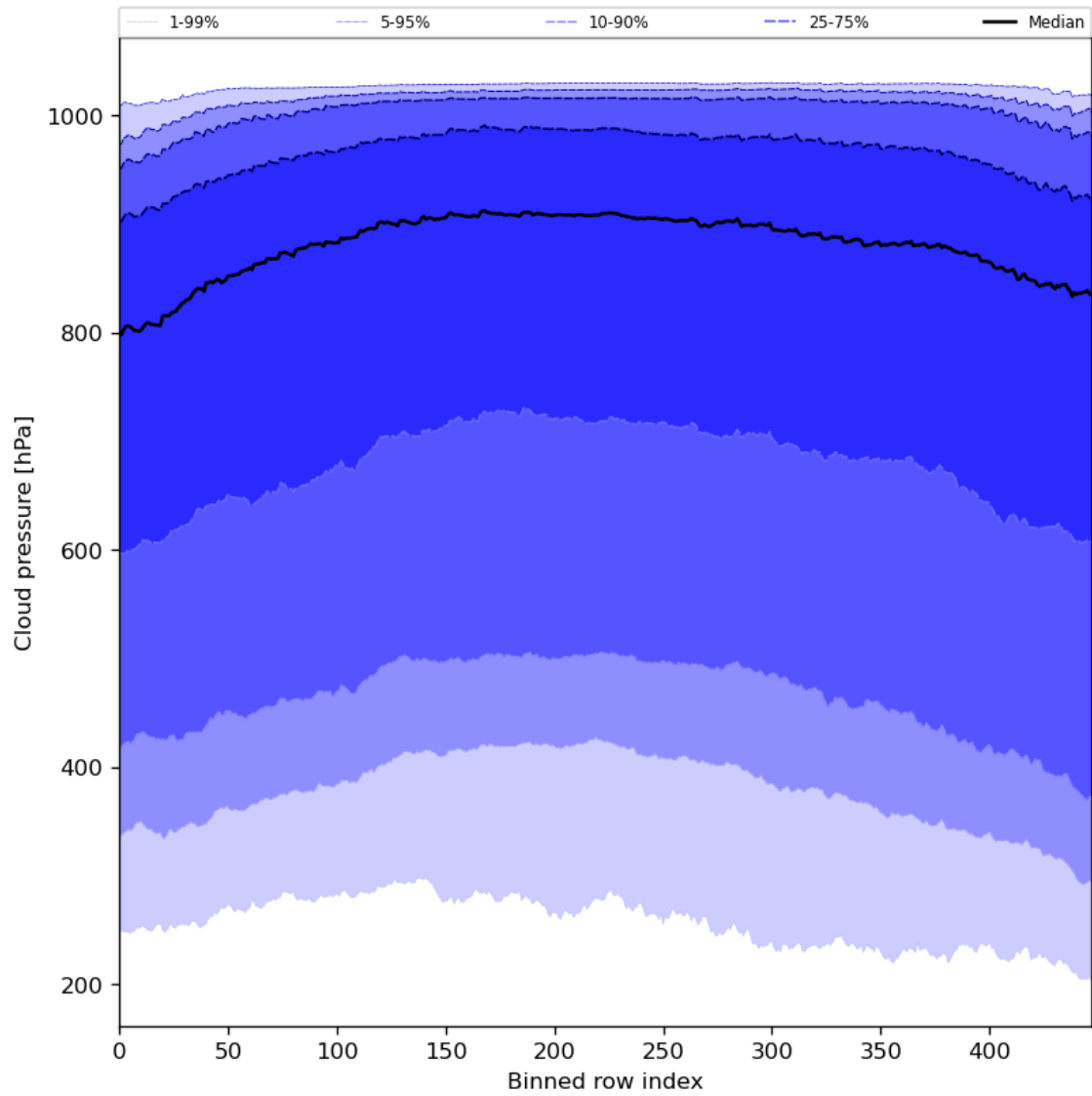
Figure 47: Along track statistics of “Cloud pressure” for 2024-05-03 to 2024-05-05
