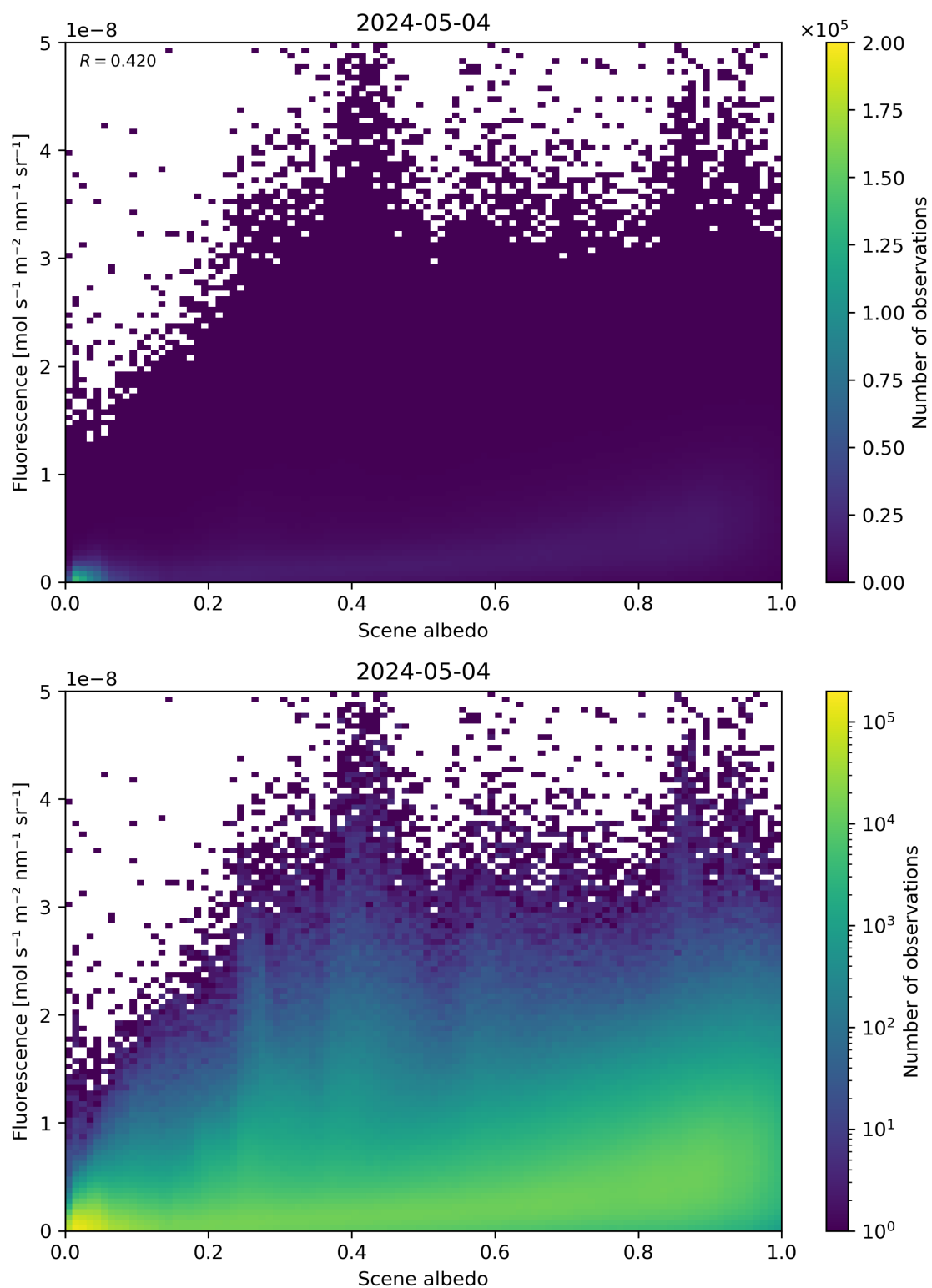
Figure 104: Scatter density plot of “Scene albedo” against “Fluorescence” for 2024-05-03 to 2024-05-05.
