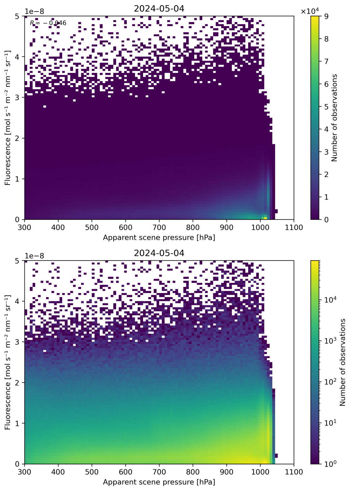
Figure 64: Scatter density plot of “Apparent scene pressure” against “Fluorescence” for 2024-05-03 to 2024-05-05.
