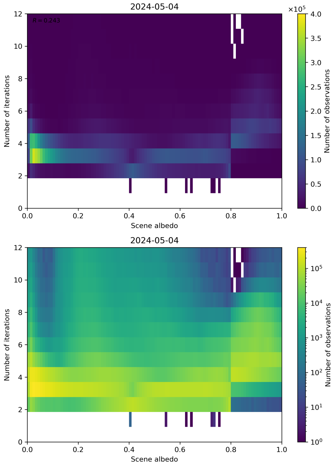
Figure 105: Scatter density plot of “Scene albedo” against “Number of iterations” for 2024-05-03 to 2024-05-05.
