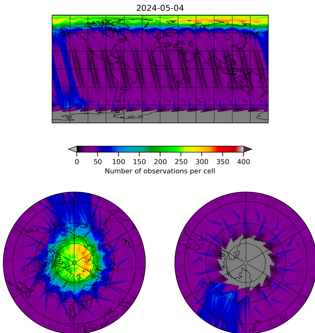
Figure 11: Map of the number of observations for 2024-05-03 to 2024-05-05
