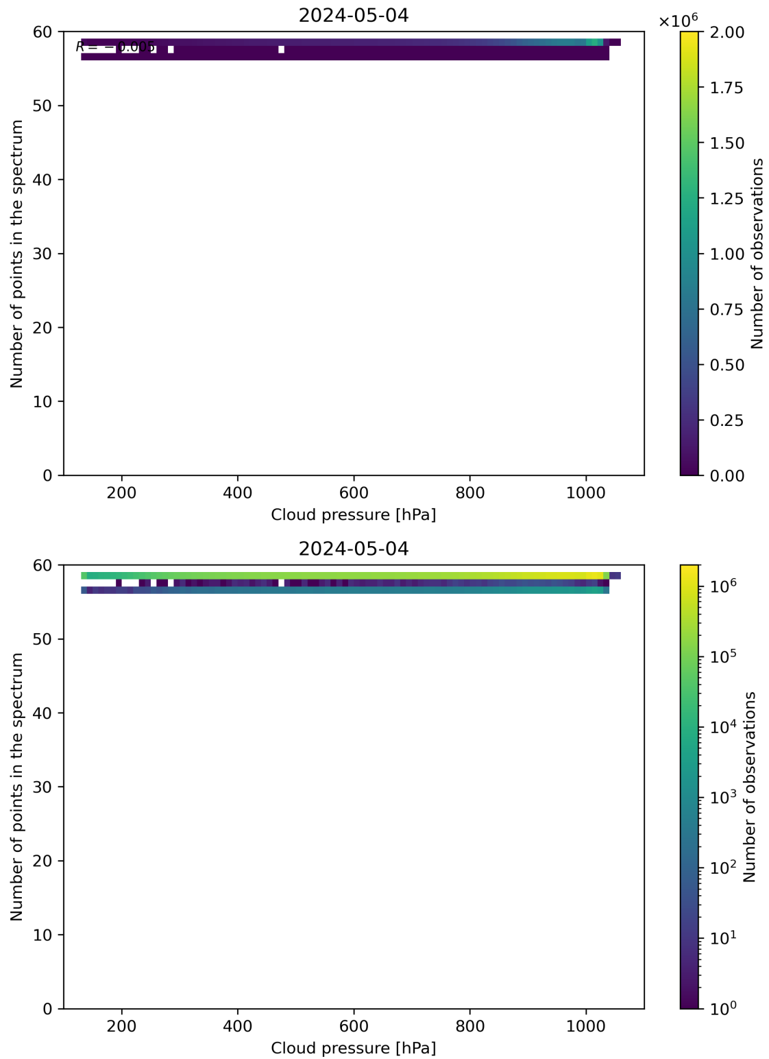
Figure 82: Scatter density plot of “Cloud pressure” against “Number of points in the spectrum” for 2024-05-03 to 2024-05-05.
