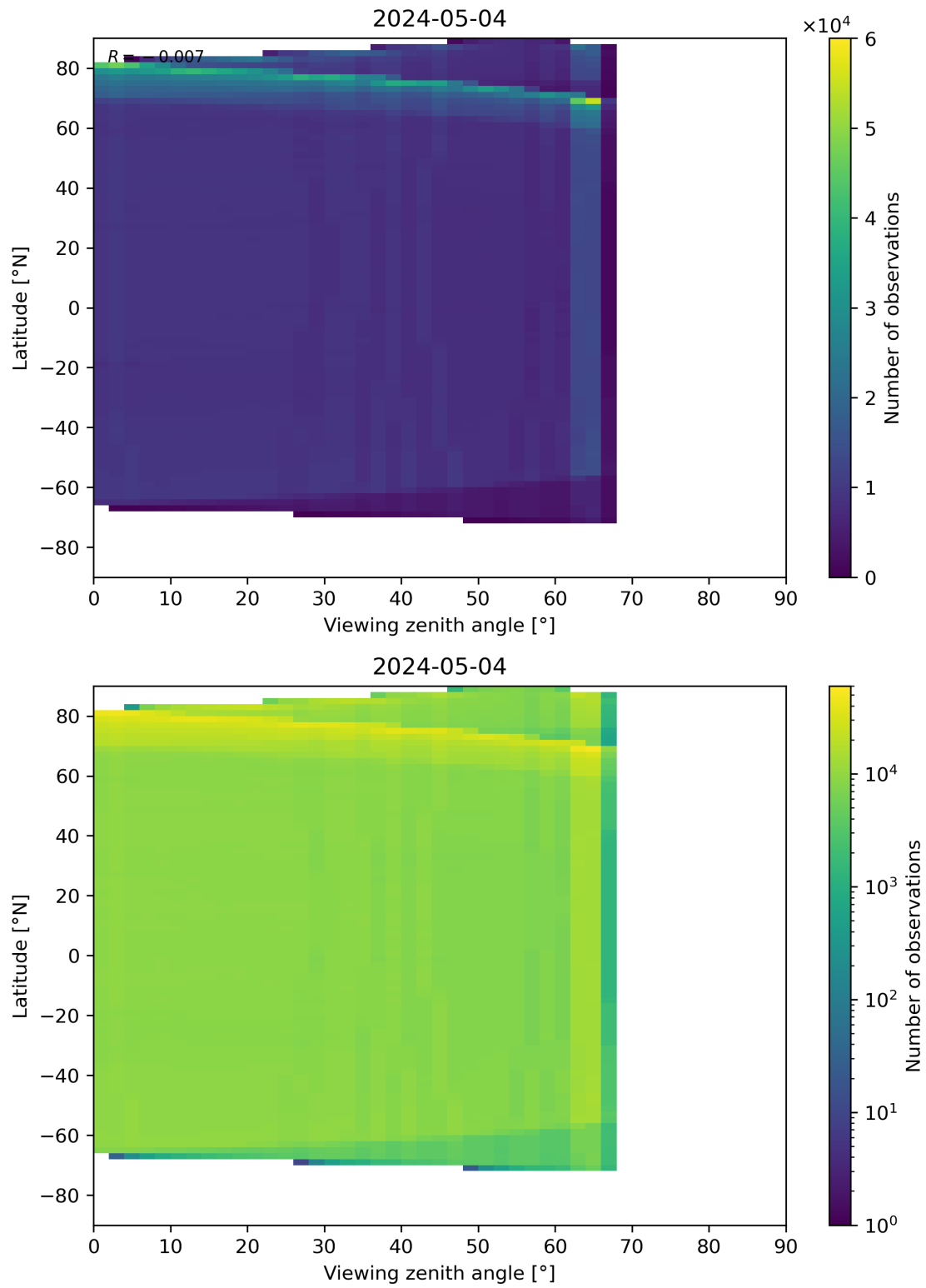
Figure 123: Scatter density plot of “Viewing zenith angle” against “Latitude” for 2024-05-03 to 2024-05-05.
