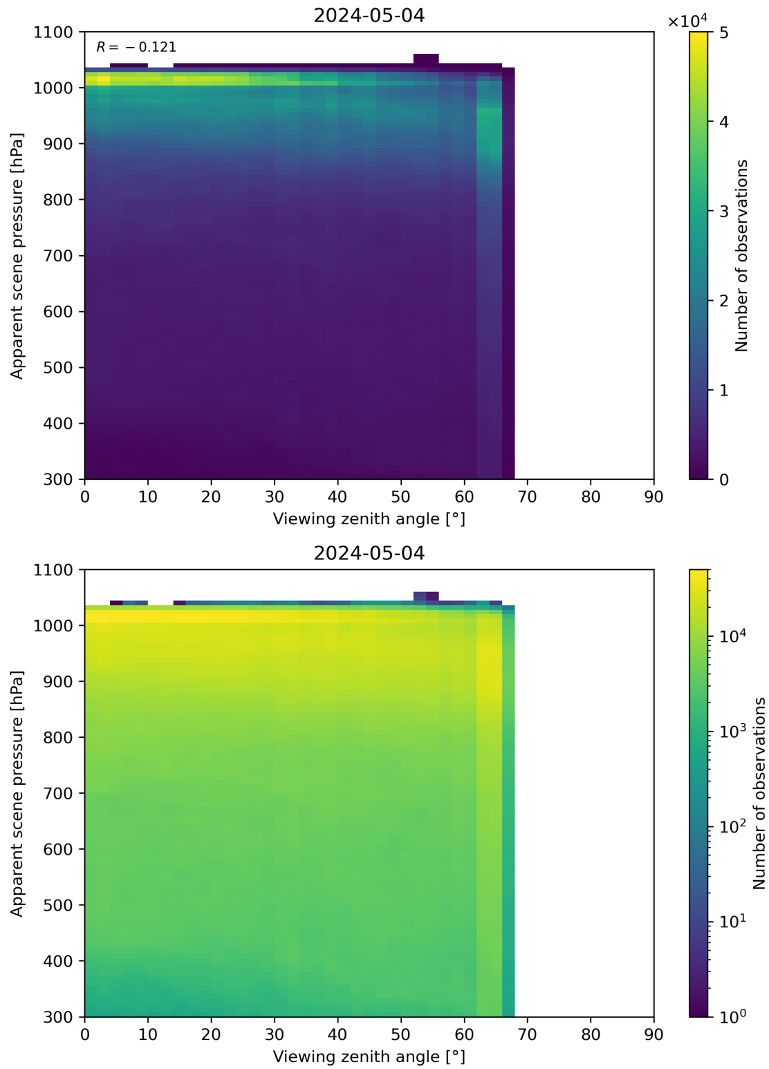
Figure 118: Scatter density plot of “Viewing zenith angle” against “Apparent scene pressure” for 2024-05-03 to 2024-05-05.
