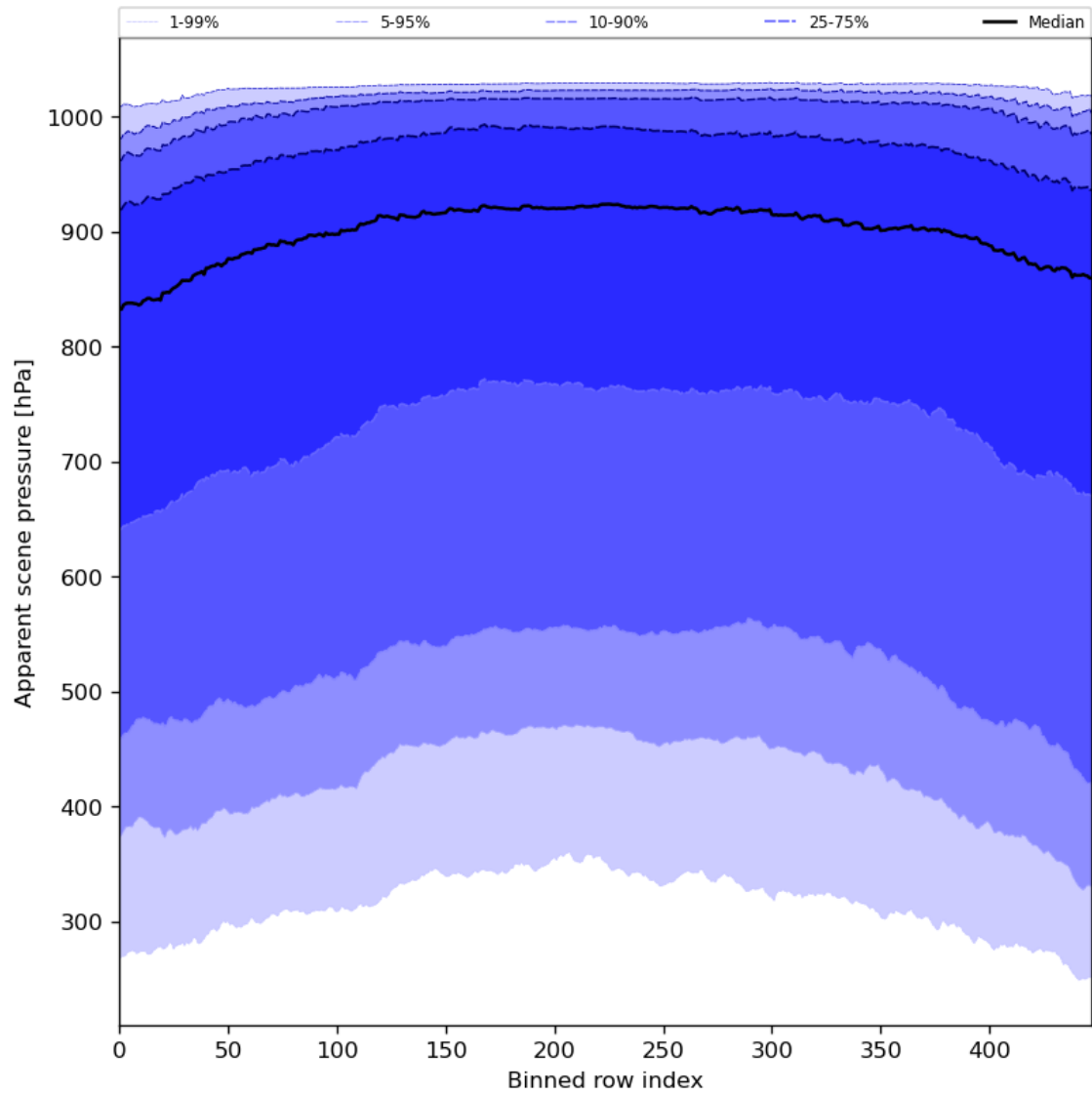
Figure 53: Along track statistics of “Apparent scene pressure” for 2024-05-03 to 2024-05-05
