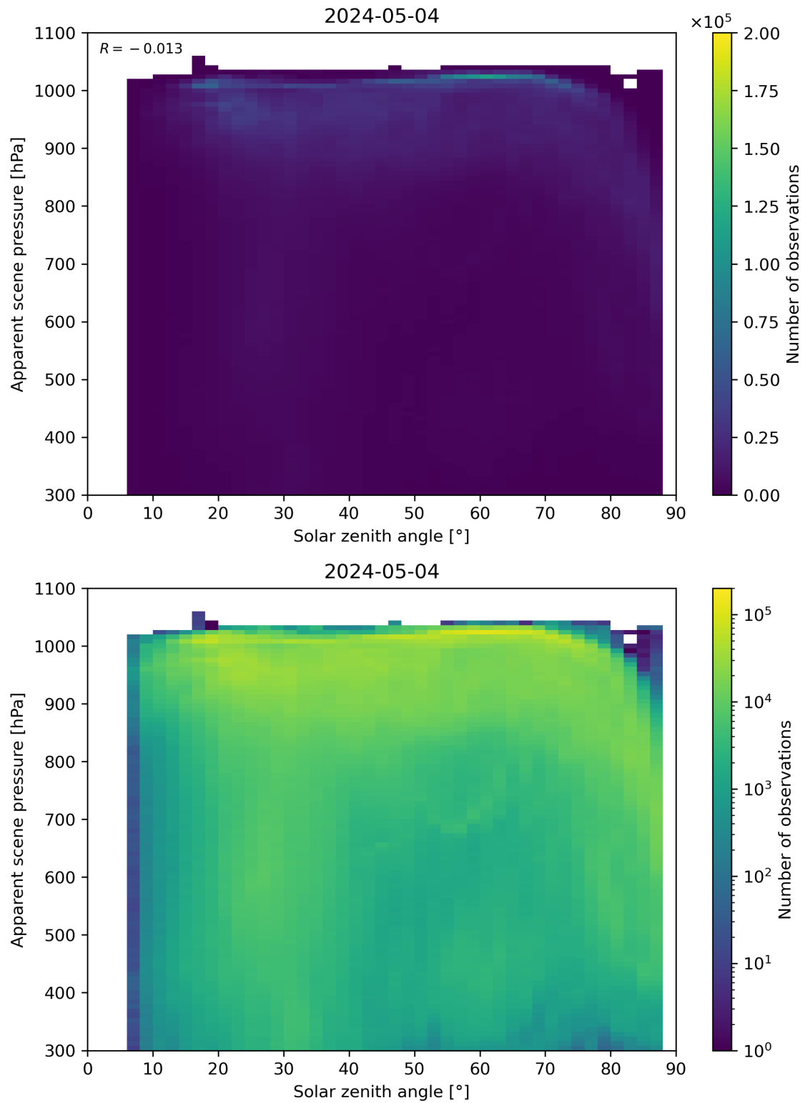
Figure 108: Scatter density plot of “Solar zenith angle” against “Apparent scene pressure” for 2024-05-03 to 2024-05-05.
