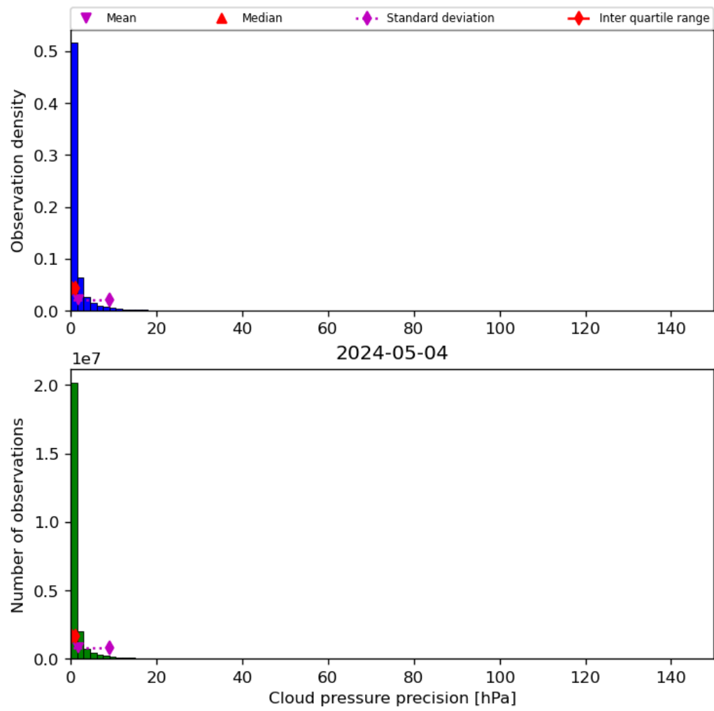
Figure 31: Histogram of “Cloud pressure precision” for 2024-05-03 to 2024-05-05
