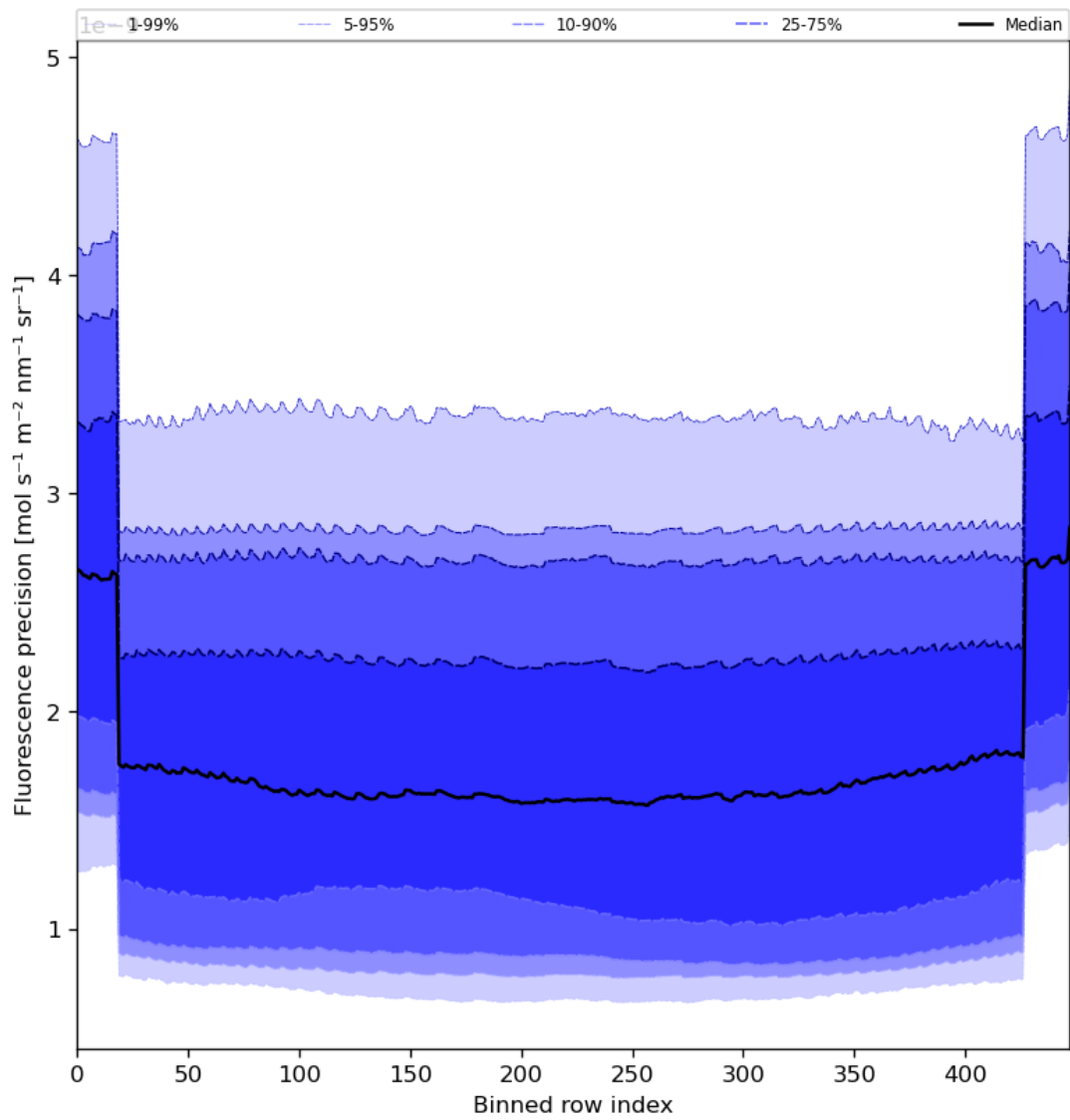
Figure 58: Along track statistics of “Fluorescence precision” for 2024-05-03 to 2024-05-05
