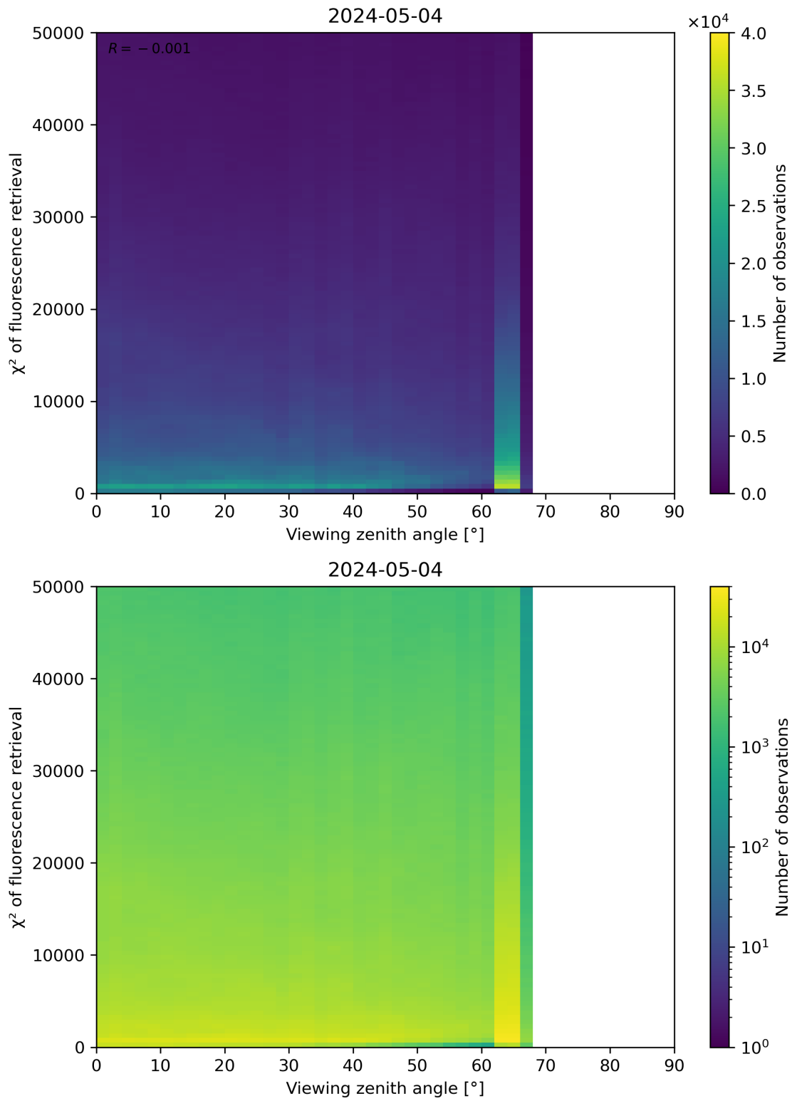
Figure 119: Scatter density plot of “Viewing zenith angle” against “ \chi^2 of fluorescence retrieval” for 2024-05-03 to 2024-05-05.
