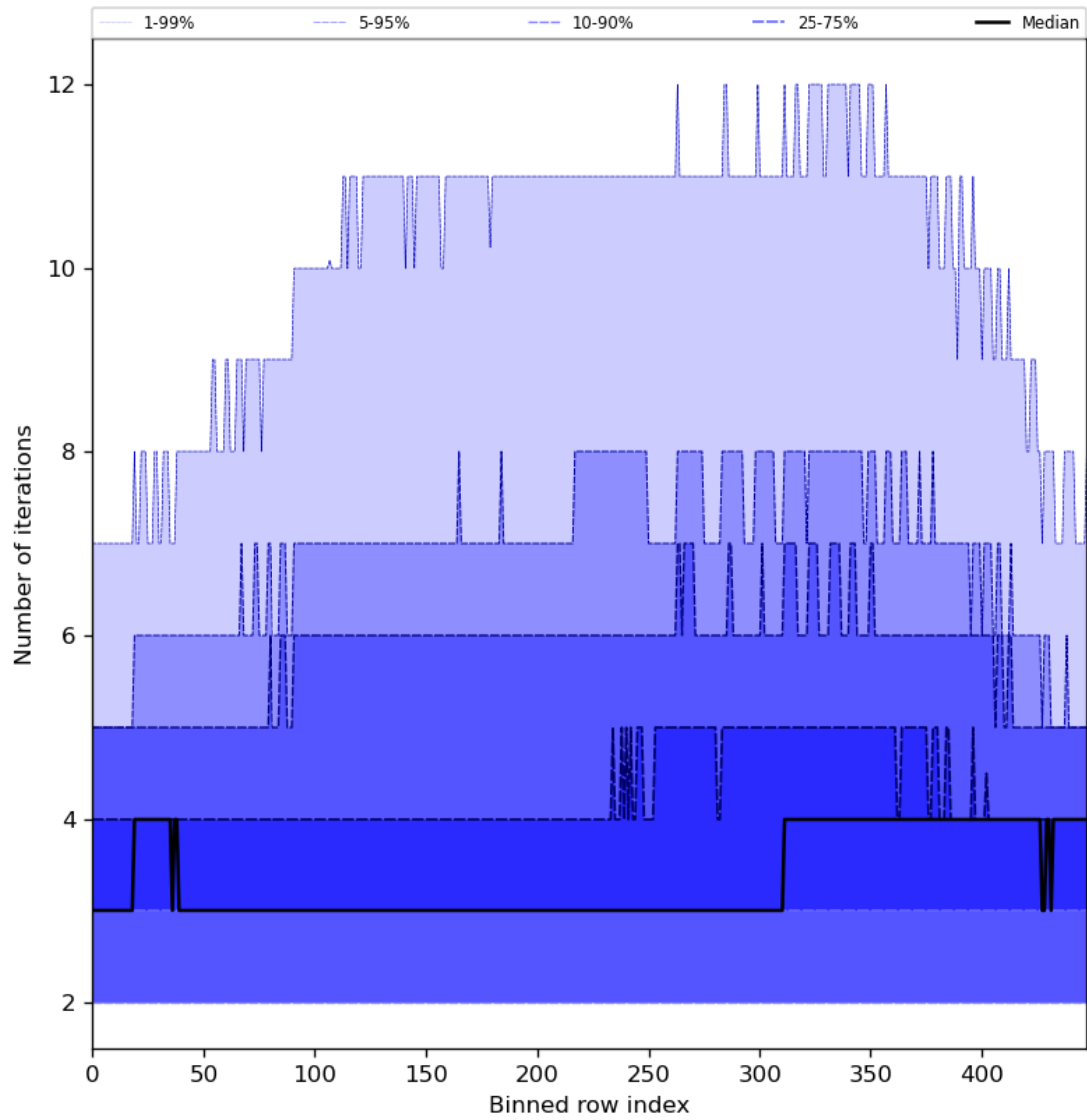
Figure 56: Along track statistics of “Number of iterations” for 2024-05-03 to 2024-05-05
