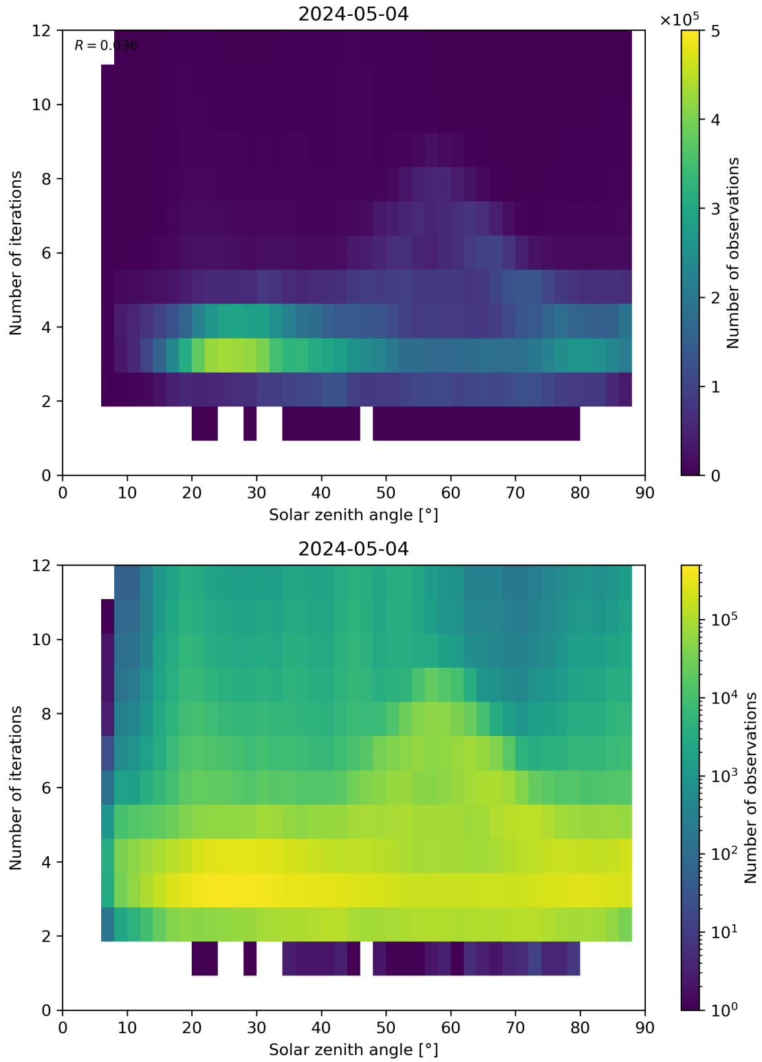
Figure 114: Scatter density plot of “Solar zenith angle” against “Number of iterations” for 2024-05-03 to 2024-05-05.
