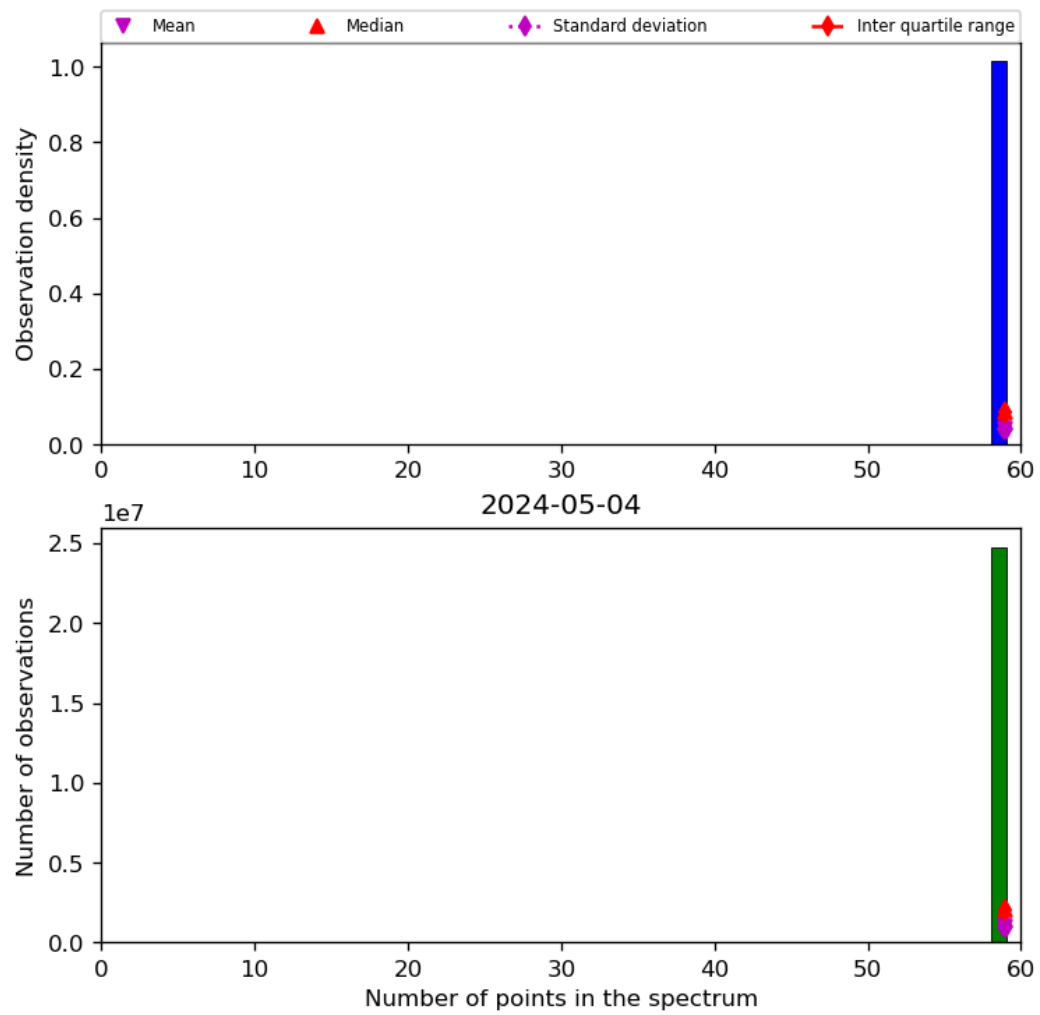
Figure 44: Histogram of “Number of points in the spectrum” for 2024-05-03 to 2024-05-05
