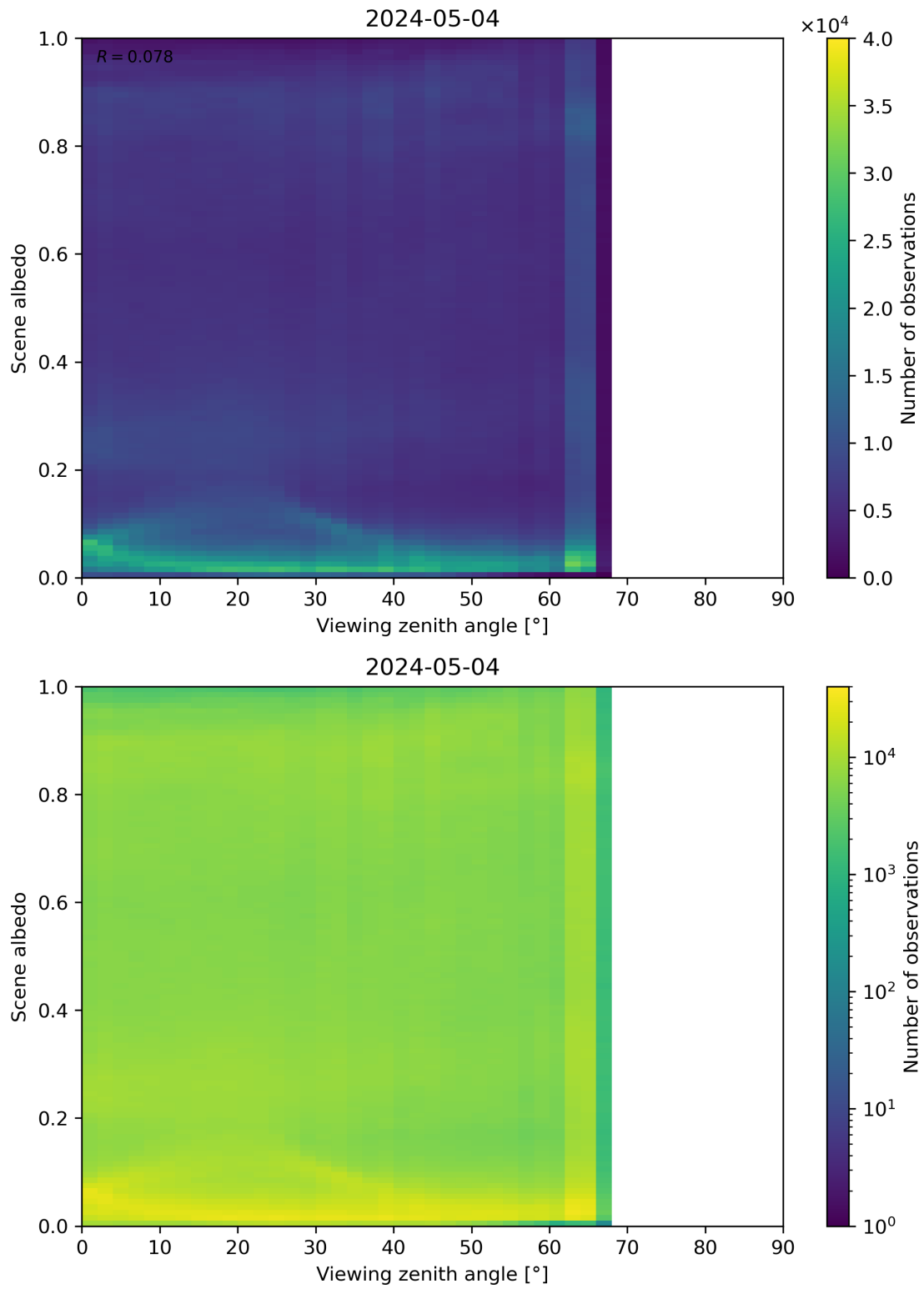
Figure 126: Scatter density plot of “Viewing zenith angle” against “Scene albedo” for 2024-05-03 to 2024-05-05.
