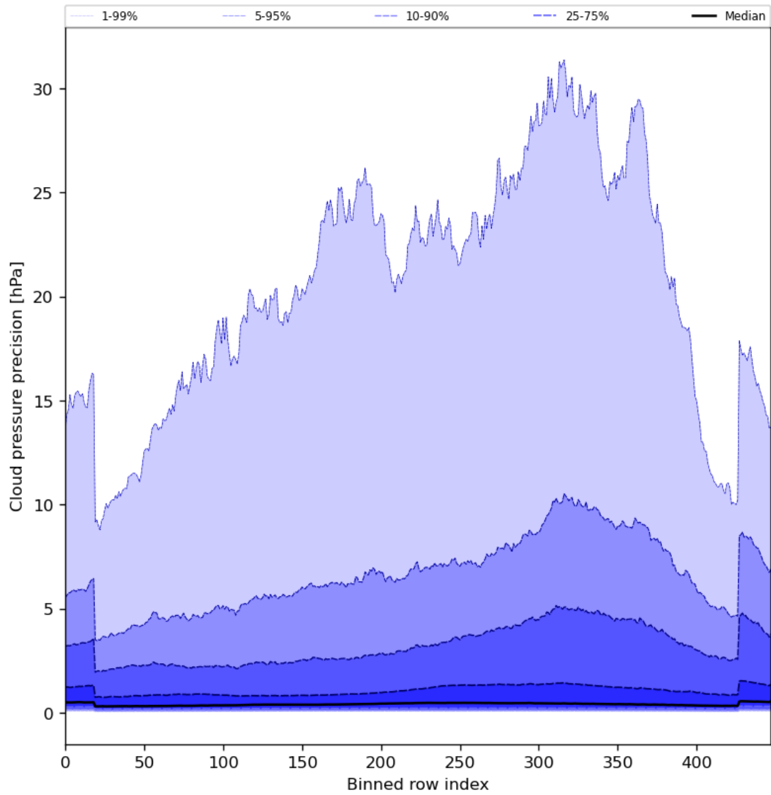
Figure 48: Along track statistics of “Cloud pressure precision” for 2024-05-03 to 2024-05-05
