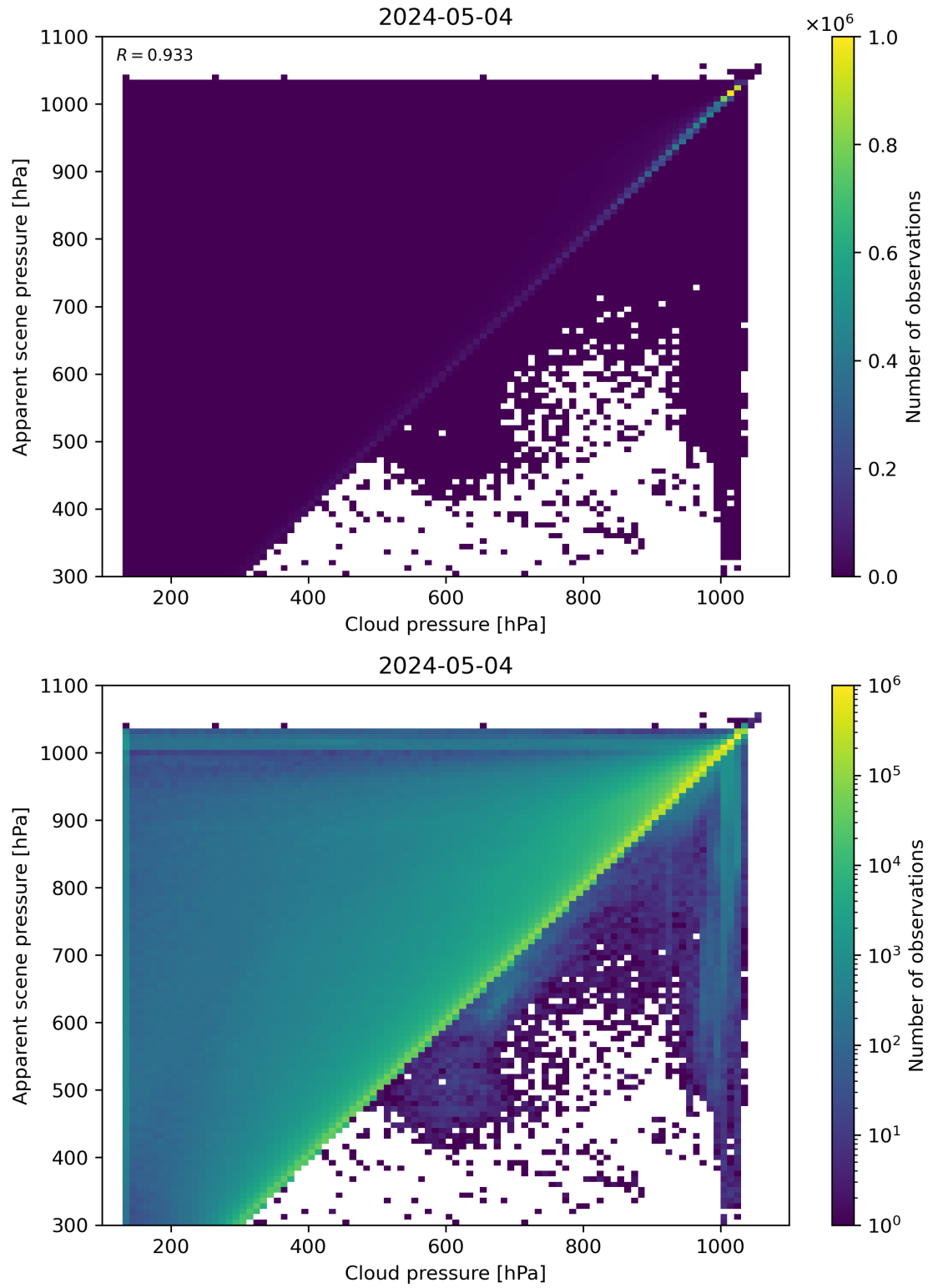
Figure 77: Scatter density plot of “Cloud pressure” against “Apparent scene pressure” for 2024-05-03 to 2024-05-05.
