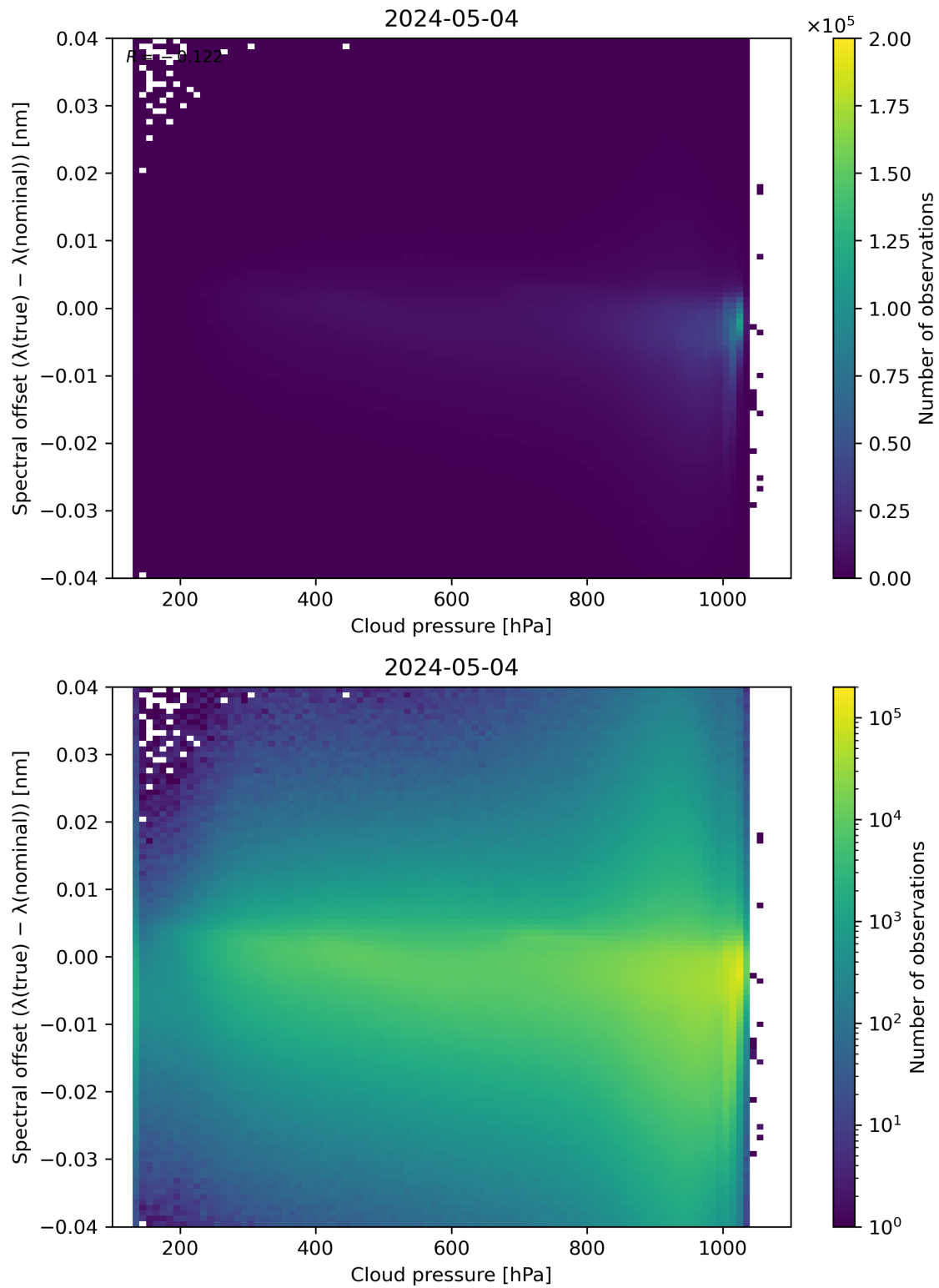
Figure 84: Scatter density plot of “Cloud pressure” against “Spectral offset ( \lambda(\text{true}) - \lambda(\text{nominal}) )” for 2024-05-03 to 2024-05-05.
