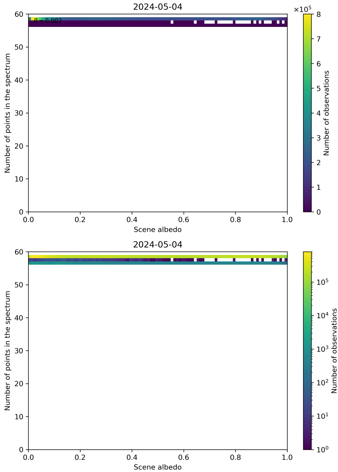
Figure 106: Scatter density plot of “Scene albedo” against “Number of points in the spectrum” for 2024-05-03 to 2024-05-05.
