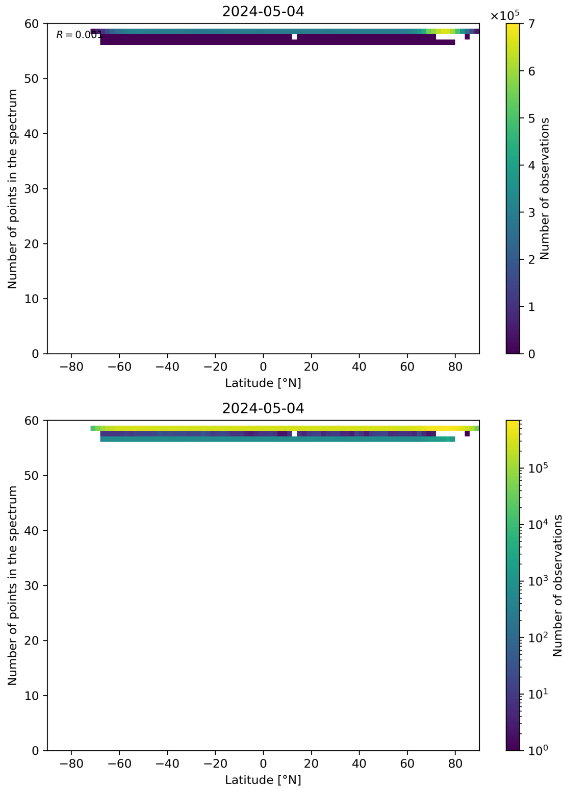
Figure 94: Scatter density plot of “Latitude” against “Number of points in the spectrum” for 2024-05-03 to 2024-05-05.
