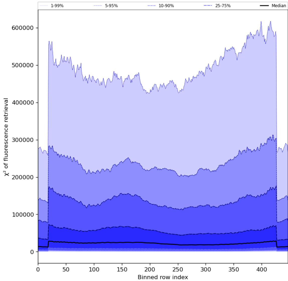
Figure 59: Along track statistics of “ \chi^2 of fluorescence retrieval” for 2024-05-03 to 2024-05-05
