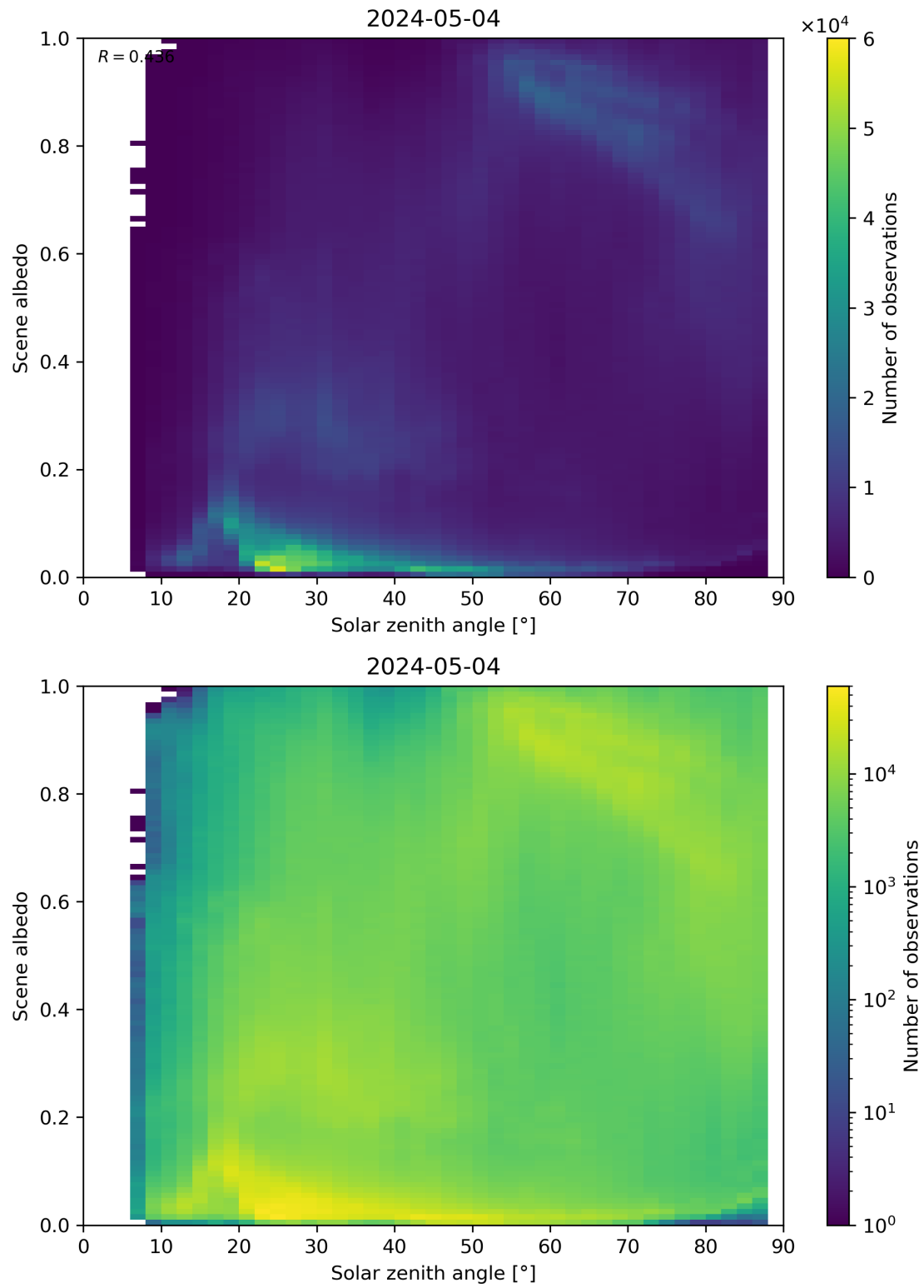
Figure 116: Scatter density plot of “Solar zenith angle” against “Scene albedo” for 2024-05-03 to 2024-05-05.
