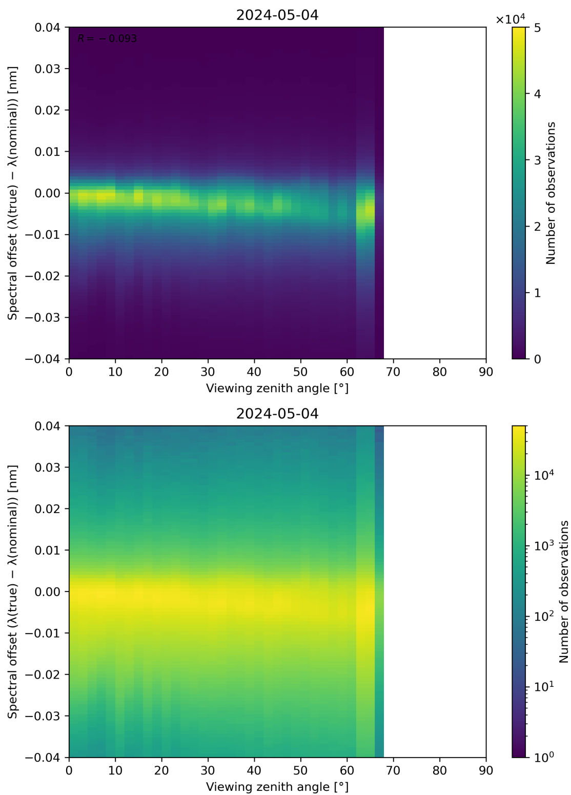
Figure 128: Scatter density plot of “Viewing zenith angle” against “Spectral offset ( \lambda(\text{true}) - \lambda(\text{nominal}) )” for 2024-05-03 to 2024-05-05.
