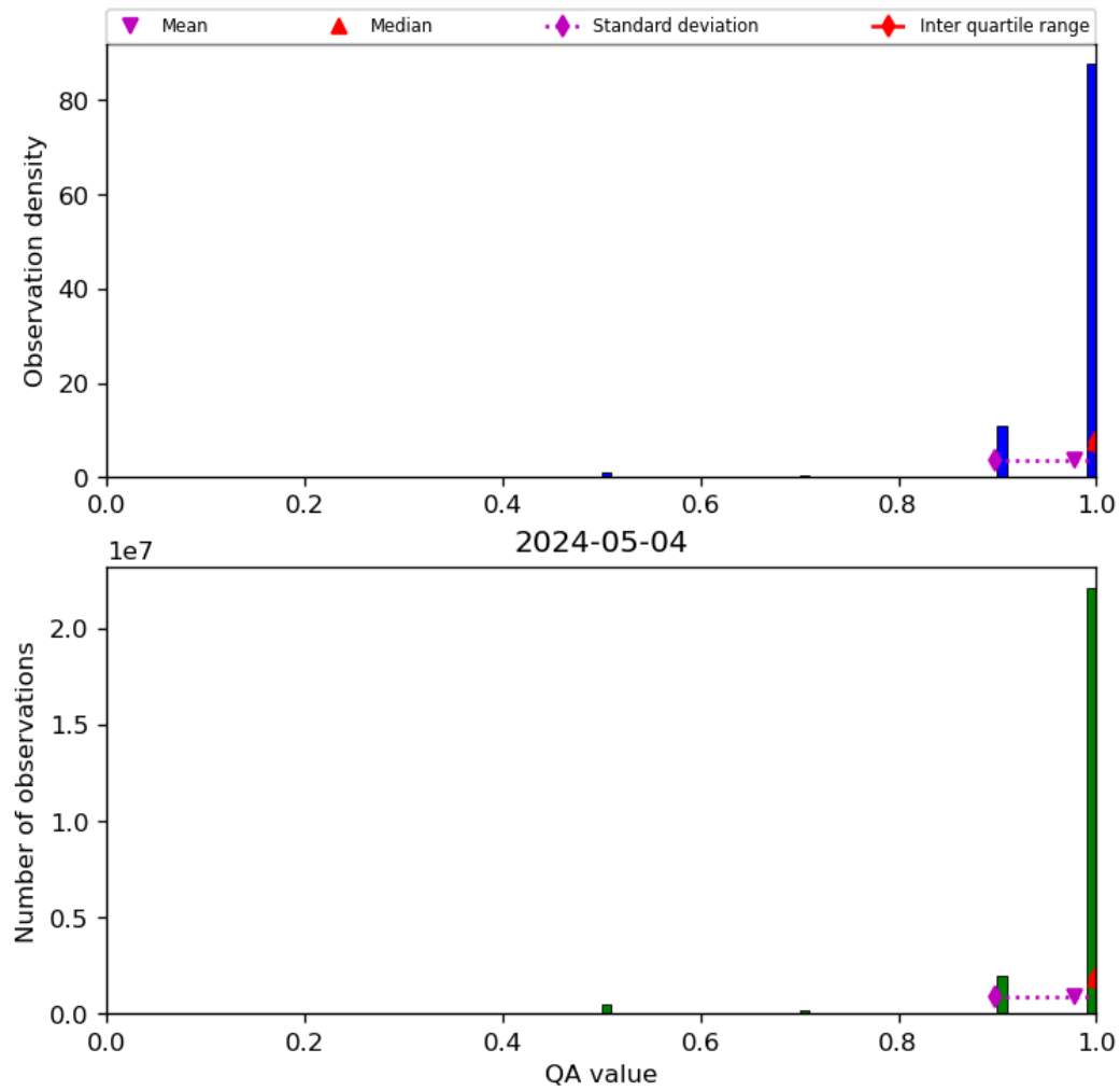
Figure 29: Histogram of “QA value” for 2024-05-03 to 2024-05-05
