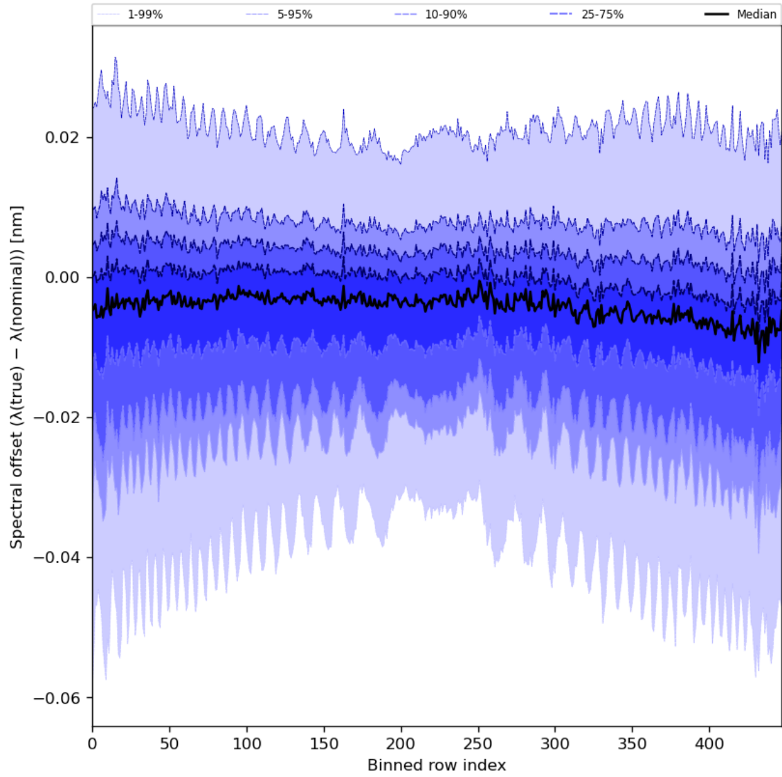
Figure 62: Along track statistics of “Spectral offset ( \lambda(\text{true}) - \lambda(\text{nominal}) )” for 2024-05-03 to 2024-05-05
