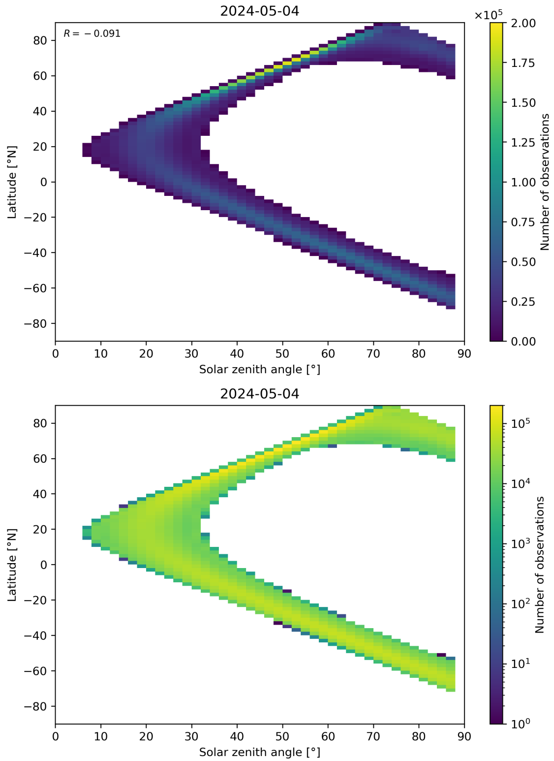
Figure 113: Scatter density plot of “Solar zenith angle” against “Latitude” for 2024-05-03 to 2024-05-05.
