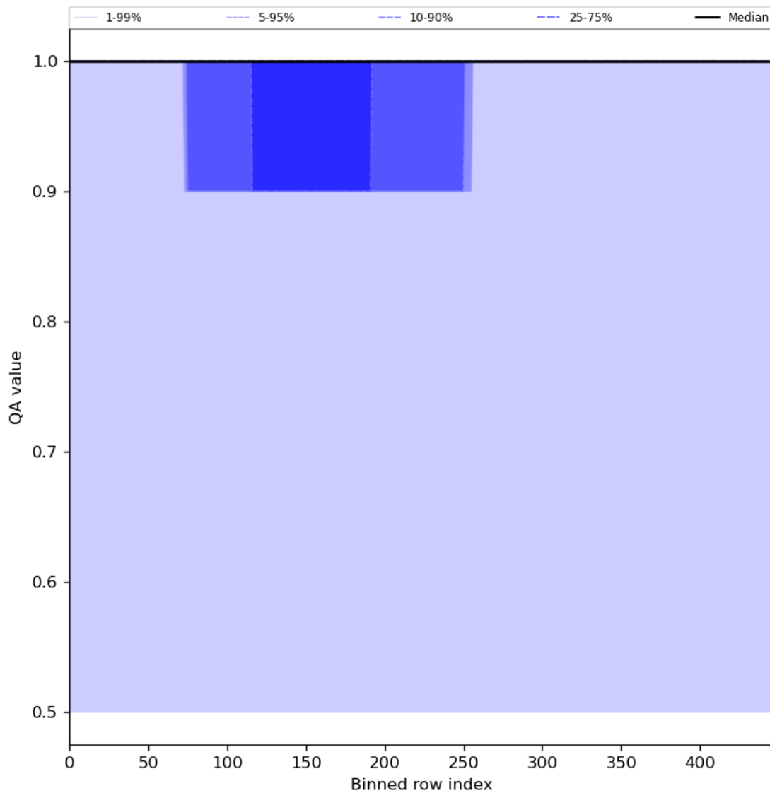
Figure 46: Along track statistics of “QA value” for 2024-05-03 to 2024-05-05
