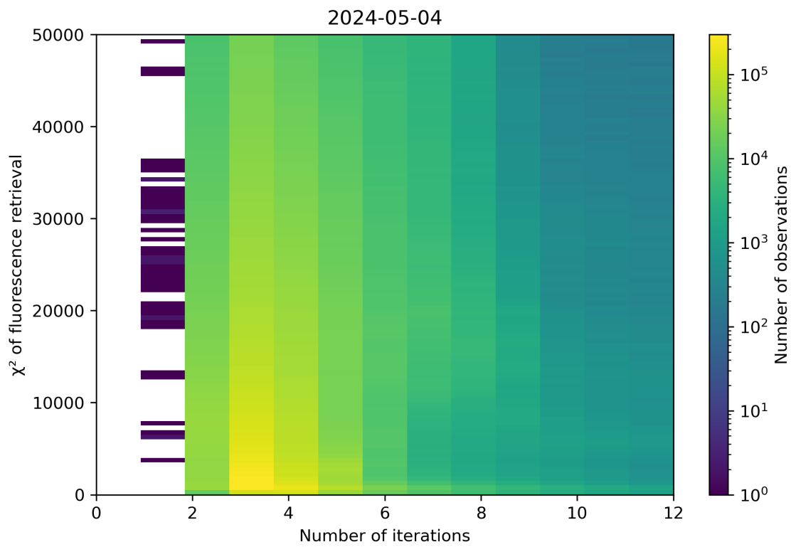
Figure 97: Scatter density plot of “Number of iterations” against “ \chi^2 of fluorescence retrieval” for 2024-05-03 to 2024-05-05.
