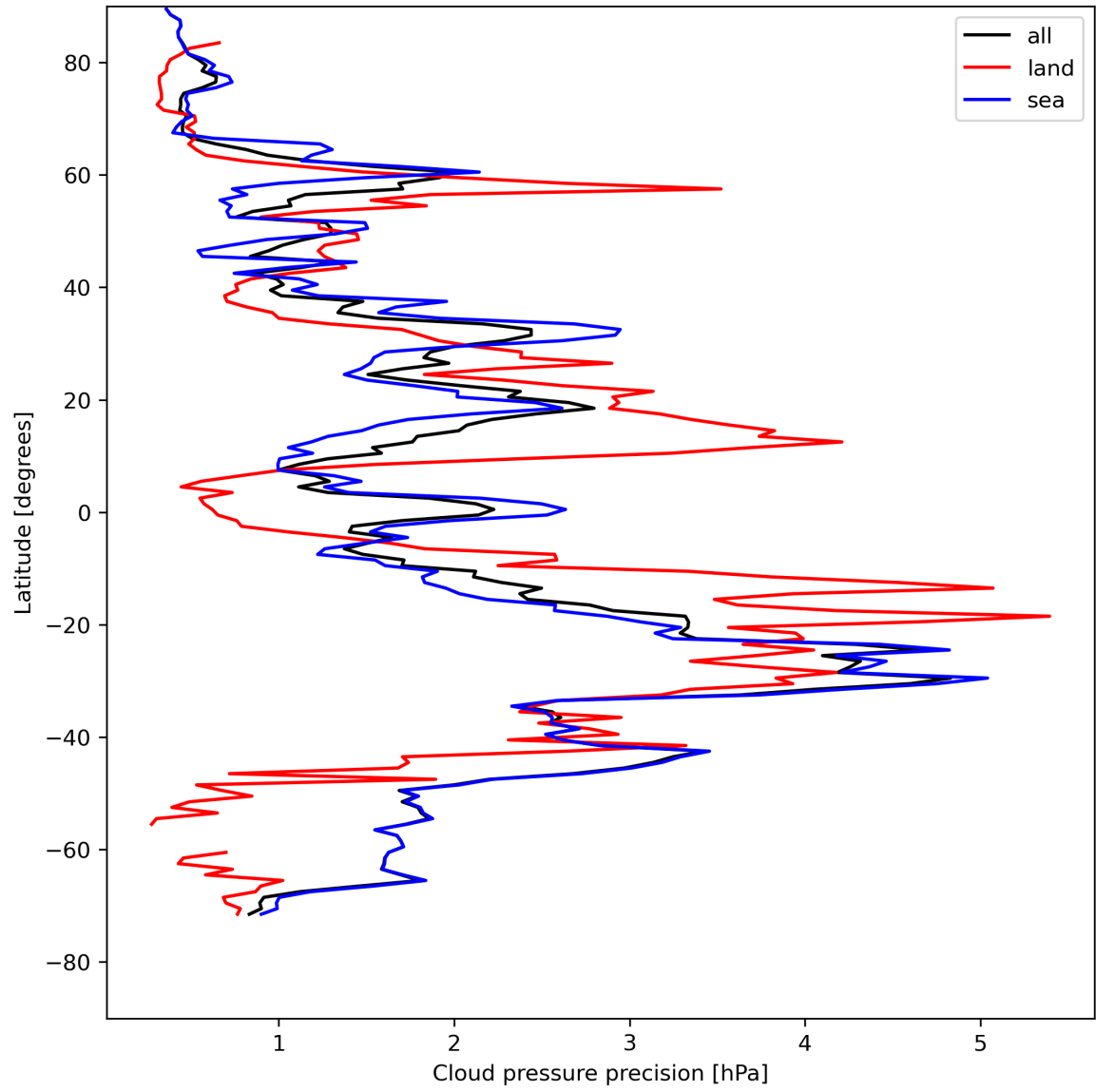
Figure 14: Zonal average of “Cloud pressure precision” for 2024-05-03 to 2024-05-05.
