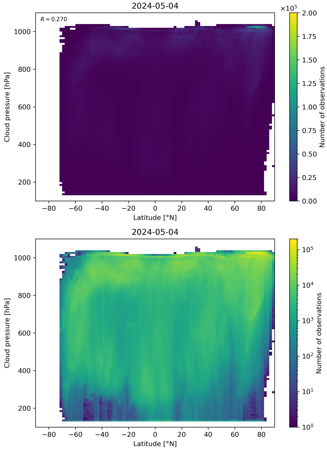
Figure 91: Scatter density plot of “Latitude” against “Cloud pressure” for 2024-05-03 to 2024-05-05.
