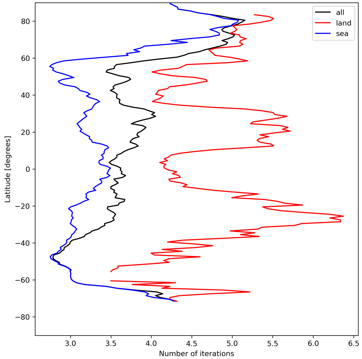
Figure 22: Zonal average of “Number of iterations” for 2024-05-03 to 2024-05-05.
