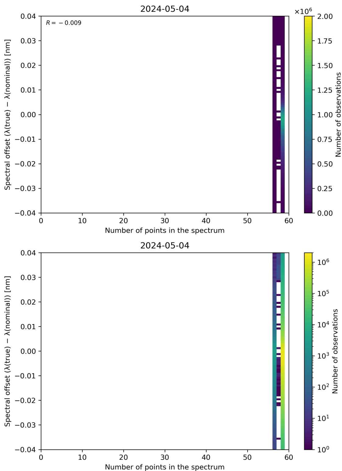
Figure 101: Scatter density plot of “Number of points in the spectrum” against “Spectral offset ( \lambda(\text{true}) - \lambda(\text{nominal}) )” for 2024-05-03 to 2024-05-05.
