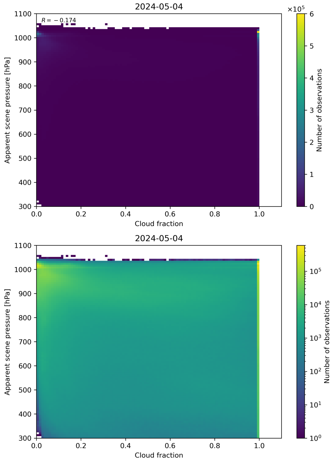
Figure 70: Scatter density plot of “Cloud fraction” against “Apparent scene pressure” for 2024-05-03 to 2024-05-05.
