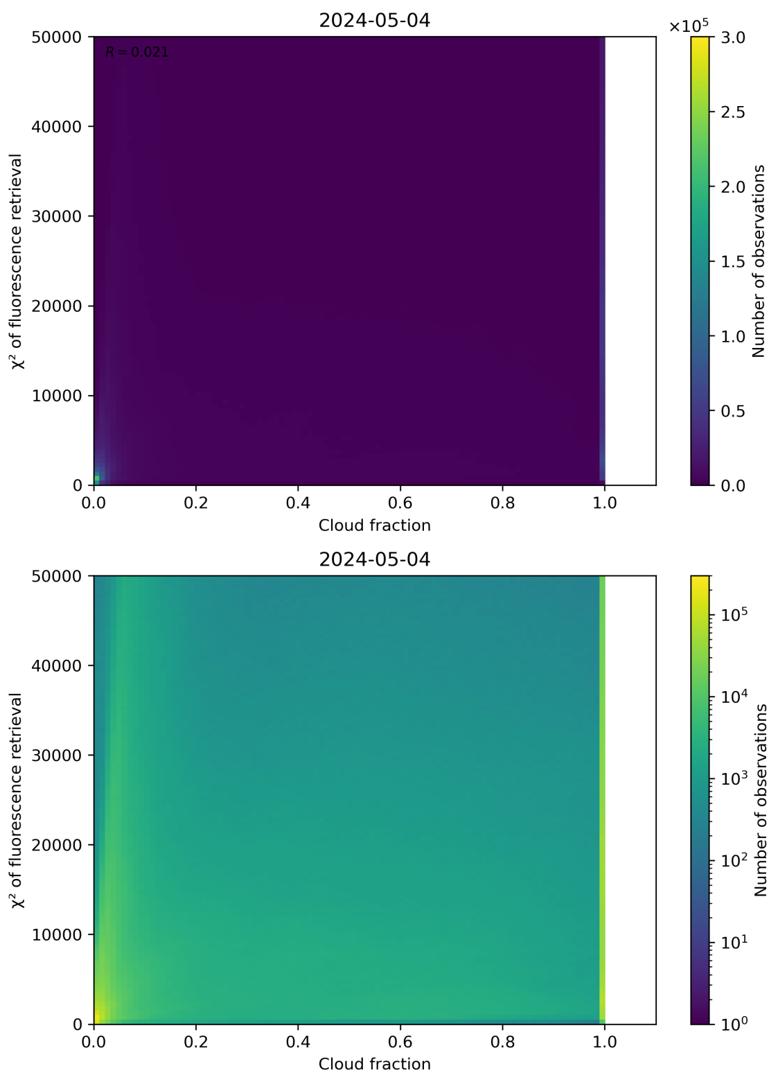
Figure 71: Scatter density plot of “Cloud fraction” against “ \chi^2 of fluorescence retrieval” for 2024-05-03 to 2024-05-05.
