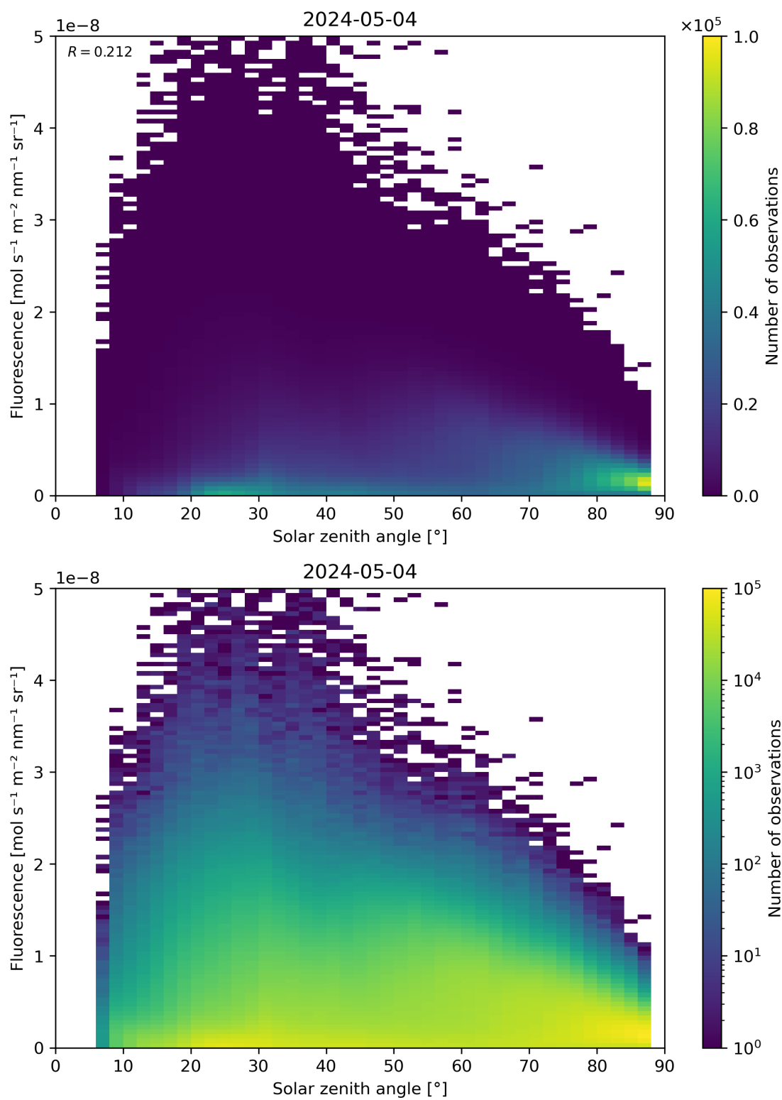
Figure 112: Scatter density plot of “Solar zenith angle” against “Fluorescence” for 2024-05-03 to 2024-05-05.
