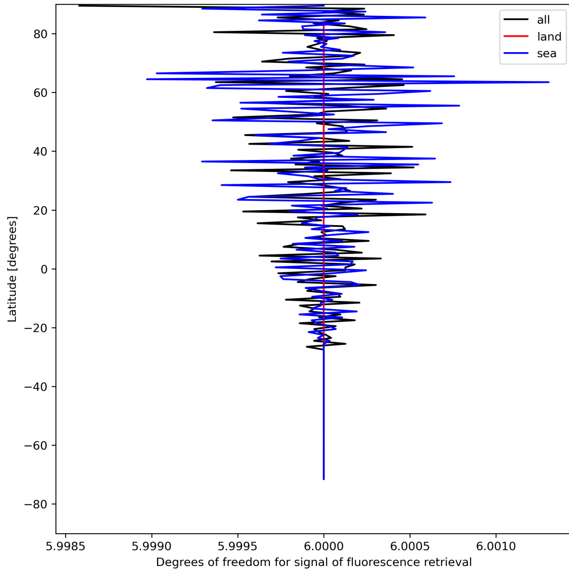
Figure 26: Zonal average of “Degrees of freedom for signal of fluorescence retrieval” for 2024-05-03 to 2024-05-05.
