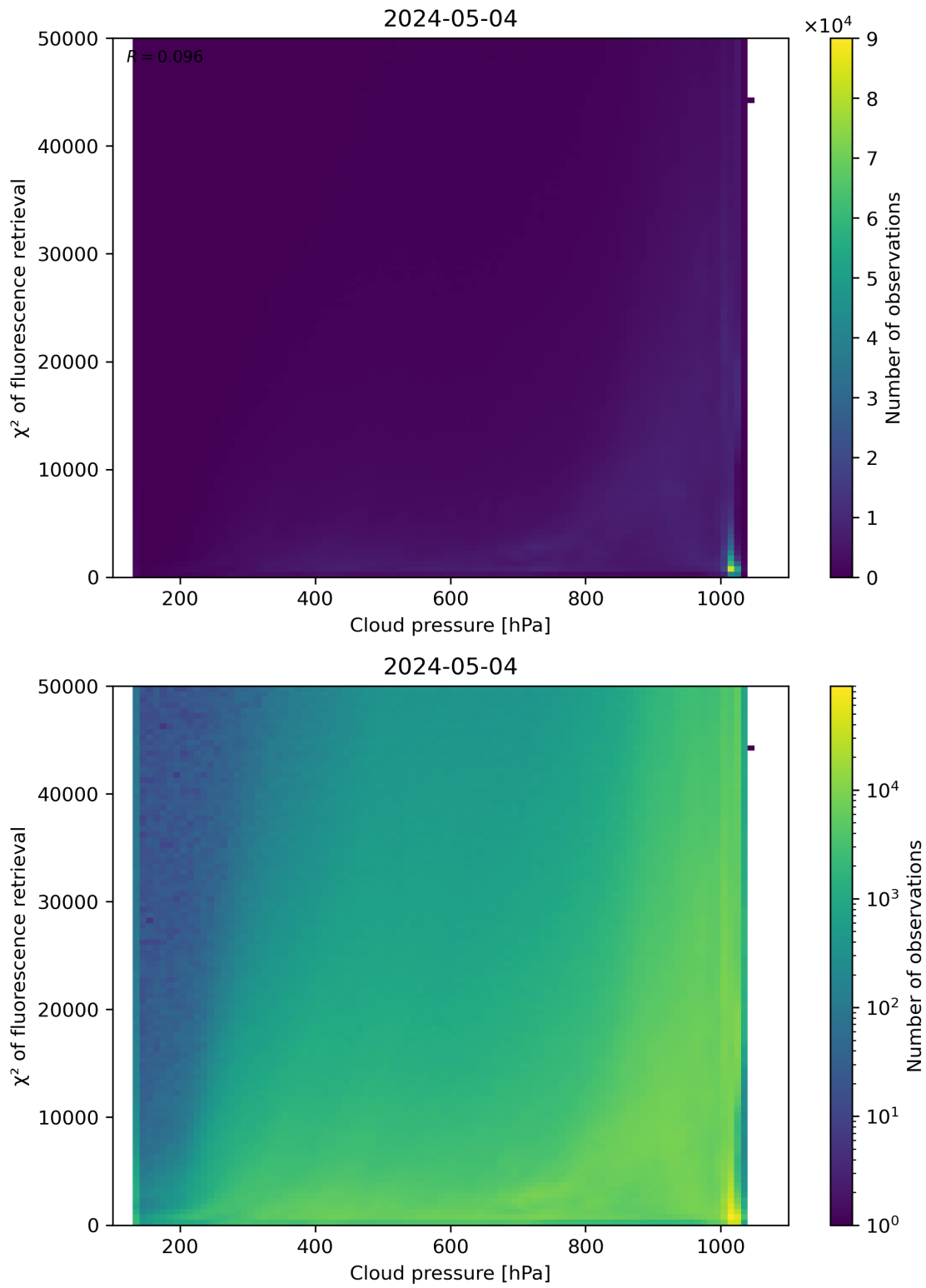
Figure 78: Scatter density plot of “Cloud pressure” against “ \chi^2 of fluorescence retrieval” for 2024-05-03 to 2024-05-05.
