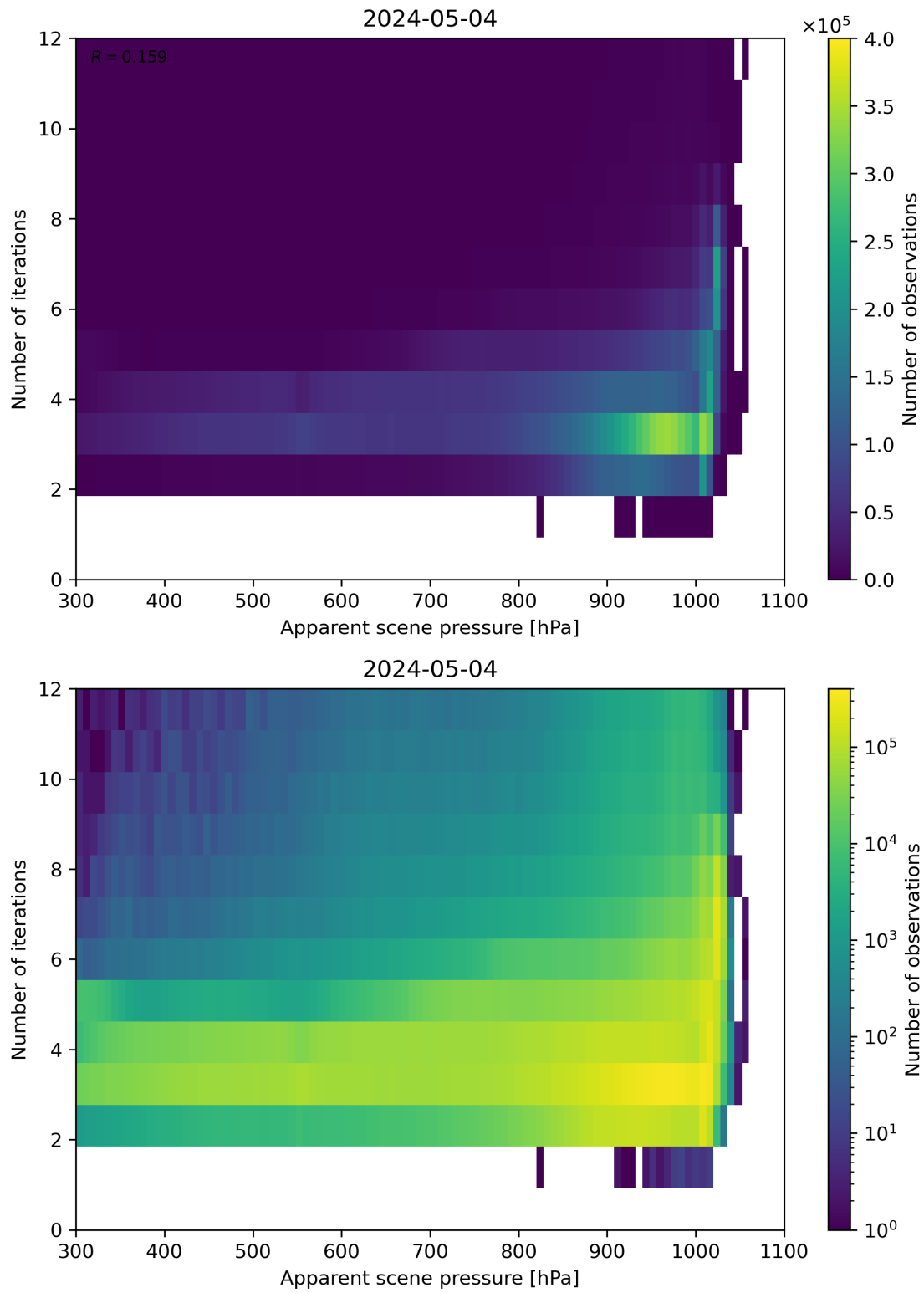
Figure 65: Scatter density plot of “Apparent scene pressure” against “Number of iterations” for 2024-05-03 to 2024-05-05.
