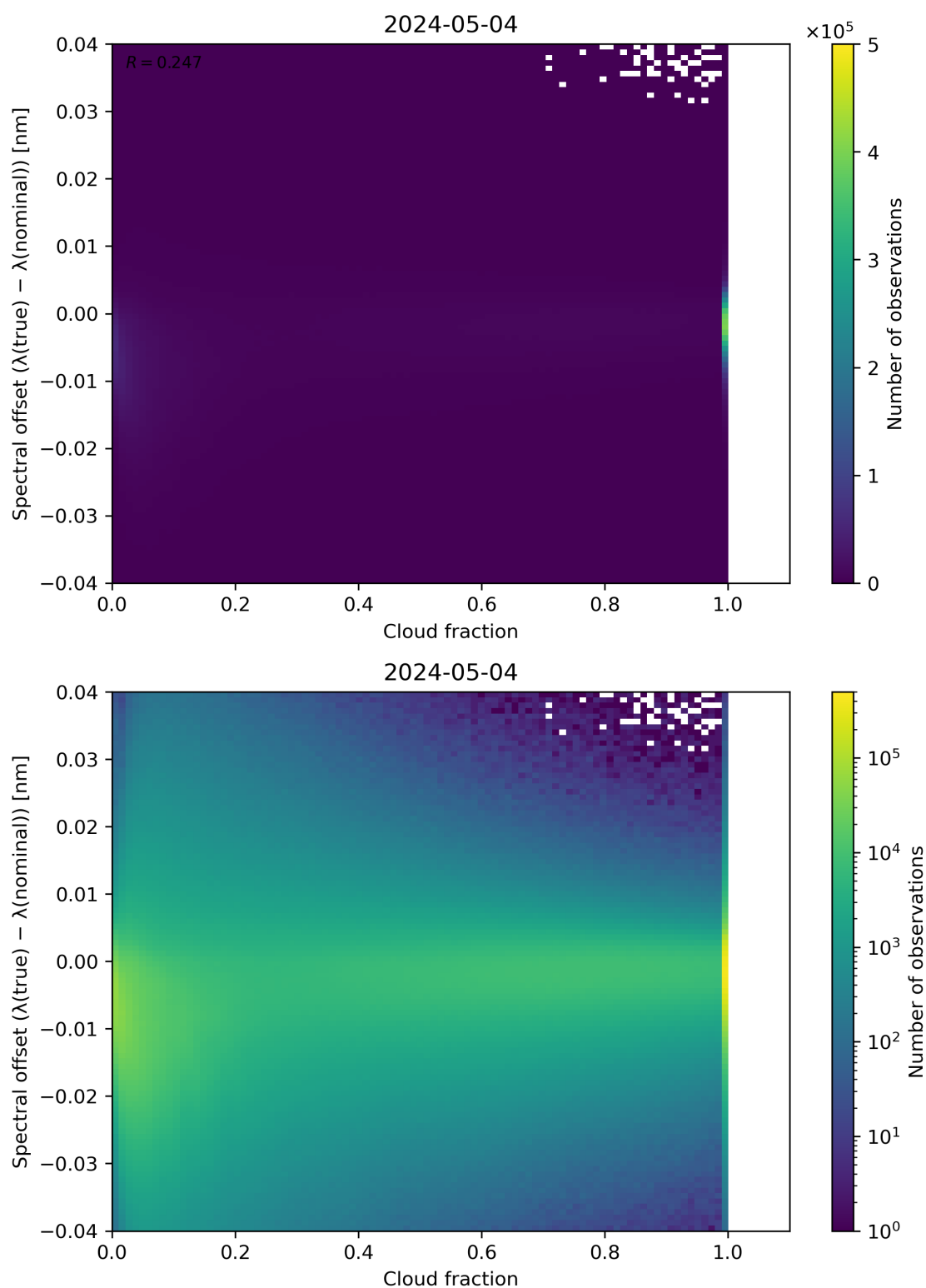
Figure 76: Scatter density plot of “Cloud fraction” against “Spectral offset ( \lambda(\text{true}) - \lambda(\text{nominal}) )” for 2024-05-03 to 2024-05-05.
