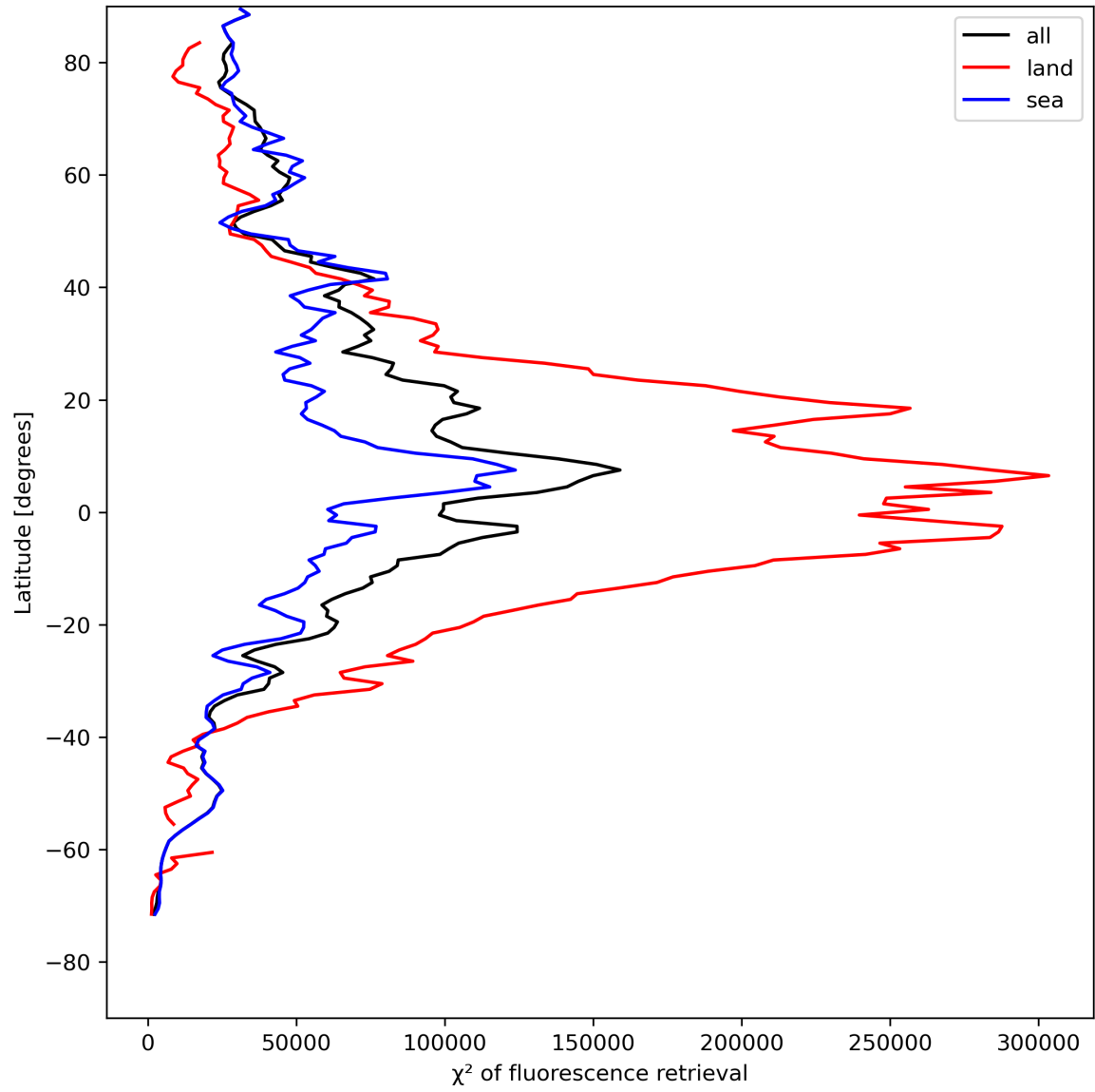
Figure 25: Zonal average of “ \chi^2 of fluorescence retrieval” for 2024-05-03 to 2024-05-05.
