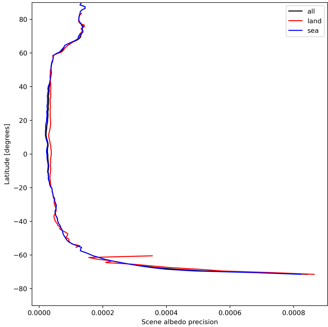
Figure 18: Zonal average of “Scene albedo precision” for 2024-05-03 to 2024-05-05.
