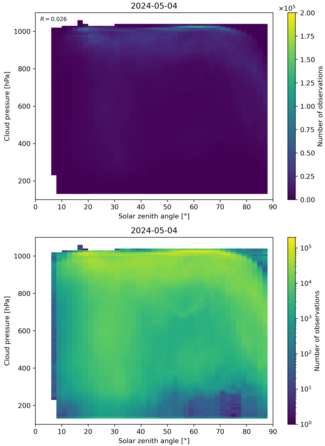
Figure 111: Scatter density plot of “Solar zenith angle” against “Cloud pressure” for 2024-05-03 to 2024-05-05.
