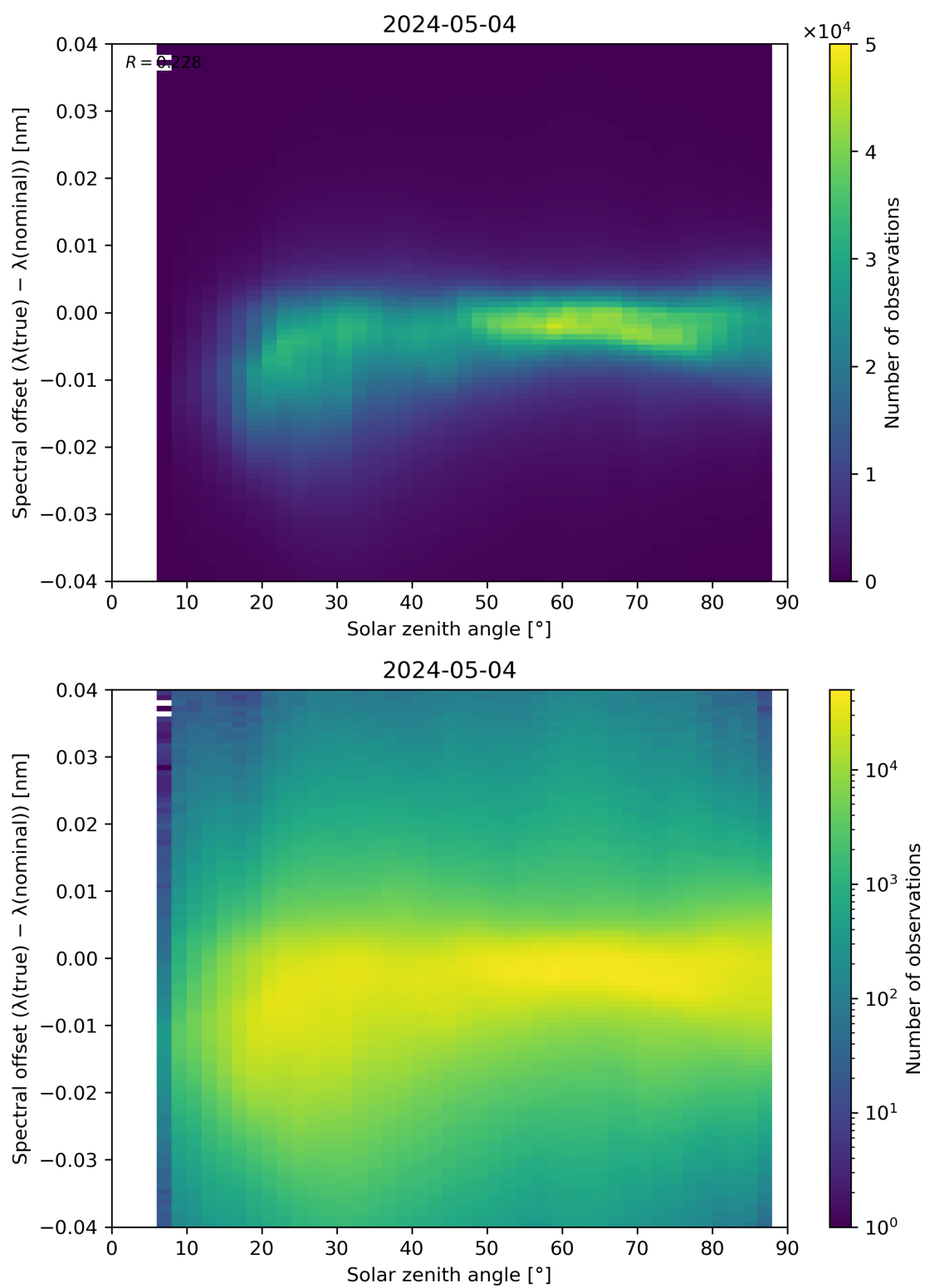
Figure 117: Scatter density plot of “Solar zenith angle” against “Spectral offset ( \lambda(\text{true}) - \lambda(\text{nominal}) )” for 2024-05-03 to 2024-05-05.
