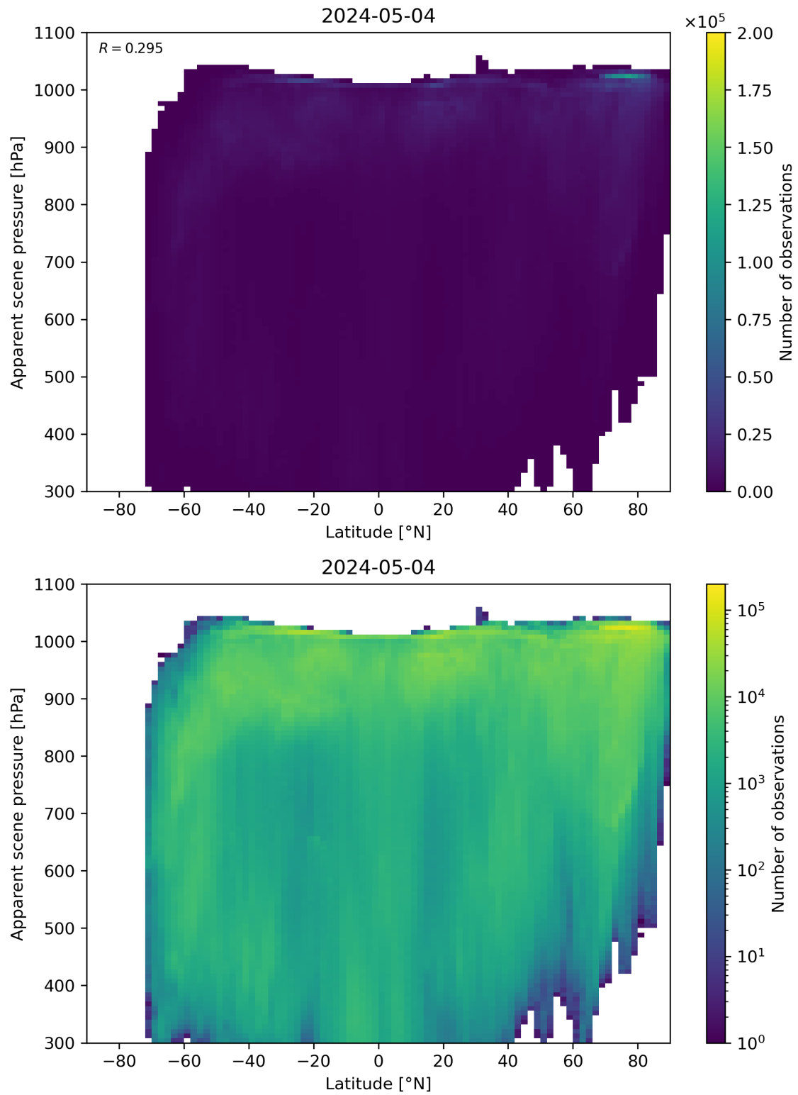
Figure 88: Scatter density plot of “Latitude” against “Apparent scene pressure” for 2024-05-03 to 2024-05-05.
