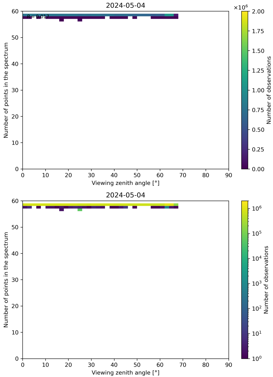
Figure 125: Scatter density plot of “Viewing zenith angle” against “Number of points in the spectrum” for 2024-05-03 to 2024-05-05.
