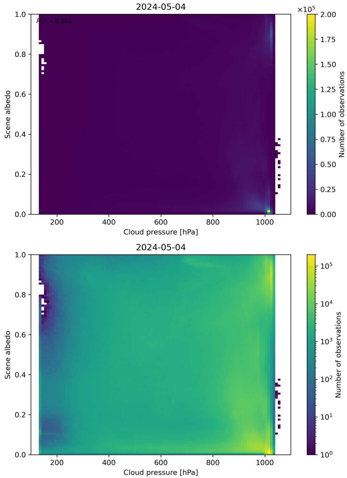
Figure 83: Scatter density plot of “Cloud pressure” against “Scene albedo” for 2024-05-03 to 2024-05-05.
