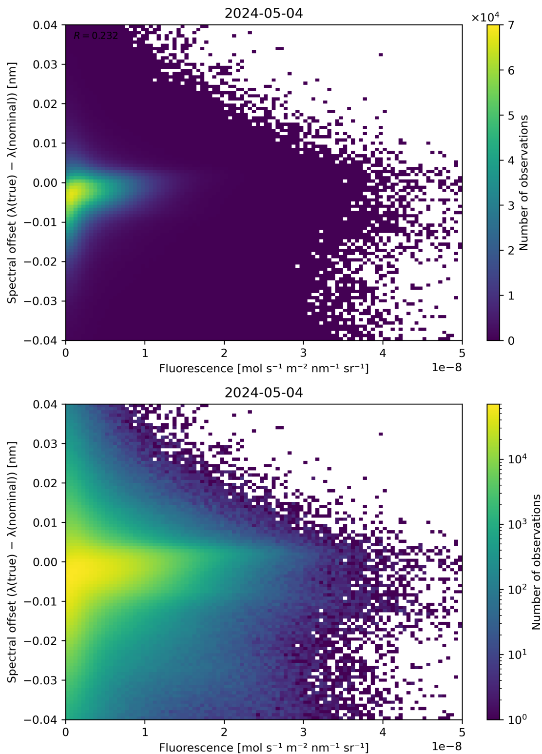
Figure 87: Scatter density plot of “Fluorescence” against “Spectral offset ( \lambda(\text{true}) - \lambda(\text{nominal}) )” for 2024-05-03 to 2024-05-05.
