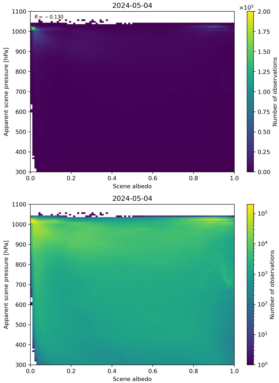
Figure 102: Scatter density plot of “Scene albedo” against “Apparent scene pressure” for 2024-05-03 to 2024-05-05.
