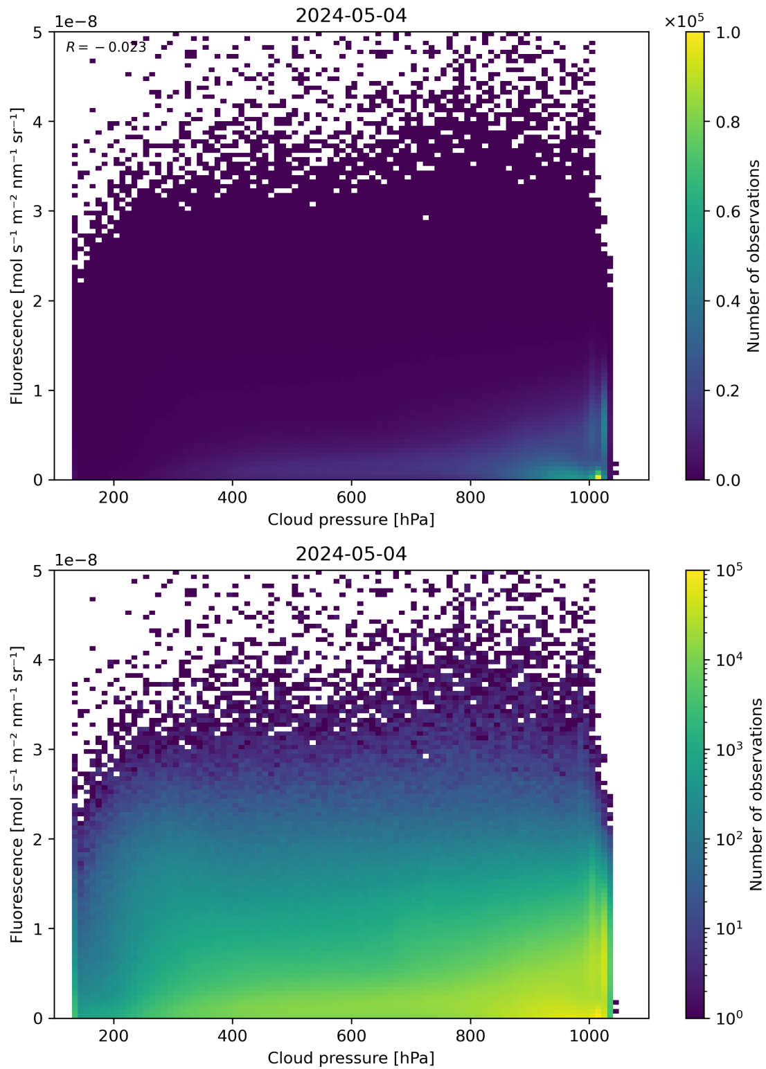
Figure 80: Scatter density plot of “Cloud pressure” against “Fluorescence” for 2024-05-03 to 2024-05-05.
