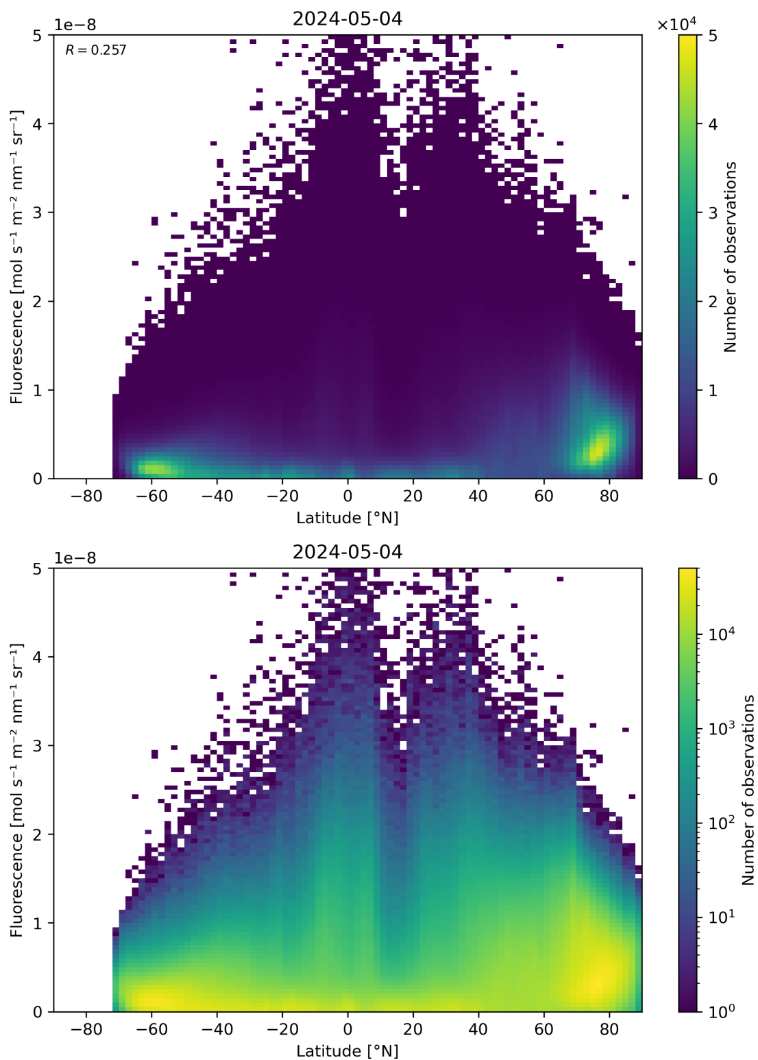
Figure 92: Scatter density plot of “Latitude” against “Fluorescence” for 2024-05-03 to 2024-05-05.
