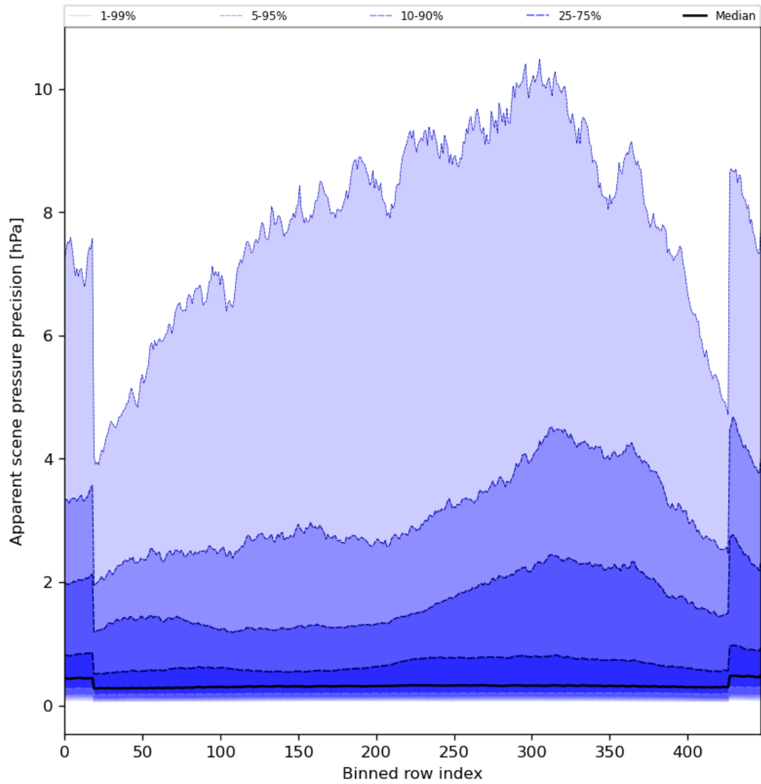
Figure 54: Along track statistics of “Apparent scene pressure precision” for 2024-05-03 to 2024-05-05
