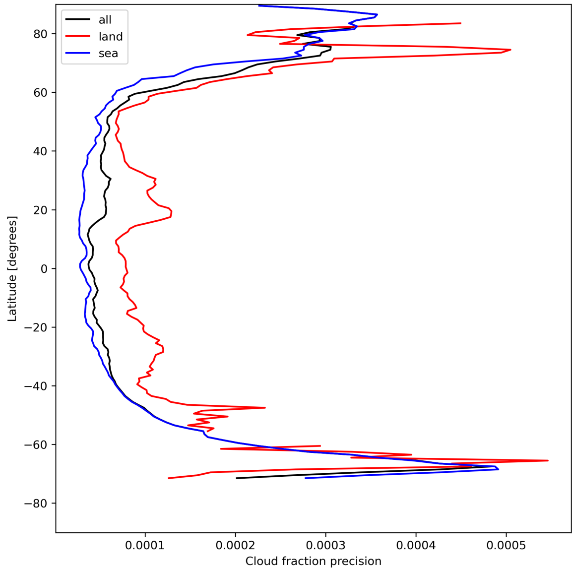
Figure 16: Zonal average of “Cloud fraction precision” for 2024-05-03 to 2024-05-05.
