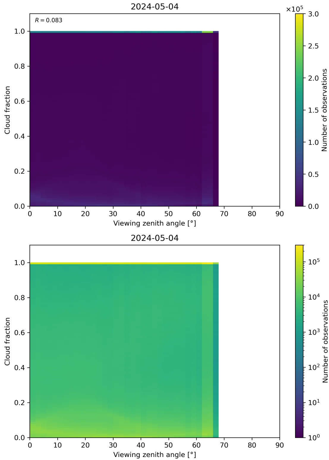
Figure 120: Scatter density plot of “Viewing zenith angle” against “Cloud fraction” for 2024-05-03 to 2024-05-05.
