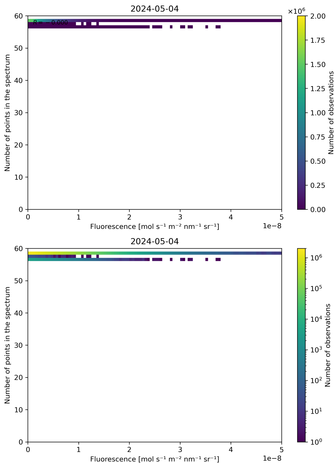
Figure 86: Scatter density plot of “Fluorescence” against “Number of points in the spectrum” for 2024-05-03 to 2024-05-05.
