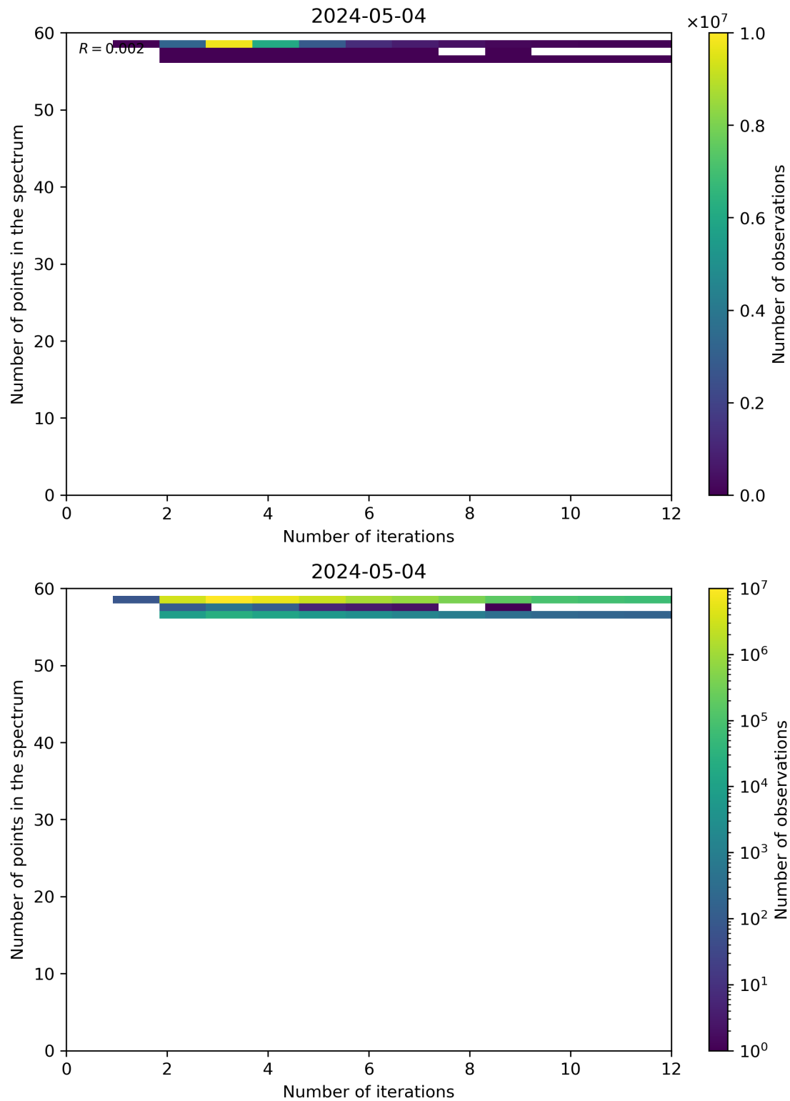
Figure 99: Scatter density plot of “Number of iterations” against “Number of points in the spectrum” for 2024-05-03 to 2024-05-05.
