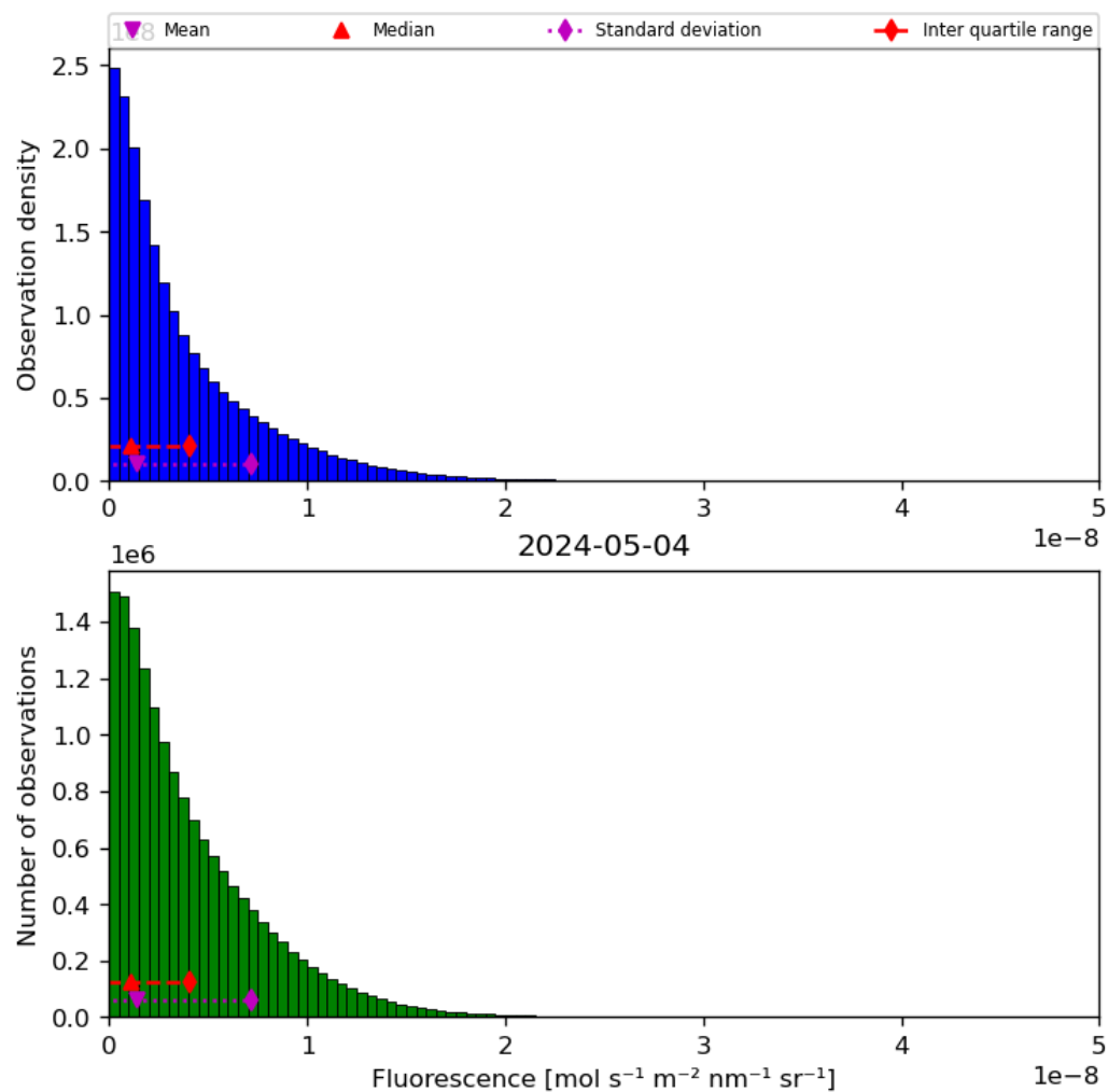
Figure 40: Histogram of “Fluorescence” for 2024-05-03 to 2024-05-05
