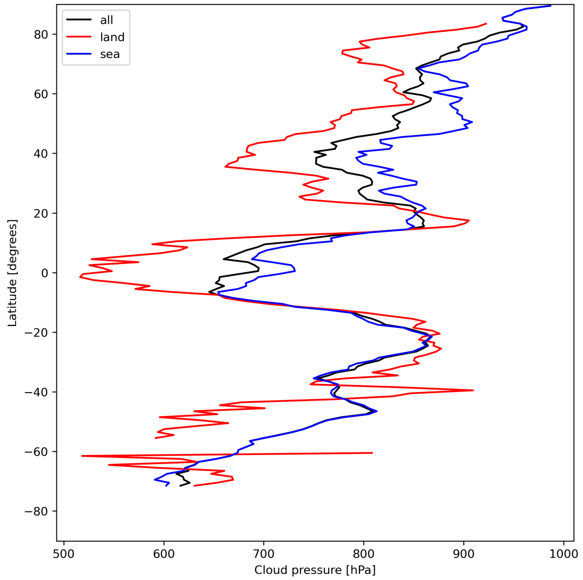
Figure 13: Zonal average of “Cloud pressure” for 2024-05-03 to 2024-05-05.
