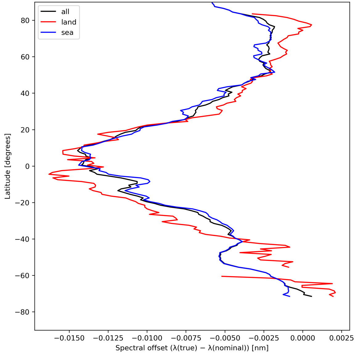
Figure 28: Zonal average of “Spectral offset ( \lambda(\text{true}) - \lambda(\text{nominal}) )” for 2024-05-03 to 2024-05-05.
