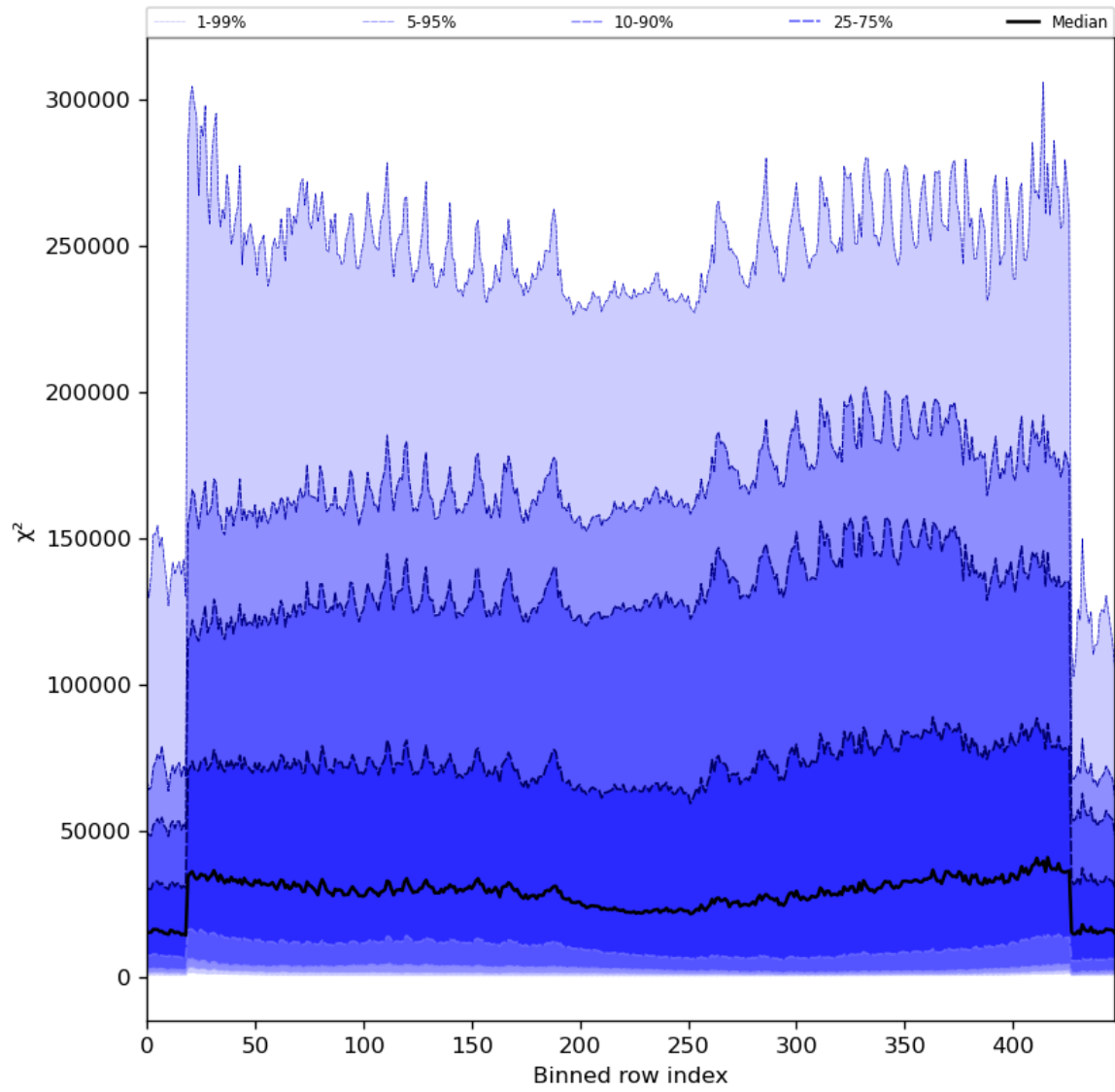
Figure 55: Along track statistics of “ \chi^2 ” for 2024-05-03 to 2024-05-05
