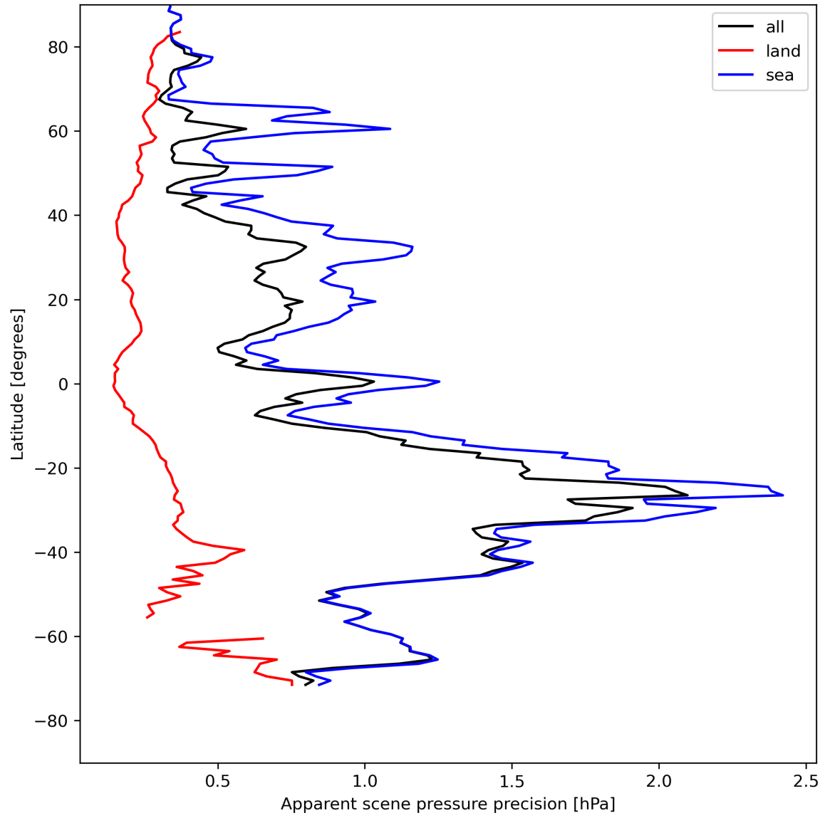
Figure 20: Zonal average of “Apparent scene pressure precision” for 2024-05-03 to 2024-05-05.
