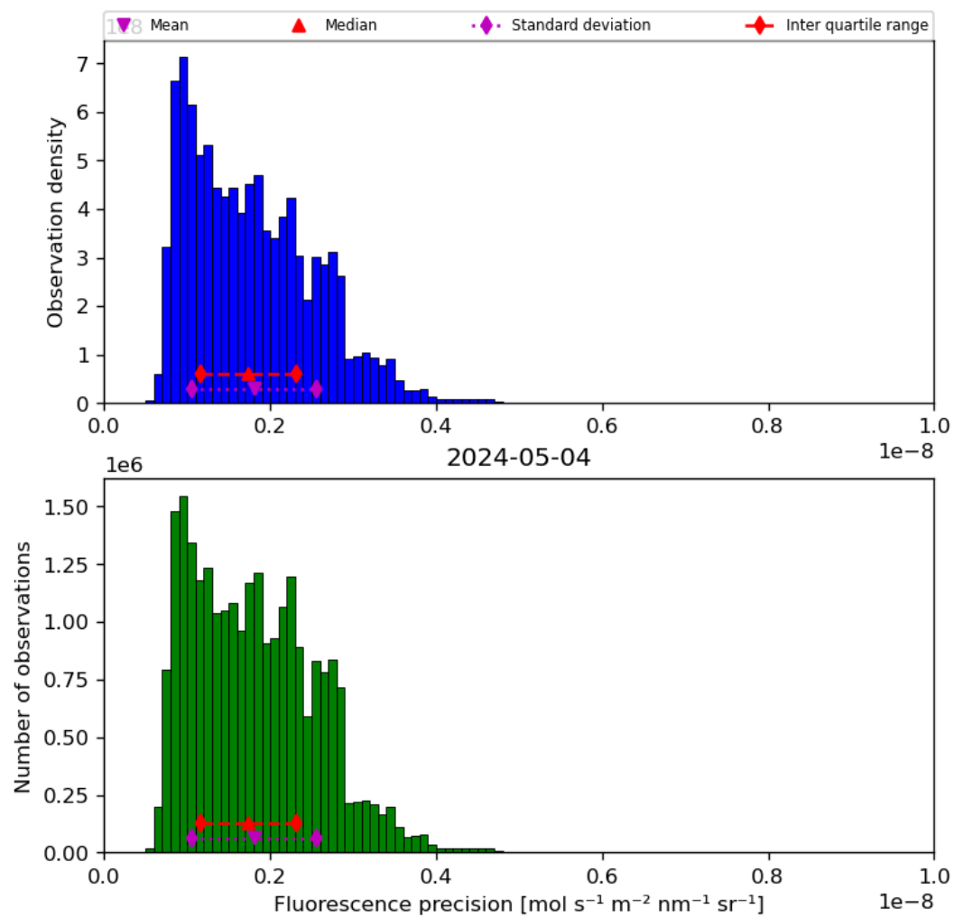
Figure 41: Histogram of “Fluorescence precision” for 2024-05-03 to 2024-05-05
