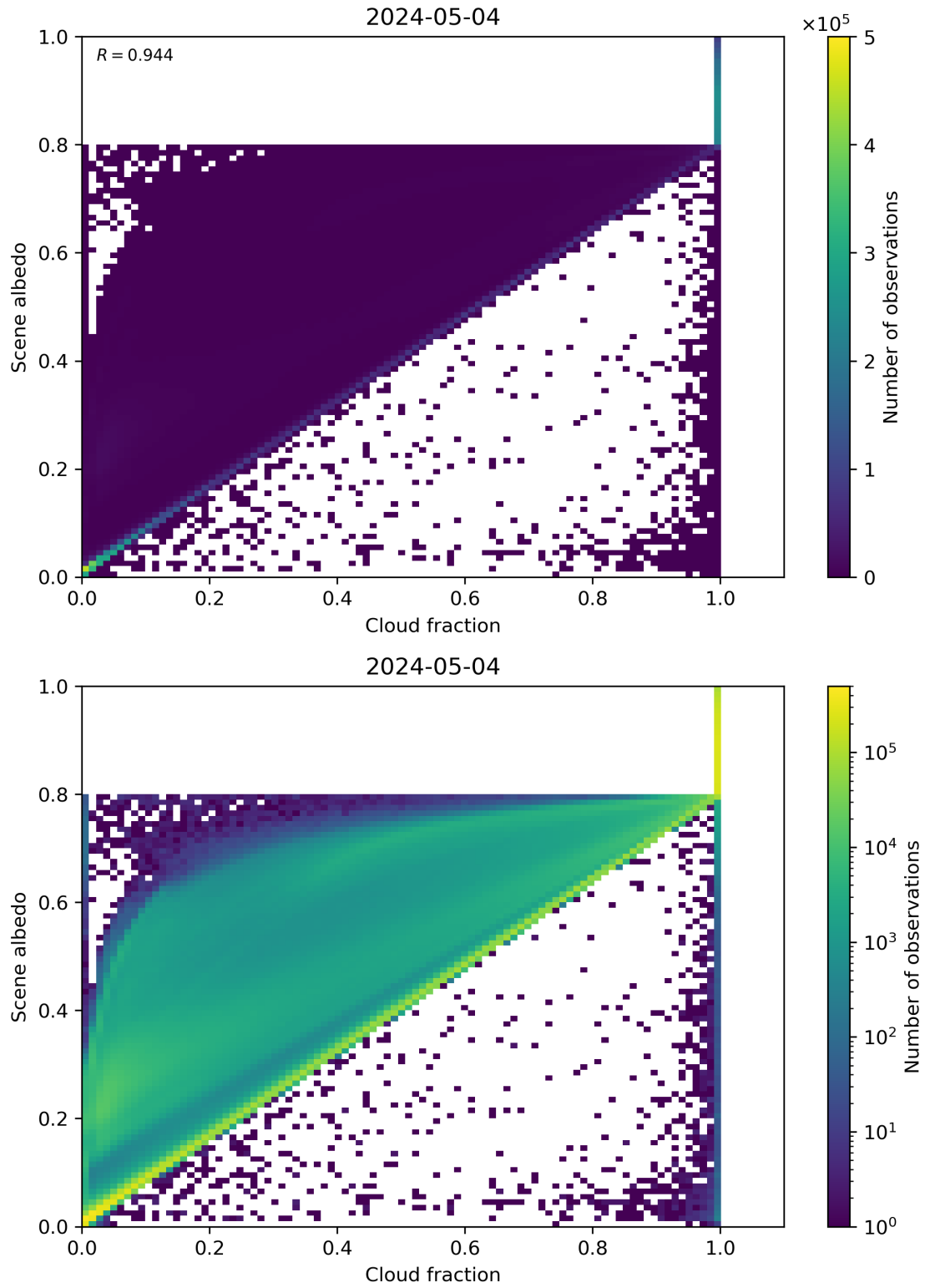
Figure 75: Scatter density plot of “Cloud fraction” against “Scene albedo” for 2024-05-03 to 2024-05-05.
