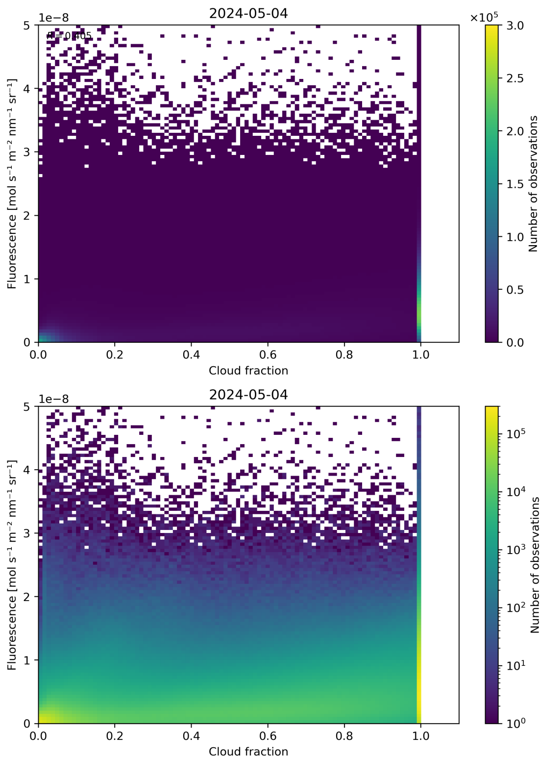
Figure 72: Scatter density plot of “Cloud fraction” against “Fluorescence” for 2024-05-03 to 2024-05-05.
