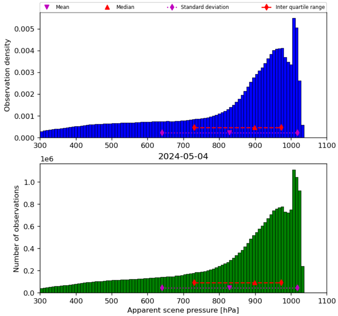
Figure 36: Histogram of “Apparent scene pressure” for 2024-05-03 to 2024-05-05
