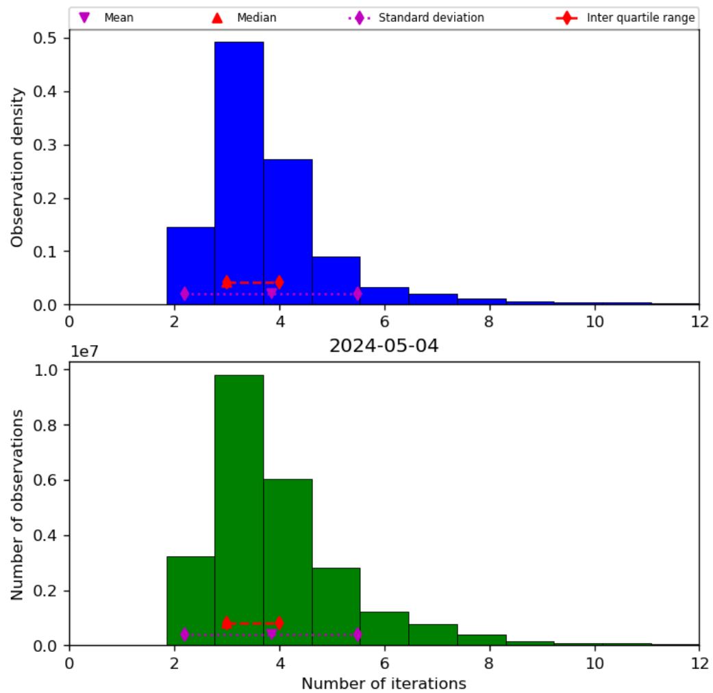
Figure 39: Histogram of “Number of iterations” for 2024-05-03 to 2024-05-05
