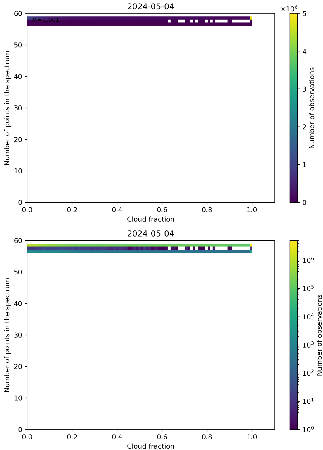
Figure 74: Scatter density plot of “Cloud fraction” against “Number of points in the spectrum” for 2024-05-03 to 2024-05-05.
