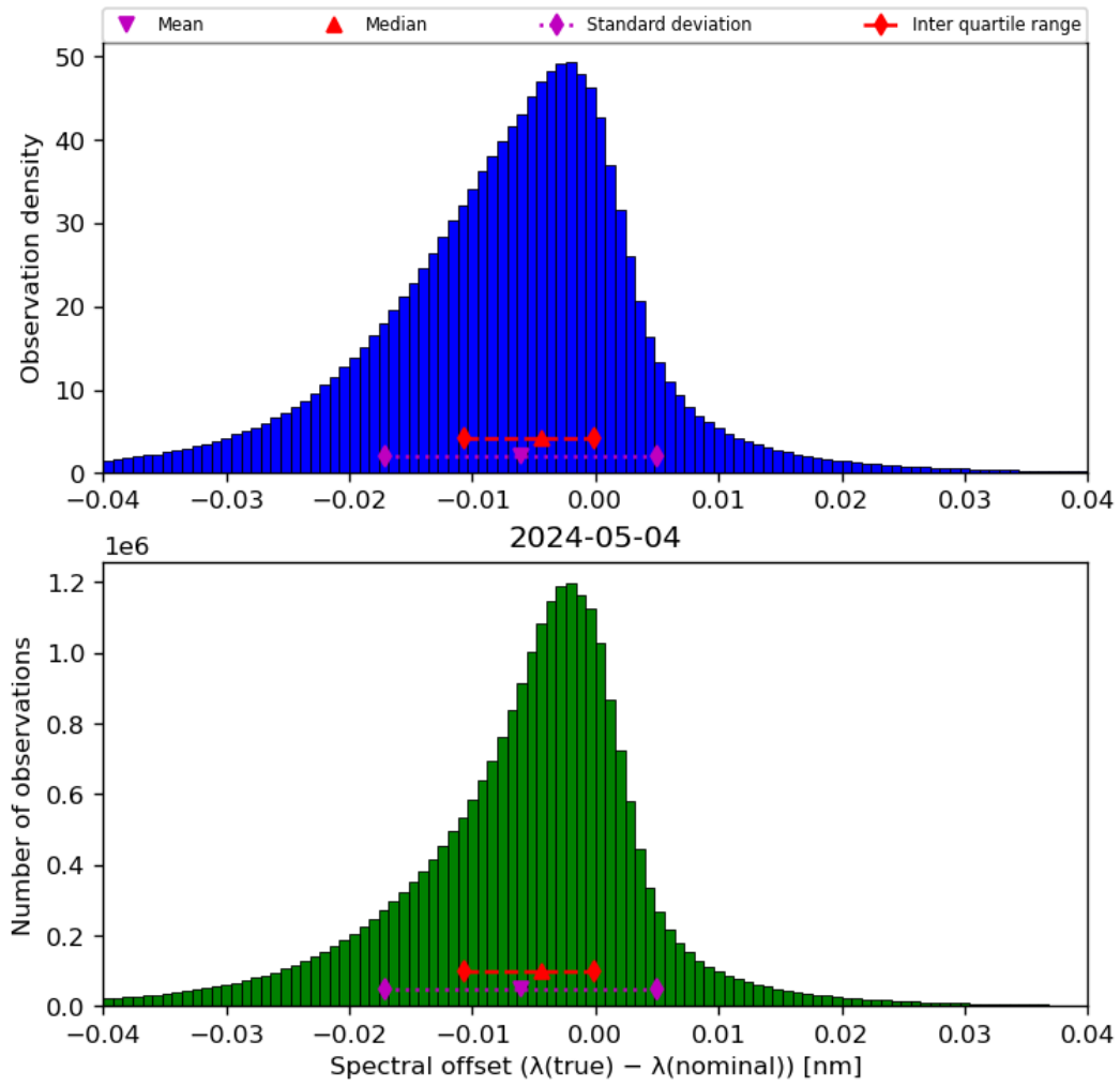
Figure 45: Histogram of “Spectral offset ( \lambda(\text{true}) - \lambda(\text{nominal}) )” for 2024-05-03 to 2024-05-05
