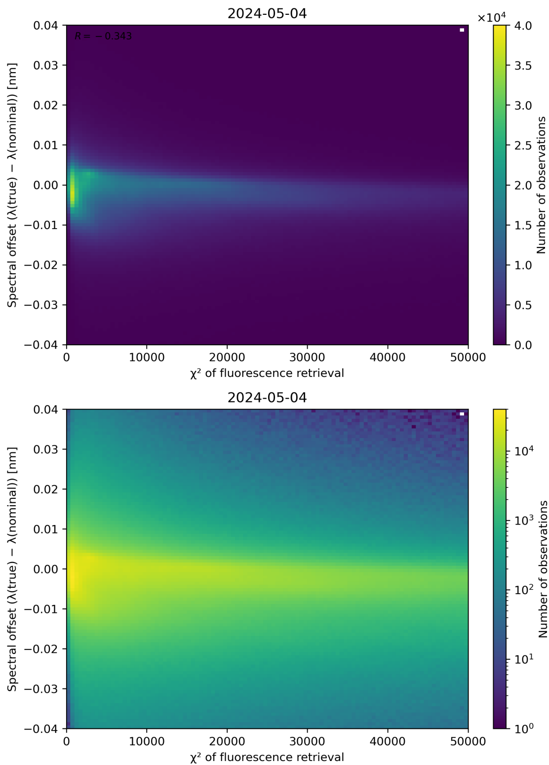
Figure 69: Scatter density plot of " \chi^2 of fluorescence retrieval" against "Spectral offset ( \lambda(\text{true}) - \lambda(\text{nominal}) )" for 2024-05-03 to 2024-05-05.
