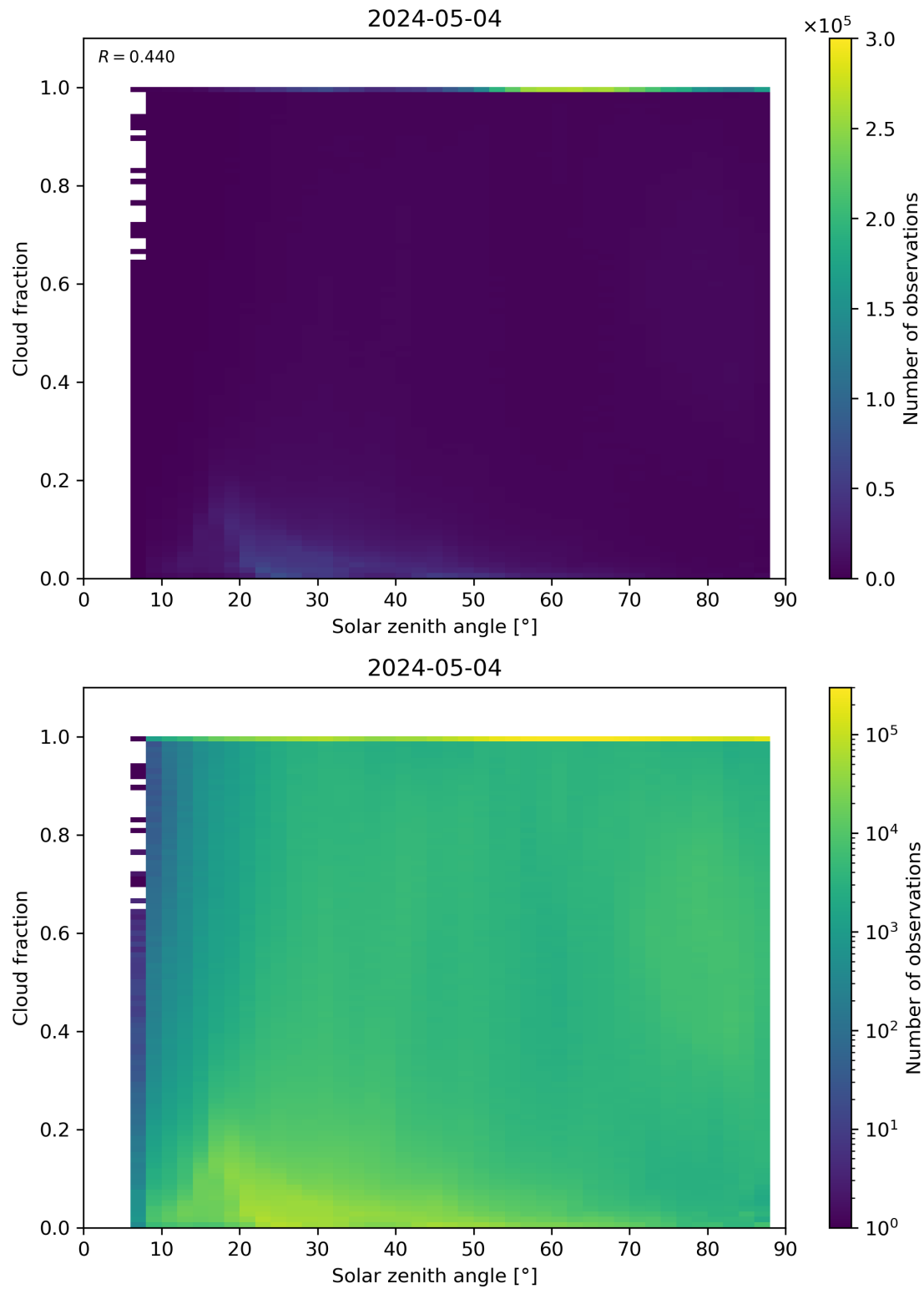
Figure 110: Scatter density plot of “Solar zenith angle” against “Cloud fraction” for 2024-05-03 to 2024-05-05.
