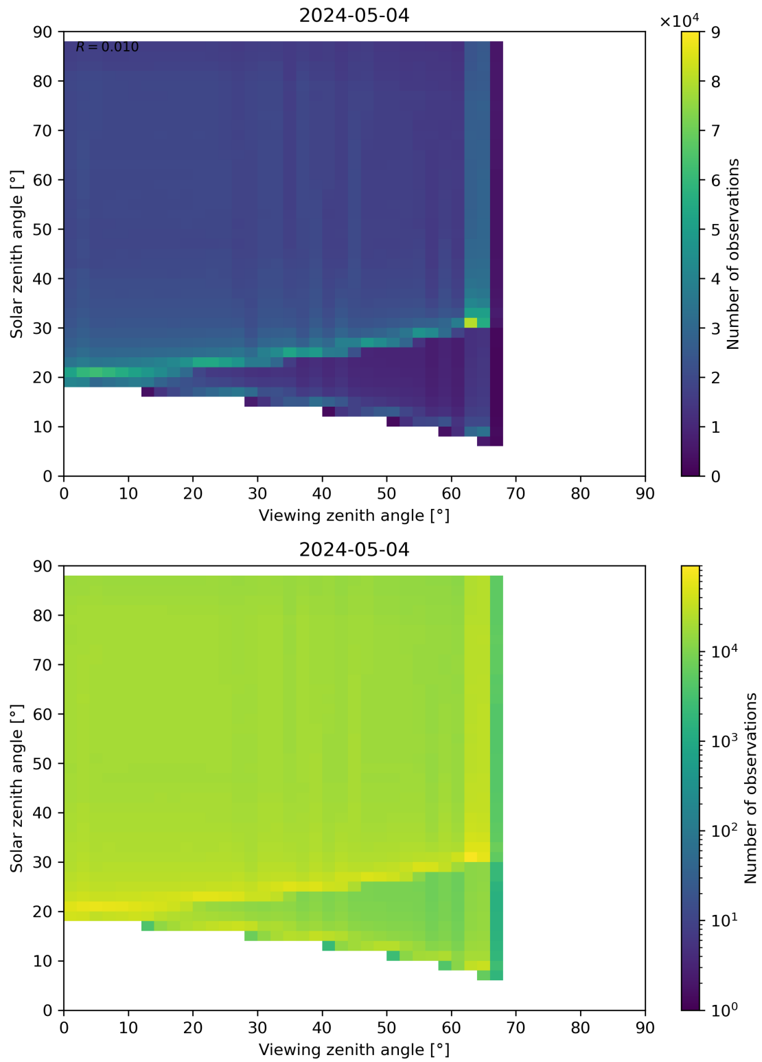
Figure 127: Scatter density plot of “Viewing zenith angle” against “Solar zenith angle” for 2024-05-03 to 2024-05-05.
