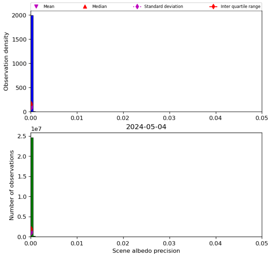
Figure 35: Histogram of “Scene albedo precision” for 2024-05-03 to 2024-05-05
