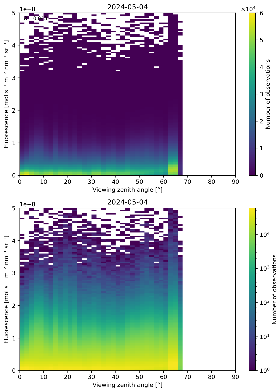
Figure 122: Scatter density plot of “Viewing zenith angle” against “Fluorescence” for 2024-05-03 to 2024-05-05.
