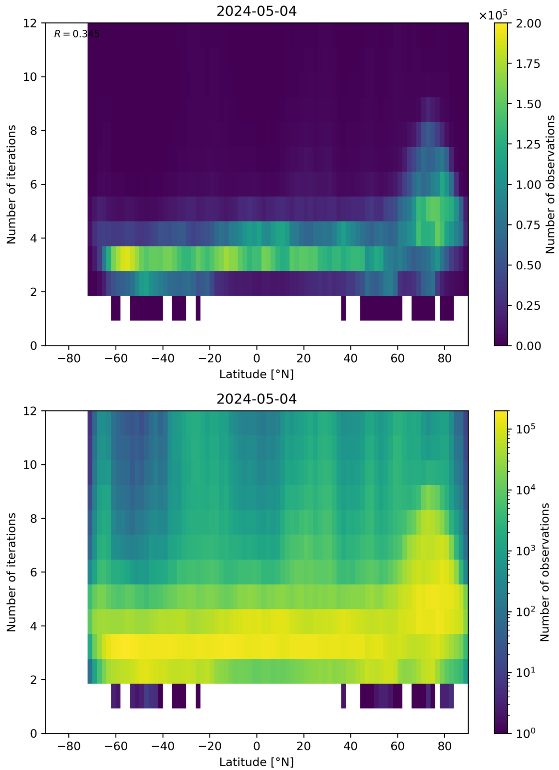
Figure 93: Scatter density plot of “Latitude” against “Number of iterations” for 2024-05-03 to 2024-05-05.
