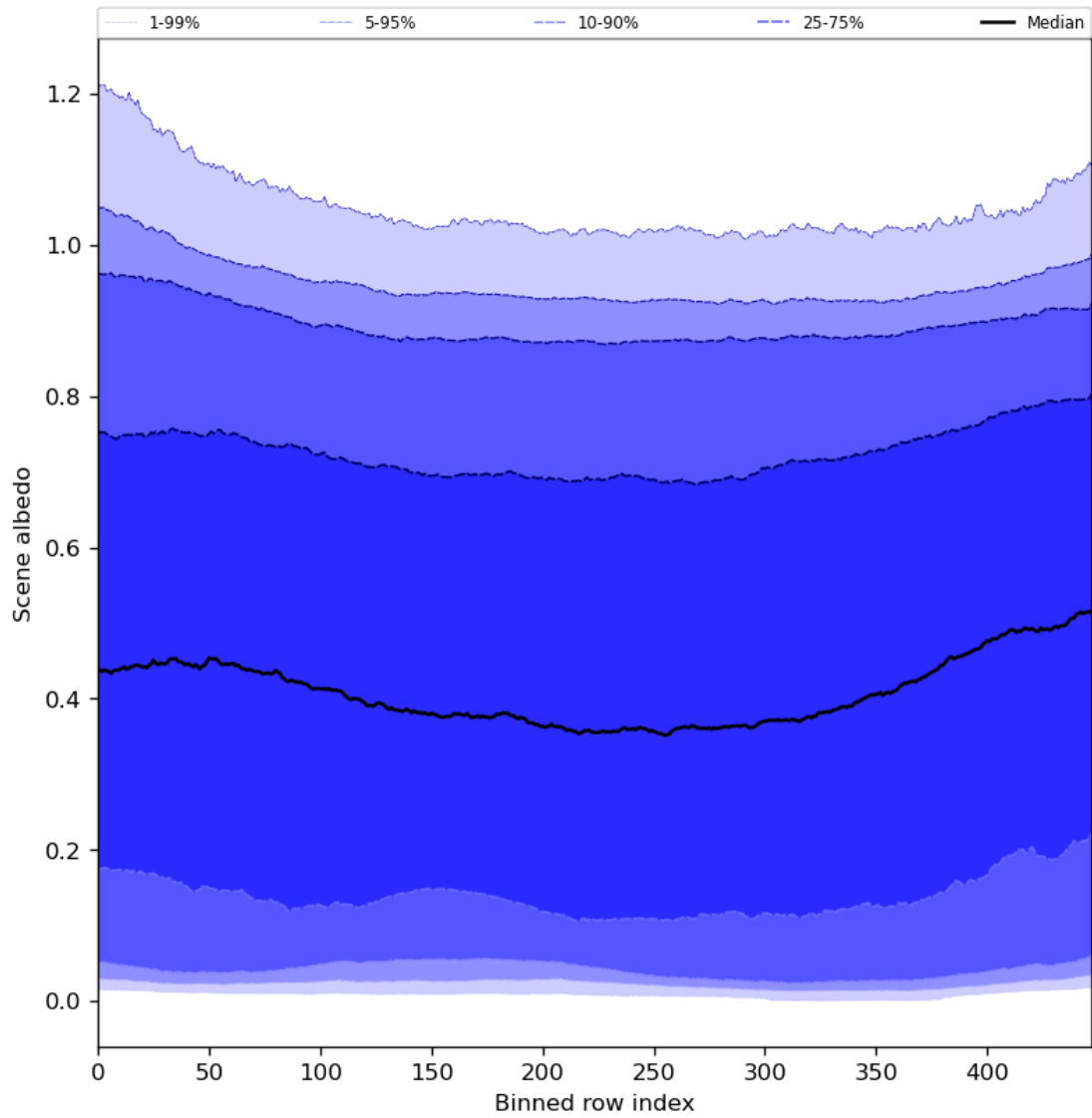
Figure 51: Along track statistics of “Scene albedo” for 2024-05-03 to 2024-05-05
