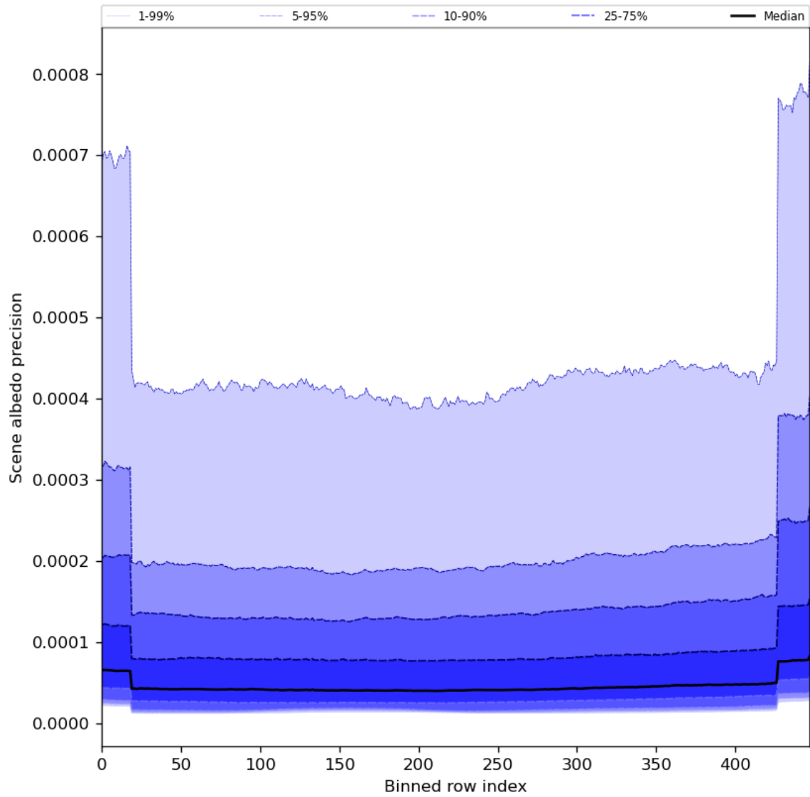
Figure 52: Along track statistics of “Scene albedo precision” for 2024-05-03 to 2024-05-05
