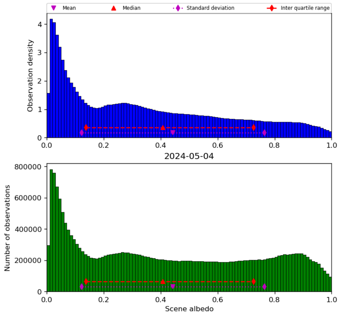
Figure 34: Histogram of “Scene albedo” for 2024-05-03 to 2024-05-05
