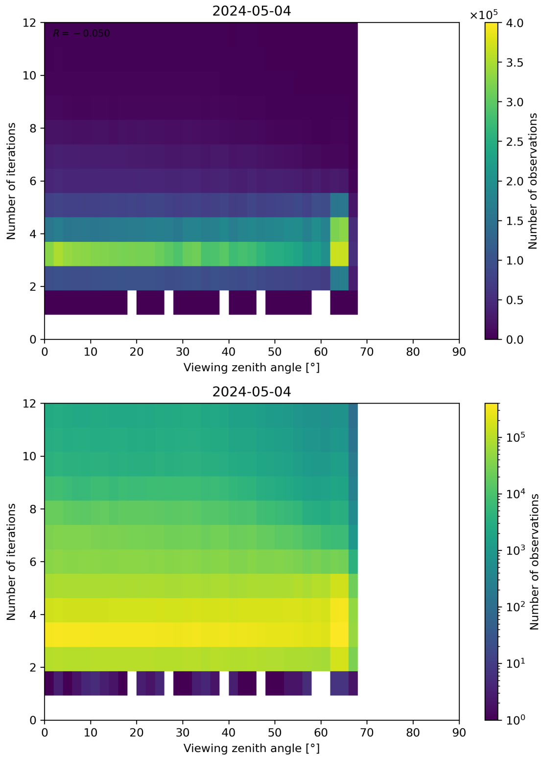
Figure 124: Scatter density plot of “Viewing zenith angle” against “Number of iterations” for 2024-05-03 to 2024-05-05.
