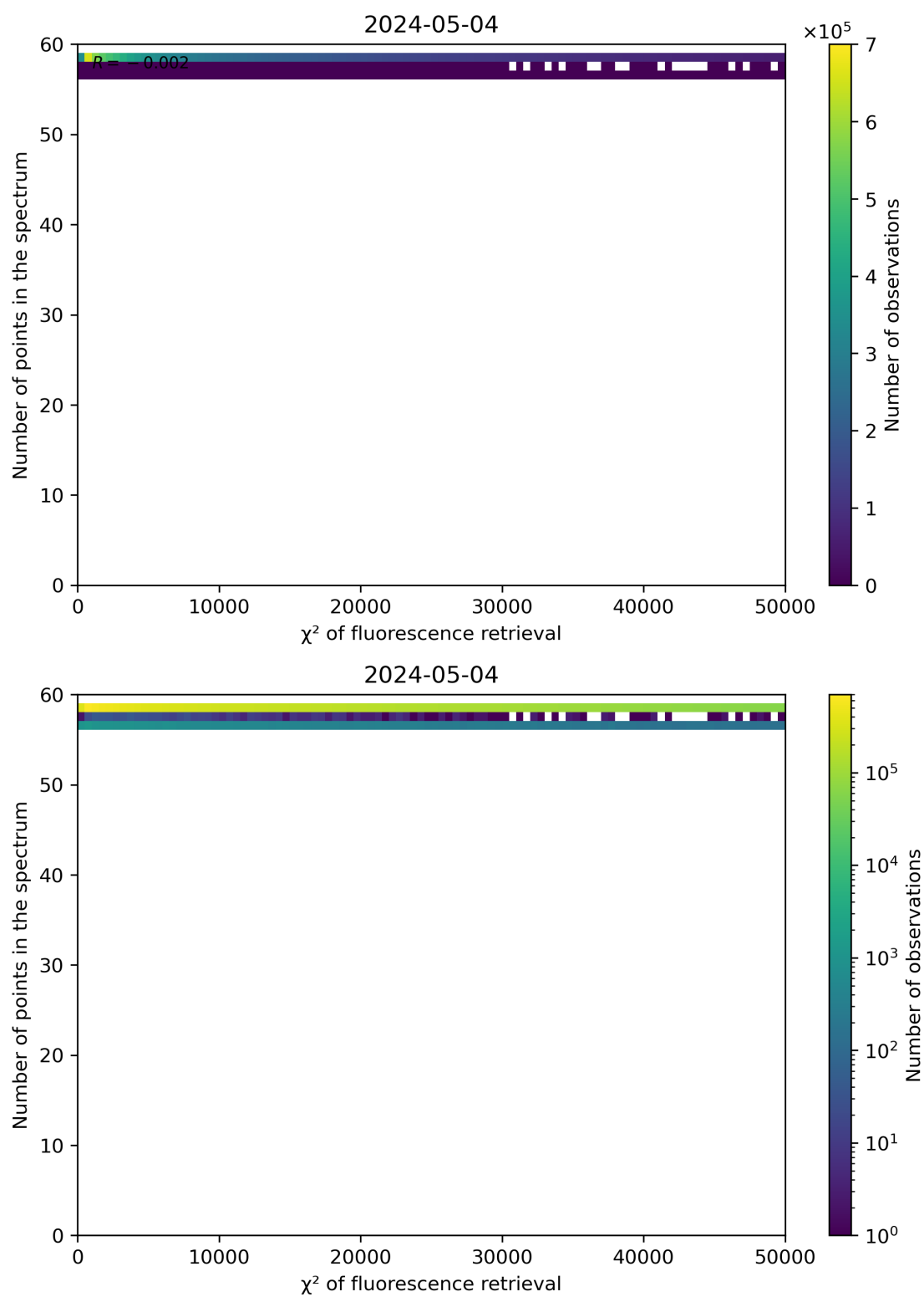
Figure 68: Scatter density plot of " \chi^2 of fluorescence retrieval" against "Number of points in the spectrum" for 2024-05-03 to 2024-05-05.
