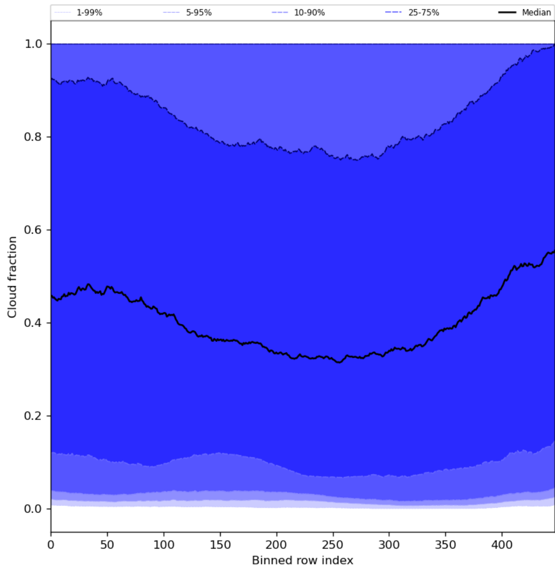
Figure 49: Along track statistics of “Cloud fraction” for 2024-05-03 to 2024-05-05
