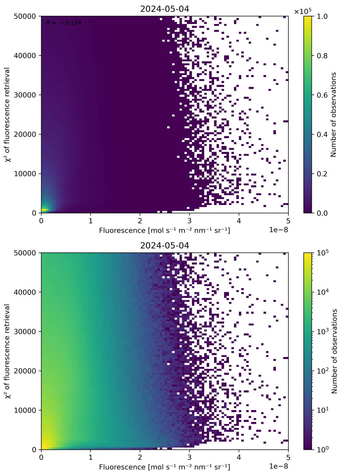
Figure 85: Scatter density plot of “Fluorescence” against “ \chi^2 of fluorescence retrieval” for 2024-05-03 to 2024-05-05.
