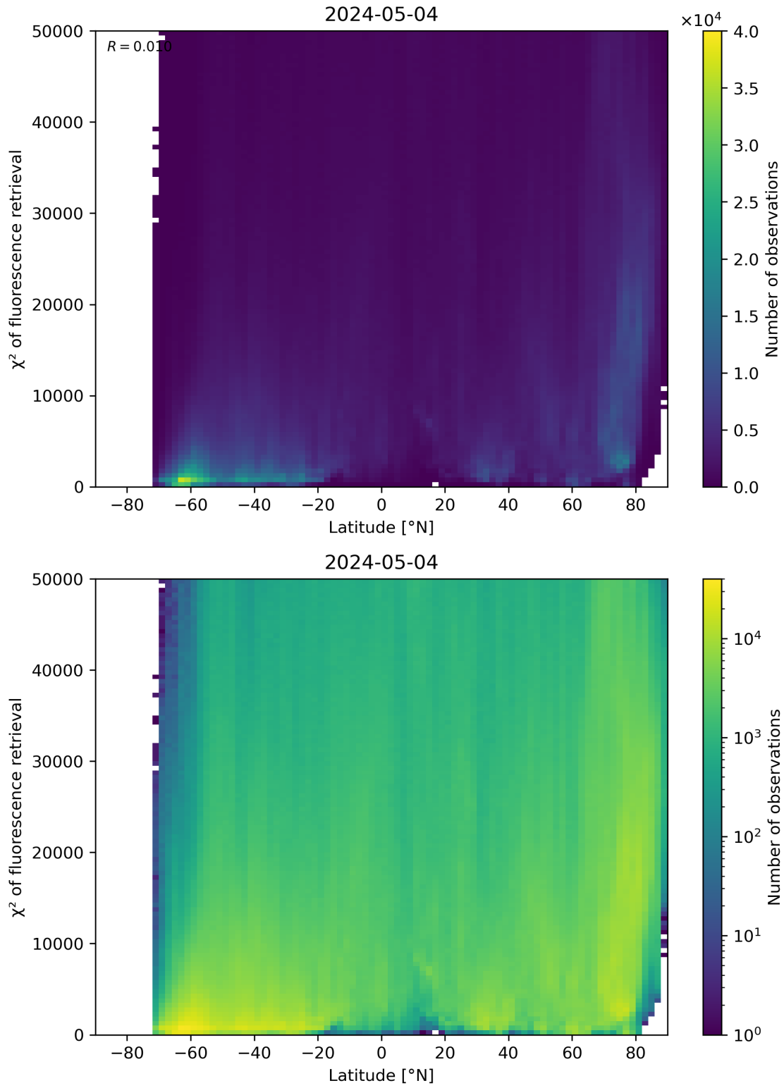
Figure 89: Scatter density plot of “Latitude” against “ \chi^2 of fluorescence retrieval” for 2024-05-03 to 2024-05-05.
