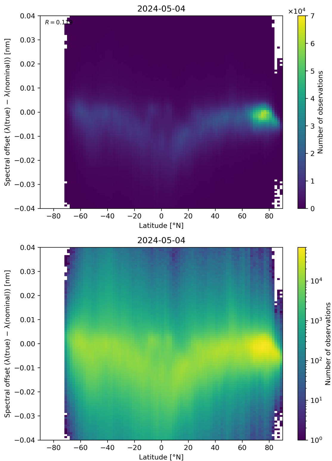
Figure 96: Scatter density plot of “Latitude” against “Spectral offset ( \lambda(\text{true}) - \lambda(\text{nominal}) )” for 2024-05-03 to 2024-05-05.
