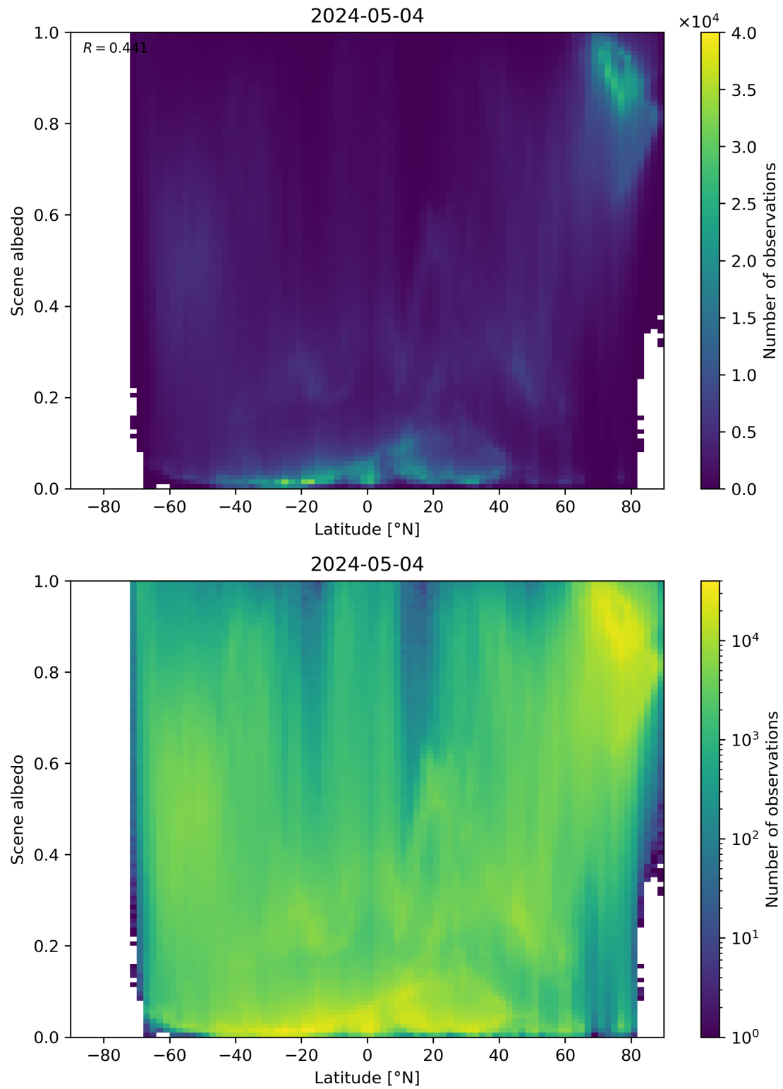
Figure 95: Scatter density plot of “Latitude” against “Scene albedo” for 2024-05-03 to 2024-05-05.
