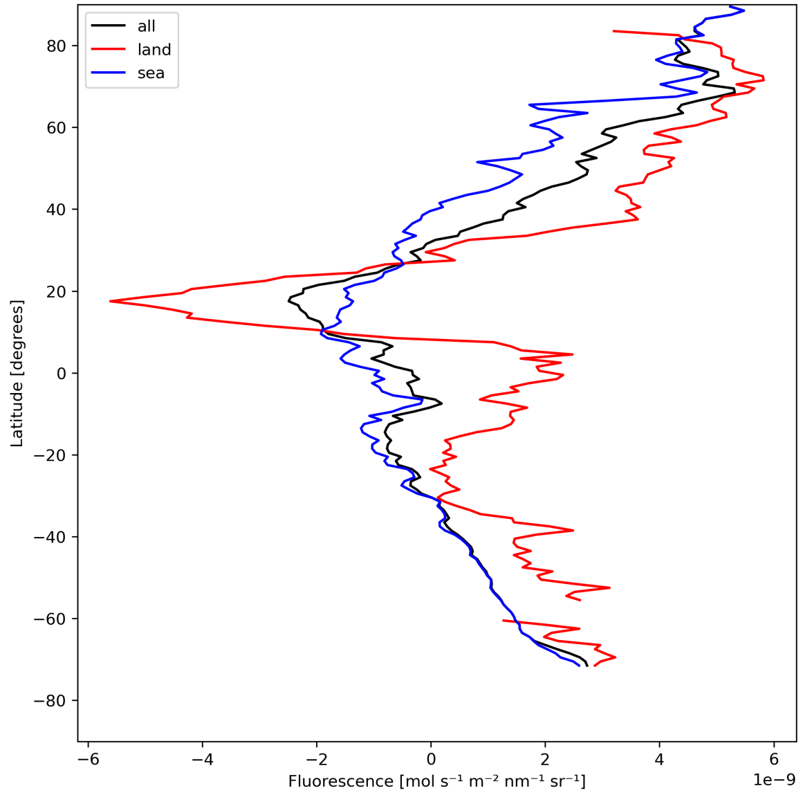
Figure 23: Zonal average of “Fluorescence” for 2024-05-03 to 2024-05-05.
