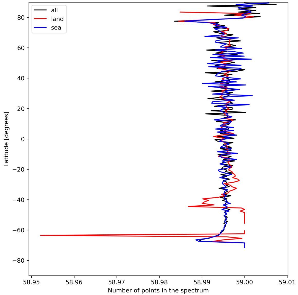
Figure 27: Zonal average of “Number of points in the spectrum” for 2024-05-03 to 2024-05-05.
