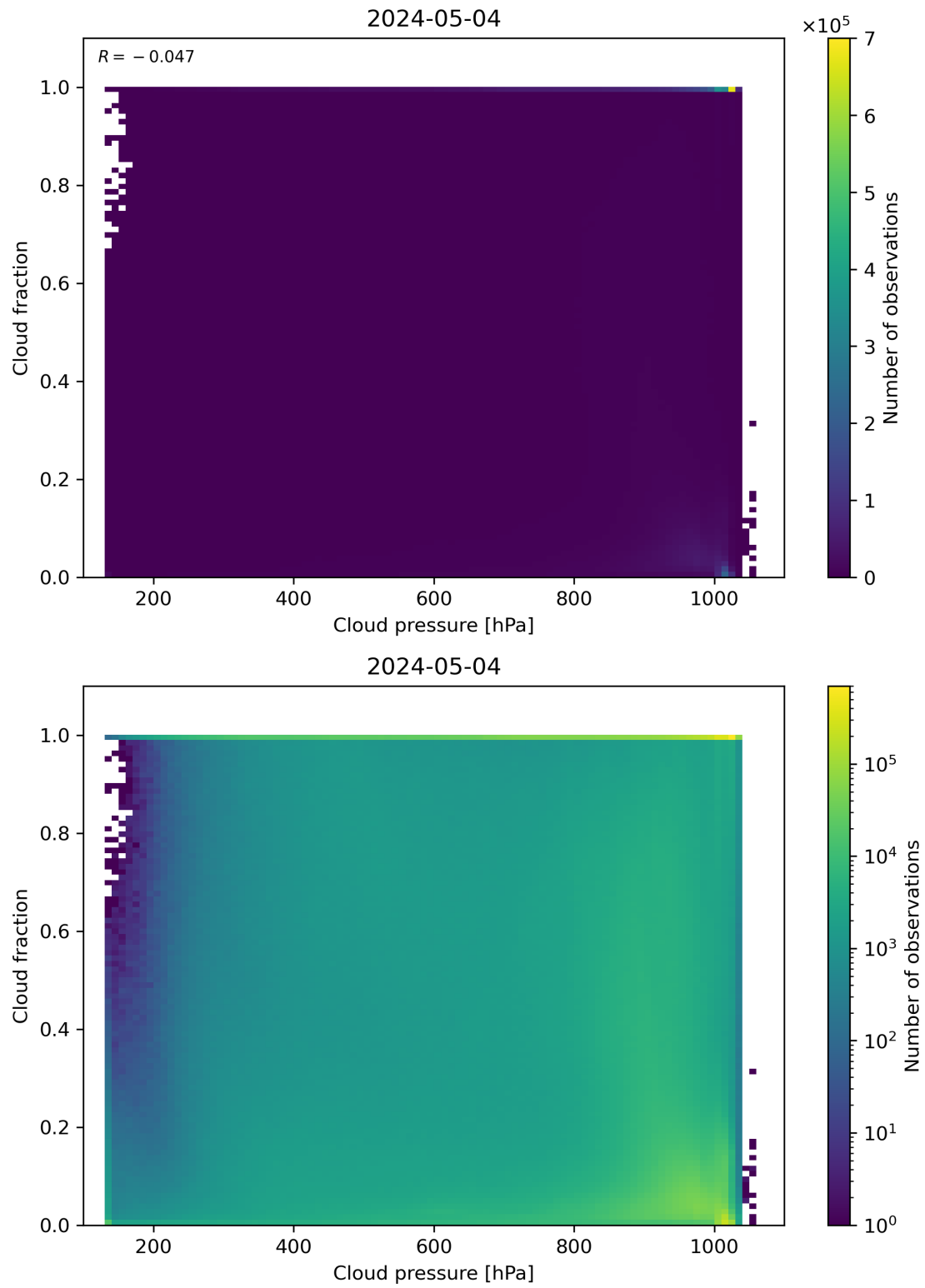
Figure 79: Scatter density plot of “Cloud pressure” against “Cloud fraction” for 2024-05-03 to 2024-05-05.
