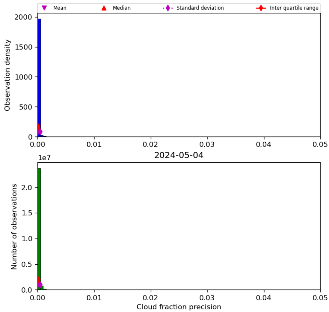
Figure 33: Histogram of “Cloud fraction precision” for 2024-05-03 to 2024-05-05
