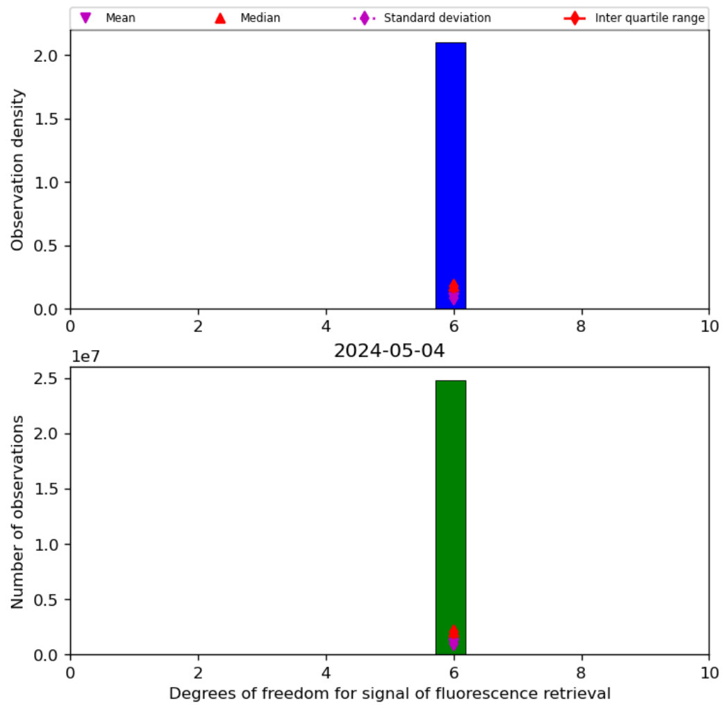
Figure 43: Histogram of “Degrees of freedom for signal of fluorescence retrieval” for 2024-05-03 to 2024-05-05
