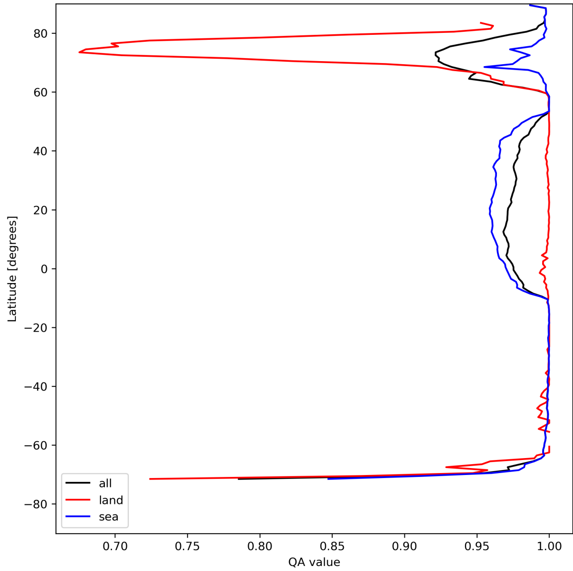
Figure 12: Zonal average of “QA value” for 2024-05-03 to 2024-05-05.
