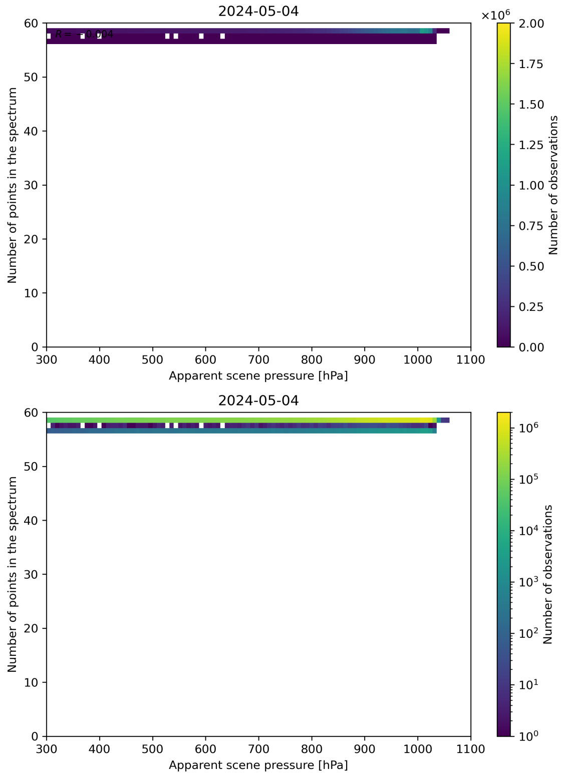
Figure 66: Scatter density plot of “Apparent scene pressure” against “Number of points in the spectrum” for 2024-05-03 to 2024-05-05.
