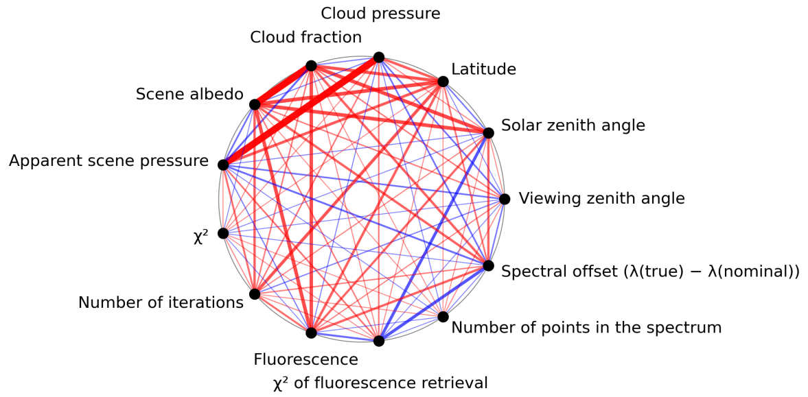
Figure 1: Map of correlation graph for 2024-05-03 to 2024-05-05.
