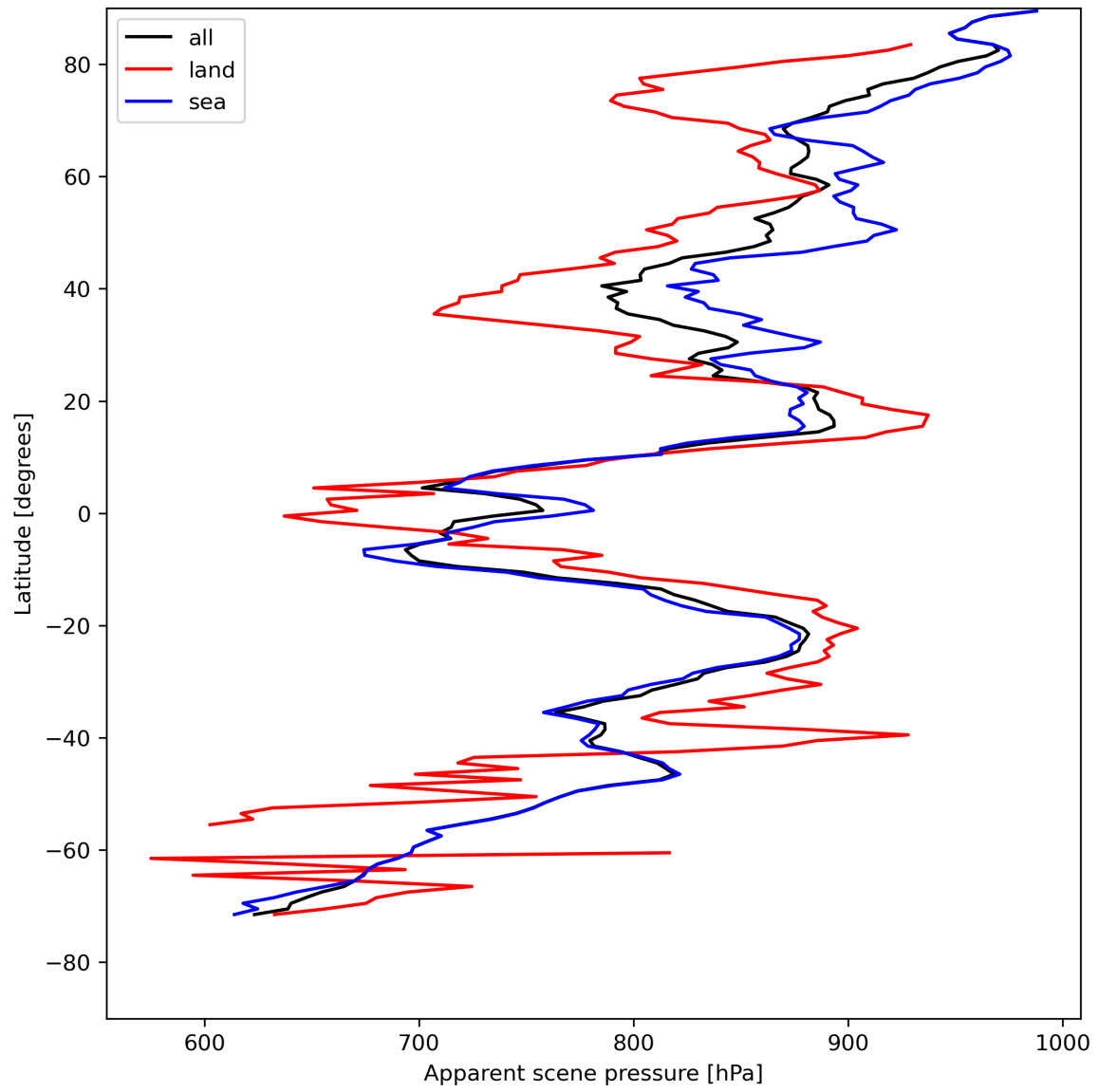
Figure 19: Zonal average of “Apparent scene pressure” for 2024-05-03 to 2024-05-05.
