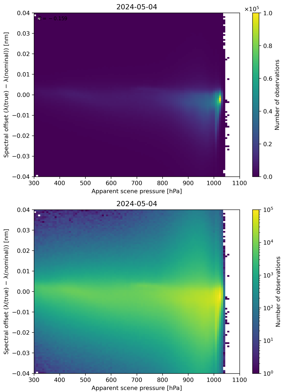
Figure 67: Scatter density plot of “Apparent scene pressure” against “Spectral offset ( \lambda(\text{true}) - \lambda(\text{nominal}) )” for 2024-05-03 to 2024-05-05.
