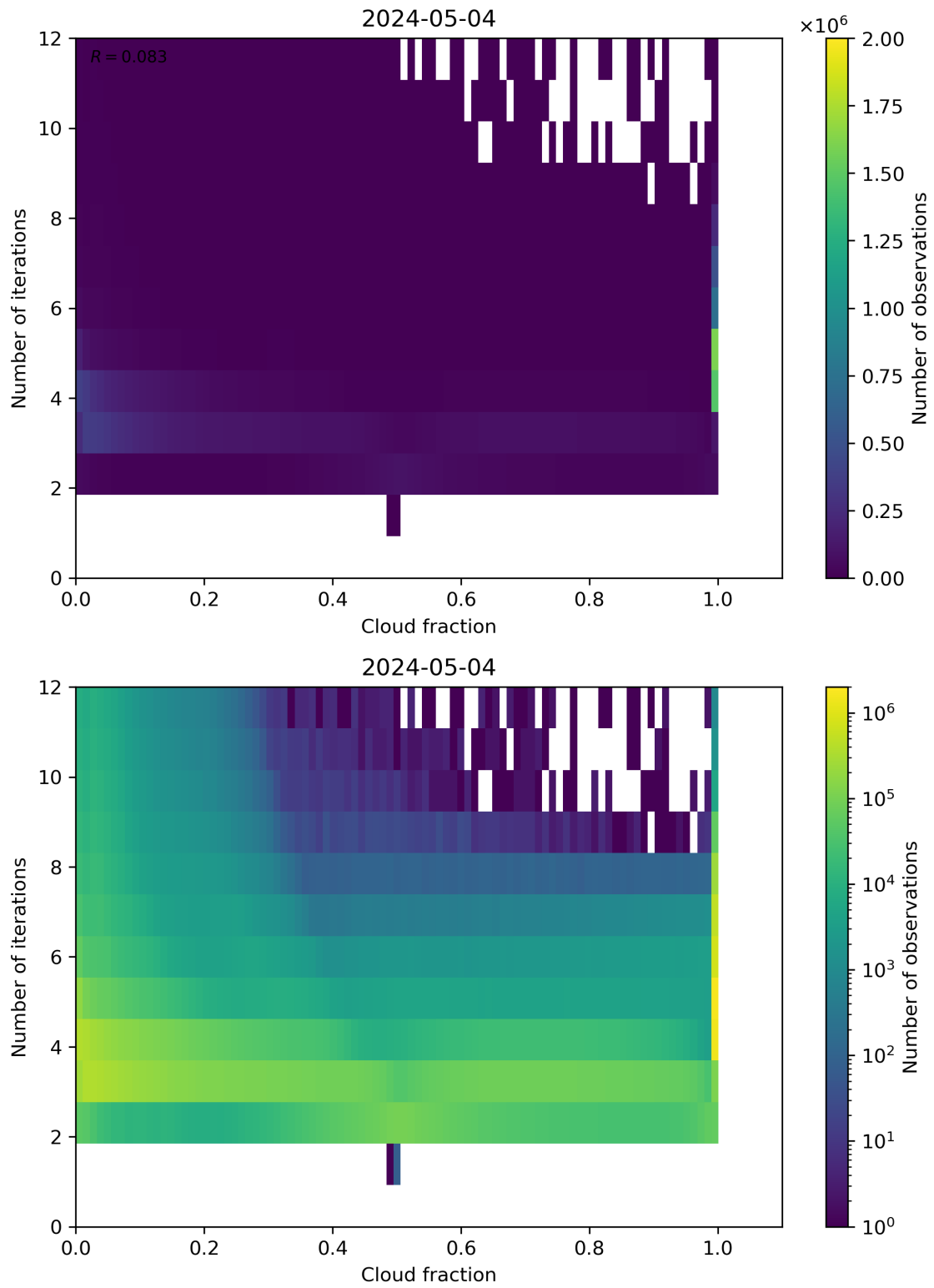
Figure 73: Scatter density plot of “Cloud fraction” against “Number of iterations” for 2024-05-03 to 2024-05-05.
