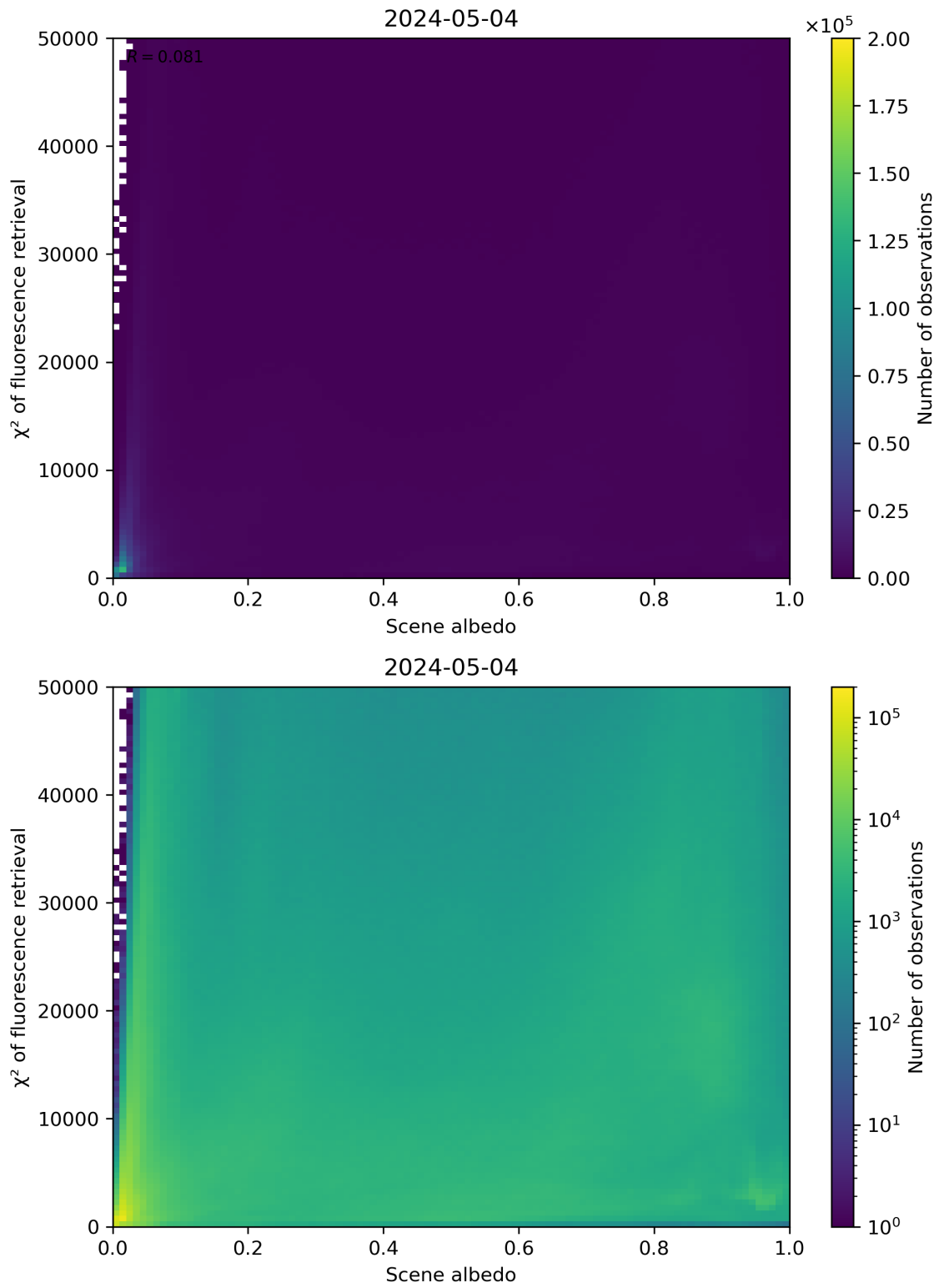
Figure 103: Scatter density plot of “Scene albedo” against “ \chi^2 of fluorescence retrieval” for 2024-05-03 to 2024-05-05.
