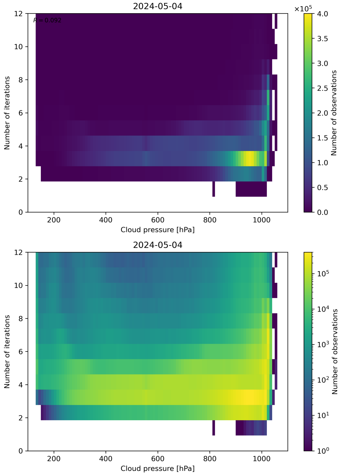
Figure 81: Scatter density plot of “Cloud pressure” against “Number of iterations” for 2024-05-03 to 2024-05-05.
