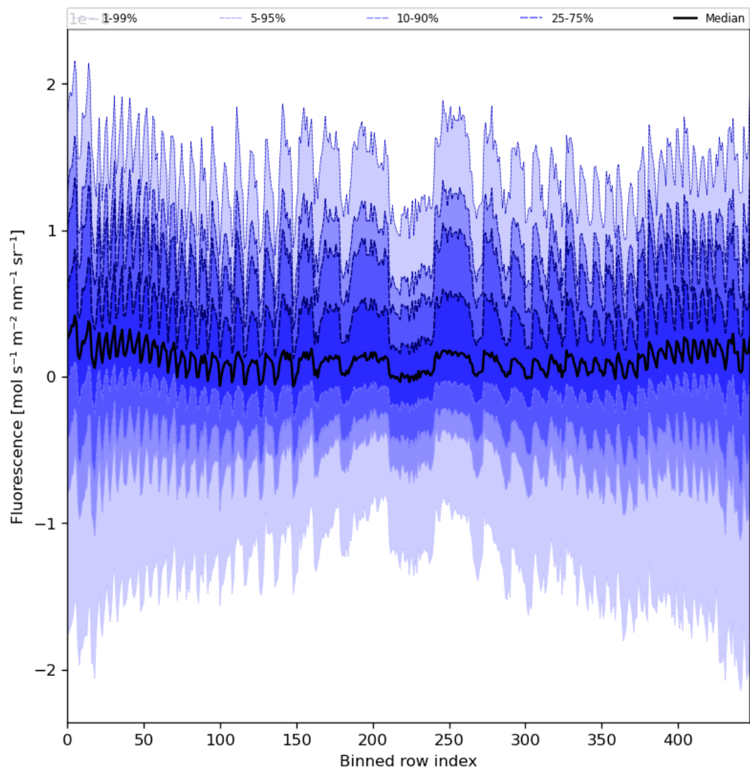
Figure 57: Along track statistics of “Fluorescence” for 2024-05-03 to 2024-05-05
