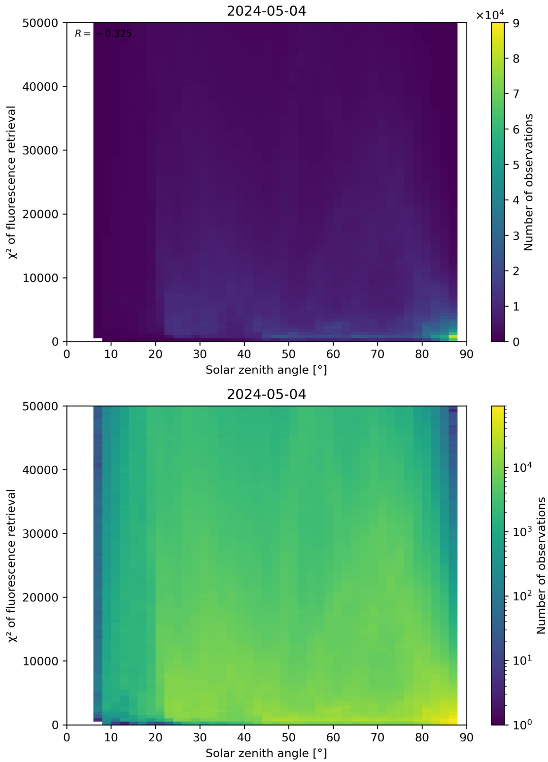
Figure 109: Scatter density plot of “Solar zenith angle” against “ \chi^2 of fluorescence retrieval” for 2024-05-03 to 2024-05-05.
