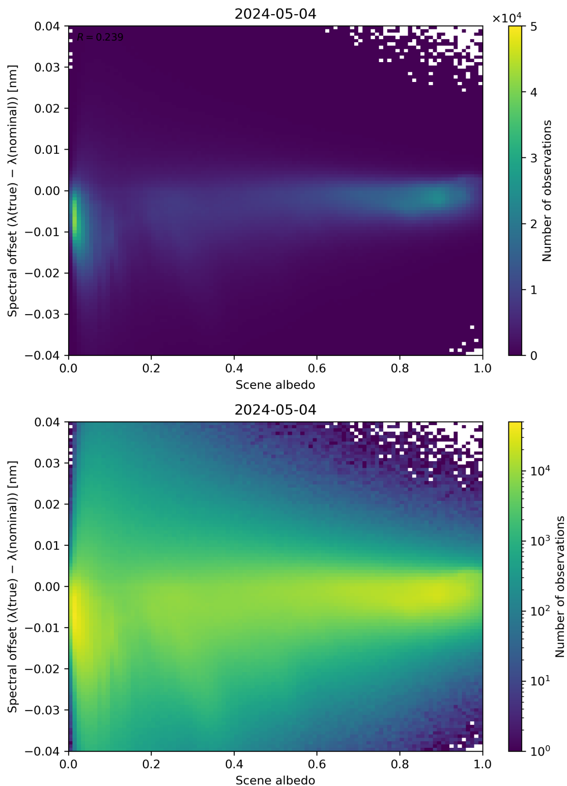
Figure 107: Scatter density plot of “Scene albedo” against “Spectral offset ( \lambda(\text{true}) - \lambda(\text{nominal}) )” for 2024-05-03 to 2024-05-05.
