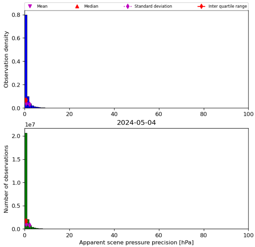
Figure 37: Histogram of “Apparent scene pressure precision” for 2024-05-03 to 2024-05-05
