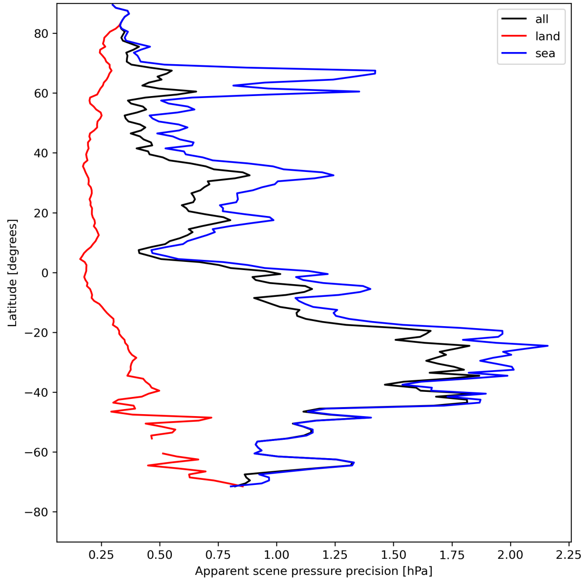
Figure 20: Zonal average of “Apparent scene pressure precision” for 2024-05-05 to 2024-05-07.
