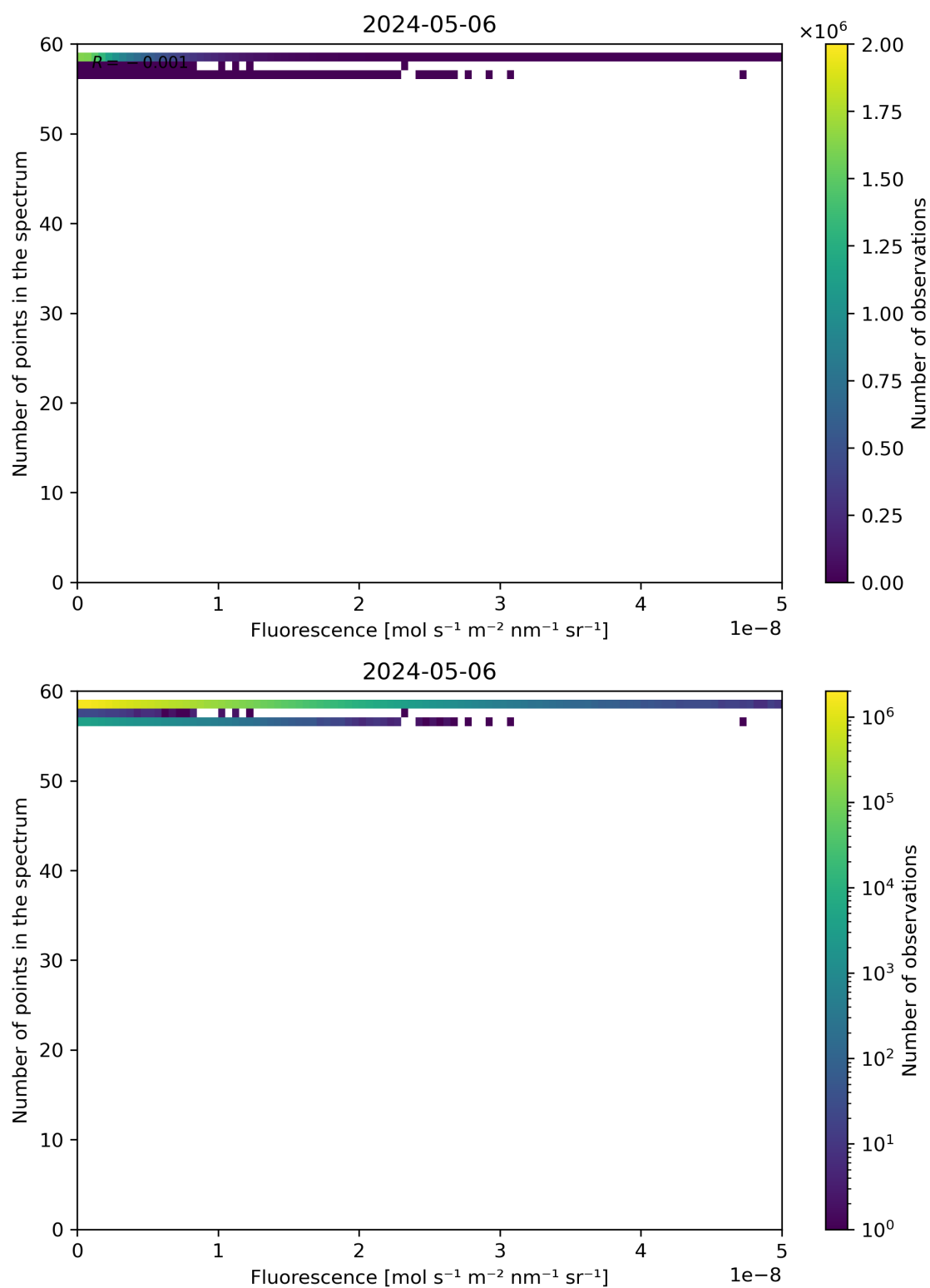
Figure 86: Scatter density plot of “Fluorescence” against “Number of points in the spectrum” for 2024-05-05 to 2024-05-07.
