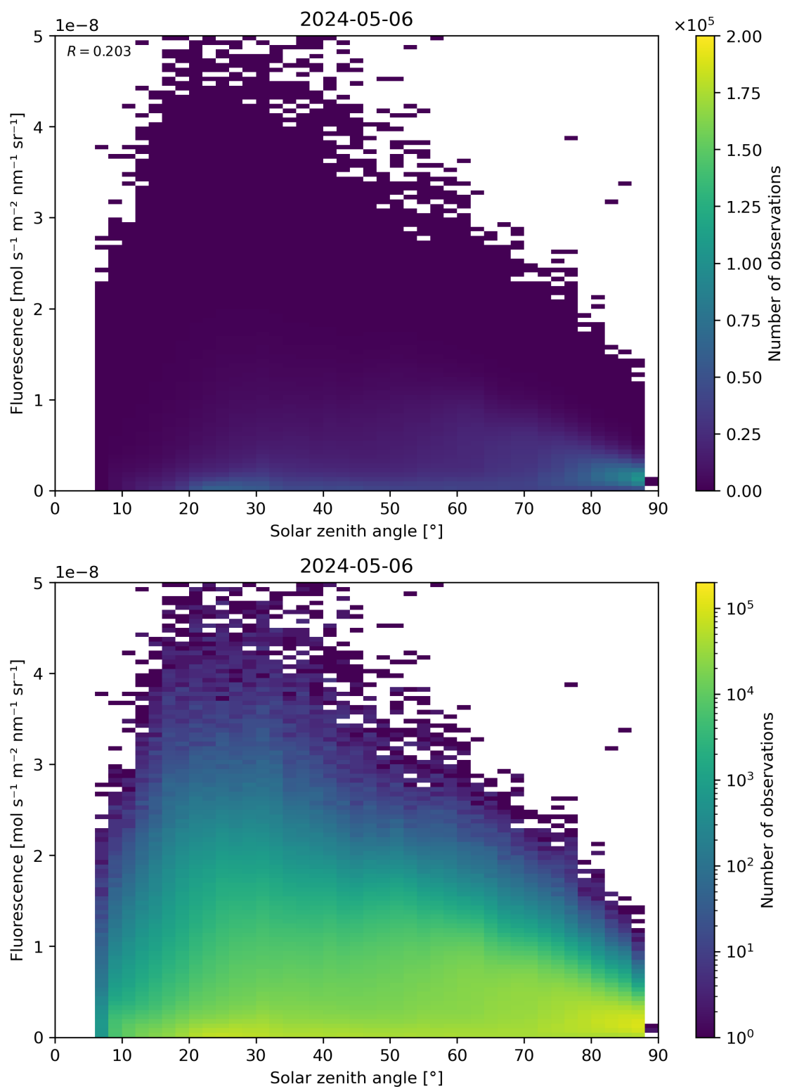
Figure 112: Scatter density plot of “Solar zenith angle” against “Fluorescence” for 2024-05-05 to 2024-05-07.
