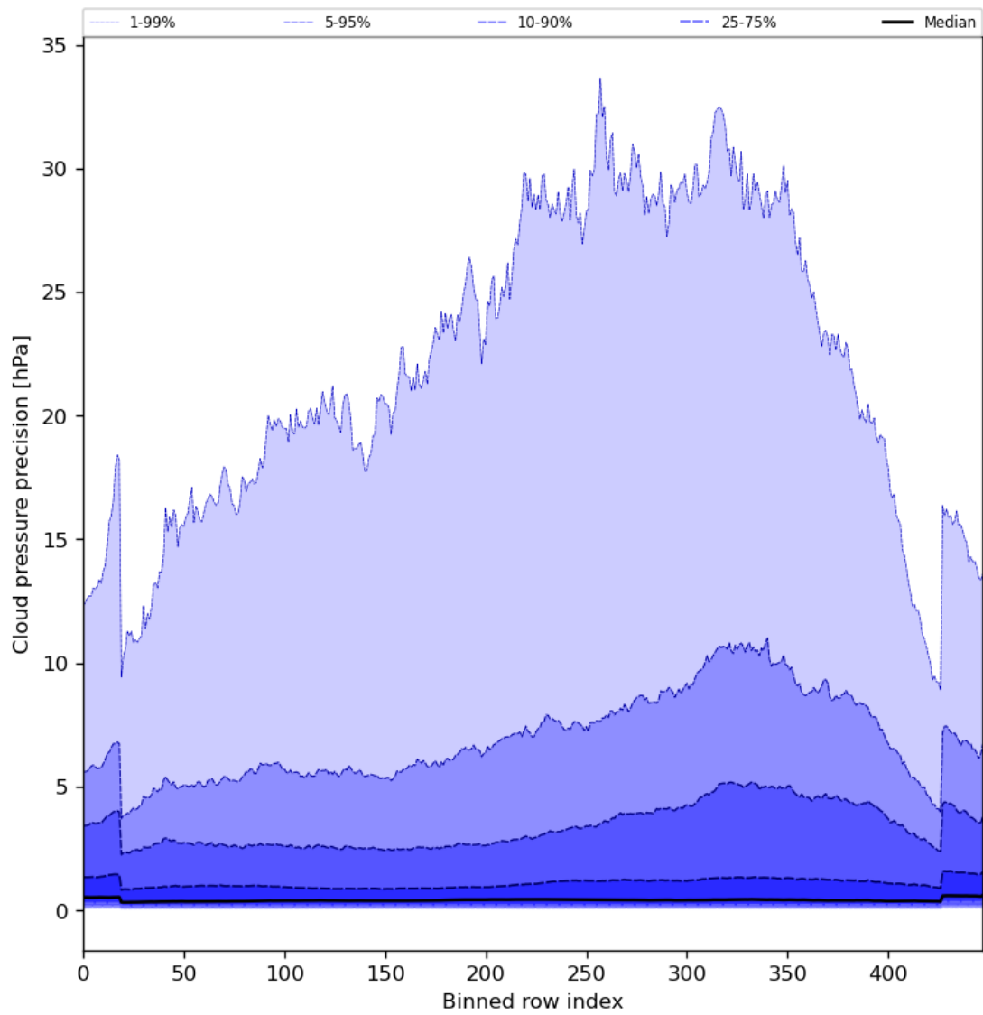
Figure 48: Along track statistics of “Cloud pressure precision” for 2024-05-05 to 2024-05-07
