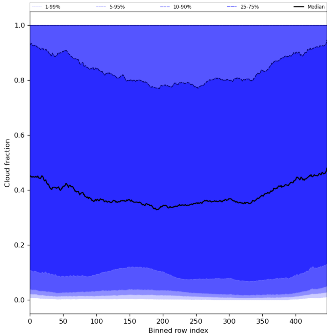
Figure 49: Along track statistics of “Cloud fraction” for 2024-05-05 to 2024-05-07
