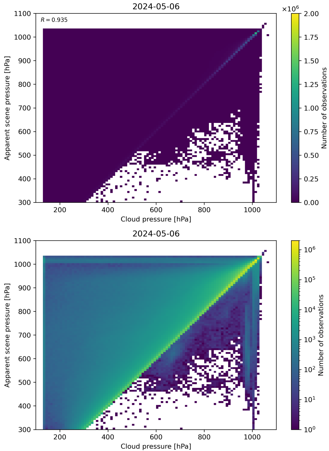
Figure 77: Scatter density plot of “Cloud pressure” against “Apparent scene pressure” for 2024-05-05 to 2024-05-07.
