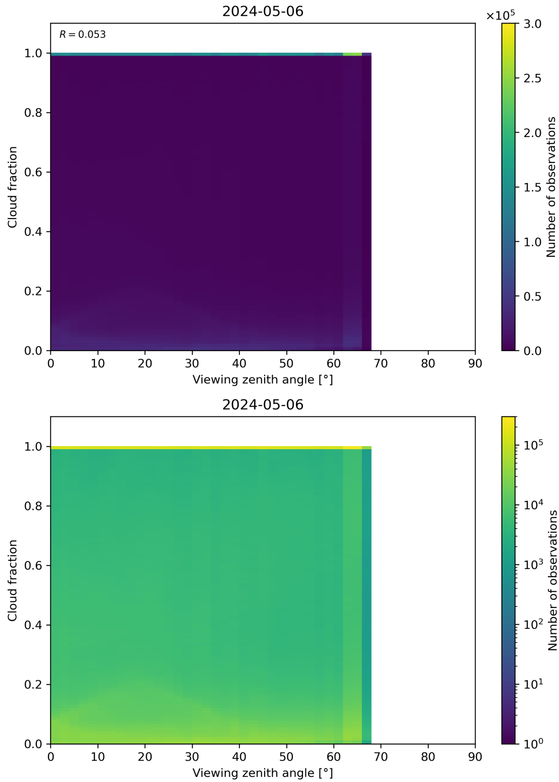
Figure 120: Scatter density plot of “Viewing zenith angle” against “Cloud fraction” for 2024-05-05 to 2024-05-07.
