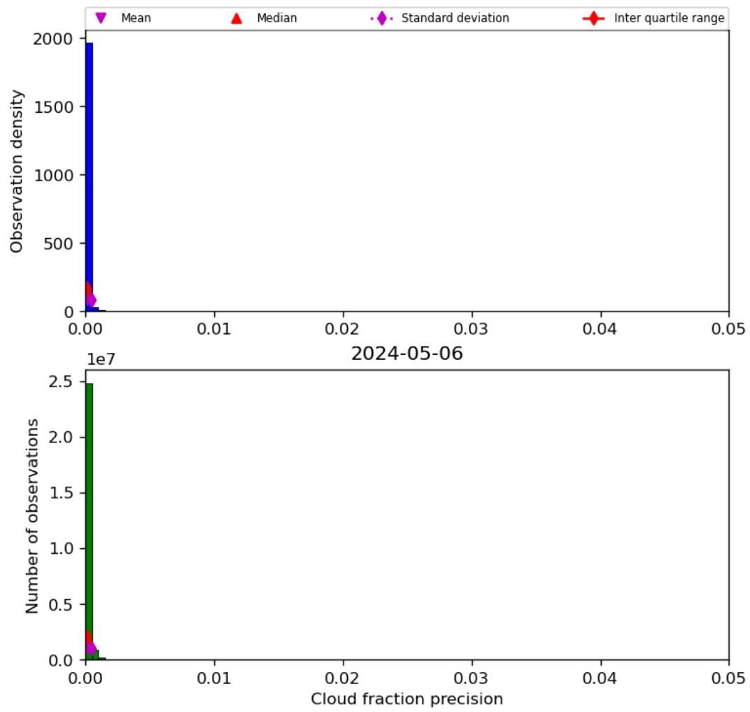
Figure 33: Histogram of “Cloud fraction precision” for 2024-05-05 to 2024-05-07
