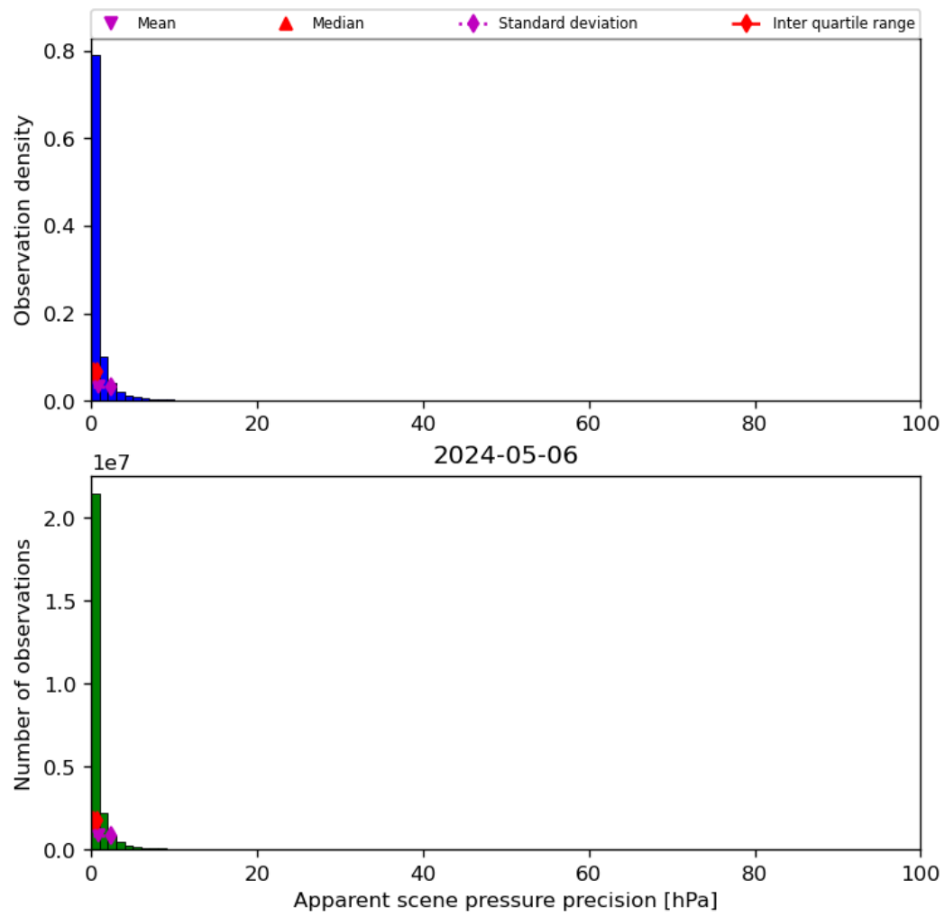
Figure 37: Histogram of “Apparent scene pressure precision” for 2024-05-05 to 2024-05-07
