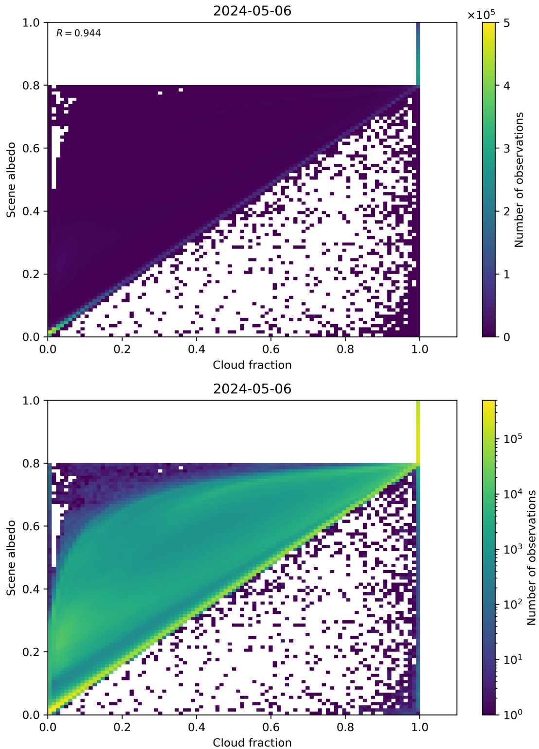
Figure 75: Scatter density plot of “Cloud fraction” against “Scene albedo” for 2024-05-05 to 2024-05-07.
