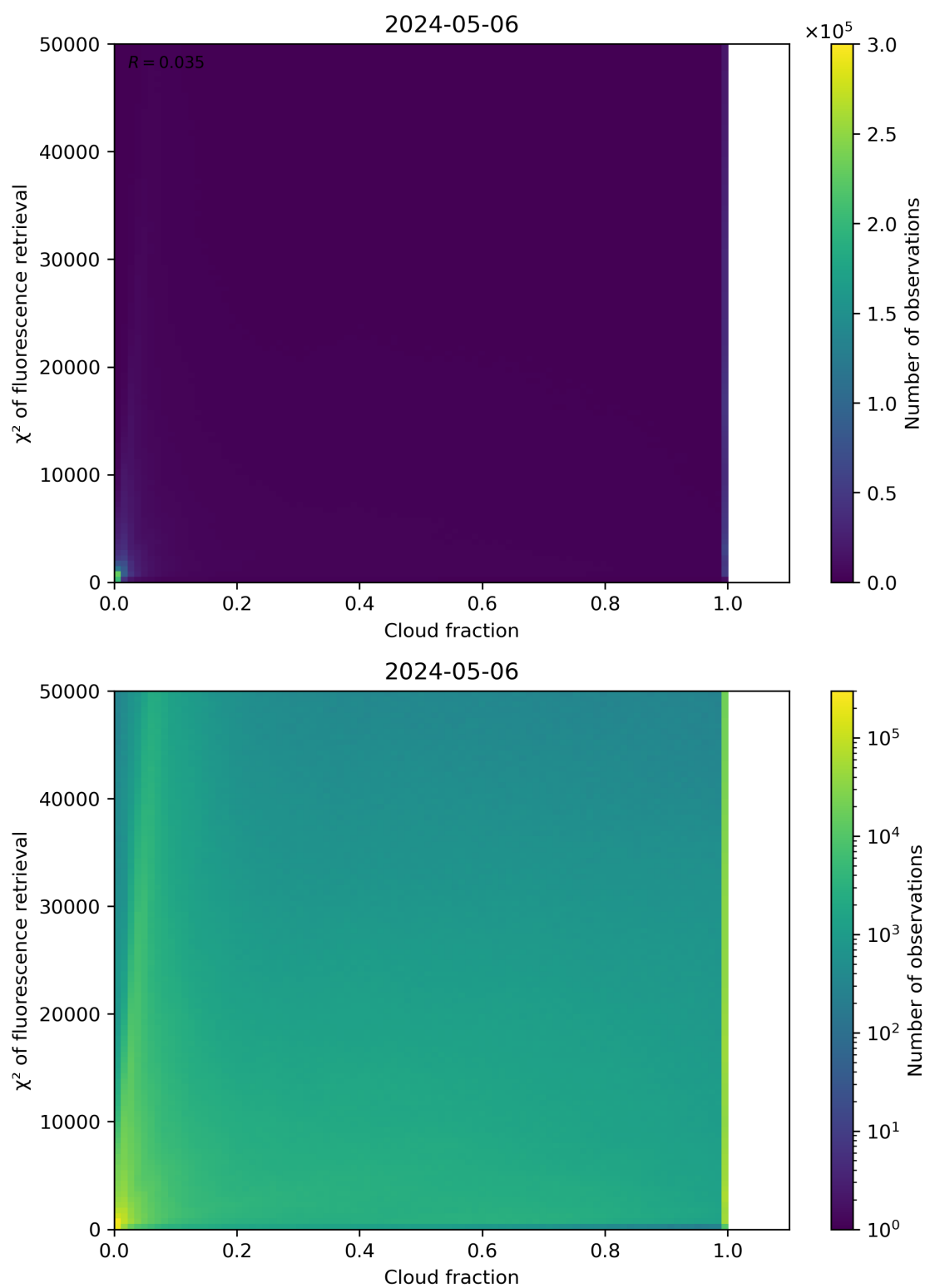
Figure 71: Scatter density plot of “Cloud fraction” against “ \chi^2 of fluorescence retrieval” for 2024-05-05 to 2024-05-07.
