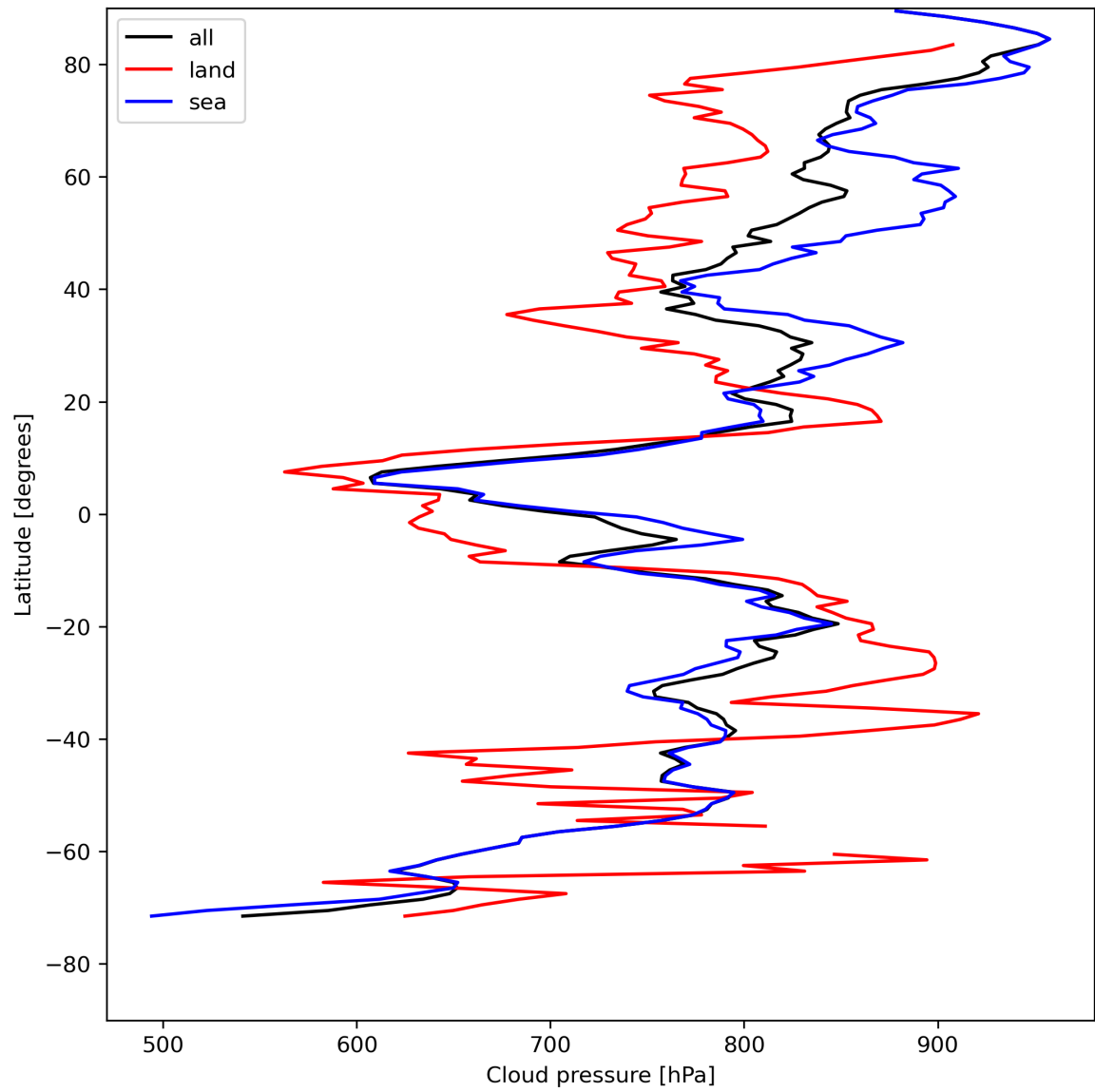
Figure 13: Zonal average of “Cloud pressure” for 2024-05-05 to 2024-05-07.
