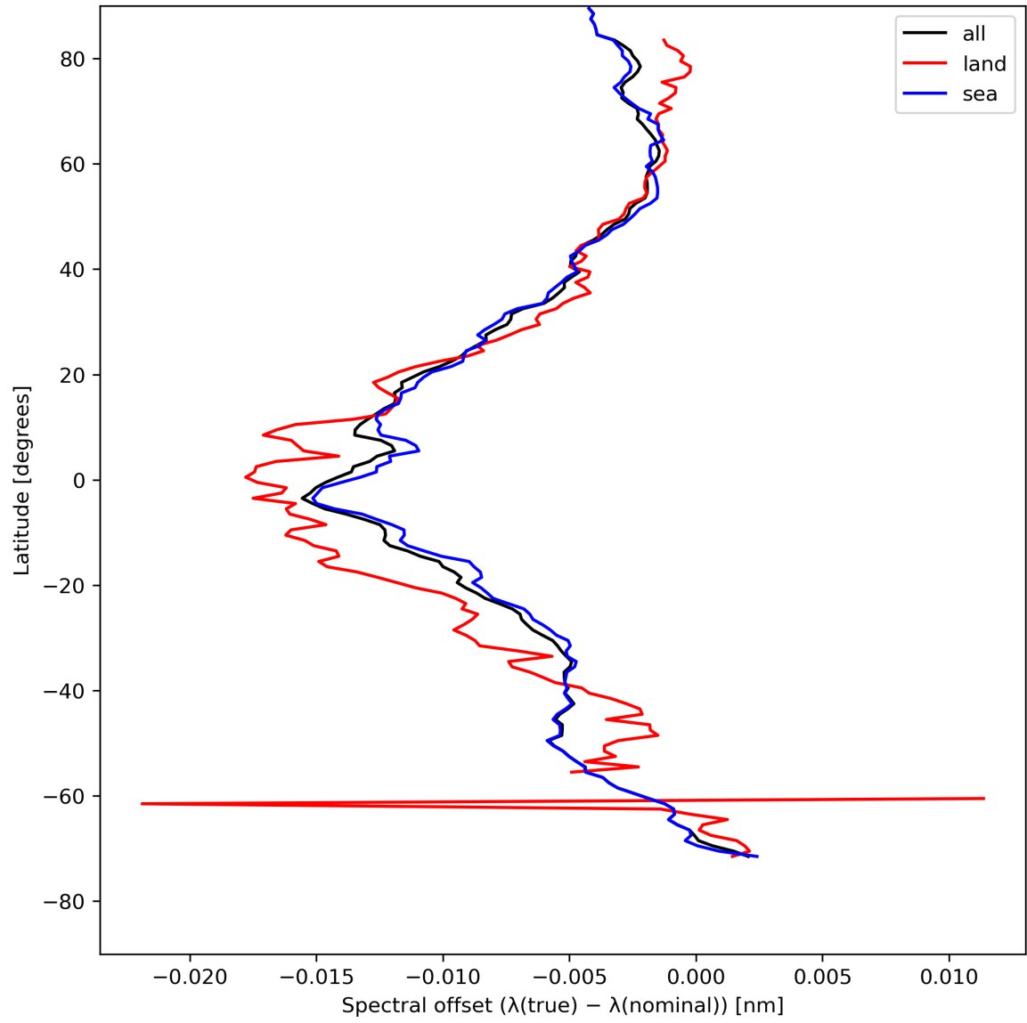
Figure 28: Zonal average of “Spectral offset ( \lambda(\text{true}) - \lambda(\text{nominal}) )” for 2024-05-05 to 2024-05-07.
