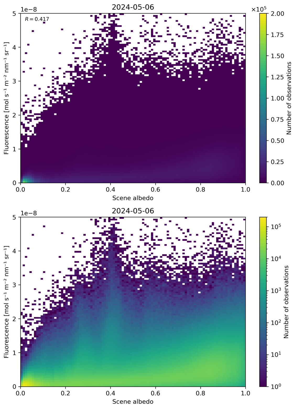
Figure 104: Scatter density plot of “Scene albedo” against “Fluorescence” for 2024-05-05 to 2024-05-07.
