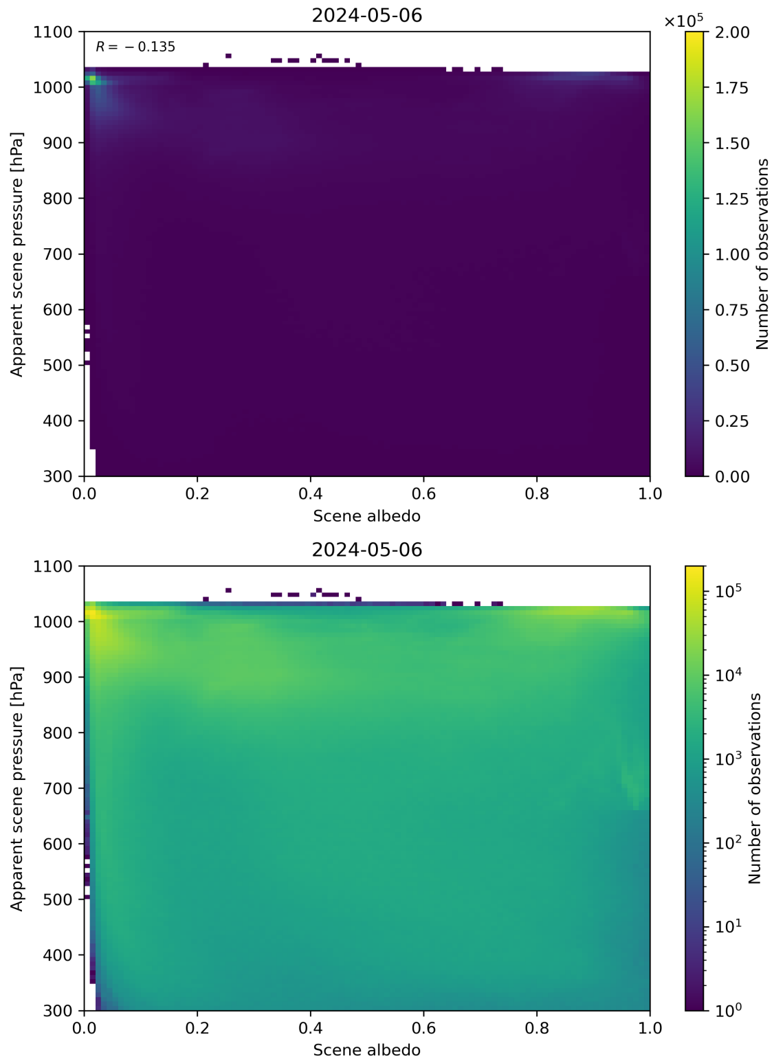
Figure 102: Scatter density plot of “Scene albedo” against “Apparent scene pressure” for 2024-05-05 to 2024-05-07.
