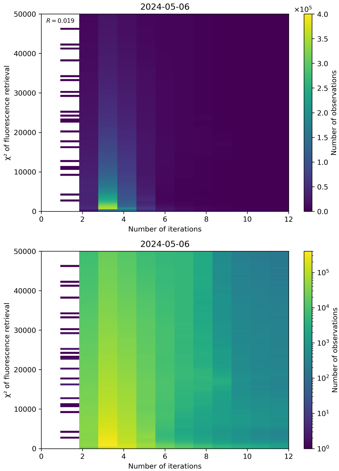
Figure 97: Scatter density plot of “Number of iterations” against “ \chi^2 of fluorescence retrieval” for 2024-05-05 to 2024-05-07.
