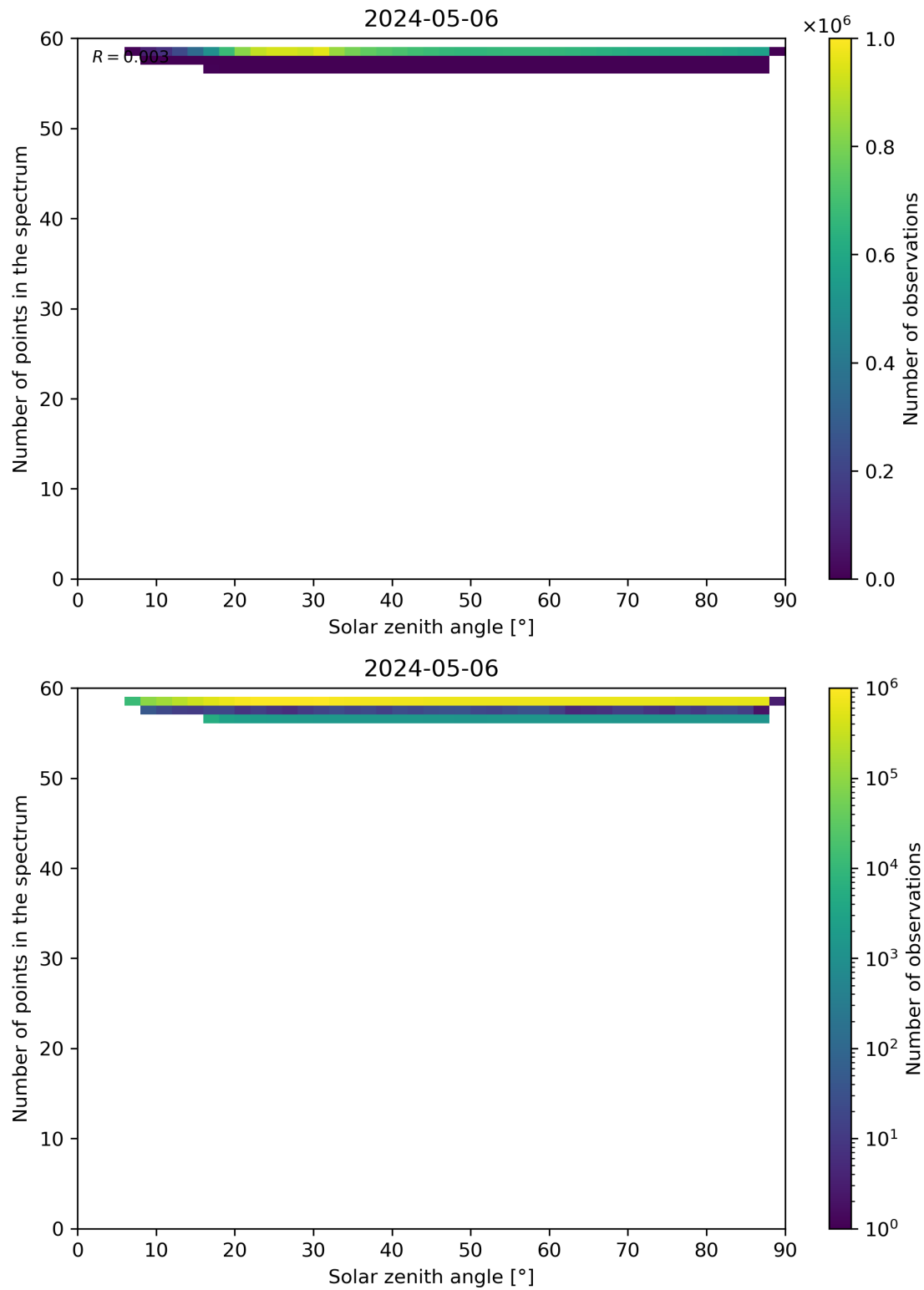
Figure 115: Scatter density plot of “Solar zenith angle” against “Number of points in the spectrum” for 2024-05-05 to 2024-05-07.
