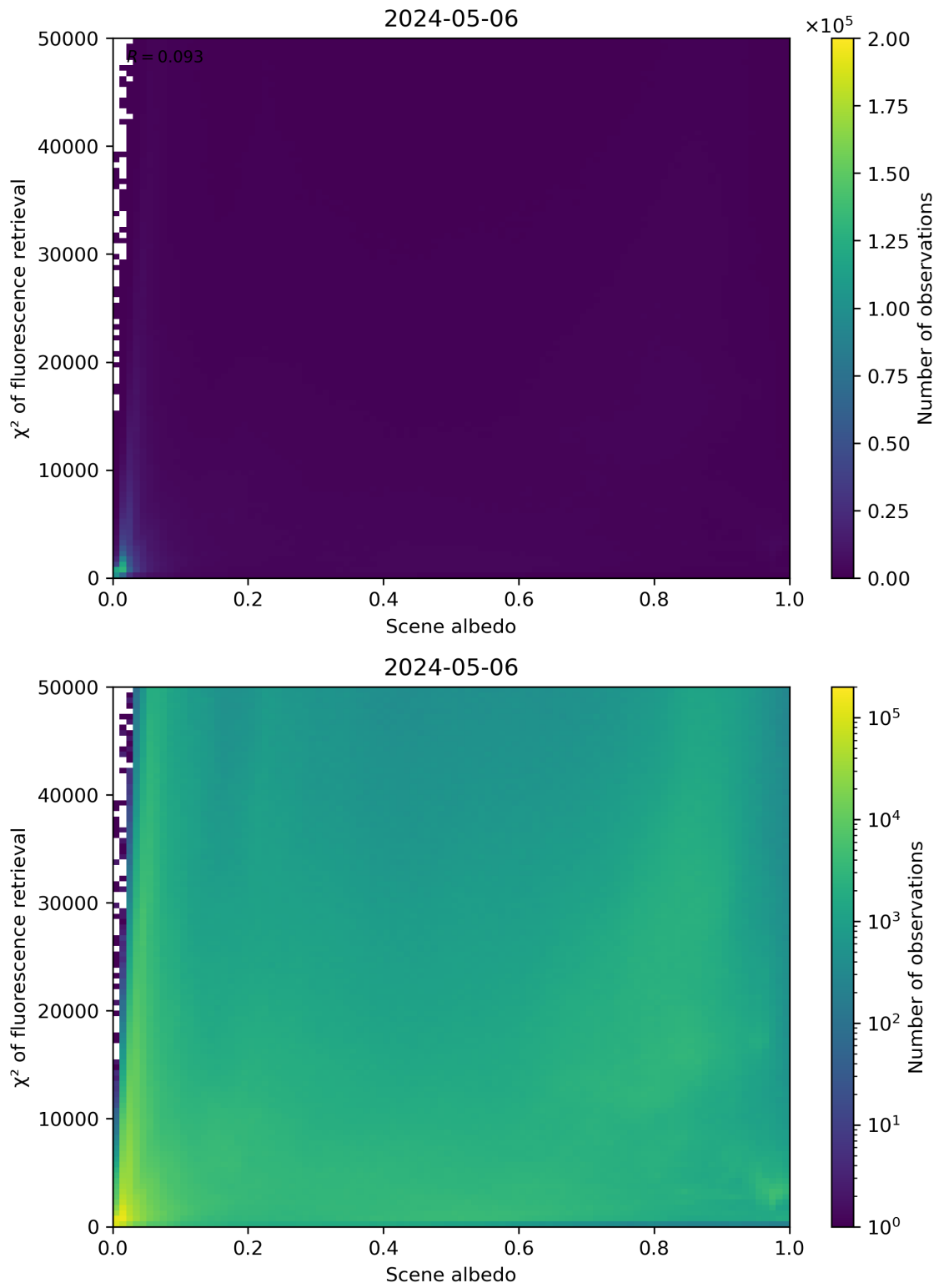
Figure 103: Scatter density plot of “Scene albedo” against “ \chi^2 of fluorescence retrieval” for 2024-05-05 to 2024-05-07.
