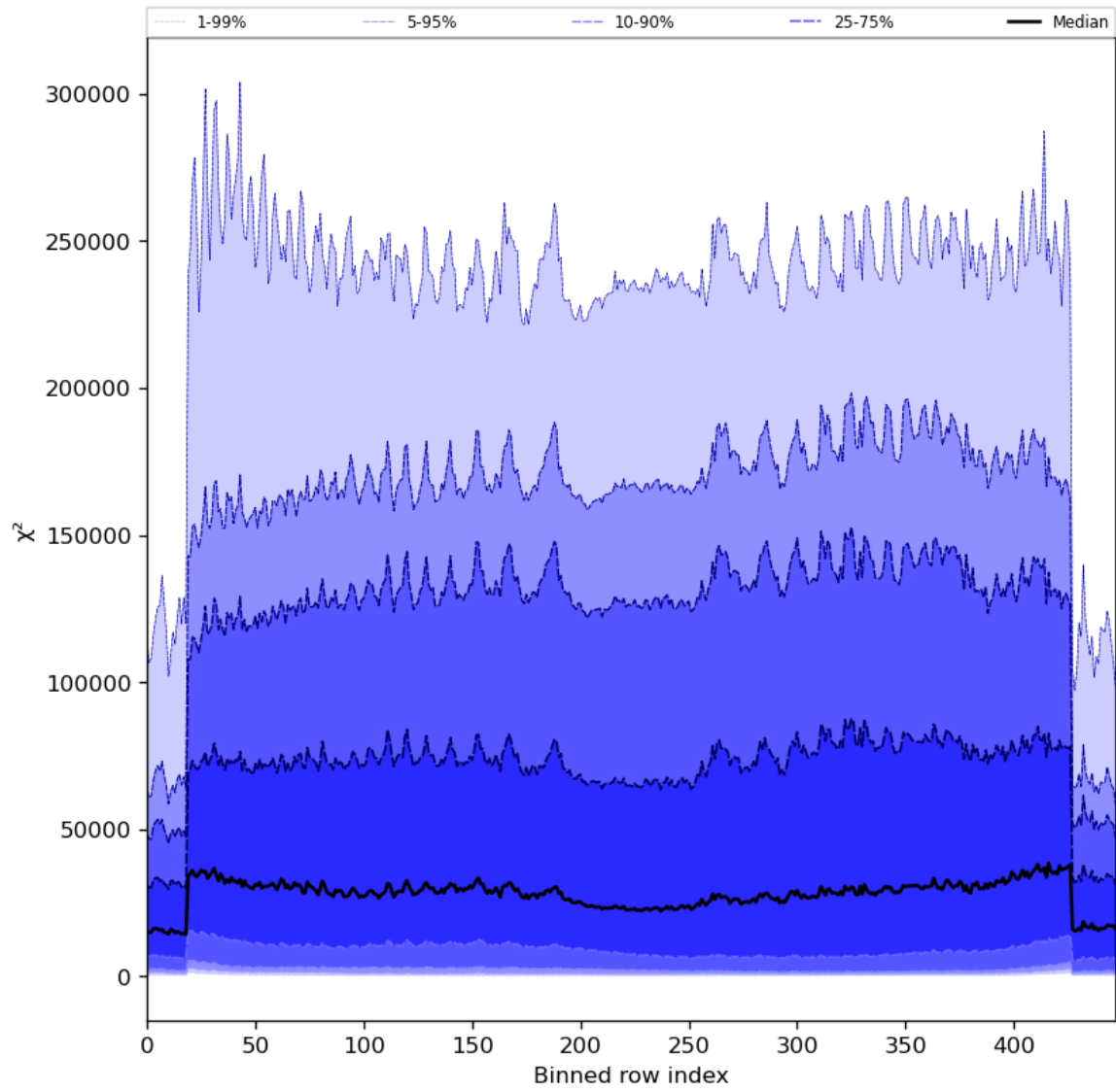
Figure 55: Along track statistics of “ \chi^2 ” for 2024-05-05 to 2024-05-07
