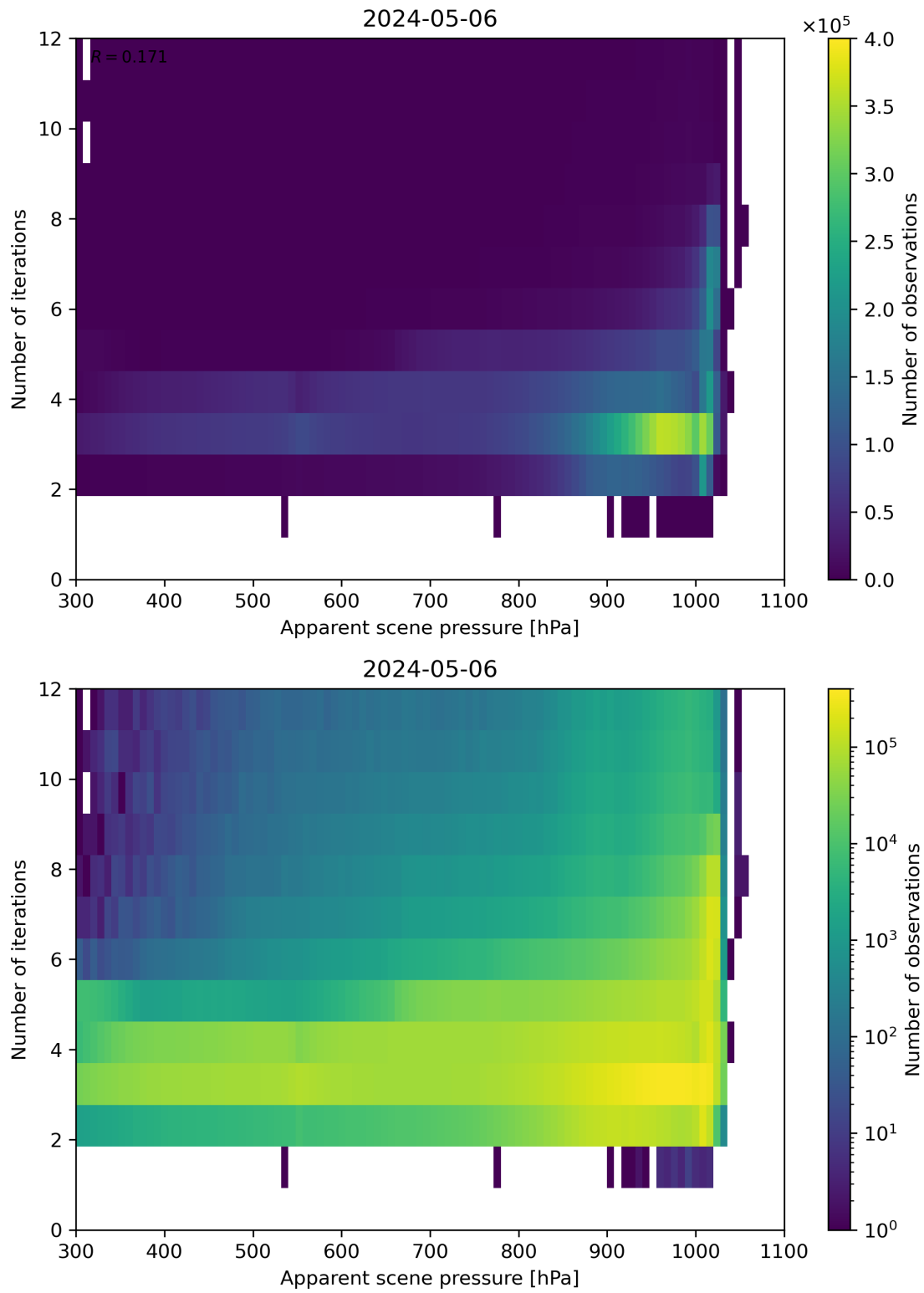
Figure 65: Scatter density plot of “Apparent scene pressure” against “Number of iterations” for 2024-05-05 to 2024-05-07.
