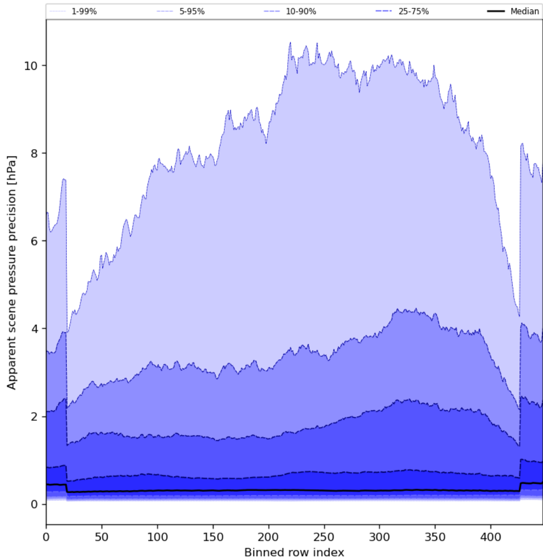
Figure 54: Along track statistics of “Apparent scene pressure precision” for 2024-05-05 to 2024-05-07
