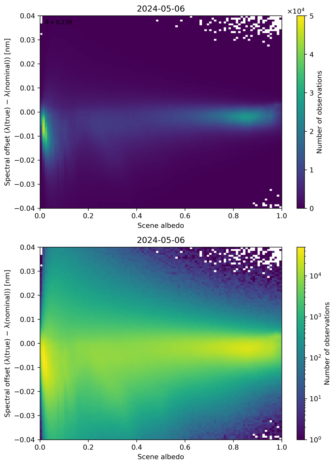
Figure 107: Scatter density plot of “Scene albedo” against “Spectral offset ( \lambda(\text{true}) - \lambda(\text{nominal}) )” for 2024-05-05 to 2024-05-07.
