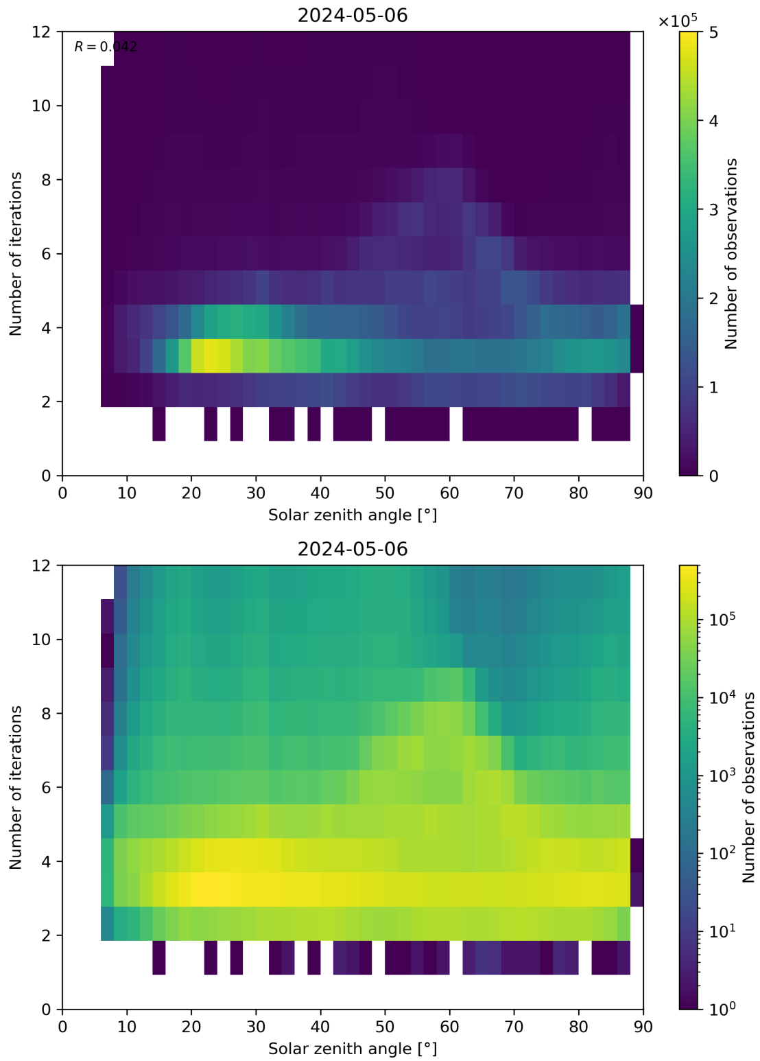
Figure 114: Scatter density plot of “Solar zenith angle” against “Number of iterations” for 2024-05-05 to 2024-05-07.
