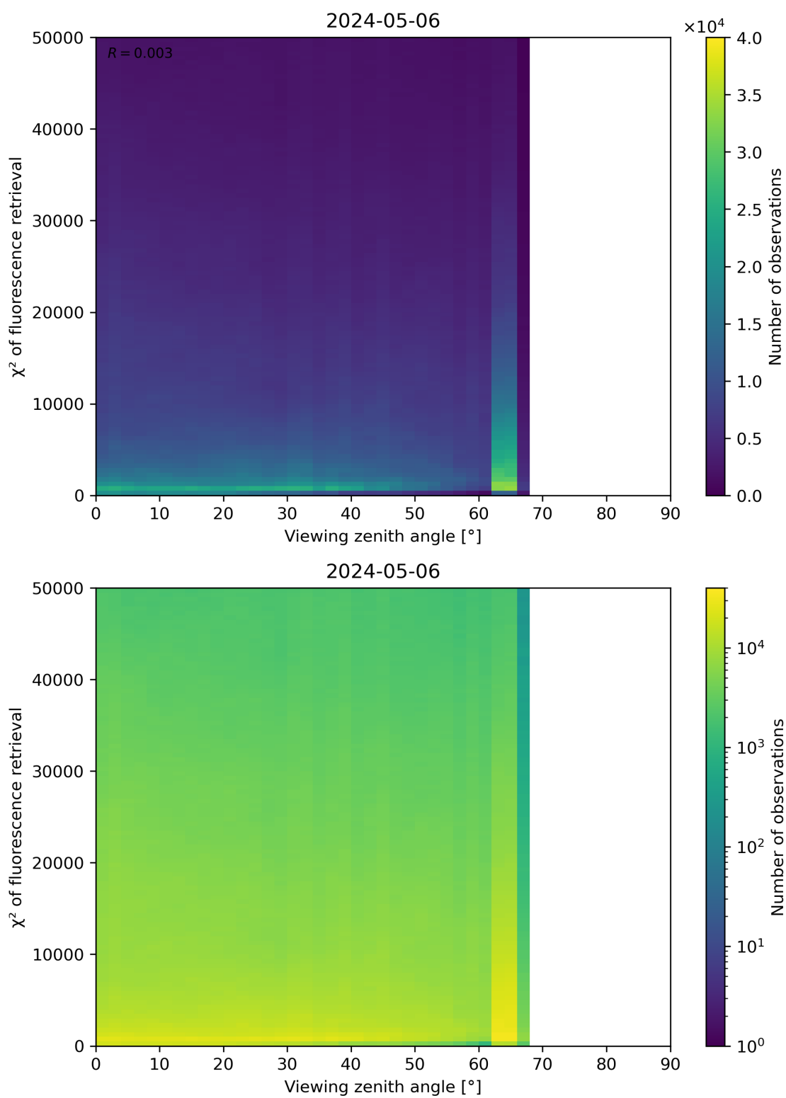
Figure 119: Scatter density plot of “Viewing zenith angle” against “ \chi^2 of fluorescence retrieval” for 2024-05-05 to 2024-05-07.
