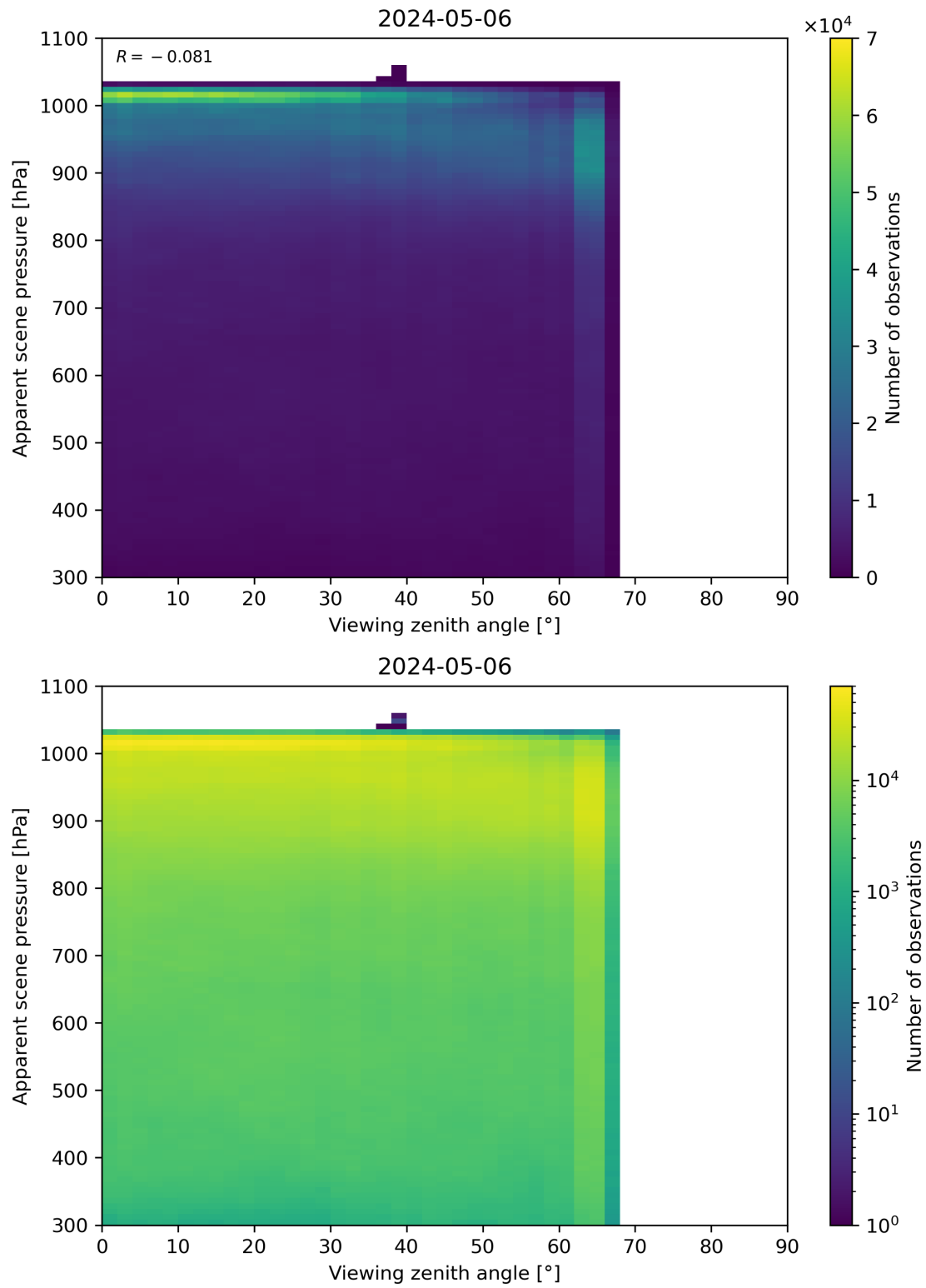
Figure 118: Scatter density plot of “Viewing zenith angle” against “Apparent scene pressure” for 2024-05-05 to 2024-05-07.
