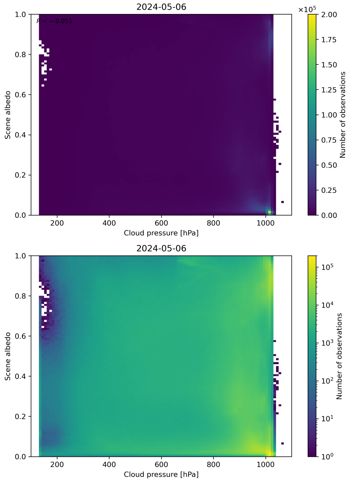
Figure 83: Scatter density plot of “Cloud pressure” against “Scene albedo” for 2024-05-05 to 2024-05-07.
