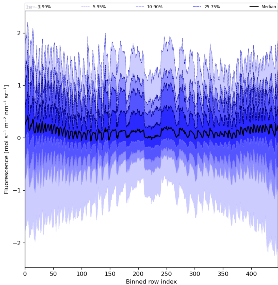
Figure 57: Along track statistics of “Fluorescence” for 2024-05-05 to 2024-05-07
