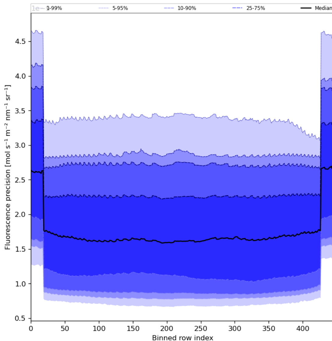
Figure 58: Along track statistics of “Fluorescence precision” for 2024-05-05 to 2024-05-07
