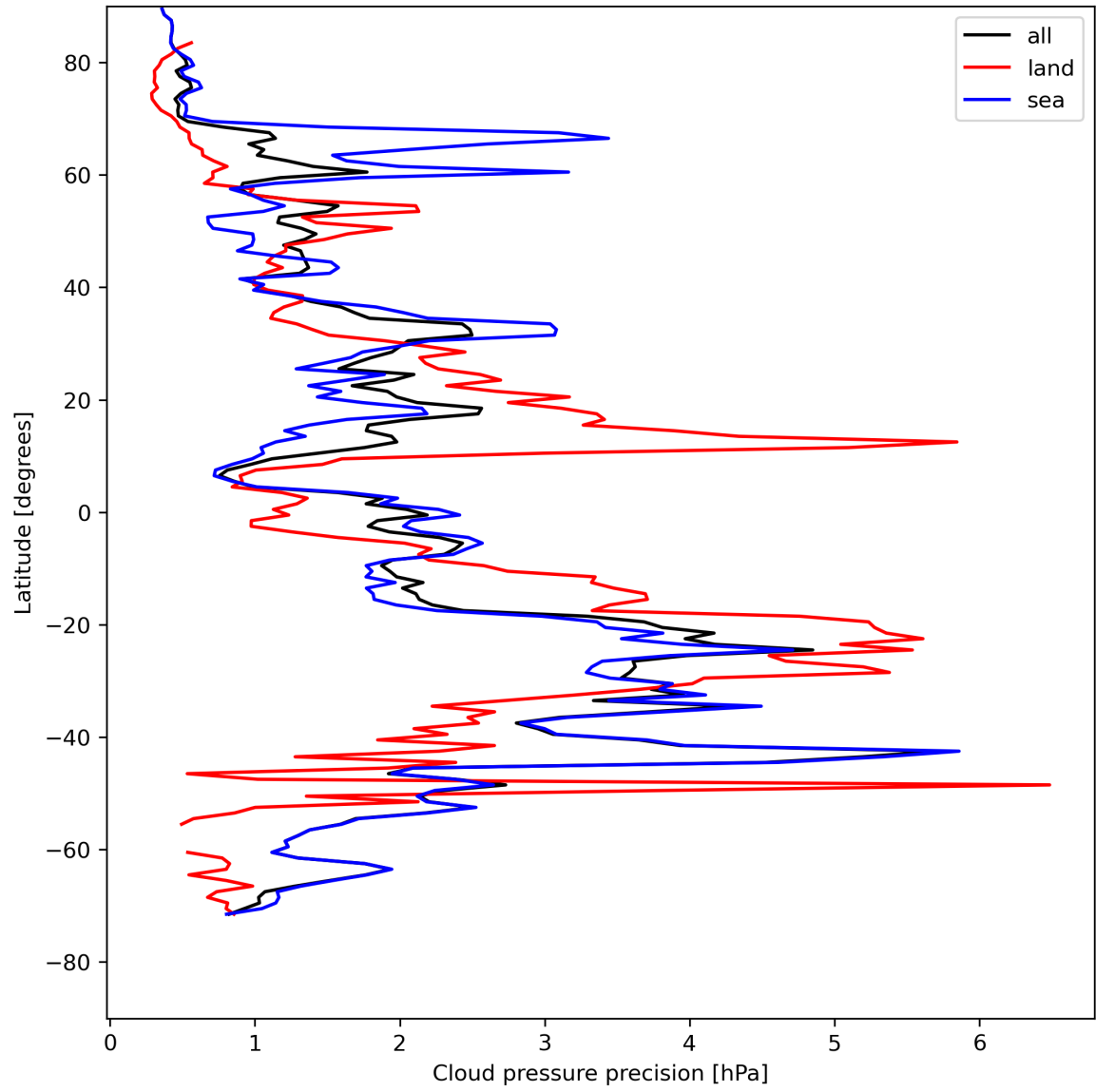
Figure 14: Zonal average of “Cloud pressure precision” for 2024-05-05 to 2024-05-07.
