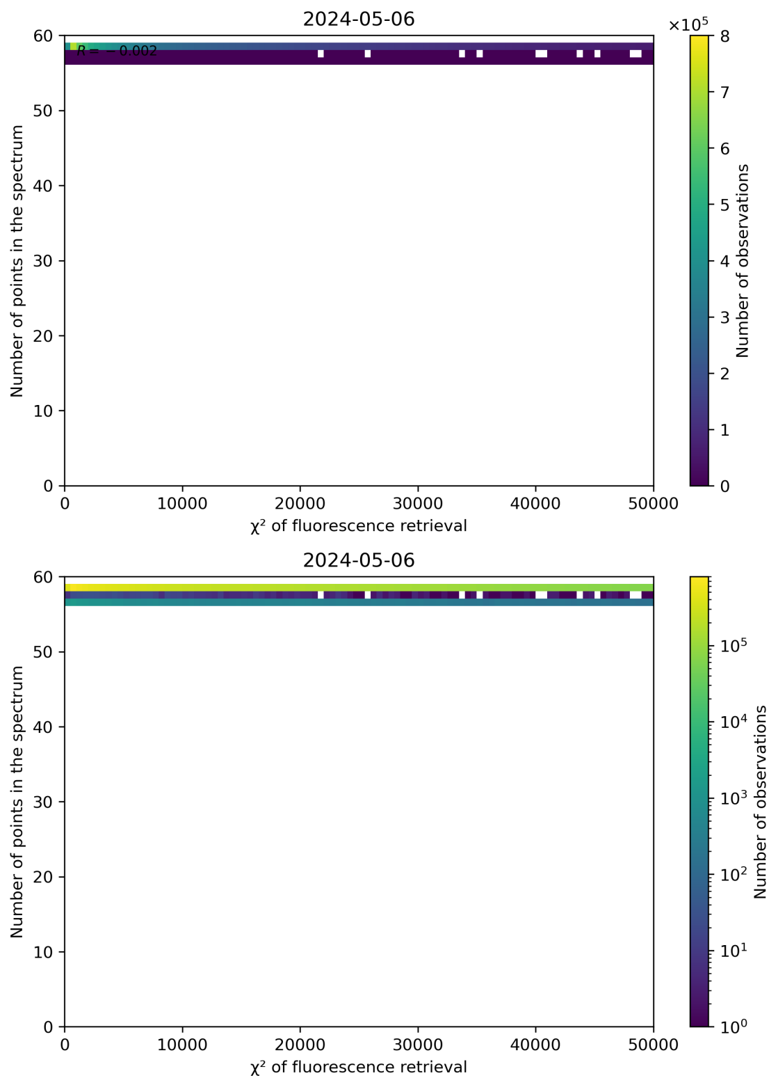
Figure 68: Scatter density plot of " \chi^2 of fluorescence retrieval" against "Number of points in the spectrum" for 2024-05-05 to 2024-05-07.
