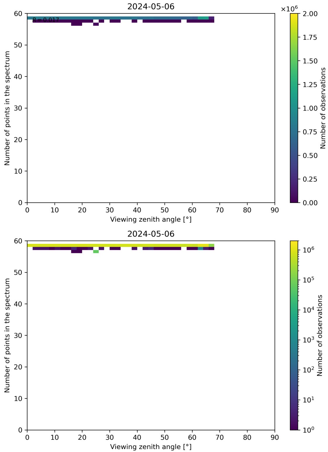
Figure 125: Scatter density plot of “Viewing zenith angle” against “Number of points in the spectrum” for 2024-05-05 to 2024-05-07.
