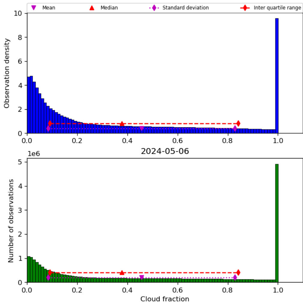
Figure 32: Histogram of “Cloud fraction” for 2024-05-05 to 2024-05-07
