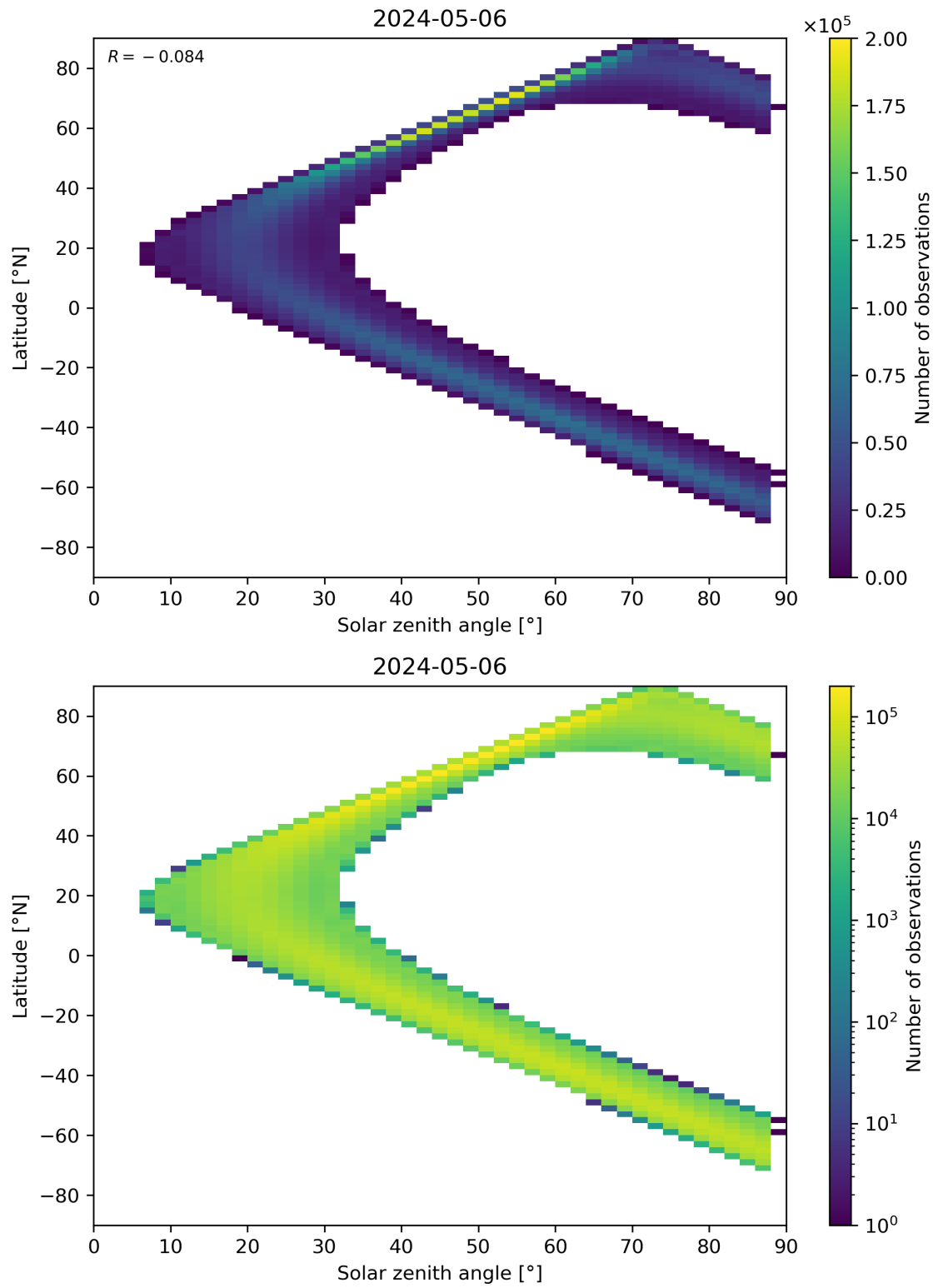
Figure 113: Scatter density plot of “Solar zenith angle” against “Latitude” for 2024-05-05 to 2024-05-07.
