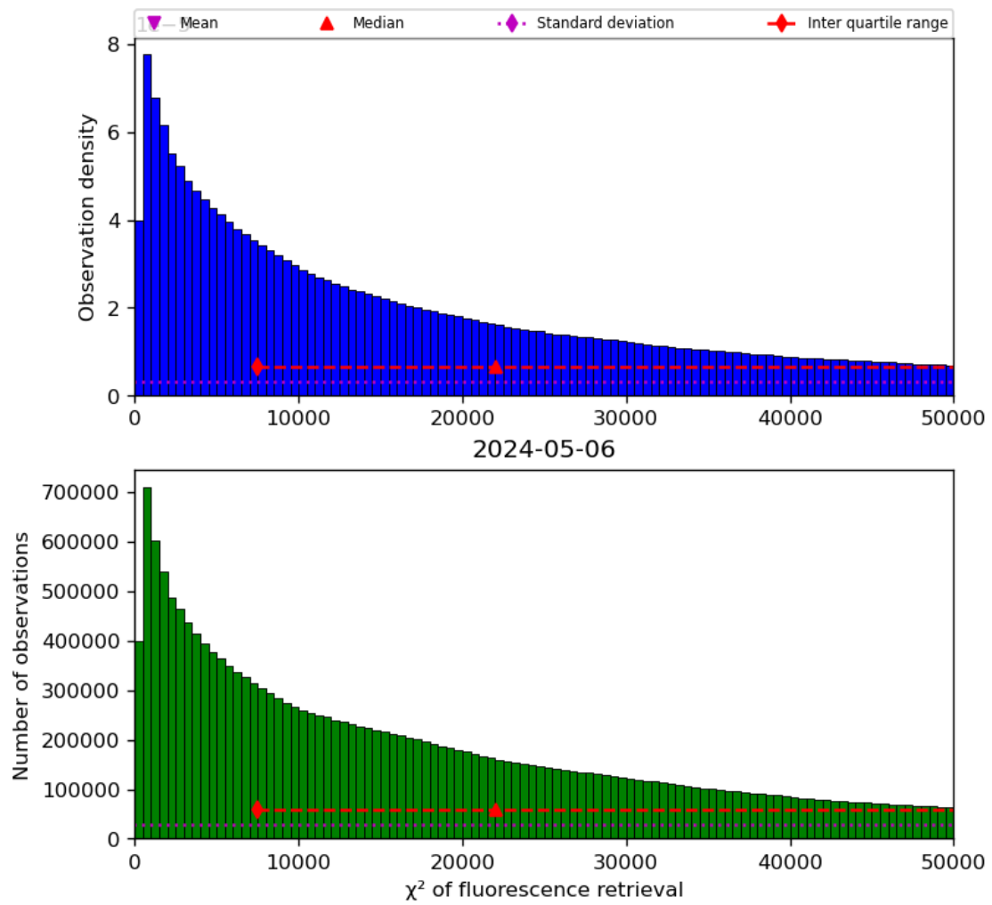
Figure 42: Histogram of “ \chi^2 of fluorescence retrieval” for 2024-05-05 to 2024-05-07
