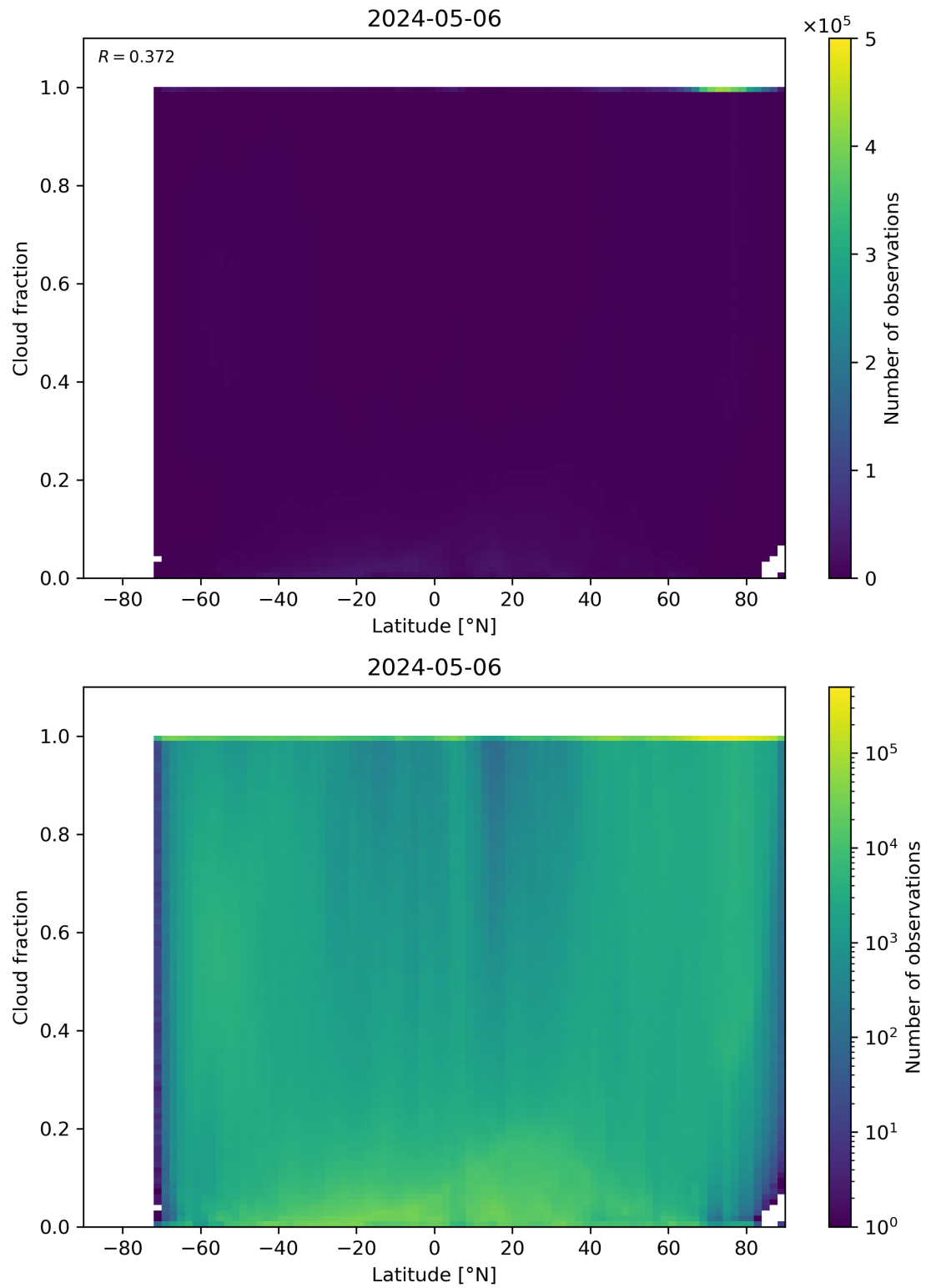
Figure 90: Scatter density plot of “Latitude” against “Cloud fraction” for 2024-05-05 to 2024-05-07.
