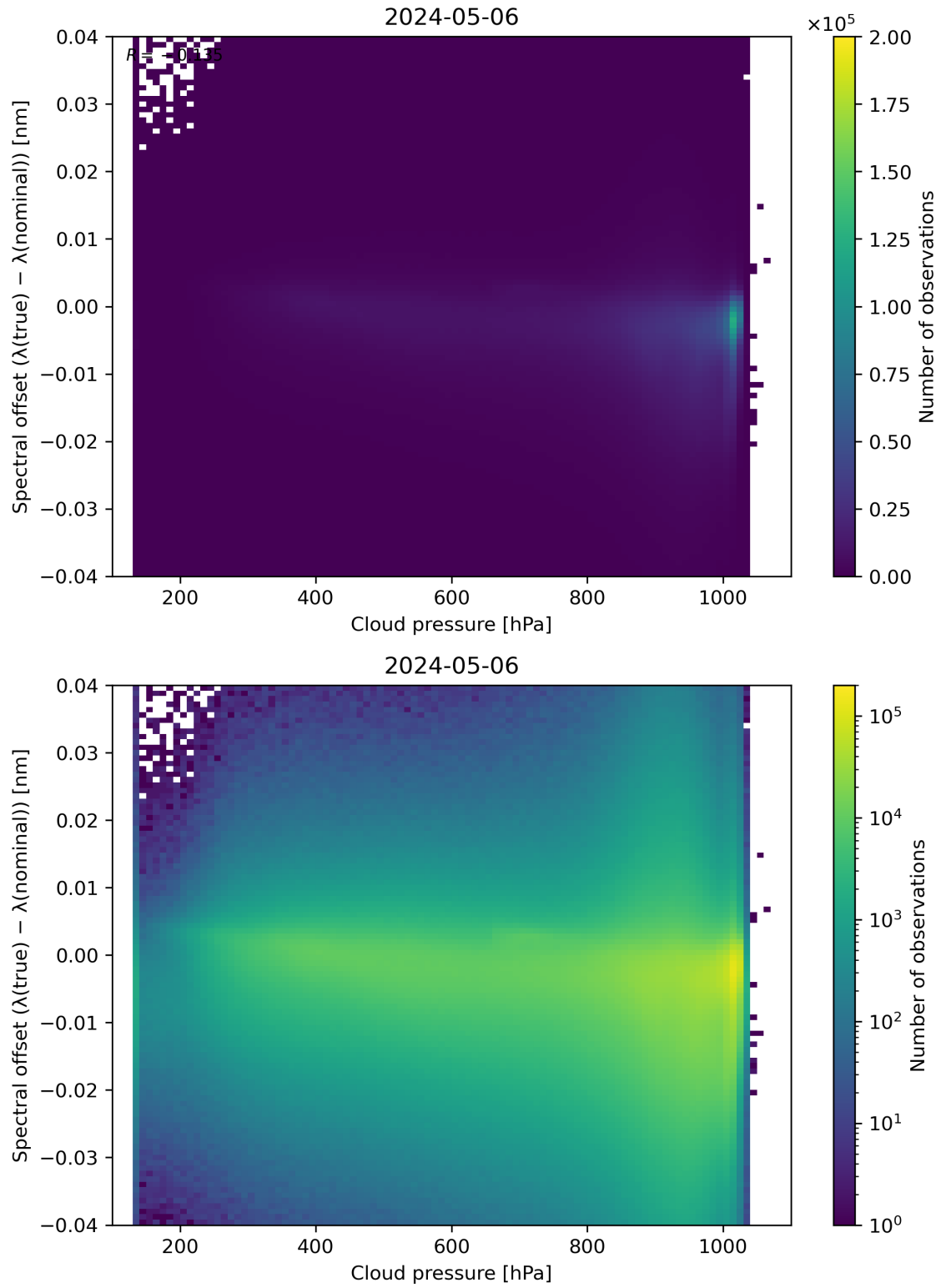
Figure 84: Scatter density plot of “Cloud pressure” against “Spectral offset ( \lambda(\text{true}) - \lambda(\text{nominal}) )” for 2024-05-05 to 2024-05-07.
