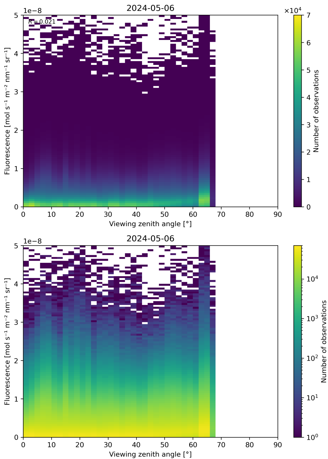
Figure 122: Scatter density plot of “Viewing zenith angle” against “Fluorescence” for 2024-05-05 to 2024-05-07.
