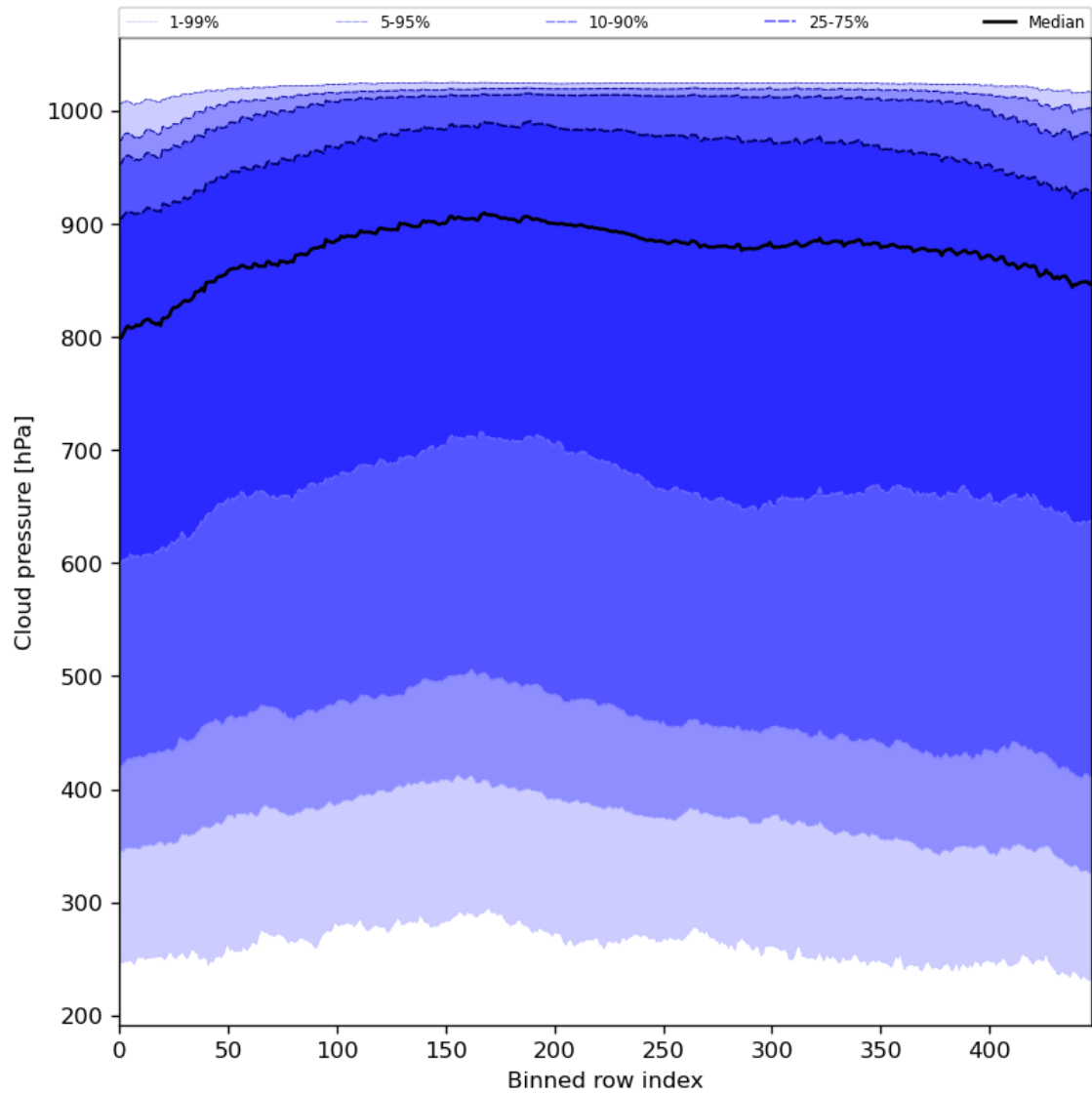
Figure 47: Along track statistics of “Cloud pressure” for 2024-05-05 to 2024-05-07
