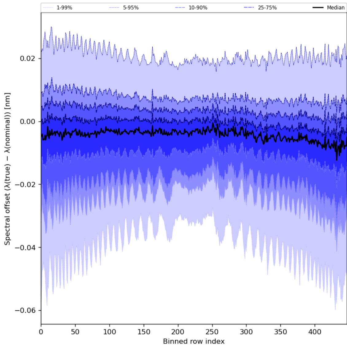
Figure 62: Along track statistics of “Spectral offset ( \lambda(\text{true}) - \lambda(\text{nominal}) )” for 2024-05-05 to 2024-05-07
