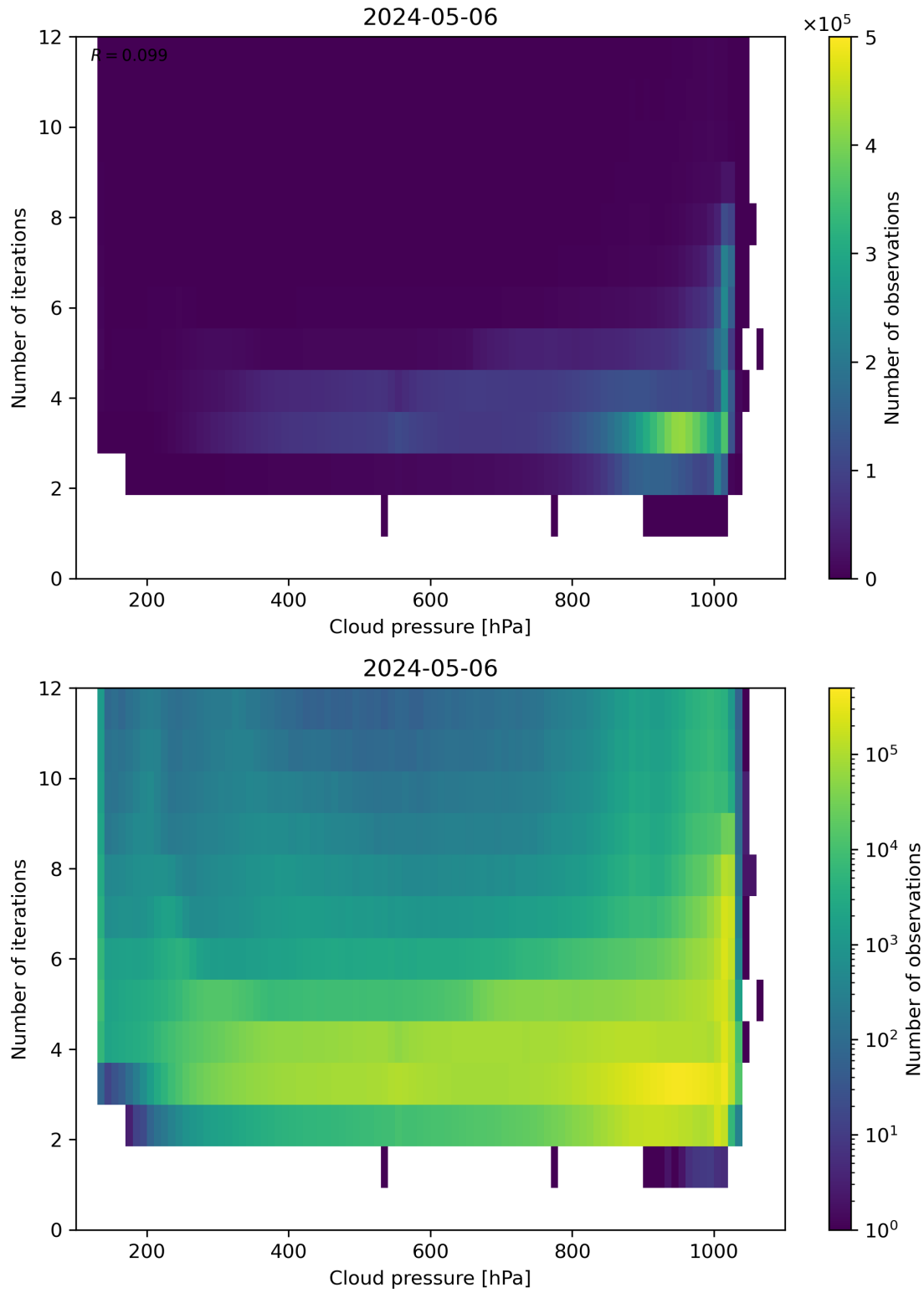
Figure 81: Scatter density plot of “Cloud pressure” against “Number of iterations” for 2024-05-05 to 2024-05-07.
