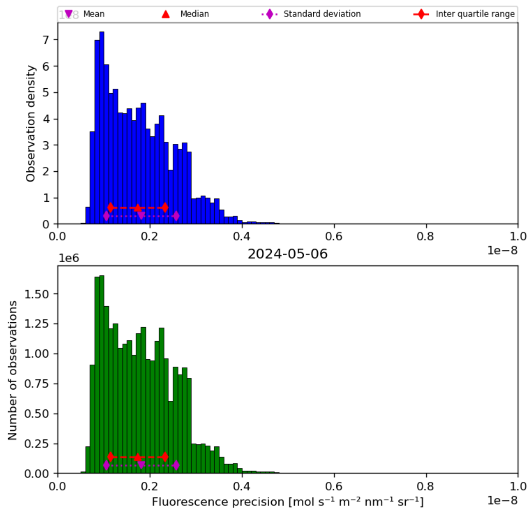
Figure 41: Histogram of “Fluorescence precision” for 2024-05-05 to 2024-05-07
