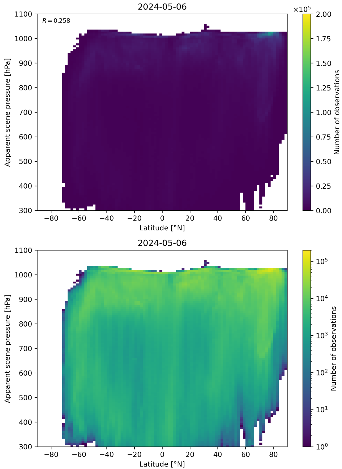
Figure 88: Scatter density plot of “Latitude” against “Apparent scene pressure” for 2024-05-05 to 2024-05-07.
