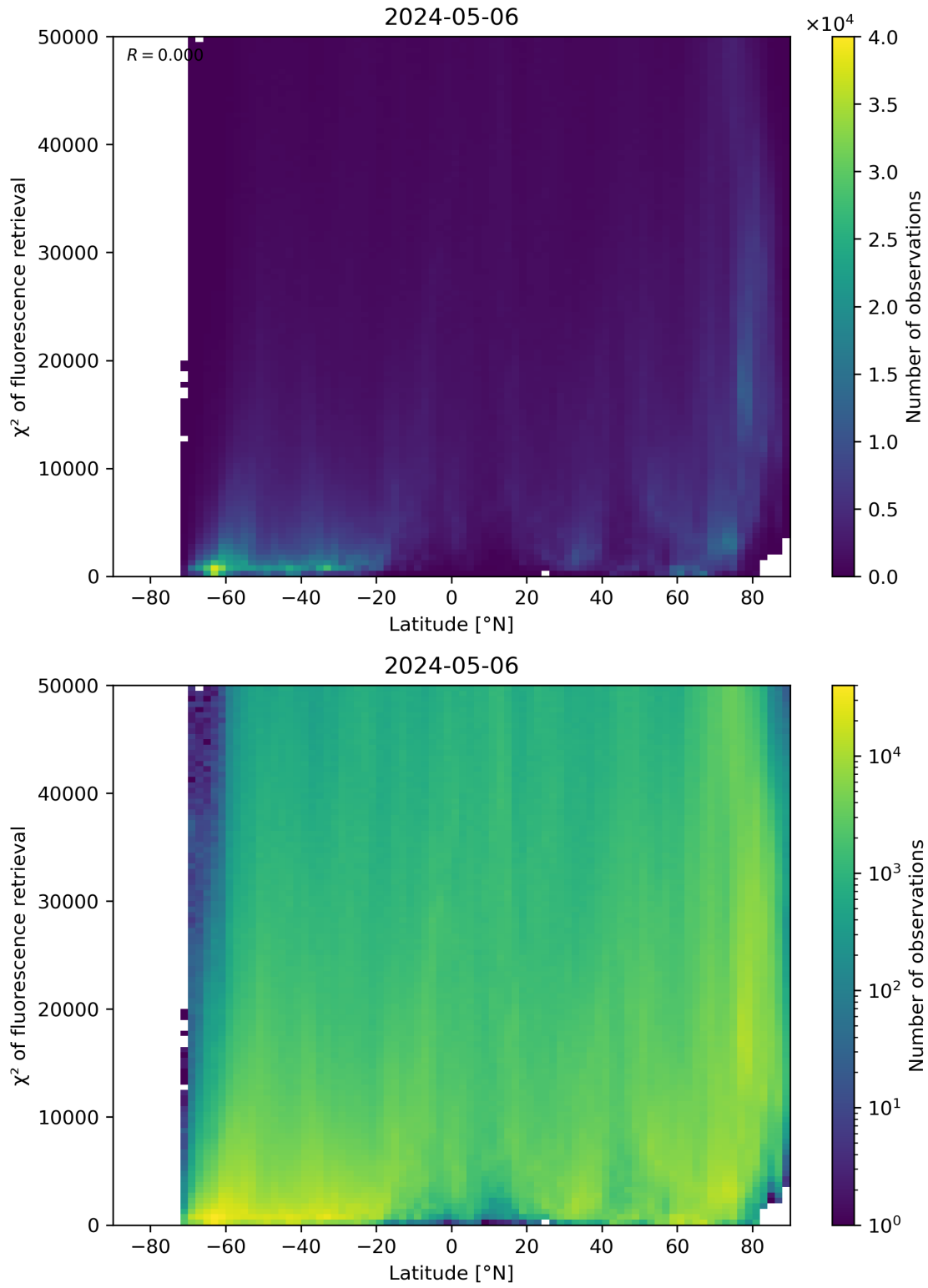
Figure 89: Scatter density plot of “Latitude” against “ \chi^2 of fluorescence retrieval” for 2024-05-05 to 2024-05-07.
