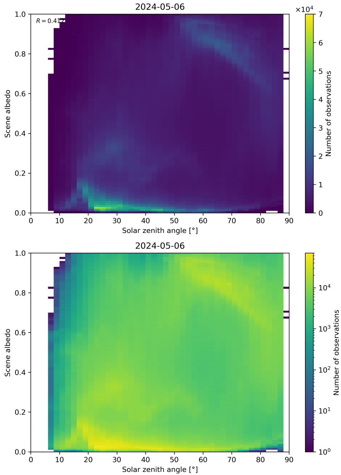
Figure 116: Scatter density plot of “Solar zenith angle” against “Scene albedo” for 2024-05-05 to 2024-05-07.
