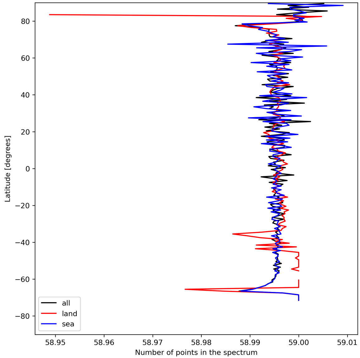
Figure 27: Zonal average of “Number of points in the spectrum” for 2024-05-05 to 2024-05-07.
