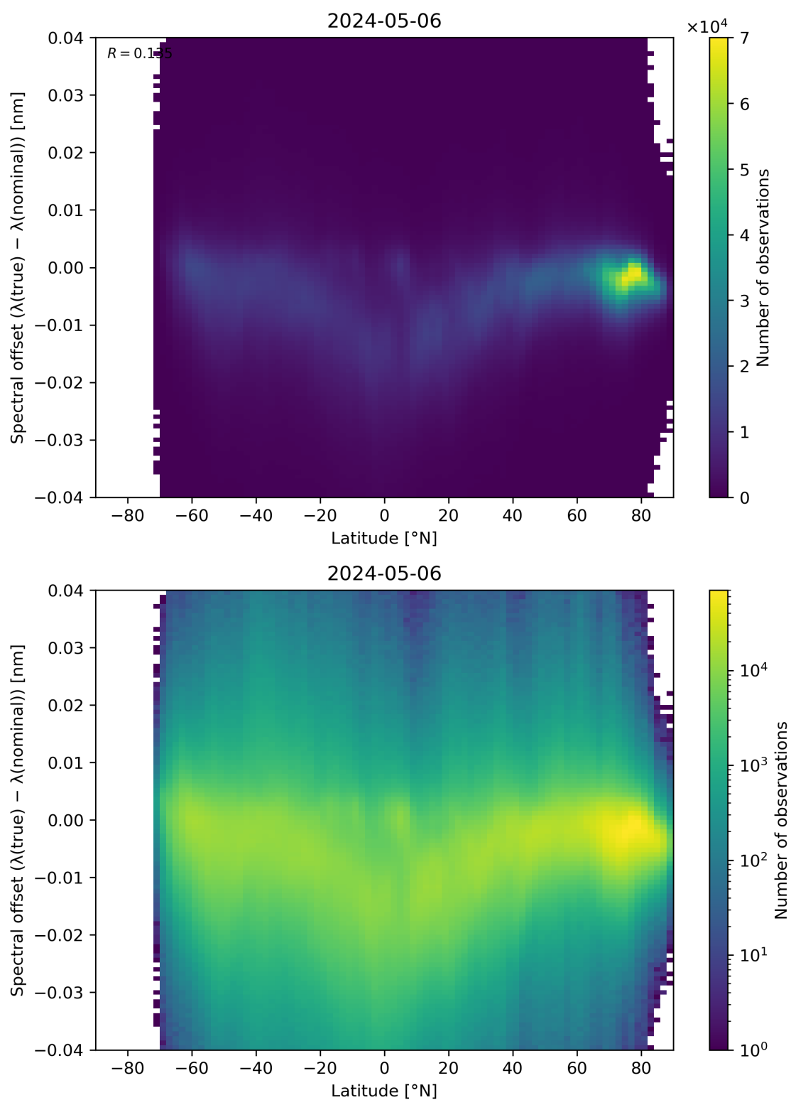
Figure 96: Scatter density plot of “Latitude” against “Spectral offset ( \lambda(\text{true}) - \lambda(\text{nominal}) )” for 2024-05-05 to 2024-05-07.
