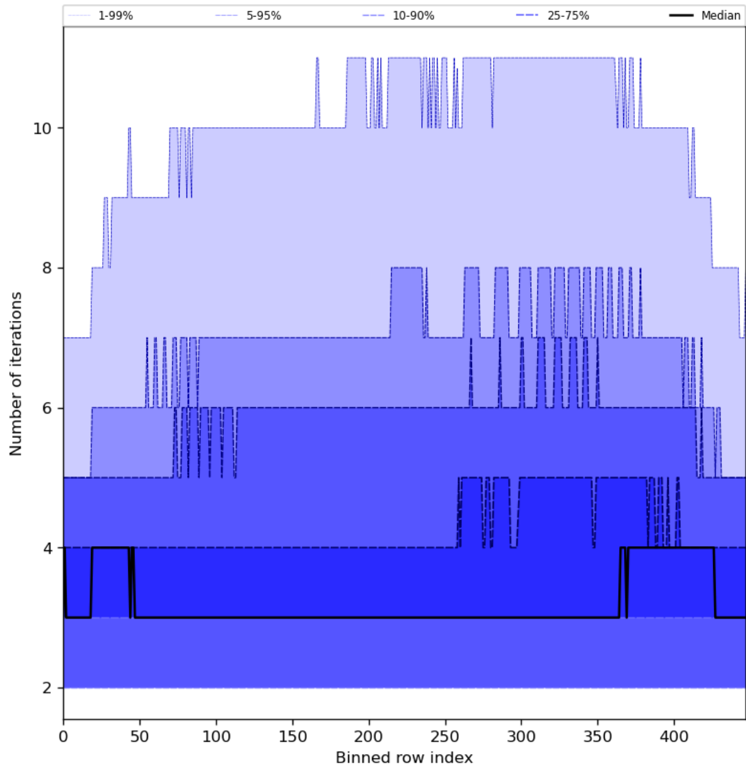
Figure 56: Along track statistics of “Number of iterations” for 2024-05-05 to 2024-05-07
