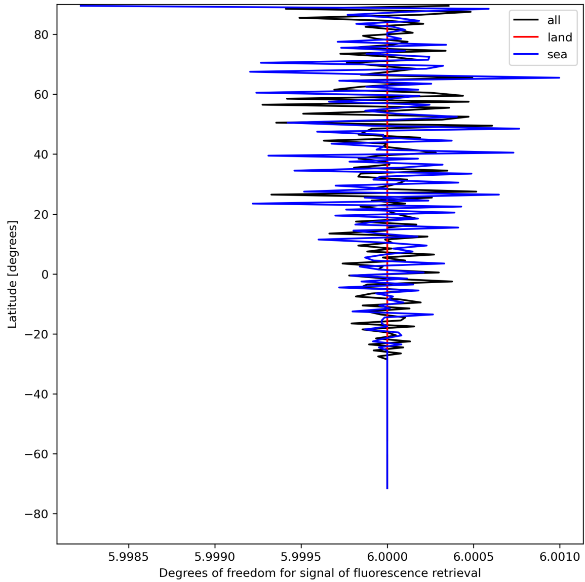
Figure 26: Zonal average of “Degrees of freedom for signal of fluorescence retrieval” for 2024-05-05 to 2024-05-07.
