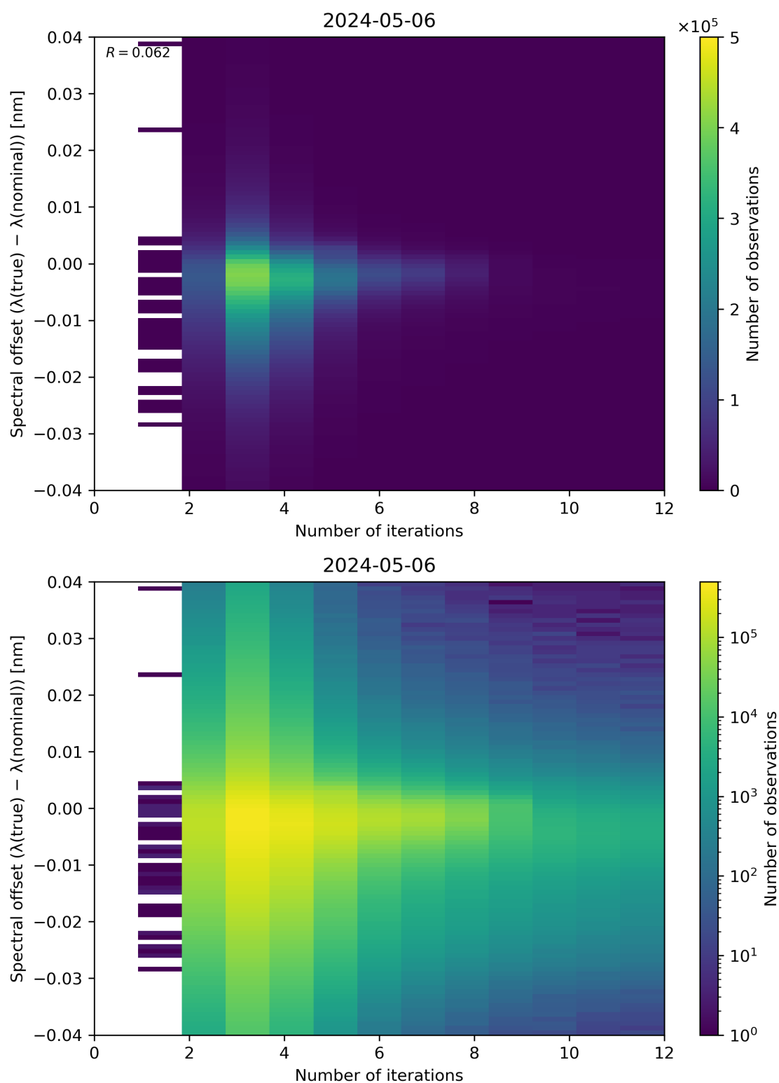
Figure 100: Scatter density plot of “Number of iterations” against “Spectral offset ( \lambda(\text{true}) - \lambda(\text{nominal}) )” for 2024-05-05 to 2024-05-07.
