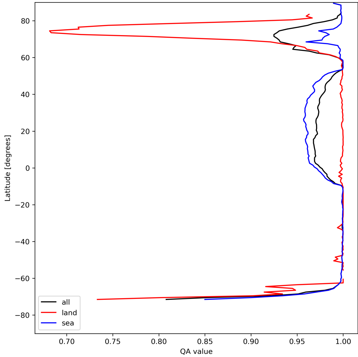
Figure 12: Zonal average of “QA value” for 2024-05-05 to 2024-05-07.
