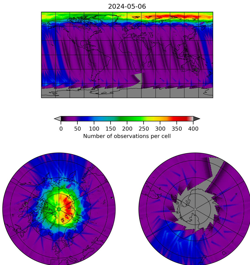
Figure 11: Map of the number of observations for 2024-05-05 to 2024-05-07
