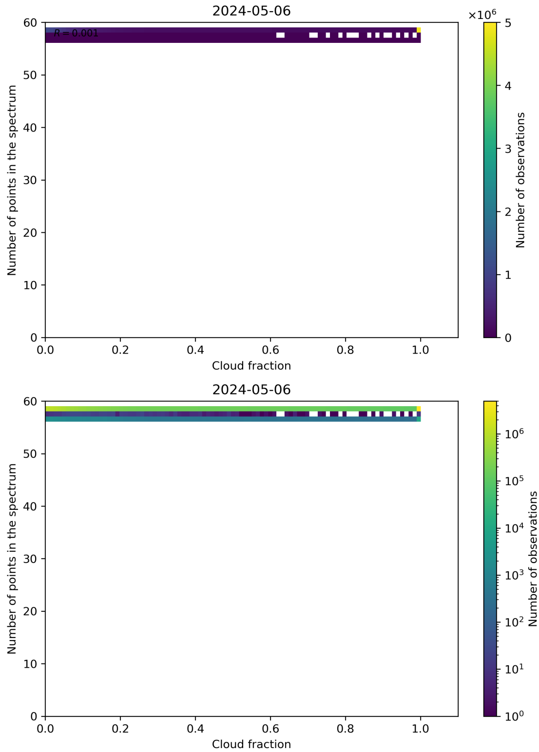
Figure 74: Scatter density plot of “Cloud fraction” against “Number of points in the spectrum” for 2024-05-05 to 2024-05-07.
