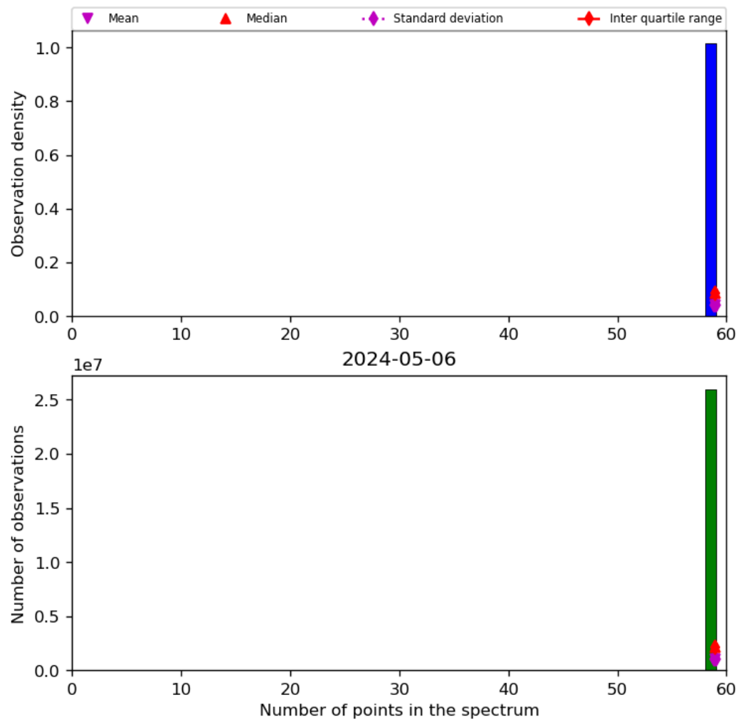
Figure 44: Histogram of “Number of points in the spectrum” for 2024-05-05 to 2024-05-07
