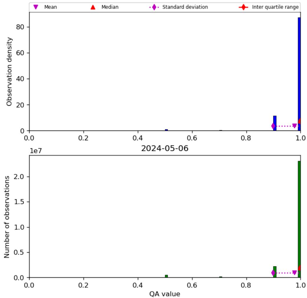
Figure 29: Histogram of “QA value” for 2024-05-05 to 2024-05-07
