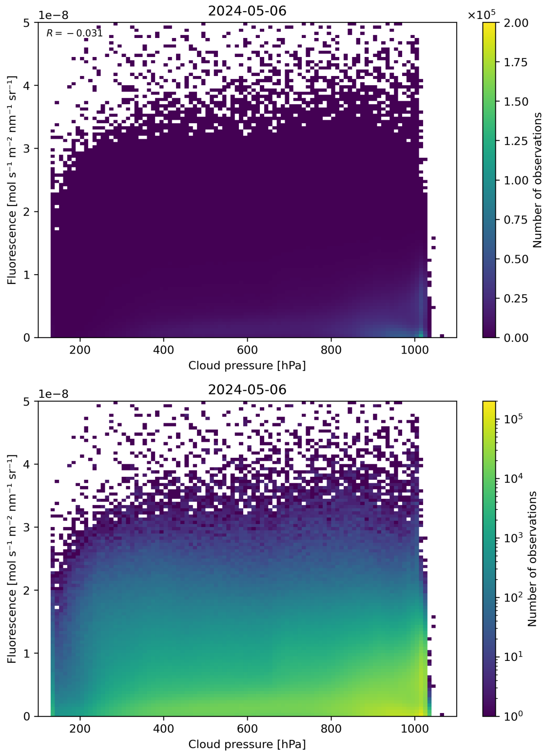
Figure 80: Scatter density plot of “Cloud pressure” against “Fluorescence” for 2024-05-05 to 2024-05-07.
