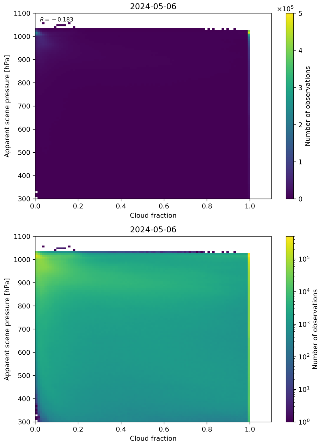
Figure 70: Scatter density plot of “Cloud fraction” against “Apparent scene pressure” for 2024-05-05 to 2024-05-07.
