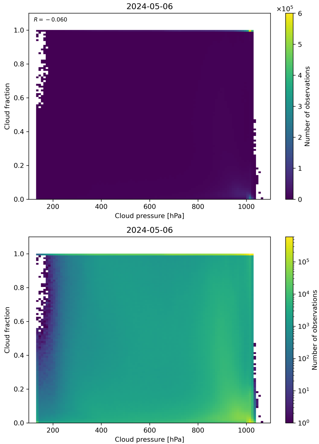
Figure 79: Scatter density plot of “Cloud pressure” against “Cloud fraction” for 2024-05-05 to 2024-05-07.
