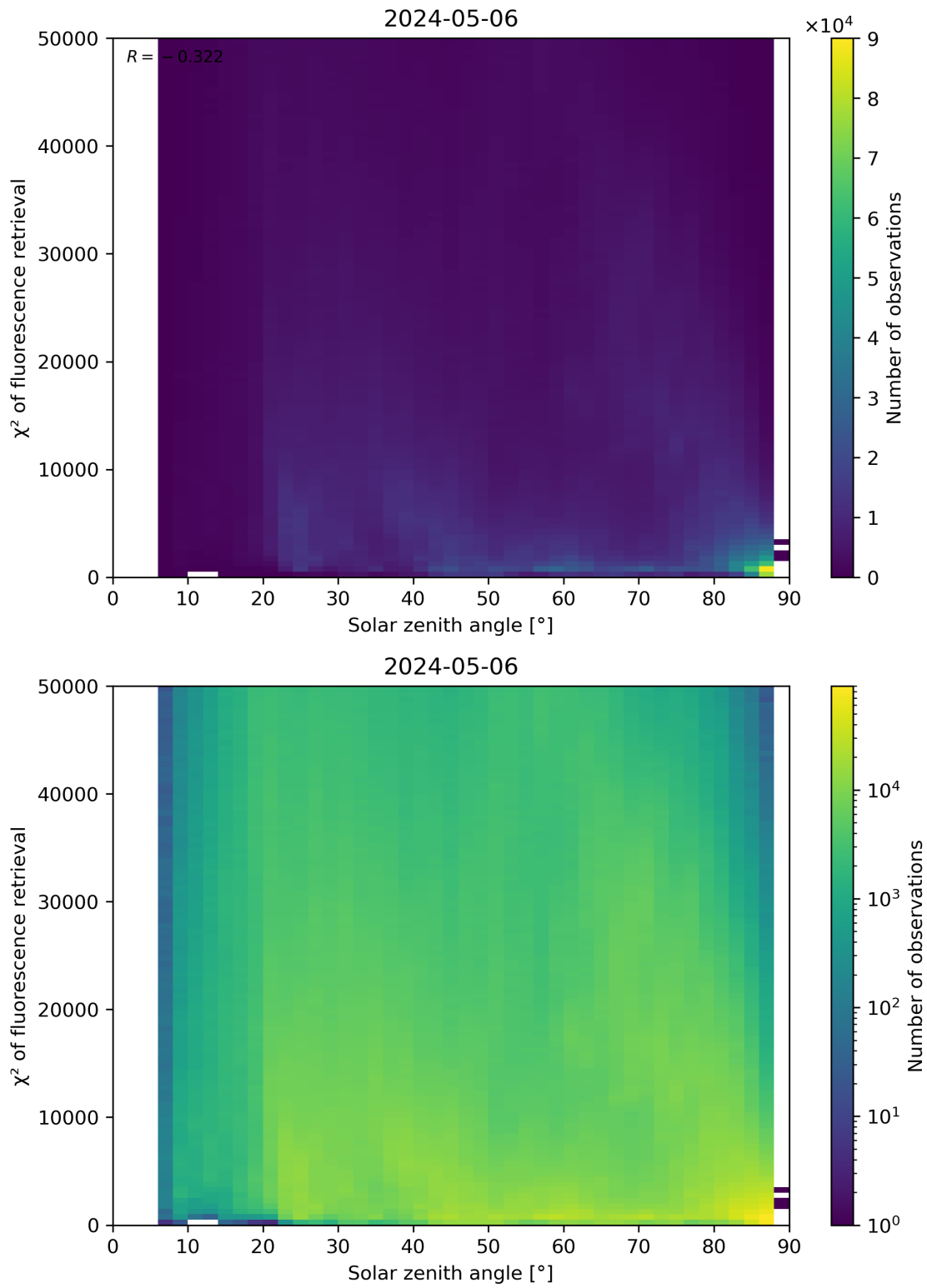
Figure 109: Scatter density plot of “Solar zenith angle” against “ \chi^2 of fluorescence retrieval” for 2024-05-05 to 2024-05-07.
