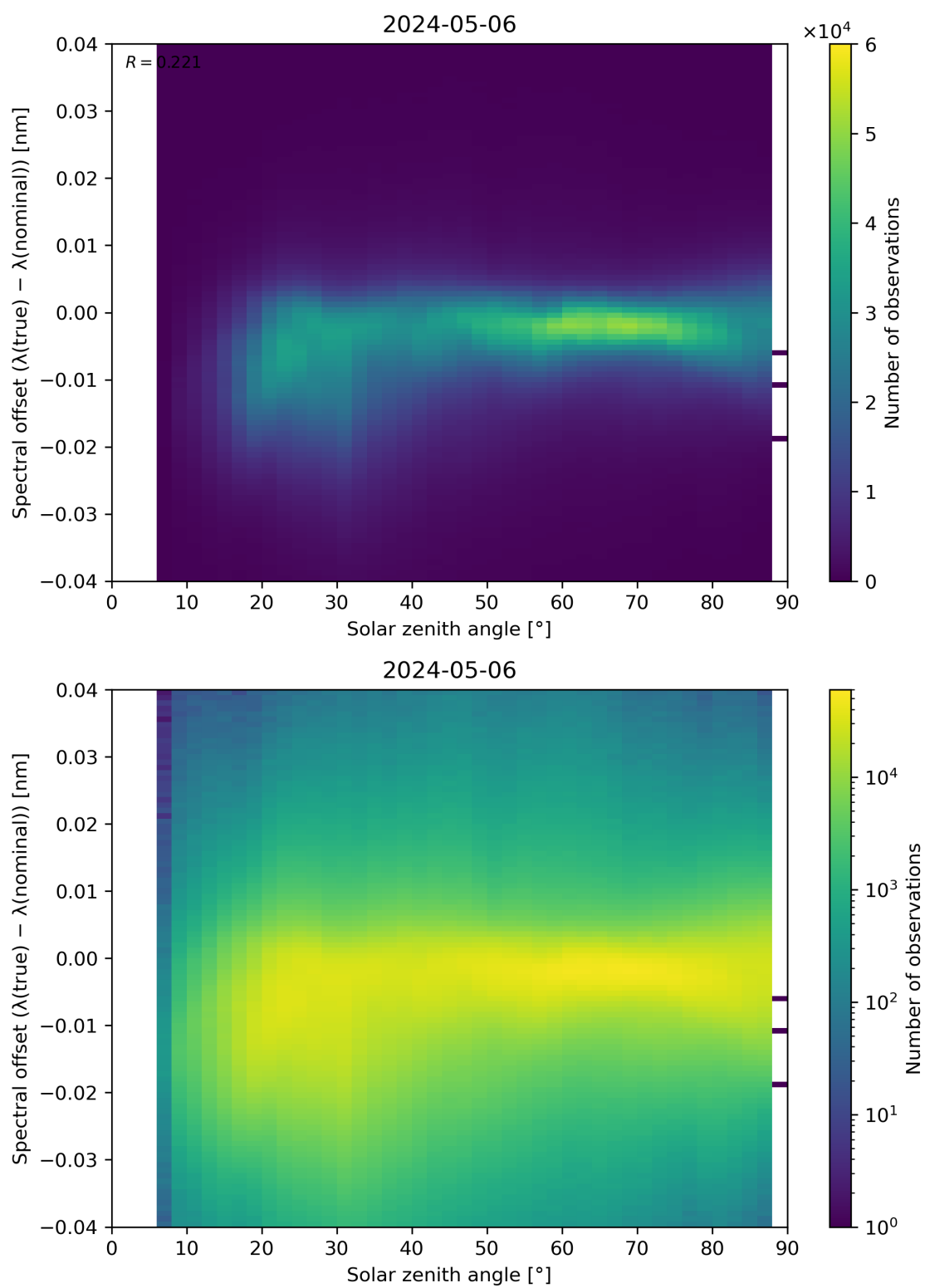
Figure 117: Scatter density plot of “Solar zenith angle” against “Spectral offset ( \lambda(\text{true}) - \lambda(\text{nominal}) )” for 2024-05-05 to 2024-05-07.
