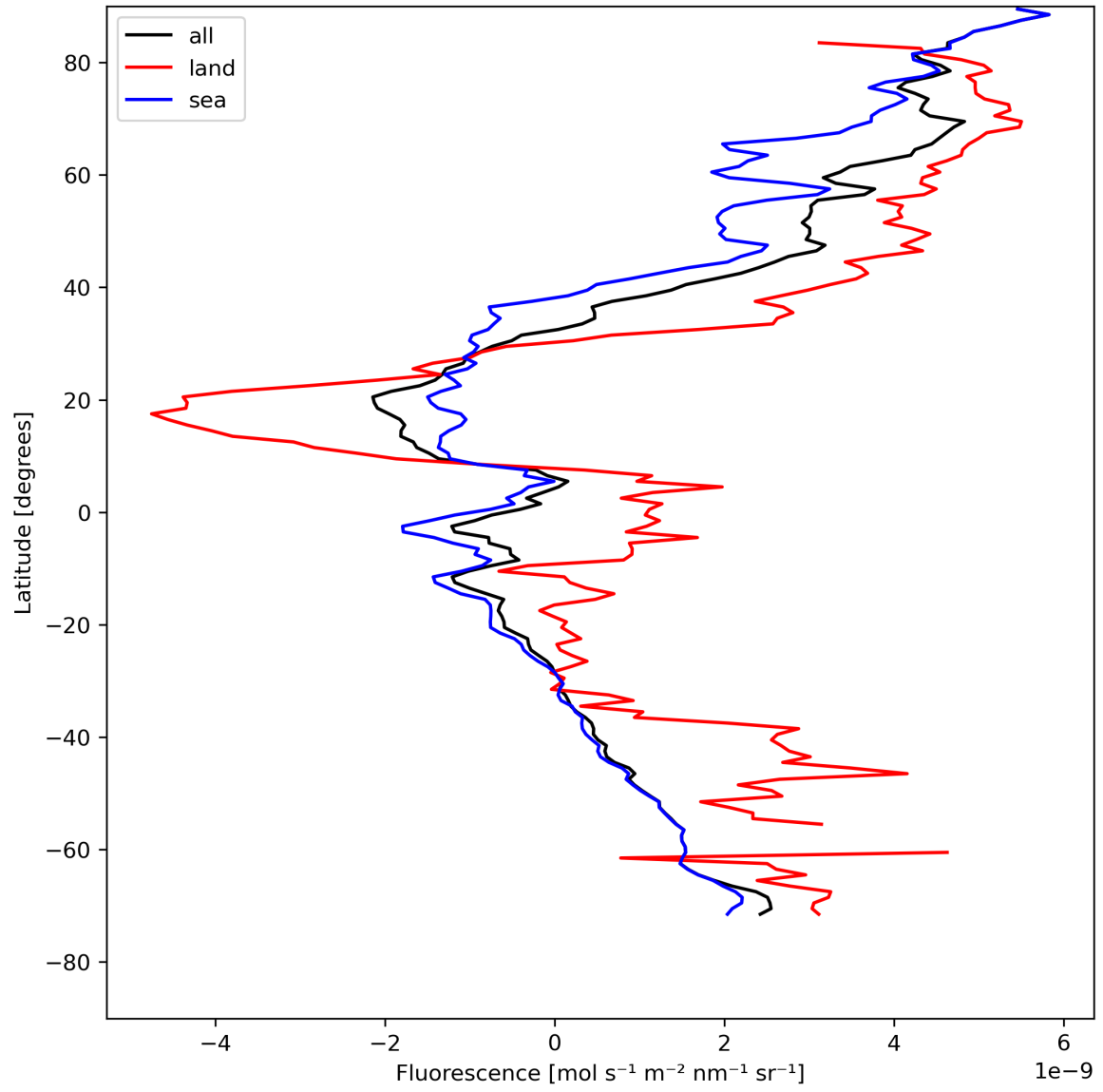
Figure 23: Zonal average of “Fluorescence” for 2024-05-05 to 2024-05-07.
