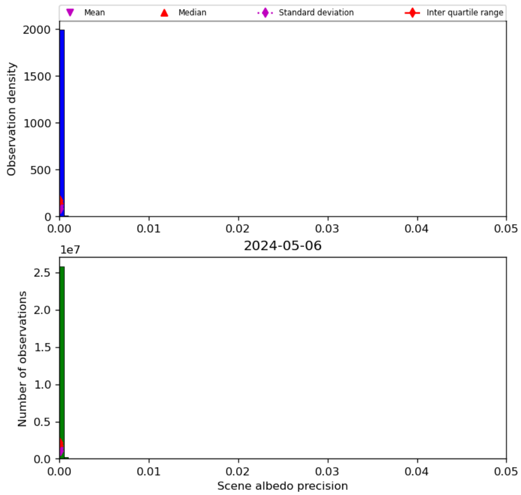
Figure 35: Histogram of “Scene albedo precision” for 2024-05-05 to 2024-05-07
