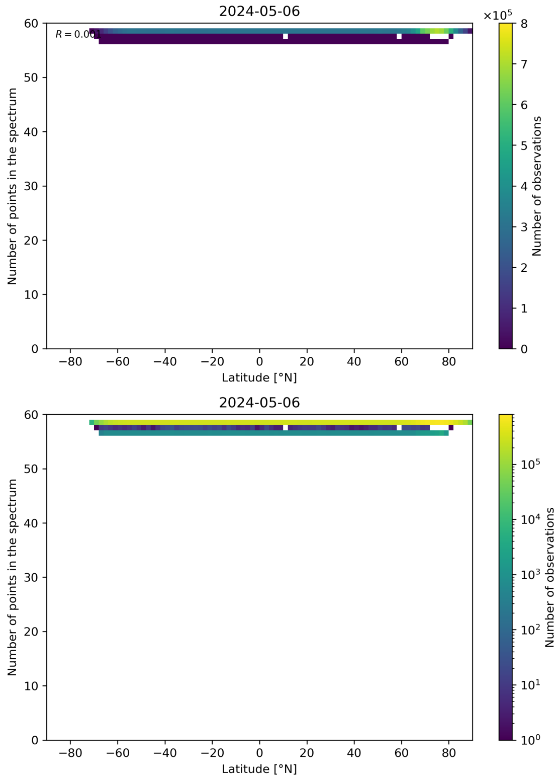
Figure 94: Scatter density plot of “Latitude” against “Number of points in the spectrum” for 2024-05-05 to 2024-05-07.
