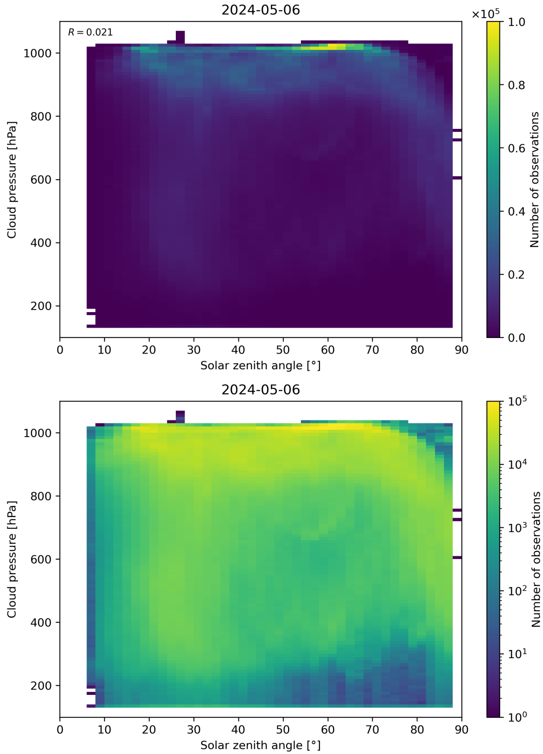
Figure 111: Scatter density plot of “Solar zenith angle” against “Cloud pressure” for 2024-05-05 to 2024-05-07.
