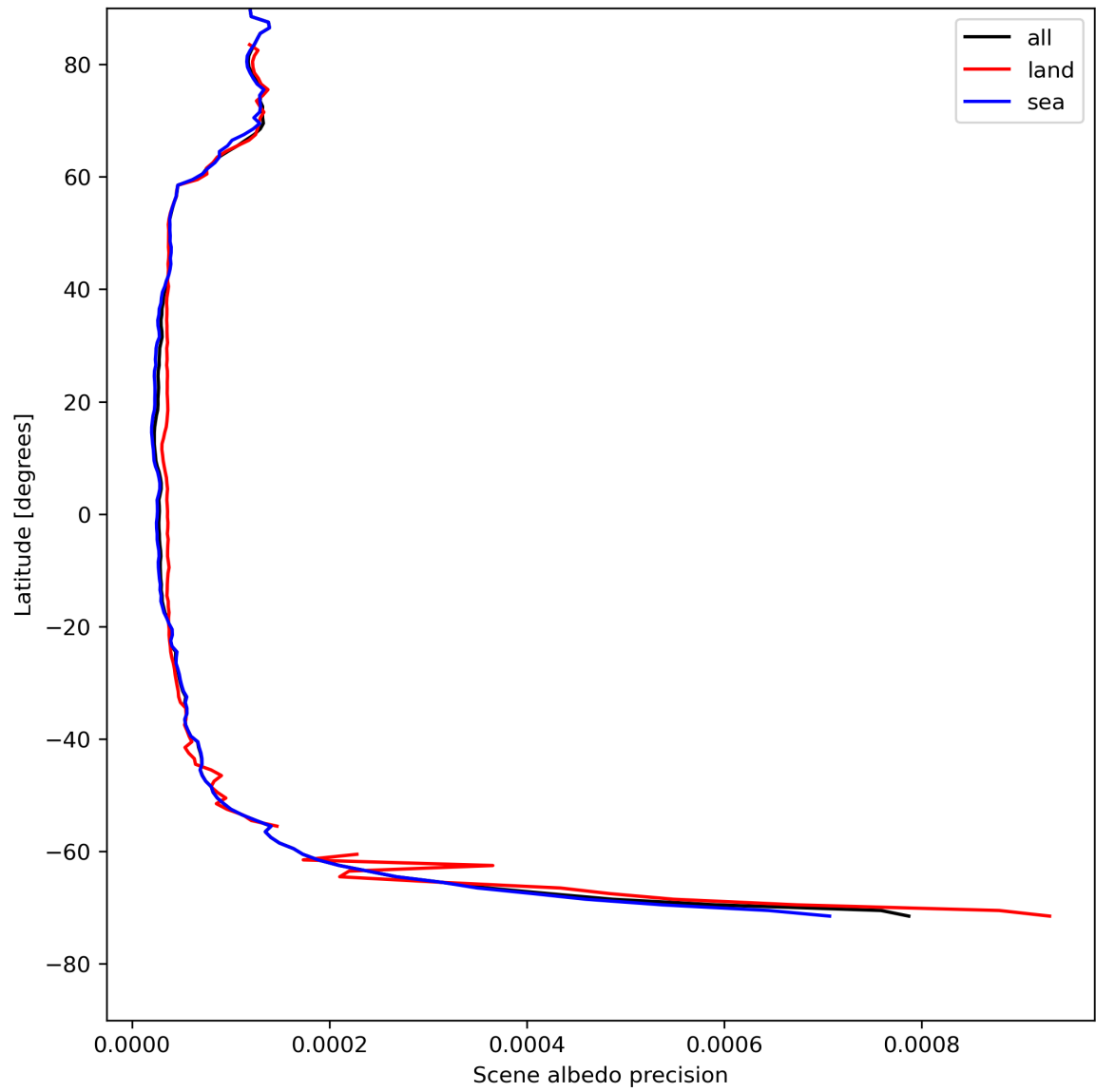
Figure 18: Zonal average of “Scene albedo precision” for 2024-05-05 to 2024-05-07.
