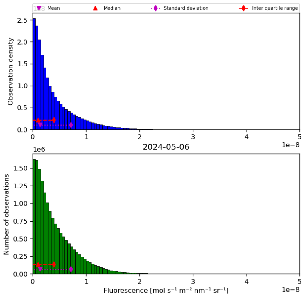
Figure 40: Histogram of “Fluorescence” for 2024-05-05 to 2024-05-07
