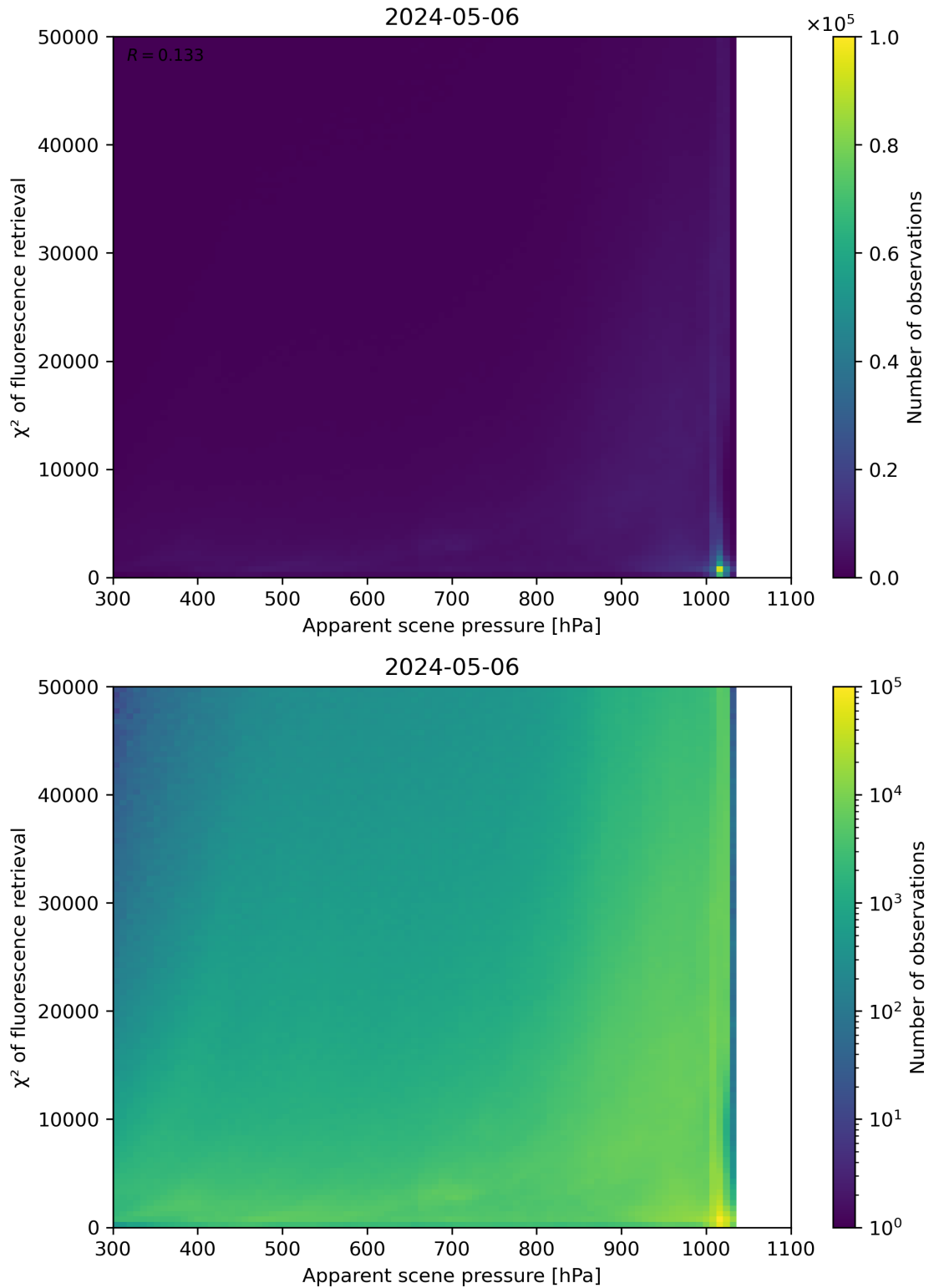
Figure 63: Scatter density plot of “Apparent scene pressure” against “ \chi^2 of fluorescence retrieval” for 2024-05-05 to 2024-05-07.
