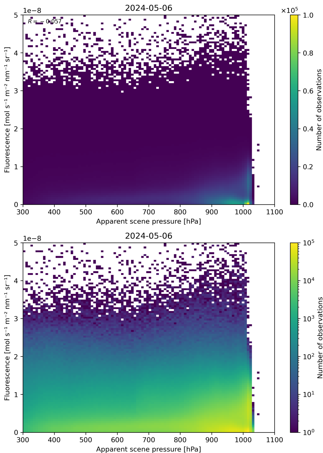
Figure 64: Scatter density plot of “Apparent scene pressure” against “Fluorescence” for 2024-05-05 to 2024-05-07.
