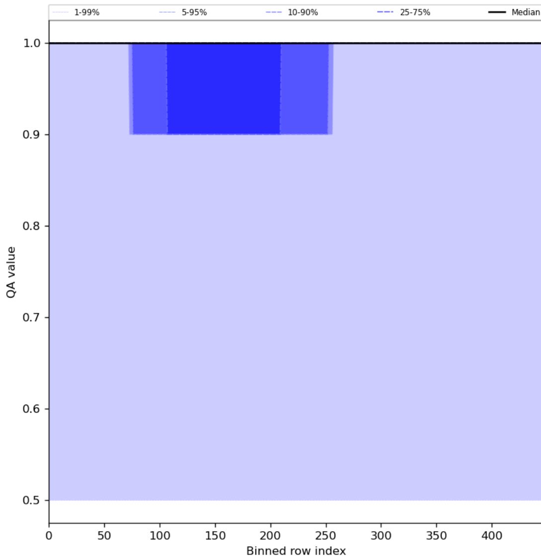
Figure 46: Along track statistics of “QA value” for 2024-05-05 to 2024-05-07
