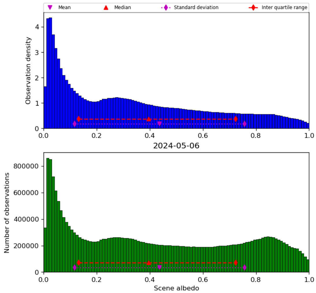
Figure 34: Histogram of “Scene albedo” for 2024-05-05 to 2024-05-07
