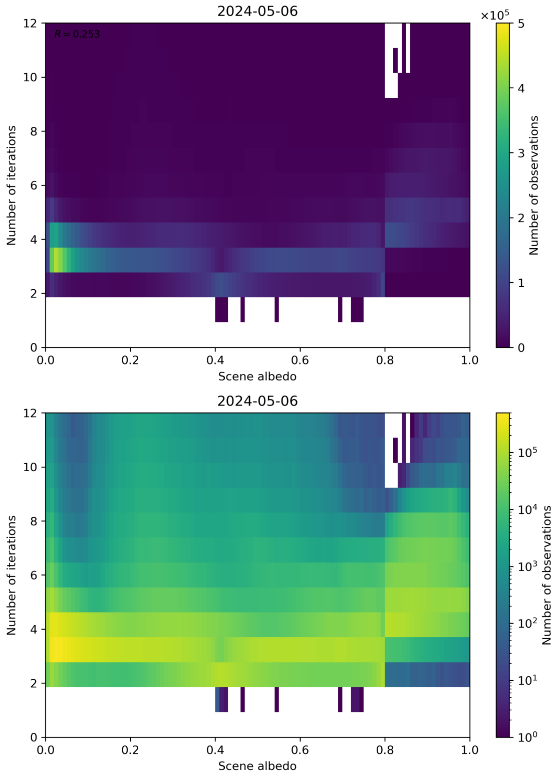
Figure 105: Scatter density plot of “Scene albedo” against “Number of iterations” for 2024-05-05 to 2024-05-07.
