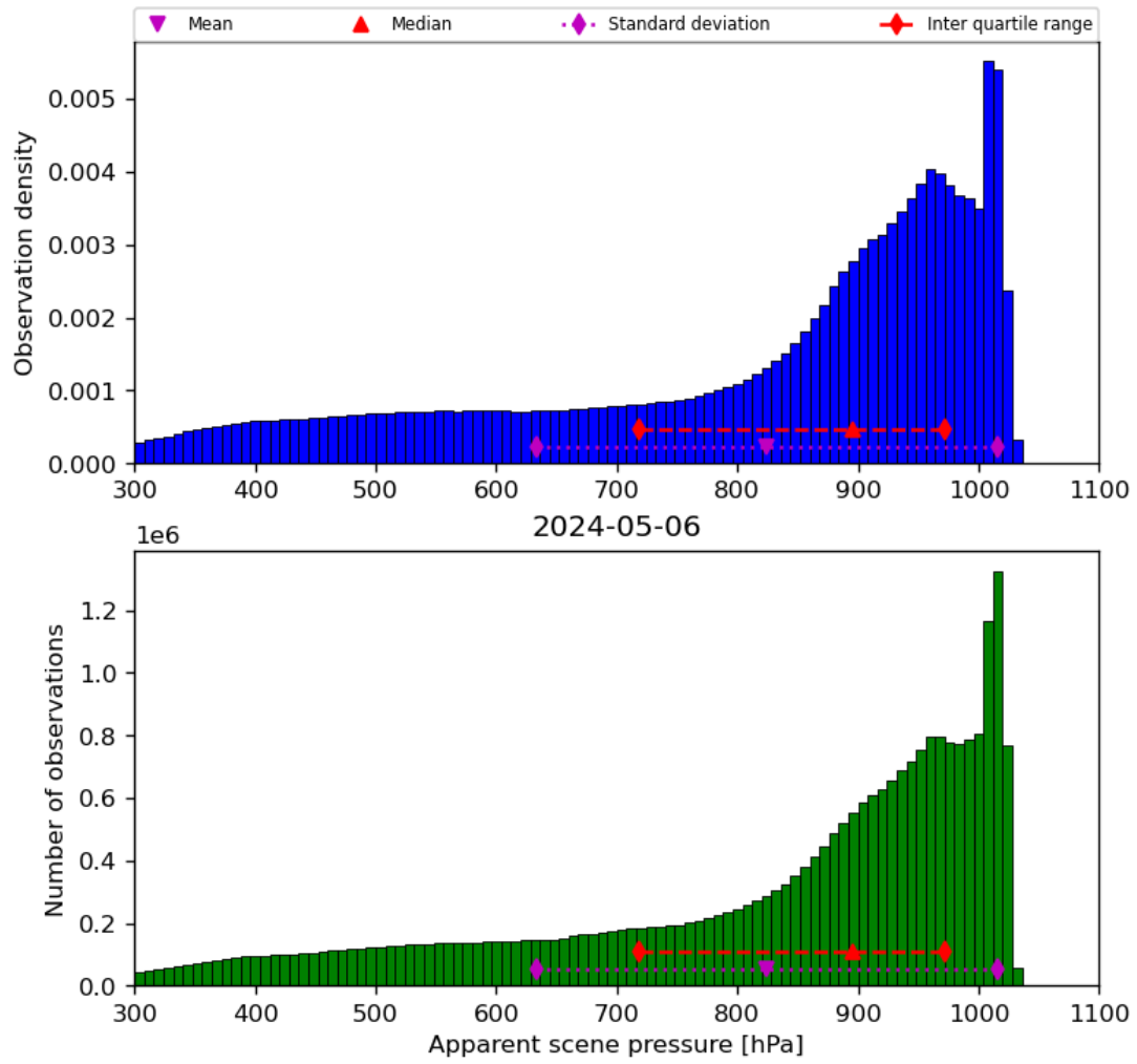
Figure 36: Histogram of “Apparent scene pressure” for 2024-05-05 to 2024-05-07
