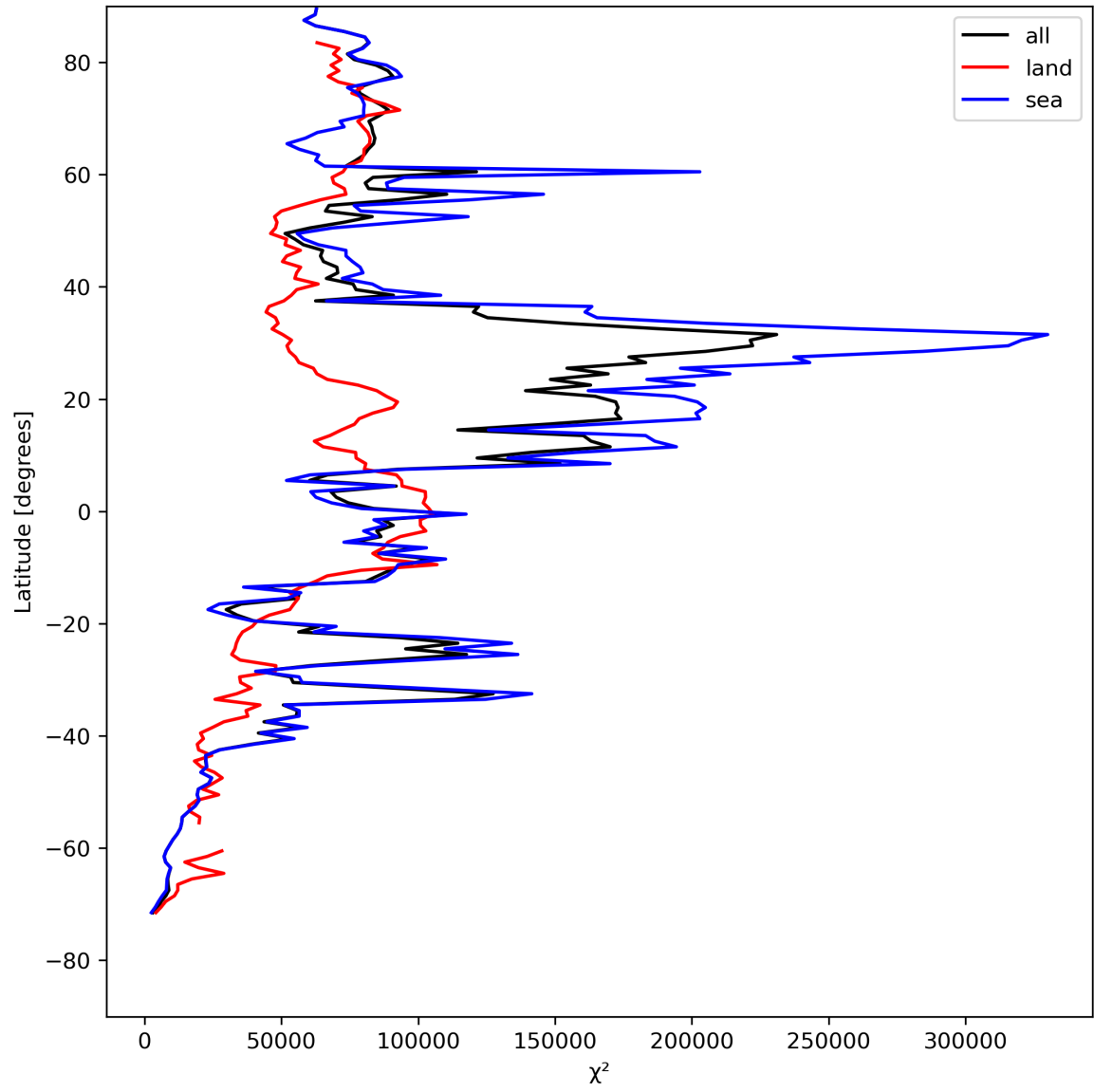
Figure 21: Zonal average of “ \chi^2 ” for 2024-05-05 to 2024-05-07.
