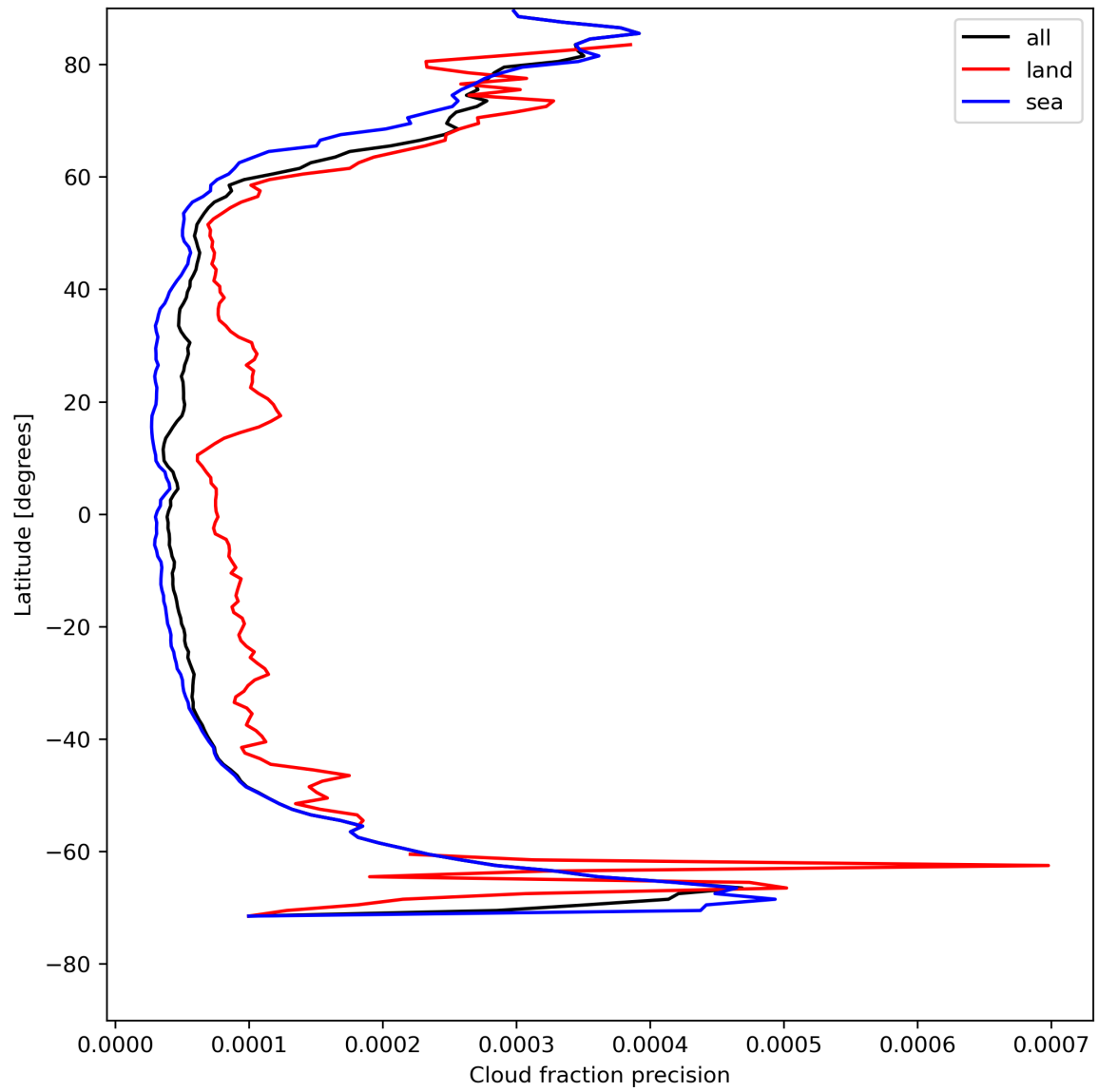
Figure 16: Zonal average of “Cloud fraction precision” for 2024-05-05 to 2024-05-07.
