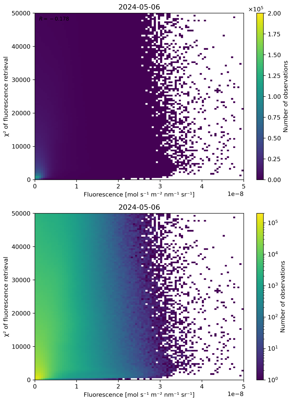
Figure 85: Scatter density plot of “Fluorescence” against “ \chi^2 of fluorescence retrieval” for 2024-05-05 to 2024-05-07.
