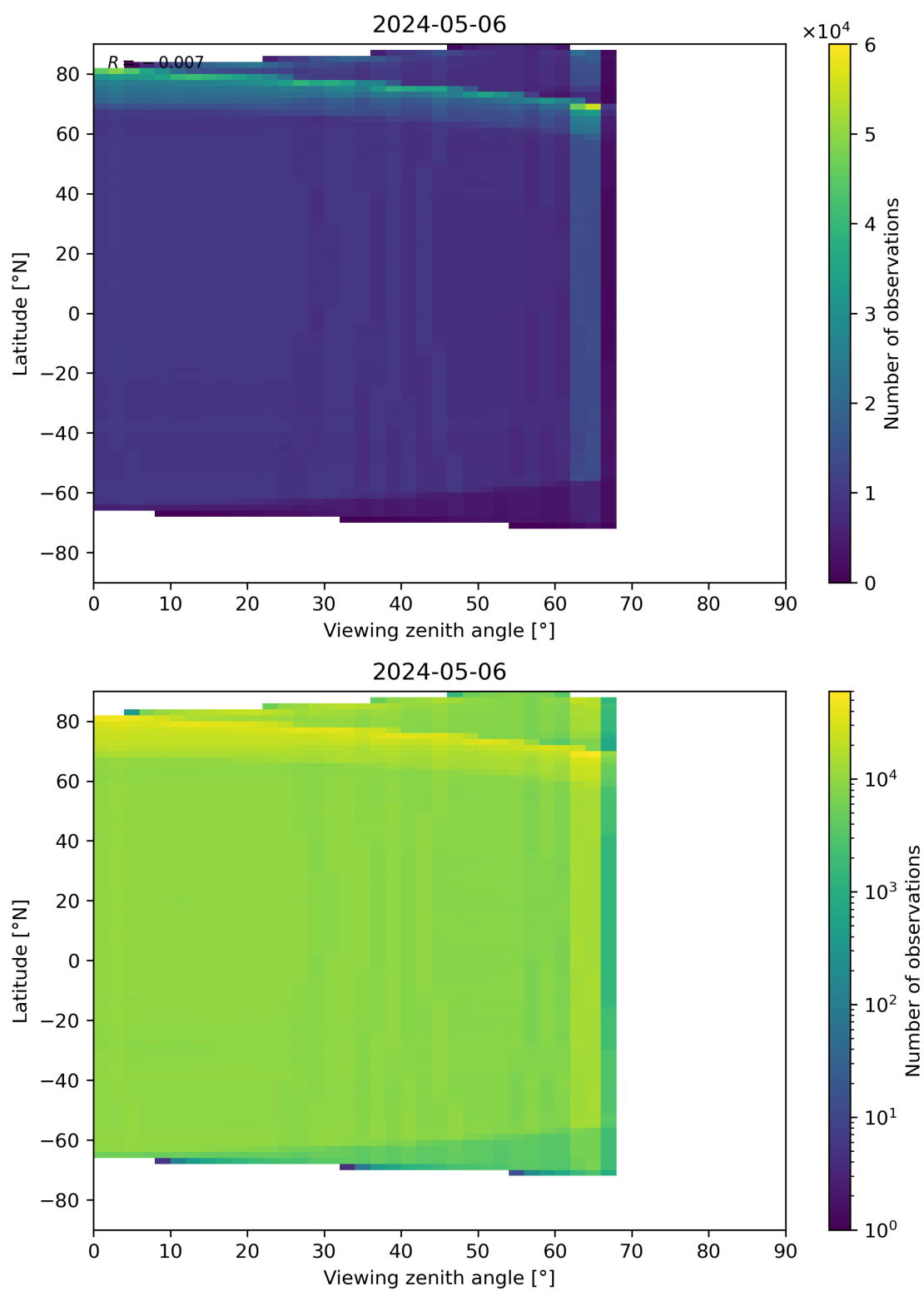
Figure 123: Scatter density plot of “Viewing zenith angle” against “Latitude” for 2024-05-05 to 2024-05-07.
