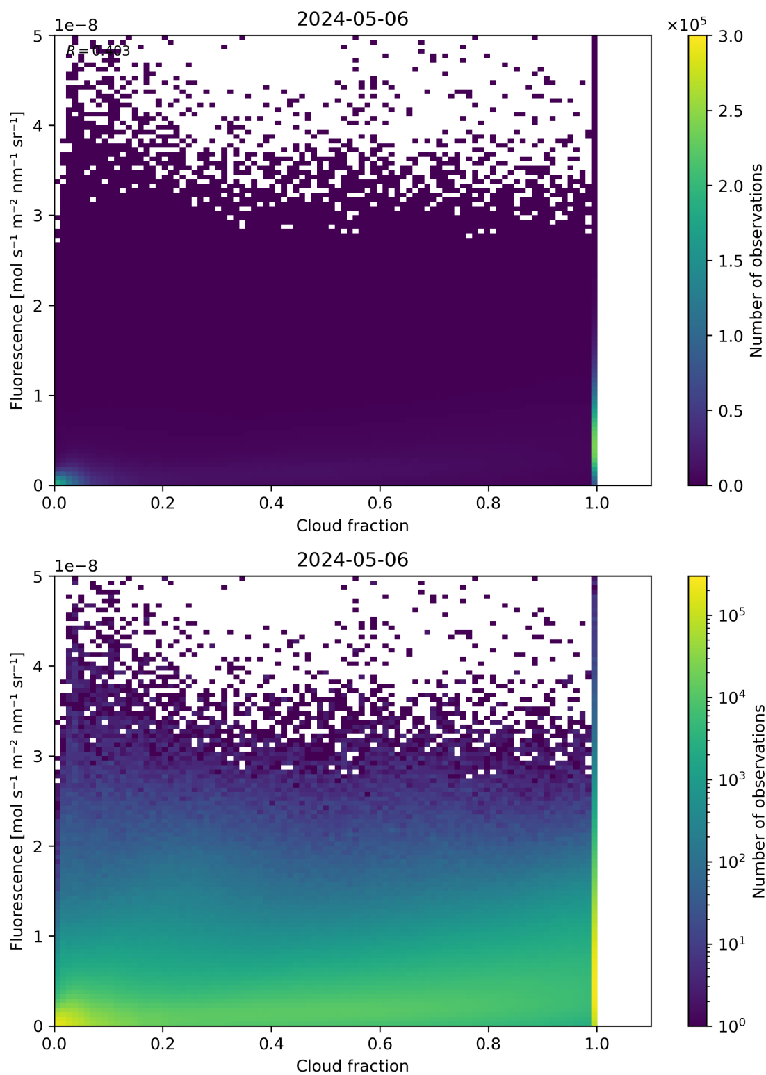
Figure 72: Scatter density plot of “Cloud fraction” against “Fluorescence” for 2024-05-05 to 2024-05-07.
