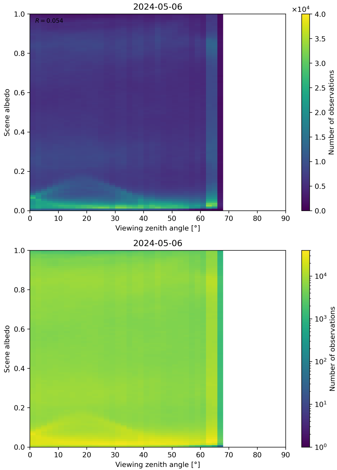
Figure 126: Scatter density plot of “Viewing zenith angle” against “Scene albedo” for 2024-05-05 to 2024-05-07.
