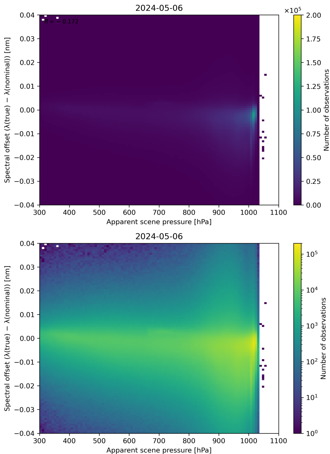
Figure 67: Scatter density plot of “Apparent scene pressure” against “Spectral offset ( \lambda(\text{true}) - \lambda(\text{nominal}) )” for 2024-05-05 to 2024-05-07.
