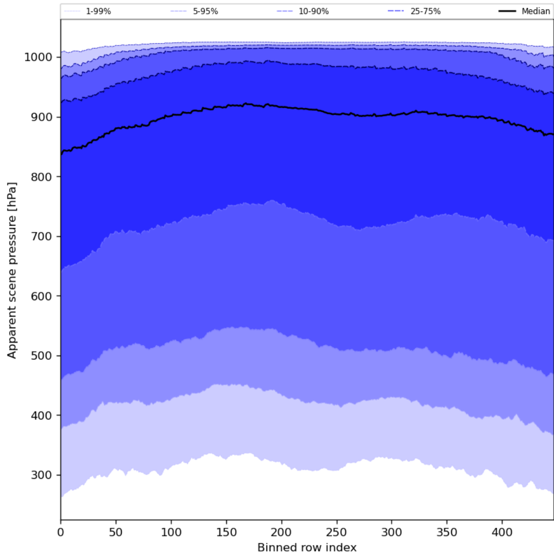
Figure 53: Along track statistics of “Apparent scene pressure” for 2024-05-05 to 2024-05-07
