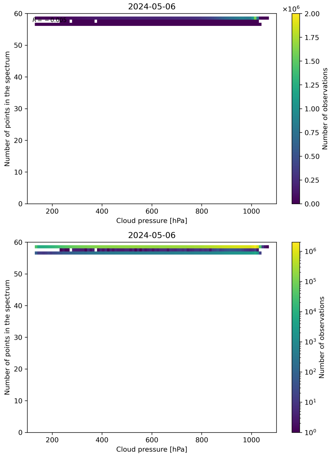
Figure 82: Scatter density plot of “Cloud pressure” against “Number of points in the spectrum” for 2024-05-05 to 2024-05-07.
