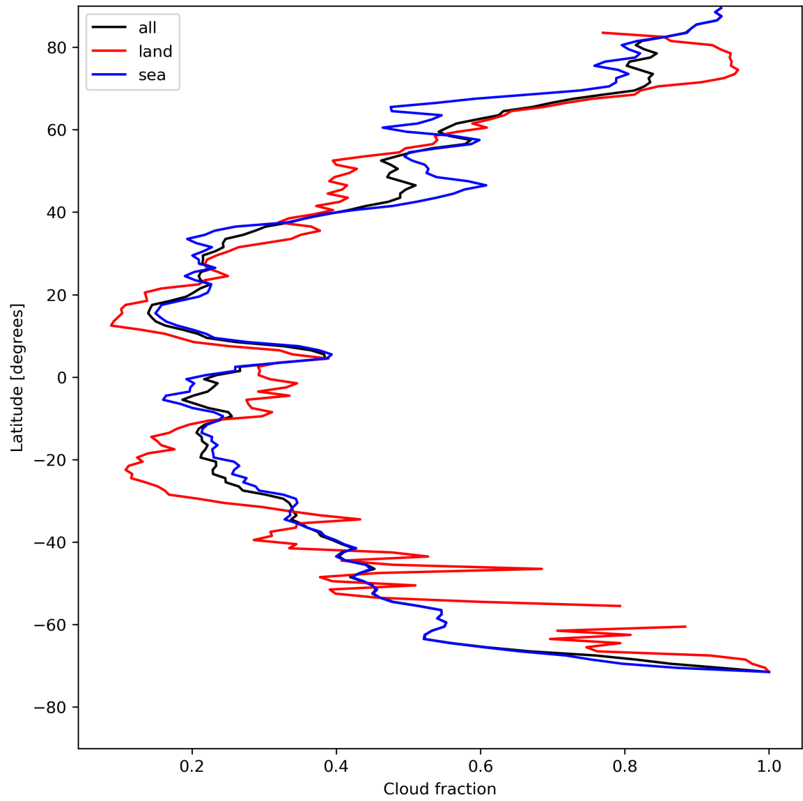
Figure 15: Zonal average of “Cloud fraction” for 2024-05-05 to 2024-05-07.
