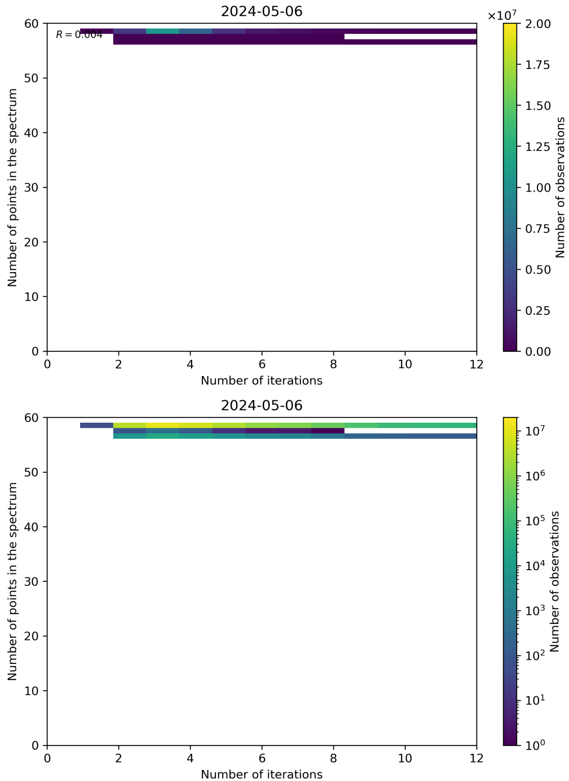
Figure 99: Scatter density plot of “Number of iterations” against “Number of points in the spectrum” for 2024-05-05 to 2024-05-07.
