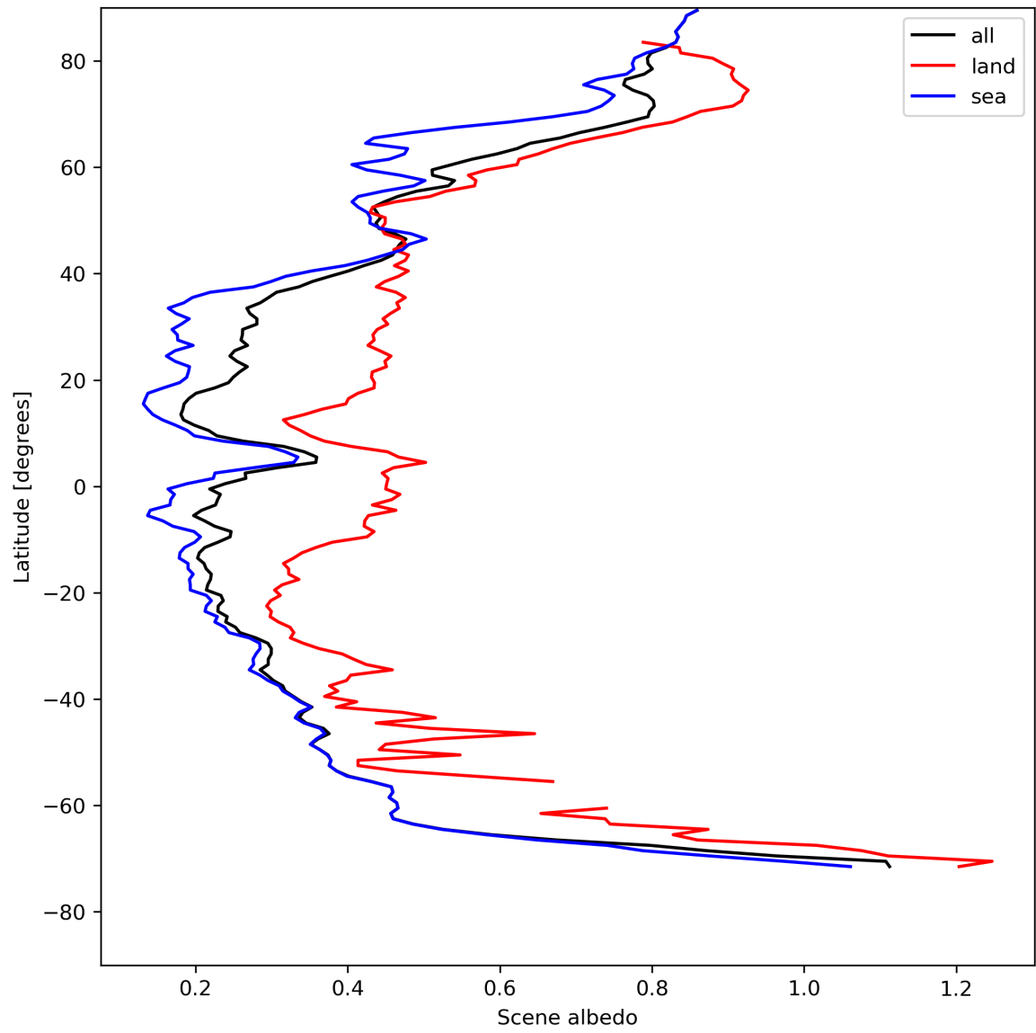
Figure 17: Zonal average of “Scene albedo” for 2024-05-05 to 2024-05-07.
