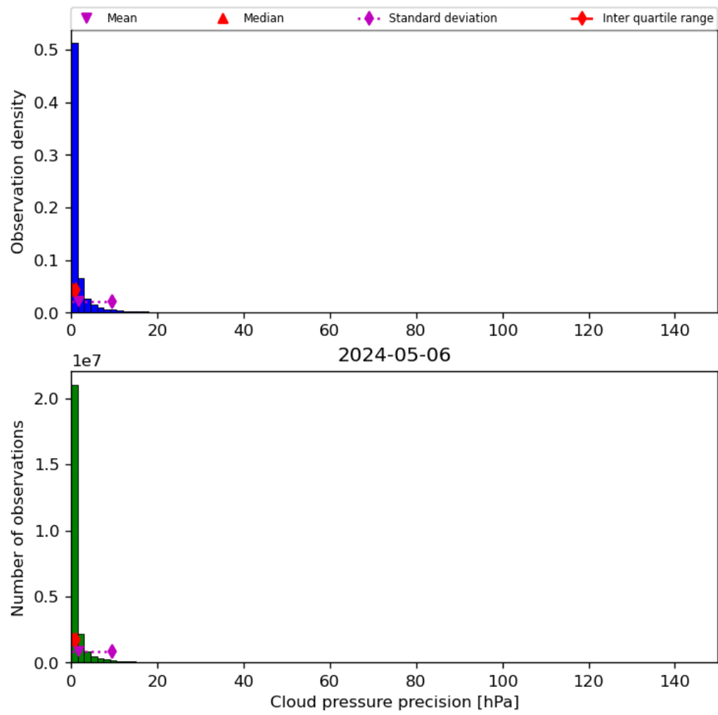
Figure 31: Histogram of “Cloud pressure precision” for 2024-05-05 to 2024-05-07
