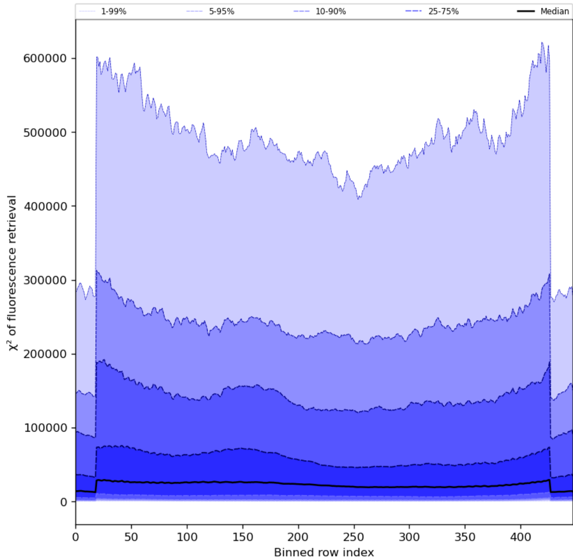
Figure 59: Along track statistics of “ \chi^2 of fluorescence retrieval” for 2024-05-05 to 2024-05-07
