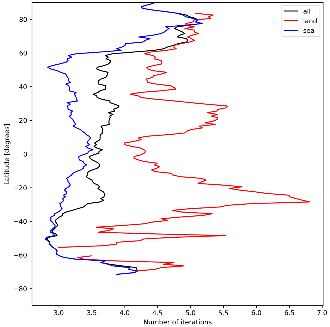
Figure 22: Zonal average of “Number of iterations” for 2024-05-05 to 2024-05-07.
