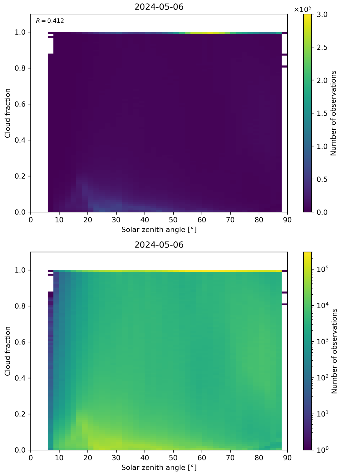
Figure 110: Scatter density plot of “Solar zenith angle” against “Cloud fraction” for 2024-05-05 to 2024-05-07.
