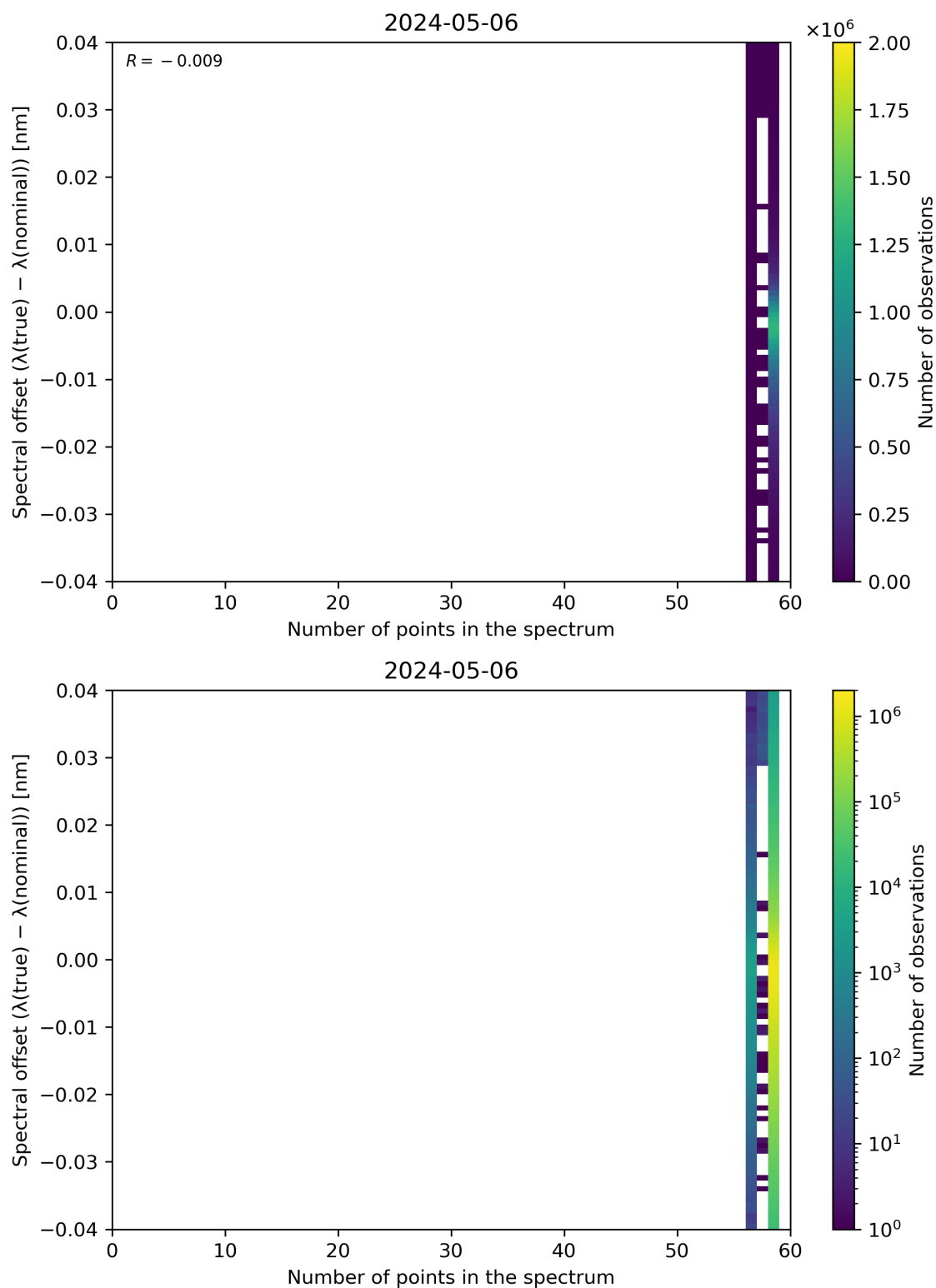
Figure 101: Scatter density plot of “Number of points in the spectrum” against “Spectral offset ( \lambda(\text{true}) - \lambda(\text{nominal}) )” for 2024-05-05 to 2024-05-07.
