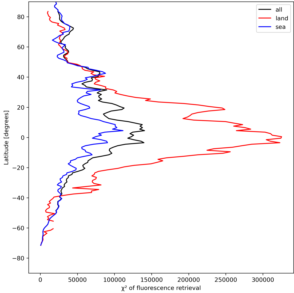
Figure 25: Zonal average of “ \chi^2 of fluorescence retrieval” for 2024-05-05 to 2024-05-07.
