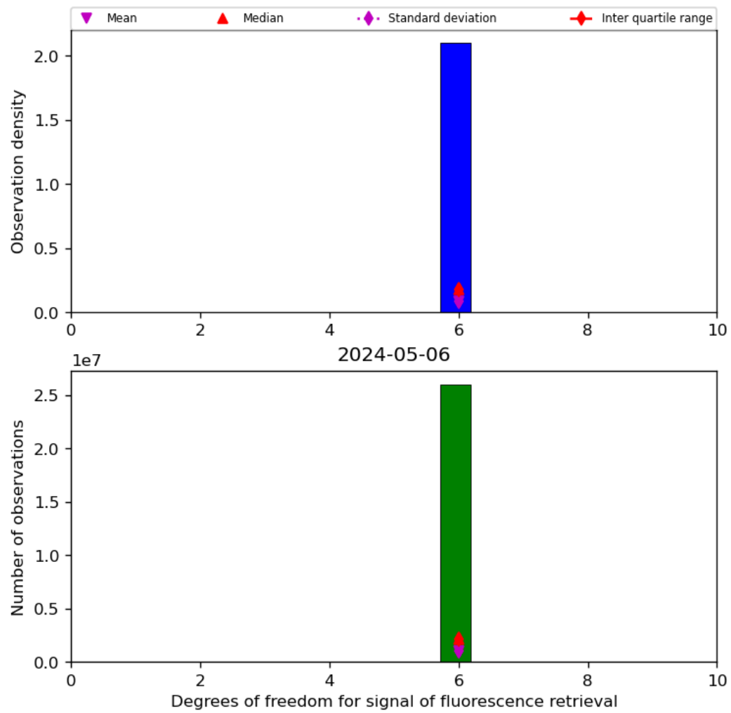
Figure 43: Histogram of “Degrees of freedom for signal of fluorescence retrieval” for 2024-05-05 to 2024-05-07
