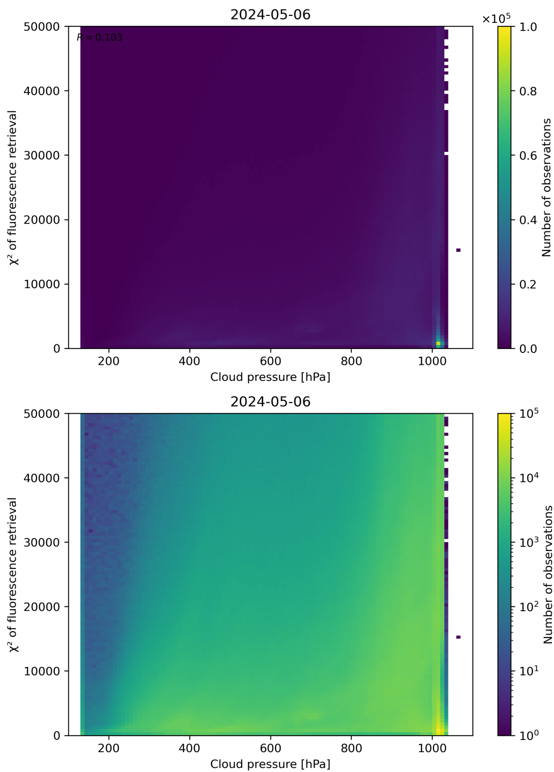
Figure 78: Scatter density plot of “Cloud pressure” against “ \chi^2 of fluorescence retrieval” for 2024-05-05 to 2024-05-07.
