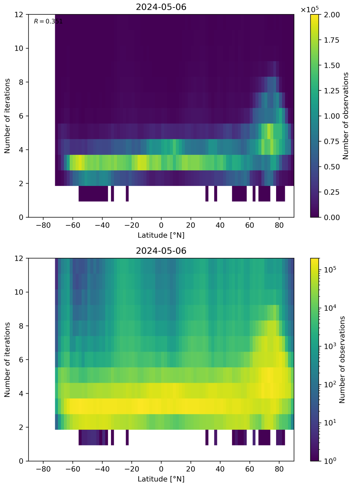
Figure 93: Scatter density plot of “Latitude” against “Number of iterations” for 2024-05-05 to 2024-05-07.
