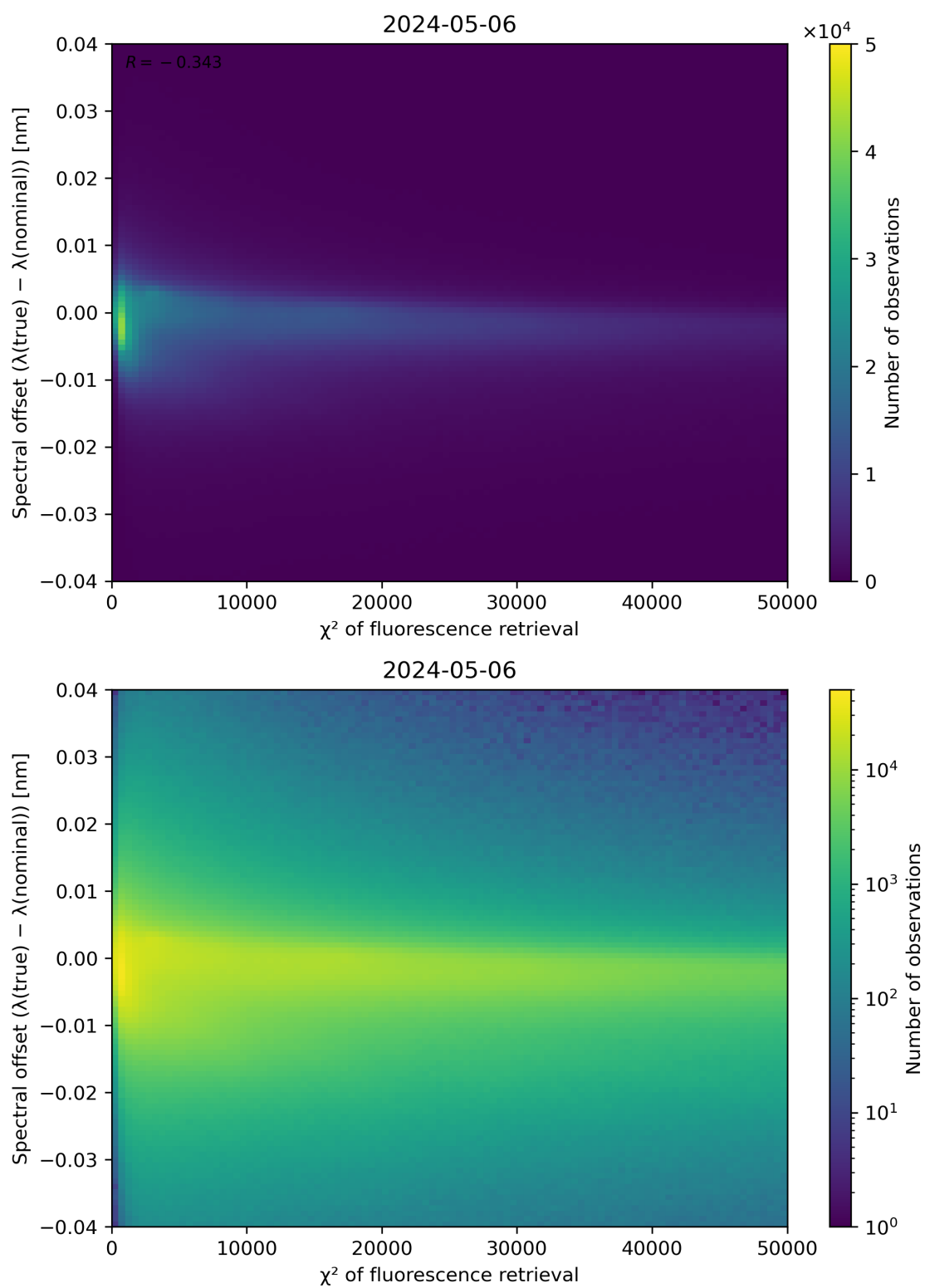
Figure 69: Scatter density plot of " \chi^2 of fluorescence retrieval" against "Spectral offset ( \lambda(\text{true}) - \lambda(\text{nominal})) " for 2024-05-05 to 2024-05-07.
