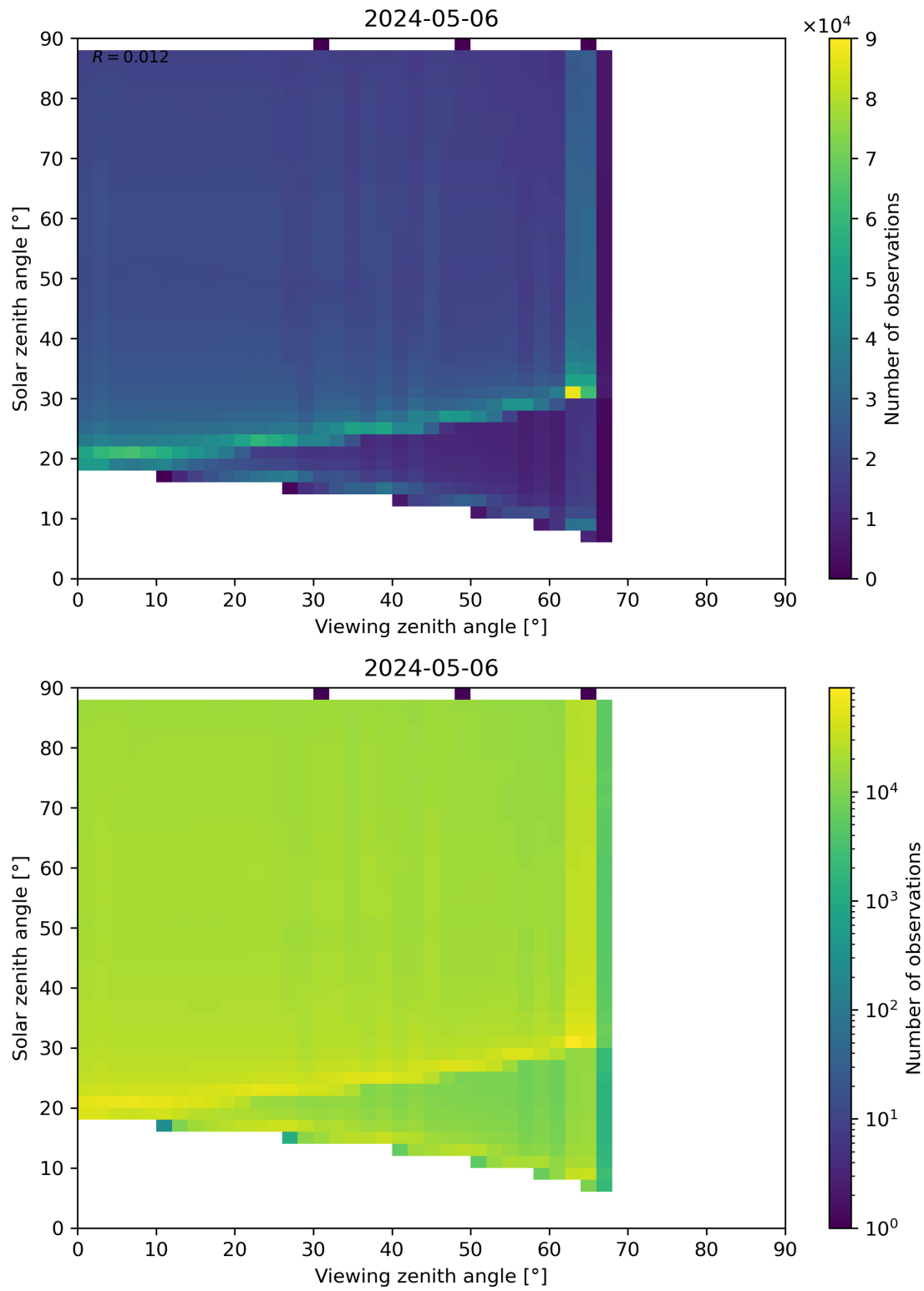
Figure 127: Scatter density plot of “Viewing zenith angle” against “Solar zenith angle” for 2024-05-05 to 2024-05-07.
