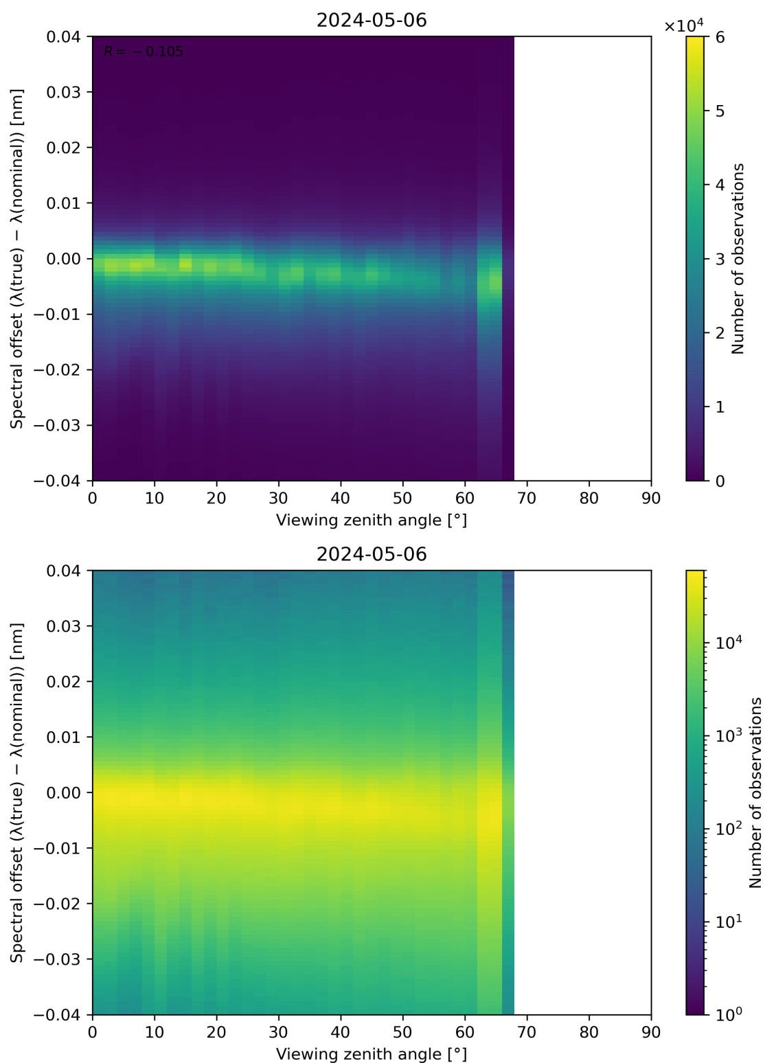
Figure 128: Scatter density plot of “Viewing zenith angle” against “Spectral offset ( \lambda(\text{true}) - \lambda(\text{nominal}) )” for 2024-05-05 to 2024-05-07.
