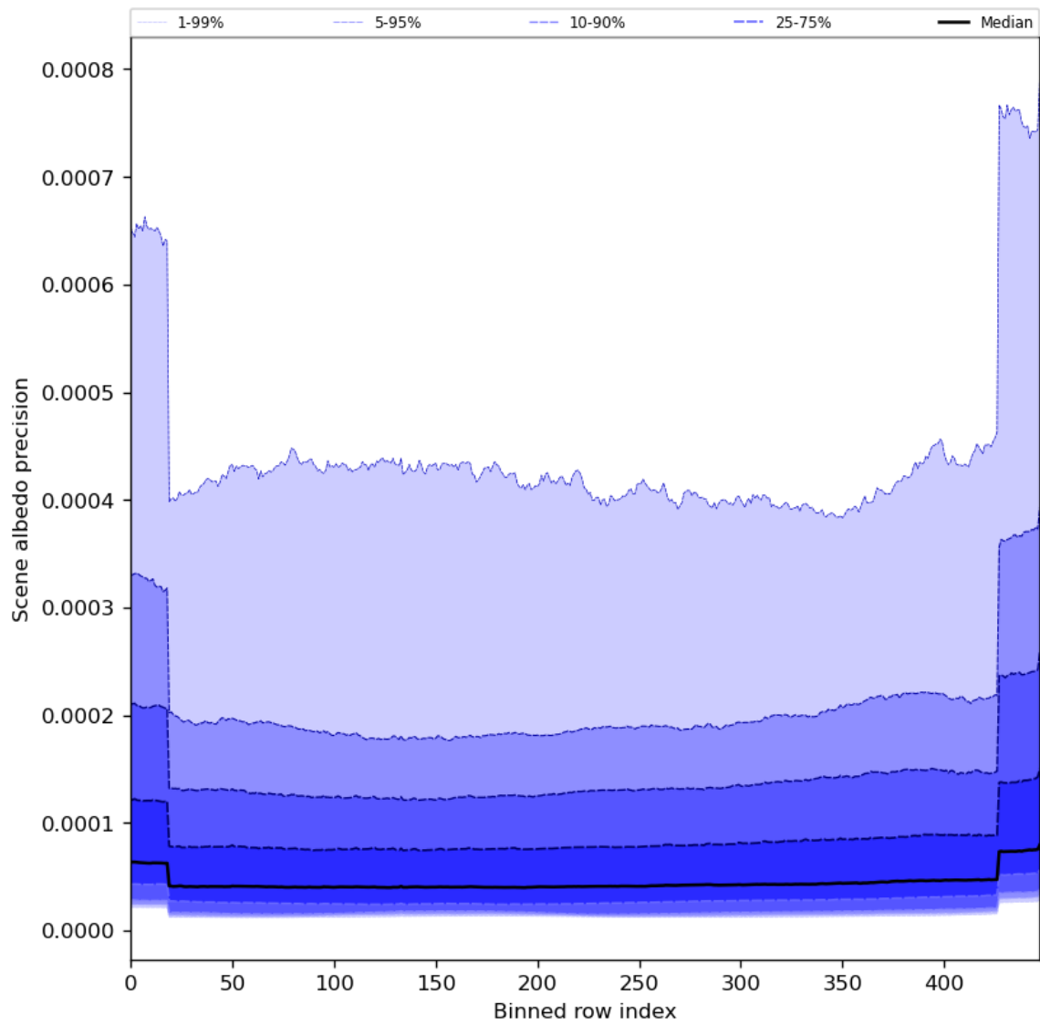
Figure 52: Along track statistics of “Scene albedo precision” for 2024-05-05 to 2024-05-07
