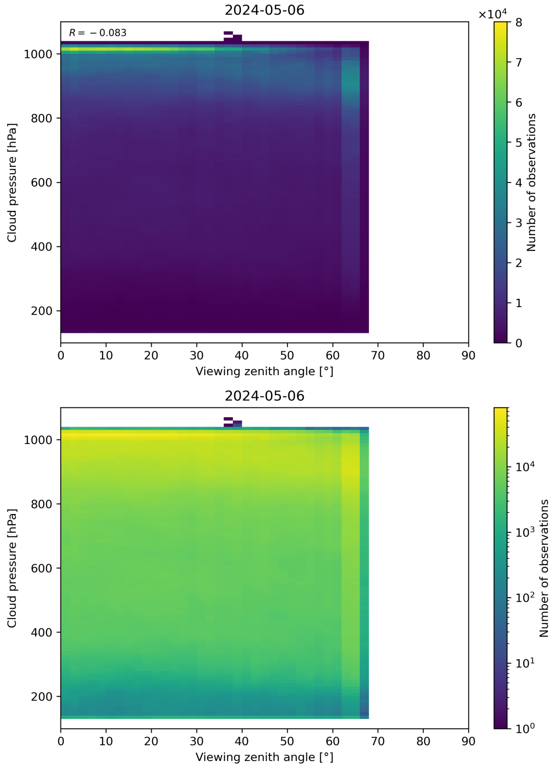
Figure 121: Scatter density plot of “Viewing zenith angle” against “Cloud pressure” for 2024-05-05 to 2024-05-07.
