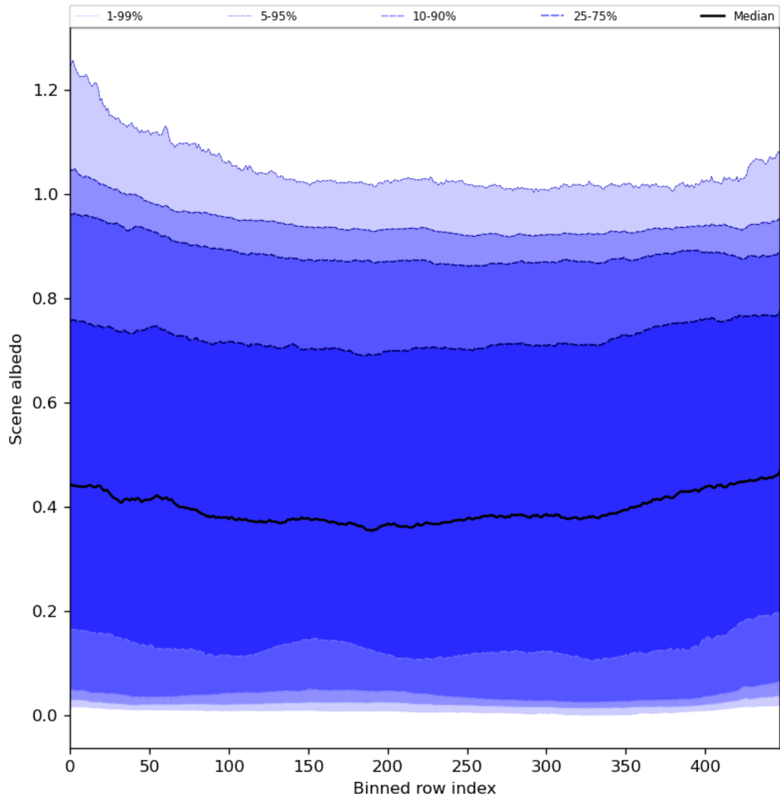
Figure 51: Along track statistics of “Scene albedo” for 2024-05-05 to 2024-05-07
