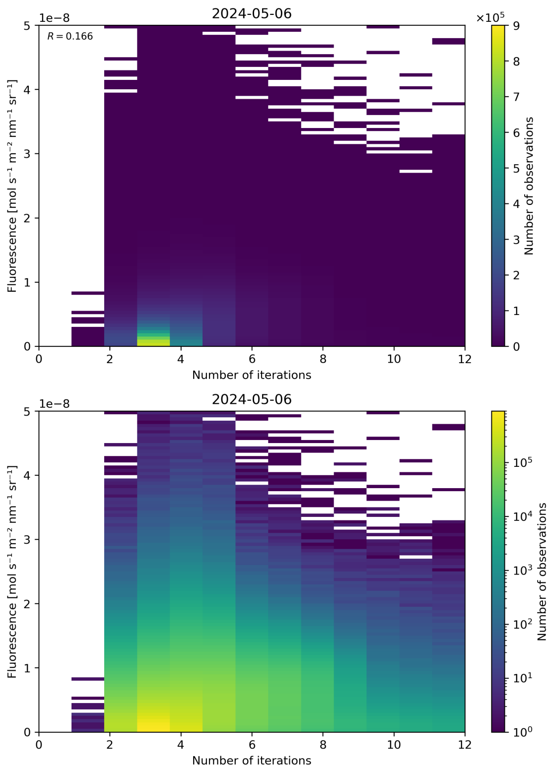
Figure 98: Scatter density plot of “Number of iterations” against “Fluorescence” for 2024-05-05 to 2024-05-07.
