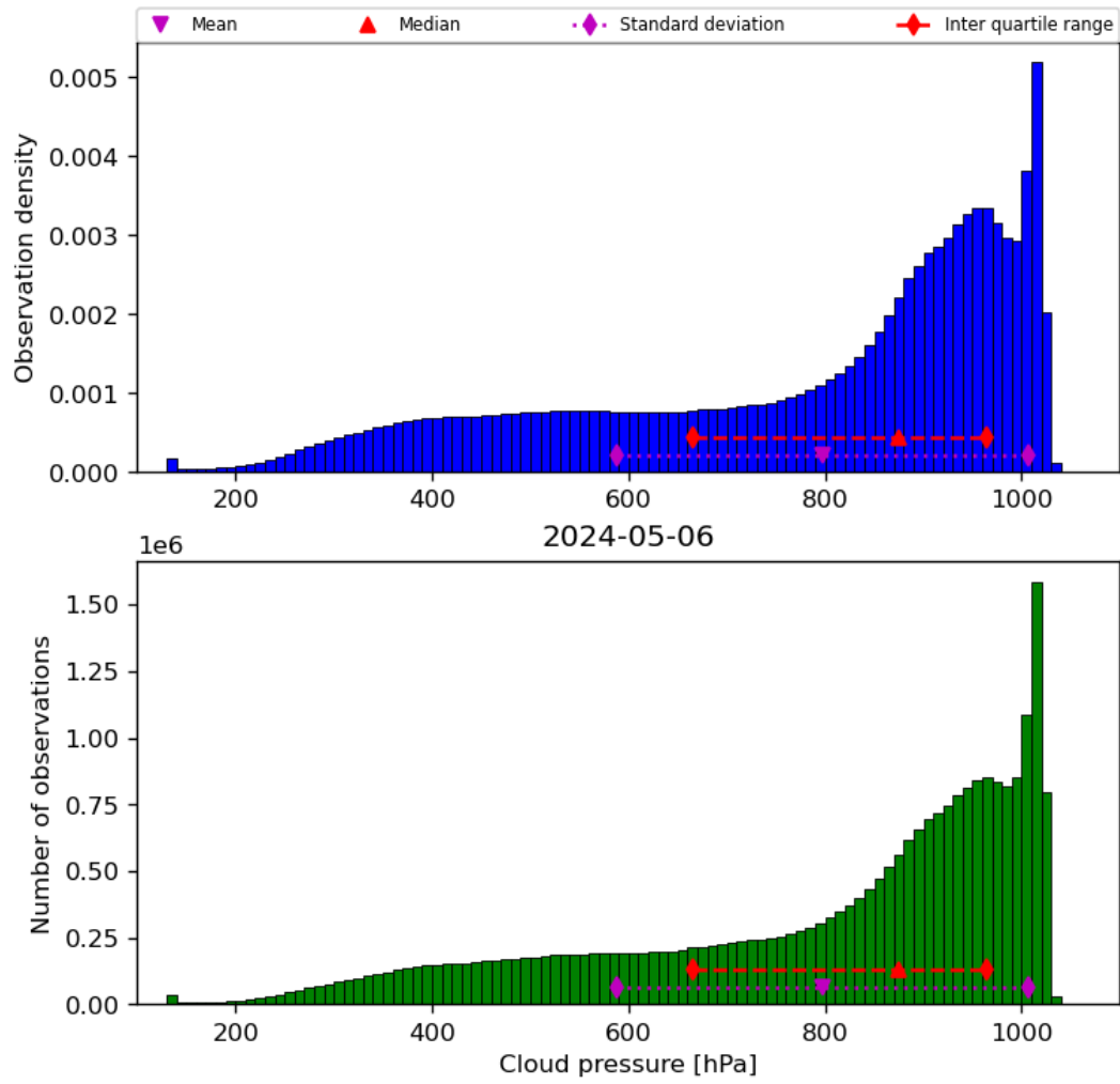
Figure 30: Histogram of “Cloud pressure” for 2024-05-05 to 2024-05-07
