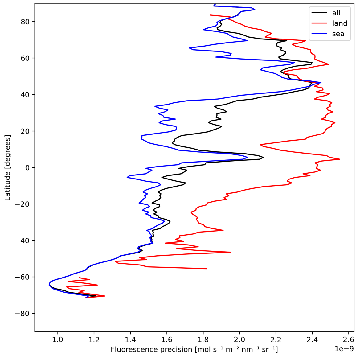
Figure 24: Zonal average of “Fluorescence precision” for 2024-05-05 to 2024-05-07.
