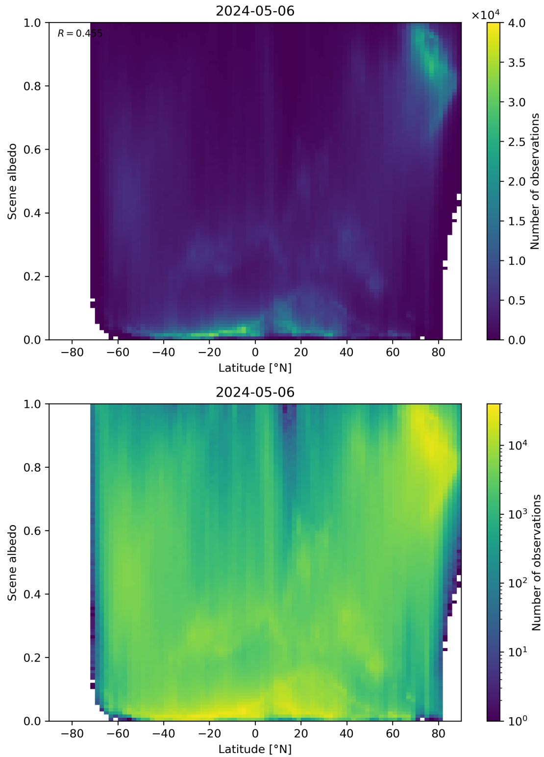
Figure 95: Scatter density plot of “Latitude” against “Scene albedo” for 2024-05-05 to 2024-05-07.
