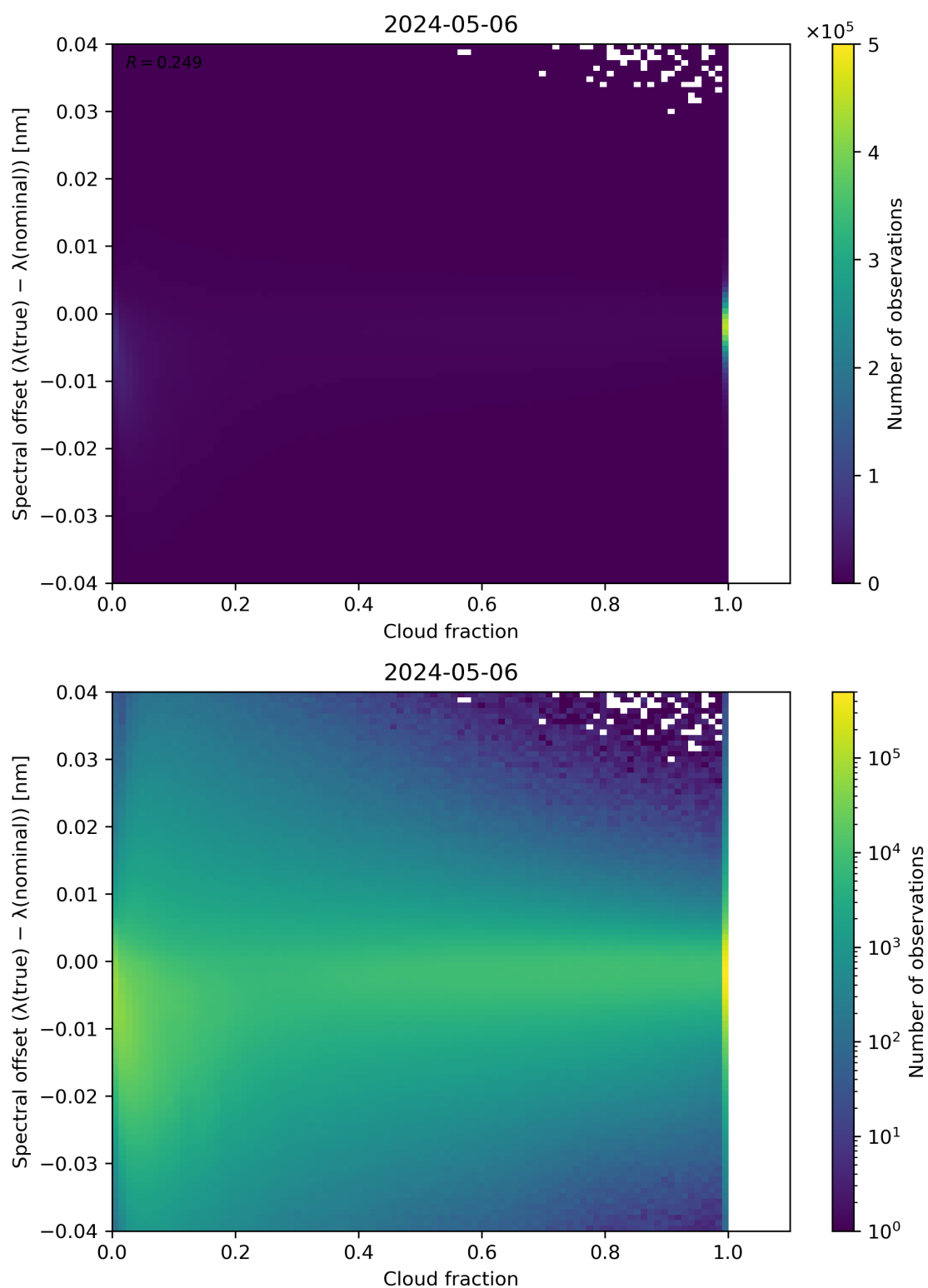
Figure 76: Scatter density plot of “Cloud fraction” against “Spectral offset ( \lambda(\text{true}) - \lambda(\text{nominal}) )” for 2024-05-05 to 2024-05-07.
