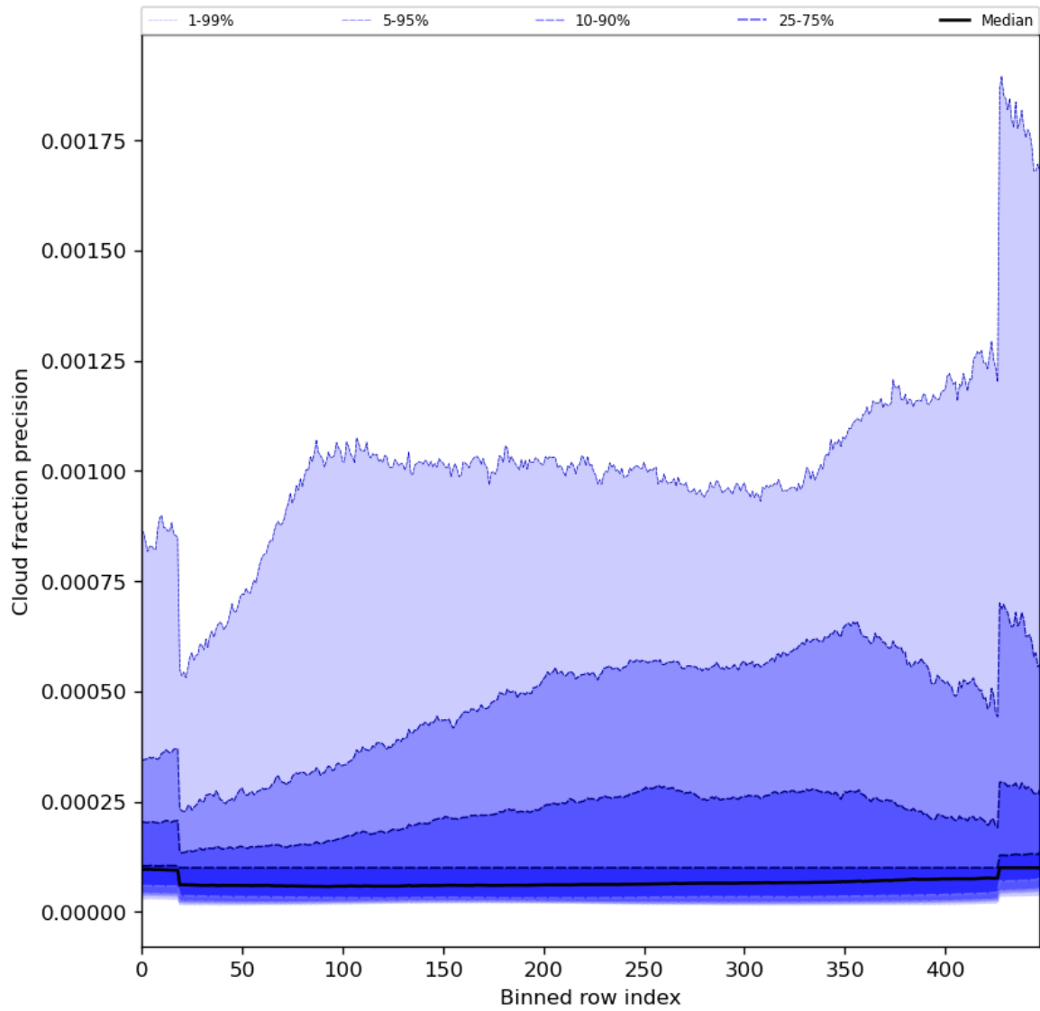
Figure 50: Along track statistics of “Cloud fraction precision” for 2024-05-05 to 2024-05-07
