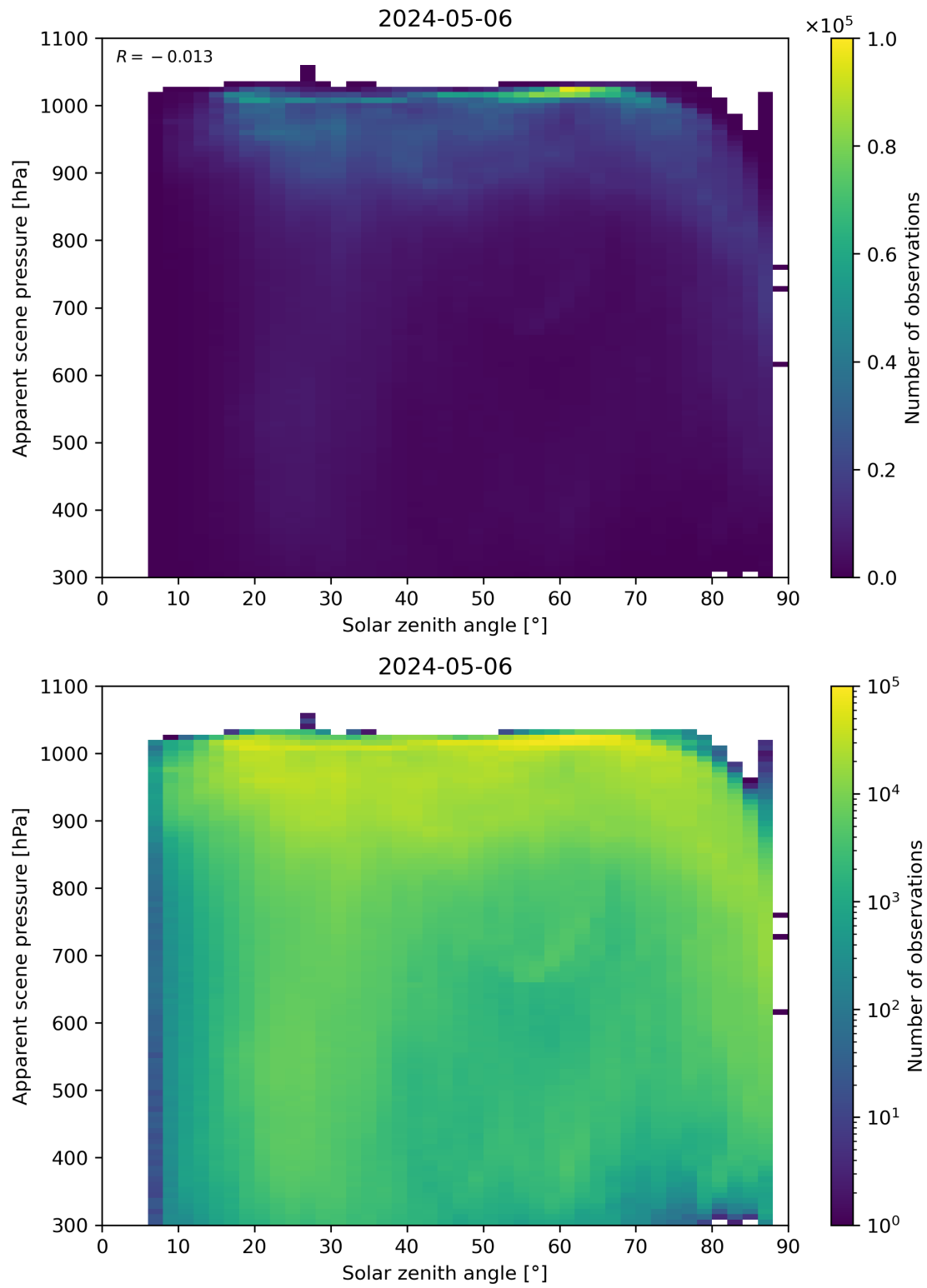
Figure 108: Scatter density plot of “Solar zenith angle” against “Apparent scene pressure” for 2024-05-05 to 2024-05-07.
