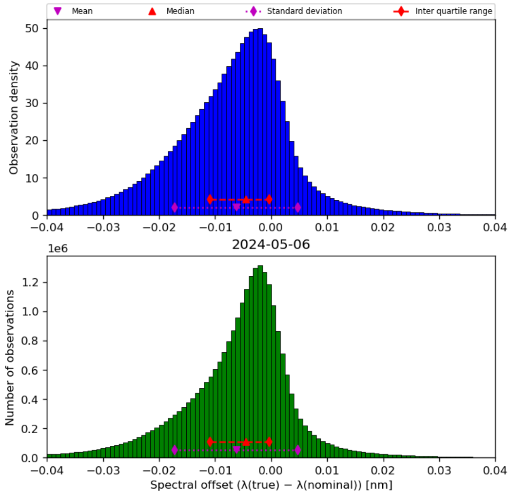
Figure 45: Histogram of “Spectral offset ( \lambda(\text{true}) - \lambda(\text{nominal}) )” for 2024-05-05 to 2024-05-07
