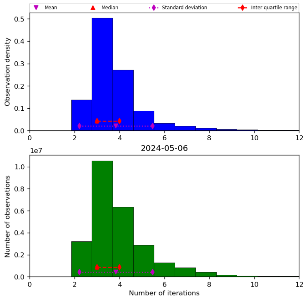
Figure 39: Histogram of “Number of iterations” for 2024-05-05 to 2024-05-07
