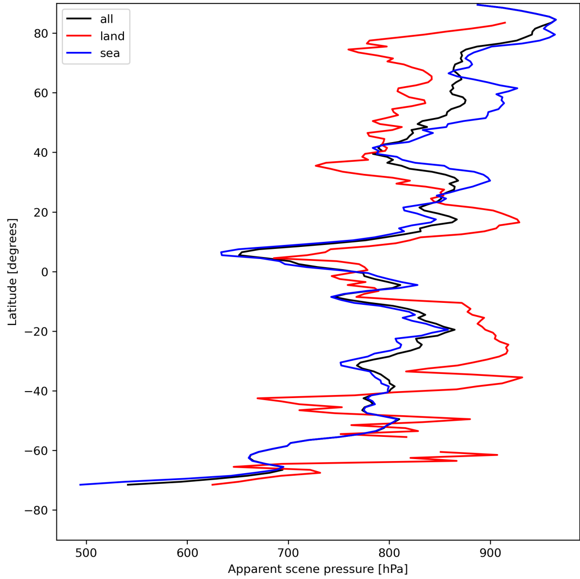
Figure 19: Zonal average of “Apparent scene pressure” for 2024-05-05 to 2024-05-07.
