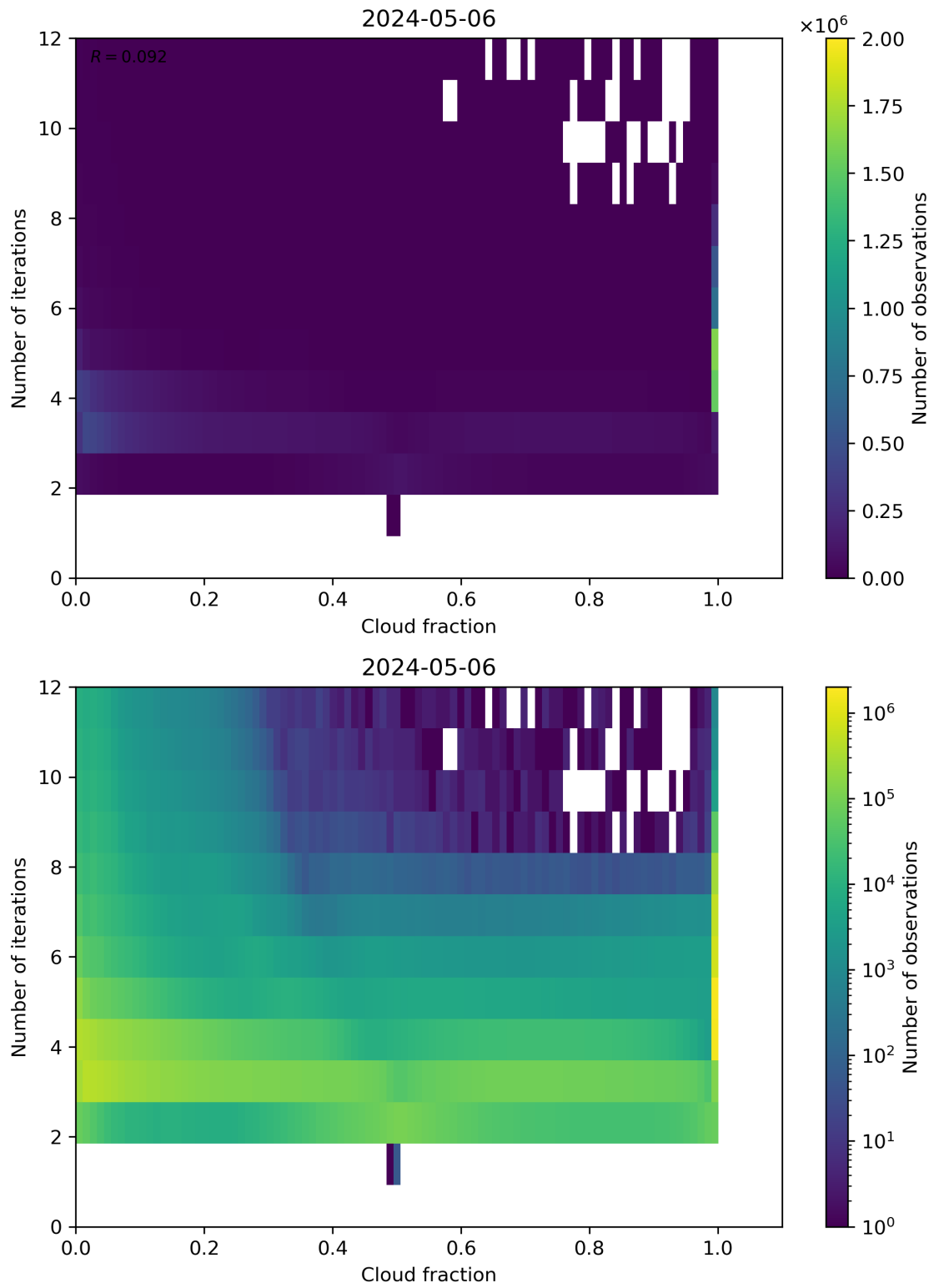
Figure 73: Scatter density plot of “Cloud fraction” against “Number of iterations” for 2024-05-05 to 2024-05-07.
