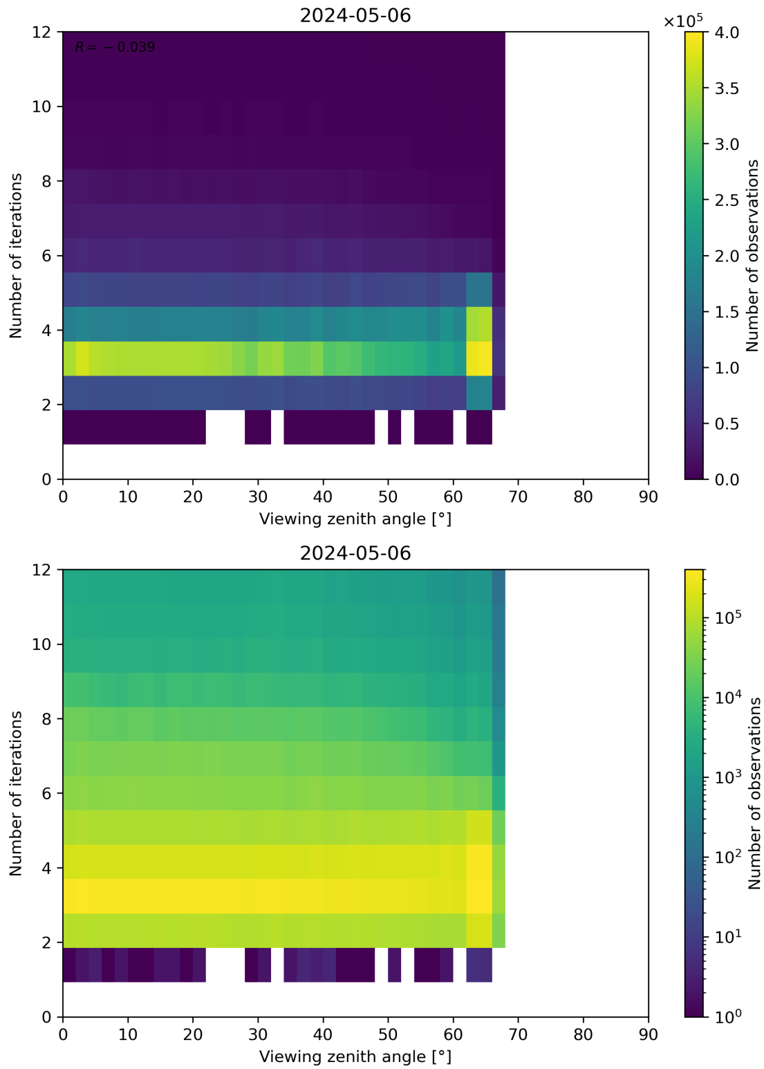
Figure 124: Scatter density plot of “Viewing zenith angle” against “Number of iterations” for 2024-05-05 to 2024-05-07.
