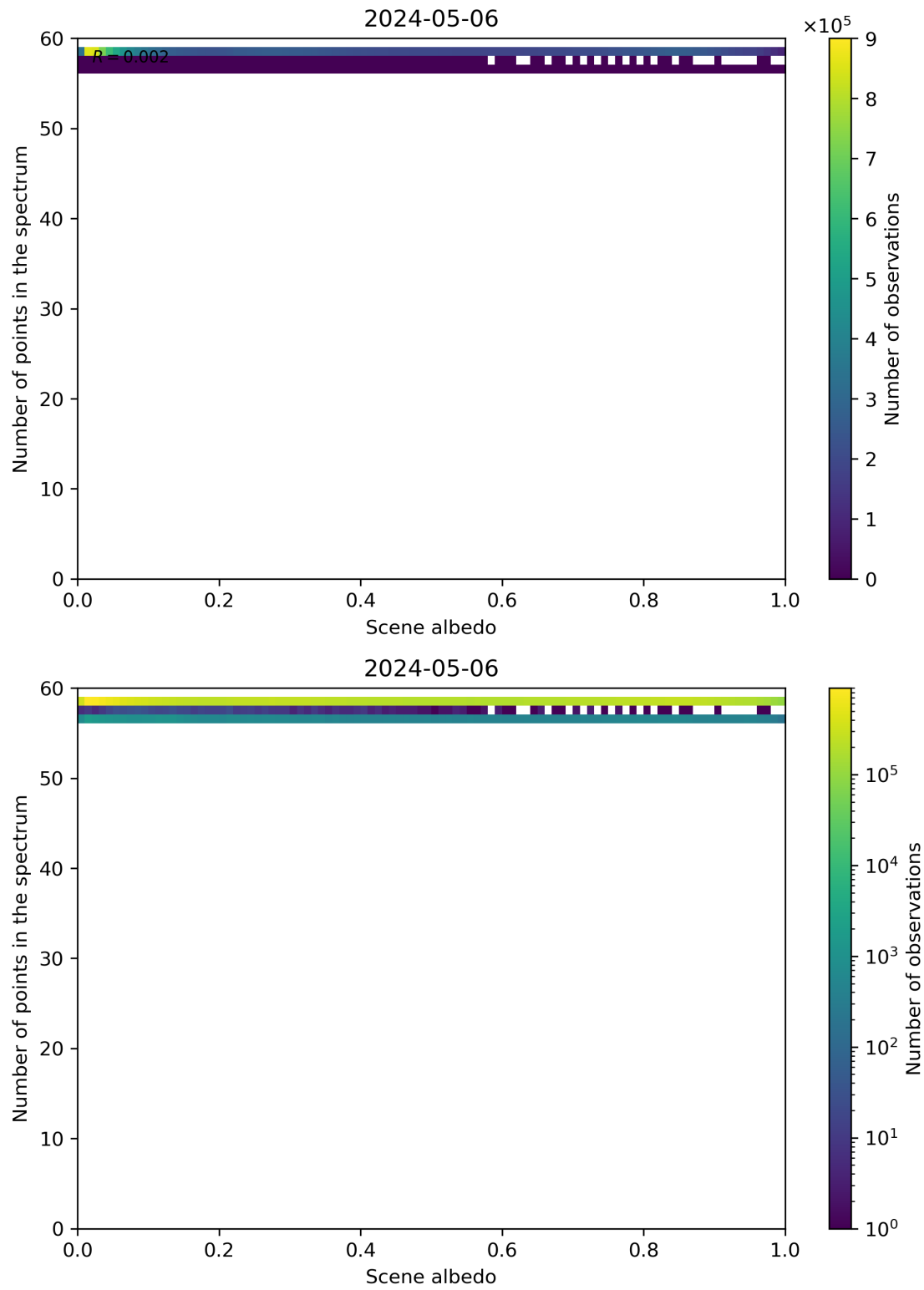
Figure 106: Scatter density plot of “Scene albedo” against “Number of points in the spectrum” for 2024-05-05 to 2024-05-07.
