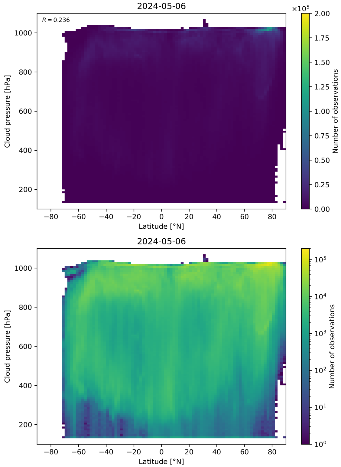
Figure 91: Scatter density plot of “Latitude” against “Cloud pressure” for 2024-05-05 to 2024-05-07.
