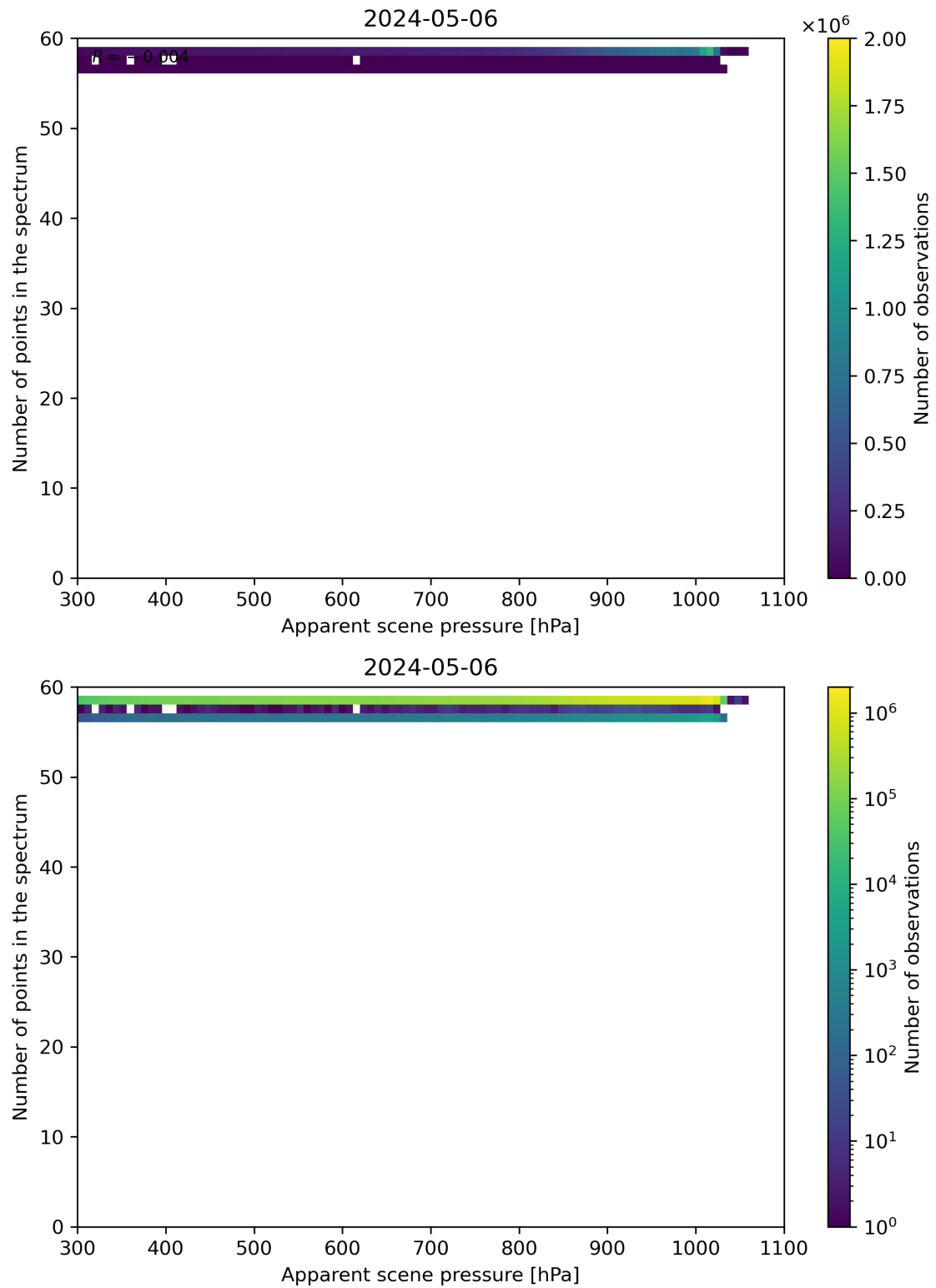
Figure 66: Scatter density plot of “Apparent scene pressure” against “Number of points in the spectrum” for 2024-05-05 to 2024-05-07.
