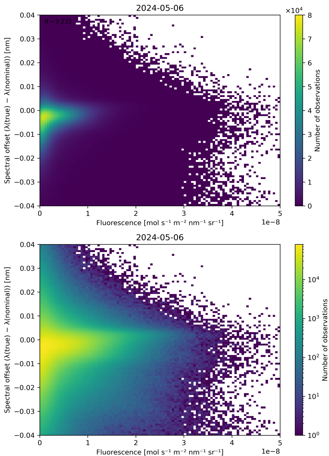
Figure 87: Scatter density plot of “Fluorescence” against “Spectral offset ( \lambda(\text{true}) - \lambda(\text{nominal}) )” for 2024-05-05 to 2024-05-07.
