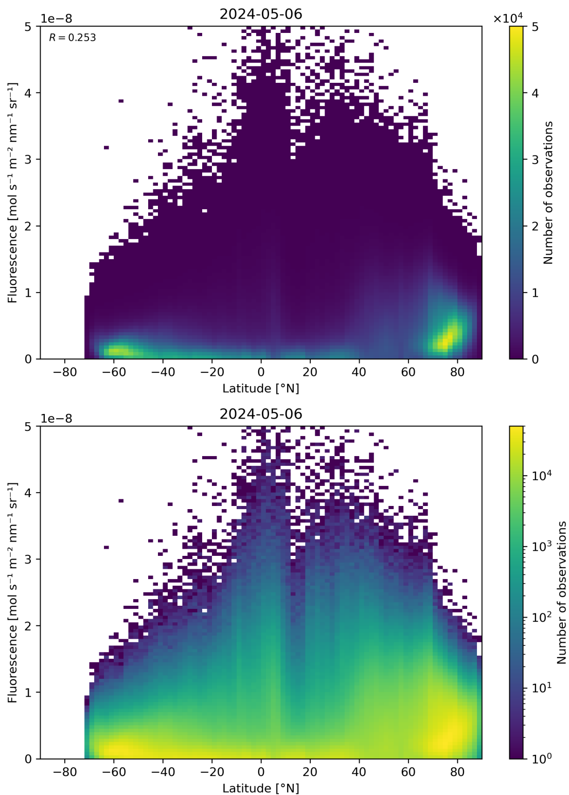
Figure 92: Scatter density plot of “Latitude” against “Fluorescence” for 2024-05-05 to 2024-05-07.
