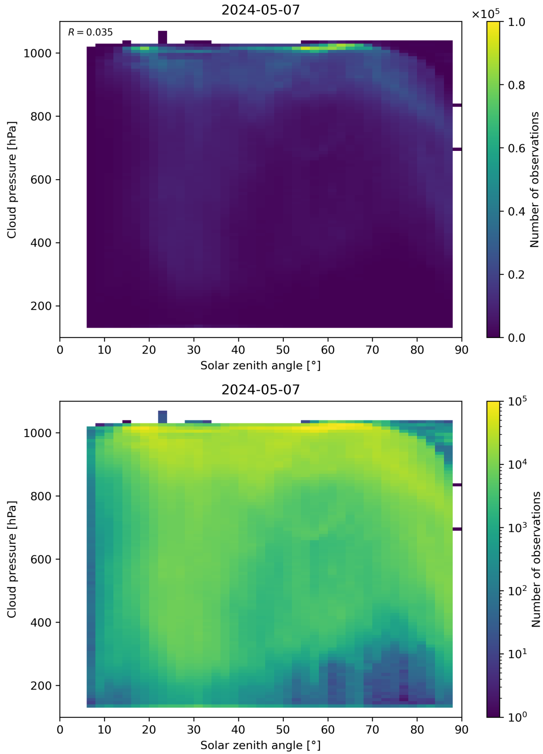
Figure 111: Scatter density plot of “Solar zenith angle” against “Cloud pressure” for 2024-05-07 to 2024-05-08.
