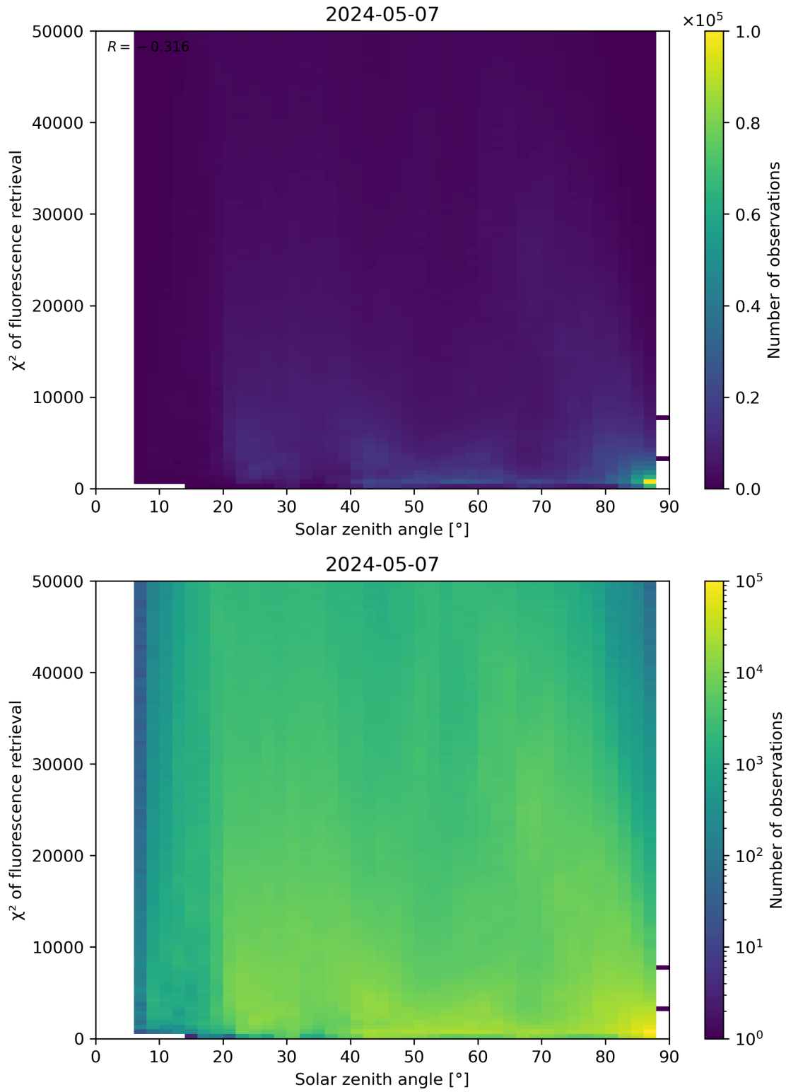
Figure 109: Scatter density plot of “Solar zenith angle” against “ \chi^2 of fluorescence retrieval” for 2024-05-07 to 2024-05-08.
