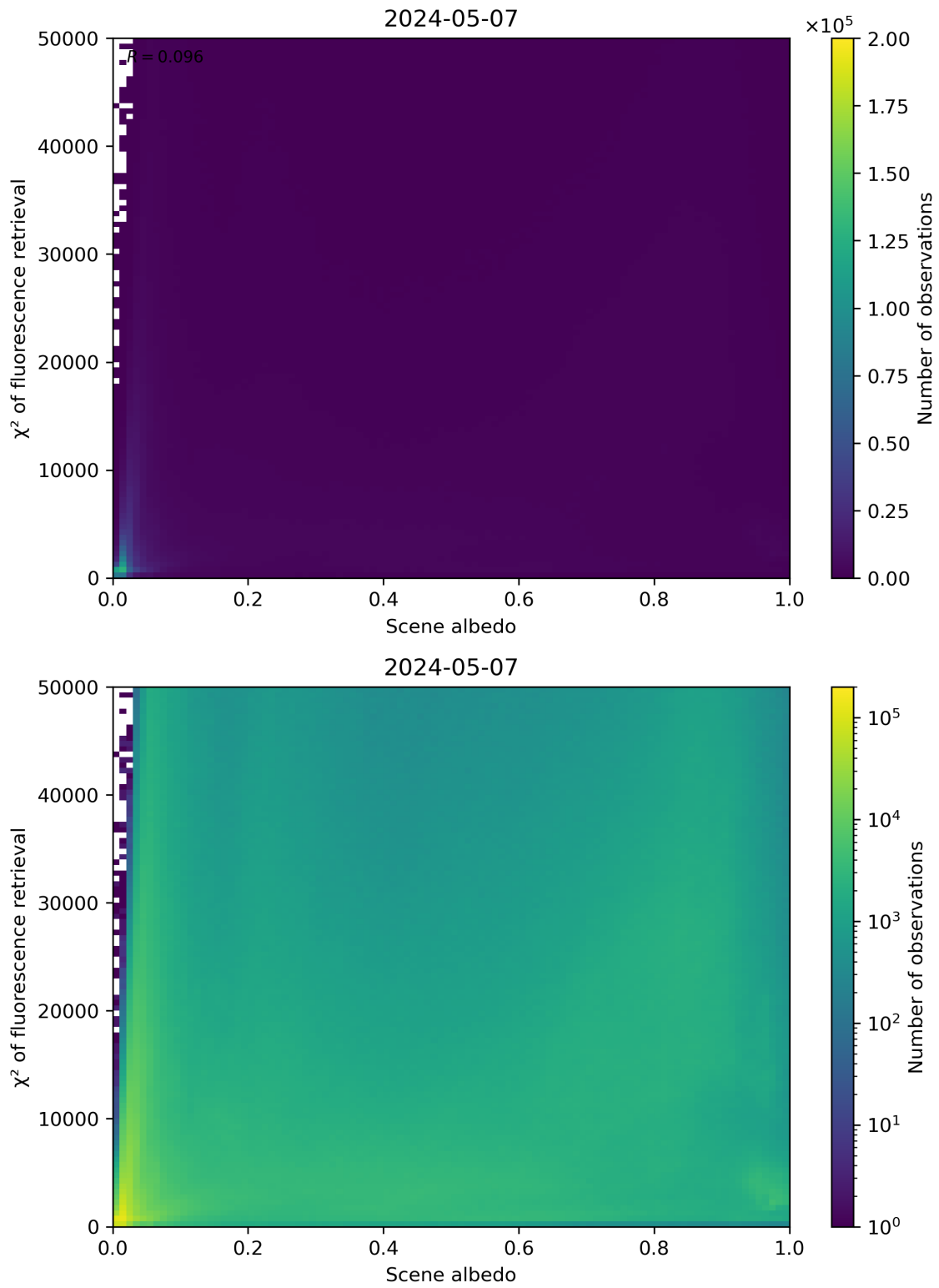
Figure 103: Scatter density plot of “Scene albedo” against “ \chi^2 of fluorescence retrieval” for 2024-05-07 to 2024-05-08.
