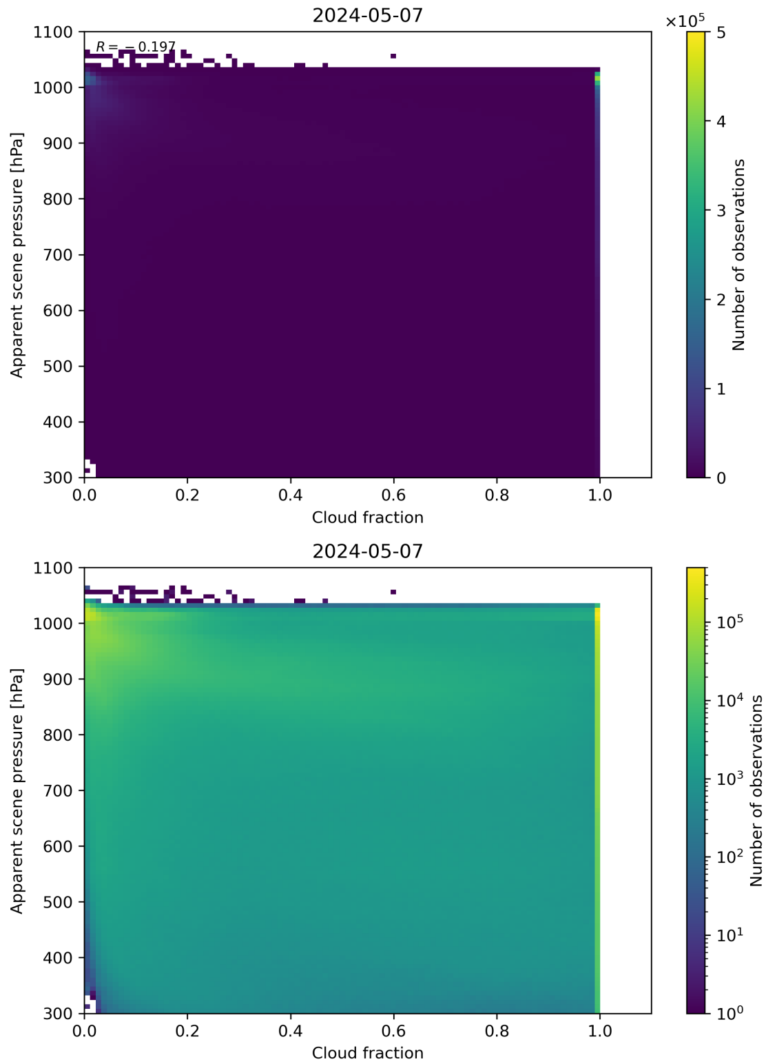
Figure 70: Scatter density plot of “Cloud fraction” against “Apparent scene pressure” for 2024-05-07 to 2024-05-08.
