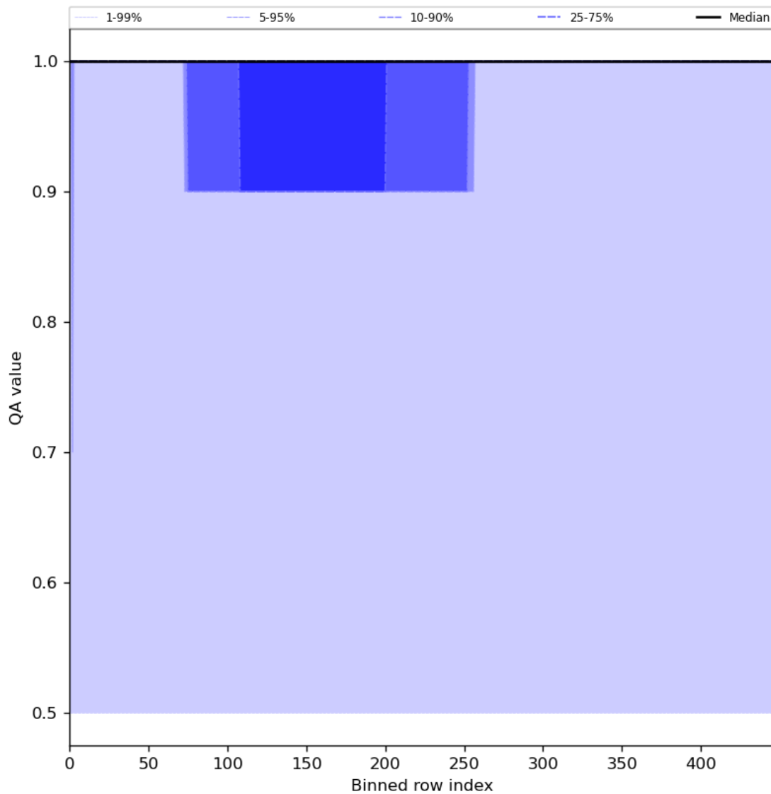
Figure 46: Along track statistics of “QA value” for 2024-05-07 to 2024-05-08
