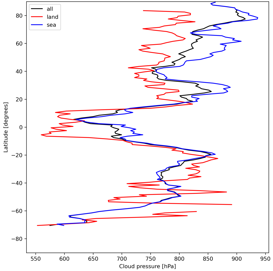
Figure 13: Zonal average of “Cloud pressure” for 2024-05-07 to 2024-05-08.
