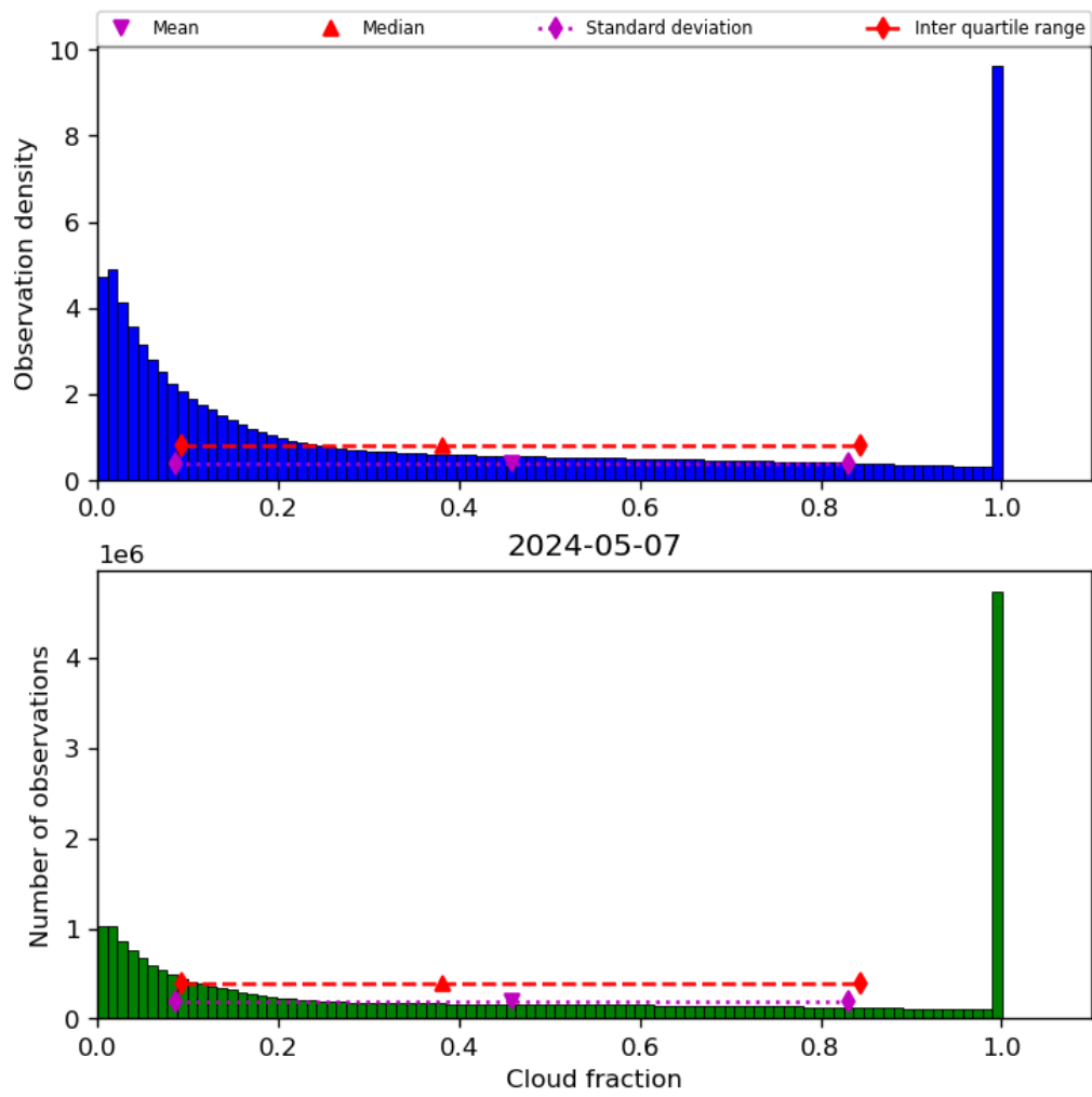
Figure 32: Histogram of “Cloud fraction” for 2024-05-07 to 2024-05-08
