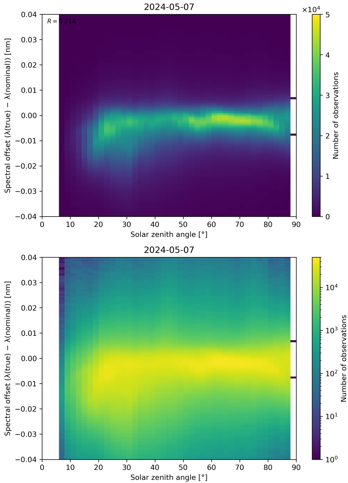
Figure 117: Scatter density plot of “Solar zenith angle” against “Spectral offset ( \lambda(\text{true}) - \lambda(\text{nominal}) )” for 2024-05-07 to 2024-05-08.
