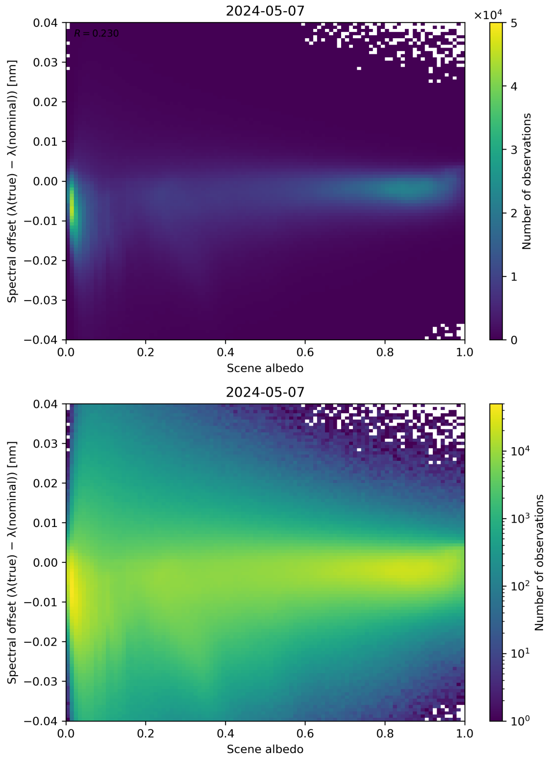
Figure 107: Scatter density plot of “Scene albedo” against “Spectral offset ( \lambda(\text{true}) - \lambda(\text{nominal}) )” for 2024-05-07 to 2024-05-08.
