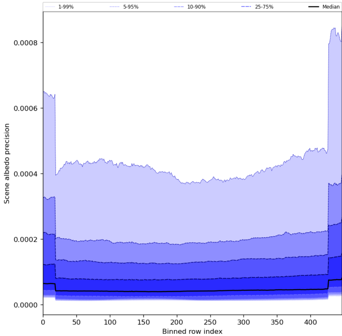
Figure 52: Along track statistics of “Scene albedo precision” for 2024-05-07 to 2024-05-08
