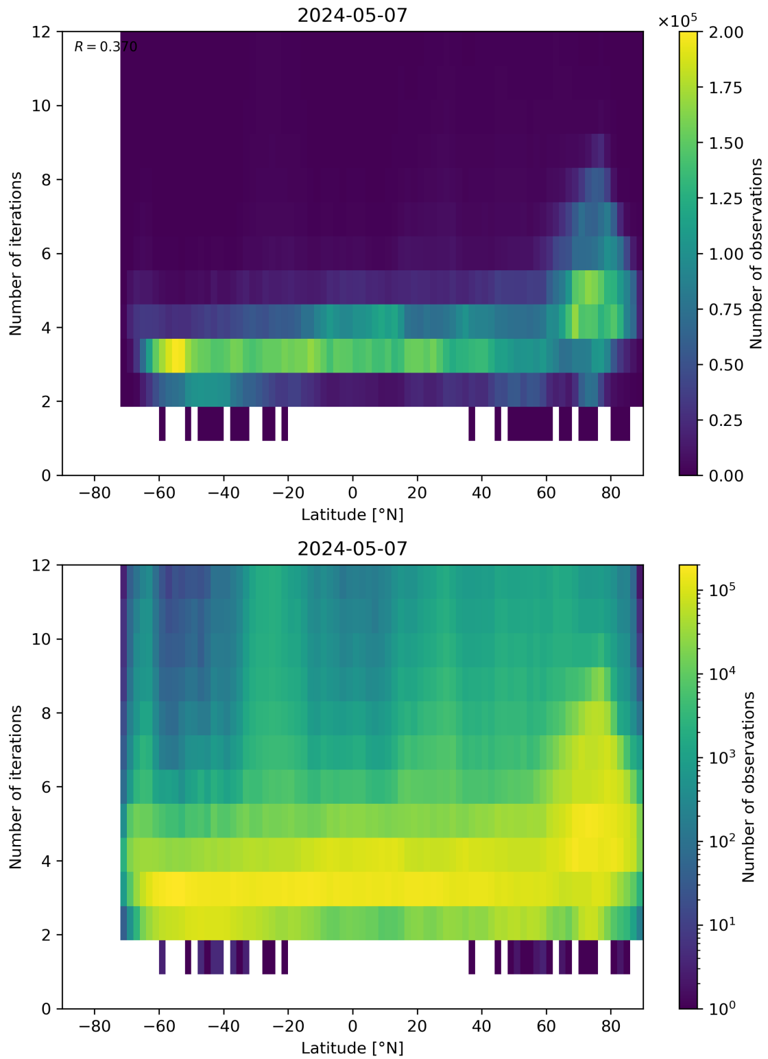
Figure 93: Scatter density plot of “Latitude” against “Number of iterations” for 2024-05-07 to 2024-05-08.
