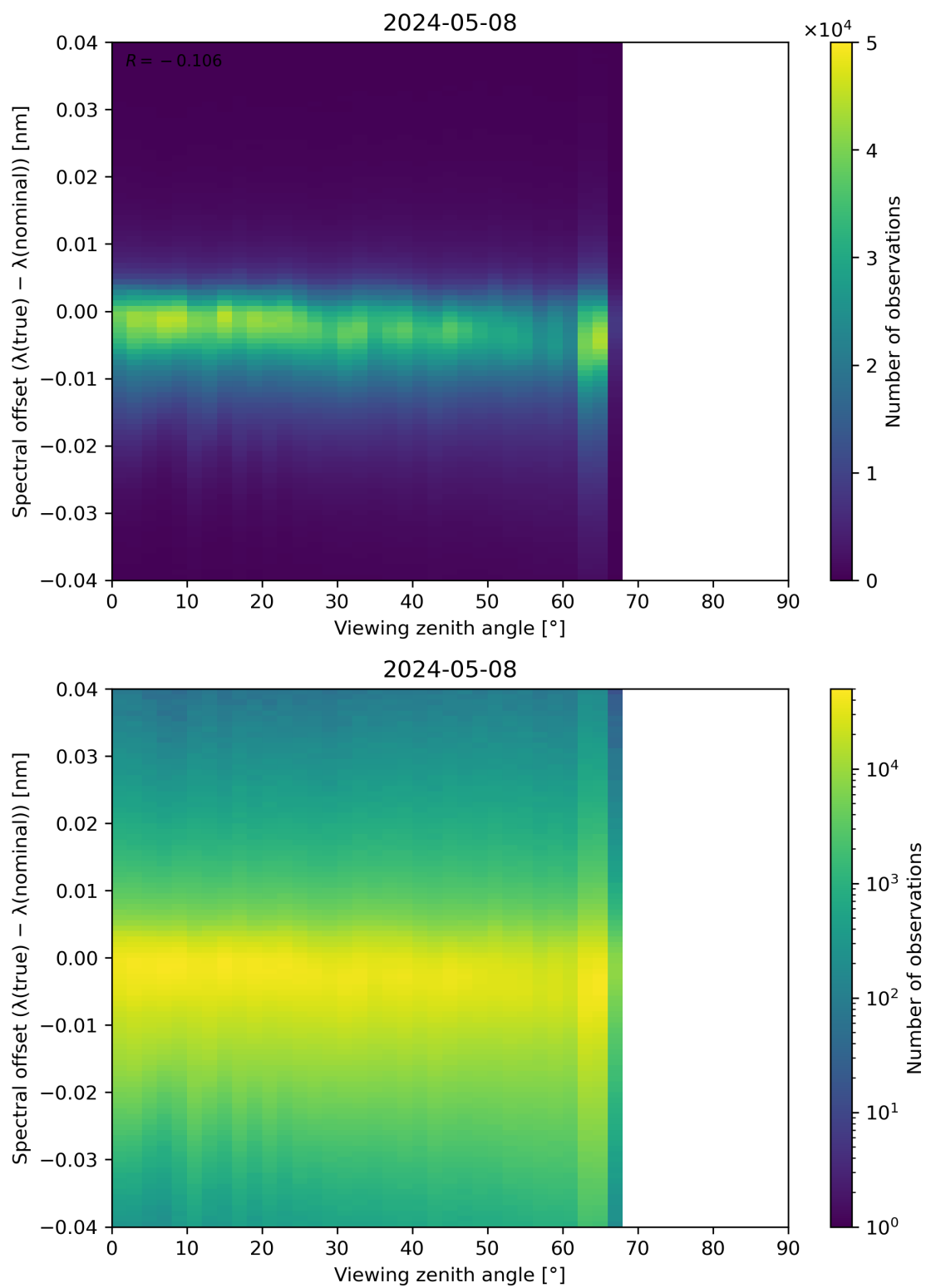
Figure 128: Scatter density plot of “Viewing zenith angle” against “Spectral offset ( \lambda(\text{true}) - \lambda(\text{nominal}) )” for 2024-05-07 to 2024-05-09.
