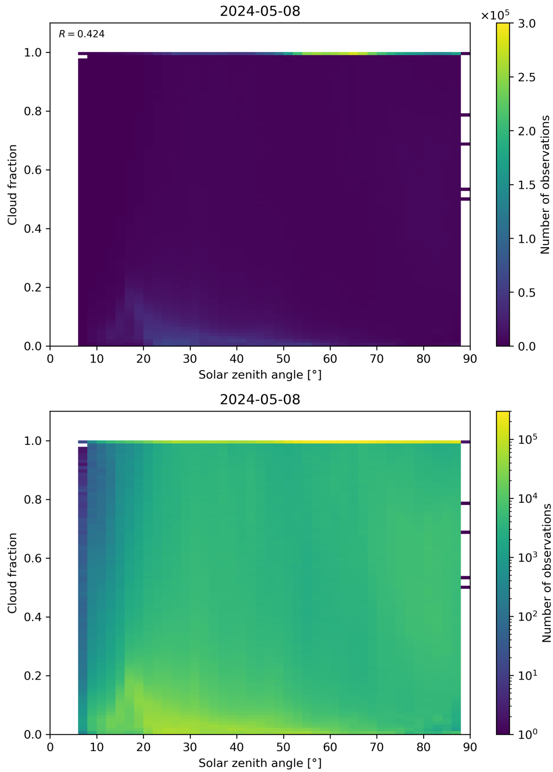
Figure 110: Scatter density plot of “Solar zenith angle” against “Cloud fraction” for 2024-05-07 to 2024-05-09.
