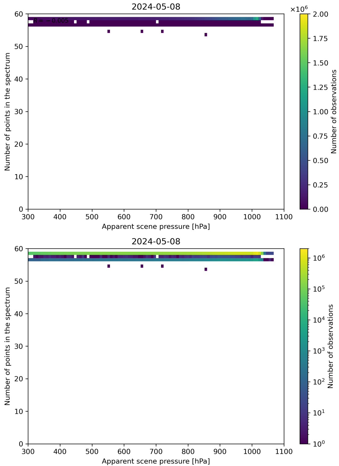
Figure 66: Scatter density plot of “Apparent scene pressure” against “Number of points in the spectrum” for 2024-05-07 to 2024-05-09.
