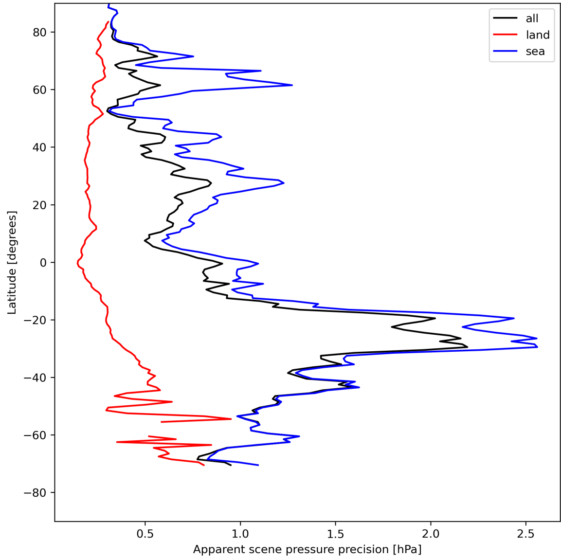
Figure 20: Zonal average of “Apparent scene pressure precision” for 2024-05-07 to 2024-05-09.
