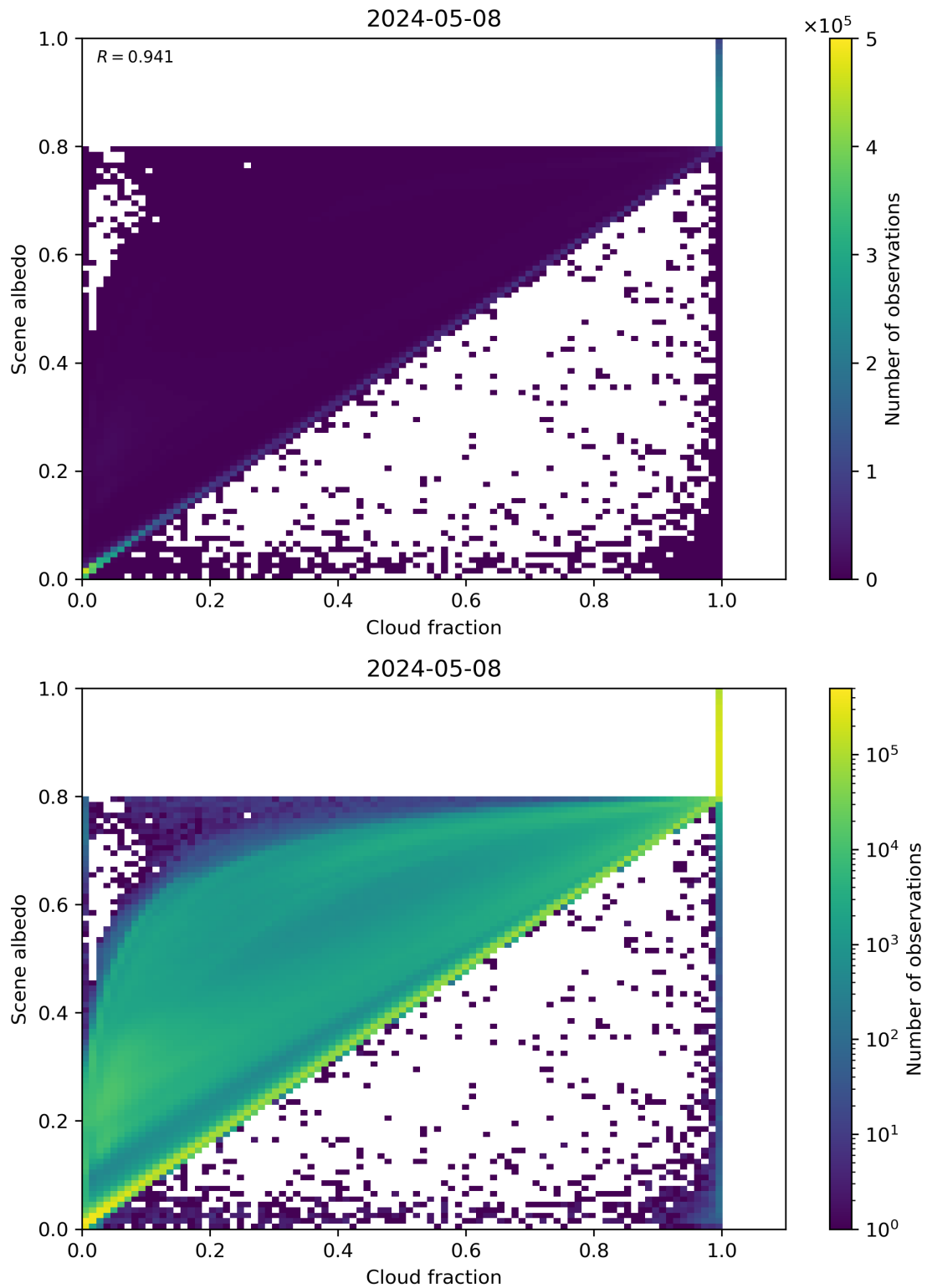
Figure 75: Scatter density plot of “Cloud fraction” against “Scene albedo” for 2024-05-07 to 2024-05-09.
