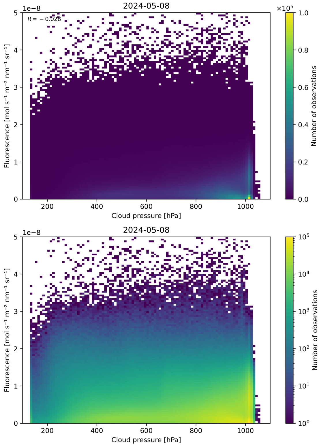
Figure 80: Scatter density plot of “Cloud pressure” against “Fluorescence” for 2024-05-07 to 2024-05-09.
