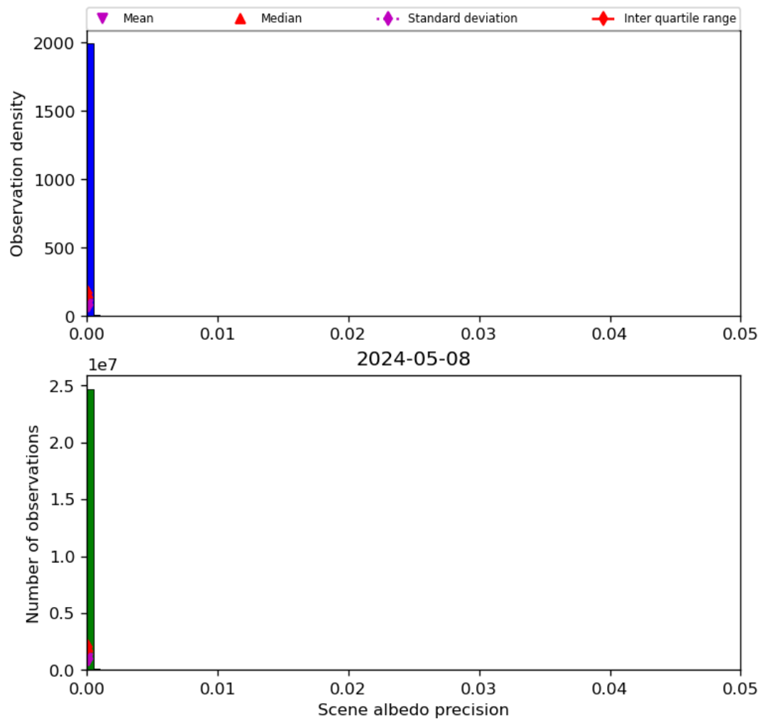
Figure 35: Histogram of “Scene albedo precision” for 2024-05-07 to 2024-05-09
