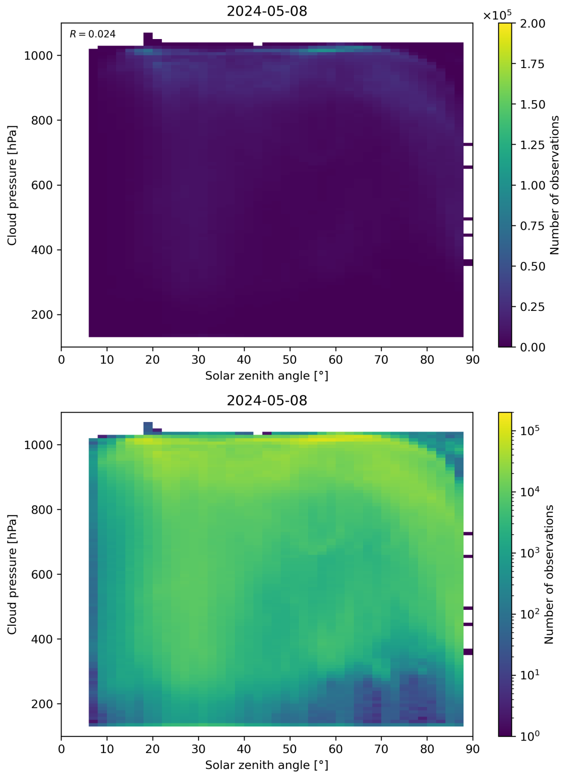
Figure 111: Scatter density plot of “Solar zenith angle” against “Cloud pressure” for 2024-05-07 to 2024-05-09.
