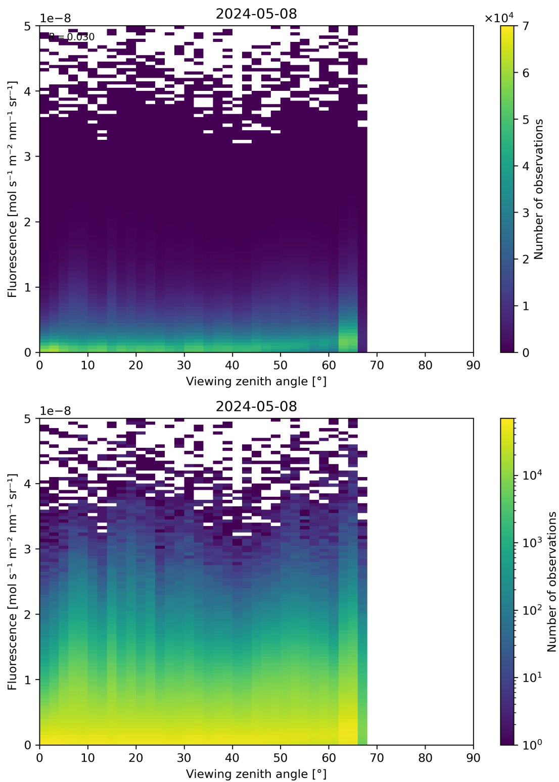
Figure 122: Scatter density plot of “Viewing zenith angle” against “Fluorescence” for 2024-05-07 to 2024-05-09.
