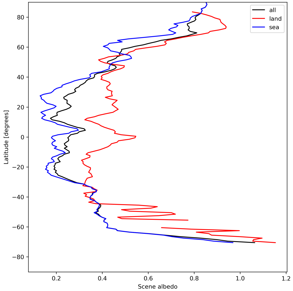
Figure 17: Zonal average of “Scene albedo” for 2024-05-07 to 2024-05-09.
