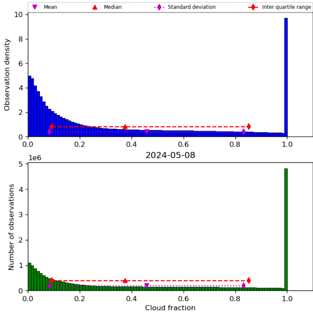
Figure 32: Histogram of “Cloud fraction” for 2024-05-07 to 2024-05-09
