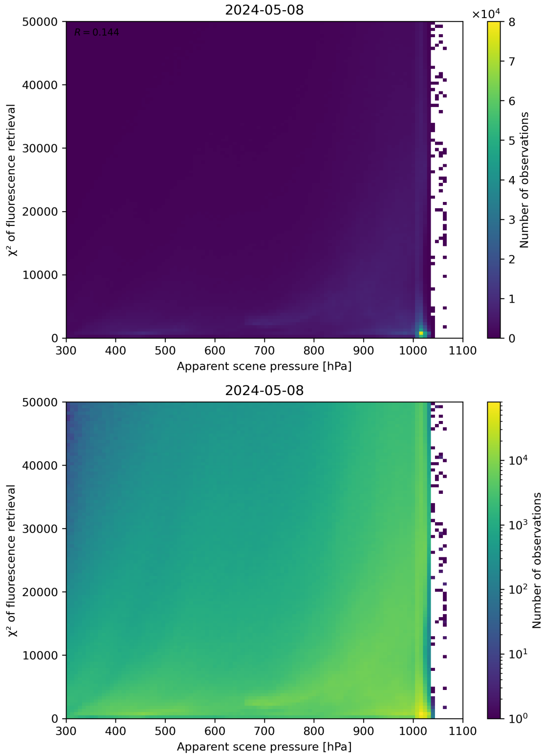
Figure 63: Scatter density plot of “Apparent scene pressure” against “ \chi^2 of fluorescence retrieval” for 2024-05-07 to 2024-05-09.
