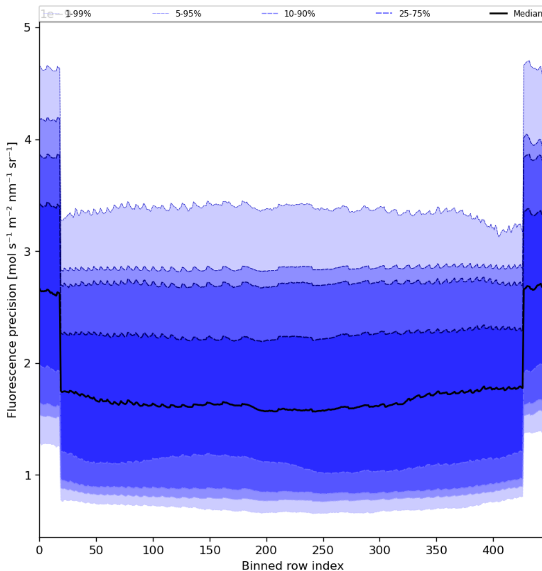
Figure 58: Along track statistics of “Fluorescence precision” for 2024-05-07 to 2024-05-09
