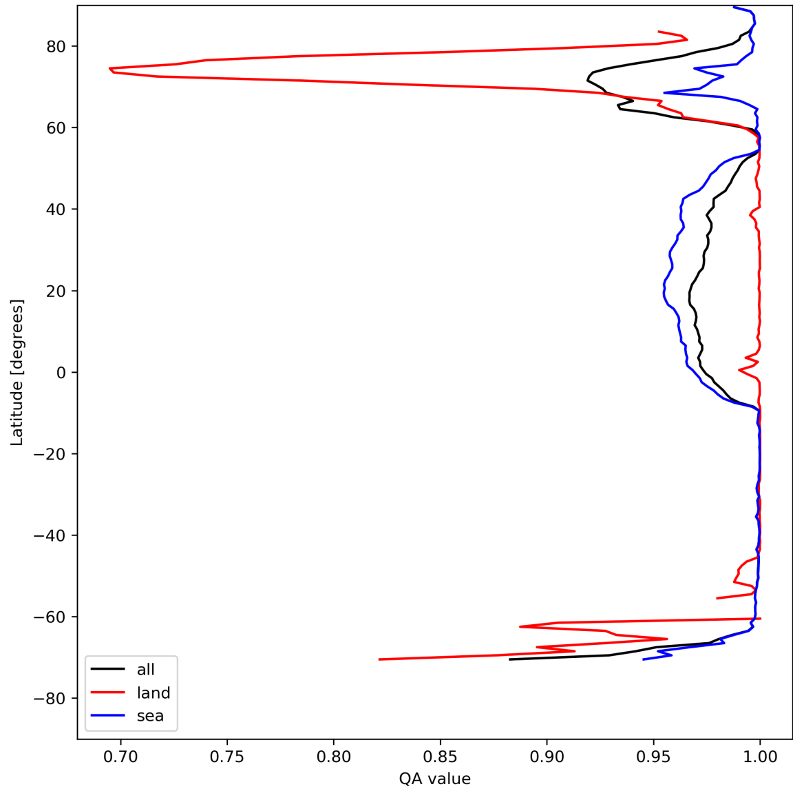
Figure 12: Zonal average of “QA value” for 2024-05-07 to 2024-05-09.
