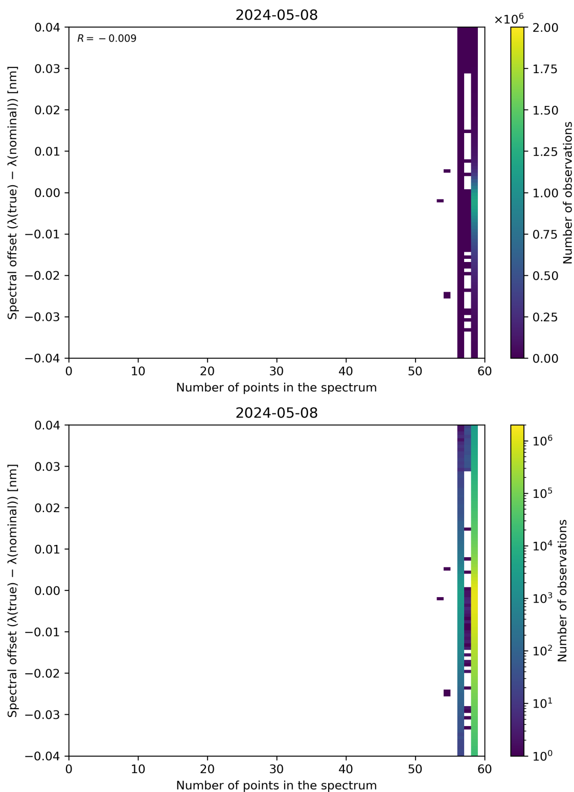
Figure 101: Scatter density plot of “Number of points in the spectrum” against “Spectral offset ( \lambda(\text{true}) - \lambda(\text{nominal}) )” for 2024-05-07 to 2024-05-09.
