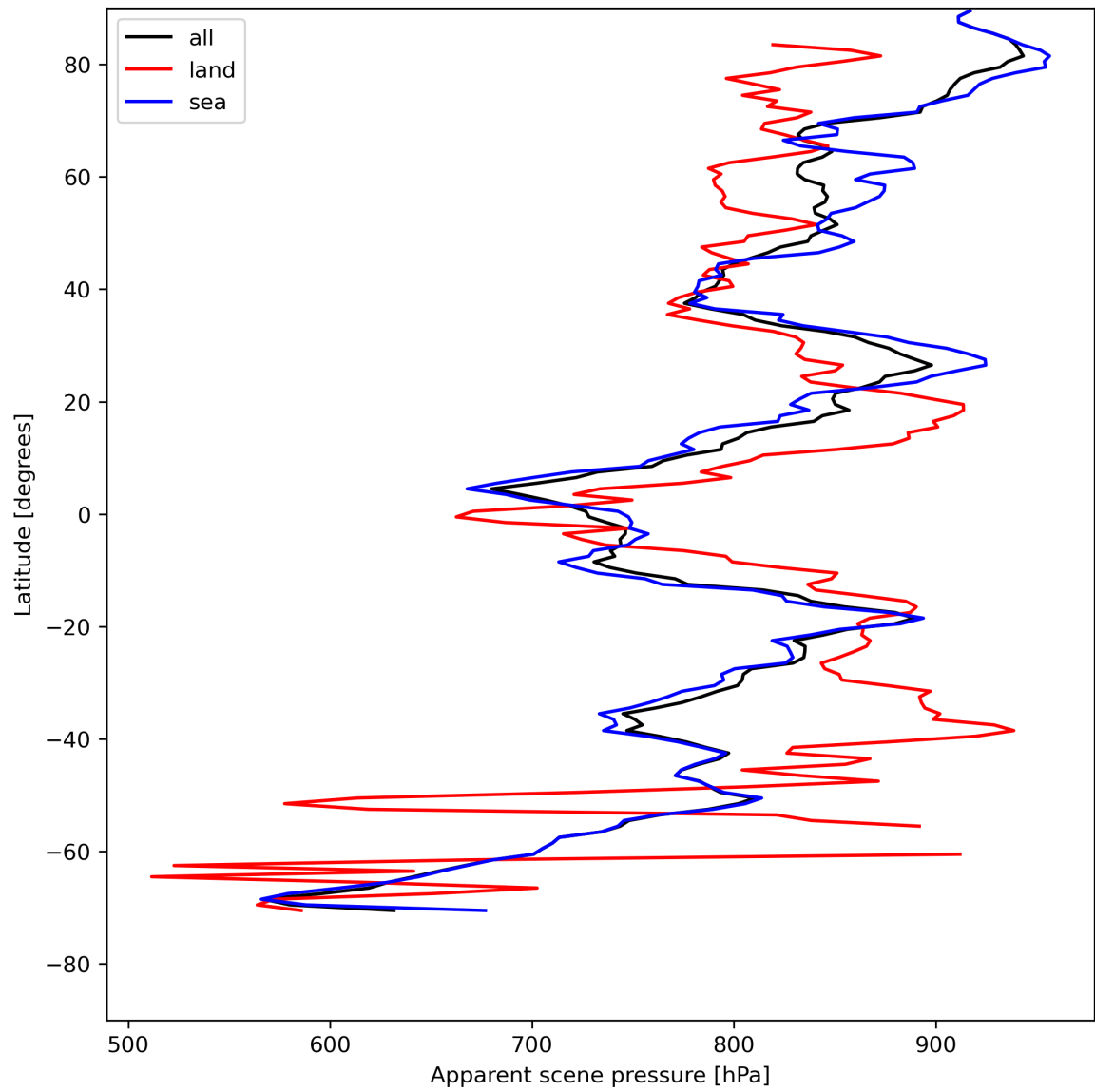
Figure 19: Zonal average of “Apparent scene pressure” for 2024-05-07 to 2024-05-09.
