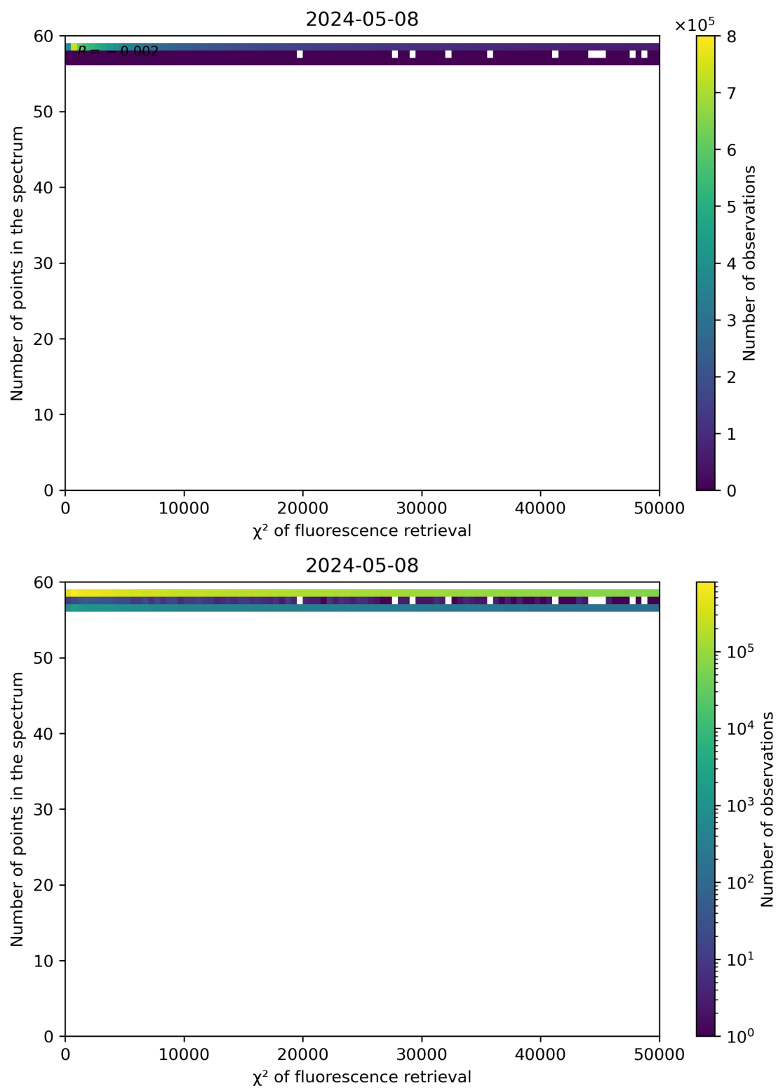
Figure 68: Scatter density plot of " \chi^2 of fluorescence retrieval" against "Number of points in the spectrum" for 2024-05-07 to 2024-05-09.
