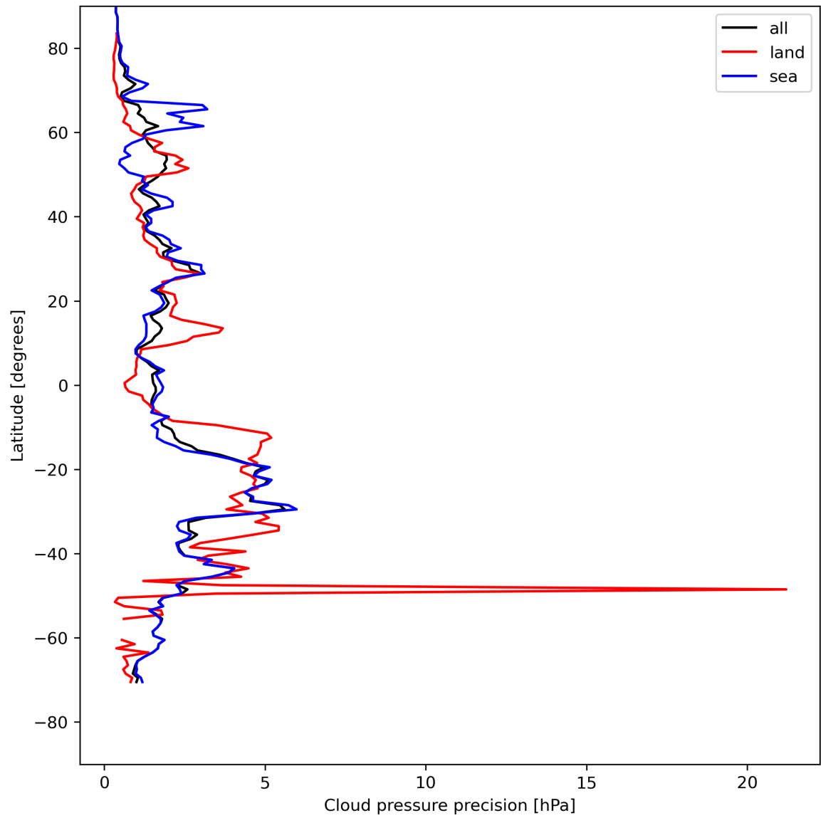
Figure 14: Zonal average of “Cloud pressure precision” for 2024-05-07 to 2024-05-09.
