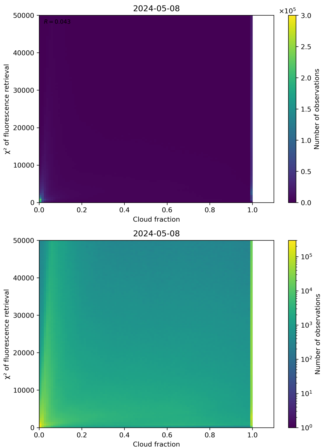
Figure 71: Scatter density plot of “Cloud fraction” against “ \chi^2 of fluorescence retrieval” for 2024-05-07 to 2024-05-09.
