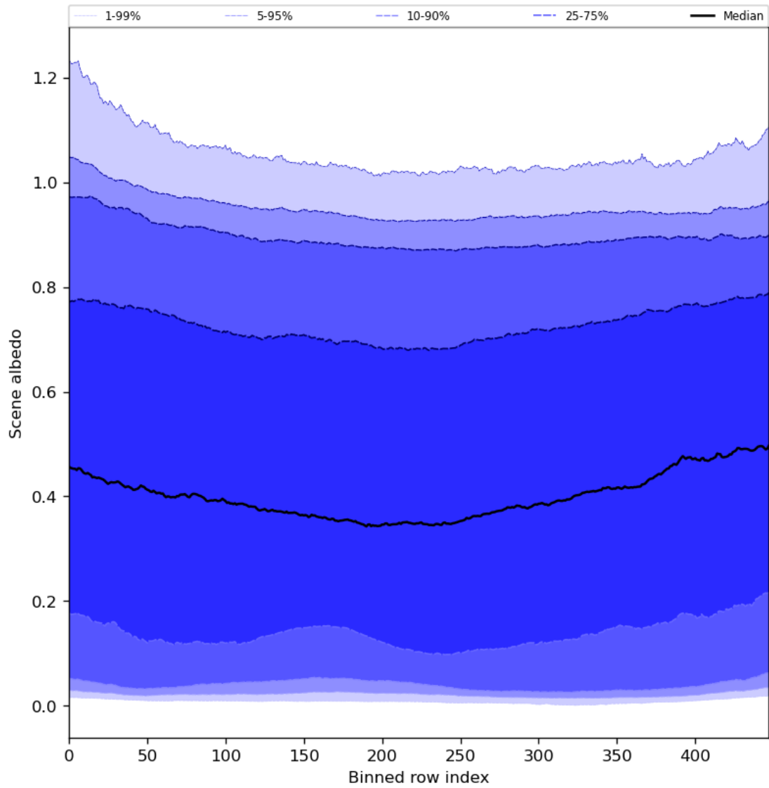
Figure 51: Along track statistics of “Scene albedo” for 2024-05-07 to 2024-05-09
