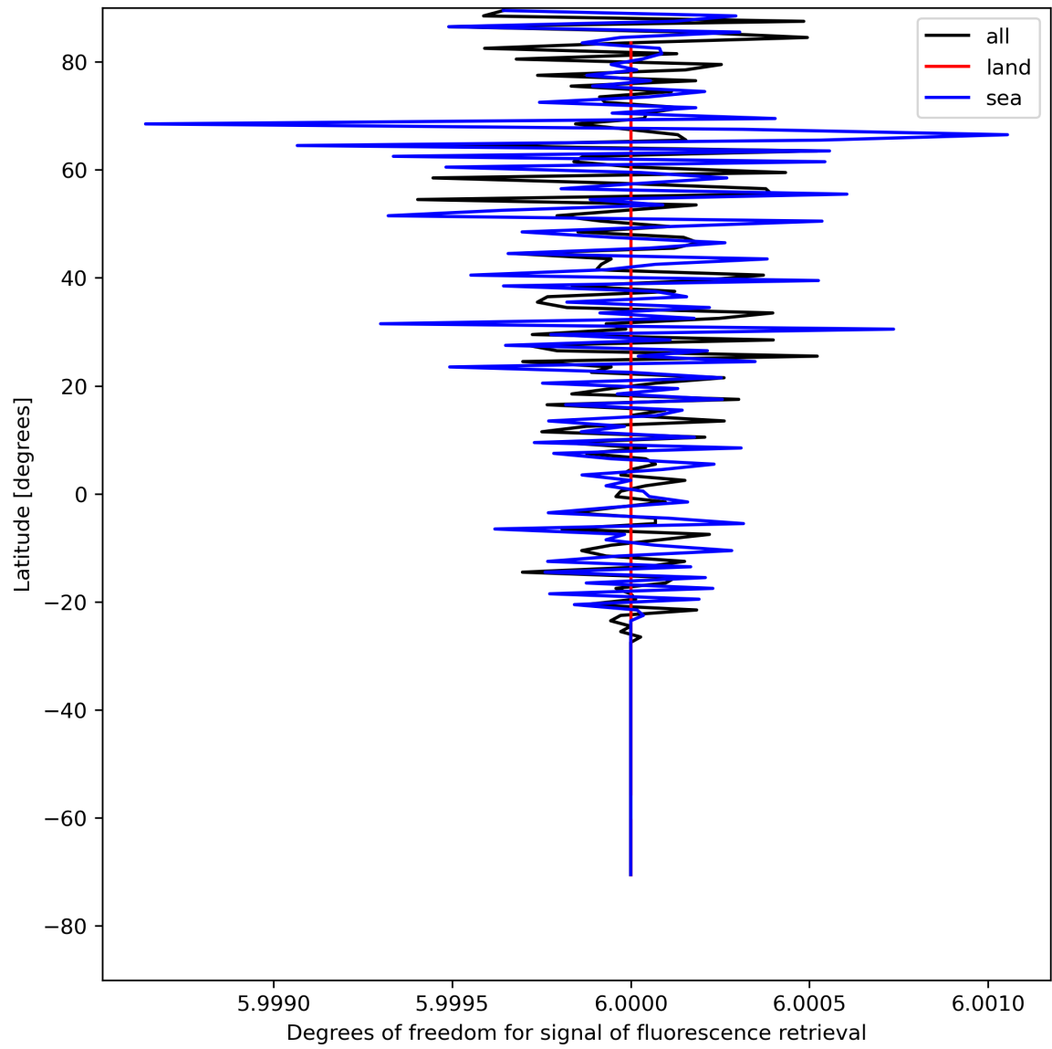
Figure 26: Zonal average of “Degrees of freedom for signal of fluorescence retrieval” for 2024-05-07 to 2024-05-09.
