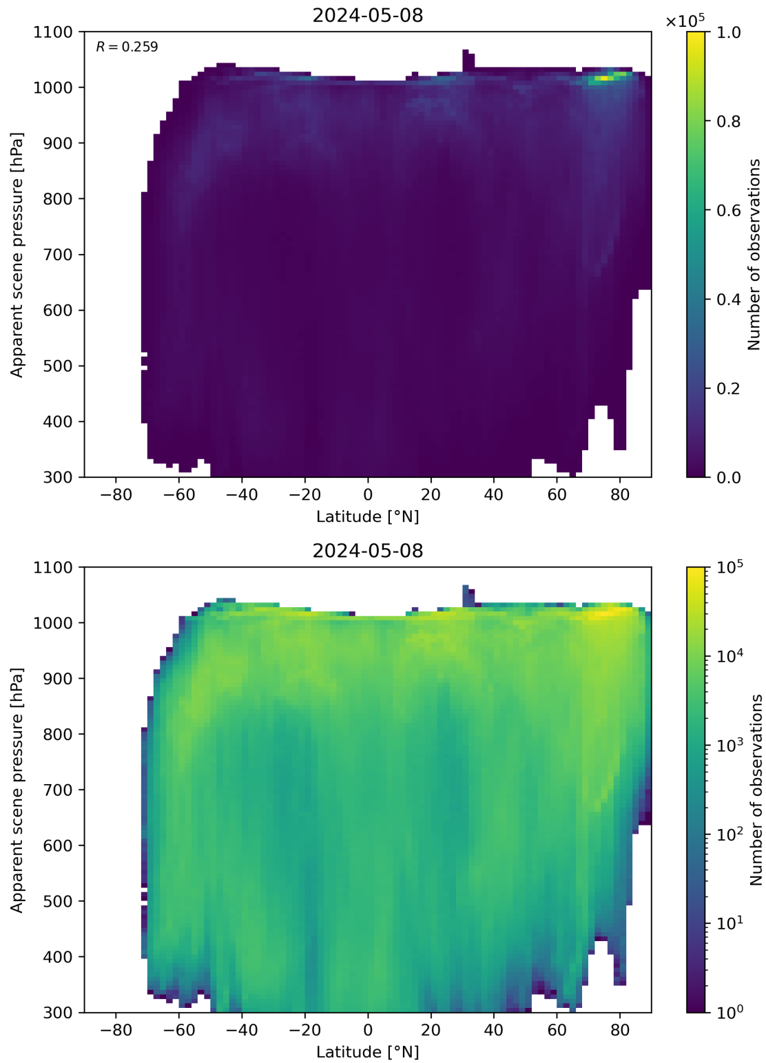
Figure 88: Scatter density plot of “Latitude” against “Apparent scene pressure” for 2024-05-07 to 2024-05-09.
