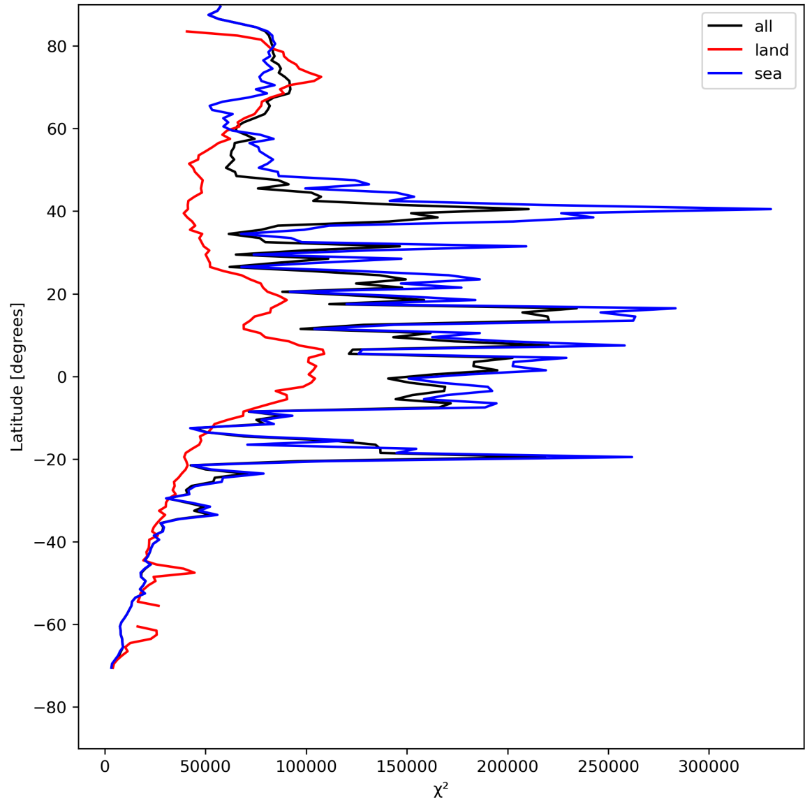
Figure 21: Zonal average of “ \chi^2 ” for 2024-05-07 to 2024-05-09.
