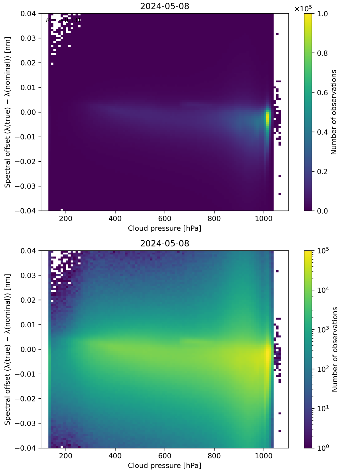
Figure 84: Scatter density plot of “Cloud pressure” against “Spectral offset ( \lambda(\text{true}) - \lambda(\text{nominal}) )” for 2024-05-07 to 2024-05-09.
