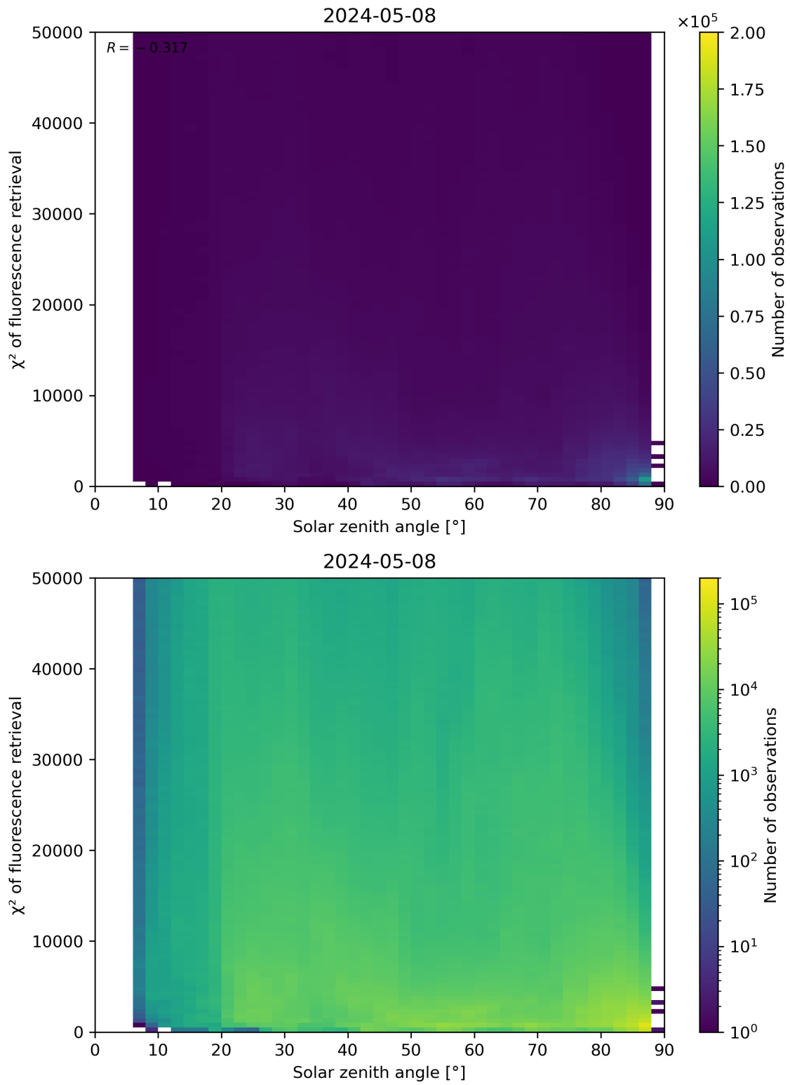
Figure 109: Scatter density plot of “Solar zenith angle” against “ \chi^2 of fluorescence retrieval” for 2024-05-07 to 2024-05-09.
