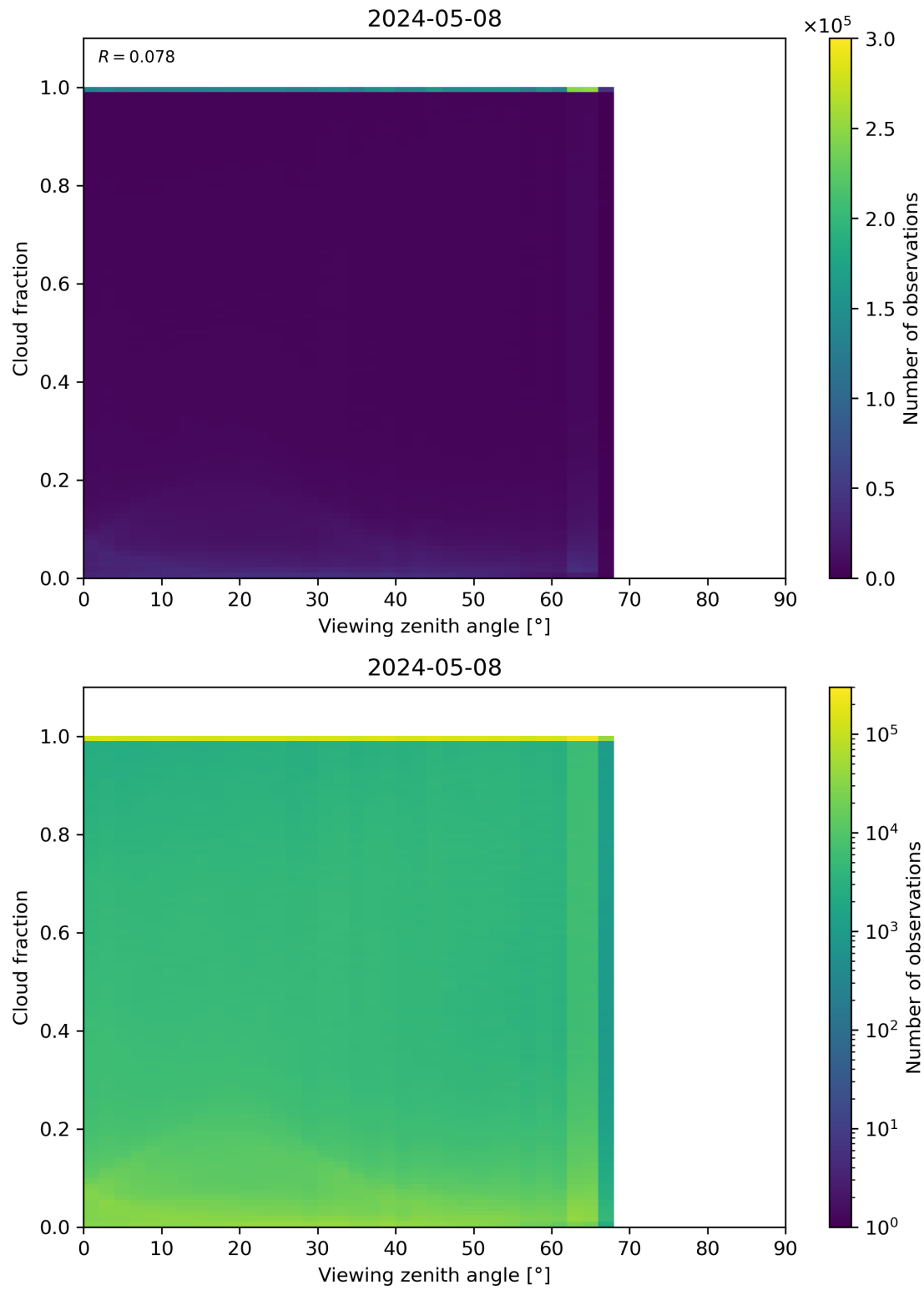
Figure 120: Scatter density plot of “Viewing zenith angle” against “Cloud fraction” for 2024-05-07 to 2024-05-09.
