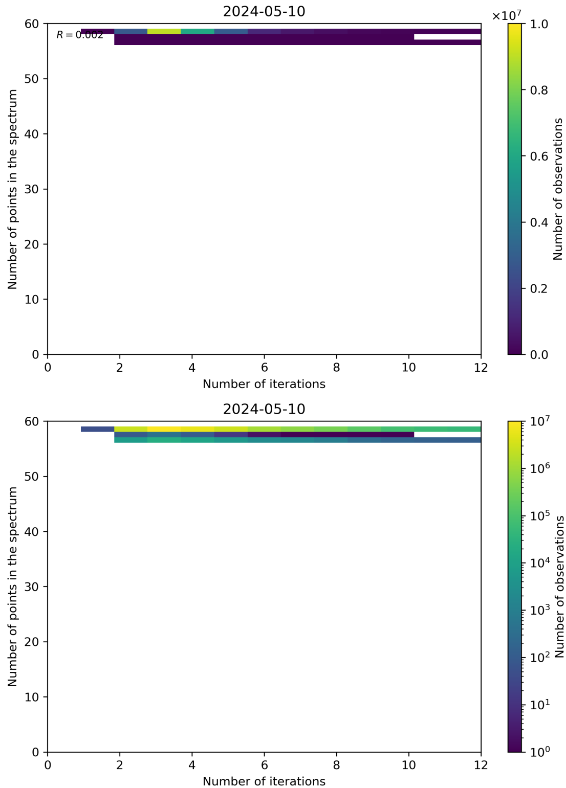
Figure 99: Scatter density plot of “Number of iterations” against “Number of points in the spectrum” for 2024-05-09 to 2024-05-11.
