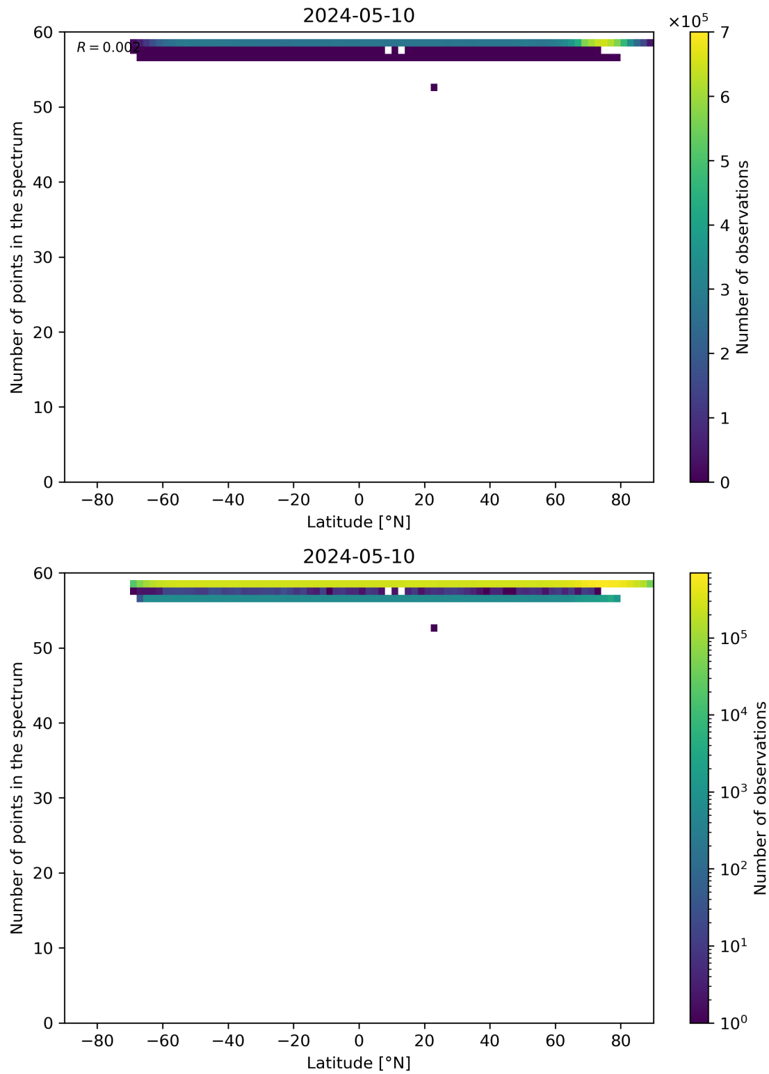
Figure 94: Scatter density plot of “Latitude” against “Number of points in the spectrum” for 2024-05-09 to 2024-05-11.
