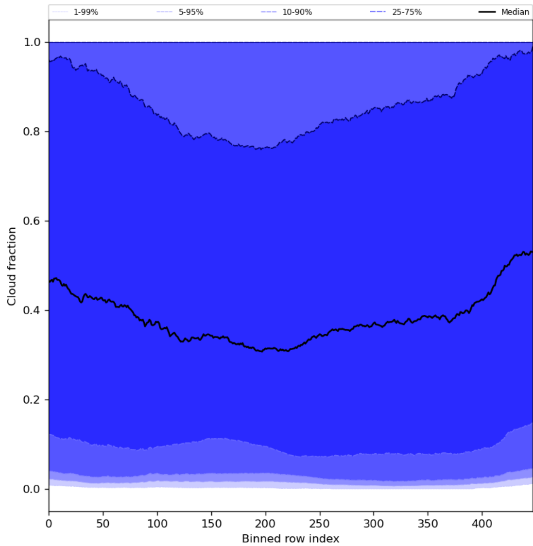
Figure 49: Along track statistics of “Cloud fraction” for 2024-05-09 to 2024-05-11
