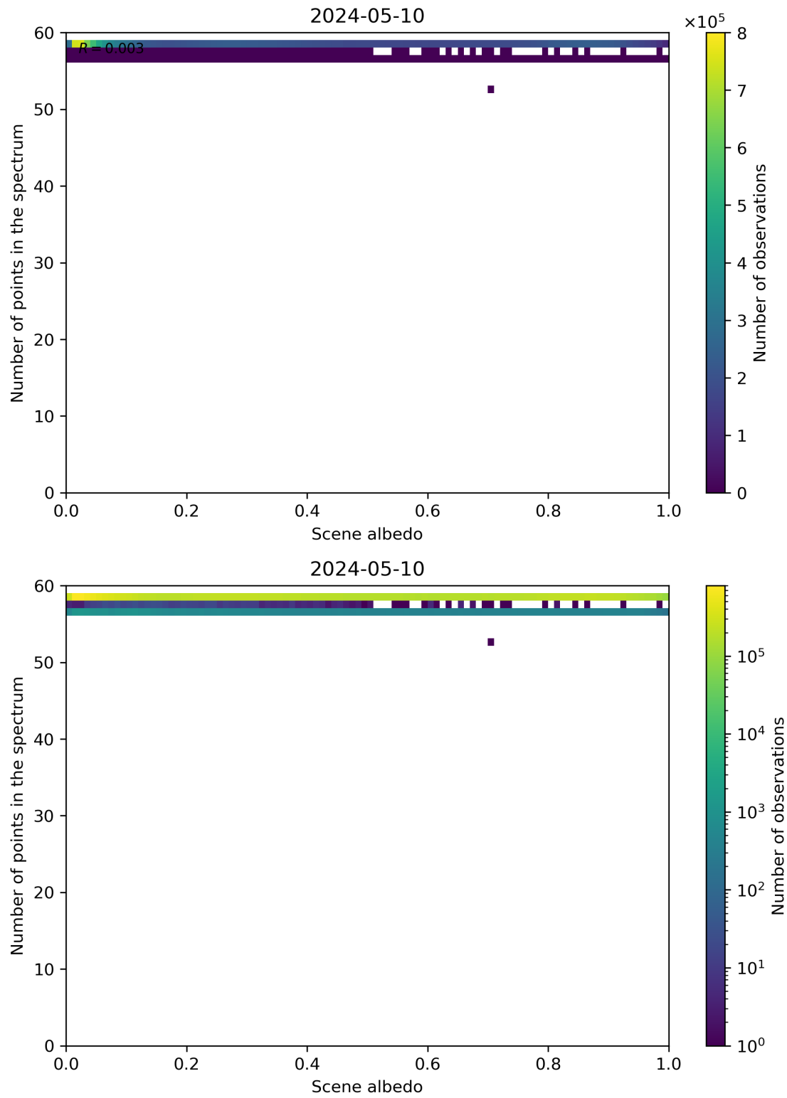
Figure 106: Scatter density plot of “Scene albedo” against “Number of points in the spectrum” for 2024-05-09 to 2024-05-11.
