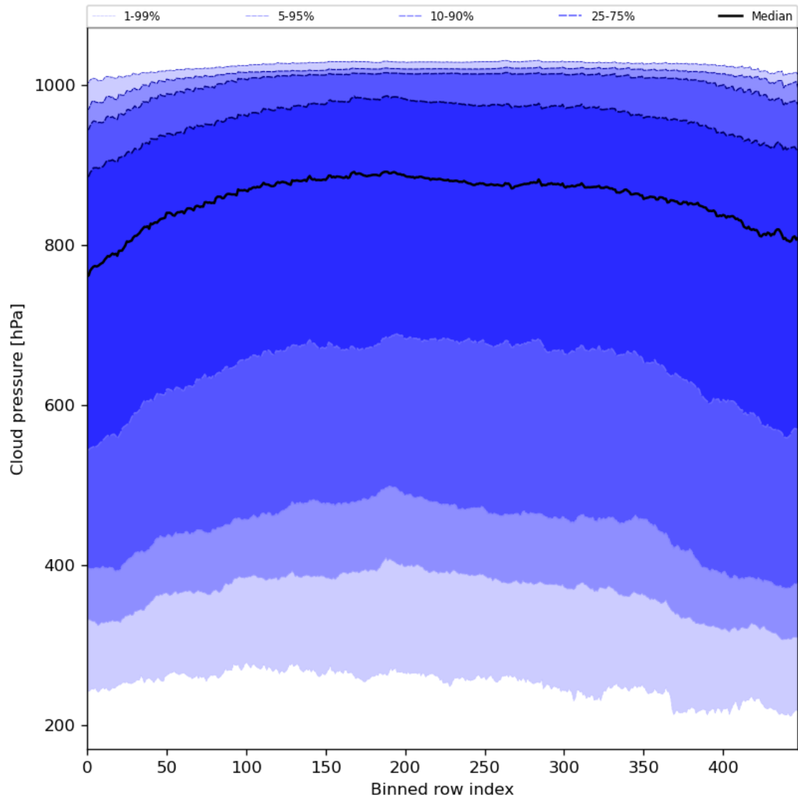
Figure 47: Along track statistics of “Cloud pressure” for 2024-05-09 to 2024-05-11
