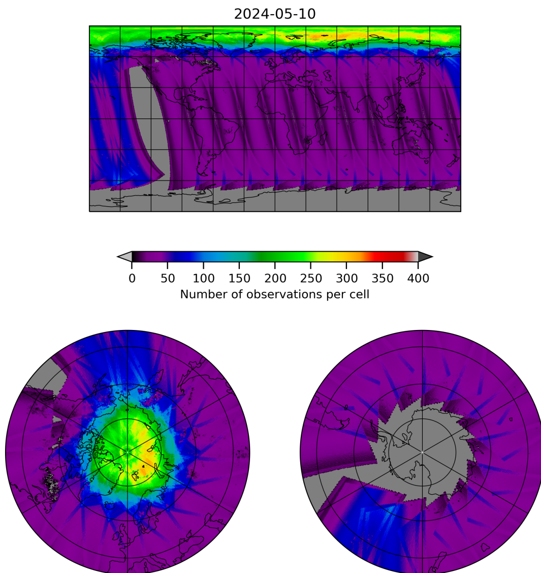
Figure 11: Map of the number of observations for 2024-05-09 to 2024-05-11
