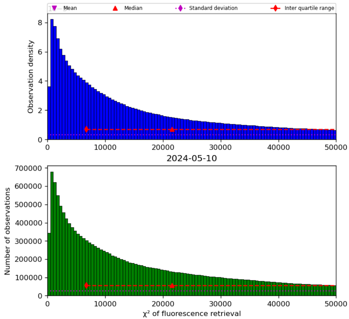
Figure 42: Histogram of “ \chi^2 of fluorescence retrieval” for 2024-05-09 to 2024-05-11
