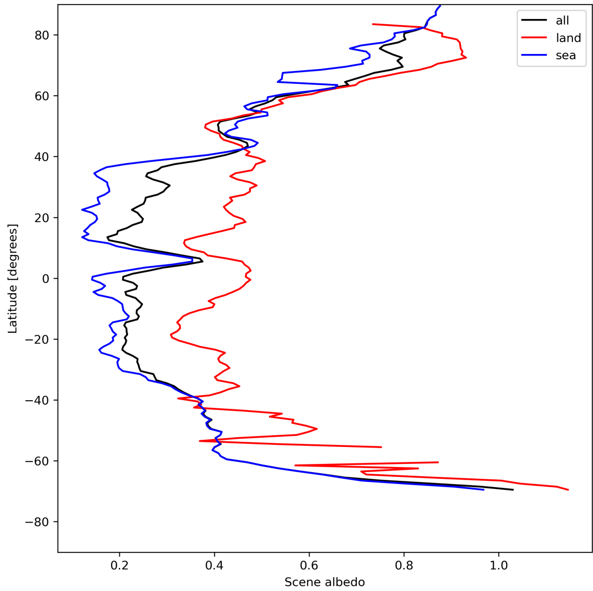
Figure 17: Zonal average of “Scene albedo” for 2024-05-09 to 2024-05-11.
