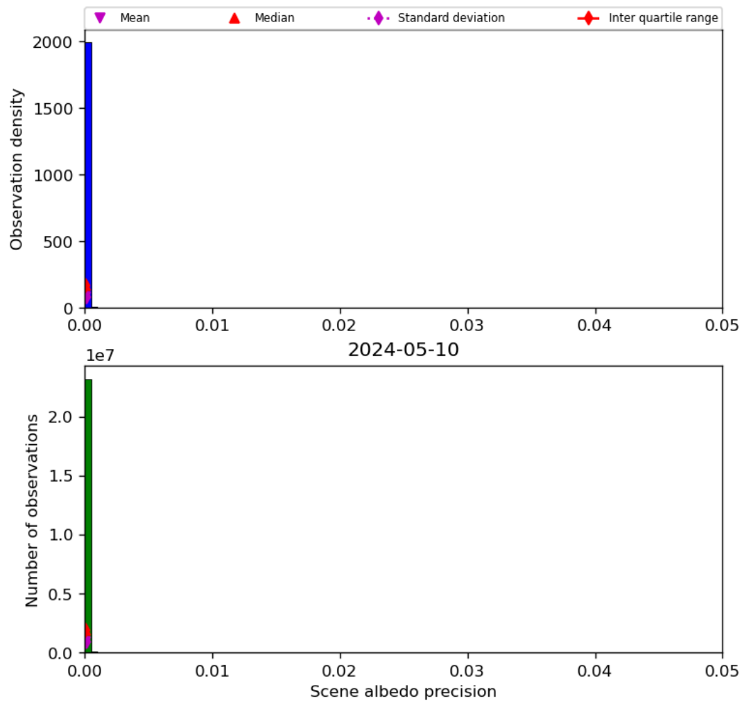
Figure 35: Histogram of “Scene albedo precision” for 2024-05-09 to 2024-05-11
