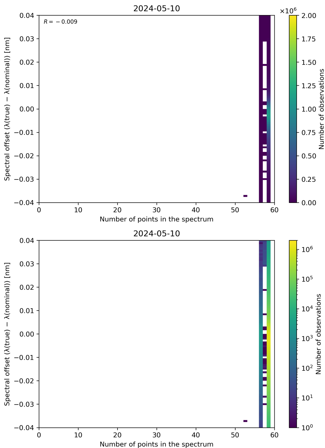
Figure 101: Scatter density plot of “Number of points in the spectrum” against “Spectral offset ( \lambda(\text{true}) - \lambda(\text{nominal}) )” for 2024-05-09 to 2024-05-11.
