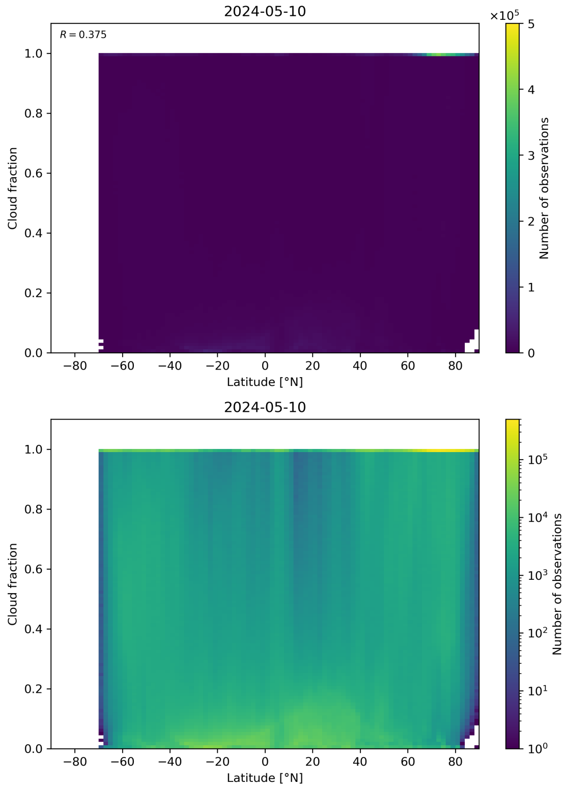
Figure 90: Scatter density plot of “Latitude” against “Cloud fraction” for 2024-05-09 to 2024-05-11.
