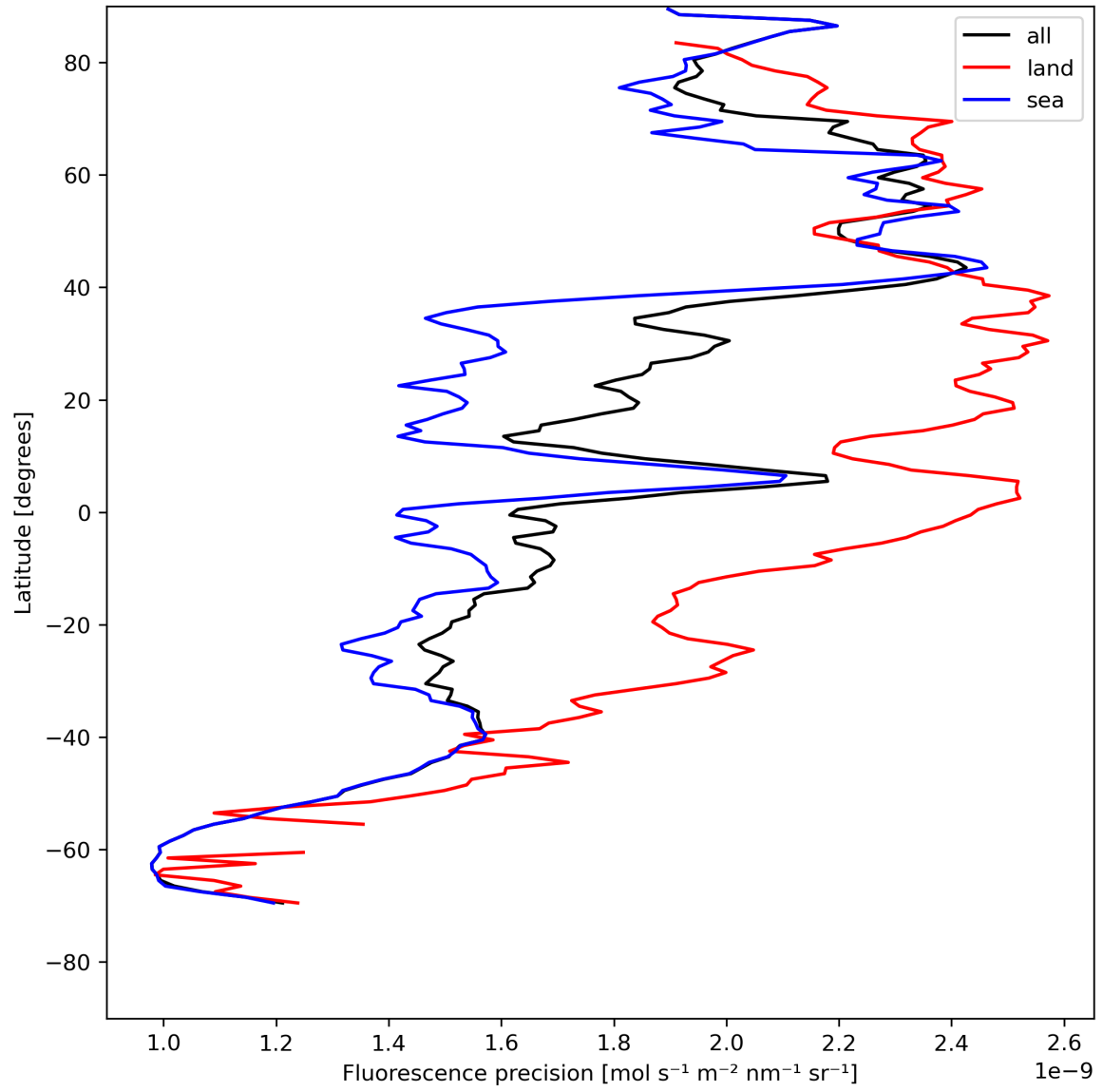
Figure 24: Zonal average of “Fluorescence precision” for 2024-05-09 to 2024-05-11.
