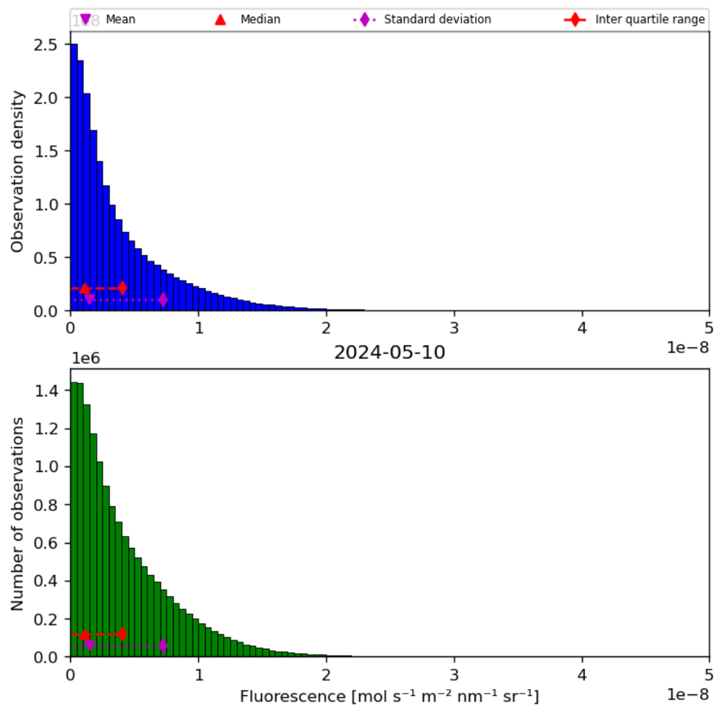
Figure 40: Histogram of “Fluorescence” for 2024-05-09 to 2024-05-11
