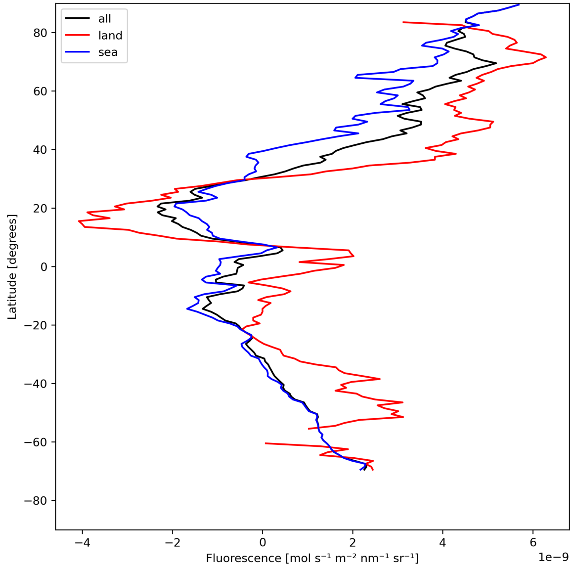
Figure 23: Zonal average of “Fluorescence” for 2024-05-09 to 2024-05-11.
