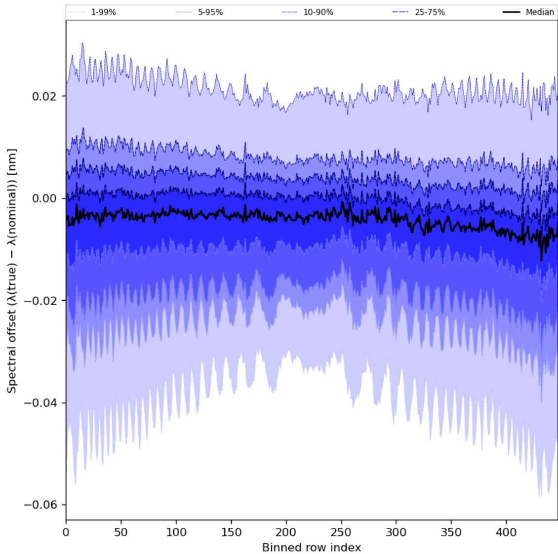
Figure 62: Along track statistics of “Spectral offset ( \lambda(\text{true}) - \lambda(\text{nominal}) )” for 2024-05-09 to 2024-05-11
