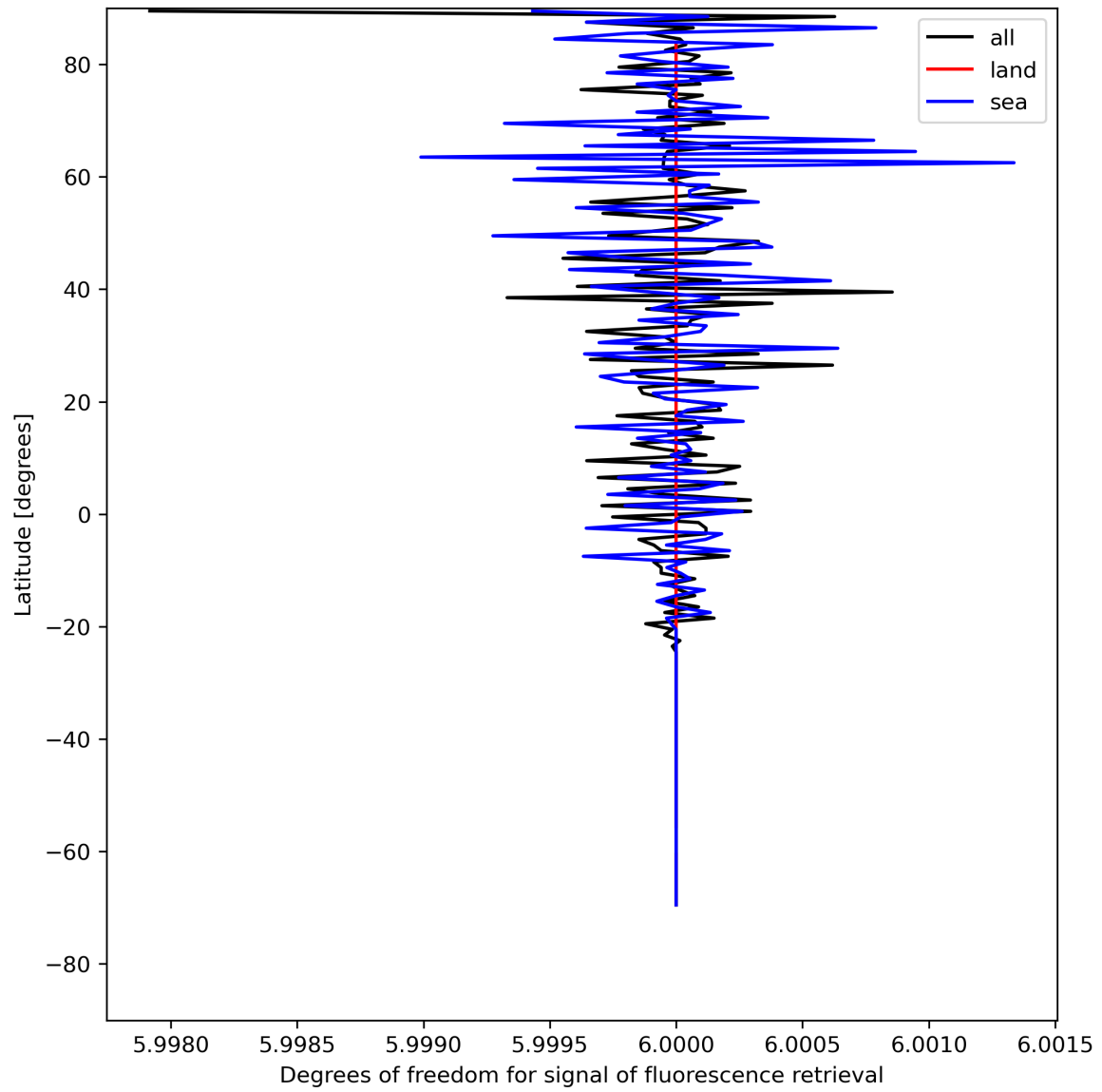
Figure 26: Zonal average of “Degrees of freedom for signal of fluorescence retrieval” for 2024-05-09 to 2024-05-11.
