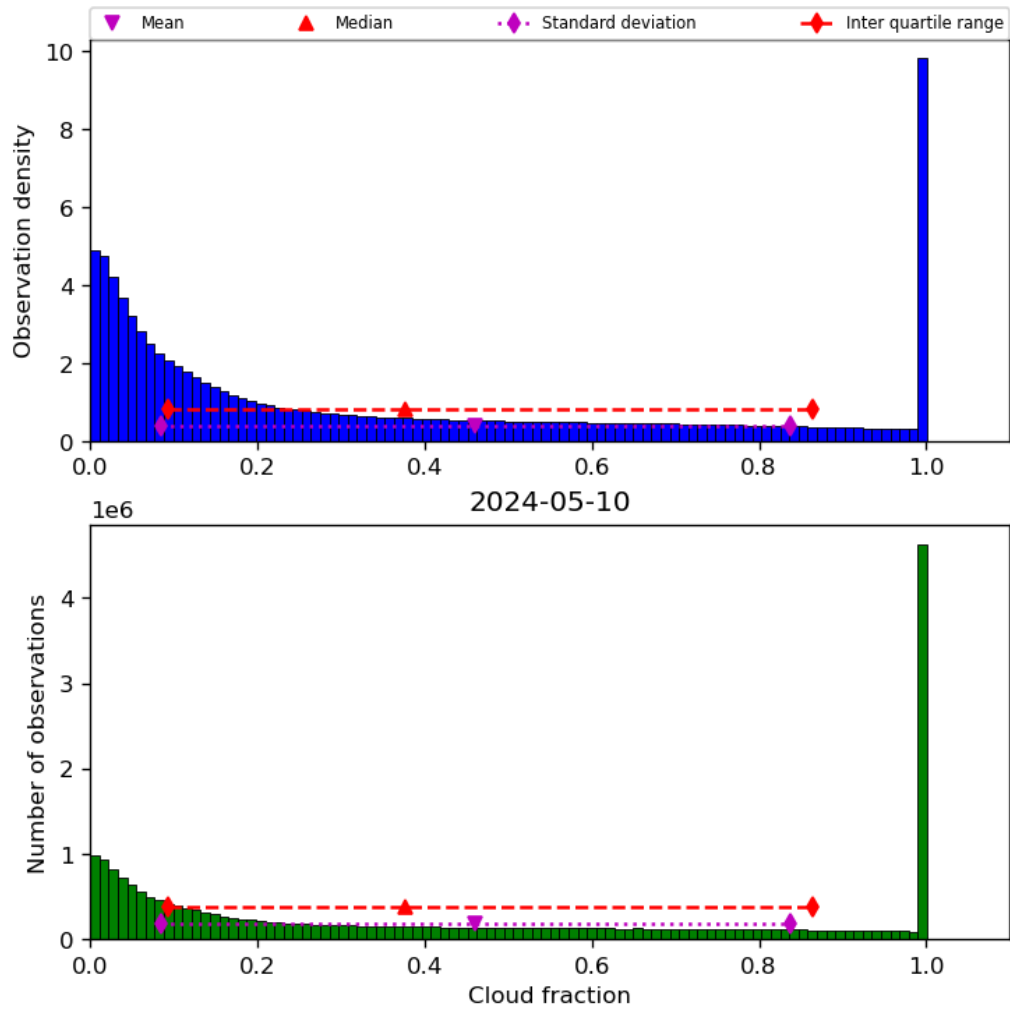
Figure 32: Histogram of “Cloud fraction” for 2024-05-09 to 2024-05-11
