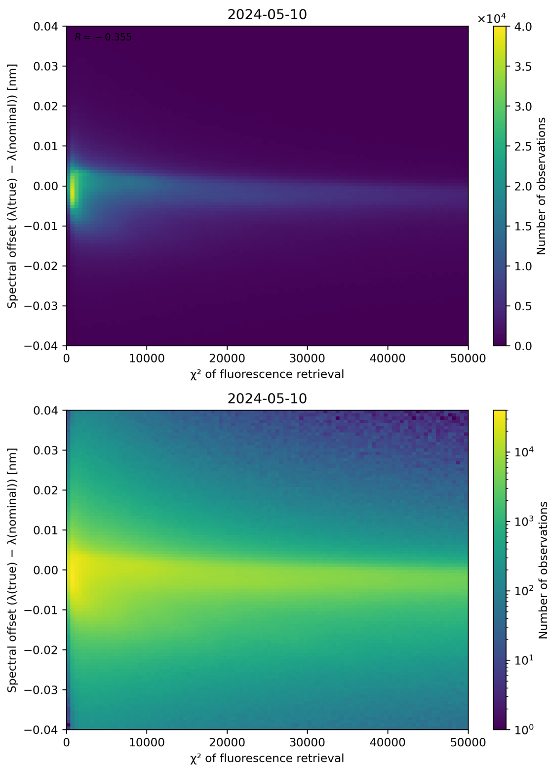
Figure 69: Scatter density plot of " \chi^2 of fluorescence retrieval" against "Spectral offset ( \lambda(\text{true}) - \lambda(\text{nominal})) " for 2024-05-09 to 2024-05-11.
