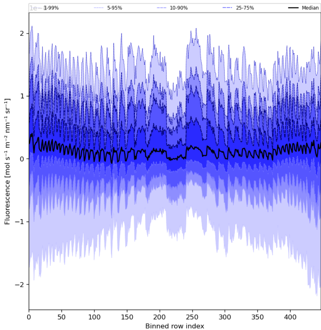
Figure 57: Along track statistics of “Fluorescence” for 2024-05-09 to 2024-05-11
