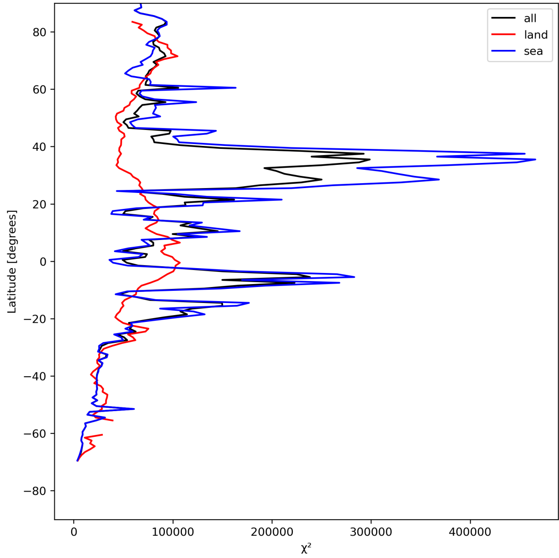
Figure 21: Zonal average of “ \chi^2 ” for 2024-05-09 to 2024-05-11.
