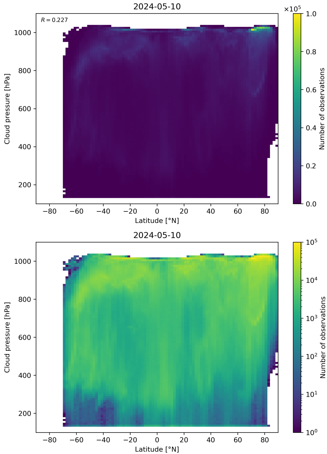
Figure 91: Scatter density plot of “Latitude” against “Cloud pressure” for 2024-05-09 to 2024-05-11.
