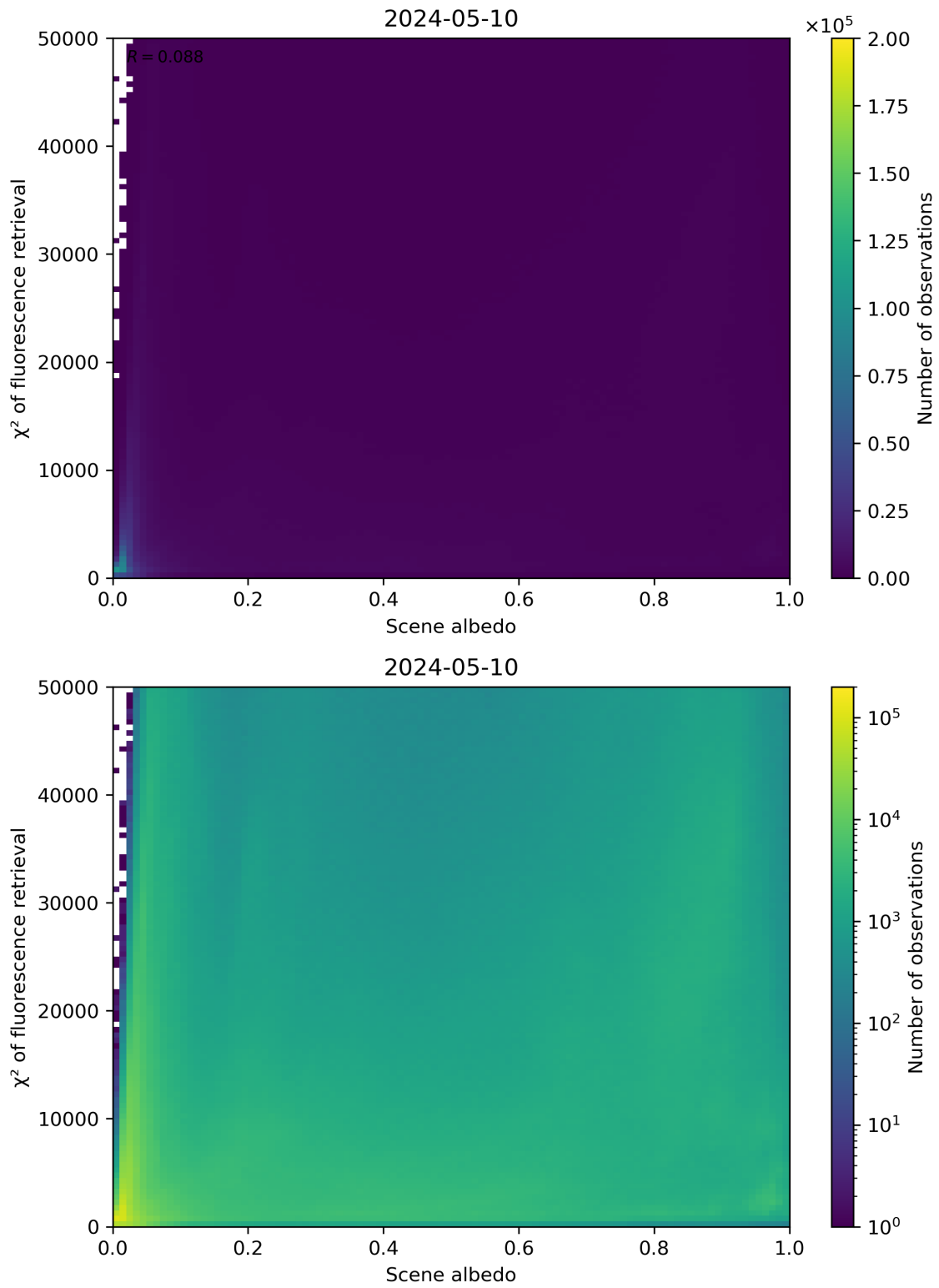
Figure 103: Scatter density plot of “Scene albedo” against “ \chi^2 of fluorescence retrieval” for 2024-05-09 to 2024-05-11.
