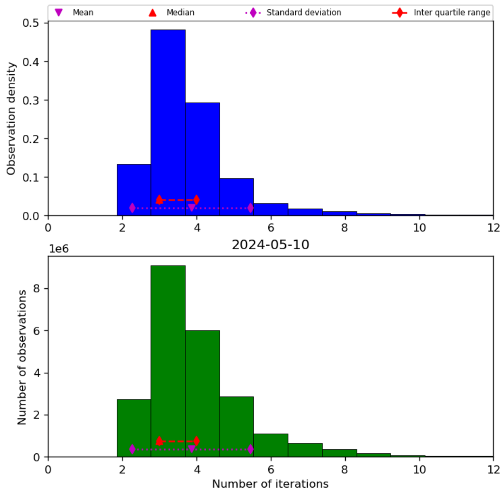
Figure 39: Histogram of “Number of iterations” for 2024-05-09 to 2024-05-11
