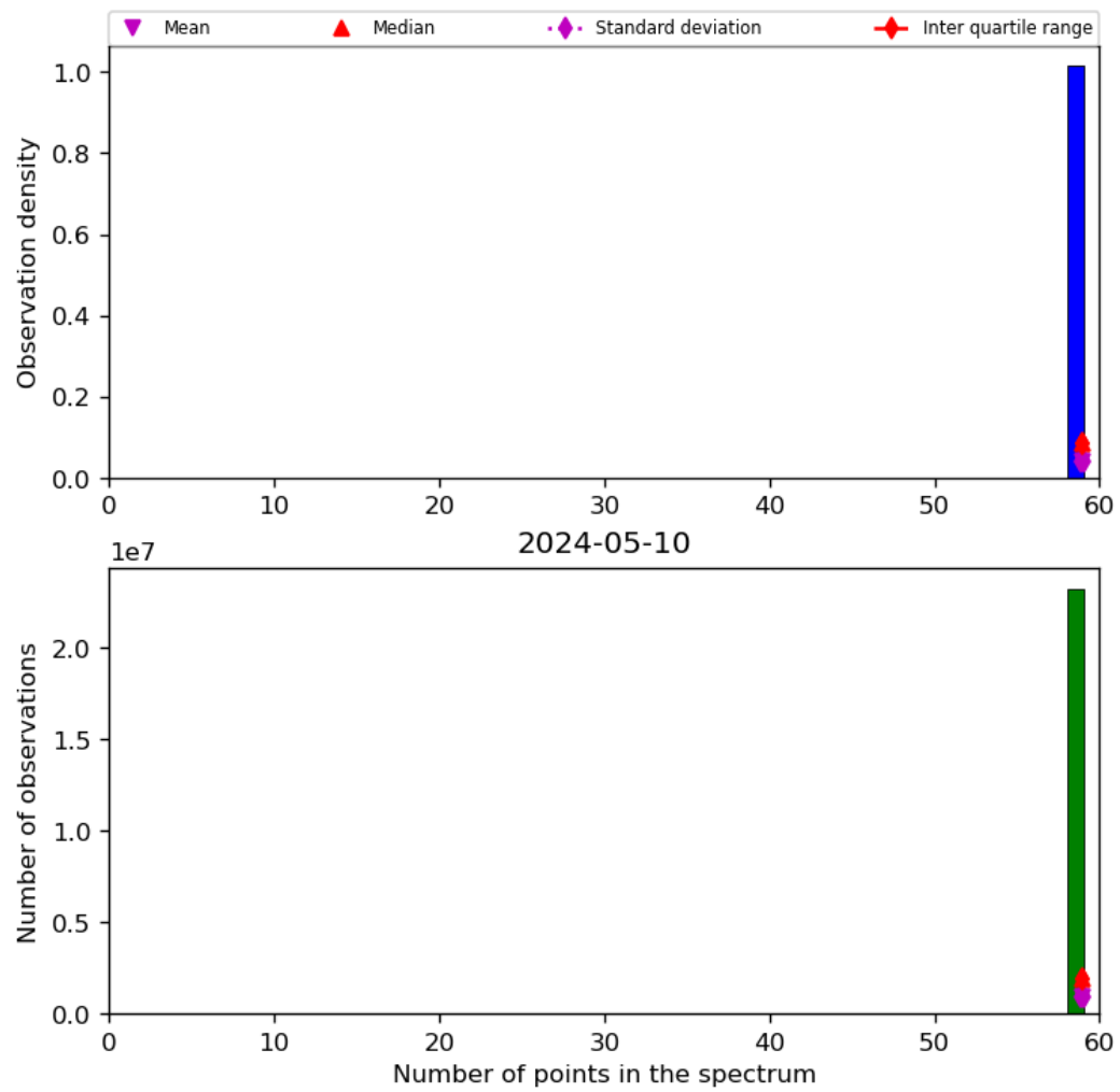
Figure 44: Histogram of "Number of points in the spectrum" for 2024-05-09 to 2024-05-11
