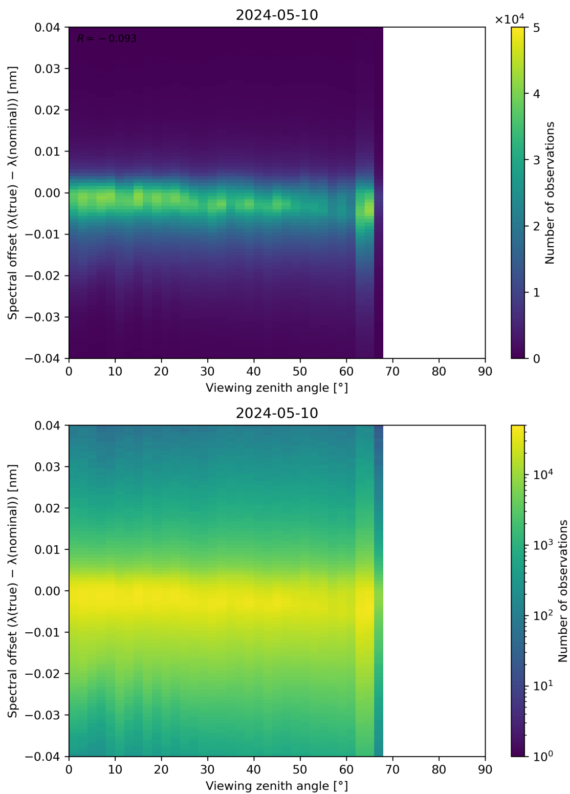
Figure 128: Scatter density plot of “Viewing zenith angle” against “Spectral offset ( \lambda(\text{true}) - \lambda(\text{nominal}) )” for 2024-05-09 to 2024-05-11.
