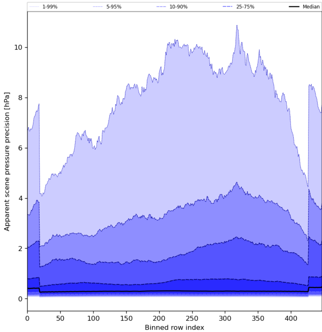
Figure 54: Along track statistics of “Apparent scene pressure precision” for 2024-05-09 to 2024-05-11
