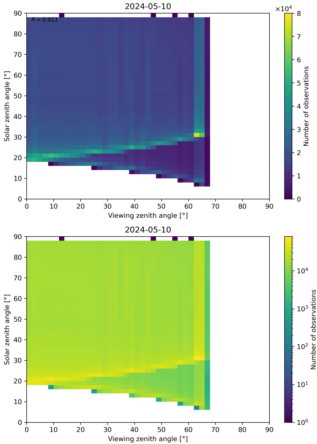
Figure 127: Scatter density plot of “Viewing zenith angle” against “Solar zenith angle” for 2024-05-09 to 2024-05-11.
