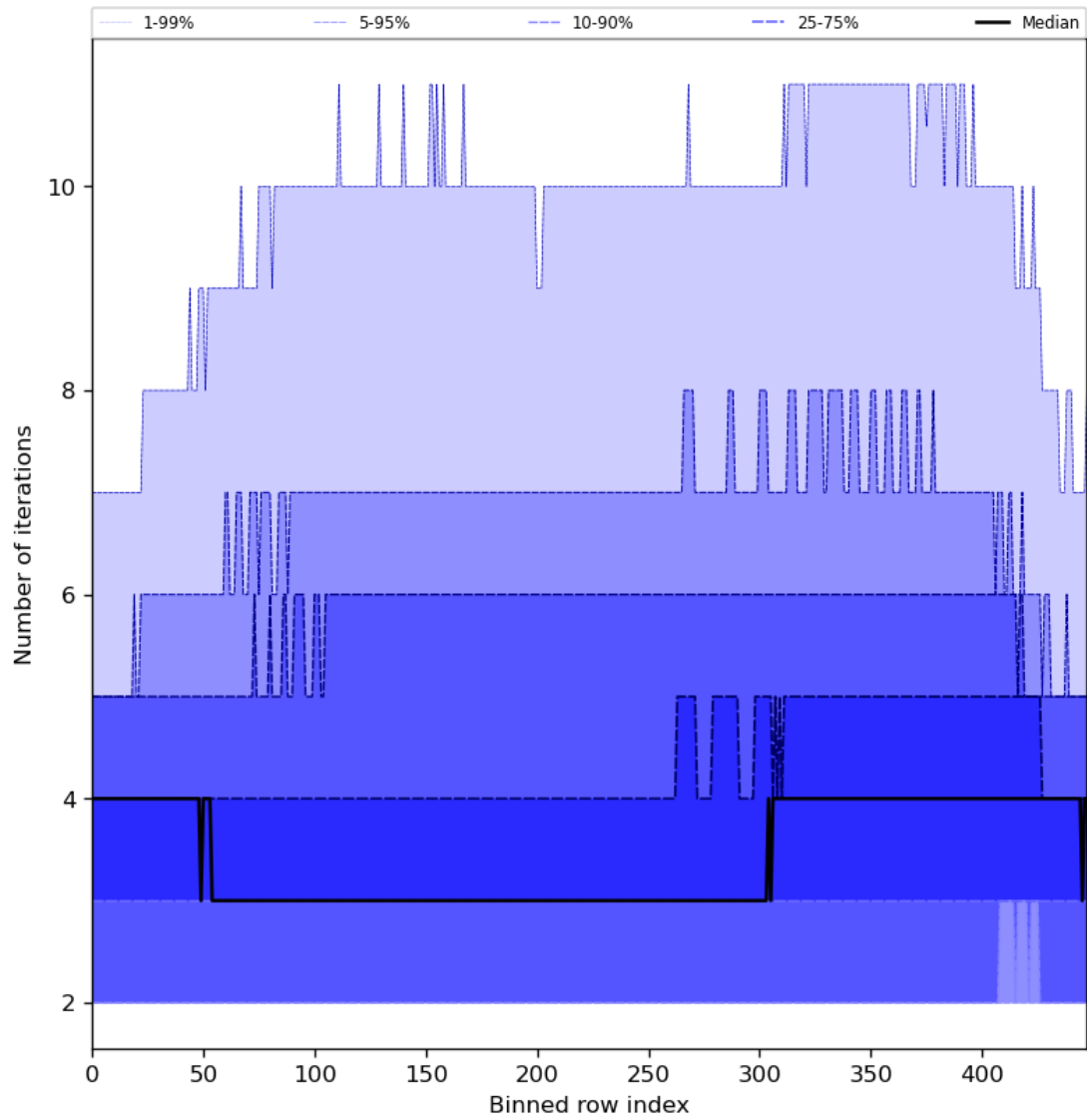
Figure 56: Along track statistics of “Number of iterations” for 2024-05-09 to 2024-05-11
