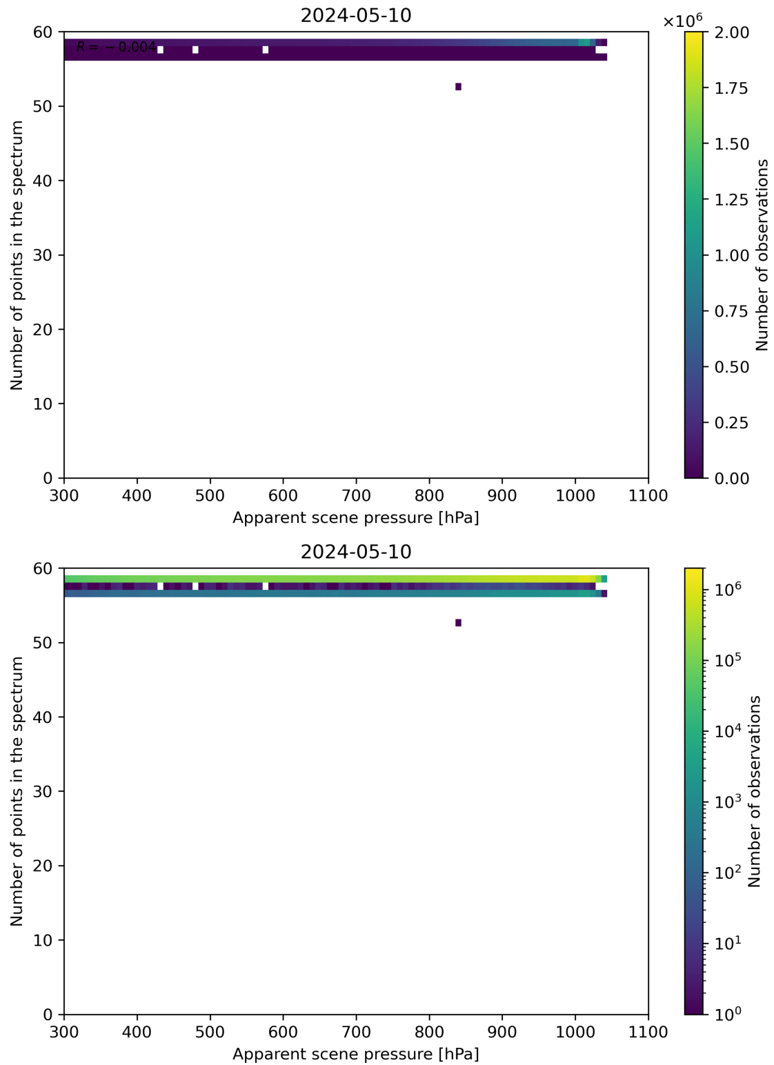
Figure 66: Scatter density plot of “Apparent scene pressure” against “Number of points in the spectrum” for 2024-05-09 to 2024-05-11.
