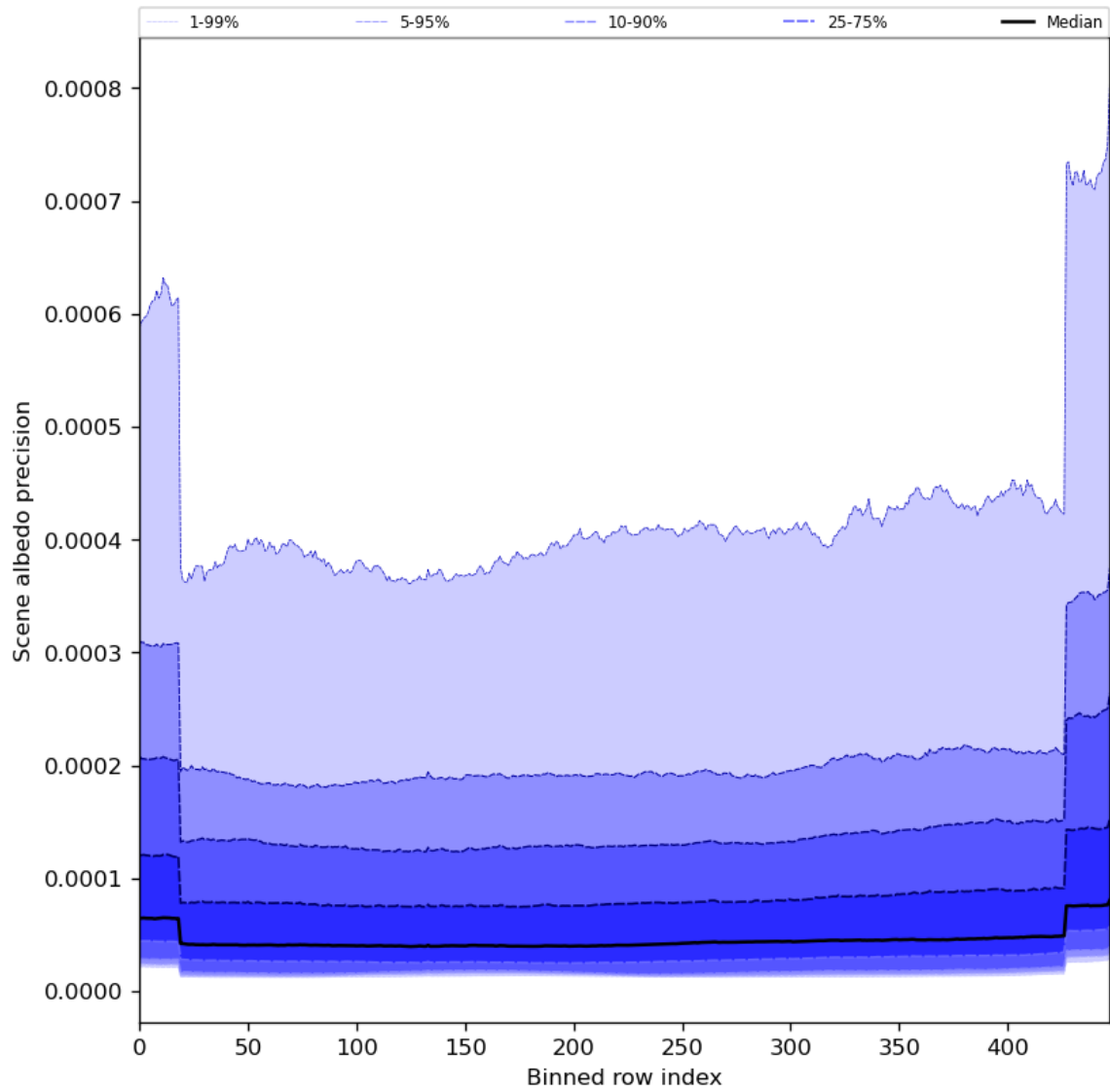
Figure 52: Along track statistics of “Scene albedo precision” for 2024-05-09 to 2024-05-11
