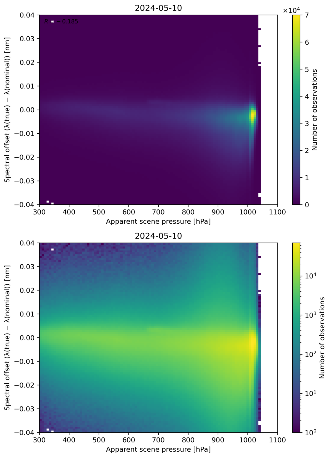
Figure 67: Scatter density plot of “Apparent scene pressure” against “Spectral offset ( \lambda(\text{true}) - \lambda(\text{nominal}) )” for 2024-05-09 to 2024-05-11.
