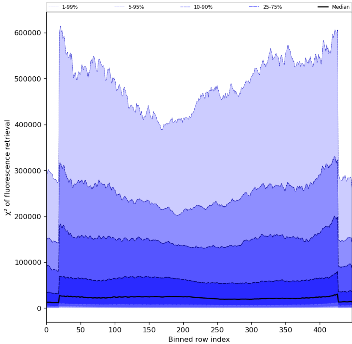
Figure 59: Along track statistics of “ \chi^2 of fluorescence retrieval” for 2024-05-09 to 2024-05-11
