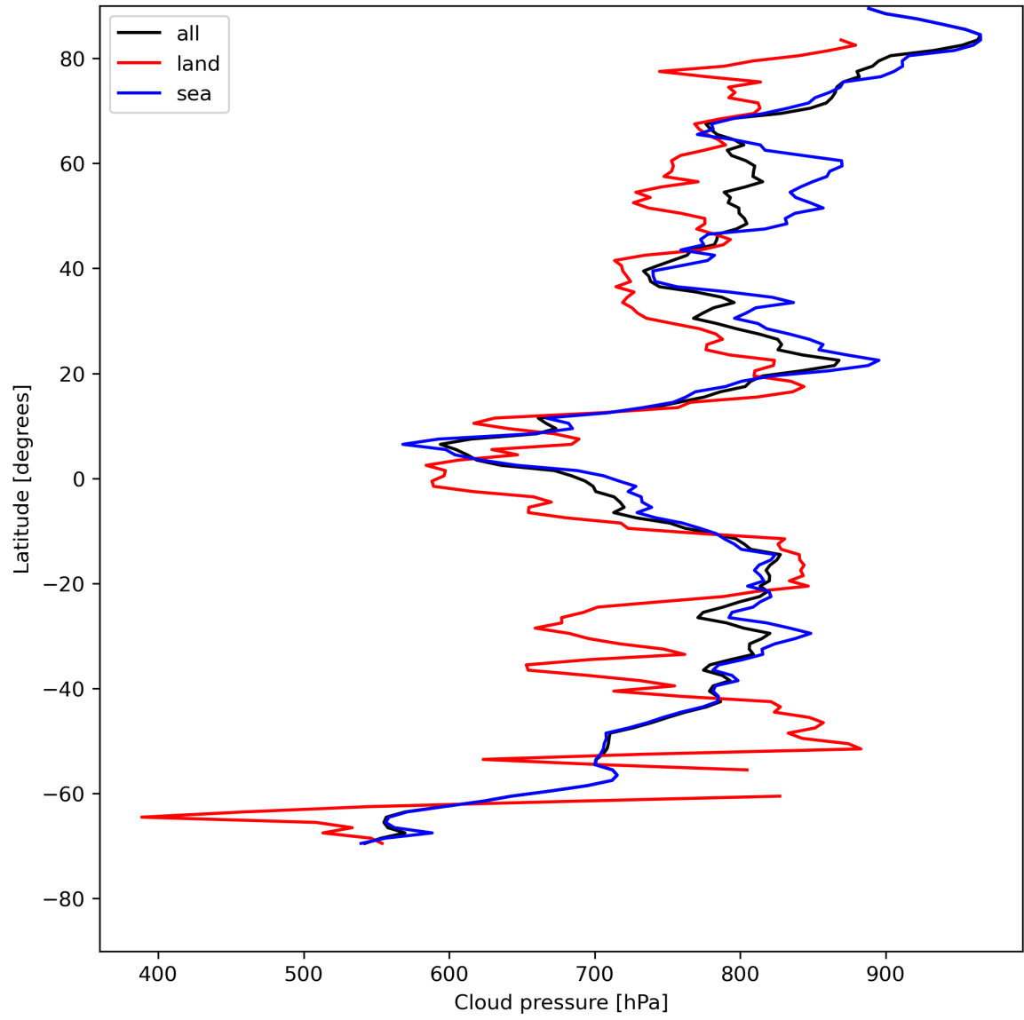
Figure 13: Zonal average of “Cloud pressure” for 2024-05-09 to 2024-05-11.
