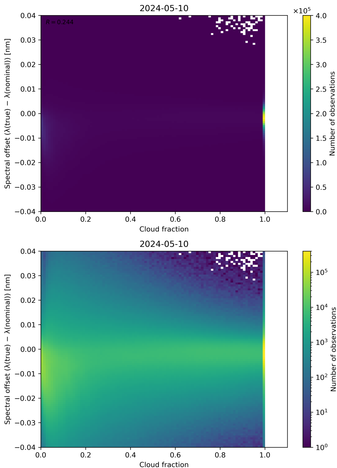
Figure 76: Scatter density plot of “Cloud fraction” against “Spectral offset ( \lambda(\text{true}) - \lambda(\text{nominal}) )” for 2024-05-09 to 2024-05-11.
