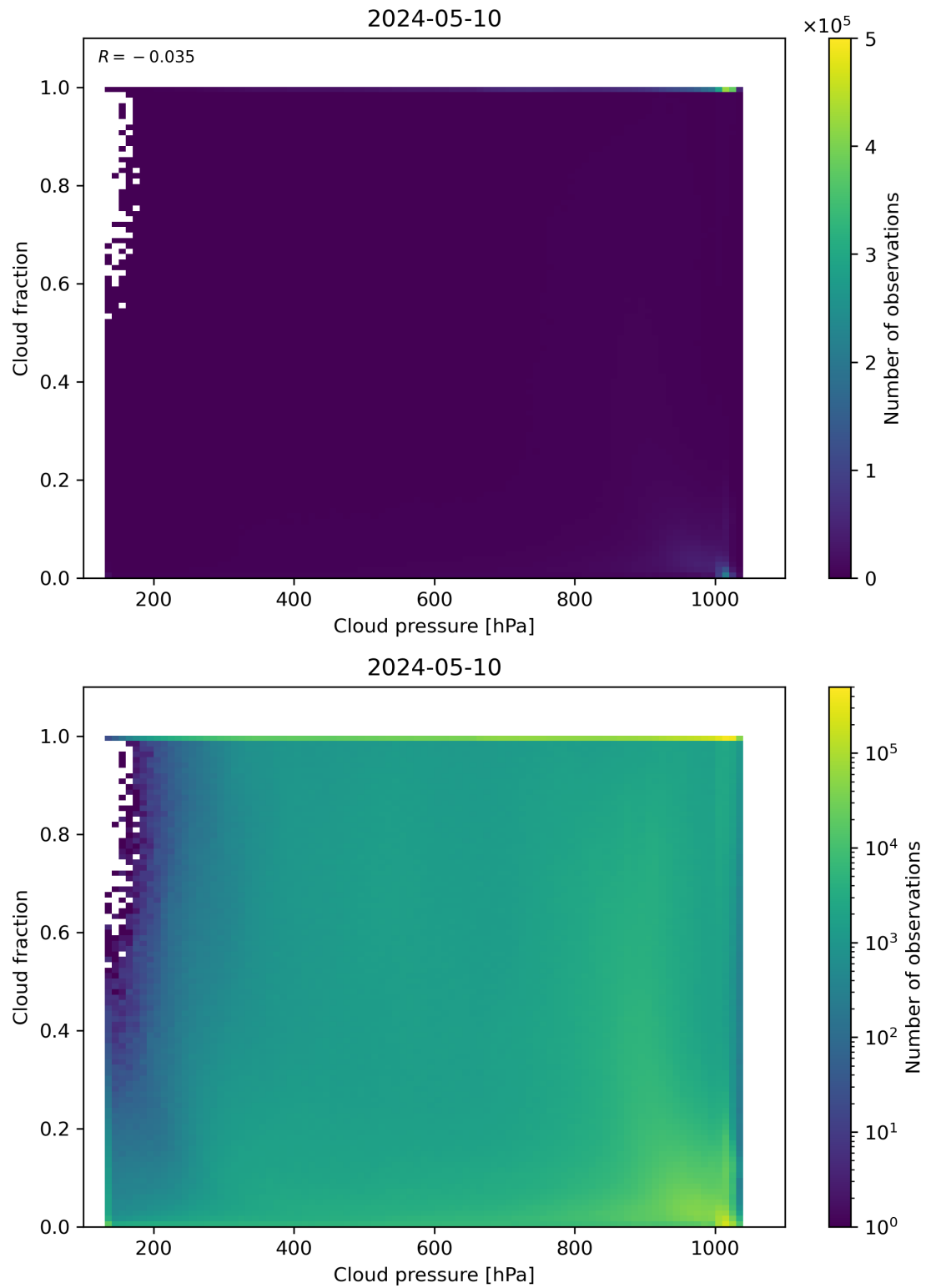
Figure 79: Scatter density plot of “Cloud pressure” against “Cloud fraction” for 2024-05-09 to 2024-05-11.
