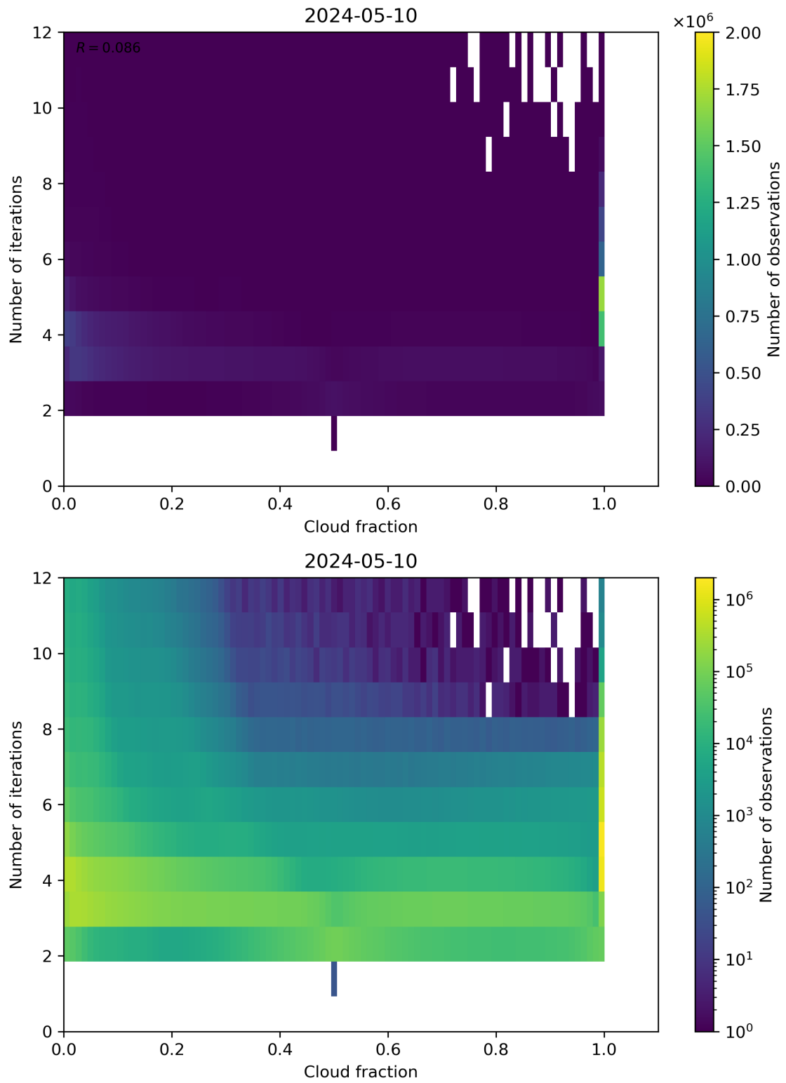
Figure 73: Scatter density plot of “Cloud fraction” against “Number of iterations” for 2024-05-09 to 2024-05-11.
