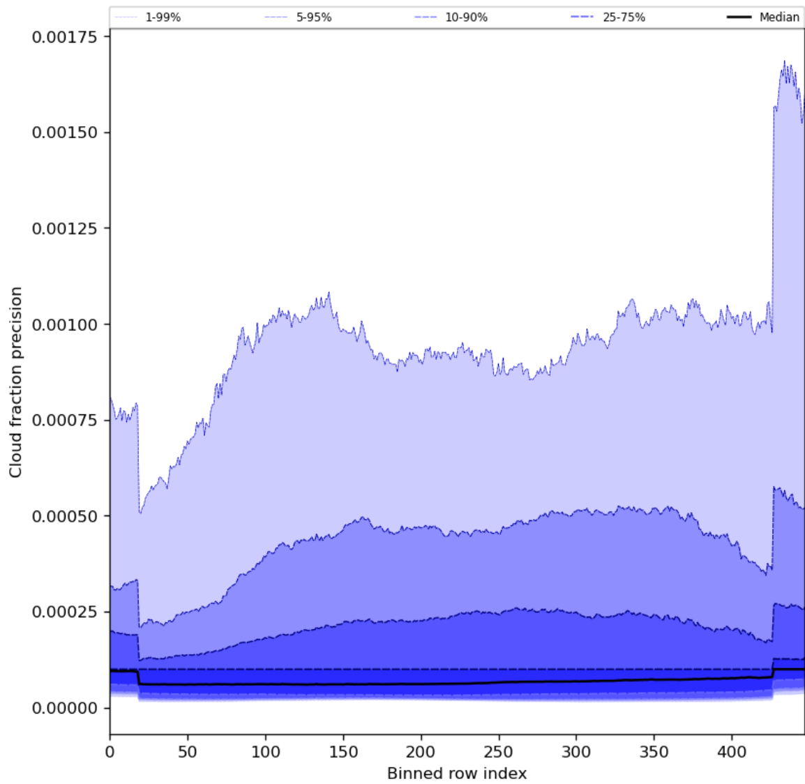
Figure 50: Along track statistics of “Cloud fraction precision” for 2024-05-09 to 2024-05-11
