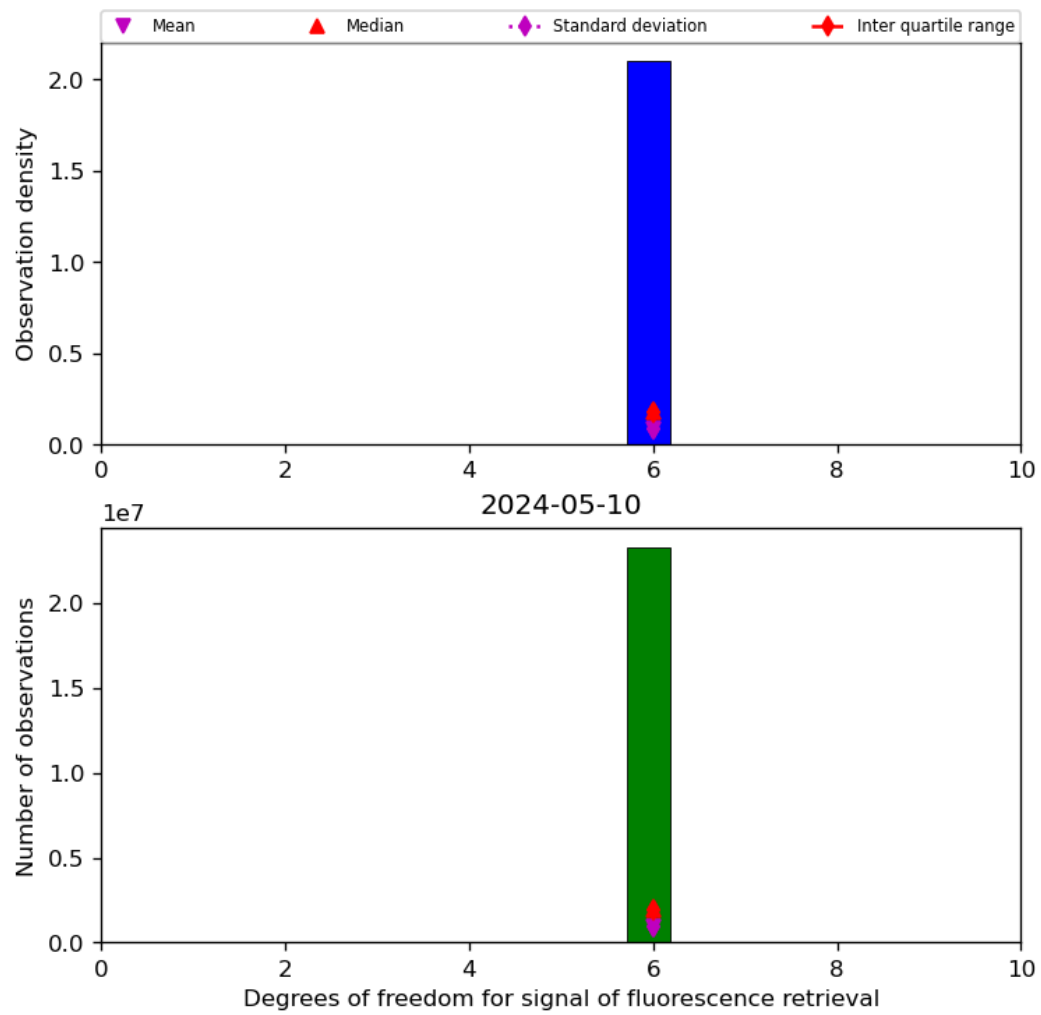
Figure 43: Histogram of “Degrees of freedom for signal of fluorescence retrieval” for 2024-05-09 to 2024-05-11
