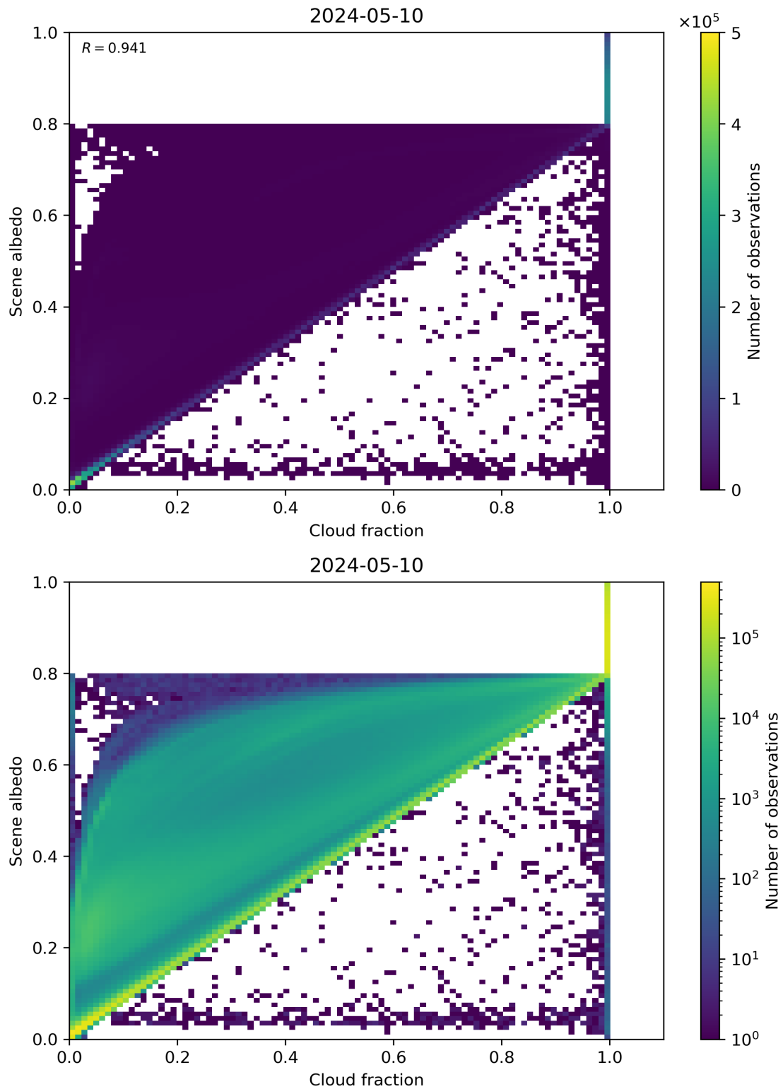
Figure 75: Scatter density plot of “Cloud fraction” against “Scene albedo” for 2024-05-09 to 2024-05-11.
