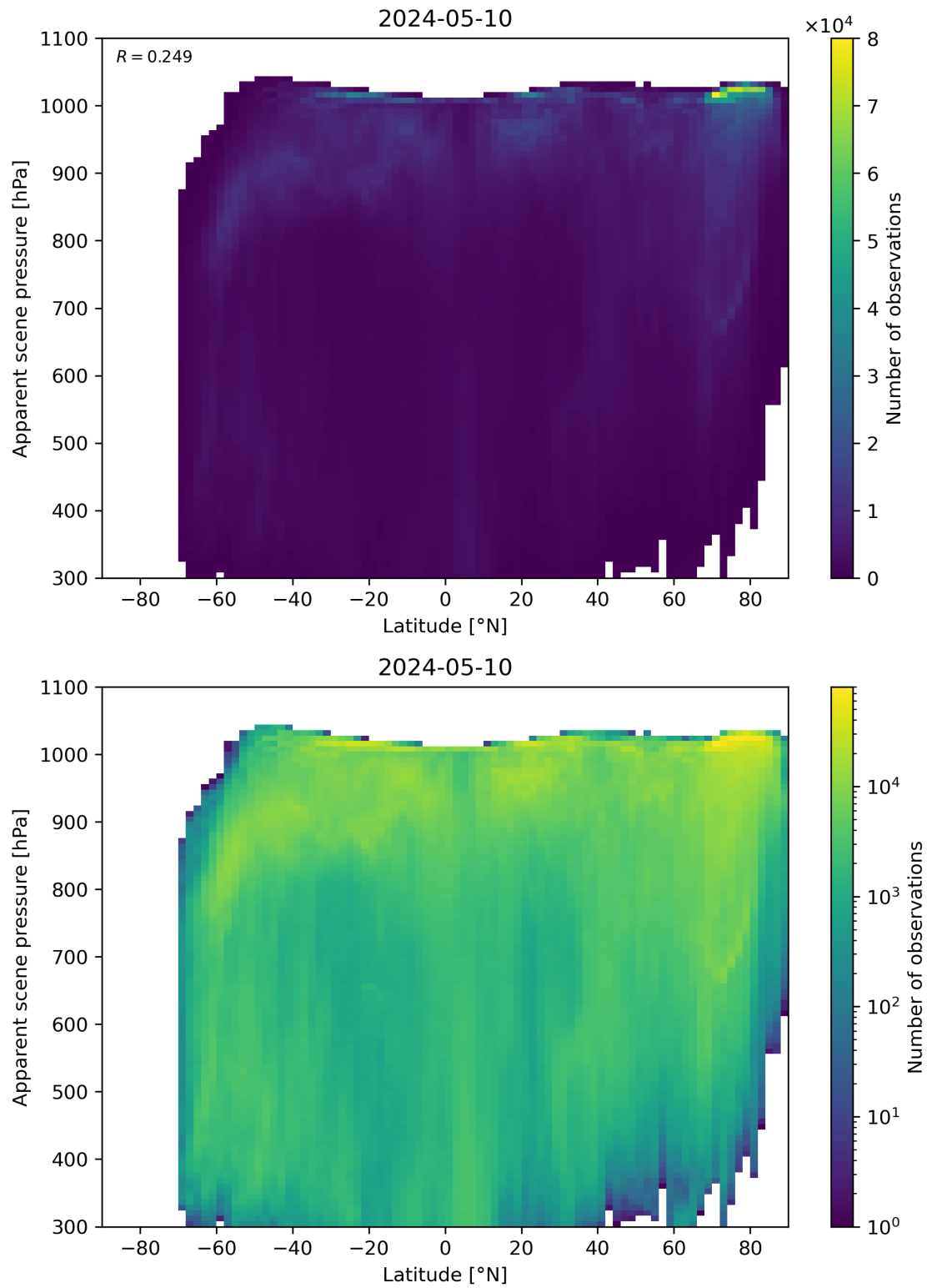
Figure 88: Scatter density plot of “Latitude” against “Apparent scene pressure” for 2024-05-09 to 2024-05-11.
