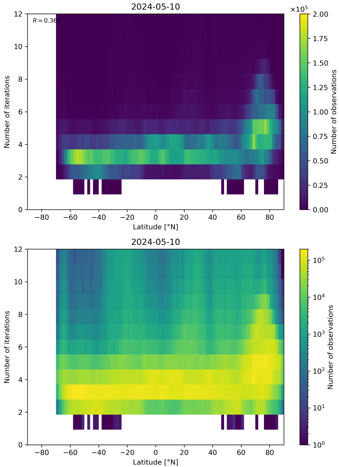
Figure 93: Scatter density plot of “Latitude” against “Number of iterations” for 2024-05-09 to 2024-05-11.
