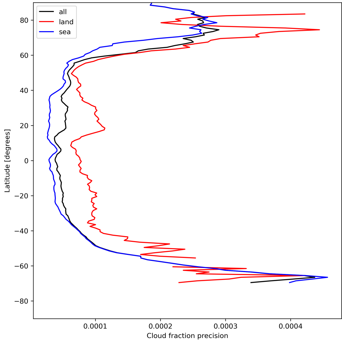
Figure 16: Zonal average of “Cloud fraction precision” for 2024-05-09 to 2024-05-11.
