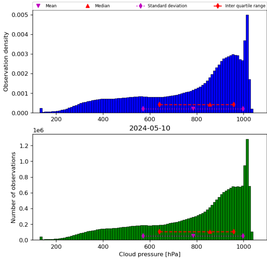
Figure 30: Histogram of “Cloud pressure” for 2024-05-09 to 2024-05-11
