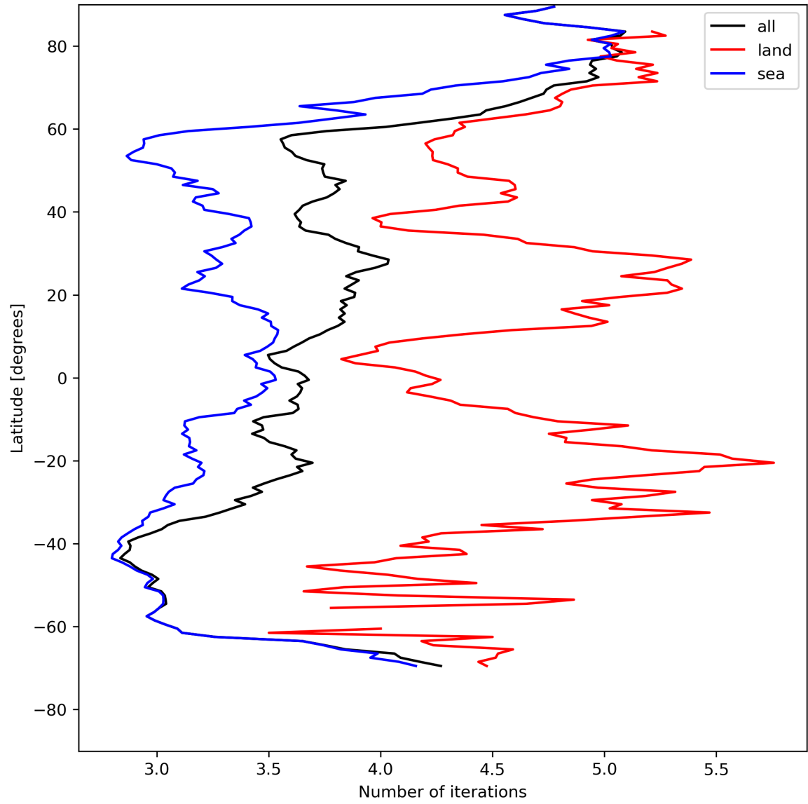
Figure 22: Zonal average of “Number of iterations” for 2024-05-09 to 2024-05-11.
