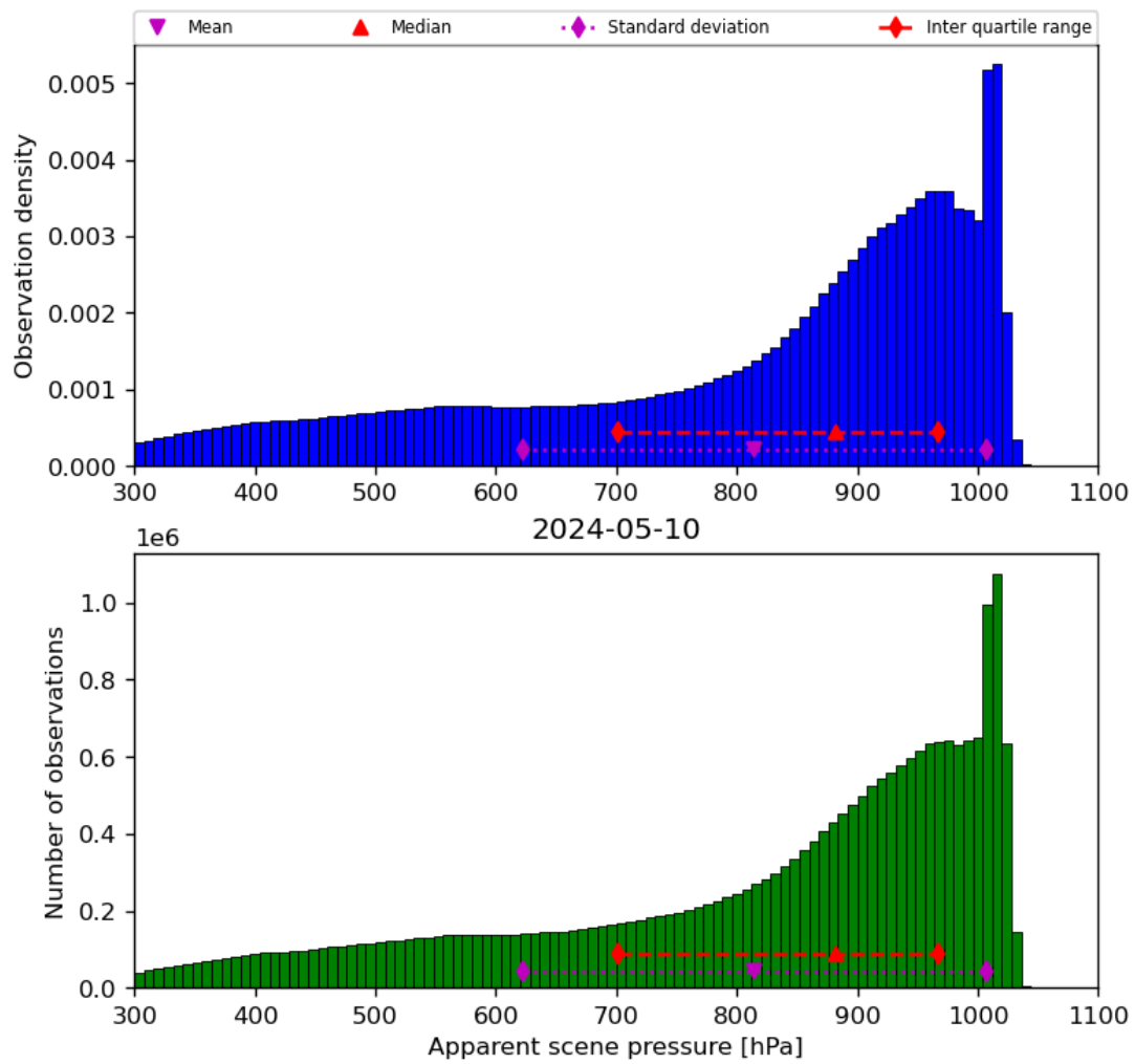
Figure 36: Histogram of “Apparent scene pressure” for 2024-05-09 to 2024-05-11
