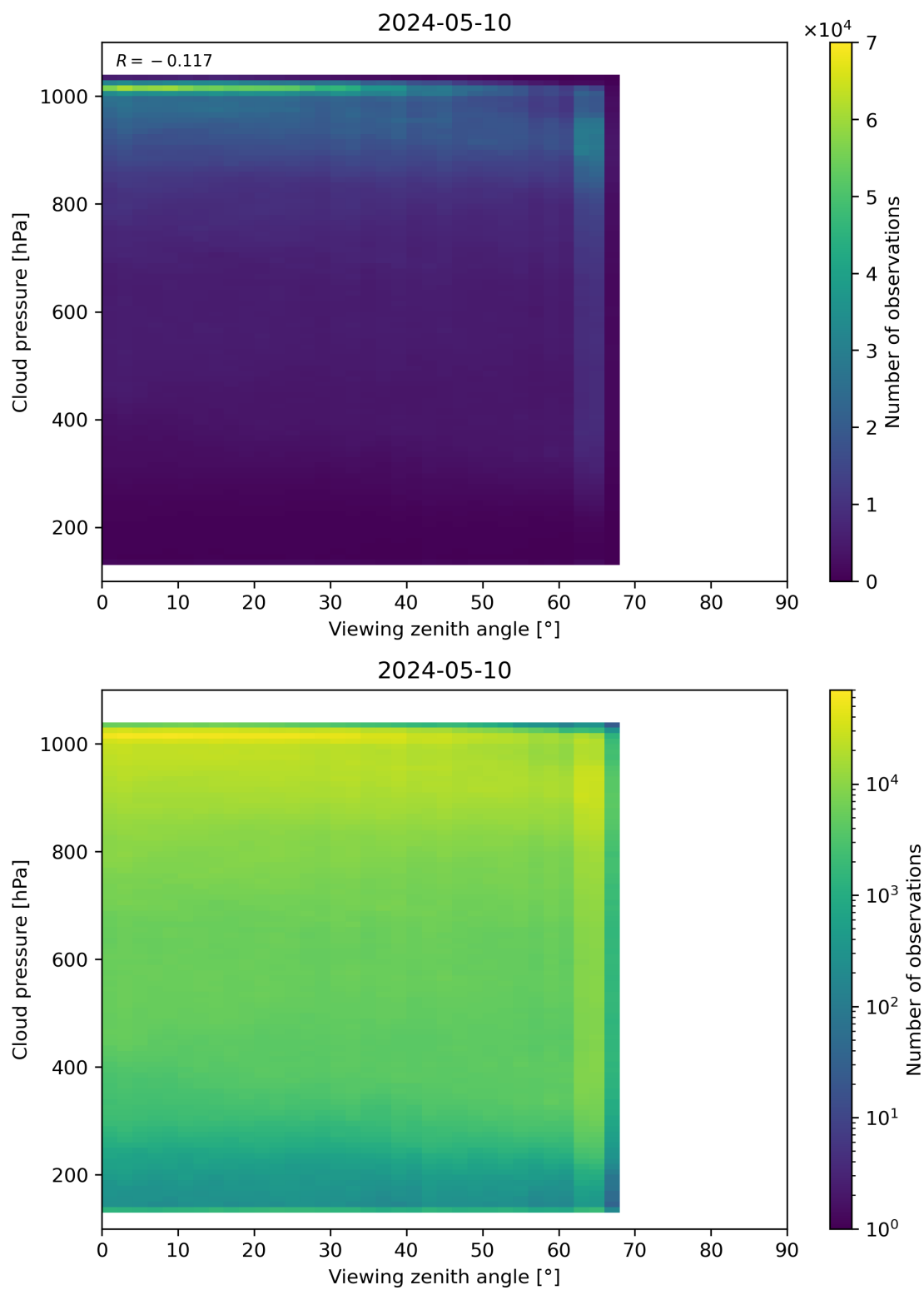
Figure 121: Scatter density plot of “Viewing zenith angle” against “Cloud pressure” for 2024-05-09 to 2024-05-11.
