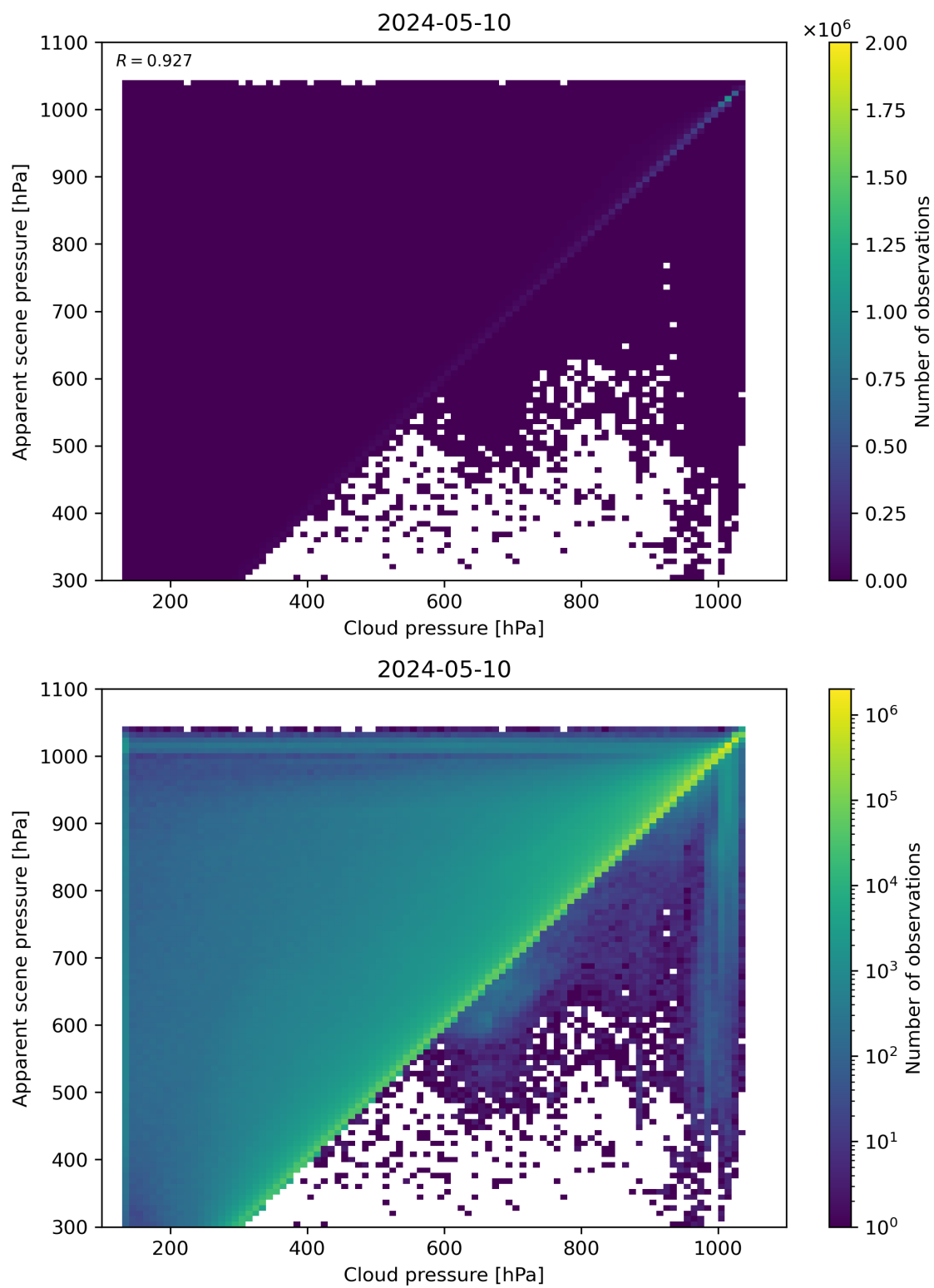
Figure 77: Scatter density plot of “Cloud pressure” against “Apparent scene pressure” for 2024-05-09 to 2024-05-11.
