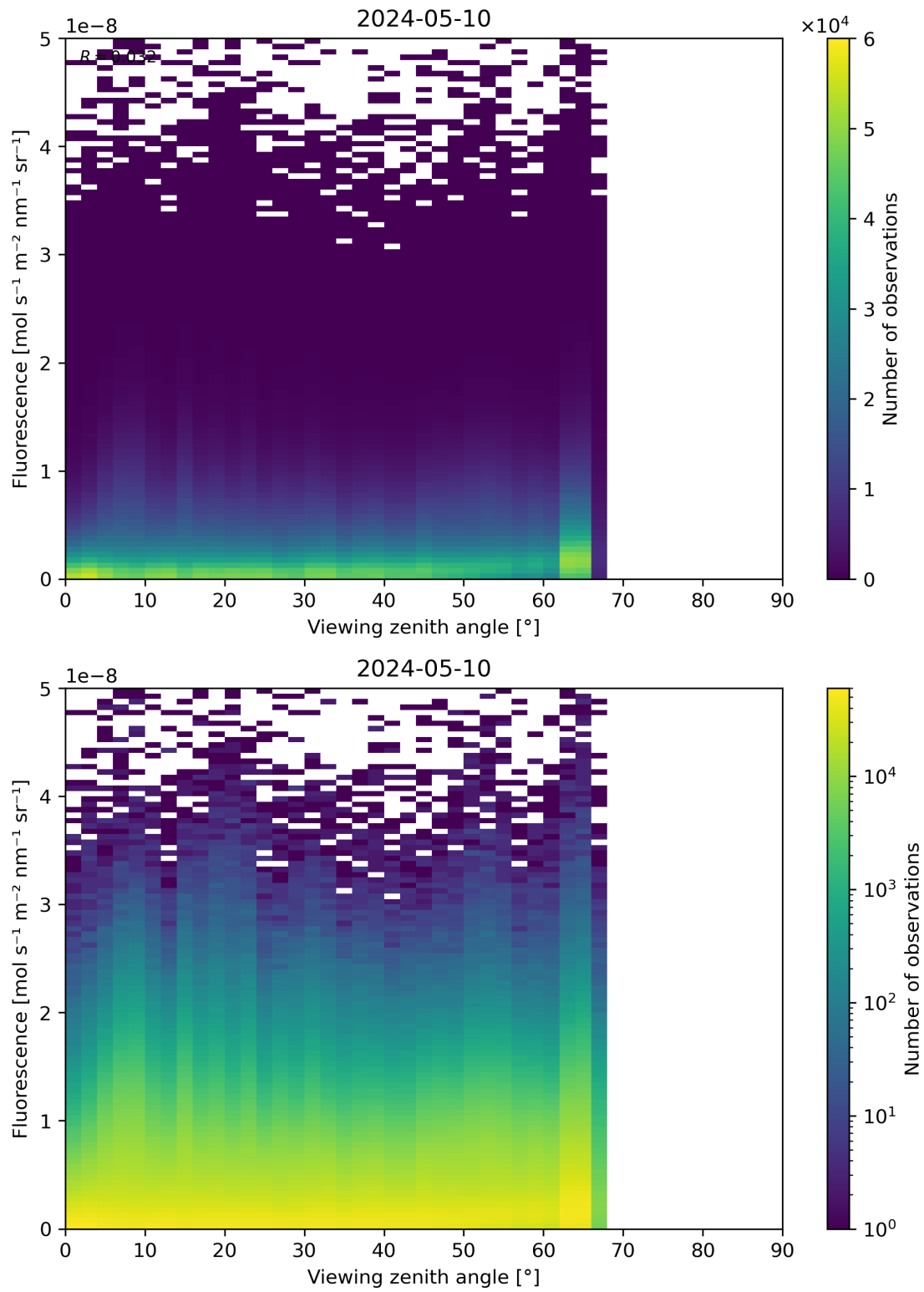
Figure 122: Scatter density plot of “Viewing zenith angle” against “Fluorescence” for 2024-05-09 to 2024-05-11.
