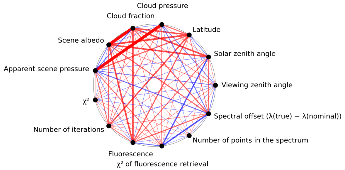
Figure 1: Map of correlation graph for 2024-05-09 to 2024-05-11.
