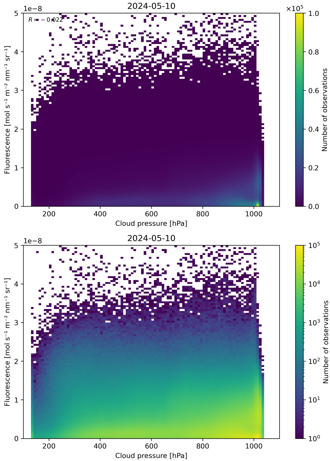
Figure 80: Scatter density plot of “Cloud pressure” against “Fluorescence” for 2024-05-09 to 2024-05-11.
