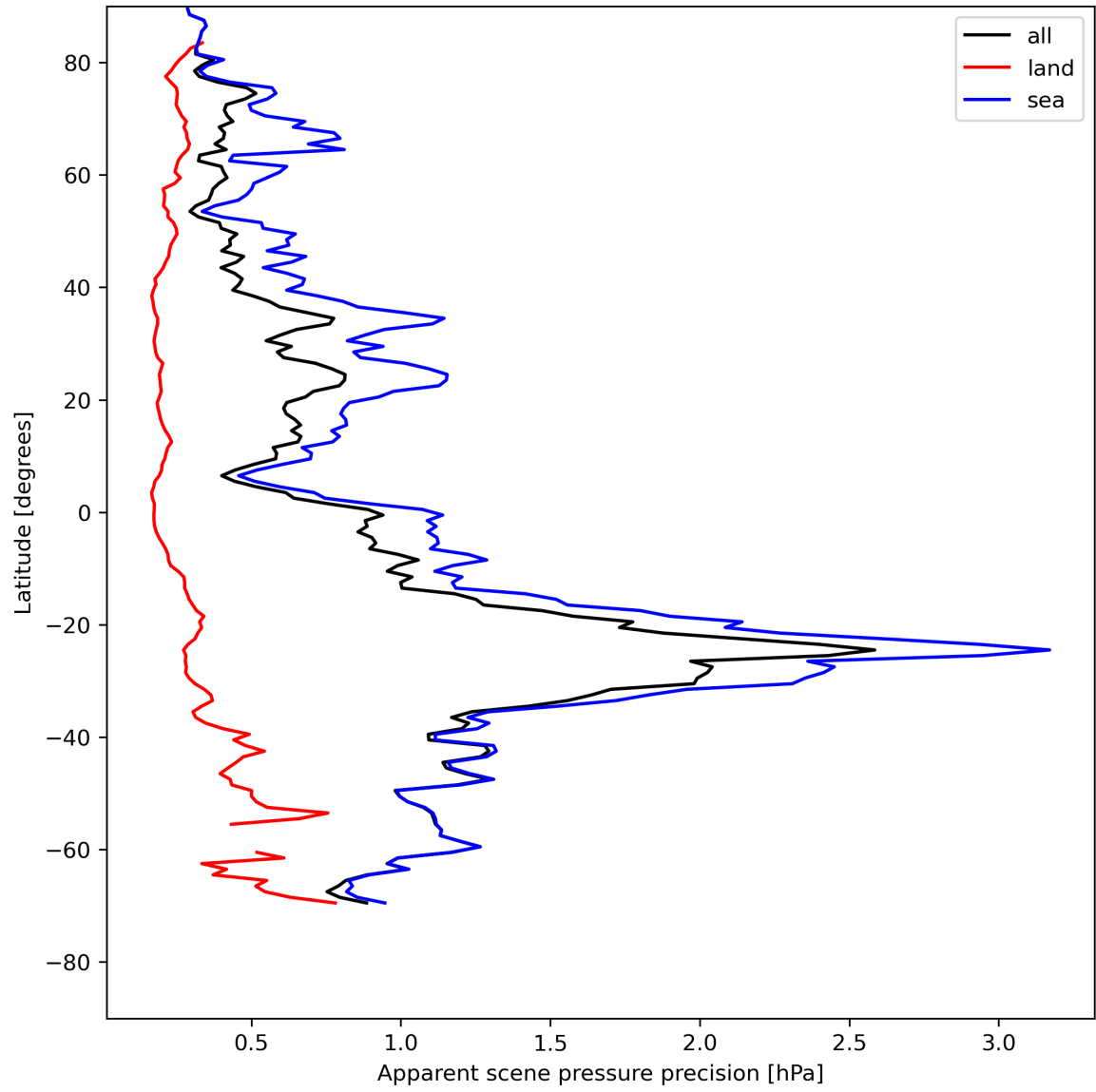
Figure 20: Zonal average of “Apparent scene pressure precision” for 2024-05-09 to 2024-05-11.
