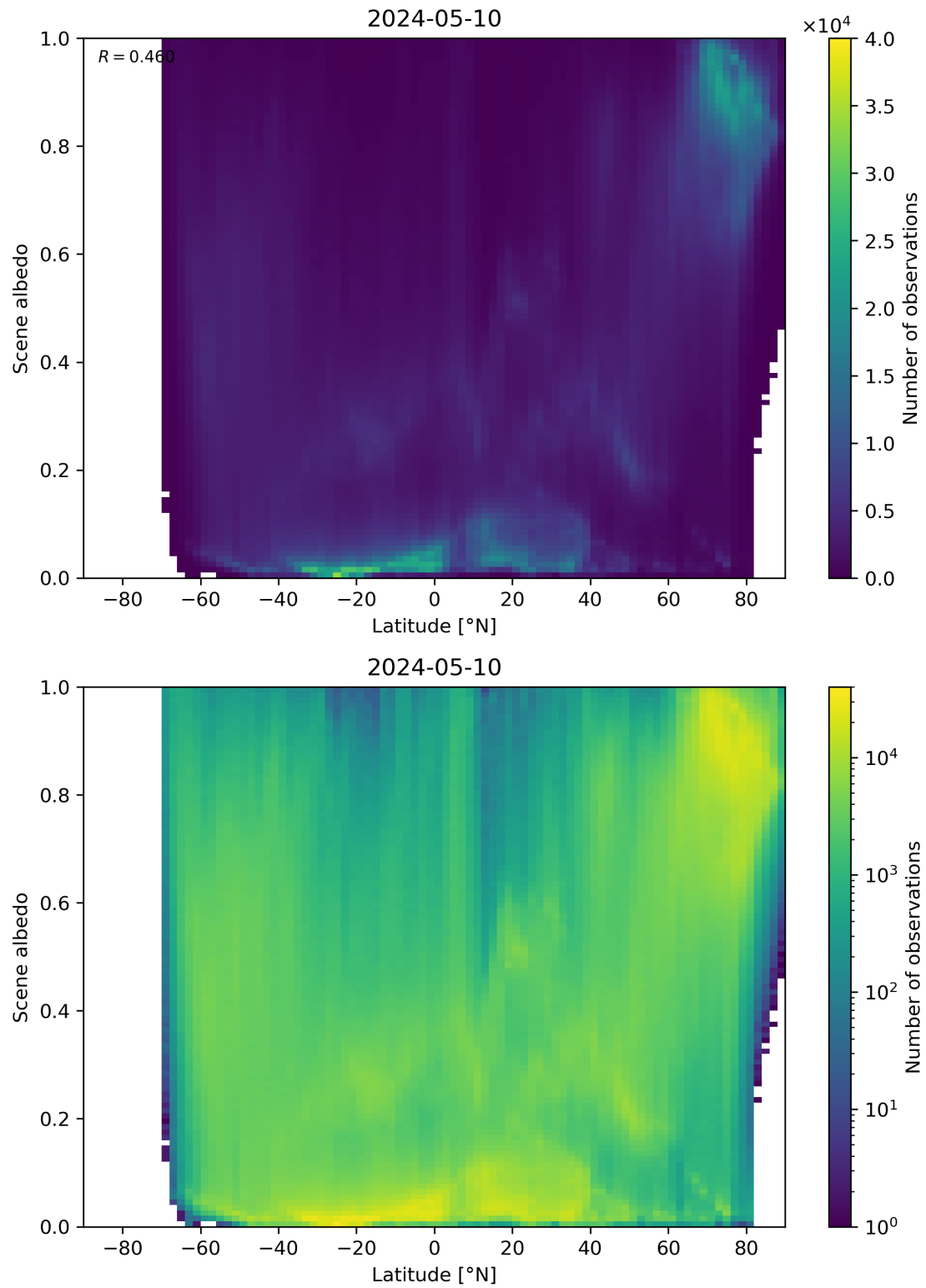
Figure 95: Scatter density plot of “Latitude” against “Scene albedo” for 2024-05-09 to 2024-05-11.
