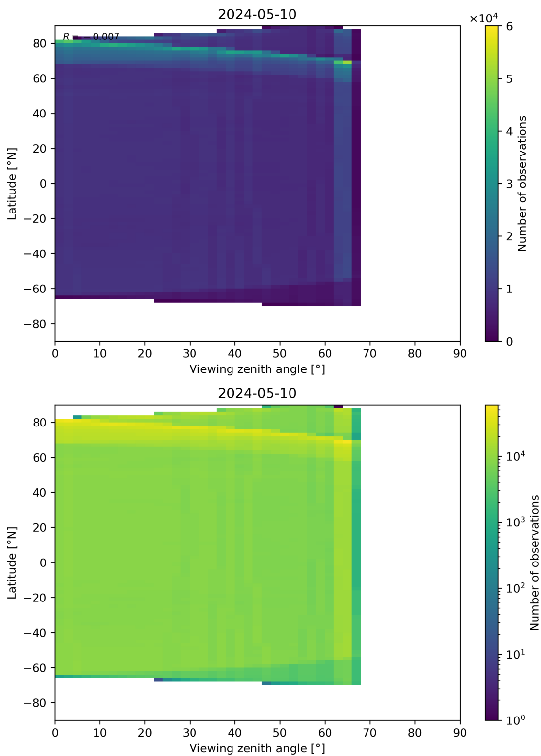
Figure 123: Scatter density plot of “Viewing zenith angle” against “Latitude” for 2024-05-09 to 2024-05-11.
