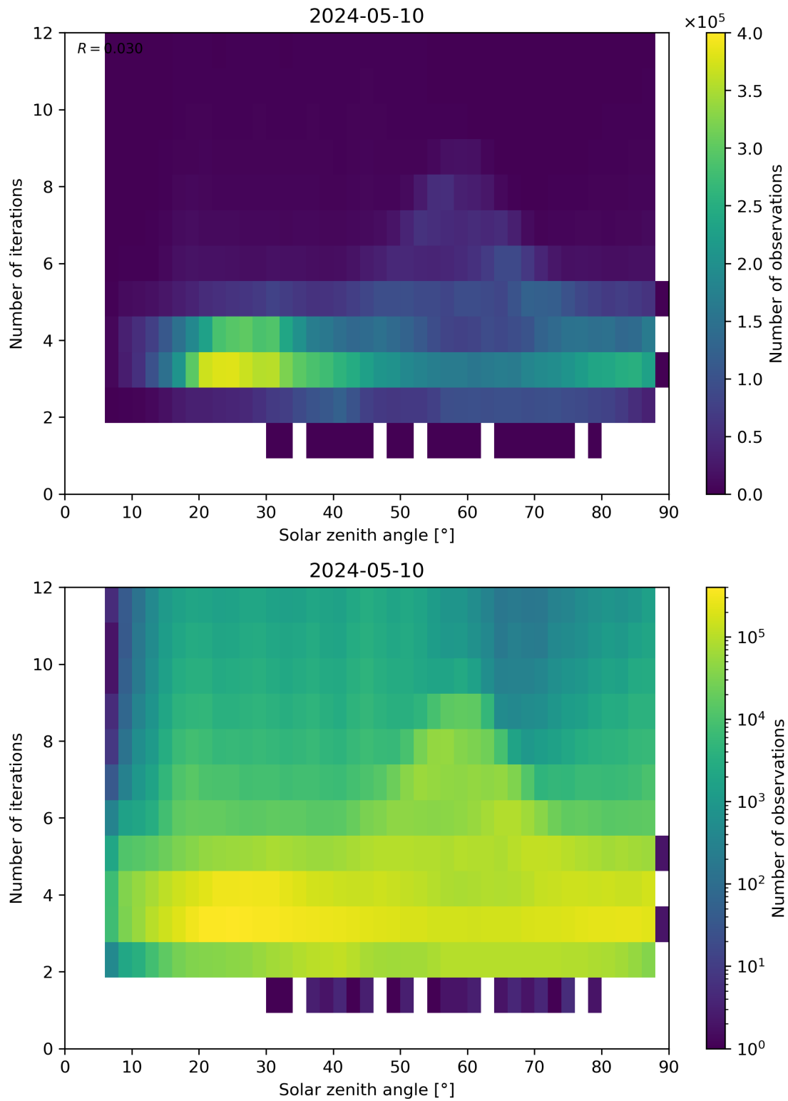
Figure 114: Scatter density plot of “Solar zenith angle” against “Number of iterations” for 2024-05-09 to 2024-05-11.
