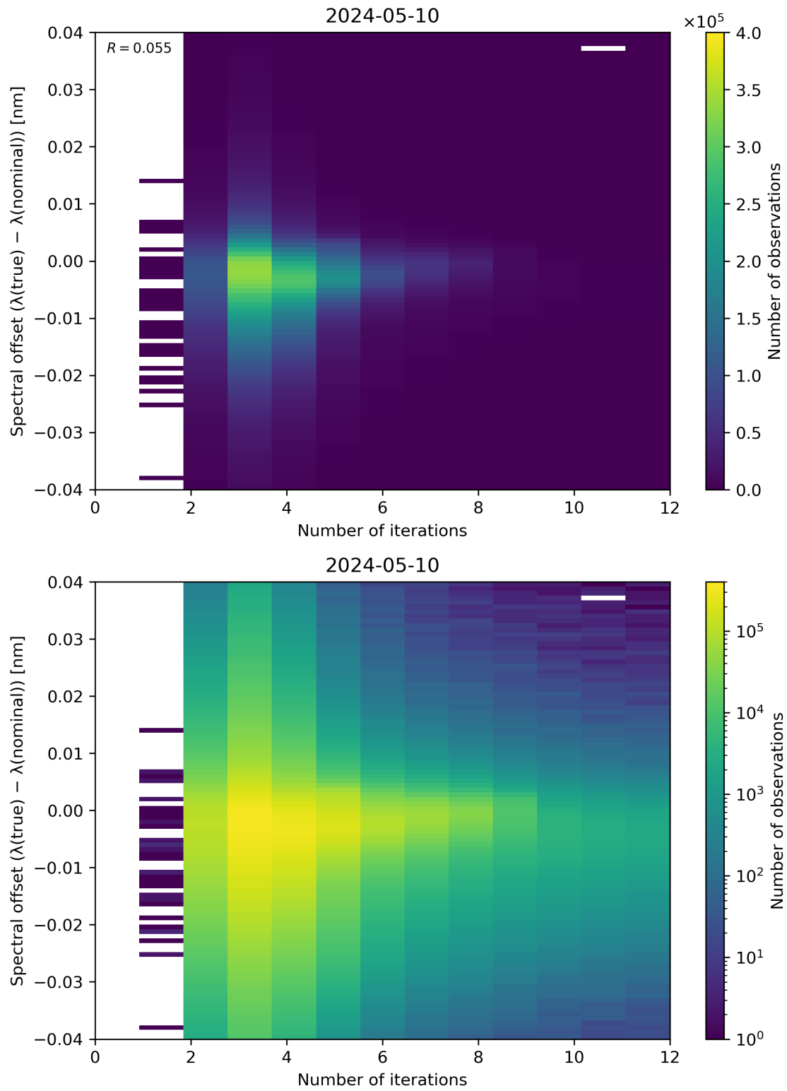
Figure 100: Scatter density plot of “Number of iterations” against “Spectral offset ( \lambda(\text{true}) - \lambda(\text{nominal}) )” for 2024-05-09 to 2024-05-11.
