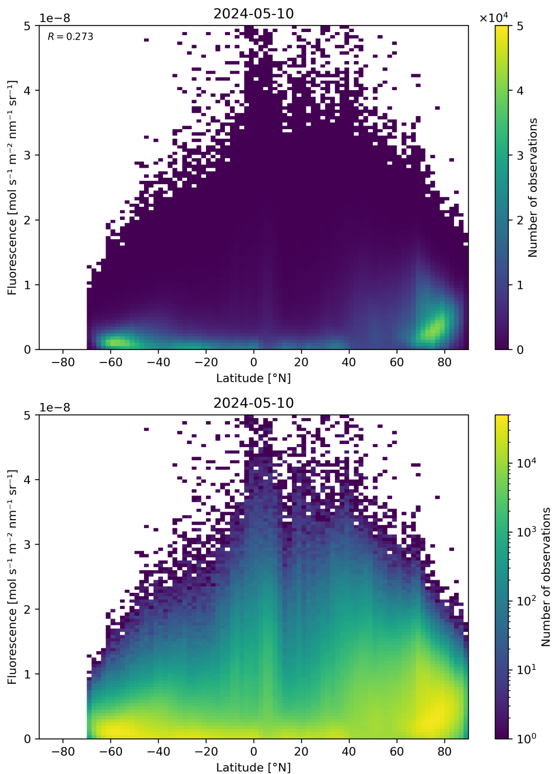
Figure 92: Scatter density plot of “Latitude” against “Fluorescence” for 2024-05-09 to 2024-05-11.
