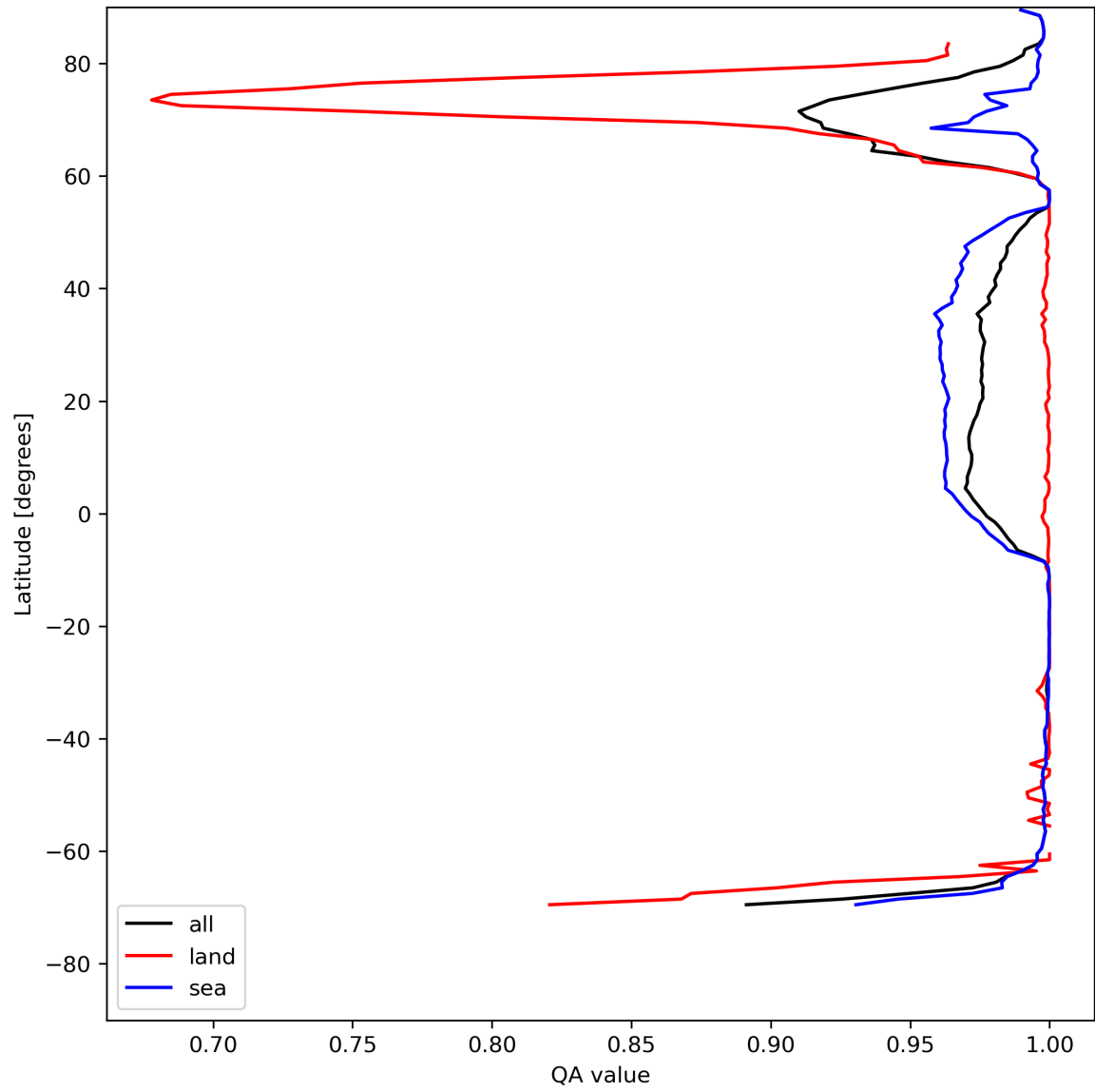
Figure 12: Zonal average of “QA value” for 2024-05-09 to 2024-05-11.
