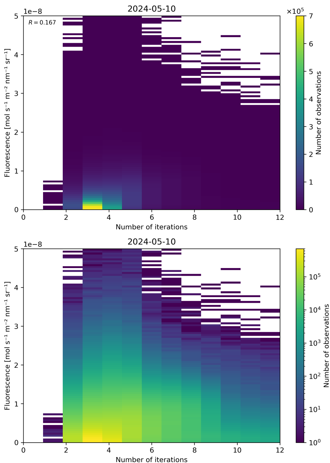
Figure 98: Scatter density plot of “Number of iterations” against “Fluorescence” for 2024-05-09 to 2024-05-11.
