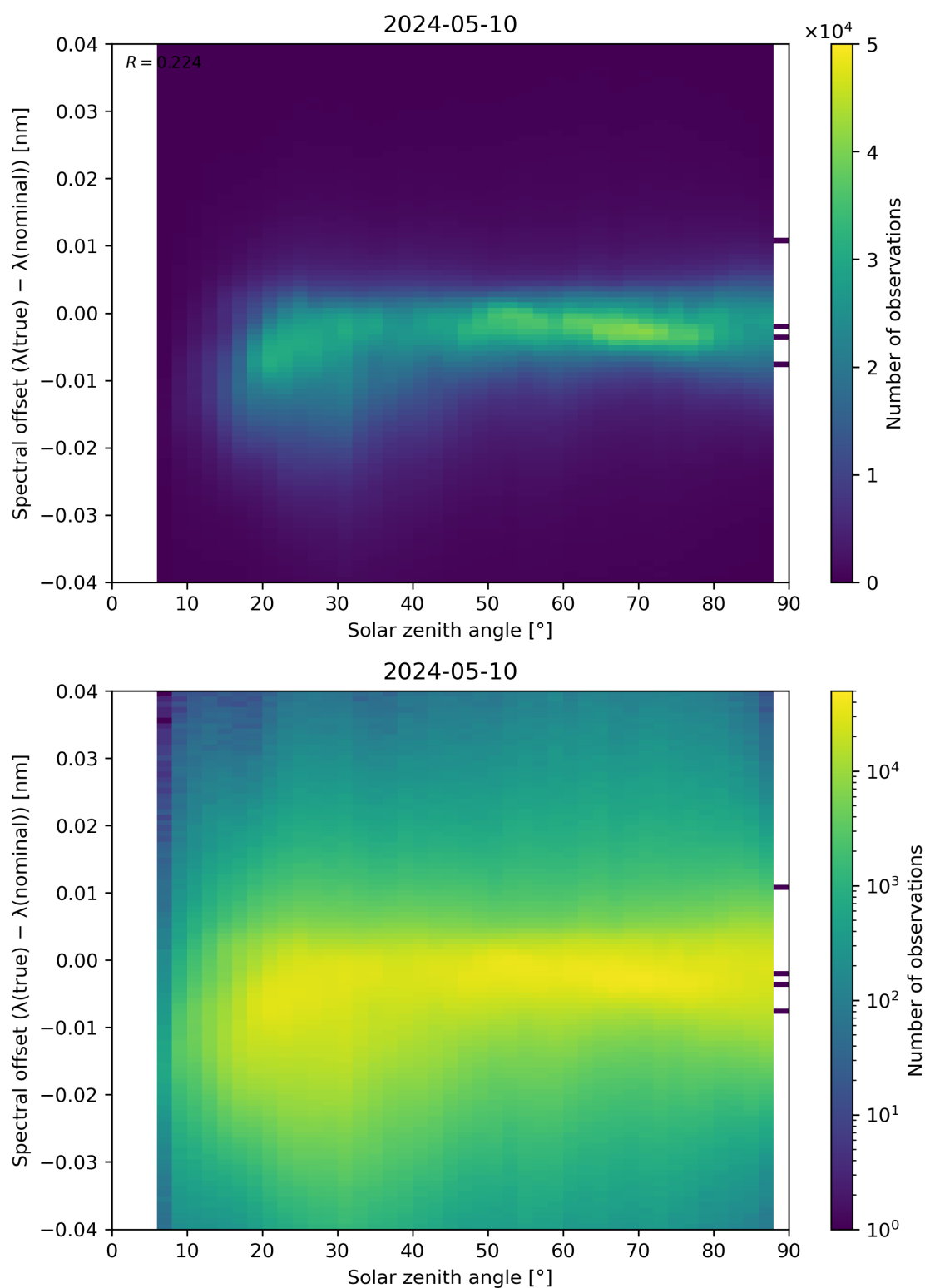
Figure 117: Scatter density plot of “Solar zenith angle” against “Spectral offset ( \lambda(\text{true}) - \lambda(\text{nominal}) )” for 2024-05-09 to 2024-05-11.
