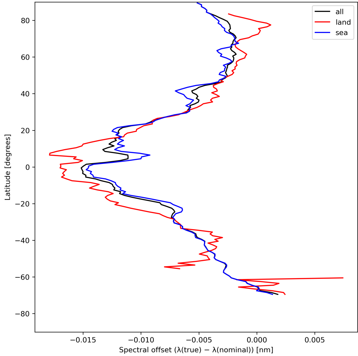
Figure 28: Zonal average of “Spectral offset ( \lambda(\text{true}) - \lambda(\text{nominal}) )” for 2024-05-09 to 2024-05-11.
