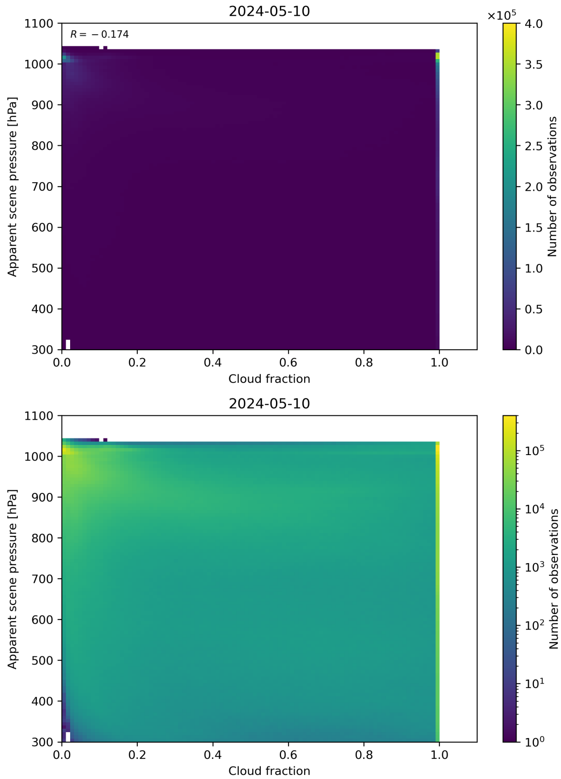
Figure 70: Scatter density plot of “Cloud fraction” against “Apparent scene pressure” for 2024-05-09 to 2024-05-11.
