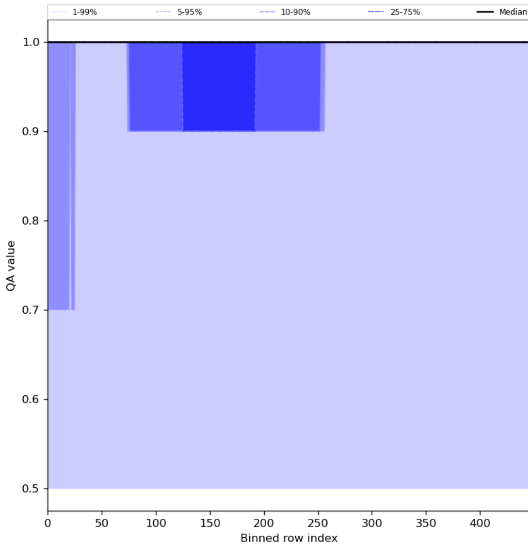
Figure 46: Along track statistics of “QA value” for 2024-05-09 to 2024-05-11
