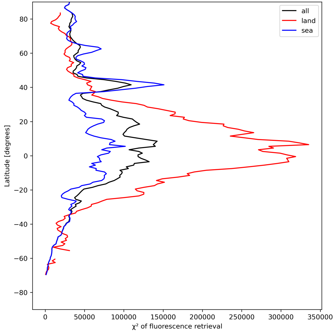
Figure 25: Zonal average of “ \chi^2 of fluorescence retrieval” for 2024-05-09 to 2024-05-11.
