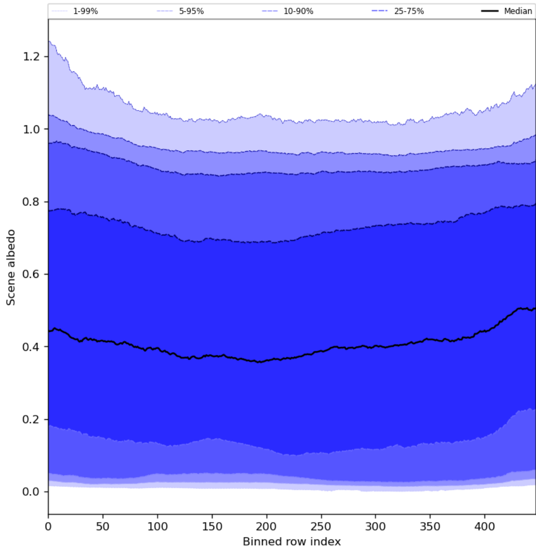
Figure 51: Along track statistics of “Scene albedo” for 2024-05-09 to 2024-05-11
