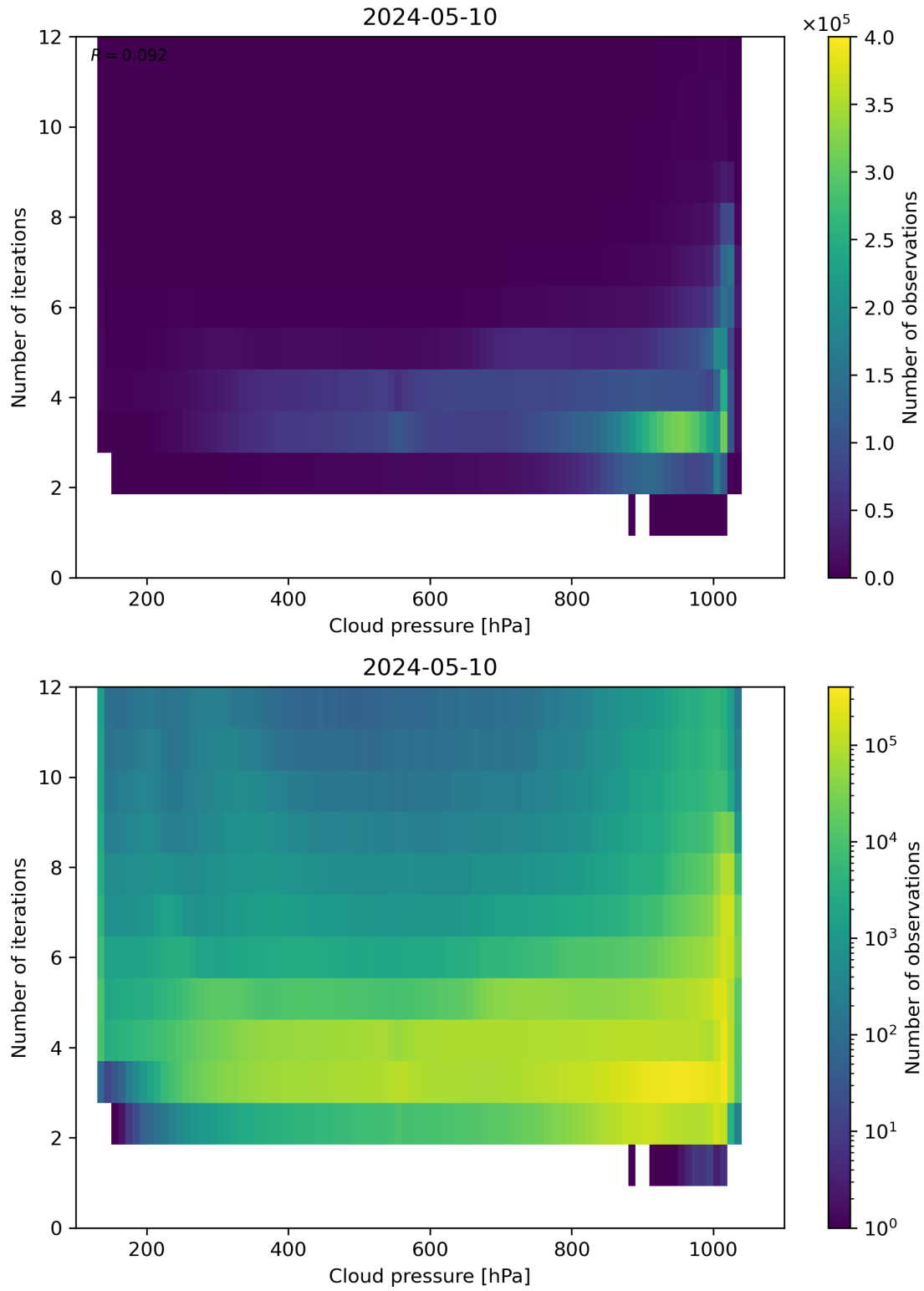
Figure 81: Scatter density plot of “Cloud pressure” against “Number of iterations” for 2024-05-09 to 2024-05-11.
