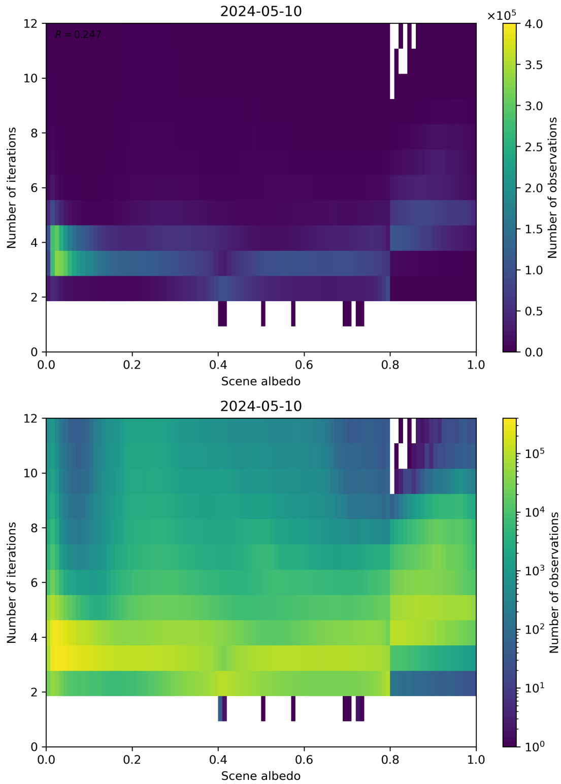
Figure 105: Scatter density plot of “Scene albedo” against “Number of iterations” for 2024-05-09 to 2024-05-11.
