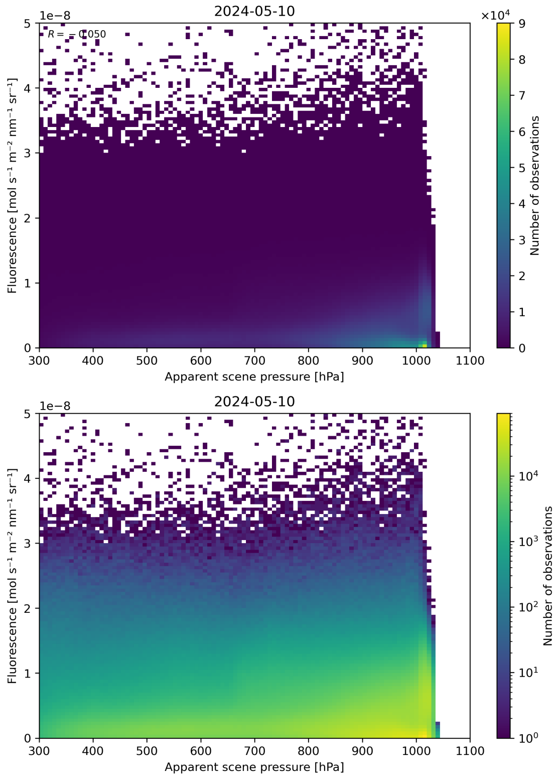
Figure 64: Scatter density plot of “Apparent scene pressure” against “Fluorescence” for 2024-05-09 to 2024-05-11.
