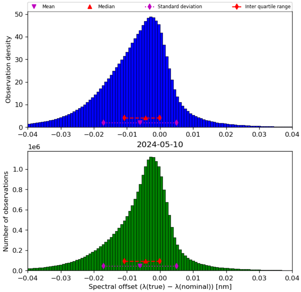
Figure 45: Histogram of “Spectral offset ( \lambda(\text{true}) - \lambda(\text{nominal}) )” for 2024-05-09 to 2024-05-11
