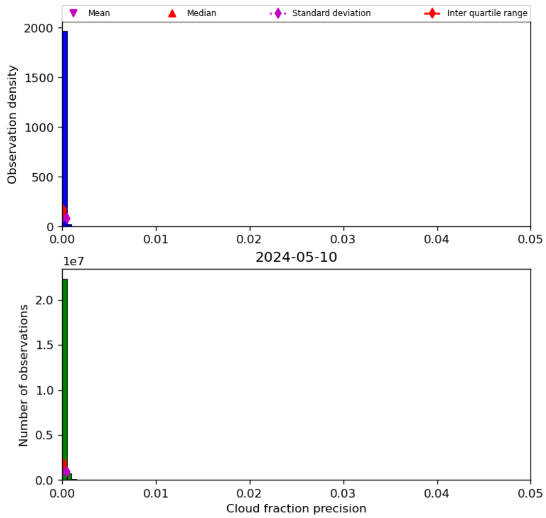
Figure 33: Histogram of “Cloud fraction precision” for 2024-05-09 to 2024-05-11
