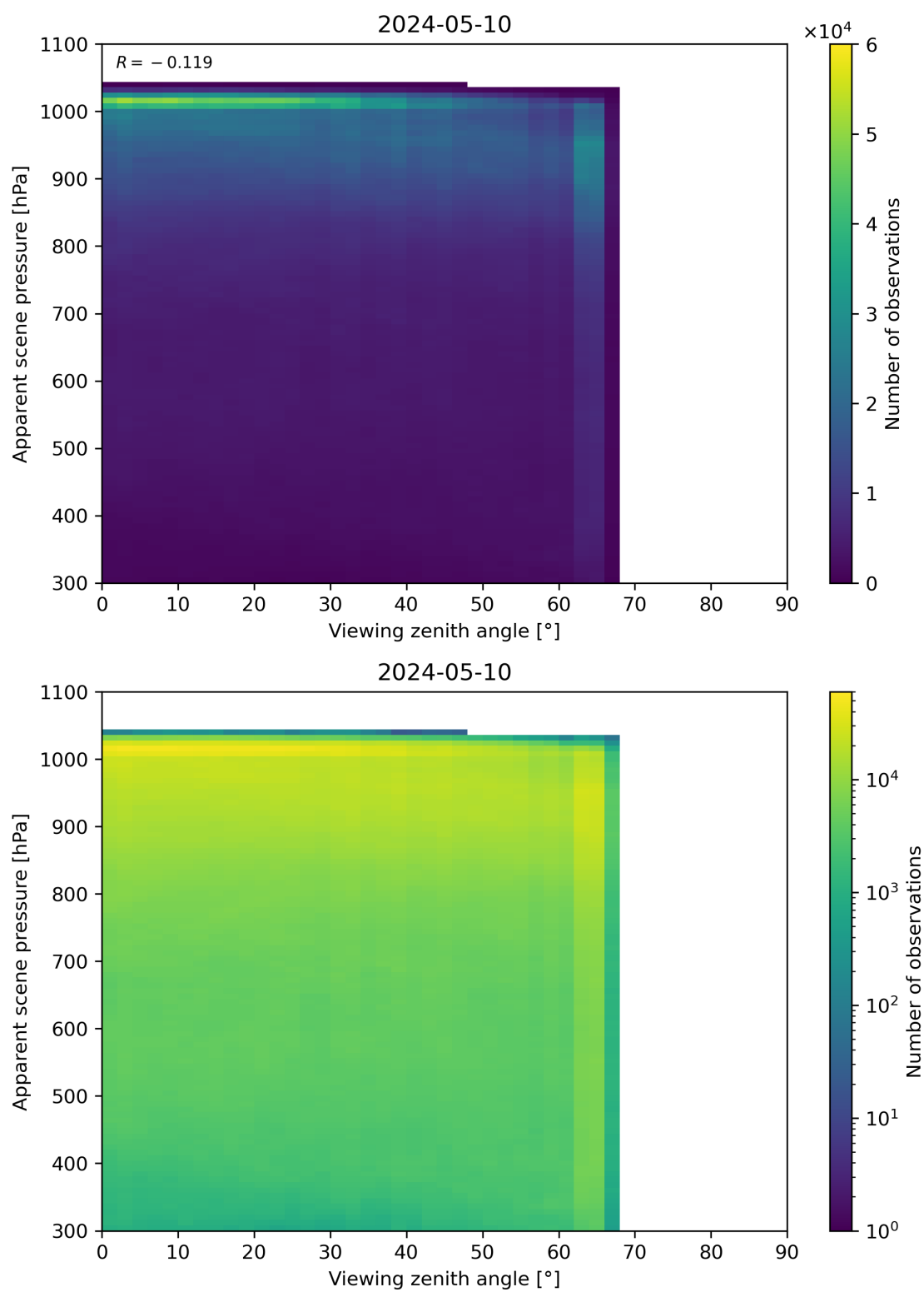
Figure 118: Scatter density plot of “Viewing zenith angle” against “Apparent scene pressure” for 2024-05-09 to 2024-05-11.
