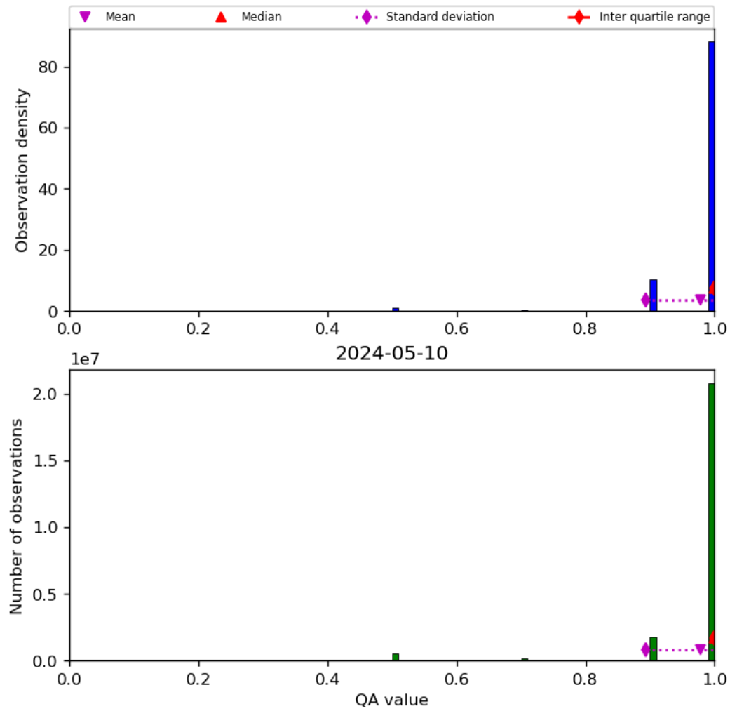
Figure 29: Histogram of “QA value” for 2024-05-09 to 2024-05-11
