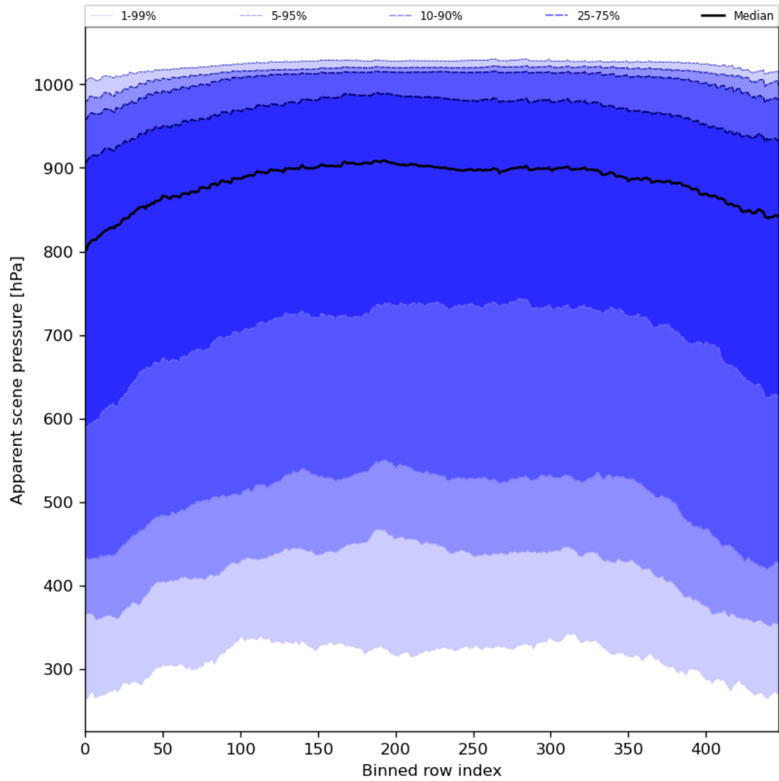
Figure 53: Along track statistics of “Apparent scene pressure” for 2024-05-09 to 2024-05-11
