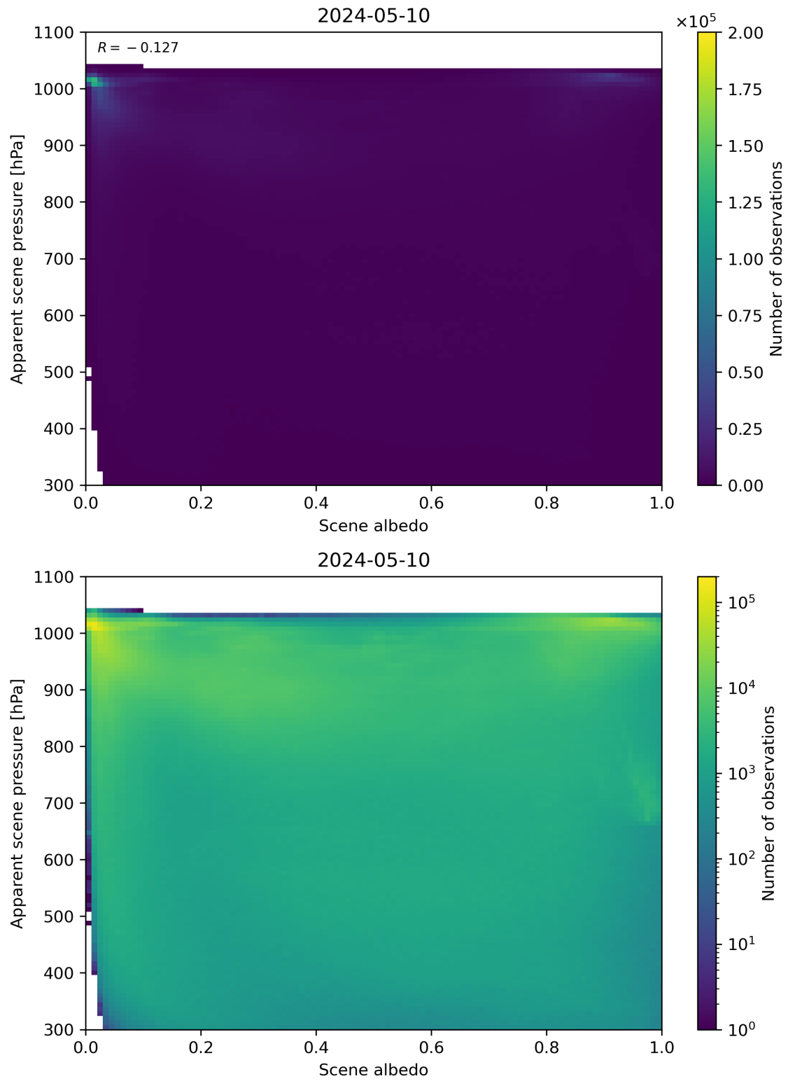
Figure 102: Scatter density plot of “Scene albedo” against “Apparent scene pressure” for 2024-05-09 to 2024-05-11.
