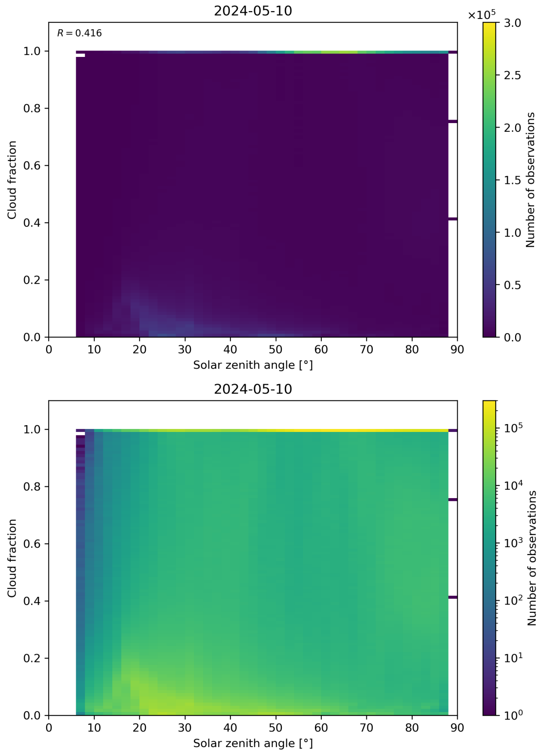
Figure 110: Scatter density plot of “Solar zenith angle” against “Cloud fraction” for 2024-05-09 to 2024-05-11.
