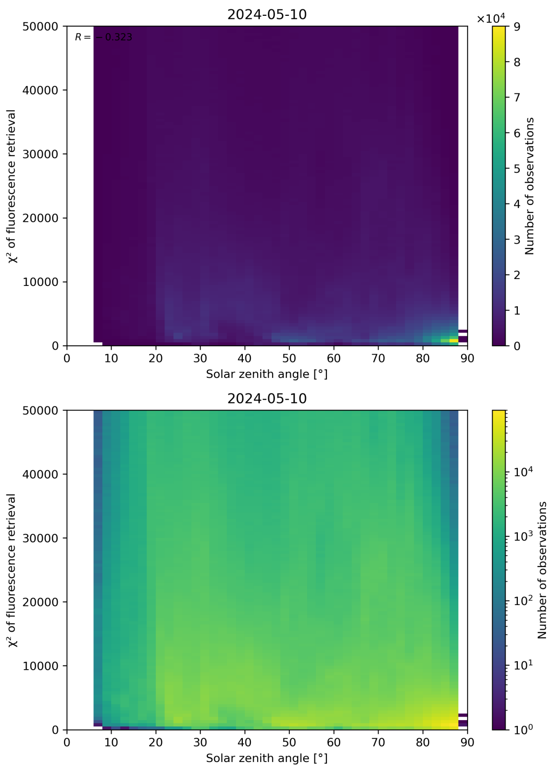
Figure 109: Scatter density plot of “Solar zenith angle” against “ \chi^2 of fluorescence retrieval” for 2024-05-09 to 2024-05-11.
