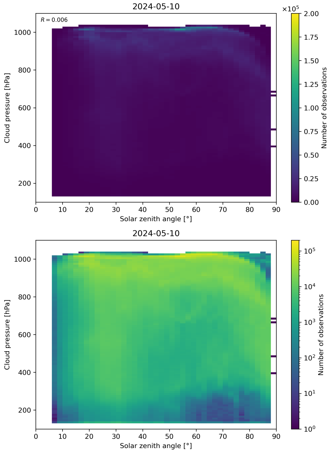
Figure 111: Scatter density plot of “Solar zenith angle” against “Cloud pressure” for 2024-05-09 to 2024-05-11.
