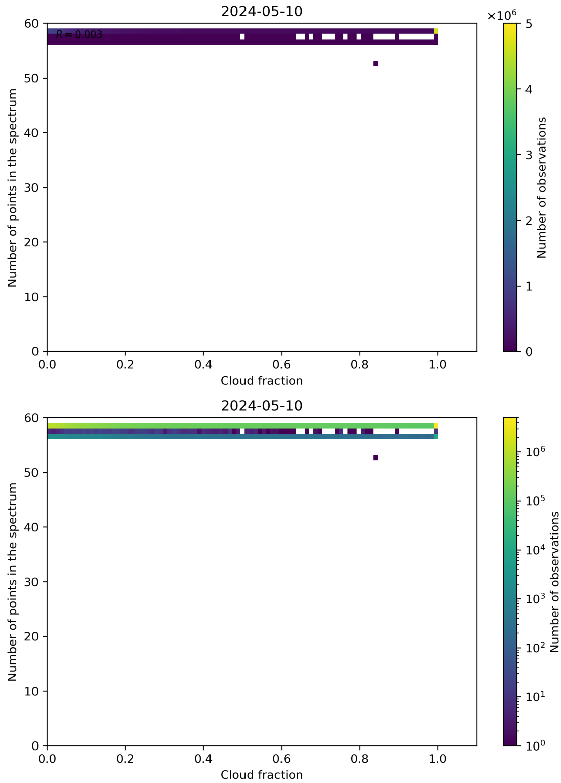
Figure 74: Scatter density plot of “Cloud fraction” against “Number of points in the spectrum” for 2024-05-09 to 2024-05-11.
