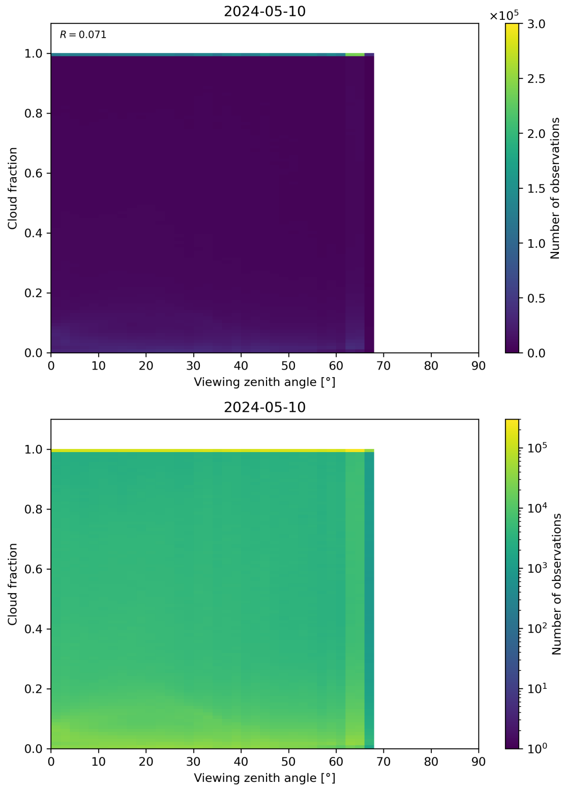
Figure 120: Scatter density plot of “Viewing zenith angle” against “Cloud fraction” for 2024-05-09 to 2024-05-11.
