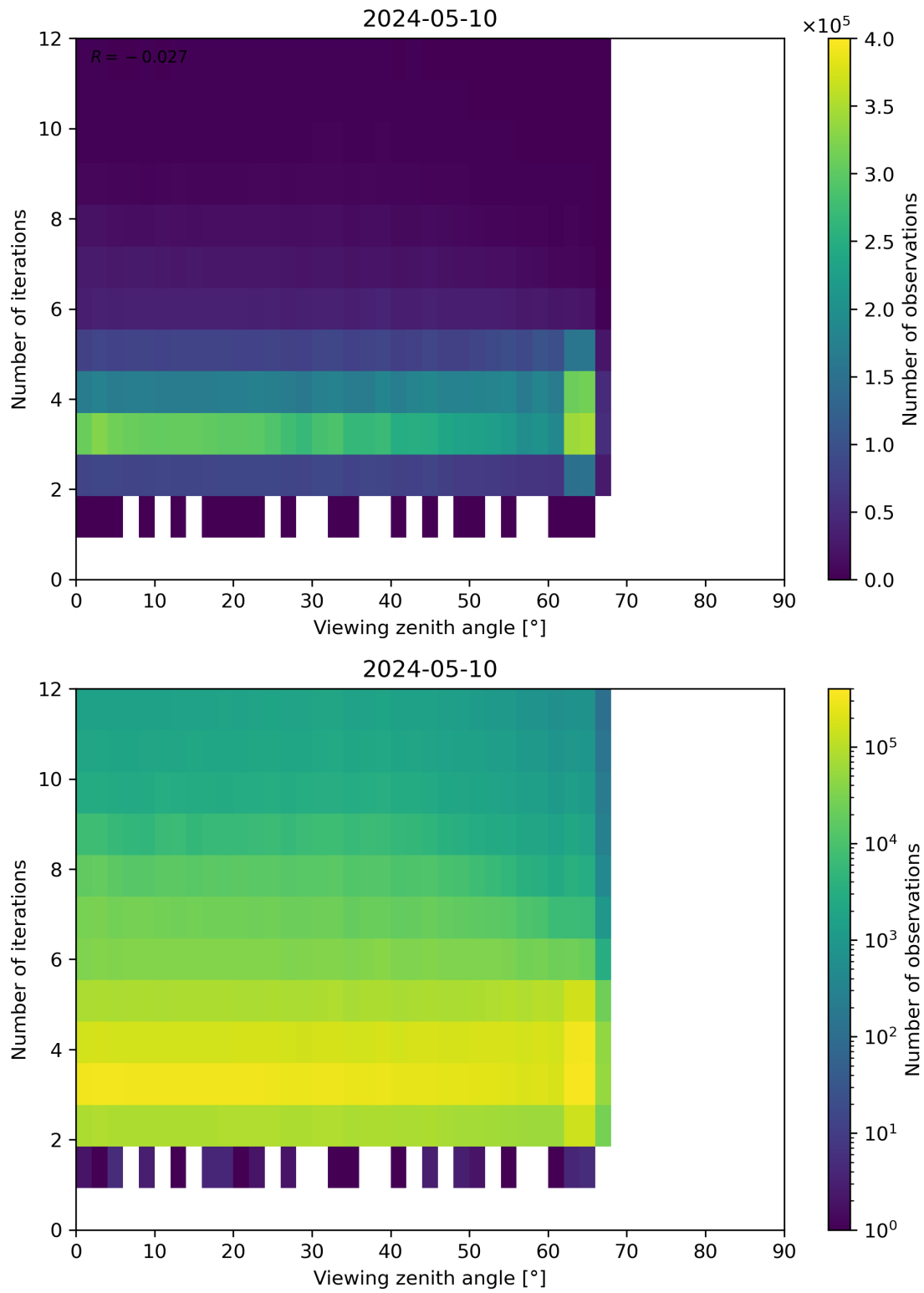
Figure 124: Scatter density plot of “Viewing zenith angle” against “Number of iterations” for 2024-05-09 to 2024-05-11.
