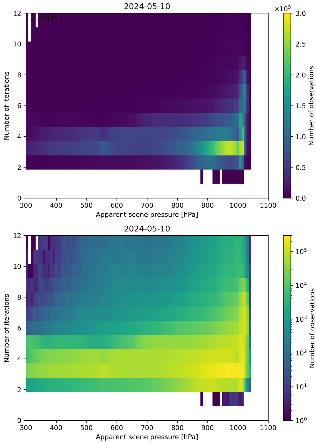
Figure 65: Scatter density plot of “Apparent scene pressure” against “Number of iterations” for 2024-05-09 to 2024-05-11.
