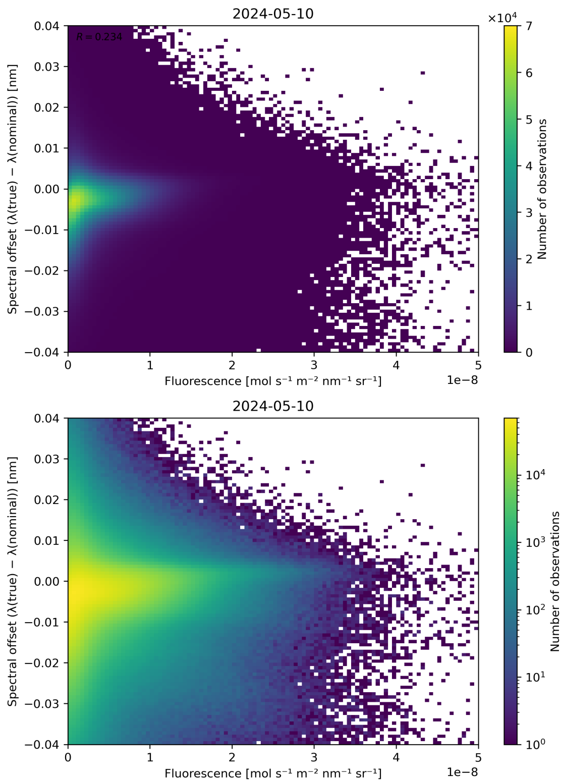
Figure 87: Scatter density plot of “Fluorescence” against “Spectral offset ( \lambda(\text{true}) - \lambda(\text{nominal}) )” for 2024-05-09 to 2024-05-11.
