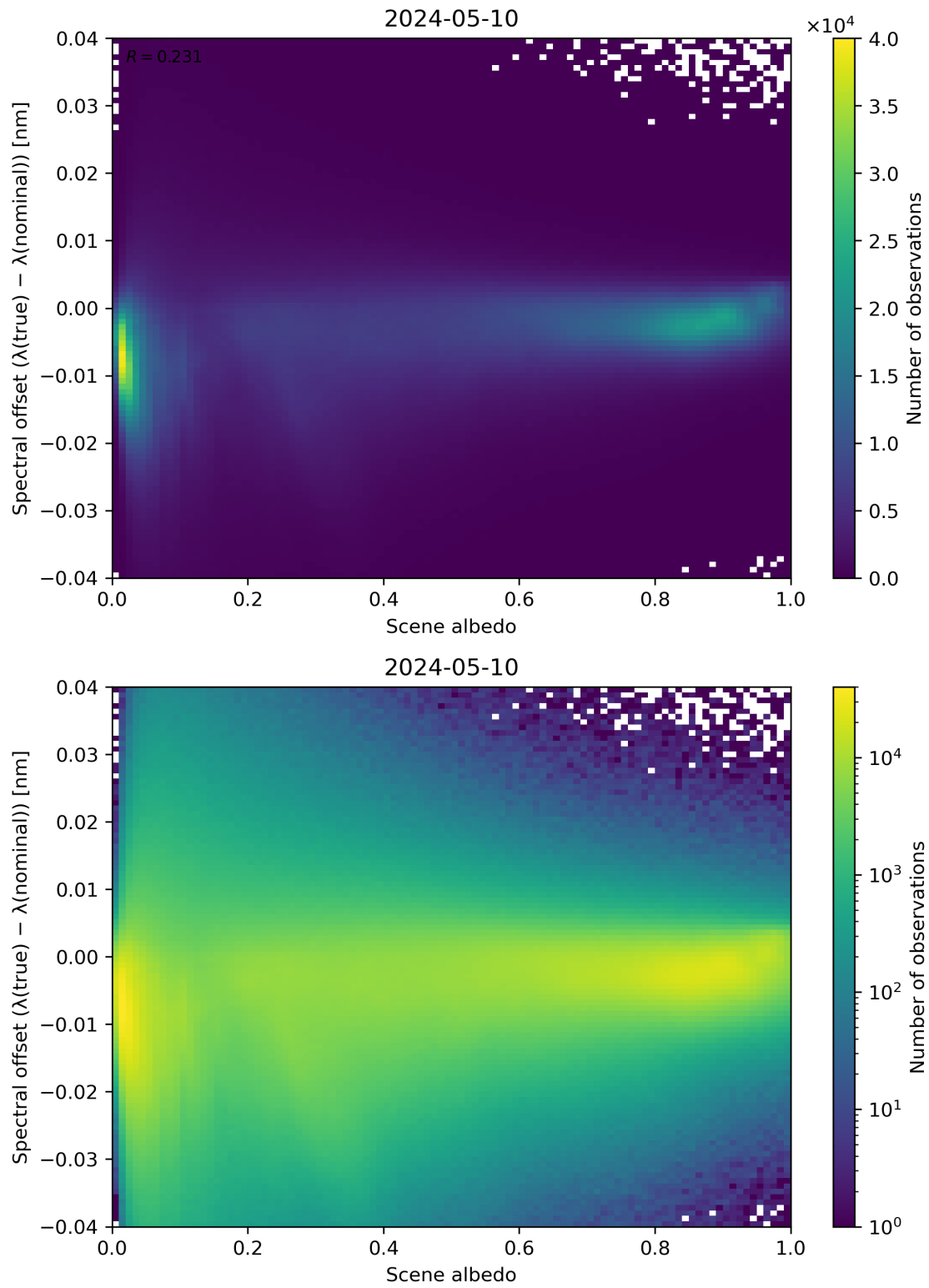
Figure 107: Scatter density plot of “Scene albedo” against “Spectral offset ( \lambda(\text{true}) - \lambda(\text{nominal}) )” for 2024-05-09 to 2024-05-11.
