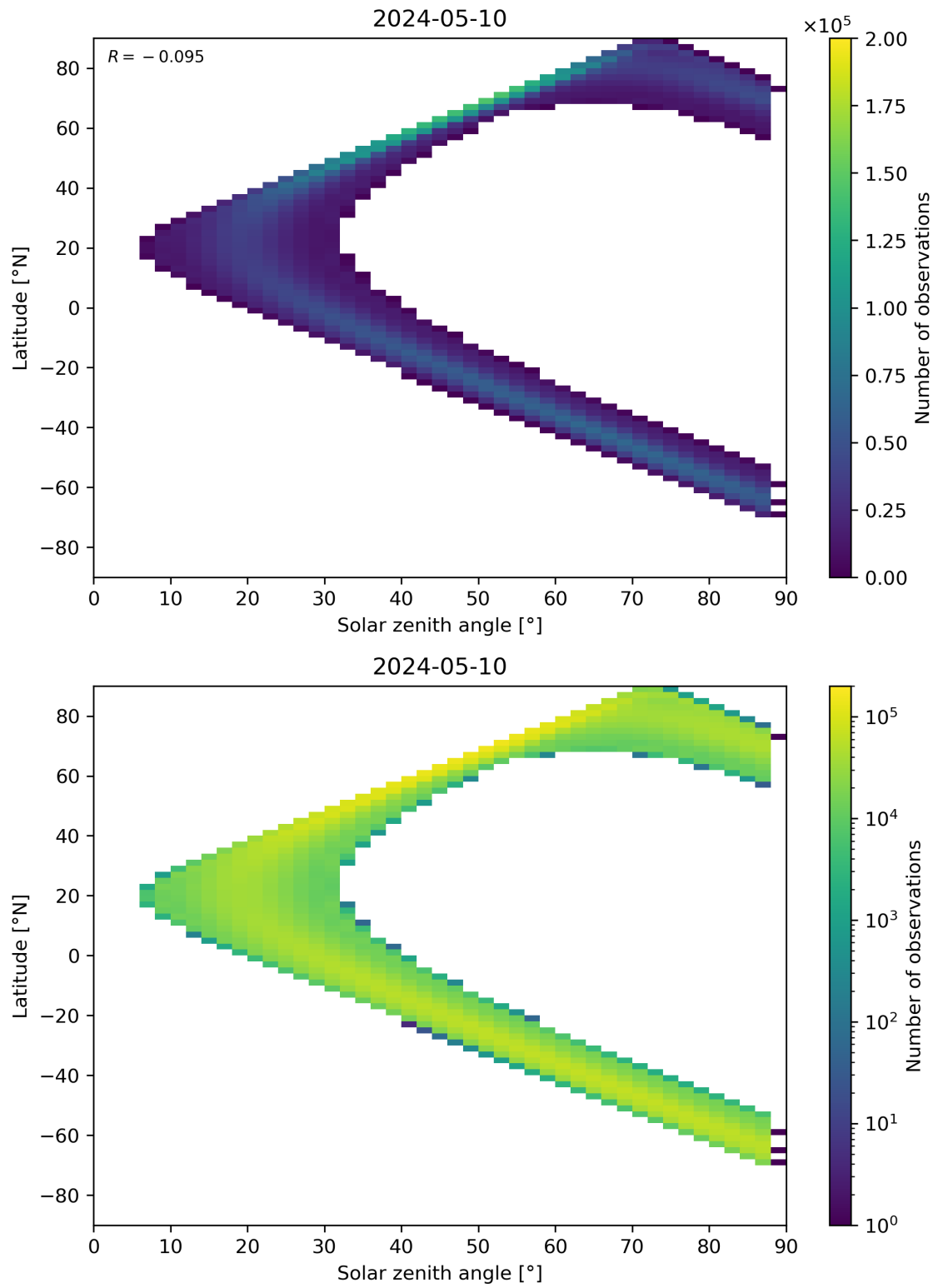
Figure 113: Scatter density plot of “Solar zenith angle” against “Latitude” for 2024-05-09 to 2024-05-11.
