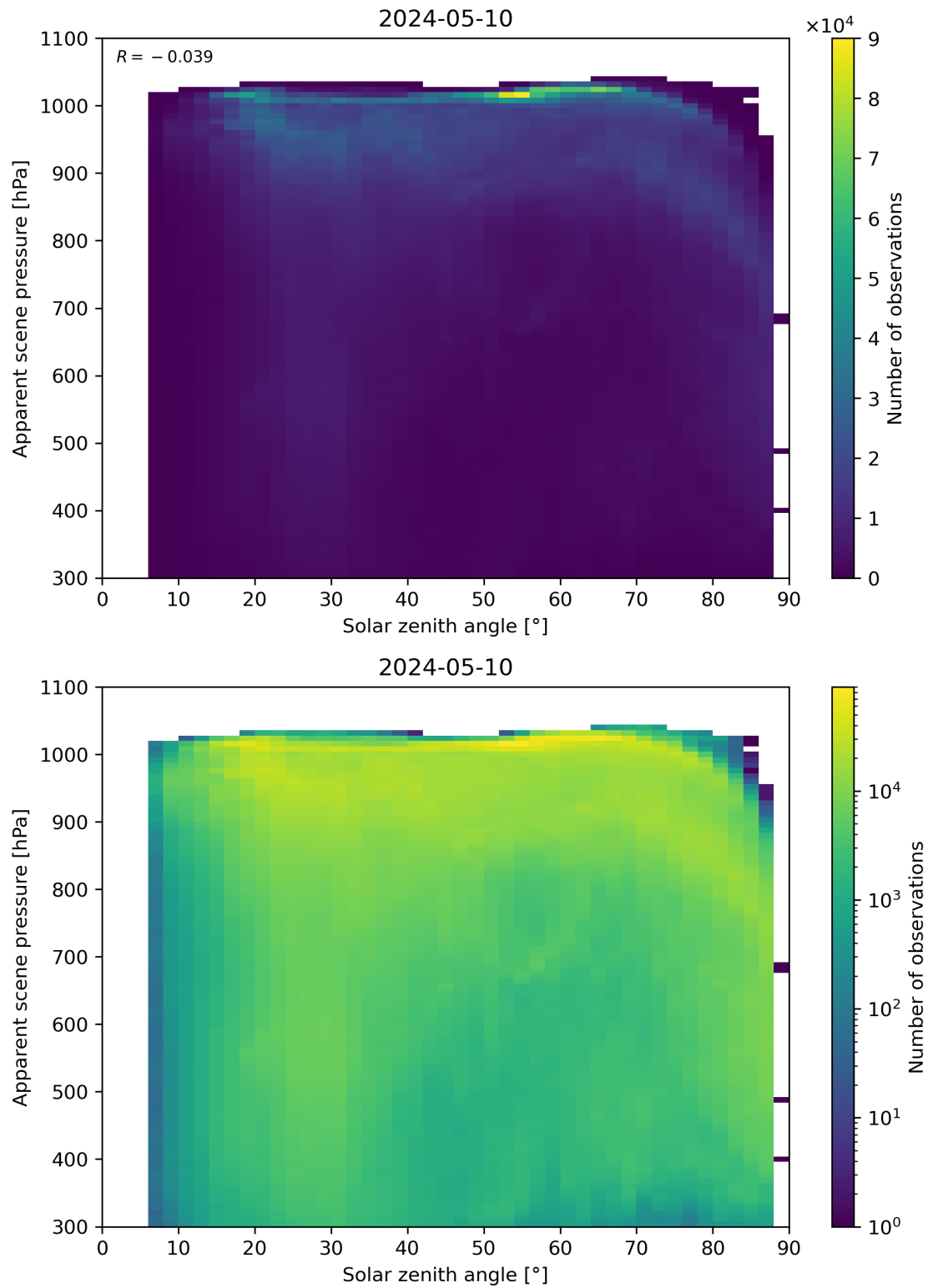
Figure 108: Scatter density plot of “Solar zenith angle” against “Apparent scene pressure” for 2024-05-09 to 2024-05-11.
