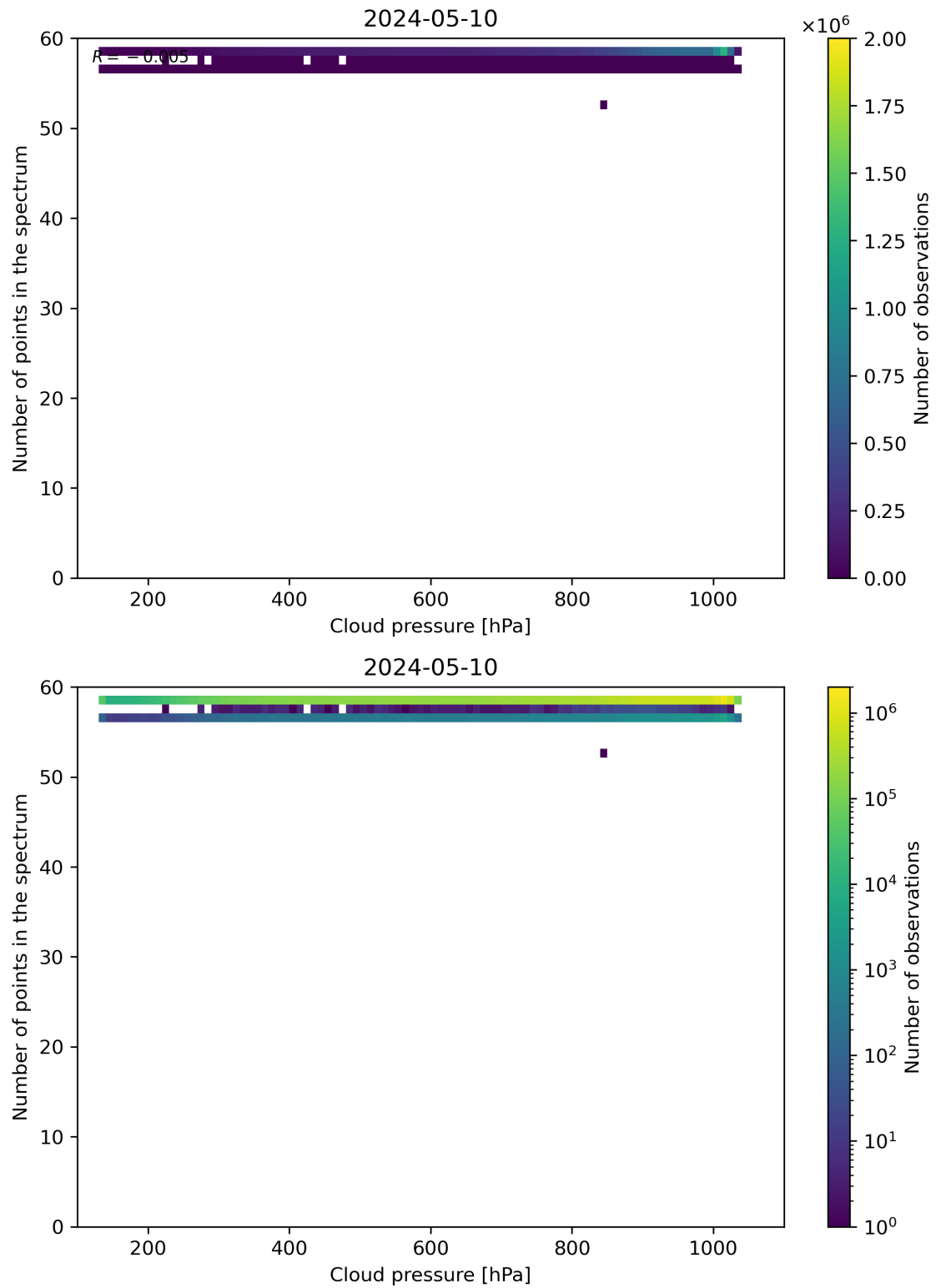
Figure 82: Scatter density plot of “Cloud pressure” against “Number of points in the spectrum” for 2024-05-09 to 2024-05-11.
