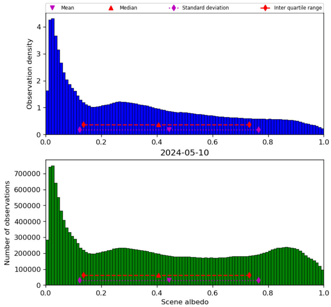
Figure 34: Histogram of “Scene albedo” for 2024-05-09 to 2024-05-11
