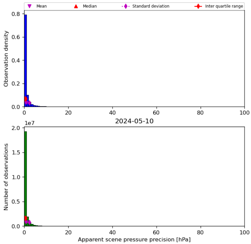
Figure 37: Histogram of “Apparent scene pressure precision” for 2024-05-09 to 2024-05-11
