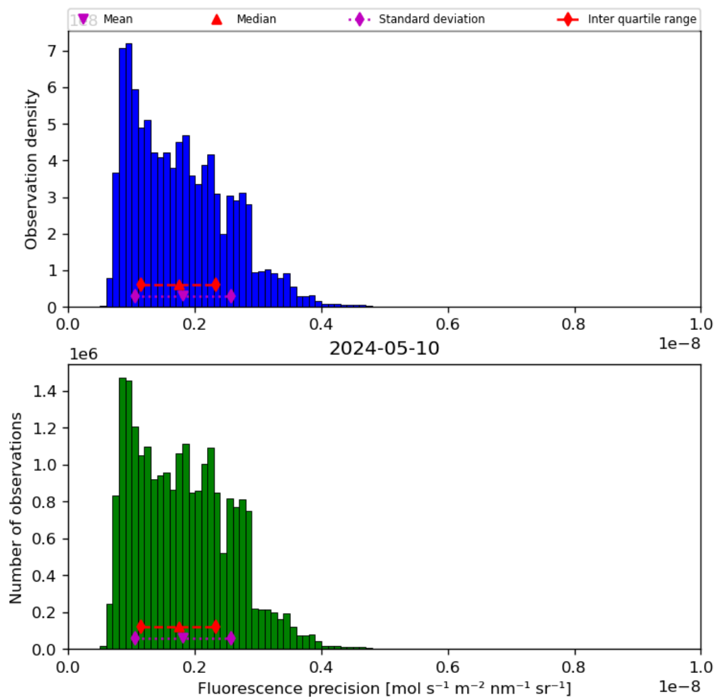
Figure 41: Histogram of “Fluorescence precision” for 2024-05-09 to 2024-05-11
