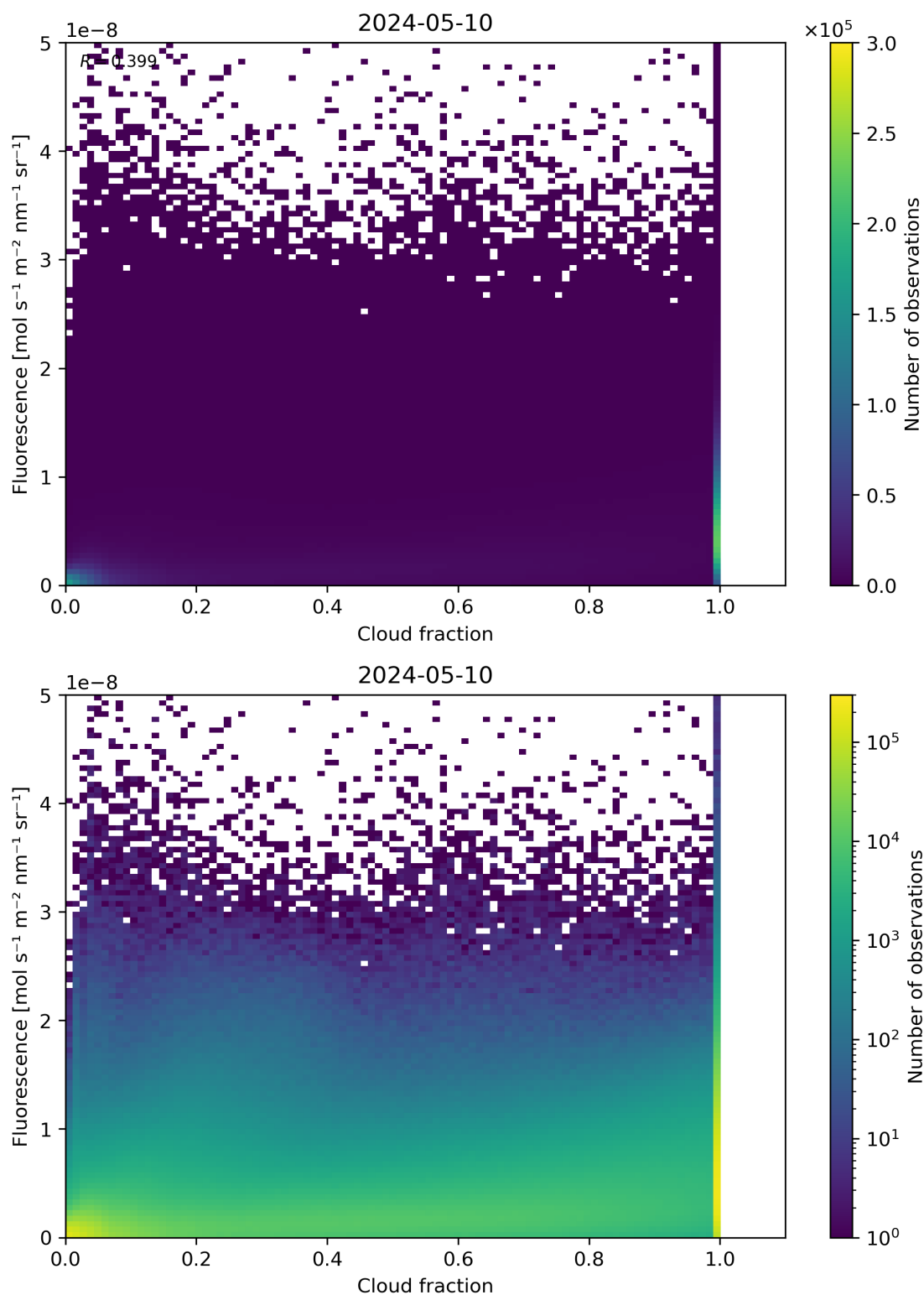
Figure 72: Scatter density plot of “Cloud fraction” against “Fluorescence” for 2024-05-09 to 2024-05-11.
