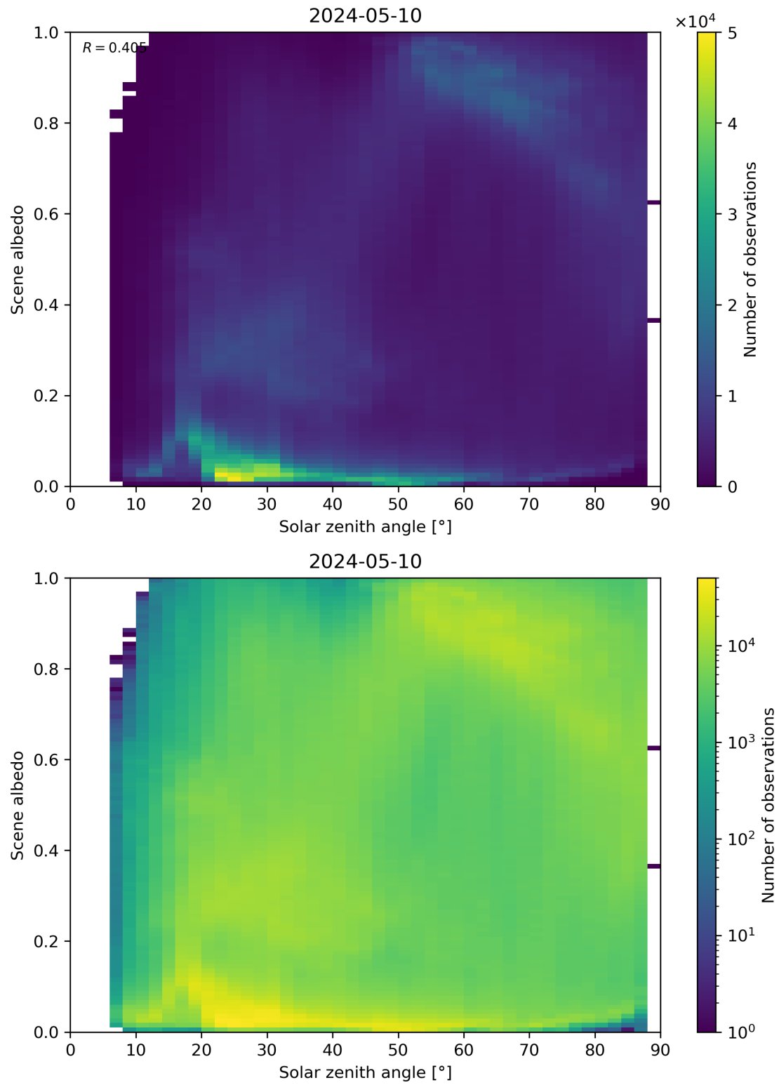
Figure 116: Scatter density plot of “Solar zenith angle” against “Scene albedo” for 2024-05-09 to 2024-05-11.
