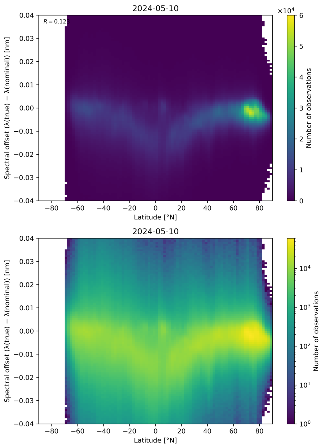
Figure 96: Scatter density plot of “Latitude” against “Spectral offset ( \lambda(\text{true}) - \lambda(\text{nominal}) )” for 2024-05-09 to 2024-05-11.
