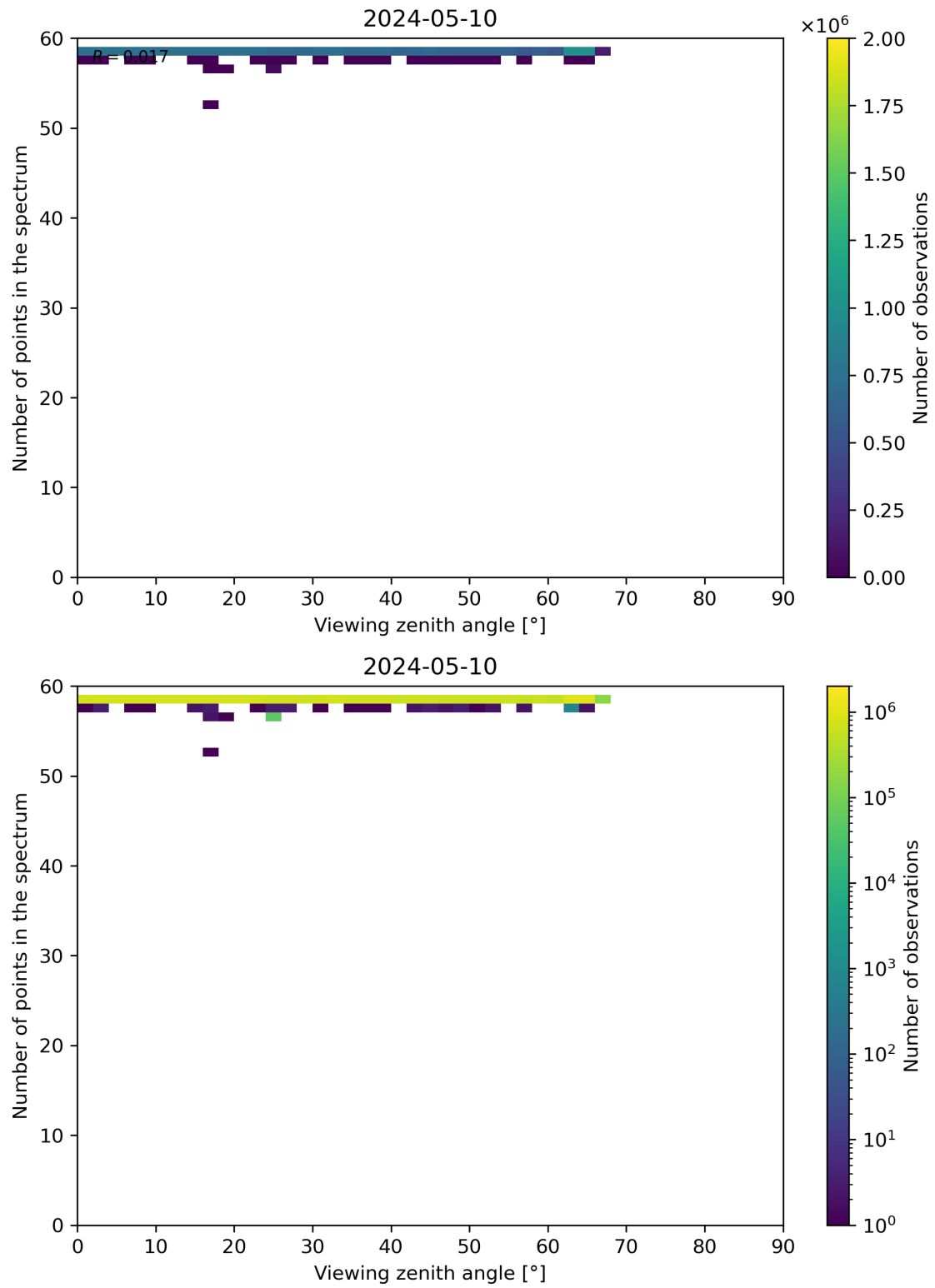
Figure 125: Scatter density plot of “Viewing zenith angle” against “Number of points in the spectrum” for 2024-05-09 to 2024-05-11.
