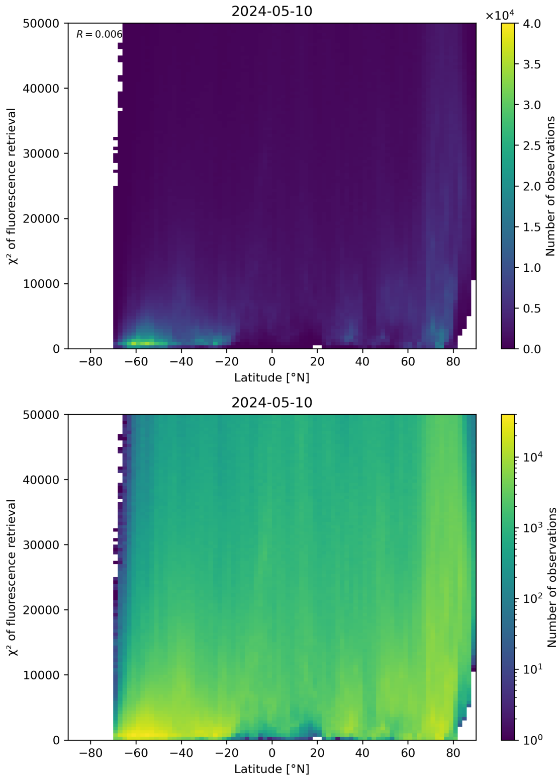
Figure 89: Scatter density plot of “Latitude” against “ \chi^2 of fluorescence retrieval” for 2024-05-09 to 2024-05-11.
