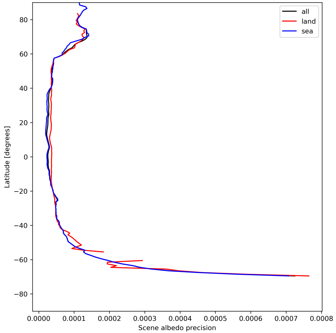
Figure 18: Zonal average of “Scene albedo precision” for 2024-05-09 to 2024-05-11.
