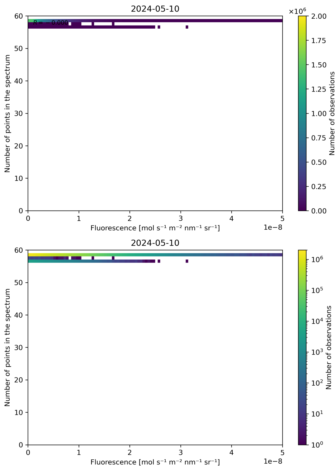
Figure 86: Scatter density plot of “Fluorescence” against “Number of points in the spectrum” for 2024-05-09 to 2024-05-11.
