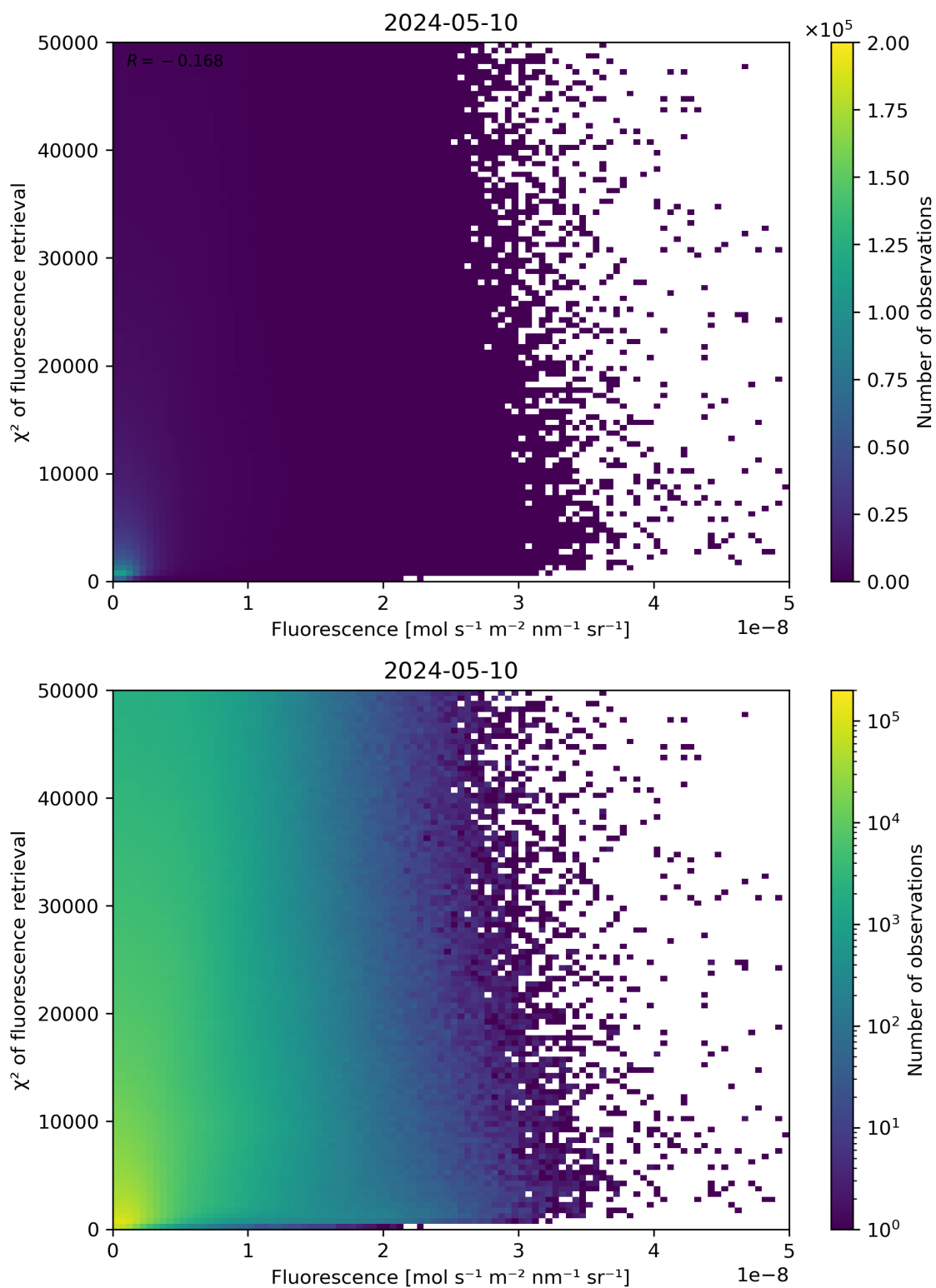
Figure 85: Scatter density plot of “Fluorescence” against “ \chi^2 of fluorescence retrieval” for 2024-05-09 to 2024-05-11.
