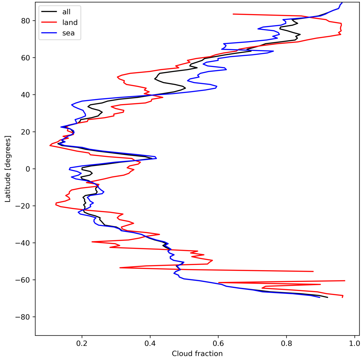
Figure 15: Zonal average of “Cloud fraction” for 2024-05-09 to 2024-05-11.
