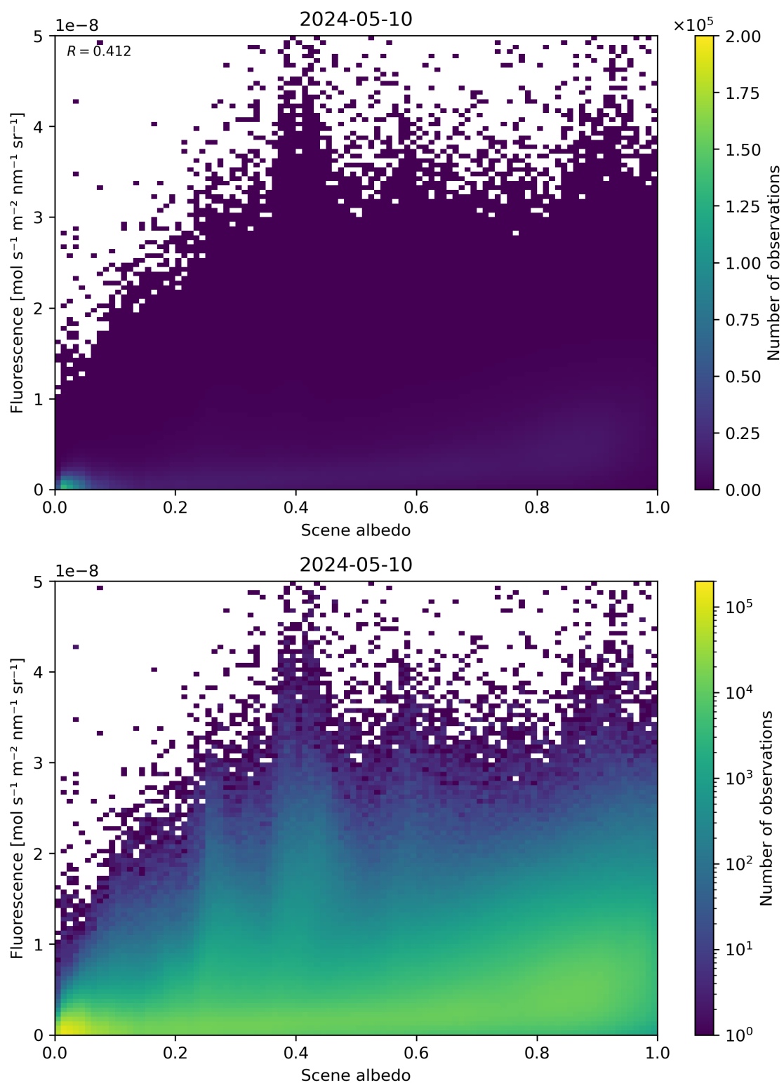
Figure 104: Scatter density plot of “Scene albedo” against “Fluorescence” for 2024-05-09 to 2024-05-11.
