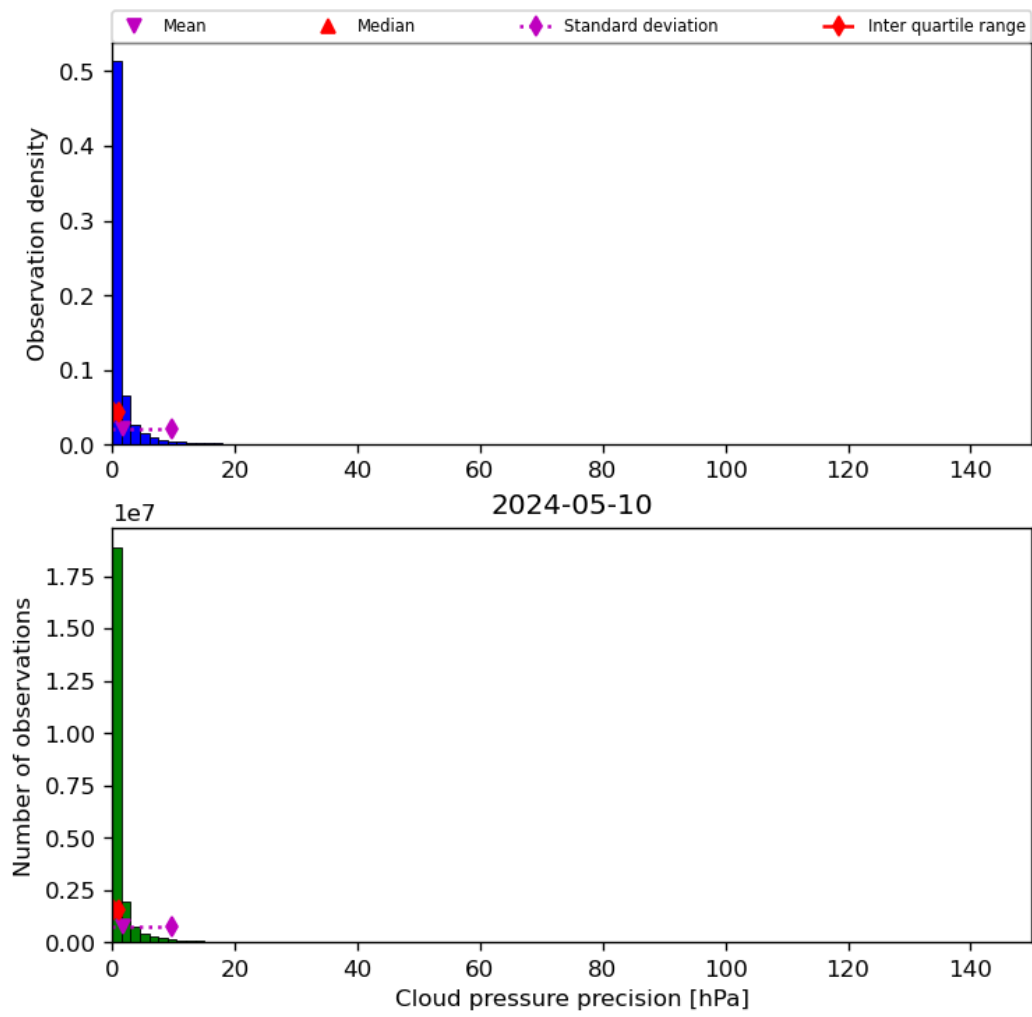
Figure 31: Histogram of “Cloud pressure precision” for 2024-05-09 to 2024-05-11
