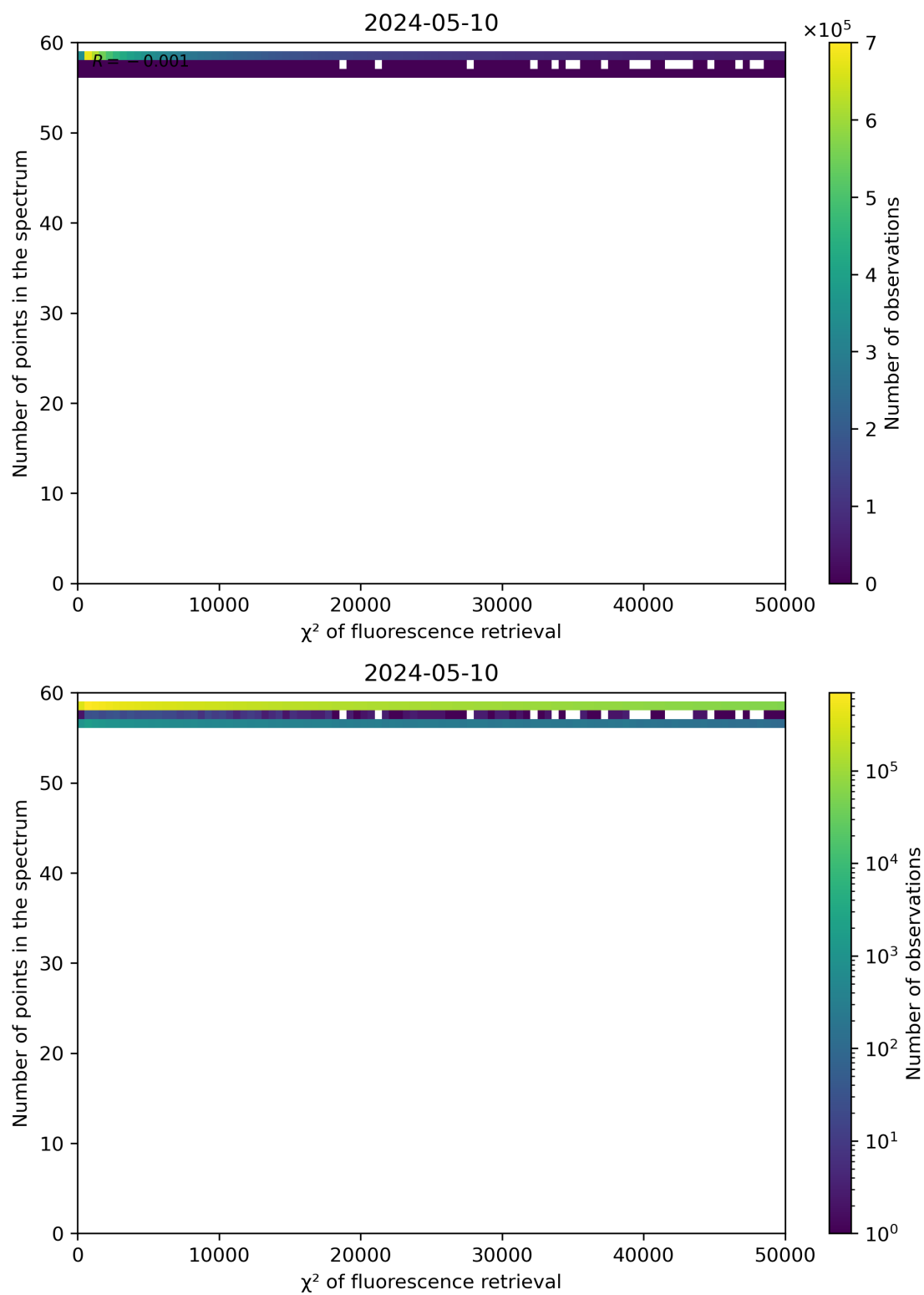
Figure 68: Scatter density plot of " \chi^2 of fluorescence retrieval" against "Number of points in the spectrum" for 2024-05-09 to 2024-05-11.
