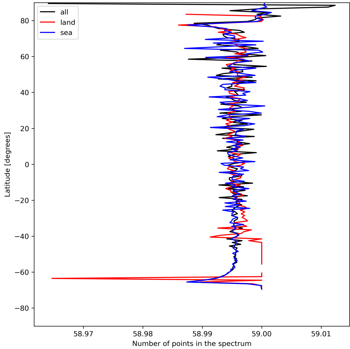
Figure 27: Zonal average of “Number of points in the spectrum” for 2024-05-09 to 2024-05-11.
