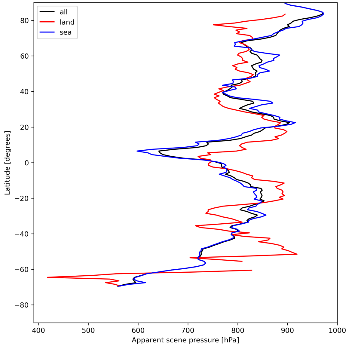
Figure 19: Zonal average of “Apparent scene pressure” for 2024-05-09 to 2024-05-11.
