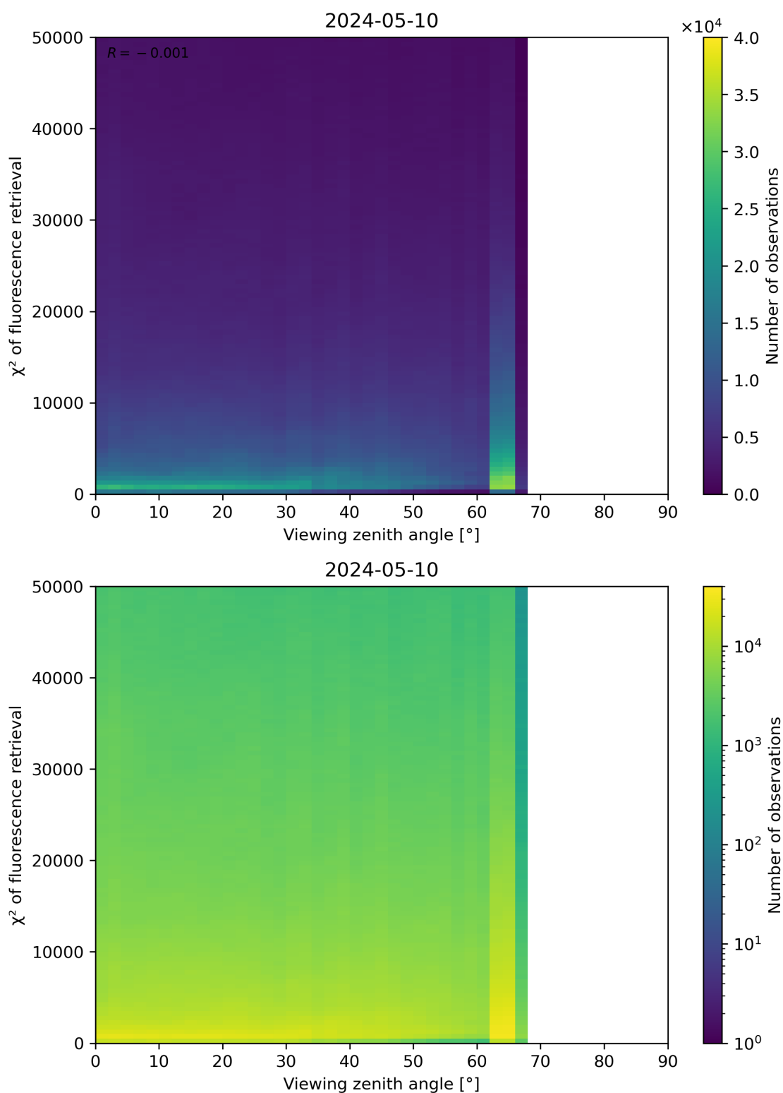
Figure 119: Scatter density plot of “Viewing zenith angle” against “ \chi^2 of fluorescence retrieval” for 2024-05-09 to 2024-05-11.
