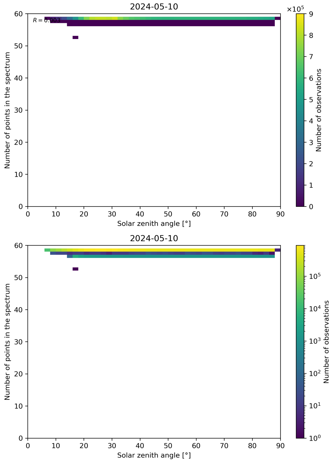
Figure 115: Scatter density plot of “Solar zenith angle” against “Number of points in the spectrum” for 2024-05-09 to 2024-05-11.
