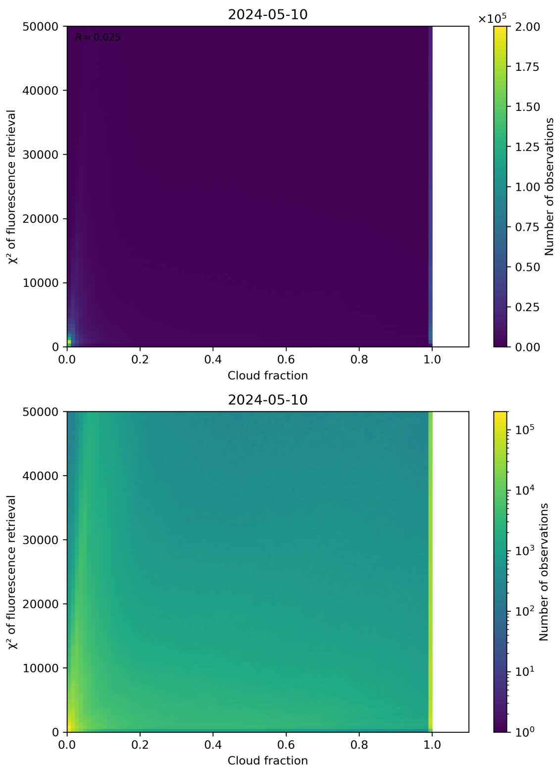
Figure 71: Scatter density plot of “Cloud fraction” against “ \chi^2 of fluorescence retrieval” for 2024-05-09 to 2024-05-11.
