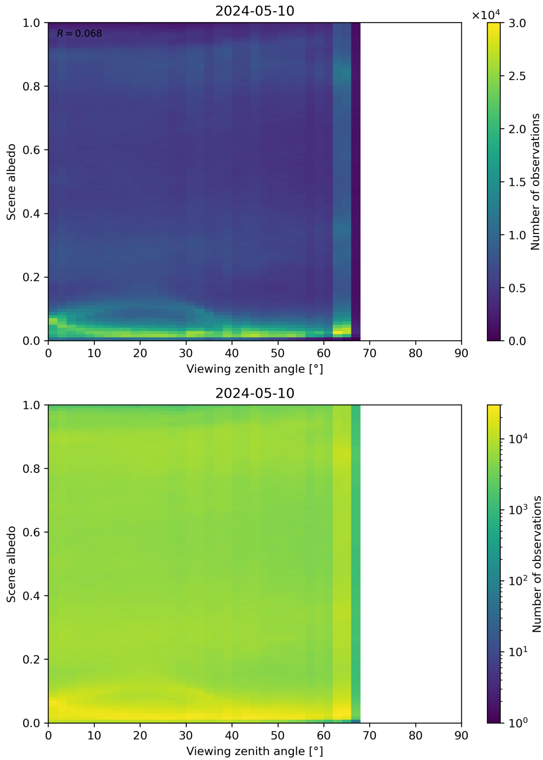
Figure 126: Scatter density plot of “Viewing zenith angle” against “Scene albedo” for 2024-05-09 to 2024-05-11.
