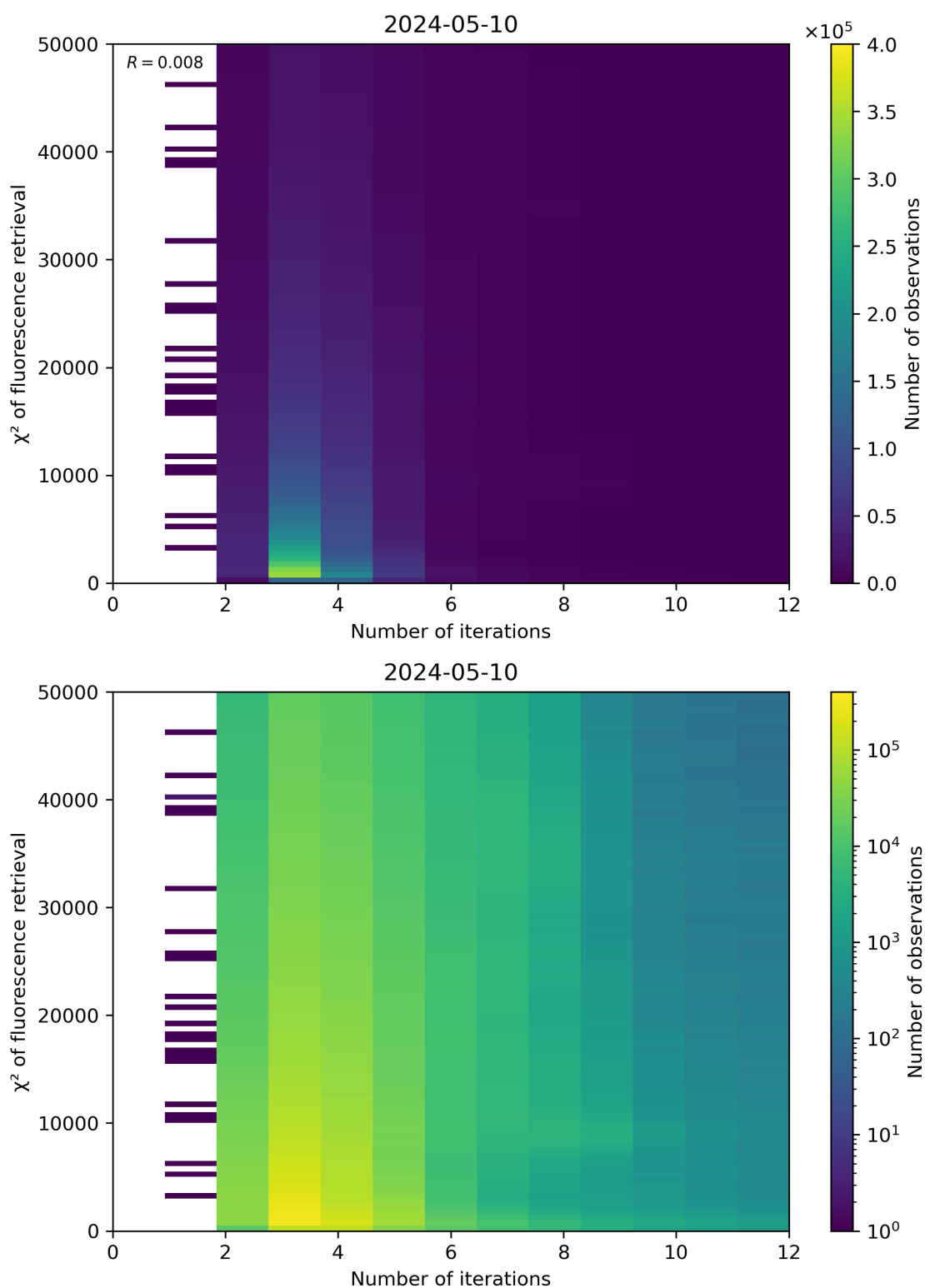
Figure 97: Scatter density plot of “Number of iterations” against “ \chi^2 of fluorescence retrieval” for 2024-05-09 to 2024-05-11.
