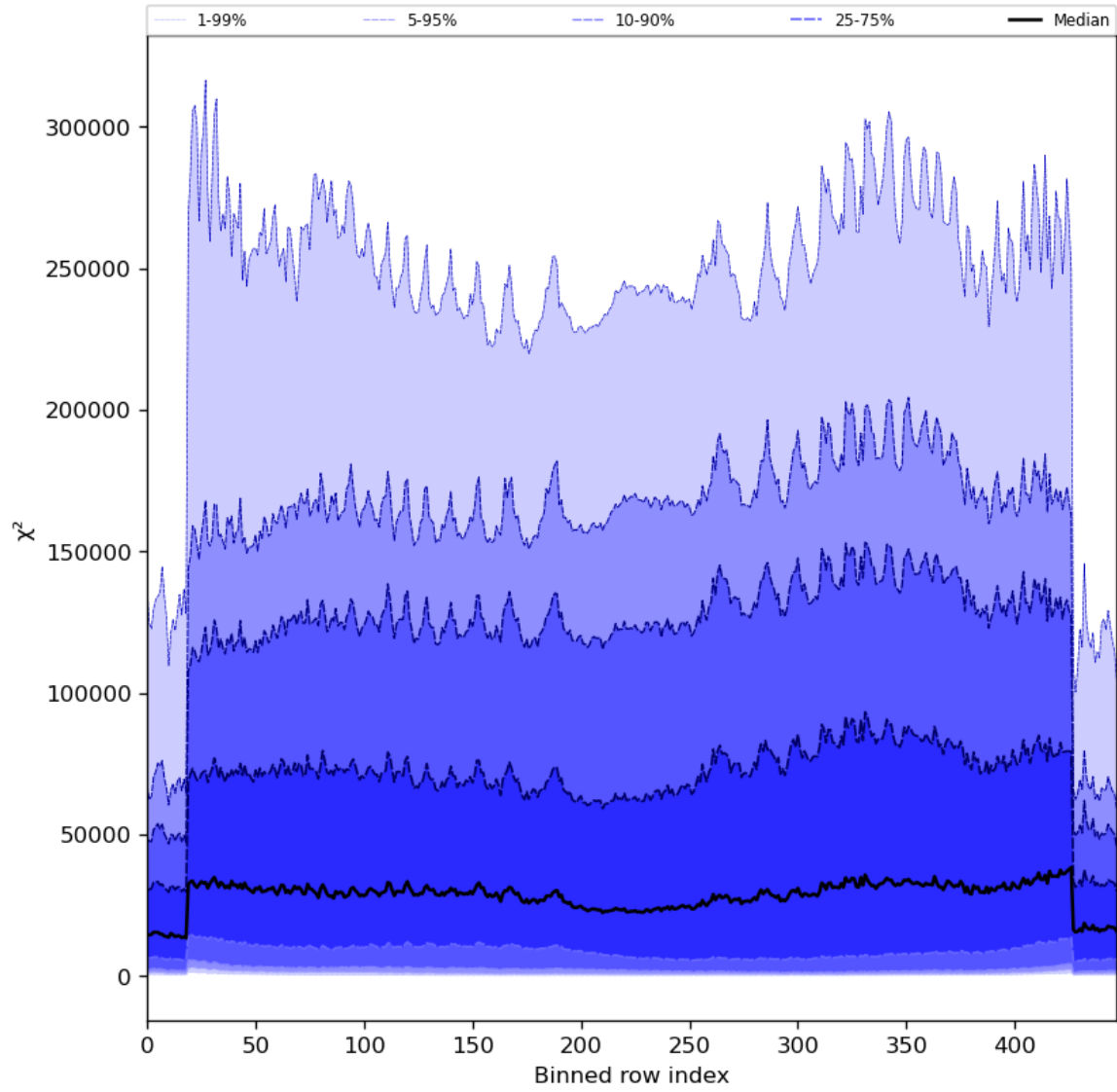
Figure 55: Along track statistics of “ \chi^2 ” for 2024-05-09 to 2024-05-11
