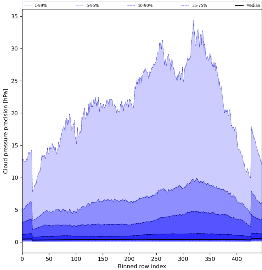
Figure 48: Along track statistics of “Cloud pressure precision” for 2024-05-09 to 2024-05-11
