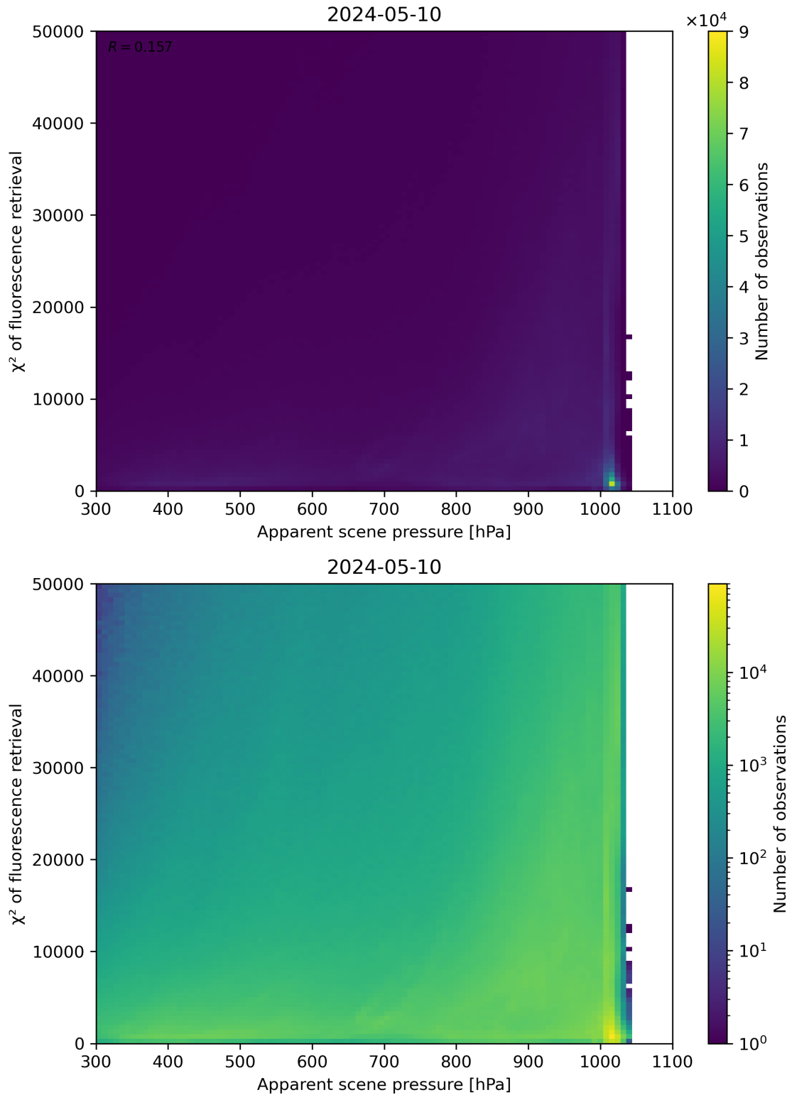
Figure 63: Scatter density plot of “Apparent scene pressure” against “ \chi^2 of fluorescence retrieval” for 2024-05-09 to 2024-05-11.
