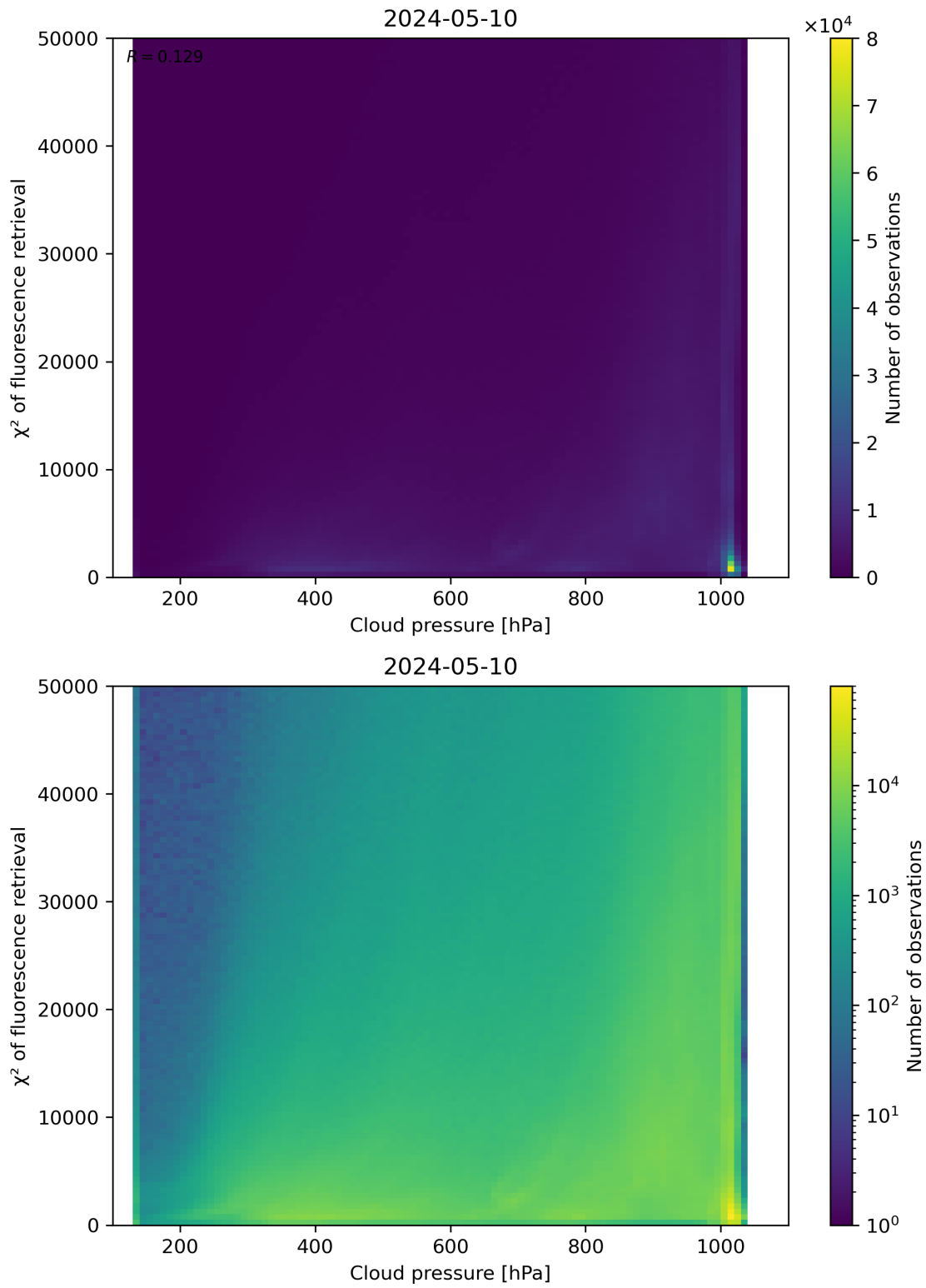
Figure 78: Scatter density plot of “Cloud pressure” against “ \chi^2 of fluorescence retrieval” for 2024-05-09 to 2024-05-11.
