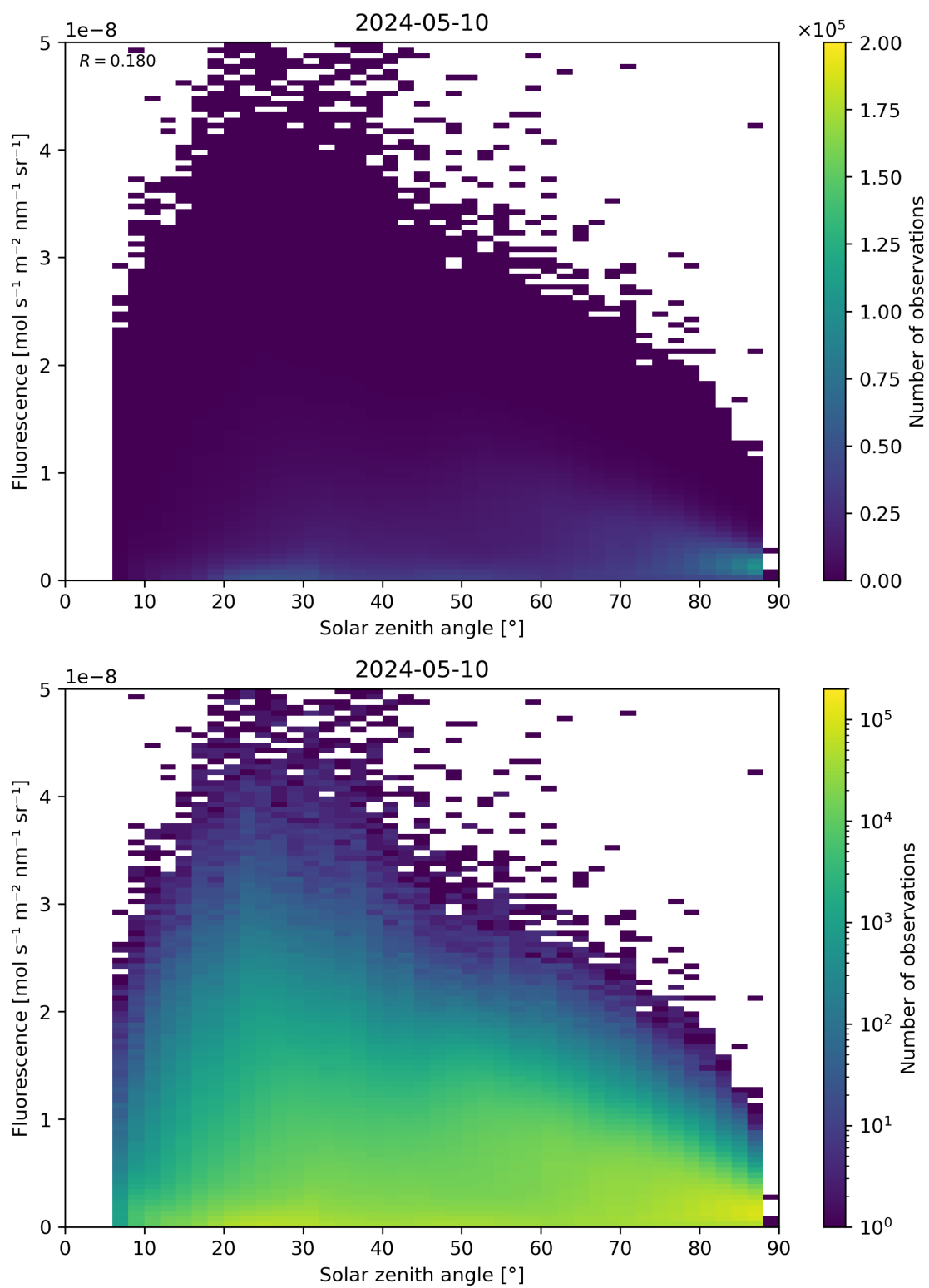
Figure 112: Scatter density plot of “Solar zenith angle” against “Fluorescence” for 2024-05-09 to 2024-05-11.
