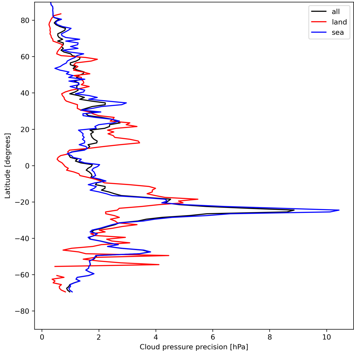
Figure 14: Zonal average of “Cloud pressure precision” for 2024-05-09 to 2024-05-11.
