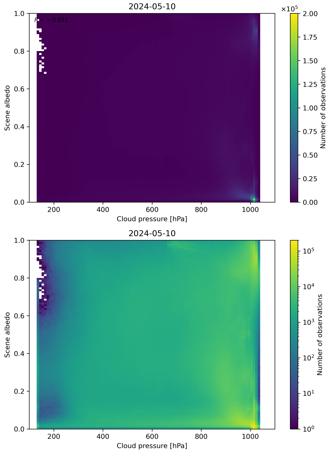
Figure 83: Scatter density plot of “Cloud pressure” against “Scene albedo” for 2024-05-09 to 2024-05-11.
