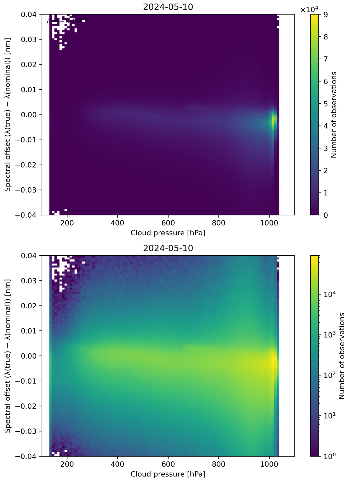
Figure 84: Scatter density plot of “Cloud pressure” against “Spectral offset ( \lambda(\text{true}) - \lambda(\text{nominal}) )” for 2024-05-09 to 2024-05-11.
