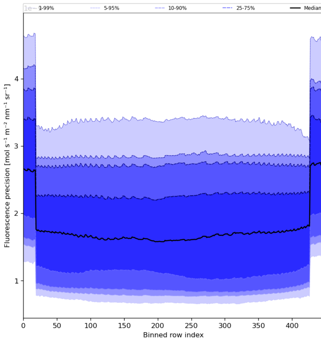
Figure 58: Along track statistics of “Fluorescence precision” for 2024-05-09 to 2024-05-11
