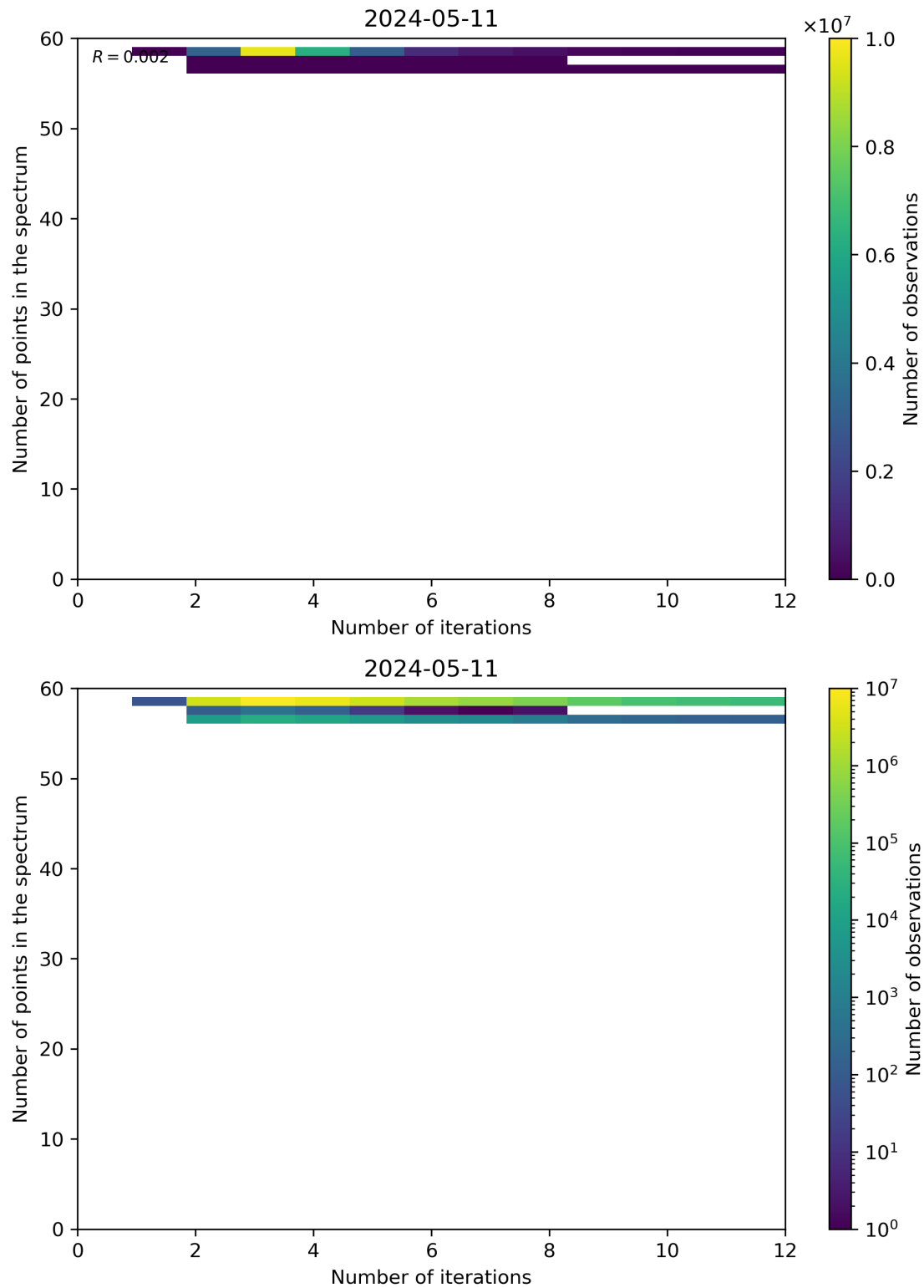
Figure 99: Scatter density plot of “Number of iterations” against “Number of points in the spectrum” for 2024-05-10 to 2024-05-12.
