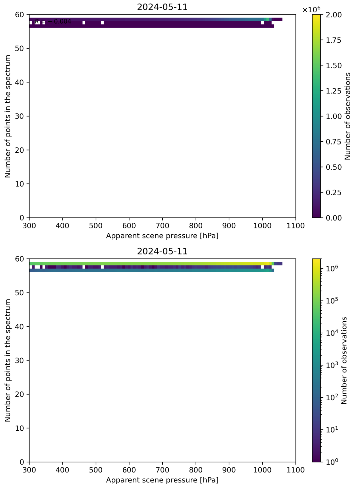
Figure 66: Scatter density plot of “Apparent scene pressure” against “Number of points in the spectrum” for 2024-05-10 to 2024-05-12.
