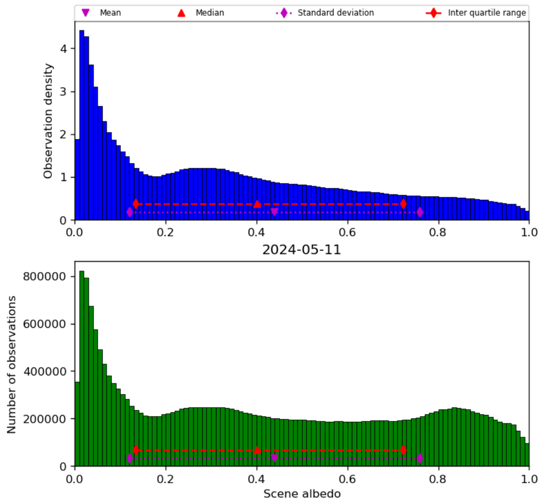
Figure 34: Histogram of “Scene albedo” for 2024-05-10 to 2024-05-12
