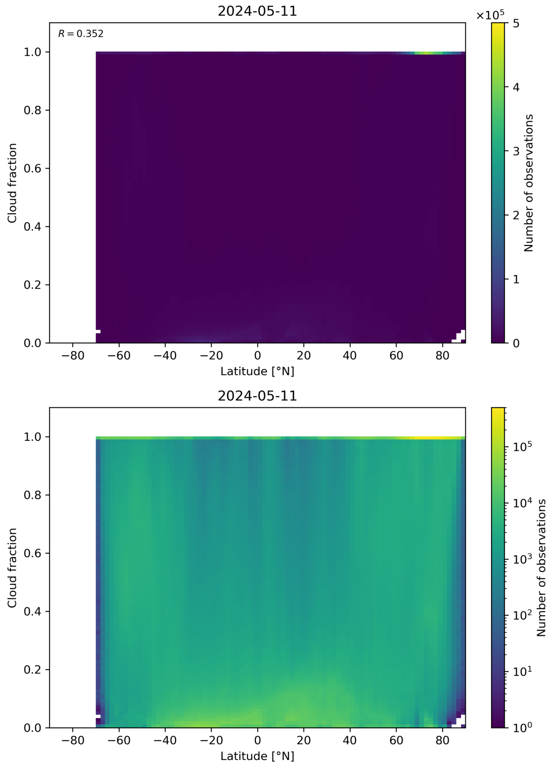
Figure 90: Scatter density plot of “Latitude” against “Cloud fraction” for 2024-05-10 to 2024-05-12.
