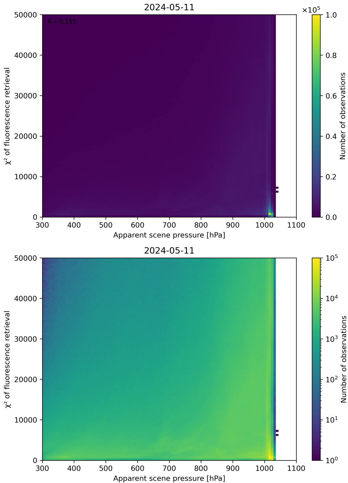
Figure 63: Scatter density plot of “Apparent scene pressure” against “ \chi^2 of fluorescence retrieval” for 2024-05-10 to 2024-05-12.
