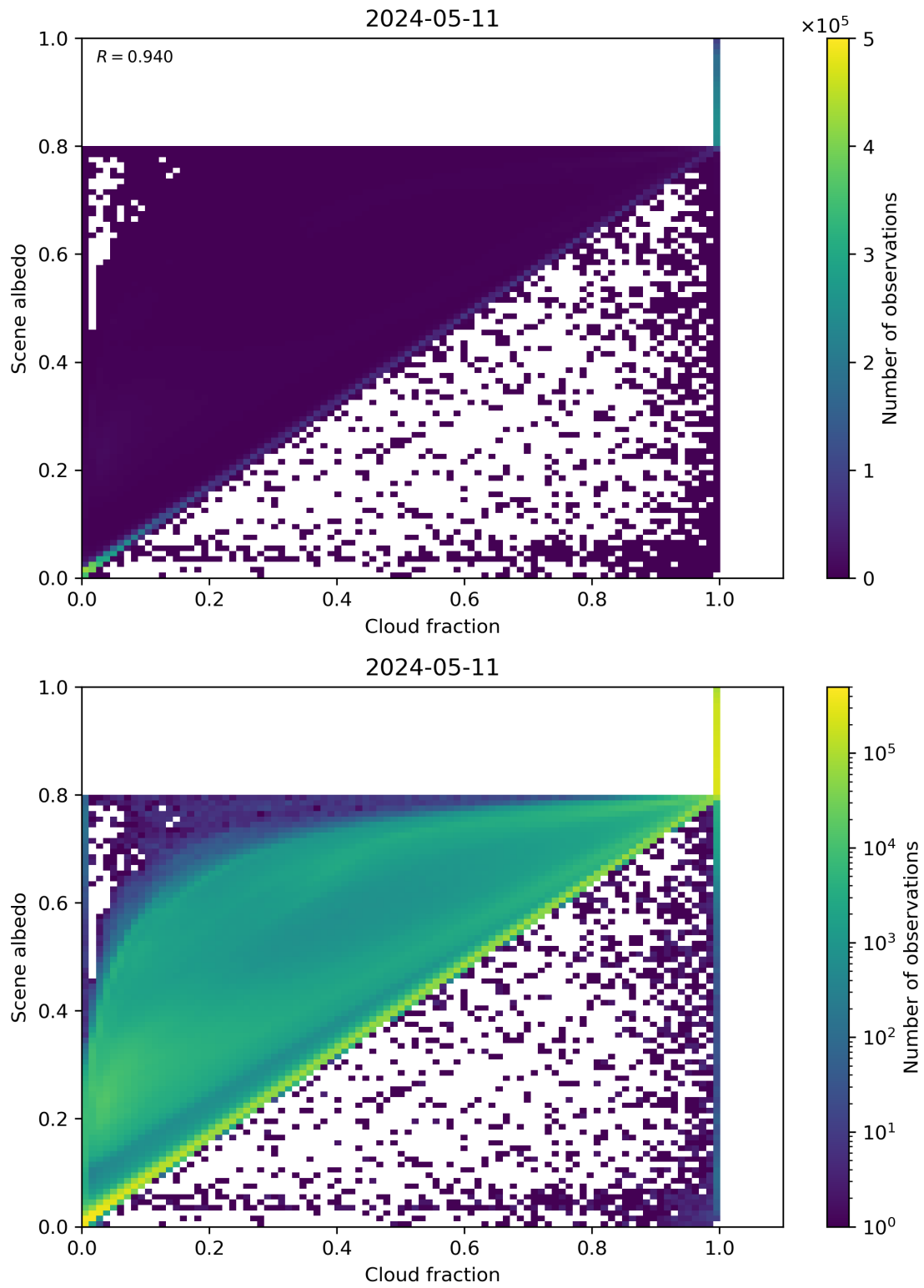
Figure 75: Scatter density plot of “Cloud fraction” against “Scene albedo” for 2024-05-10 to 2024-05-12.
