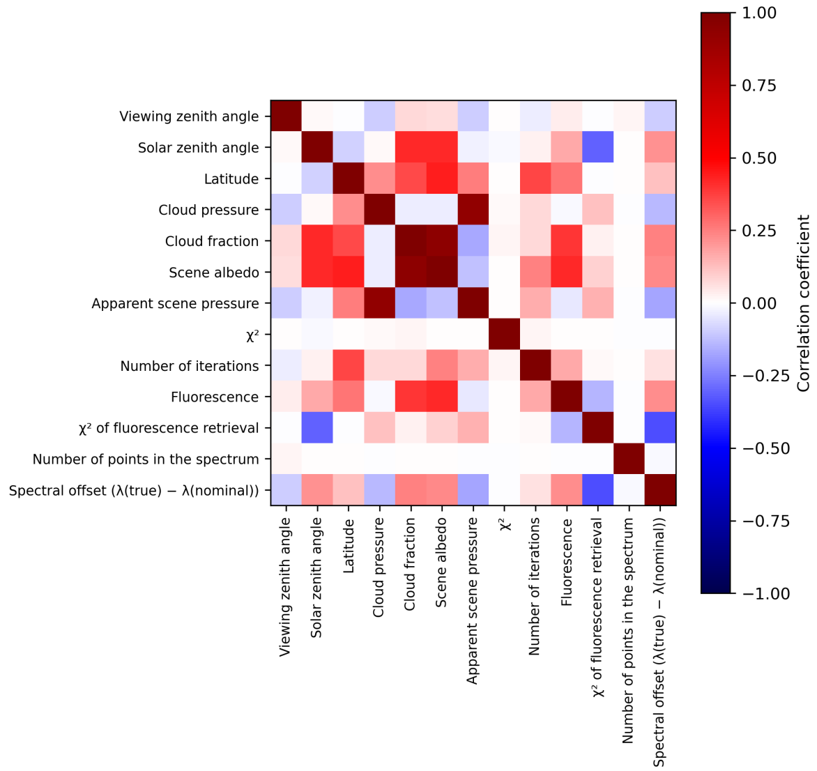
Figure 2: Map of correlation matrix for 2024-05-10 to 2024-05-12.
