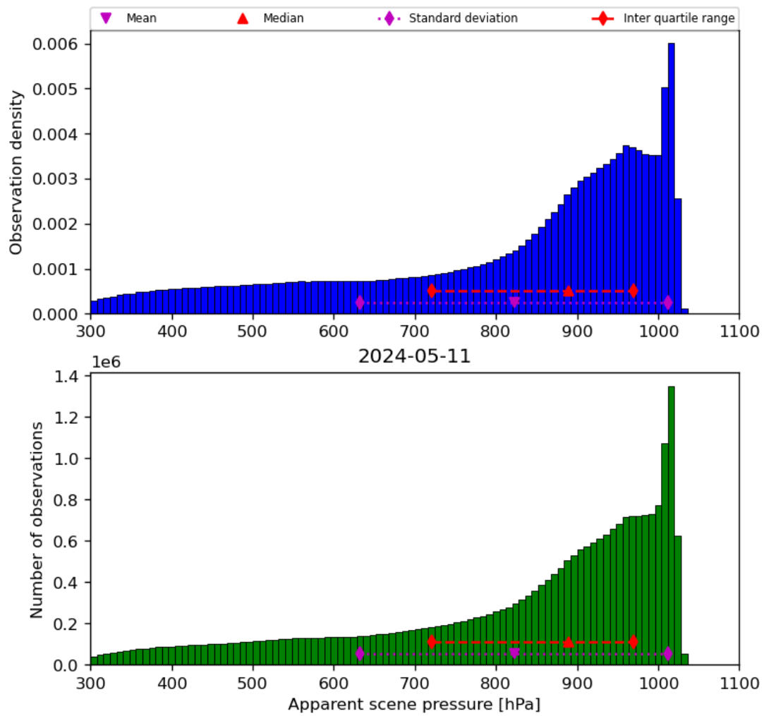
Figure 36: Histogram of “Apparent scene pressure” for 2024-05-10 to 2024-05-12
