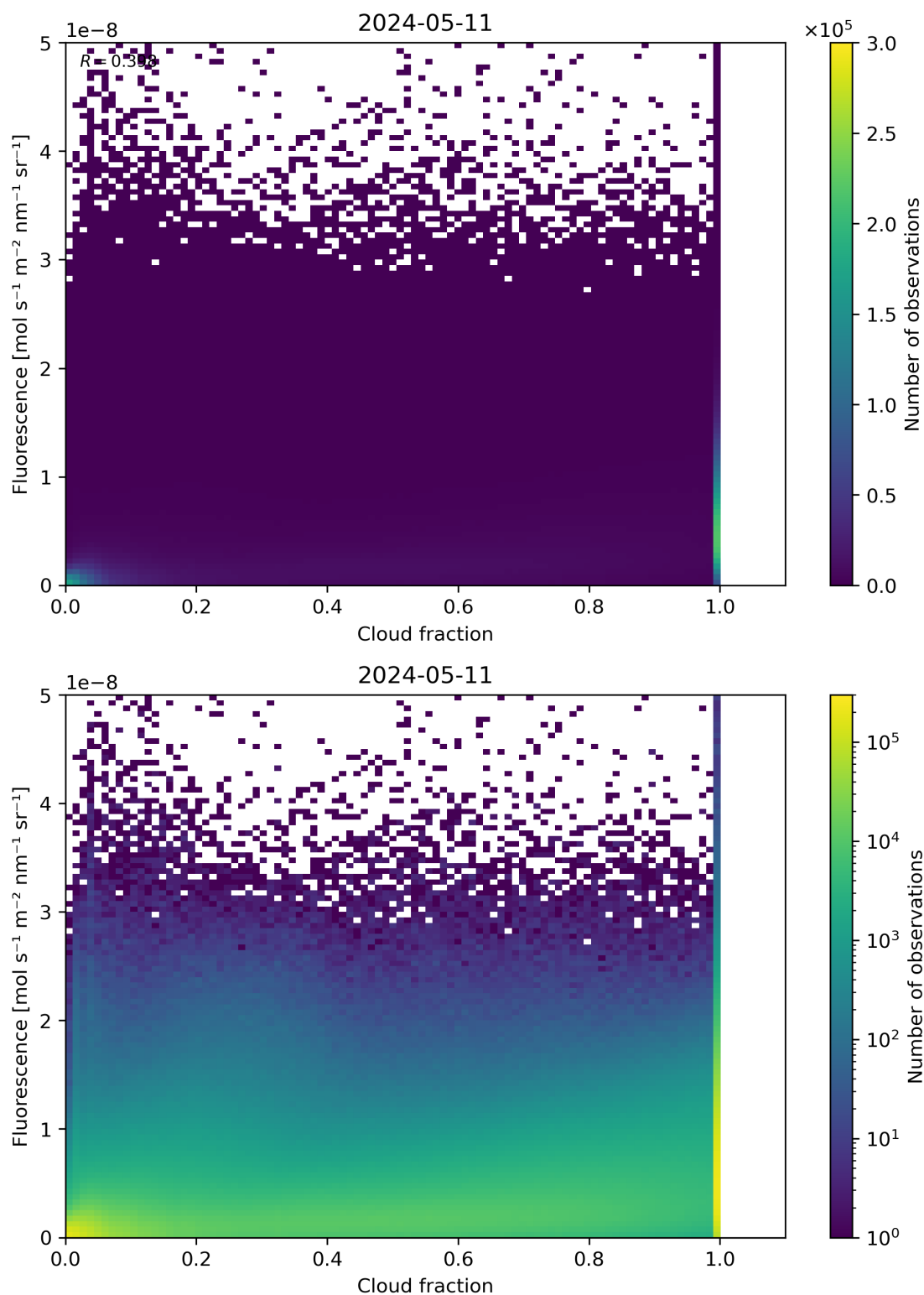
Figure 72: Scatter density plot of “Cloud fraction” against “Fluorescence” for 2024-05-10 to 2024-05-12.
