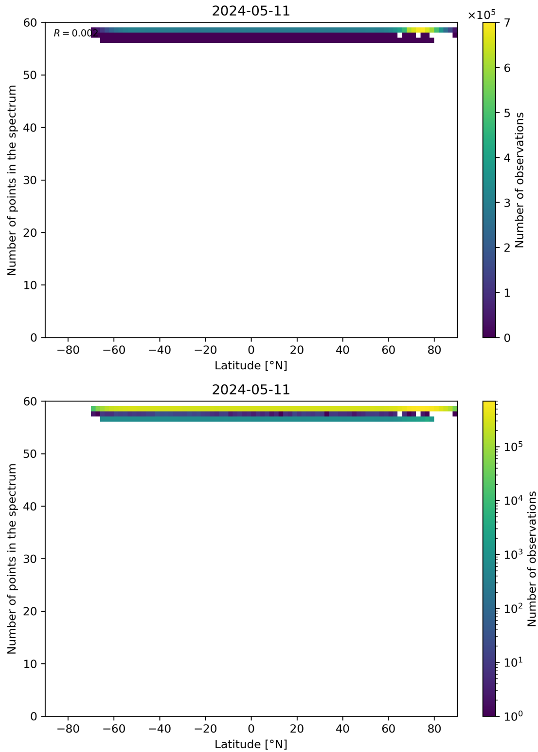
Figure 94: Scatter density plot of “Latitude” against “Number of points in the spectrum” for 2024-05-10 to 2024-05-12.
