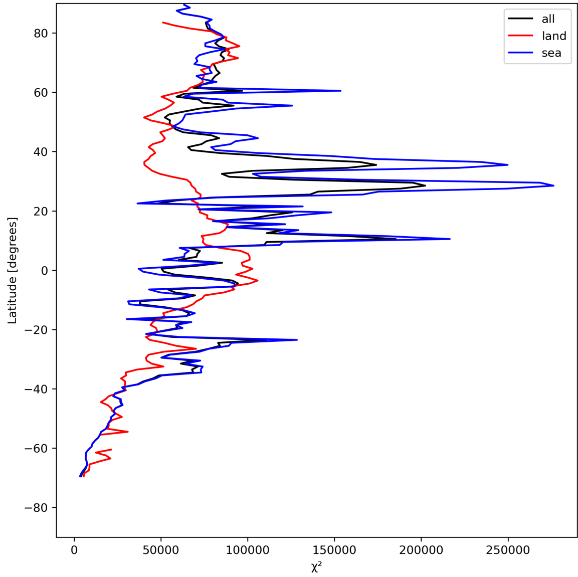
Figure 21: Zonal average of “ \chi^2 ” for 2024-05-10 to 2024-05-12.
