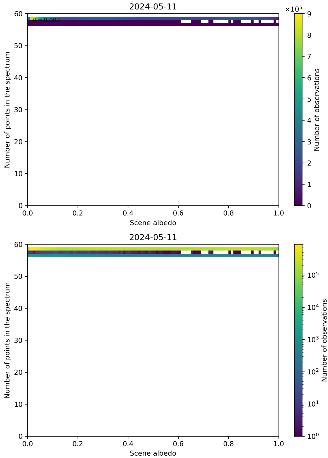
Figure 106: Scatter density plot of “Scene albedo” against “Number of points in the spectrum” for 2024-05-10 to 2024-05-12.
