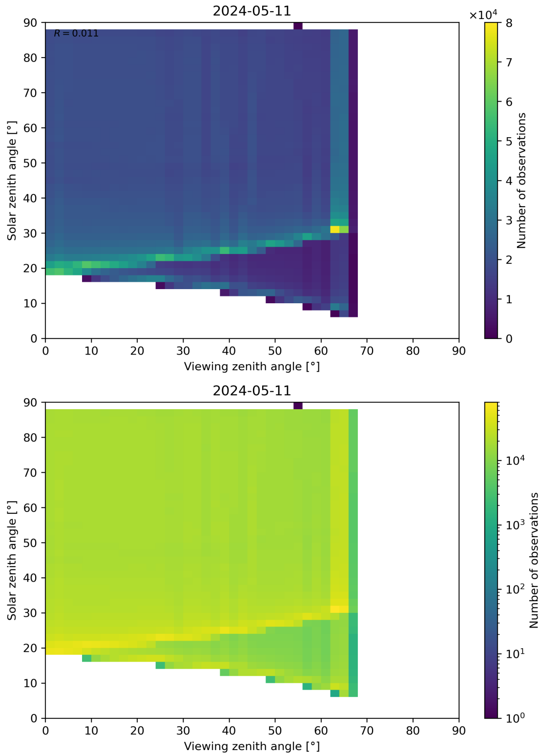
Figure 127: Scatter density plot of “Viewing zenith angle” against “Solar zenith angle” for 2024-05-10 to 2024-05-12.
