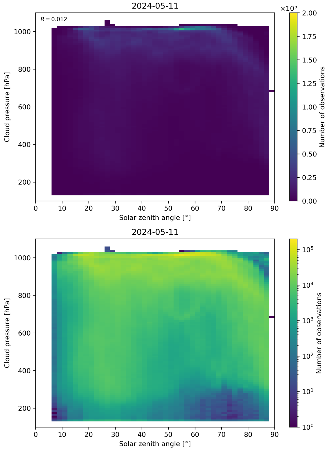
Figure 111: Scatter density plot of “Solar zenith angle” against “Cloud pressure” for 2024-05-10 to 2024-05-12.
