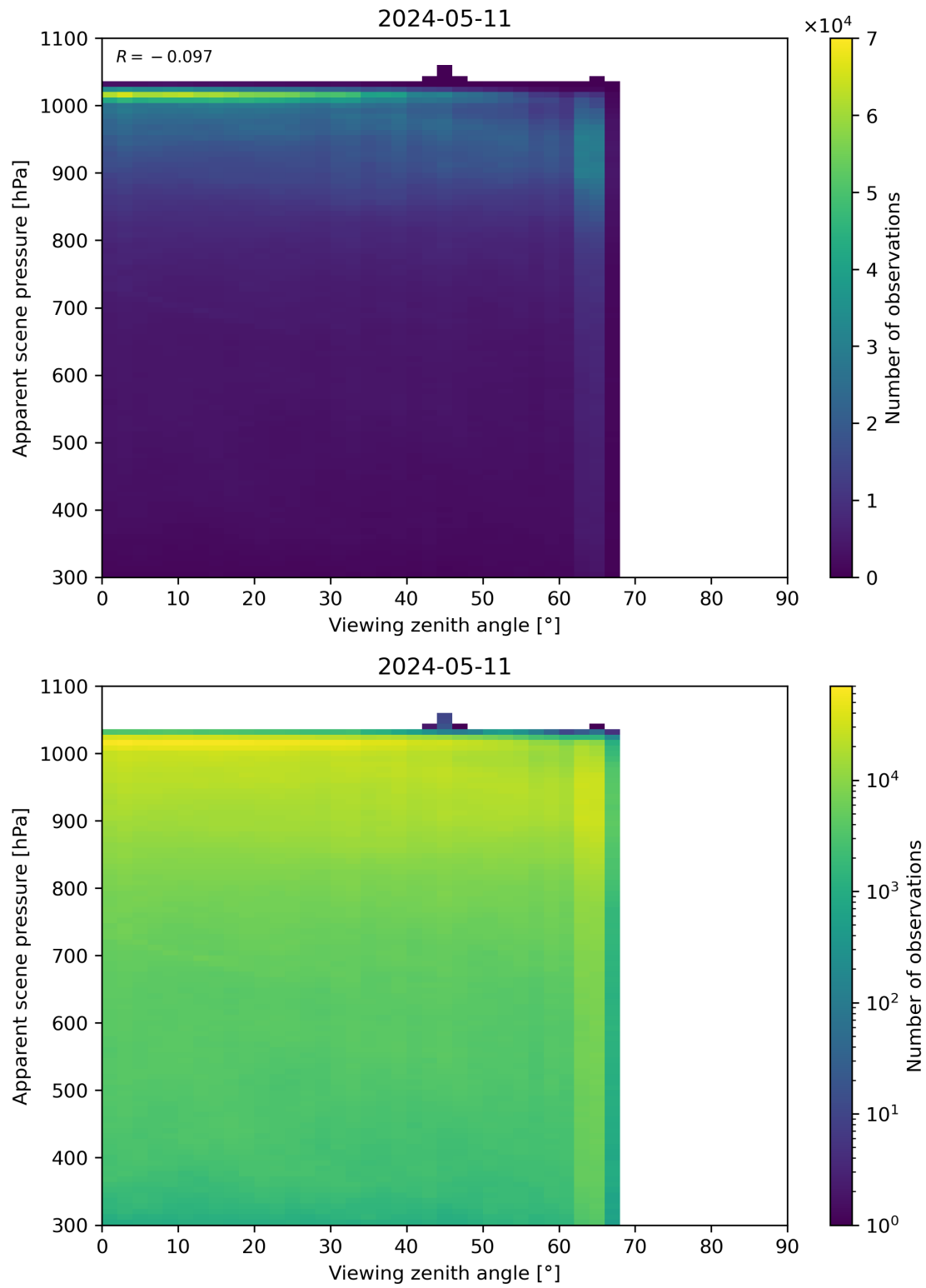
Figure 118: Scatter density plot of “Viewing zenith angle” against “Apparent scene pressure” for 2024-05-10 to 2024-05-12.
