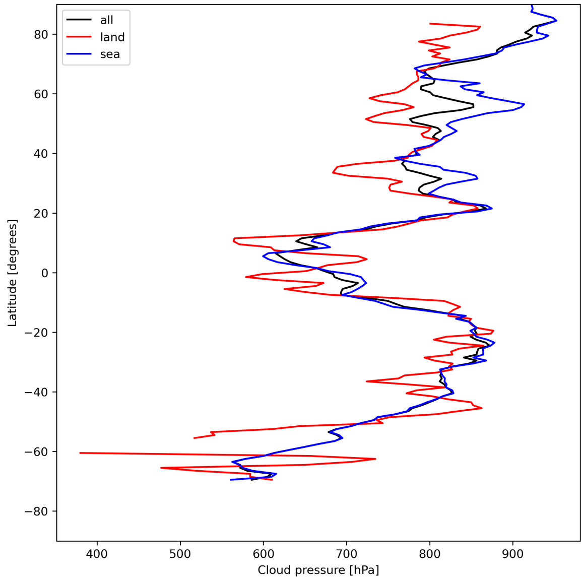
Figure 13: Zonal average of “Cloud pressure” for 2024-05-10 to 2024-05-12.
