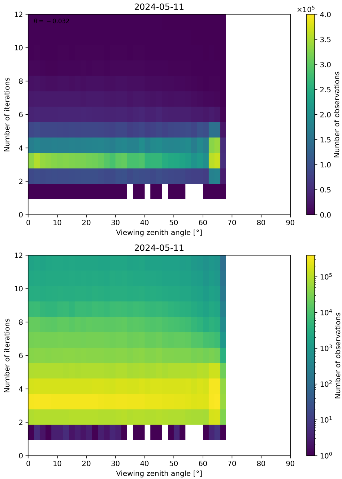
Figure 124: Scatter density plot of “Viewing zenith angle” against “Number of iterations” for 2024-05-10 to 2024-05-12.
