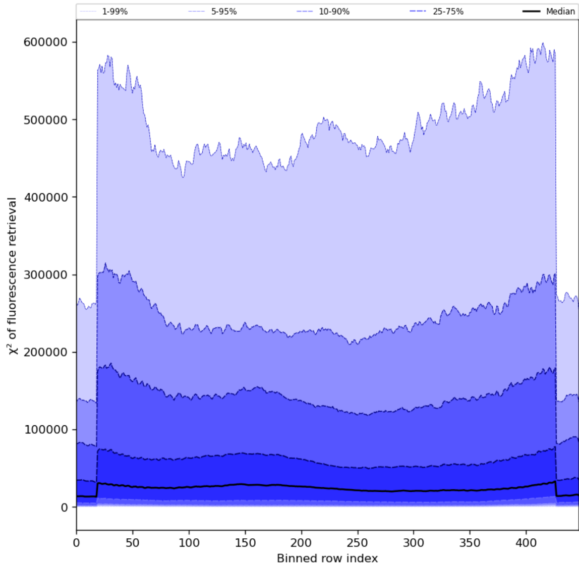
Figure 59: Along track statistics of “ \chi^2 of fluorescence retrieval” for 2024-05-10 to 2024-05-12
