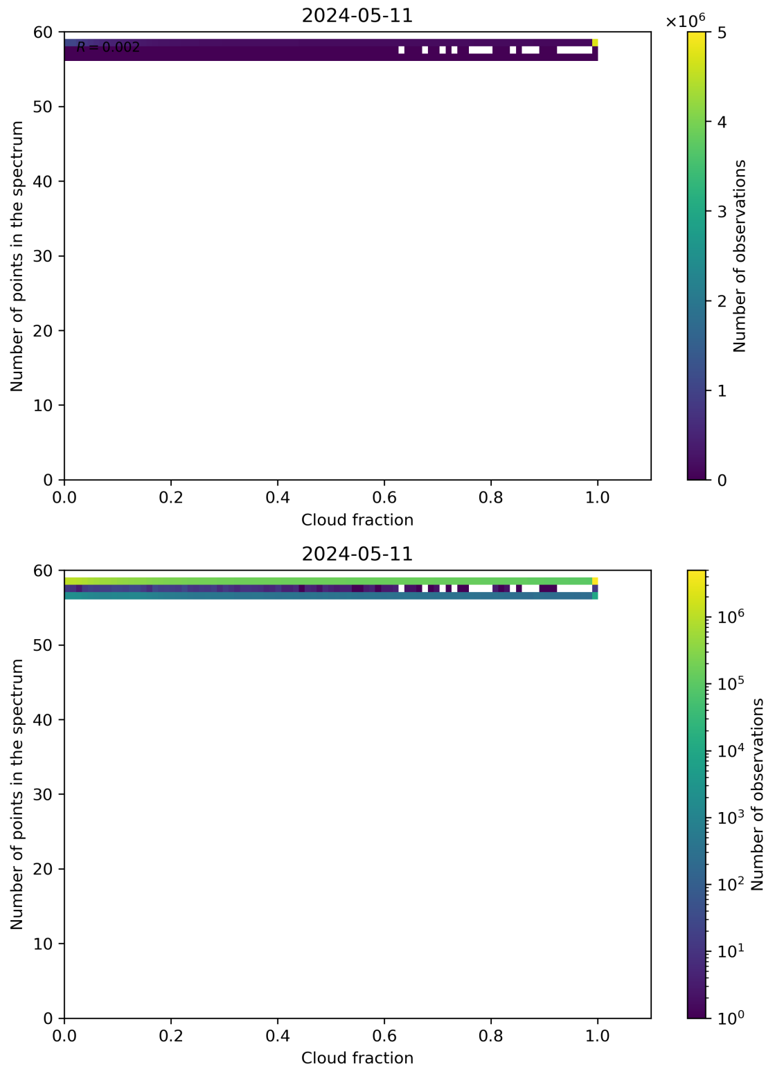
Figure 74: Scatter density plot of “Cloud fraction” against “Number of points in the spectrum” for 2024-05-10 to 2024-05-12.
