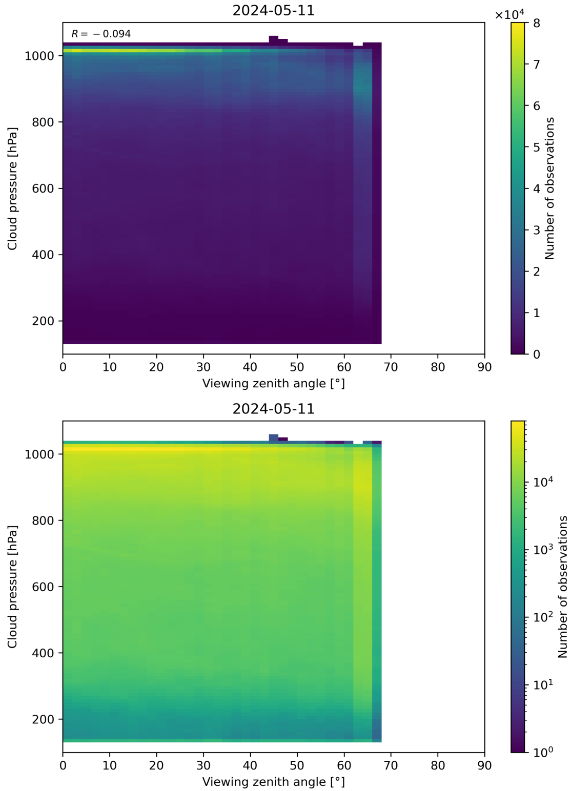
Figure 121: Scatter density plot of “Viewing zenith angle” against “Cloud pressure” for 2024-05-10 to 2024-05-12.
