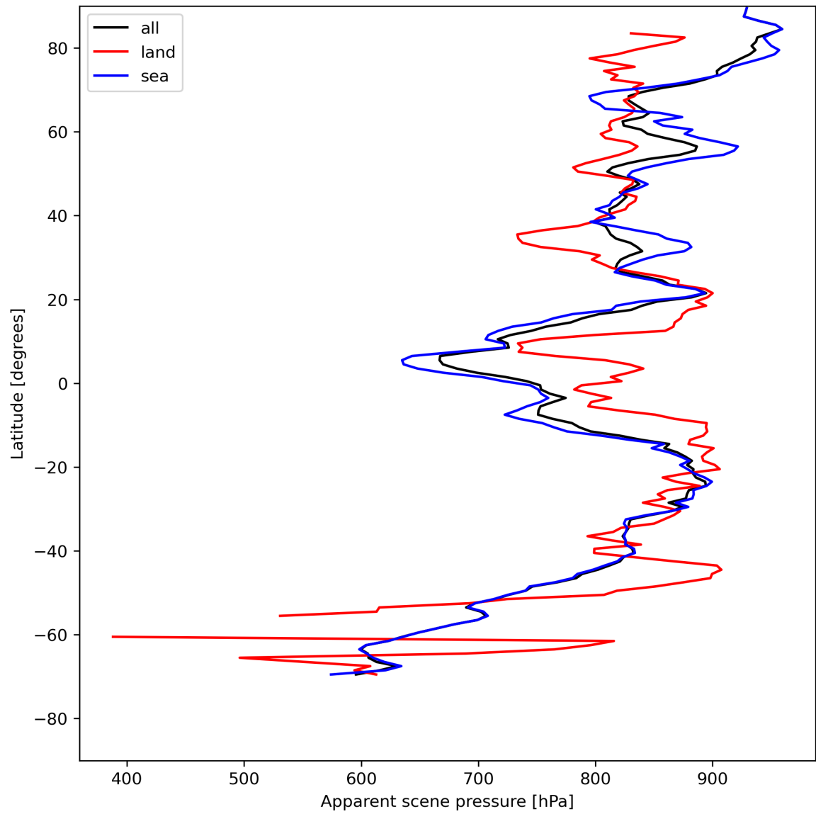
Figure 19: Zonal average of “Apparent scene pressure” for 2024-05-10 to 2024-05-12.
