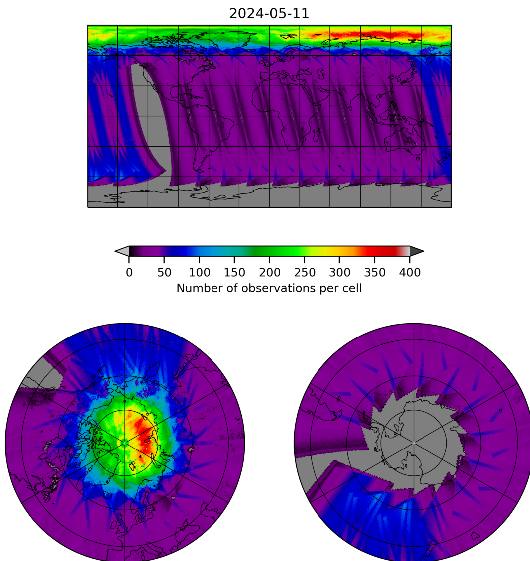
Figure 11: Map of the number of observations for 2024-05-10 to 2024-05-12
