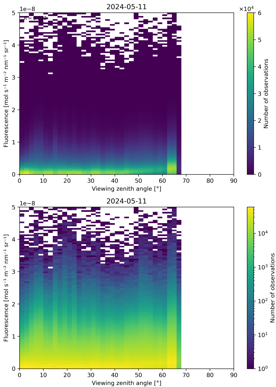
Figure 122: Scatter density plot of “Viewing zenith angle” against “Fluorescence” for 2024-05-10 to 2024-05-12.
