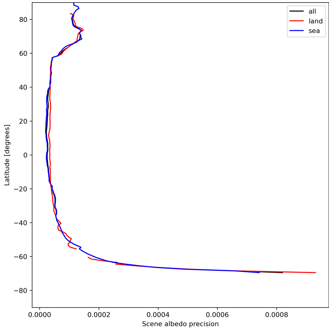
Figure 18: Zonal average of “Scene albedo precision” for 2024-05-10 to 2024-05-12.
