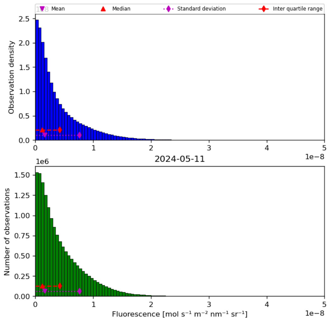
Figure 40: Histogram of “Fluorescence” for 2024-05-10 to 2024-05-12
