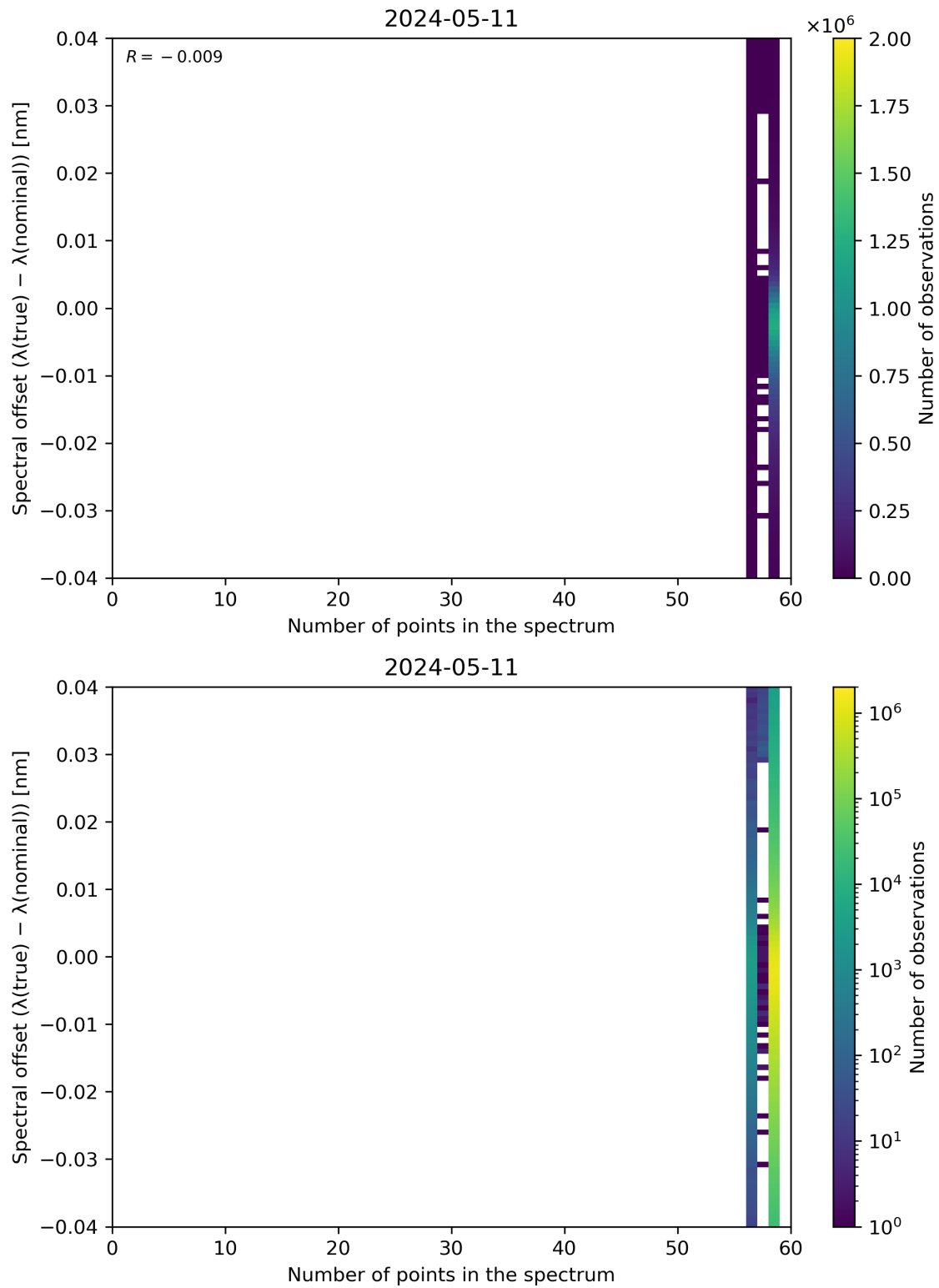
Figure 101: Scatter density plot of “Number of points in the spectrum” against “Spectral offset ( \lambda(\text{true}) - \lambda(\text{nominal}) )” for 2024-05-10 to 2024-05-12.
