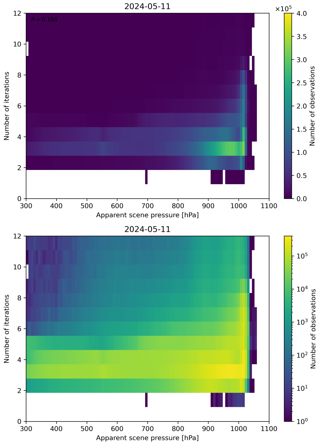
Figure 65: Scatter density plot of “Apparent scene pressure” against “Number of iterations” for 2024-05-10 to 2024-05-12.
