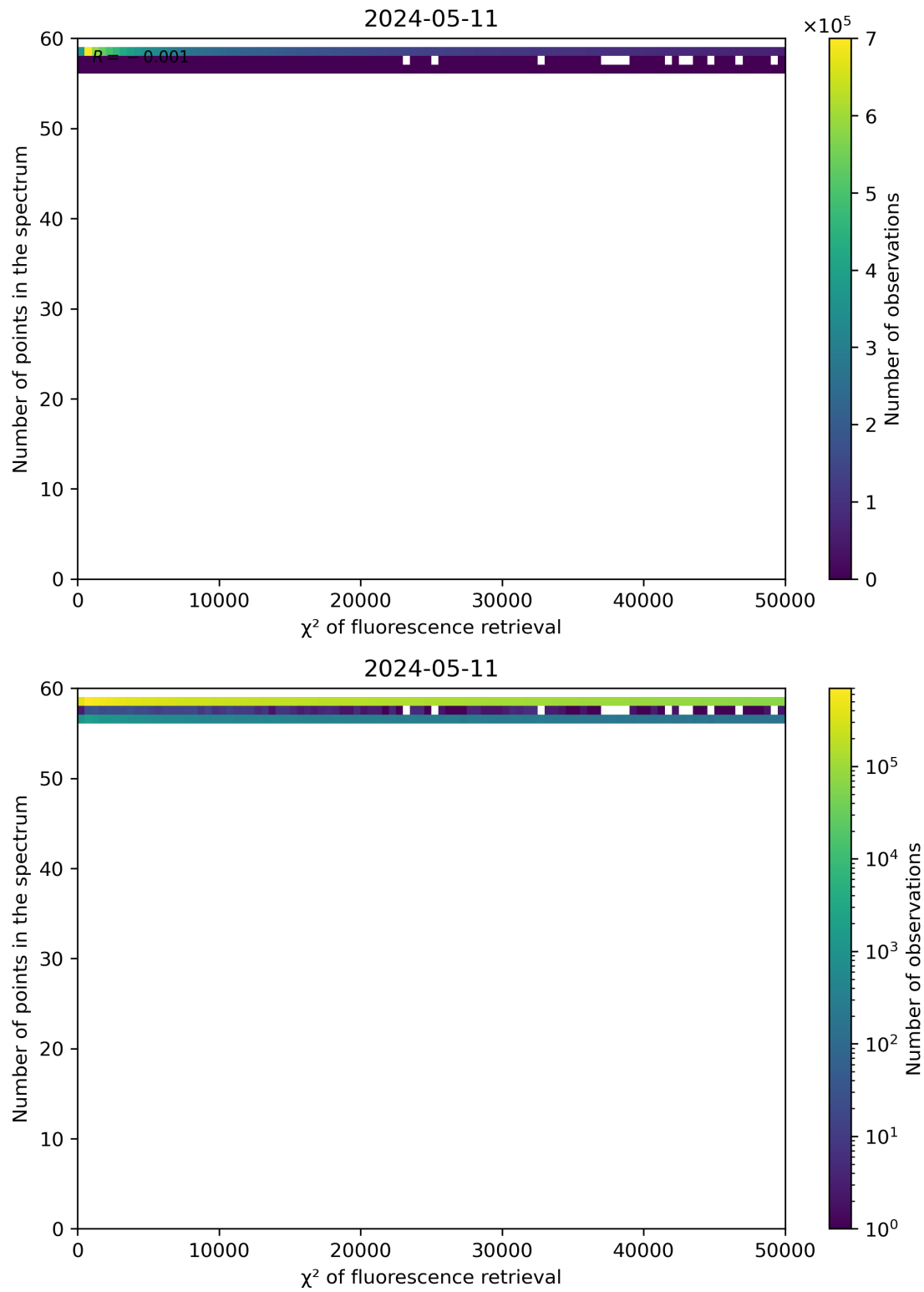
Figure 68: Scatter density plot of " \chi^2 of fluorescence retrieval" against "Number of points in the spectrum" for 2024-05-10 to 2024-05-12.
