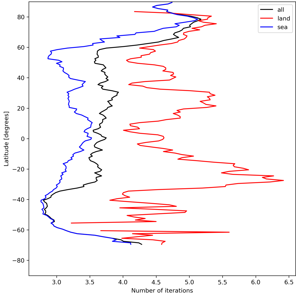
Figure 22: Zonal average of “Number of iterations” for 2024-05-10 to 2024-05-12.
