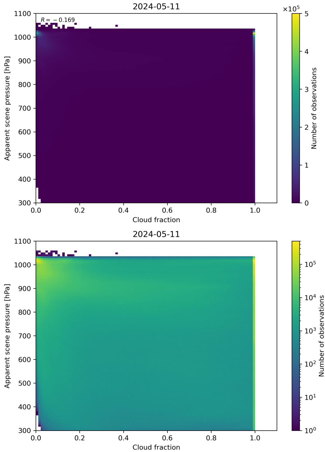
Figure 70: Scatter density plot of “Cloud fraction” against “Apparent scene pressure” for 2024-05-10 to 2024-05-12.
