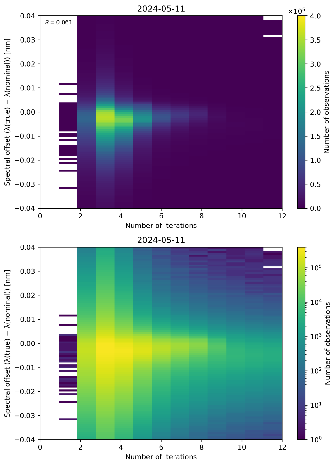
Figure 100: Scatter density plot of “Number of iterations” against “Spectral offset ( \lambda(\text{true}) - \lambda(\text{nominal}) )” for 2024-05-10 to 2024-05-12.
