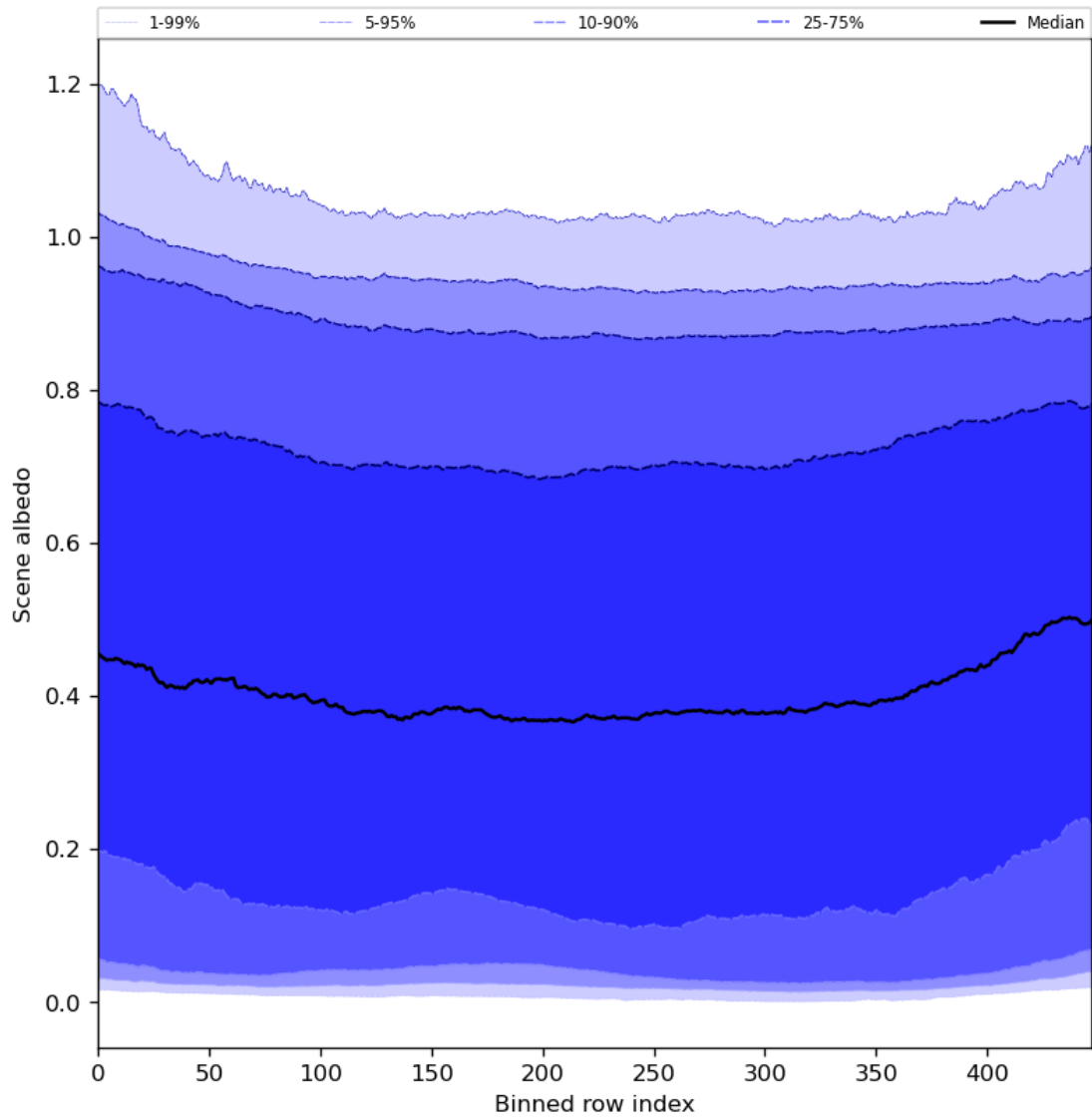
Figure 51: Along track statistics of “Scene albedo” for 2024-05-10 to 2024-05-12
