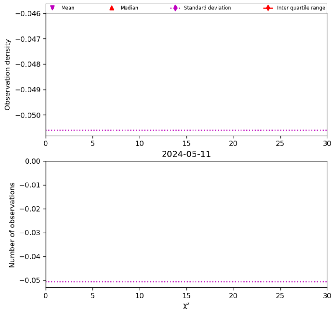
Figure 38: Histogram of “ \chi^2 ” for 2024-05-10 to 2024-05-12
