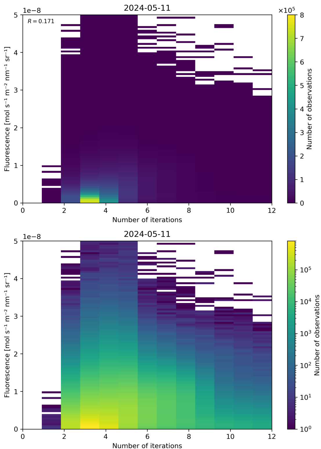
Figure 98: Scatter density plot of “Number of iterations” against “Fluorescence” for 2024-05-10 to 2024-05-12.
