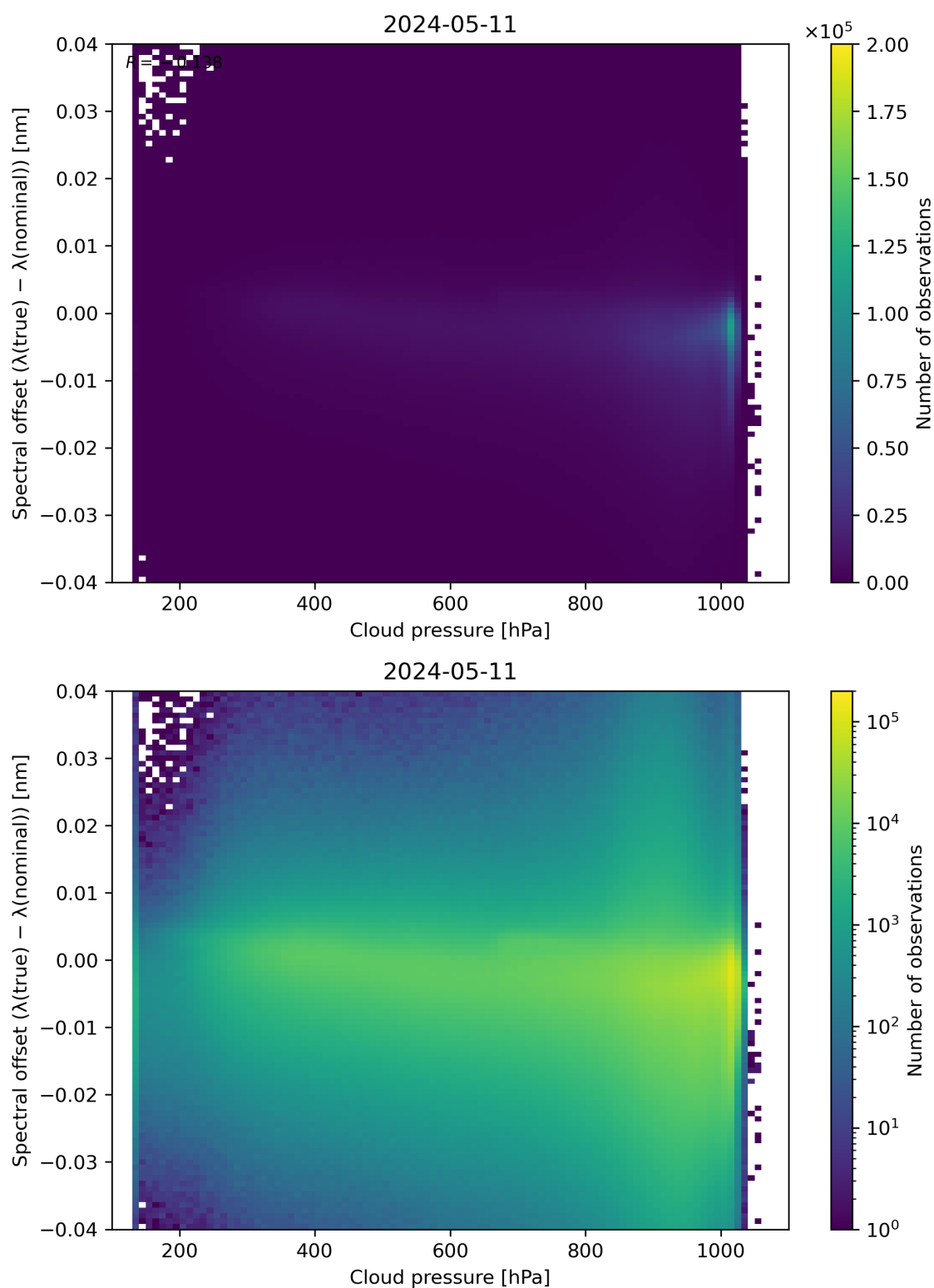
Figure 84: Scatter density plot of “Cloud pressure” against “Spectral offset ( \lambda(\text{true}) - \lambda(\text{nominal}) )” for 2024-05-10 to 2024-05-12.
