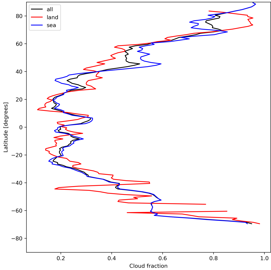
Figure 15: Zonal average of “Cloud fraction” for 2024-05-10 to 2024-05-12.
