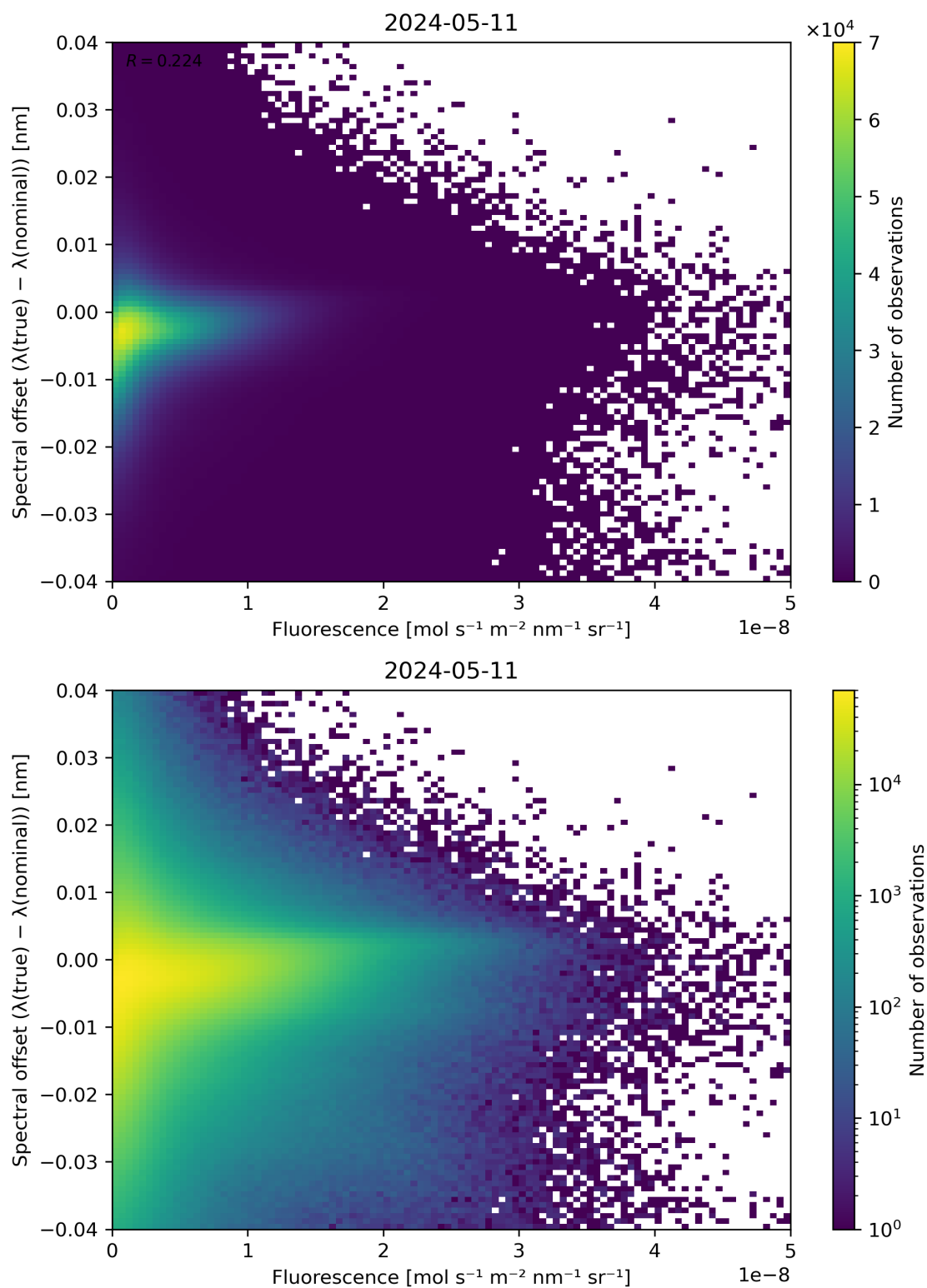
Figure 87: Scatter density plot of “Fluorescence” against “Spectral offset ( \lambda(\text{true}) - \lambda(\text{nominal}) )” for 2024-05-10 to 2024-05-12.
