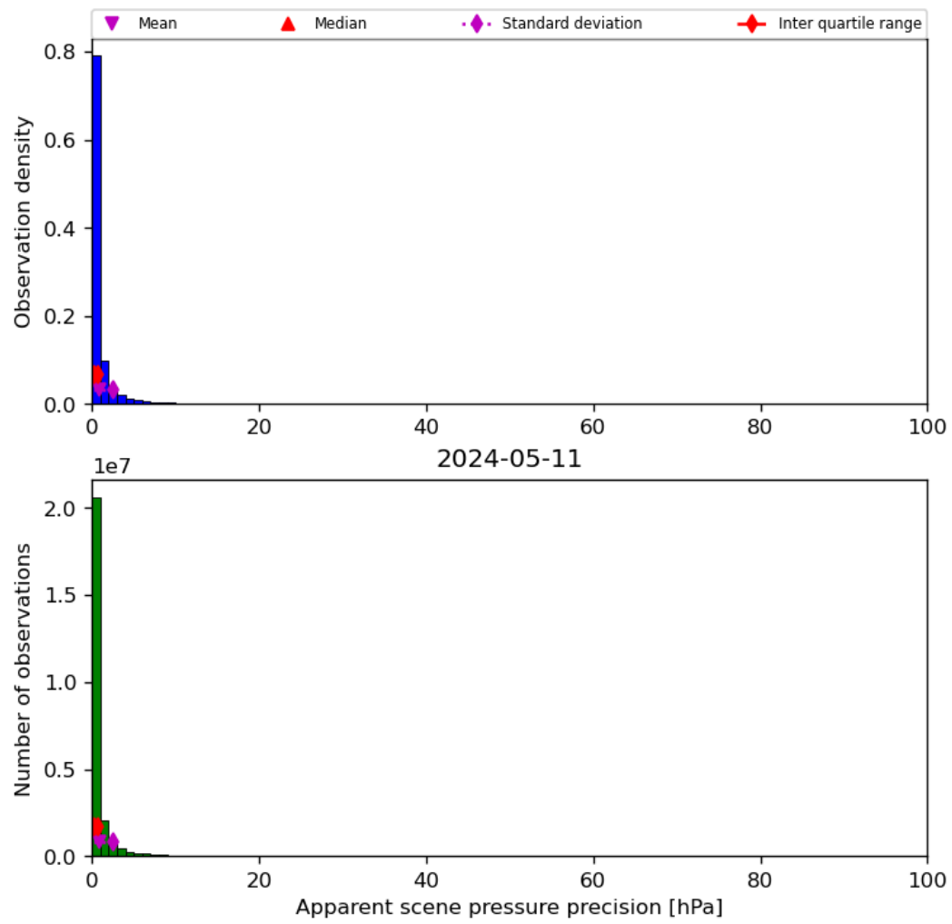
Figure 37: Histogram of “Apparent scene pressure precision” for 2024-05-10 to 2024-05-12
