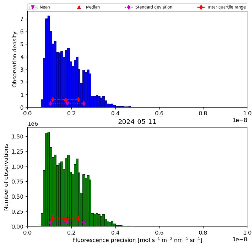
Figure 41: Histogram of “Fluorescence precision” for 2024-05-10 to 2024-05-12
