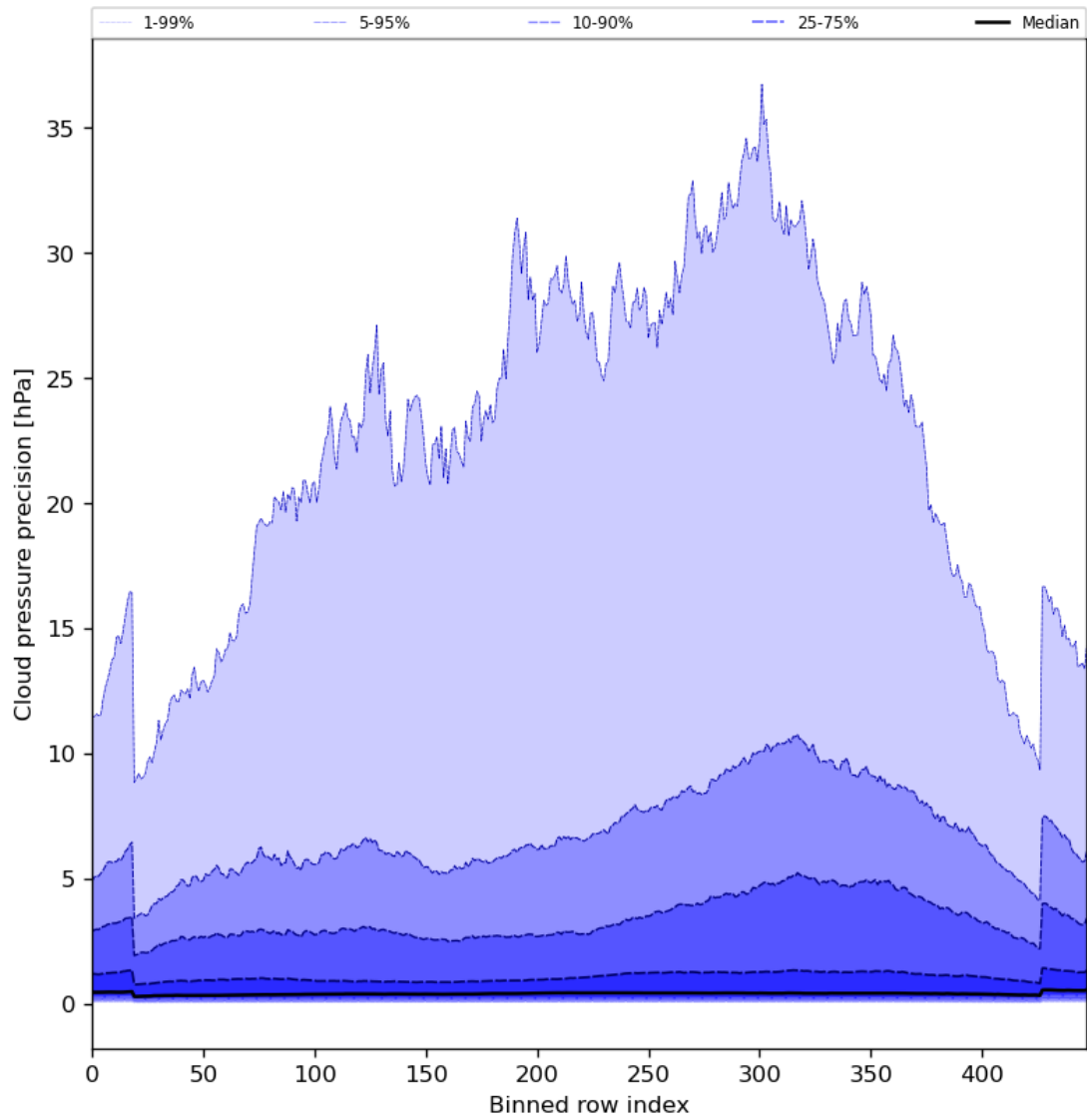
Figure 48: Along track statistics of “Cloud pressure precision” for 2024-05-10 to 2024-05-12
