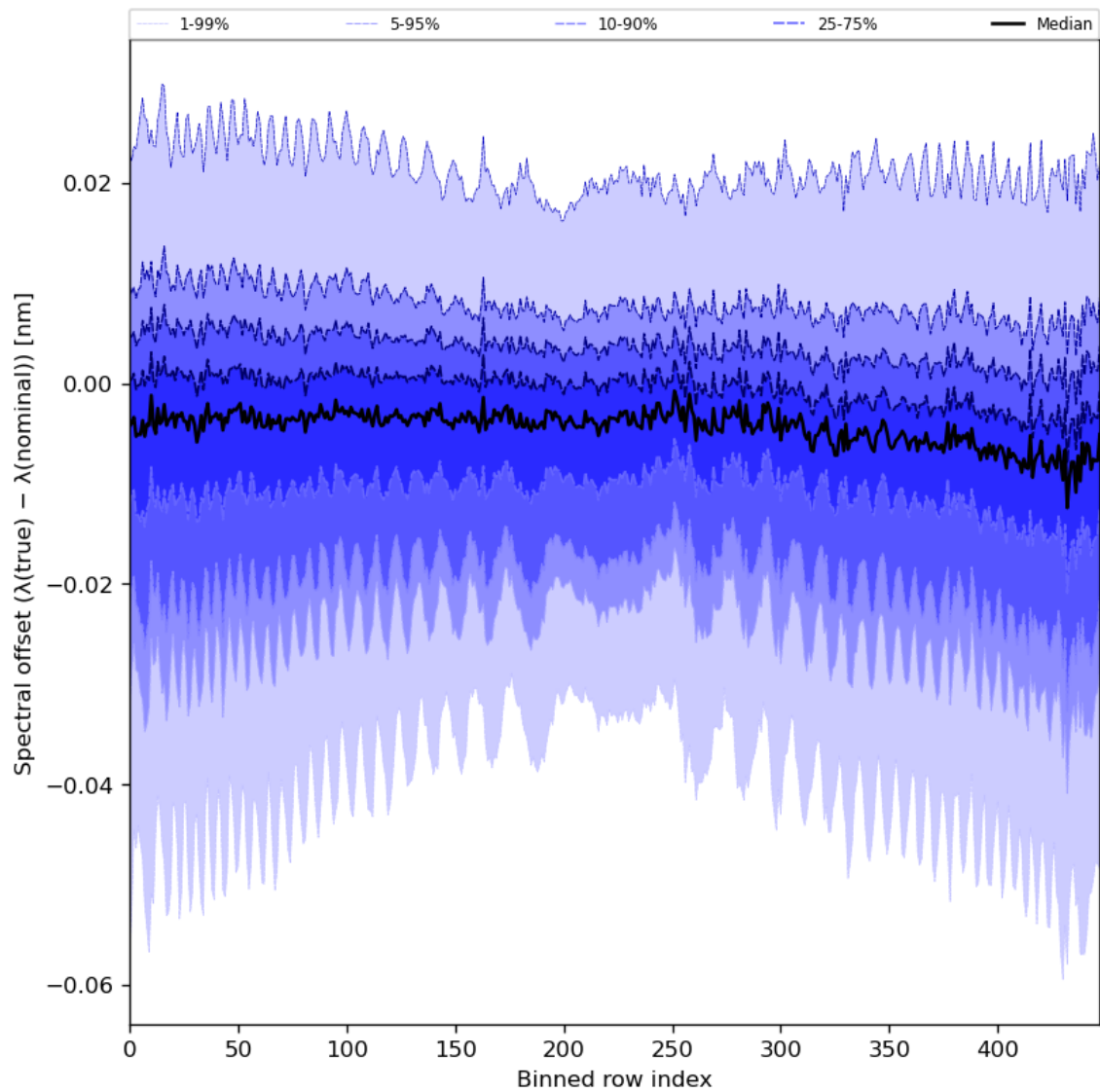
Figure 62: Along track statistics of “Spectral offset ( \lambda(\text{true}) - \lambda(\text{nominal}) )” for 2024-05-10 to 2024-05-12
