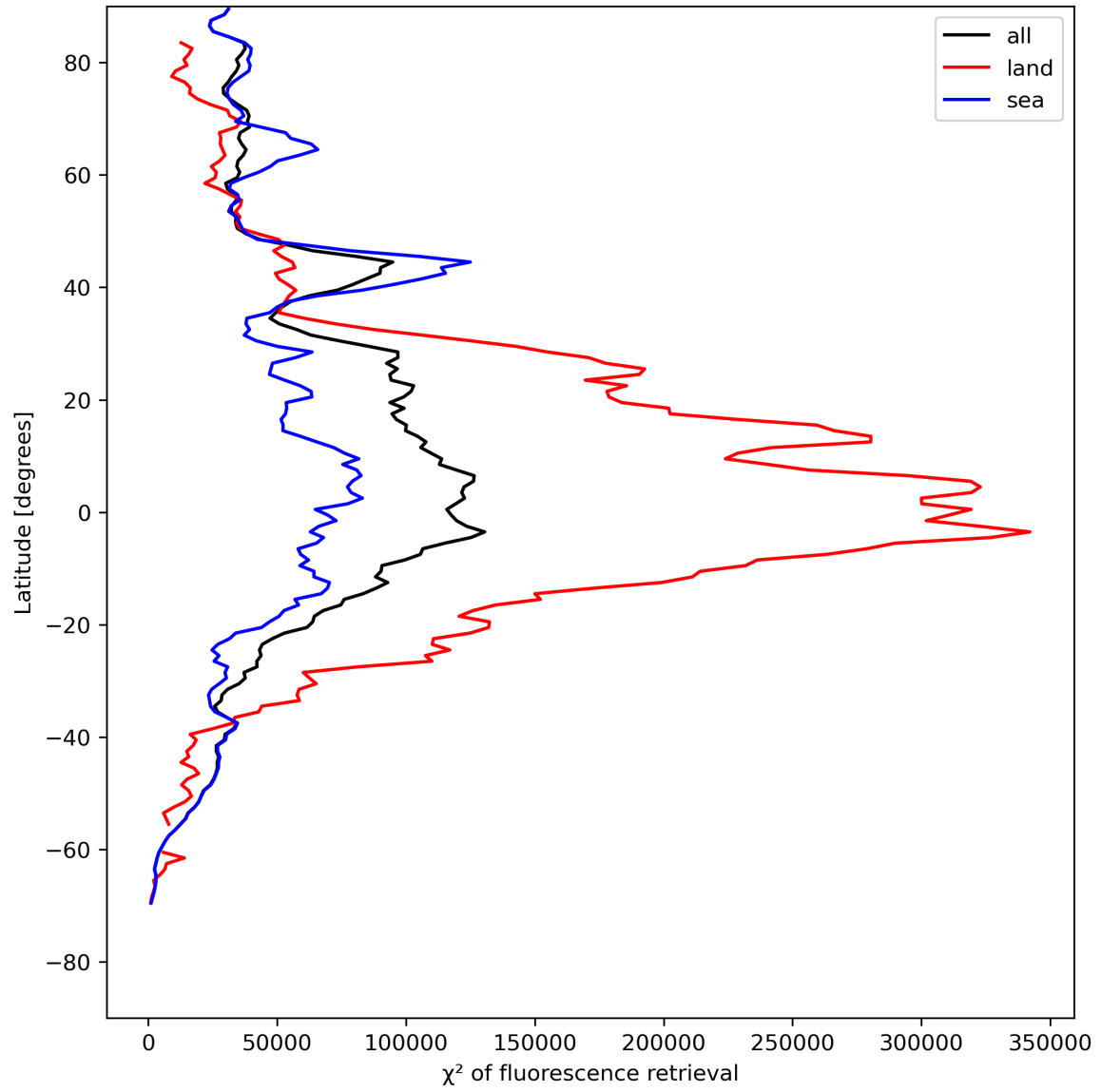
Figure 25: Zonal average of “ \chi^2 of fluorescence retrieval” for 2024-05-10 to 2024-05-12.
