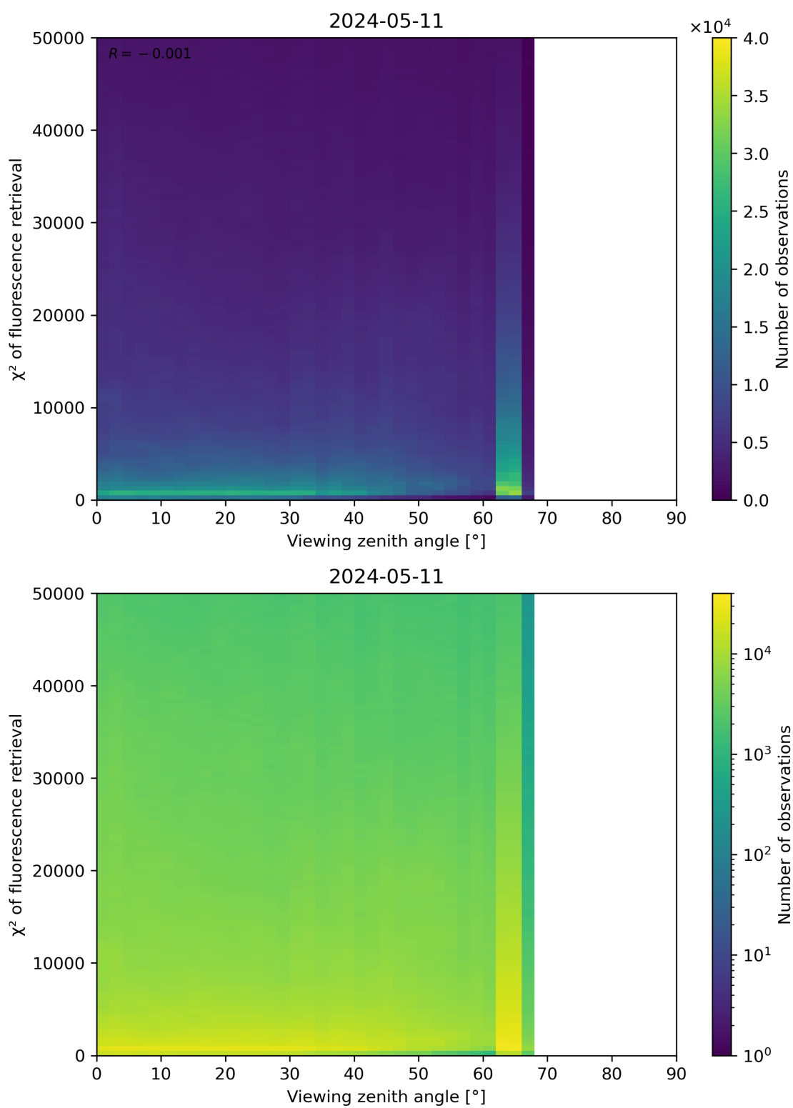
Figure 119: Scatter density plot of “Viewing zenith angle” against “ \chi^2 of fluorescence retrieval” for 2024-05-10 to 2024-05-12.
