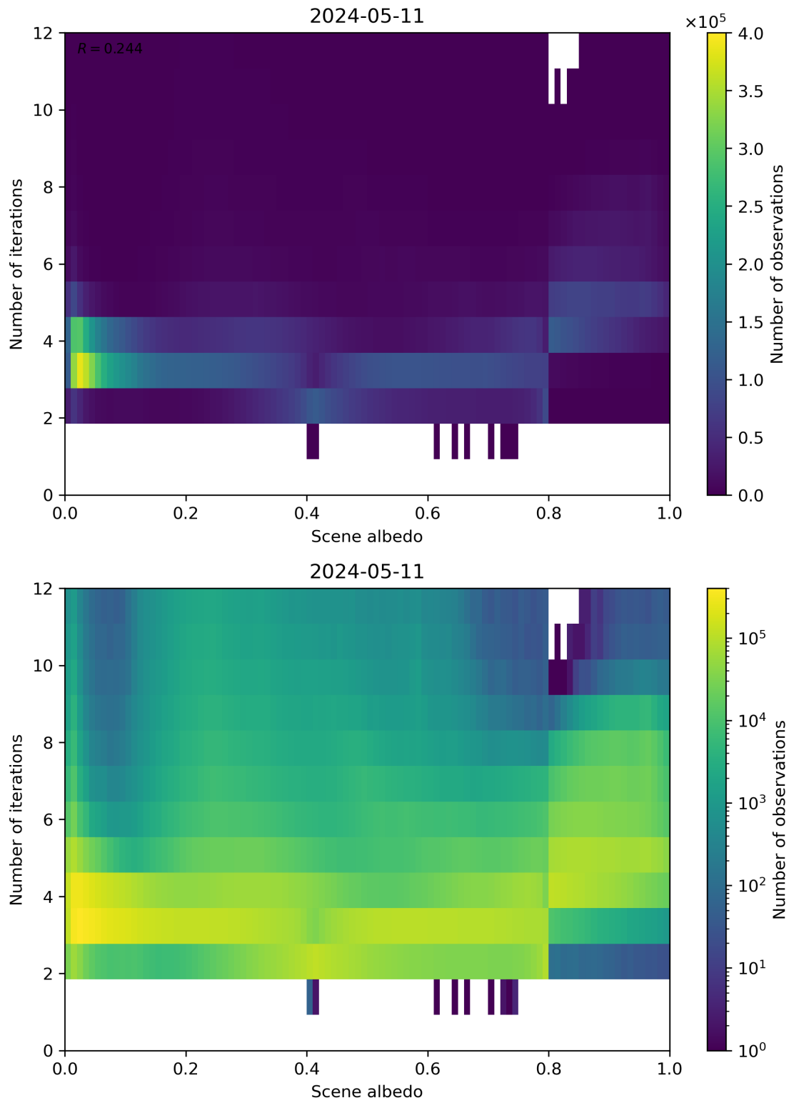
Figure 105: Scatter density plot of “Scene albedo” against “Number of iterations” for 2024-05-10 to 2024-05-12.
