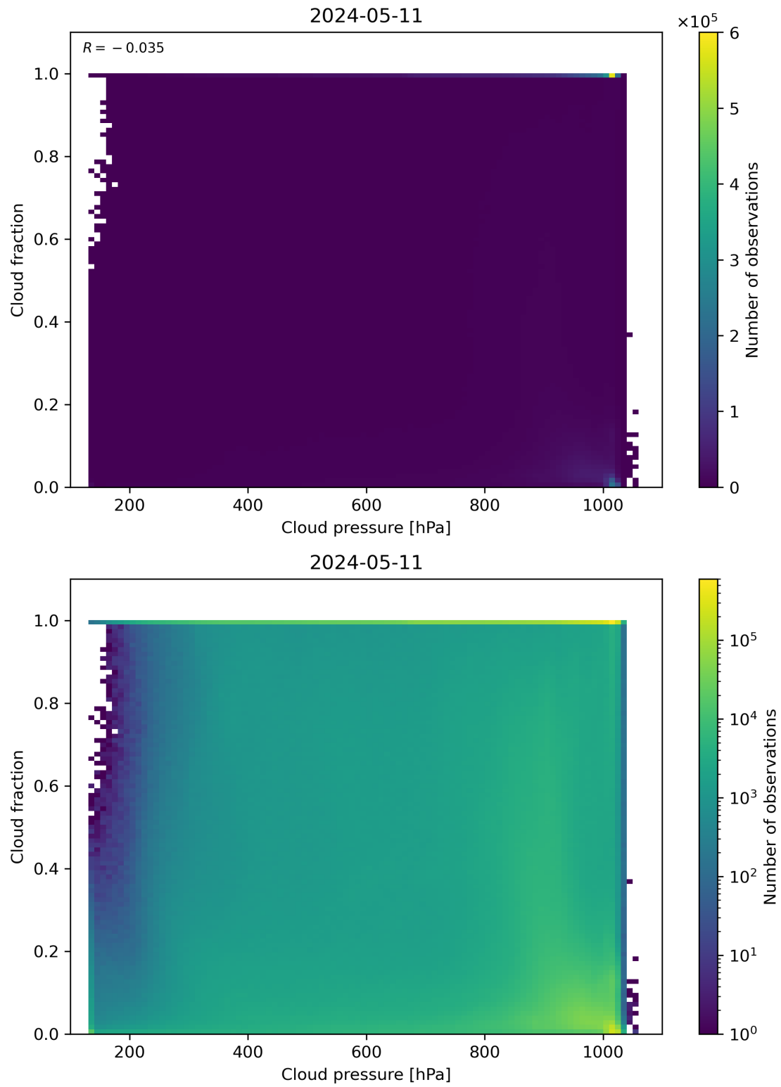
Figure 79: Scatter density plot of “Cloud pressure” against “Cloud fraction” for 2024-05-10 to 2024-05-12.
