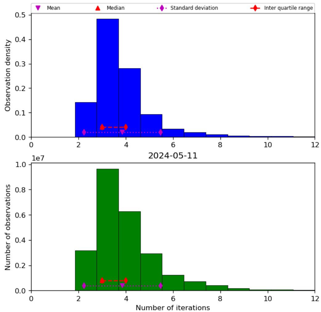
Figure 39: Histogram of “Number of iterations” for 2024-05-10 to 2024-05-12
