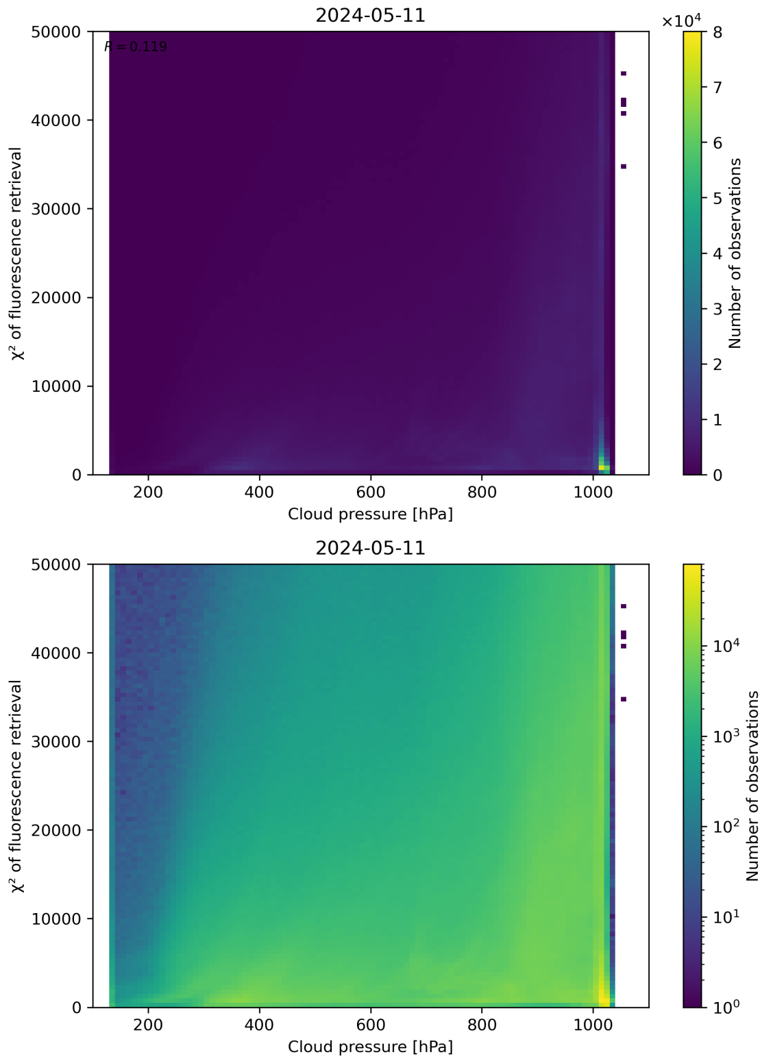
Figure 78: Scatter density plot of “Cloud pressure” against “ \chi^2 of fluorescence retrieval” for 2024-05-10 to 2024-05-12.
