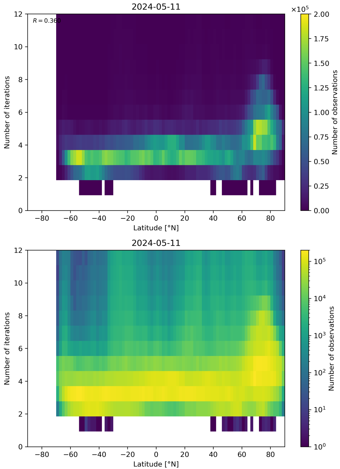
Figure 93: Scatter density plot of “Latitude” against “Number of iterations” for 2024-05-10 to 2024-05-12.
