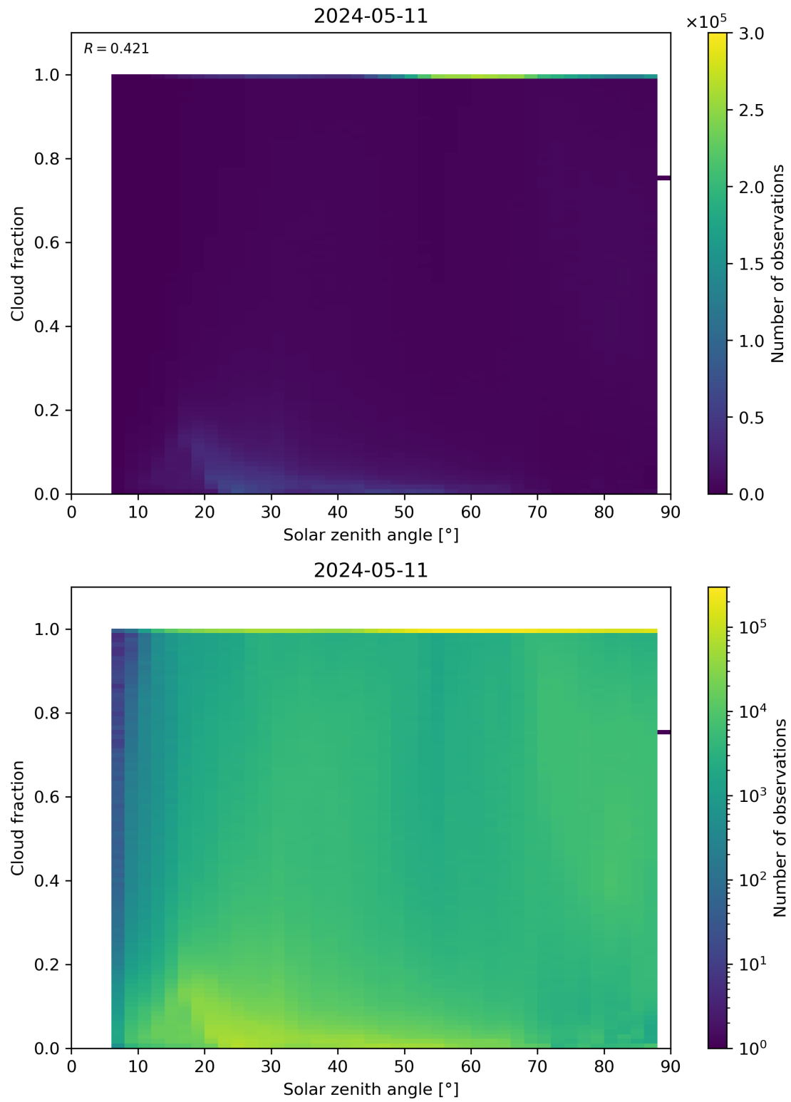
Figure 110: Scatter density plot of “Solar zenith angle” against “Cloud fraction” for 2024-05-10 to 2024-05-12.
