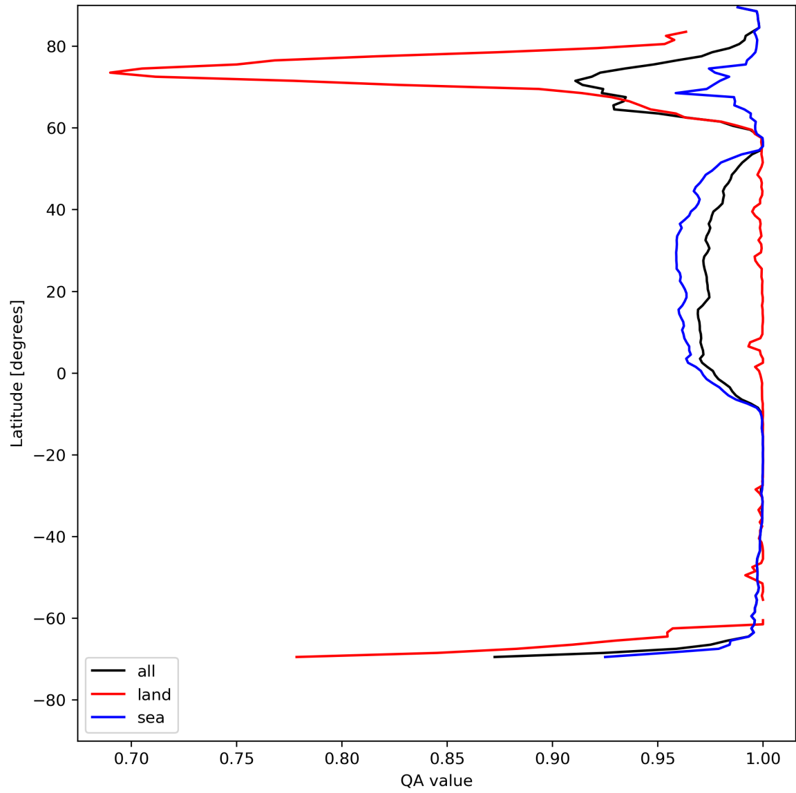
Figure 12: Zonal average of “QA value” for 2024-05-10 to 2024-05-12.
