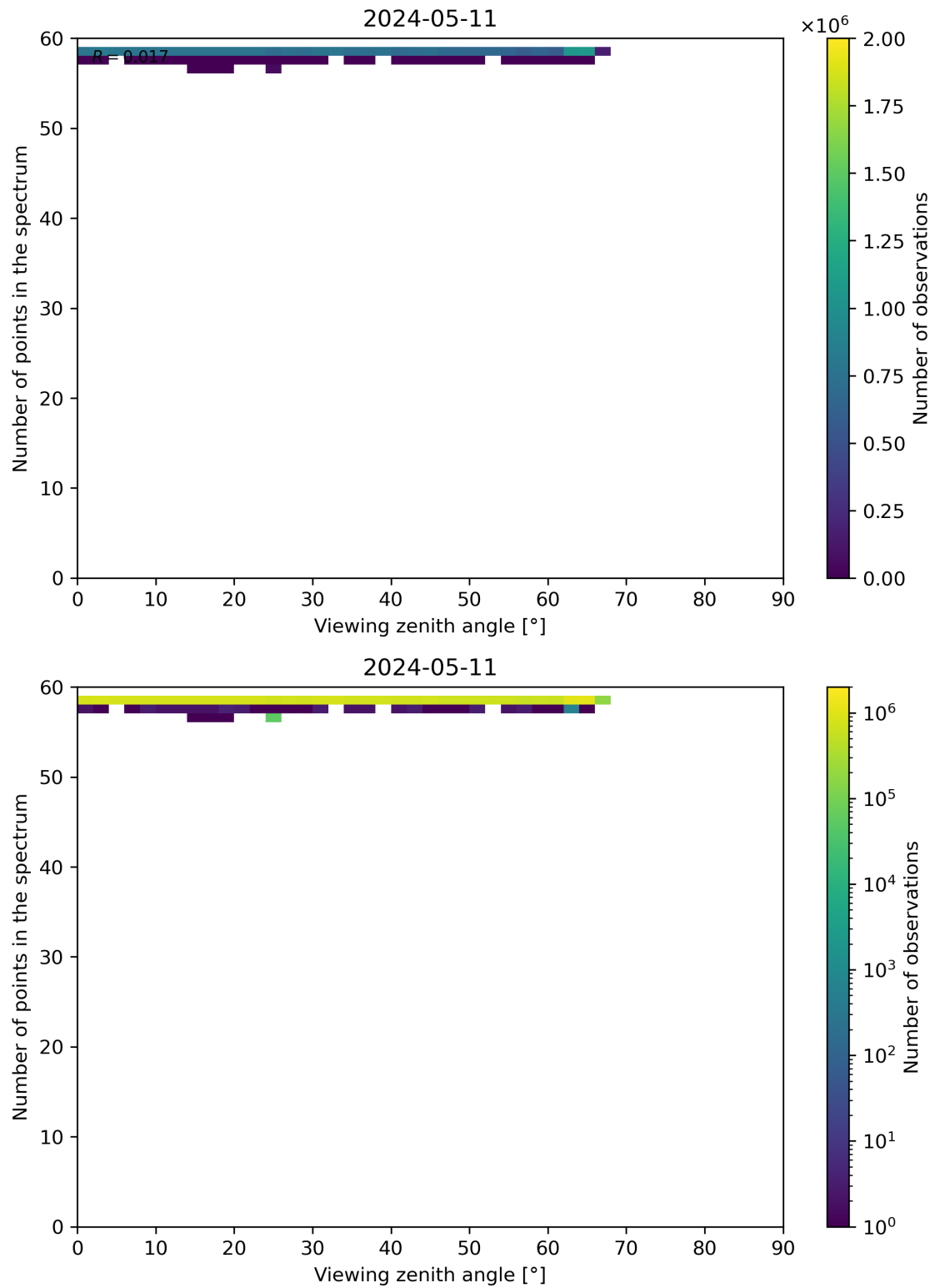
Figure 125: Scatter density plot of “Viewing zenith angle” against “Number of points in the spectrum” for 2024-05-10 to 2024-05-12.
