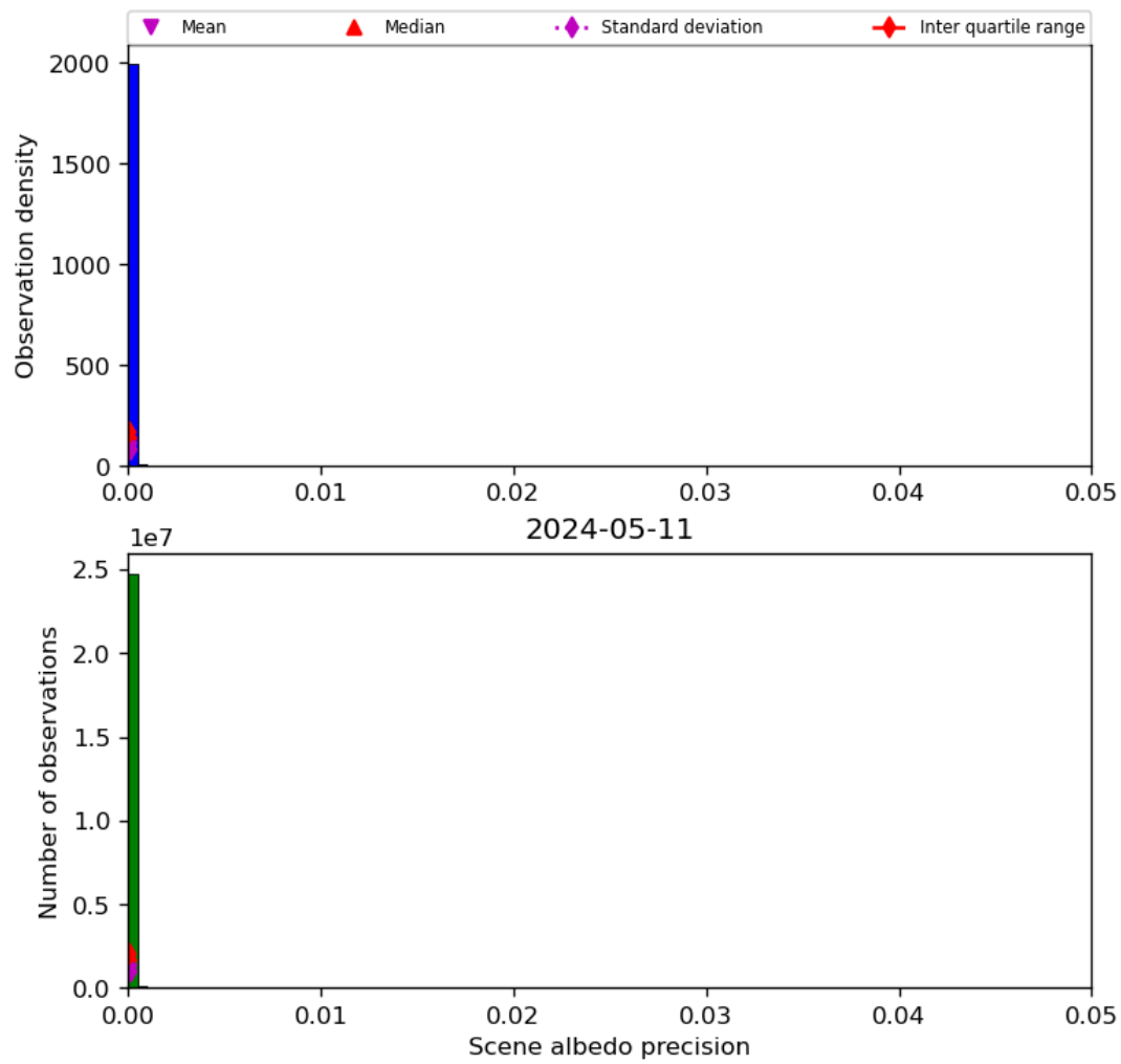
Figure 35: Histogram of “Scene albedo precision” for 2024-05-10 to 2024-05-12
