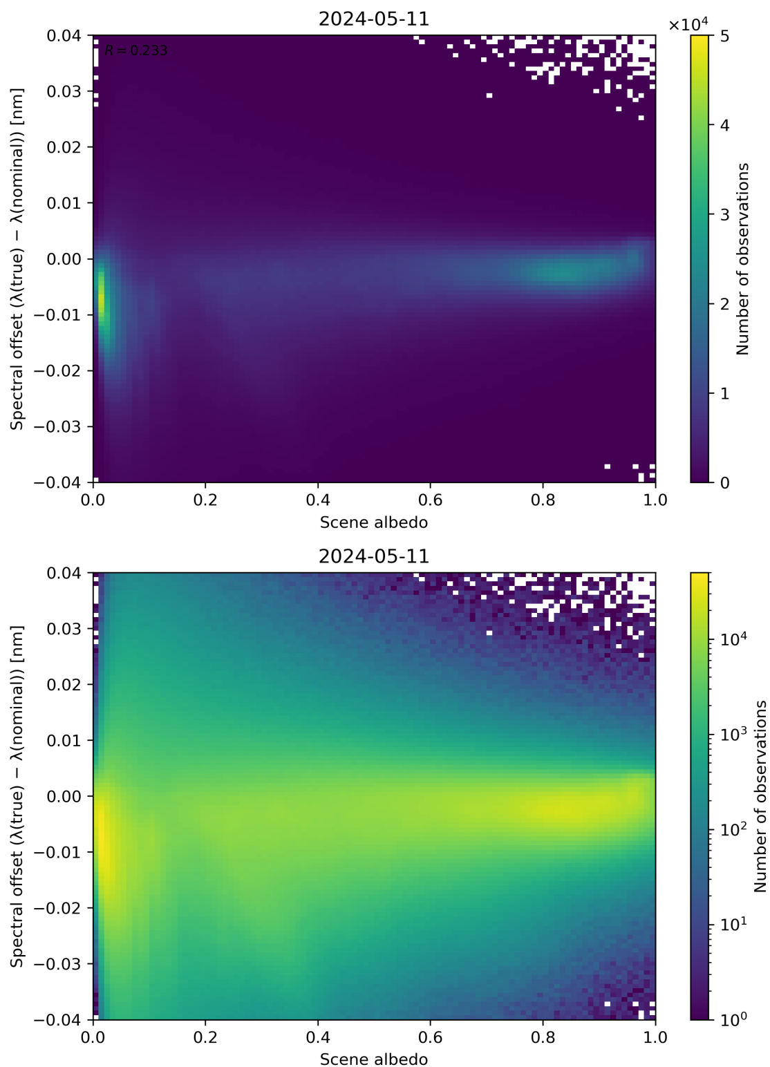
Figure 107: Scatter density plot of “Scene albedo” against “Spectral offset ( \lambda(\text{true}) - \lambda(\text{nominal}) )” for 2024-05-10 to 2024-05-12.
