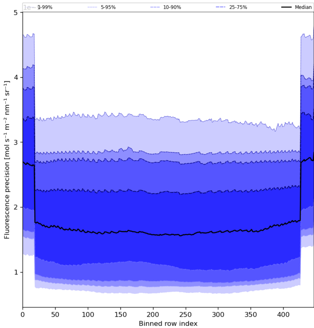
Figure 58: Along track statistics of “Fluorescence precision” for 2024-05-10 to 2024-05-12
