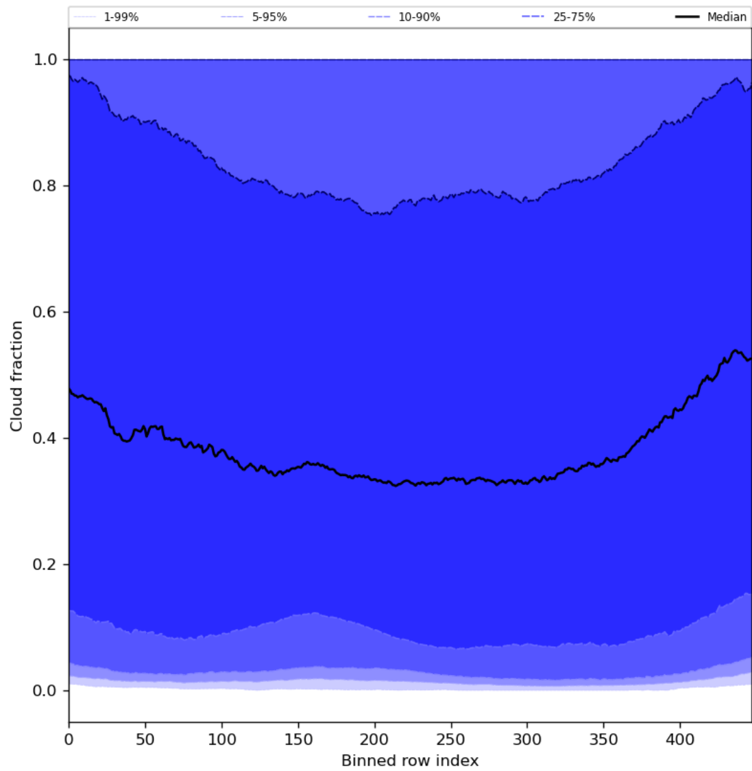
Figure 49: Along track statistics of “Cloud fraction” for 2024-05-10 to 2024-05-12
