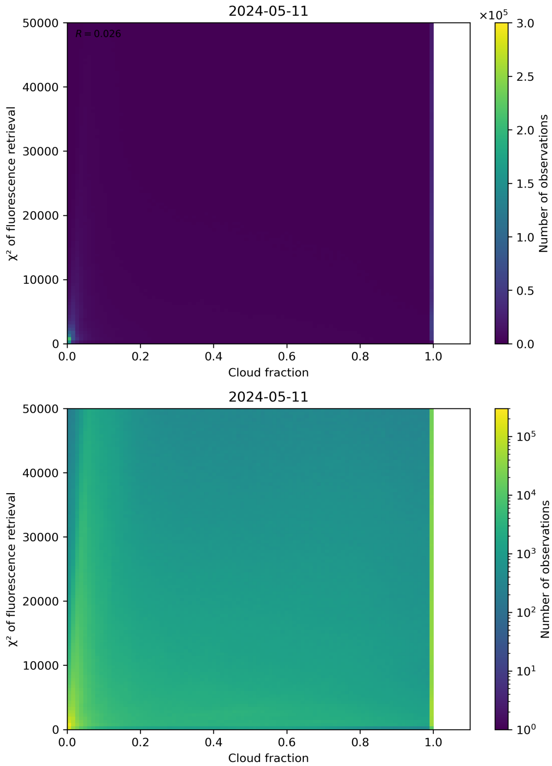
Figure 71: Scatter density plot of “Cloud fraction” against “ \chi^2 of fluorescence retrieval” for 2024-05-10 to 2024-05-12.
