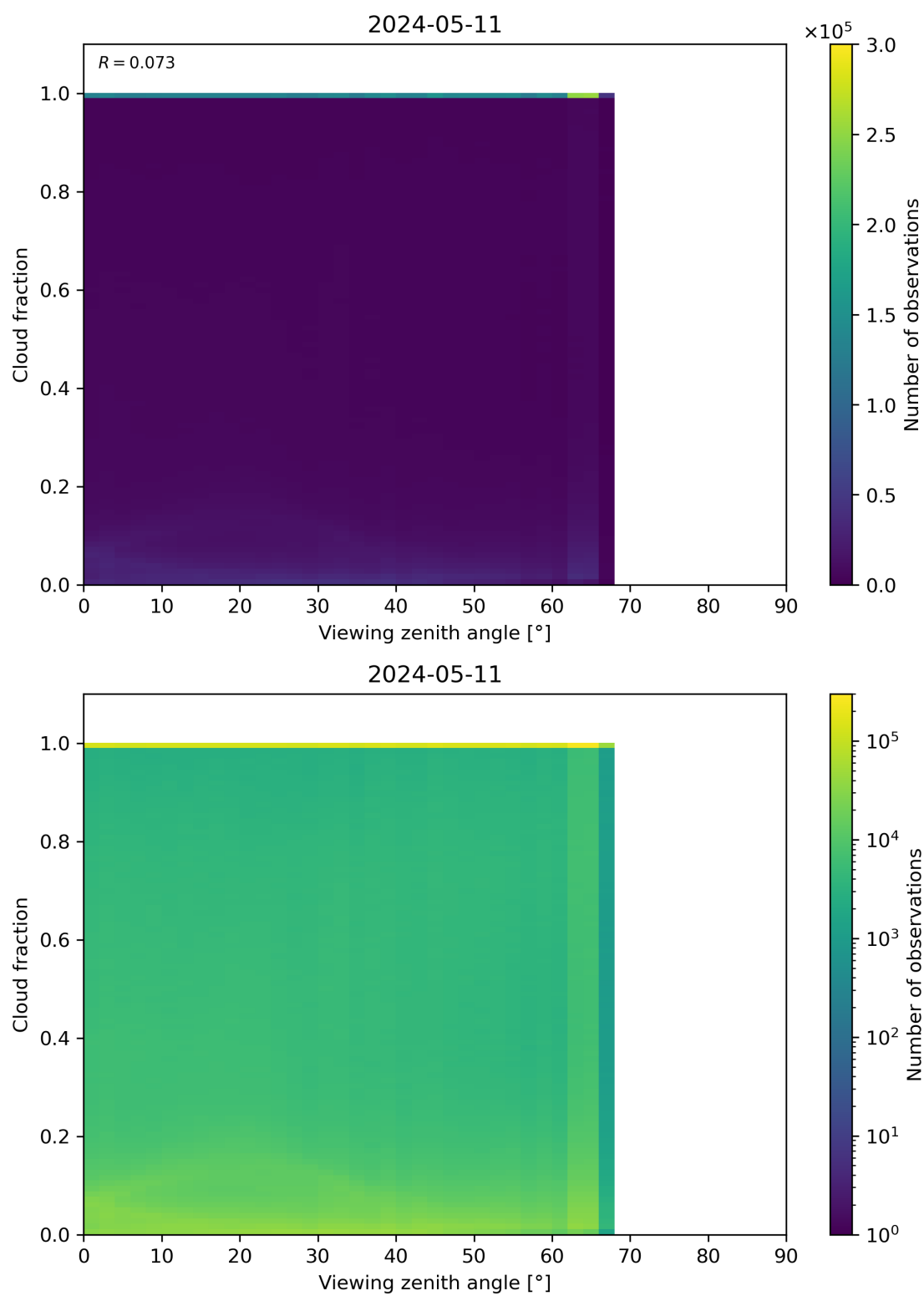
Figure 120: Scatter density plot of “Viewing zenith angle” against “Cloud fraction” for 2024-05-10 to 2024-05-12.
