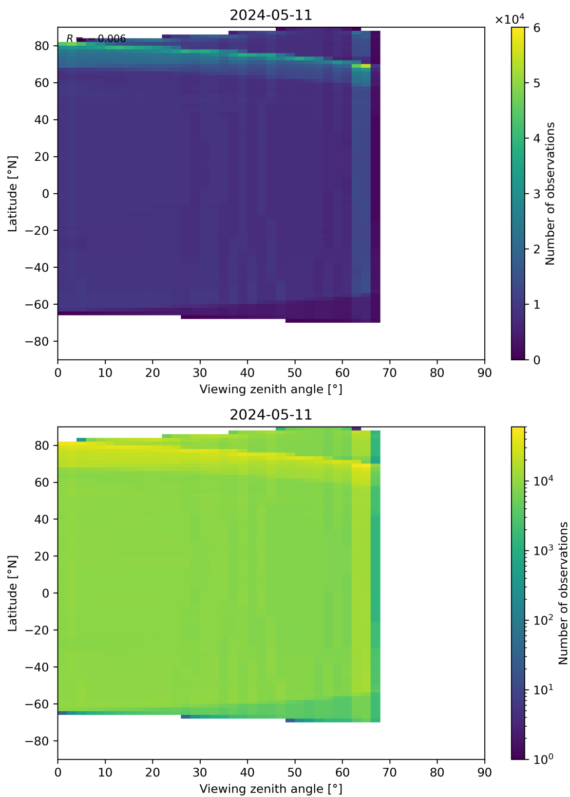
Figure 123: Scatter density plot of “Viewing zenith angle” against “Latitude” for 2024-05-10 to 2024-05-12.
