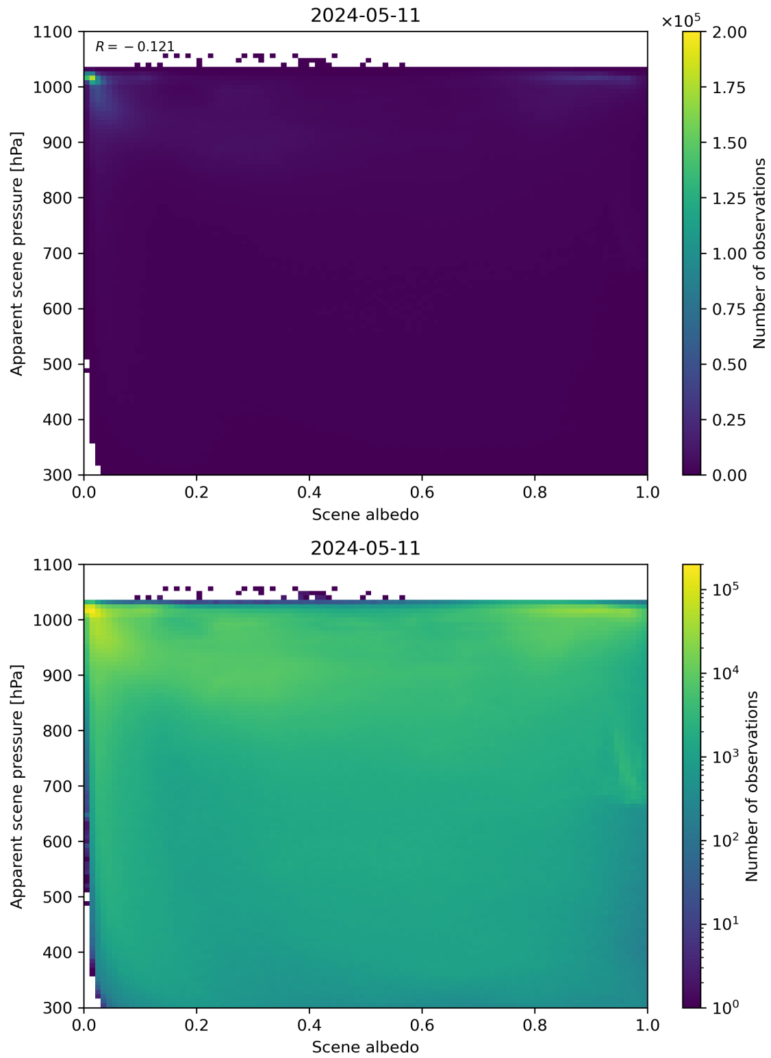
Figure 102: Scatter density plot of “Scene albedo” against “Apparent scene pressure” for 2024-05-10 to 2024-05-12.
