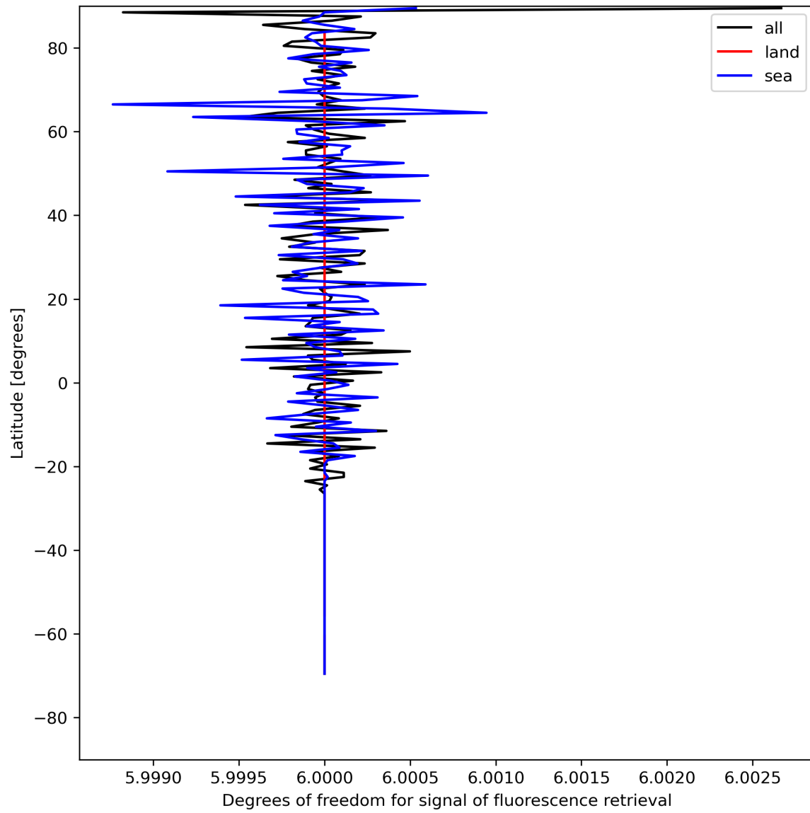
Figure 26: Zonal average of “Degrees of freedom for signal of fluorescence retrieval” for 2024-05-10 to 2024-05-12.
