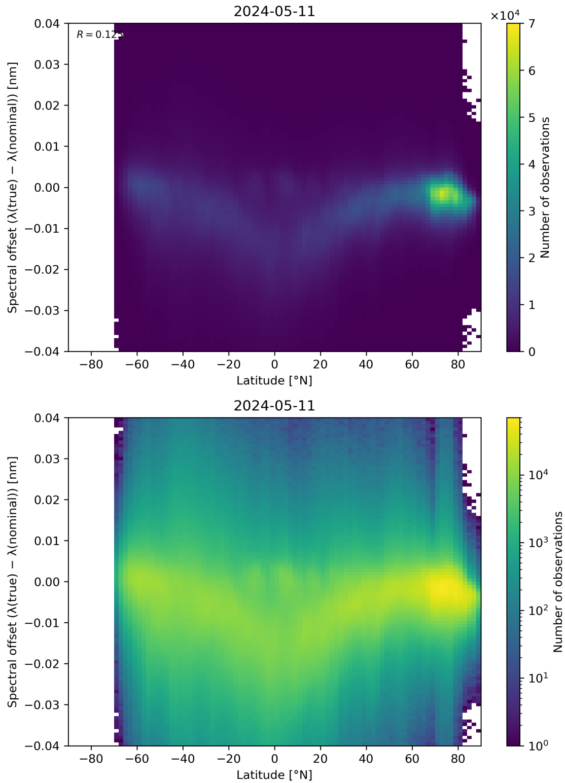
Figure 96: Scatter density plot of “Latitude” against “Spectral offset ( \lambda(\text{true}) - \lambda(\text{nominal}) )” for 2024-05-10 to 2024-05-12.
