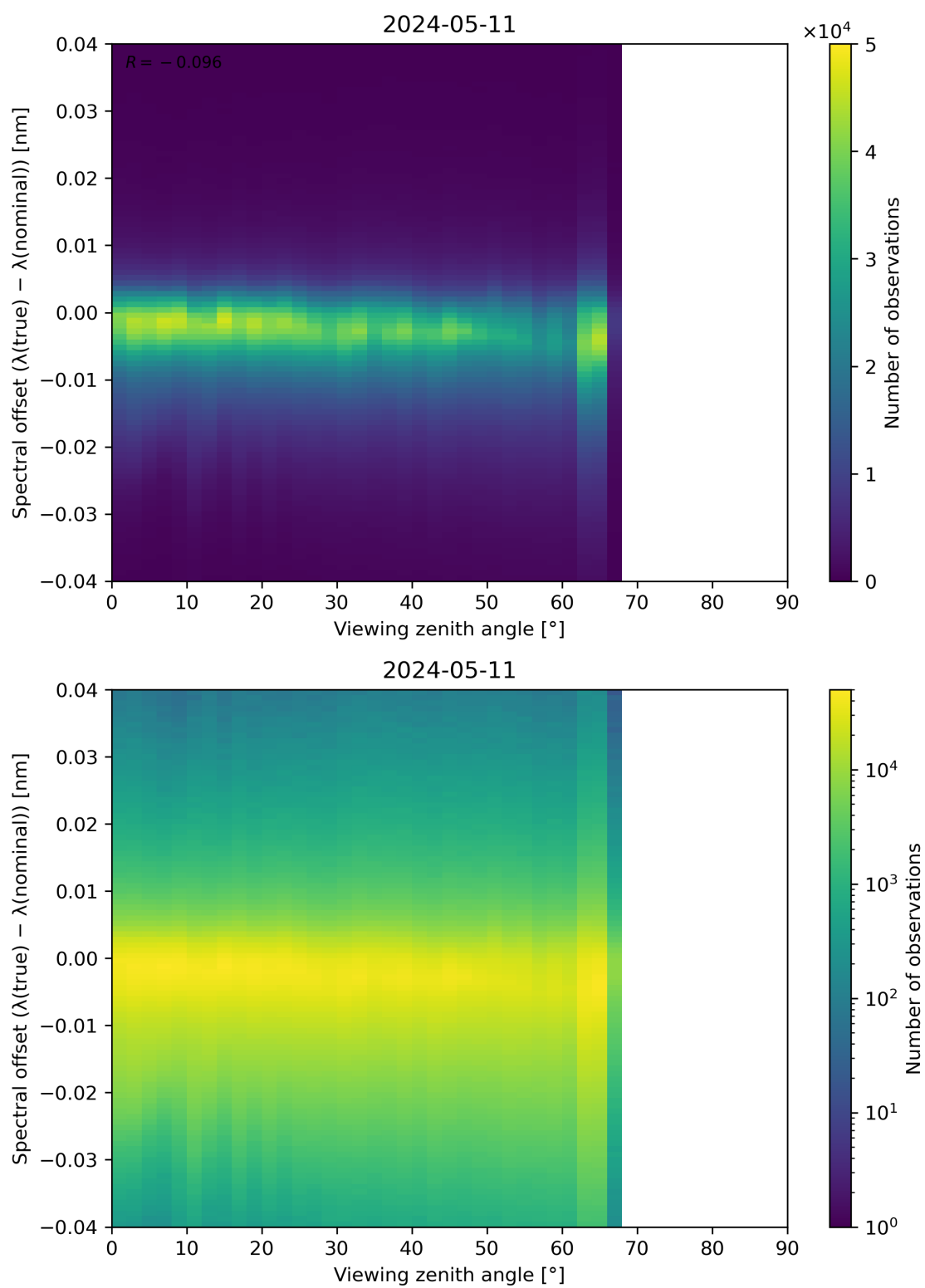
Figure 128: Scatter density plot of “Viewing zenith angle” against “Spectral offset ( \lambda(\text{true}) - \lambda(\text{nominal}) )” for 2024-05-10 to 2024-05-12.
