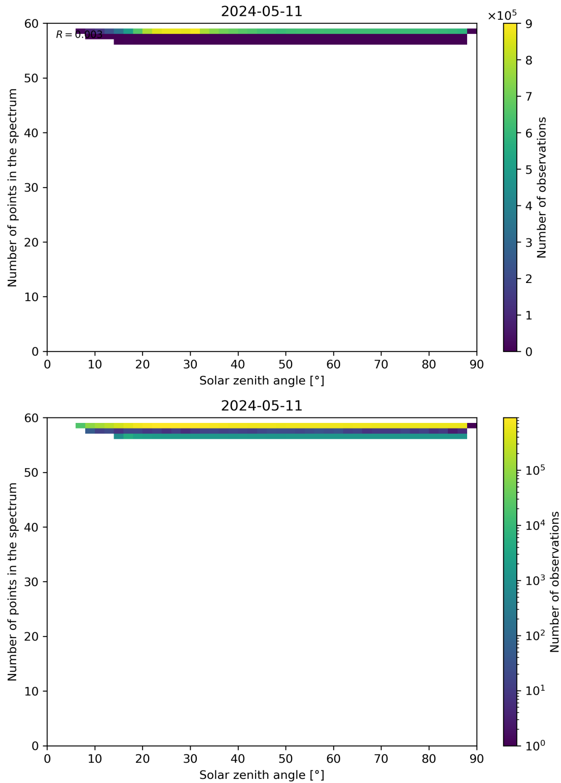
Figure 115: Scatter density plot of “Solar zenith angle” against “Number of points in the spectrum” for 2024-05-10 to 2024-05-12.
