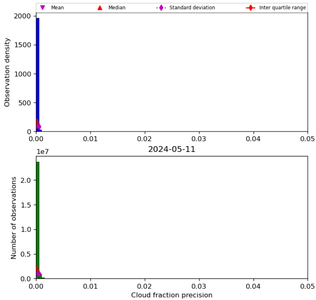
Figure 33: Histogram of “Cloud fraction precision” for 2024-05-10 to 2024-05-12
