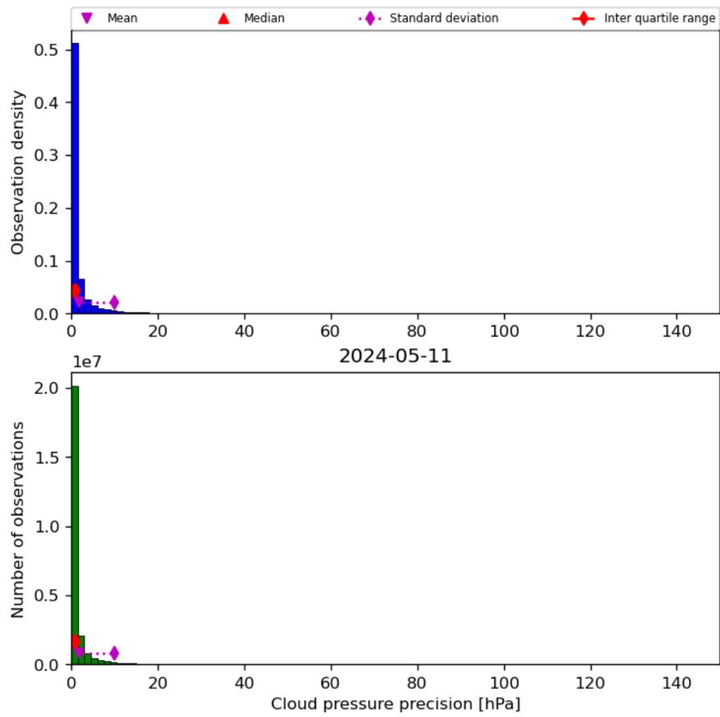
Figure 31: Histogram of “Cloud pressure precision” for 2024-05-10 to 2024-05-12
