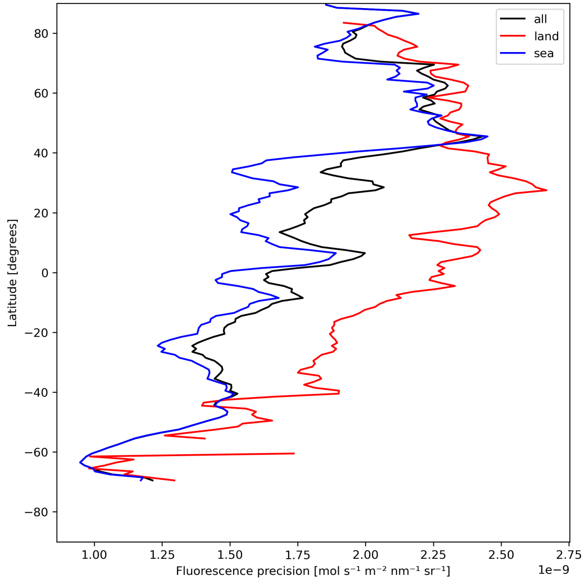
Figure 24: Zonal average of “Fluorescence precision” for 2024-05-10 to 2024-05-12.
