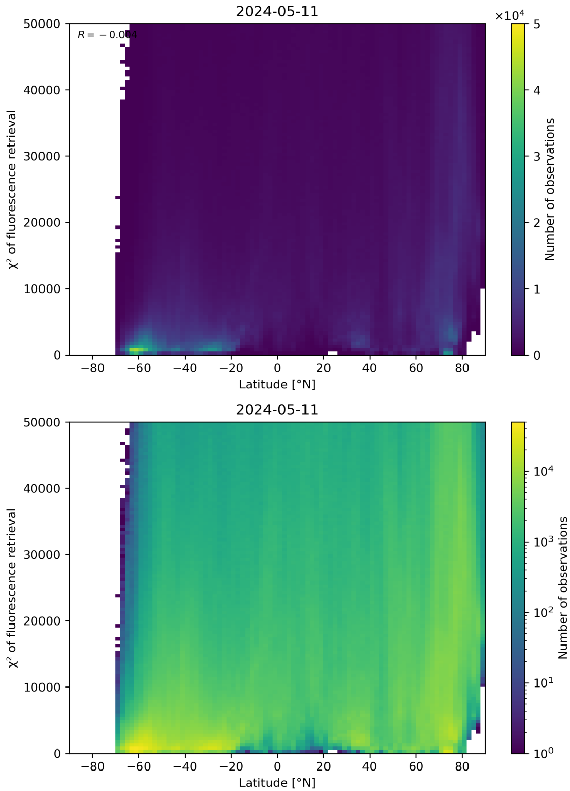
Figure 89: Scatter density plot of “Latitude” against “ \chi^2 of fluorescence retrieval” for 2024-05-10 to 2024-05-12.
