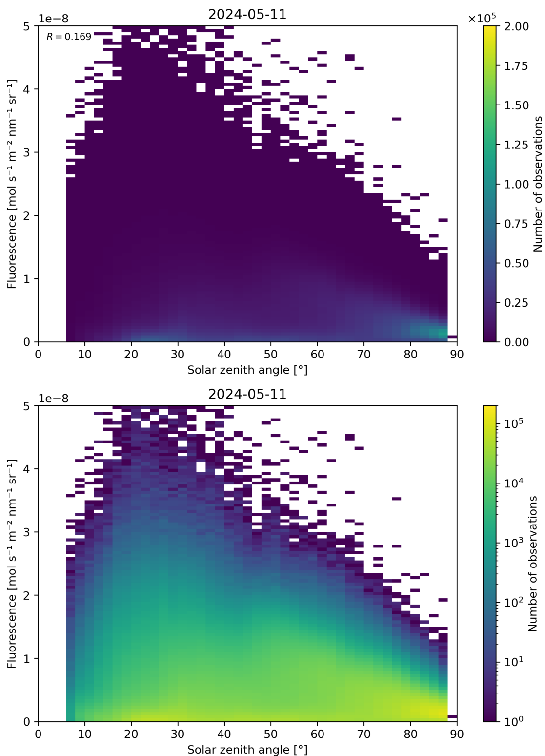
Figure 112: Scatter density plot of “Solar zenith angle” against “Fluorescence” for 2024-05-10 to 2024-05-12.
