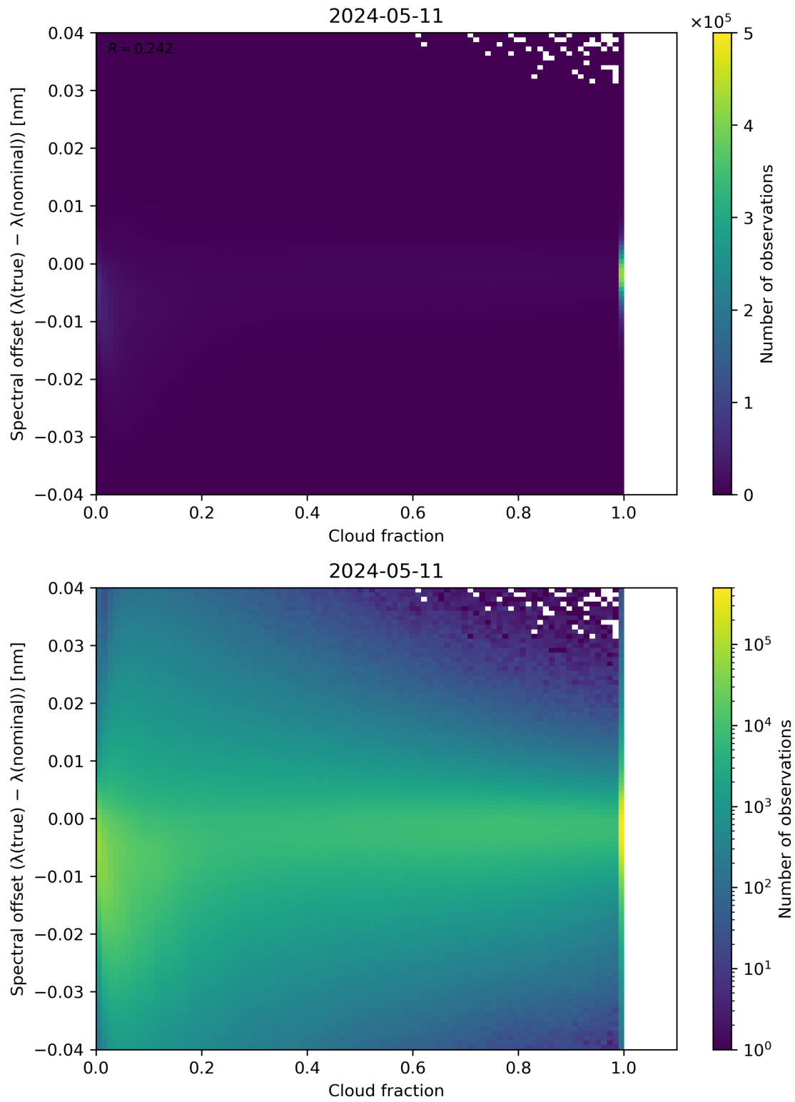
Figure 76: Scatter density plot of “Cloud fraction” against “Spectral offset ( \lambda(\text{true}) - \lambda(\text{nominal}) )” for 2024-05-10 to 2024-05-12.
