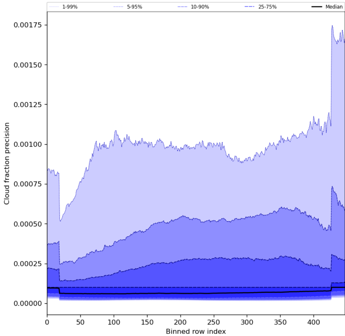
Figure 50: Along track statistics of “Cloud fraction precision” for 2024-05-10 to 2024-05-12
