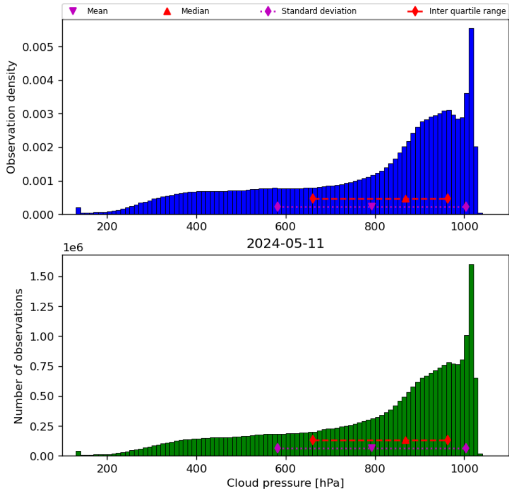
Figure 30: Histogram of “Cloud pressure” for 2024-05-10 to 2024-05-12
