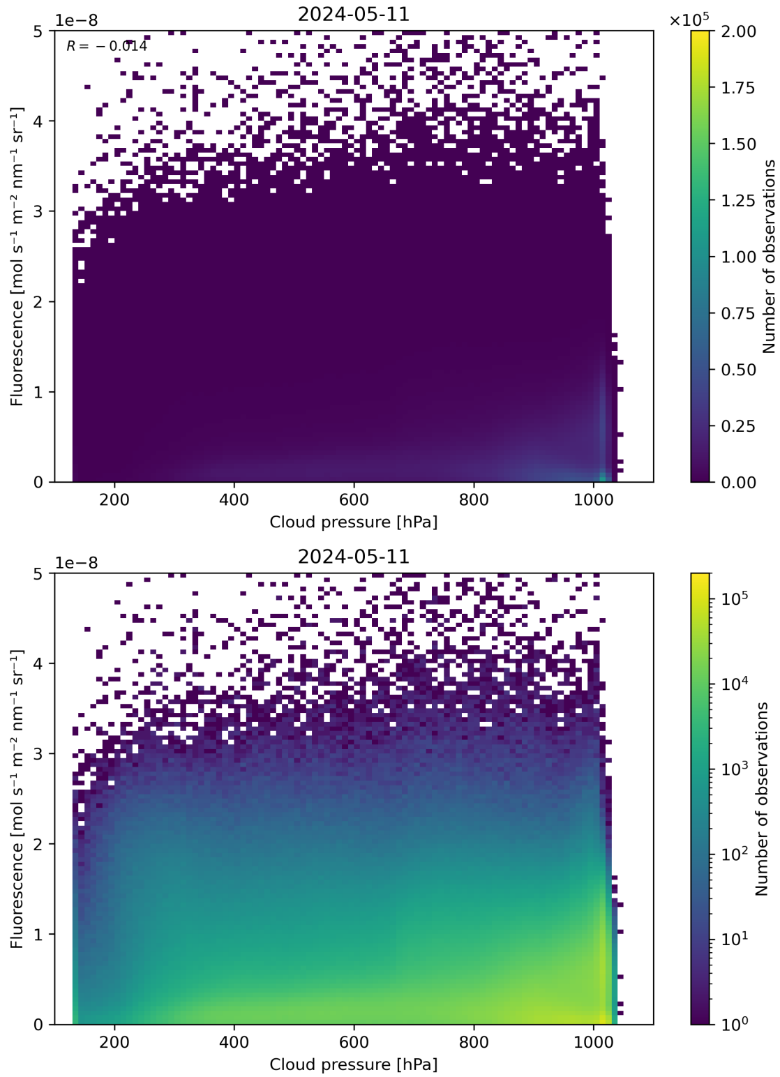
Figure 80: Scatter density plot of “Cloud pressure” against “Fluorescence” for 2024-05-10 to 2024-05-12.
