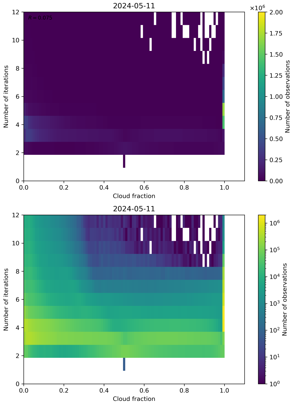
Figure 73: Scatter density plot of “Cloud fraction” against “Number of iterations” for 2024-05-10 to 2024-05-12.
