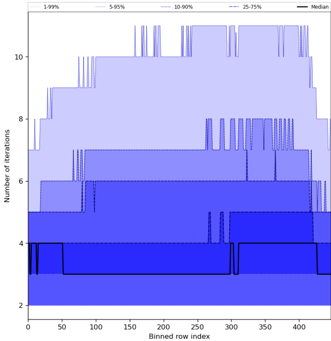
Figure 56: Along track statistics of “Number of iterations” for 2024-05-10 to 2024-05-12
