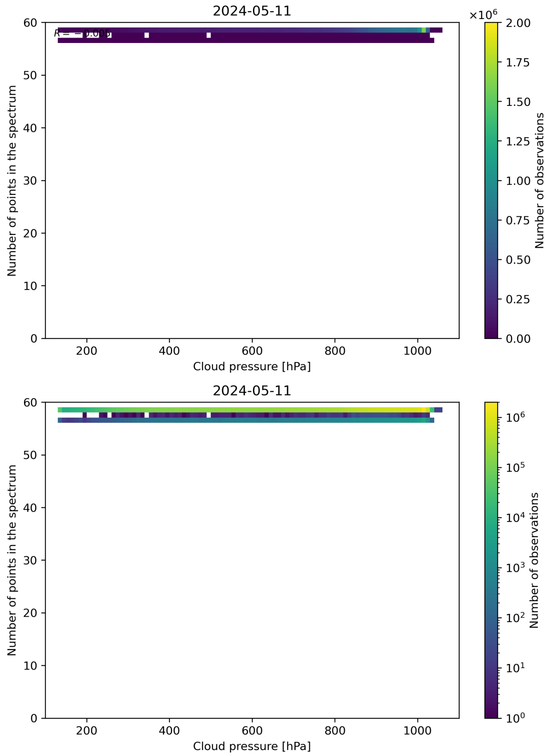
Figure 82: Scatter density plot of “Cloud pressure” against “Number of points in the spectrum” for 2024-05-10 to 2024-05-12.
