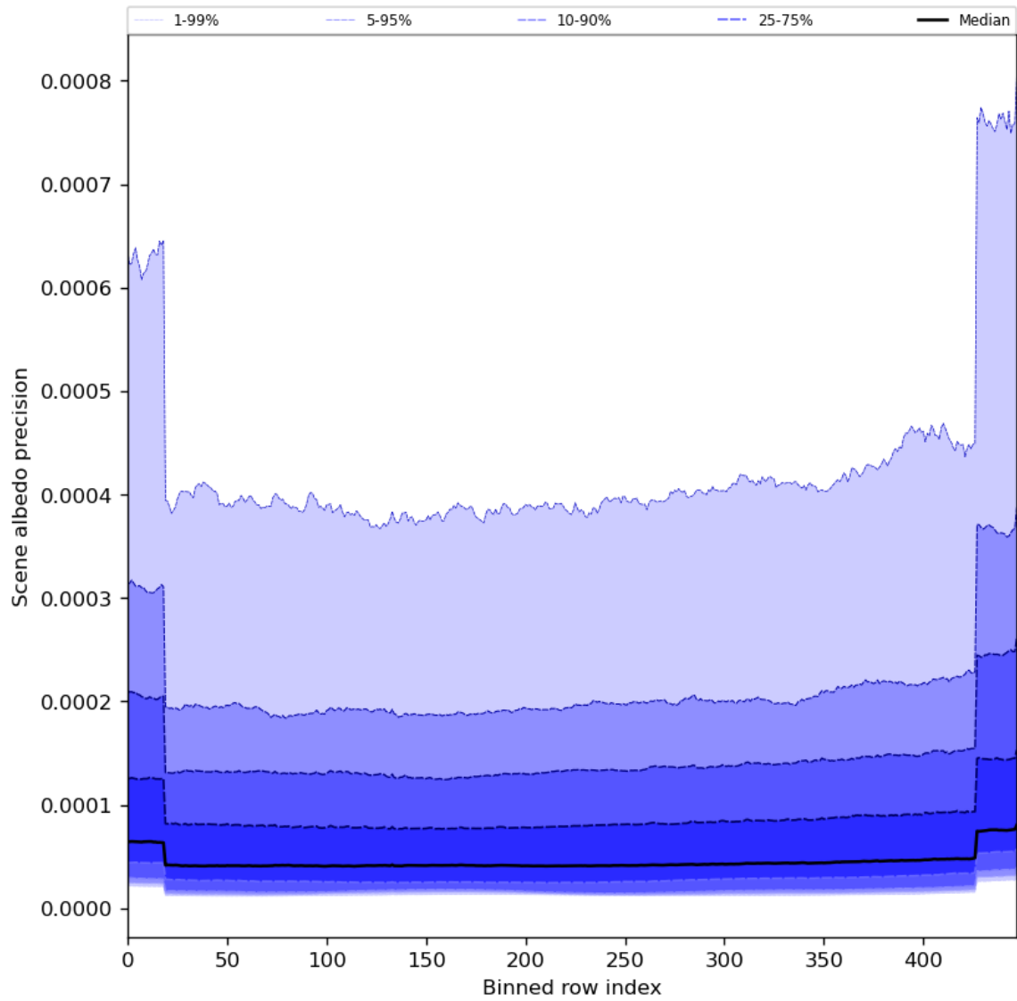
Figure 52: Along track statistics of “Scene albedo precision” for 2024-05-10 to 2024-05-12
