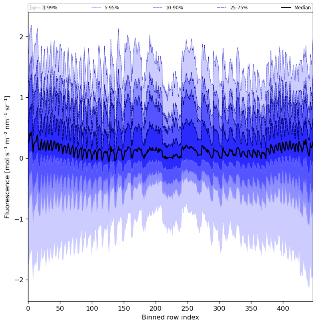
Figure 57: Along track statistics of “Fluorescence” for 2024-05-10 to 2024-05-12
