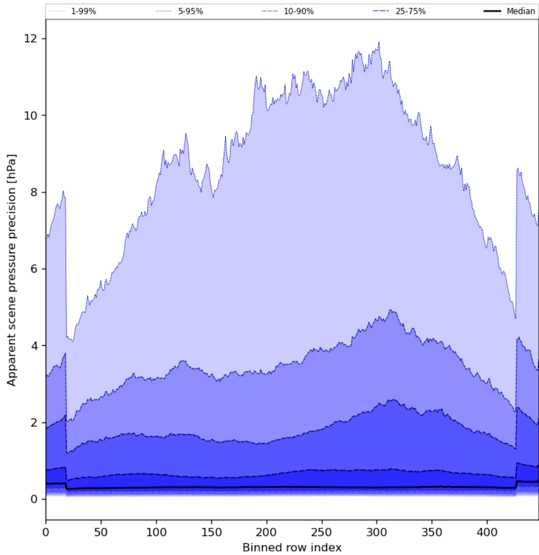
Figure 54: Along track statistics of “Apparent scene pressure precision” for 2024-05-10 to 2024-05-12
