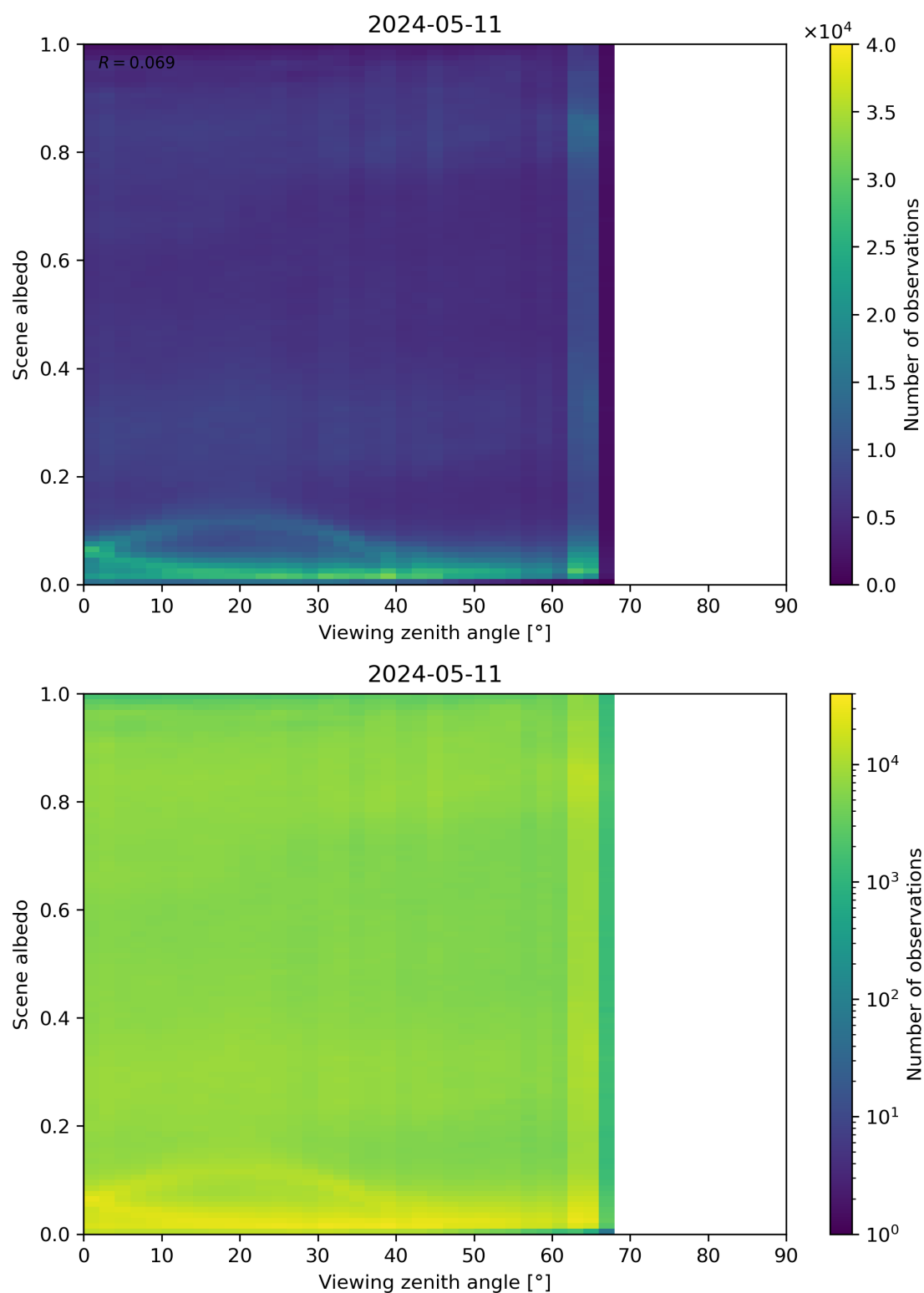
Figure 126: Scatter density plot of “Viewing zenith angle” against “Scene albedo” for 2024-05-10 to 2024-05-12.
