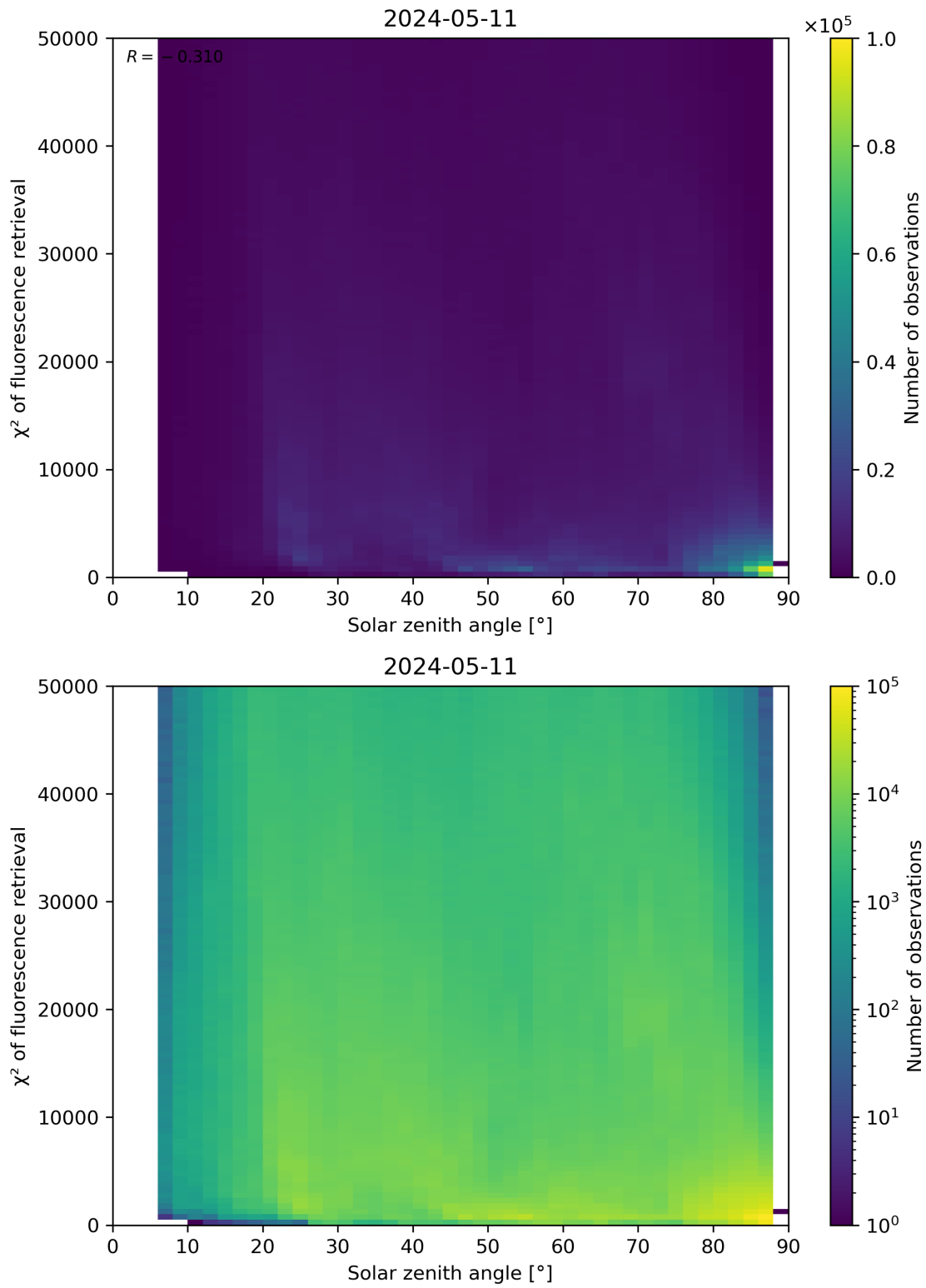
Figure 109: Scatter density plot of “Solar zenith angle” against “ \chi^2 of fluorescence retrieval” for 2024-05-10 to 2024-05-12.
