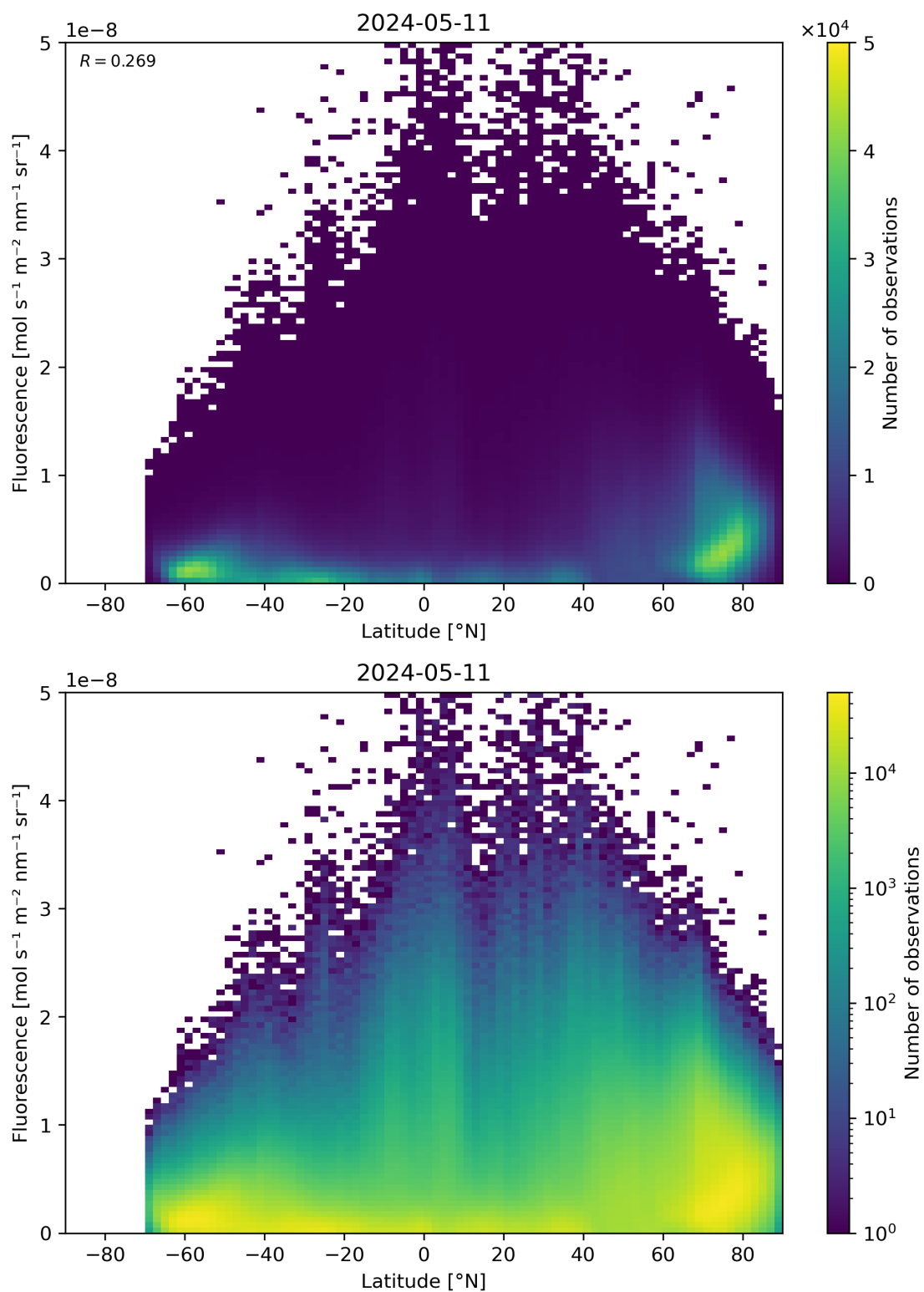
Figure 92: Scatter density plot of “Latitude” against “Fluorescence” for 2024-05-10 to 2024-05-12.
