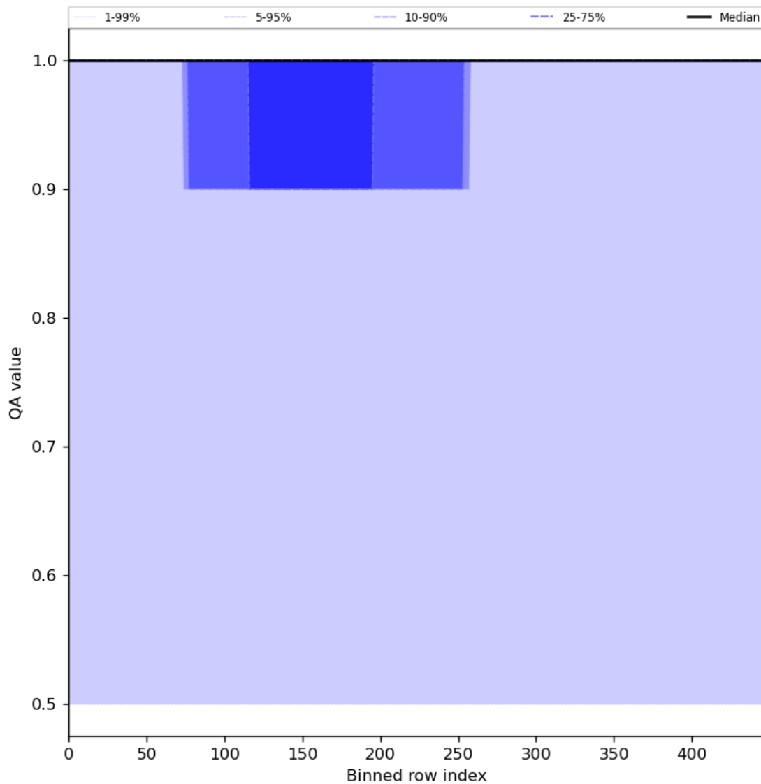
Figure 46: Along track statistics of “QA value” for 2024-05-10 to 2024-05-12
