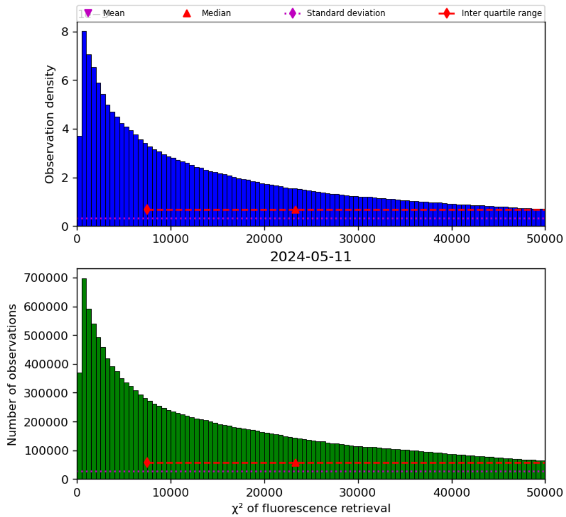
Figure 42: Histogram of “ \chi^2 of fluorescence retrieval” for 2024-05-10 to 2024-05-12
