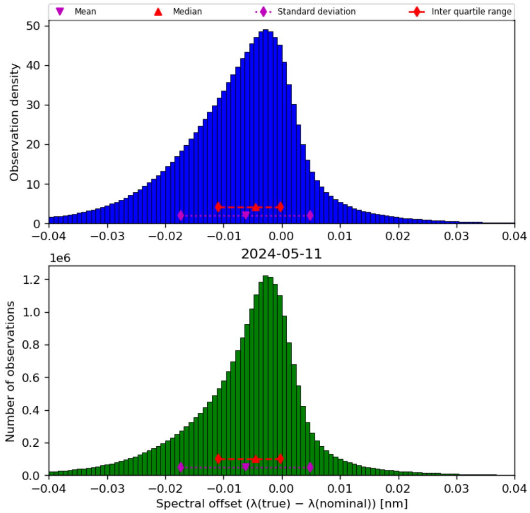
Figure 45: Histogram of “Spectral offset ( \lambda(\text{true}) - \lambda(\text{nominal}) )” for 2024-05-10 to 2024-05-12
