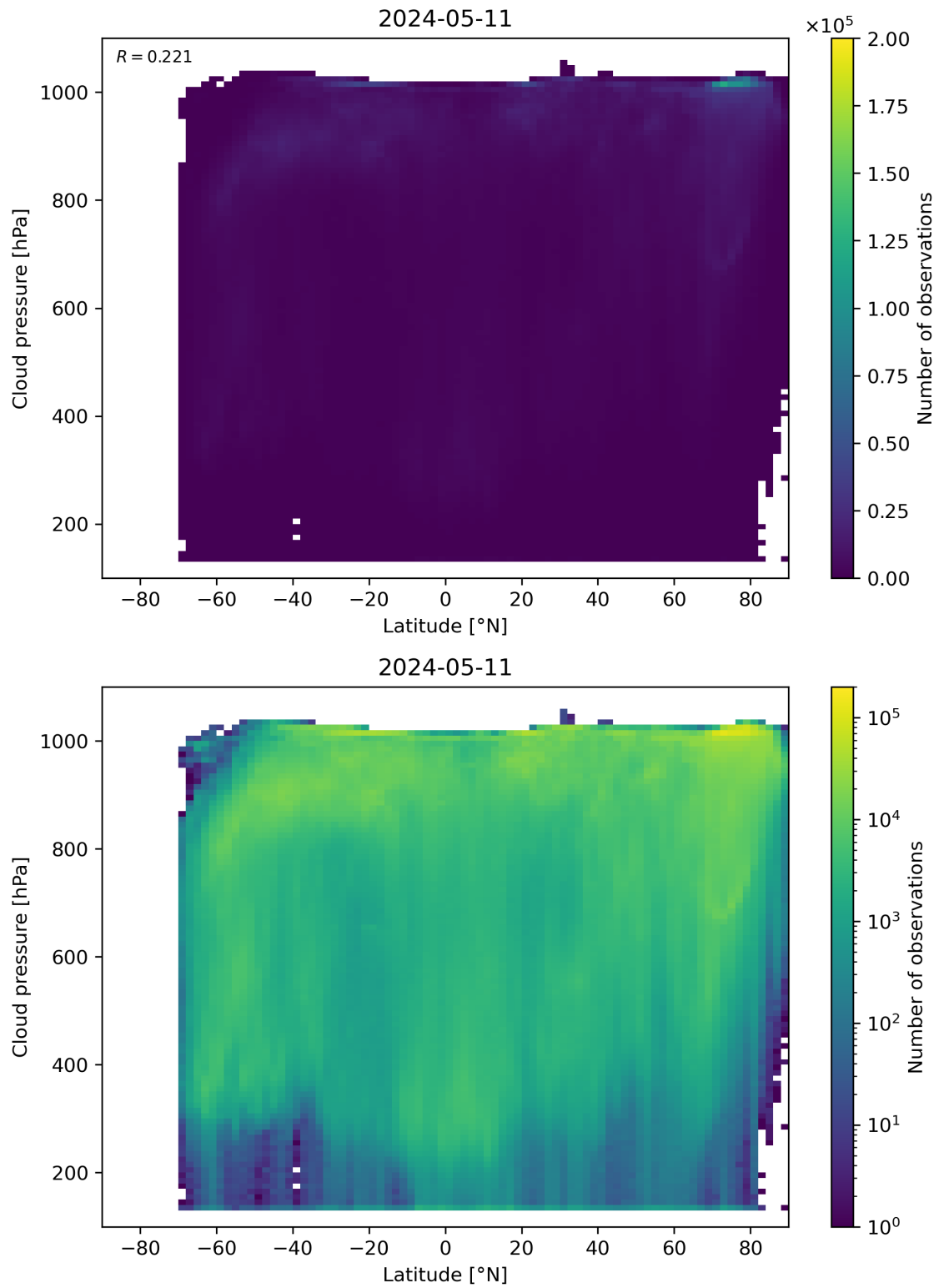
Figure 91: Scatter density plot of “Latitude” against “Cloud pressure” for 2024-05-10 to 2024-05-12.
