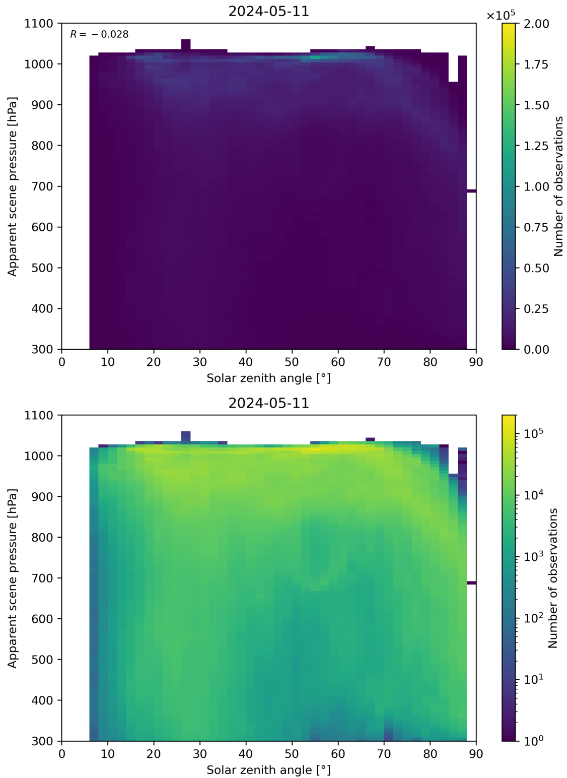
Figure 108: Scatter density plot of “Solar zenith angle” against “Apparent scene pressure” for 2024-05-10 to 2024-05-12.
