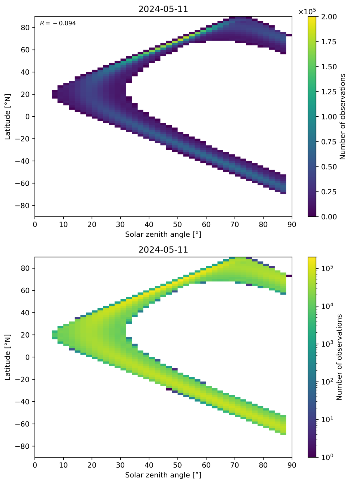
Figure 113: Scatter density plot of “Solar zenith angle” against “Latitude” for 2024-05-10 to 2024-05-12.
