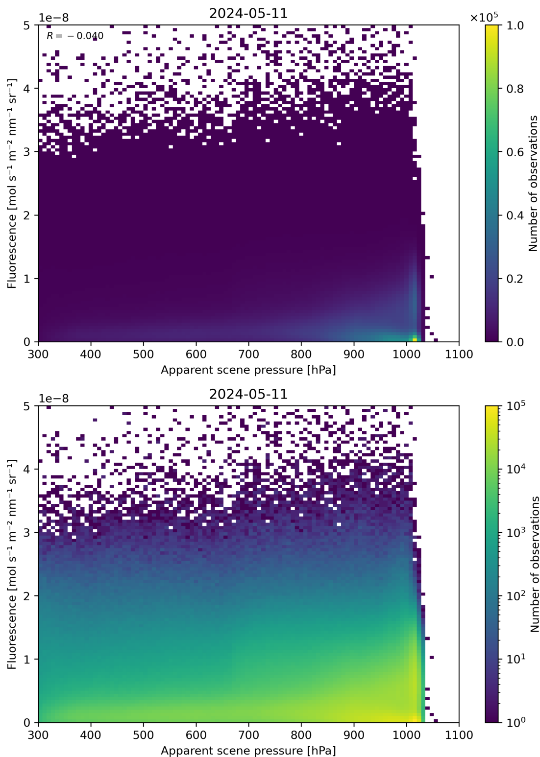
Figure 64: Scatter density plot of “Apparent scene pressure” against “Fluorescence” for 2024-05-10 to 2024-05-12.
