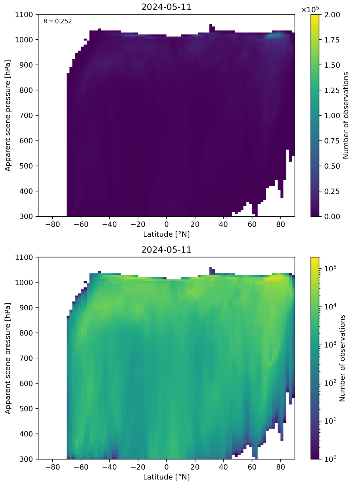
Figure 88: Scatter density plot of “Latitude” against “Apparent scene pressure” for 2024-05-10 to 2024-05-12.
