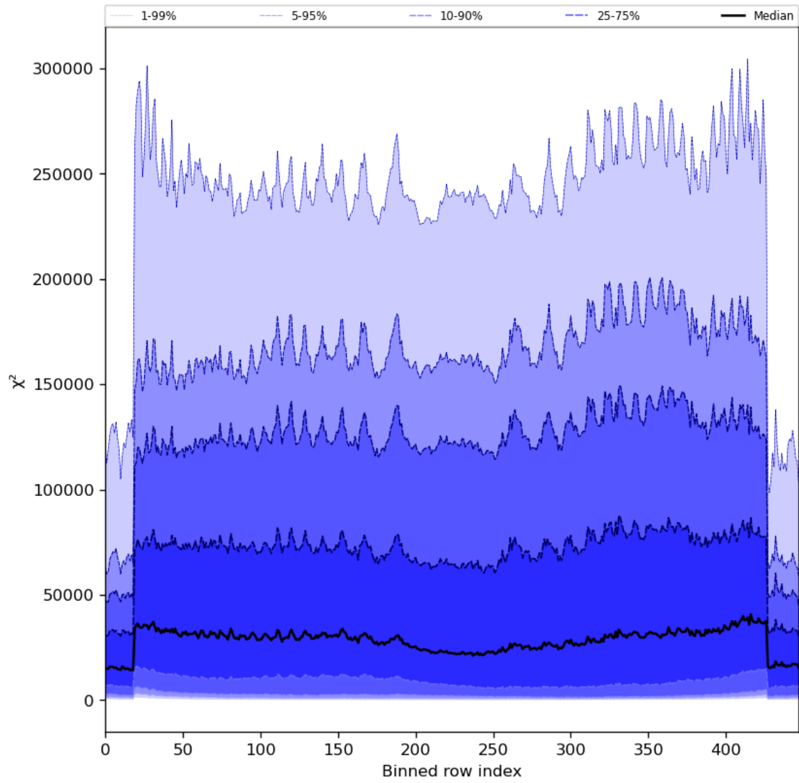
Figure 55: Along track statistics of “ \chi^2 ” for 2024-05-10 to 2024-05-12
