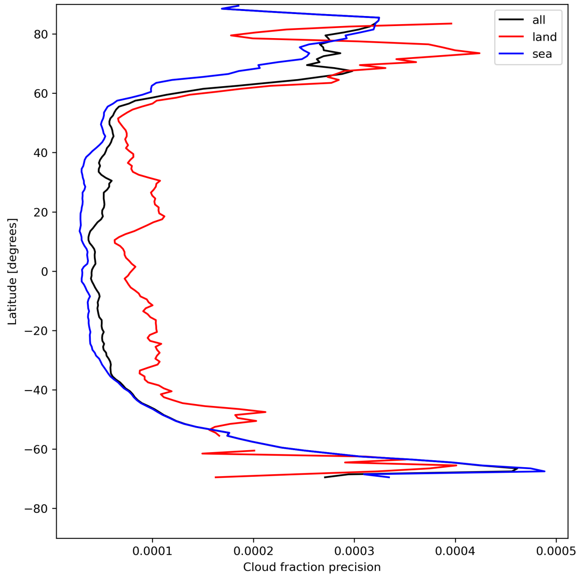
Figure 16: Zonal average of “Cloud fraction precision” for 2024-05-10 to 2024-05-12.
