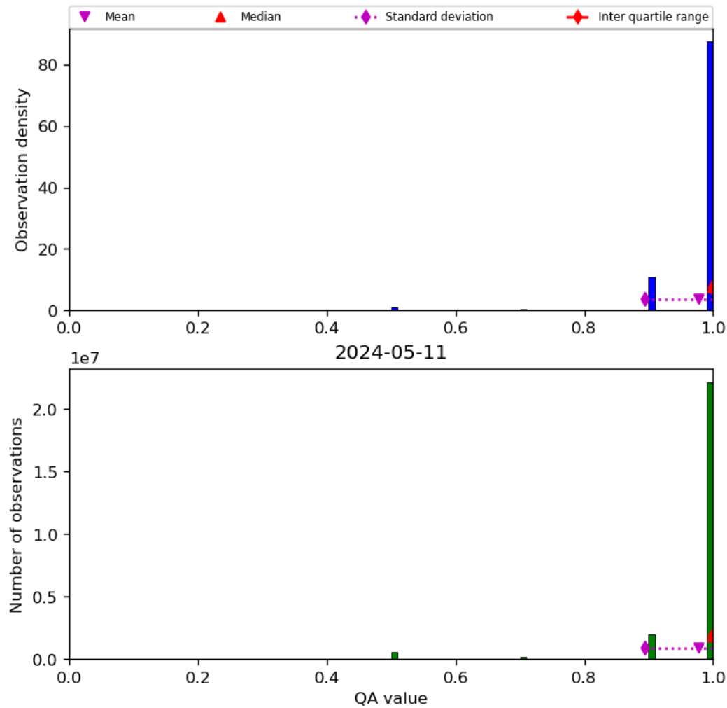
Figure 29: Histogram of “QA value” for 2024-05-10 to 2024-05-12
