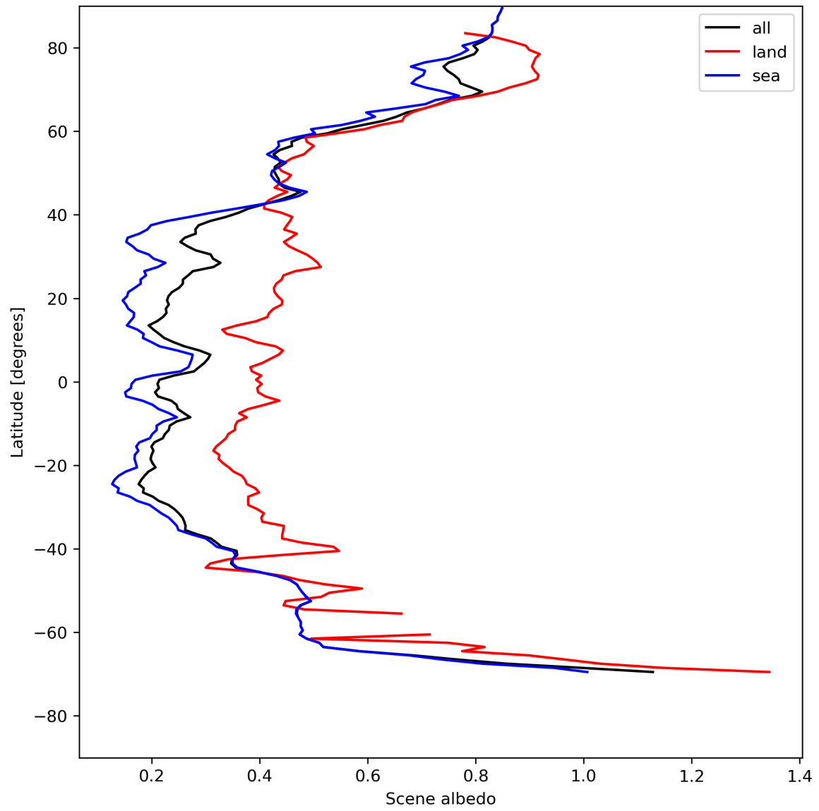
Figure 17: Zonal average of “Scene albedo” for 2024-05-10 to 2024-05-12.
