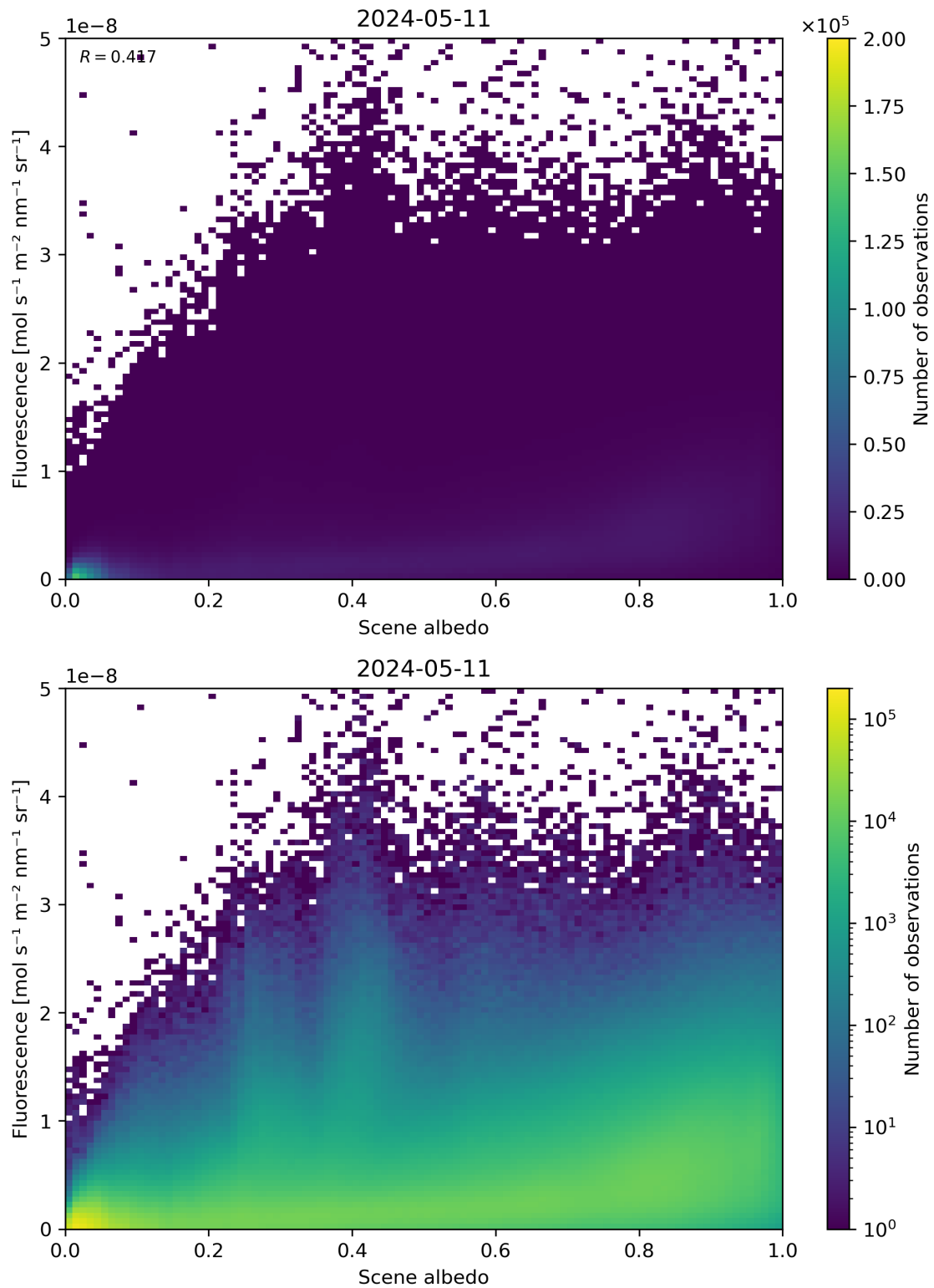
Figure 104: Scatter density plot of “Scene albedo” against “Fluorescence” for 2024-05-10 to 2024-05-12.
