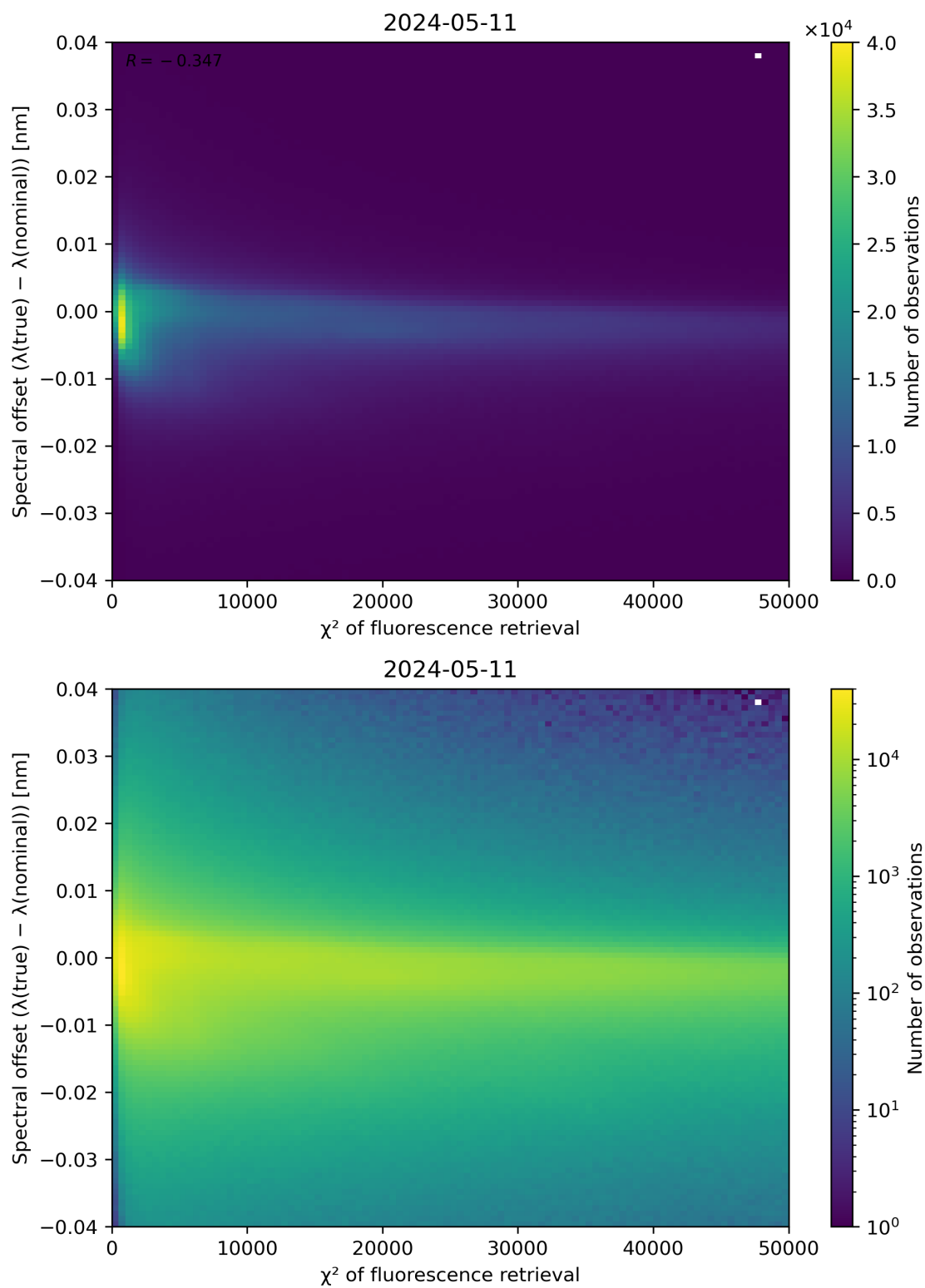
Figure 69: Scatter density plot of “ \chi^2 of fluorescence retrieval” against “Spectral offset ( \lambda(\text{true}) - \lambda(\text{nominal}) )” for 2024-05-10 to 2024-05-12.
