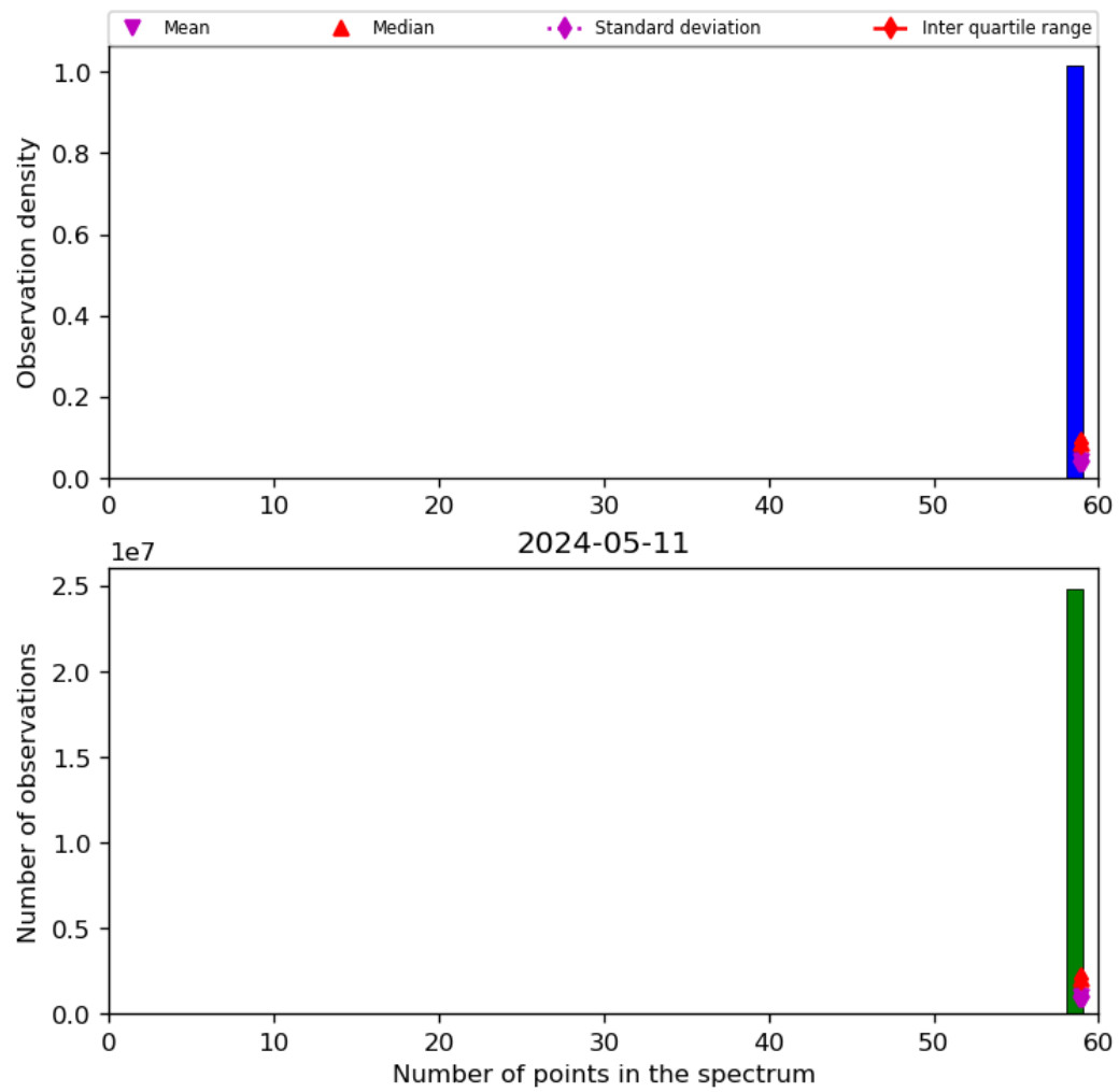
Figure 44: Histogram of “Number of points in the spectrum” for 2024-05-10 to 2024-05-12
