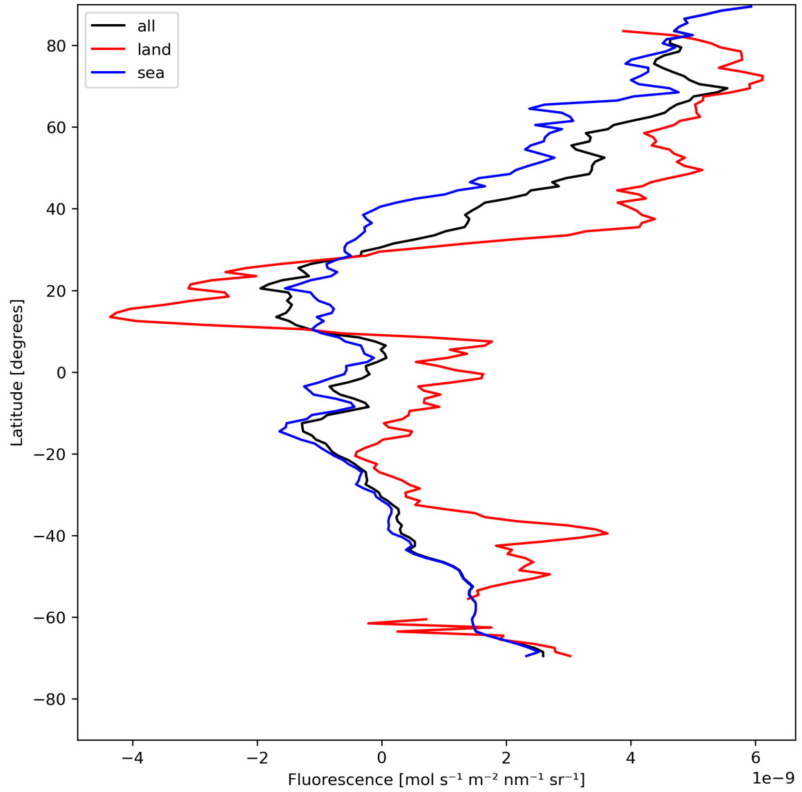
Figure 23: Zonal average of “Fluorescence” for 2024-05-10 to 2024-05-12.
