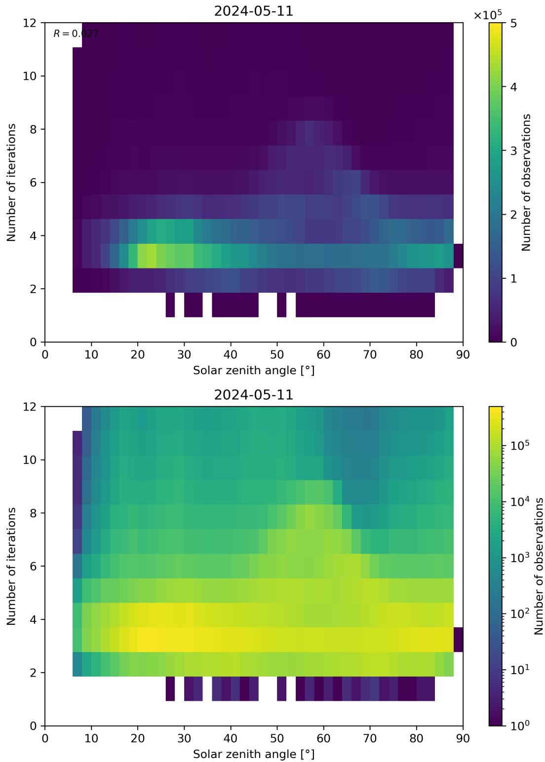
Figure 114: Scatter density plot of “Solar zenith angle” against “Number of iterations” for 2024-05-10 to 2024-05-12.
