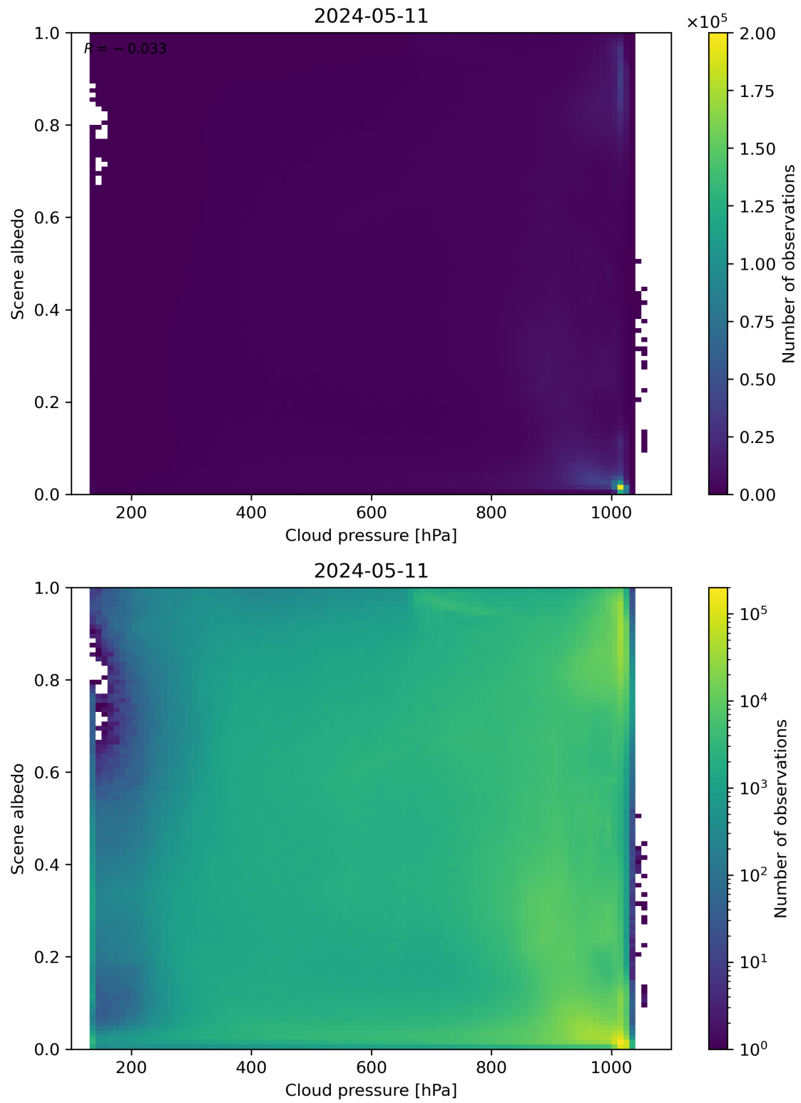
Figure 83: Scatter density plot of “Cloud pressure” against “Scene albedo” for 2024-05-10 to 2024-05-12.
