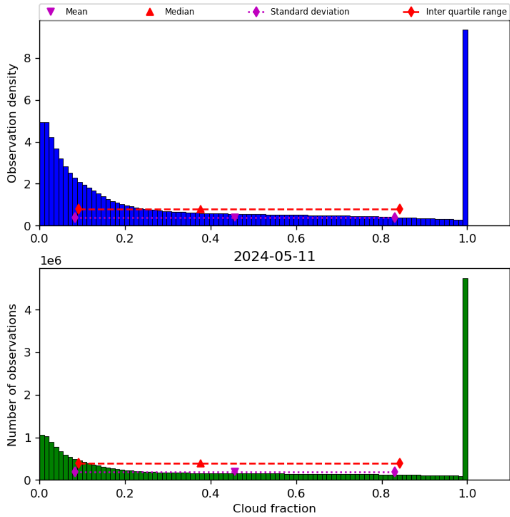
Figure 32: Histogram of “Cloud fraction” for 2024-05-10 to 2024-05-12
