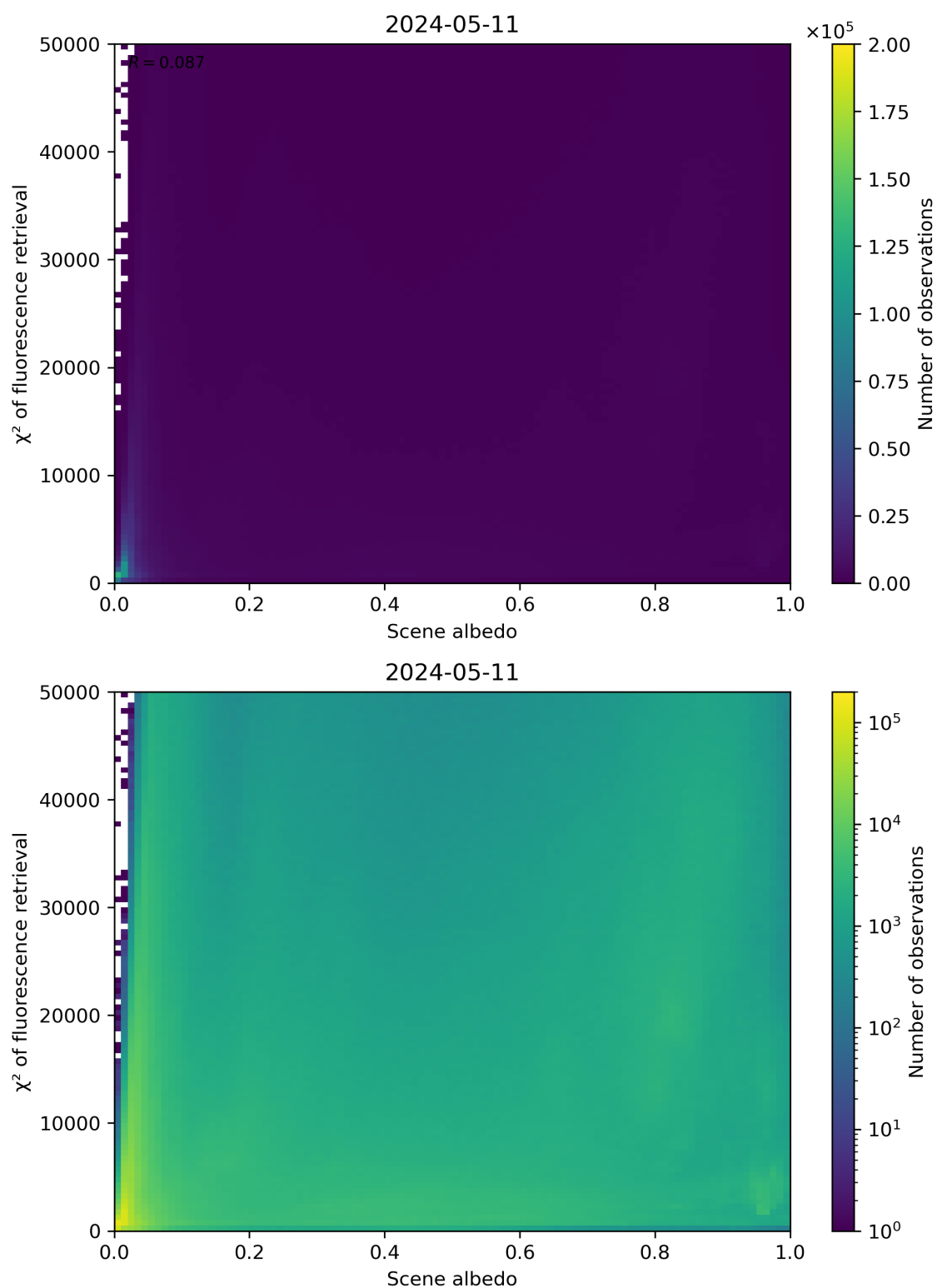
Figure 103: Scatter density plot of “Scene albedo” against “ \chi^2 of fluorescence retrieval” for 2024-05-10 to 2024-05-12.
