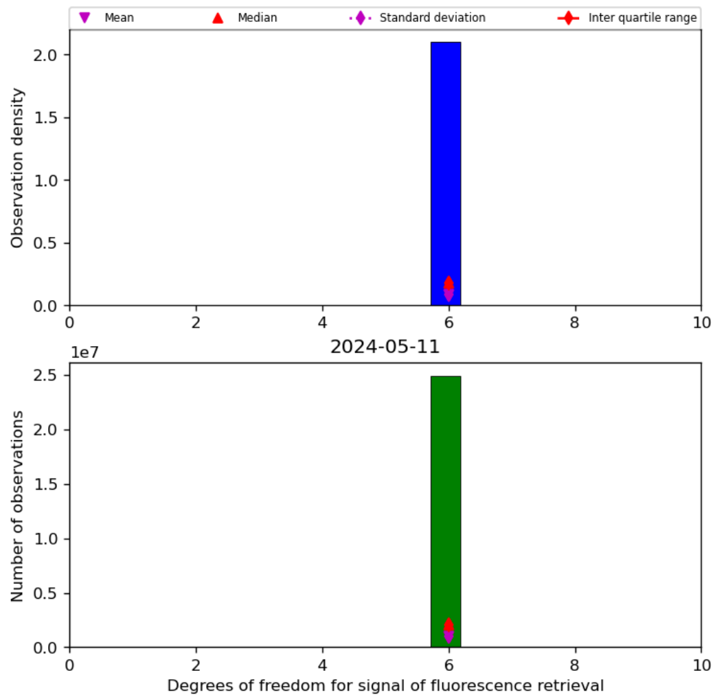
Figure 43: Histogram of “Degrees of freedom for signal of fluorescence retrieval” for 2024-05-10 to 2024-05-12
