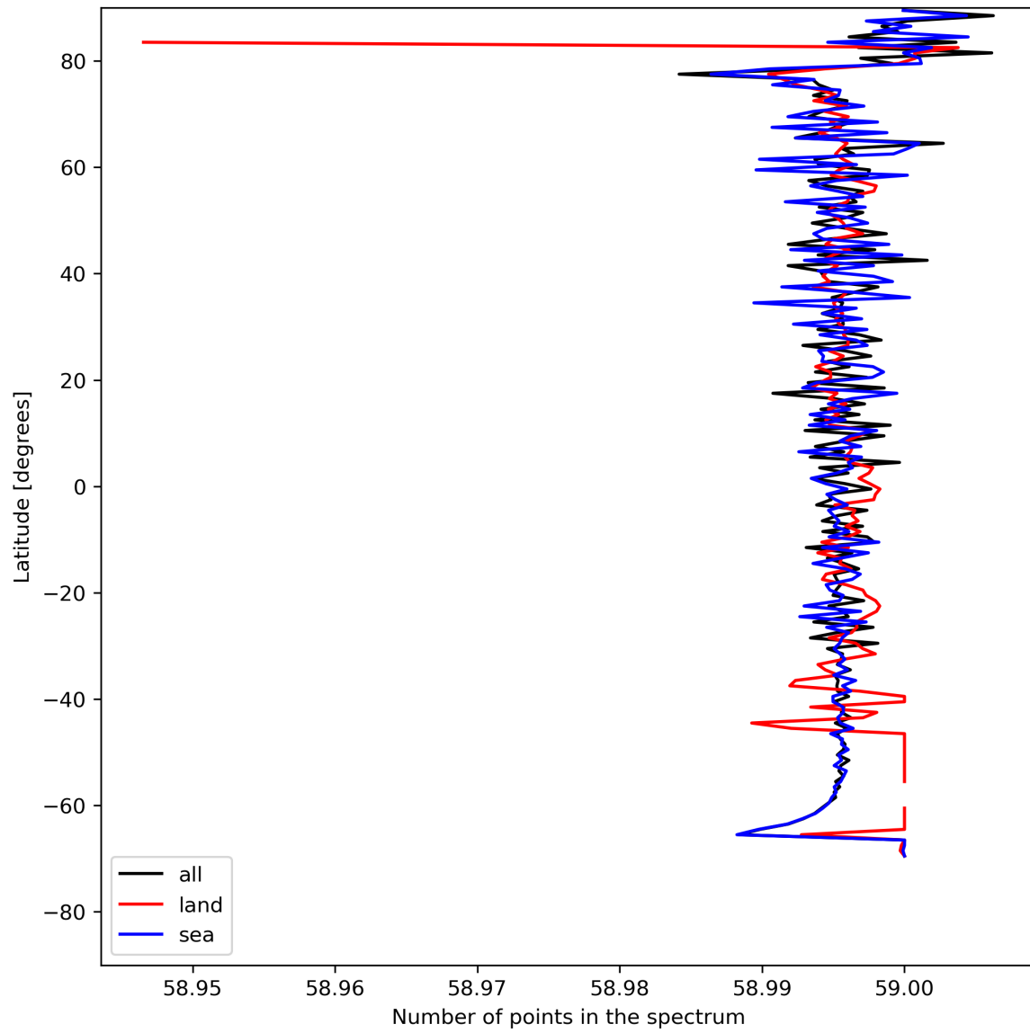
Figure 27: Zonal average of “Number of points in the spectrum” for 2024-05-10 to 2024-05-12.
