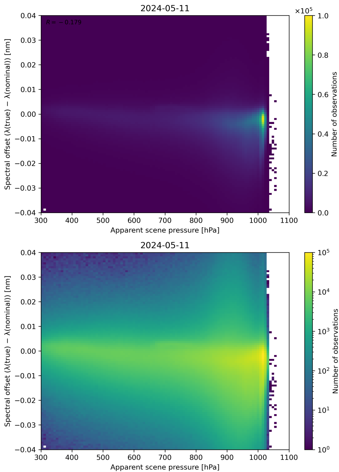
Figure 67: Scatter density plot of “Apparent scene pressure” against “Spectral offset ( \lambda(\text{true}) - \lambda(\text{nominal}) )” for 2024-05-10 to 2024-05-12.
