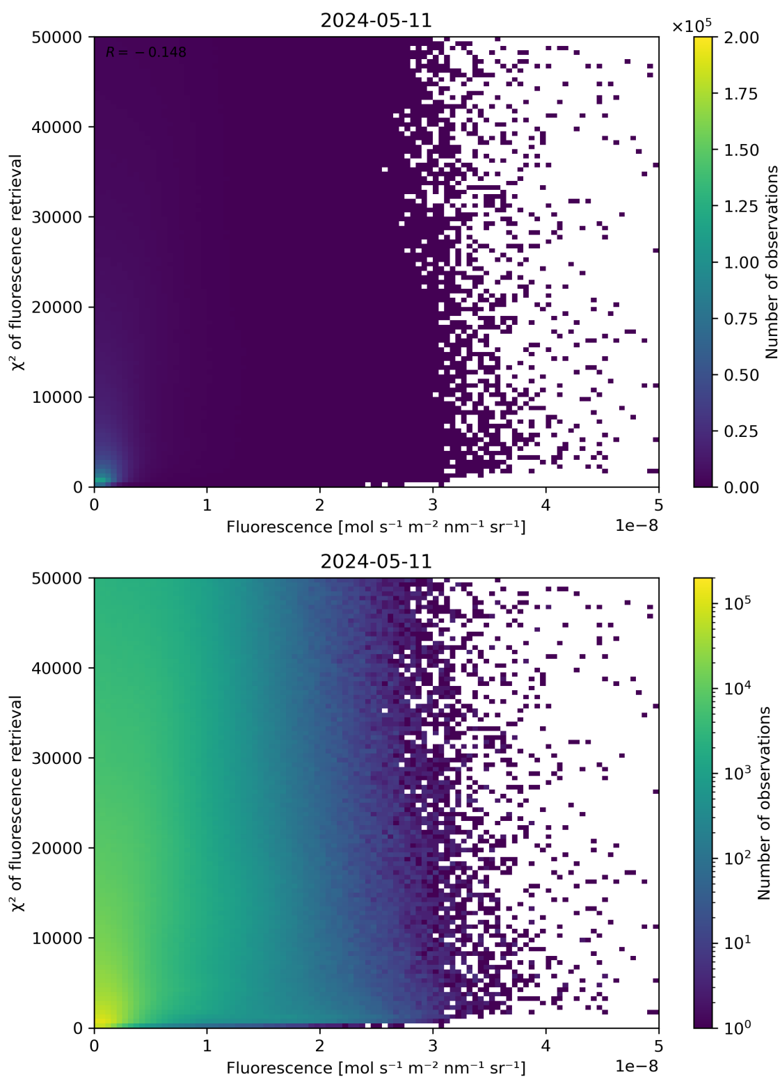
Figure 85: Scatter density plot of “Fluorescence” against “ \chi^2 of fluorescence retrieval” for 2024-05-10 to 2024-05-12.
