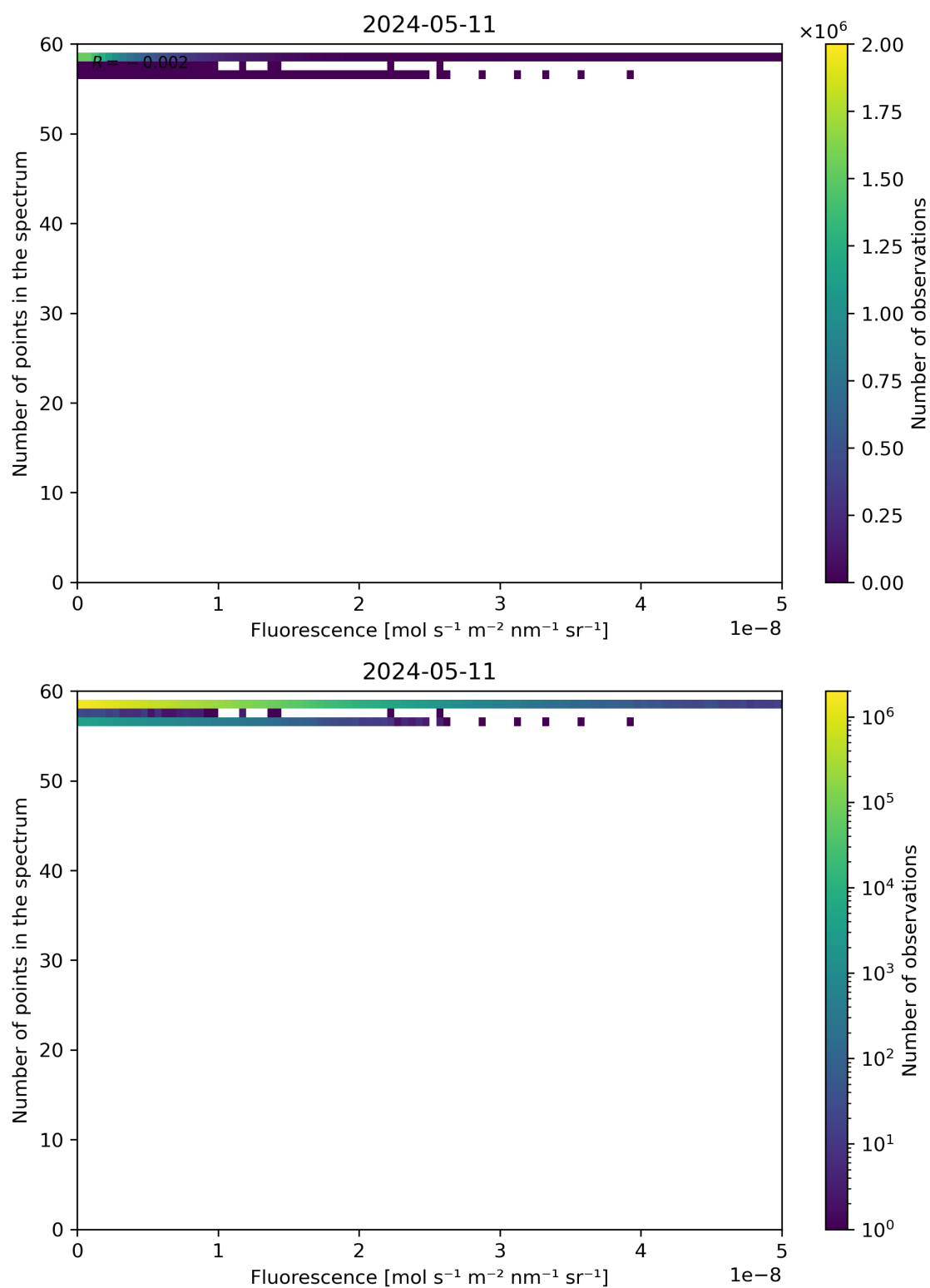
Figure 86: Scatter density plot of “Fluorescence” against “Number of points in the spectrum” for 2024-05-10 to 2024-05-12.
