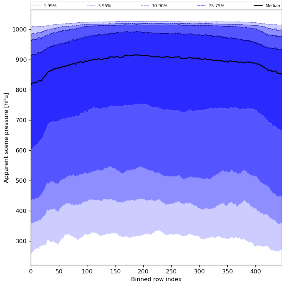
Figure 53: Along track statistics of “Apparent scene pressure” for 2024-05-10 to 2024-05-12
