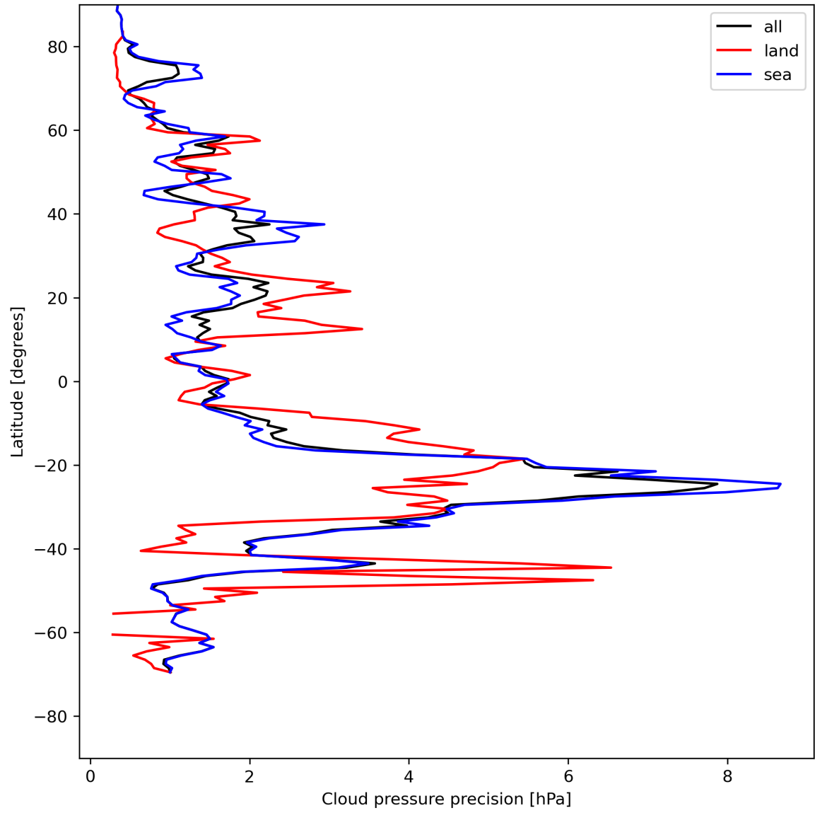
Figure 14: Zonal average of “Cloud pressure precision” for 2024-05-10 to 2024-05-12.
