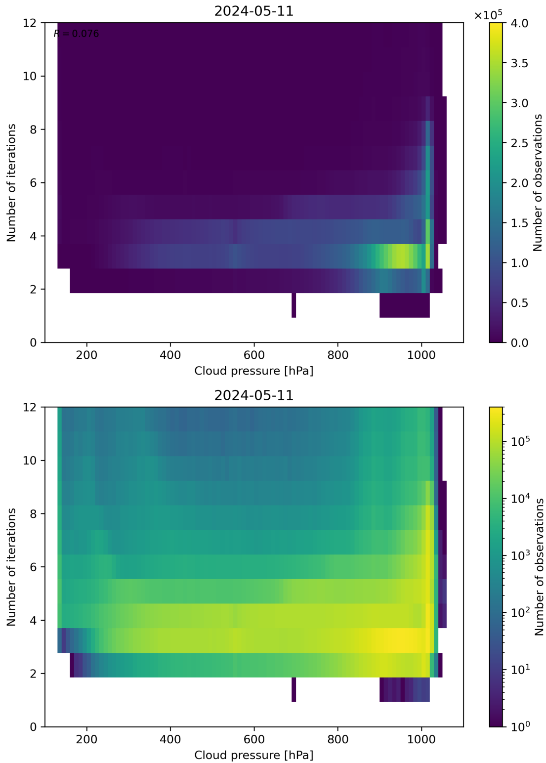
Figure 81: Scatter density plot of “Cloud pressure” against “Number of iterations” for 2024-05-10 to 2024-05-12.
