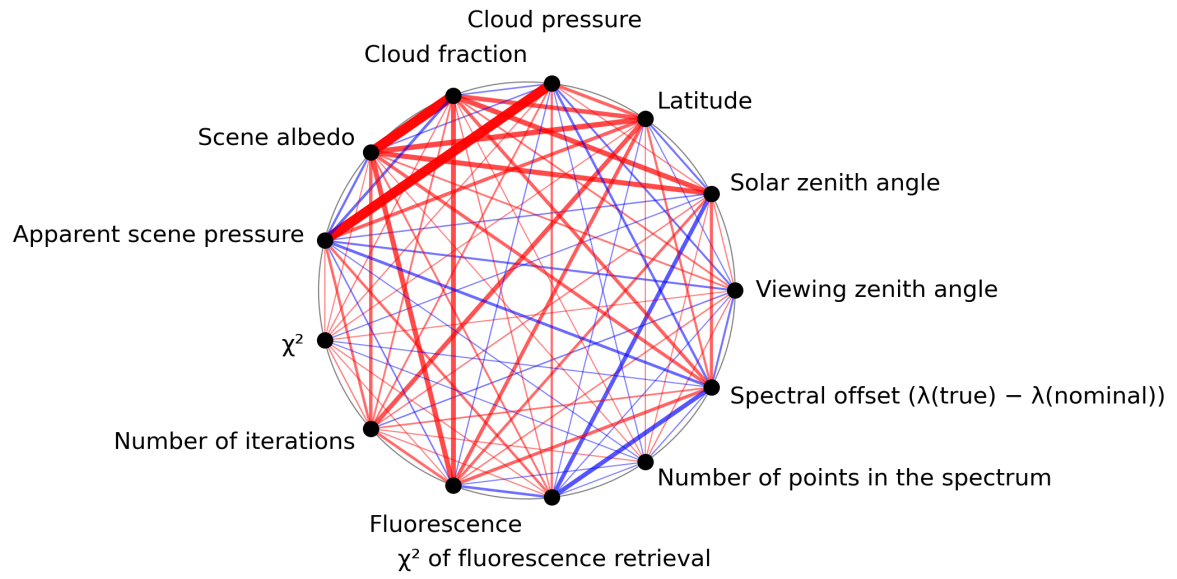
Figure 1: Map of correlation graph for 2024-05-10 to 2024-05-12.
