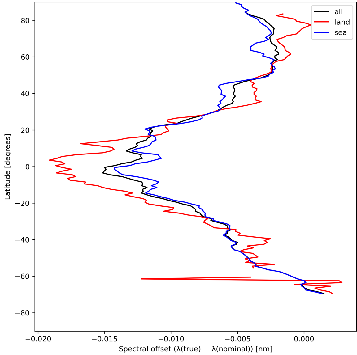
Figure 28: Zonal average of “Spectral offset ( \lambda(\text{true}) - \lambda(\text{nominal}) )” for 2024-05-10 to 2024-05-12.
