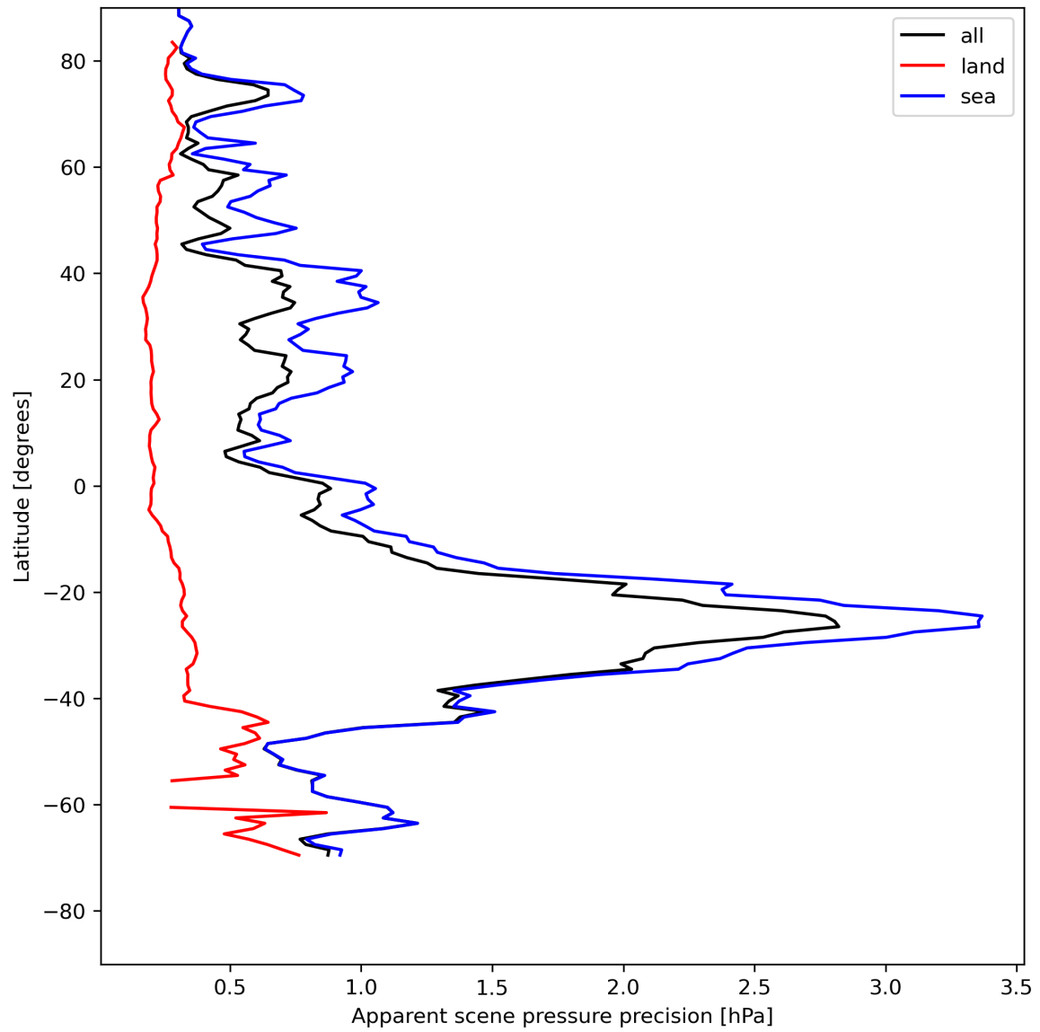
Figure 20: Zonal average of “Apparent scene pressure precision” for 2024-05-10 to 2024-05-12.
