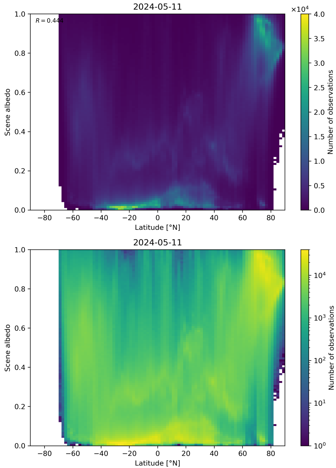
Figure 95: Scatter density plot of “Latitude” against “Scene albedo” for 2024-05-10 to 2024-05-12.
