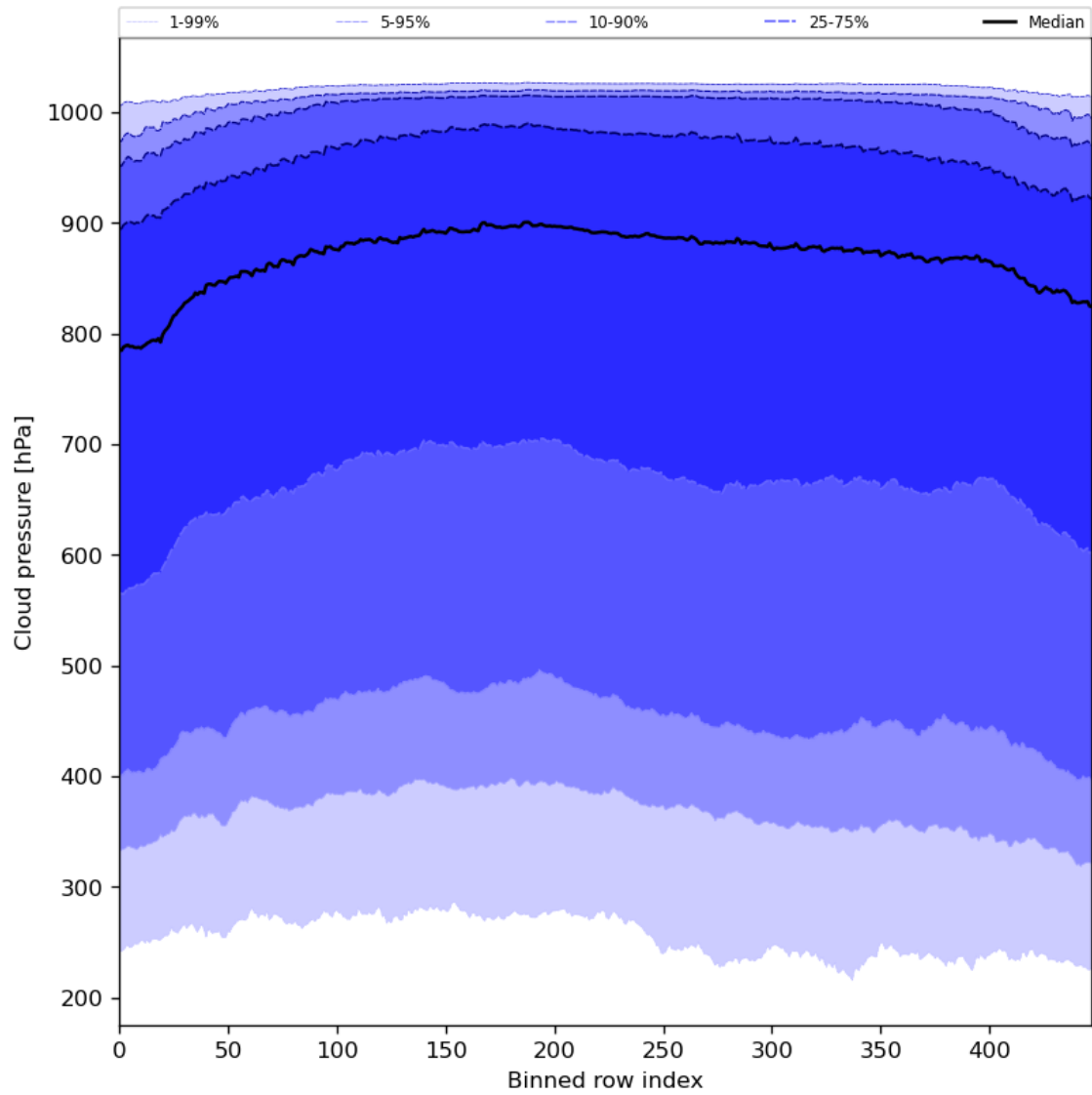
Figure 47: Along track statistics of “Cloud pressure” for 2024-05-10 to 2024-05-12
