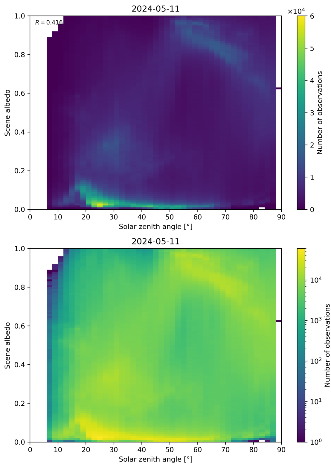
Figure 116: Scatter density plot of “Solar zenith angle” against “Scene albedo” for 2024-05-10 to 2024-05-12.
