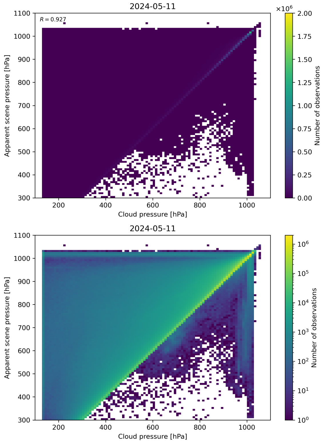
Figure 77: Scatter density plot of “Cloud pressure” against “Apparent scene pressure” for 2024-05-10 to 2024-05-12.
