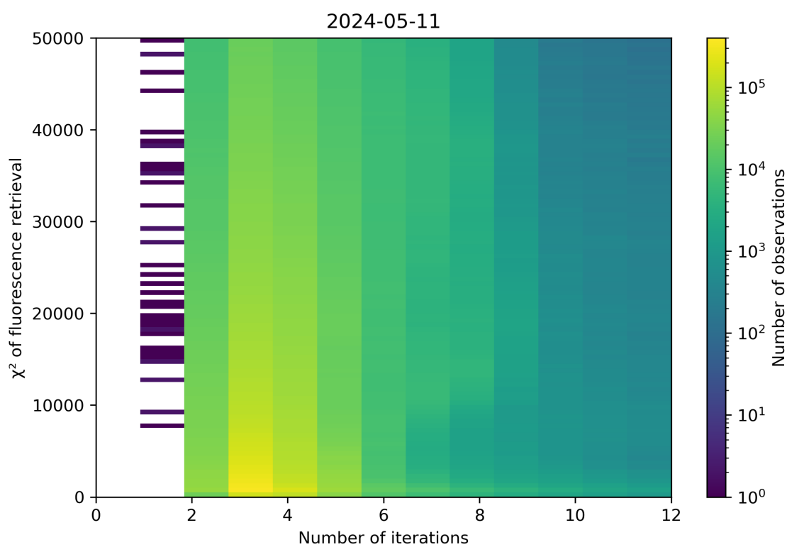
Figure 97: Scatter density plot of “Number of iterations” against “ \chi^2 of fluorescence retrieval” for 2024-05-10 to 2024-05-12.
