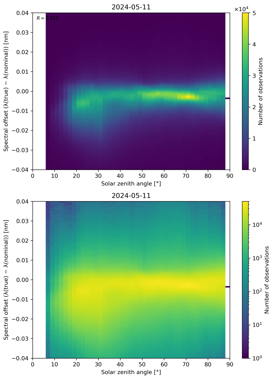
Figure 117: Scatter density plot of “Solar zenith angle” against “Spectral offset ( \lambda(\text{true}) - \lambda(\text{nominal}) )” for 2024-05-10 to 2024-05-12.
