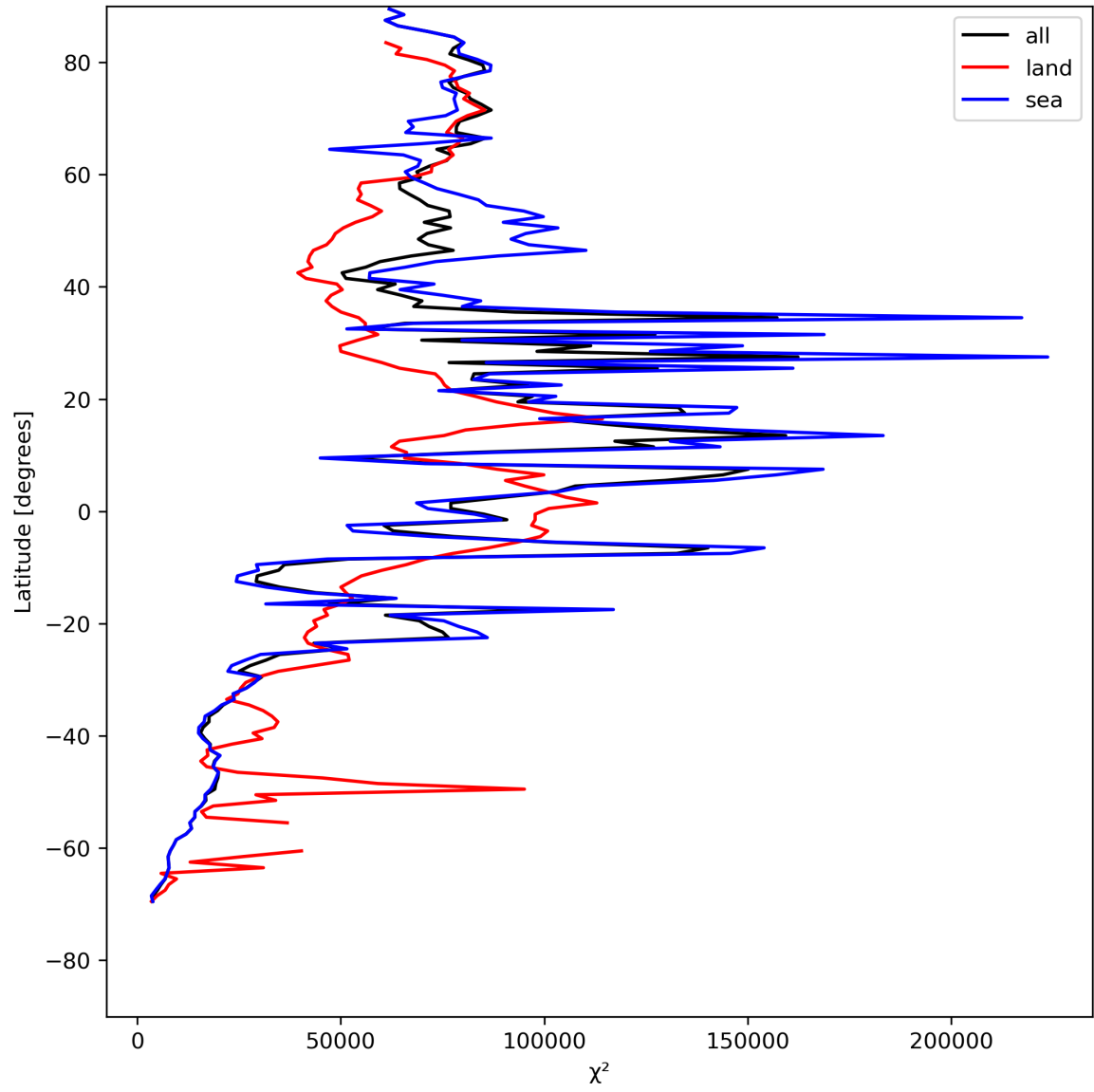
Figure 21: Zonal average of “ \chi^2 ” for 2024-05-12 to 2024-05-14.
