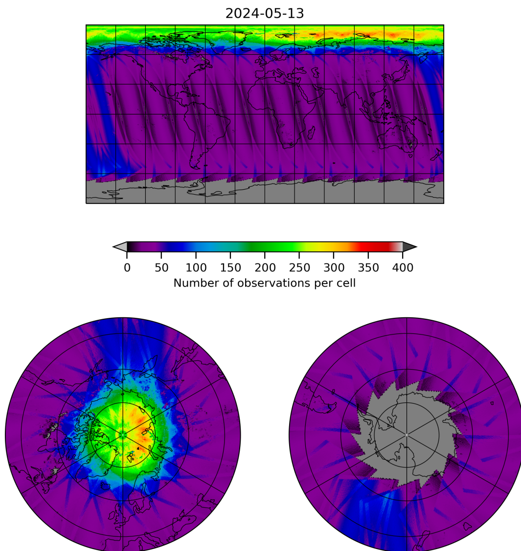
Figure 11: Map of the number of observations for 2024-05-12 to 2024-05-14
