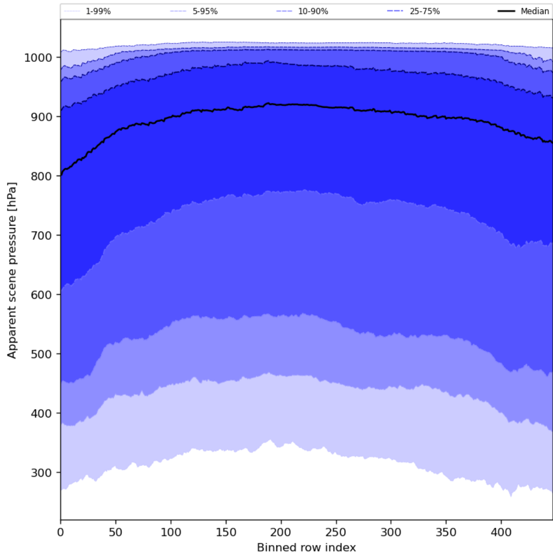
Figure 53: Along track statistics of “Apparent scene pressure” for 2024-05-12 to 2024-05-14
