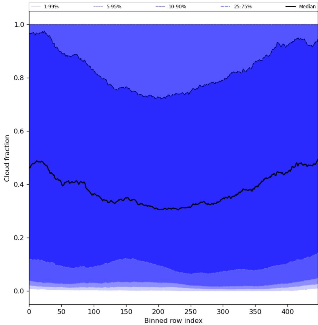
Figure 49: Along track statistics of “Cloud fraction” for 2024-05-12 to 2024-05-14
