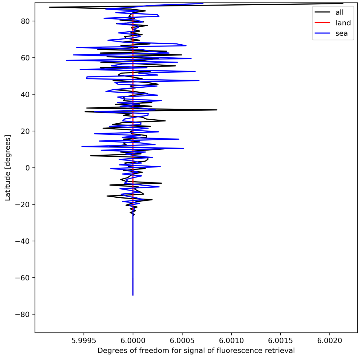
Figure 26: Zonal average of “Degrees of freedom for signal of fluorescence retrieval” for 2024-05-12 to 2024-05-14.
