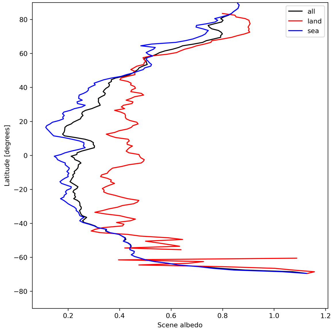
Figure 17: Zonal average of “Scene albedo” for 2024-05-12 to 2024-05-14.
