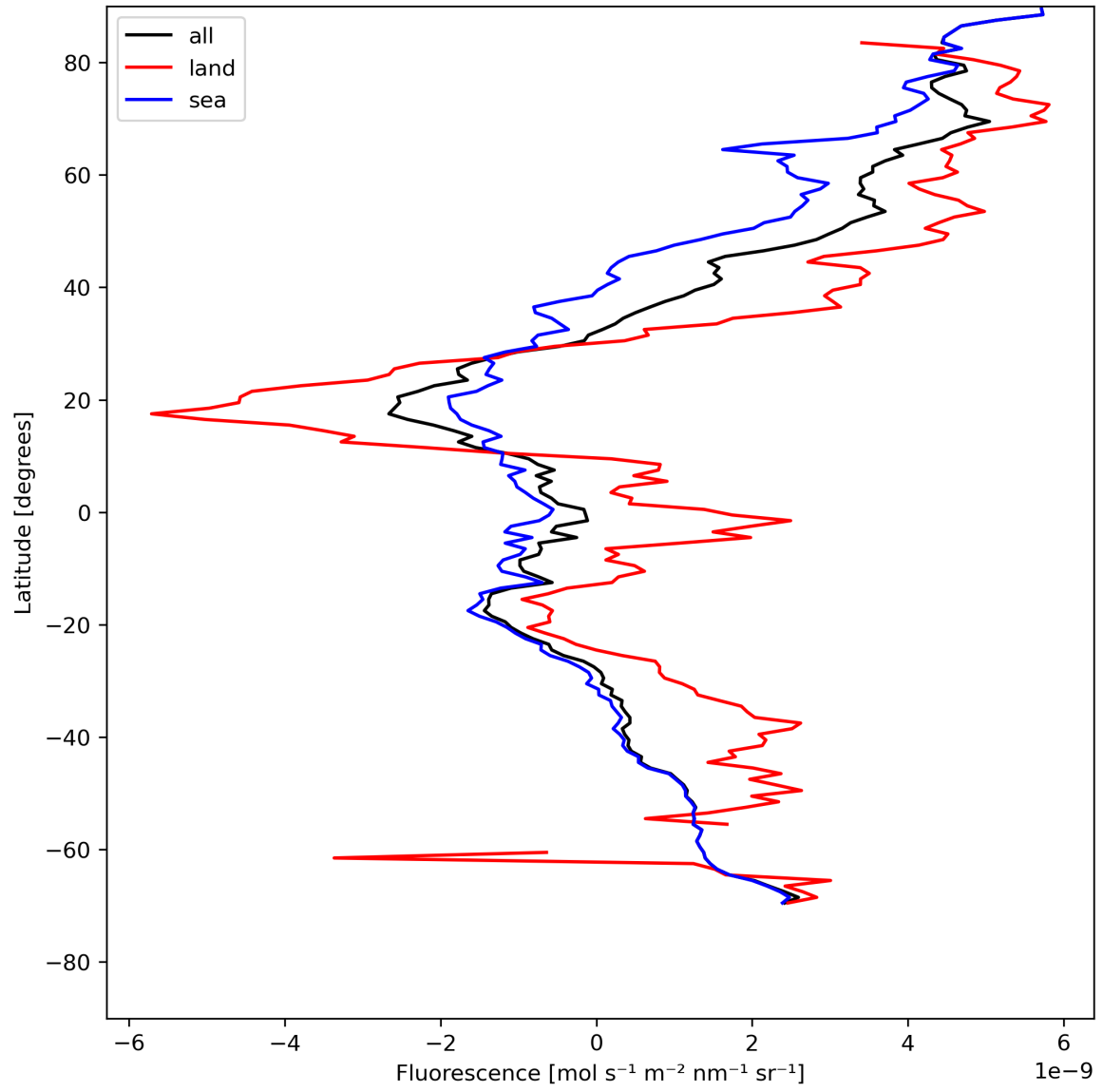
Figure 23: Zonal average of “Fluorescence” for 2024-05-12 to 2024-05-14.
