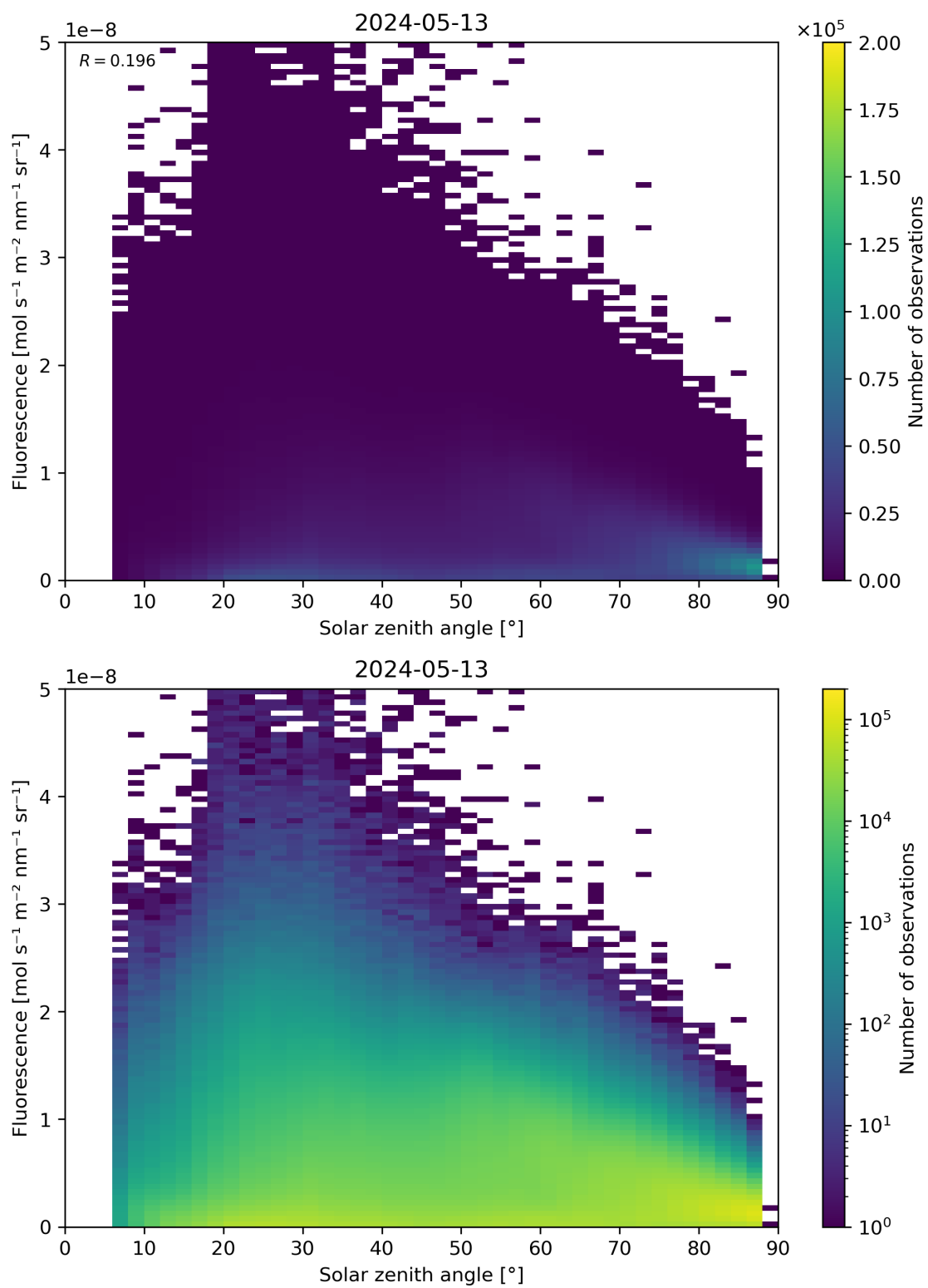
Figure 112: Scatter density plot of “Solar zenith angle” against “Fluorescence” for 2024-05-12 to 2024-05-14.
