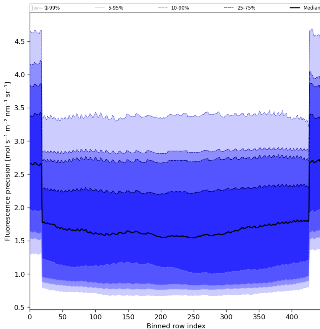
Figure 58: Along track statistics of “Fluorescence precision” for 2024-05-12 to 2024-05-14
