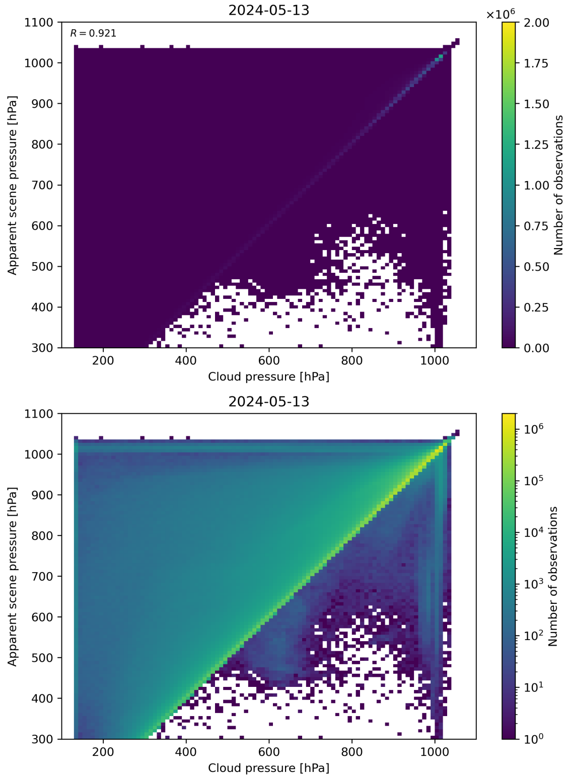
Figure 77: Scatter density plot of “Cloud pressure” against “Apparent scene pressure” for 2024-05-12 to 2024-05-14.
