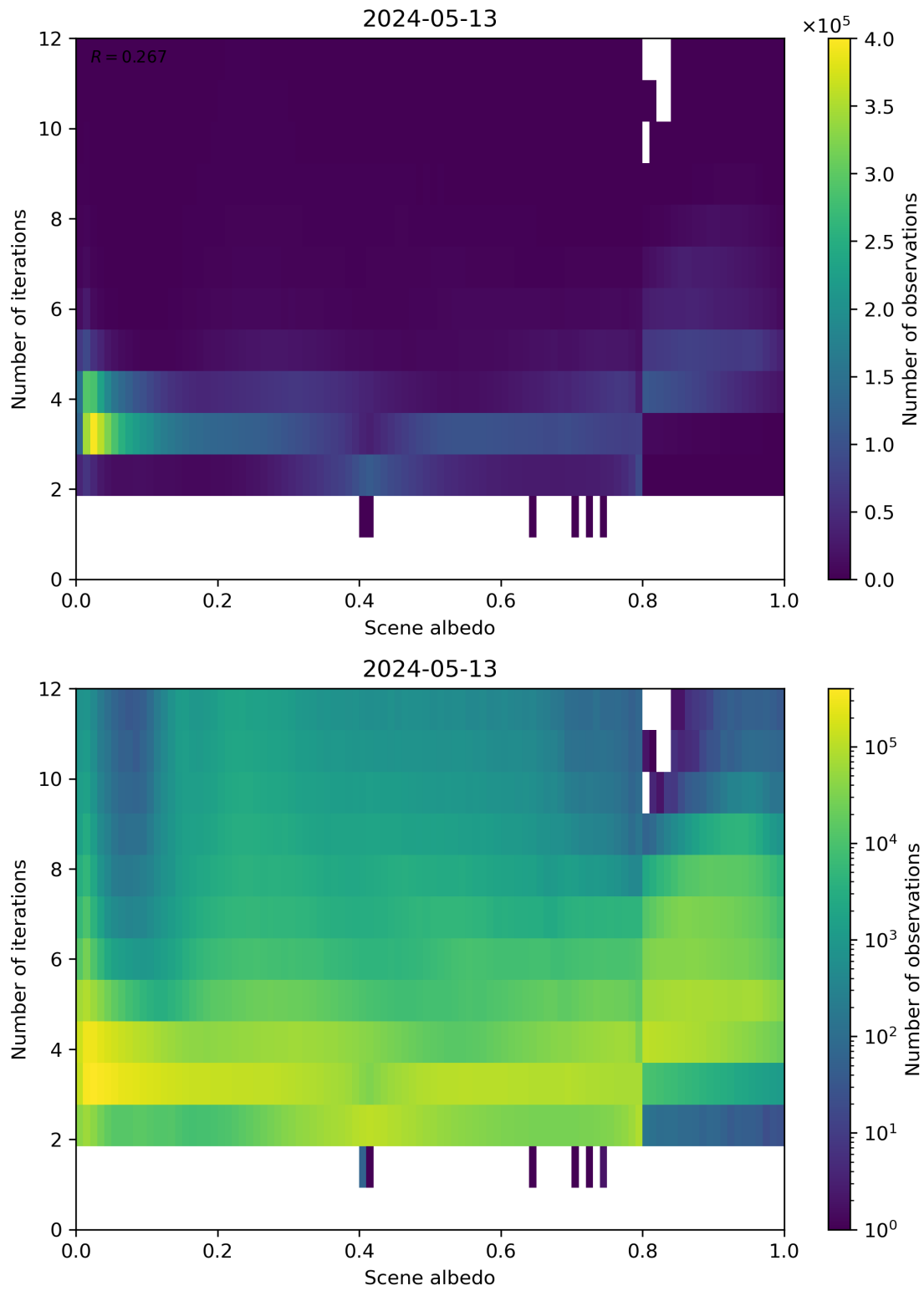
Figure 105: Scatter density plot of “Scene albedo” against “Number of iterations” for 2024-05-12 to 2024-05-14.
