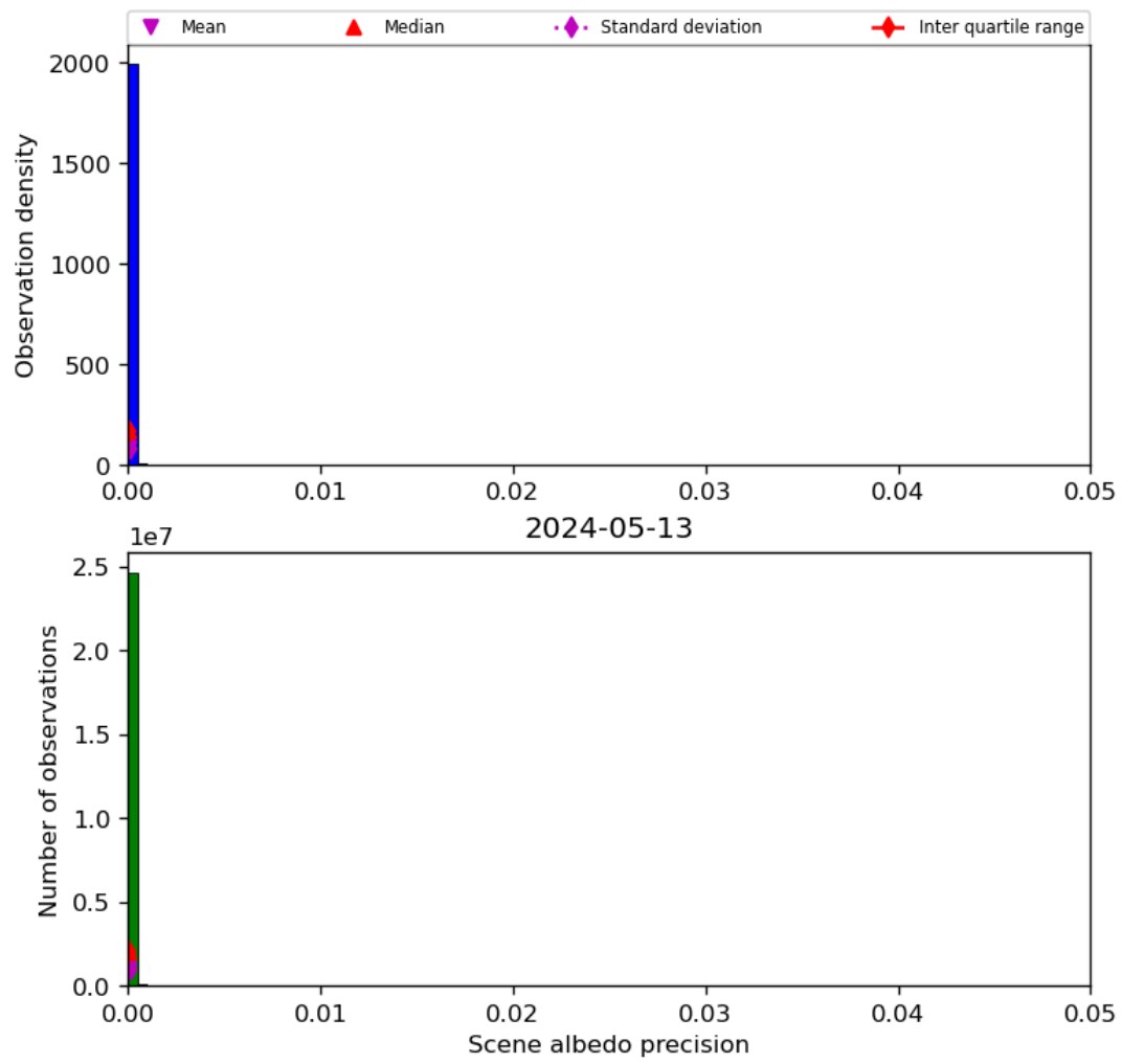
Figure 35: Histogram of “Scene albedo precision” for 2024-05-12 to 2024-05-14
