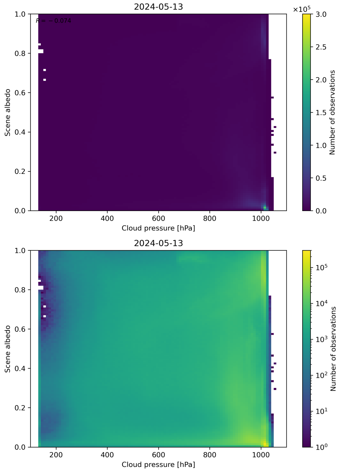
Figure 83: Scatter density plot of “Cloud pressure” against “Scene albedo” for 2024-05-12 to 2024-05-14.
