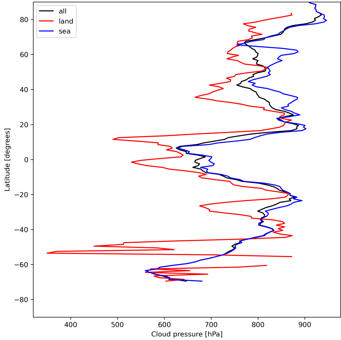
Figure 13: Zonal average of “Cloud pressure” for 2024-05-12 to 2024-05-14.
