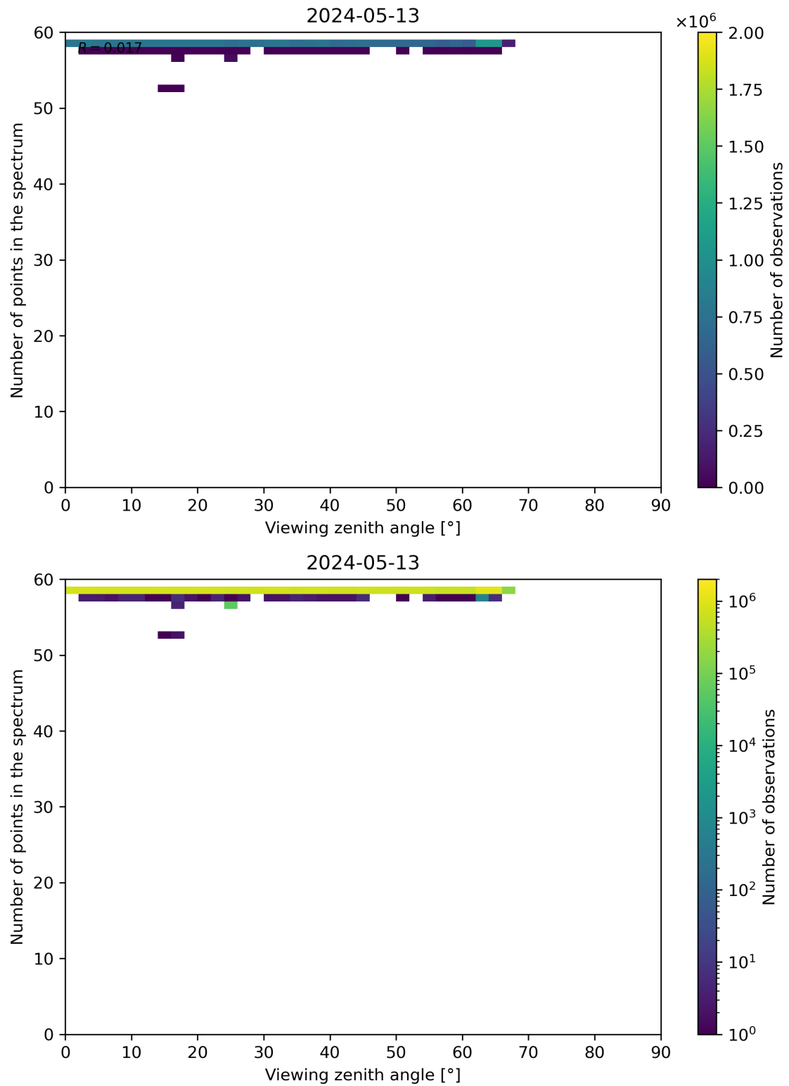
Figure 125: Scatter density plot of “Viewing zenith angle” against “Number of points in the spectrum” for 2024-05-12 to 2024-05-14.
