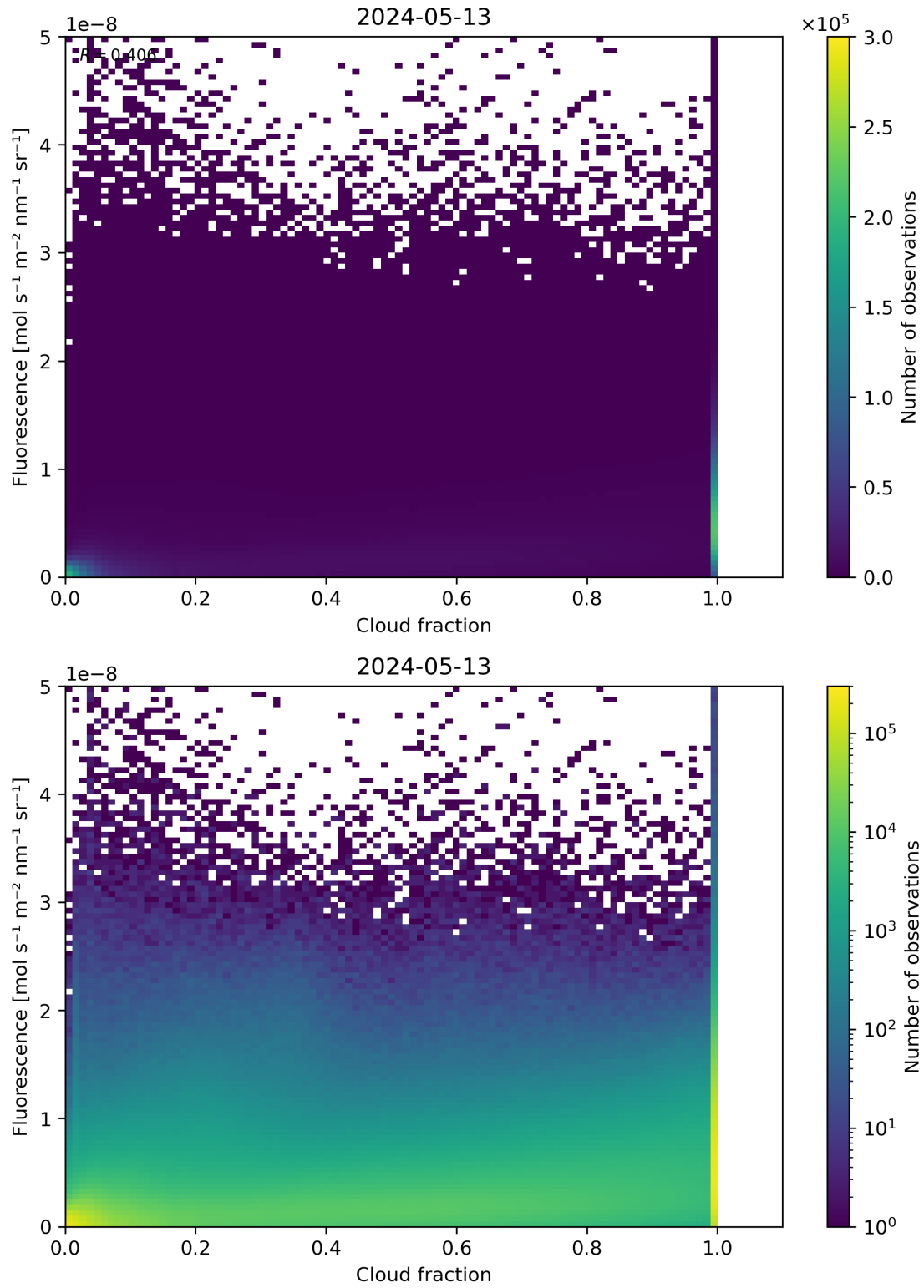
Figure 72: Scatter density plot of “Cloud fraction” against “Fluorescence” for 2024-05-12 to 2024-05-14.
