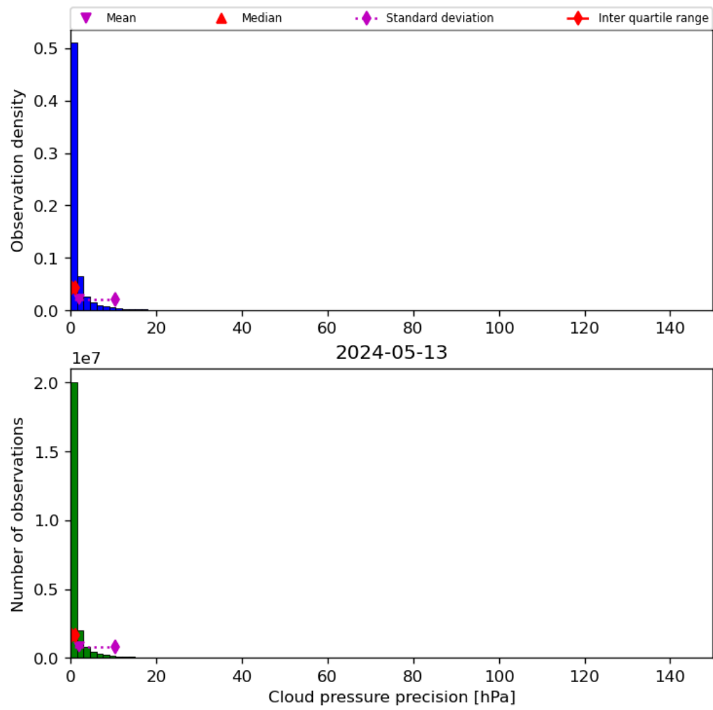
Figure 31: Histogram of “Cloud pressure precision” for 2024-05-12 to 2024-05-14
