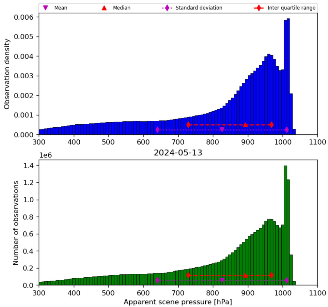
Figure 36: Histogram of “Apparent scene pressure” for 2024-05-12 to 2024-05-14
