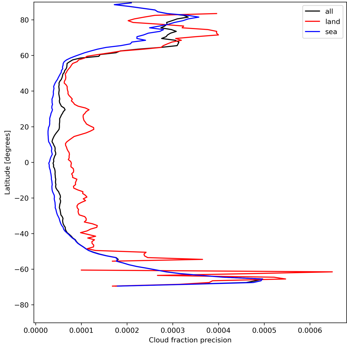
Figure 16: Zonal average of “Cloud fraction precision” for 2024-05-12 to 2024-05-14.
