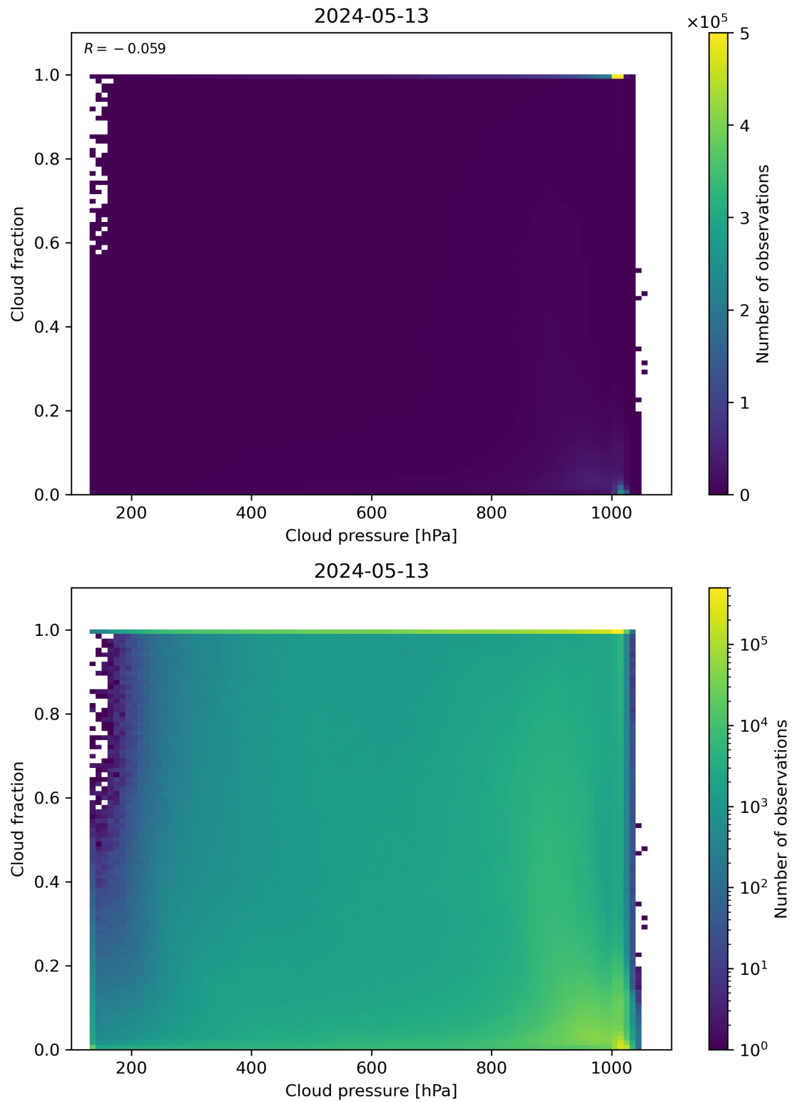
Figure 79: Scatter density plot of “Cloud pressure” against “Cloud fraction” for 2024-05-12 to 2024-05-14.
