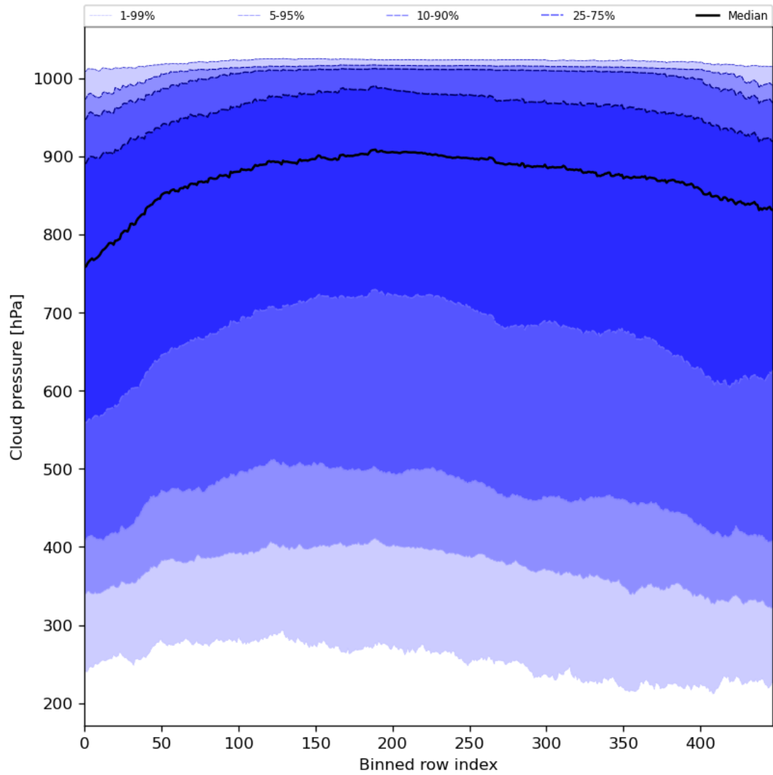
Figure 47: Along track statistics of “Cloud pressure” for 2024-05-12 to 2024-05-14
