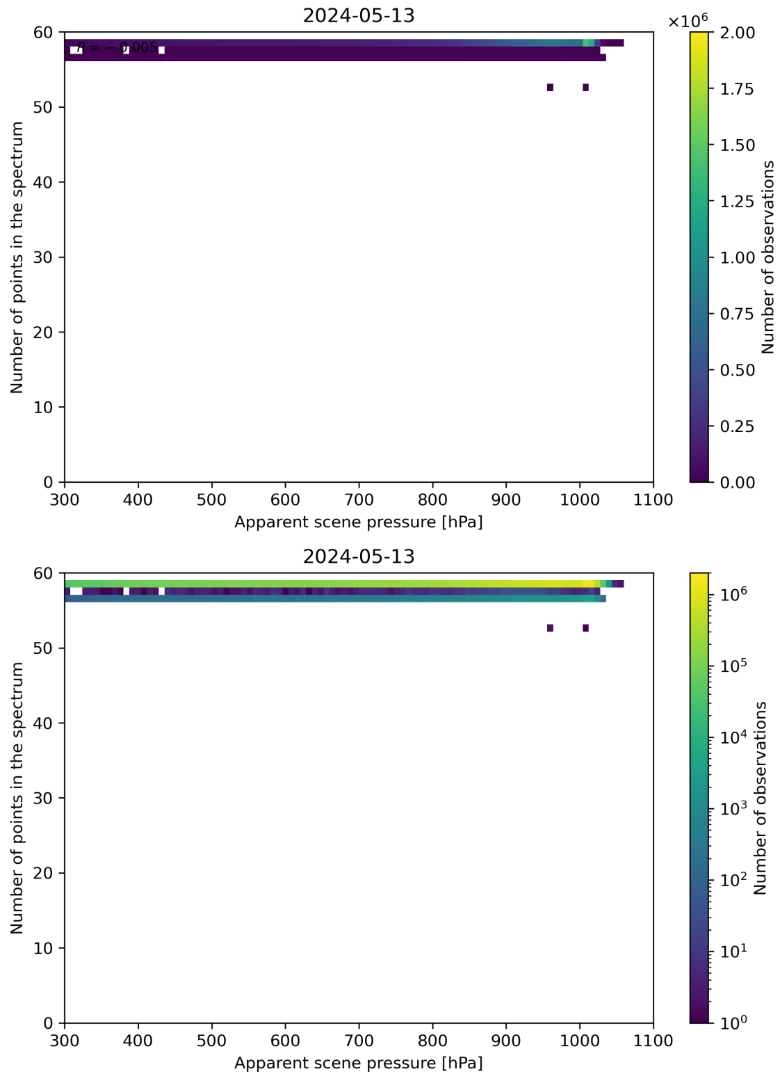
Figure 66: Scatter density plot of “Apparent scene pressure” against “Number of points in the spectrum” for 2024-05-12 to 2024-05-14.
