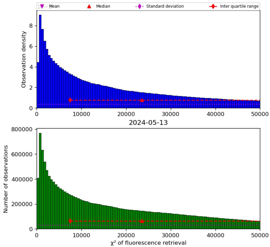
Figure 42: Histogram of “ \chi^2 of fluorescence retrieval” for 2024-05-12 to 2024-05-14
