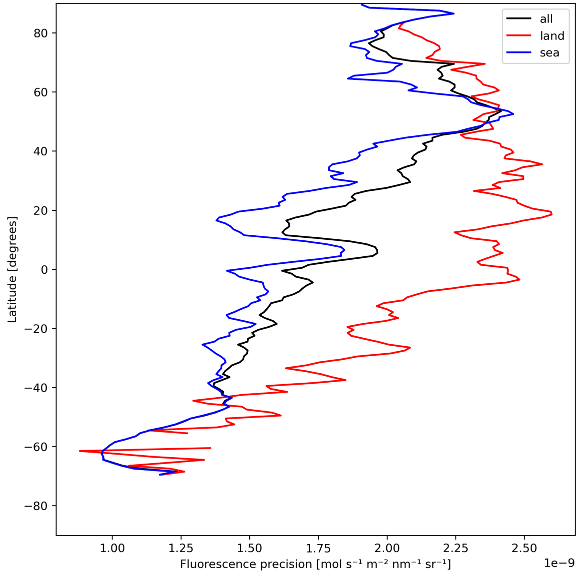
Figure 24: Zonal average of “Fluorescence precision” for 2024-05-12 to 2024-05-14.
