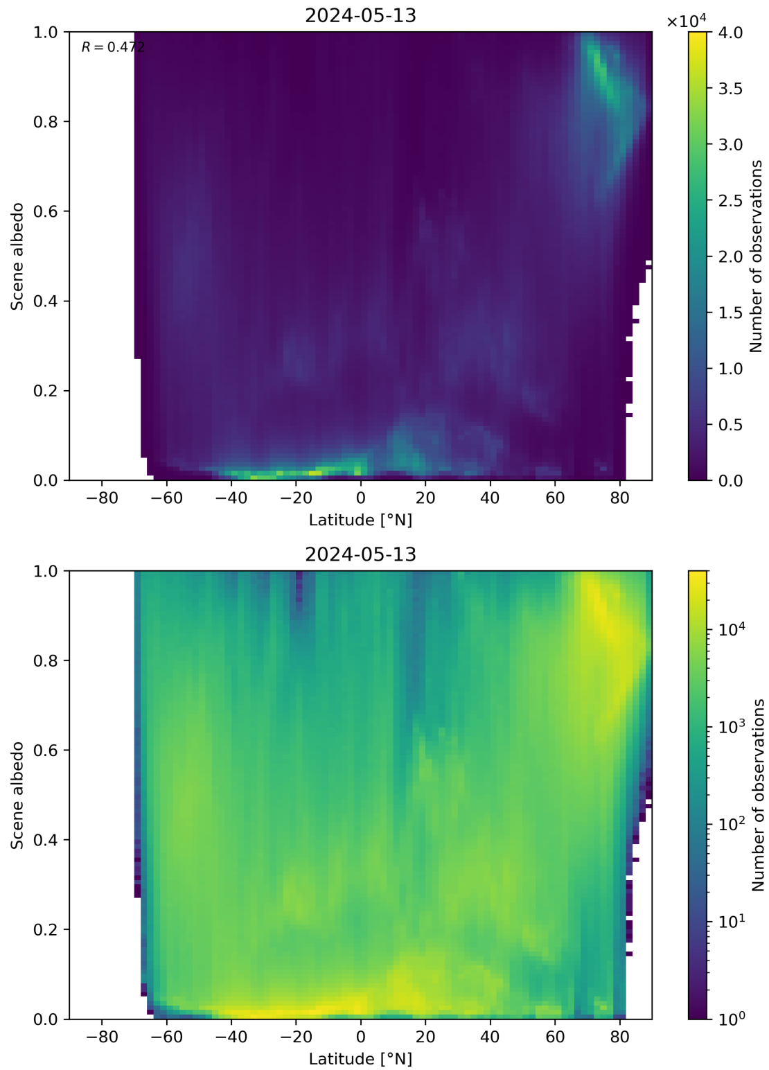
Figure 95: Scatter density plot of “Latitude” against “Scene albedo” for 2024-05-12 to 2024-05-14.
