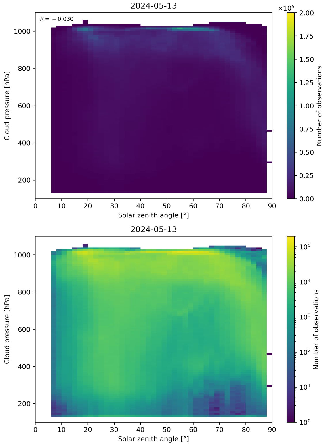
Figure 111: Scatter density plot of “Solar zenith angle” against “Cloud pressure” for 2024-05-12 to 2024-05-14.
