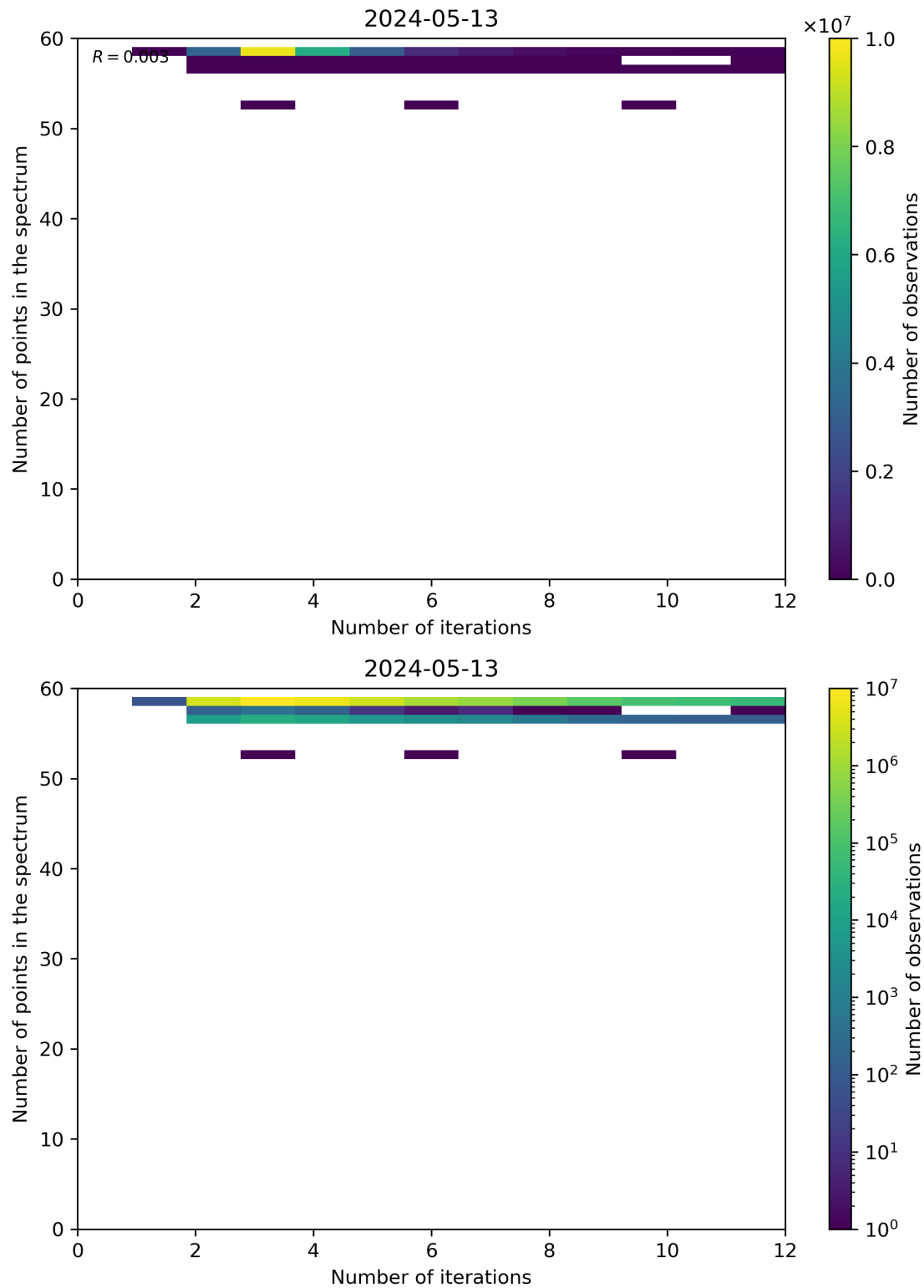
Figure 99: Scatter density plot of “Number of iterations” against “Number of points in the spectrum” for 2024-05-12 to 2024-05-14.
