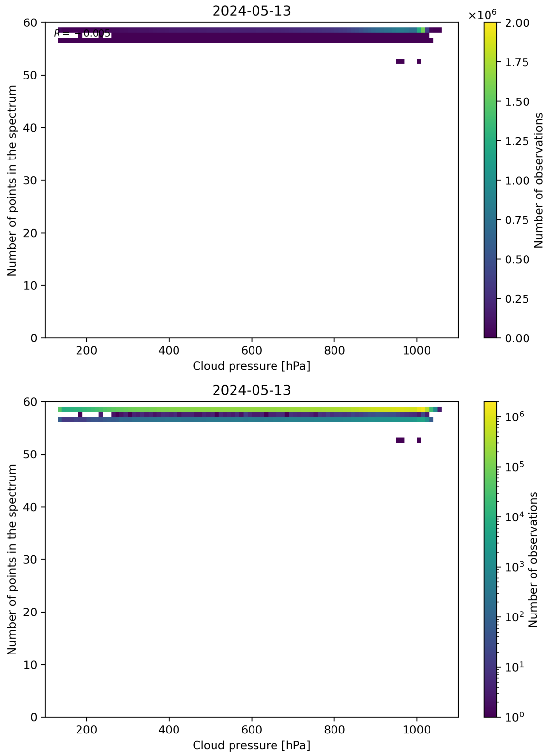
Figure 82: Scatter density plot of “Cloud pressure” against “Number of points in the spectrum” for 2024-05-12 to 2024-05-14.
