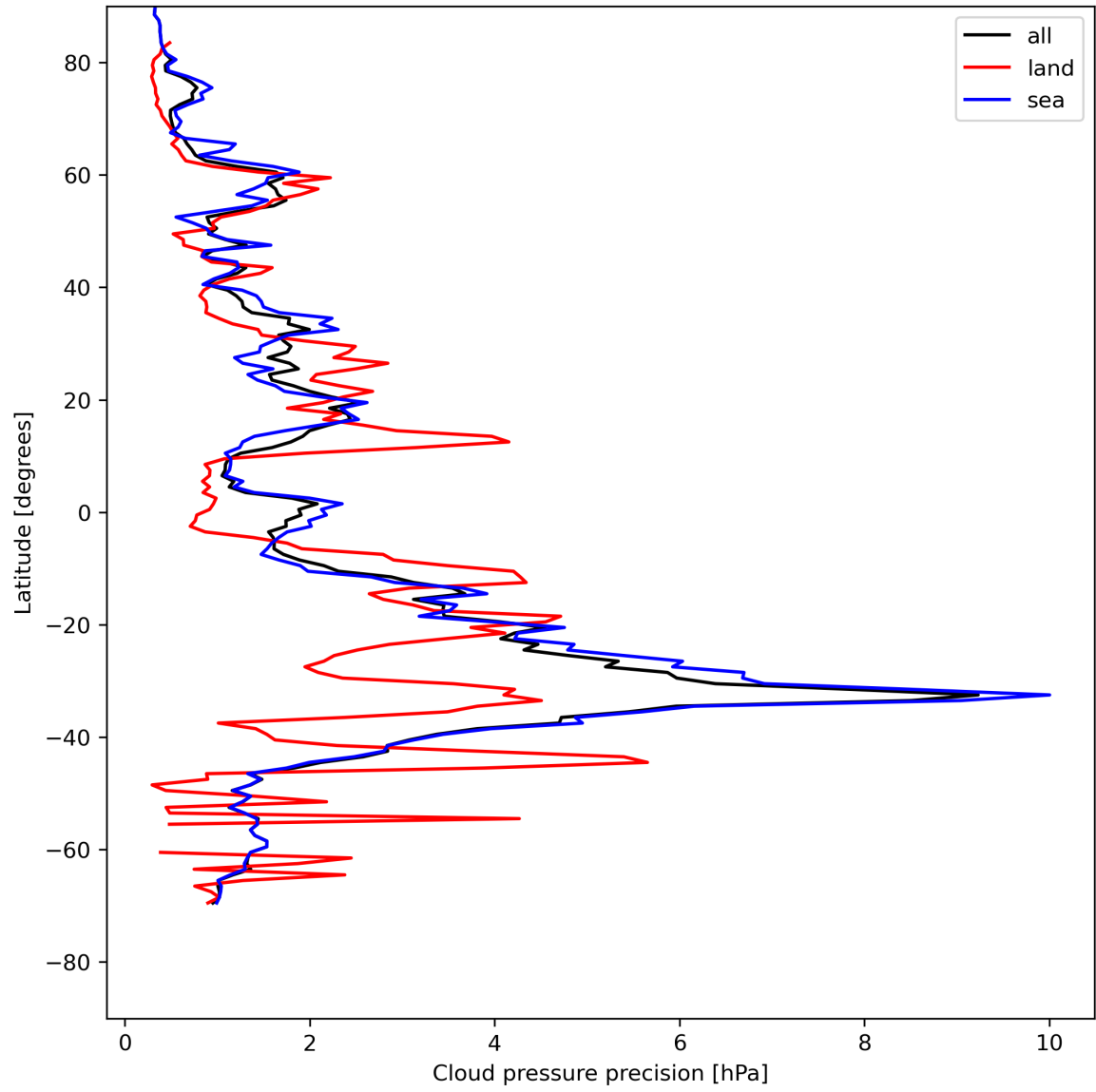
Figure 14: Zonal average of “Cloud pressure precision” for 2024-05-12 to 2024-05-14.
