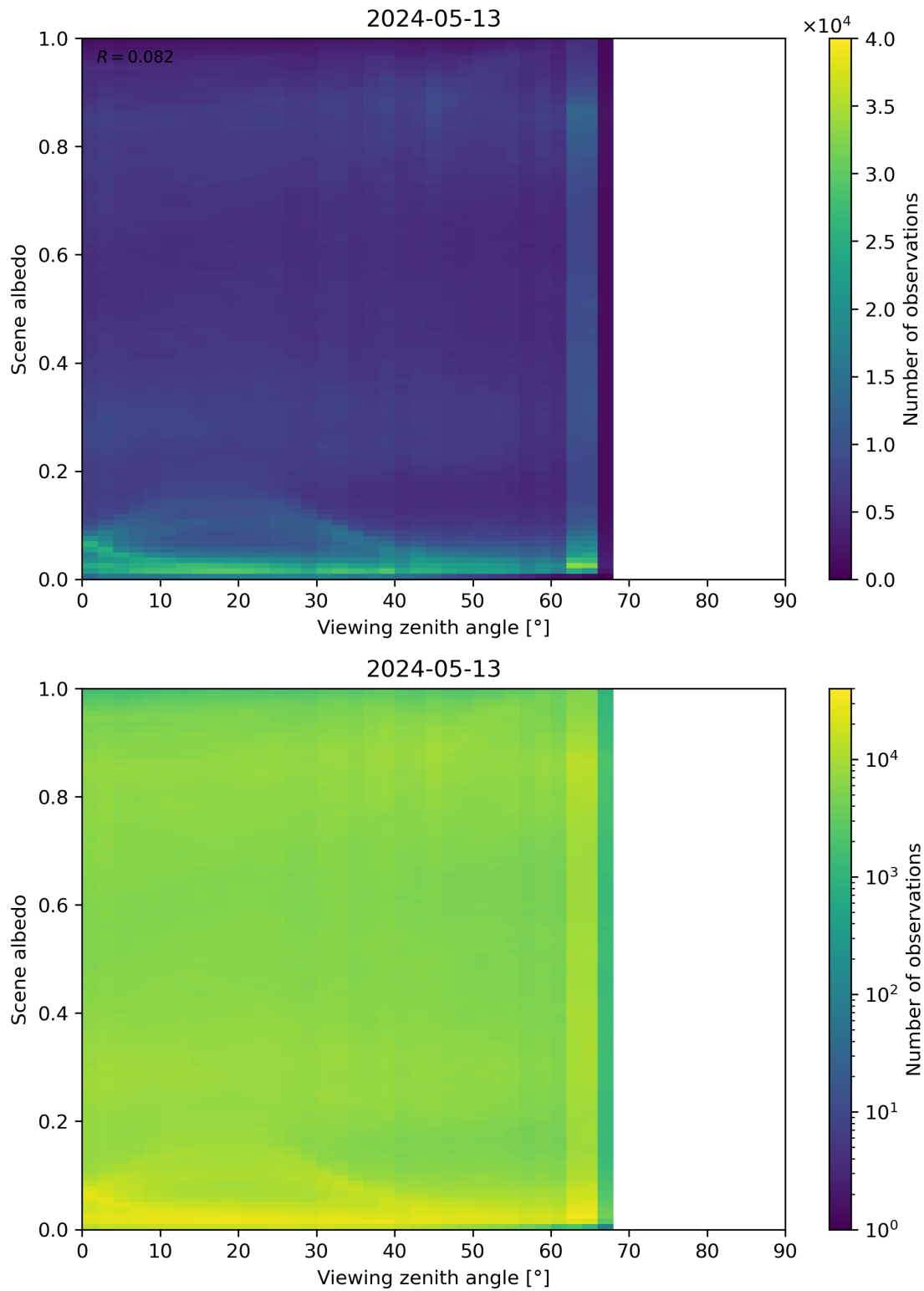
Figure 126: Scatter density plot of “Viewing zenith angle” against “Scene albedo” for 2024-05-12 to 2024-05-14.
