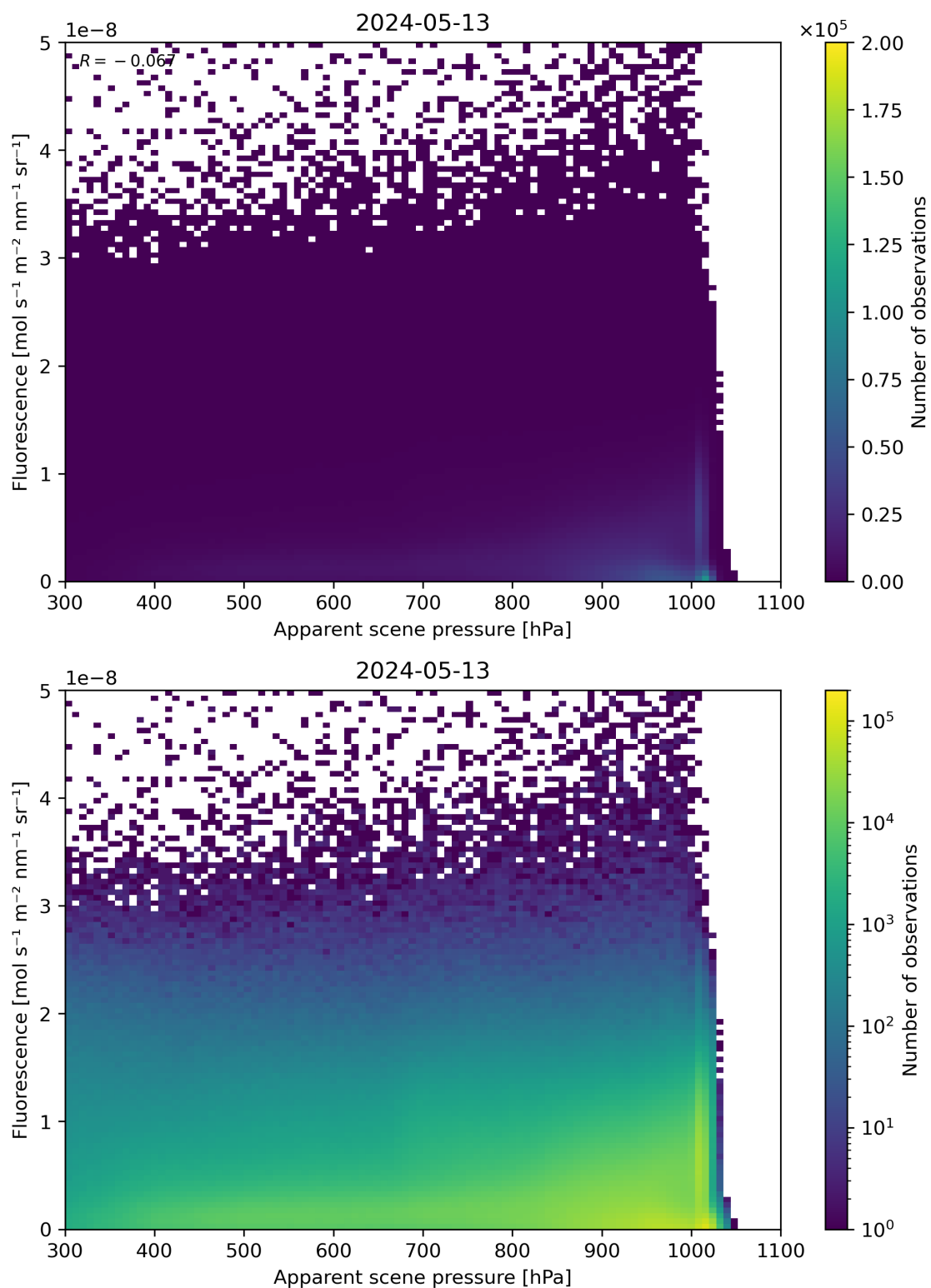
Figure 64: Scatter density plot of “Apparent scene pressure” against “Fluorescence” for 2024-05-12 to 2024-05-14.
