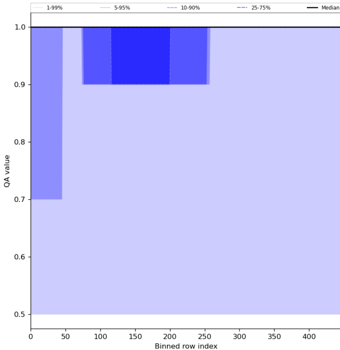
Figure 46: Along track statistics of “QA value” for 2024-05-12 to 2024-05-14
