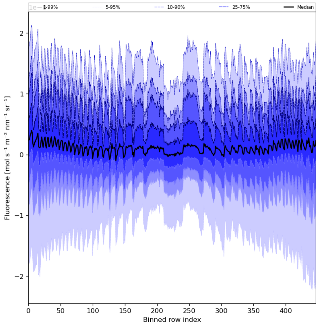
Figure 57: Along track statistics of “Fluorescence” for 2024-05-12 to 2024-05-14
