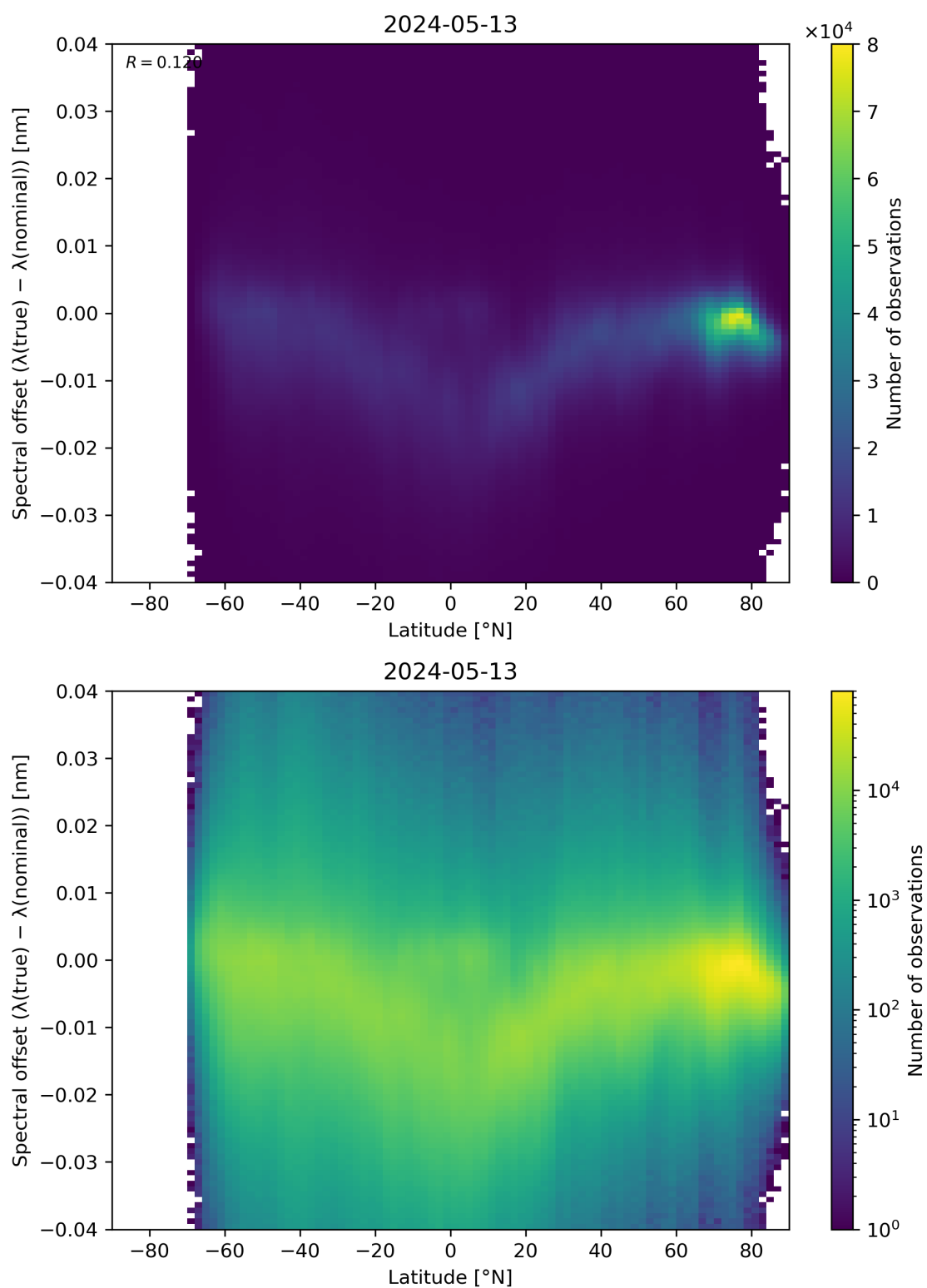
Figure 96: Scatter density plot of “Latitude” against “Spectral offset ( \lambda(\text{true}) - \lambda(\text{nominal}) )” for 2024-05-12 to 2024-05-14.
