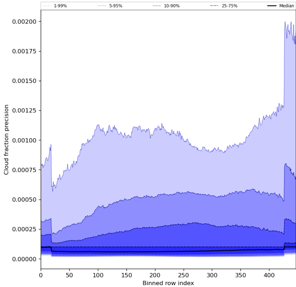
Figure 50: Along track statistics of “Cloud fraction precision” for 2024-05-12 to 2024-05-14
