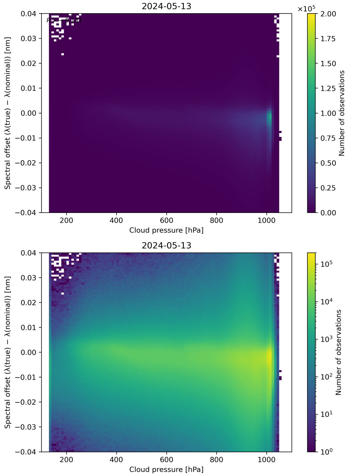
Figure 84: Scatter density plot of “Cloud pressure” against “Spectral offset ( \lambda(\text{true}) - \lambda(\text{nominal}) )” for 2024-05-12 to 2024-05-14.
