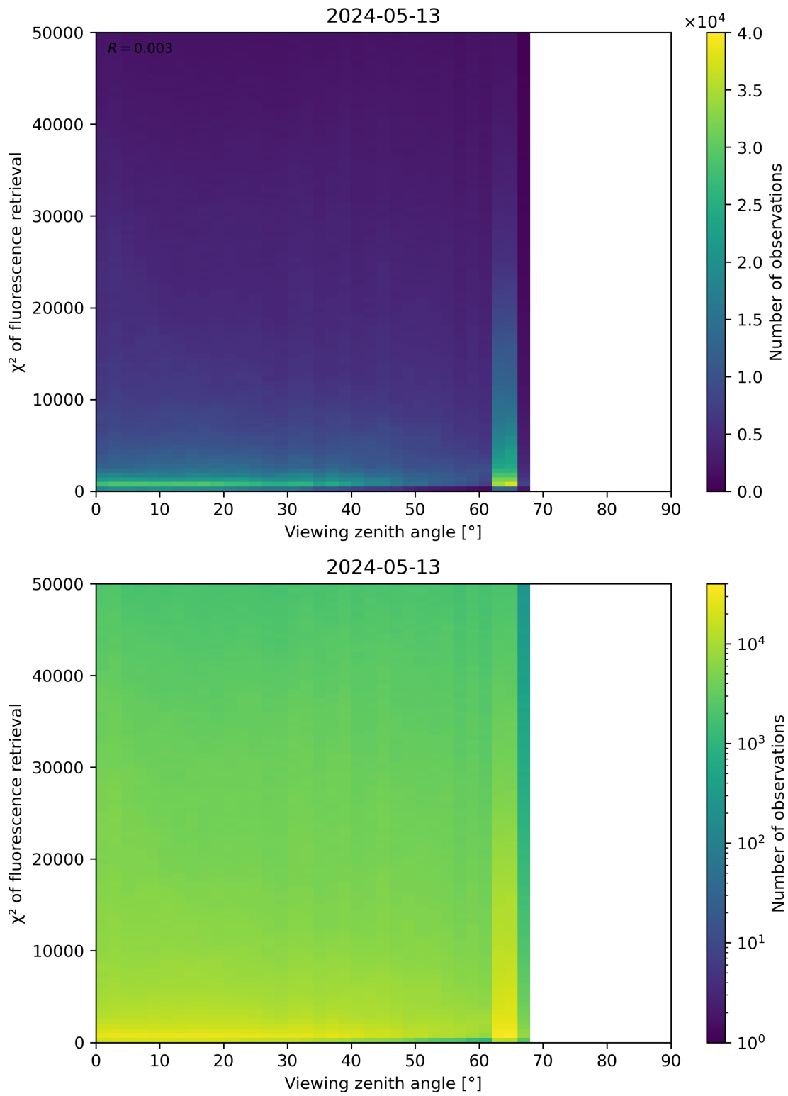
Figure 119: Scatter density plot of “Viewing zenith angle” against “ \chi^2 of fluorescence retrieval” for 2024-05-12 to 2024-05-14.
