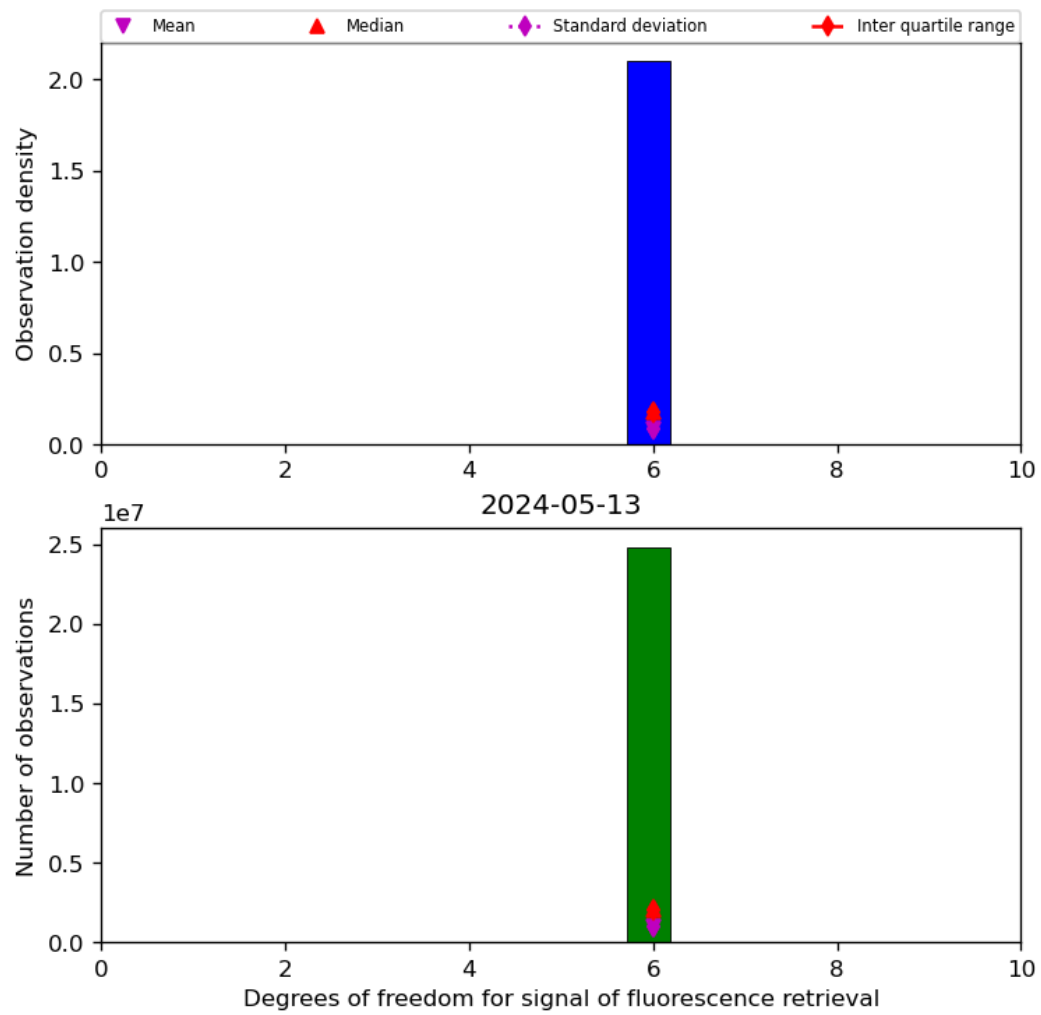
Figure 43: Histogram of “Degrees of freedom for signal of fluorescence retrieval” for 2024-05-12 to 2024-05-14
