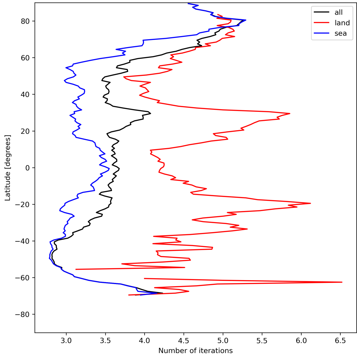
Figure 22: Zonal average of “Number of iterations” for 2024-05-12 to 2024-05-14.
