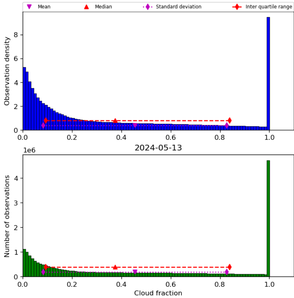
Figure 32: Histogram of “Cloud fraction” for 2024-05-12 to 2024-05-14
