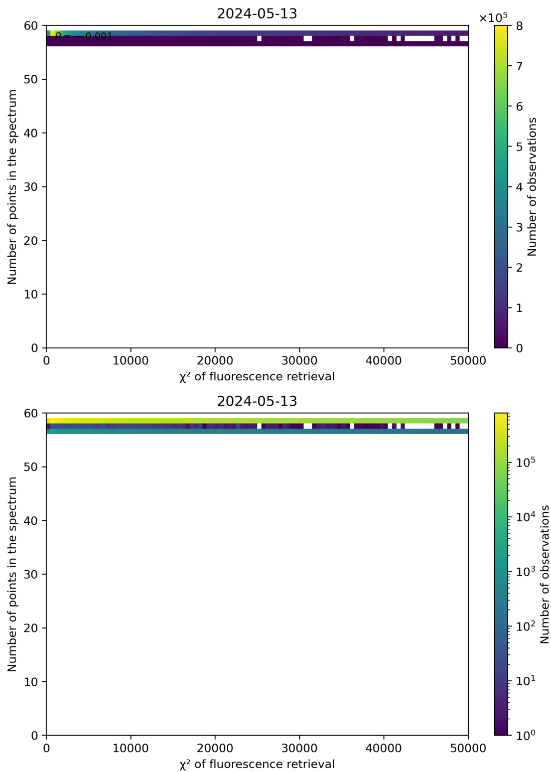
Figure 68: Scatter density plot of " \chi^2 of fluorescence retrieval" against "Number of points in the spectrum" for 2024-05-12 to 2024-05-14.
