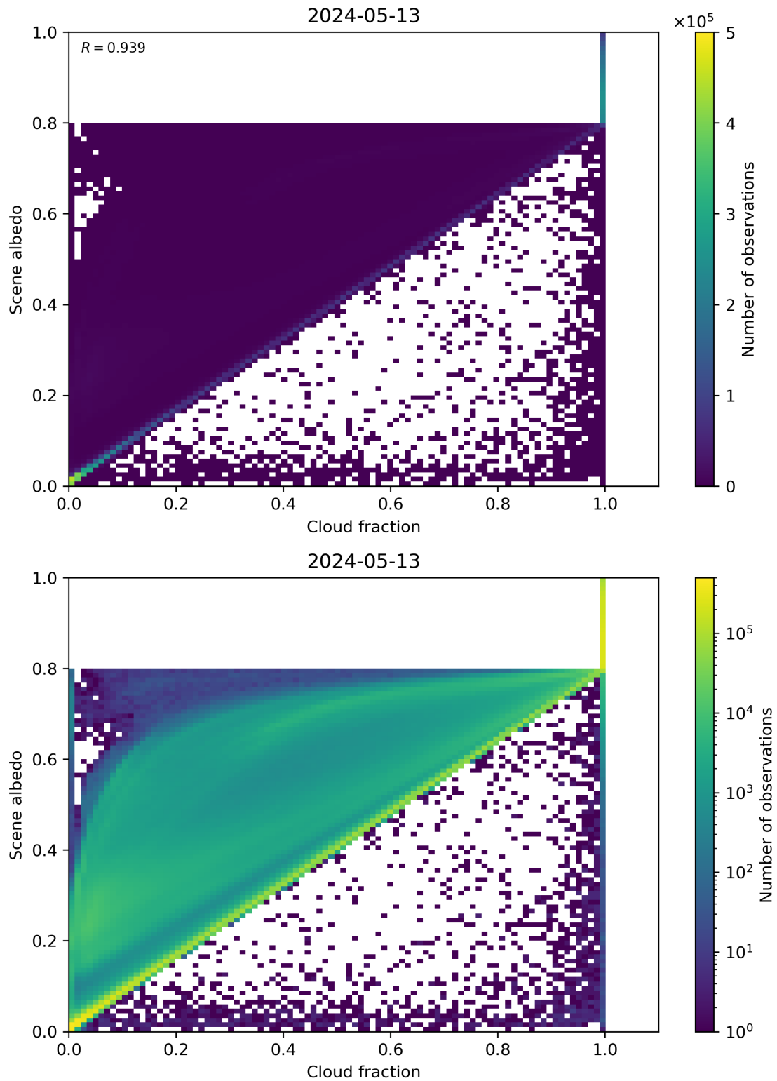
Figure 75: Scatter density plot of “Cloud fraction” against “Scene albedo” for 2024-05-12 to 2024-05-14.
