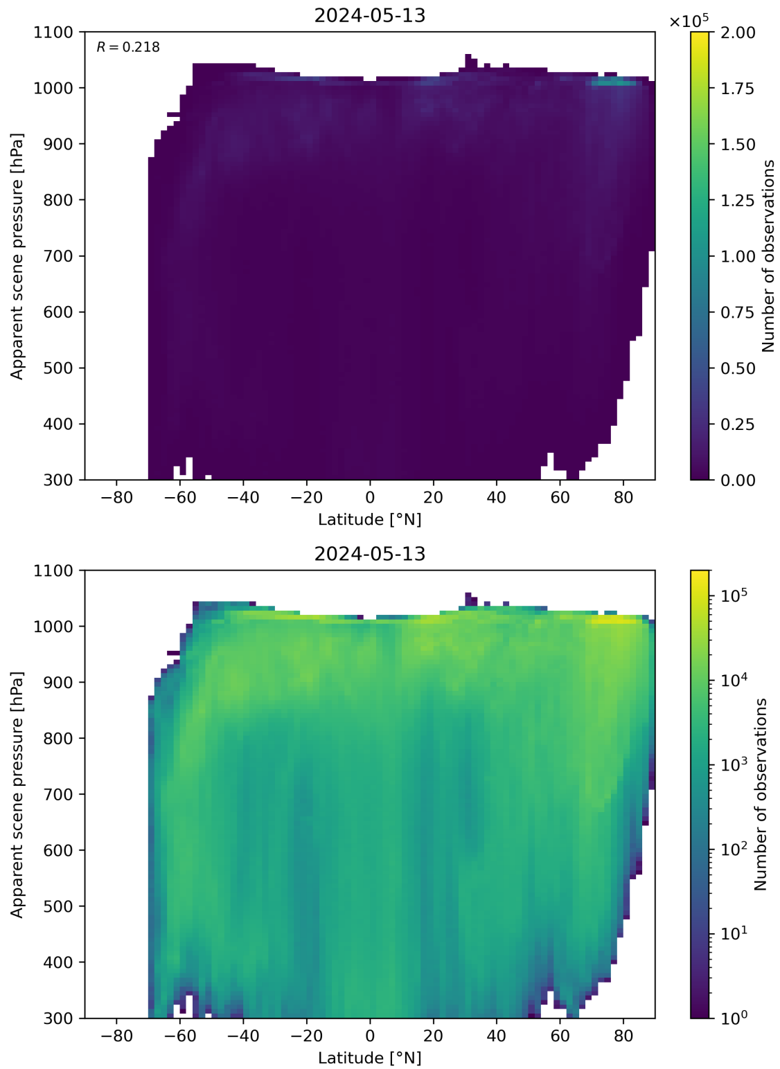
Figure 88: Scatter density plot of “Latitude” against “Apparent scene pressure” for 2024-05-12 to 2024-05-14.
