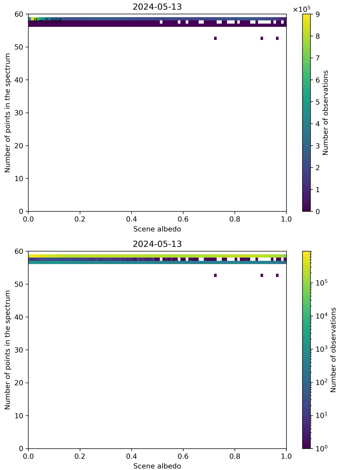
Figure 106: Scatter density plot of “Scene albedo” against “Number of points in the spectrum” for 2024-05-12 to 2024-05-14.
