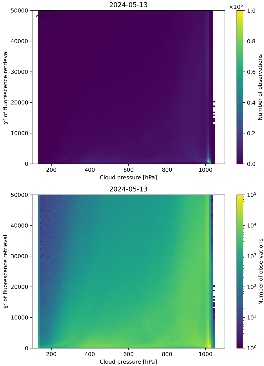
Figure 78: Scatter density plot of “Cloud pressure” against “ \chi^2 of fluorescence retrieval” for 2024-05-12 to 2024-05-14.
