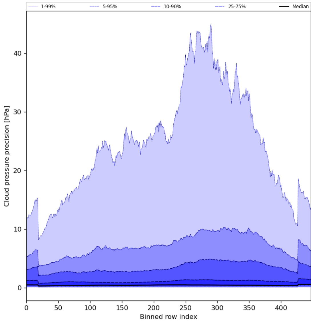
Figure 48: Along track statistics of “Cloud pressure precision” for 2024-05-12 to 2024-05-14
