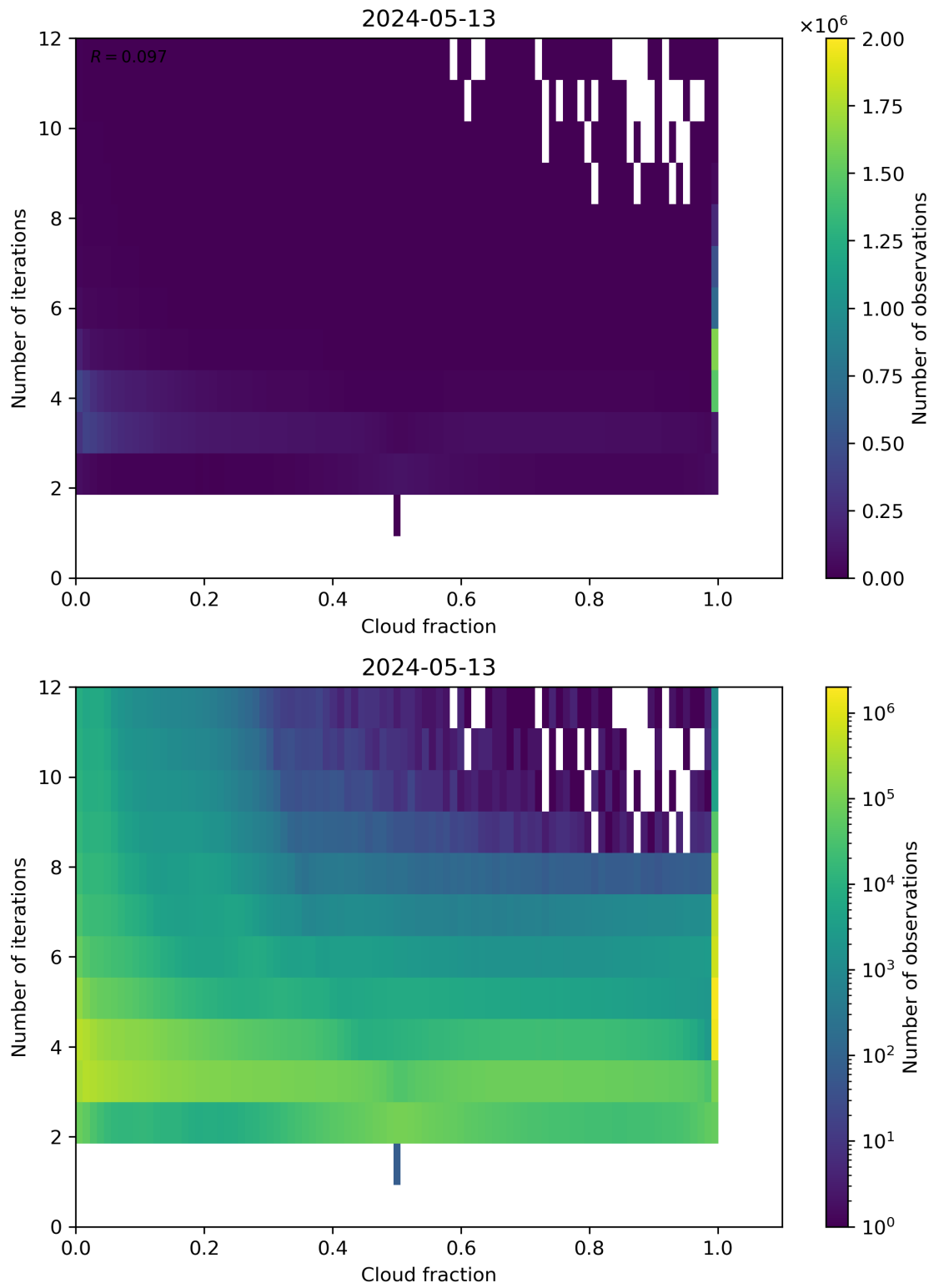
Figure 73: Scatter density plot of “Cloud fraction” against “Number of iterations” for 2024-05-12 to 2024-05-14.
