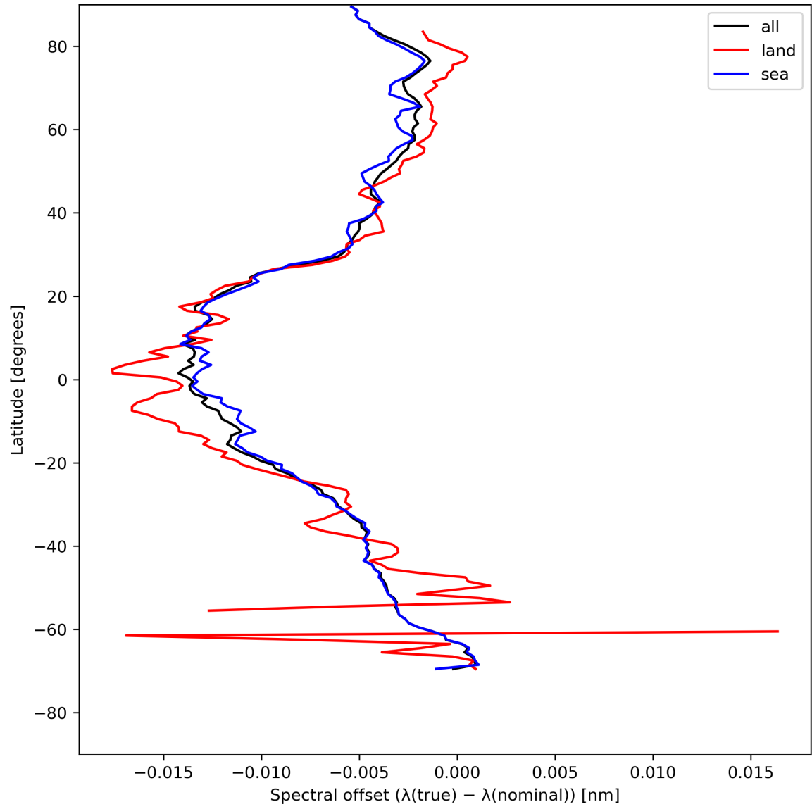
Figure 28: Zonal average of “Spectral offset ( \lambda(\text{true}) - \lambda(\text{nominal}) )” for 2024-05-12 to 2024-05-14.
