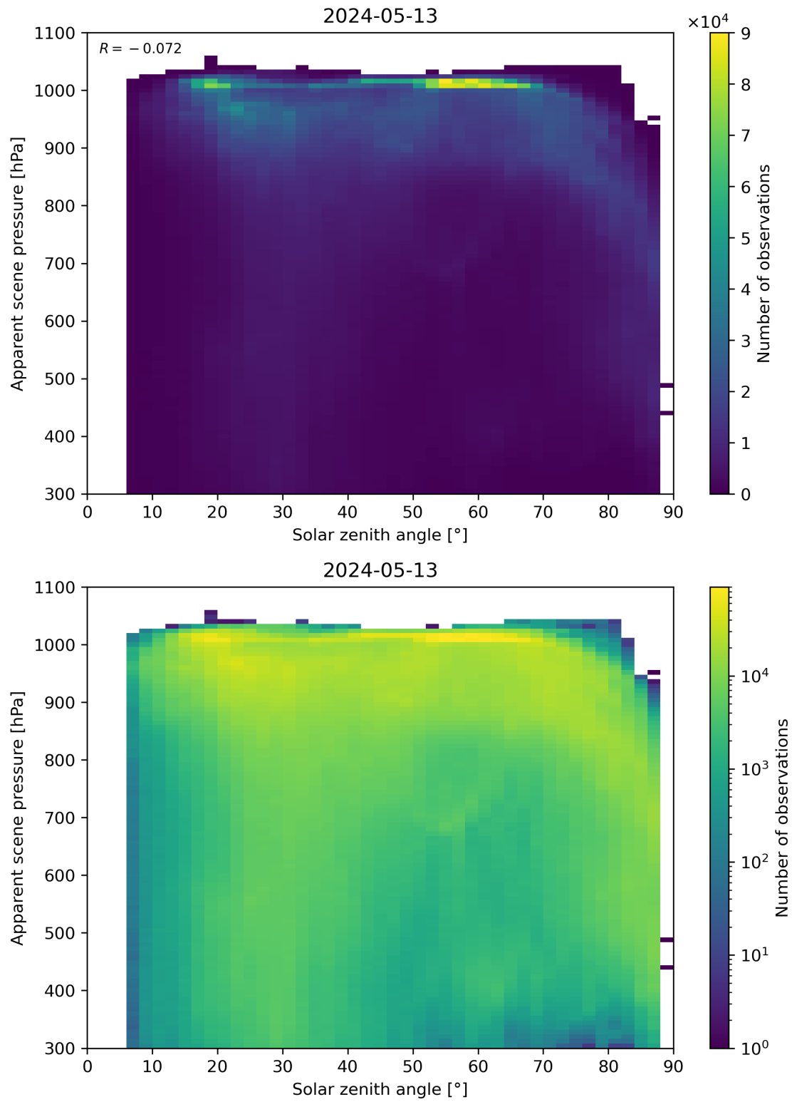
Figure 108: Scatter density plot of “Solar zenith angle” against “Apparent scene pressure” for 2024-05-12 to 2024-05-14.
