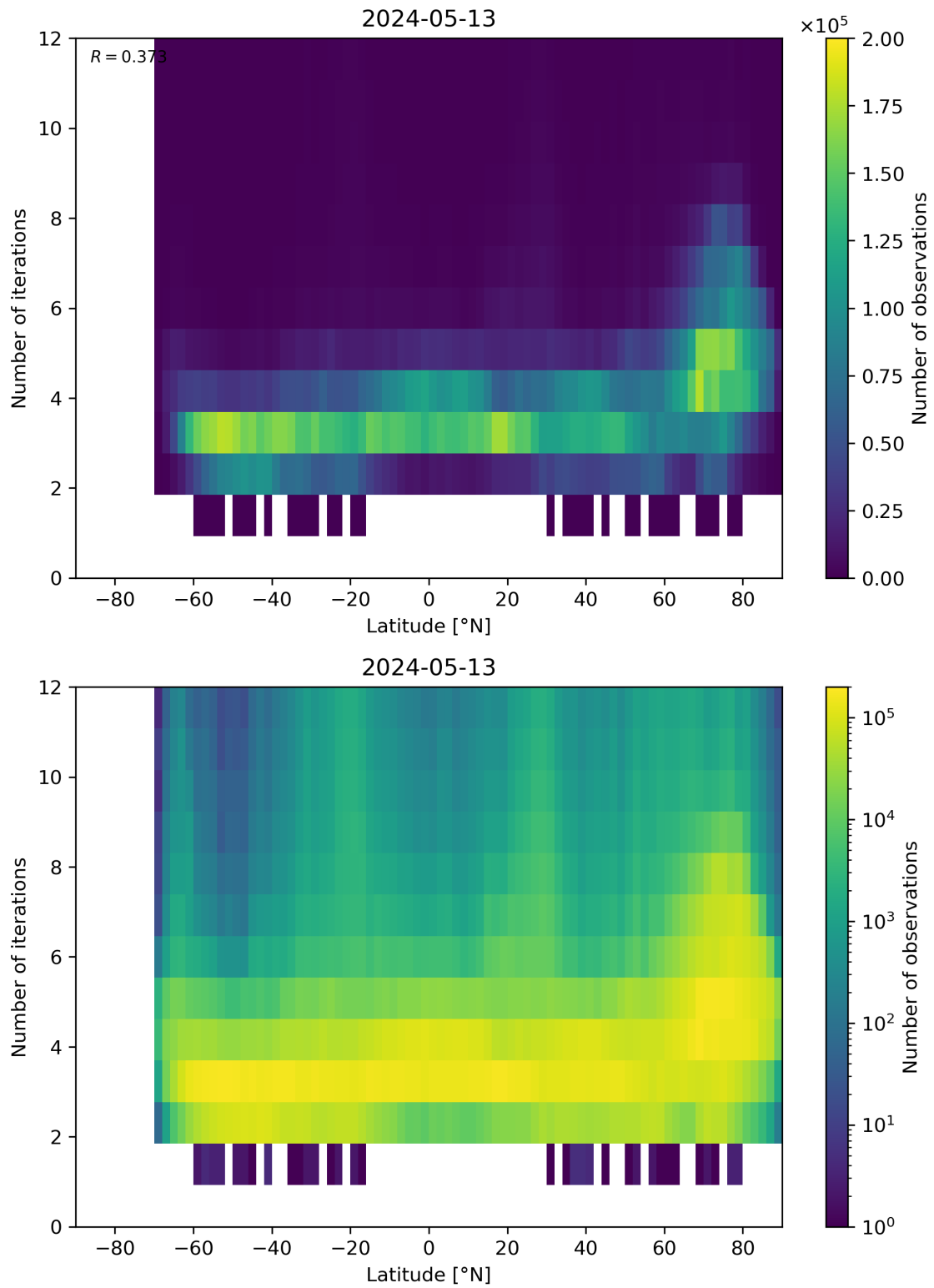
Figure 93: Scatter density plot of “Latitude” against “Number of iterations” for 2024-05-12 to 2024-05-14.
