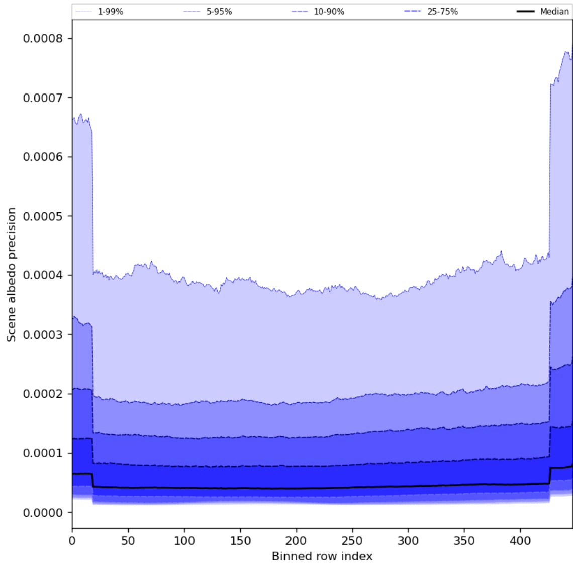
Figure 52: Along track statistics of “Scene albedo precision” for 2024-05-12 to 2024-05-14
