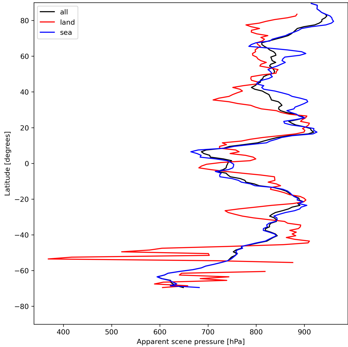
Figure 19: Zonal average of “Apparent scene pressure” for 2024-05-12 to 2024-05-14.
