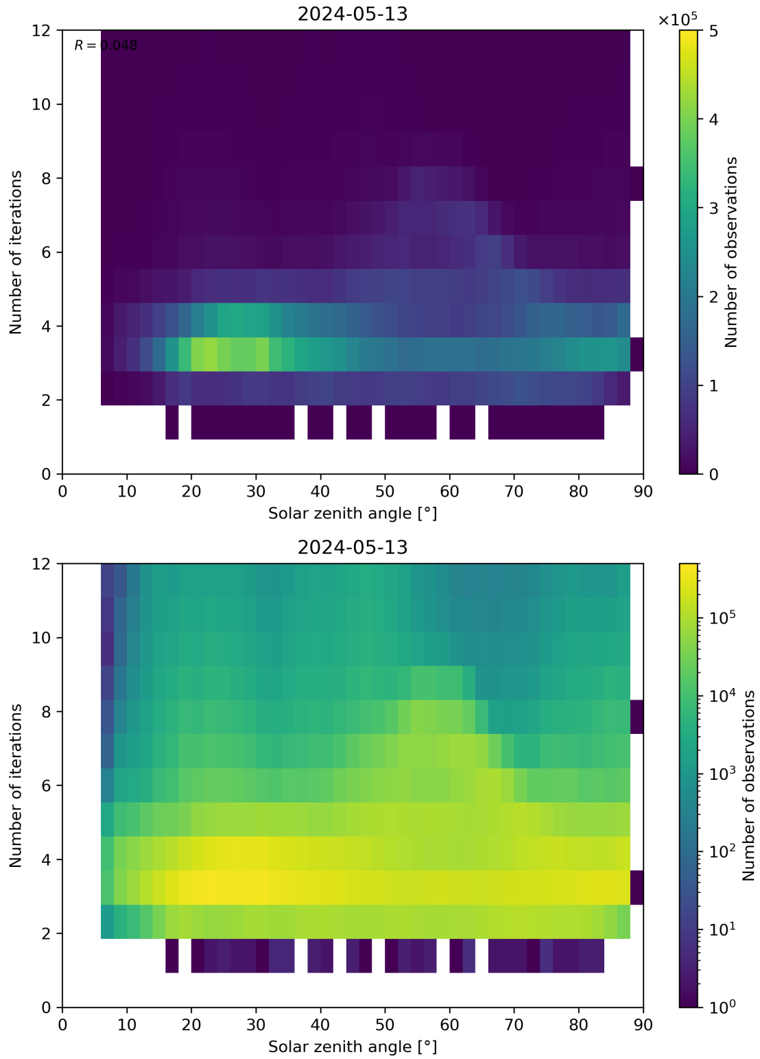
Figure 114: Scatter density plot of “Solar zenith angle” against “Number of iterations” for 2024-05-12 to 2024-05-14.
