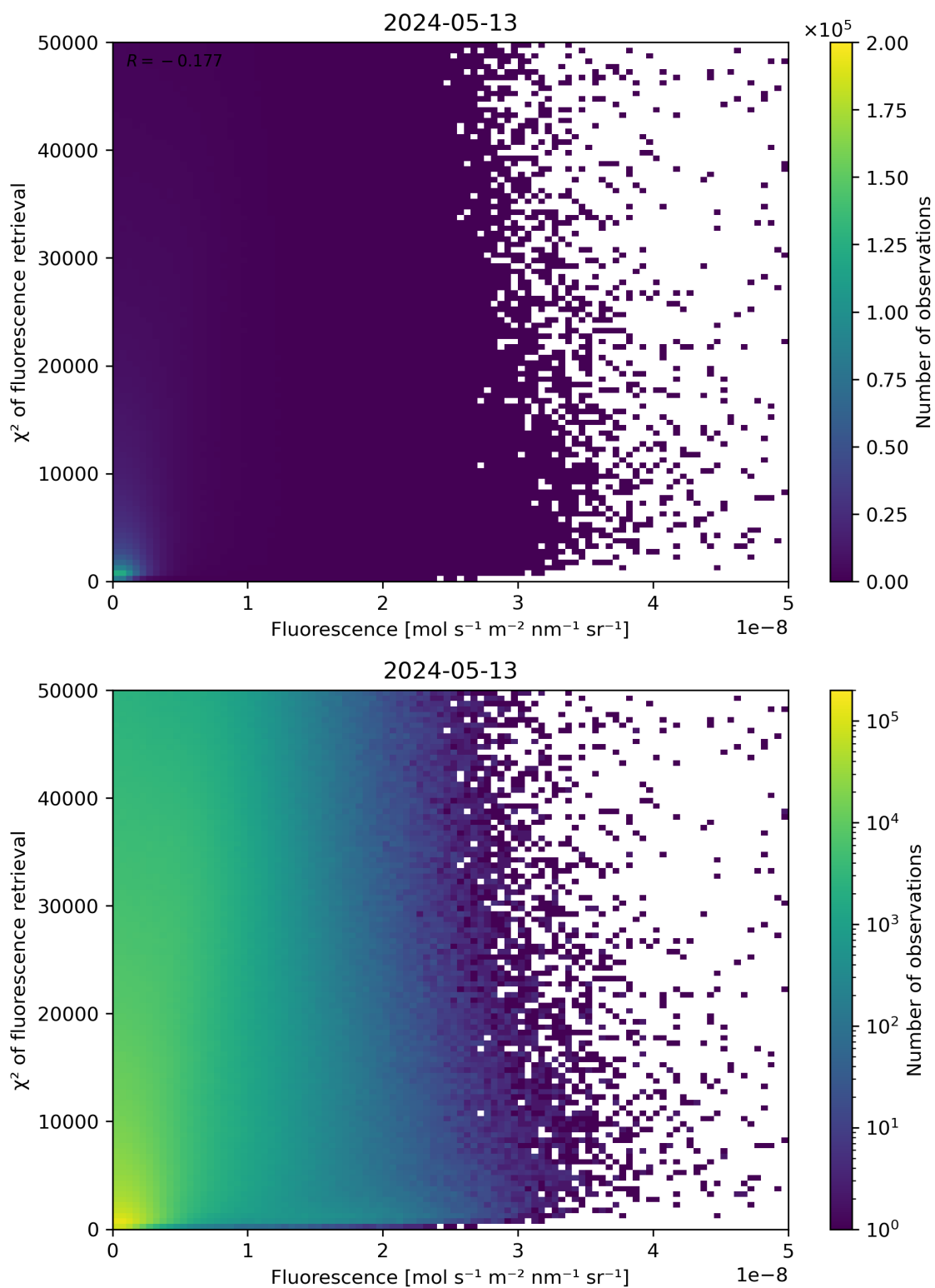
Figure 85: Scatter density plot of “Fluorescence” against “ \chi^2 of fluorescence retrieval” for 2024-05-12 to 2024-05-14.
