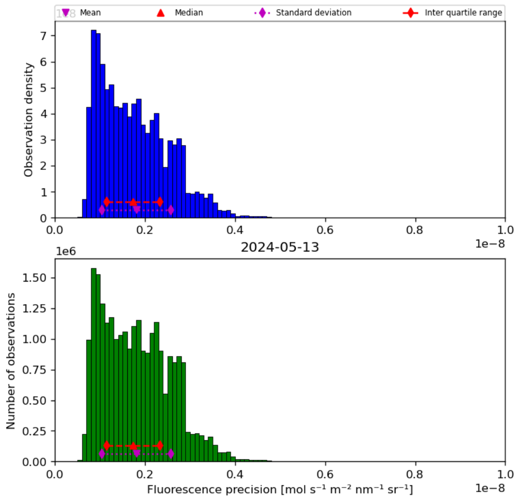
Figure 41: Histogram of “Fluorescence precision” for 2024-05-12 to 2024-05-14
