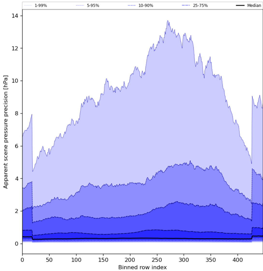
Figure 54: Along track statistics of “Apparent scene pressure precision” for 2024-05-12 to 2024-05-14
