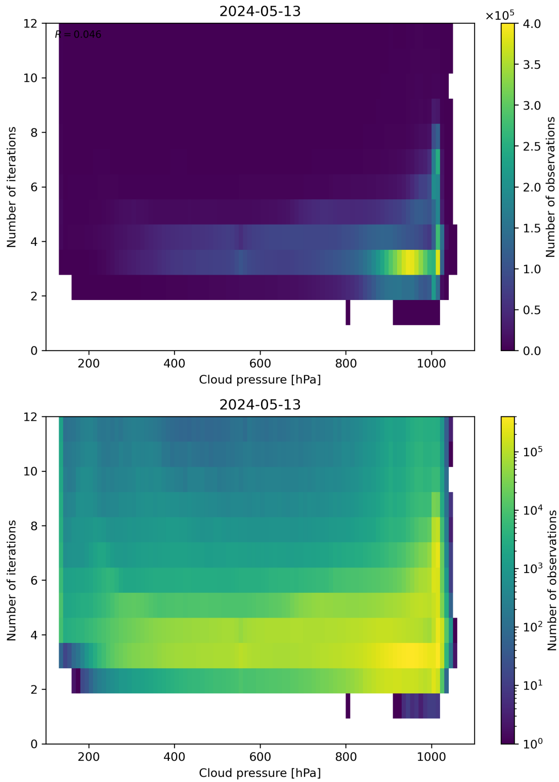
Figure 81: Scatter density plot of “Cloud pressure” against “Number of iterations” for 2024-05-12 to 2024-05-14.
