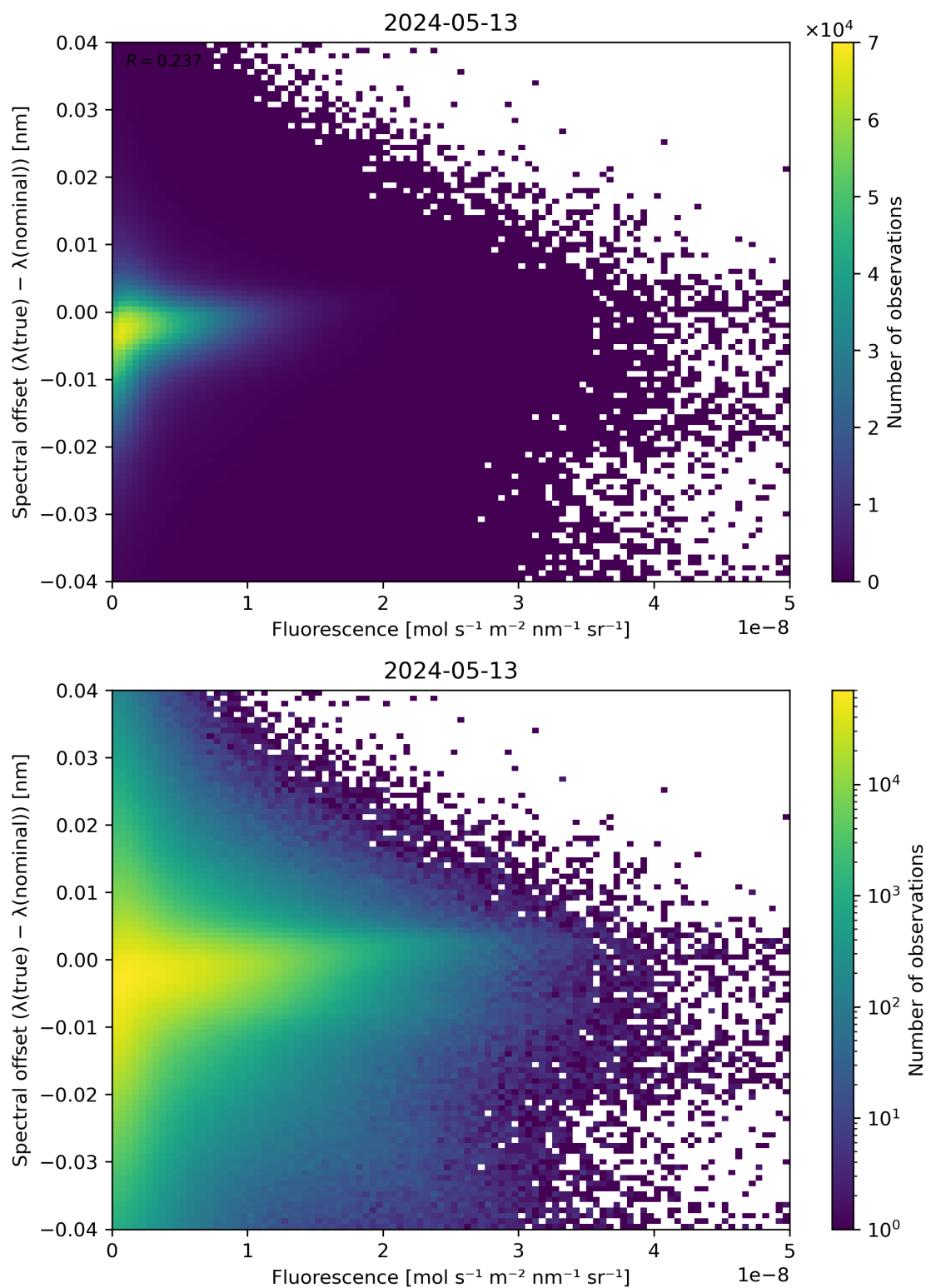
Figure 87: Scatter density plot of “Fluorescence” against “Spectral offset ( \lambda(\text{true}) - \lambda(\text{nominal}) )” for 2024-05-12 to 2024-05-14.
