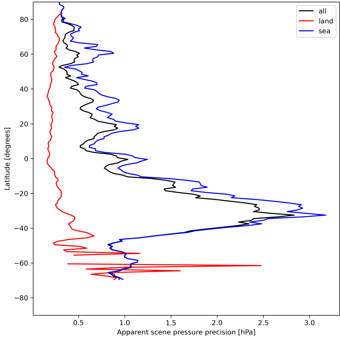
Figure 20: Zonal average of “Apparent scene pressure precision” for 2024-05-12 to 2024-05-14.
