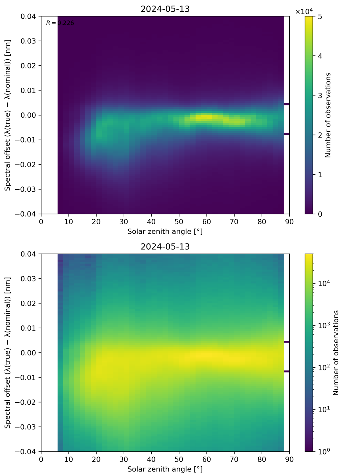
Figure 117: Scatter density plot of “Solar zenith angle” against “Spectral offset ( \lambda(\text{true}) - \lambda(\text{nominal}) )” for 2024-05-12 to 2024-05-14.
