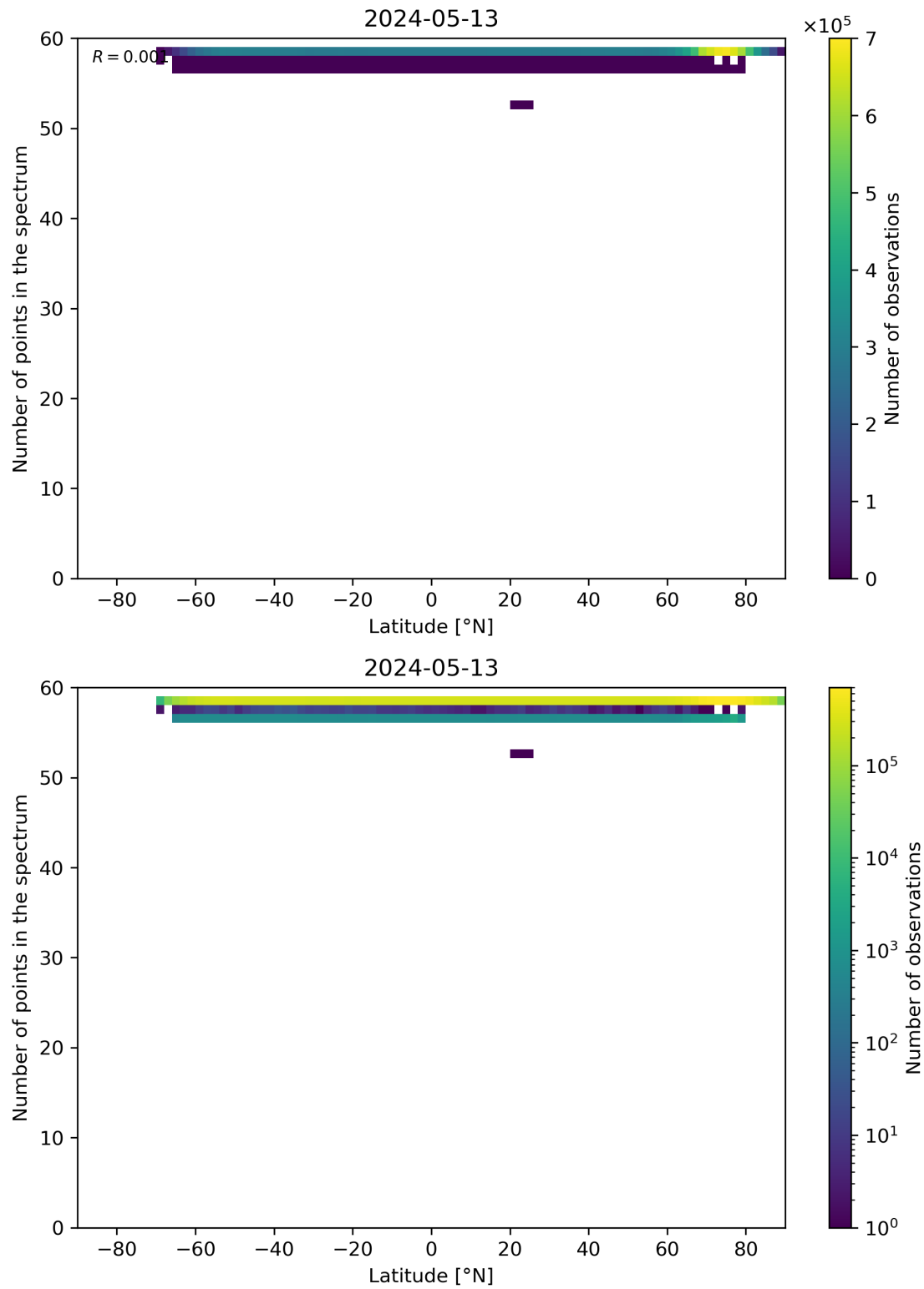
Figure 94: Scatter density plot of “Latitude” against “Number of points in the spectrum” for 2024-05-12 to 2024-05-14.
