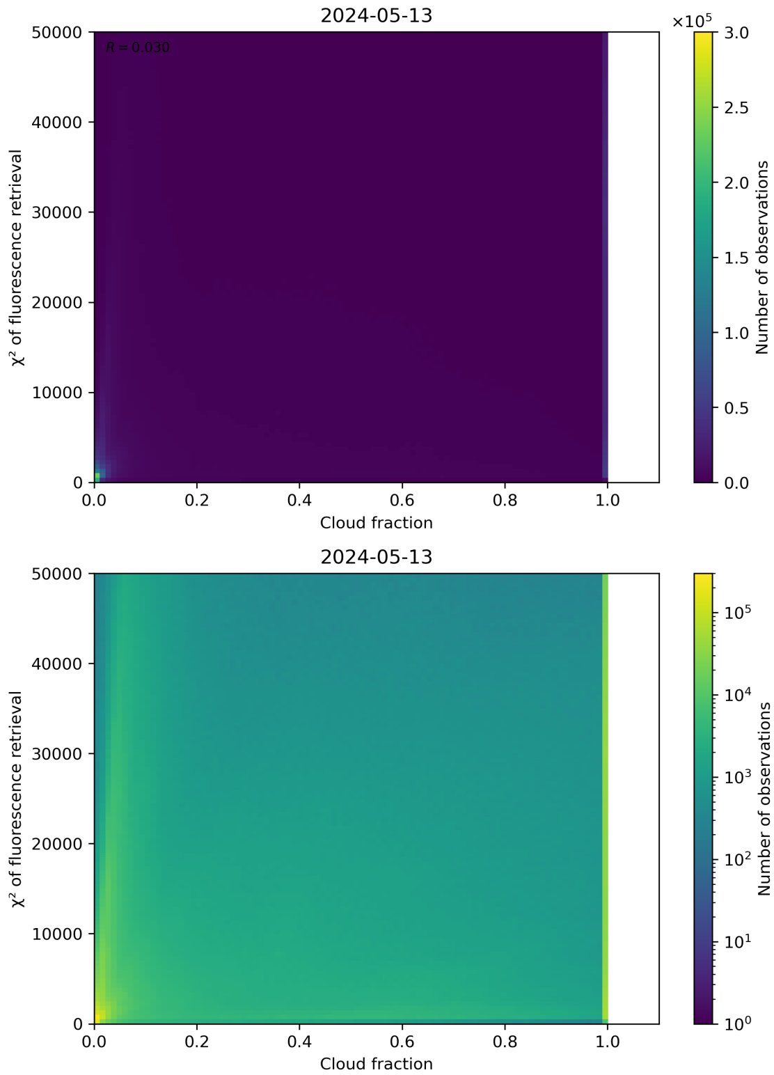
Figure 71: Scatter density plot of “Cloud fraction” against “ \chi^2 of fluorescence retrieval” for 2024-05-12 to 2024-05-14.
