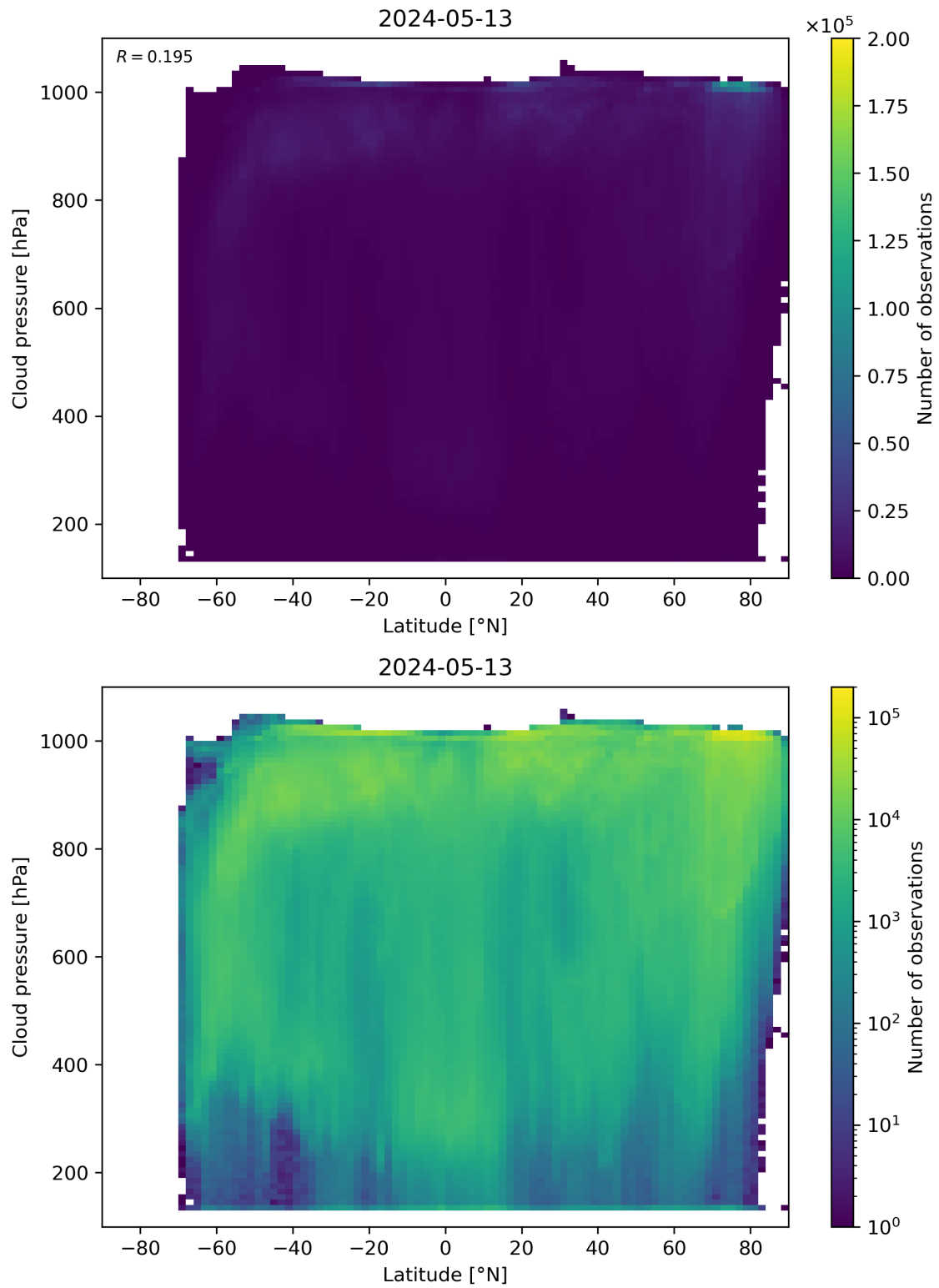
Figure 91: Scatter density plot of “Latitude” against “Cloud pressure” for 2024-05-12 to 2024-05-14.
