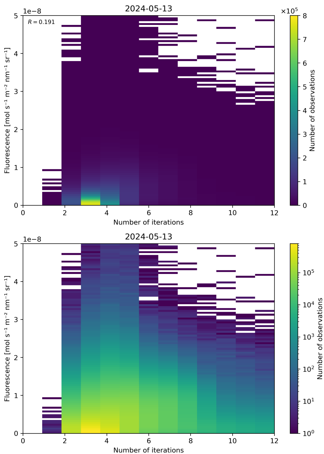
Figure 98: Scatter density plot of “Number of iterations” against “Fluorescence” for 2024-05-12 to 2024-05-14.
