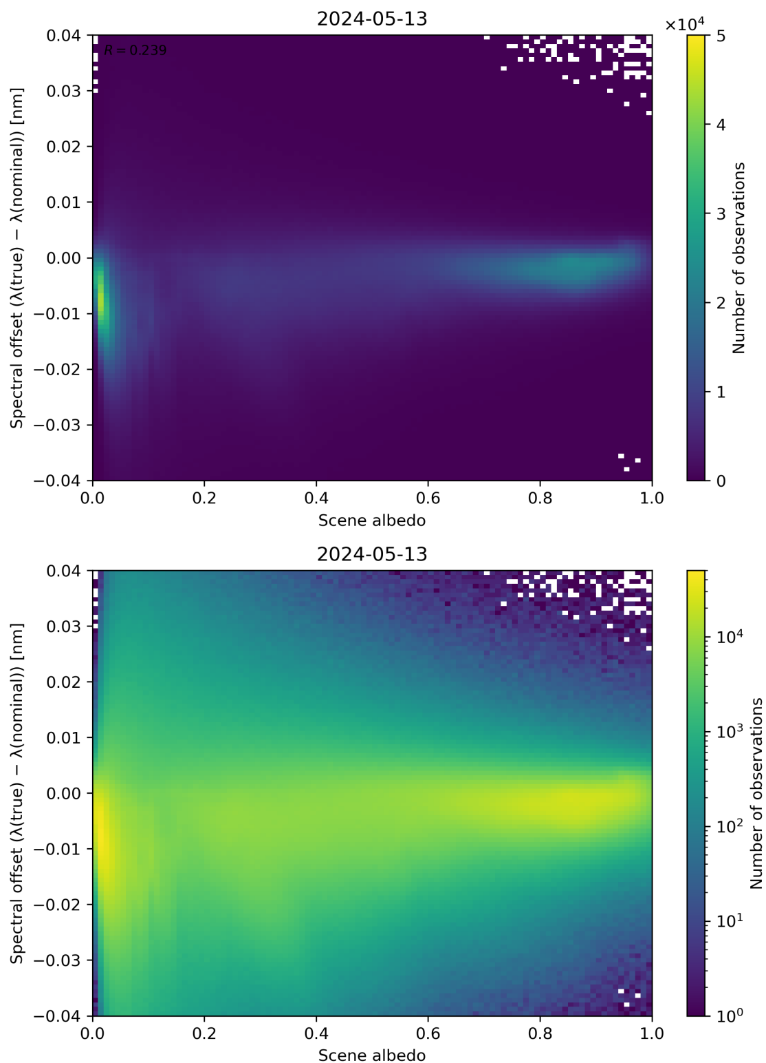
Figure 107: Scatter density plot of “Scene albedo” against “Spectral offset ( \lambda(\text{true}) - \lambda(\text{nominal}) )” for 2024-05-12 to 2024-05-14.
