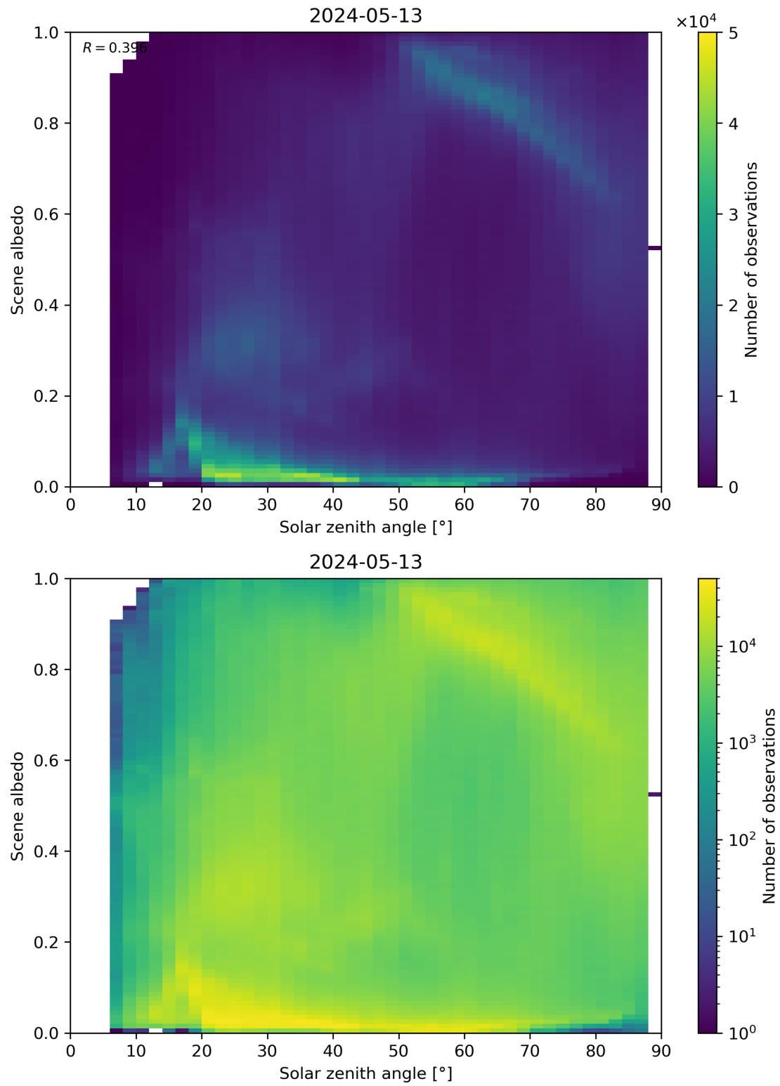
Figure 116: Scatter density plot of “Solar zenith angle” against “Scene albedo” for 2024-05-12 to 2024-05-14.
