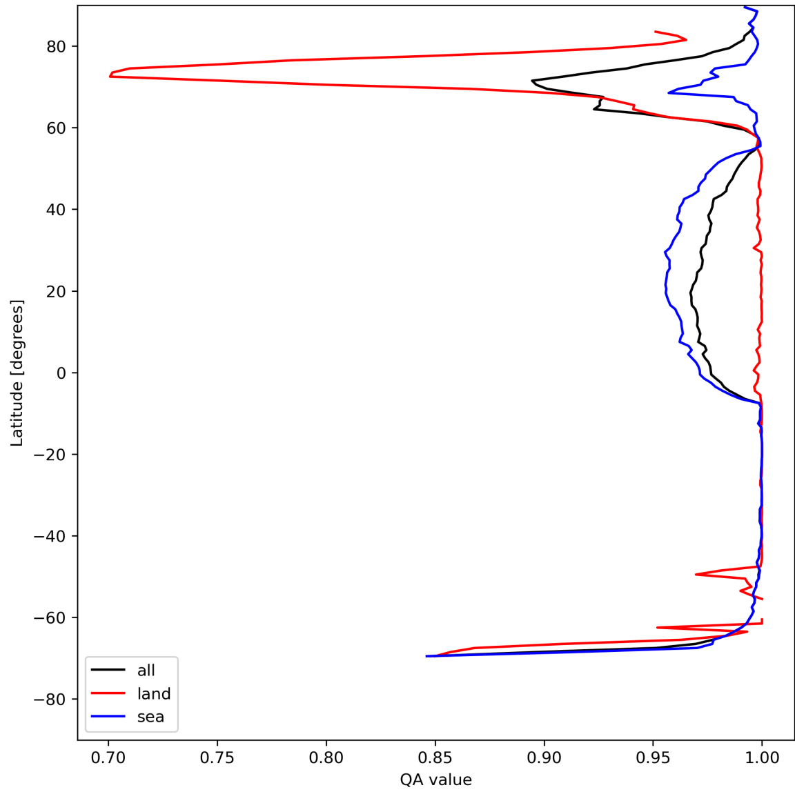
Figure 12: Zonal average of “QA value” for 2024-05-12 to 2024-05-14.
