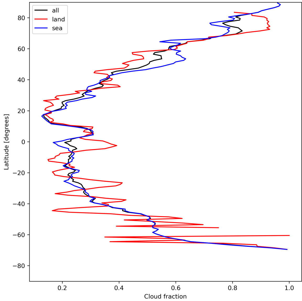
Figure 15: Zonal average of “Cloud fraction” for 2024-05-12 to 2024-05-14.
