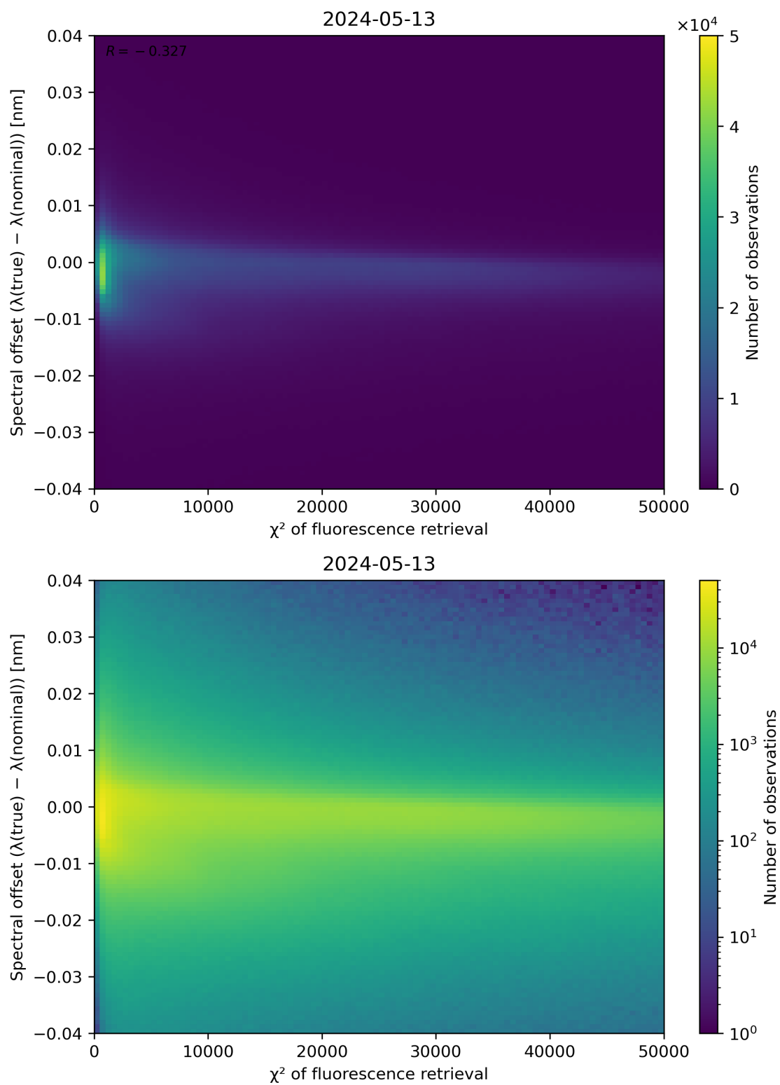
Figure 69: Scatter density plot of " \chi^2 of fluorescence retrieval" against "Spectral offset ( \lambda(\text{true}) - \lambda(\text{nominal}) )" for 2024-05-12 to 2024-05-14.
