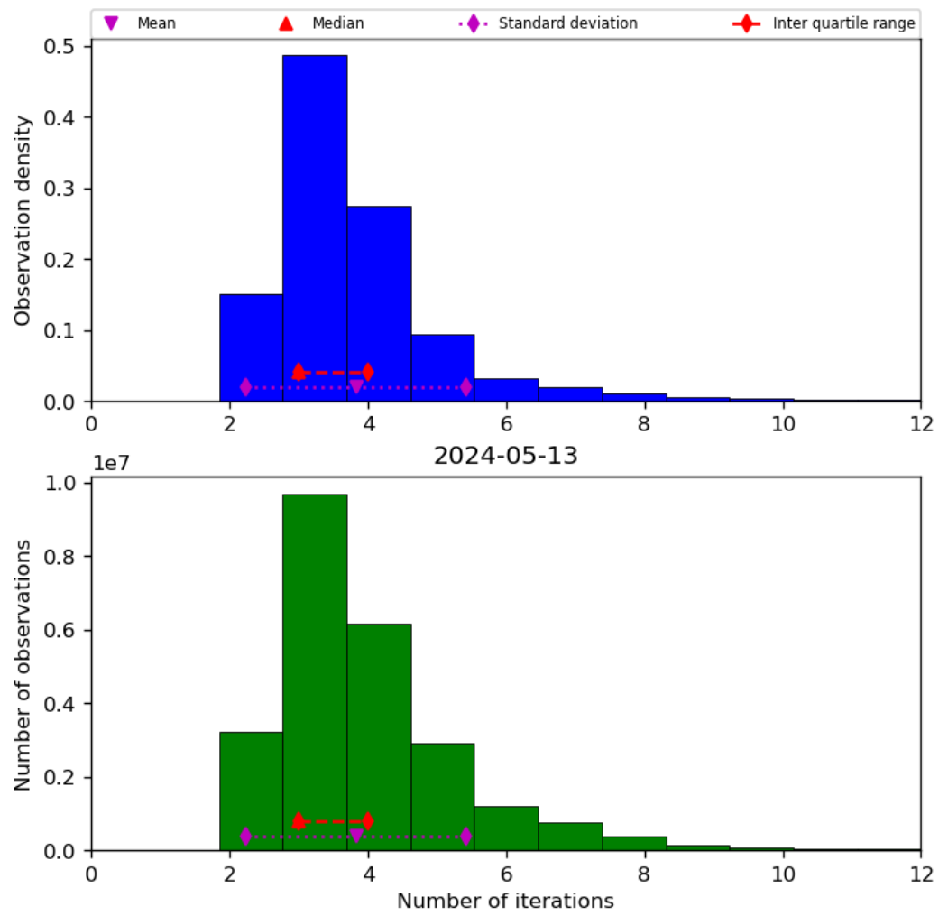
Figure 39: Histogram of “Number of iterations” for 2024-05-12 to 2024-05-14
