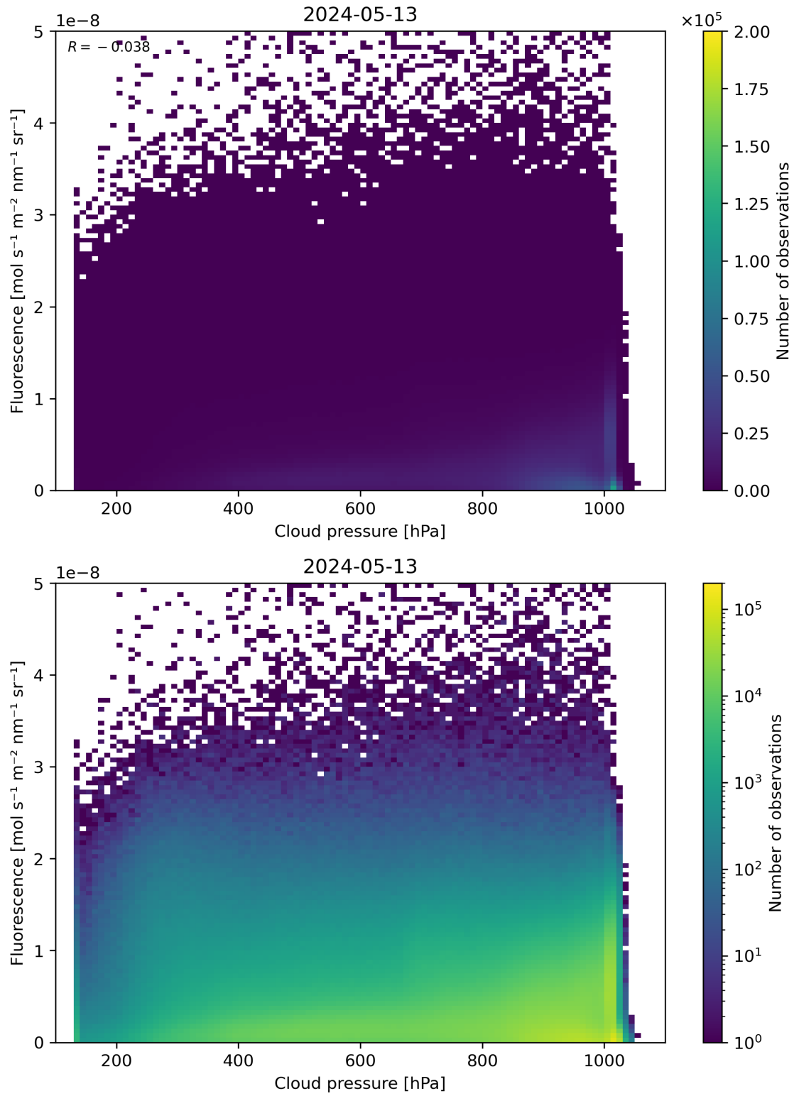
Figure 80: Scatter density plot of “Cloud pressure” against “Fluorescence” for 2024-05-12 to 2024-05-14.
