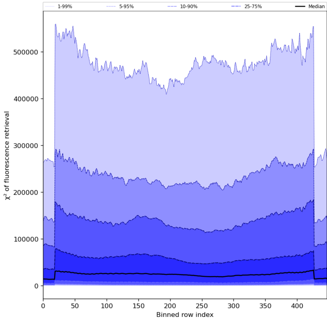
Figure 59: Along track statistics of “ \chi^2 of fluorescence retrieval” for 2024-05-12 to 2024-05-14
