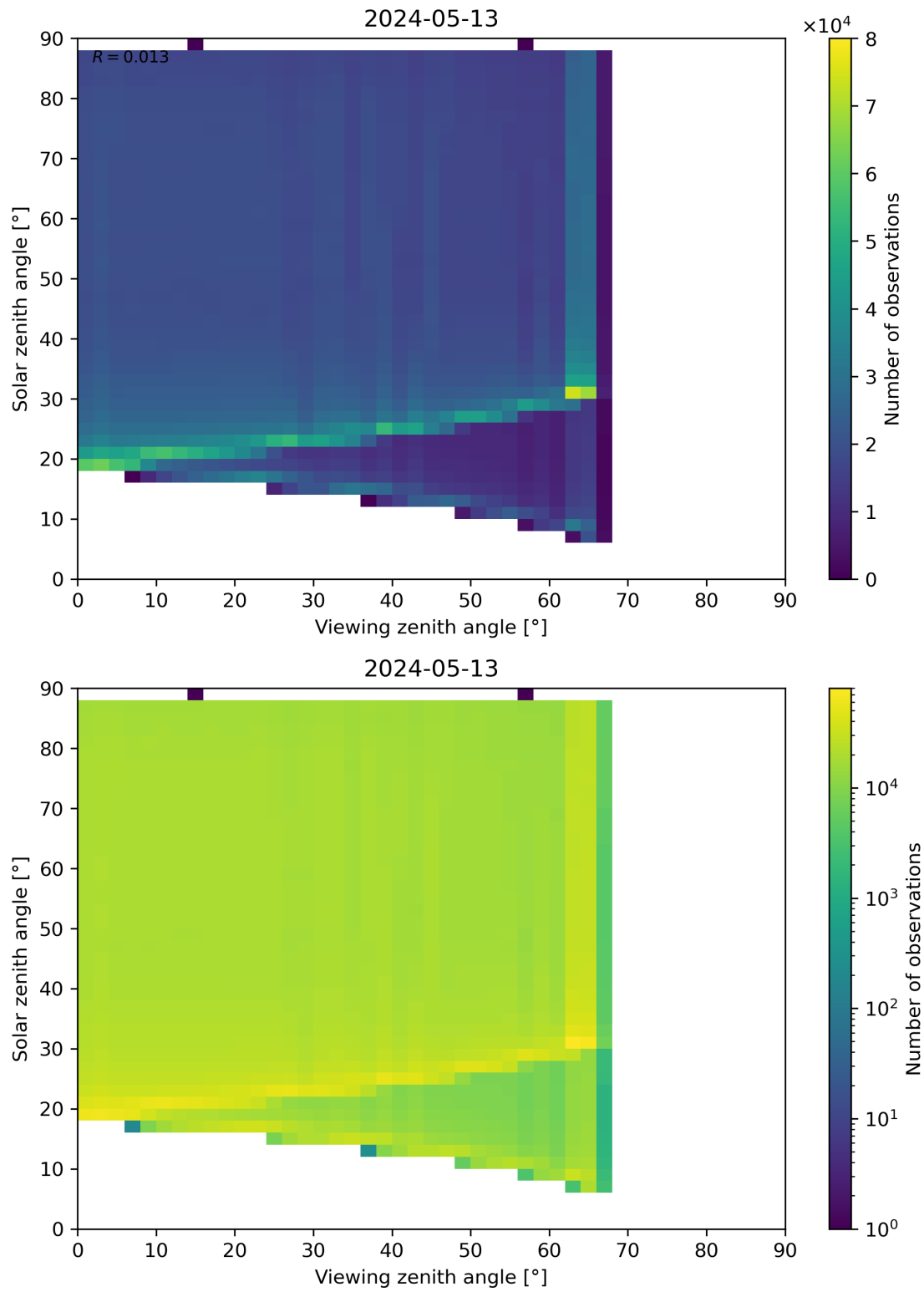
Figure 127: Scatter density plot of “Viewing zenith angle” against “Solar zenith angle” for 2024-05-12 to 2024-05-14.
