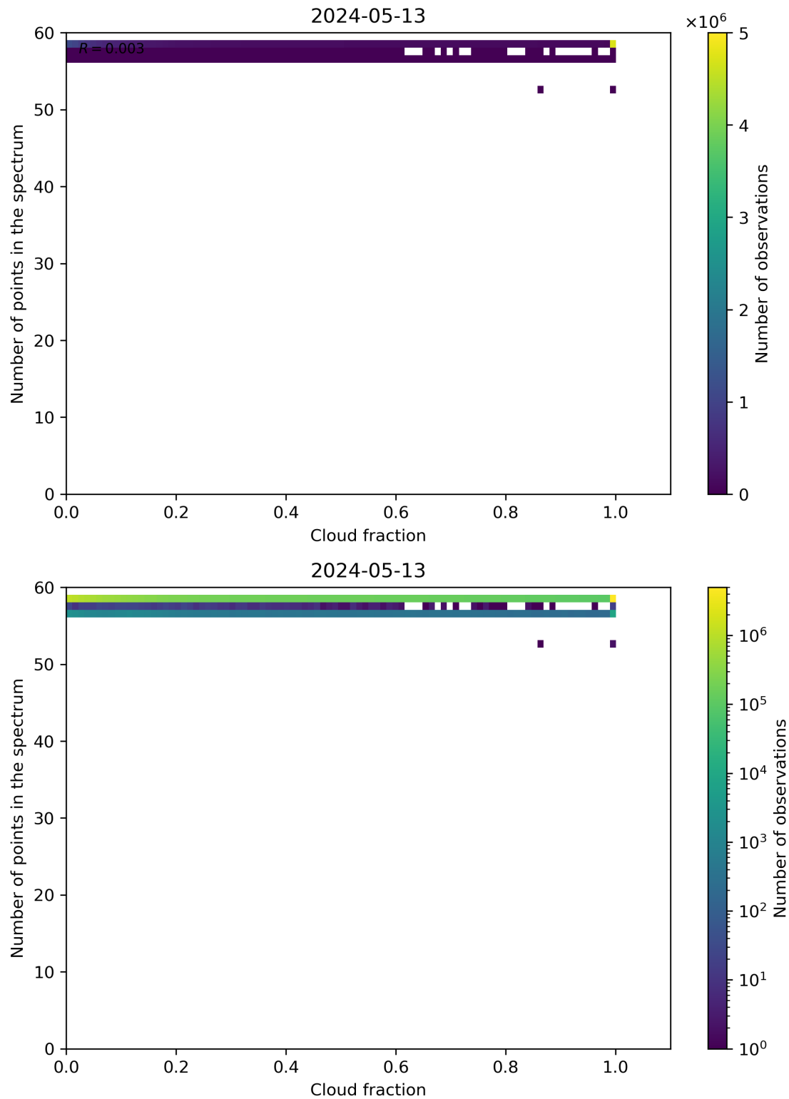
Figure 74: Scatter density plot of “Cloud fraction” against “Number of points in the spectrum” for 2024-05-12 to 2024-05-14.
