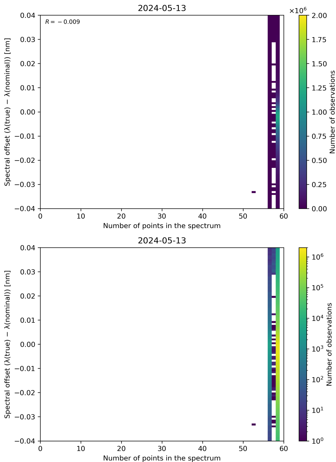
Figure 101: Scatter density plot of “Number of points in the spectrum” against “Spectral offset ( \lambda(\text{true}) - \lambda(\text{nominal}) )” for 2024-05-12 to 2024-05-14.
