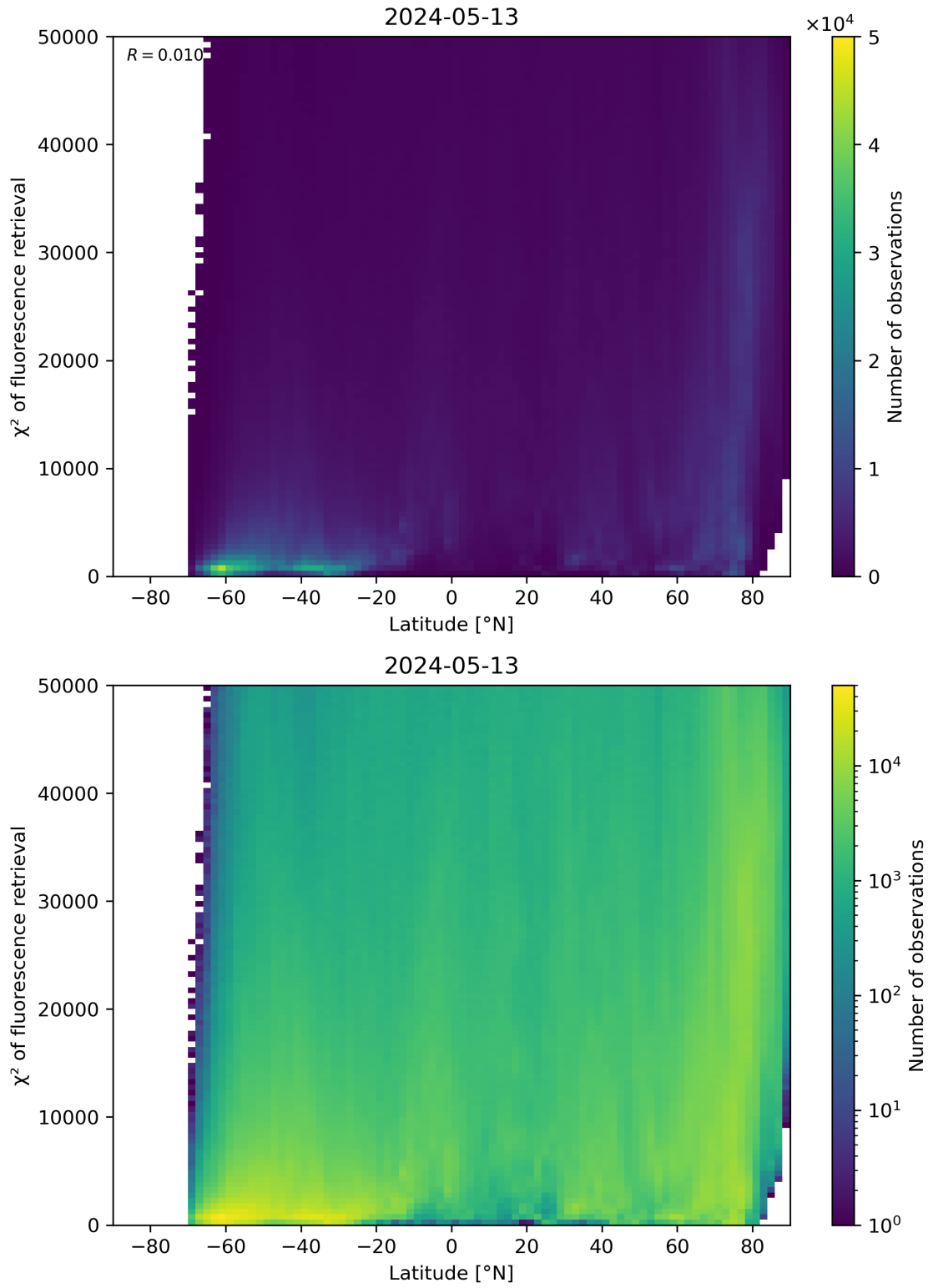
Figure 89: Scatter density plot of “Latitude” against “ \chi^2 of fluorescence retrieval” for 2024-05-12 to 2024-05-14.
