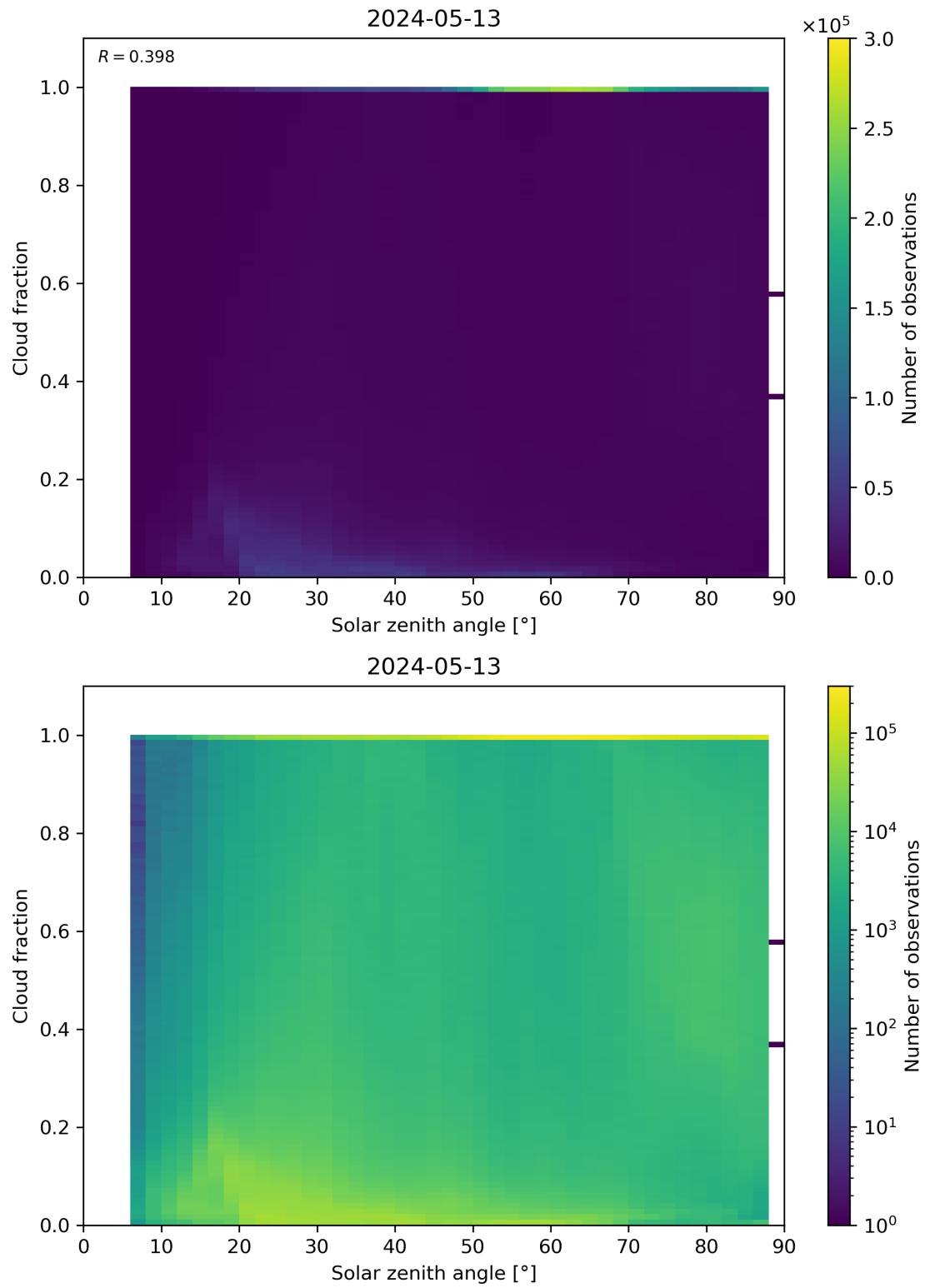
Figure 110: Scatter density plot of “Solar zenith angle” against “Cloud fraction” for 2024-05-12 to 2024-05-14.
