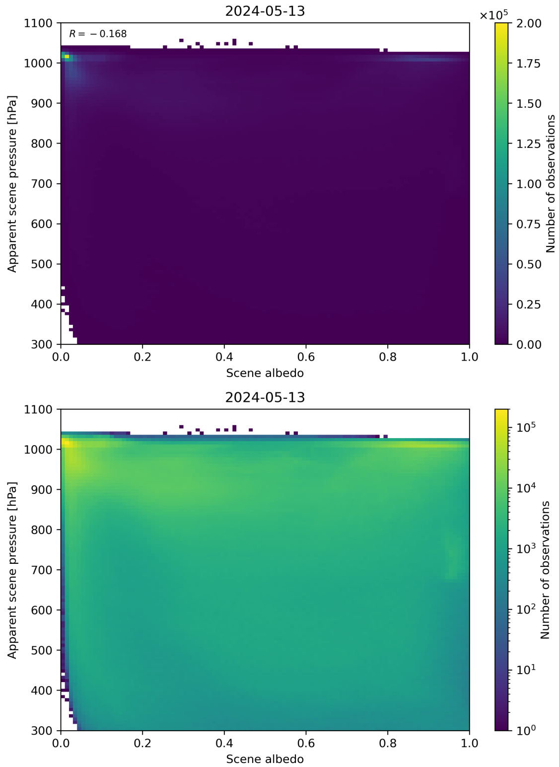
Figure 102: Scatter density plot of “Scene albedo” against “Apparent scene pressure” for 2024-05-12 to 2024-05-14.
