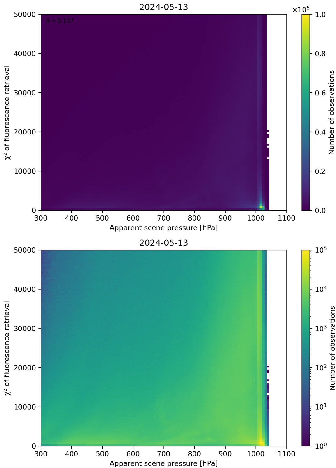
Figure 63: Scatter density plot of “Apparent scene pressure” against “ \chi^2 of fluorescence retrieval” for 2024-05-12 to 2024-05-14.
