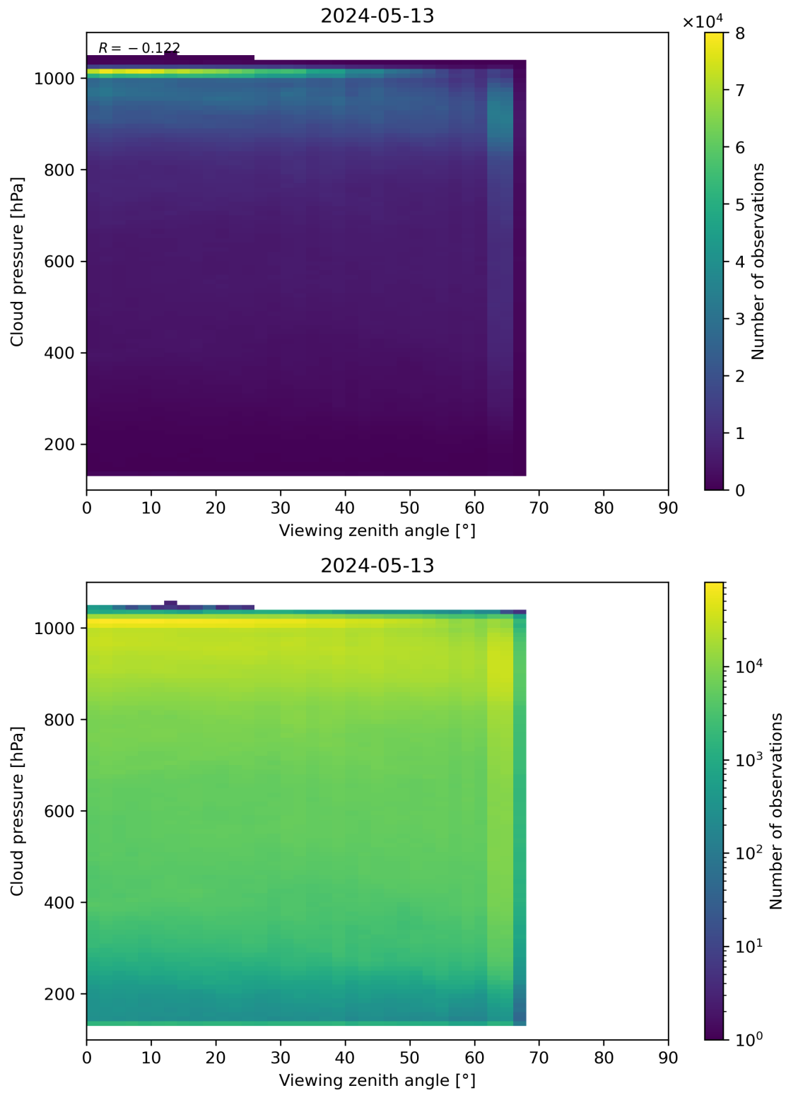
Figure 121: Scatter density plot of “Viewing zenith angle” against “Cloud pressure” for 2024-05-12 to 2024-05-14.
