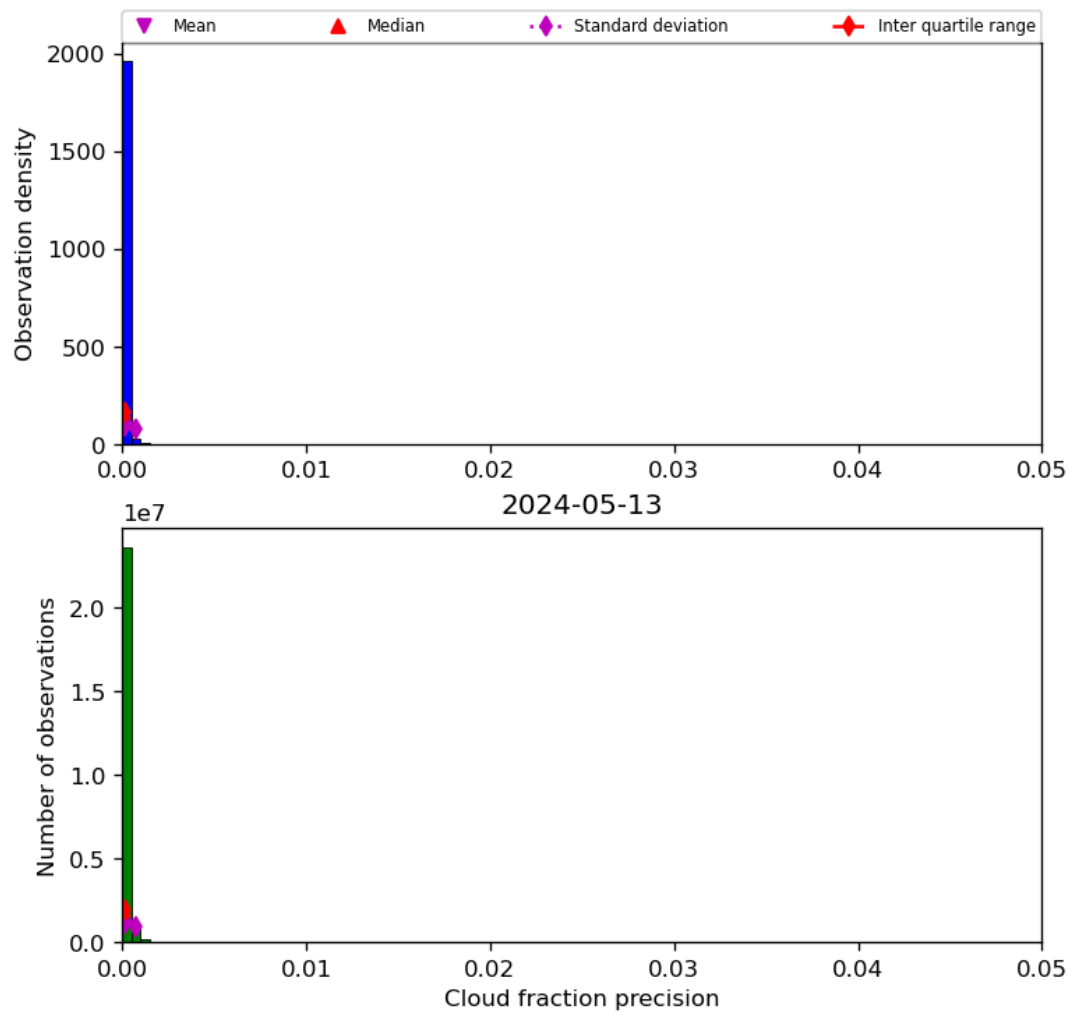
Figure 33: Histogram of “Cloud fraction precision” for 2024-05-12 to 2024-05-14
