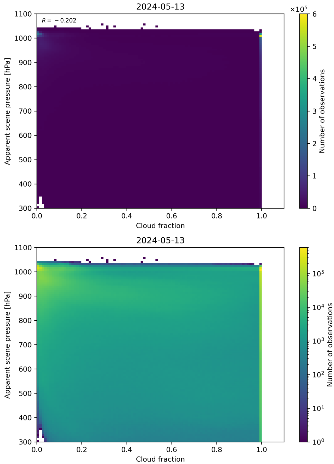
Figure 70: Scatter density plot of “Cloud fraction” against “Apparent scene pressure” for 2024-05-12 to 2024-05-14.
