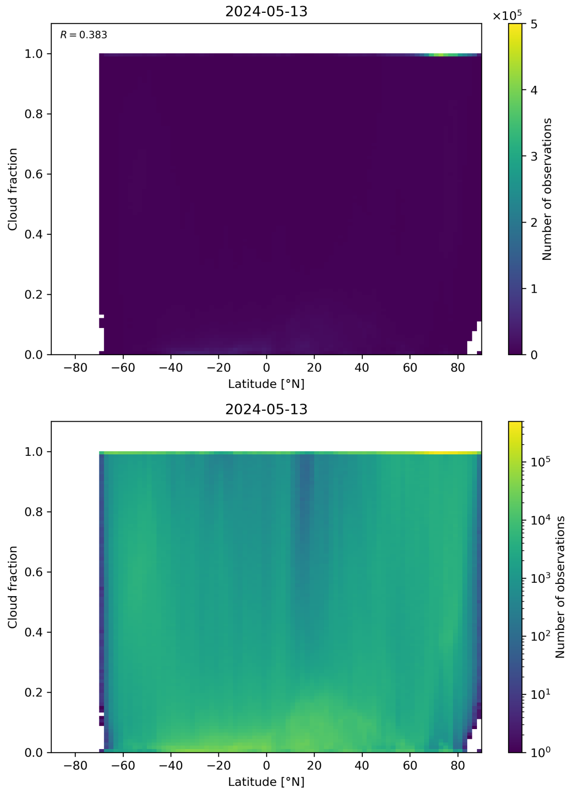
Figure 90: Scatter density plot of “Latitude” against “Cloud fraction” for 2024-05-12 to 2024-05-14.
