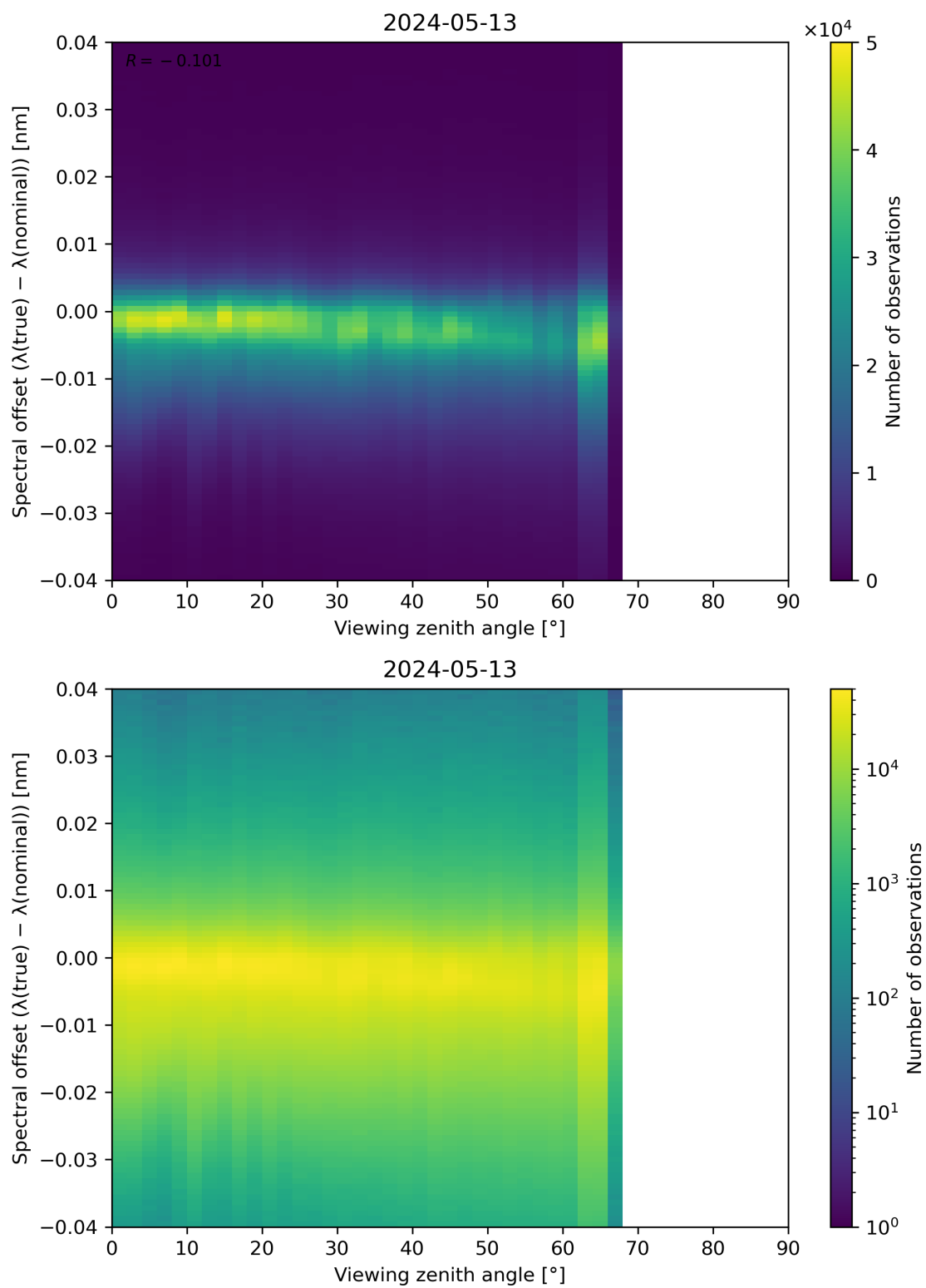
Figure 128: Scatter density plot of “Viewing zenith angle” against “Spectral offset ( \lambda(\text{true}) - \lambda(\text{nominal}) )” for 2024-05-12 to 2024-05-14.
