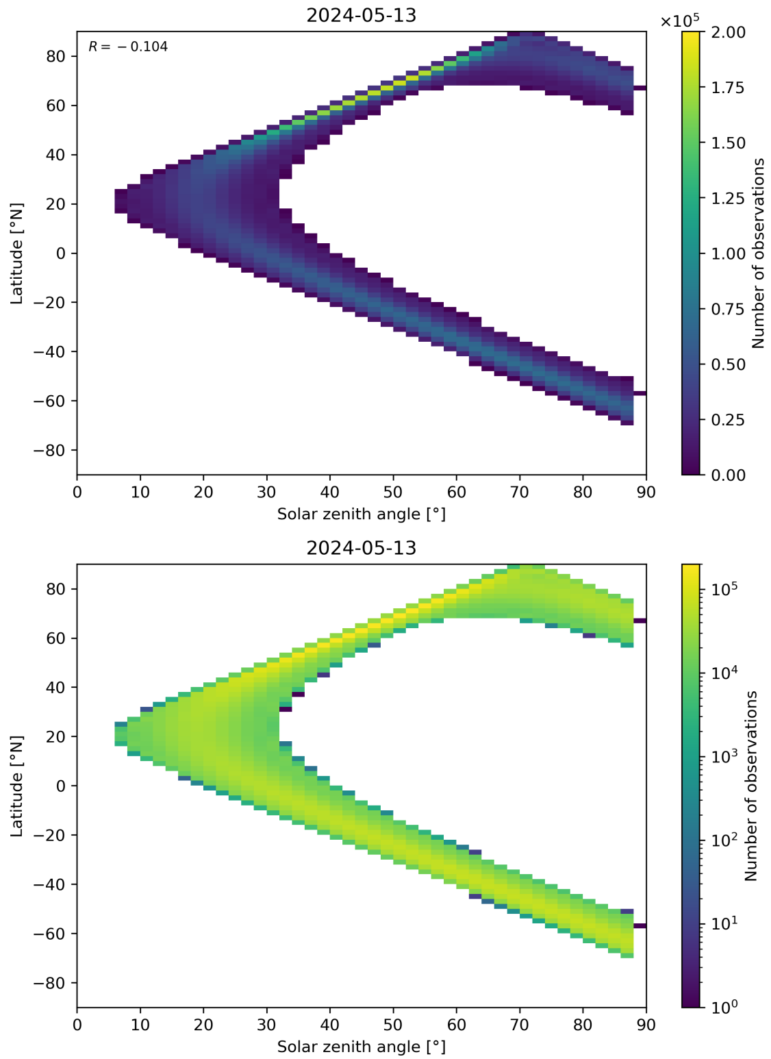
Figure 113: Scatter density plot of “Solar zenith angle” against “Latitude” for 2024-05-12 to 2024-05-14.
