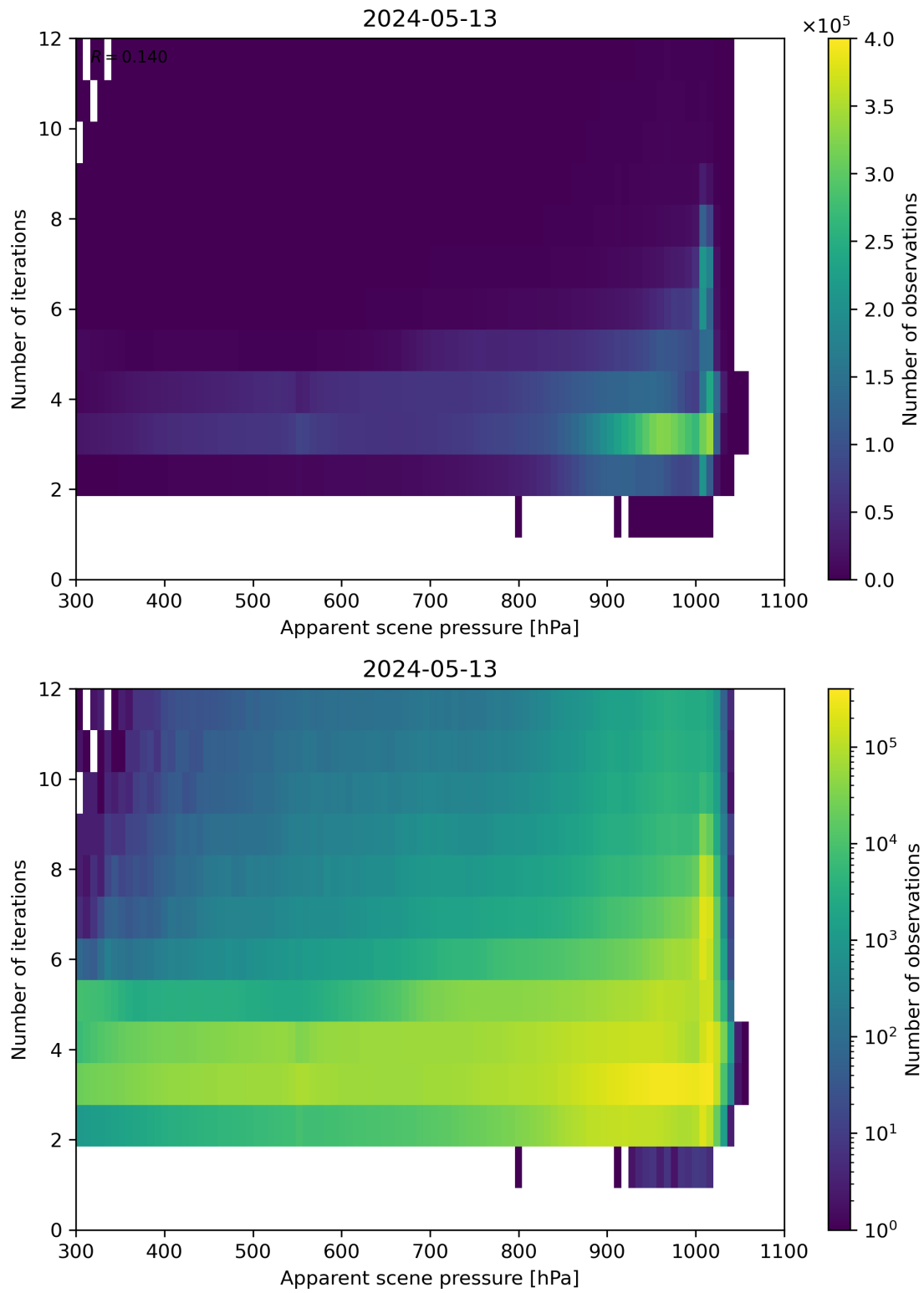
Figure 65: Scatter density plot of “Apparent scene pressure” against “Number of iterations” for 2024-05-12 to 2024-05-14.
