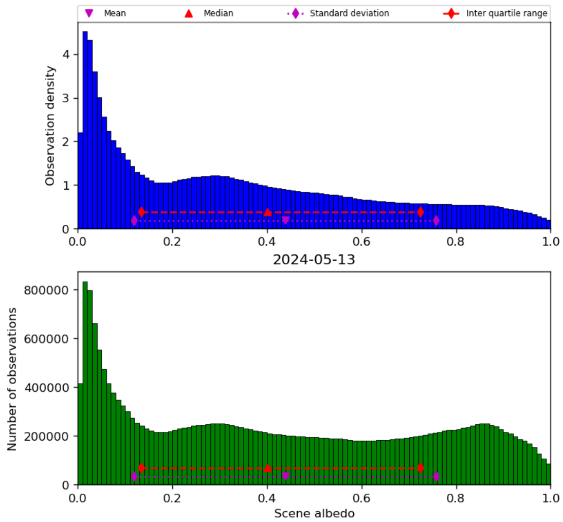
Figure 34: Histogram of “Scene albedo” for 2024-05-12 to 2024-05-14
