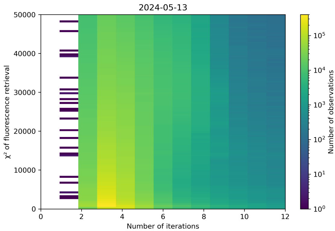
Figure 97: Scatter density plot of “Number of iterations” against “ \chi^2 of fluorescence retrieval” for 2024-05-12 to 2024-05-14.
