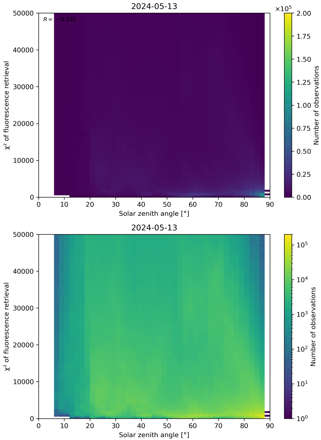
Figure 109: Scatter density plot of “Solar zenith angle” against “ \chi^2 of fluorescence retrieval” for 2024-05-12 to 2024-05-14.
