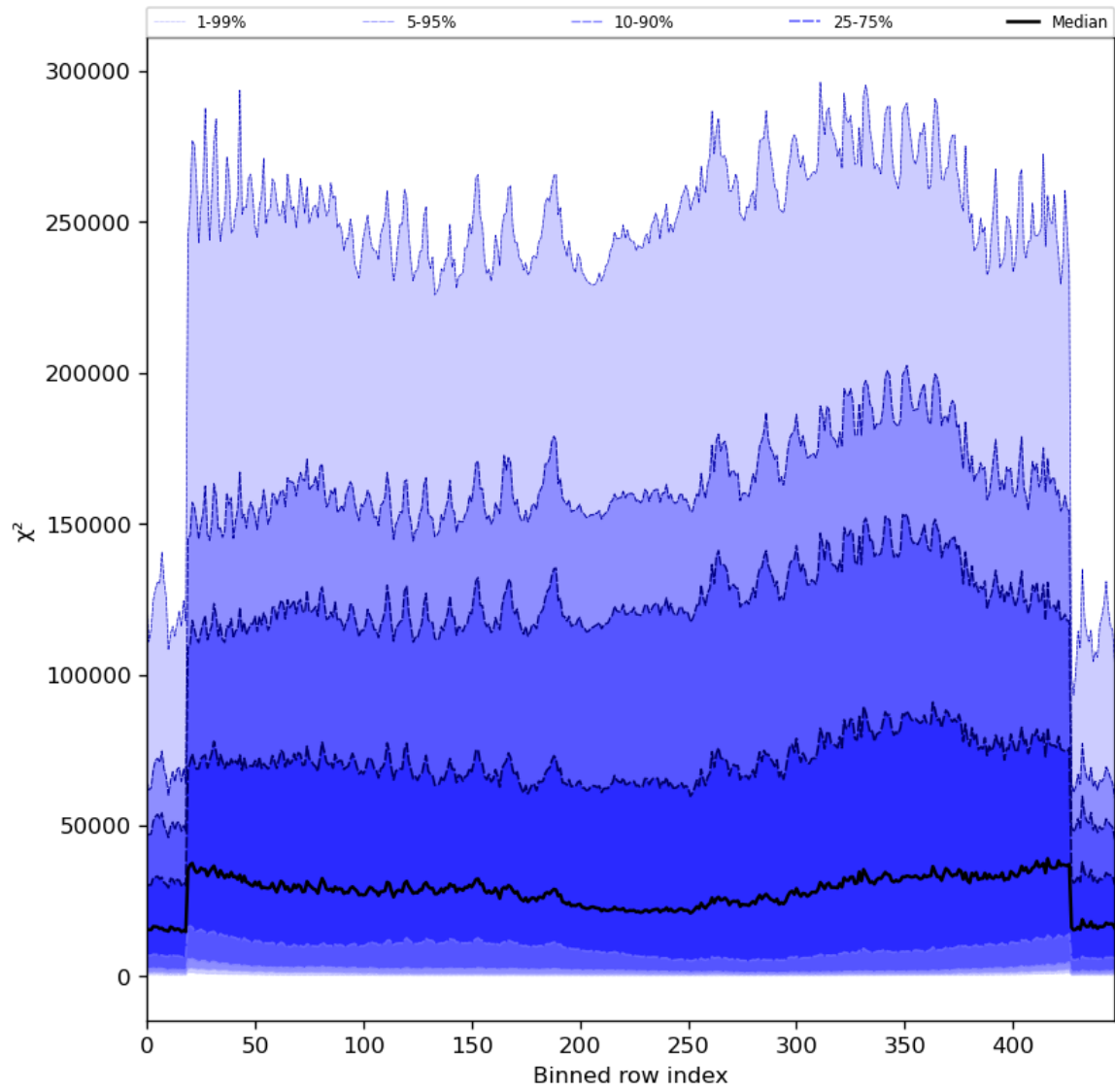
Figure 55: Along track statistics of “ \chi^2 ” for 2024-05-12 to 2024-05-14
