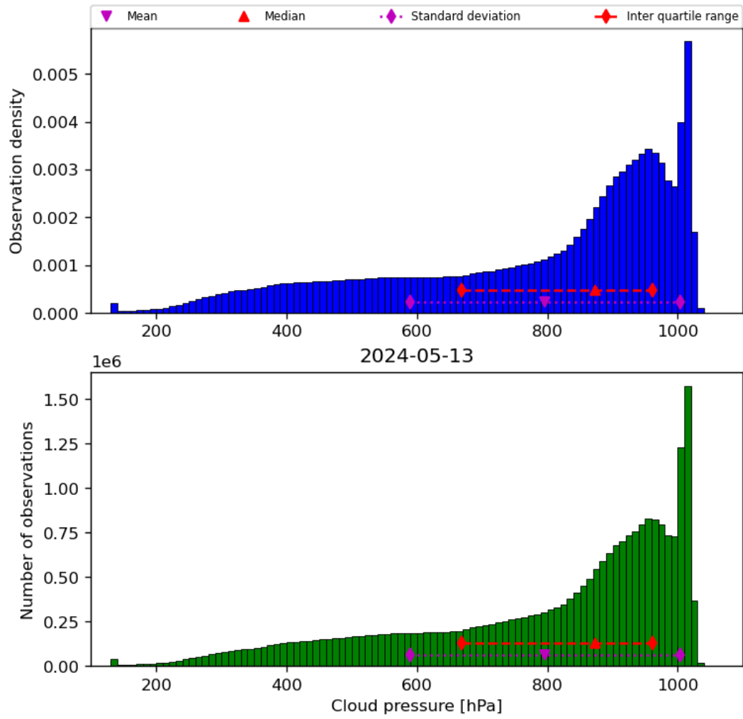
Figure 30: Histogram of “Cloud pressure” for 2024-05-12 to 2024-05-14
