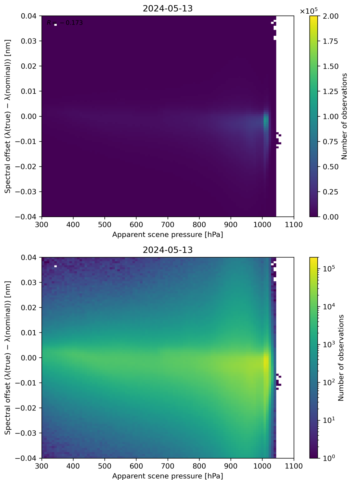
Figure 67: Scatter density plot of “Apparent scene pressure” against “Spectral offset ( \lambda(\text{true}) - \lambda(\text{nominal}) )” for 2024-05-12 to 2024-05-14.
