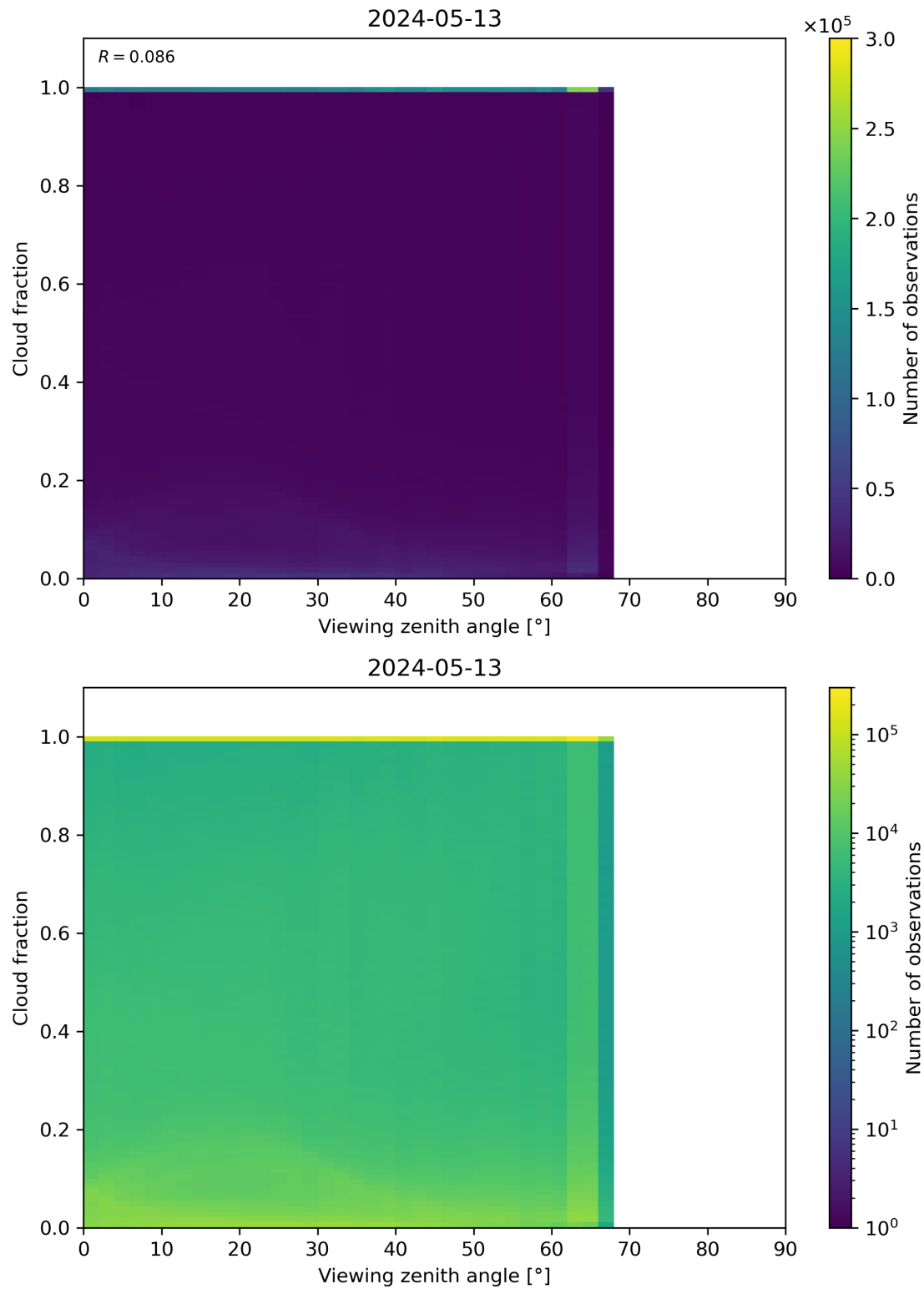
Figure 120: Scatter density plot of “Viewing zenith angle” against “Cloud fraction” for 2024-05-12 to 2024-05-14.
