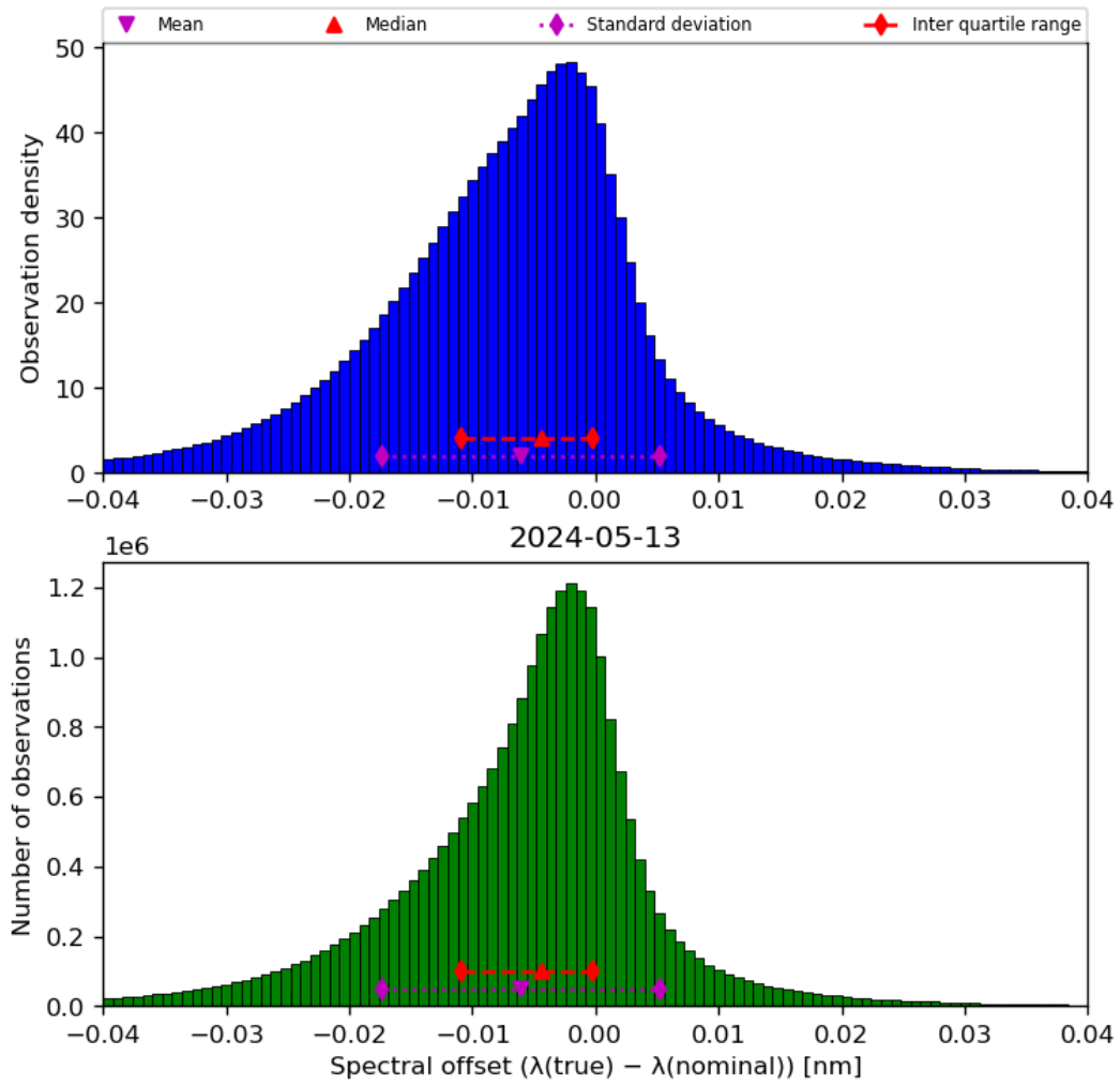
Figure 45: Histogram of “Spectral offset ( \lambda(\text{true}) - \lambda(\text{nominal}) )” for 2024-05-12 to 2024-05-14
