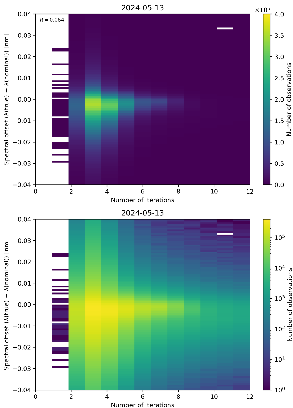
Figure 100: Scatter density plot of “Number of iterations” against “Spectral offset ( \lambda(\text{true}) - \lambda(\text{nominal}) )” for 2024-05-12 to 2024-05-14.
