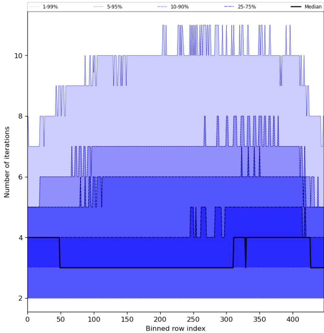
Figure 56: Along track statistics of “Number of iterations” for 2024-05-12 to 2024-05-14
