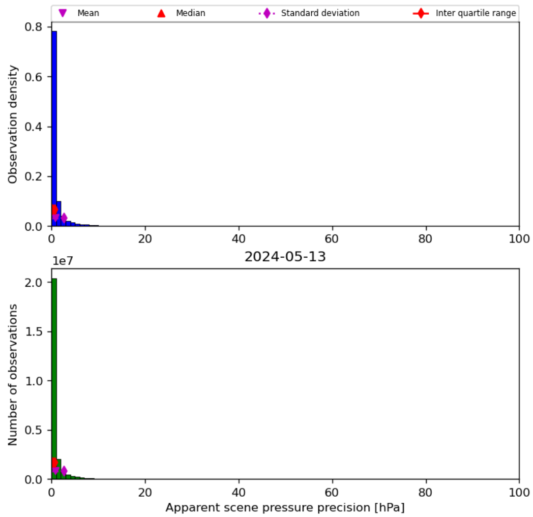
Figure 37: Histogram of “Apparent scene pressure precision” for 2024-05-12 to 2024-05-14
