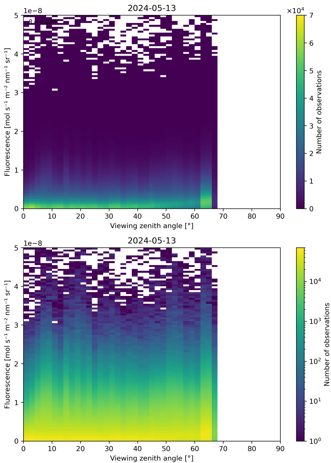
Figure 122: Scatter density plot of “Viewing zenith angle” against “Fluorescence” for 2024-05-12 to 2024-05-14.
