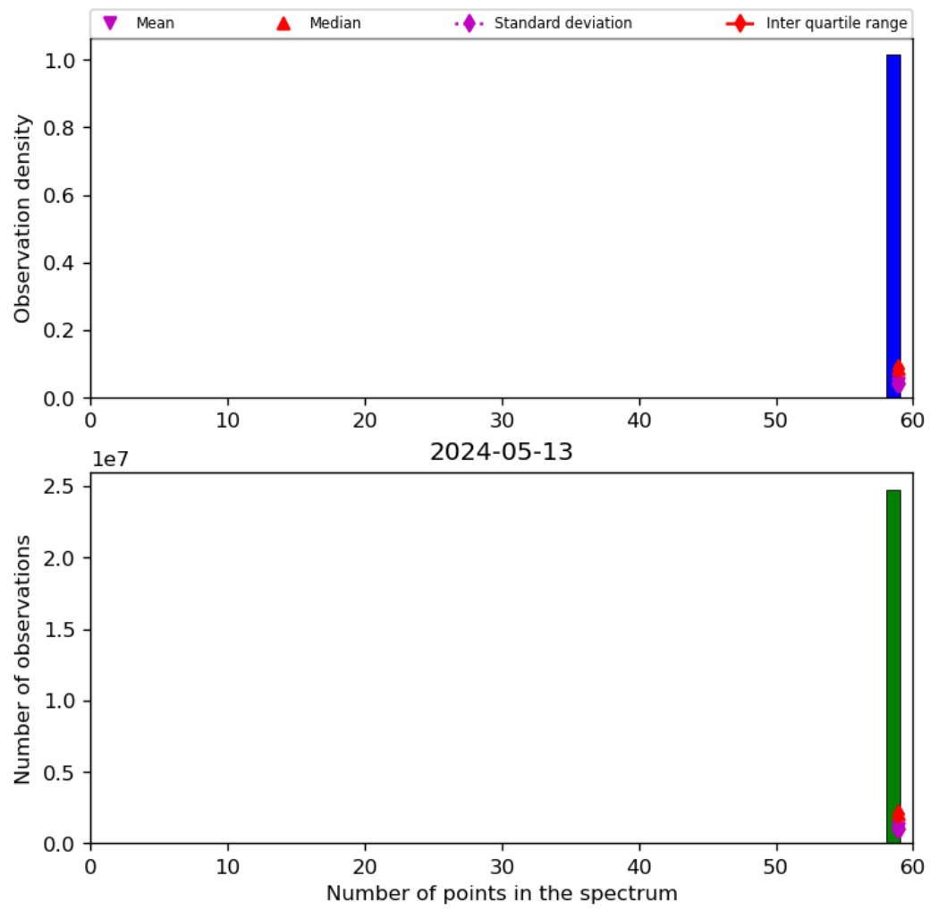
Figure 44: Histogram of “Number of points in the spectrum” for 2024-05-12 to 2024-05-14
