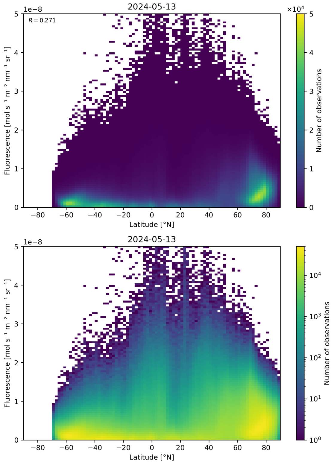
Figure 92: Scatter density plot of “Latitude” against “Fluorescence” for 2024-05-12 to 2024-05-14.
