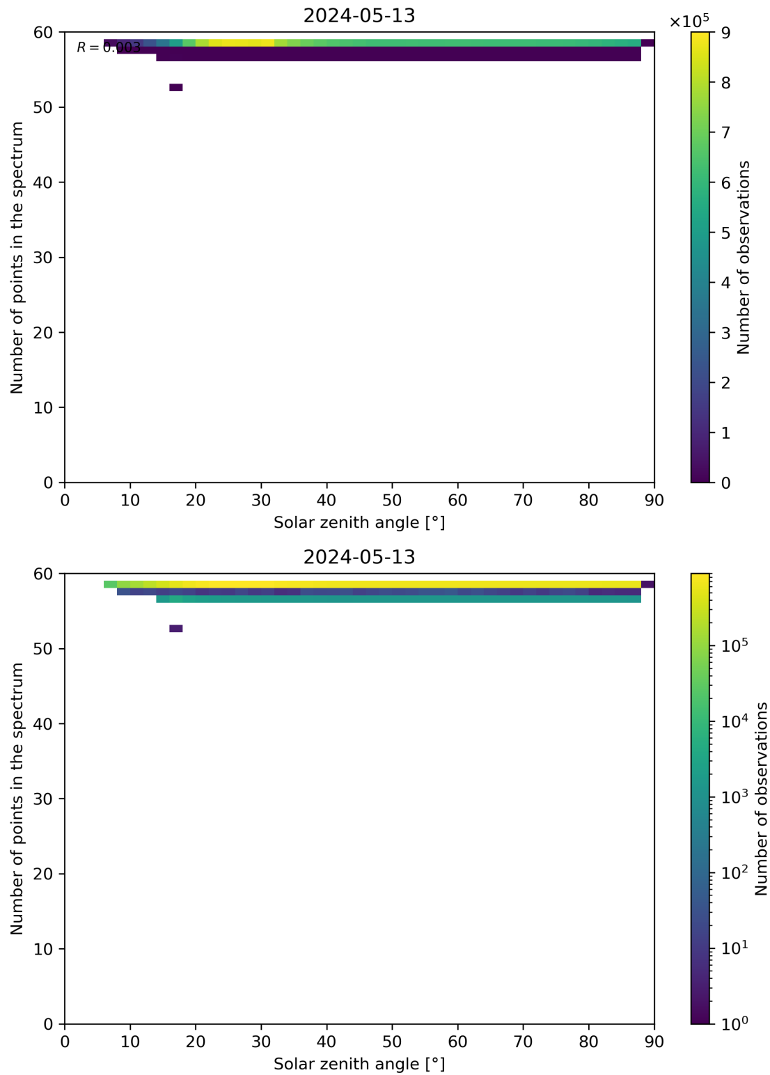
Figure 115: Scatter density plot of “Solar zenith angle” against “Number of points in the spectrum” for 2024-05-12 to 2024-05-14.
