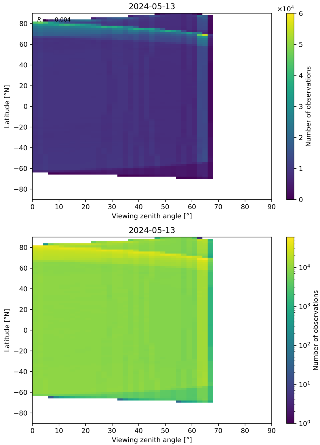
Figure 123: Scatter density plot of “Viewing zenith angle” against “Latitude” for 2024-05-12 to 2024-05-14.
