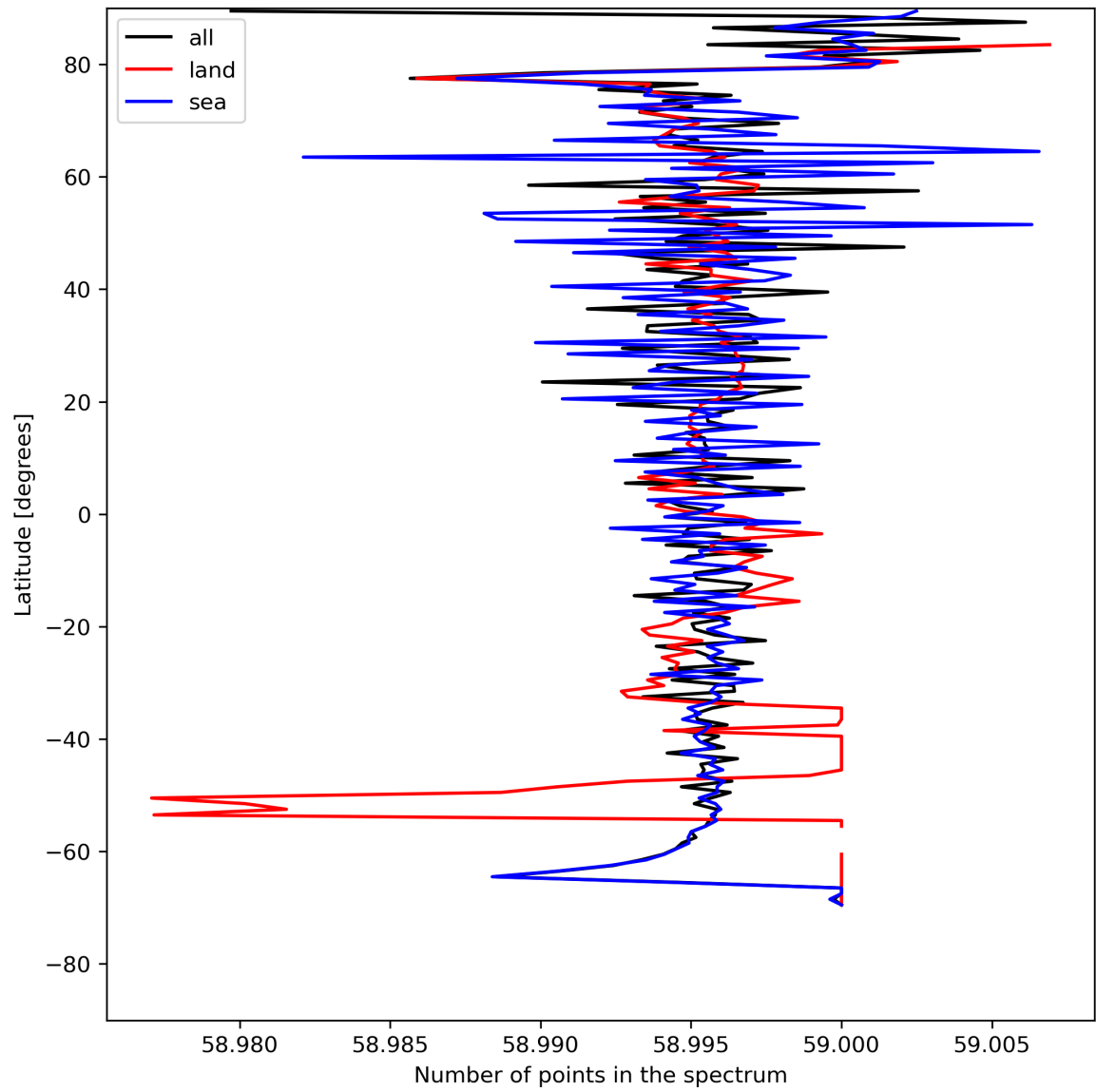
Figure 27: Zonal average of “Number of points in the spectrum” for 2024-05-12 to 2024-05-14.
