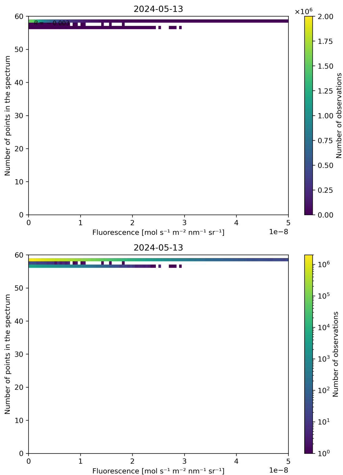
Figure 86: Scatter density plot of “Fluorescence” against “Number of points in the spectrum” for 2024-05-12 to 2024-05-14.
