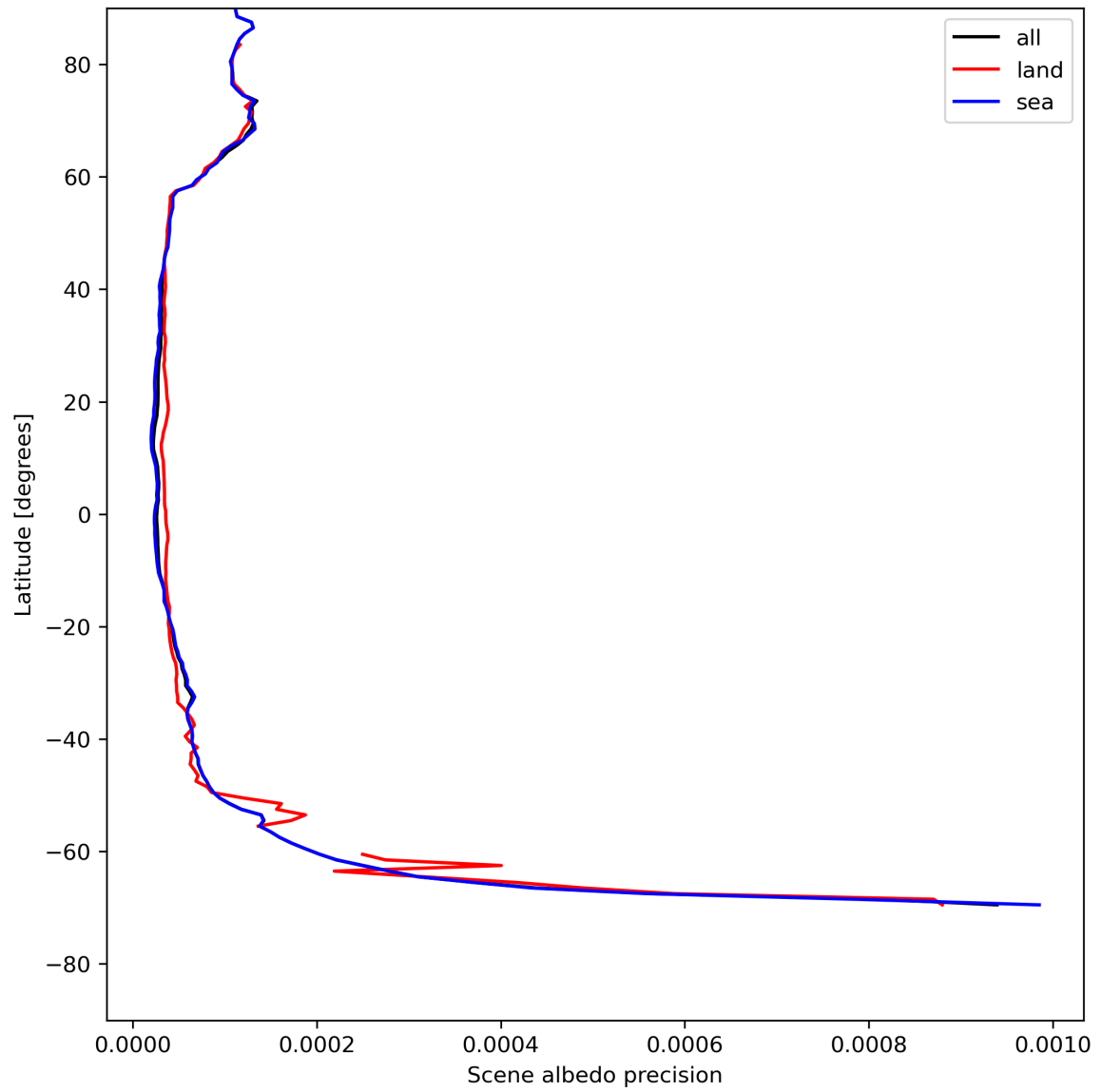
Figure 18: Zonal average of “Scene albedo precision” for 2024-05-12 to 2024-05-14.
