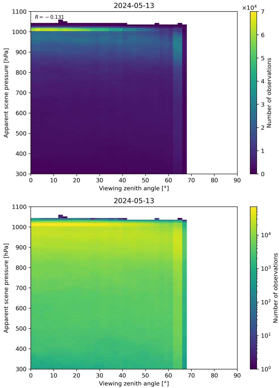
Figure 118: Scatter density plot of “Viewing zenith angle” against “Apparent scene pressure” for 2024-05-12 to 2024-05-14.
