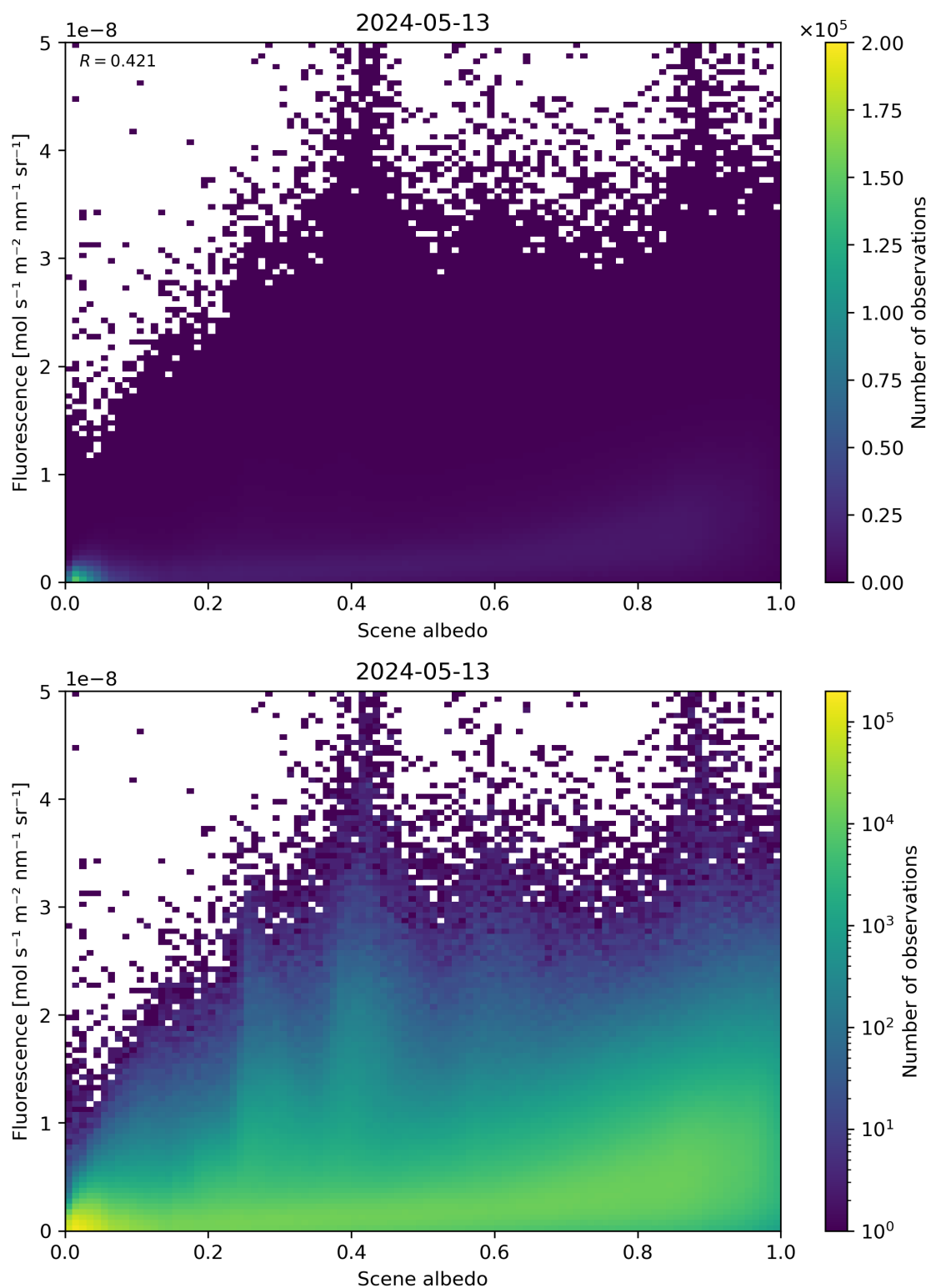
Figure 104: Scatter density plot of “Scene albedo” against “Fluorescence” for 2024-05-12 to 2024-05-14.
