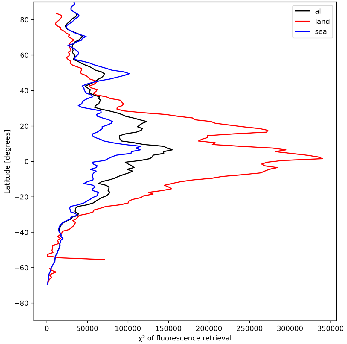
Figure 25: Zonal average of “ \chi^2 of fluorescence retrieval” for 2024-05-12 to 2024-05-14.
