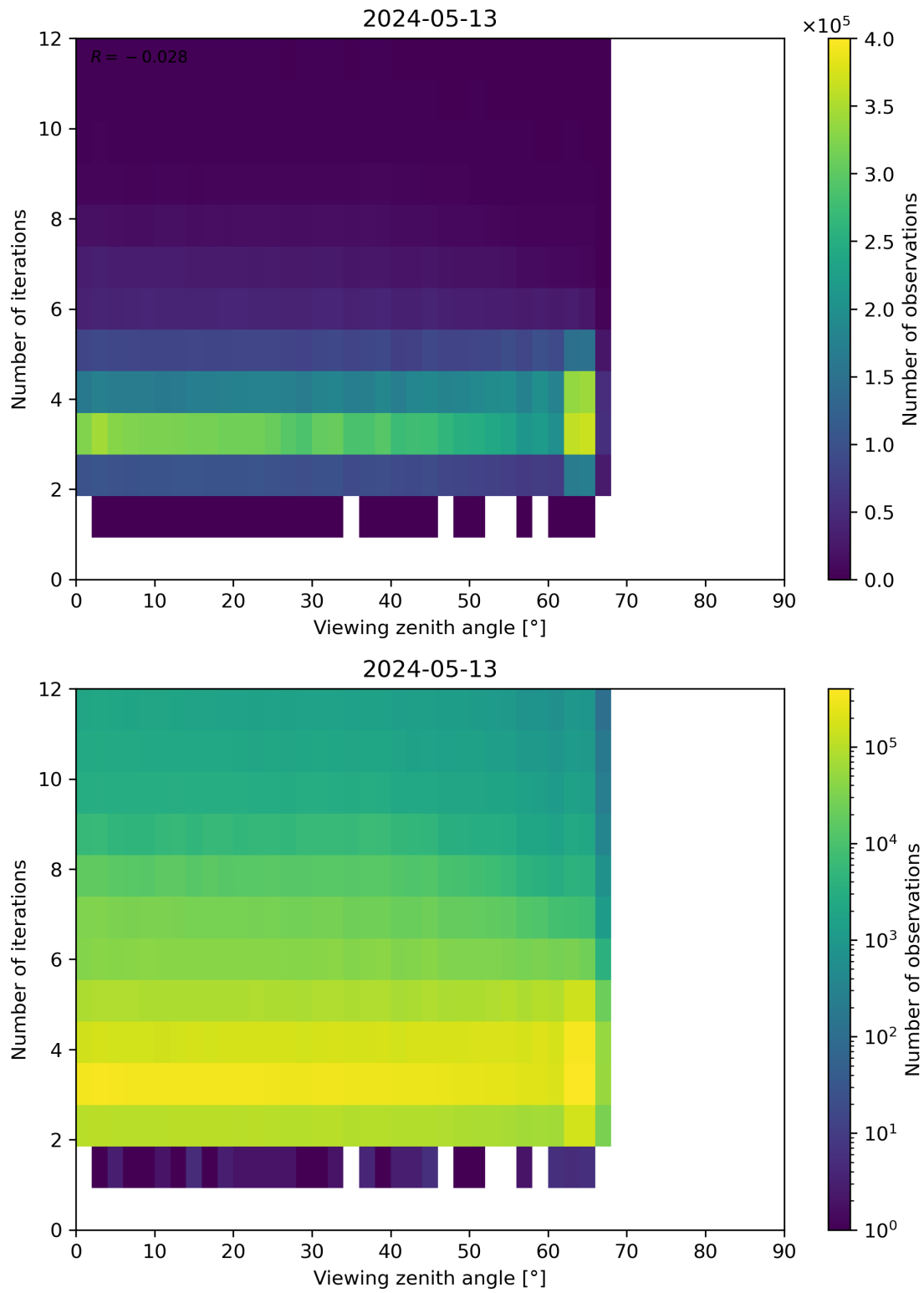
Figure 124: Scatter density plot of “Viewing zenith angle” against “Number of iterations” for 2024-05-12 to 2024-05-14.
