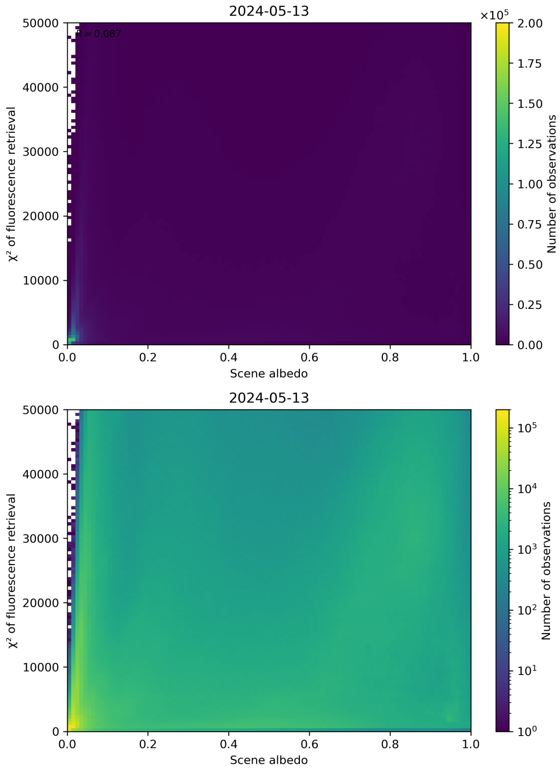
Figure 103: Scatter density plot of “Scene albedo” against “ \chi^2 of fluorescence retrieval” for 2024-05-12 to 2024-05-14.
