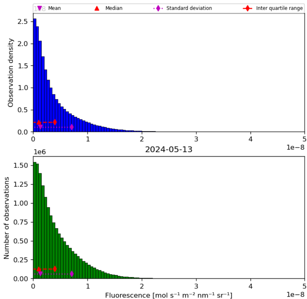
Figure 40: Histogram of “Fluorescence” for 2024-05-12 to 2024-05-14
