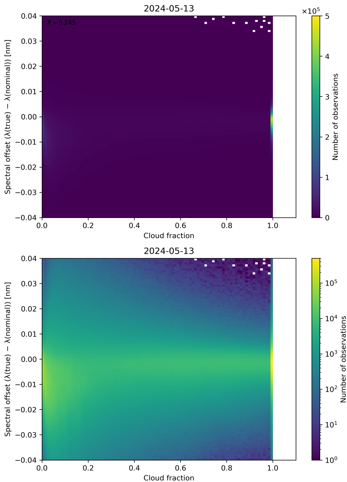
Figure 76: Scatter density plot of “Cloud fraction” against “Spectral offset ( \lambda(\text{true}) - \lambda(\text{nominal}) )” for 2024-05-12 to 2024-05-14.
