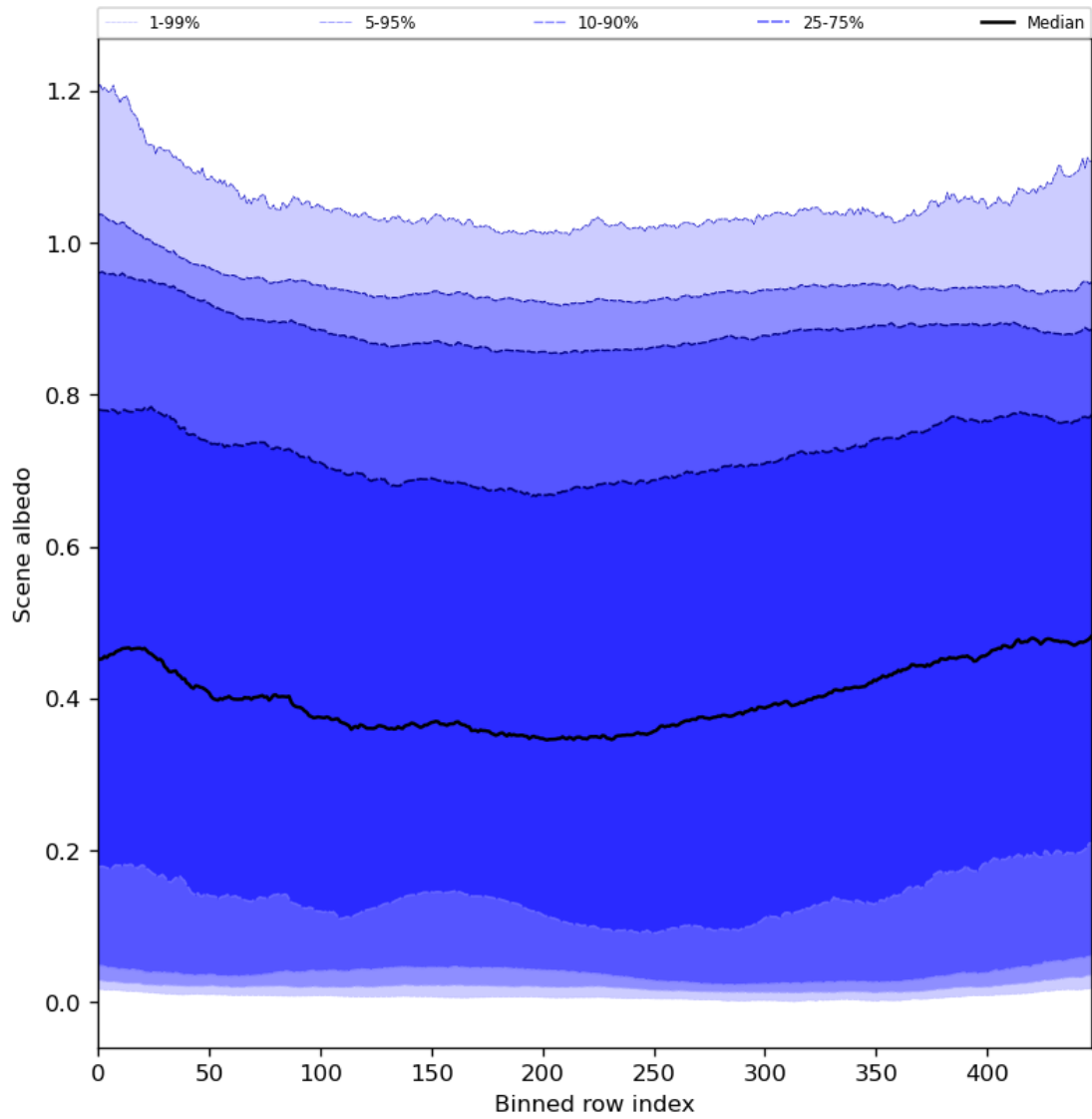
Figure 51: Along track statistics of “Scene albedo” for 2024-05-12 to 2024-05-14
