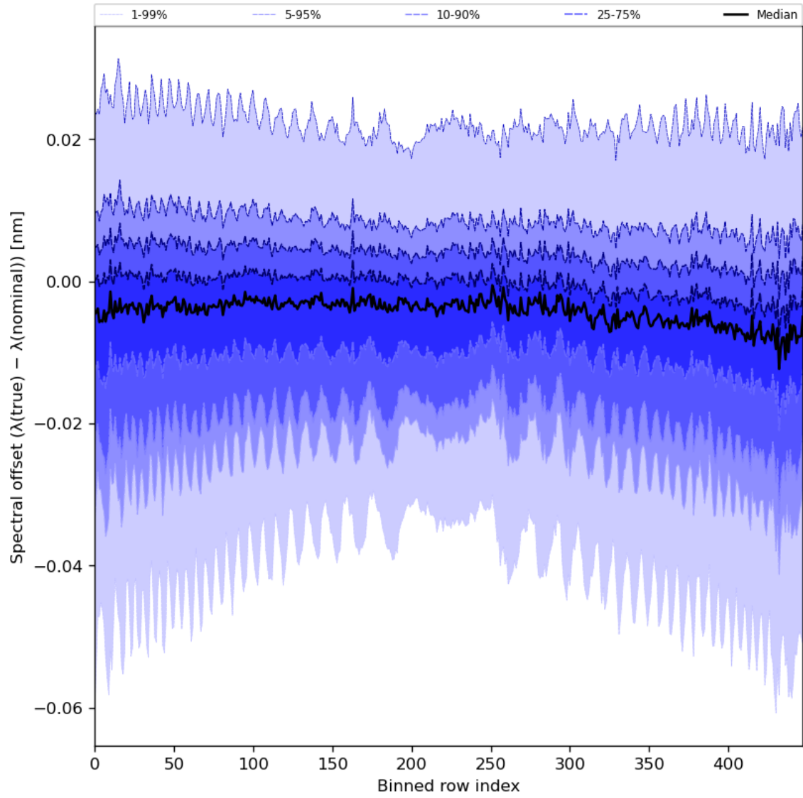
Figure 62: Along track statistics of “Spectral offset ( \lambda(\text{true}) - \lambda(\text{nominal}) )” for 2024-05-12 to 2024-05-14
