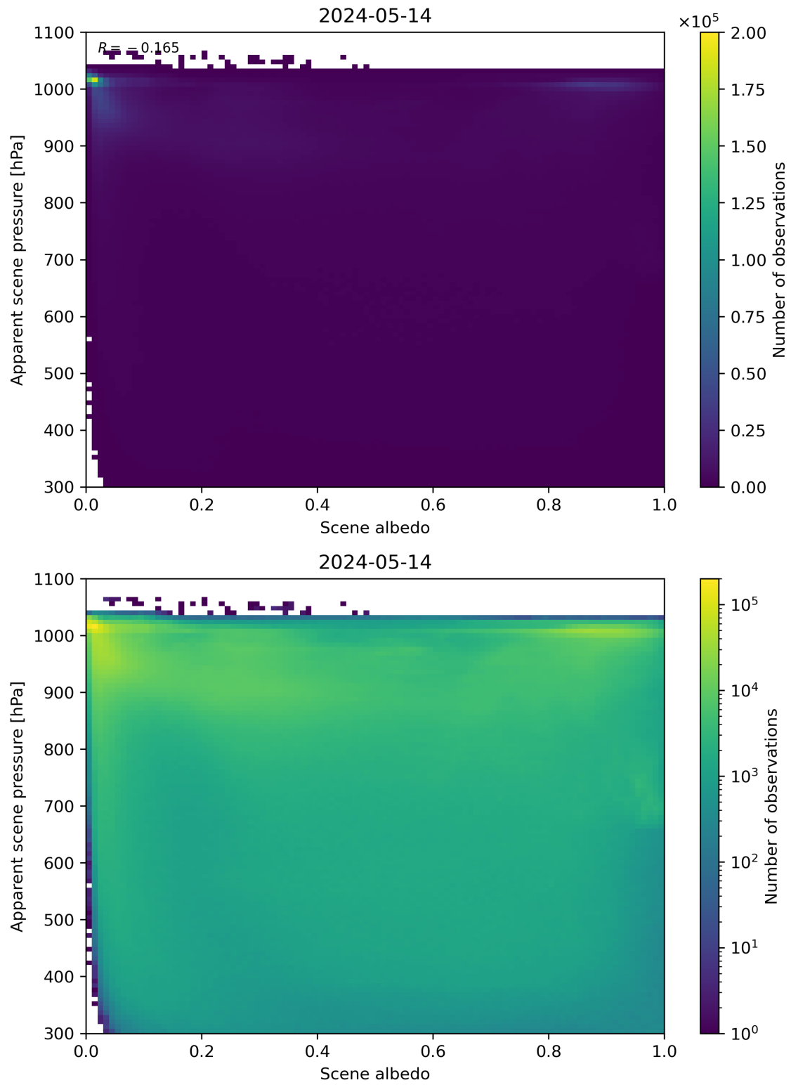
Figure 102: Scatter density plot of “Scene albedo” against “Apparent scene pressure” for 2024-05-13 to 2024-05-15.
