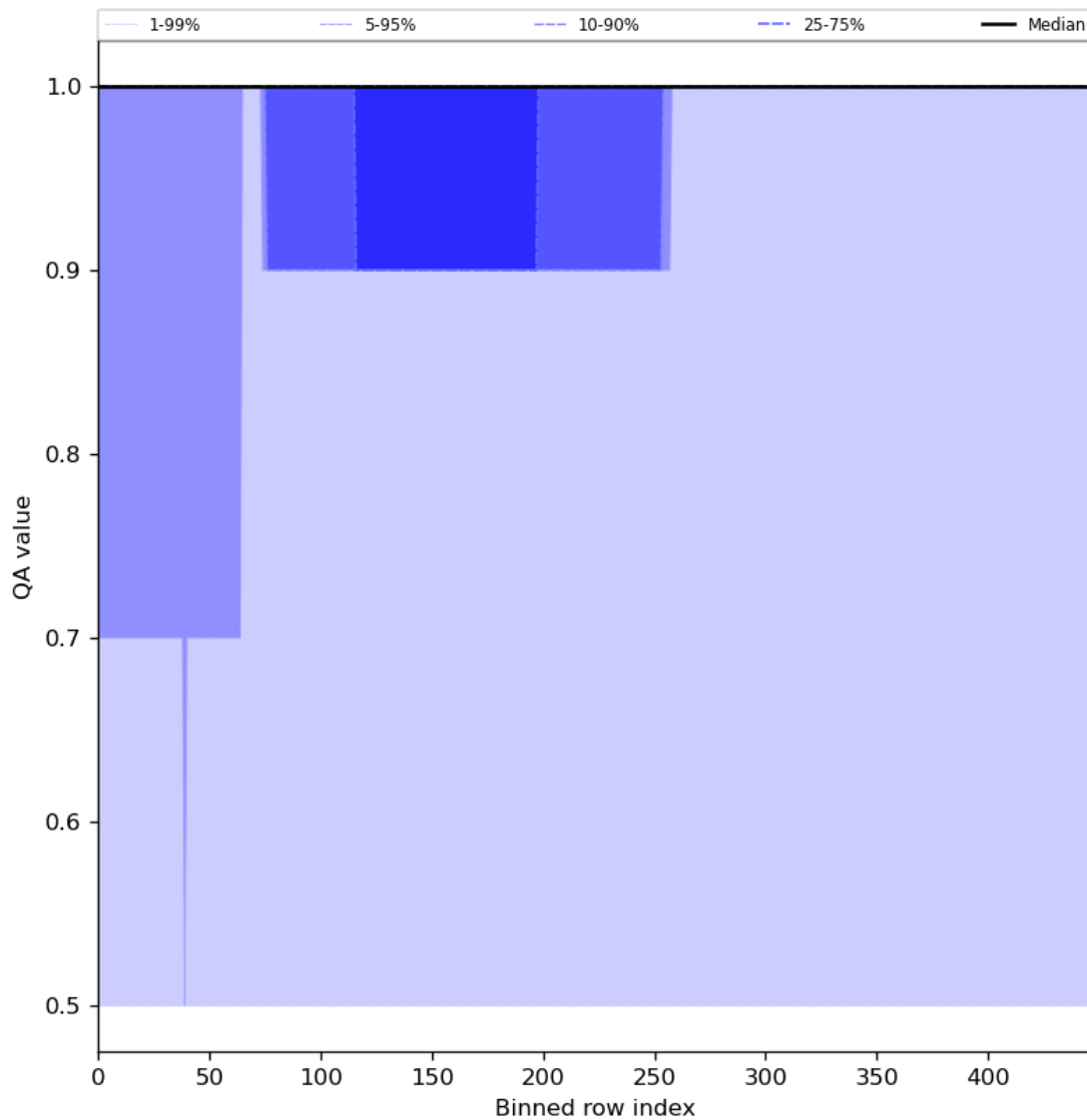
Figure 46: Along track statistics of “QA value” for 2024-05-13 to 2024-05-15
