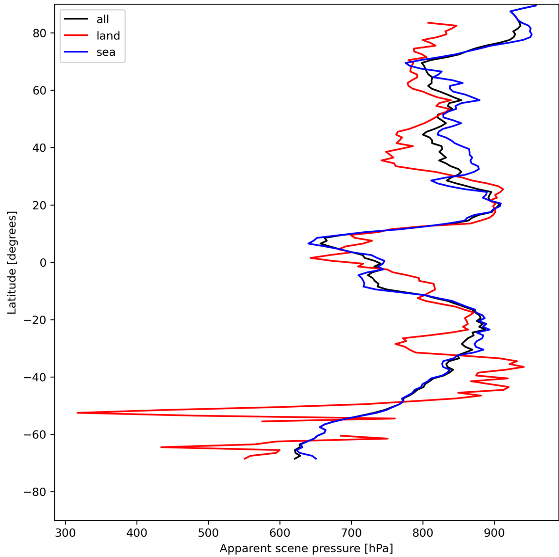
Figure 19: Zonal average of “Apparent scene pressure” for 2024-05-13 to 2024-05-15.
