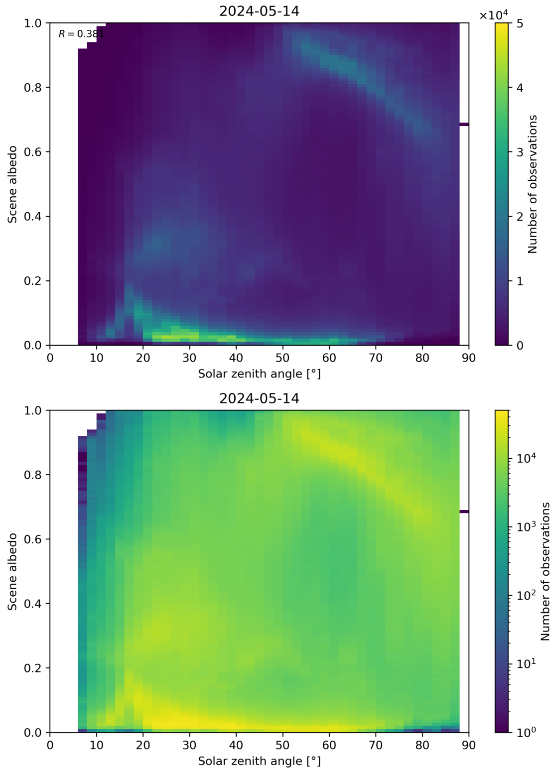
Figure 116: Scatter density plot of “Solar zenith angle” against “Scene albedo” for 2024-05-13 to 2024-05-15.
