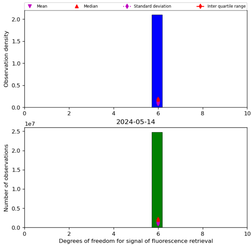
Figure 43: Histogram of “Degrees of freedom for signal of fluorescence retrieval” for 2024-05-13 to 2024-05-15
