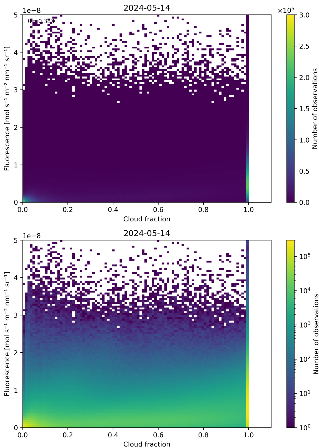
Figure 72: Scatter density plot of “Cloud fraction” against “Fluorescence” for 2024-05-13 to 2024-05-15.
