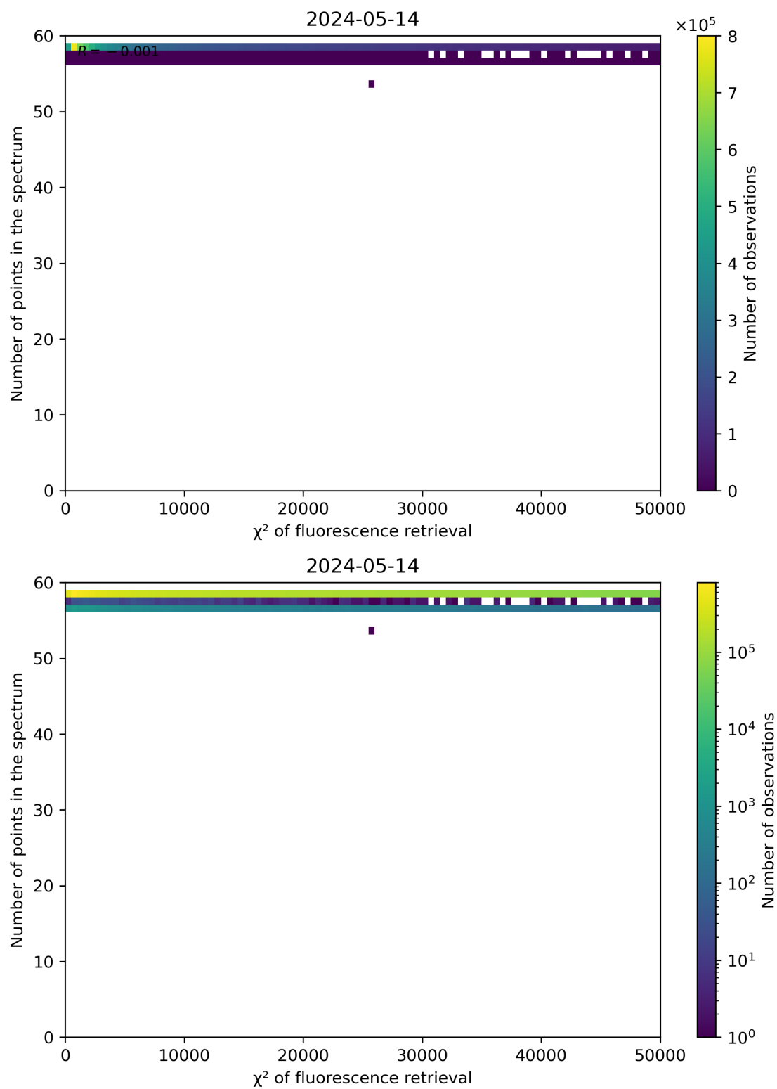
Figure 68: Scatter density plot of " \chi^2 of fluorescence retrieval" against "Number of points in the spectrum" for 2024-05-13 to 2024-05-15.
