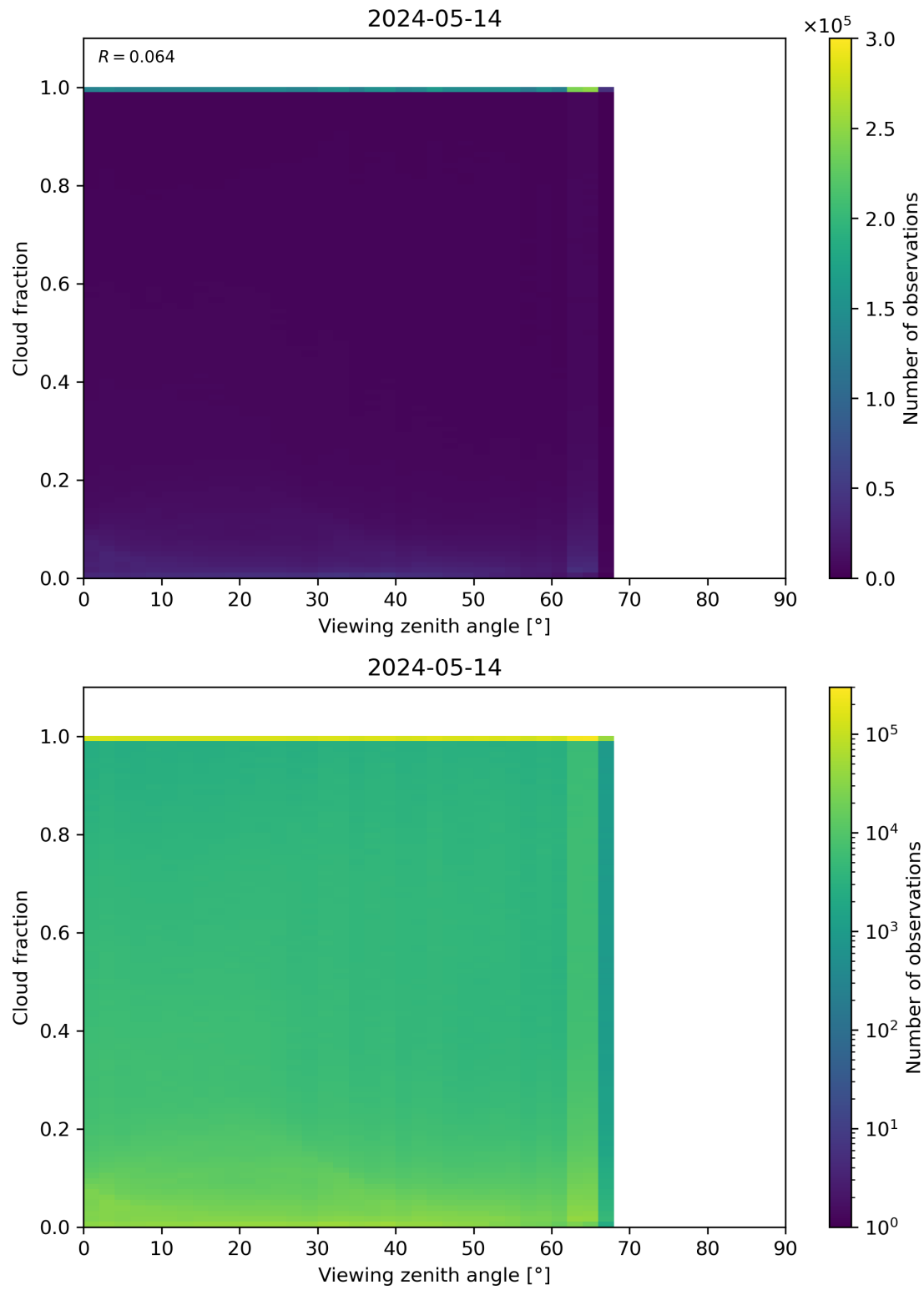
Figure 120: Scatter density plot of “Viewing zenith angle” against “Cloud fraction” for 2024-05-13 to 2024-05-15.
