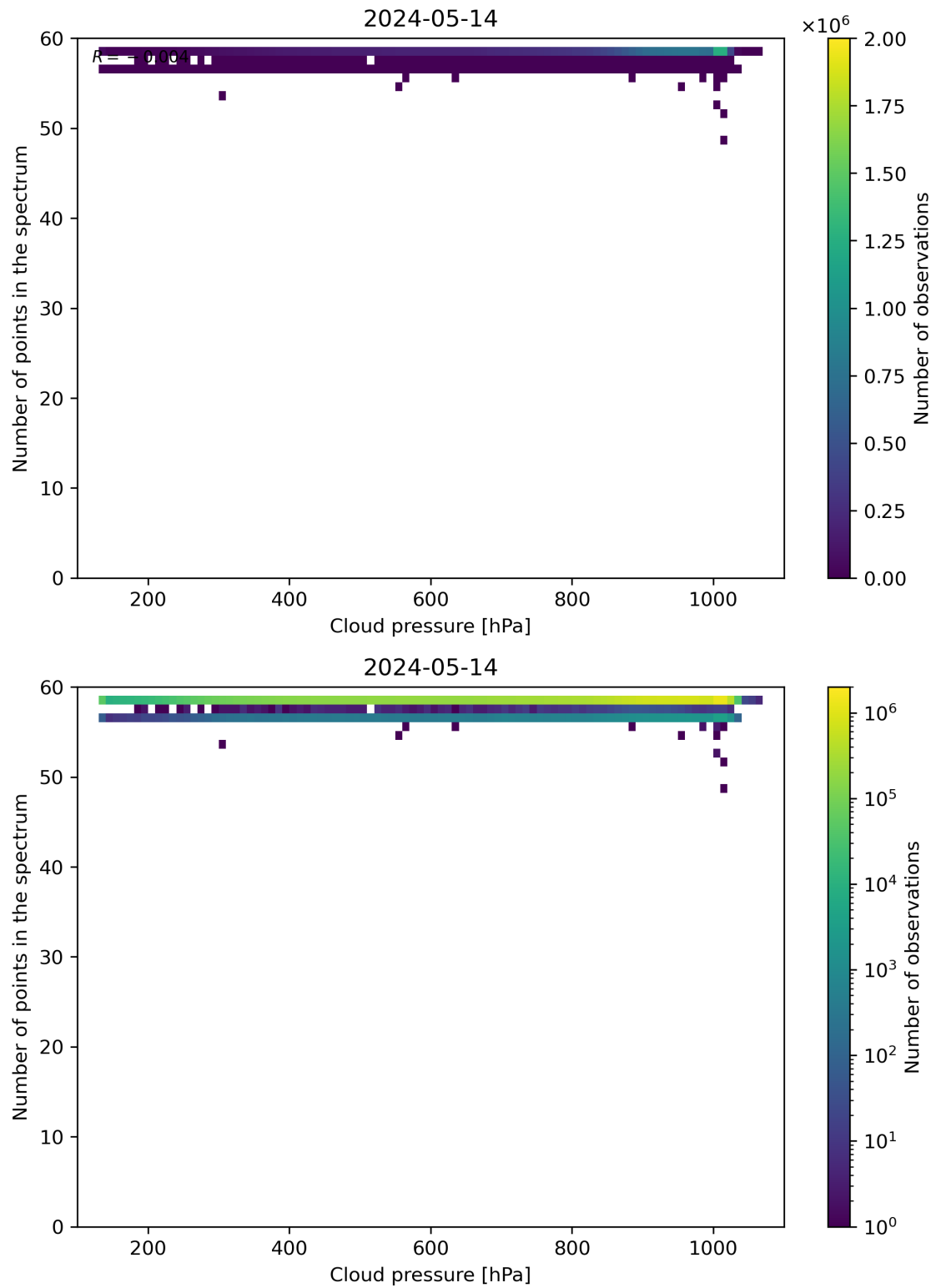
Figure 82: Scatter density plot of “Cloud pressure” against “Number of points in the spectrum” for 2024-05-13 to 2024-05-15.
