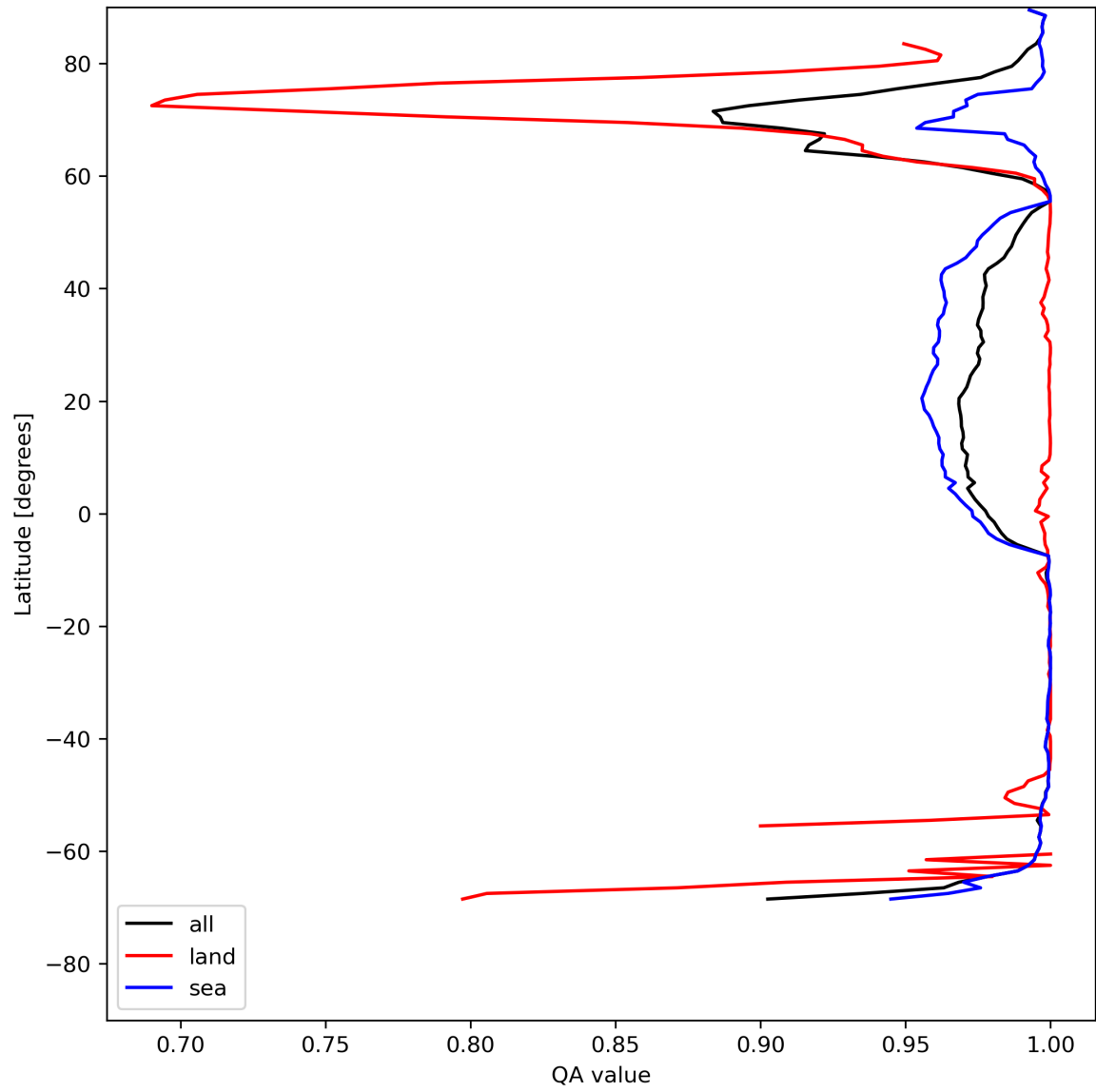
Figure 12: Zonal average of “QA value” for 2024-05-13 to 2024-05-15.
