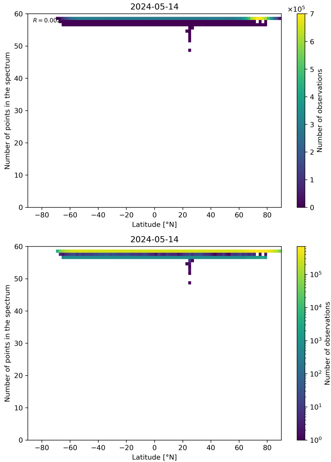
Figure 94: Scatter density plot of “Latitude” against “Number of points in the spectrum” for 2024-05-13 to 2024-05-15.
