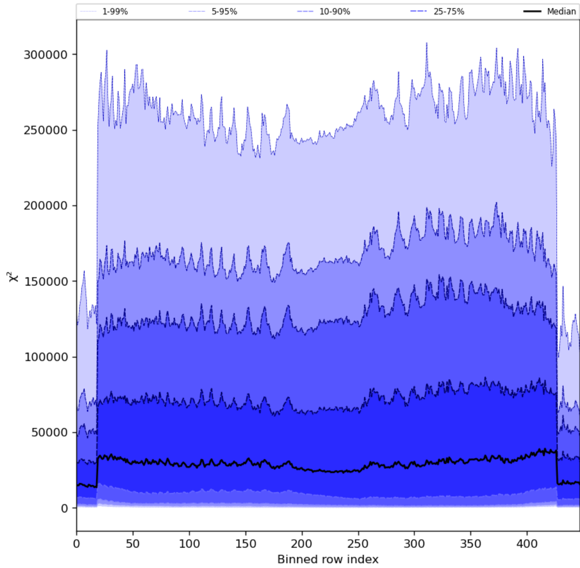
Figure 55: Along track statistics of “ \chi^2 ” for 2024-05-13 to 2024-05-15
