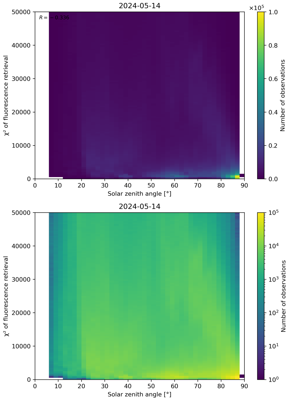
Figure 109: Scatter density plot of “Solar zenith angle” against “ \chi^2 of fluorescence retrieval” for 2024-05-13 to 2024-05-15.
