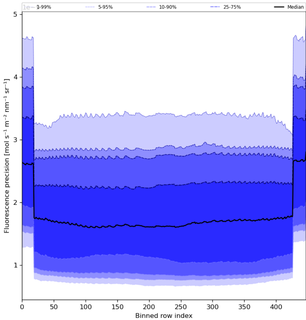
Figure 58: Along track statistics of “Fluorescence precision” for 2024-05-13 to 2024-05-15
