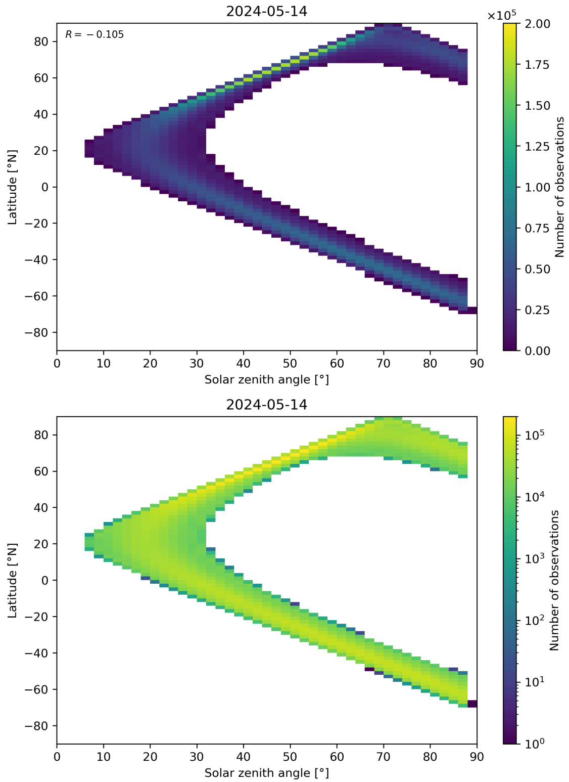
Figure 113: Scatter density plot of “Solar zenith angle” against “Latitude” for 2024-05-13 to 2024-05-15.
