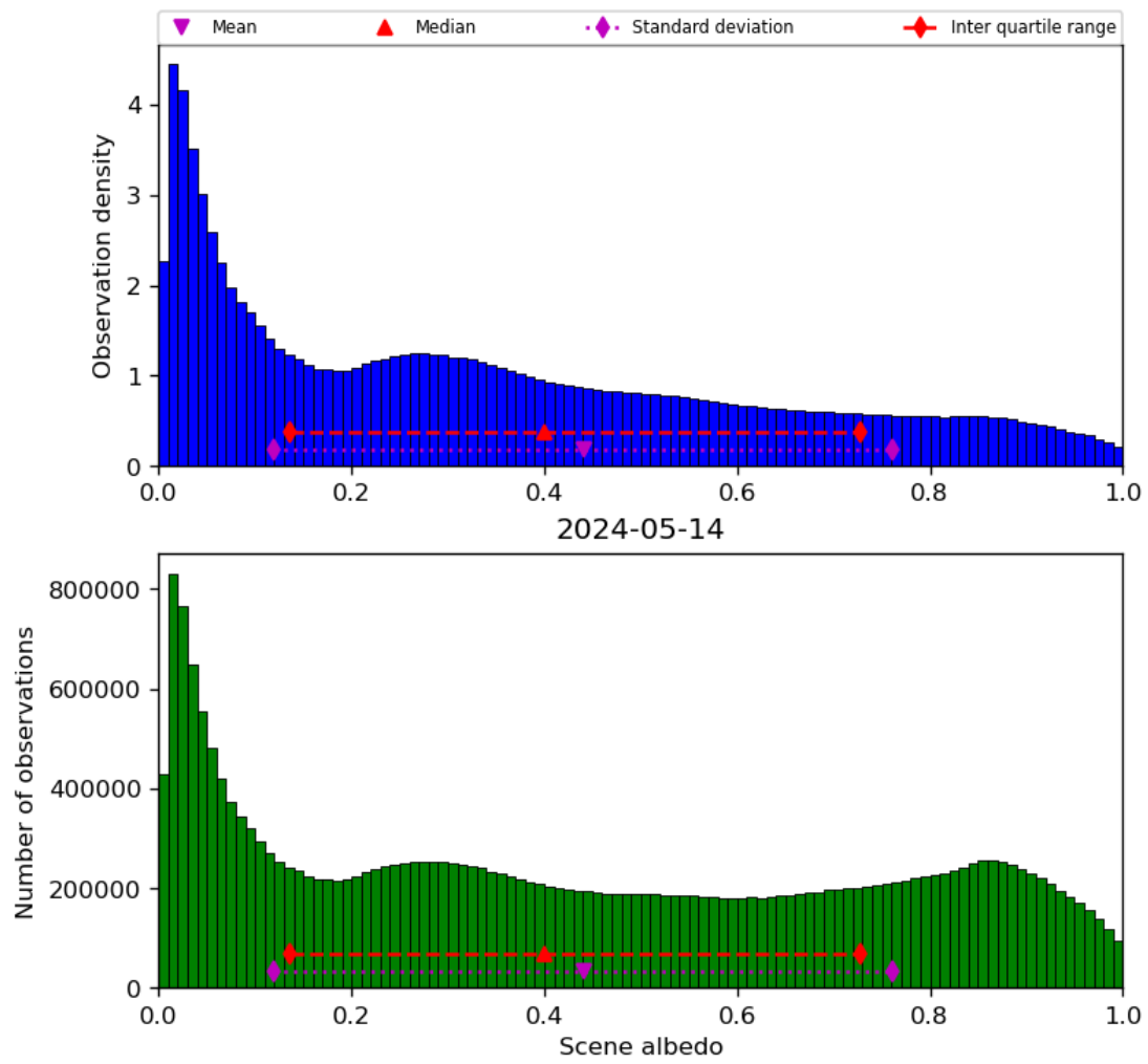
Figure 34: Histogram of “Scene albedo” for 2024-05-13 to 2024-05-15
