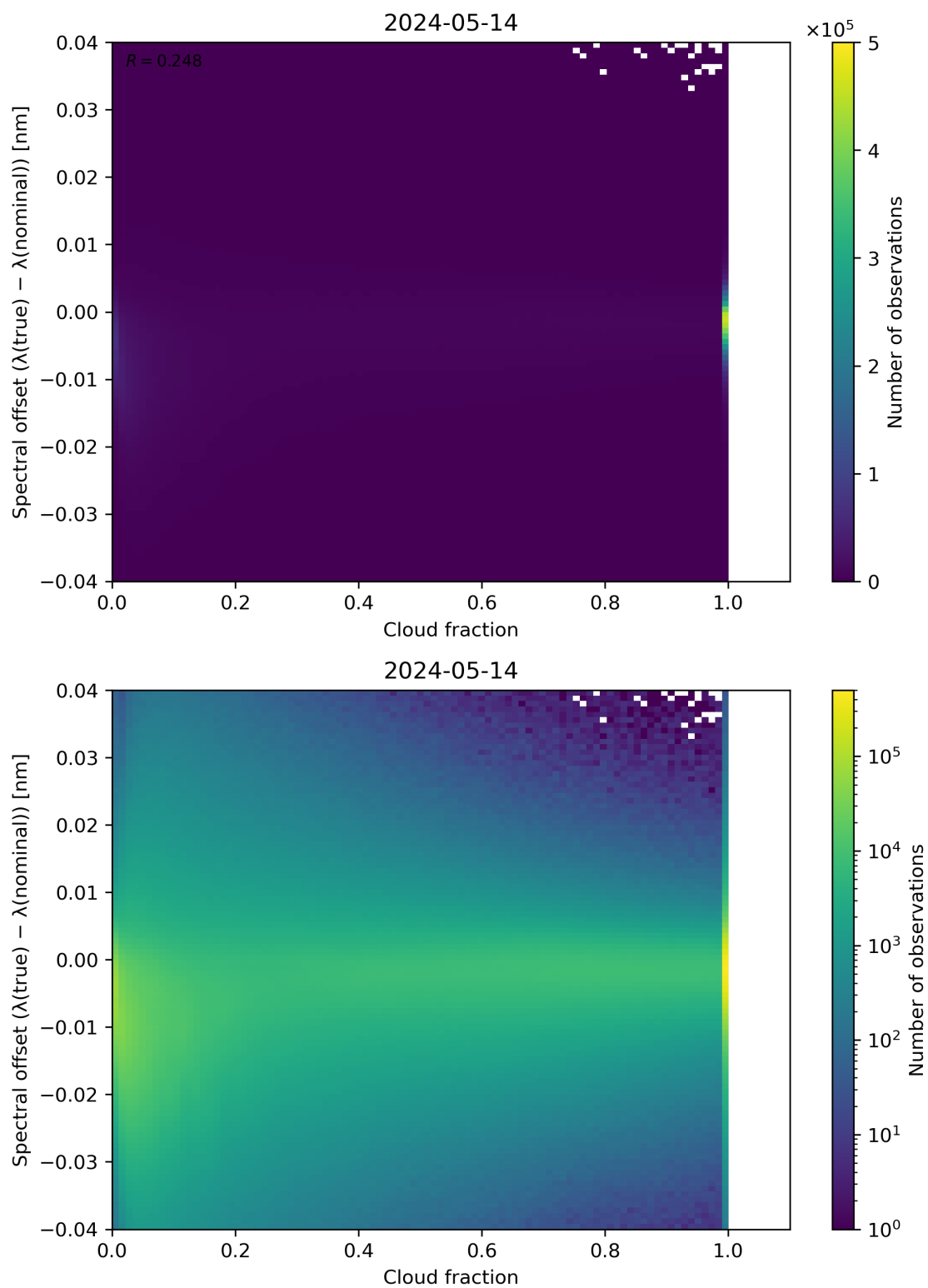
Figure 76: Scatter density plot of “Cloud fraction” against “Spectral offset ( \lambda(\text{true}) - \lambda(\text{nominal}) )” for 2024-05-13 to 2024-05-15.
