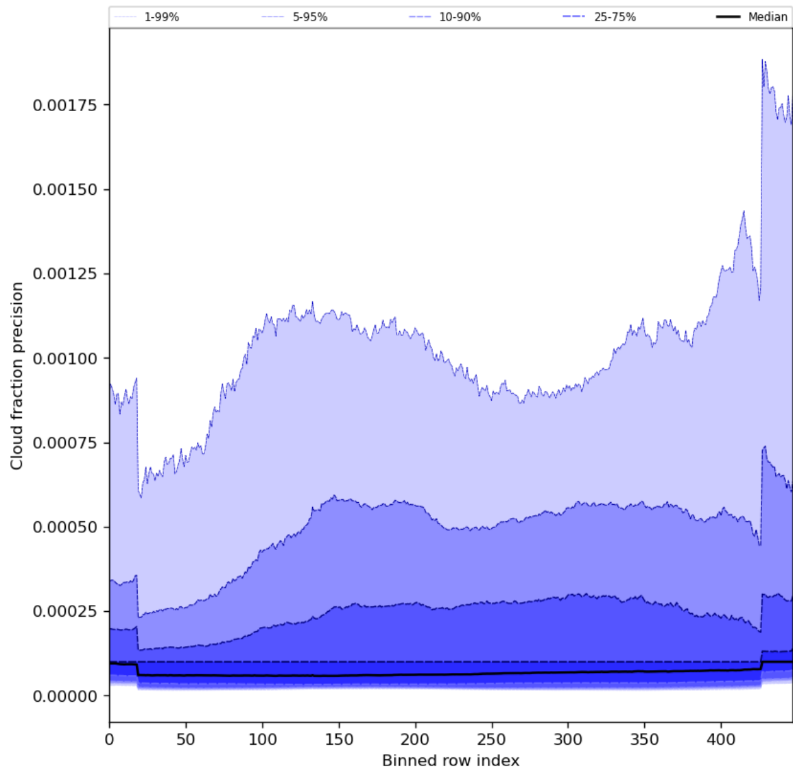
Figure 50: Along track statistics of “Cloud fraction precision” for 2024-05-13 to 2024-05-15
