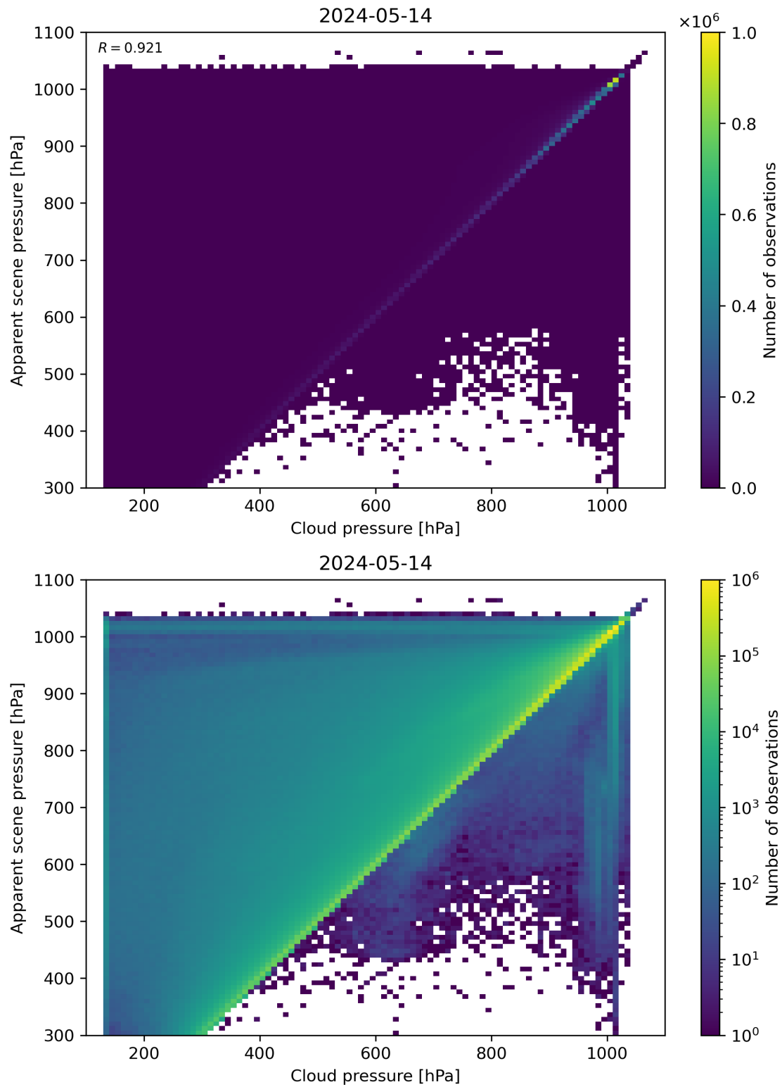
Figure 77: Scatter density plot of “Cloud pressure” against “Apparent scene pressure” for 2024-05-13 to 2024-05-15.
