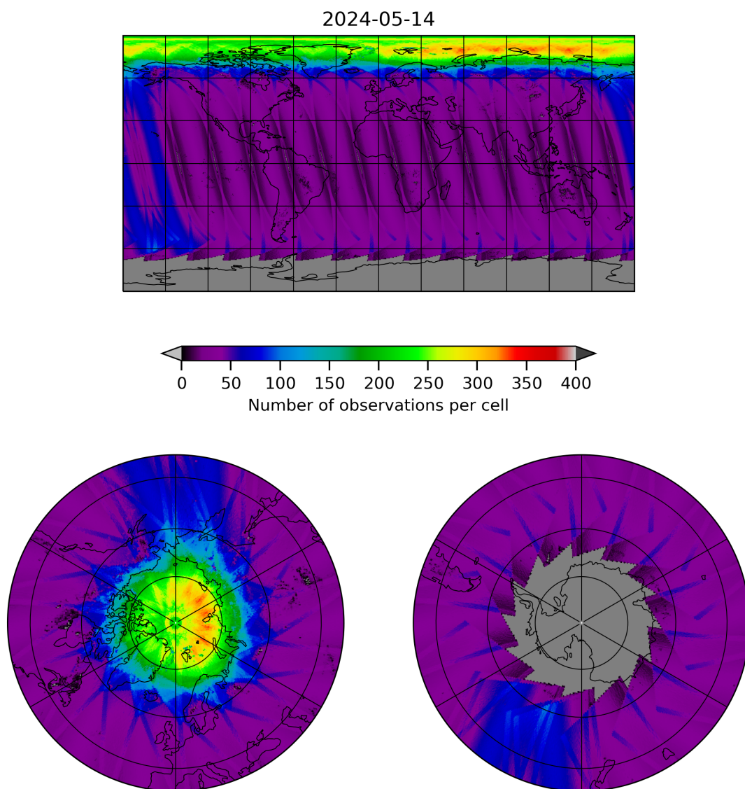
Figure 11: Map of the number of observations for 2024-05-13 to 2024-05-15
