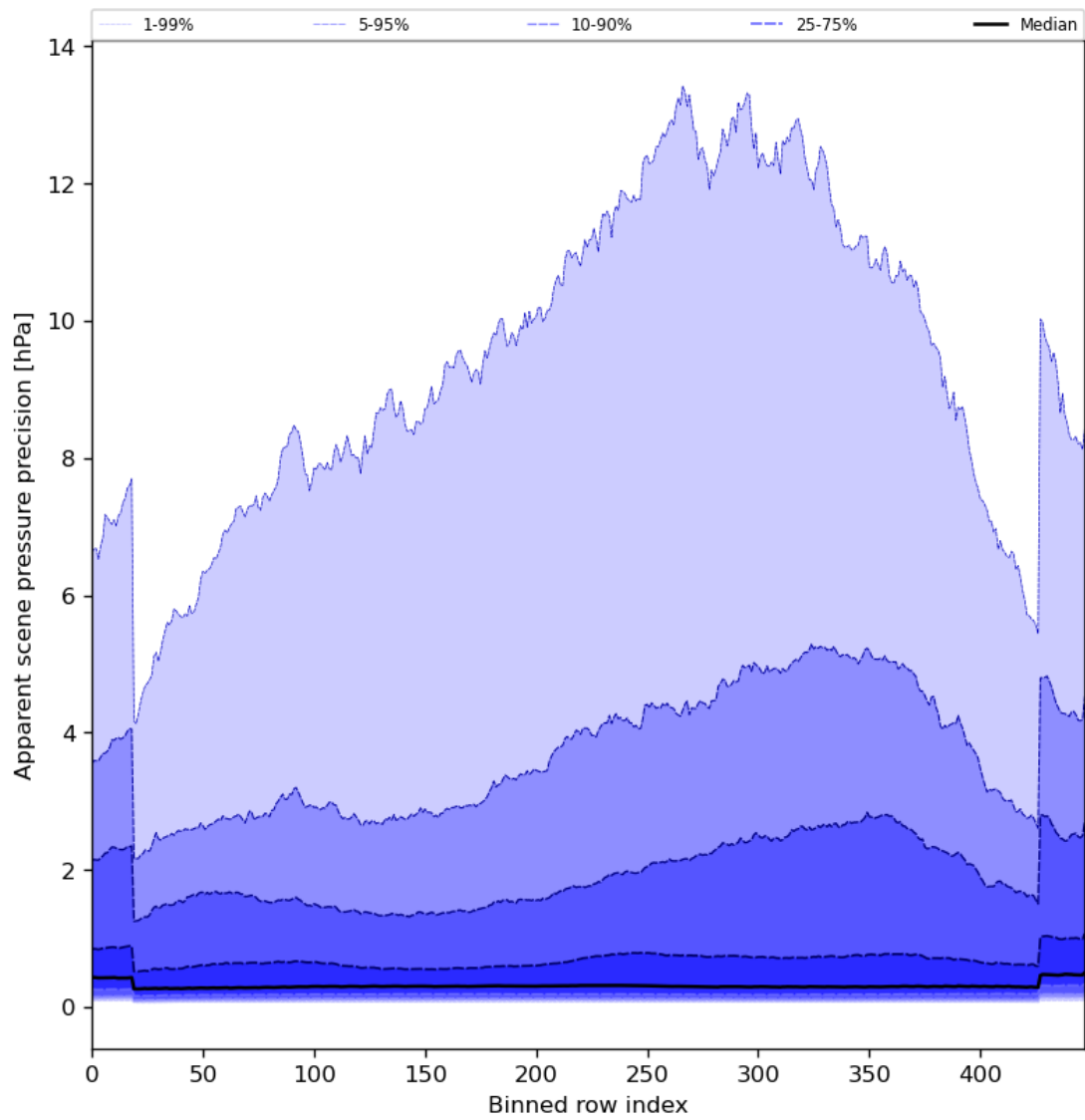
Figure 54: Along track statistics of “Apparent scene pressure precision” for 2024-05-13 to 2024-05-15
