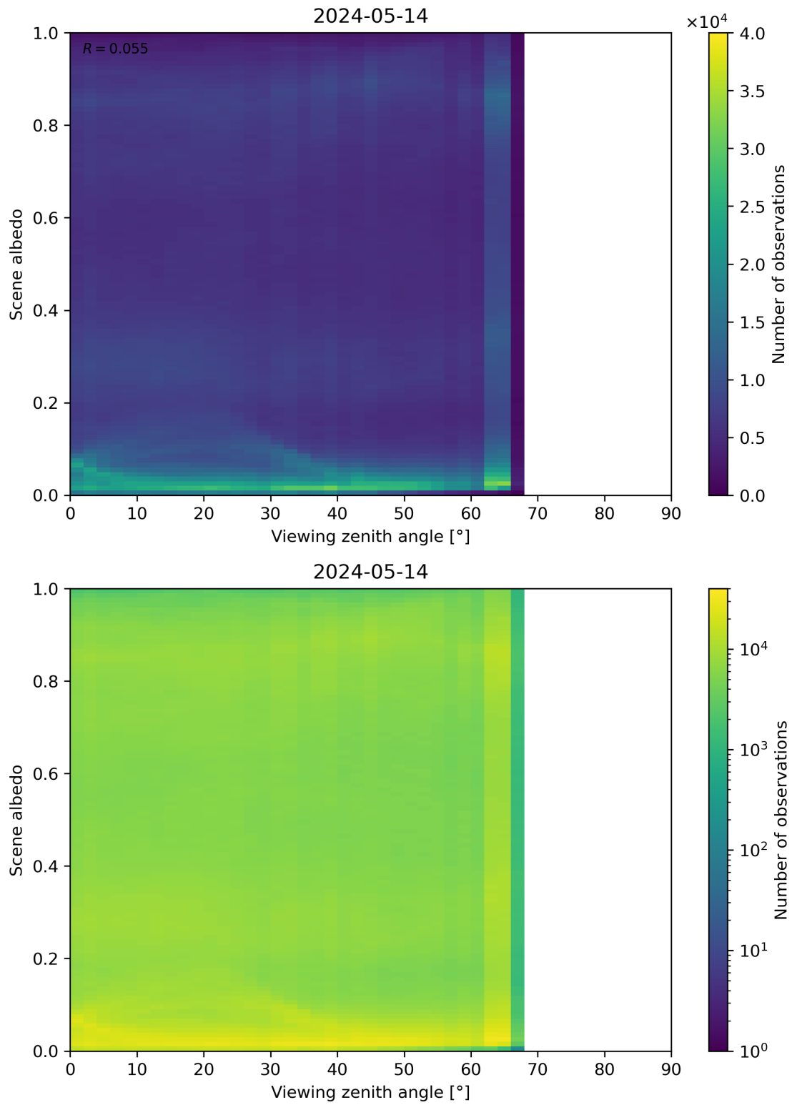
Figure 126: Scatter density plot of “Viewing zenith angle” against “Scene albedo” for 2024-05-13 to 2024-05-15.
