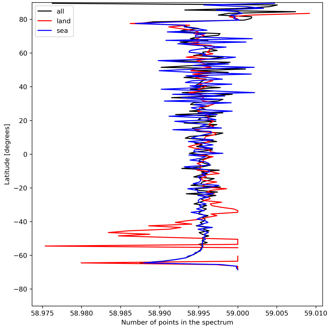
Figure 27: Zonal average of “Number of points in the spectrum” for 2024-05-13 to 2024-05-15.
