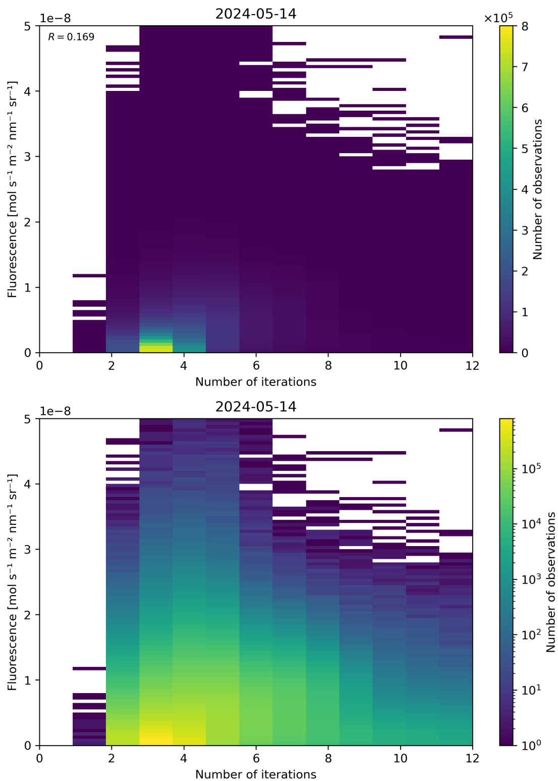
Figure 98: Scatter density plot of “Number of iterations” against “Fluorescence” for 2024-05-13 to 2024-05-15.
