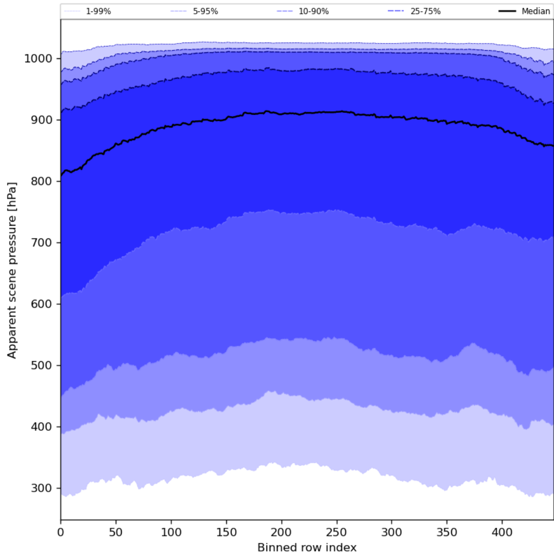
Figure 53: Along track statistics of “Apparent scene pressure” for 2024-05-13 to 2024-05-15
