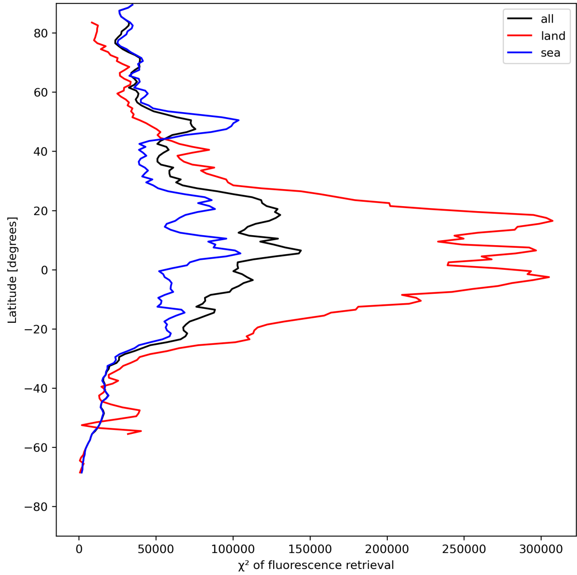
Figure 25: Zonal average of “ \chi^2 of fluorescence retrieval” for 2024-05-13 to 2024-05-15.
