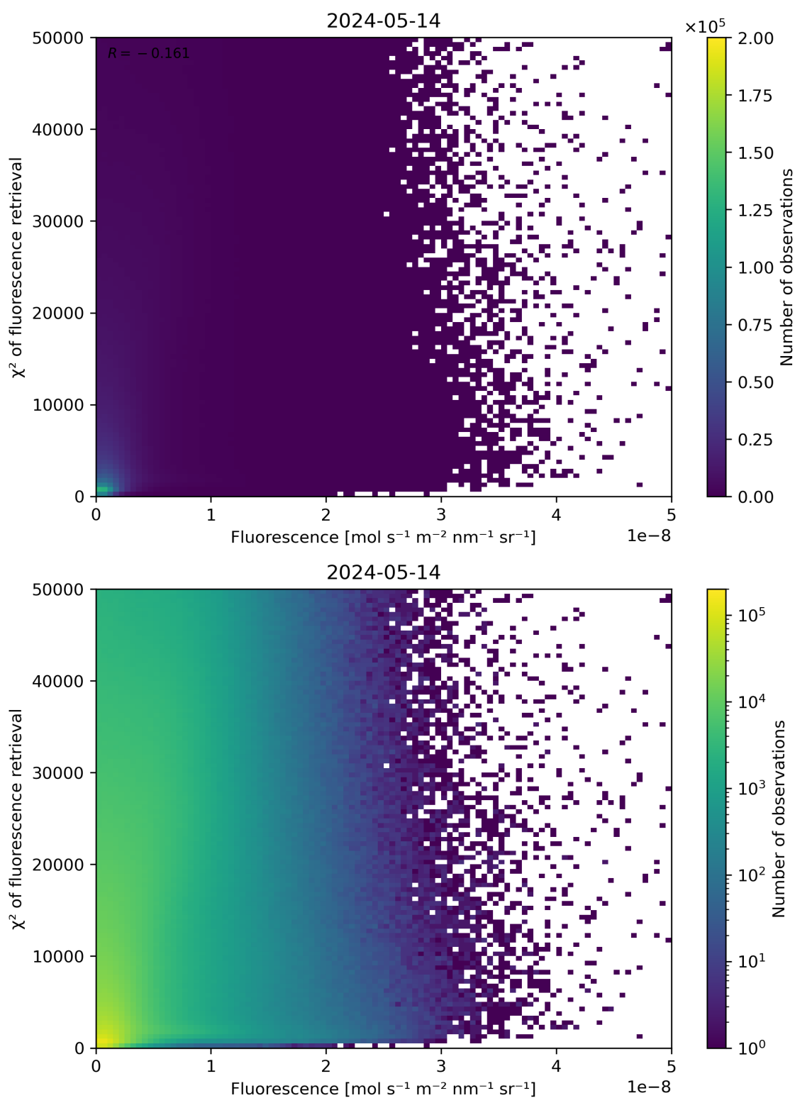
Figure 85: Scatter density plot of “Fluorescence” against “ \chi^2 of fluorescence retrieval” for 2024-05-13 to 2024-05-15.
