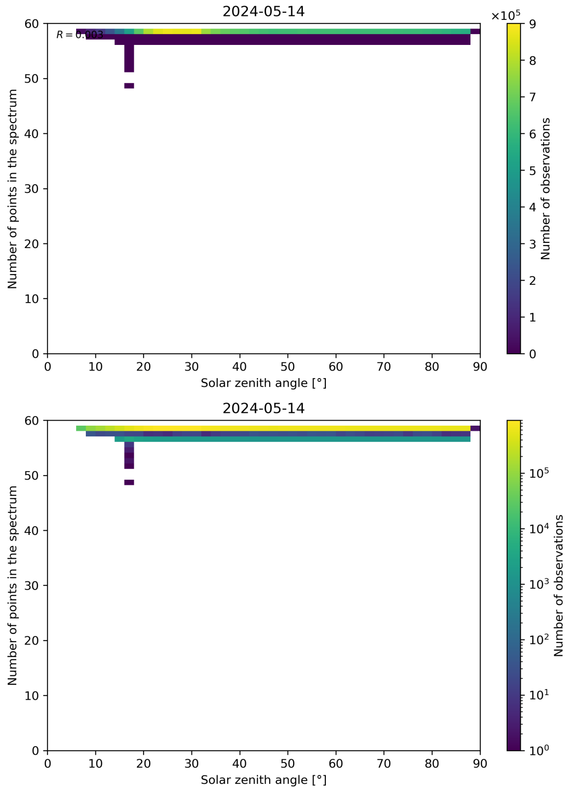
Figure 115: Scatter density plot of “Solar zenith angle” against “Number of points in the spectrum” for 2024-05-13 to 2024-05-15.
