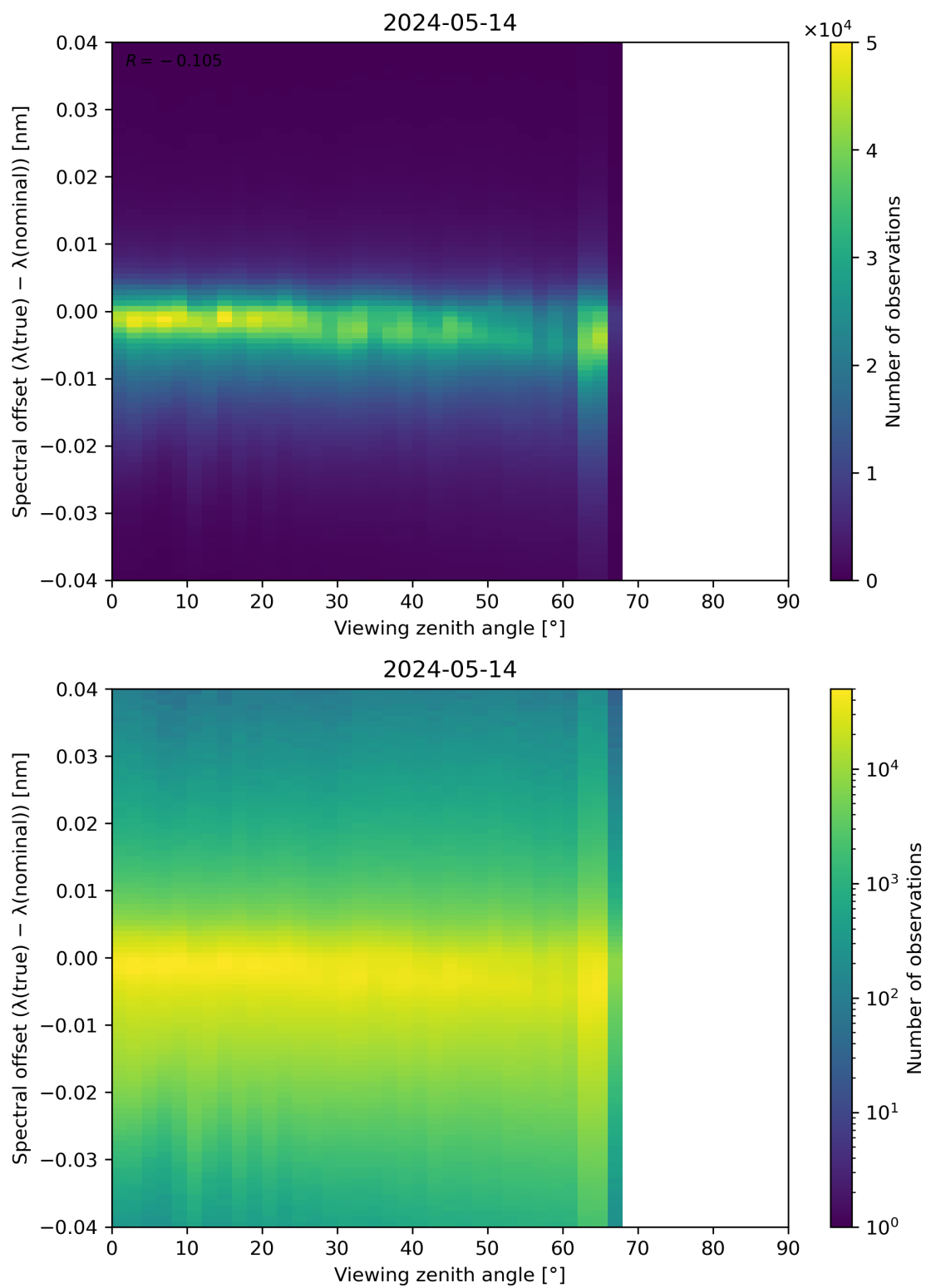
Figure 128: Scatter density plot of “Viewing zenith angle” against “Spectral offset ( \lambda(\text{true}) - \lambda(\text{nominal}) )” for 2024-05-13 to 2024-05-15.
