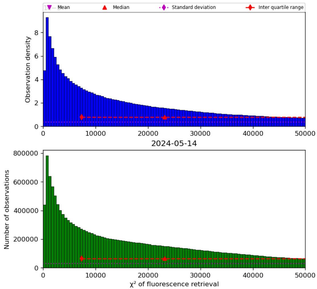
Figure 42: Histogram of “ \chi^2 of fluorescence retrieval” for 2024-05-13 to 2024-05-15
