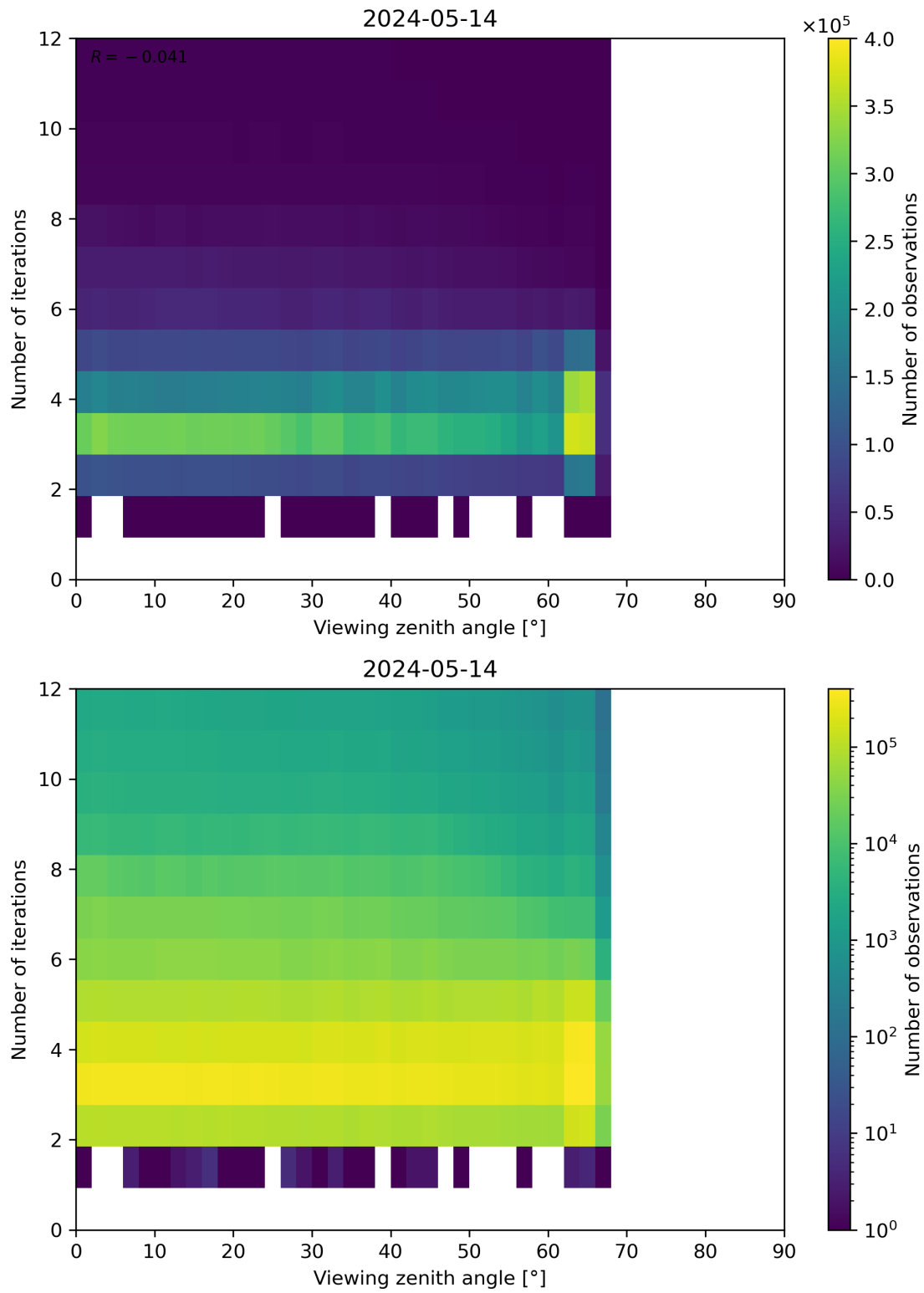
Figure 124: Scatter density plot of “Viewing zenith angle” against “Number of iterations” for 2024-05-13 to 2024-05-15.
