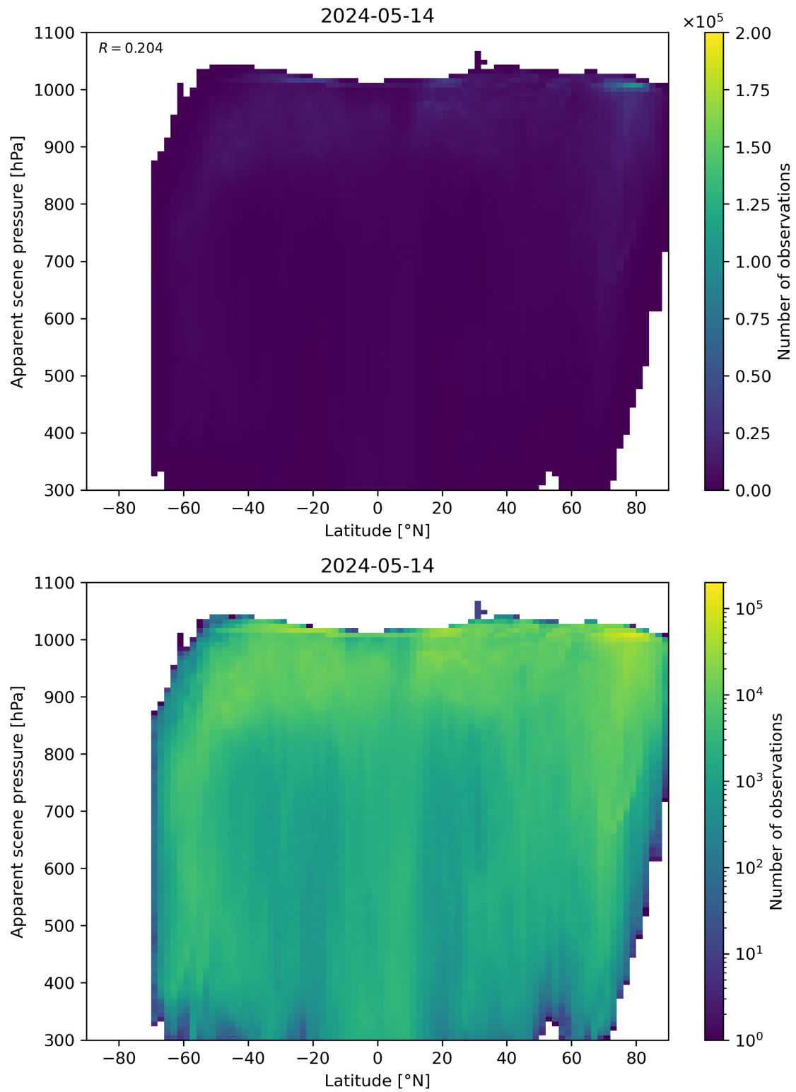
Figure 88: Scatter density plot of “Latitude” against “Apparent scene pressure” for 2024-05-13 to 2024-05-15.
