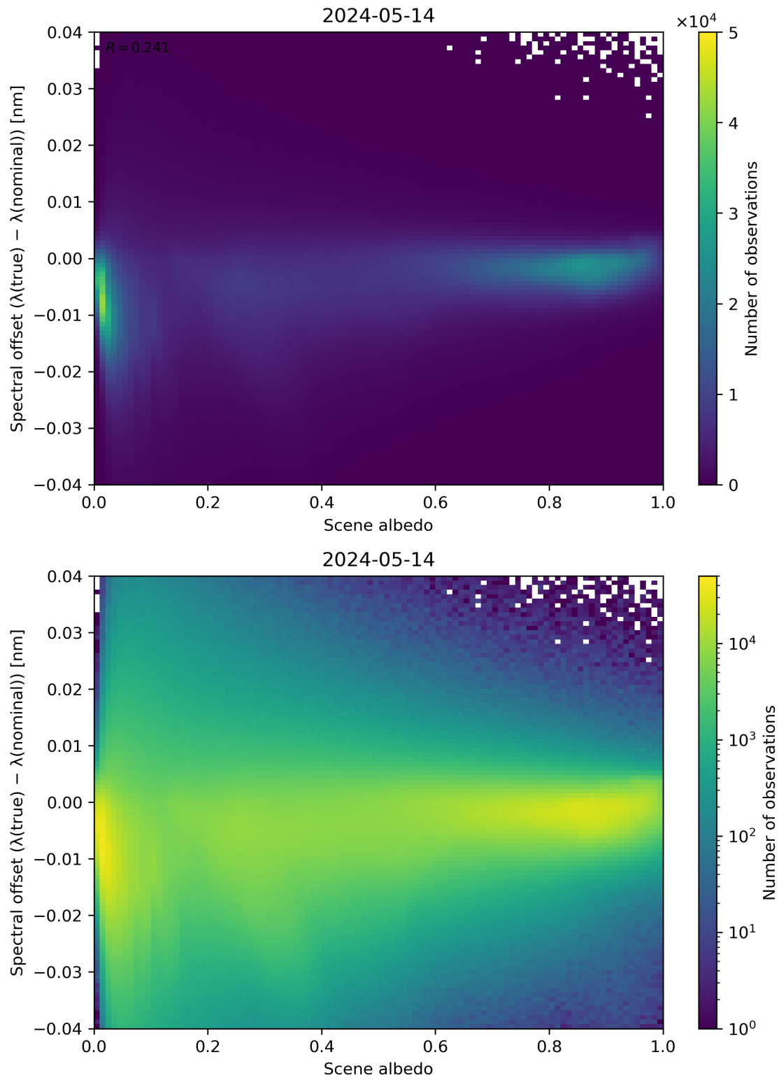
Figure 107: Scatter density plot of “Scene albedo” against “Spectral offset ( \lambda(\text{true}) - \lambda(\text{nominal}) )” for 2024-05-13 to 2024-05-15.
