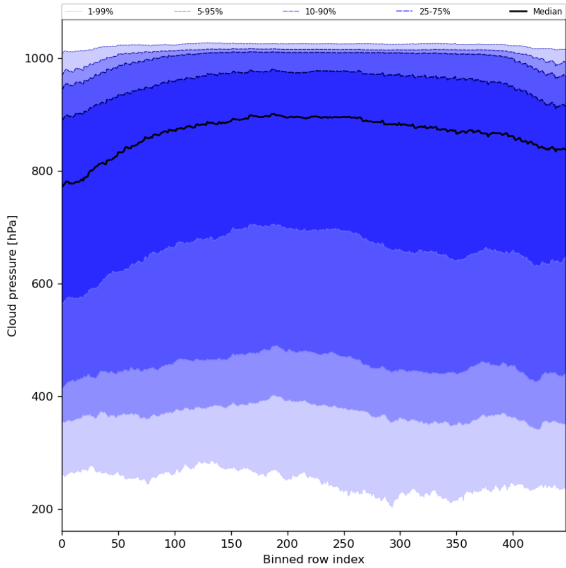
Figure 47: Along track statistics of “Cloud pressure” for 2024-05-13 to 2024-05-15
