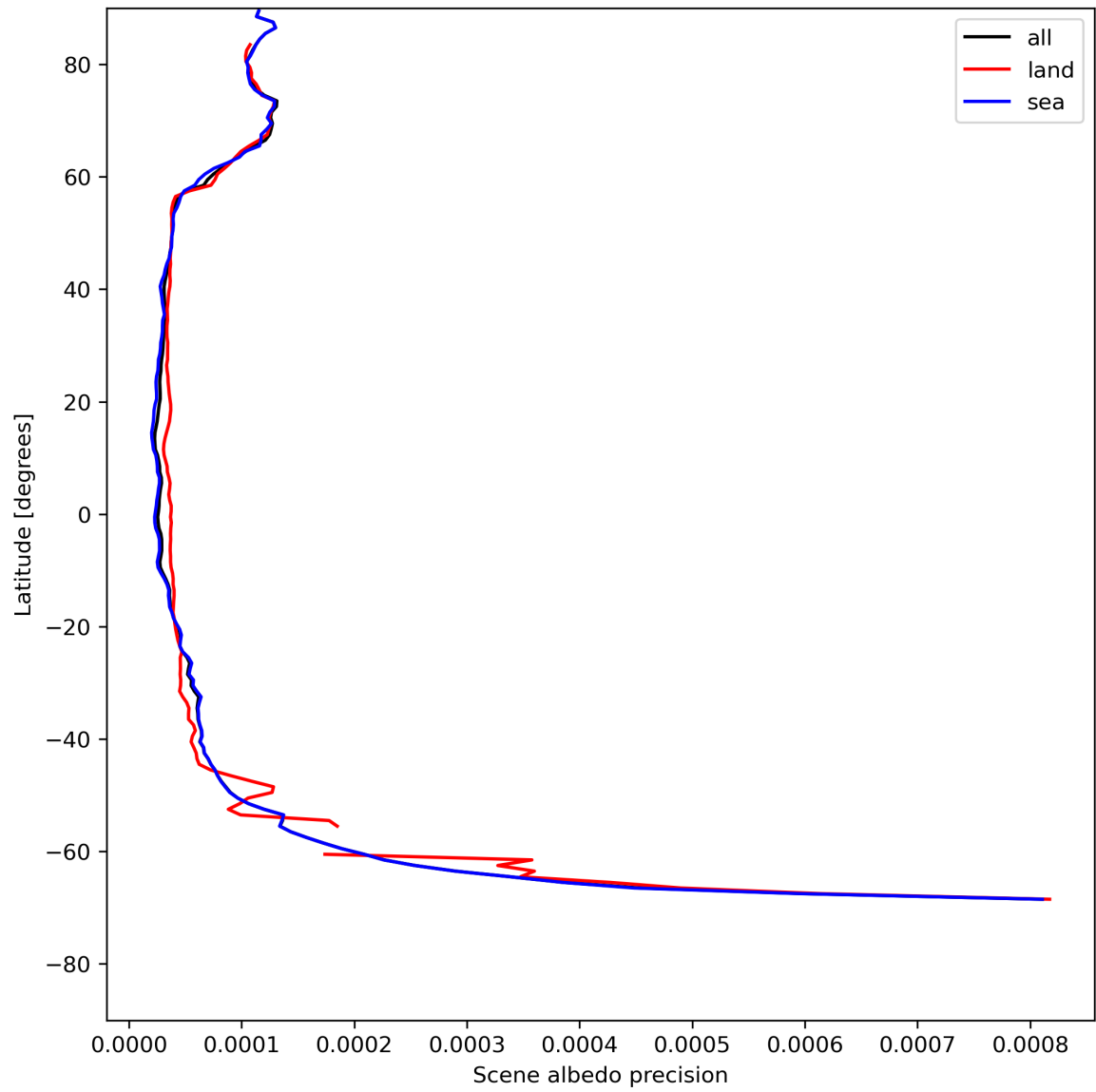
Figure 18: Zonal average of “Scene albedo precision” for 2024-05-13 to 2024-05-15.
