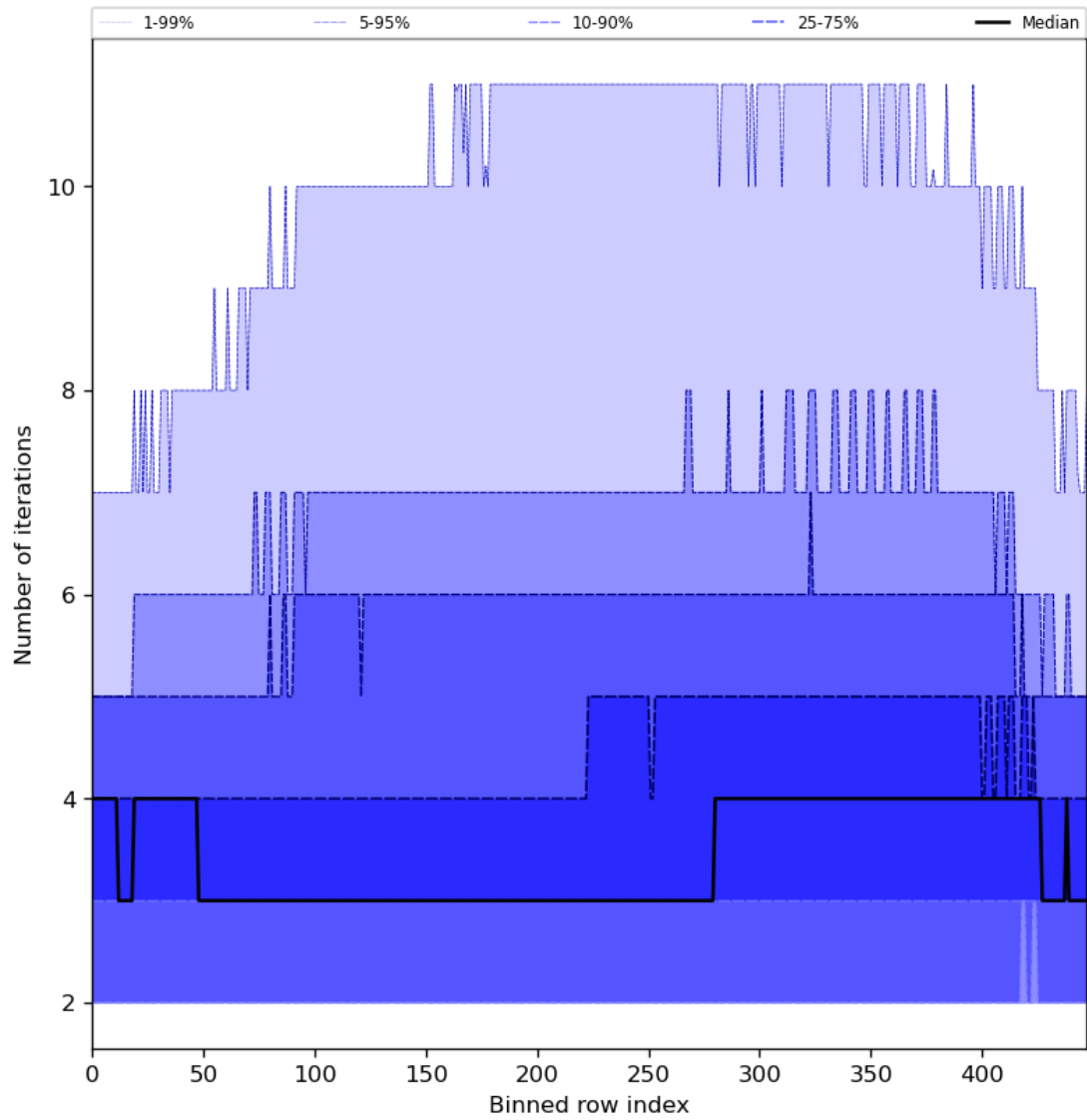
Figure 56: Along track statistics of “Number of iterations” for 2024-05-13 to 2024-05-15
