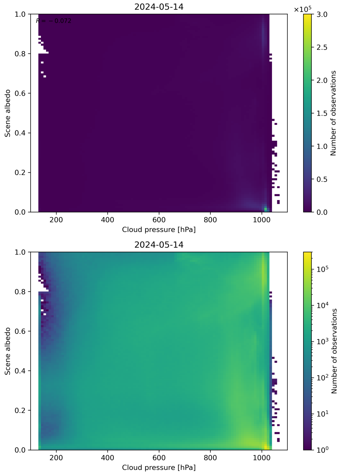
Figure 83: Scatter density plot of “Cloud pressure” against “Scene albedo” for 2024-05-13 to 2024-05-15.
