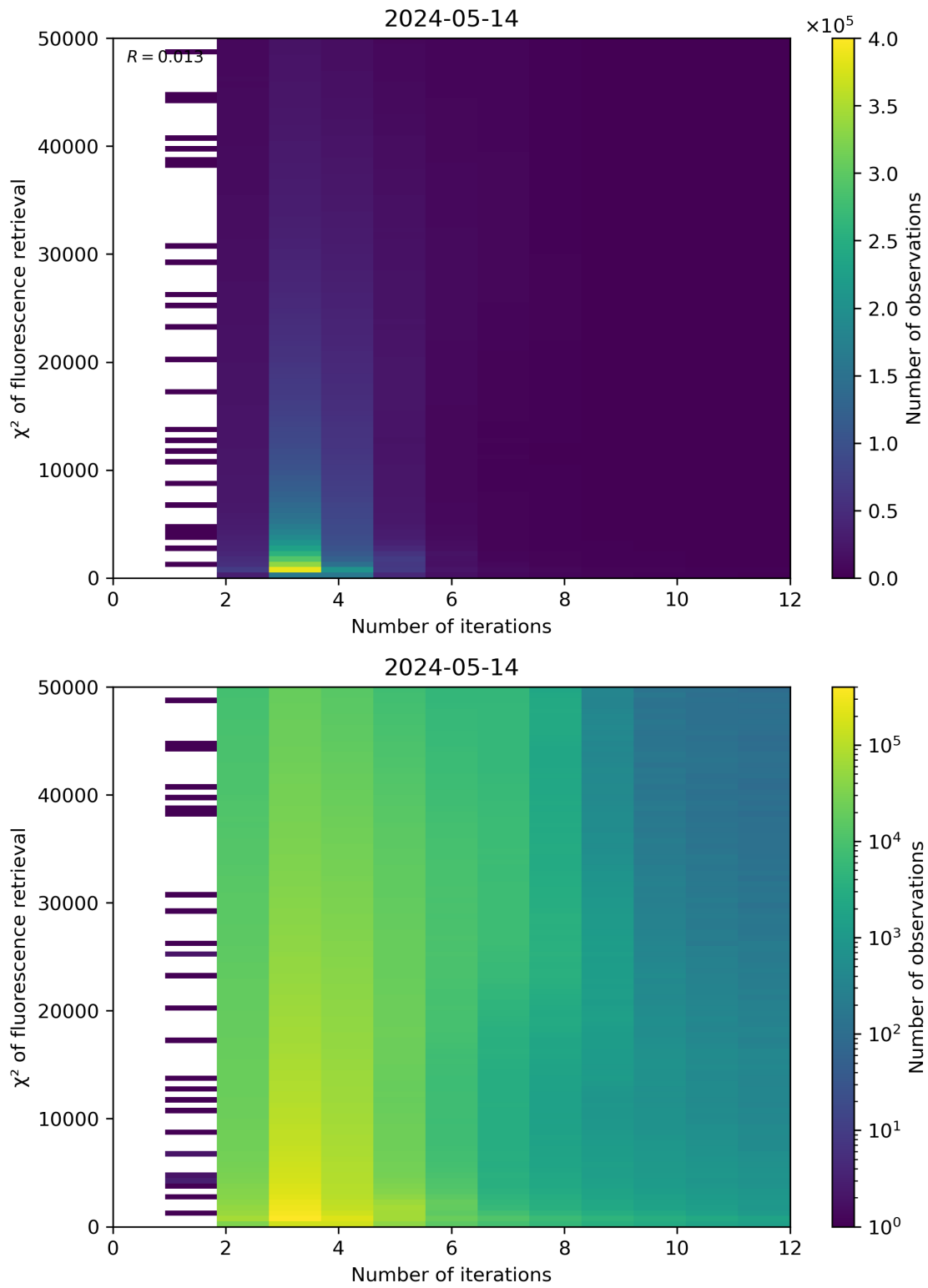
Figure 97: Scatter density plot of “Number of iterations” against “ \chi^2 of fluorescence retrieval” for 2024-05-13 to 2024-05-15.
