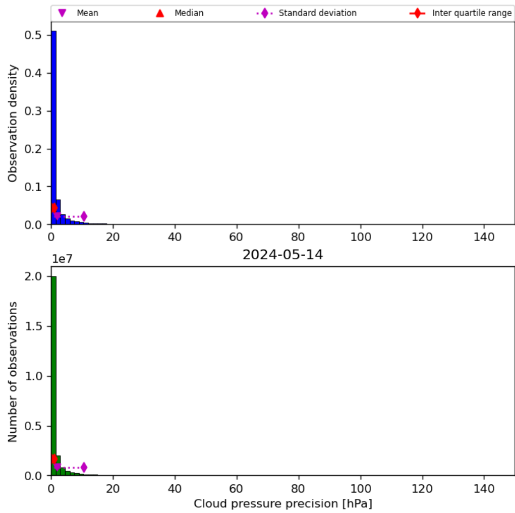
Figure 31: Histogram of “Cloud pressure precision” for 2024-05-13 to 2024-05-15
