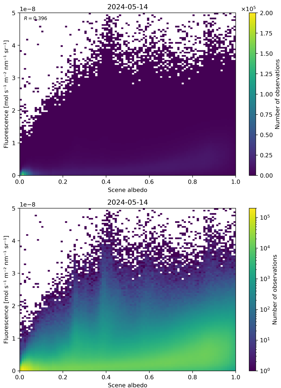
Figure 104: Scatter density plot of “Scene albedo” against “Fluorescence” for 2024-05-13 to 2024-05-15.
