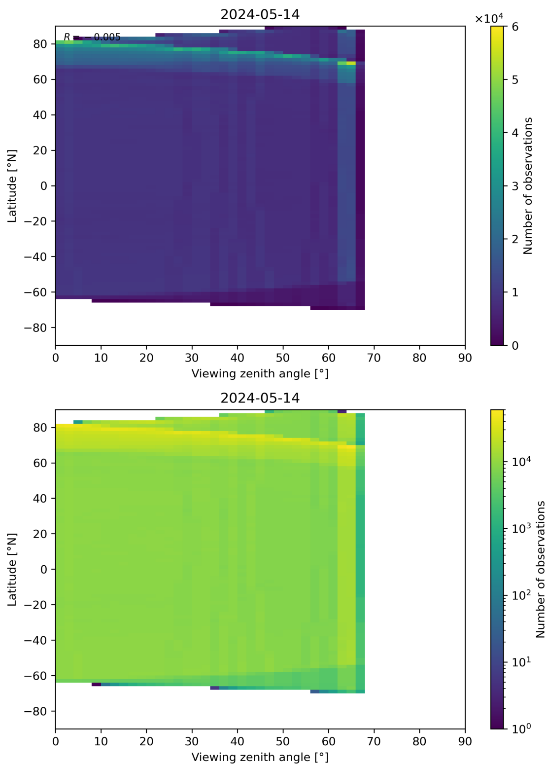
Figure 123: Scatter density plot of “Viewing zenith angle” against “Latitude” for 2024-05-13 to 2024-05-15.
