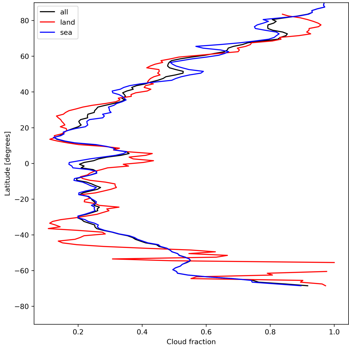
Figure 15: Zonal average of “Cloud fraction” for 2024-05-13 to 2024-05-15.
