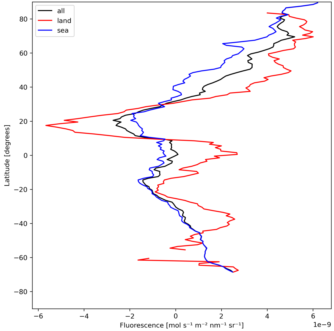
Figure 23: Zonal average of “Fluorescence” for 2024-05-13 to 2024-05-15.
