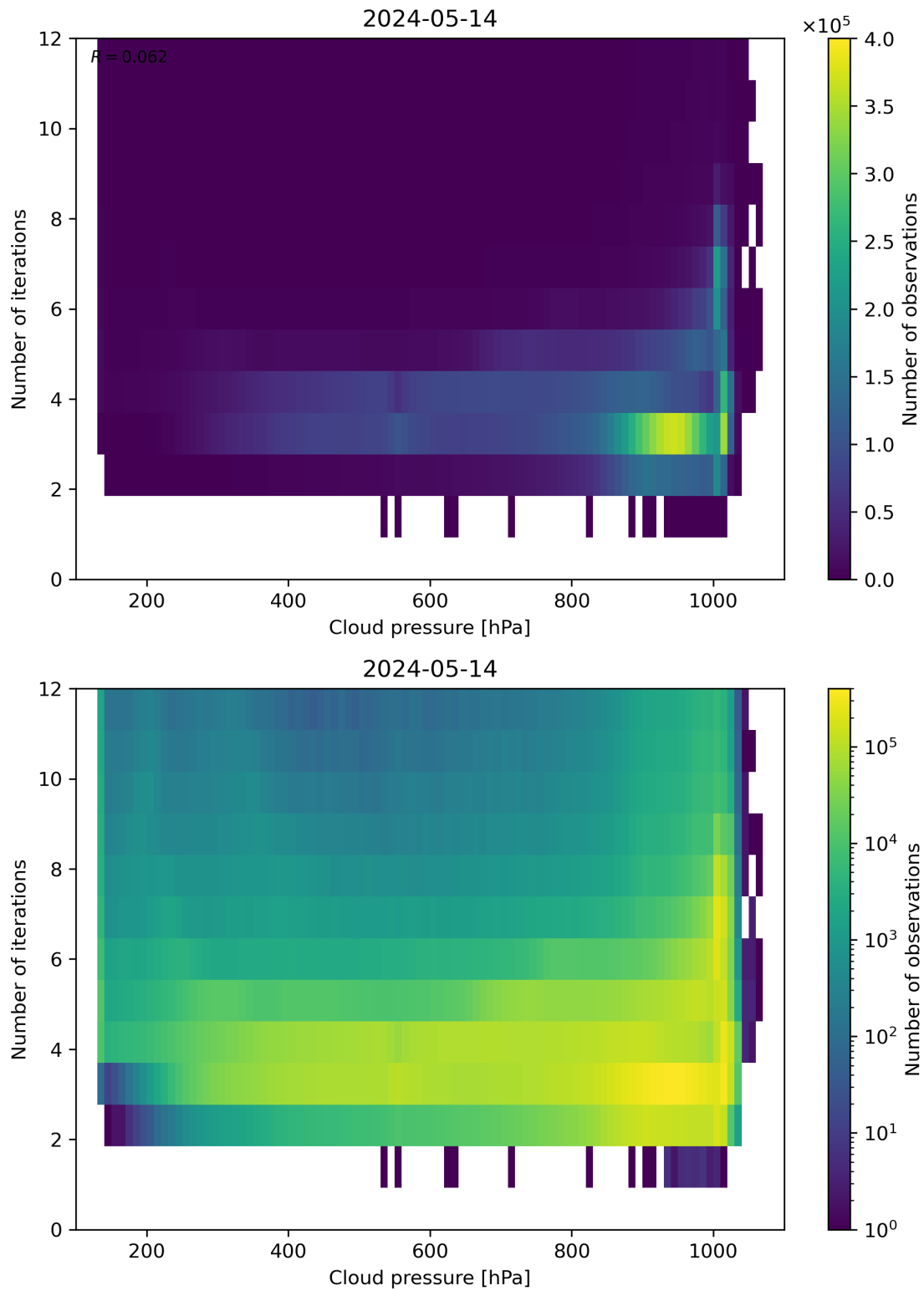
Figure 81: Scatter density plot of “Cloud pressure” against “Number of iterations” for 2024-05-13 to 2024-05-15.
