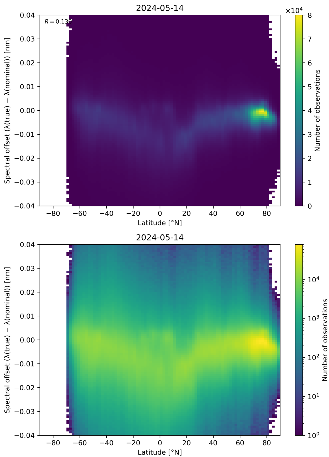
Figure 96: Scatter density plot of “Latitude” against “Spectral offset ( \lambda(\text{true}) - \lambda(\text{nominal}) )” for 2024-05-13 to 2024-05-15.
