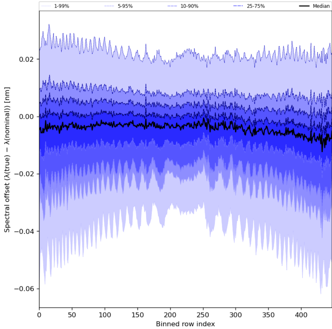
Figure 62: Along track statistics of “Spectral offset ( \lambda(\text{true}) - \lambda(\text{nominal}) )” for 2024-05-13 to 2024-05-15
