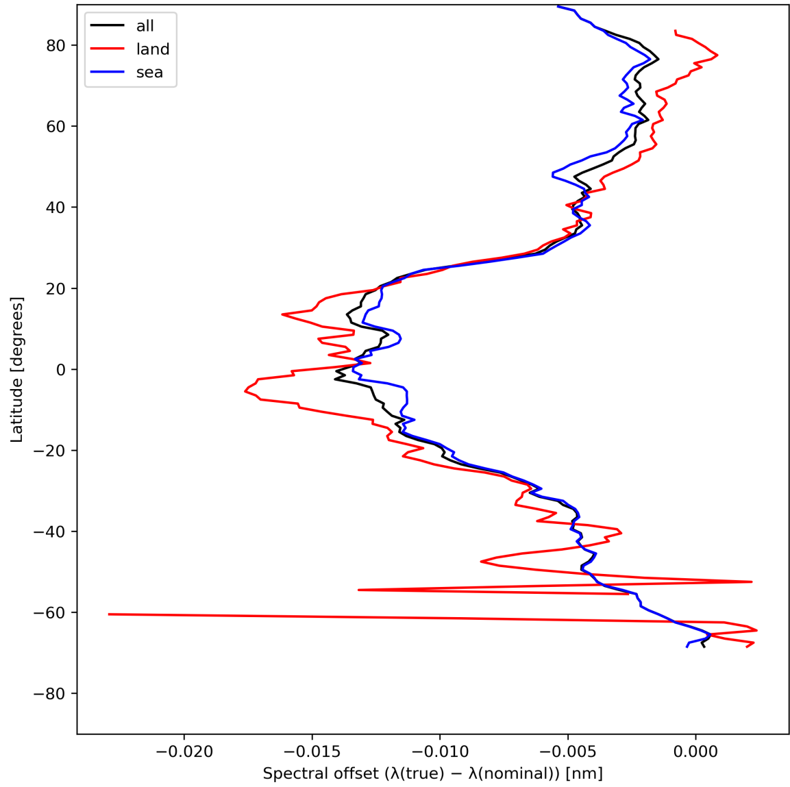
Figure 28: Zonal average of “Spectral offset ( \lambda(\text{true}) - \lambda(\text{nominal}) )” for 2024-05-13 to 2024-05-15.
