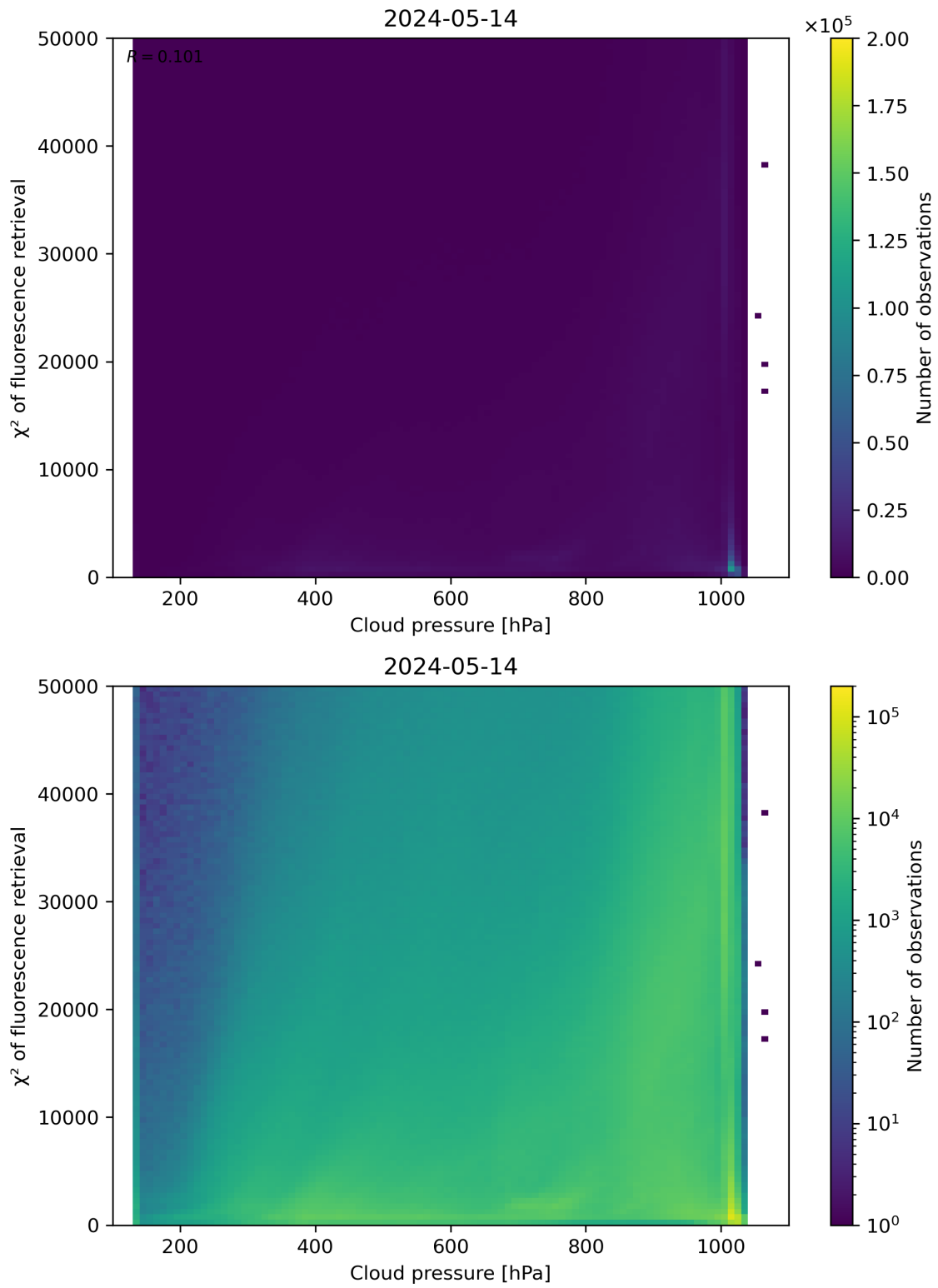
Figure 78: Scatter density plot of “Cloud pressure” against “ \chi^2 of fluorescence retrieval” for 2024-05-13 to 2024-05-15.
