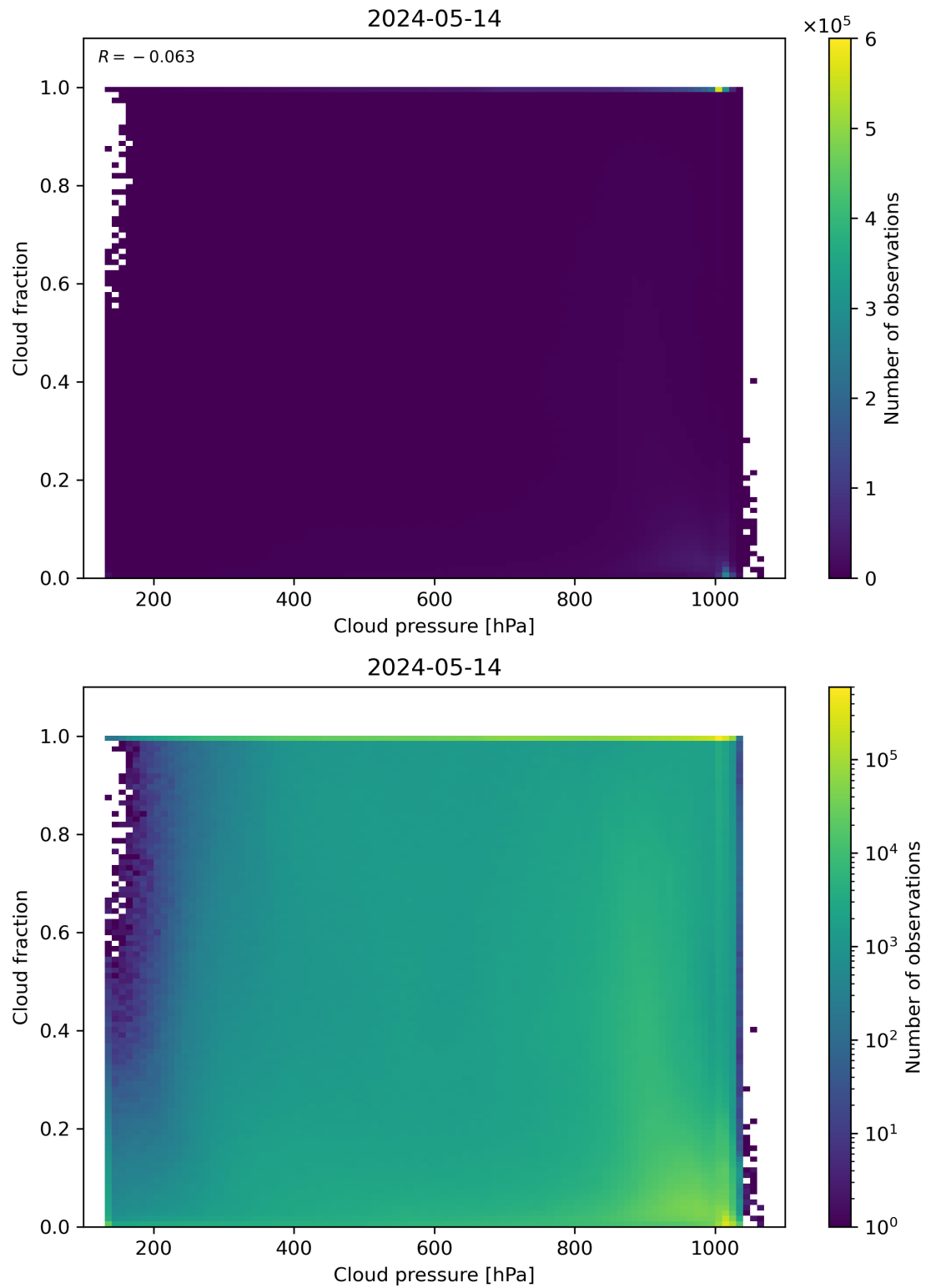
Figure 79: Scatter density plot of “Cloud pressure” against “Cloud fraction” for 2024-05-13 to 2024-05-15.
