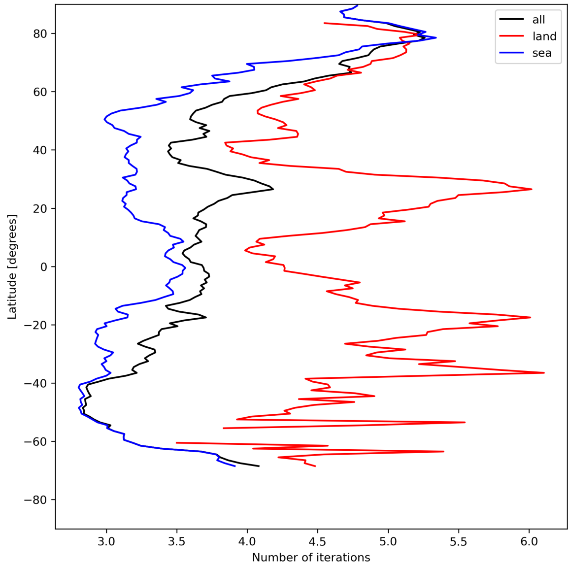
Figure 22: Zonal average of “Number of iterations” for 2024-05-13 to 2024-05-15.
