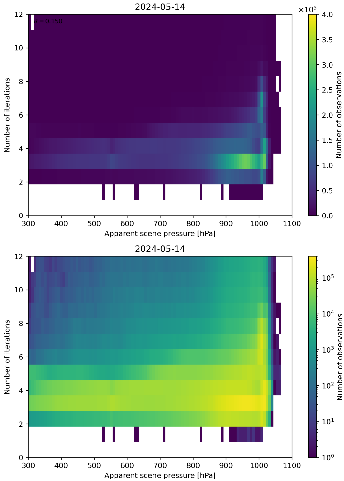
Figure 65: Scatter density plot of “Apparent scene pressure” against “Number of iterations” for 2024-05-13 to 2024-05-15.
