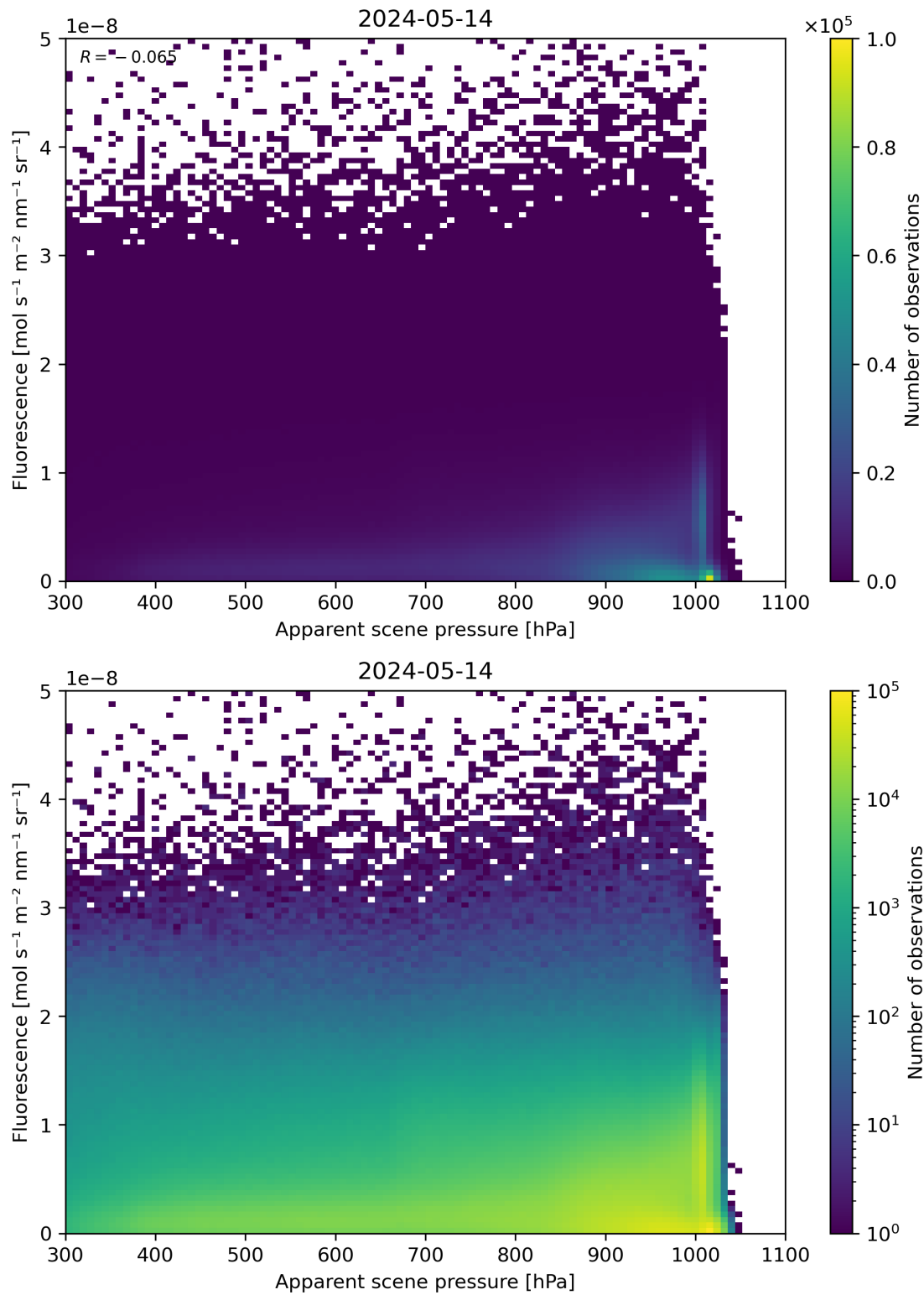
Figure 64: Scatter density plot of “Apparent scene pressure” against “Fluorescence” for 2024-05-13 to 2024-05-15.
