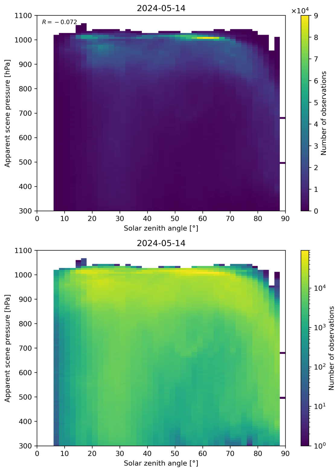
Figure 108: Scatter density plot of “Solar zenith angle” against “Apparent scene pressure” for 2024-05-13 to 2024-05-15.
