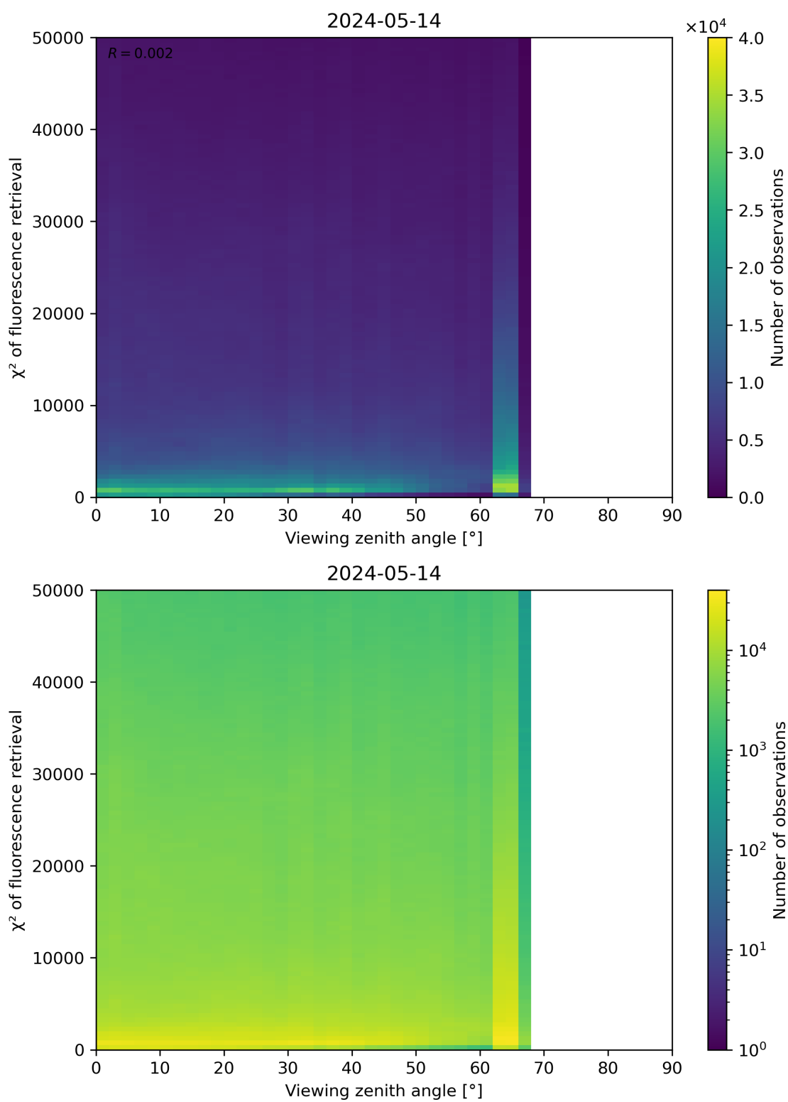
Figure 119: Scatter density plot of “Viewing zenith angle” against “ \chi^2 of fluorescence retrieval” for 2024-05-13 to 2024-05-15.
