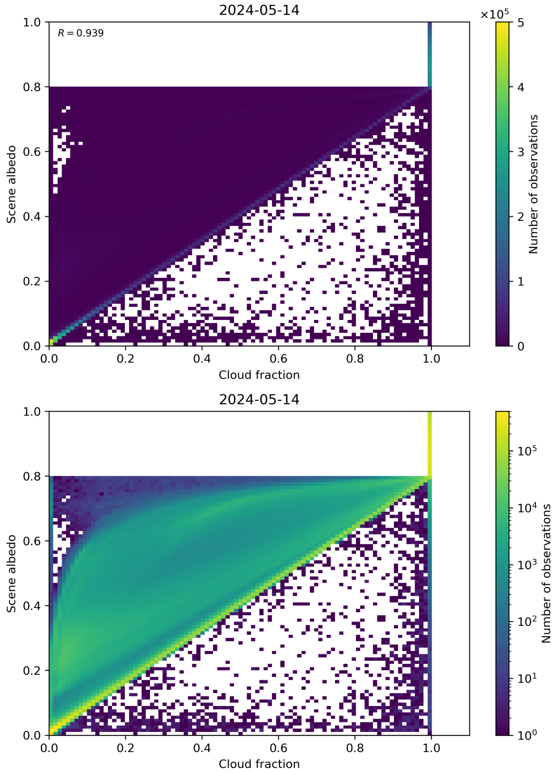
Figure 75: Scatter density plot of “Cloud fraction” against “Scene albedo” for 2024-05-13 to 2024-05-15.
