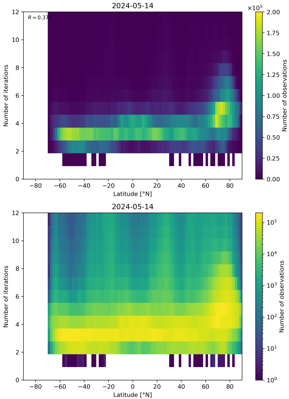
Figure 93: Scatter density plot of “Latitude” against “Number of iterations” for 2024-05-13 to 2024-05-15.
