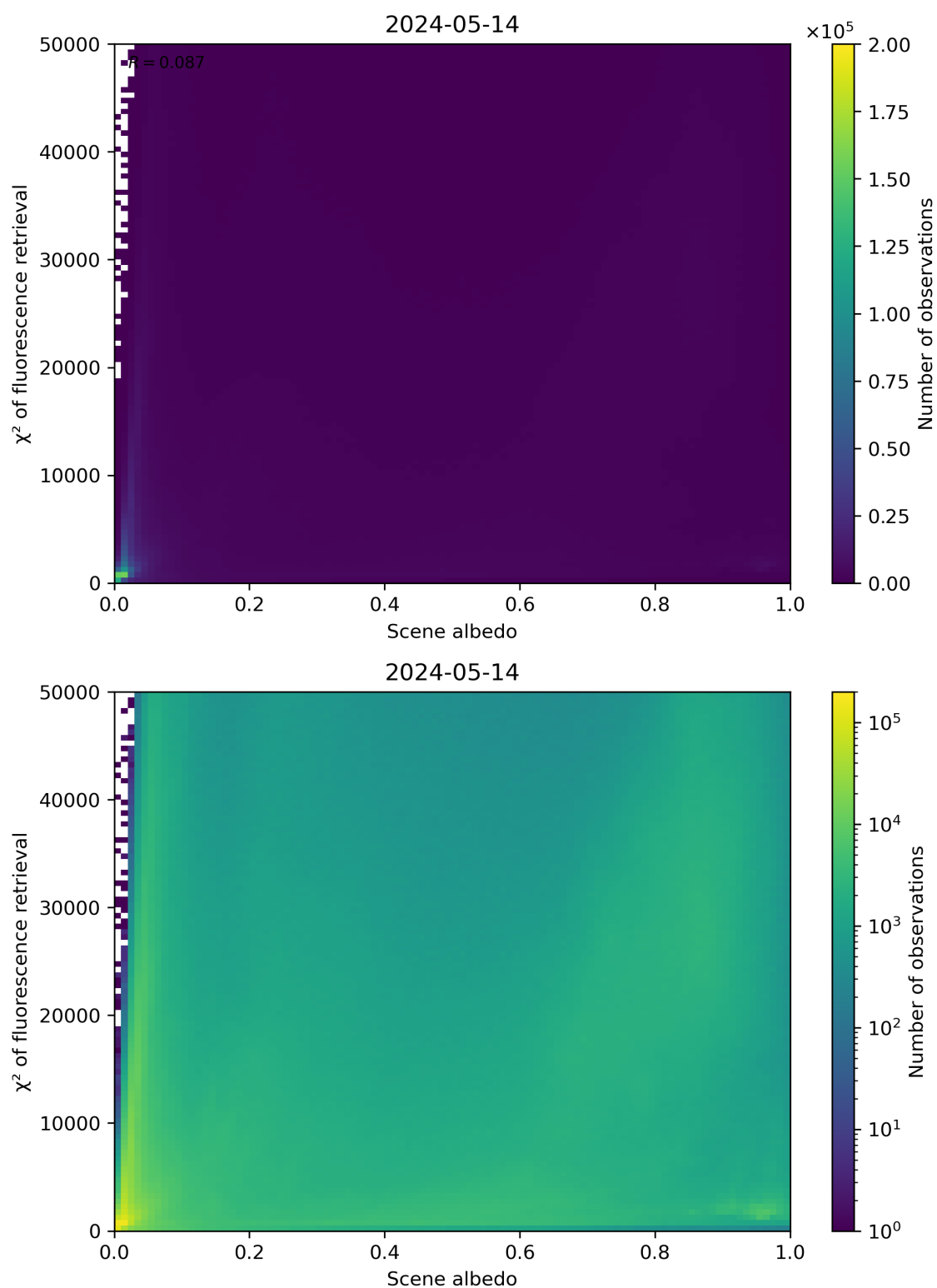
Figure 103: Scatter density plot of “Scene albedo” against “ \chi^2 of fluorescence retrieval” for 2024-05-13 to 2024-05-15.
