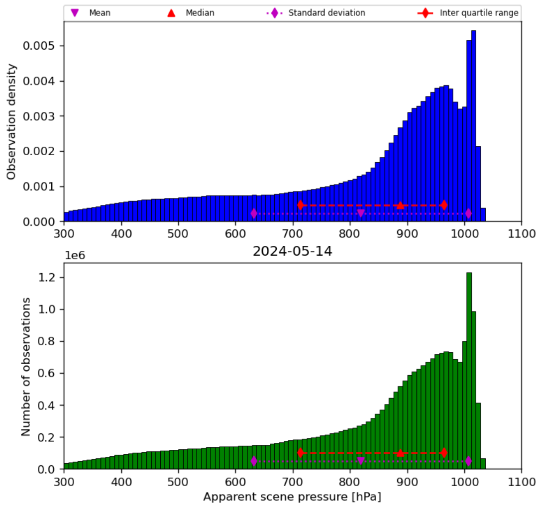
Figure 36: Histogram of “Apparent scene pressure” for 2024-05-13 to 2024-05-15
