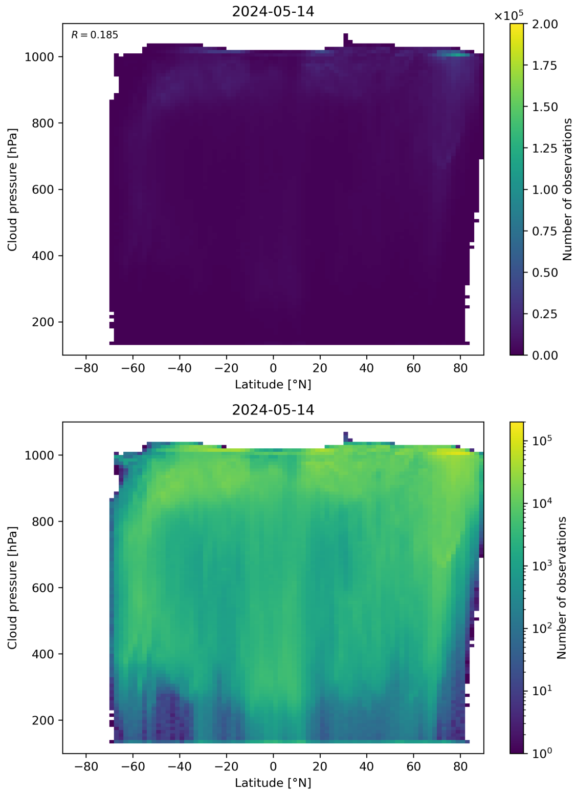
Figure 91: Scatter density plot of “Latitude” against “Cloud pressure” for 2024-05-13 to 2024-05-15.
