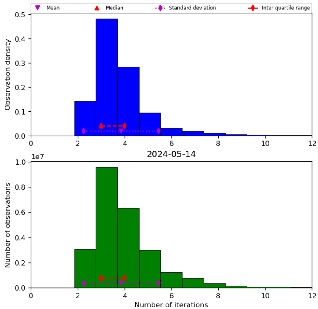
Figure 39: Histogram of “Number of iterations” for 2024-05-13 to 2024-05-15
