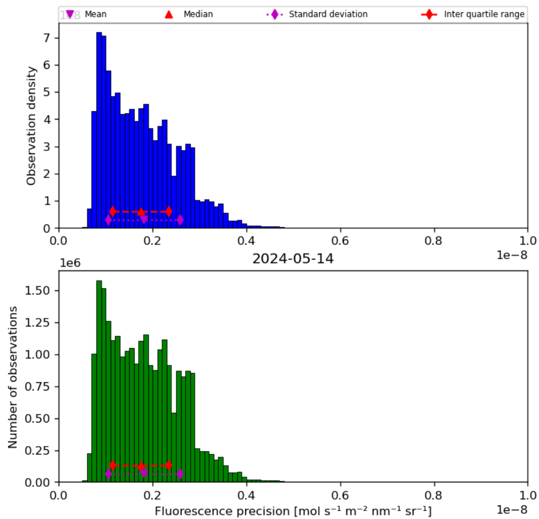
Figure 41: Histogram of “Fluorescence precision” for 2024-05-13 to 2024-05-15
