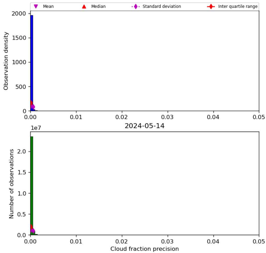
Figure 33: Histogram of “Cloud fraction precision” for 2024-05-13 to 2024-05-15
