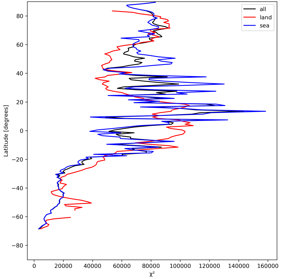
Figure 21: Zonal average of “ \chi^2 ” for 2024-05-13 to 2024-05-15.
