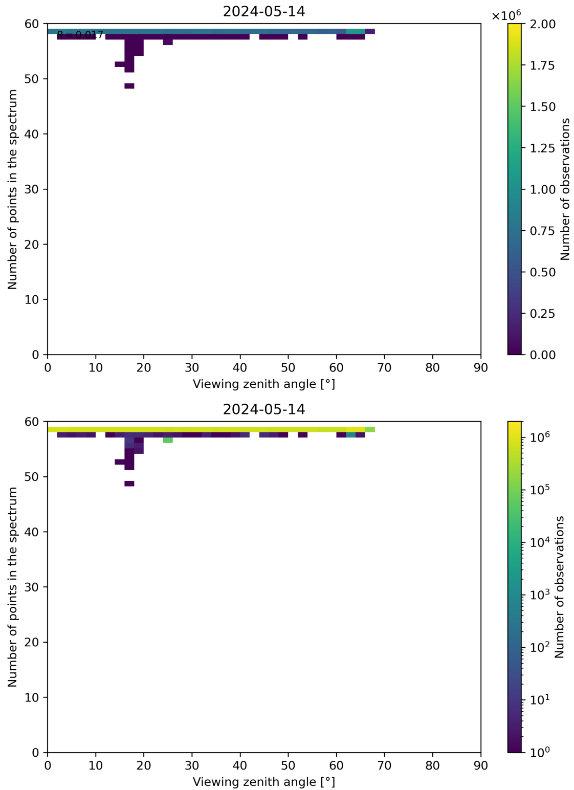
Figure 125: Scatter density plot of “Viewing zenith angle” against “Number of points in the spectrum” for 2024-05-13 to 2024-05-15.
