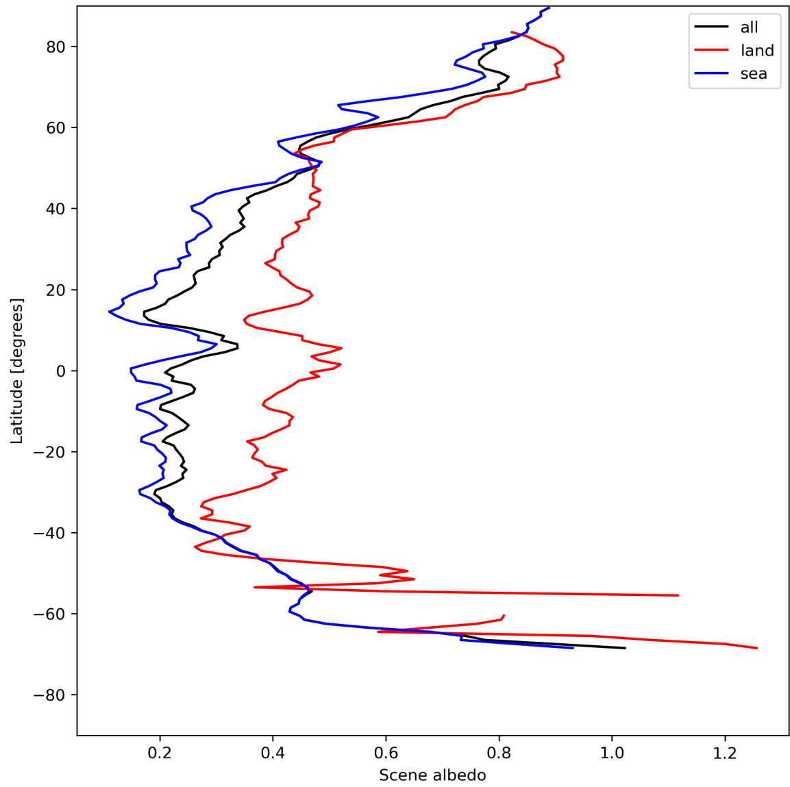
Figure 17: Zonal average of “Scene albedo” for 2024-05-13 to 2024-05-15.
