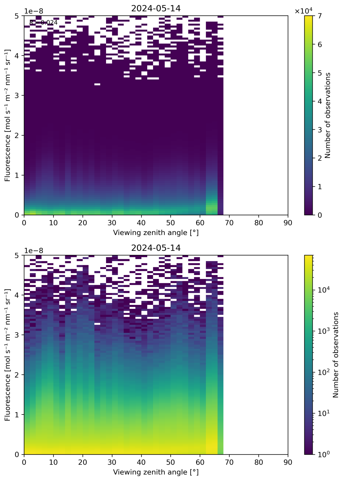
Figure 122: Scatter density plot of “Viewing zenith angle” against “Fluorescence” for 2024-05-13 to 2024-05-15.
