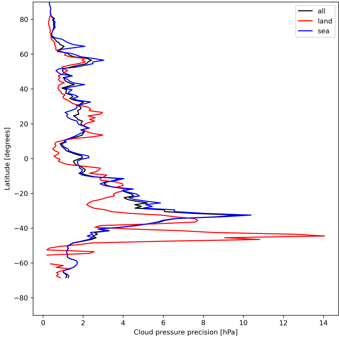
Figure 14: Zonal average of “Cloud pressure precision” for 2024-05-13 to 2024-05-15.
