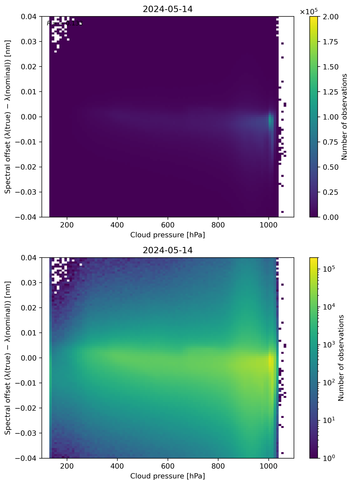
Figure 84: Scatter density plot of “Cloud pressure” against “Spectral offset ( \lambda(\text{true}) - \lambda(\text{nominal}) )” for 2024-05-13 to 2024-05-15.
