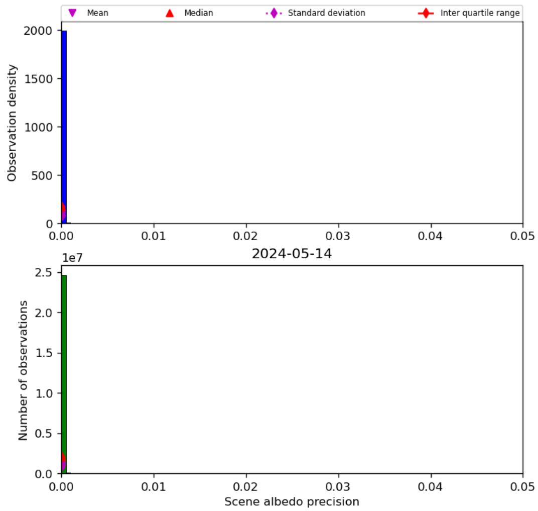
Figure 35: Histogram of “Scene albedo precision” for 2024-05-13 to 2024-05-15
