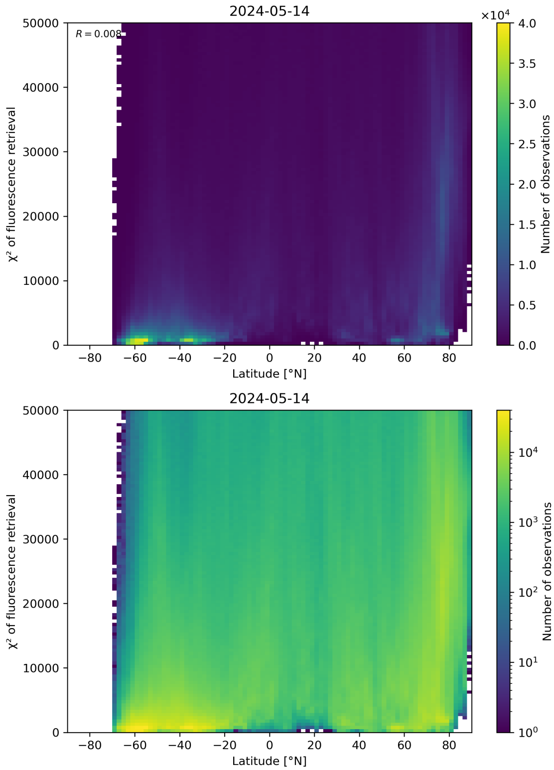
Figure 89: Scatter density plot of “Latitude” against “ \chi^2 of fluorescence retrieval” for 2024-05-13 to 2024-05-15.
