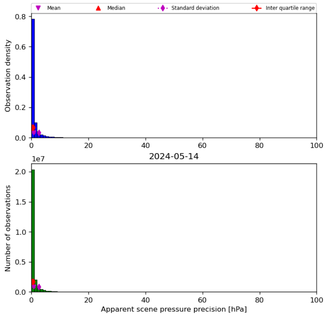
Figure 37: Histogram of “Apparent scene pressure precision” for 2024-05-13 to 2024-05-15
