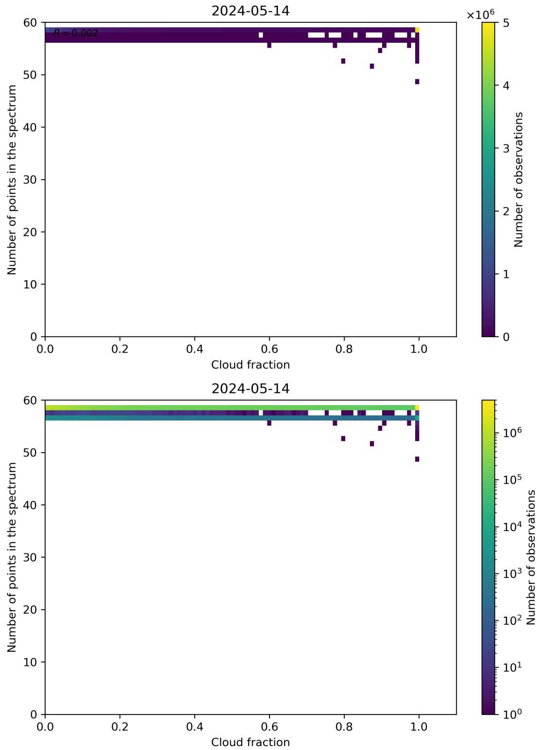
Figure 74: Scatter density plot of “Cloud fraction” against “Number of points in the spectrum” for 2024-05-13 to 2024-05-15.
