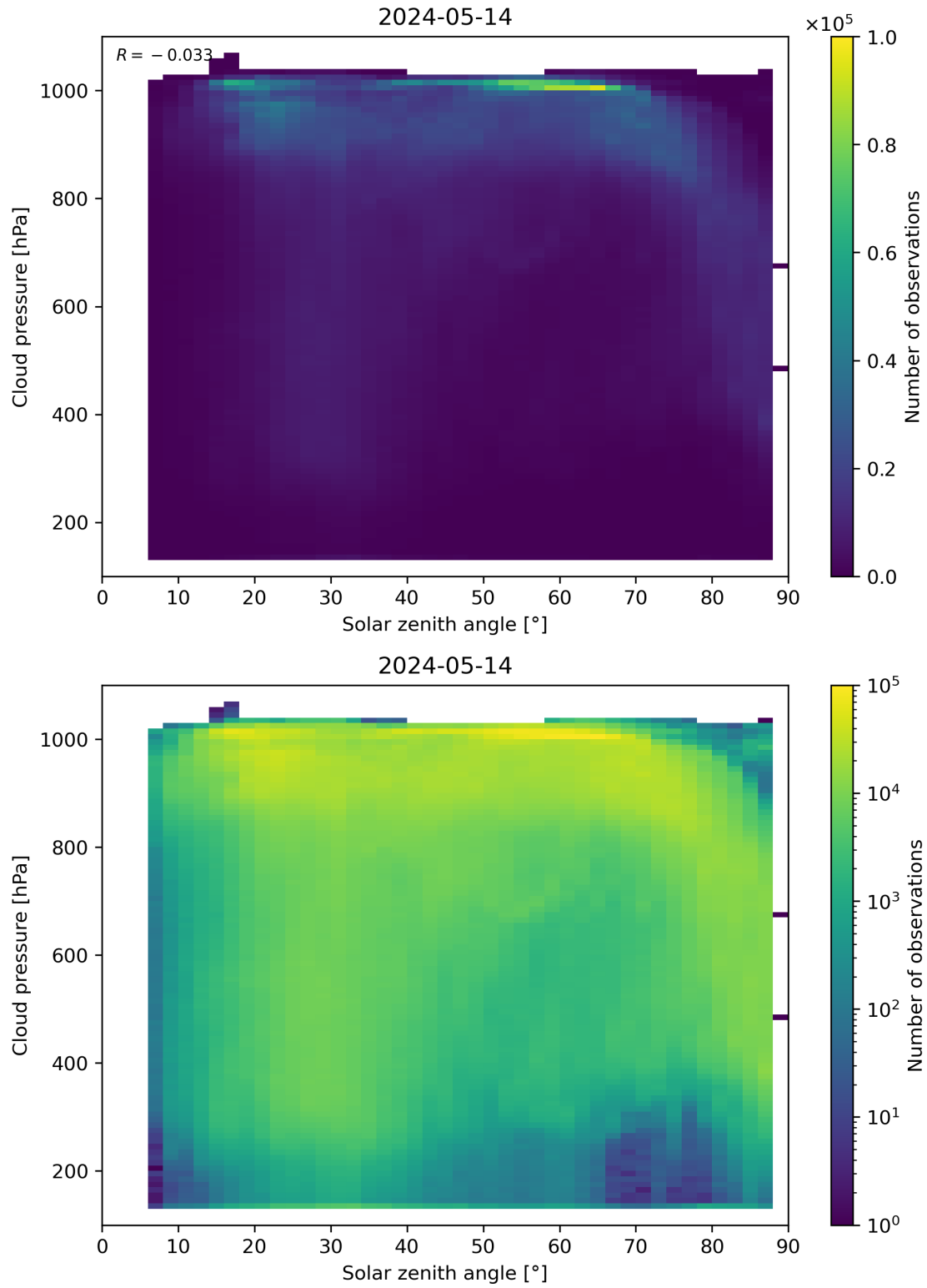
Figure 111: Scatter density plot of “Solar zenith angle” against “Cloud pressure” for 2024-05-13 to 2024-05-15.
