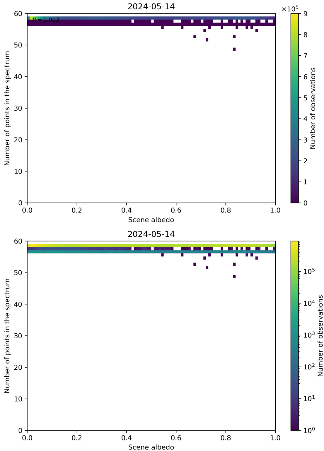
Figure 106: Scatter density plot of “Scene albedo” against “Number of points in the spectrum” for 2024-05-13 to 2024-05-15.
