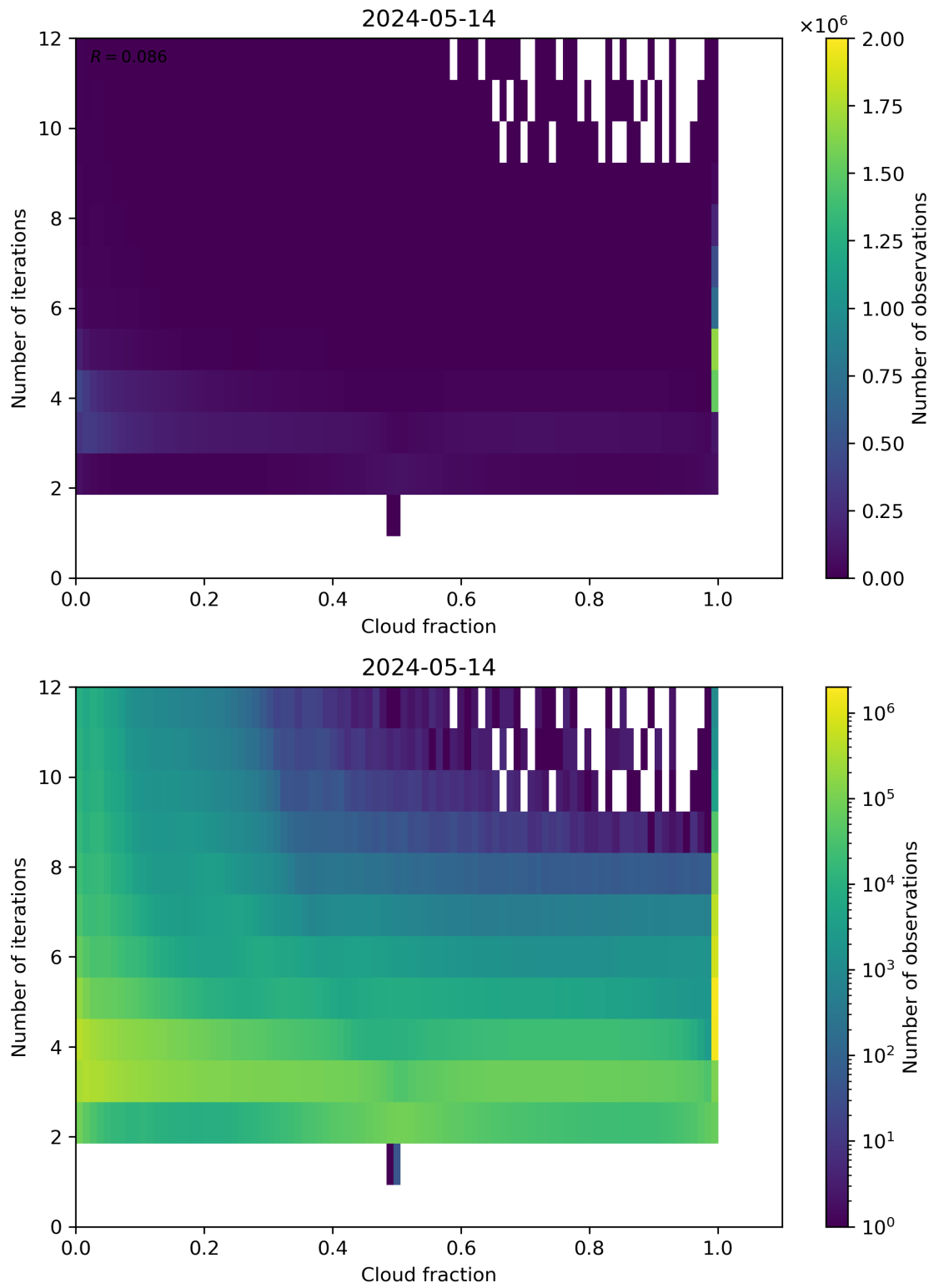
Figure 73: Scatter density plot of “Cloud fraction” against “Number of iterations” for 2024-05-13 to 2024-05-15.
