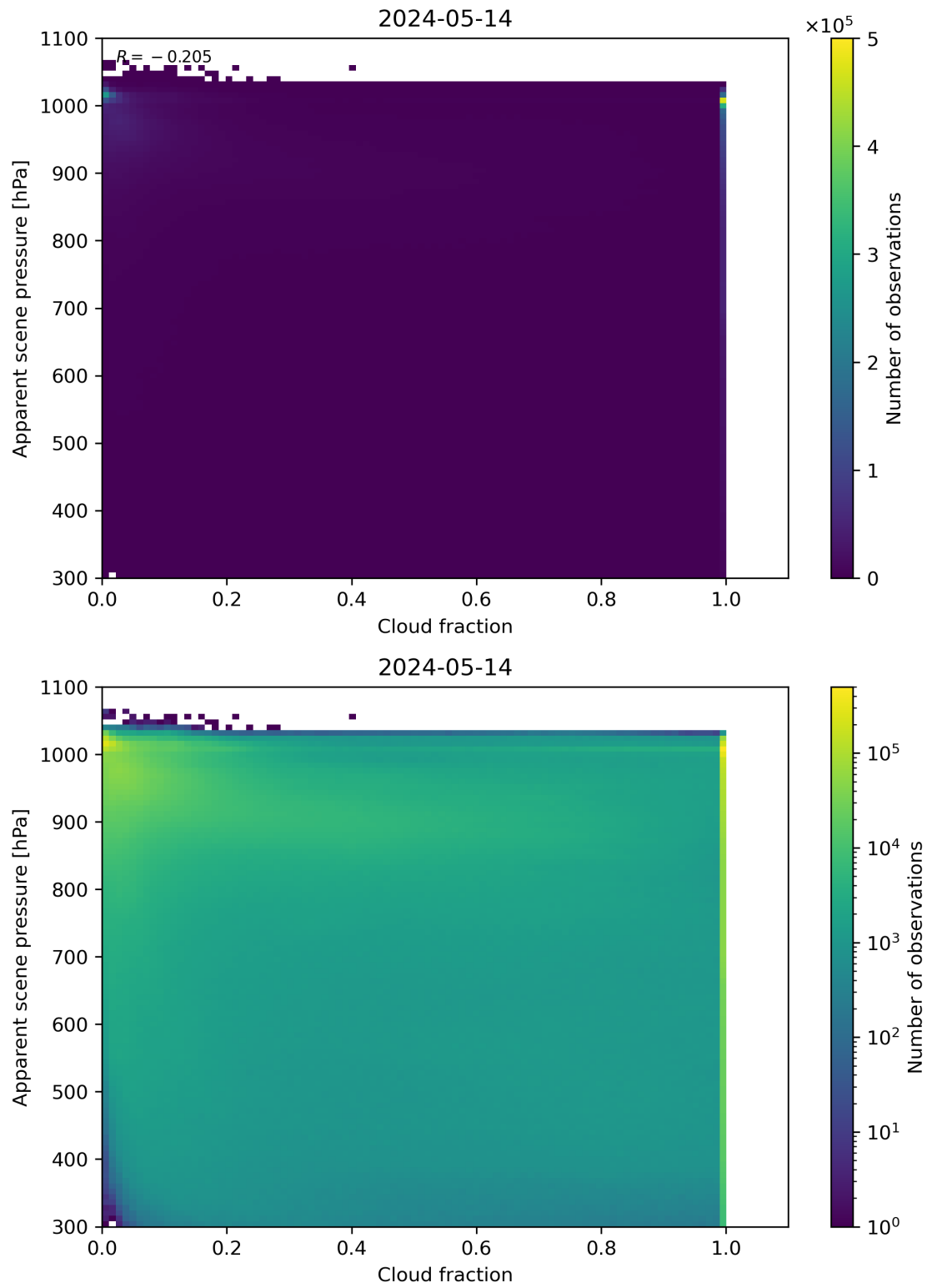
Figure 70: Scatter density plot of “Cloud fraction” against “Apparent scene pressure” for 2024-05-13 to 2024-05-15.
