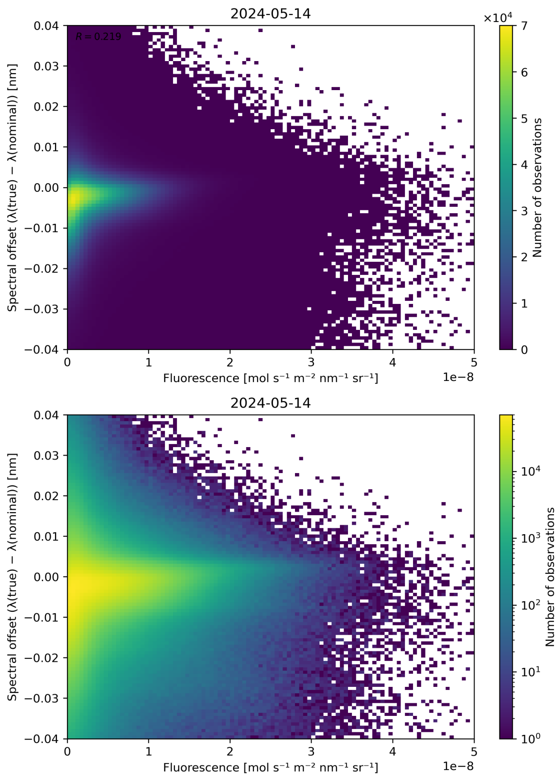
Figure 87: Scatter density plot of “Fluorescence” against “Spectral offset ( \lambda(\text{true}) - \lambda(\text{nominal}) )” for 2024-05-13 to 2024-05-15.
