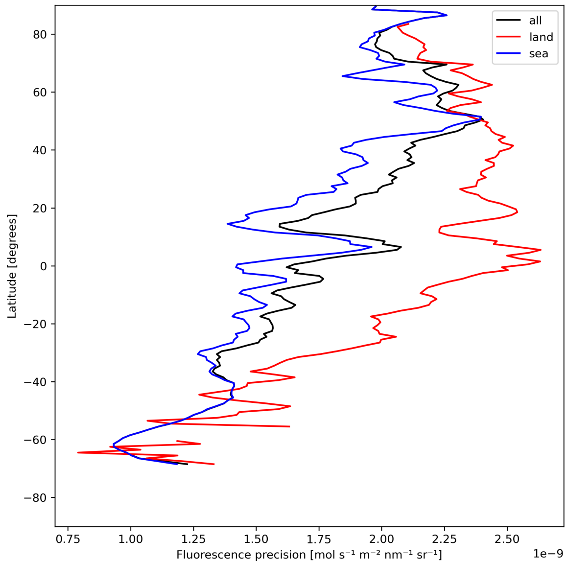
Figure 24: Zonal average of “Fluorescence precision” for 2024-05-13 to 2024-05-15.
