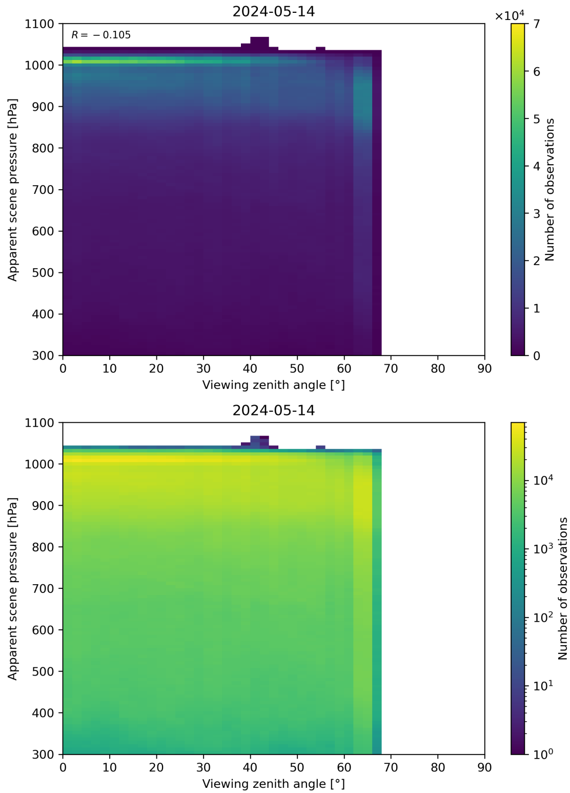
Figure 118: Scatter density plot of “Viewing zenith angle” against “Apparent scene pressure” for 2024-05-13 to 2024-05-15.
