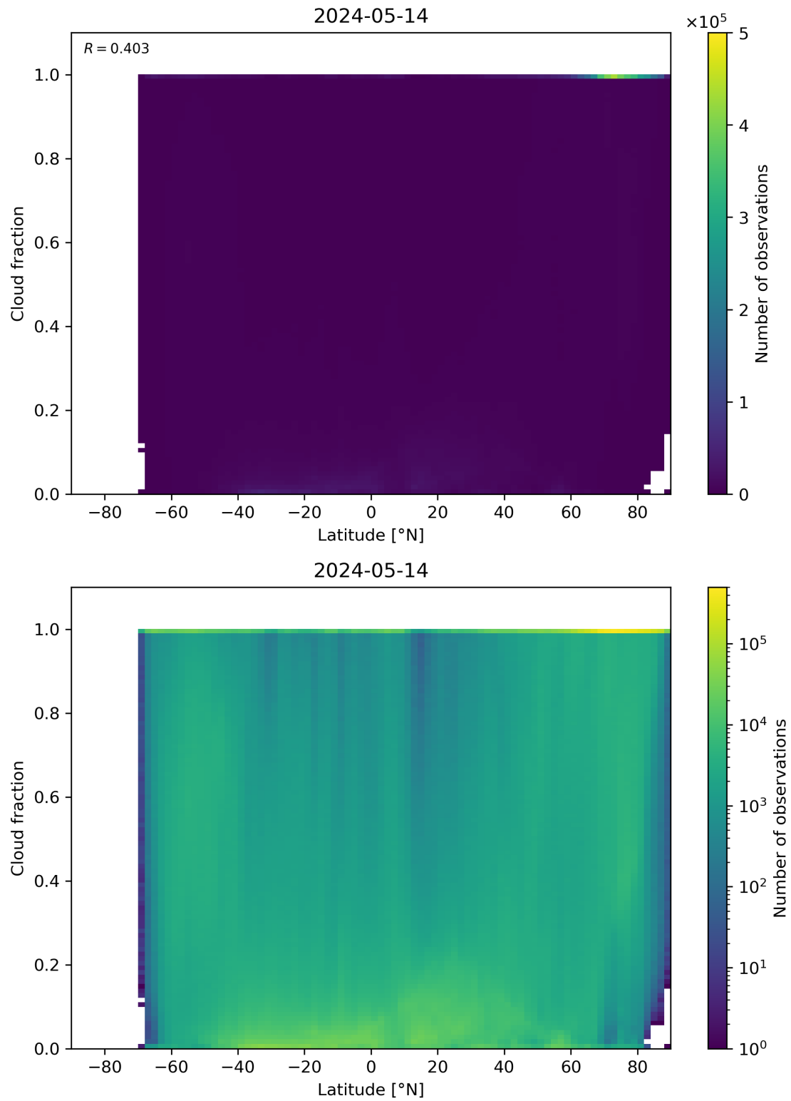
Figure 90: Scatter density plot of “Latitude” against “Cloud fraction” for 2024-05-13 to 2024-05-15.
