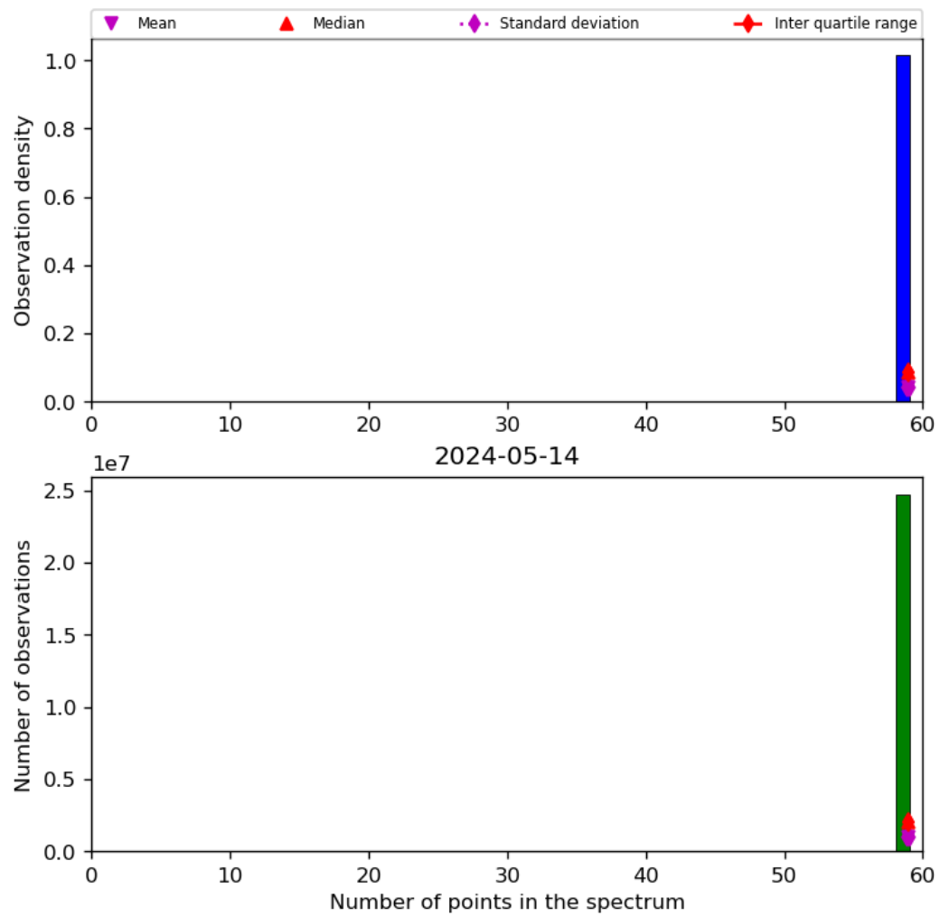
Figure 44: Histogram of “Number of points in the spectrum” for 2024-05-13 to 2024-05-15
