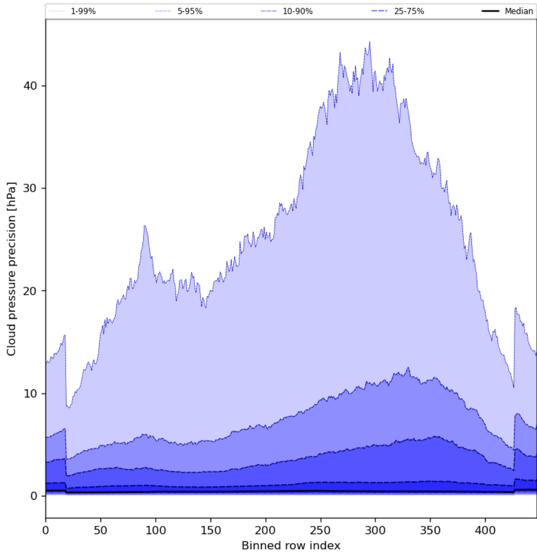
Figure 48: Along track statistics of “Cloud pressure precision” for 2024-05-13 to 2024-05-15
