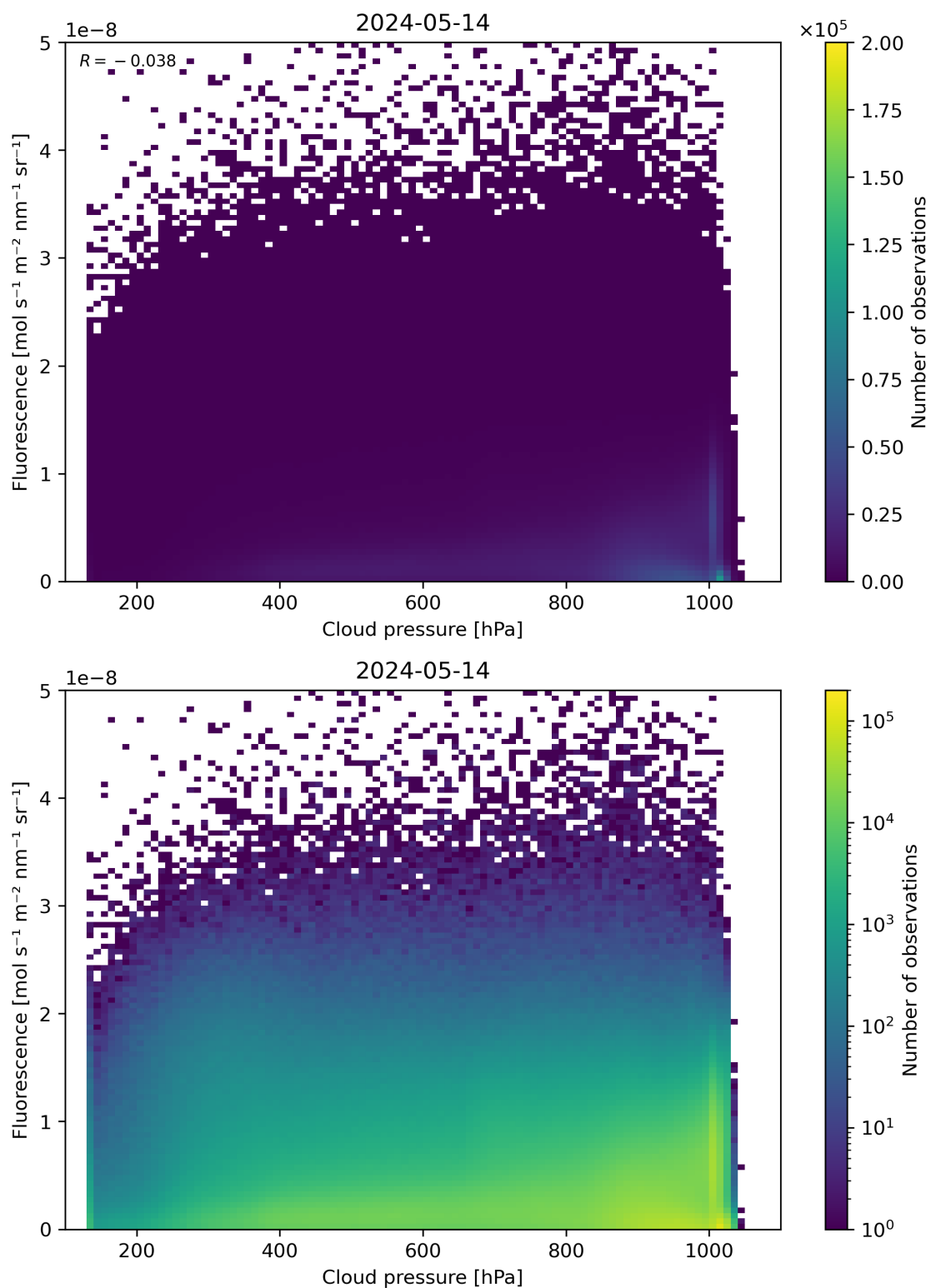
Figure 80: Scatter density plot of “Cloud pressure” against “Fluorescence” for 2024-05-13 to 2024-05-15.
