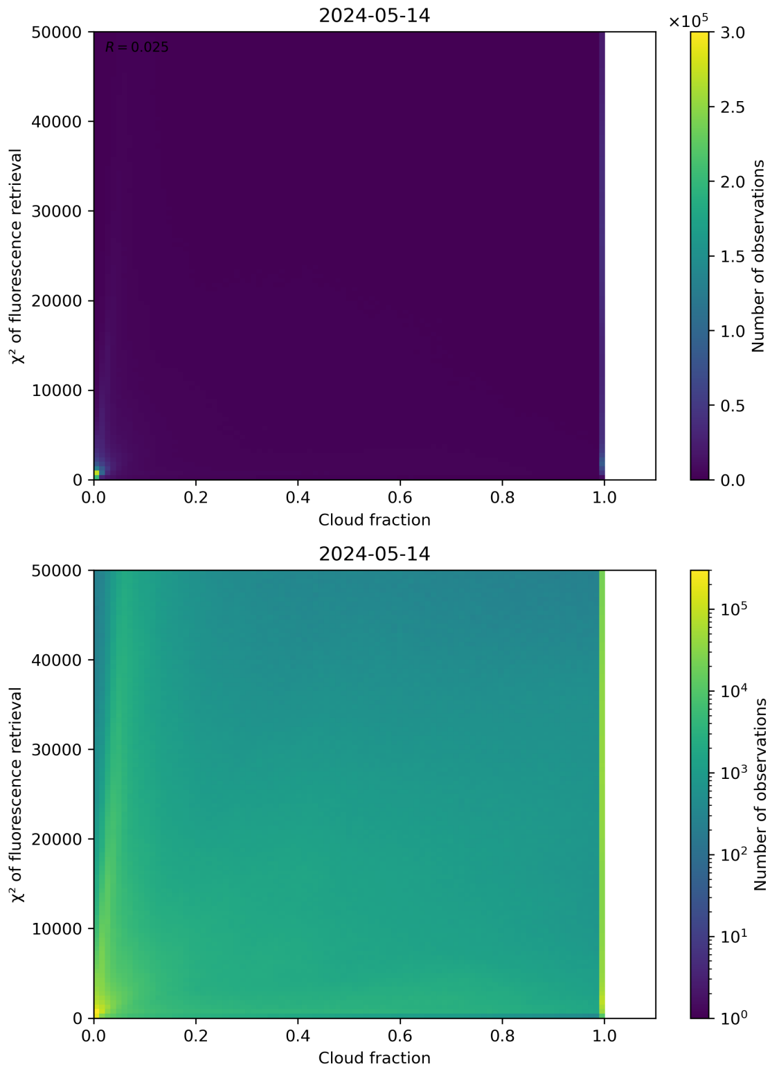
Figure 71: Scatter density plot of “Cloud fraction” against “ \chi^2 of fluorescence retrieval” for 2024-05-13 to 2024-05-15.
