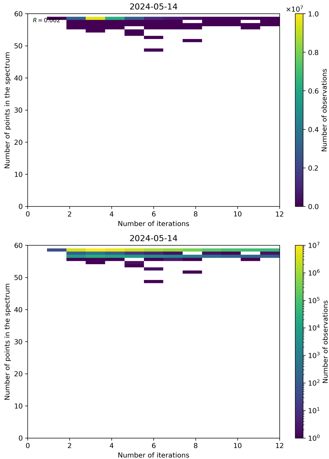
Figure 99: Scatter density plot of “Number of iterations” against “Number of points in the spectrum” for 2024-05-13 to 2024-05-15.
