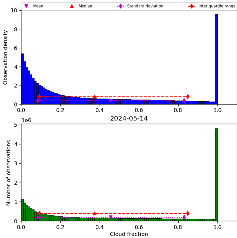
Figure 32: Histogram of “Cloud fraction” for 2024-05-13 to 2024-05-15
