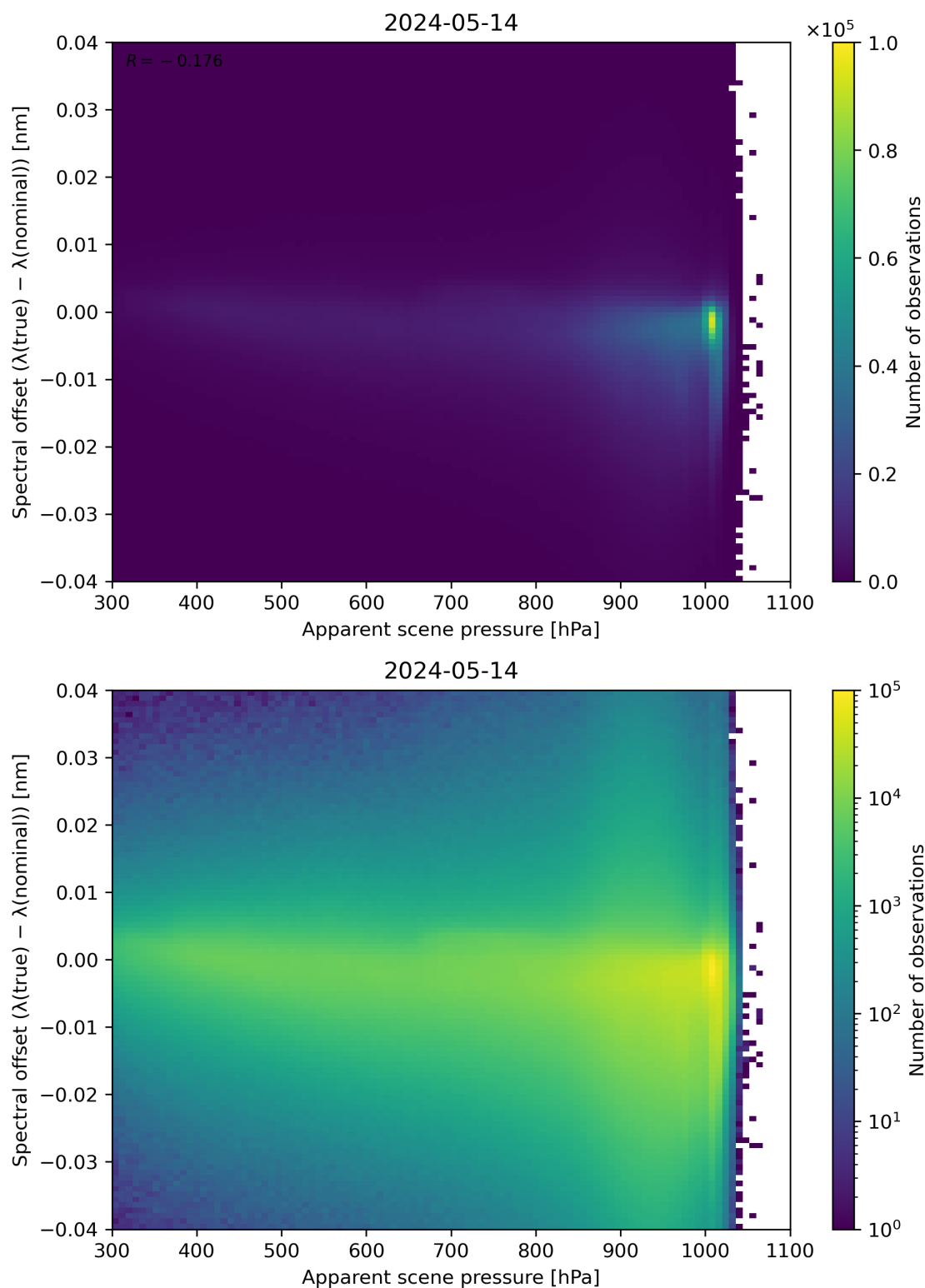
Figure 67: Scatter density plot of “Apparent scene pressure” against “Spectral offset ( \lambda(\text{true}) - \lambda(\text{nominal}) )” for 2024-05-13 to 2024-05-15.
