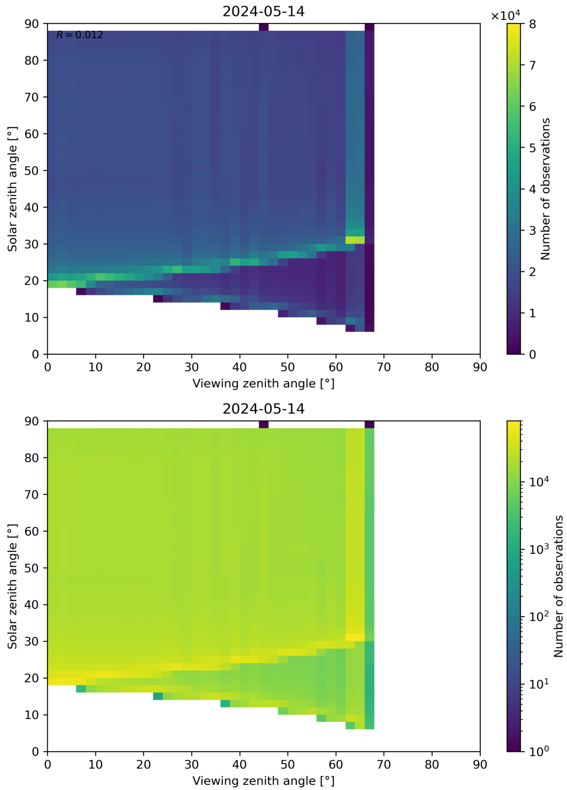
Figure 127: Scatter density plot of “Viewing zenith angle” against “Solar zenith angle” for 2024-05-13 to 2024-05-15.
