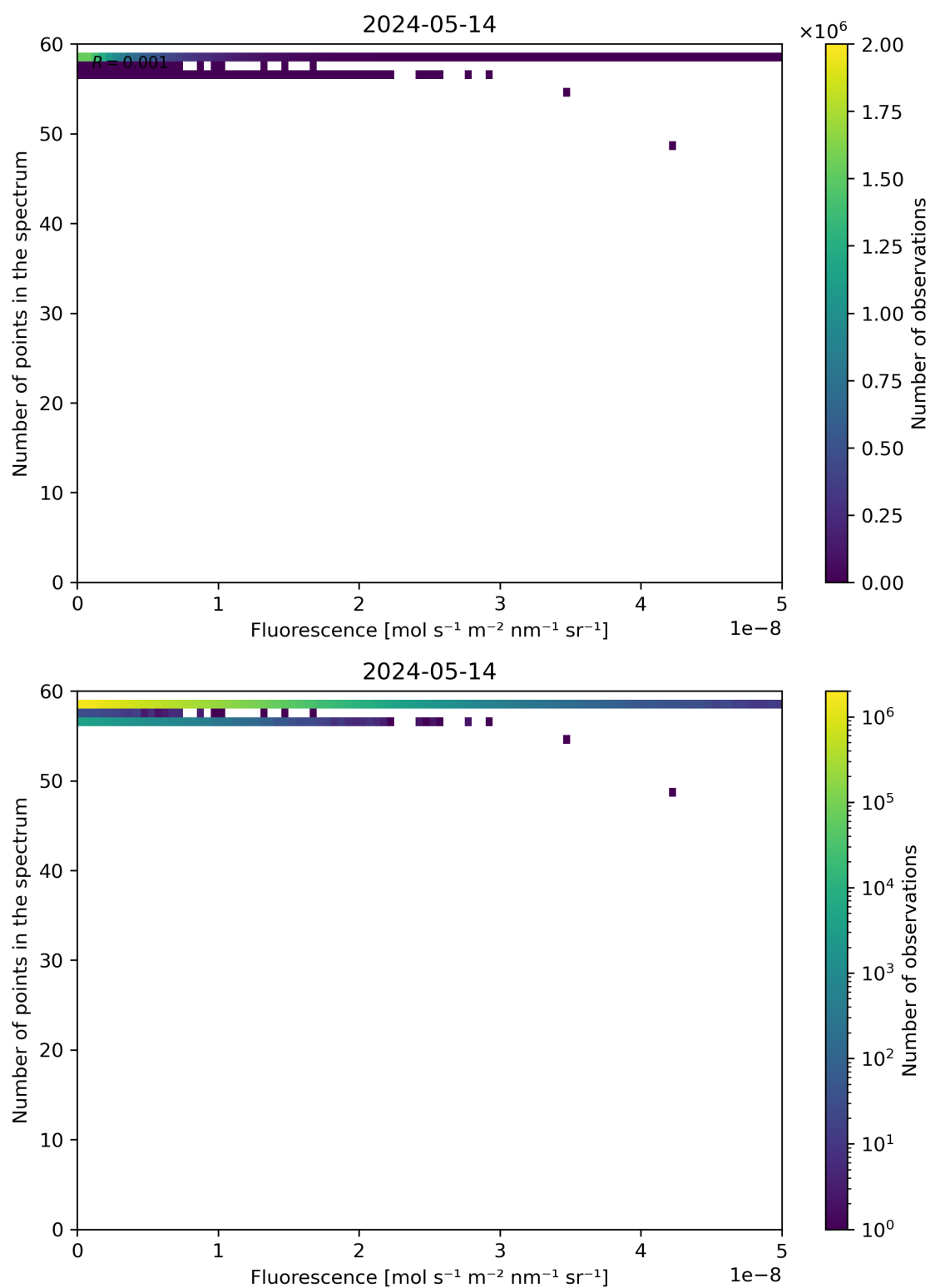
Figure 86: Scatter density plot of “Fluorescence” against “Number of points in the spectrum” for 2024-05-13 to 2024-05-15.
