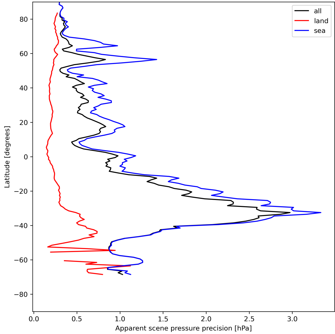
Figure 20: Zonal average of “Apparent scene pressure precision” for 2024-05-13 to 2024-05-15.
