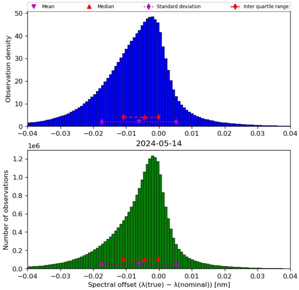
Figure 45: Histogram of “Spectral offset ( \lambda(\text{true}) - \lambda(\text{nominal}) )” for 2024-05-13 to 2024-05-15
