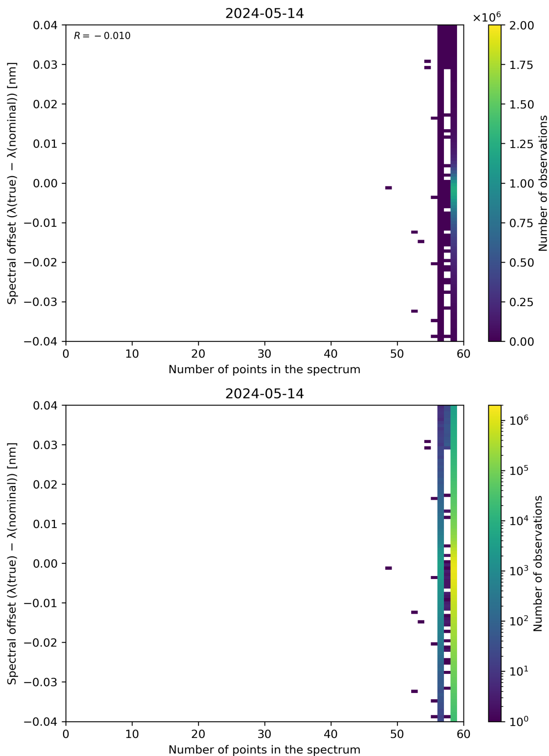
Figure 101: Scatter density plot of “Number of points in the spectrum” against “Spectral offset ( \lambda(\text{true}) - \lambda(\text{nominal}) )” for 2024-05-13 to 2024-05-15.
