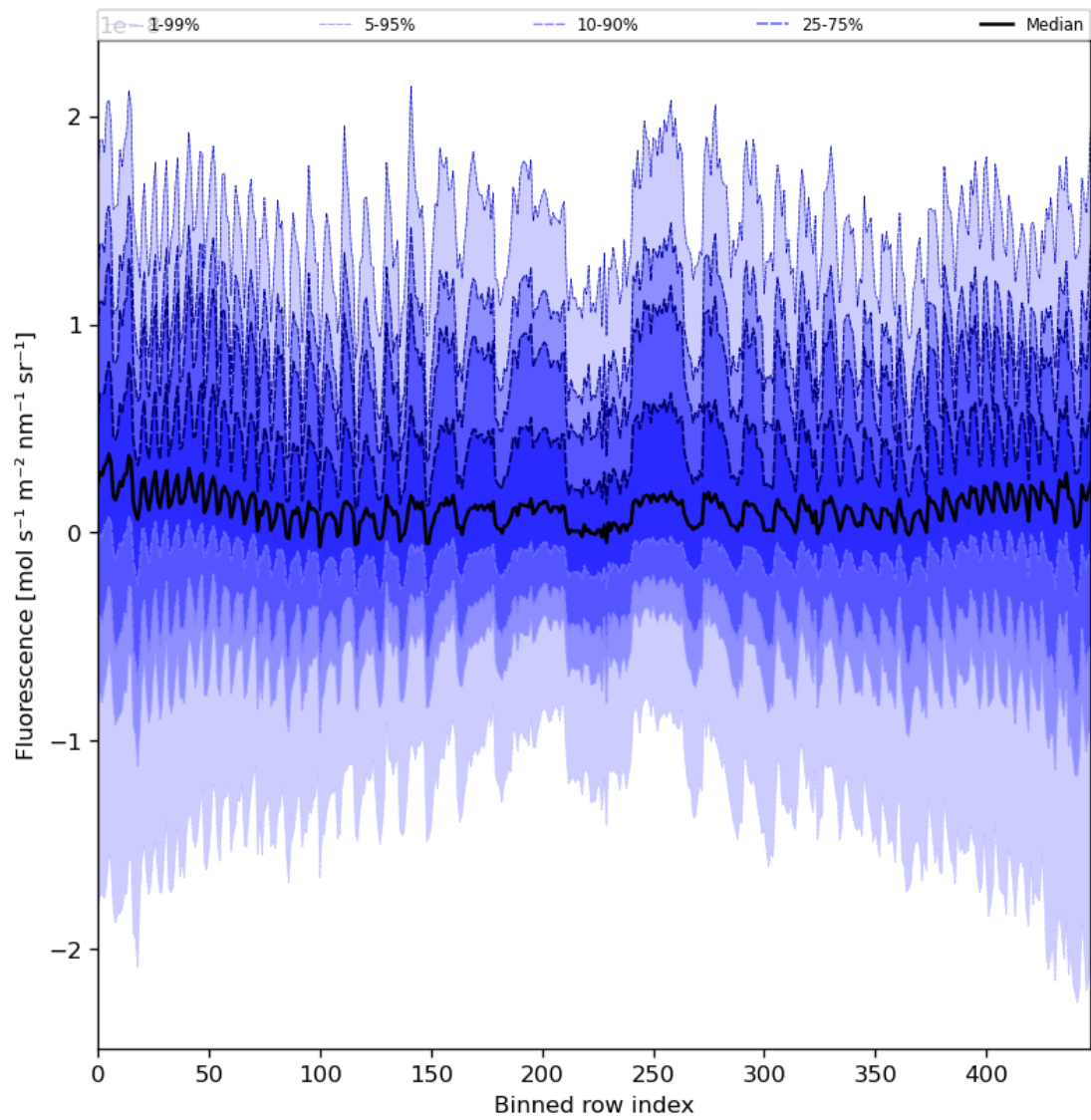
Figure 57: Along track statistics of “Fluorescence” for 2024-05-13 to 2024-05-15
