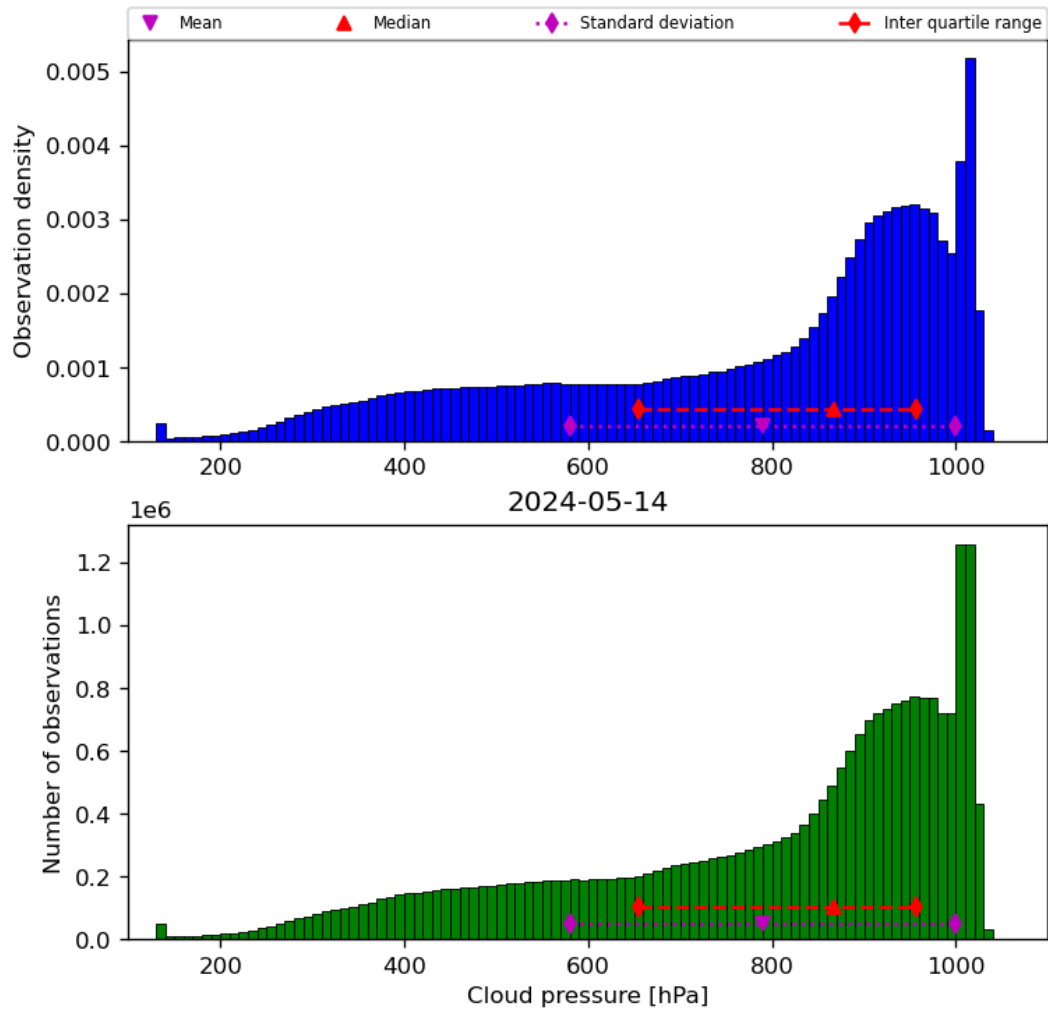
Figure 30: Histogram of “Cloud pressure” for 2024-05-13 to 2024-05-15
