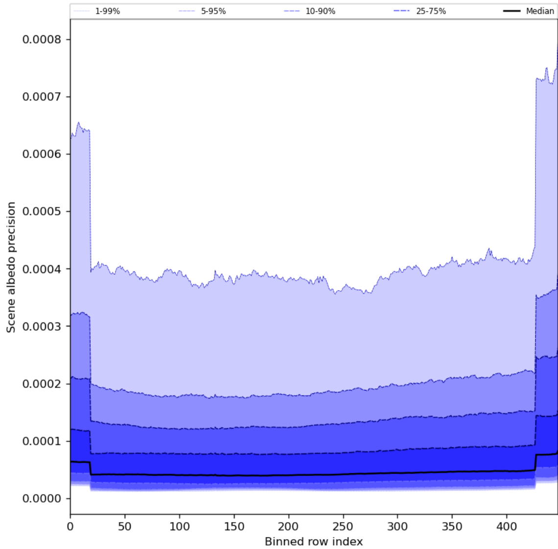
Figure 52: Along track statistics of “Scene albedo precision” for 2024-05-13 to 2024-05-15
