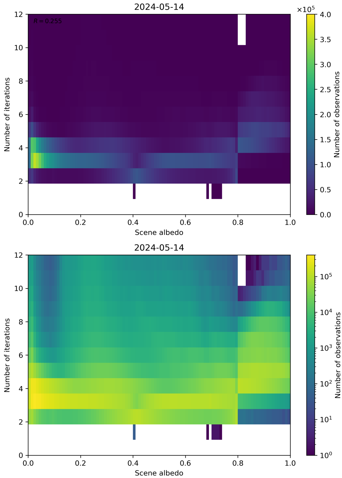
Figure 105: Scatter density plot of “Scene albedo” against “Number of iterations” for 2024-05-13 to 2024-05-15.
