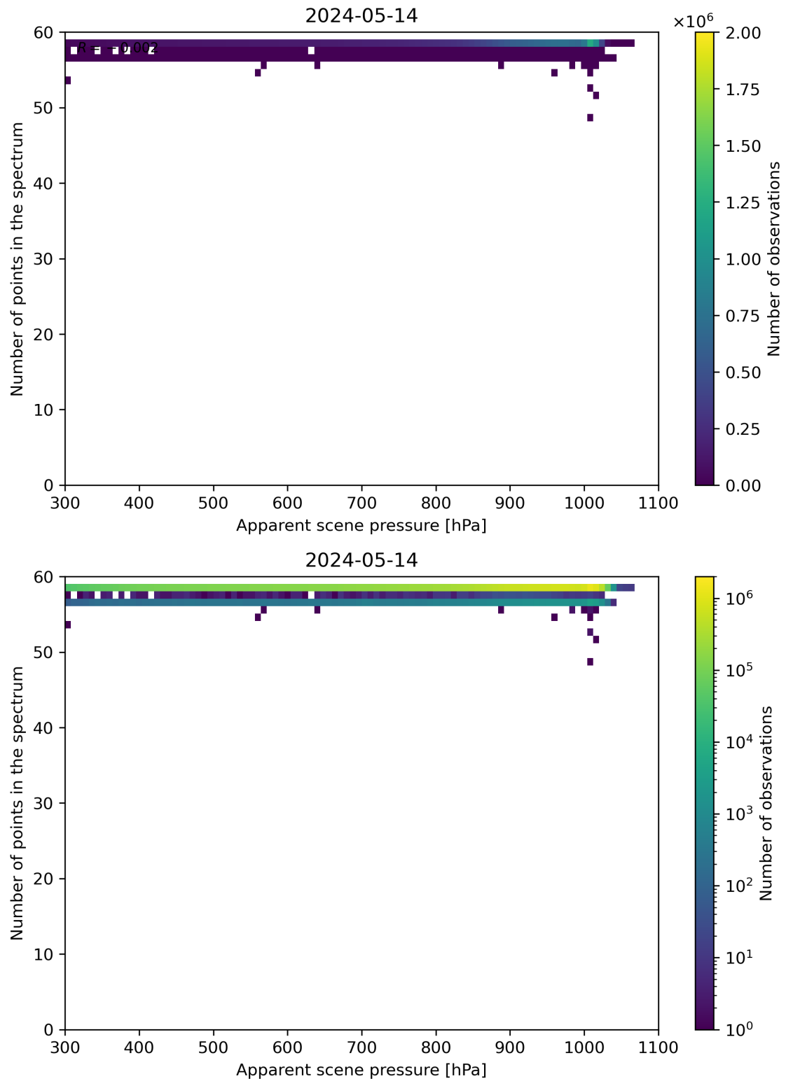
Figure 66: Scatter density plot of “Apparent scene pressure” against “Number of points in the spectrum” for 2024-05-13 to 2024-05-15.
