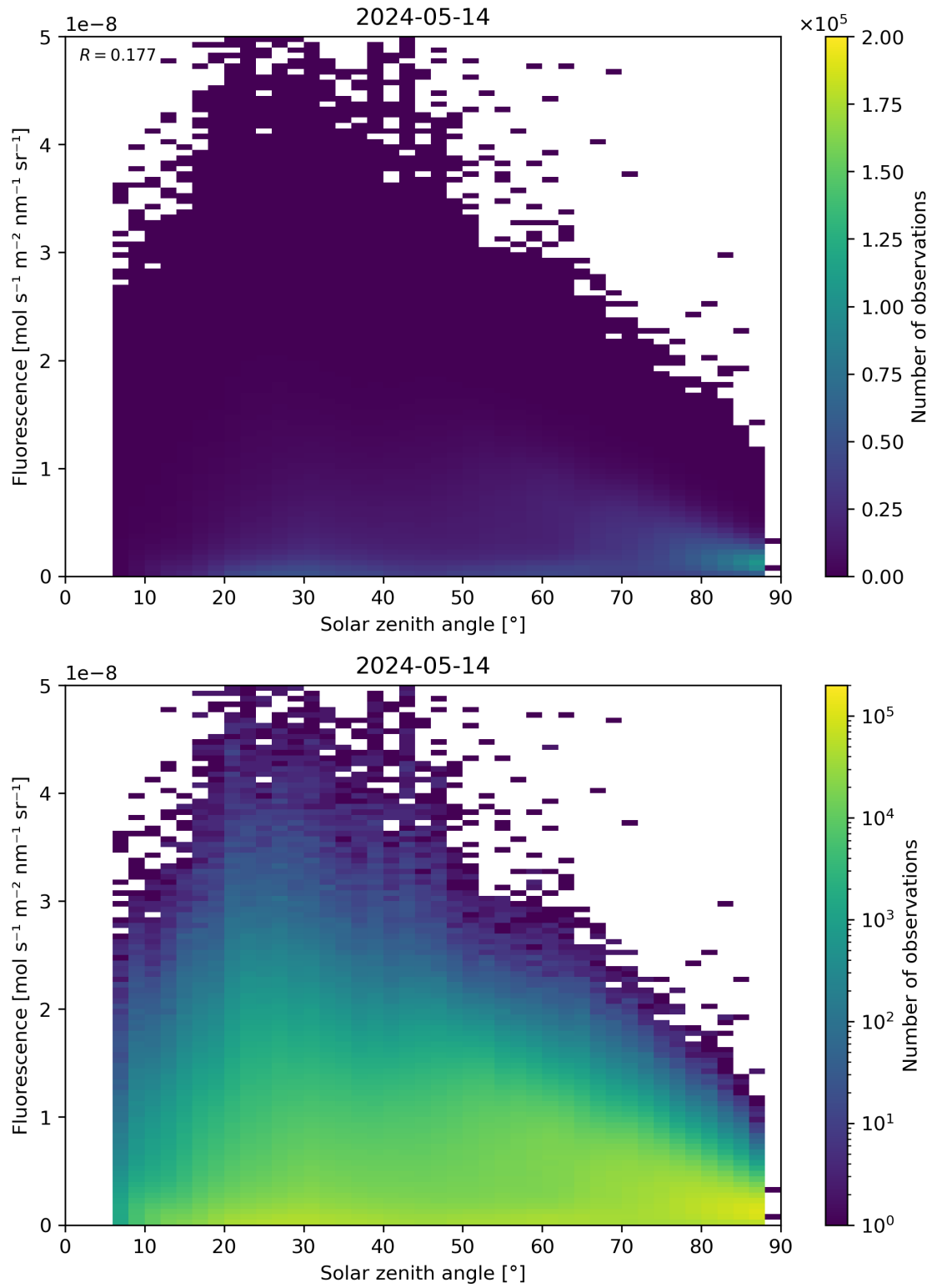
Figure 112: Scatter density plot of “Solar zenith angle” against “Fluorescence” for 2024-05-13 to 2024-05-15.
