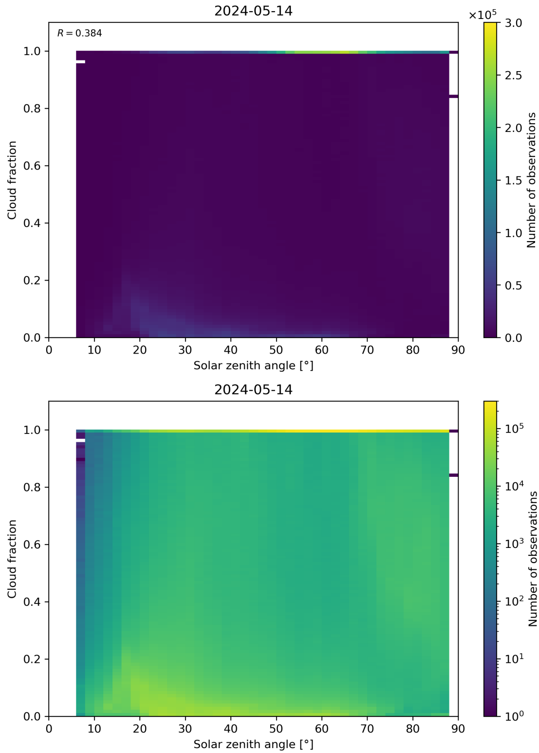
Figure 110: Scatter density plot of “Solar zenith angle” against “Cloud fraction” for 2024-05-13 to 2024-05-15.
