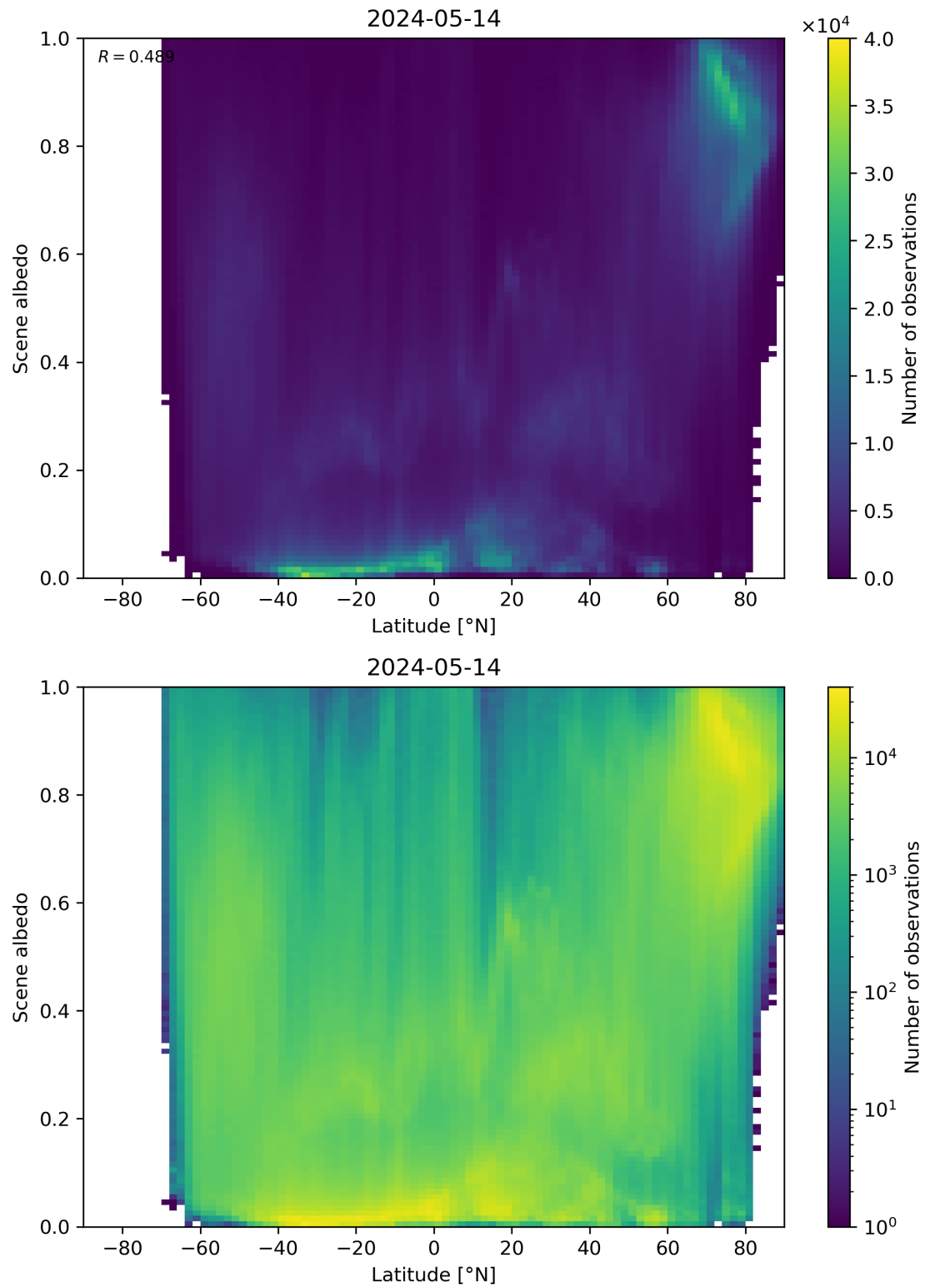
Figure 95: Scatter density plot of “Latitude” against “Scene albedo” for 2024-05-13 to 2024-05-15.
