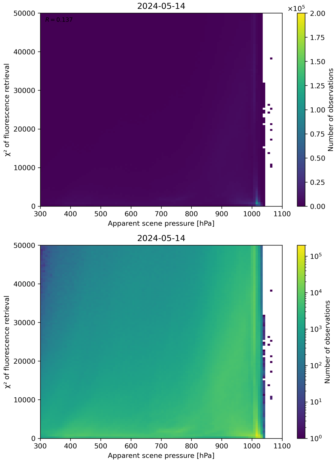
Figure 63: Scatter density plot of “Apparent scene pressure” against “ \chi^2 of fluorescence retrieval” for 2024-05-13 to 2024-05-15.
