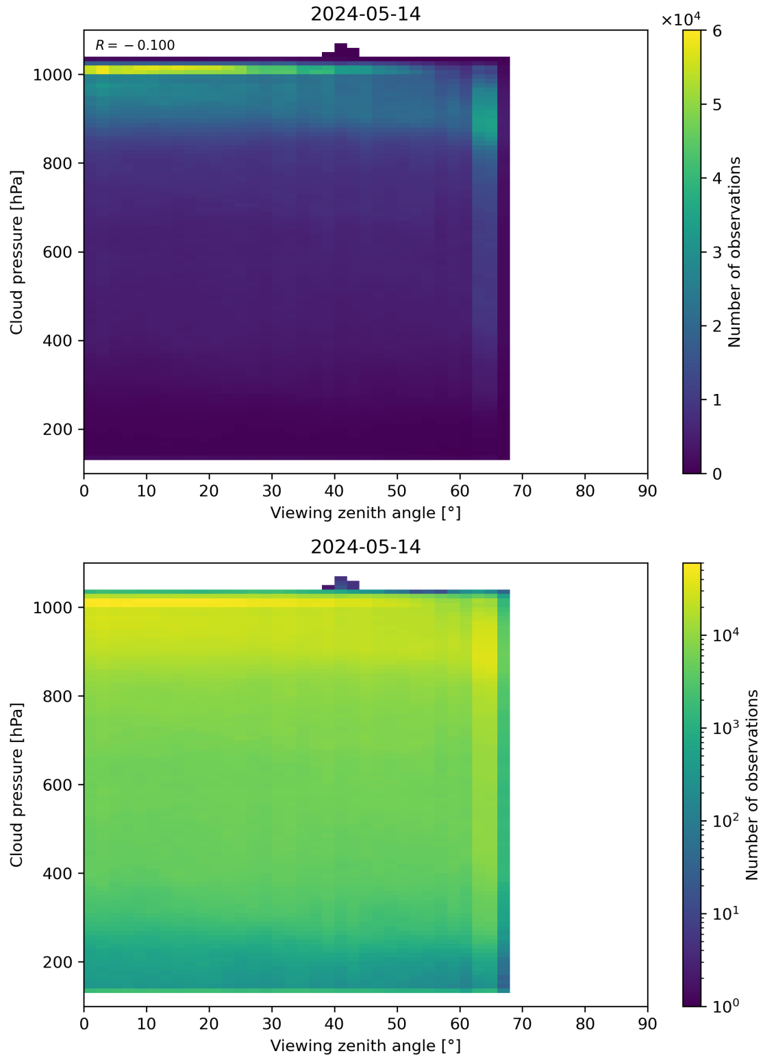
Figure 121: Scatter density plot of “Viewing zenith angle” against “Cloud pressure” for 2024-05-13 to 2024-05-15.
