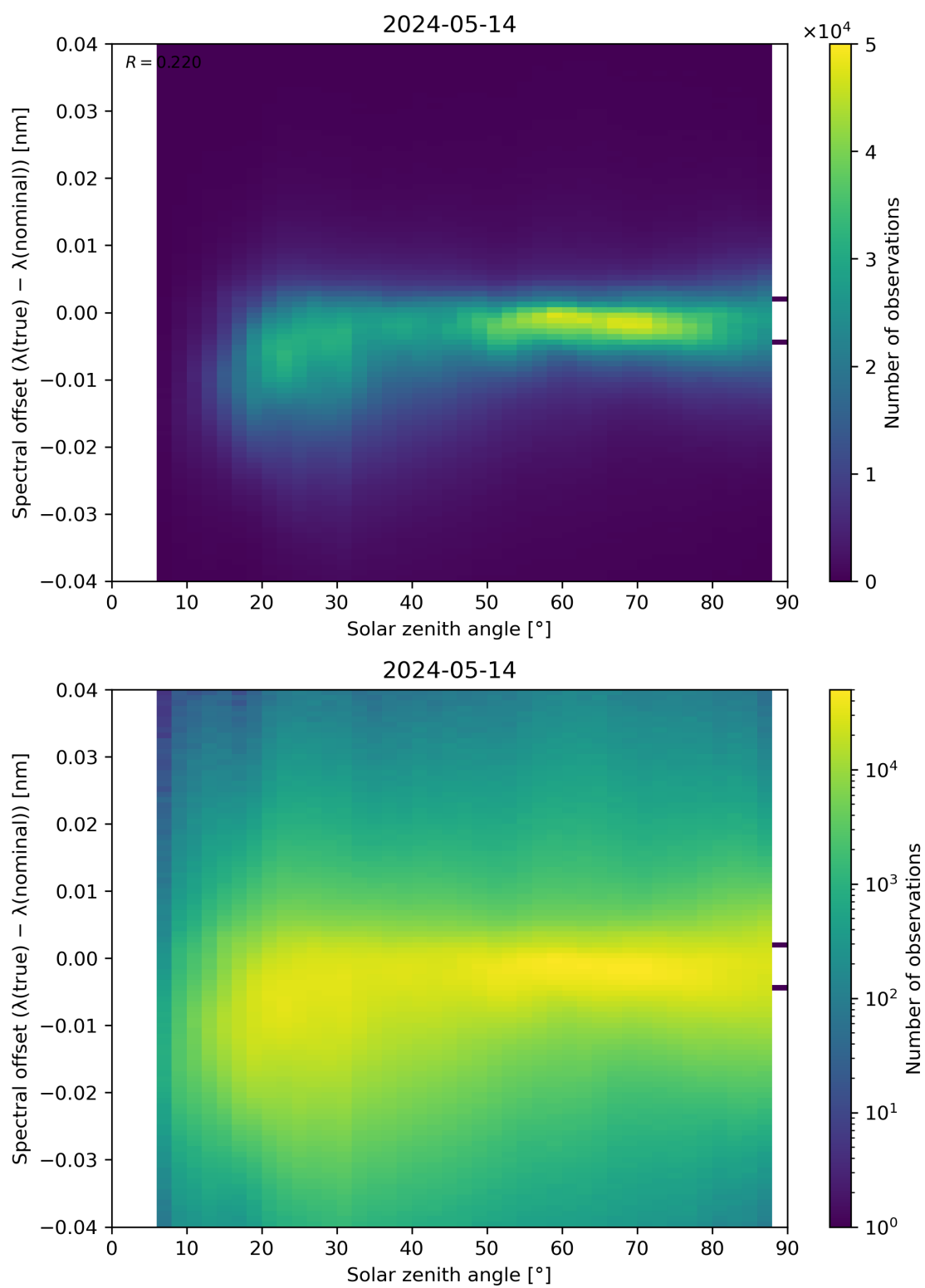
Figure 117: Scatter density plot of “Solar zenith angle” against “Spectral offset ( \lambda(\text{true}) - \lambda(\text{nominal}) )” for 2024-05-13 to 2024-05-15.
