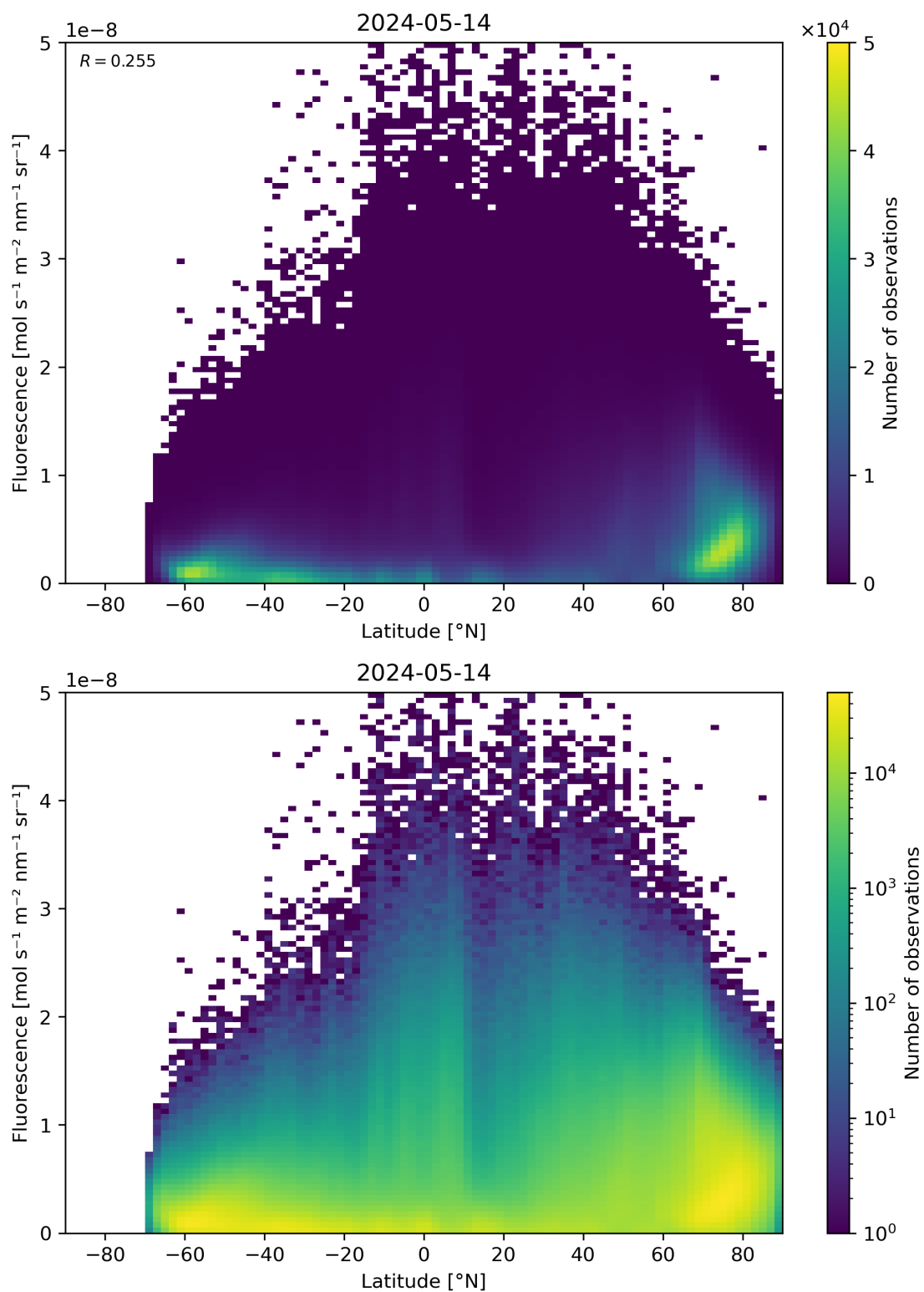
Figure 92: Scatter density plot of “Latitude” against “Fluorescence” for 2024-05-13 to 2024-05-15.
