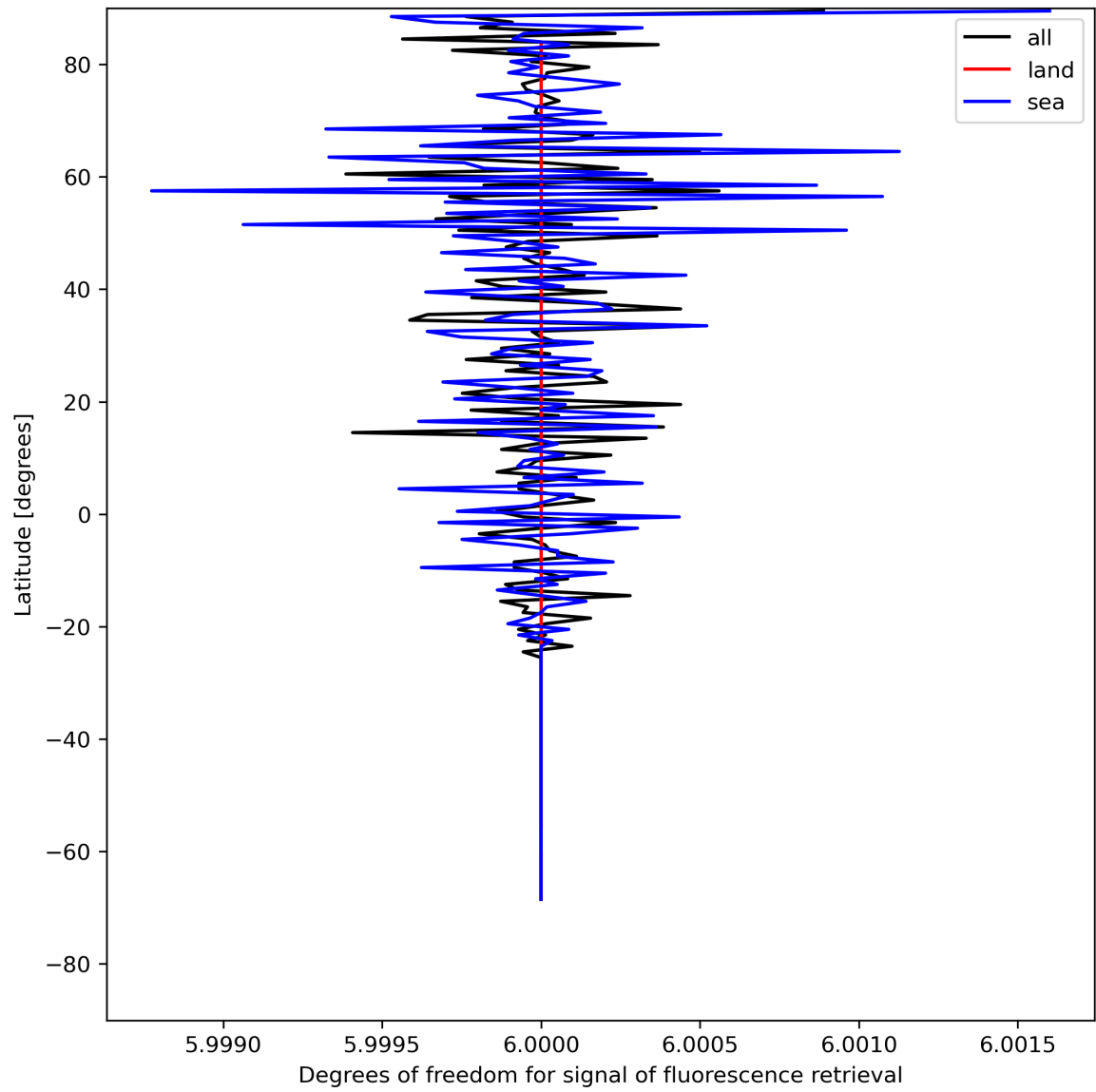
Figure 26: Zonal average of “Degrees of freedom for signal of fluorescence retrieval” for 2024-05-13 to 2024-05-15.
