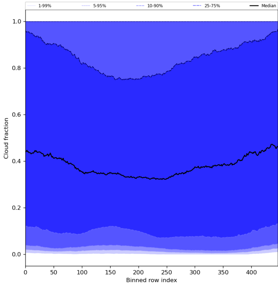
Figure 49: Along track statistics of “Cloud fraction” for 2024-05-13 to 2024-05-15
