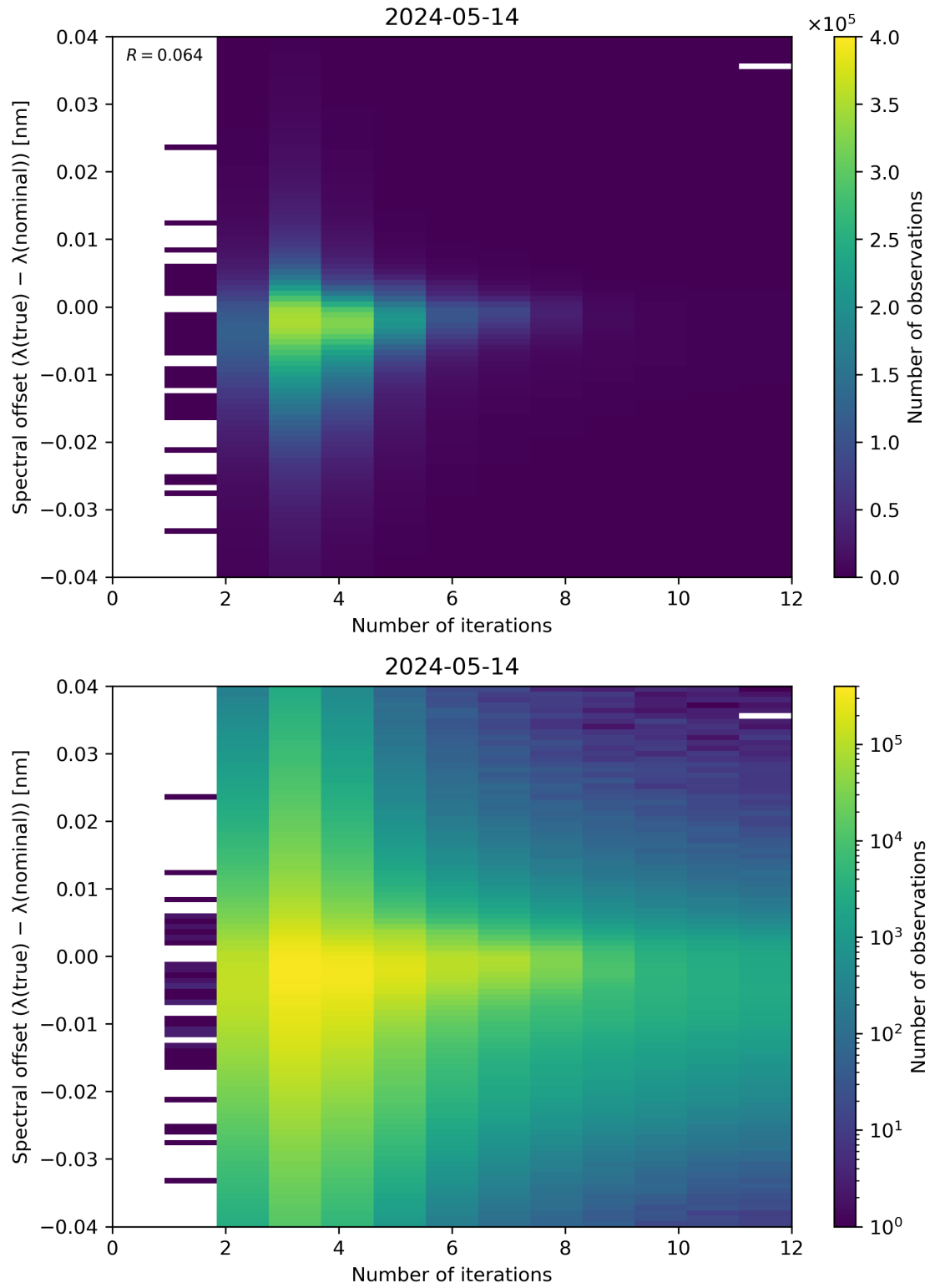
Figure 100: Scatter density plot of “Number of iterations” against “Spectral offset ( \lambda(\text{true}) - \lambda(\text{nominal}) )” for 2024-05-13 to 2024-05-15.
