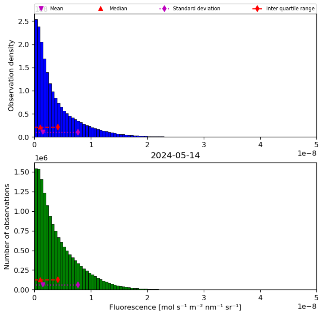
Figure 40: Histogram of “Fluorescence” for 2024-05-13 to 2024-05-15
