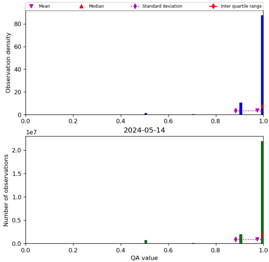
Figure 29: Histogram of “QA value” for 2024-05-13 to 2024-05-15
