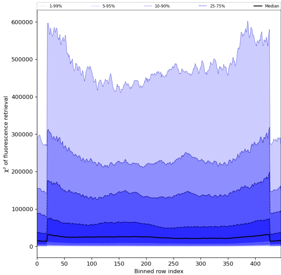
Figure 59: Along track statistics of “ \chi^2 of fluorescence retrieval” for 2024-05-13 to 2024-05-15
