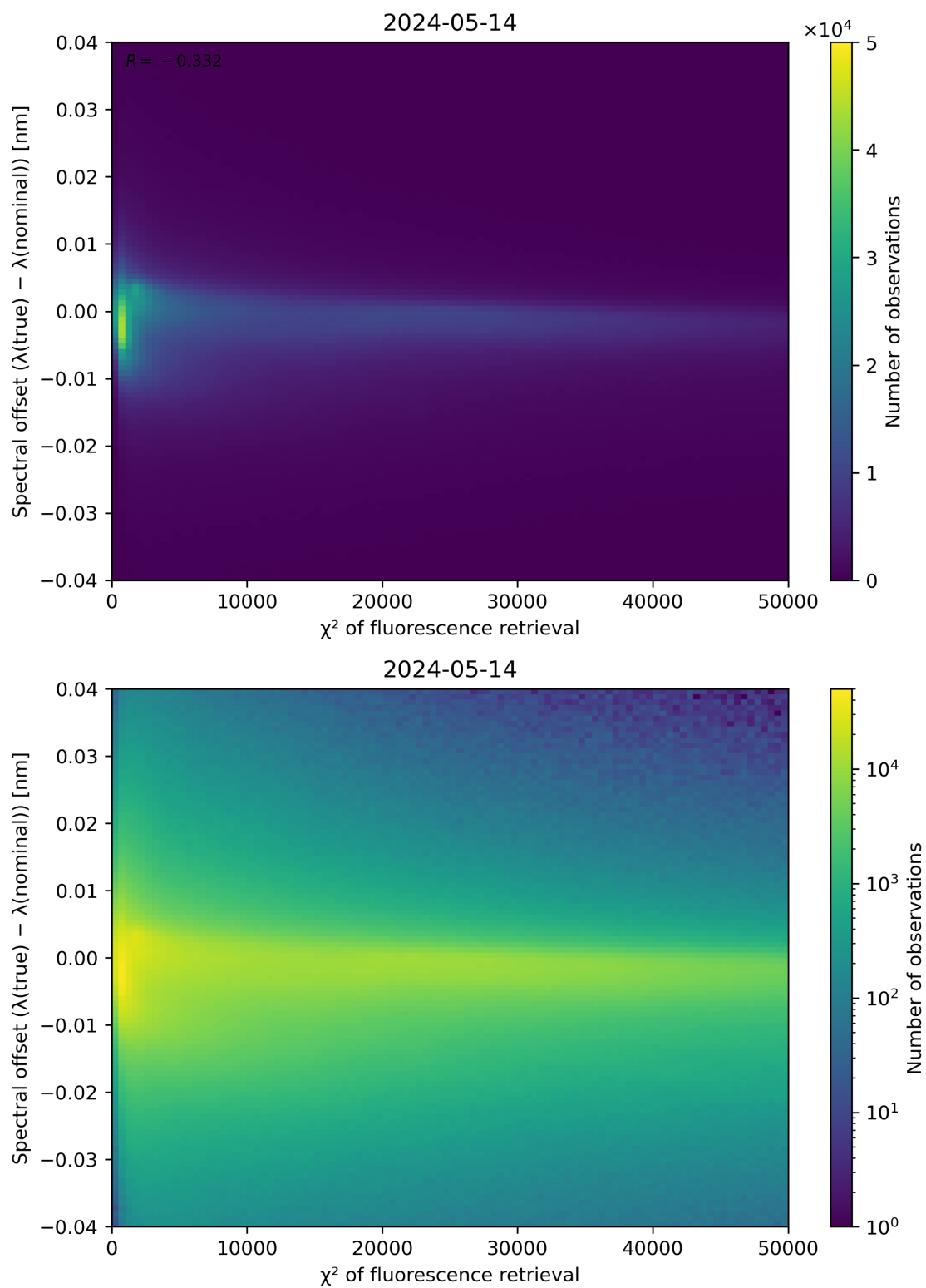
Figure 69: Scatter density plot of “ \chi^2 of fluorescence retrieval” against “Spectral offset ( \lambda(\text{true}) - \lambda(\text{nominal}) )” for 2024-05-13 to 2024-05-15.
