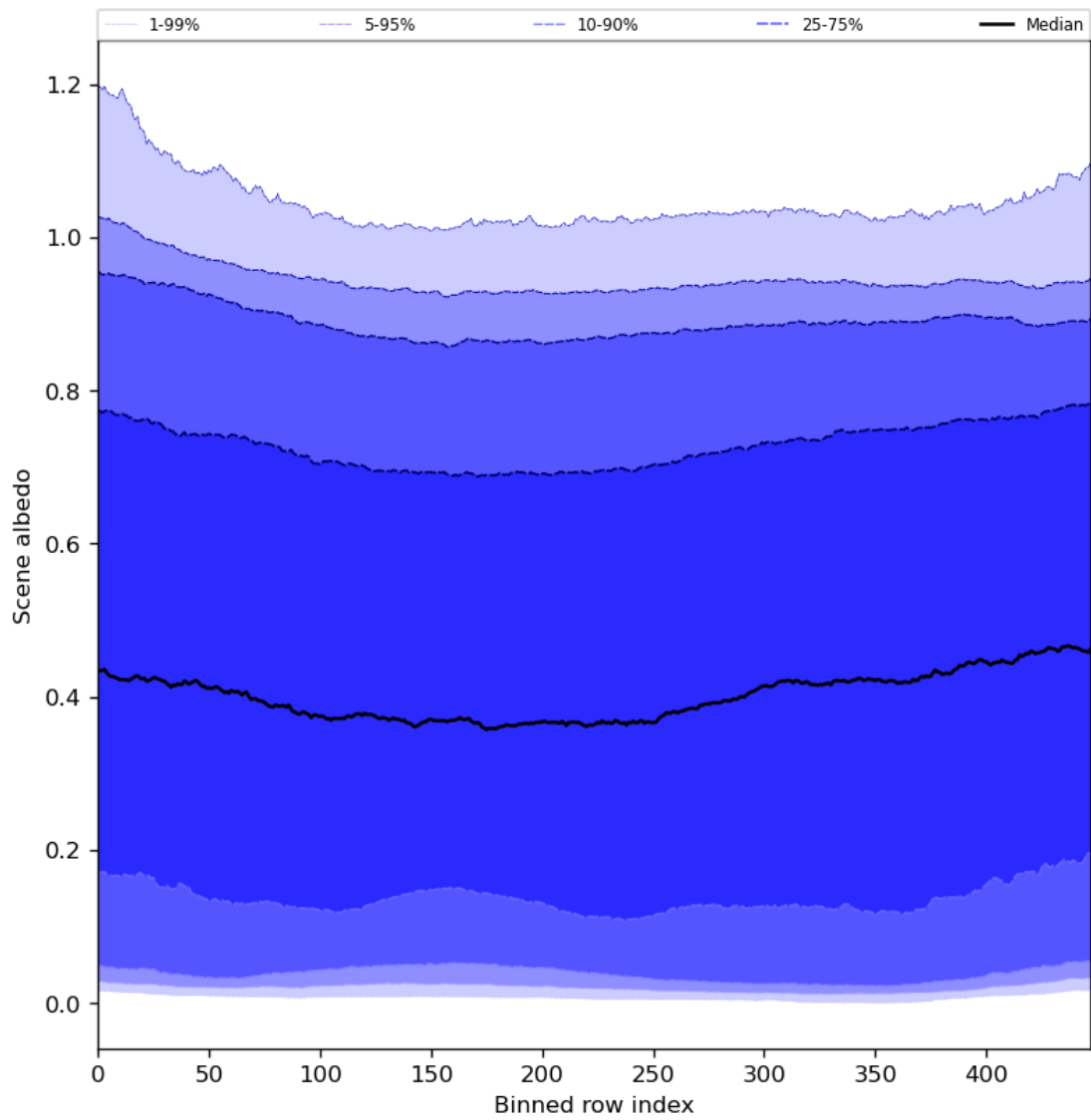
Figure 51: Along track statistics of “Scene albedo” for 2024-05-13 to 2024-05-15
