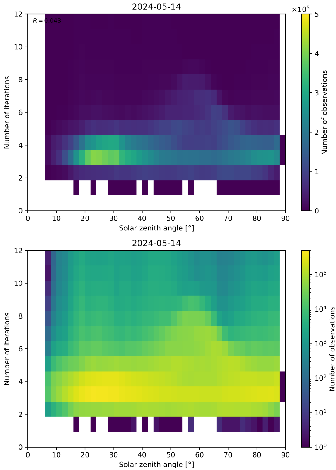
Figure 114: Scatter density plot of “Solar zenith angle” against “Number of iterations” for 2024-05-13 to 2024-05-15.
