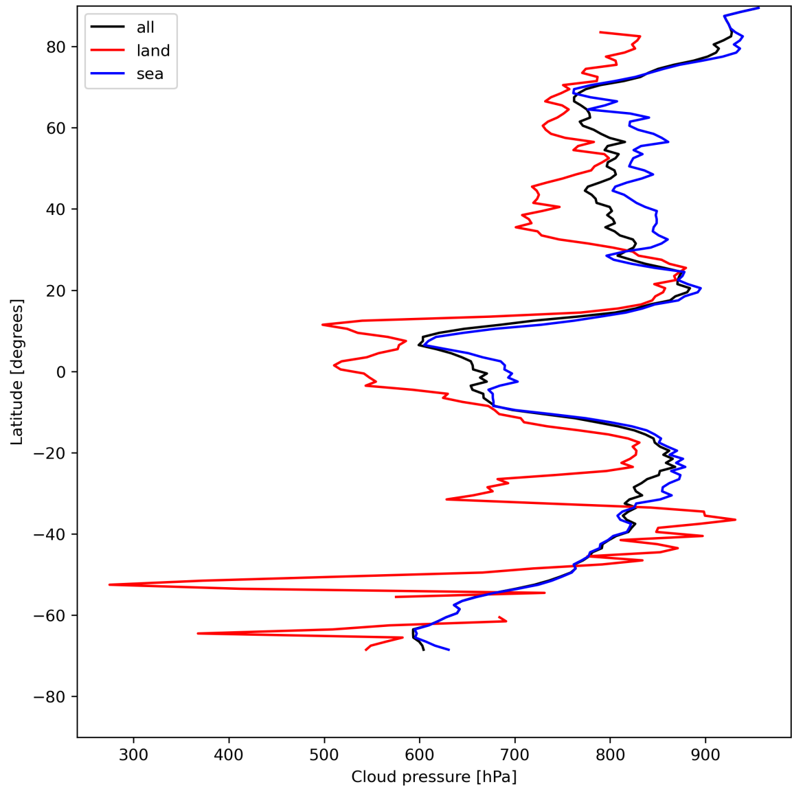
Figure 13: Zonal average of “Cloud pressure” for 2024-05-13 to 2024-05-15.
