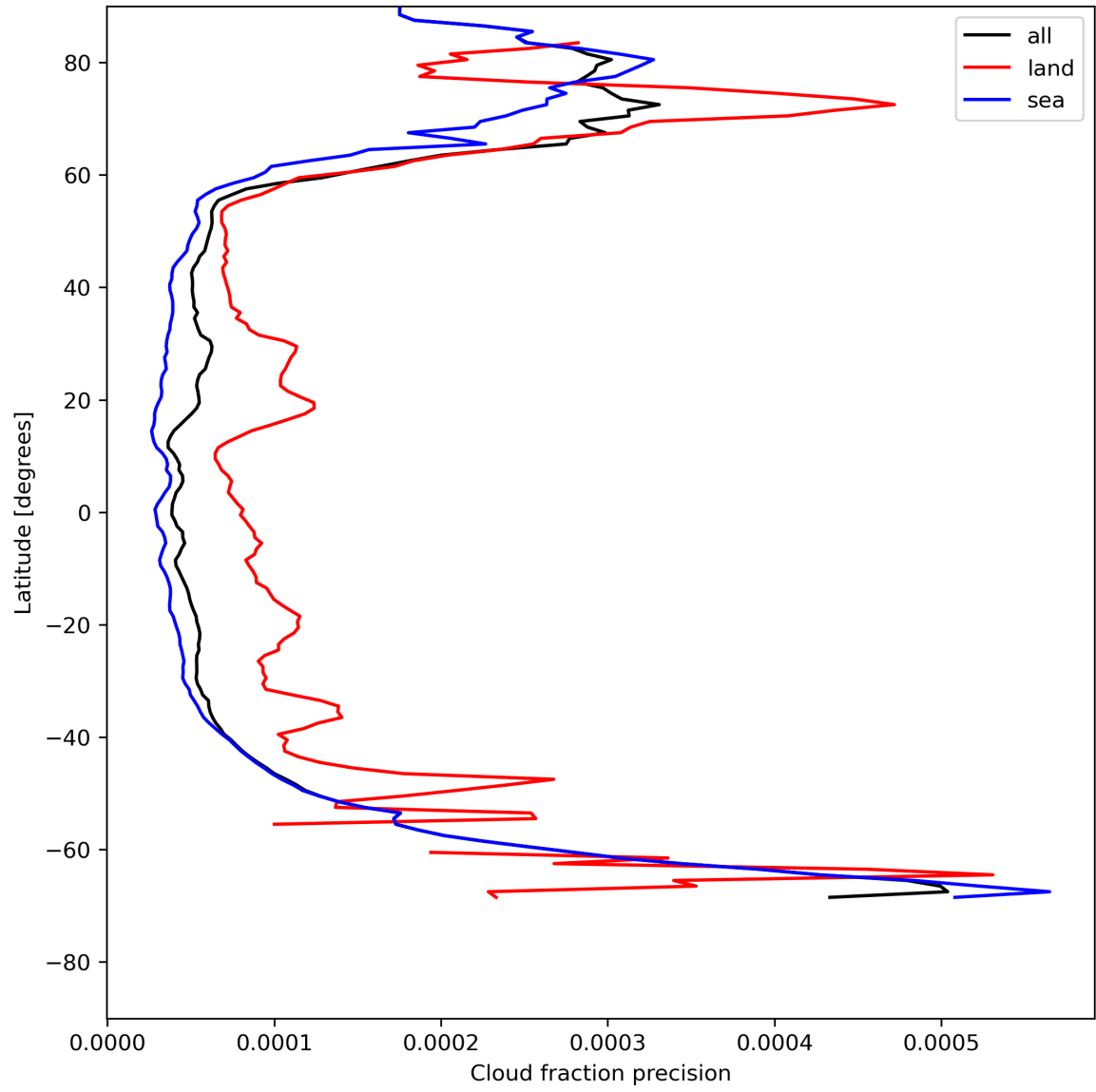
Figure 16: Zonal average of “Cloud fraction precision” for 2024-05-13 to 2024-05-15.
