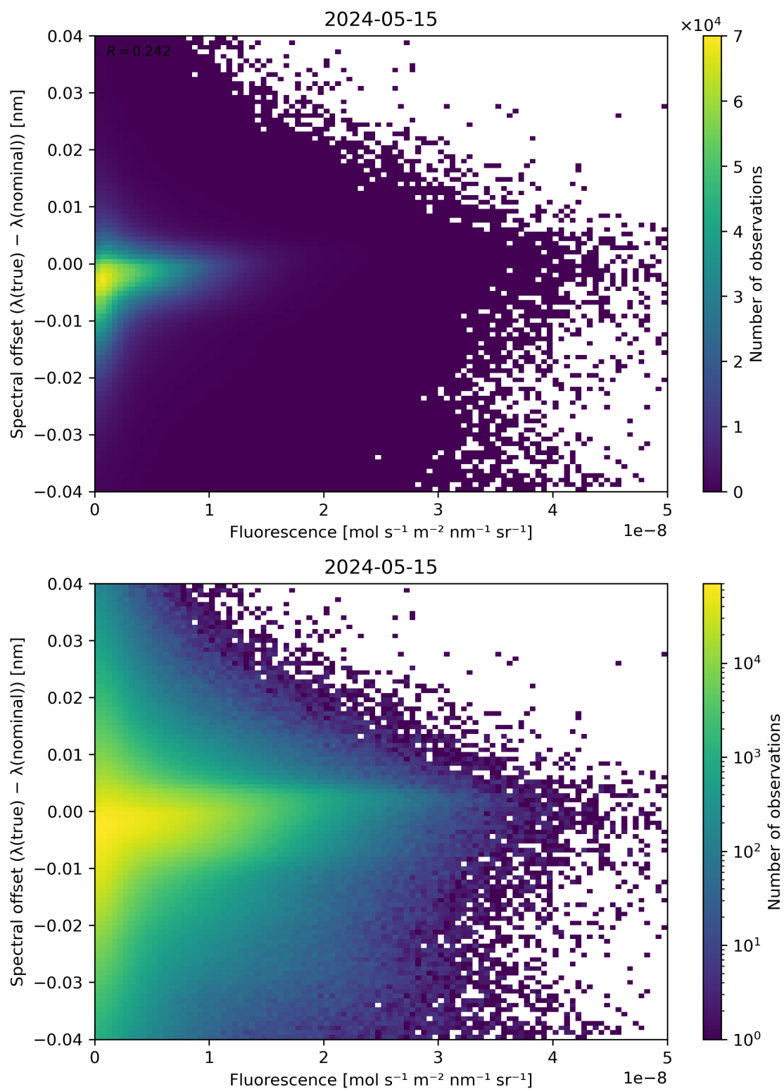
Figure 87: Scatter density plot of “Fluorescence” against “Spectral offset ( \lambda(\text{true}) - \lambda(\text{nominal}) )” for 2024-05-14 to 2024-05-16.
