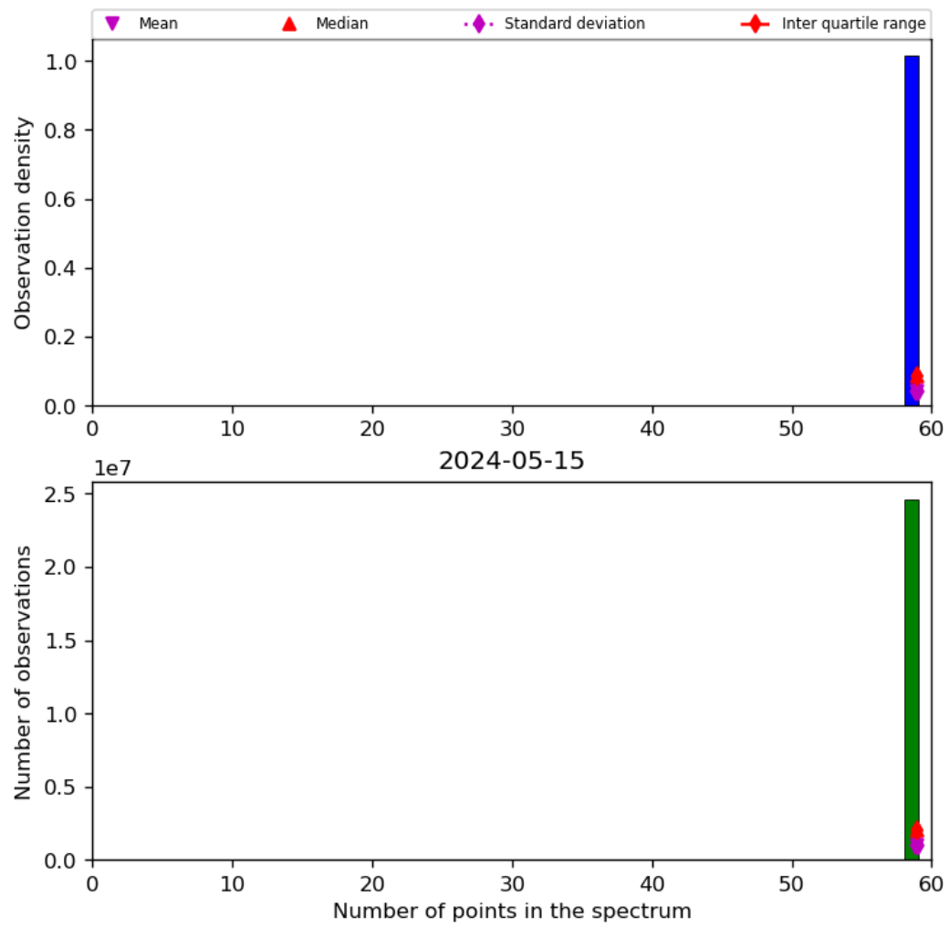
Figure 44: Histogram of “Number of points in the spectrum” for 2024-05-14 to 2024-05-16
