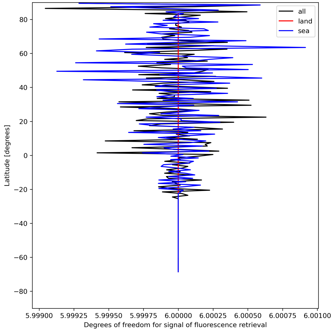
Figure 26: Zonal average of “Degrees of freedom for signal of fluorescence retrieval” for 2024-05-14 to 2024-05-16.
