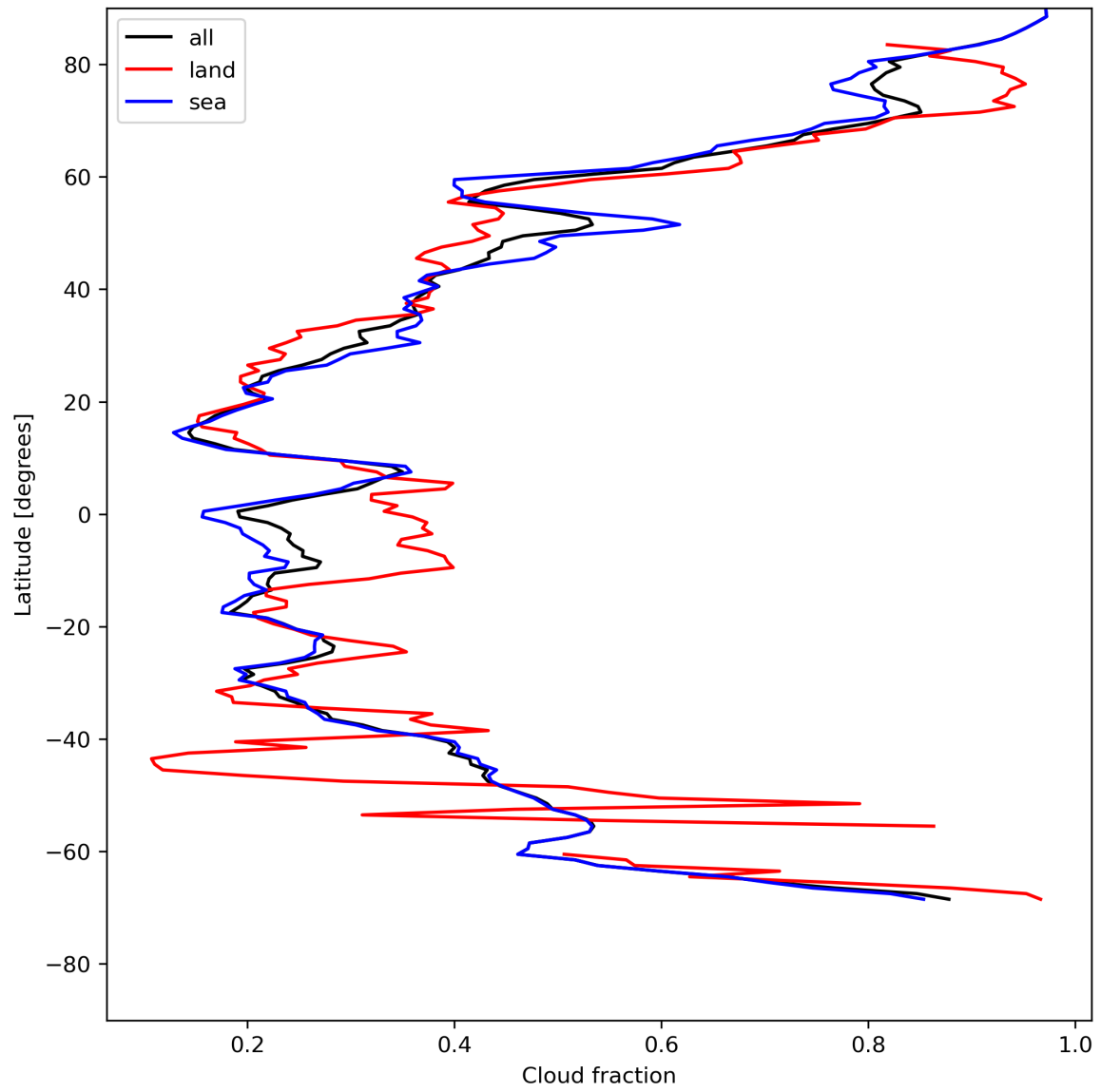
Figure 15: Zonal average of “Cloud fraction” for 2024-05-14 to 2024-05-16.
