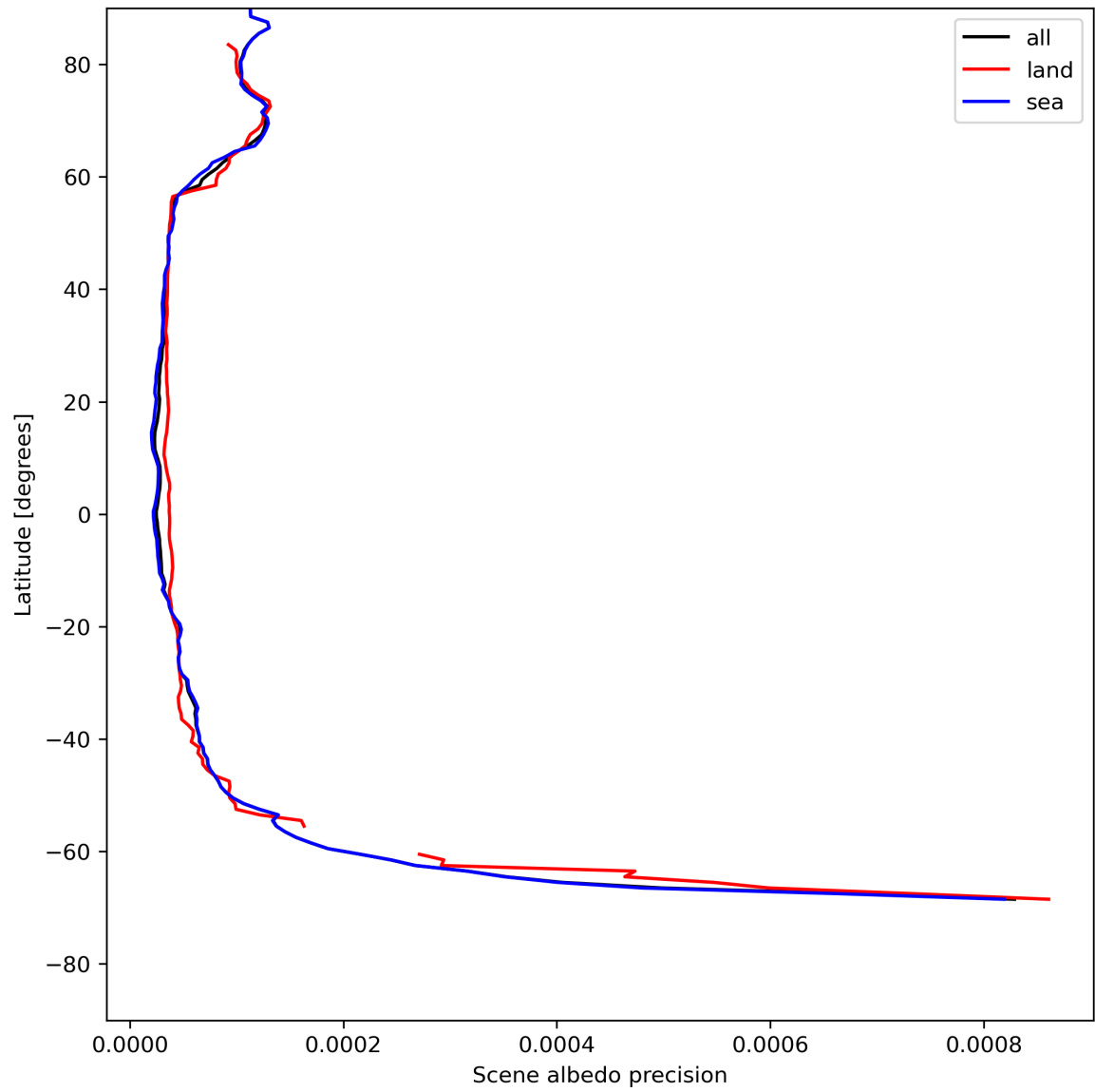
Figure 18: Zonal average of “Scene albedo precision” for 2024-05-14 to 2024-05-16.
