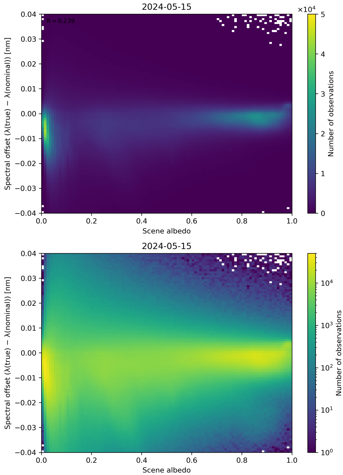
Figure 107: Scatter density plot of “Scene albedo” against “Spectral offset ( \lambda(\text{true}) - \lambda(\text{nominal}) )” for 2024-05-14 to 2024-05-16.
