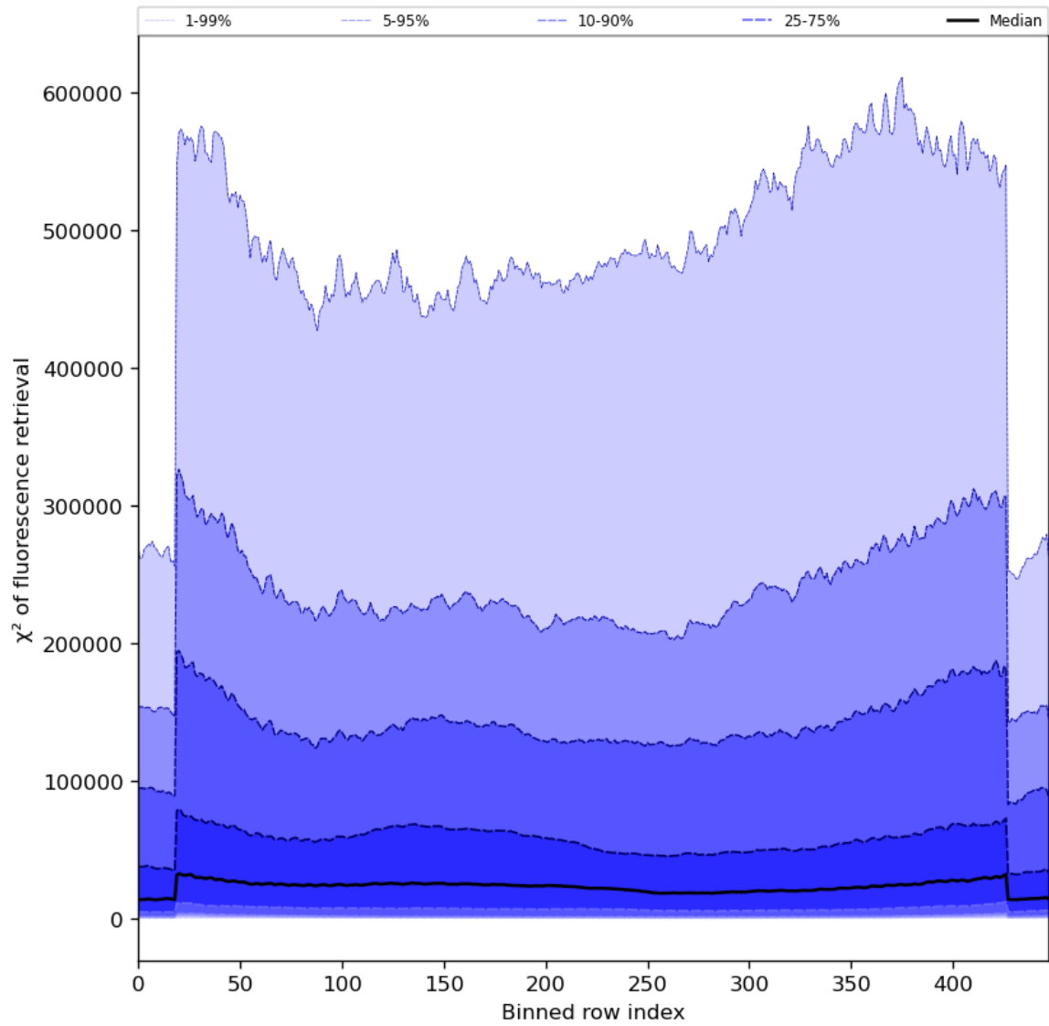
Figure 59: Along track statistics of “ \chi^2 of fluorescence retrieval” for 2024-05-14 to 2024-05-16
