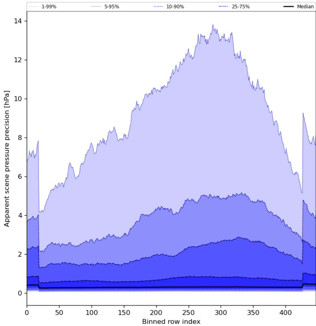
Figure 54: Along track statistics of “Apparent scene pressure precision” for 2024-05-14 to 2024-05-16
