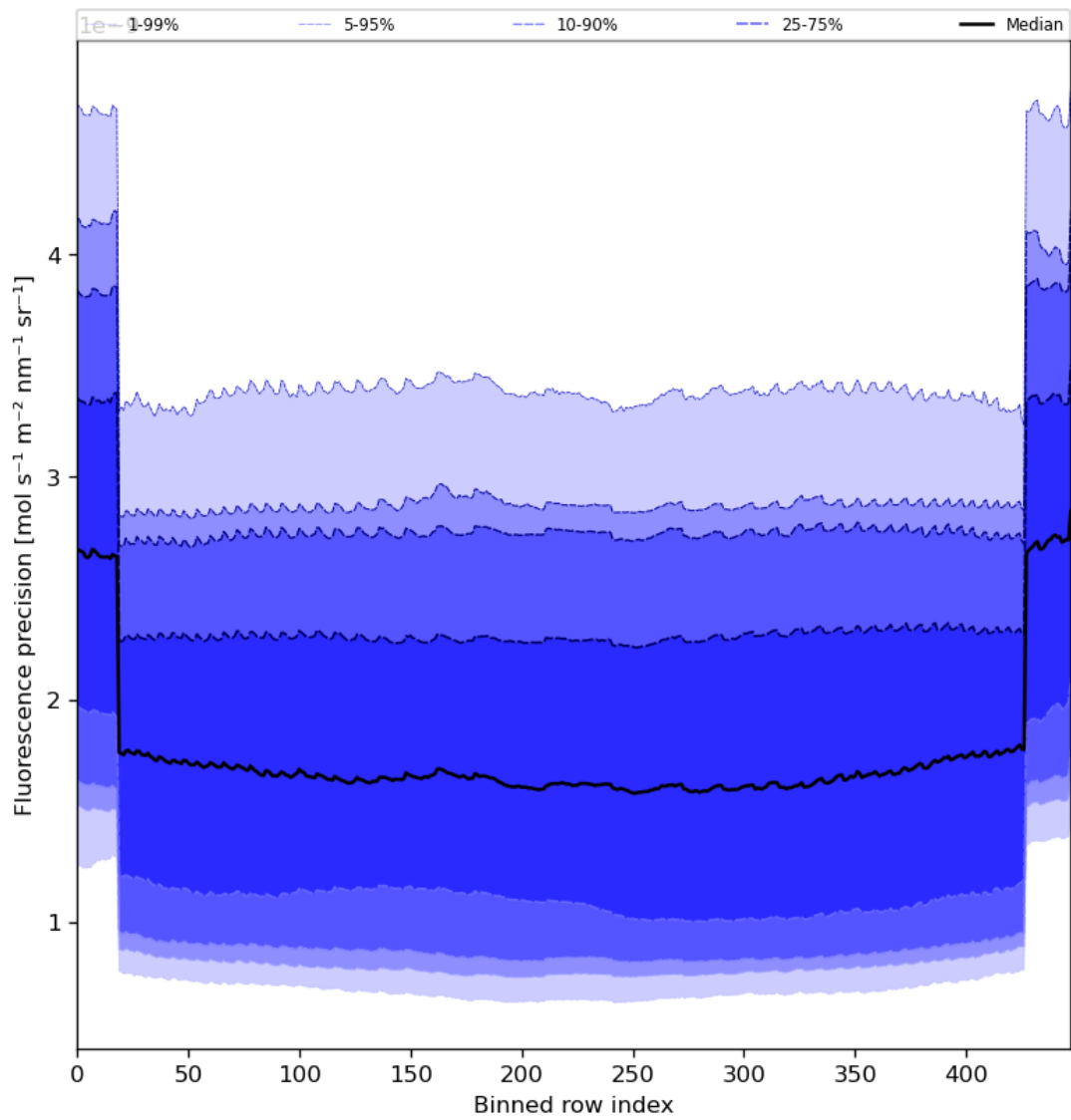
Figure 58: Along track statistics of “Fluorescence precision” for 2024-05-14 to 2024-05-16
