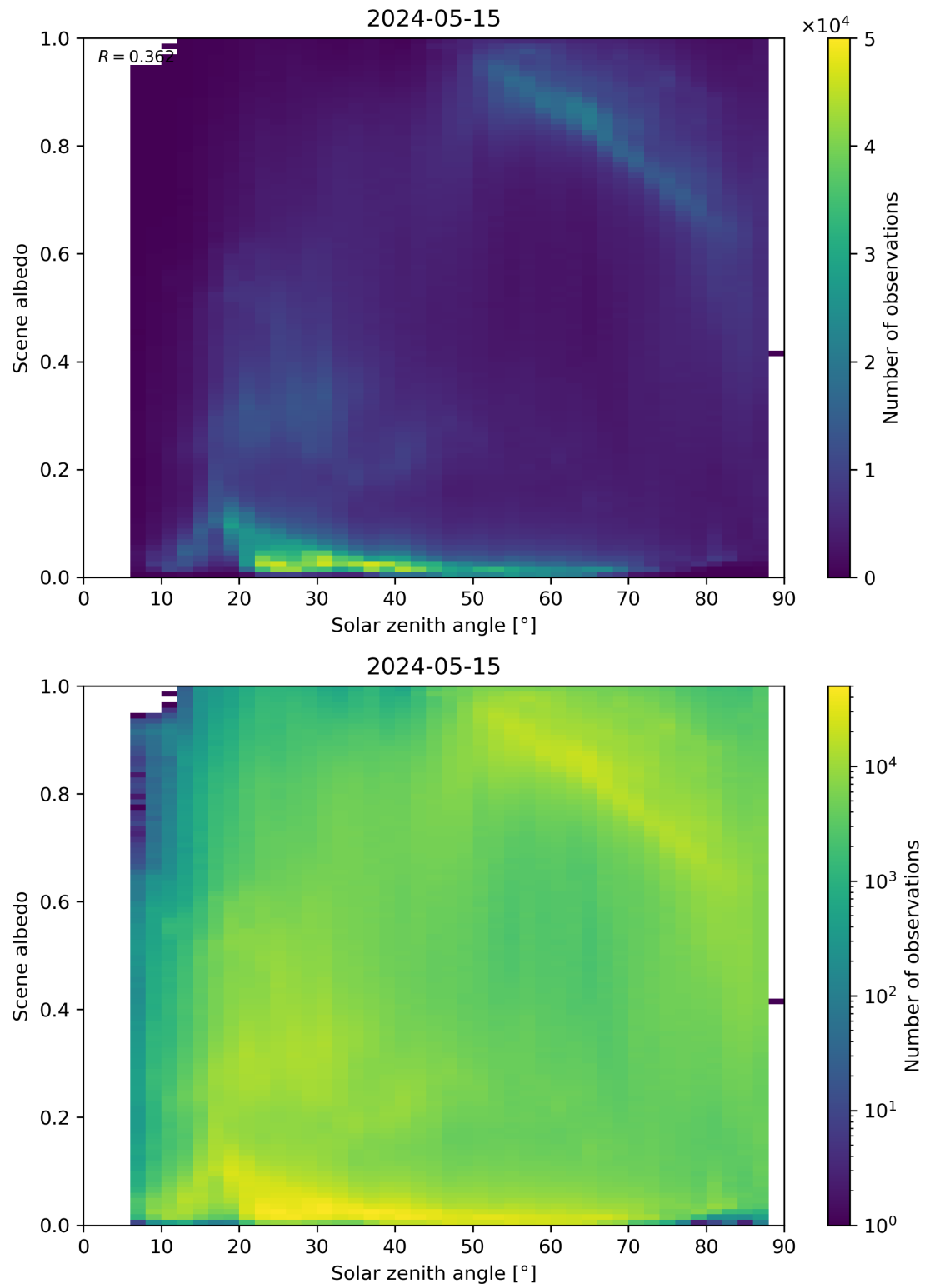
Figure 116: Scatter density plot of “Solar zenith angle” against “Scene albedo” for 2024-05-14 to 2024-05-16.
