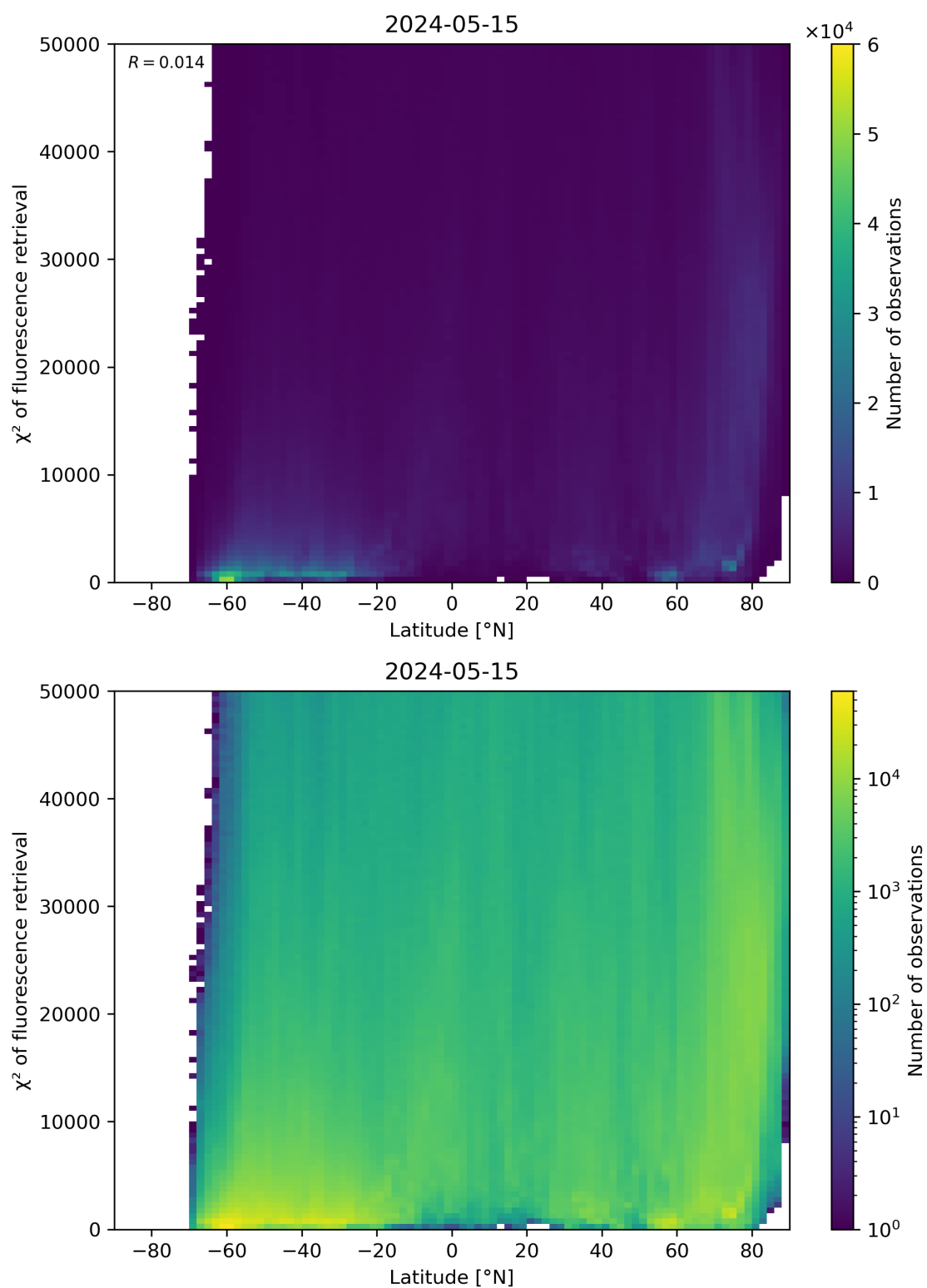
Figure 89: Scatter density plot of “Latitude” against “ \chi^2 of fluorescence retrieval” for 2024-05-14 to 2024-05-16.
