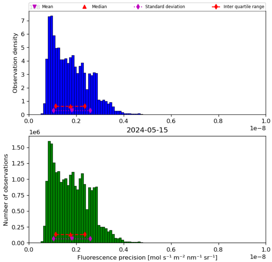
Figure 41: Histogram of “Fluorescence precision” for 2024-05-14 to 2024-05-16
