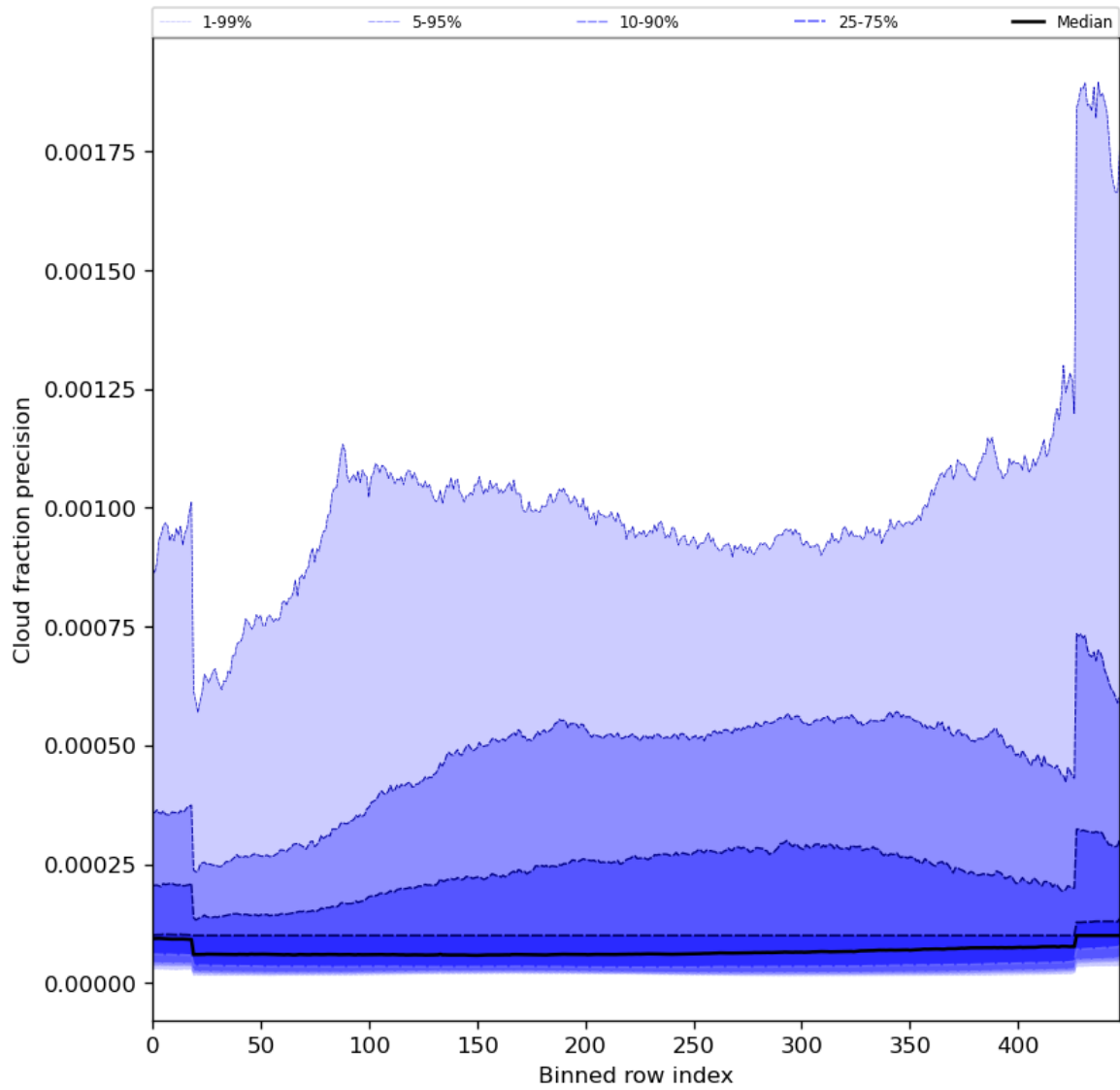
Figure 50: Along track statistics of “Cloud fraction precision” for 2024-05-14 to 2024-05-16
