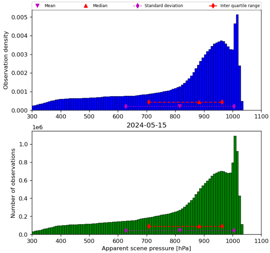
Figure 36: Histogram of “Apparent scene pressure” for 2024-05-14 to 2024-05-16
