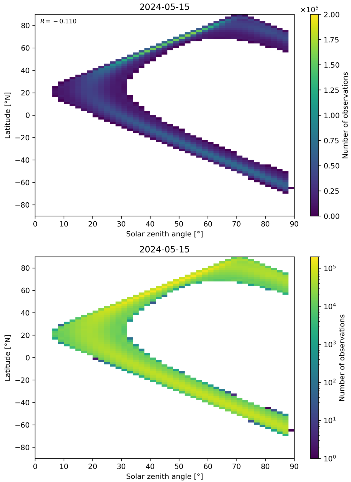
Figure 113: Scatter density plot of “Solar zenith angle” against “Latitude” for 2024-05-14 to 2024-05-16.
