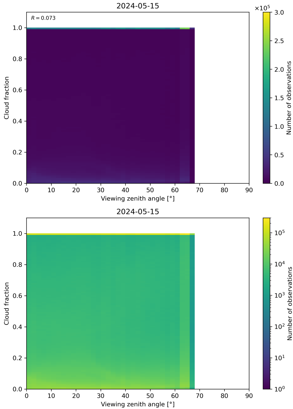
Figure 120: Scatter density plot of “Viewing zenith angle” against “Cloud fraction” for 2024-05-14 to 2024-05-16.
