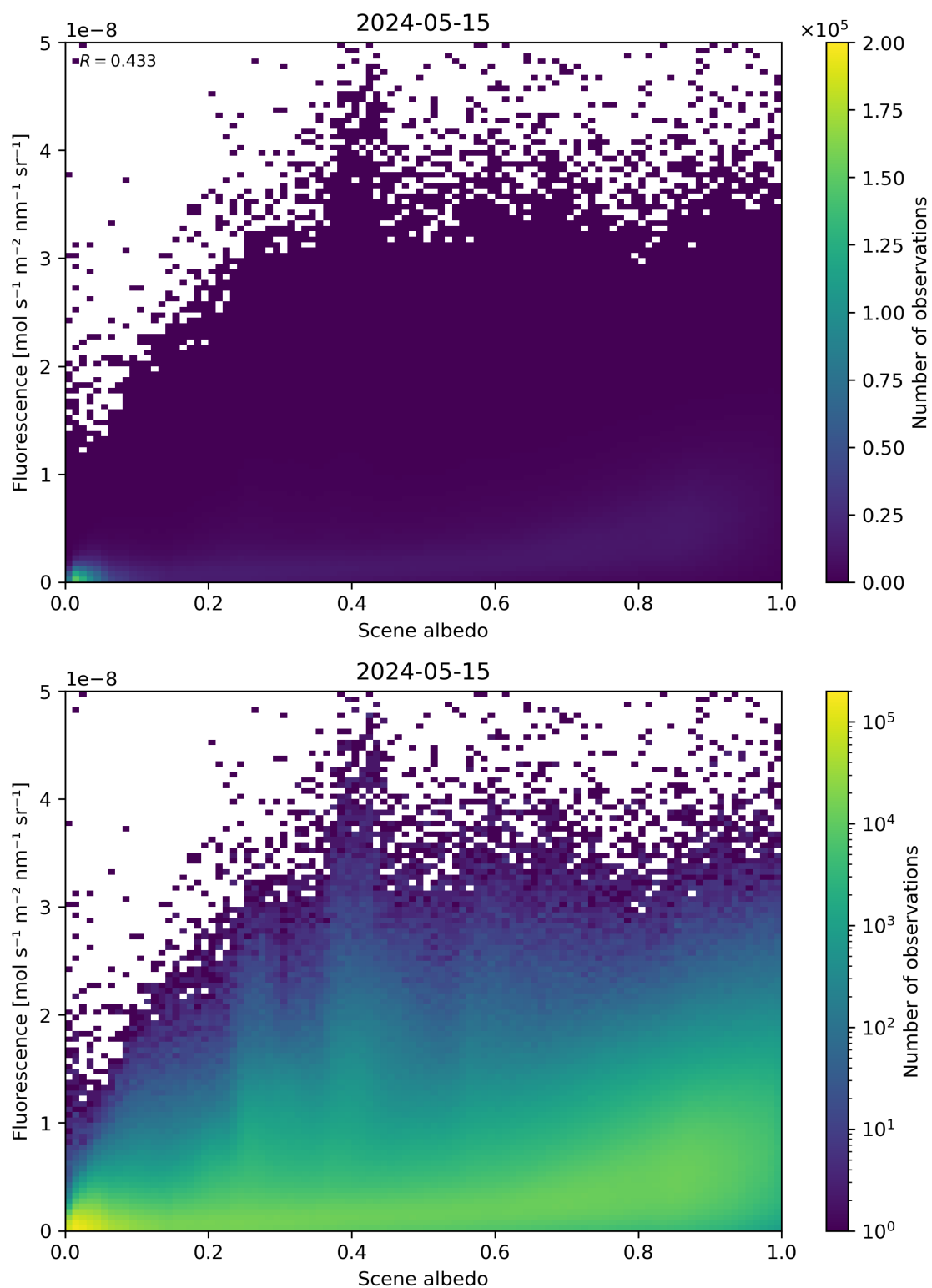
Figure 104: Scatter density plot of “Scene albedo” against “Fluorescence” for 2024-05-14 to 2024-05-16.
