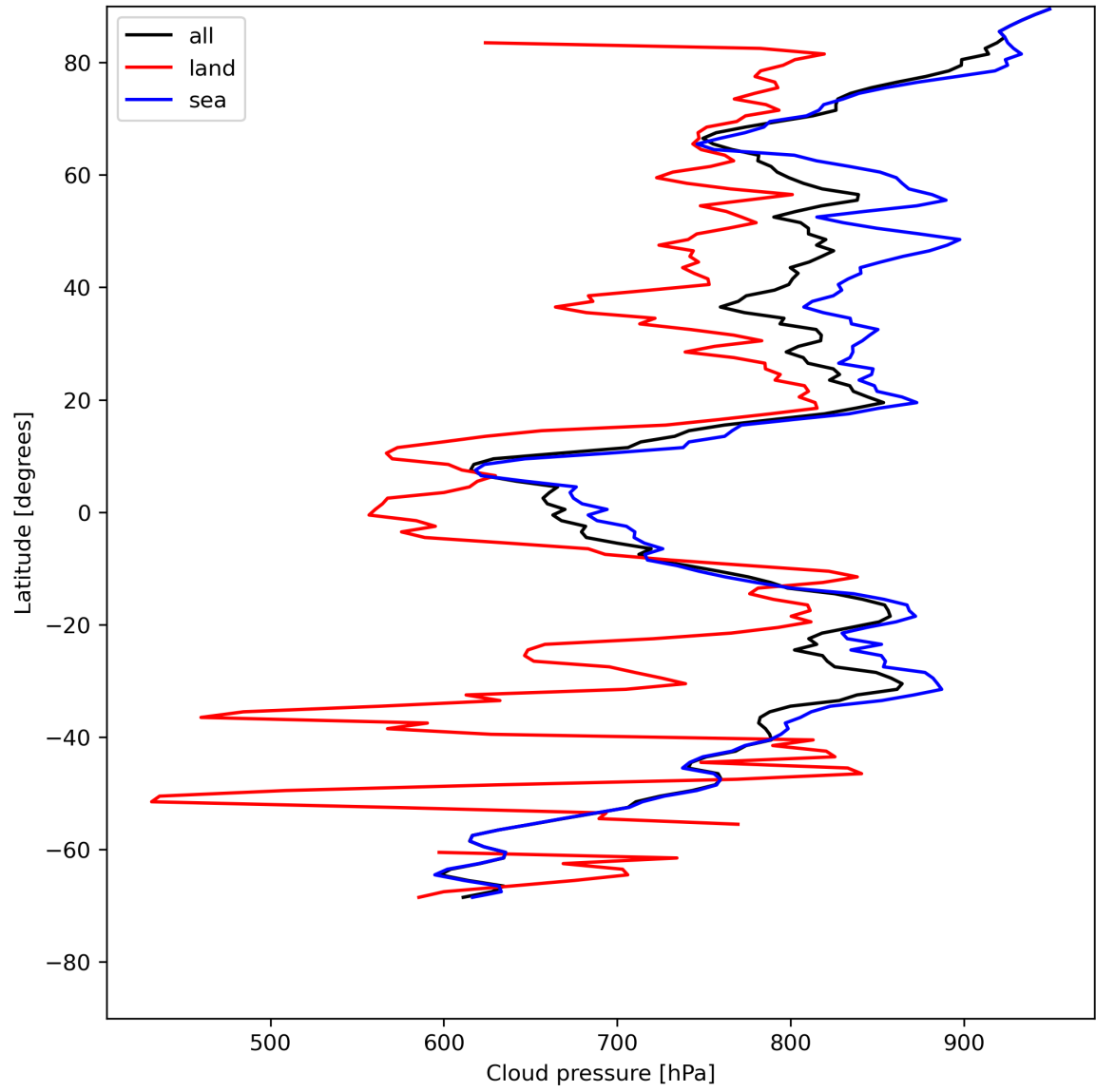
Figure 13: Zonal average of “Cloud pressure” for 2024-05-14 to 2024-05-16.
