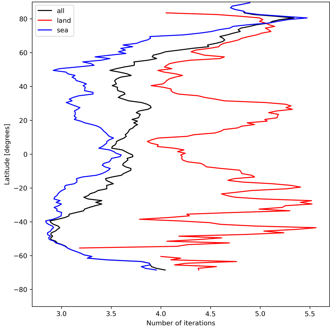
Figure 22: Zonal average of “Number of iterations” for 2024-05-14 to 2024-05-16.
