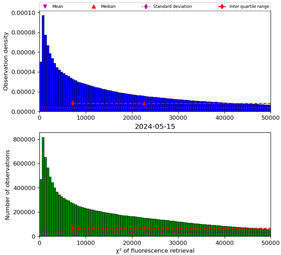
Figure 42: Histogram of “ \chi^2 of fluorescence retrieval” for 2024-05-14 to 2024-05-16
