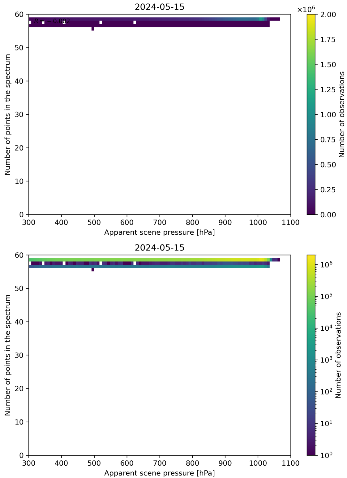
Figure 66: Scatter density plot of “Apparent scene pressure” against “Number of points in the spectrum” for 2024-05-14 to 2024-05-16.
