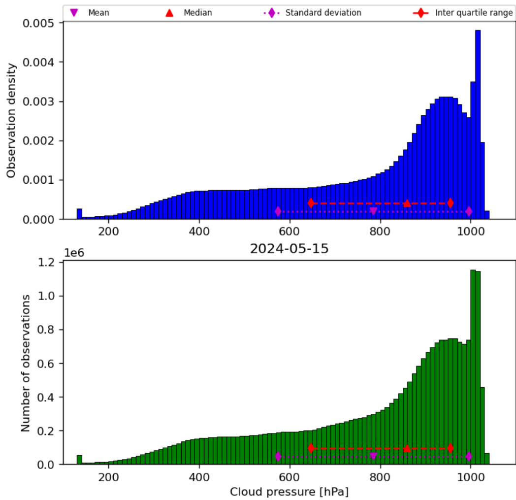
Figure 30: Histogram of “Cloud pressure” for 2024-05-14 to 2024-05-16
