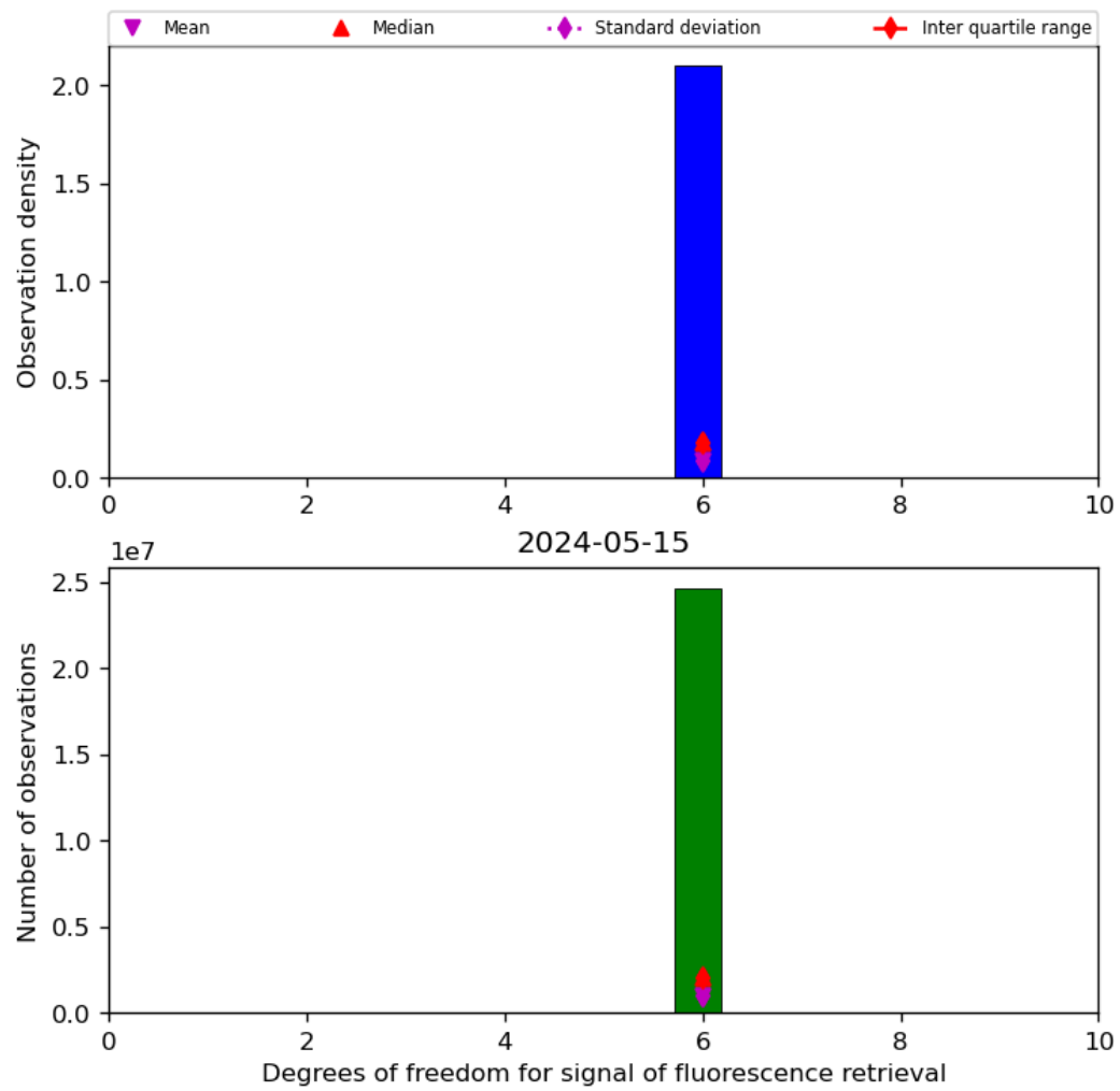
Figure 43: Histogram of “Degrees of freedom for signal of fluorescence retrieval” for 2024-05-14 to 2024-05-16
