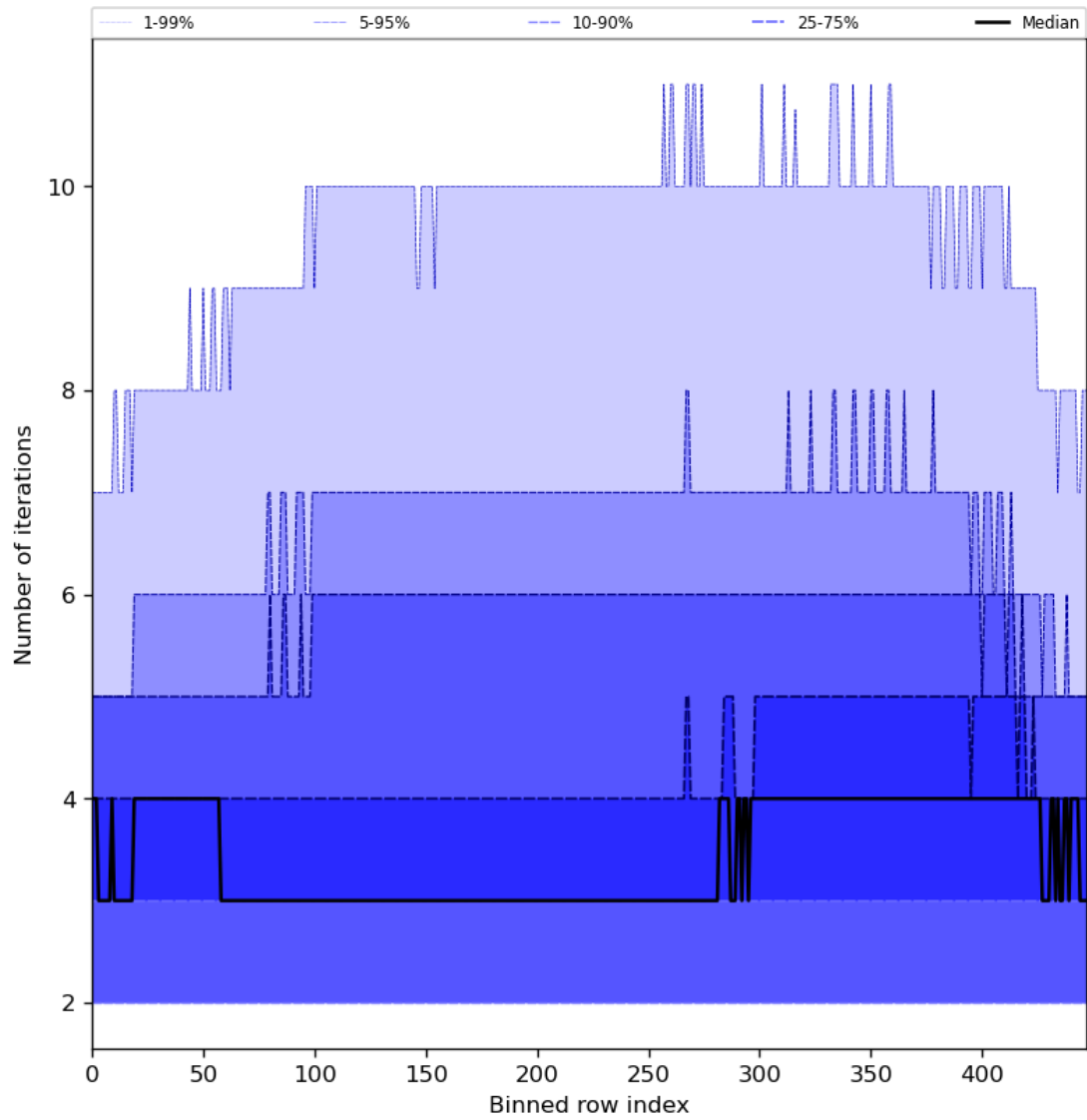
Figure 56: Along track statistics of “Number of iterations” for 2024-05-14 to 2024-05-16
