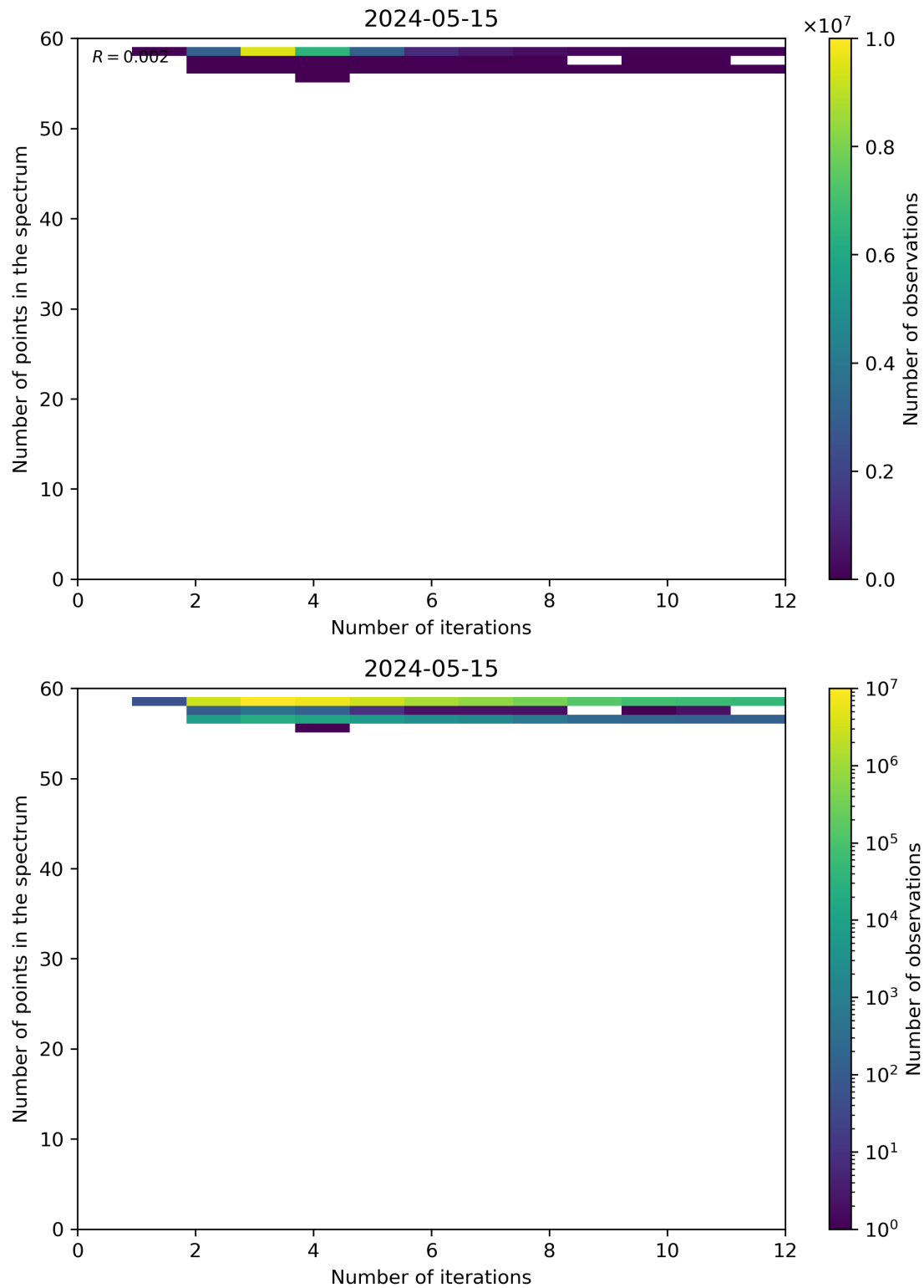
Figure 99: Scatter density plot of “Number of iterations” against “Number of points in the spectrum” for 2024-05-14 to 2024-05-16.
