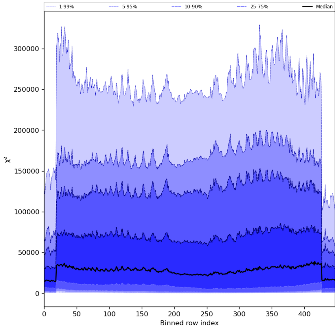
Figure 55: Along track statistics of “ \chi^2 ” for 2024-05-14 to 2024-05-16
