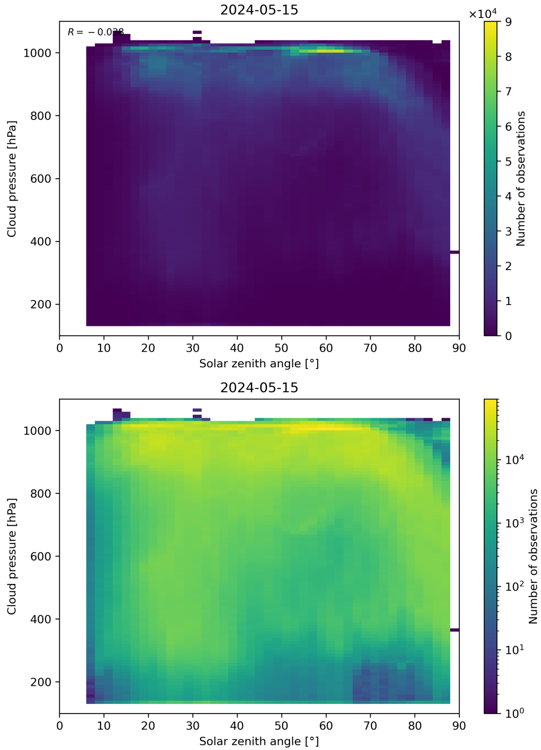
Figure 111: Scatter density plot of “Solar zenith angle” against “Cloud pressure” for 2024-05-14 to 2024-05-16.
