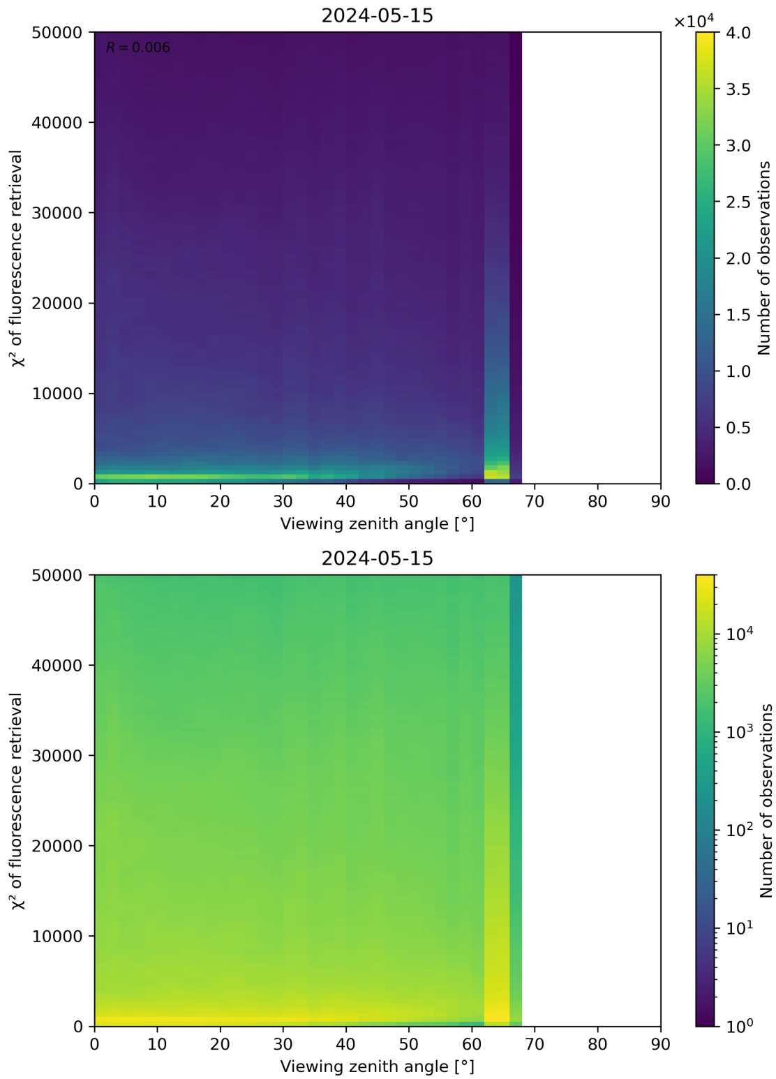
Figure 119: Scatter density plot of “Viewing zenith angle” against “ \chi^2 of fluorescence retrieval” for 2024-05-14 to 2024-05-16.
