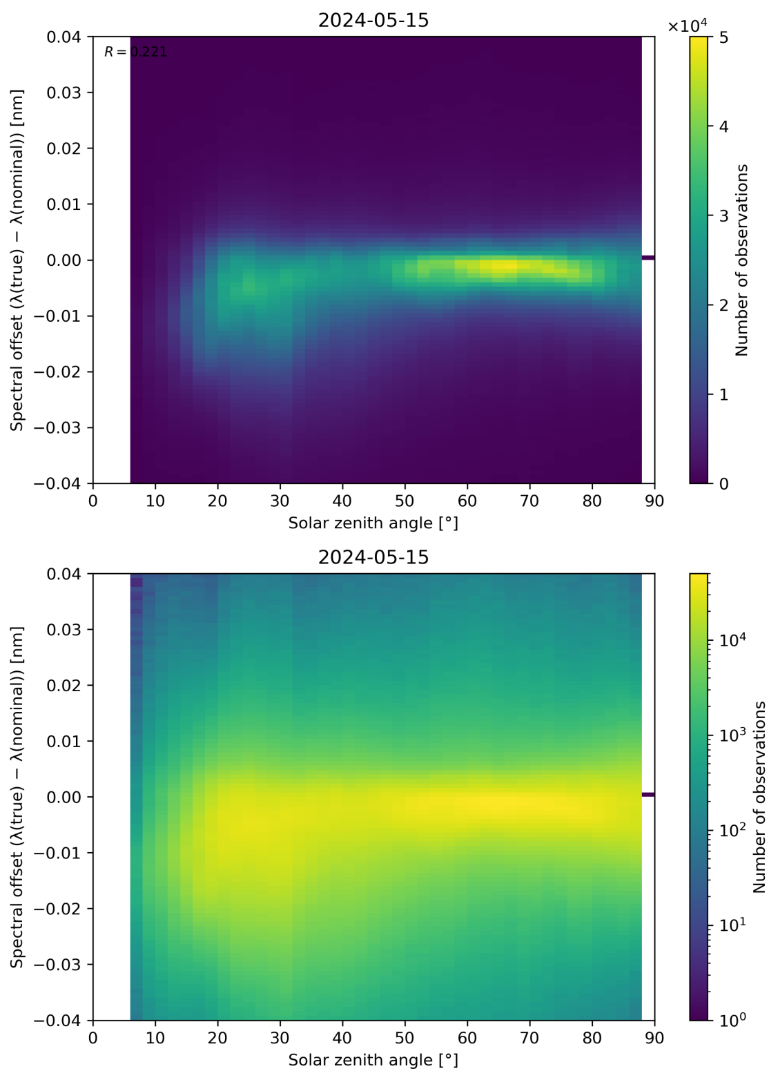
Figure 117: Scatter density plot of “Solar zenith angle” against “Spectral offset ( \lambda(\text{true}) - \lambda(\text{nominal}) )” for 2024-05-14 to 2024-05-16.
