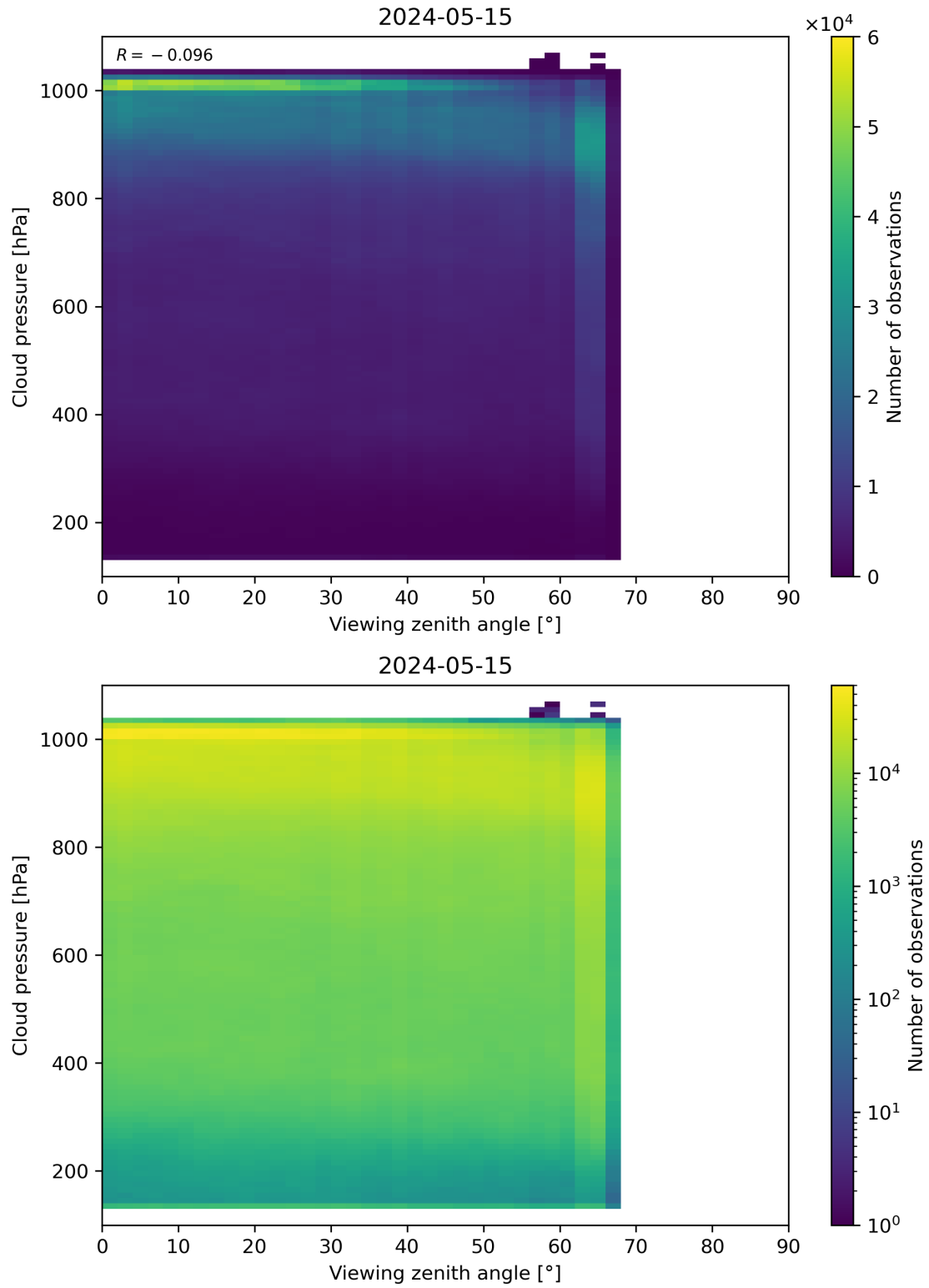
Figure 121: Scatter density plot of “Viewing zenith angle” against “Cloud pressure” for 2024-05-14 to 2024-05-16.
