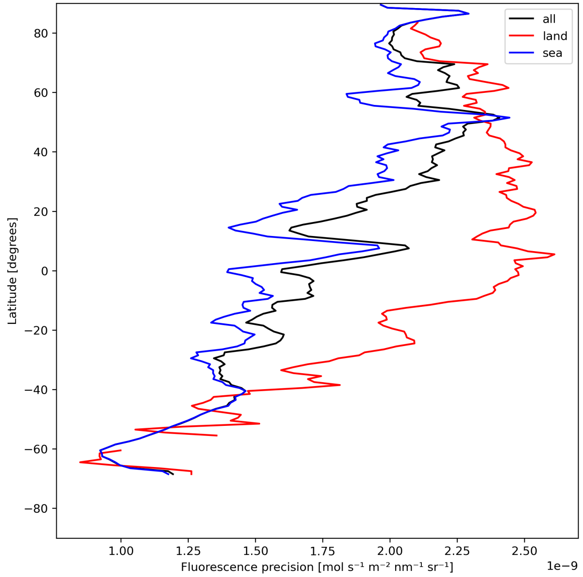
Figure 24: Zonal average of “Fluorescence precision” for 2024-05-14 to 2024-05-16.
