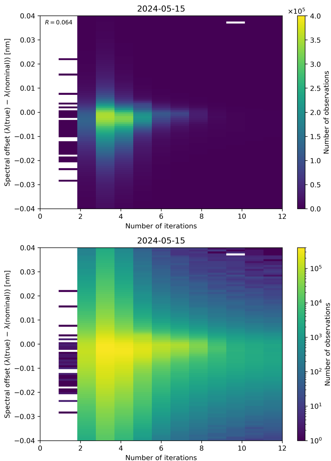
Figure 100: Scatter density plot of “Number of iterations” against “Spectral offset ( \lambda(\text{true}) - \lambda(\text{nominal}) )” for 2024-05-14 to 2024-05-16.
