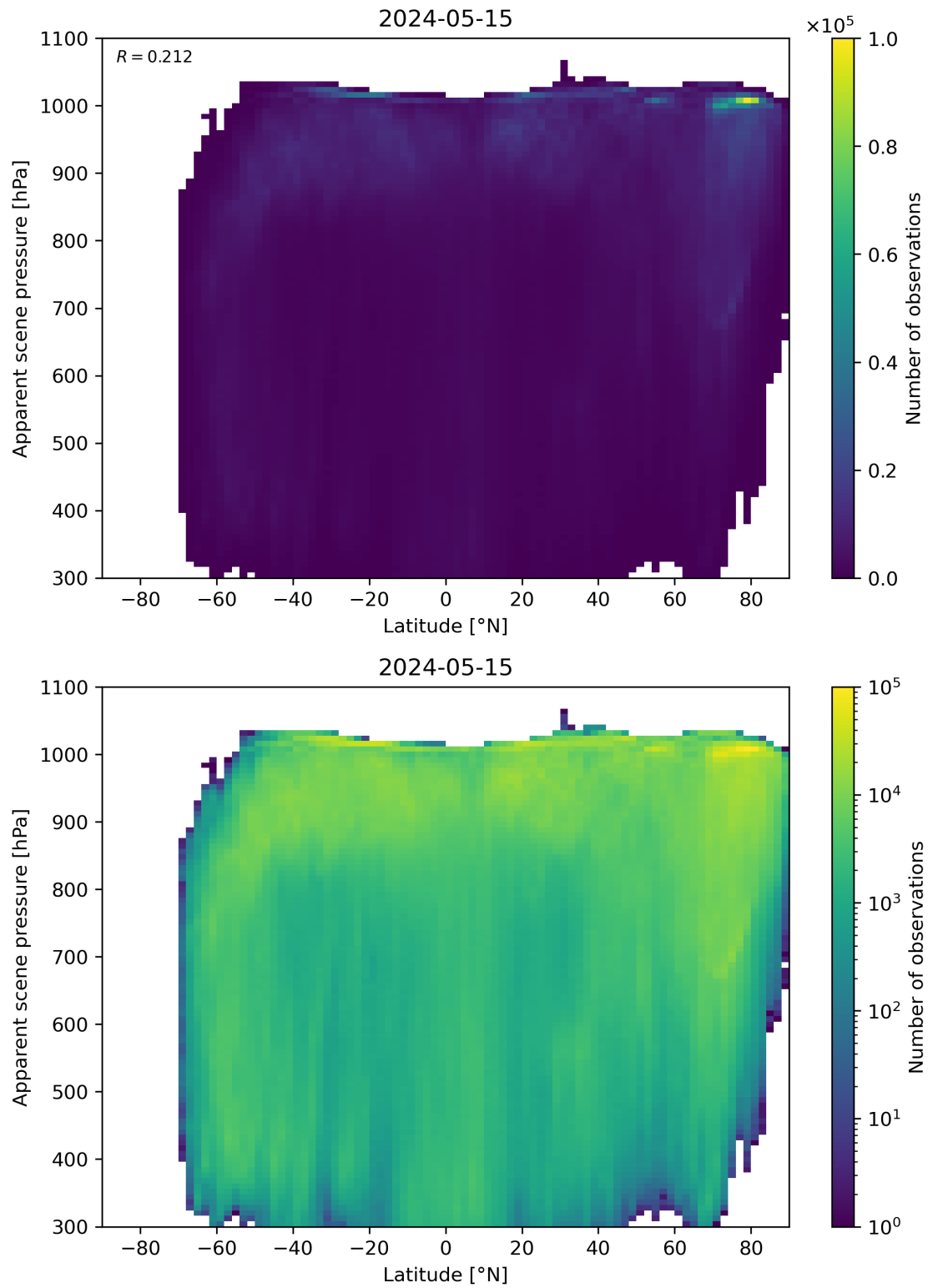
Figure 88: Scatter density plot of “Latitude” against “Apparent scene pressure” for 2024-05-14 to 2024-05-16.
