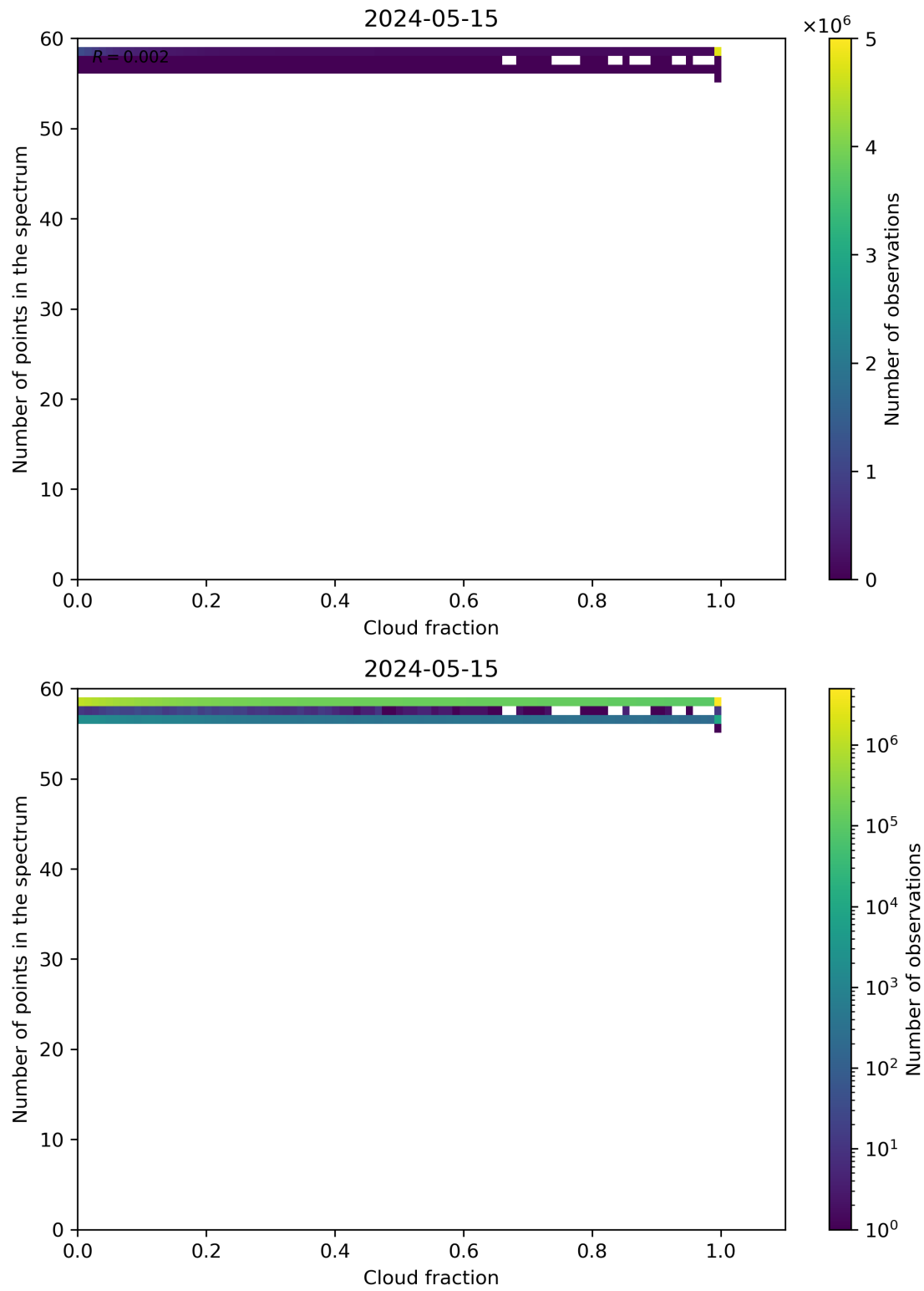
Figure 74: Scatter density plot of “Cloud fraction” against “Number of points in the spectrum” for 2024-05-14 to 2024-05-16.
