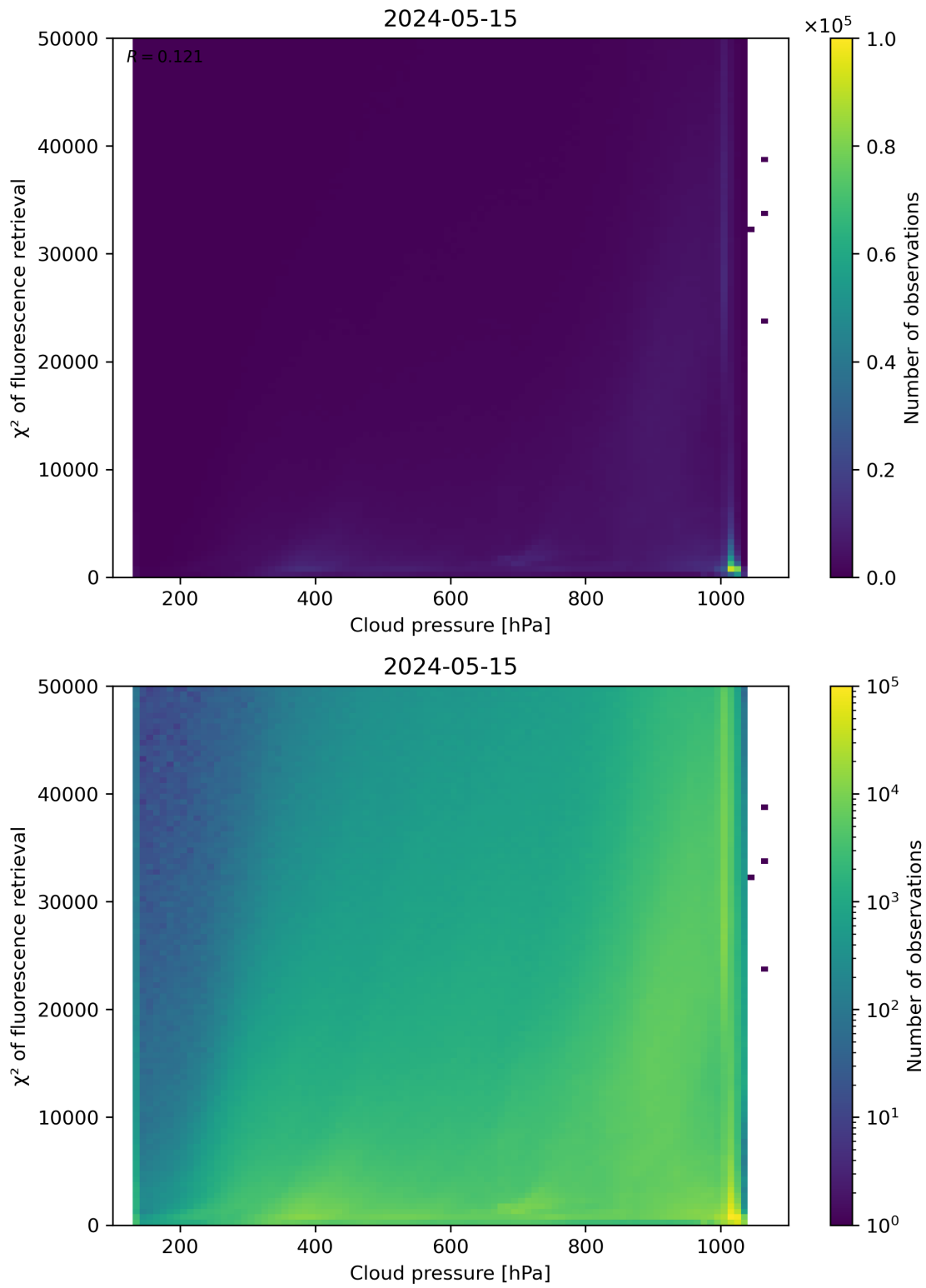
Figure 78: Scatter density plot of “Cloud pressure” against “ \chi^2 of fluorescence retrieval” for 2024-05-14 to 2024-05-16.
