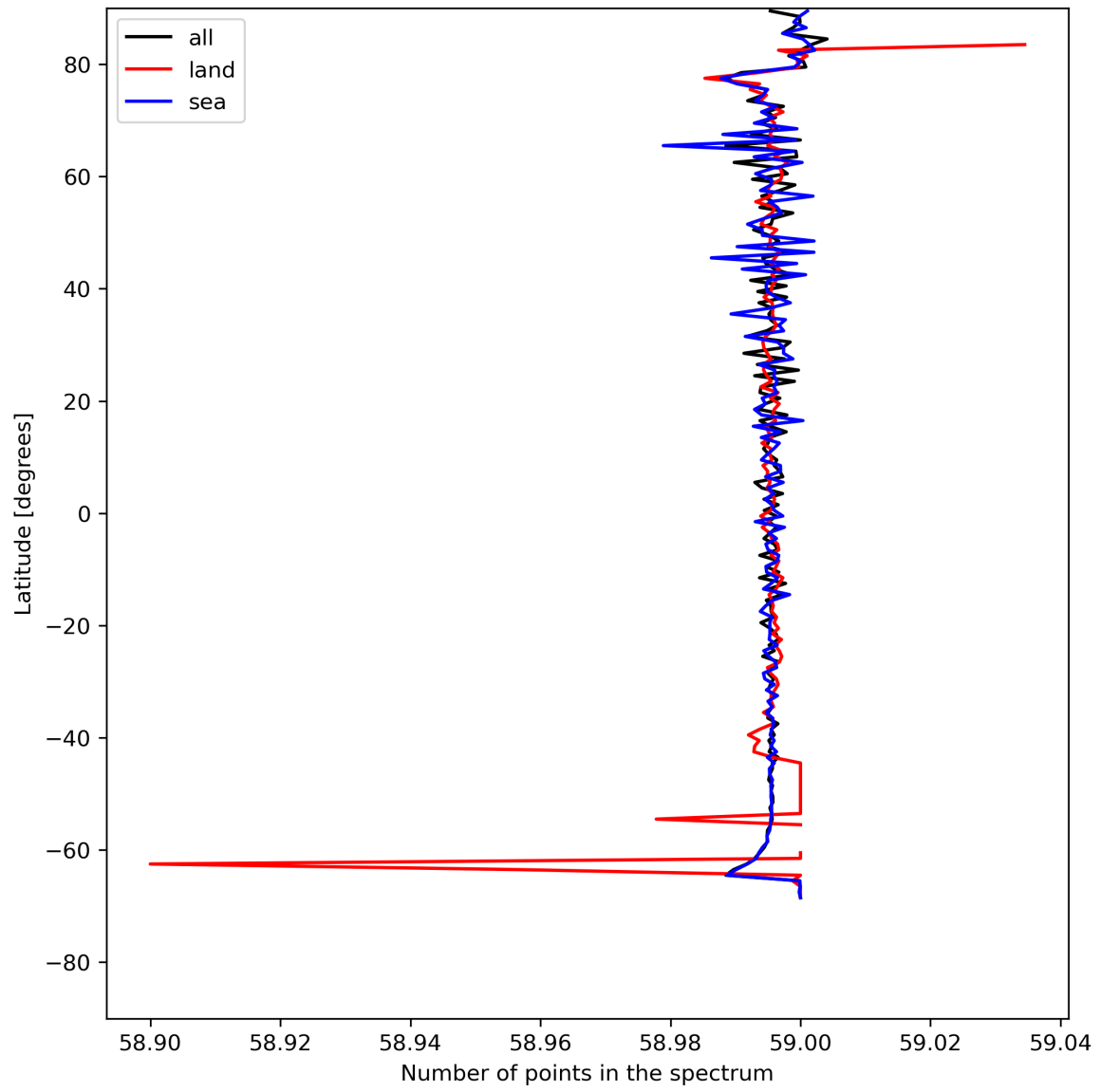
Figure 27: Zonal average of “Number of points in the spectrum” for 2024-05-14 to 2024-05-16.
