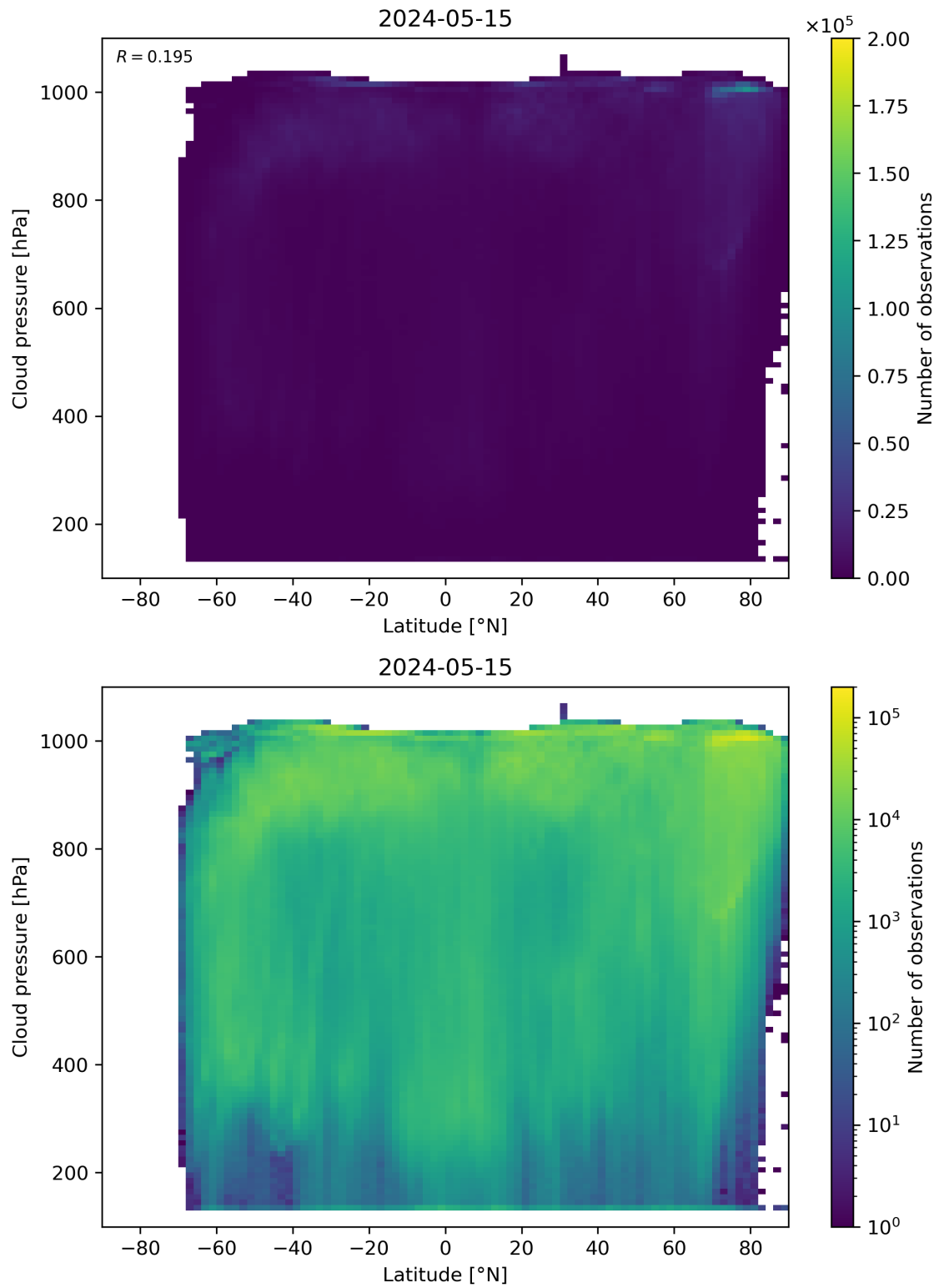
Figure 91: Scatter density plot of “Latitude” against “Cloud pressure” for 2024-05-14 to 2024-05-16.
