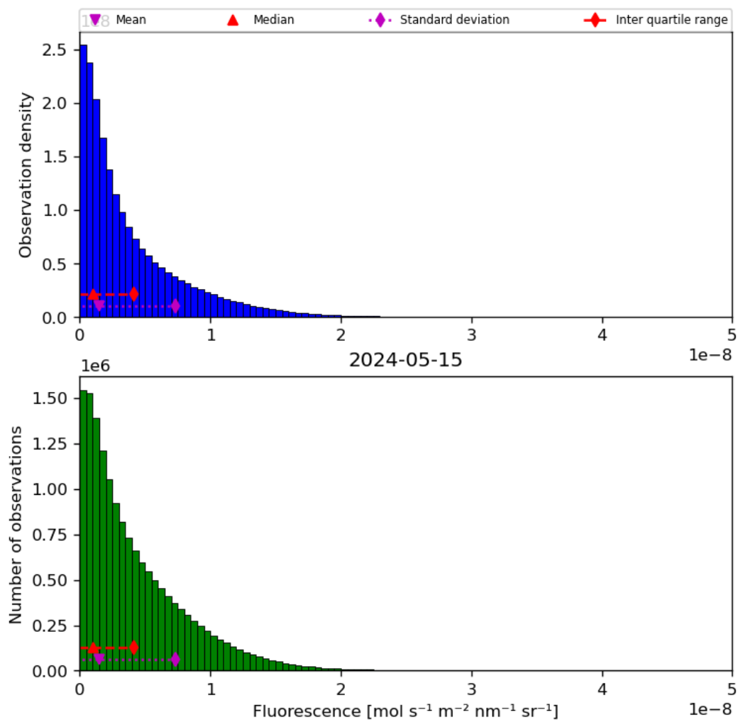
Figure 40: Histogram of “Fluorescence” for 2024-05-14 to 2024-05-16
