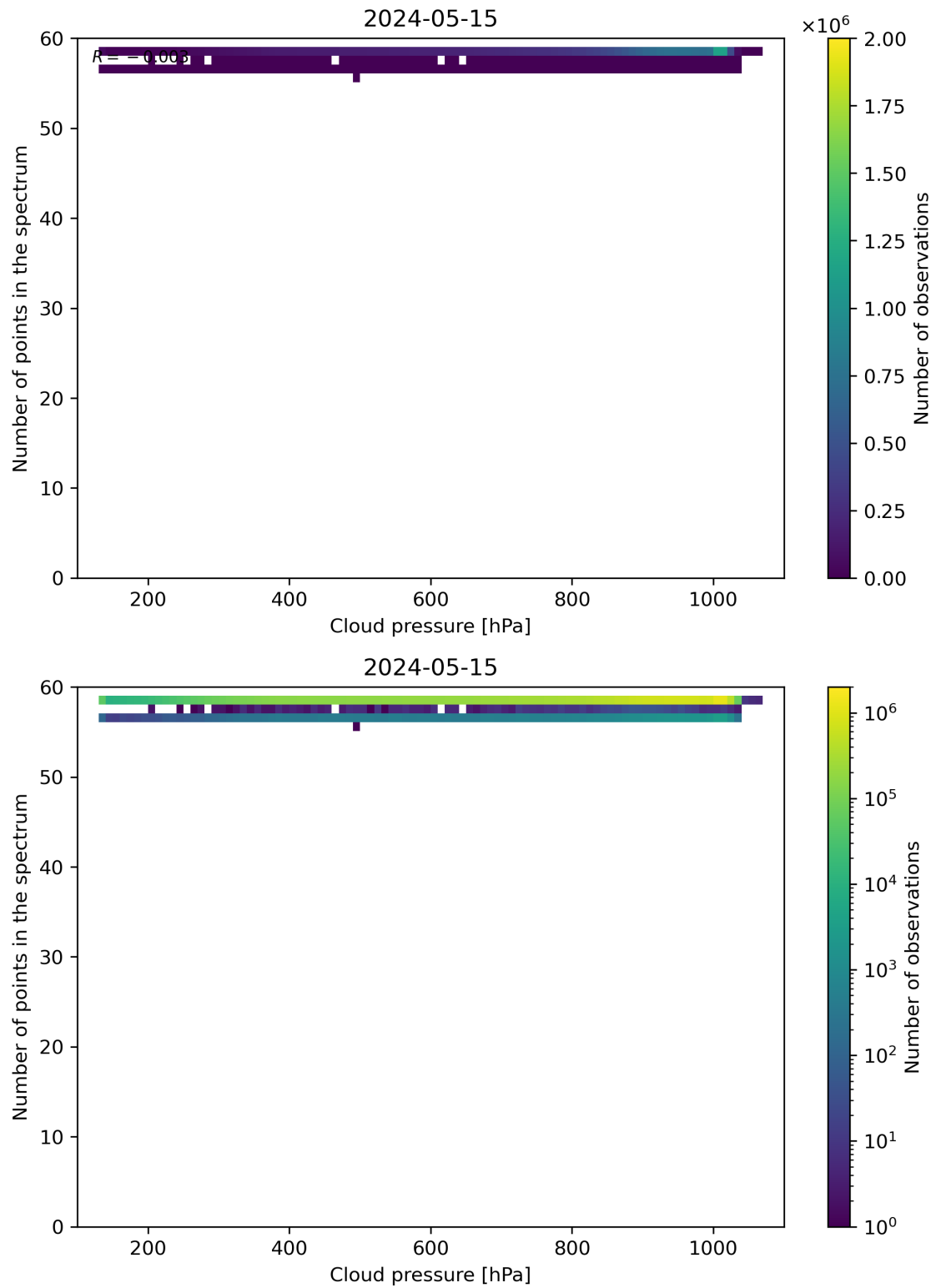
Figure 82: Scatter density plot of “Cloud pressure” against “Number of points in the spectrum” for 2024-05-14 to 2024-05-16.
