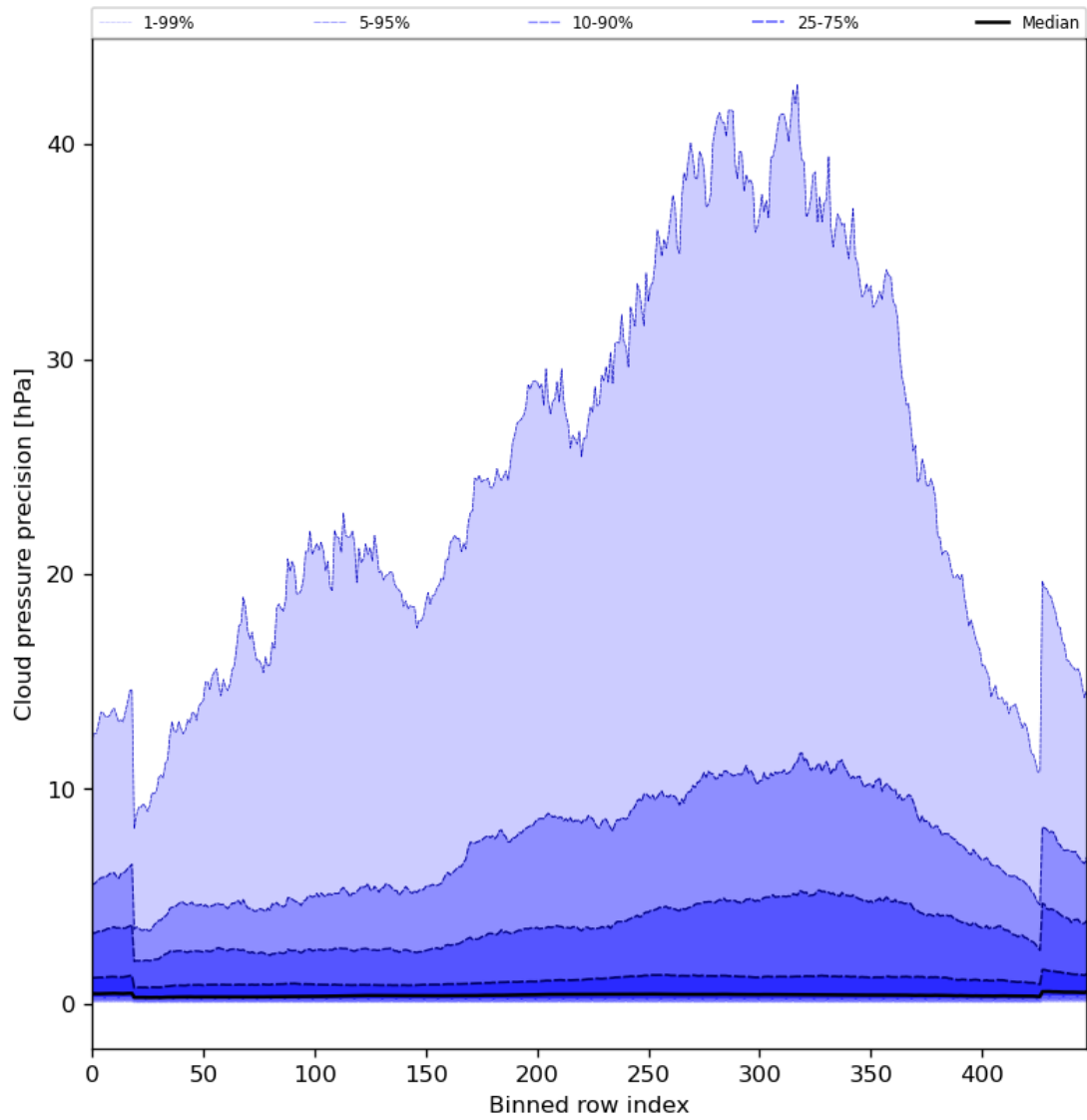
Figure 48: Along track statistics of “Cloud pressure precision” for 2024-05-14 to 2024-05-16
