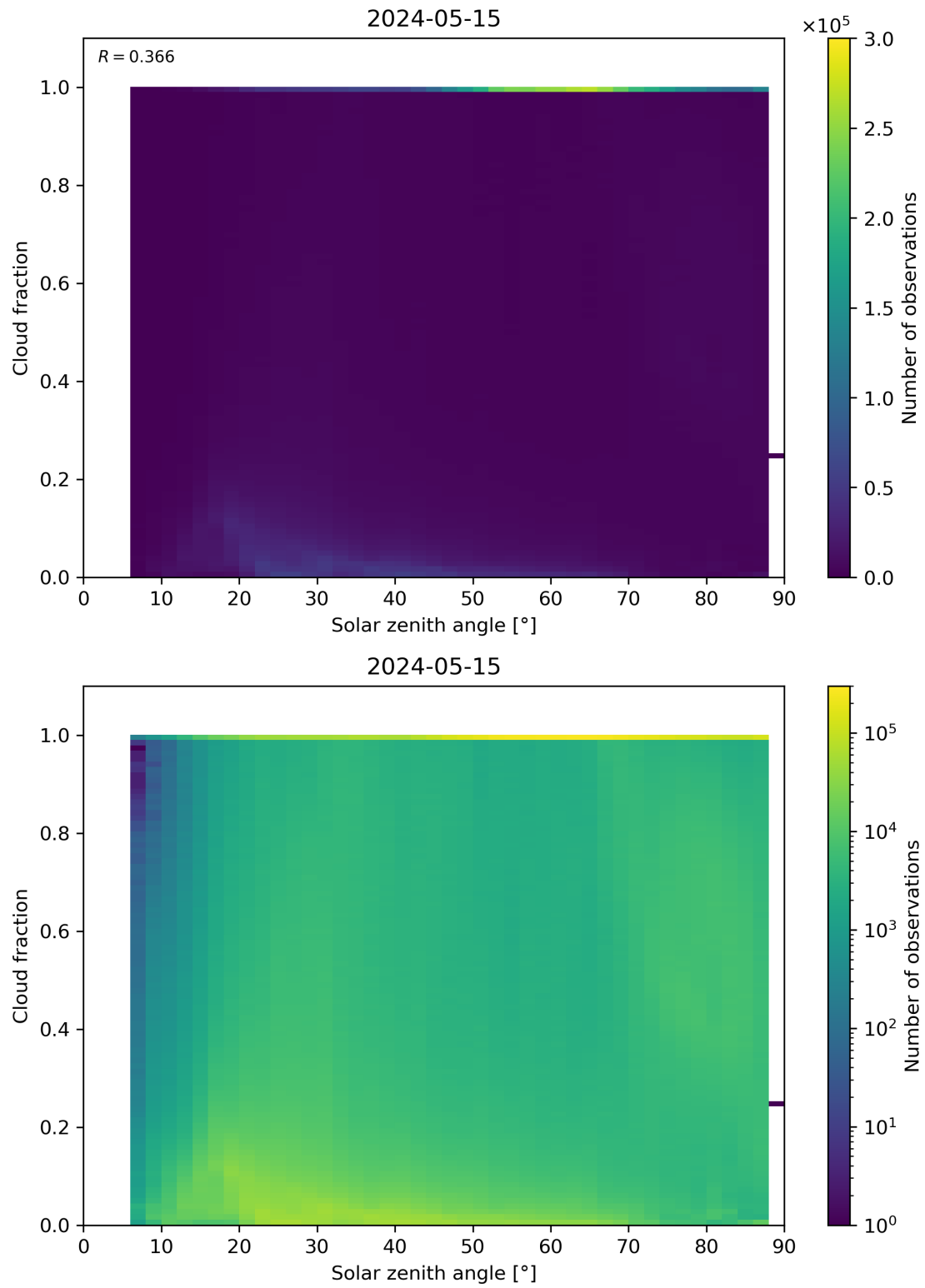
Figure 110: Scatter density plot of “Solar zenith angle” against “Cloud fraction” for 2024-05-14 to 2024-05-16.
