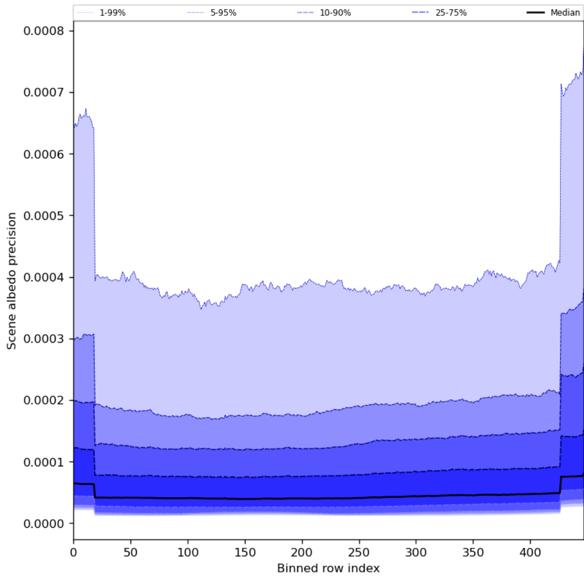
Figure 52: Along track statistics of “Scene albedo precision” for 2024-05-14 to 2024-05-16
