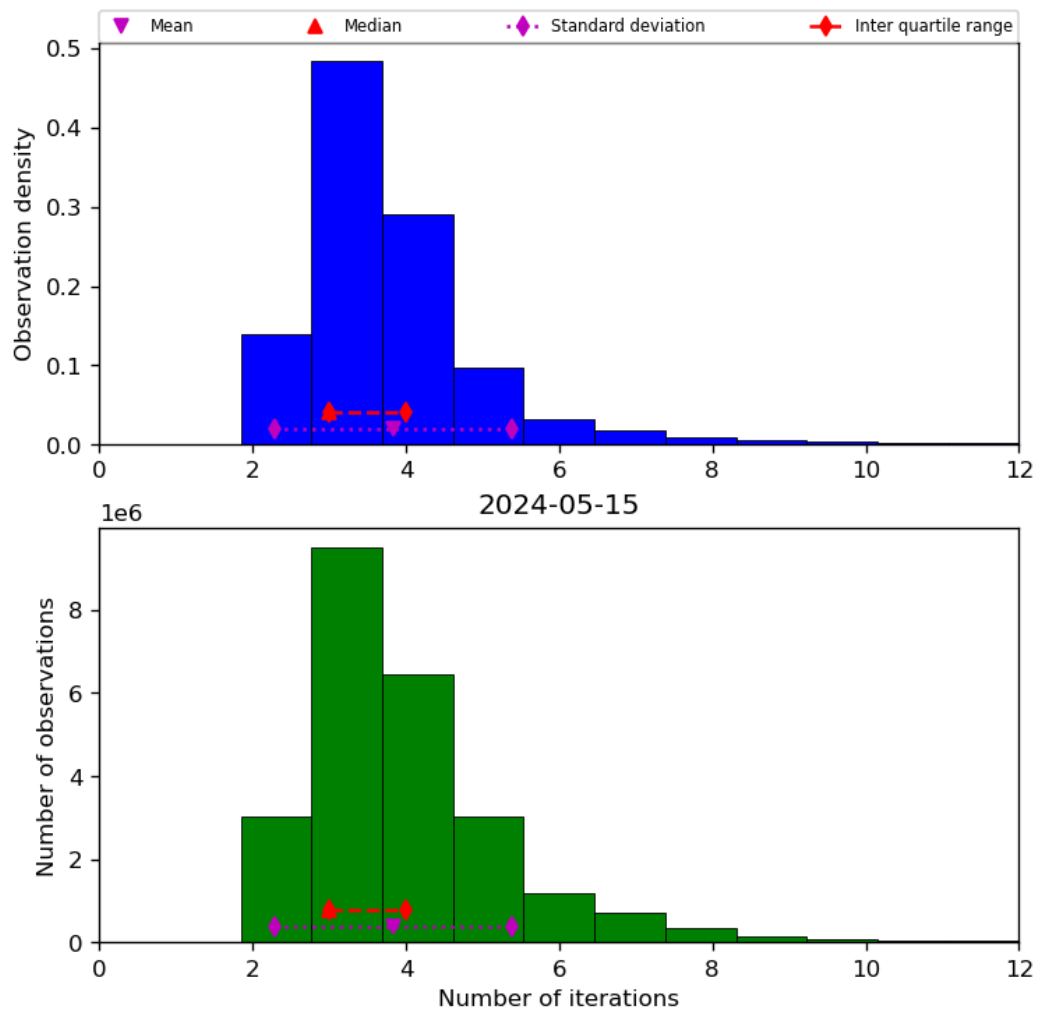
Figure 39: Histogram of “Number of iterations” for 2024-05-14 to 2024-05-16
