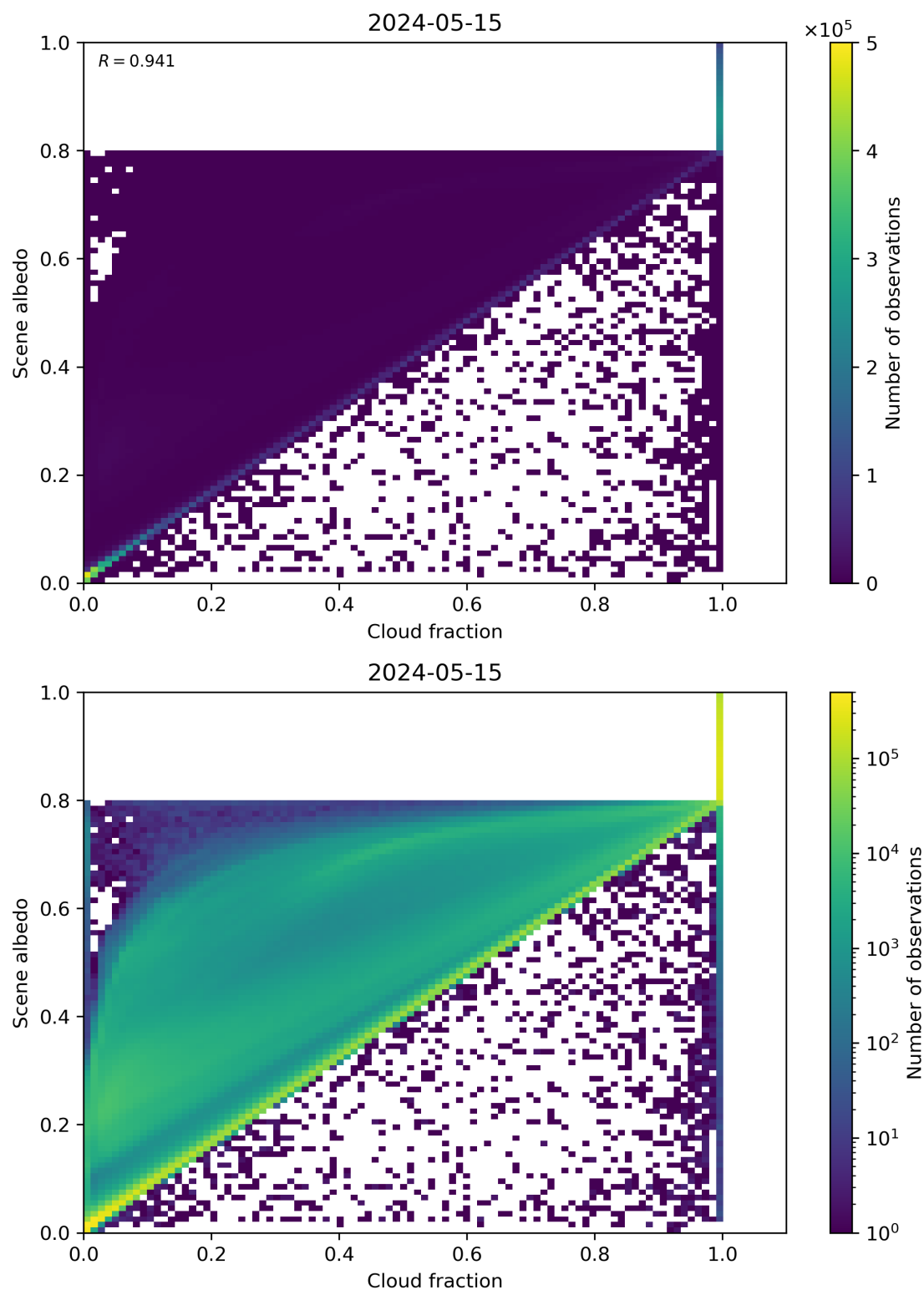
Figure 75: Scatter density plot of “Cloud fraction” against “Scene albedo” for 2024-05-14 to 2024-05-16.
