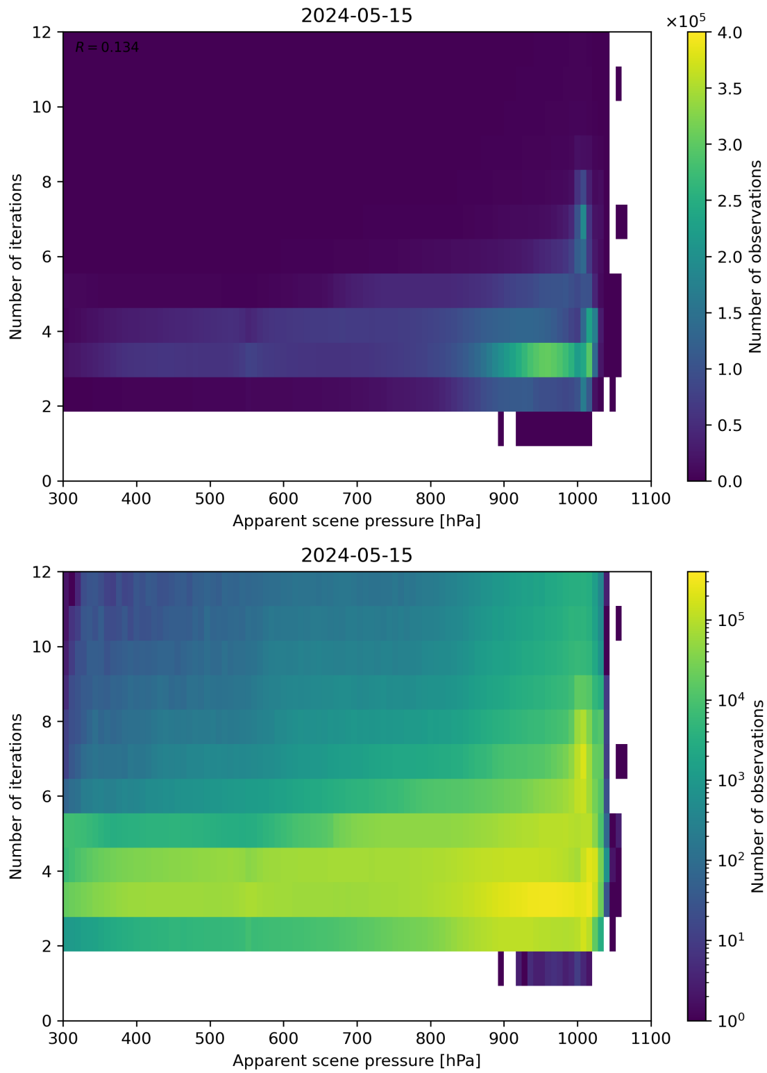
Figure 65: Scatter density plot of “Apparent scene pressure” against “Number of iterations” for 2024-05-14 to 2024-05-16.
