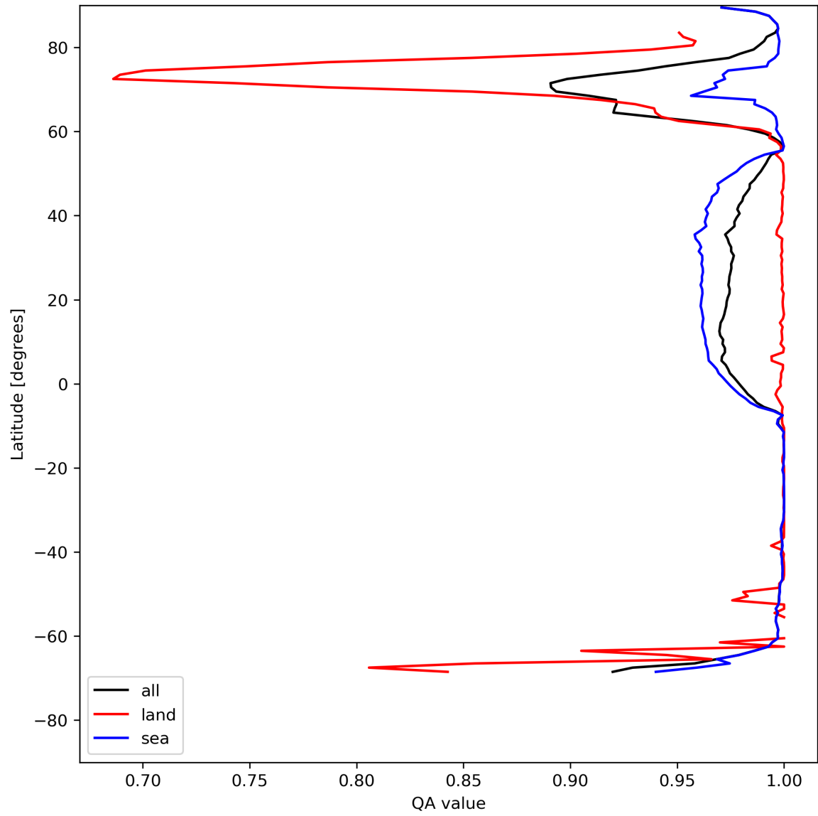
Figure 12: Zonal average of “QA value” for 2024-05-14 to 2024-05-16.
