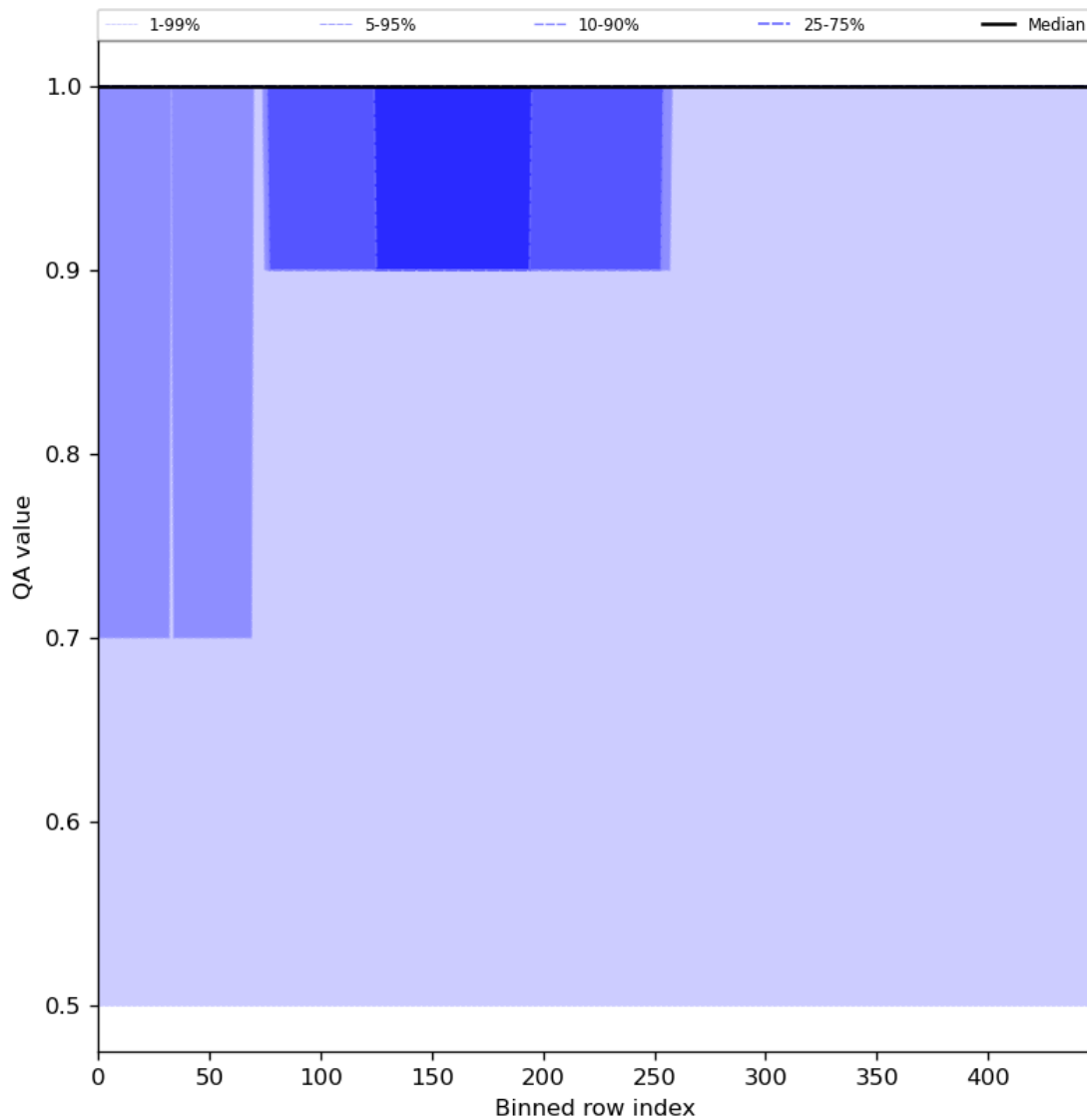
Figure 46: Along track statistics of “QA value” for 2024-05-14 to 2024-05-16
