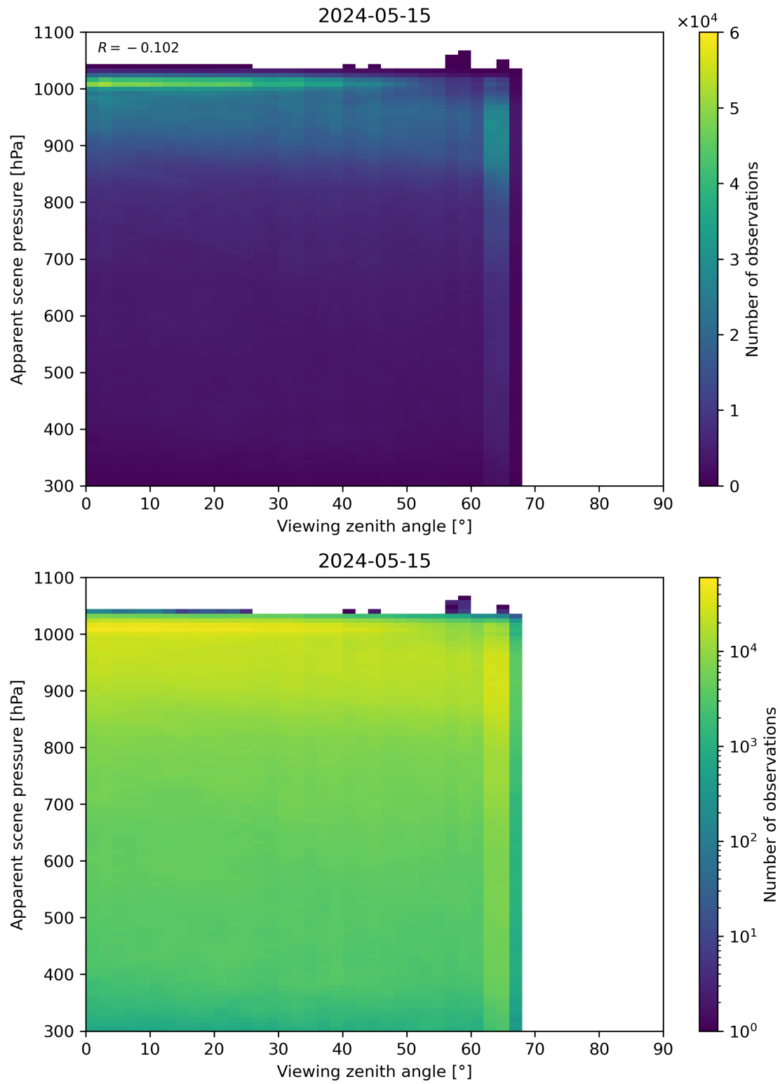
Figure 118: Scatter density plot of “Viewing zenith angle” against “Apparent scene pressure” for 2024-05-14 to 2024-05-16.
