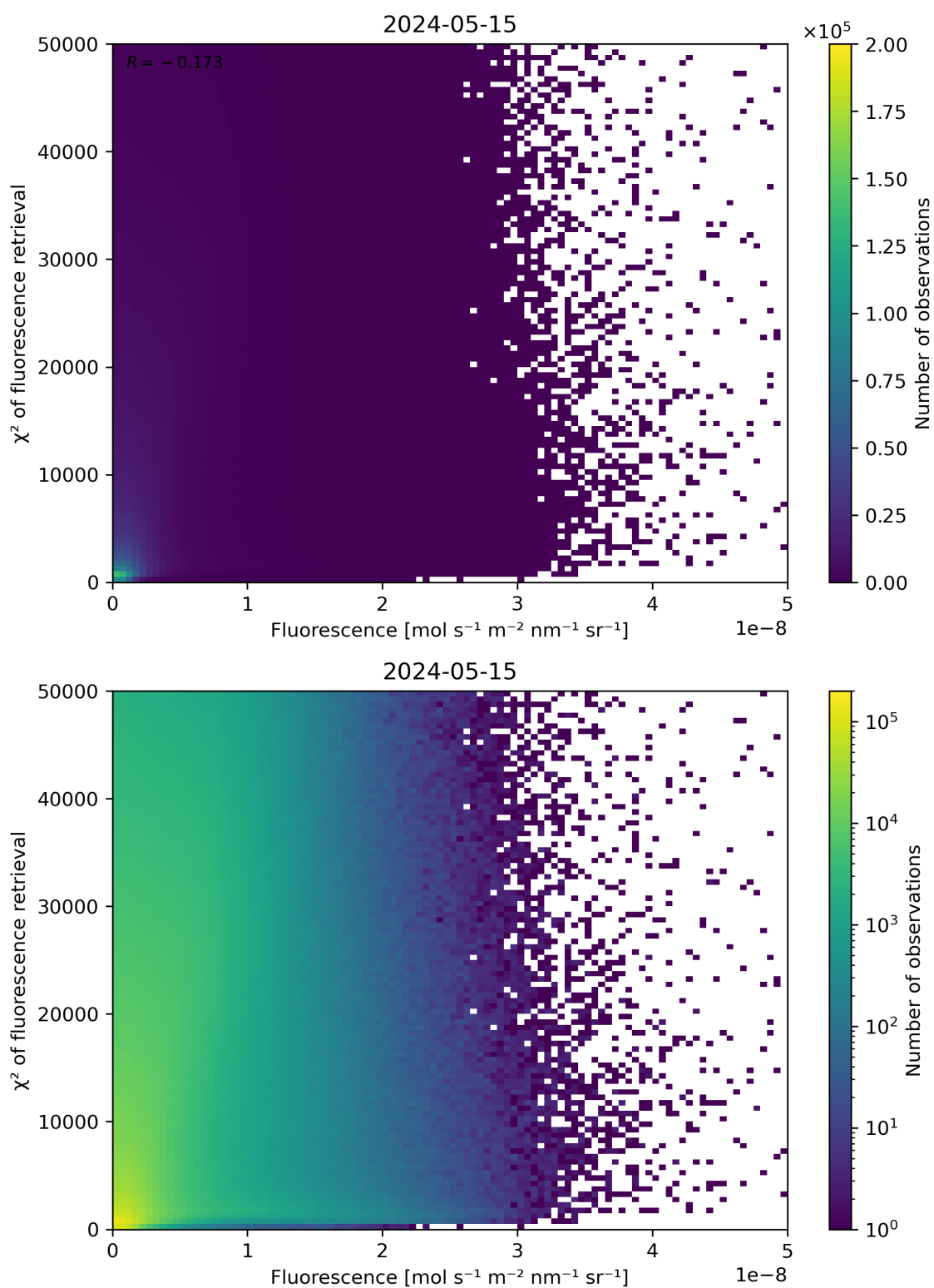
Figure 85: Scatter density plot of “Fluorescence” against “ \chi^2 of fluorescence retrieval” for 2024-05-14 to 2024-05-16.
