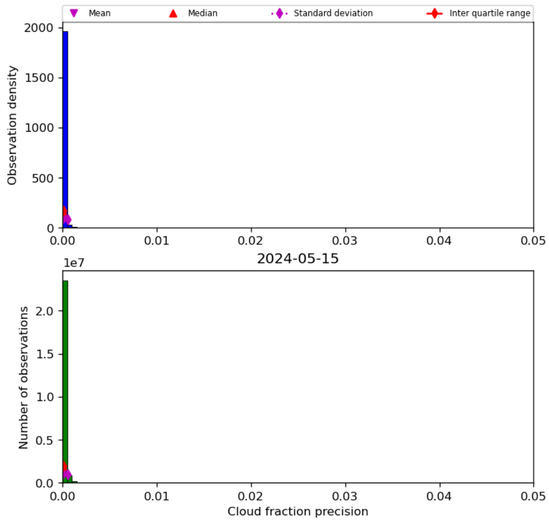
Figure 33: Histogram of “Cloud fraction precision” for 2024-05-14 to 2024-05-16
