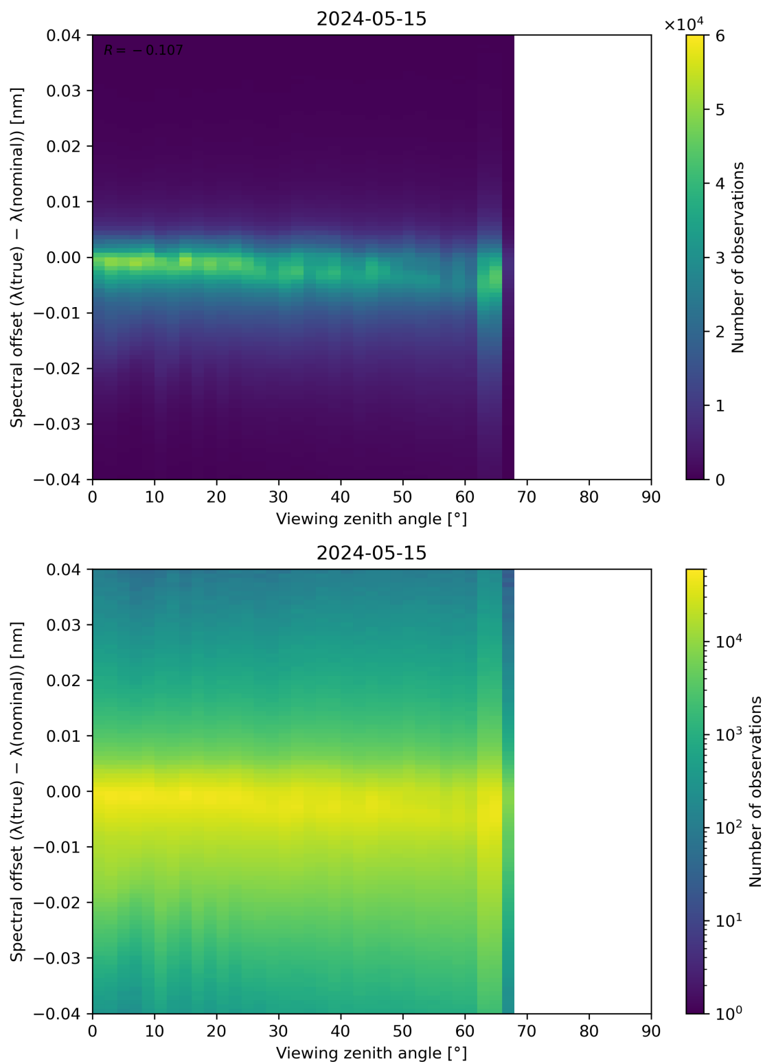
Figure 128: Scatter density plot of “Viewing zenith angle” against “Spectral offset ( \lambda(\text{true}) - \lambda(\text{nominal}) )” for 2024-05-14 to 2024-05-16.
