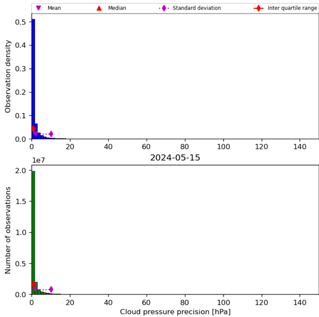
Figure 31: Histogram of “Cloud pressure precision” for 2024-05-14 to 2024-05-16
