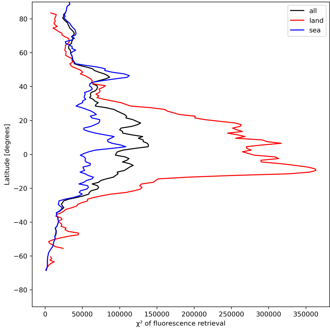
Figure 25: Zonal average of “ \chi^2 of fluorescence retrieval” for 2024-05-14 to 2024-05-16.
