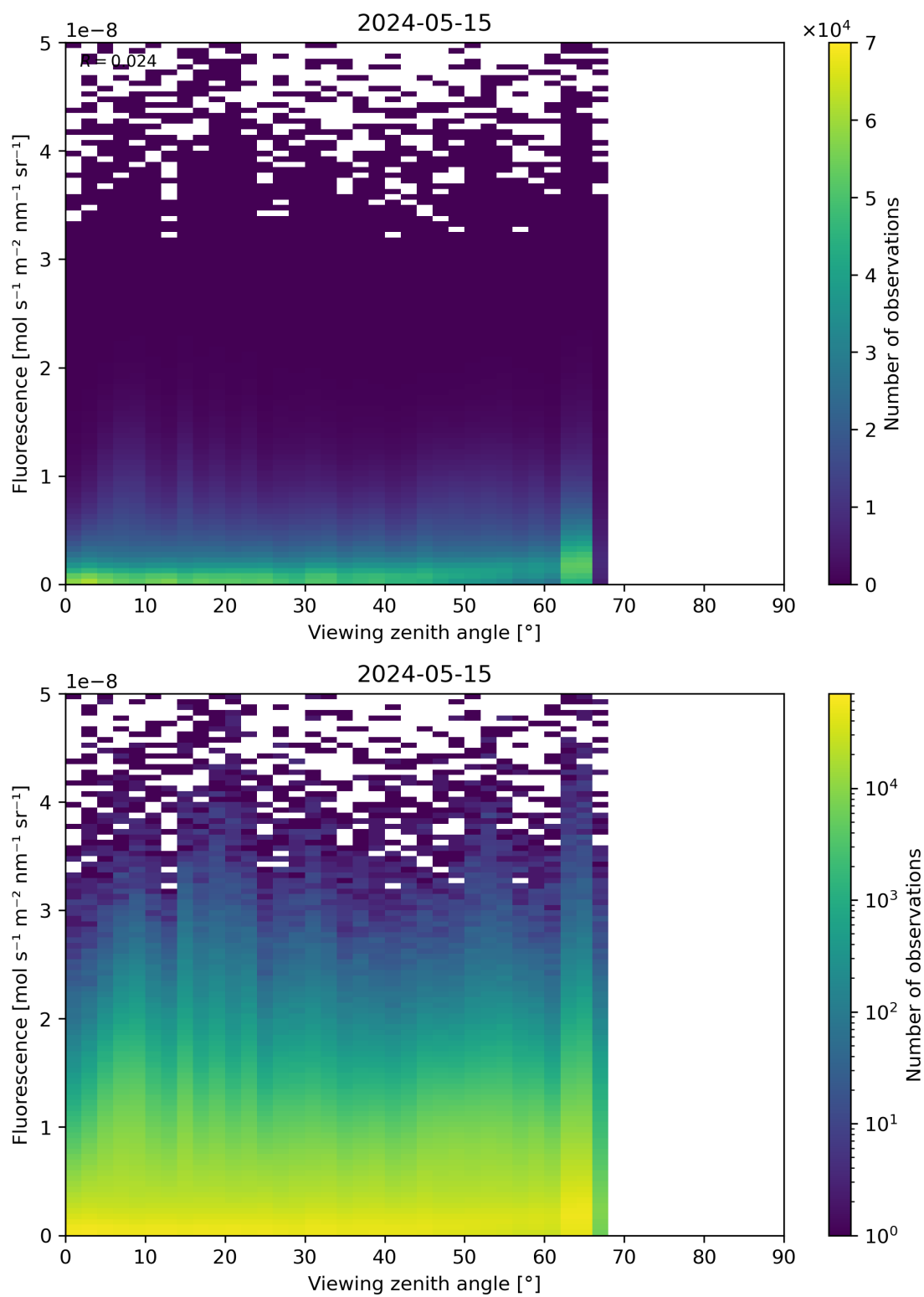
Figure 122: Scatter density plot of “Viewing zenith angle” against “Fluorescence” for 2024-05-14 to 2024-05-16.
