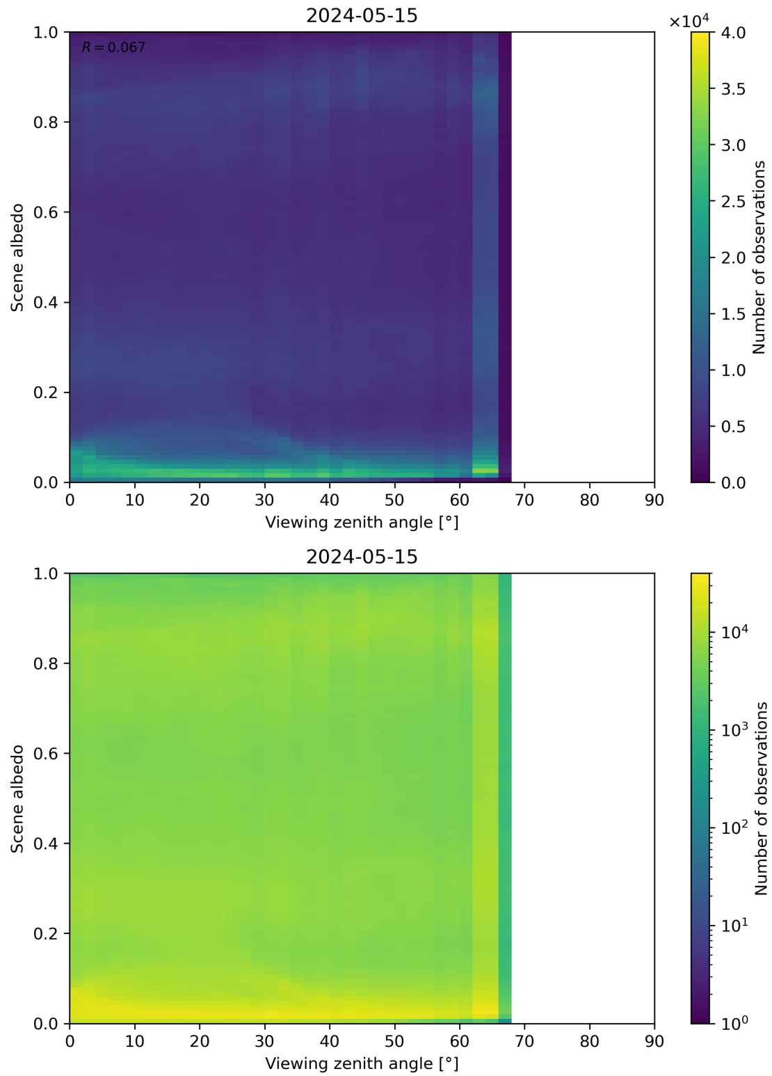
Figure 126: Scatter density plot of “Viewing zenith angle” against “Scene albedo” for 2024-05-14 to 2024-05-16.
