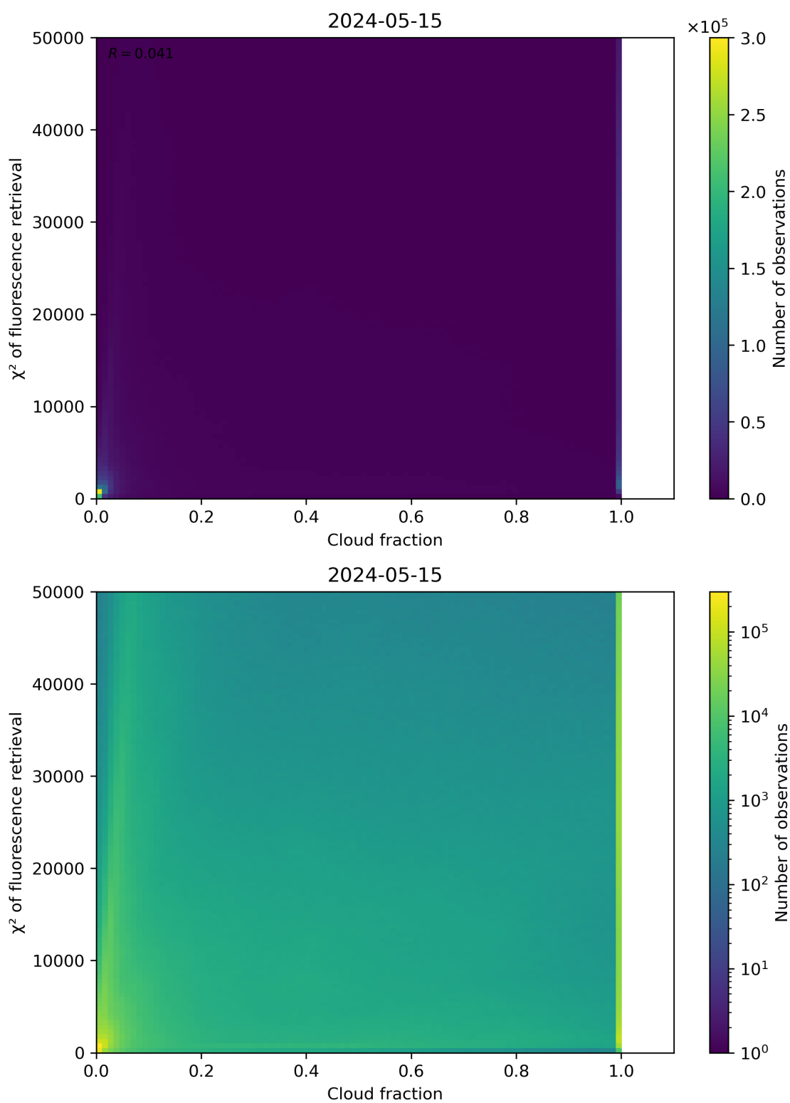
Figure 71: Scatter density plot of “Cloud fraction” against “ \chi^2 of fluorescence retrieval” for 2024-05-14 to 2024-05-16.
