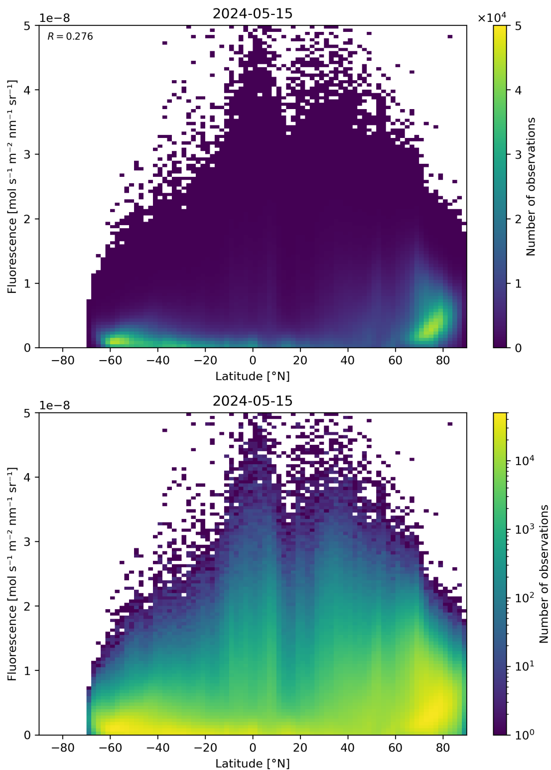
Figure 92: Scatter density plot of “Latitude” against “Fluorescence” for 2024-05-14 to 2024-05-16.
