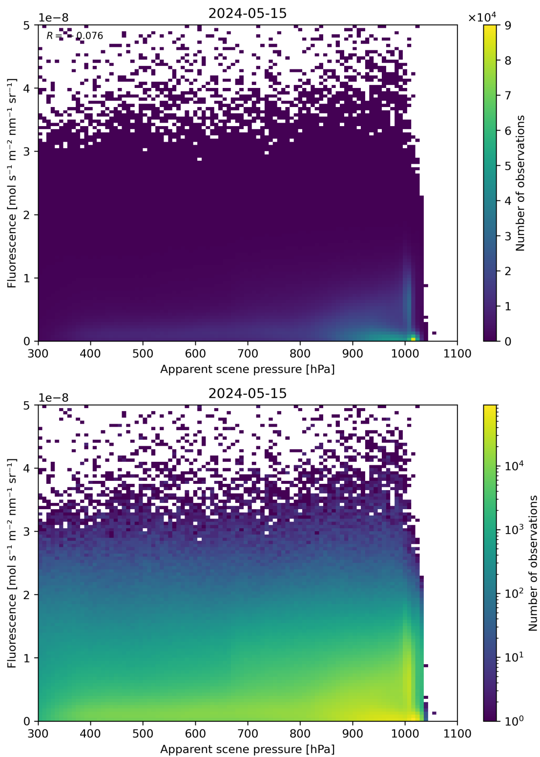
Figure 64: Scatter density plot of “Apparent scene pressure” against “Fluorescence” for 2024-05-14 to 2024-05-16.
