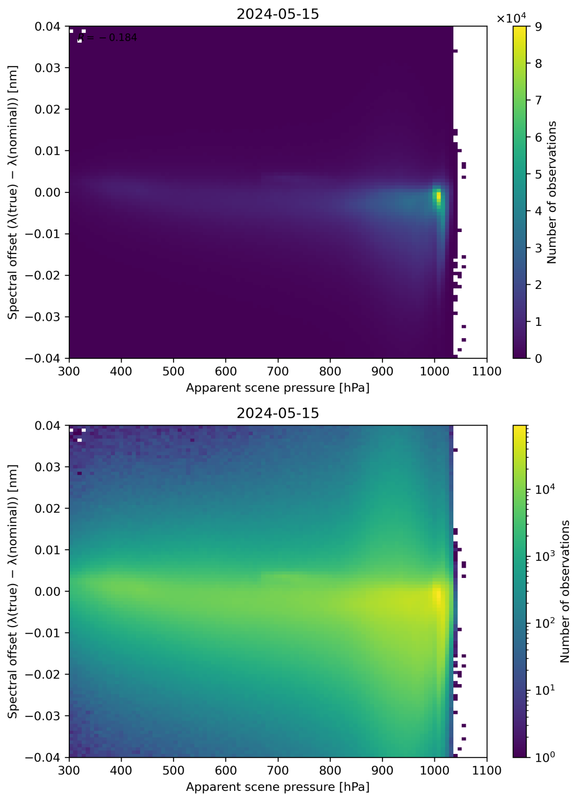
Figure 67: Scatter density plot of “Apparent scene pressure” against “Spectral offset ( \lambda(\text{true}) - \lambda(\text{nominal}) )” for 2024-05-14 to 2024-05-16.
