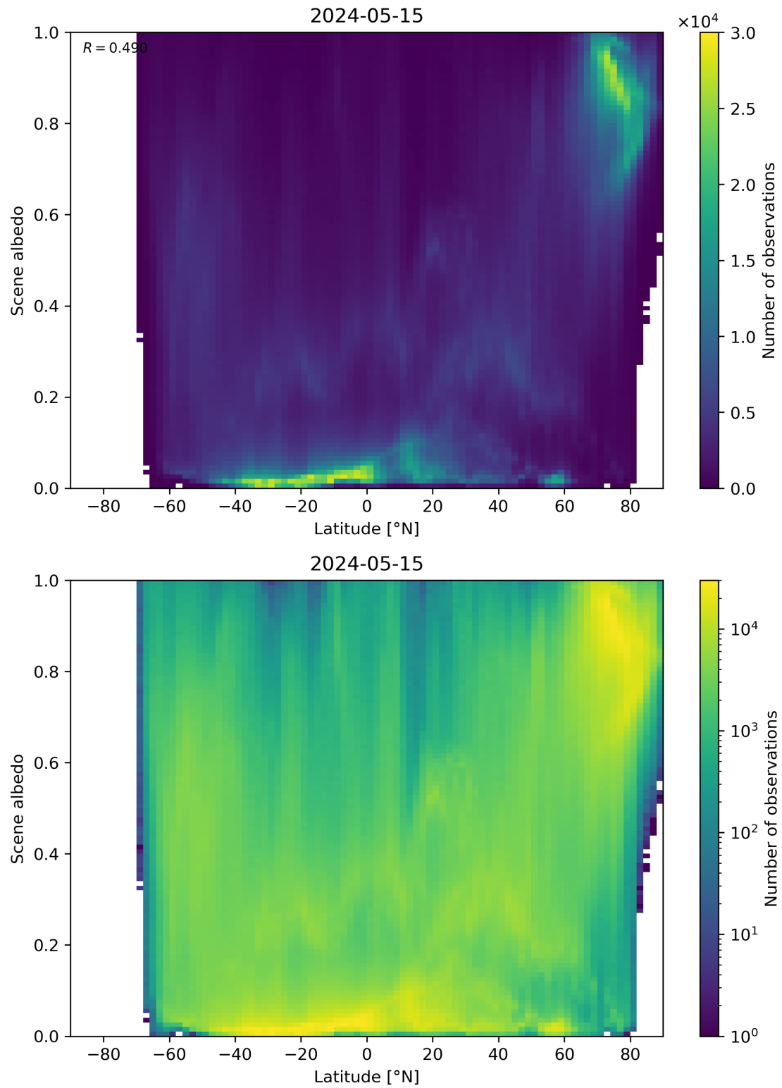
Figure 95: Scatter density plot of “Latitude” against “Scene albedo” for 2024-05-14 to 2024-05-16.
