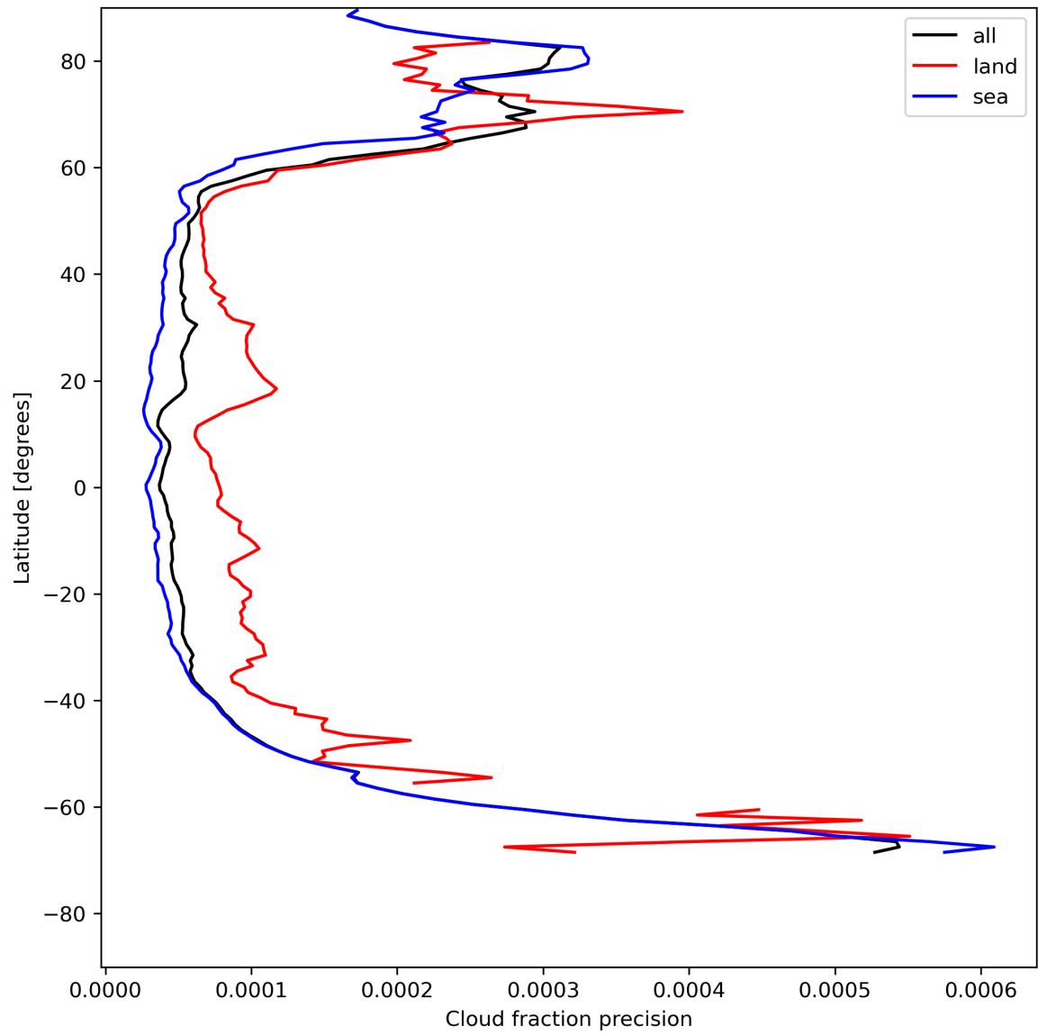
Figure 16: Zonal average of “Cloud fraction precision” for 2024-05-14 to 2024-05-16.
