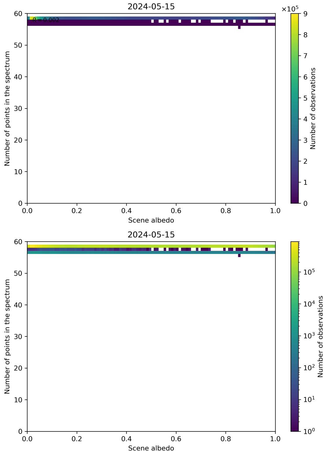
Figure 106: Scatter density plot of “Scene albedo” against “Number of points in the spectrum” for 2024-05-14 to 2024-05-16.
