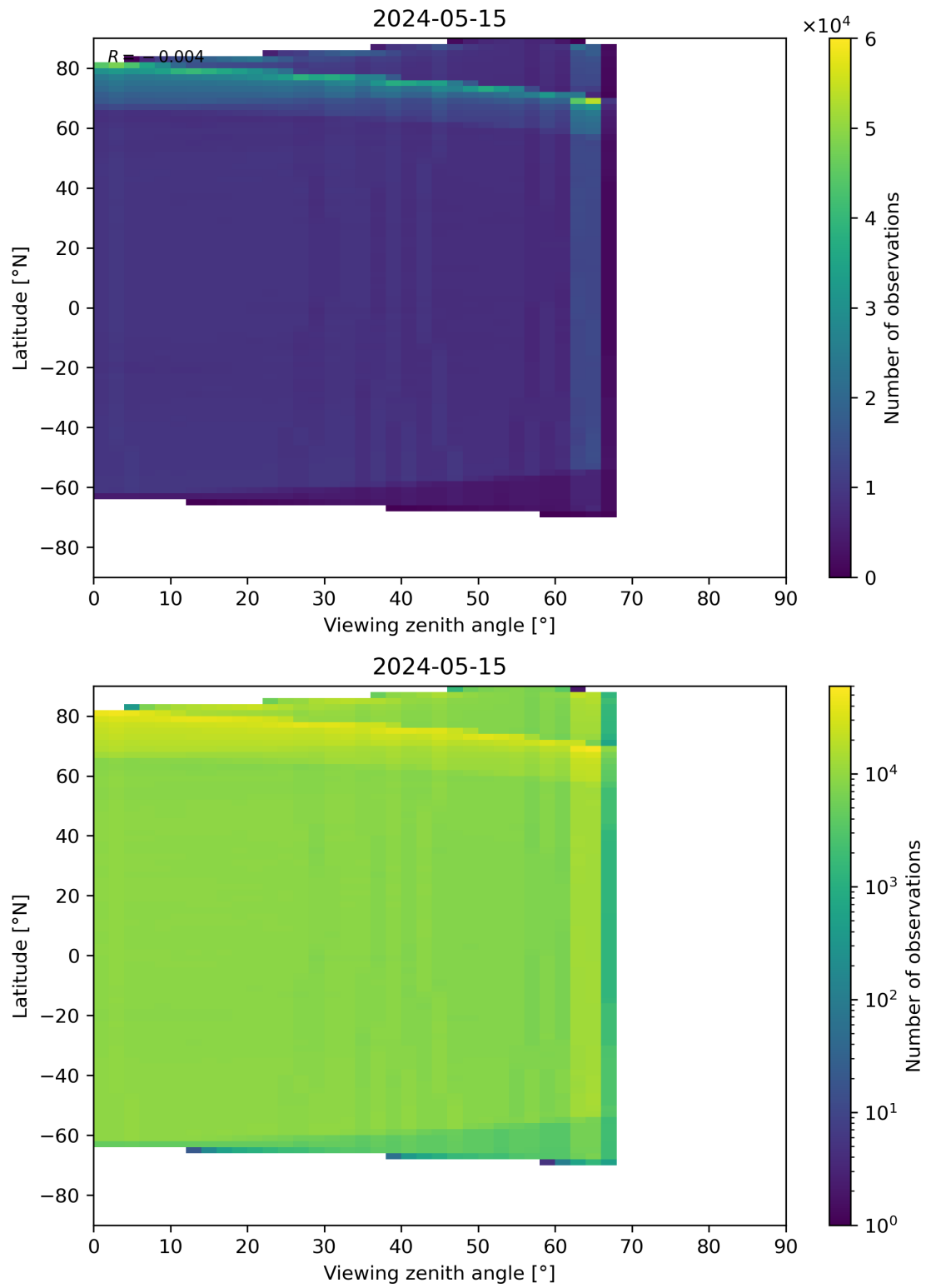
Figure 123: Scatter density plot of “Viewing zenith angle” against “Latitude” for 2024-05-14 to 2024-05-16.
