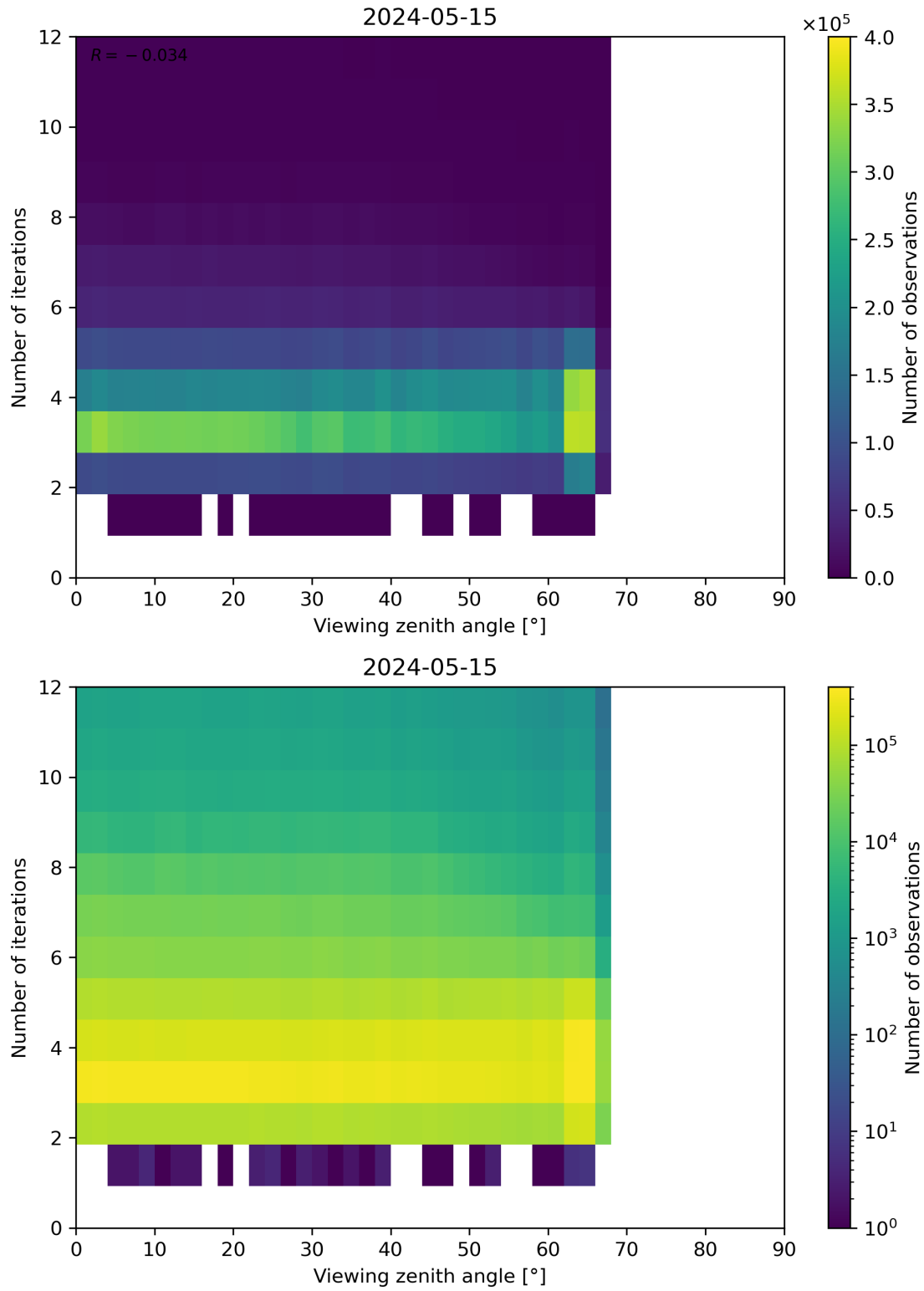
Figure 124: Scatter density plot of “Viewing zenith angle” against “Number of iterations” for 2024-05-14 to 2024-05-16.
