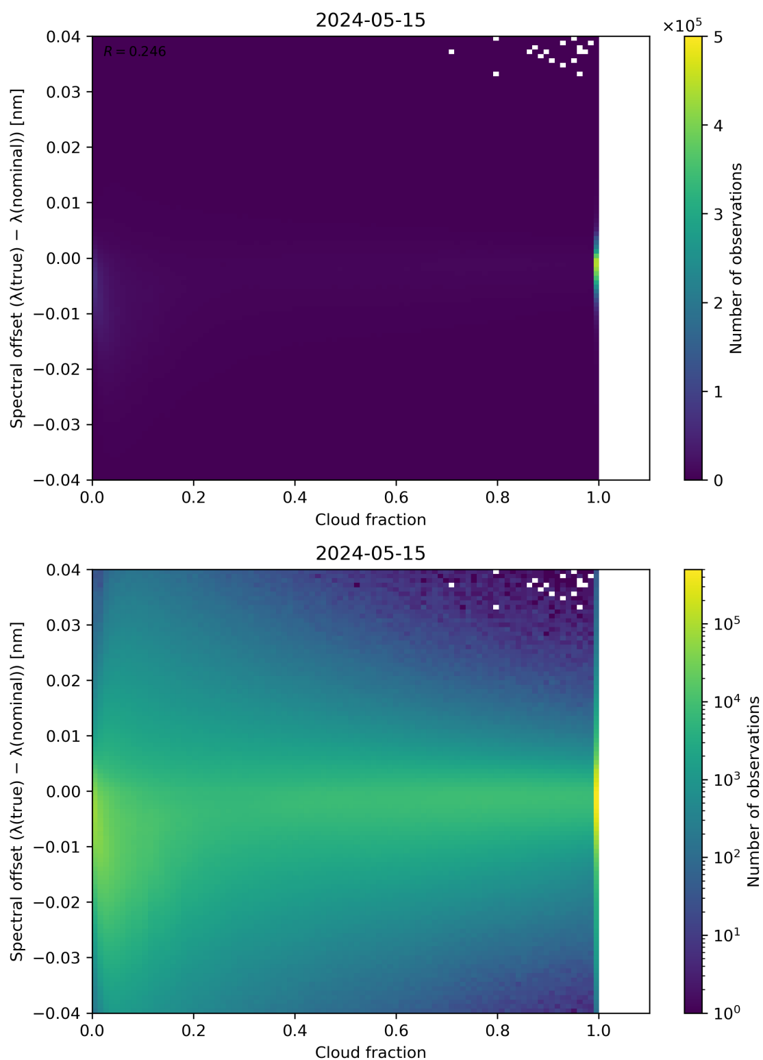
Figure 76: Scatter density plot of “Cloud fraction” against “Spectral offset ( \lambda(\text{true}) - \lambda(\text{nominal}) )” for 2024-05-14 to 2024-05-16.
