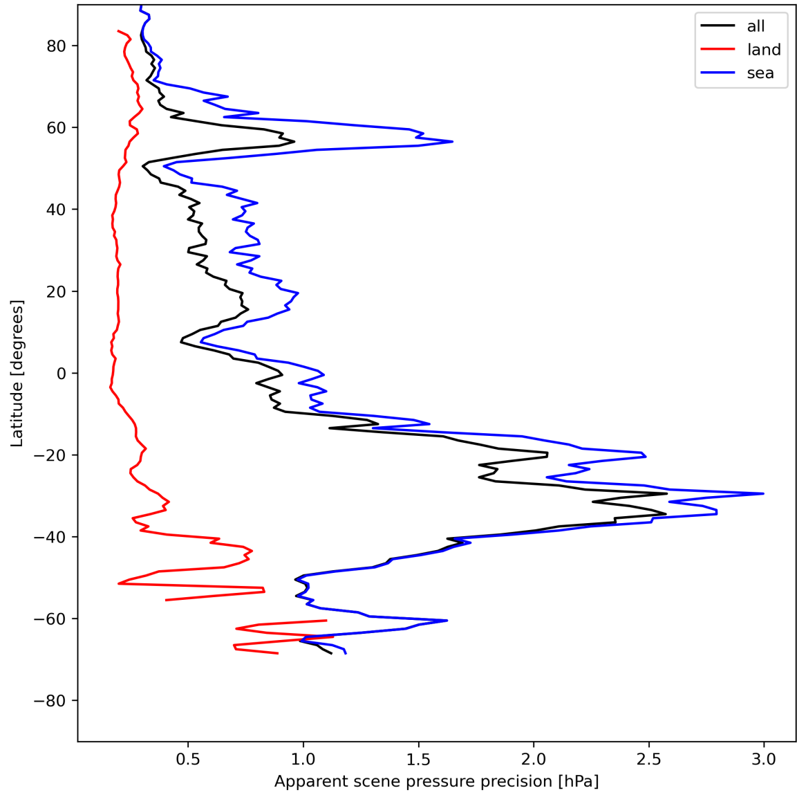
Figure 20: Zonal average of “Apparent scene pressure precision” for 2024-05-14 to 2024-05-16.
