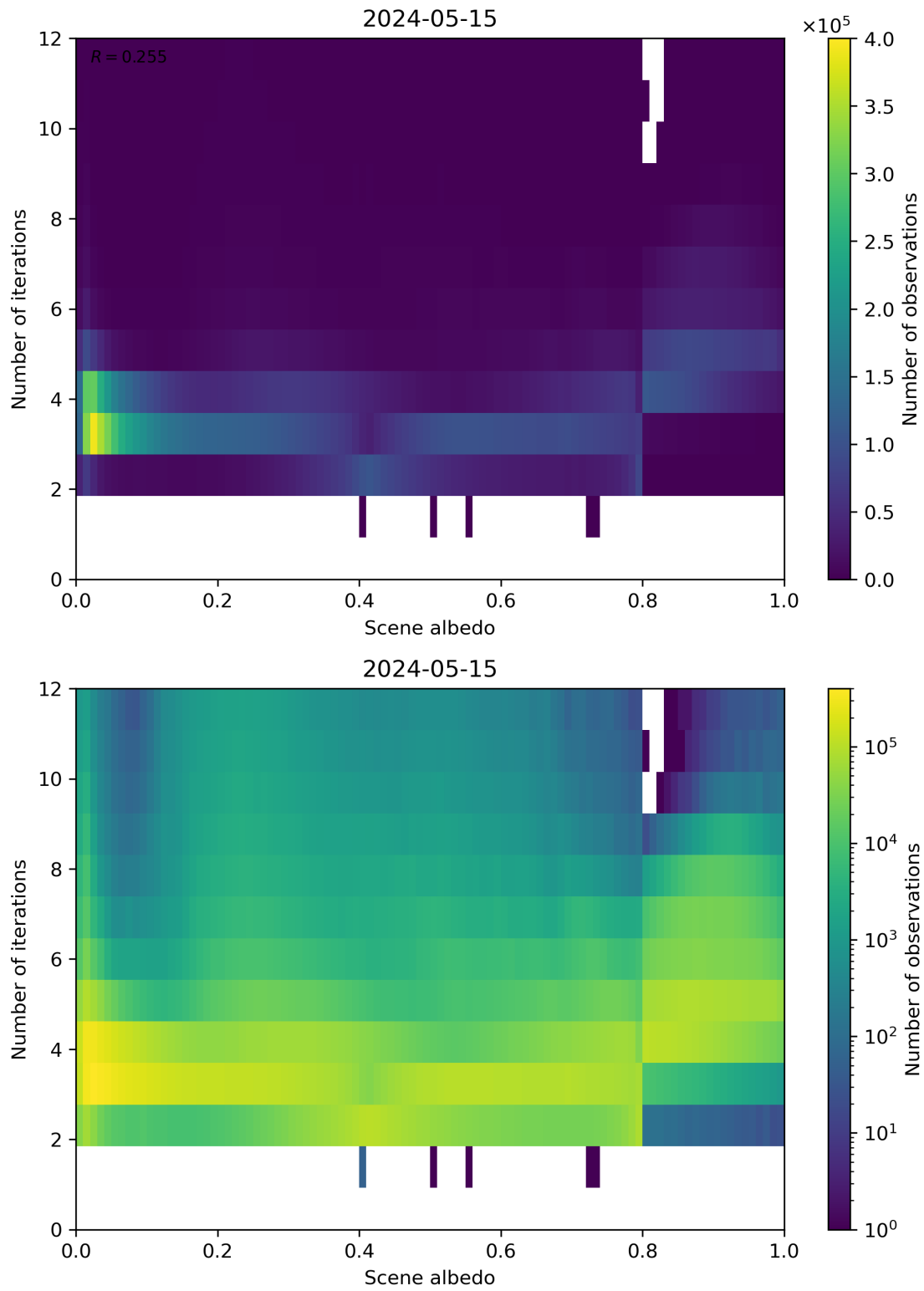
Figure 105: Scatter density plot of “Scene albedo” against “Number of iterations” for 2024-05-14 to 2024-05-16.
