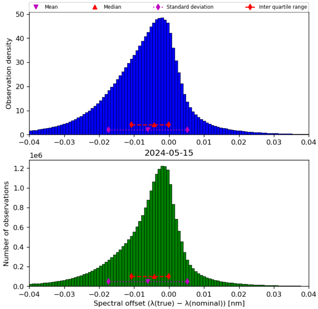
Figure 45: Histogram of “Spectral offset ( \lambda(\text{true}) - \lambda(\text{nominal}) )” for 2024-05-14 to 2024-05-16
