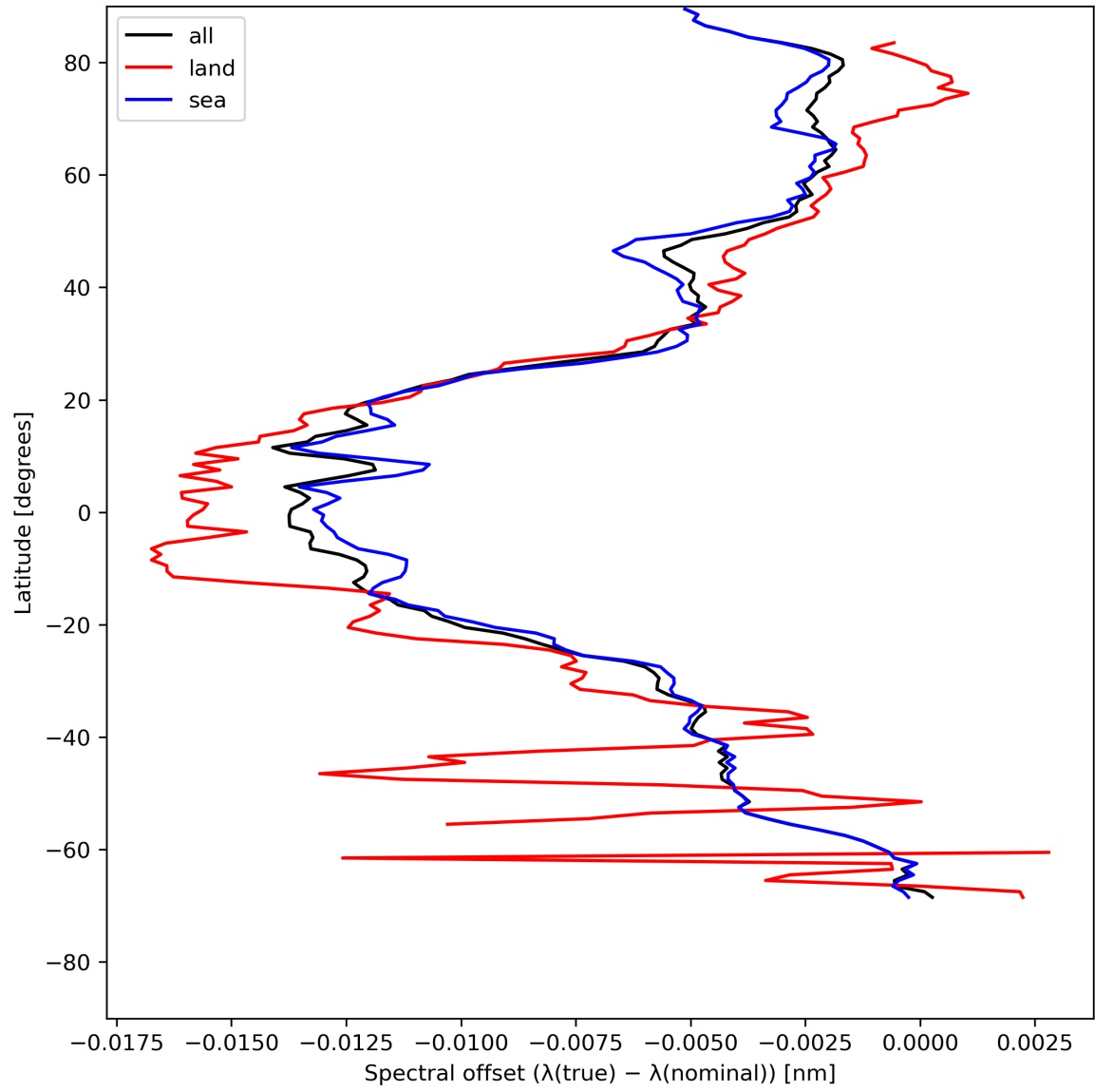
Figure 28: Zonal average of “Spectral offset ( \lambda(\text{true}) - \lambda(\text{nominal}) )” for 2024-05-14 to 2024-05-16.
