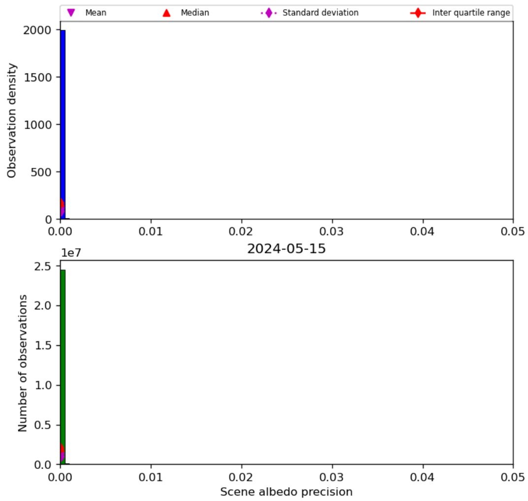
Figure 35: Histogram of “Scene albedo precision” for 2024-05-14 to 2024-05-16
