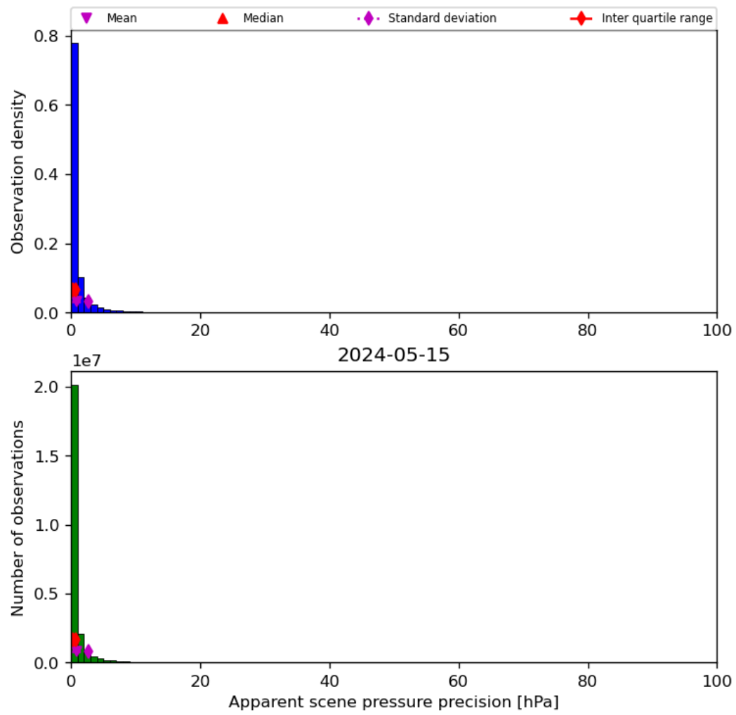
Figure 37: Histogram of “Apparent scene pressure precision” for 2024-05-14 to 2024-05-16
