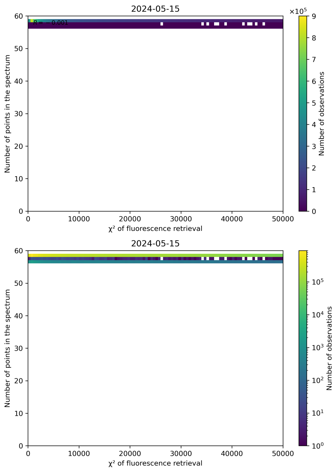
Figure 68: Scatter density plot of " \chi^2 of fluorescence retrieval" against "Number of points in the spectrum" for 2024-05-14 to 2024-05-16.
