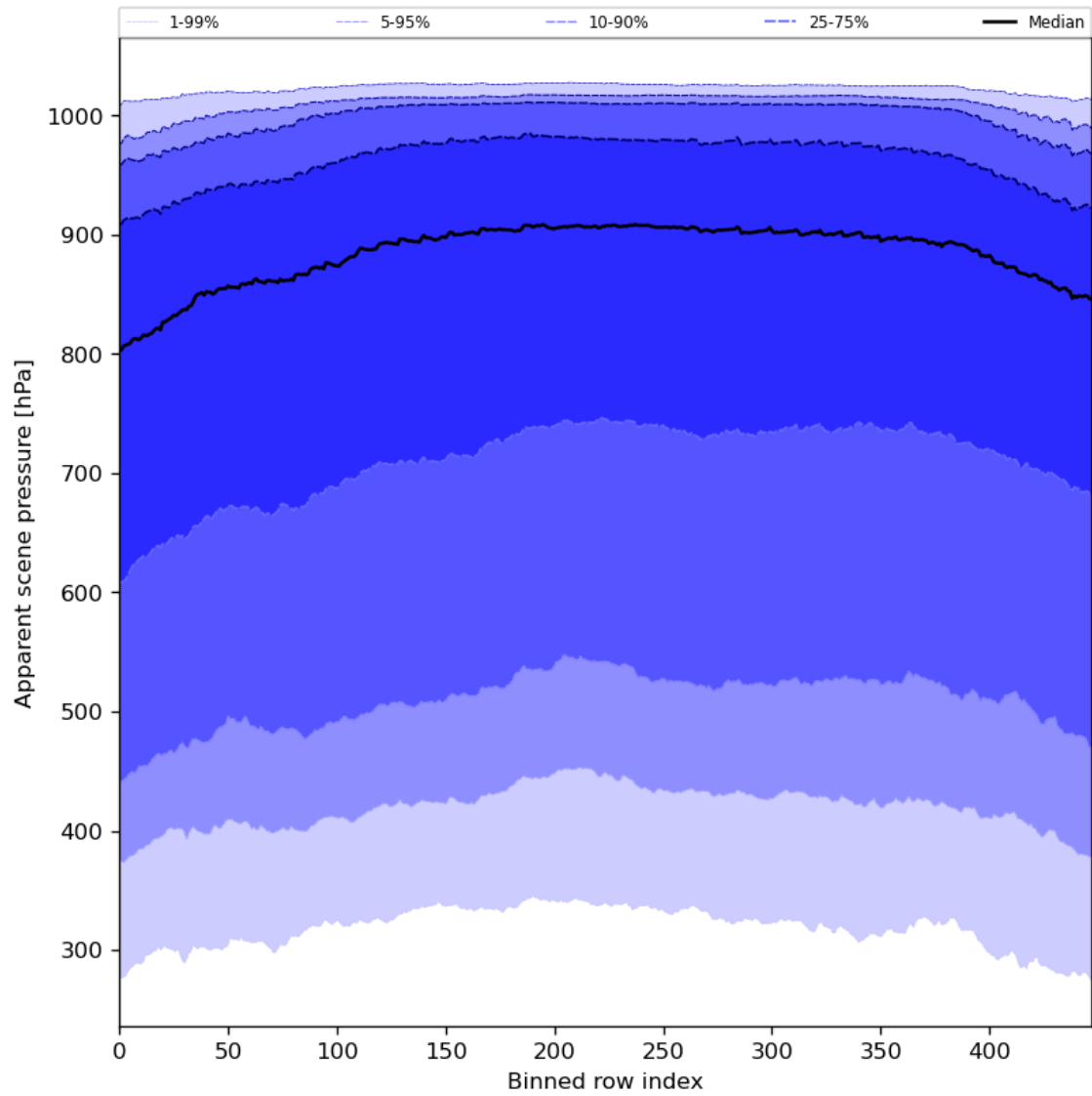
Figure 53: Along track statistics of “Apparent scene pressure” for 2024-05-14 to 2024-05-16
