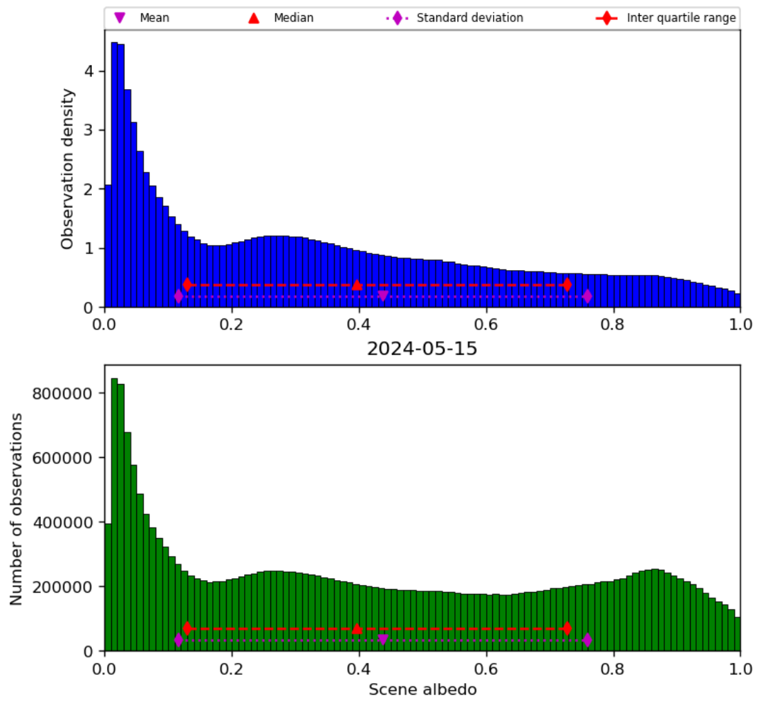
Figure 34: Histogram of “Scene albedo” for 2024-05-14 to 2024-05-16
