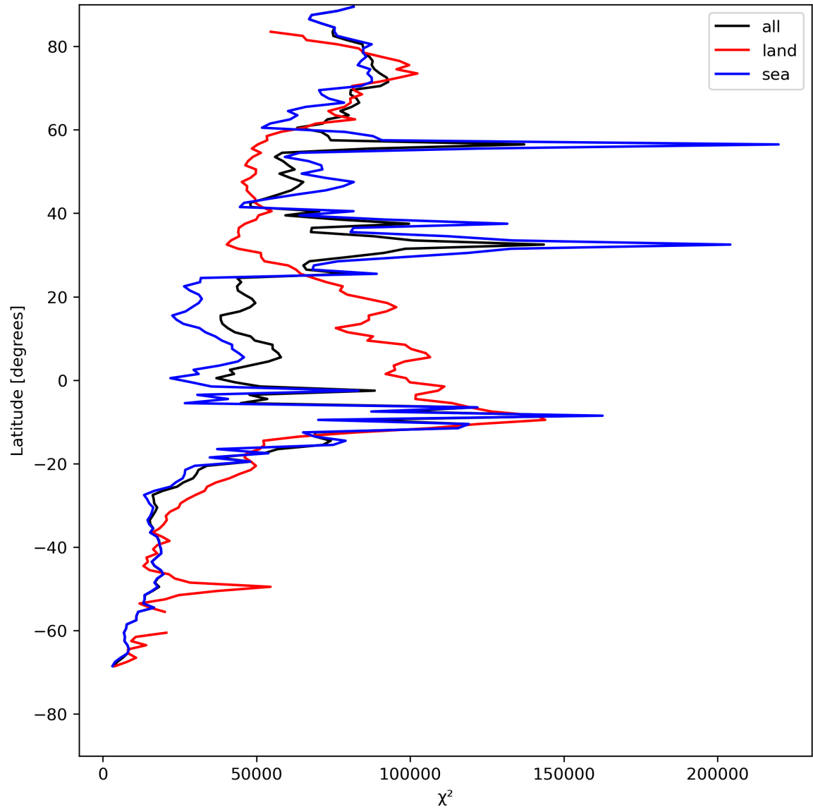
Figure 21: Zonal average of “ \chi^2 ” for 2024-05-14 to 2024-05-16.
