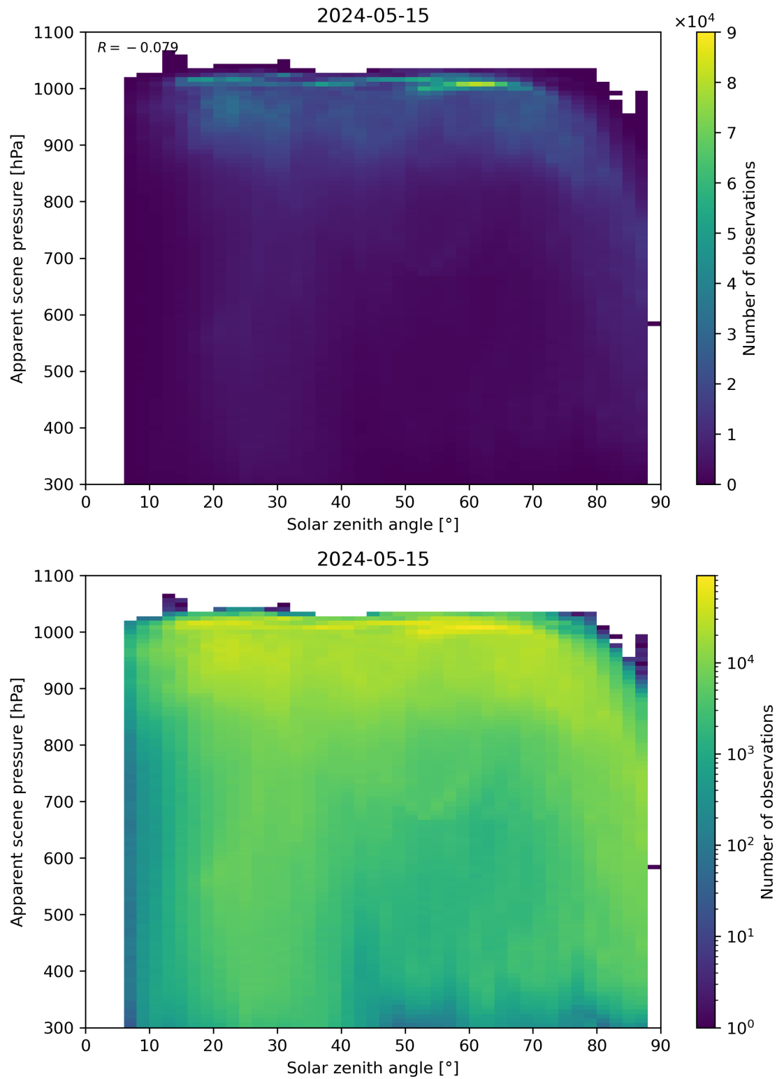
Figure 108: Scatter density plot of “Solar zenith angle” against “Apparent scene pressure” for 2024-05-14 to 2024-05-16.
