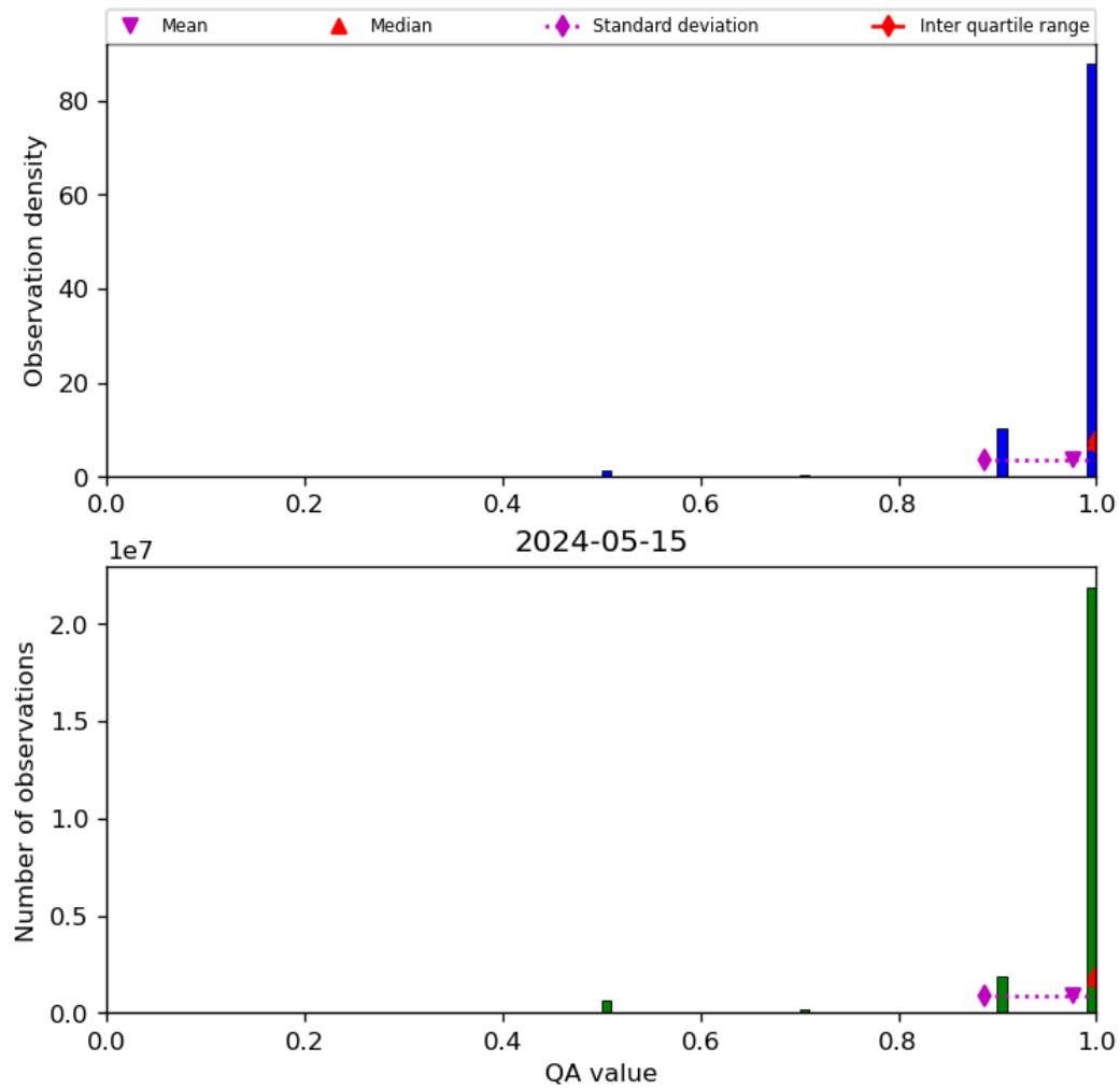
Figure 29: Histogram of “QA value” for 2024-05-14 to 2024-05-16
