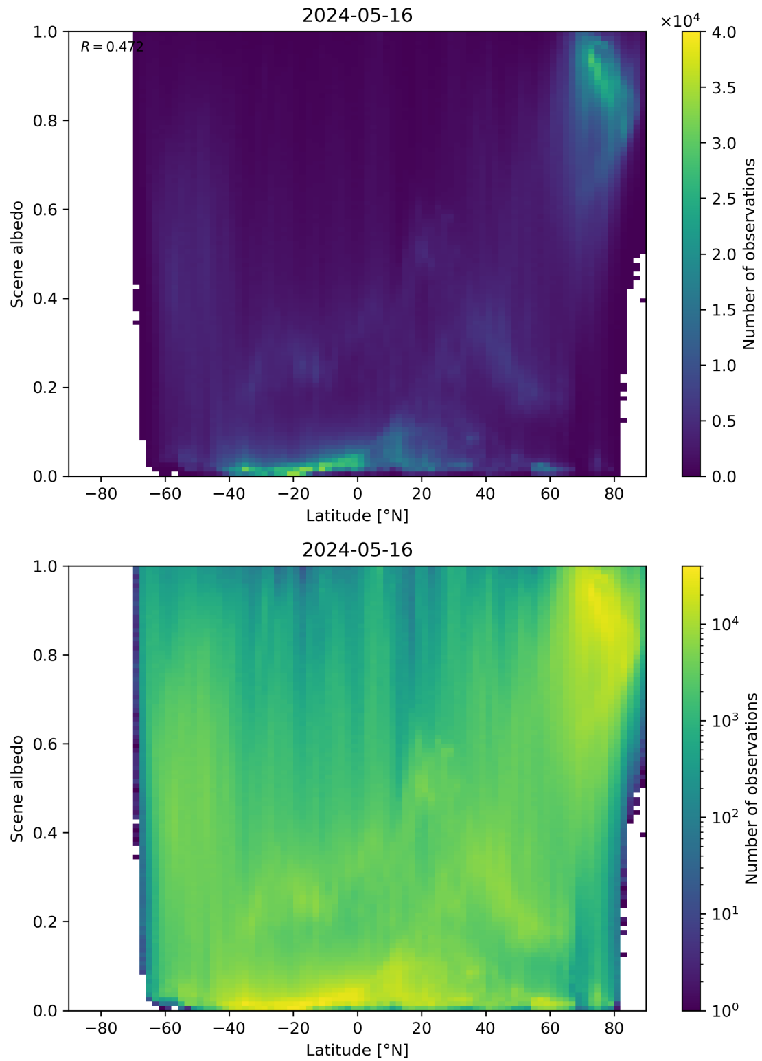
Figure 95: Scatter density plot of “Latitude” against “Scene albedo” for 2024-05-15 to 2024-05-17.
