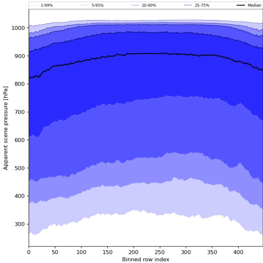
Figure 53: Along track statistics of “Apparent scene pressure” for 2024-05-15 to 2024-05-17
