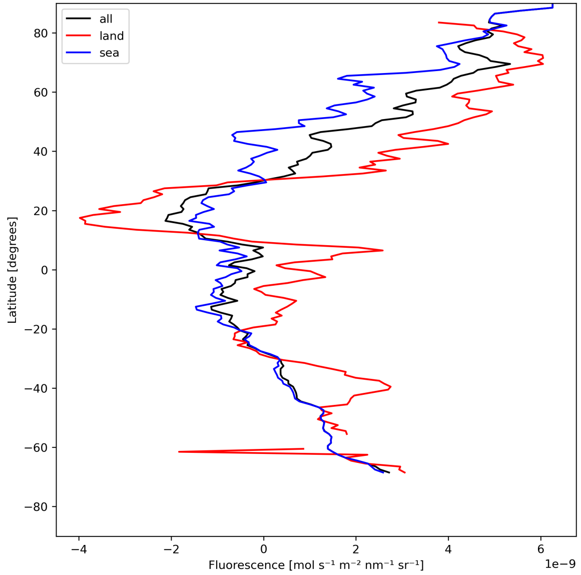
Figure 23: Zonal average of “Fluorescence” for 2024-05-15 to 2024-05-17.
