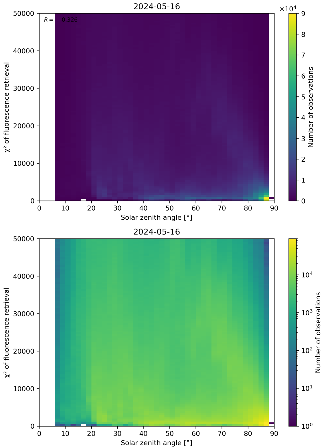
Figure 109: Scatter density plot of “Solar zenith angle” against “ \chi^2 of fluorescence retrieval” for 2024-05-15 to 2024-05-17.
