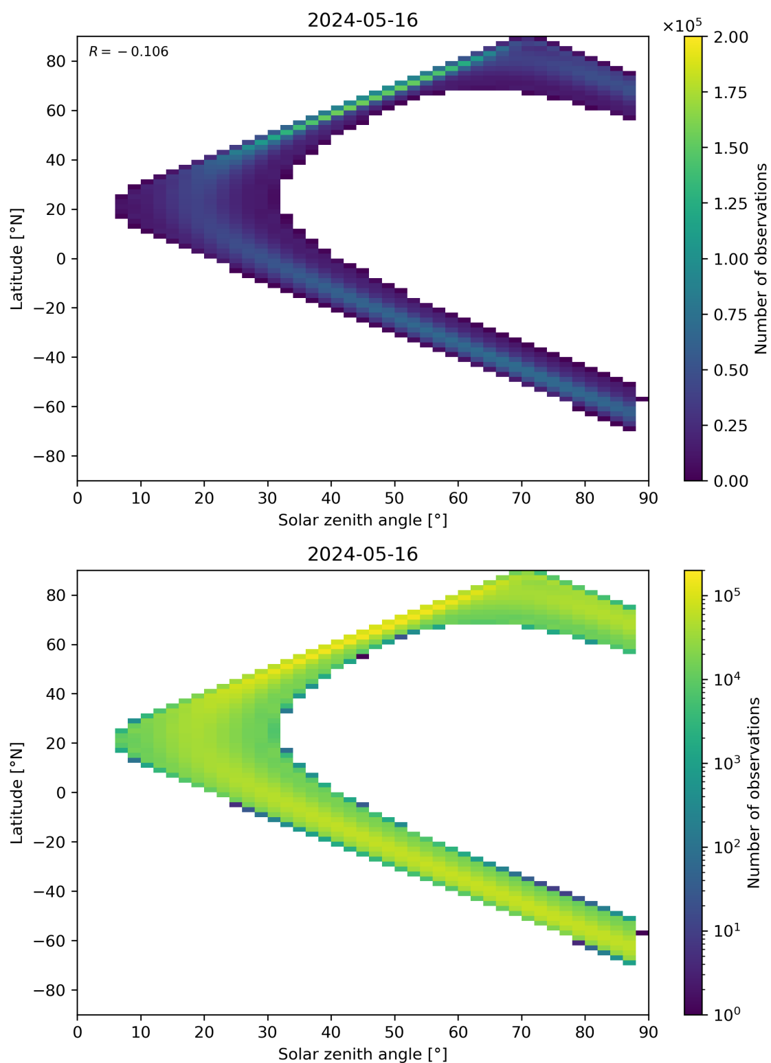
Figure 113: Scatter density plot of “Solar zenith angle” against “Latitude” for 2024-05-15 to 2024-05-17.
