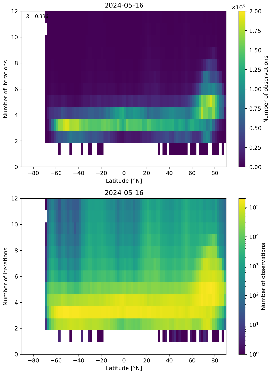
Figure 93: Scatter density plot of “Latitude” against “Number of iterations” for 2024-05-15 to 2024-05-17.
