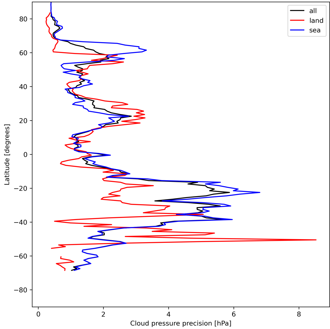
Figure 14: Zonal average of “Cloud pressure precision” for 2024-05-15 to 2024-05-17.
