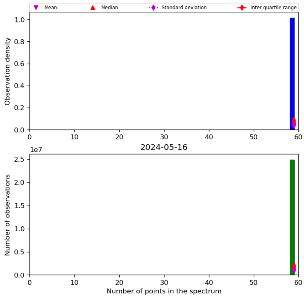
Figure 44: Histogram of “Number of points in the spectrum” for 2024-05-15 to 2024-05-17
