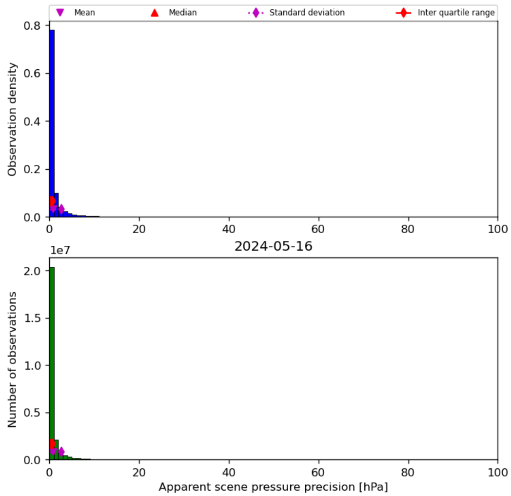
Figure 37: Histogram of “Apparent scene pressure precision” for 2024-05-15 to 2024-05-17
