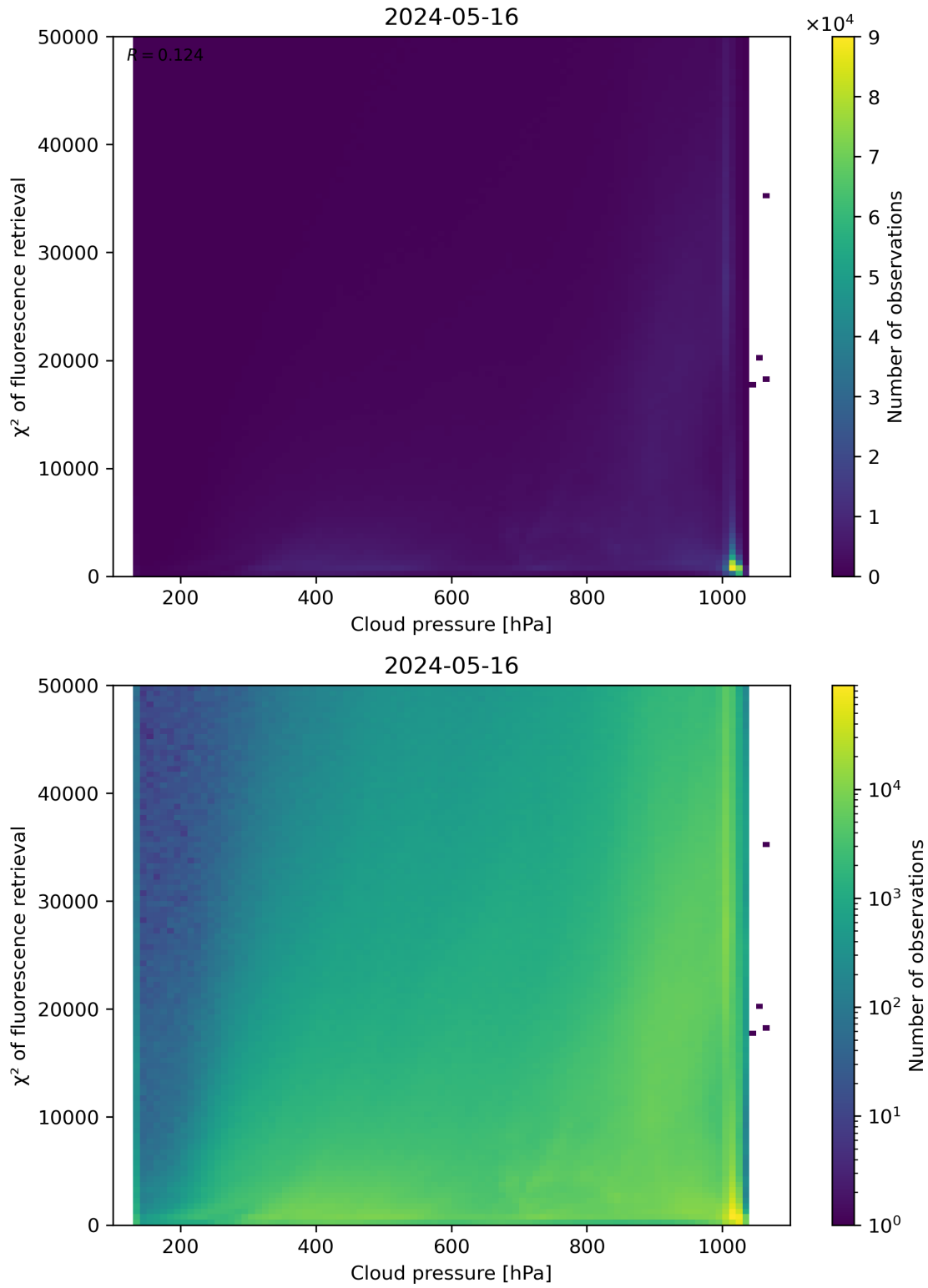
Figure 78: Scatter density plot of “Cloud pressure” against “ \chi^2 of fluorescence retrieval” for 2024-05-15 to 2024-05-17.
