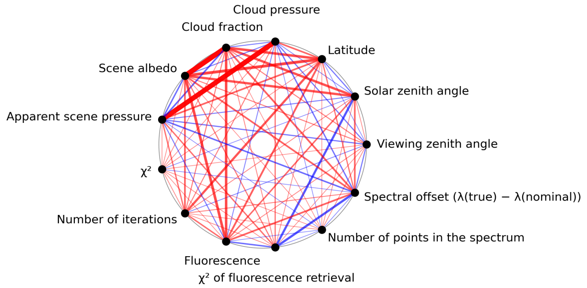
Figure 1: Map of correlation graph for 2024-05-15 to 2024-05-17.
