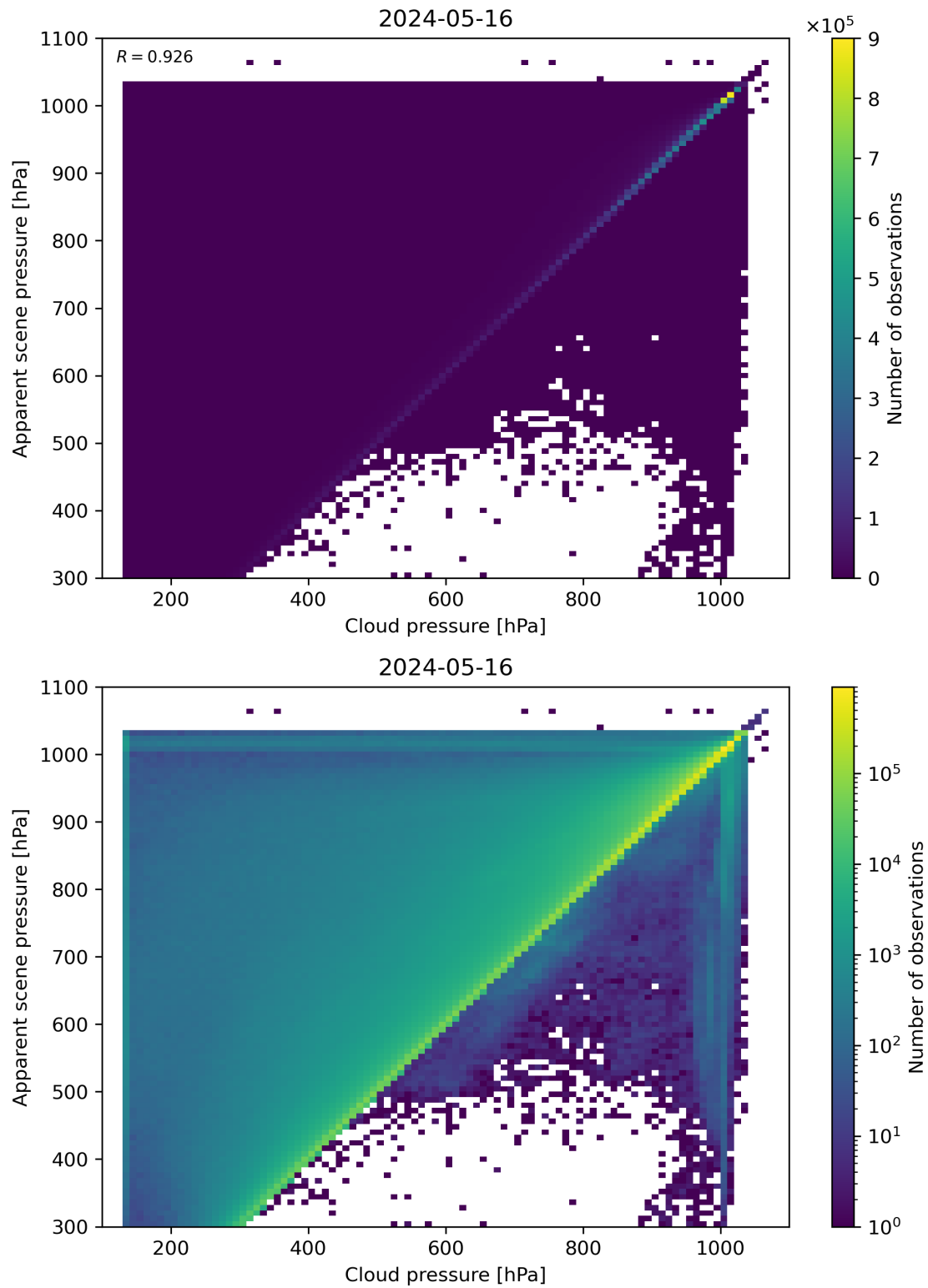
Figure 77: Scatter density plot of “Cloud pressure” against “Apparent scene pressure” for 2024-05-15 to 2024-05-17.
