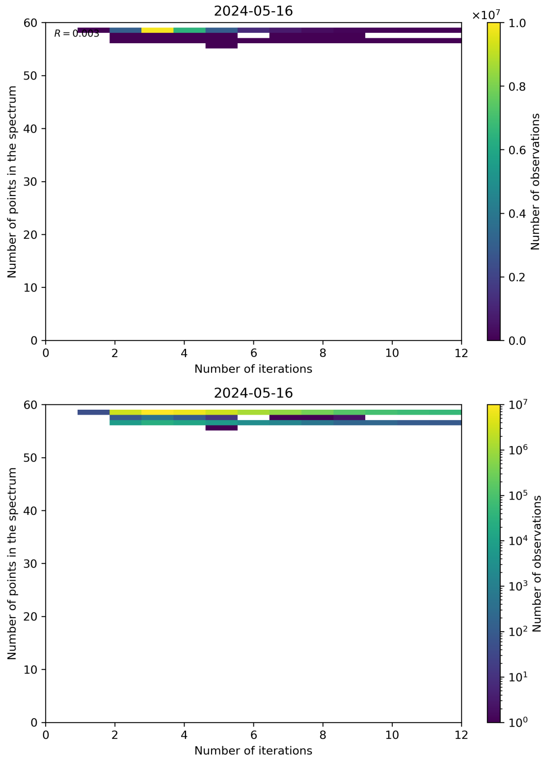
Figure 99: Scatter density plot of “Number of iterations” against “Number of points in the spectrum” for 2024-05-15 to 2024-05-17.
