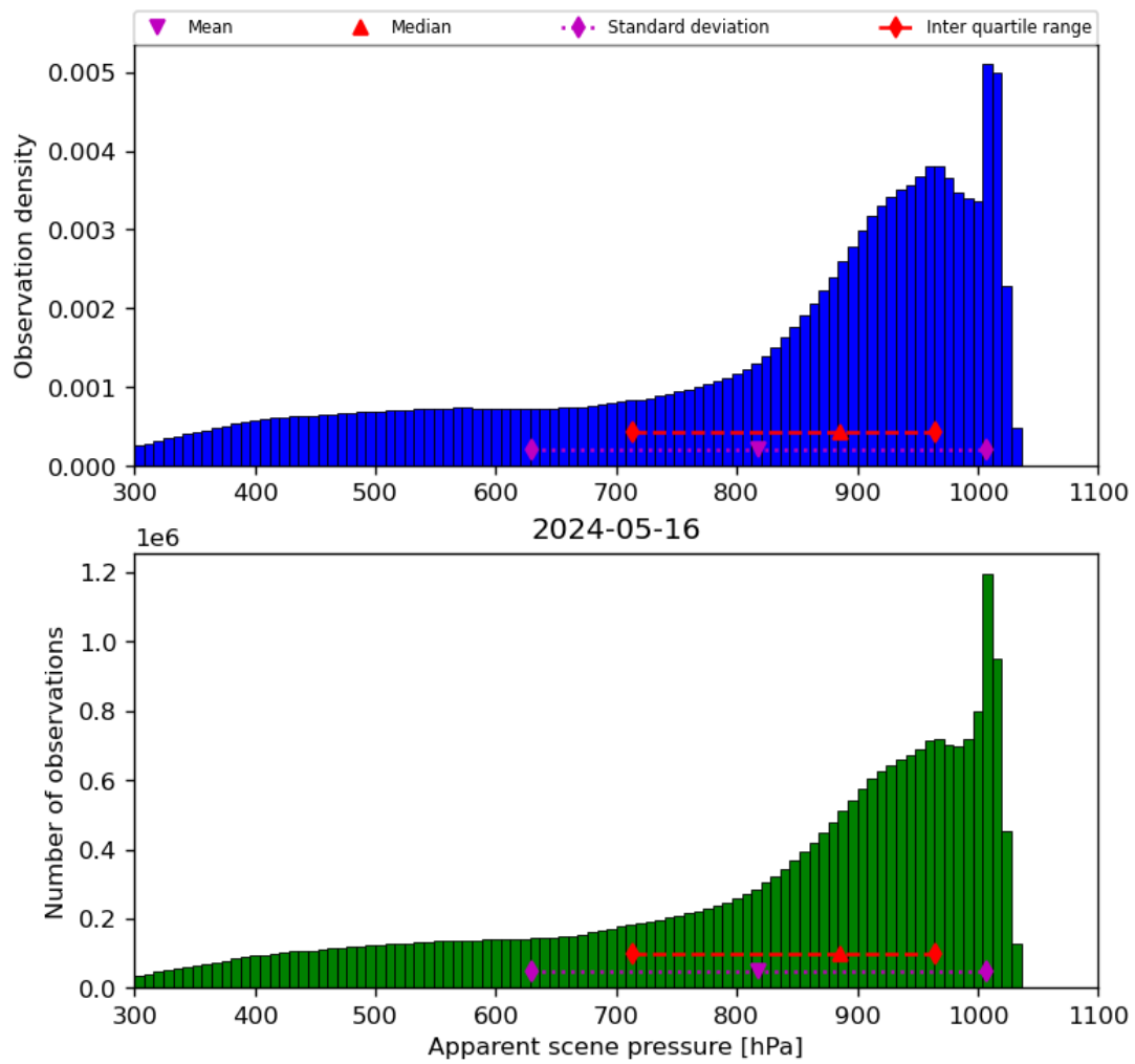
Figure 36: Histogram of “Apparent scene pressure” for 2024-05-15 to 2024-05-17
