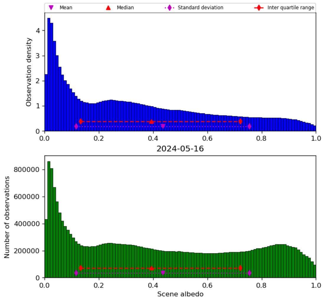
Figure 34: Histogram of “Scene albedo” for 2024-05-15 to 2024-05-17
