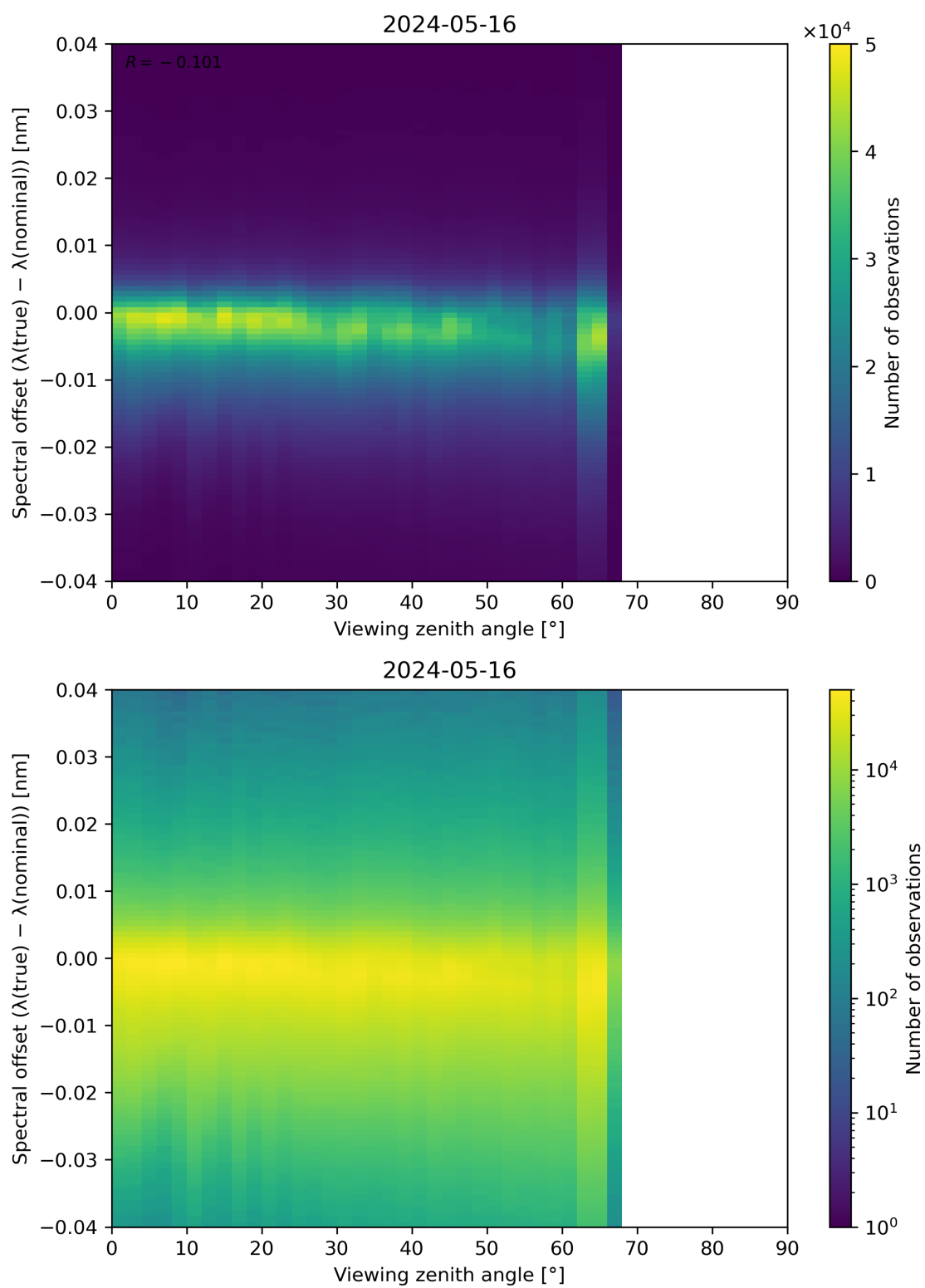
Figure 128: Scatter density plot of “Viewing zenith angle” against “Spectral offset ( \lambda(\text{true}) - \lambda(\text{nominal}) )” for 2024-05-15 to 2024-05-17.
