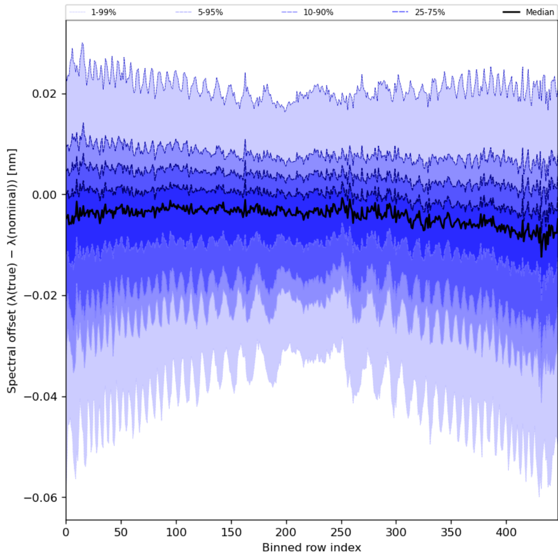
Figure 62: Along track statistics of “Spectral offset ( \lambda(\text{true}) - \lambda(\text{nominal}) )” for 2024-05-15 to 2024-05-17
