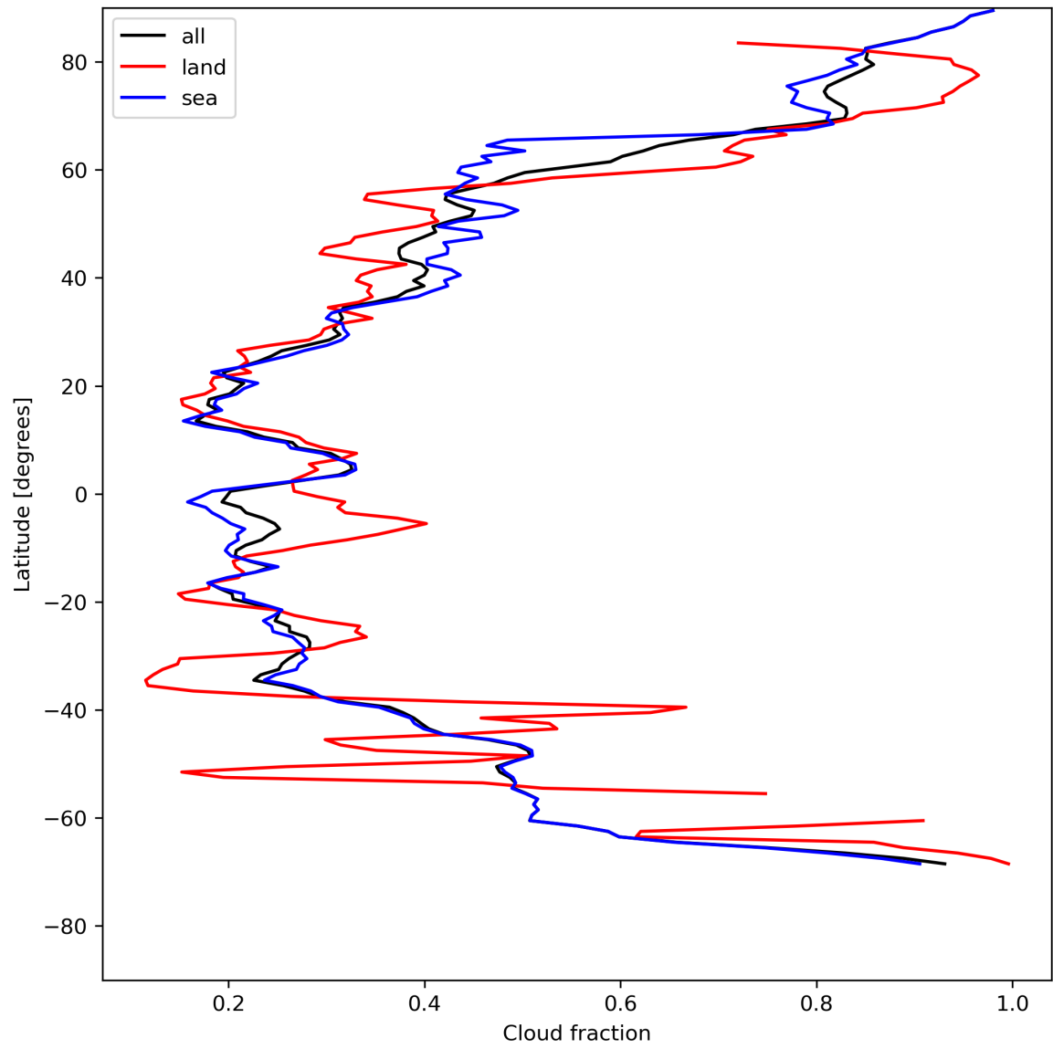
Figure 15: Zonal average of “Cloud fraction” for 2024-05-15 to 2024-05-17.
