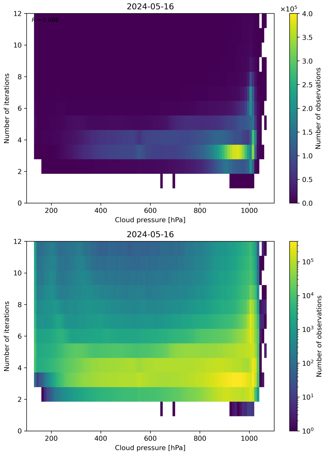
Figure 81: Scatter density plot of “Cloud pressure” against “Number of iterations” for 2024-05-15 to 2024-05-17.
