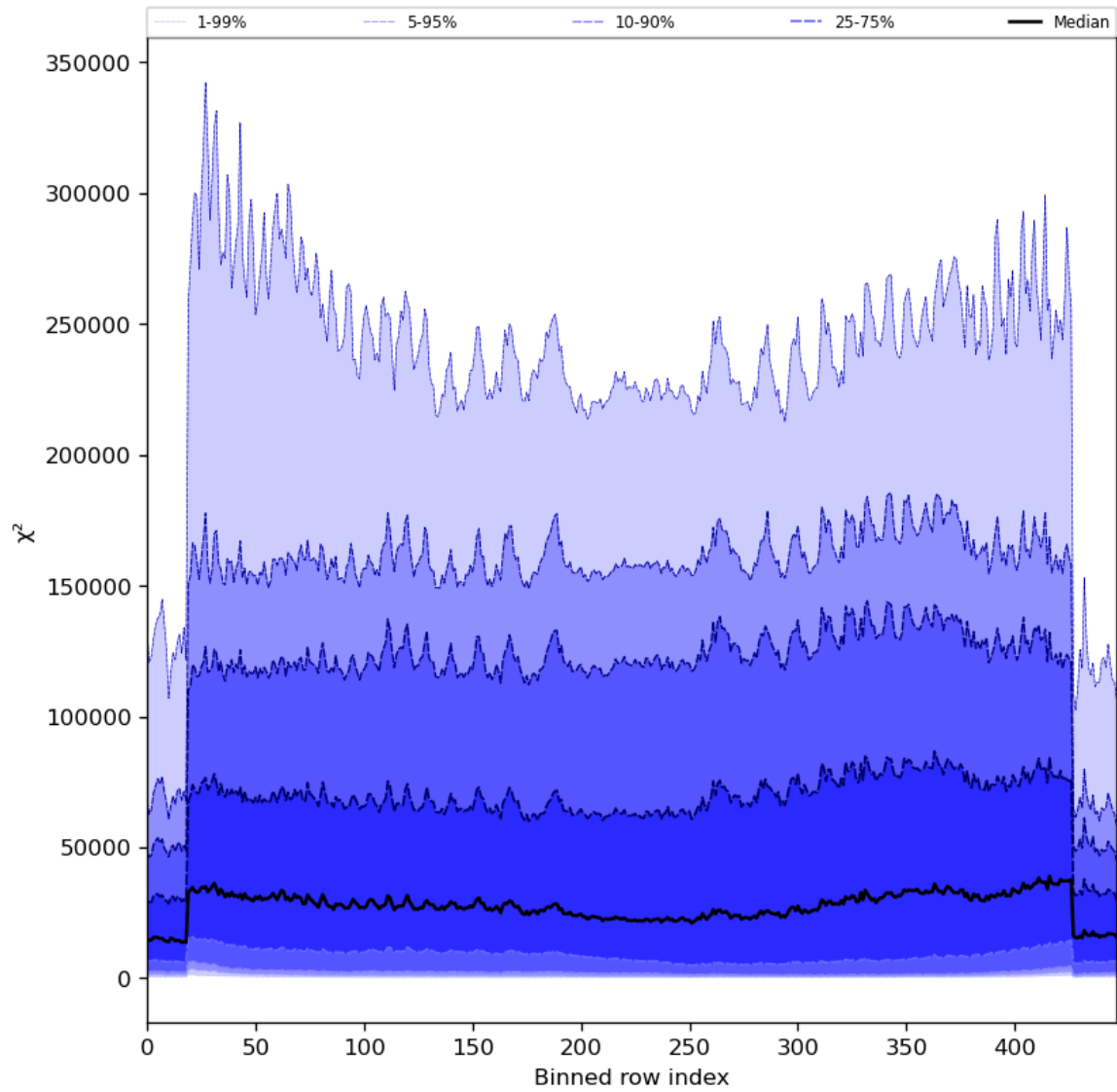
Figure 55: Along track statistics of “ \chi^2 ” for 2024-05-15 to 2024-05-17
