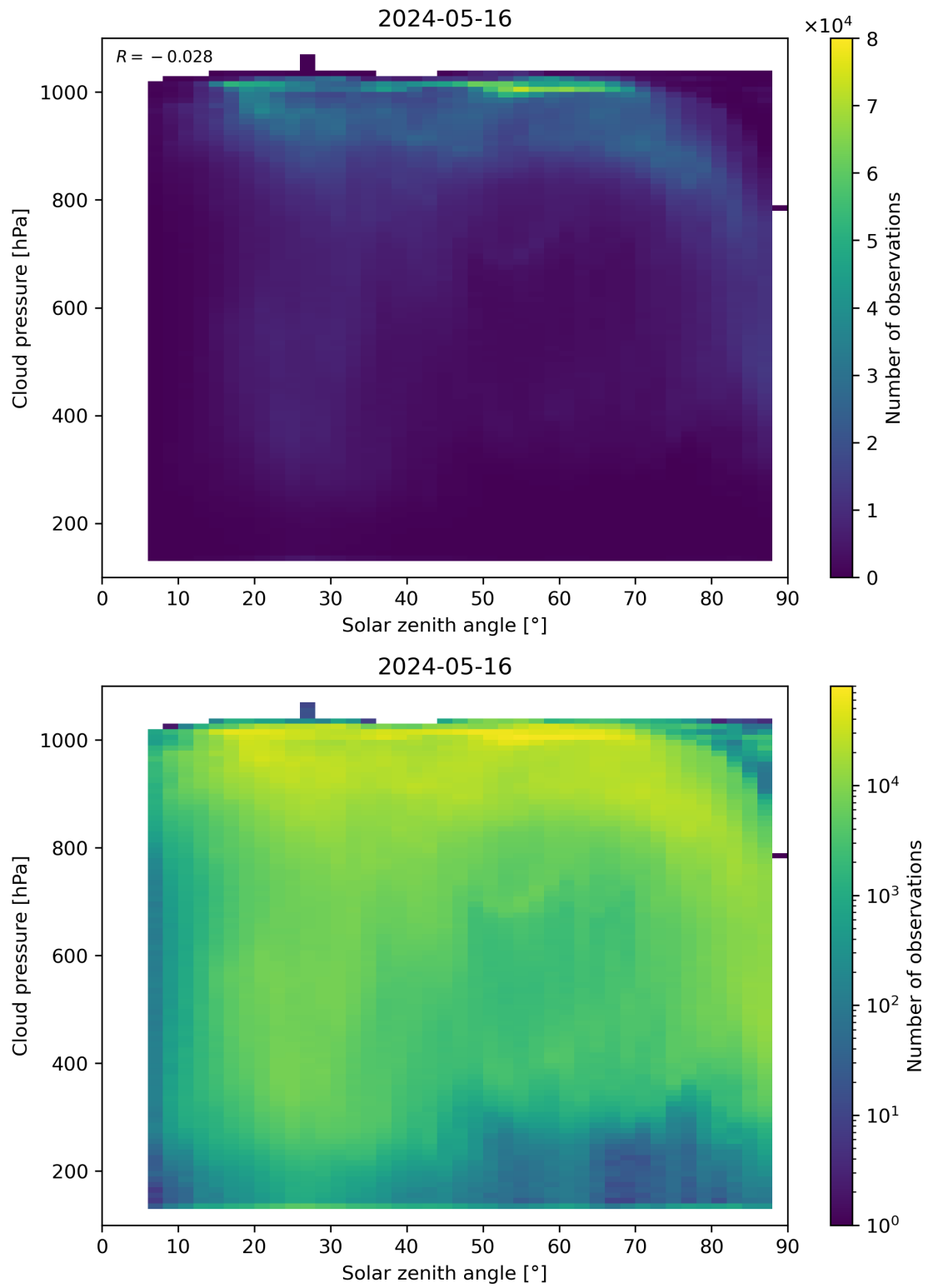
Figure 111: Scatter density plot of “Solar zenith angle” against “Cloud pressure” for 2024-05-15 to 2024-05-17.
