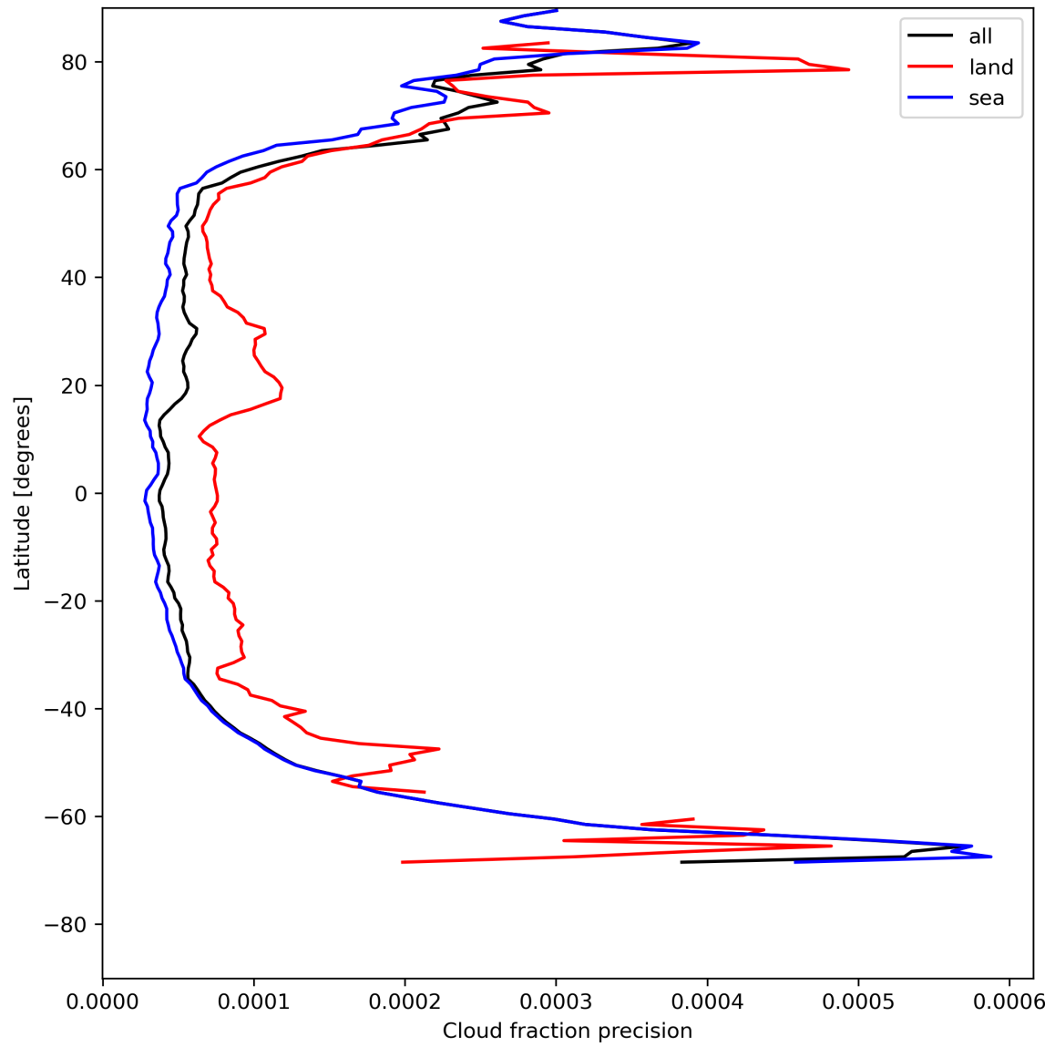
Figure 16: Zonal average of “Cloud fraction precision” for 2024-05-15 to 2024-05-17.
