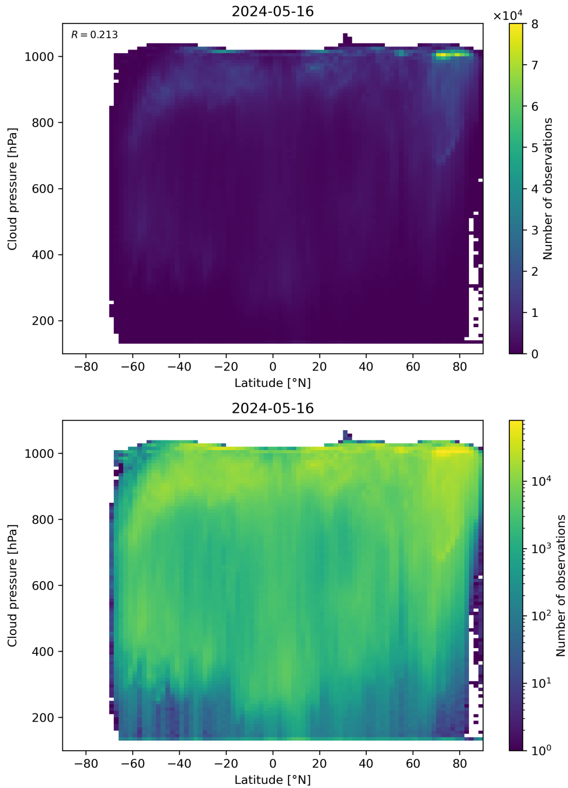
Figure 91: Scatter density plot of “Latitude” against “Cloud pressure” for 2024-05-15 to 2024-05-17.
