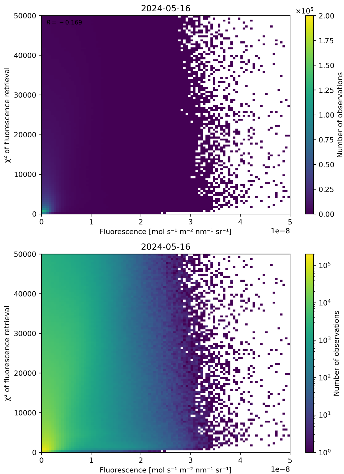
Figure 85: Scatter density plot of “Fluorescence” against “ \chi^2 of fluorescence retrieval” for 2024-05-15 to 2024-05-17.
