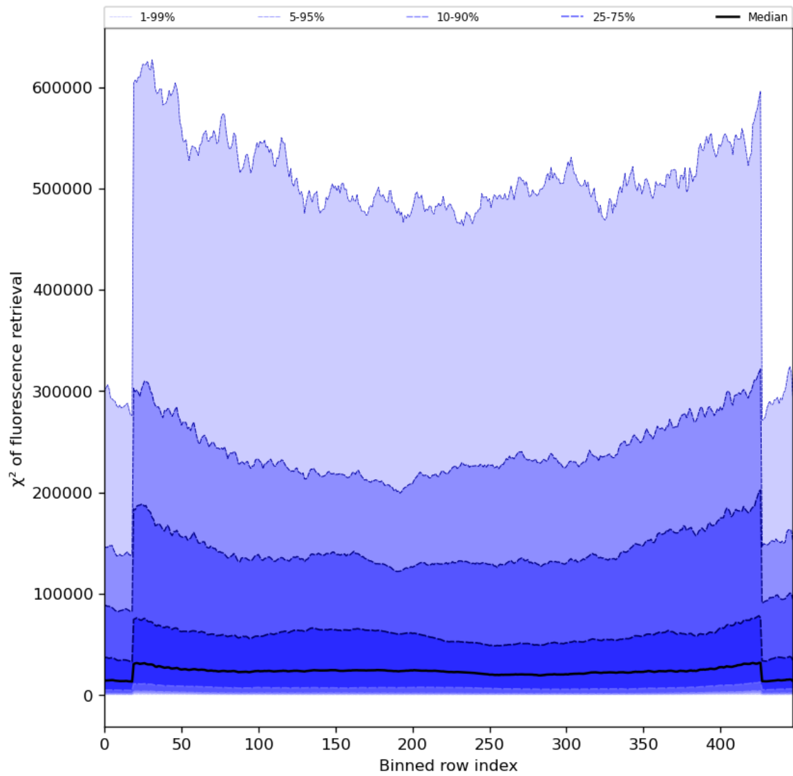
Figure 59: Along track statistics of “ \chi^2 of fluorescence retrieval” for 2024-05-15 to 2024-05-17
