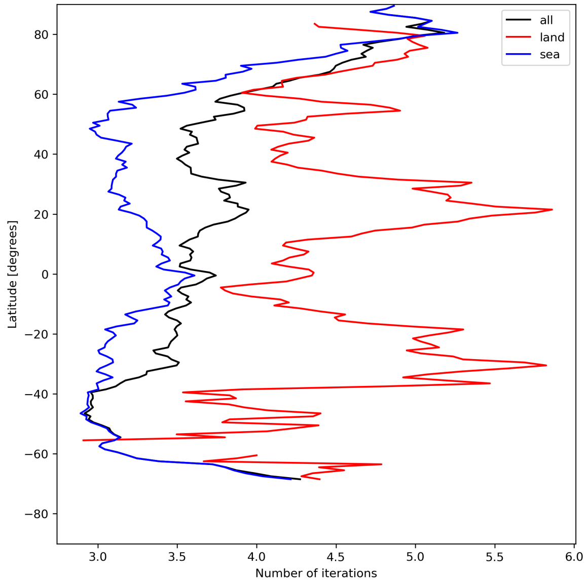
Figure 22: Zonal average of “Number of iterations” for 2024-05-15 to 2024-05-17.
