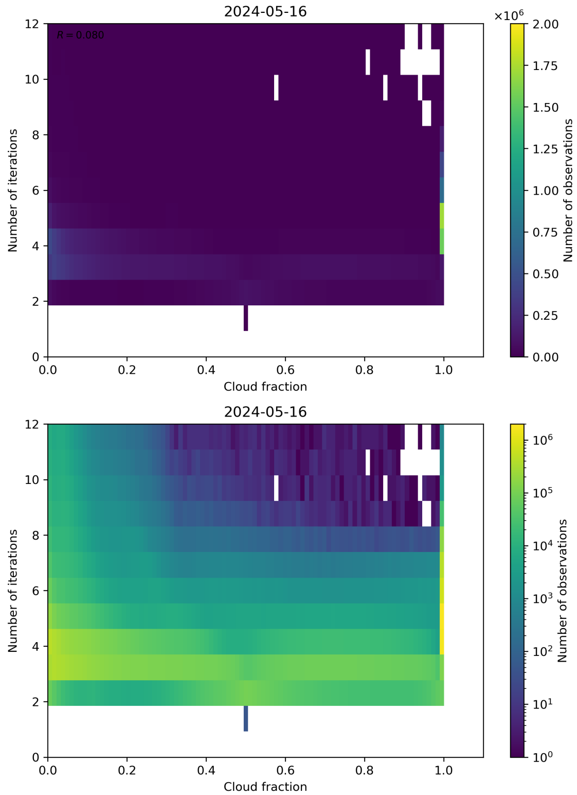
Figure 73: Scatter density plot of “Cloud fraction” against “Number of iterations” for 2024-05-15 to 2024-05-17.
