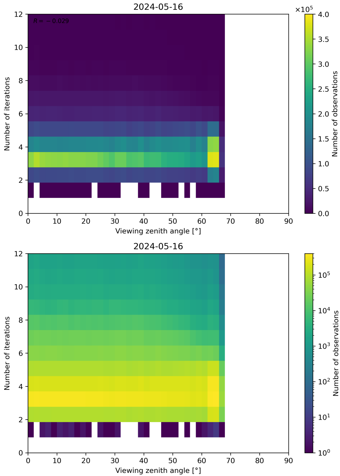
Figure 124: Scatter density plot of “Viewing zenith angle” against “Number of iterations” for 2024-05-15 to 2024-05-17.
