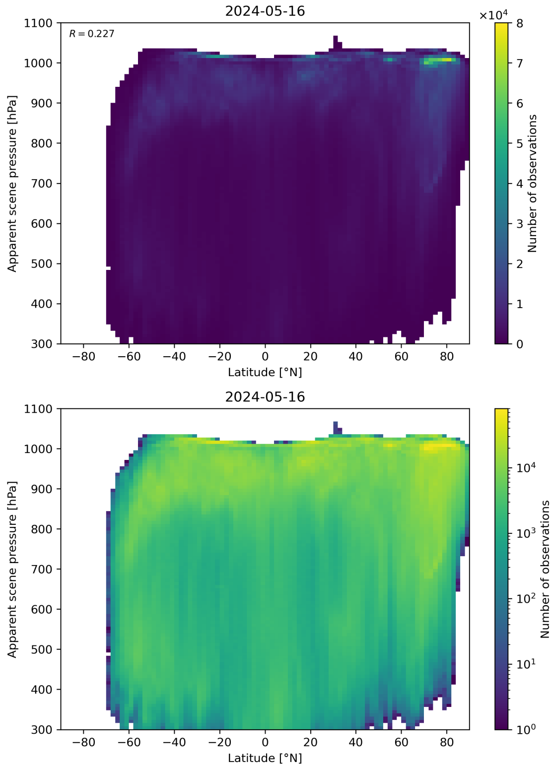
Figure 88: Scatter density plot of “Latitude” against “Apparent scene pressure” for 2024-05-15 to 2024-05-17.
