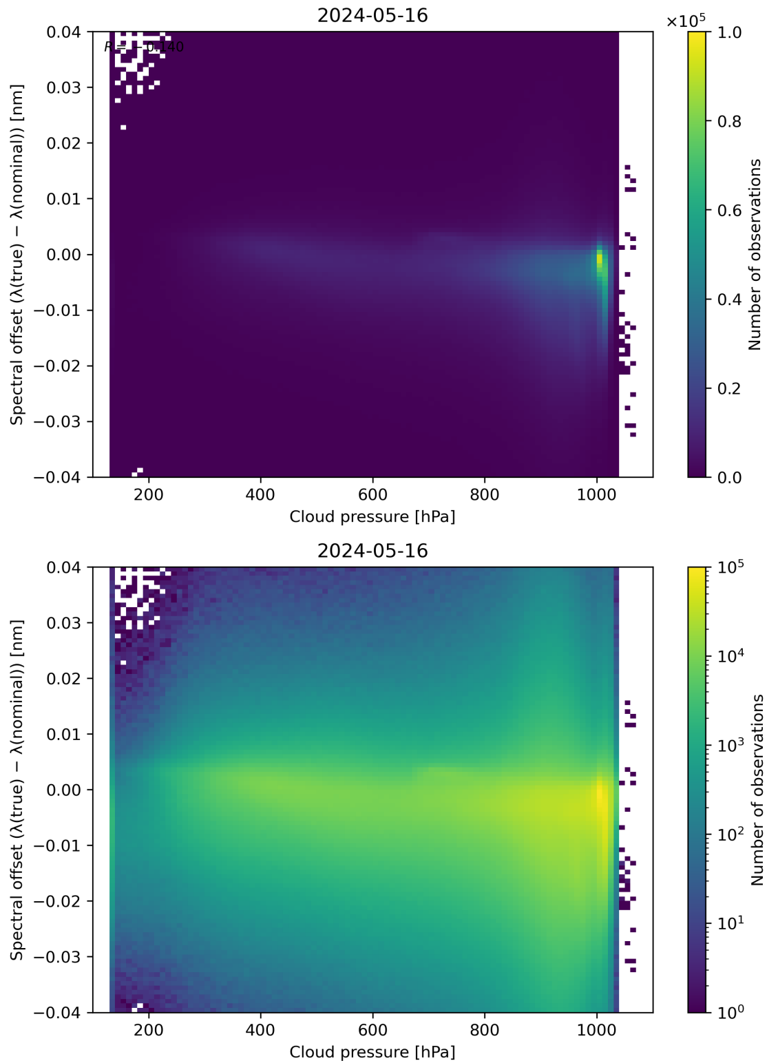
Figure 84: Scatter density plot of “Cloud pressure” against “Spectral offset ( \lambda(\text{true}) - \lambda(\text{nominal}) )” for 2024-05-15 to 2024-05-17.
