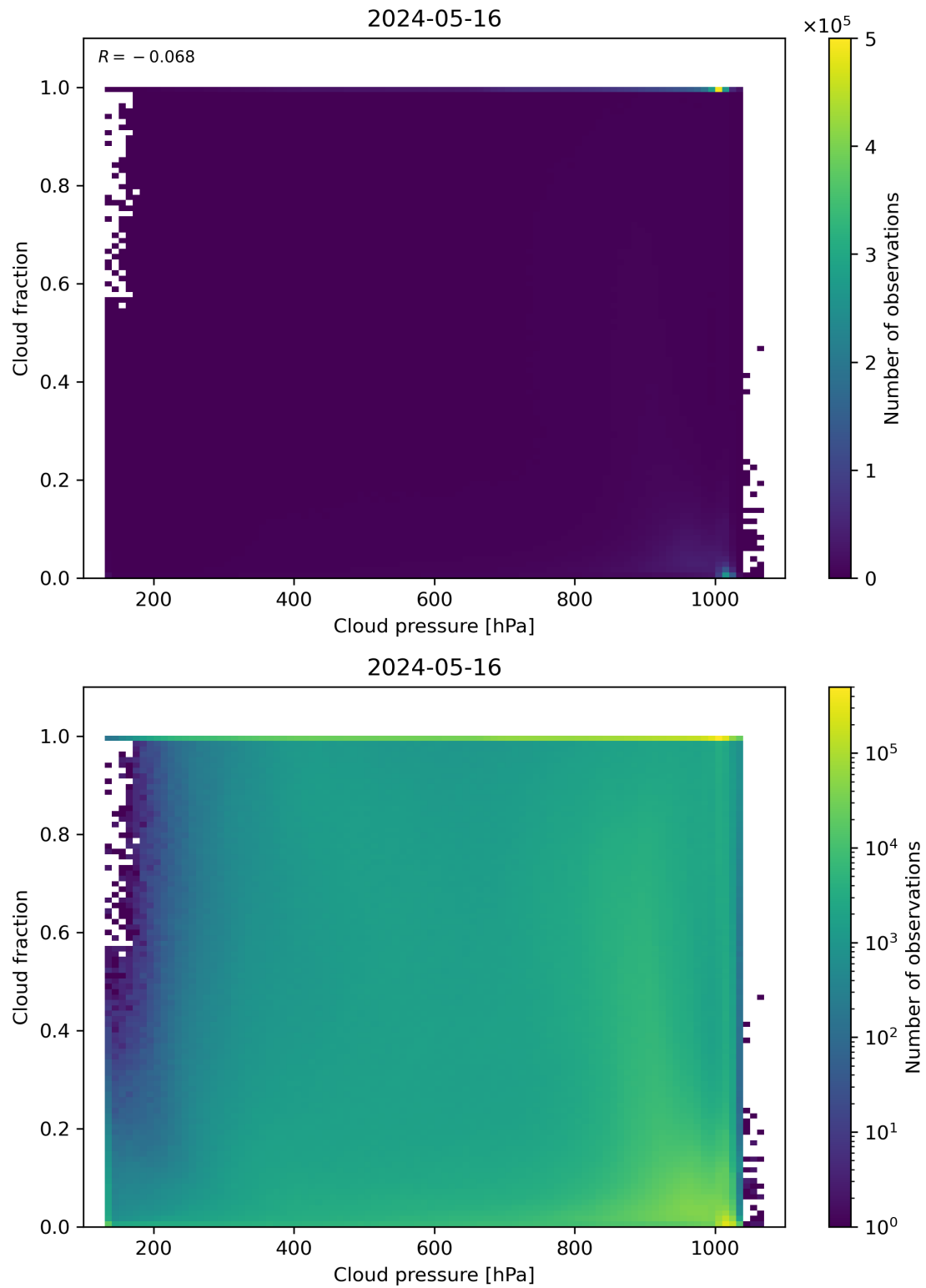
Figure 79: Scatter density plot of “Cloud pressure” against “Cloud fraction” for 2024-05-15 to 2024-05-17.
