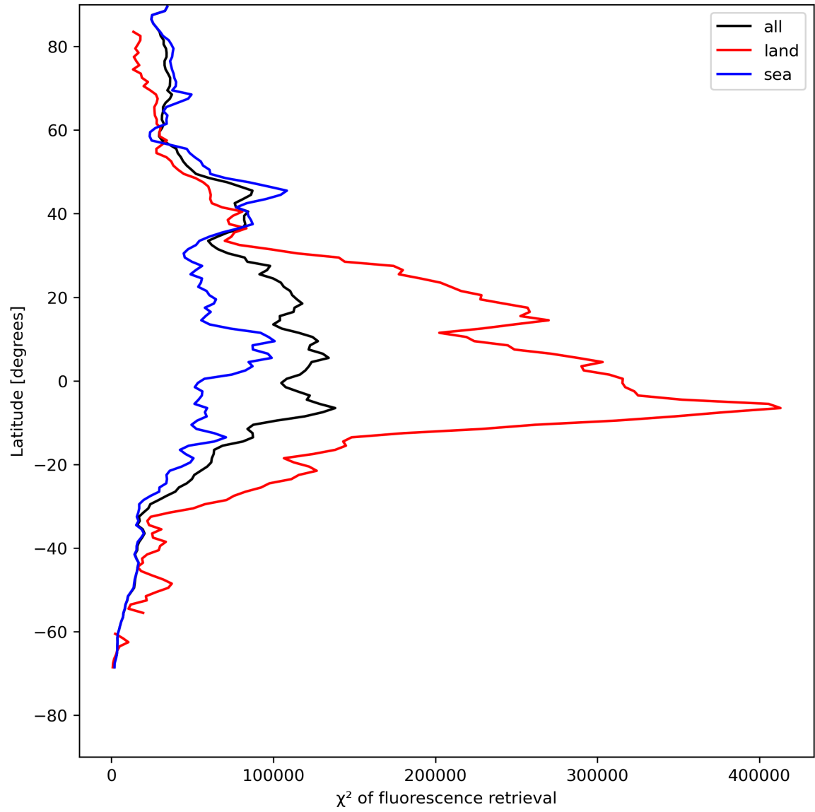
Figure 25: Zonal average of “ \chi^2 of fluorescence retrieval” for 2024-05-15 to 2024-05-17.
