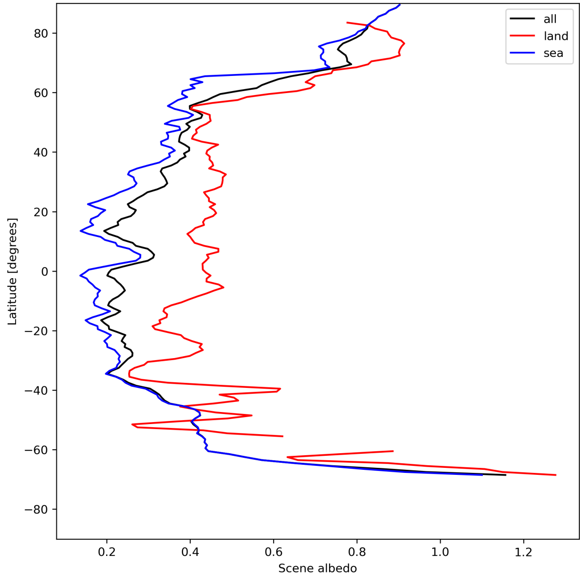
Figure 17: Zonal average of “Scene albedo” for 2024-05-15 to 2024-05-17.
