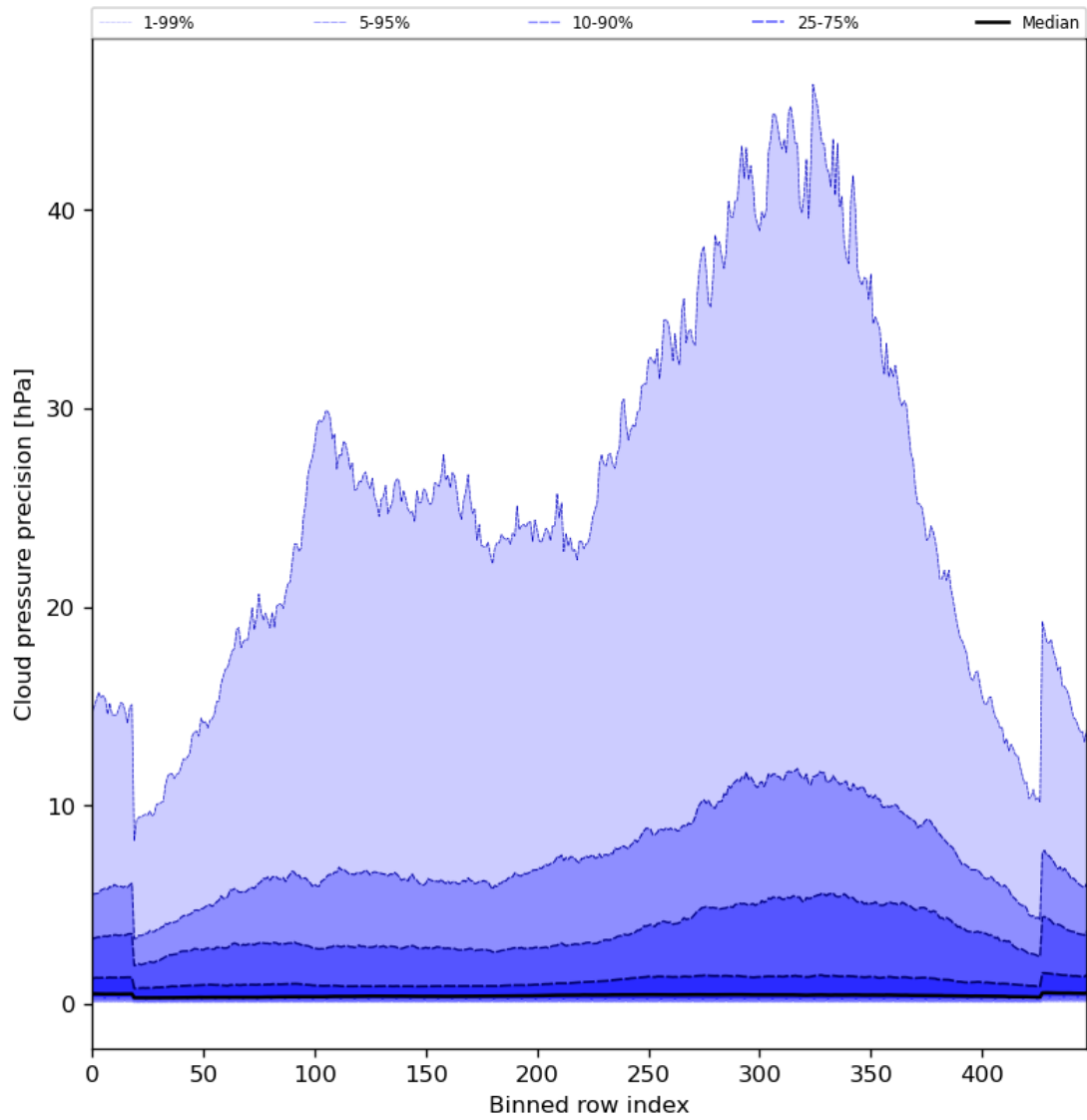
Figure 48: Along track statistics of “Cloud pressure precision” for 2024-05-15 to 2024-05-17
