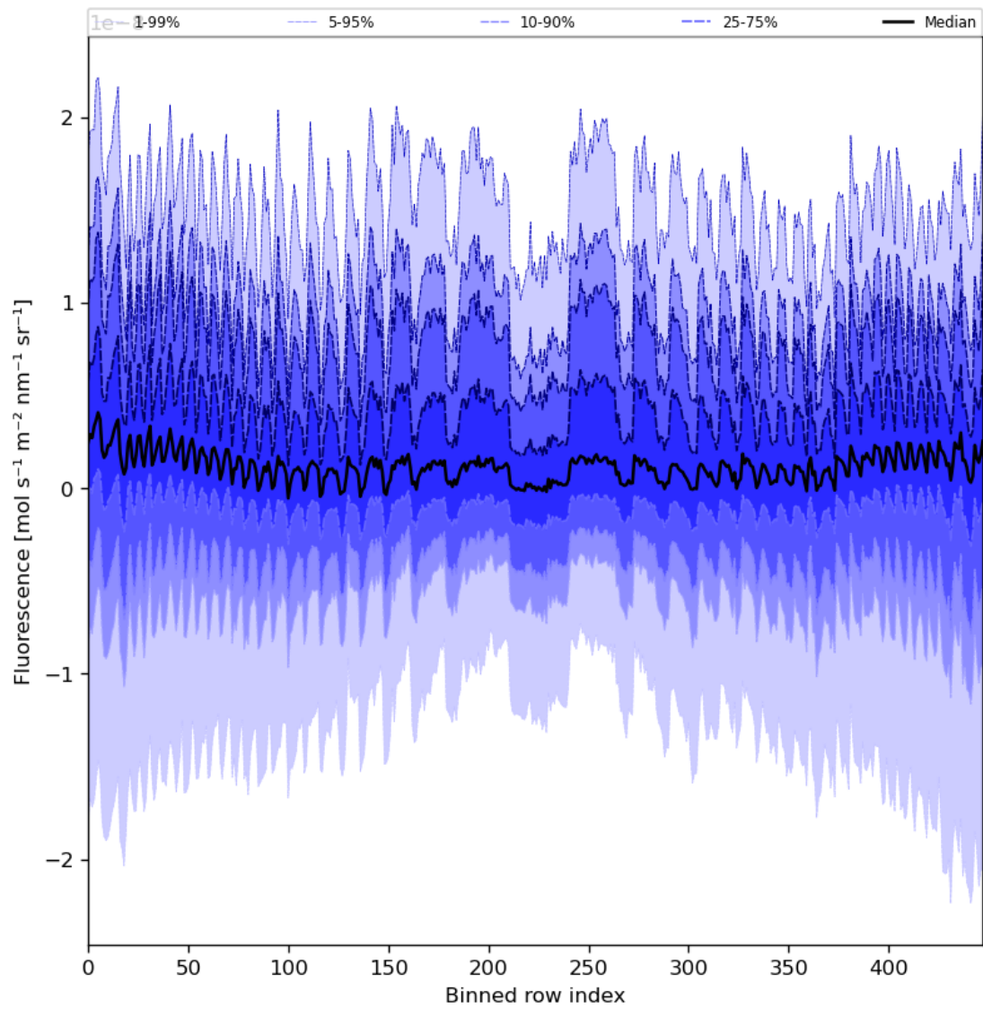
Figure 57: Along track statistics of “Fluorescence” for 2024-05-15 to 2024-05-17
