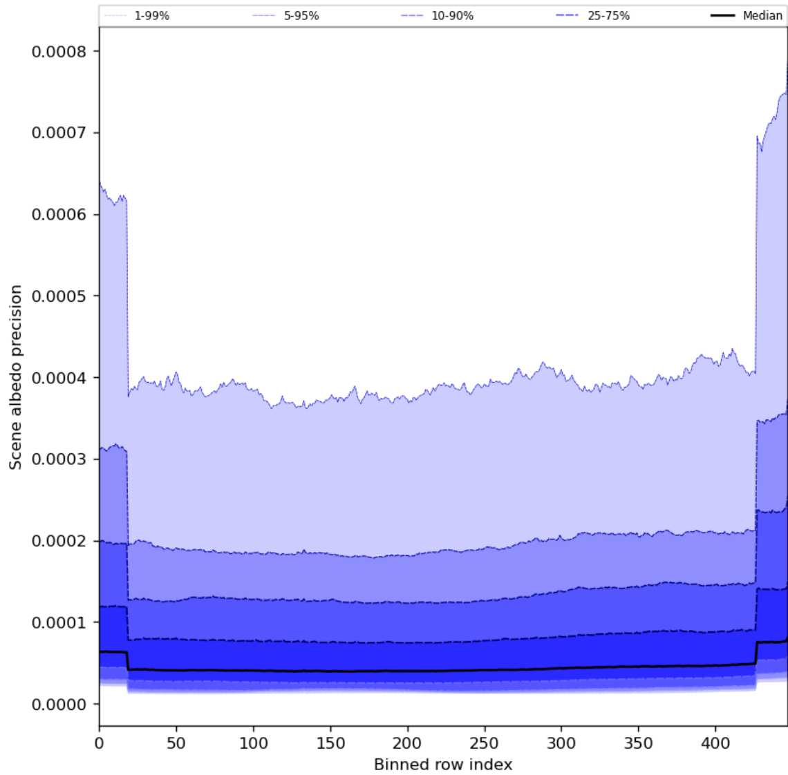
Figure 52: Along track statistics of “Scene albedo precision” for 2024-05-15 to 2024-05-17
