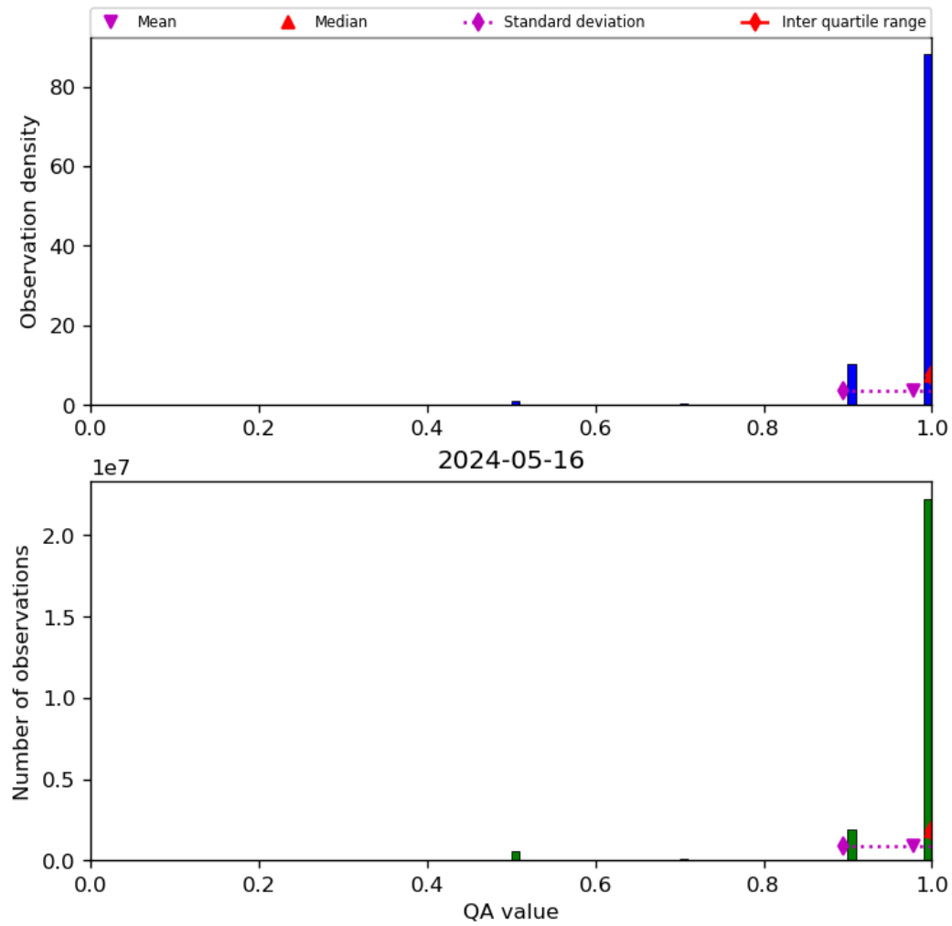
Figure 29: Histogram of “QA value” for 2024-05-15 to 2024-05-17
