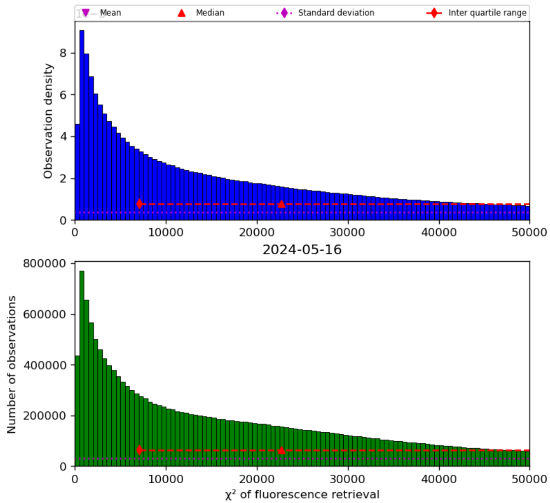
Figure 42: Histogram of “ \chi^2 of fluorescence retrieval” for 2024-05-15 to 2024-05-17
