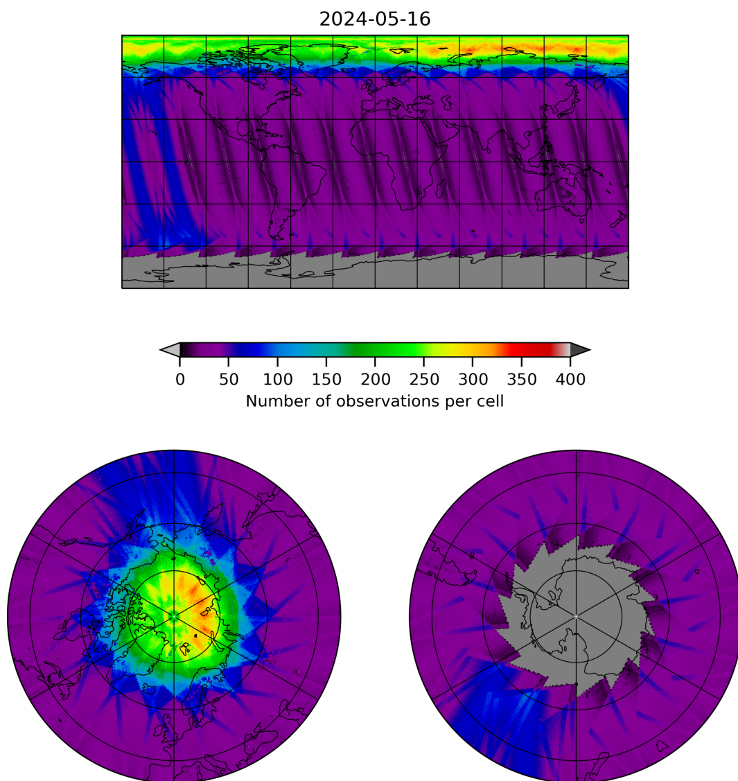
Figure 11: Map of the number of observations for 2024-05-15 to 2024-05-17
