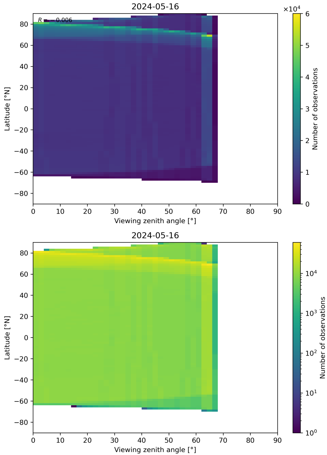
Figure 123: Scatter density plot of “Viewing zenith angle” against “Latitude” for 2024-05-15 to 2024-05-17.
