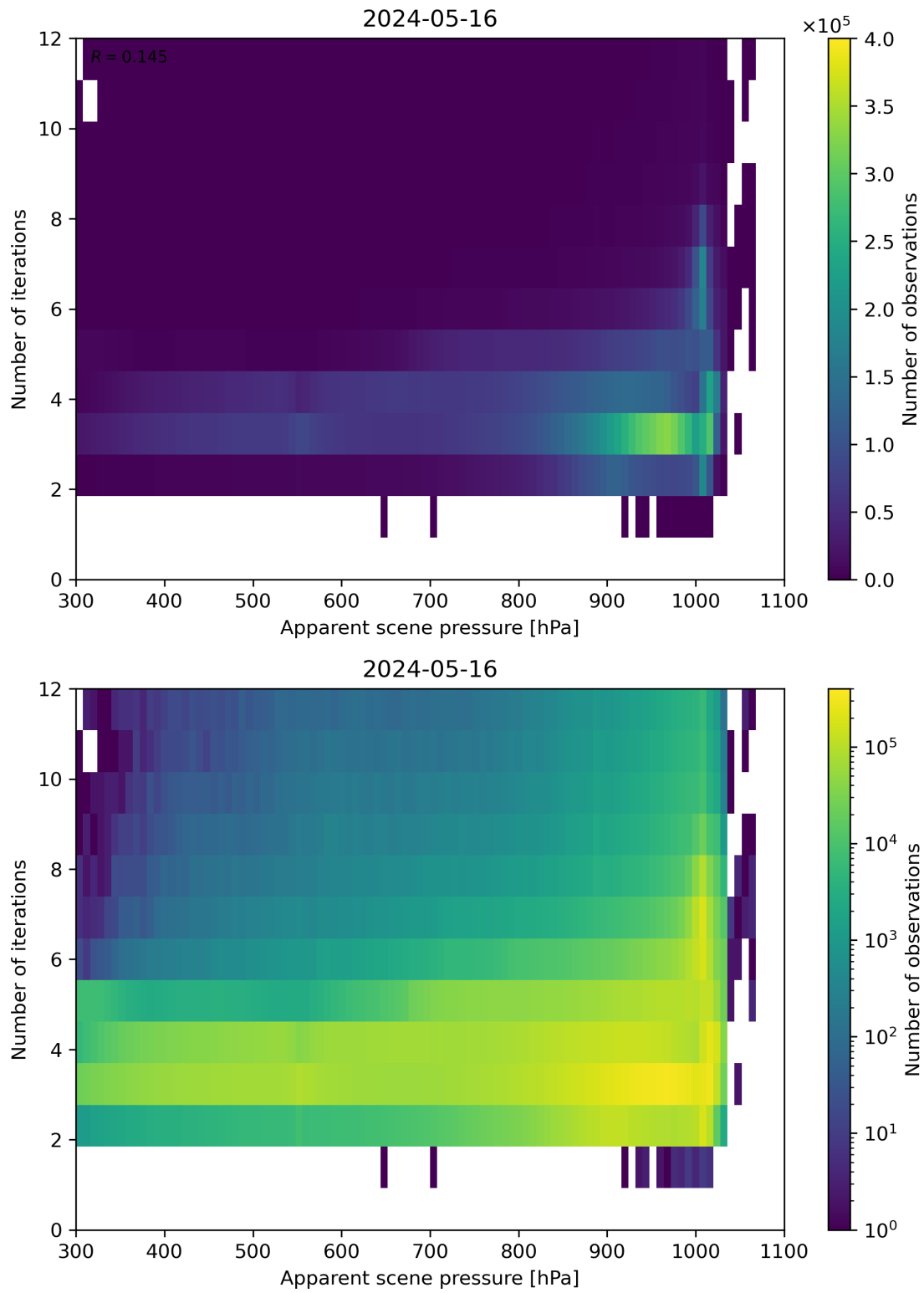
Figure 65: Scatter density plot of “Apparent scene pressure” against “Number of iterations” for 2024-05-15 to 2024-05-17.
