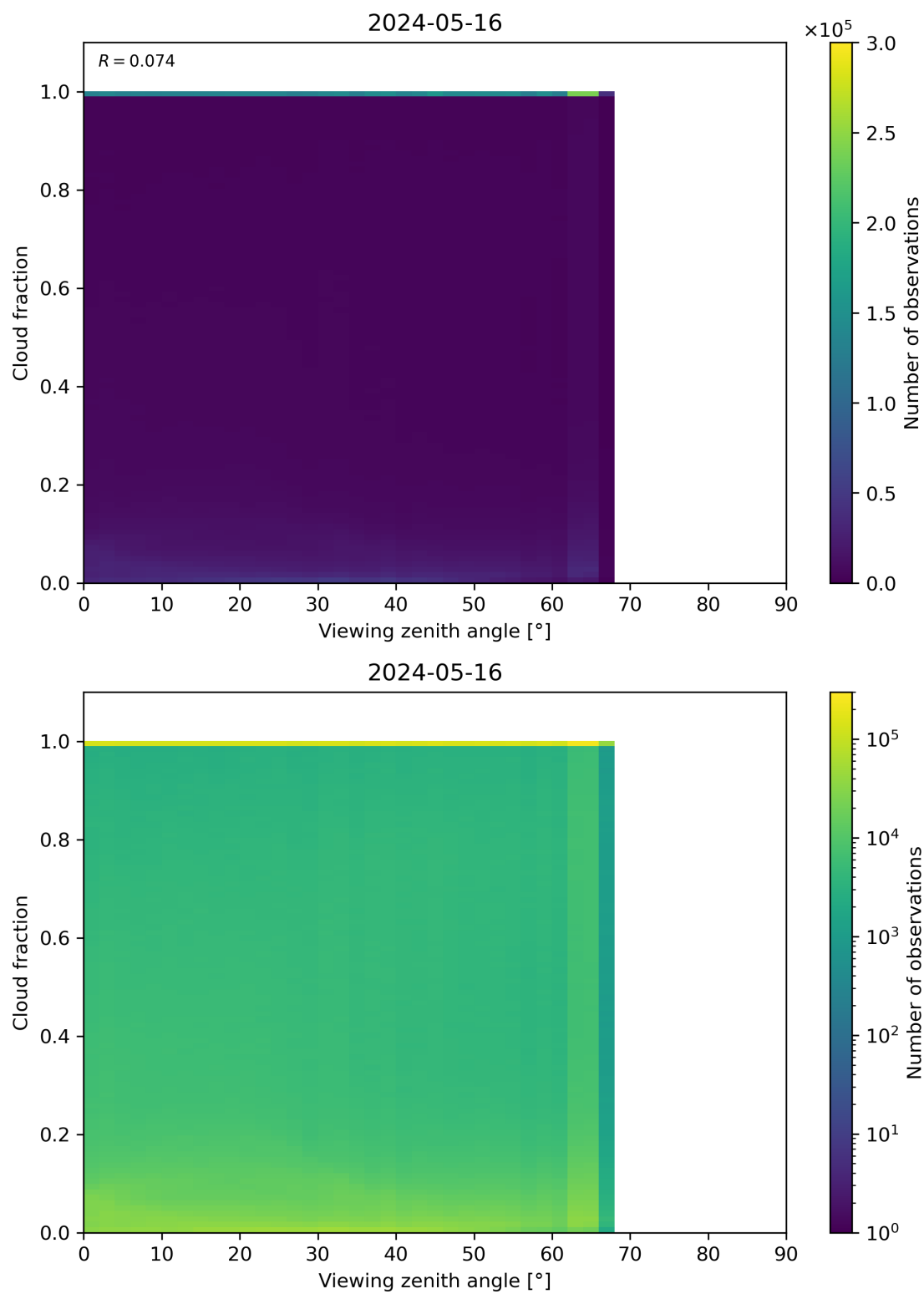
Figure 120: Scatter density plot of “Viewing zenith angle” against “Cloud fraction” for 2024-05-15 to 2024-05-17.
