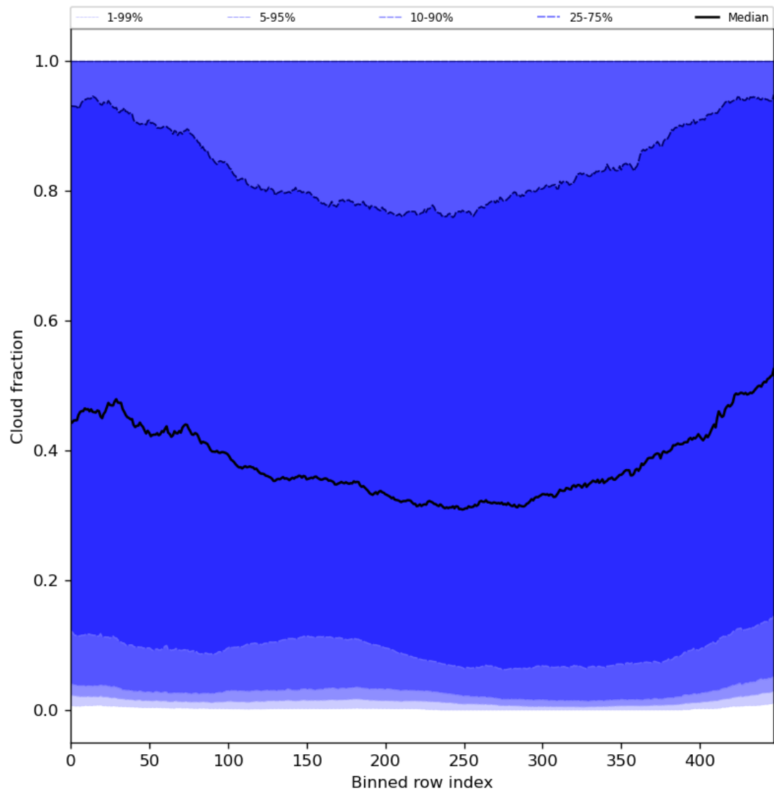
Figure 49: Along track statistics of “Cloud fraction” for 2024-05-15 to 2024-05-17
