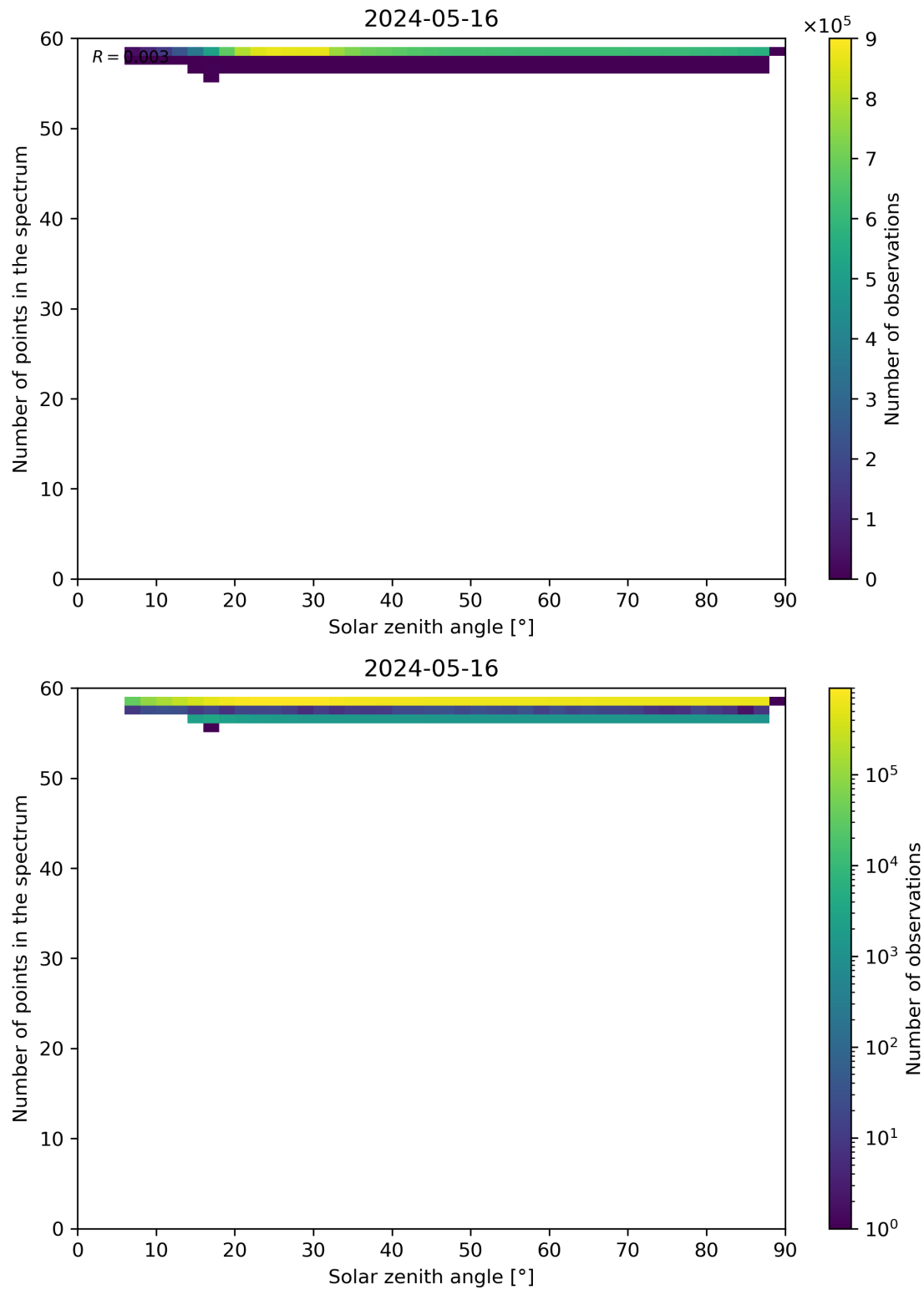
Figure 115: Scatter density plot of “Solar zenith angle” against “Number of points in the spectrum” for 2024-05-15 to 2024-05-17.
