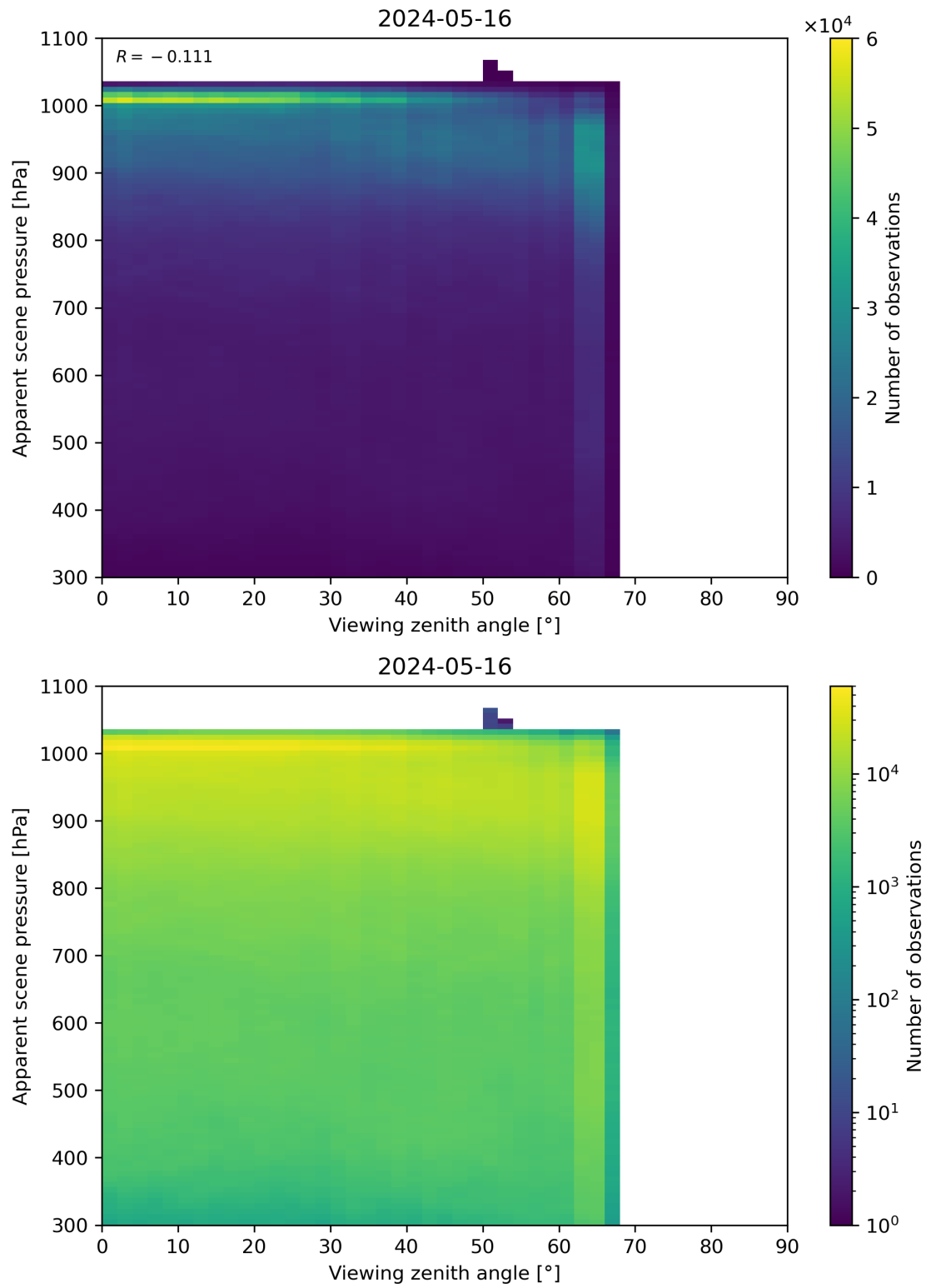
Figure 118: Scatter density plot of “Viewing zenith angle” against “Apparent scene pressure” for 2024-05-15 to 2024-05-17.
