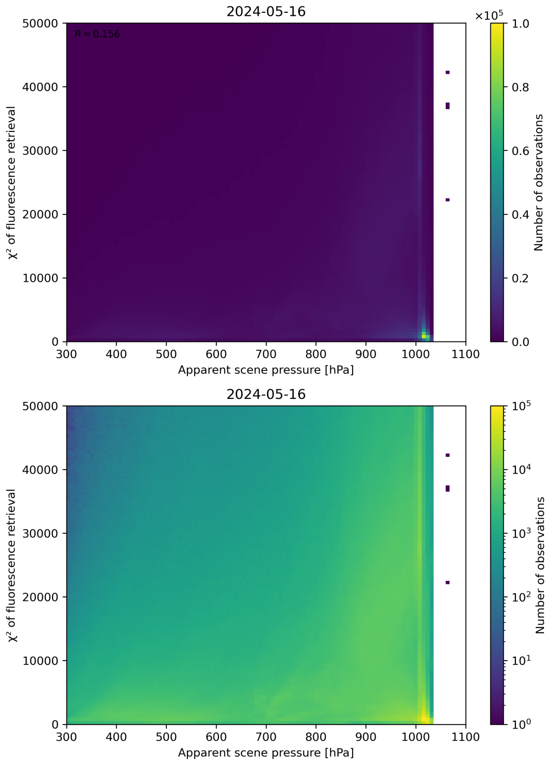
Figure 63: Scatter density plot of “Apparent scene pressure” against “ \chi^2 of fluorescence retrieval” for 2024-05-15 to 2024-05-17.
