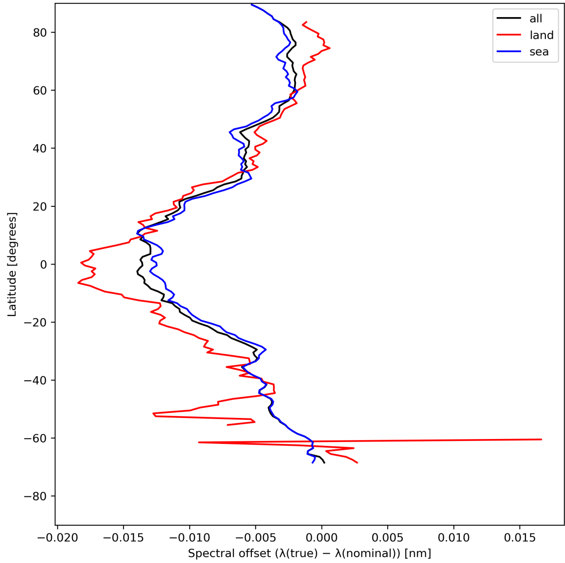
Figure 28: Zonal average of “Spectral offset ( \lambda(\text{true}) - \lambda(\text{nominal}) )” for 2024-05-15 to 2024-05-17.
