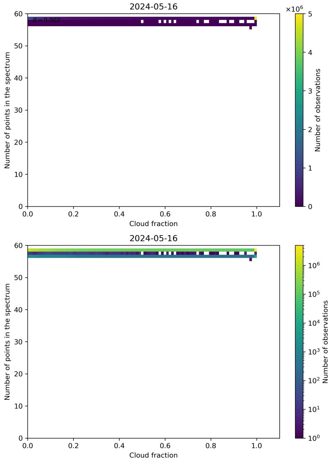
Figure 74: Scatter density plot of “Cloud fraction” against “Number of points in the spectrum” for 2024-05-15 to 2024-05-17.
