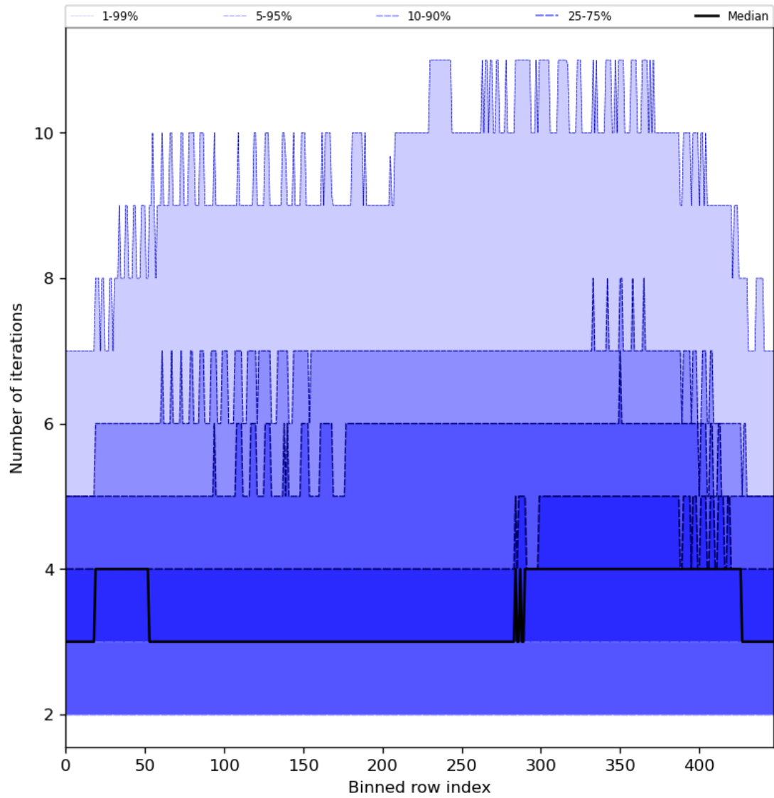
Figure 56: Along track statistics of “Number of iterations” for 2024-05-15 to 2024-05-17
