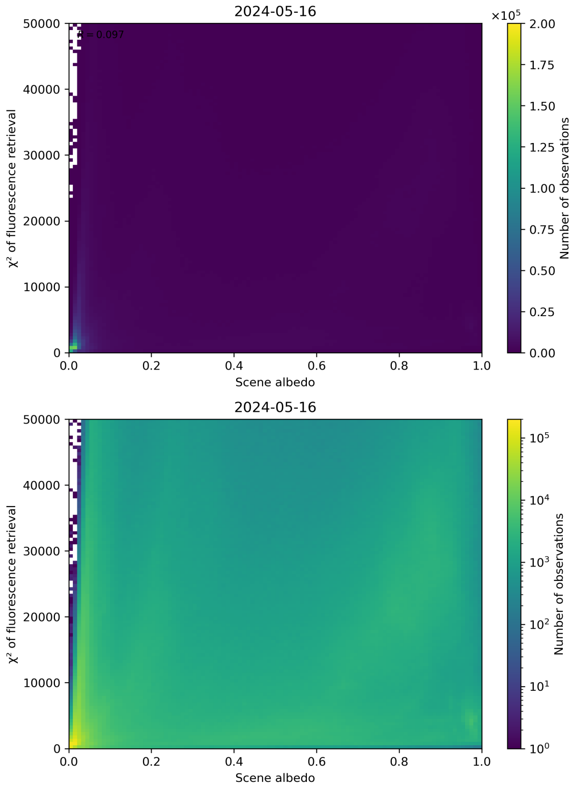
Figure 103: Scatter density plot of “Scene albedo” against “ \chi^2 of fluorescence retrieval” for 2024-05-15 to 2024-05-17.
