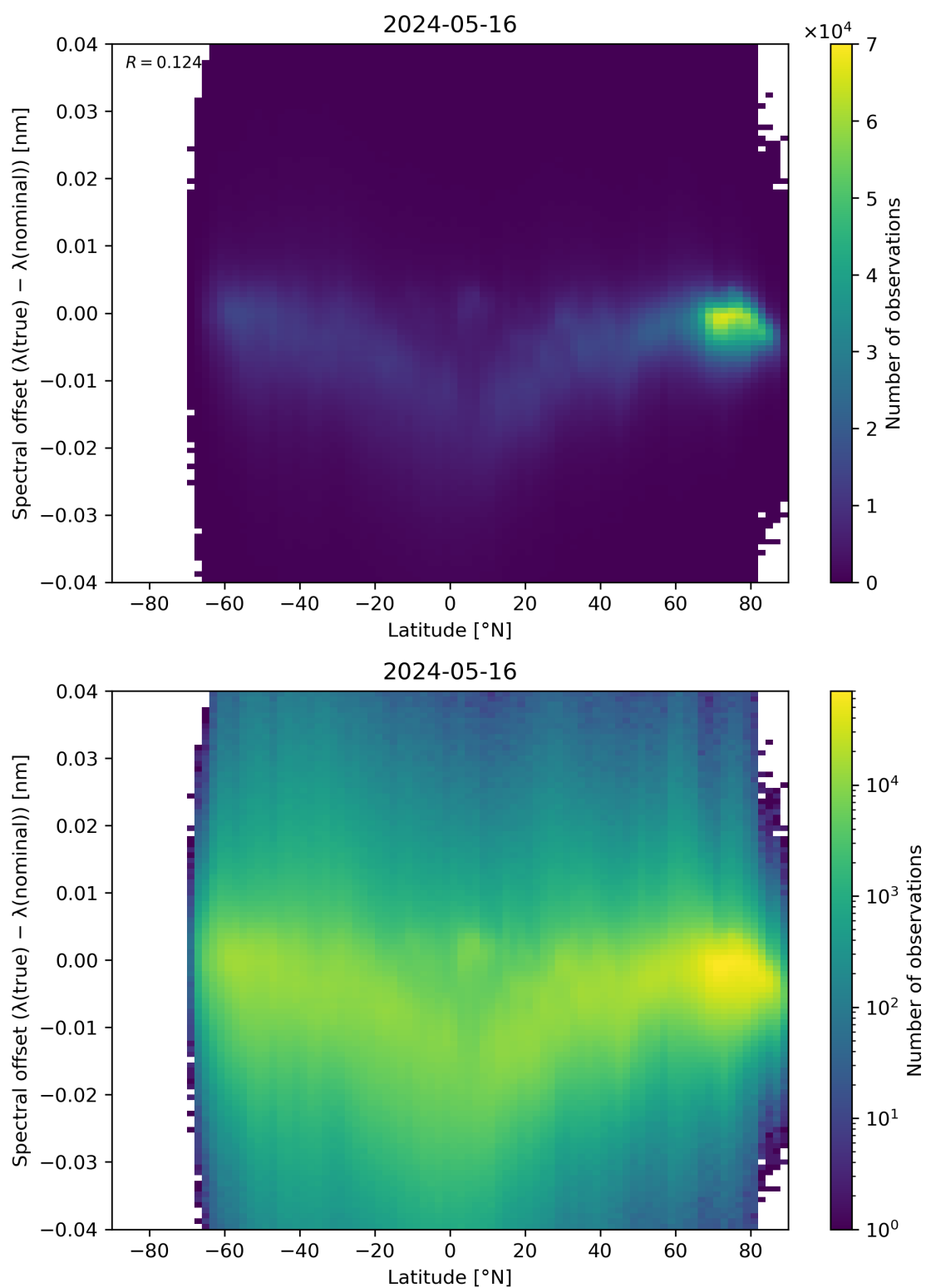
Figure 96: Scatter density plot of “Latitude” against “Spectral offset ( \lambda(\text{true}) - \lambda(\text{nominal}) )” for 2024-05-15 to 2024-05-17.
