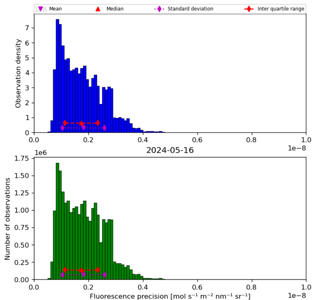
Figure 41: Histogram of “Fluorescence precision” for 2024-05-15 to 2024-05-17
