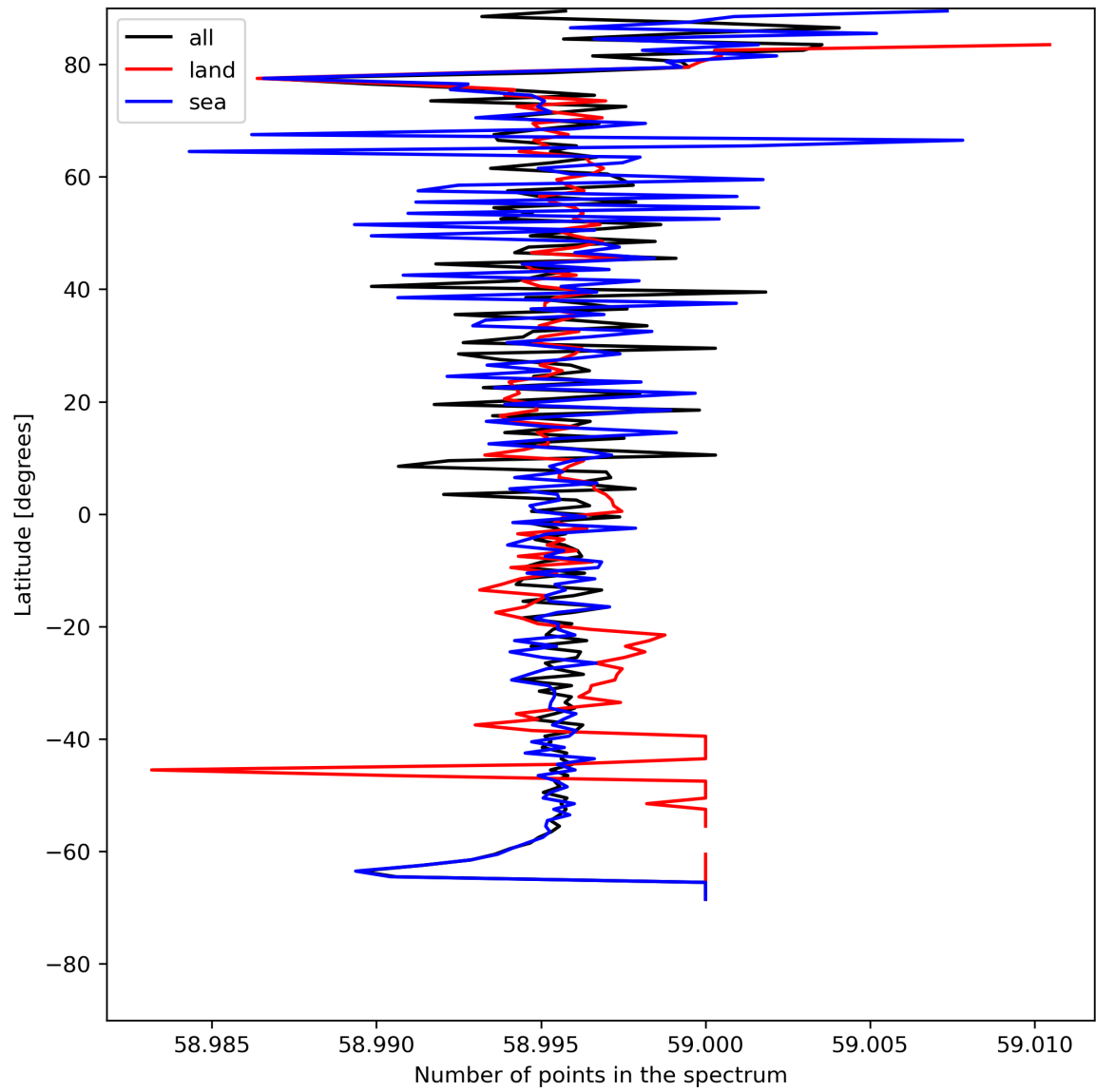
Figure 27: Zonal average of “Number of points in the spectrum” for 2024-05-15 to 2024-05-17.
