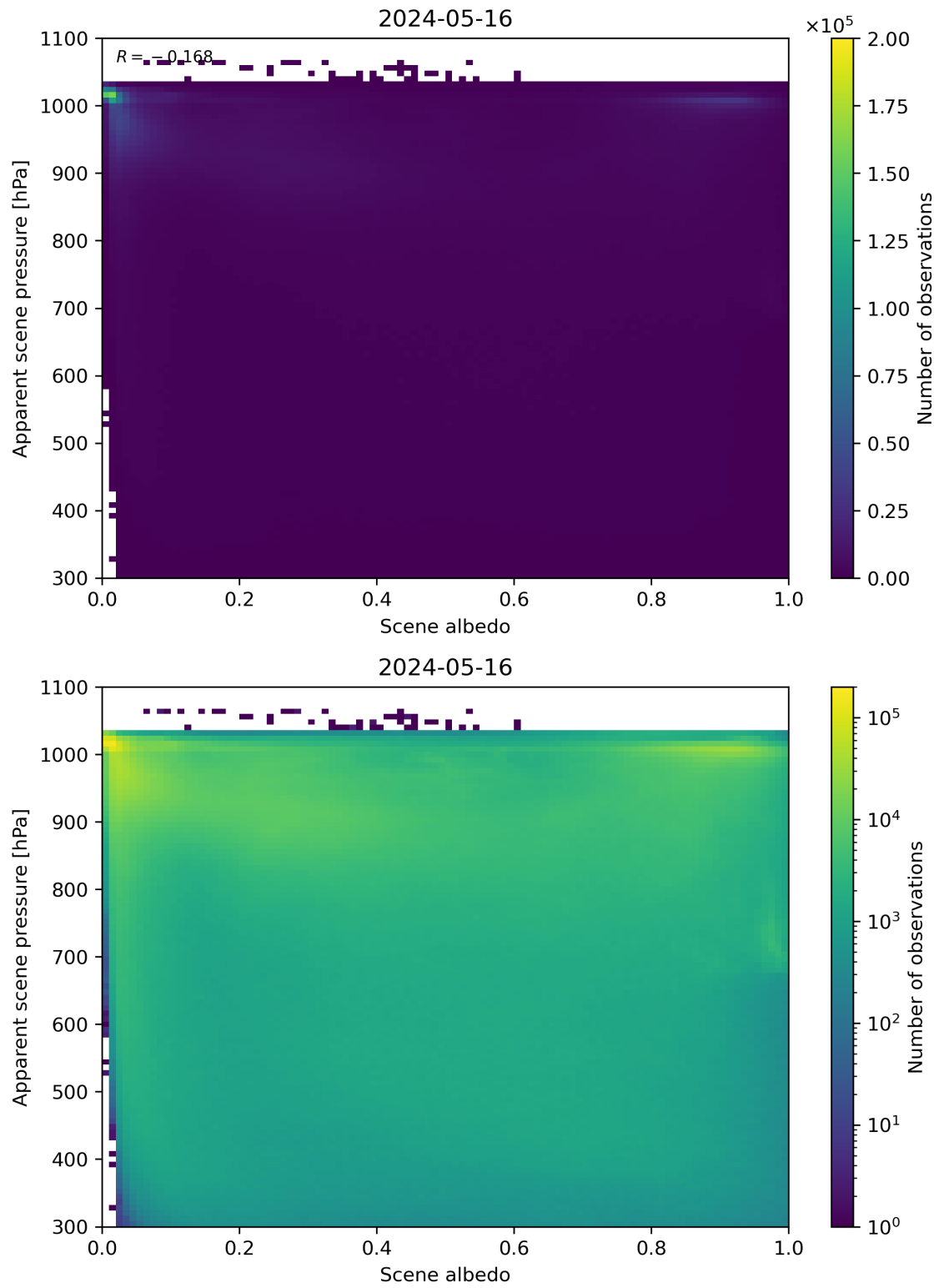
Figure 102: Scatter density plot of “Scene albedo” against “Apparent scene pressure” for 2024-05-15 to 2024-05-17.
