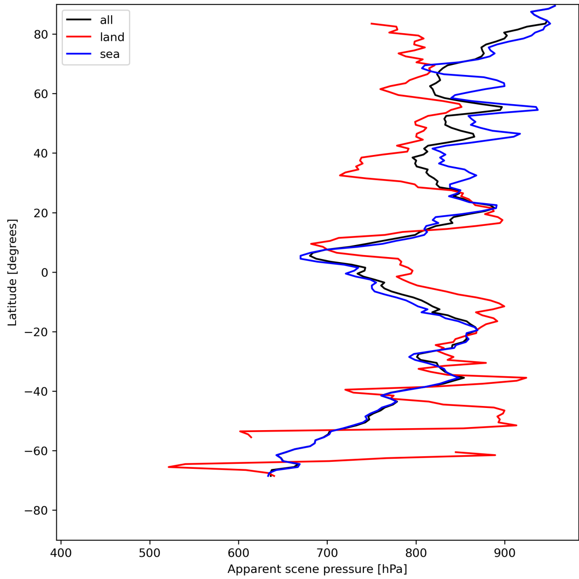
Figure 19: Zonal average of “Apparent scene pressure” for 2024-05-15 to 2024-05-17.
