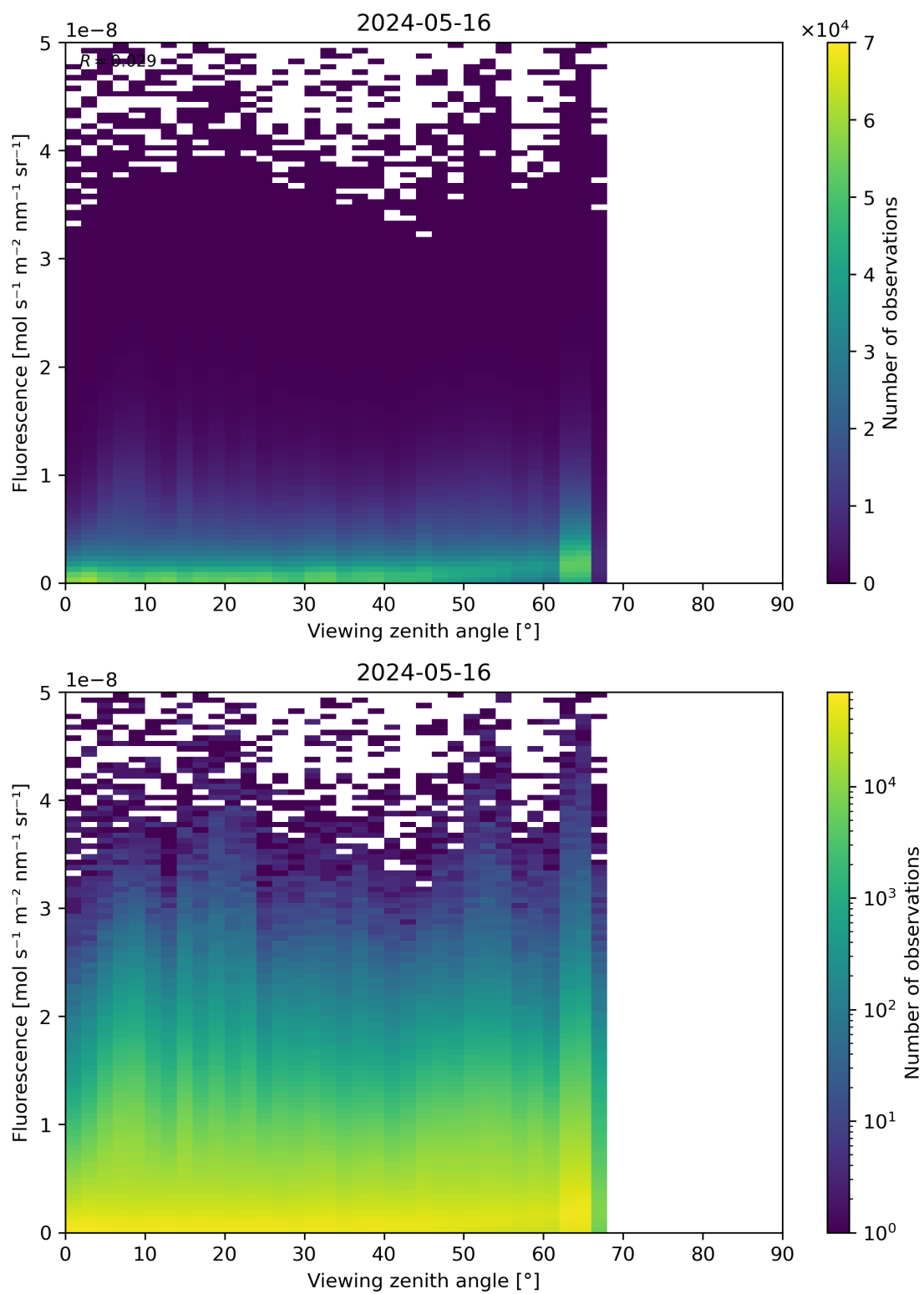
Figure 122: Scatter density plot of “Viewing zenith angle” against “Fluorescence” for 2024-05-15 to 2024-05-17.
