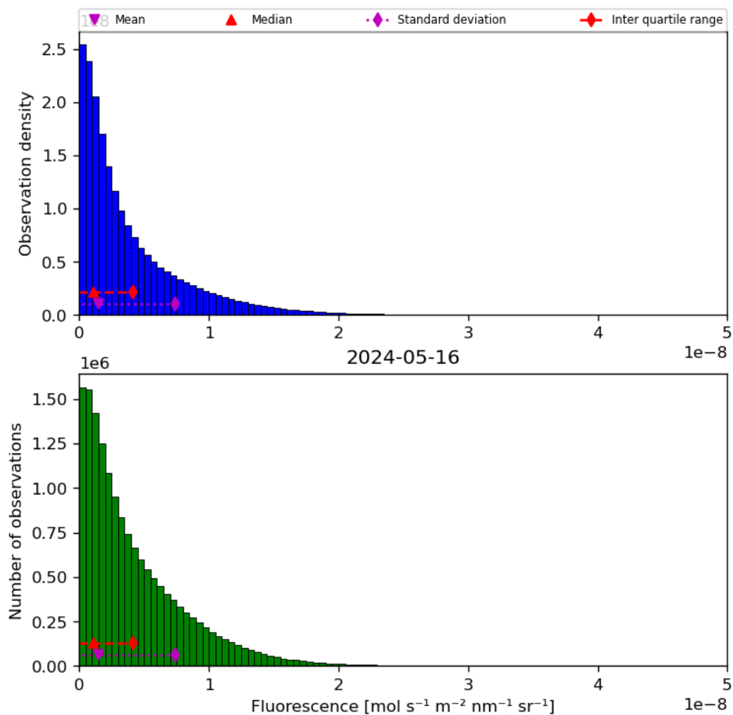
Figure 40: Histogram of “Fluorescence” for 2024-05-15 to 2024-05-17
