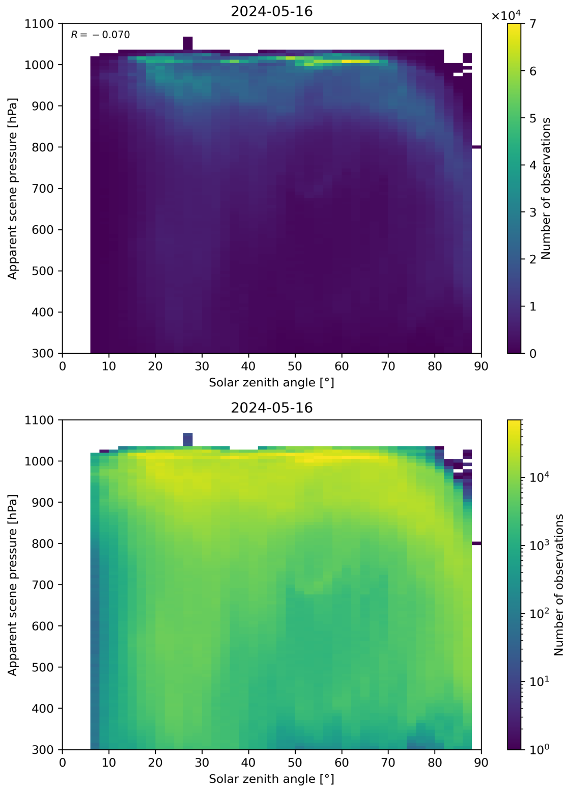
Figure 108: Scatter density plot of “Solar zenith angle” against “Apparent scene pressure” for 2024-05-15 to 2024-05-17.
