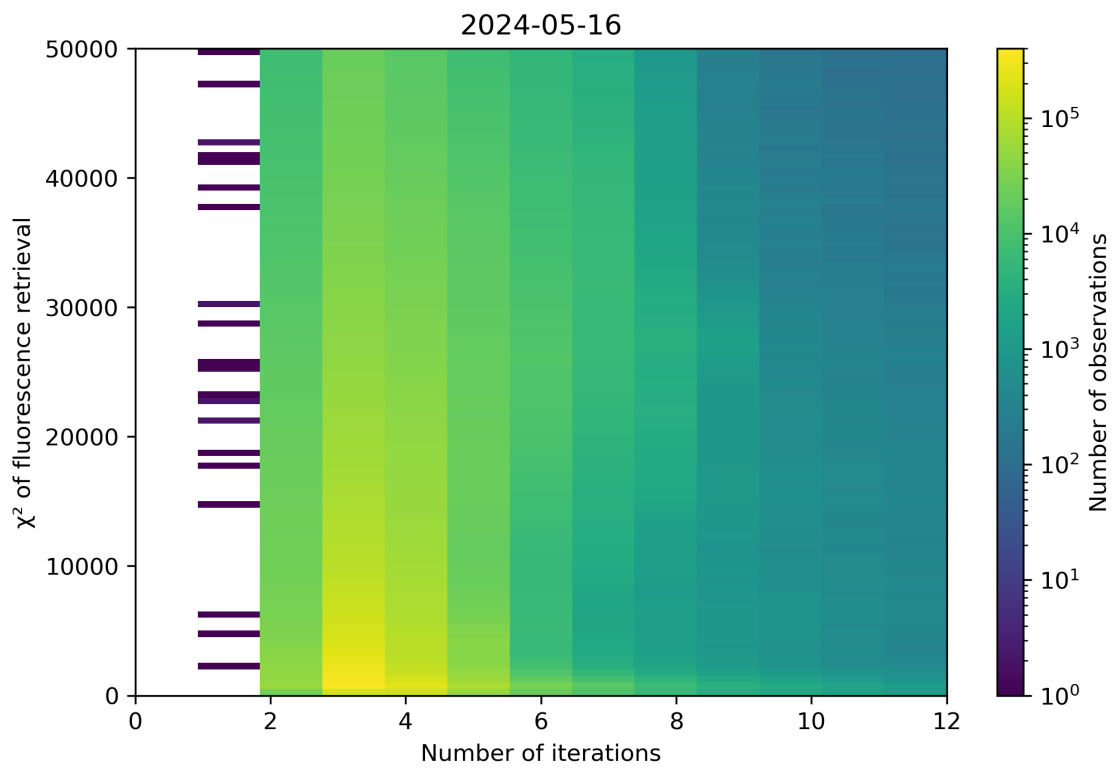
Figure 97: Scatter density plot of “Number of iterations” against “ \chi^2 of fluorescence retrieval” for 2024-05-15 to 2024-05-17.
