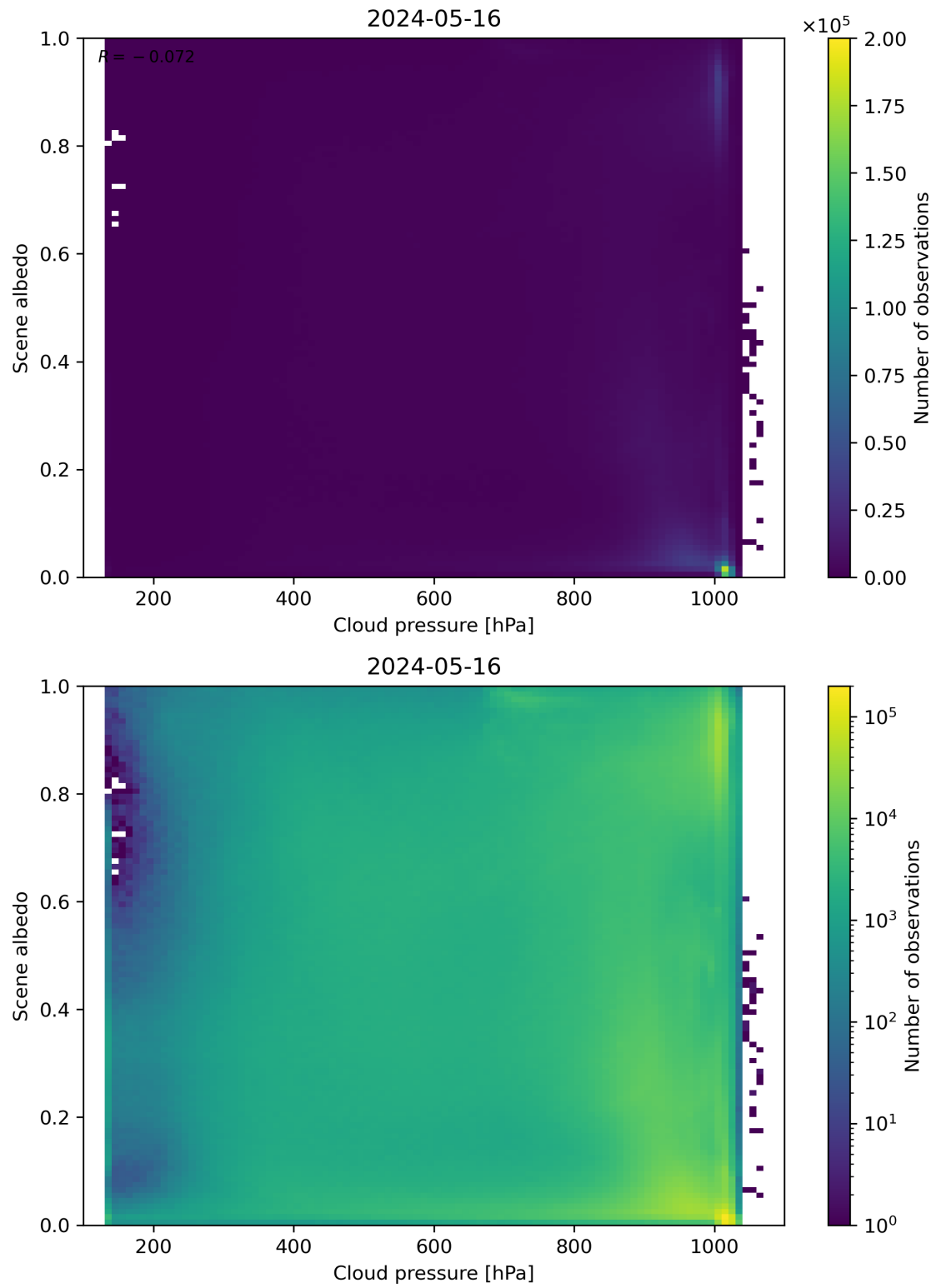
Figure 83: Scatter density plot of “Cloud pressure” against “Scene albedo” for 2024-05-15 to 2024-05-17.
