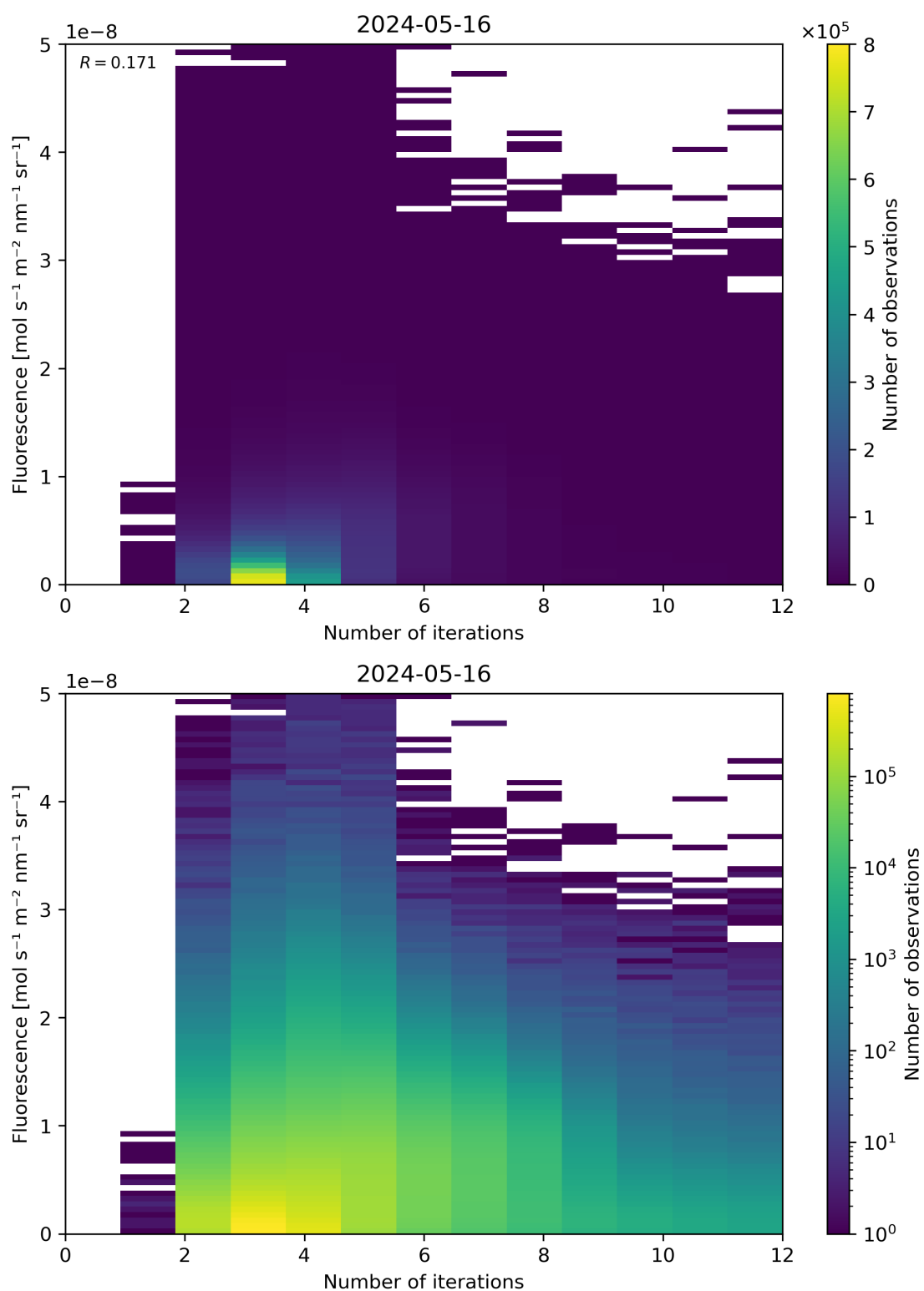
Figure 98: Scatter density plot of “Number of iterations” against “Fluorescence” for 2024-05-15 to 2024-05-17.
