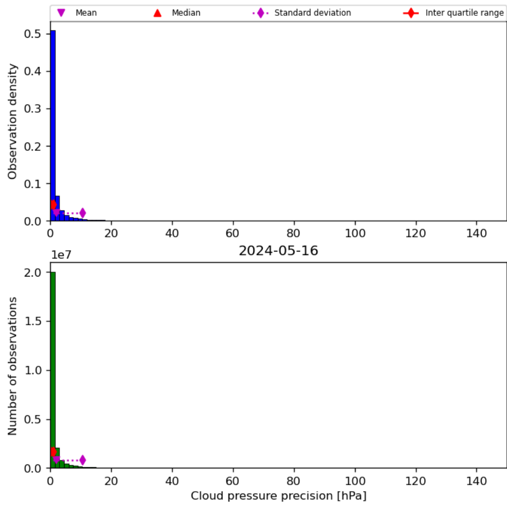
Figure 31: Histogram of “Cloud pressure precision” for 2024-05-15 to 2024-05-17
