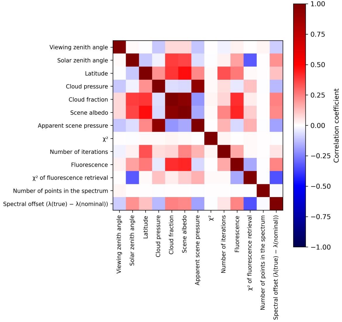
Figure 2: Map of correlation matrix for 2024-05-15 to 2024-05-17.
