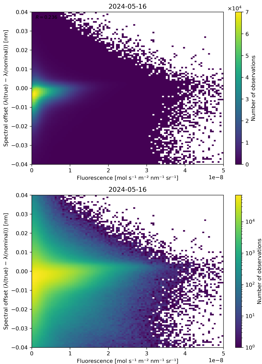
Figure 87: Scatter density plot of “Fluorescence” against “Spectral offset ( \lambda(\text{true}) - \lambda(\text{nominal}) )” for 2024-05-15 to 2024-05-17.
