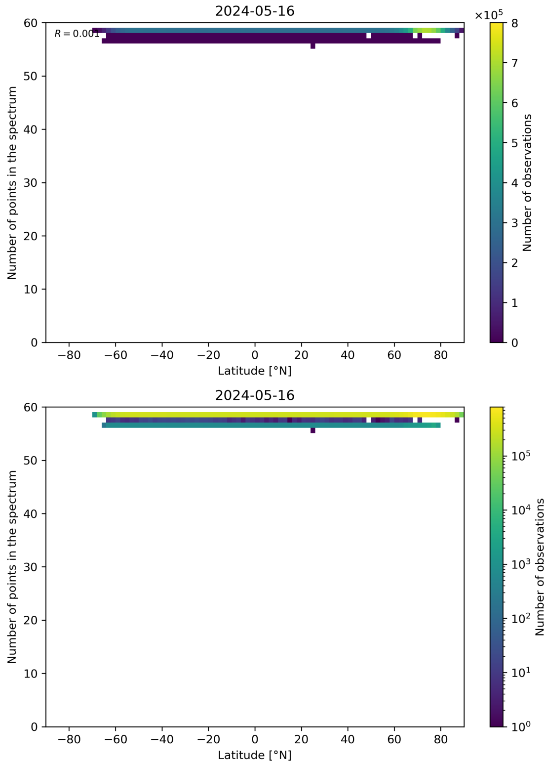
Figure 94: Scatter density plot of “Latitude” against “Number of points in the spectrum” for 2024-05-15 to 2024-05-17.
