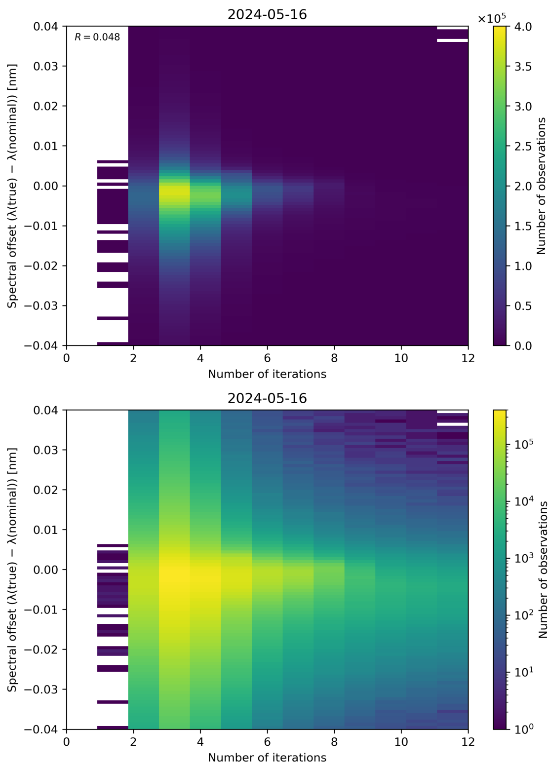
Figure 100: Scatter density plot of “Number of iterations” against “Spectral offset ( \lambda(\text{true}) - \lambda(\text{nominal}) )” for 2024-05-15 to 2024-05-17.
