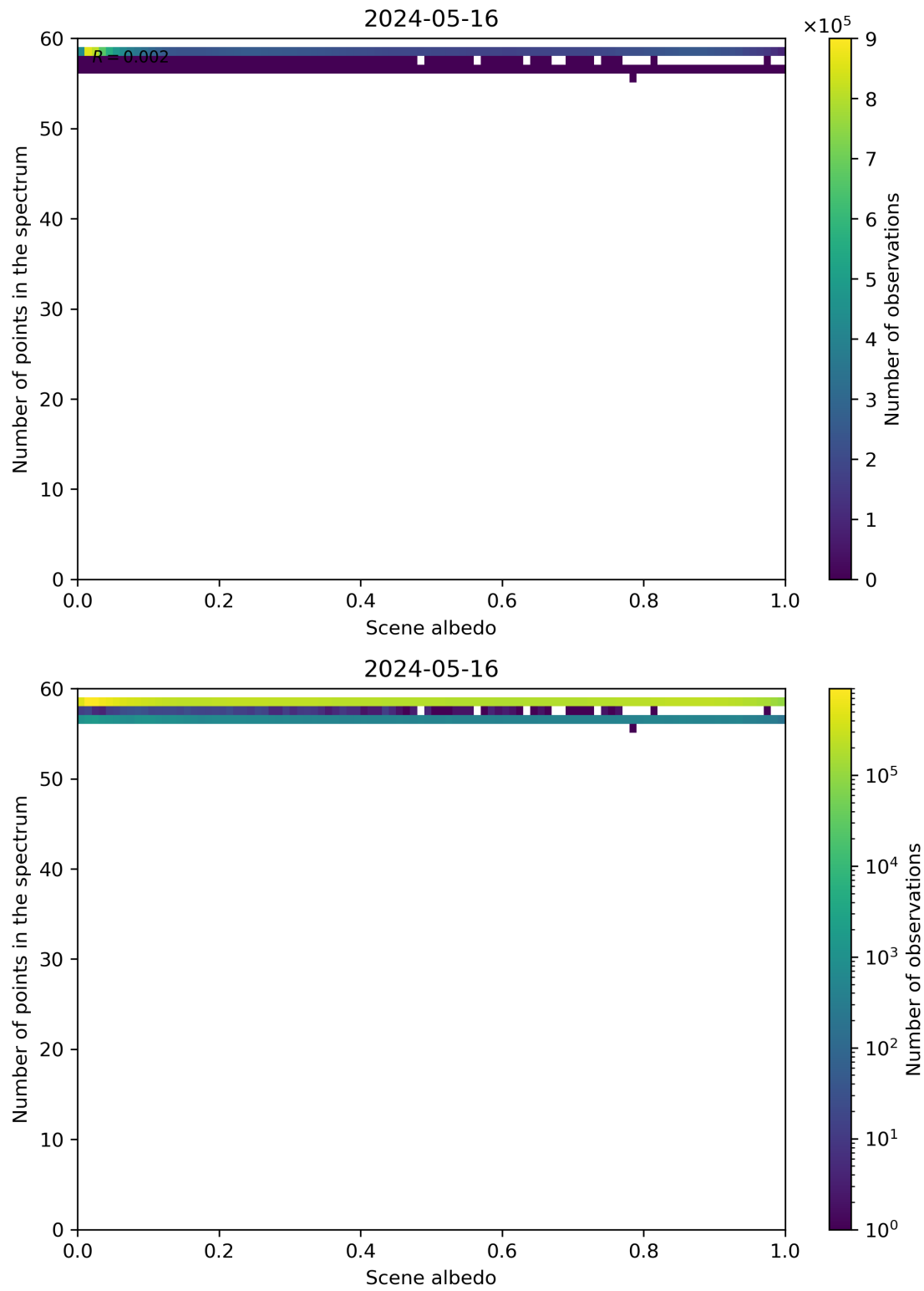
Figure 106: Scatter density plot of “Scene albedo” against “Number of points in the spectrum” for 2024-05-15 to 2024-05-17.
