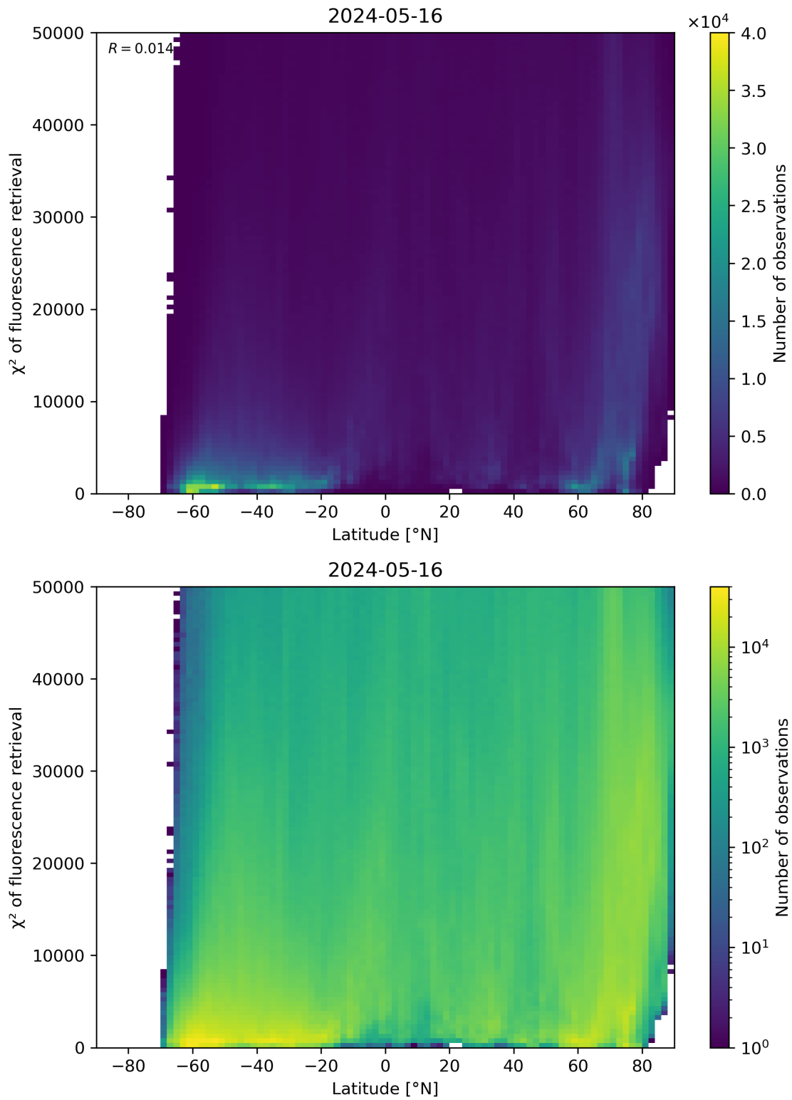
Figure 89: Scatter density plot of “Latitude” against “ \chi^2 of fluorescence retrieval” for 2024-05-15 to 2024-05-17.
