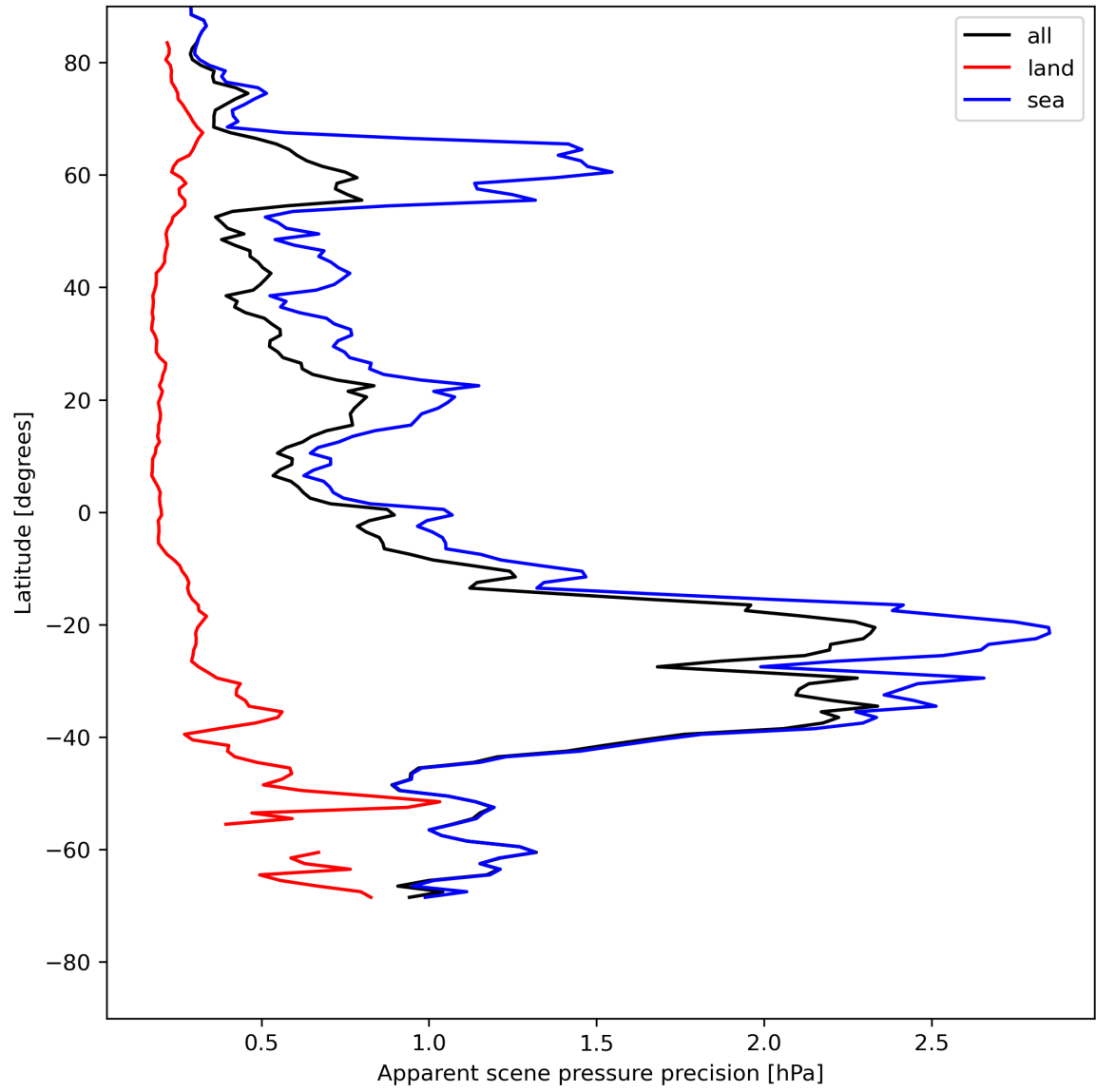
Figure 20: Zonal average of “Apparent scene pressure precision” for 2024-05-15 to 2024-05-17.
