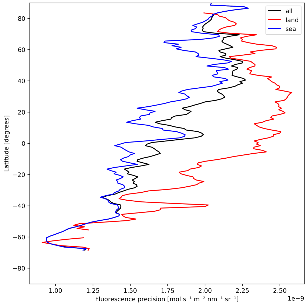
Figure 24: Zonal average of “Fluorescence precision” for 2024-05-15 to 2024-05-17.
