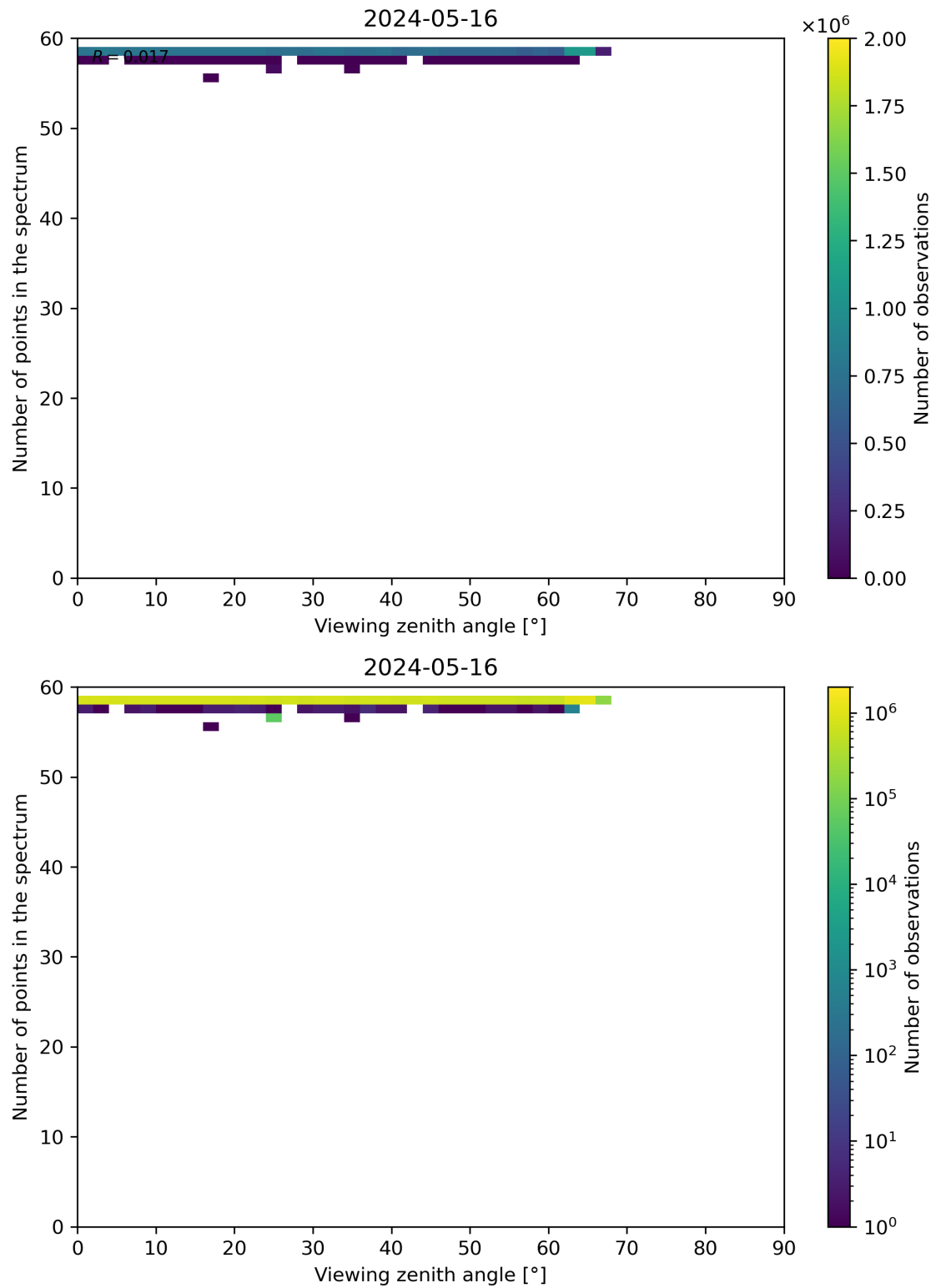
Figure 125: Scatter density plot of “Viewing zenith angle” against “Number of points in the spectrum” for 2024-05-15 to 2024-05-17.
