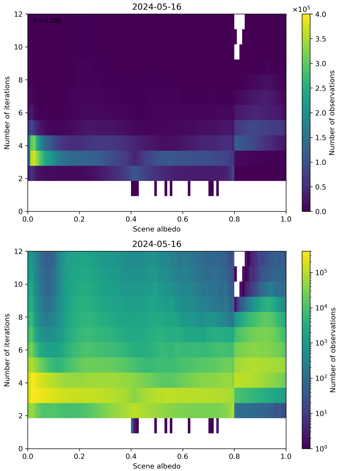
Figure 105: Scatter density plot of “Scene albedo” against “Number of iterations” for 2024-05-15 to 2024-05-17.
