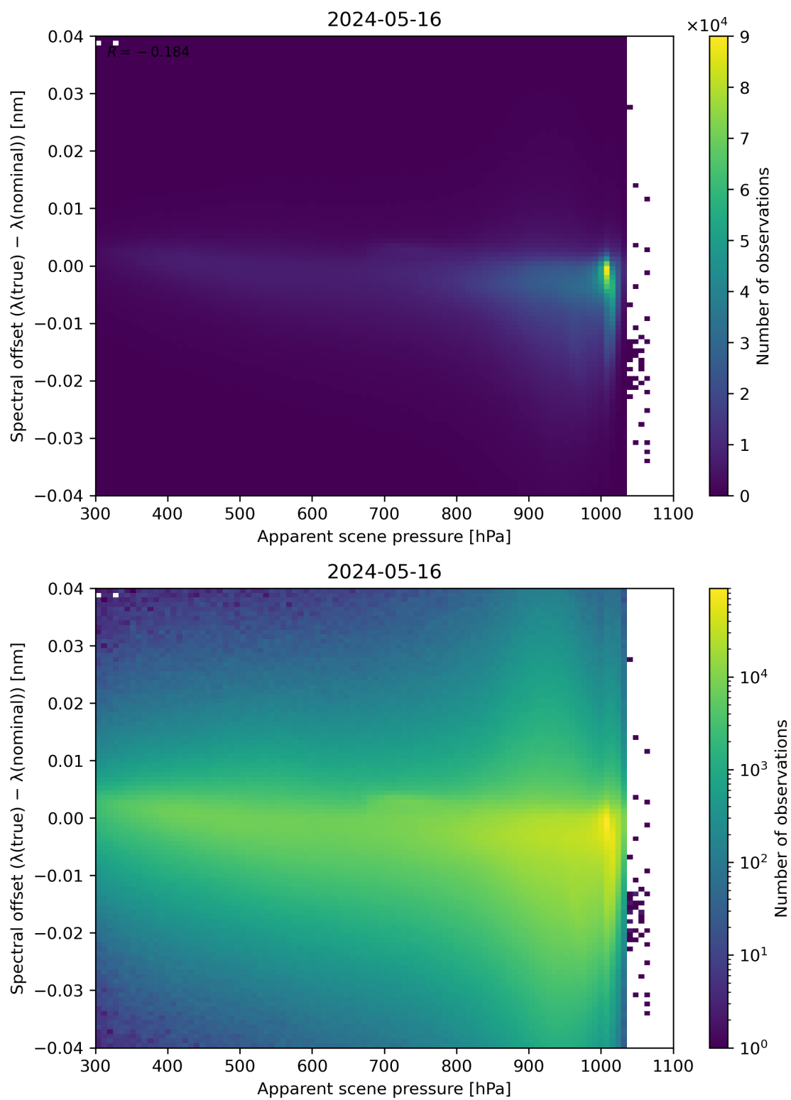
Figure 67: Scatter density plot of “Apparent scene pressure” against “Spectral offset ( \lambda(\text{true}) - \lambda(\text{nominal}) )” for 2024-05-15 to 2024-05-17.
