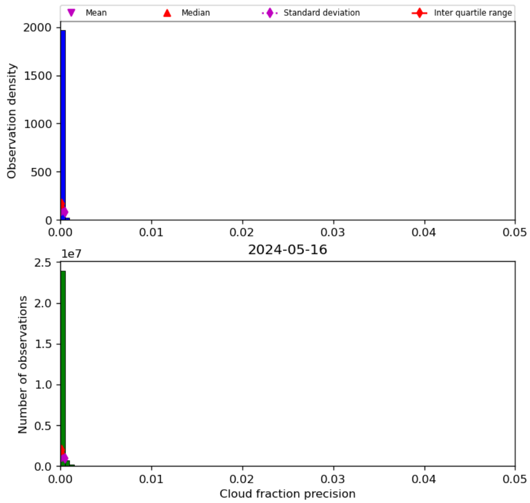
Figure 33: Histogram of “Cloud fraction precision” for 2024-05-15 to 2024-05-17
