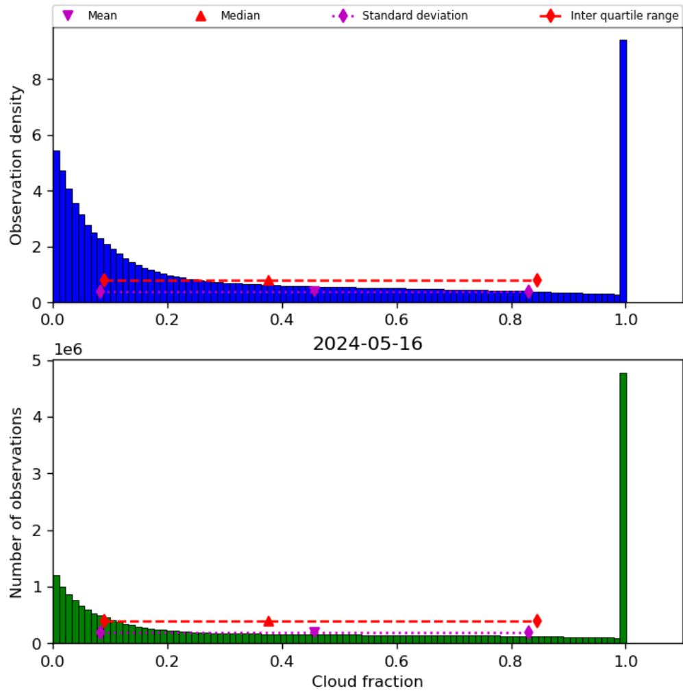
Figure 32: Histogram of “Cloud fraction” for 2024-05-15 to 2024-05-17
