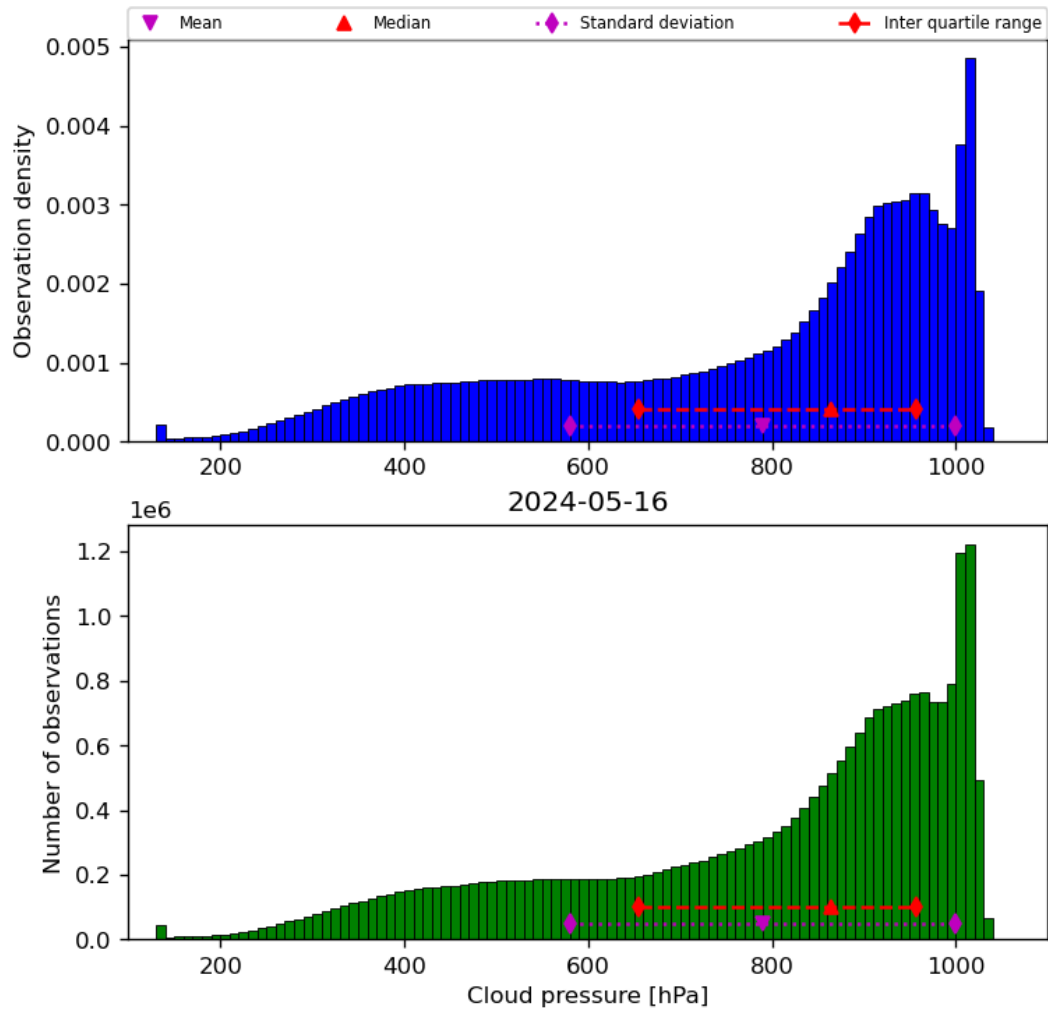
Figure 30: Histogram of “Cloud pressure” for 2024-05-15 to 2024-05-17
