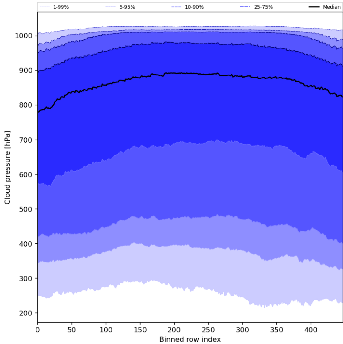
Figure 47: Along track statistics of “Cloud pressure” for 2024-05-15 to 2024-05-17
