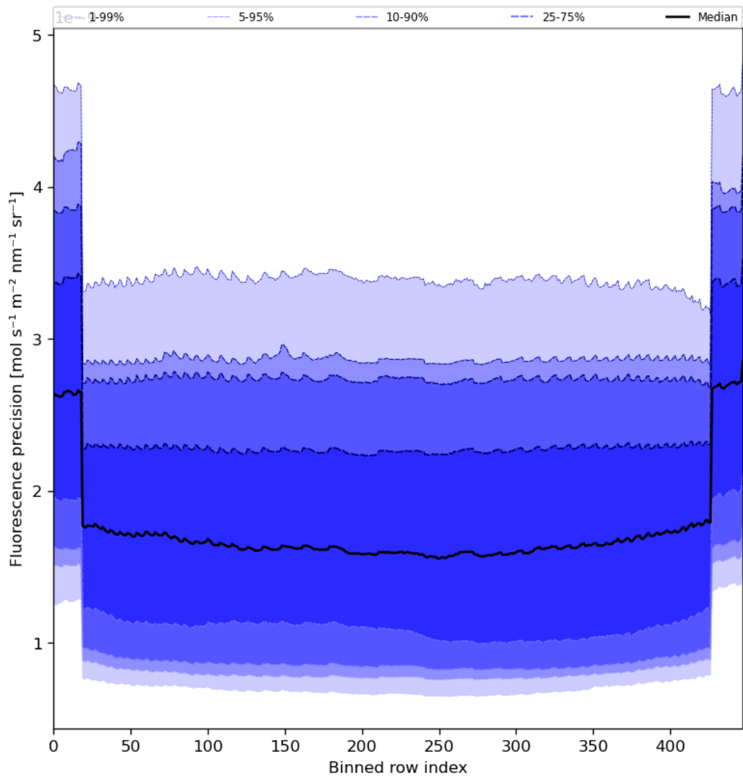
Figure 58: Along track statistics of “Fluorescence precision” for 2024-05-15 to 2024-05-17
