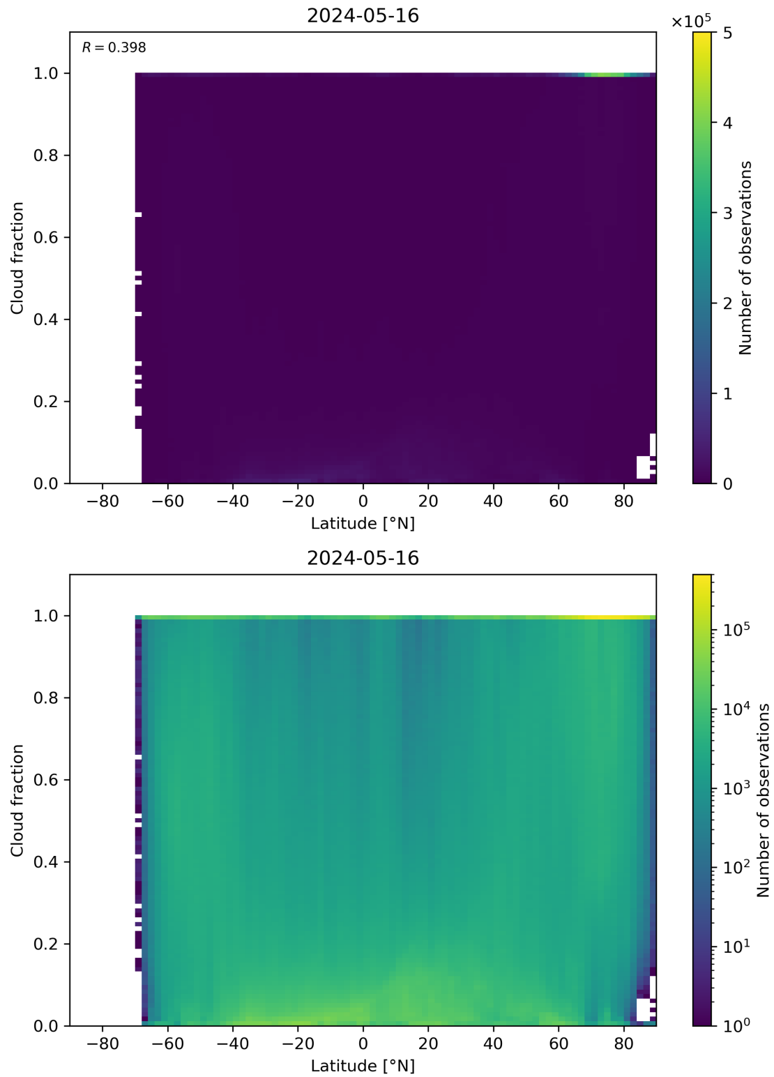
Figure 90: Scatter density plot of “Latitude” against “Cloud fraction” for 2024-05-15 to 2024-05-17.
