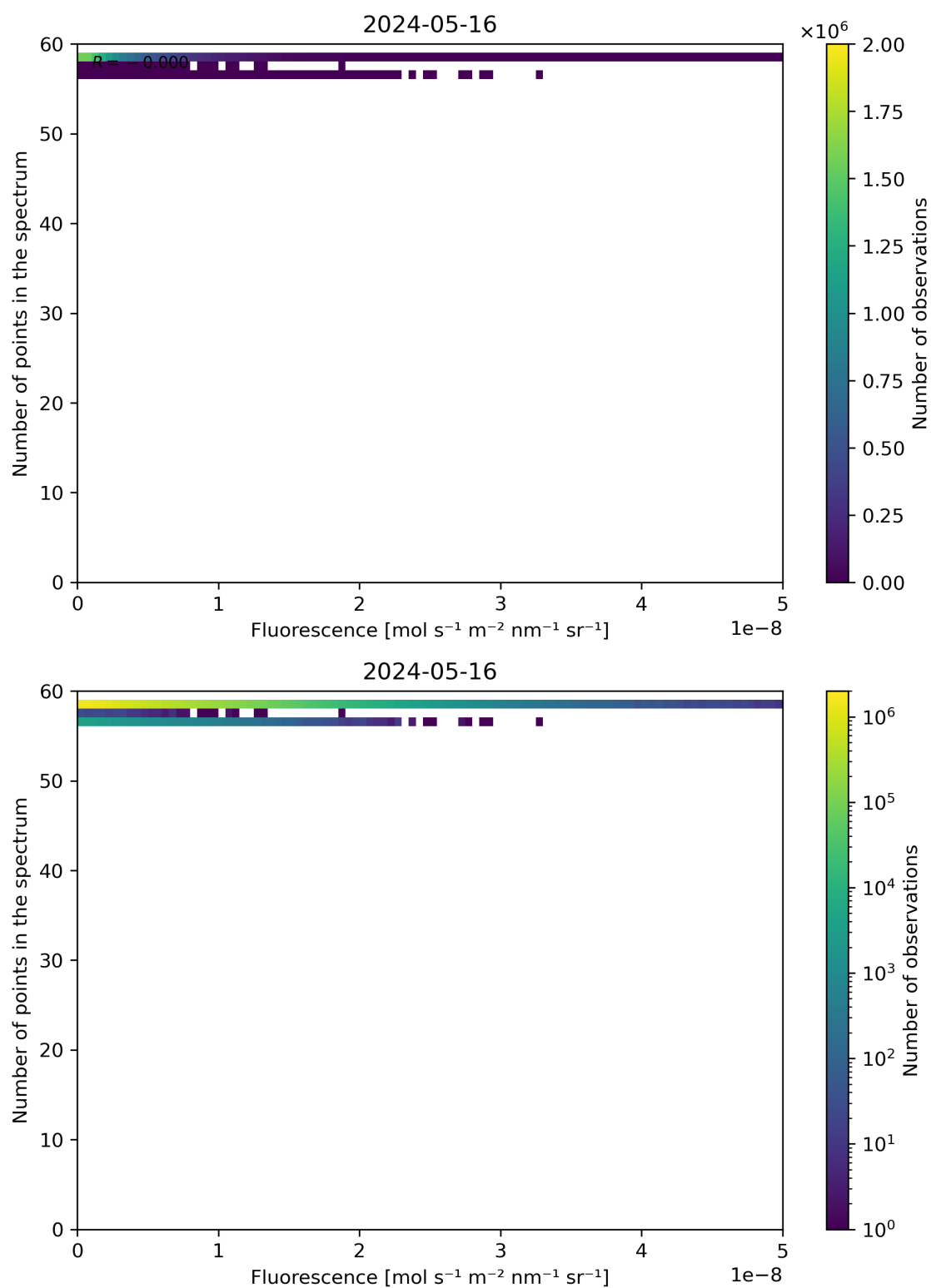
Figure 86: Scatter density plot of “Fluorescence” against “Number of points in the spectrum” for 2024-05-15 to 2024-05-17.
