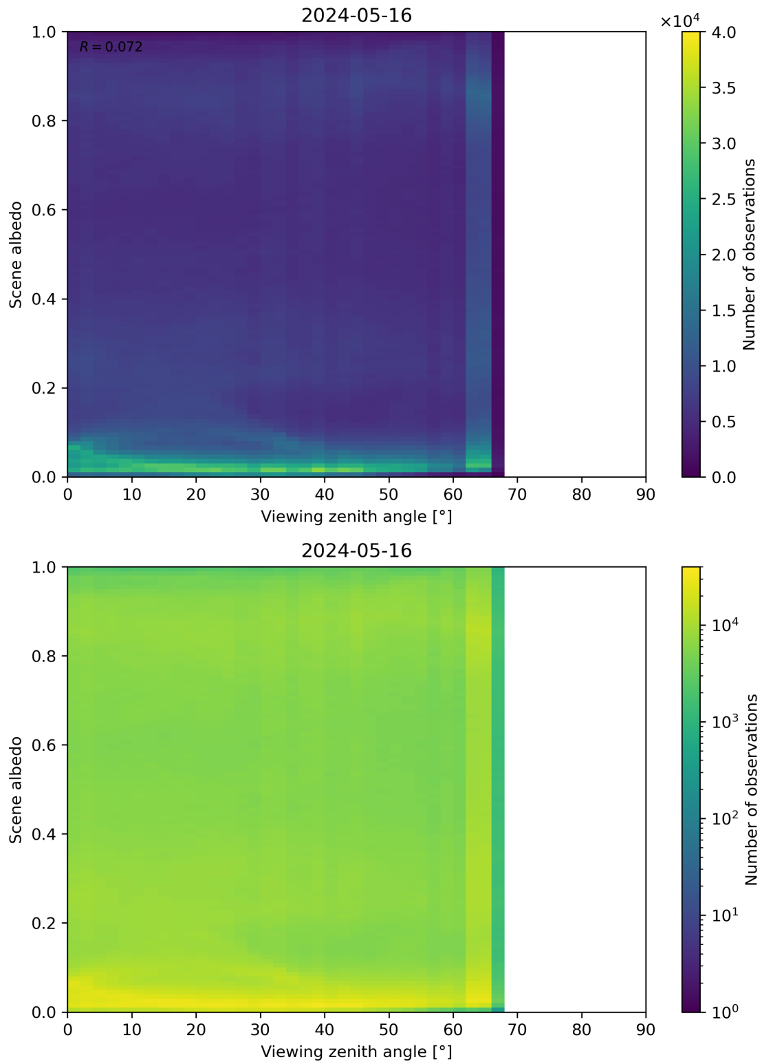
Figure 126: Scatter density plot of “Viewing zenith angle” against “Scene albedo” for 2024-05-15 to 2024-05-17.
