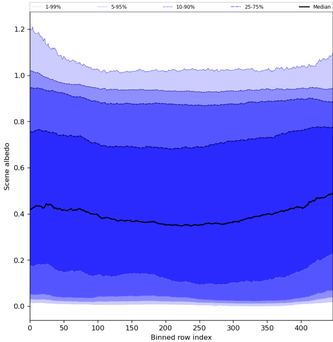
Figure 51: Along track statistics of “Scene albedo” for 2024-05-15 to 2024-05-17
