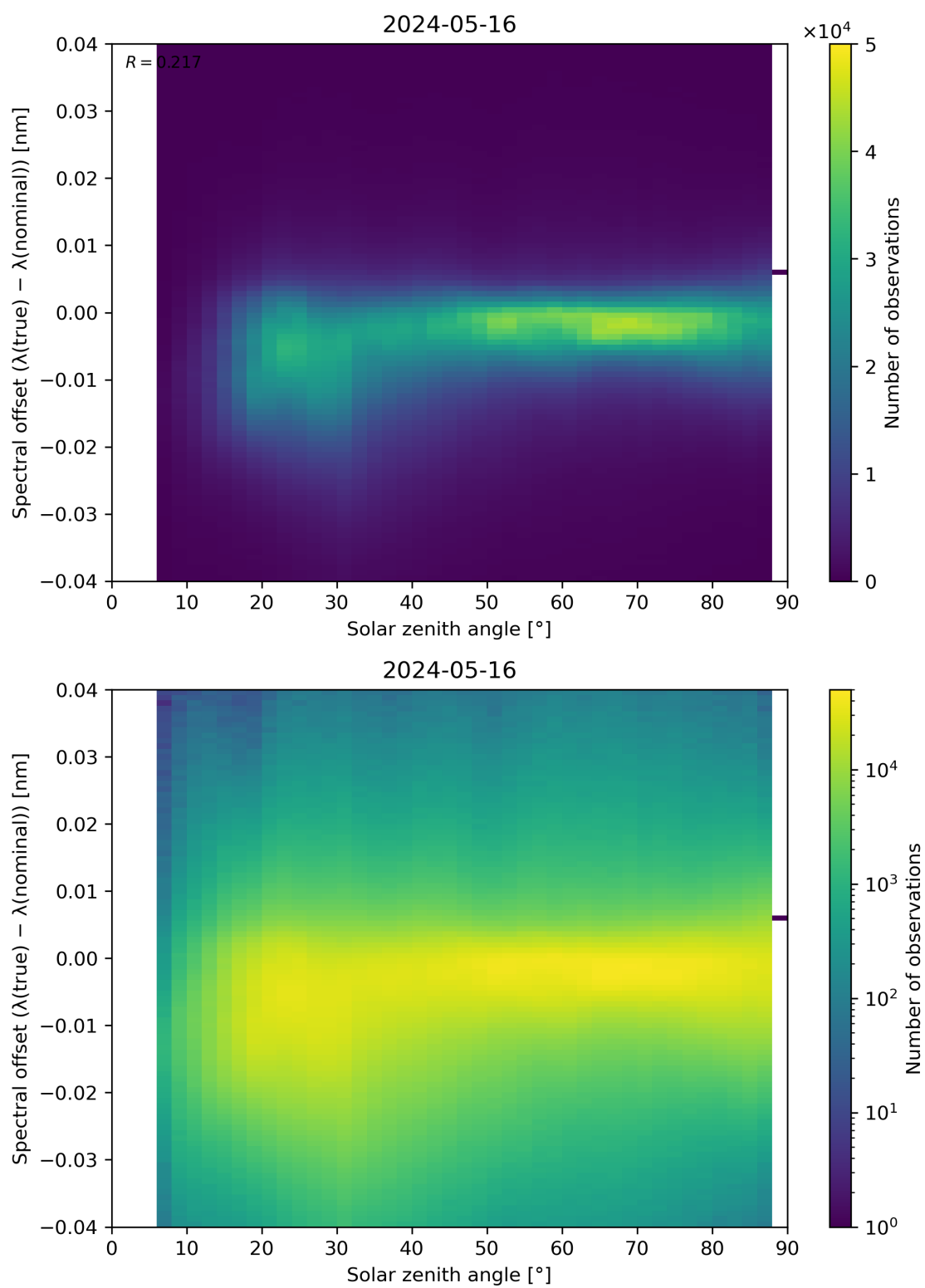
Figure 117: Scatter density plot of “Solar zenith angle” against “Spectral offset ( \lambda(\text{true}) - \lambda(\text{nominal}) )” for 2024-05-15 to 2024-05-17.
