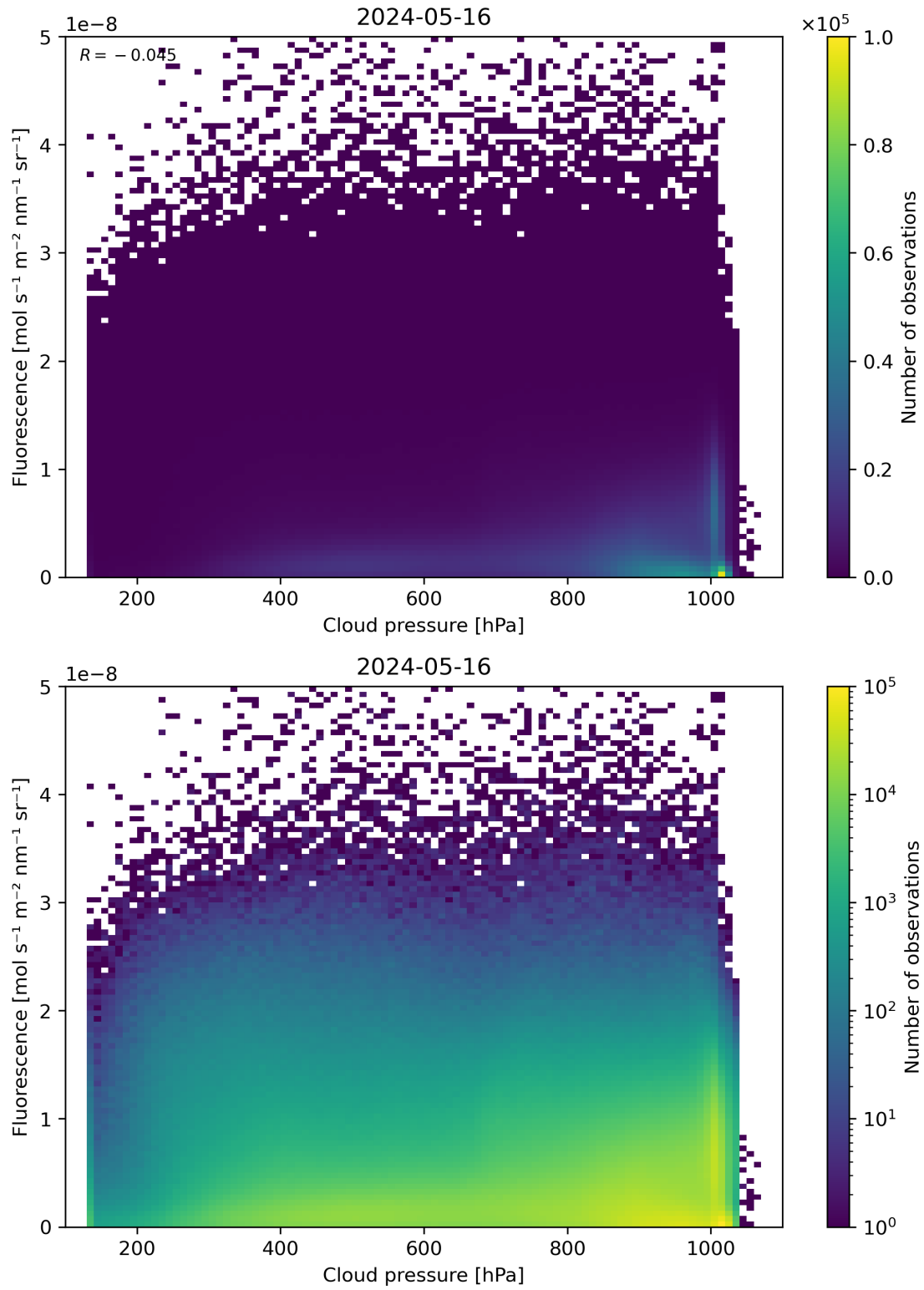
Figure 80: Scatter density plot of “Cloud pressure” against “Fluorescence” for 2024-05-15 to 2024-05-17.
