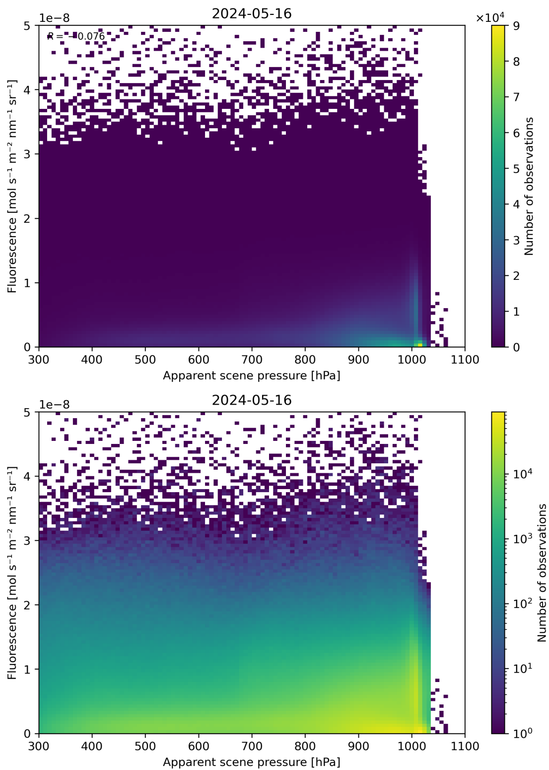
Figure 64: Scatter density plot of “Apparent scene pressure” against “Fluorescence” for 2024-05-15 to 2024-05-17.
