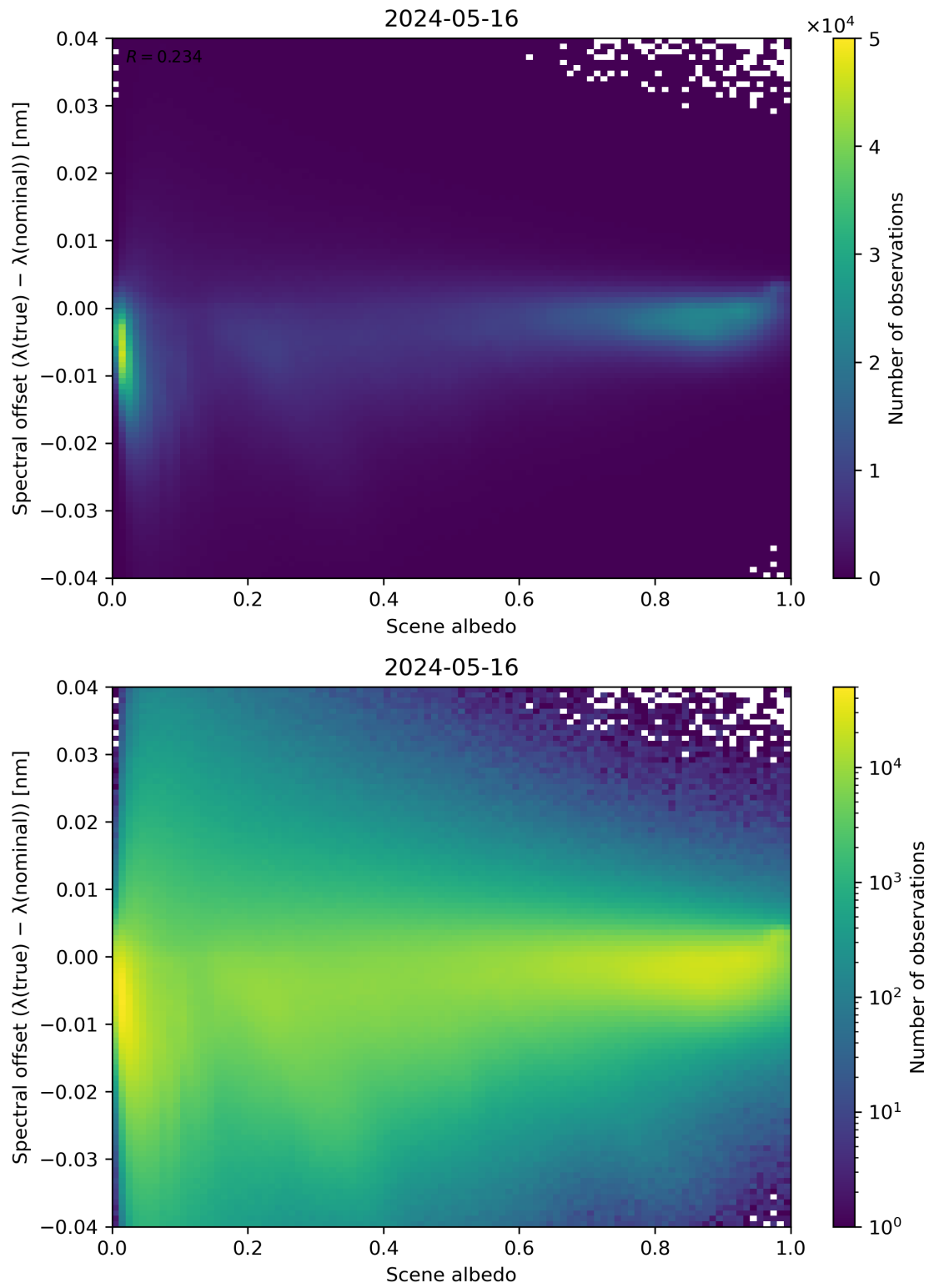
Figure 107: Scatter density plot of “Scene albedo” against “Spectral offset ( \lambda(\text{true}) - \lambda(\text{nominal}) )” for 2024-05-15 to 2024-05-17.
