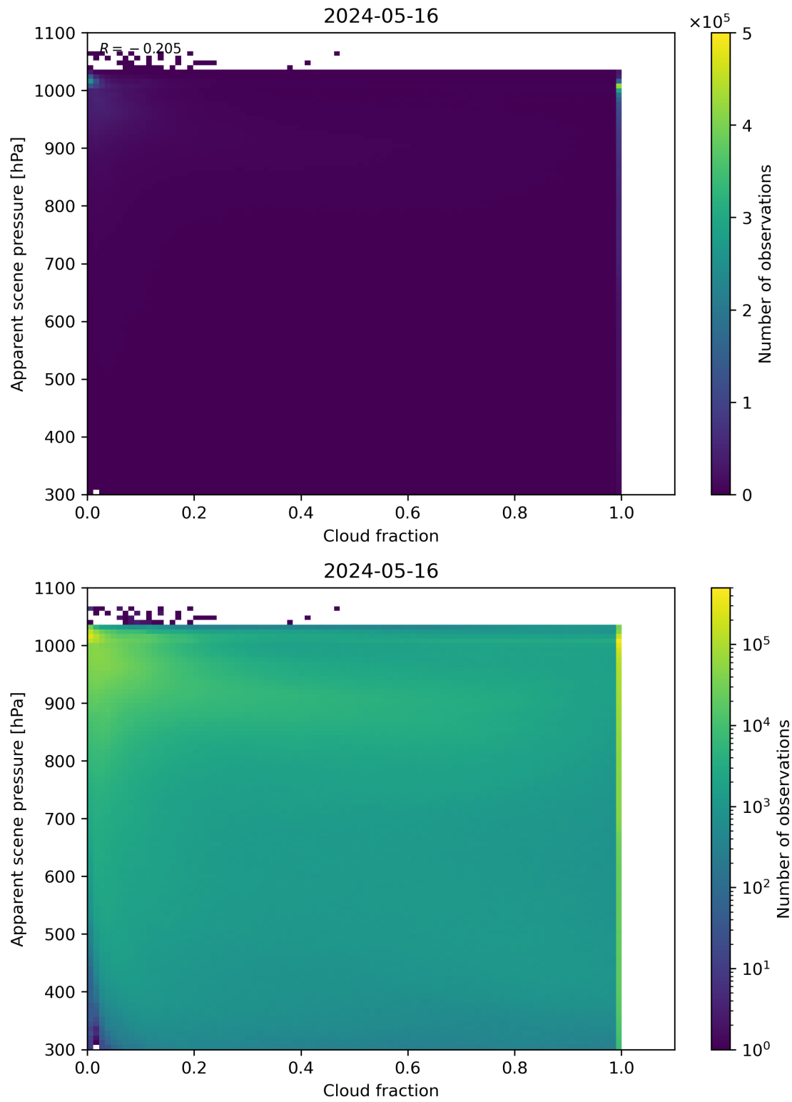
Figure 70: Scatter density plot of “Cloud fraction” against “Apparent scene pressure” for 2024-05-15 to 2024-05-17.
