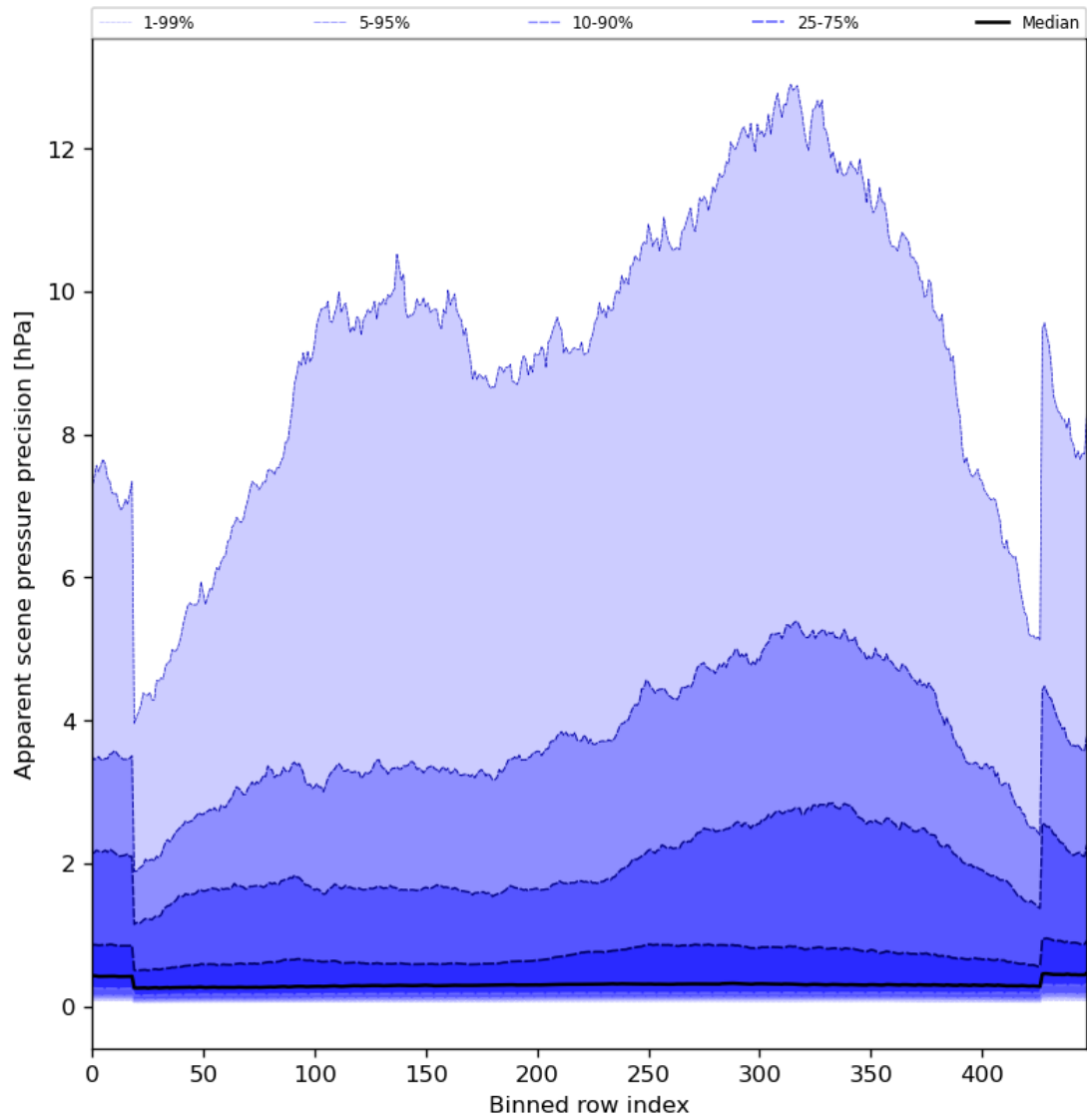
Figure 54: Along track statistics of “Apparent scene pressure precision” for 2024-05-15 to 2024-05-17
