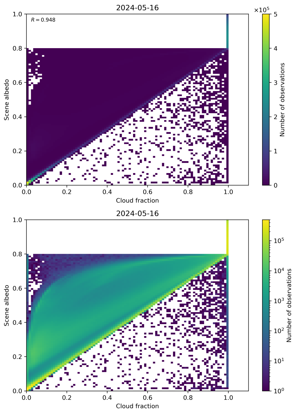
Figure 75: Scatter density plot of “Cloud fraction” against “Scene albedo” for 2024-05-15 to 2024-05-17.
