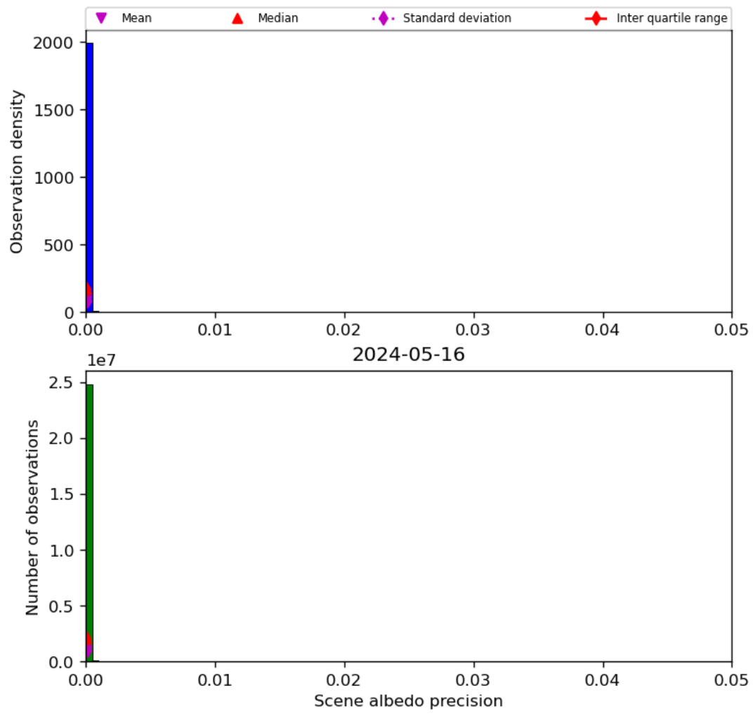
Figure 35: Histogram of “Scene albedo precision” for 2024-05-15 to 2024-05-17
