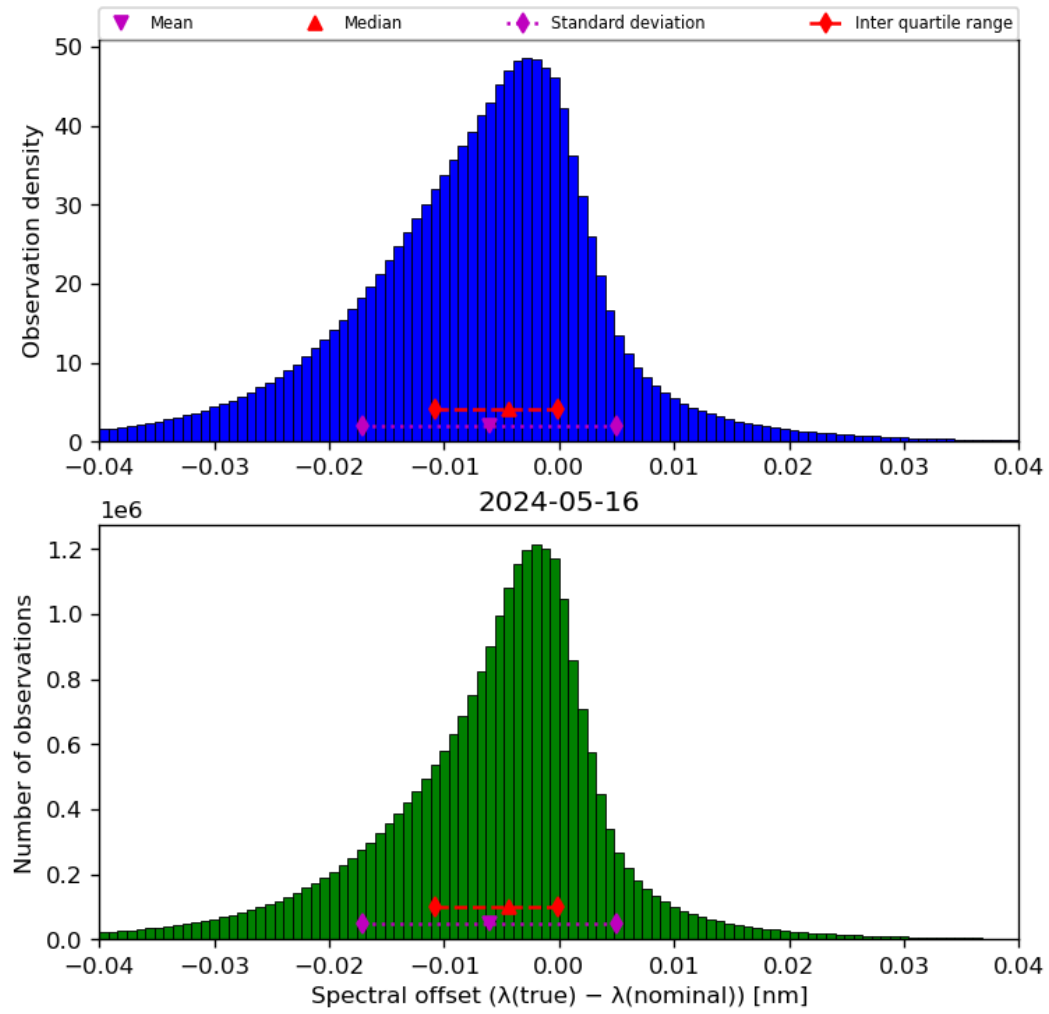
Figure 45: Histogram of “Spectral offset ( \lambda(\text{true}) - \lambda(\text{nominal}) )” for 2024-05-15 to 2024-05-17
