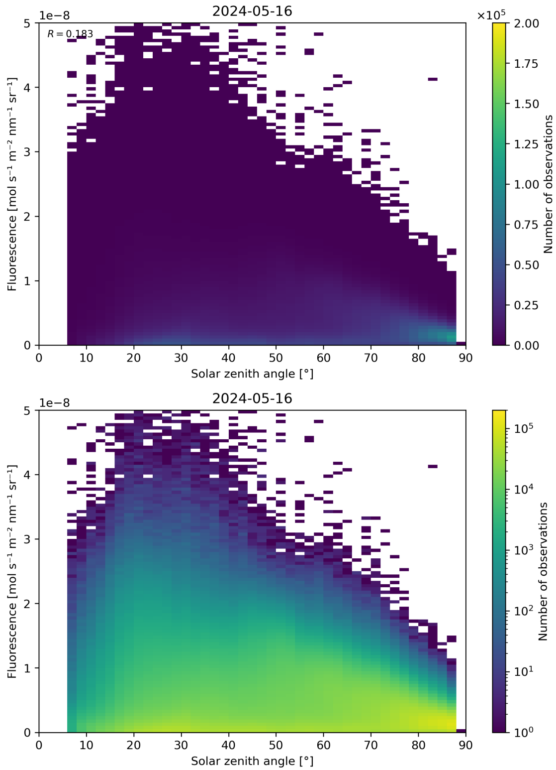
Figure 112: Scatter density plot of “Solar zenith angle” against “Fluorescence” for 2024-05-15 to 2024-05-17.
