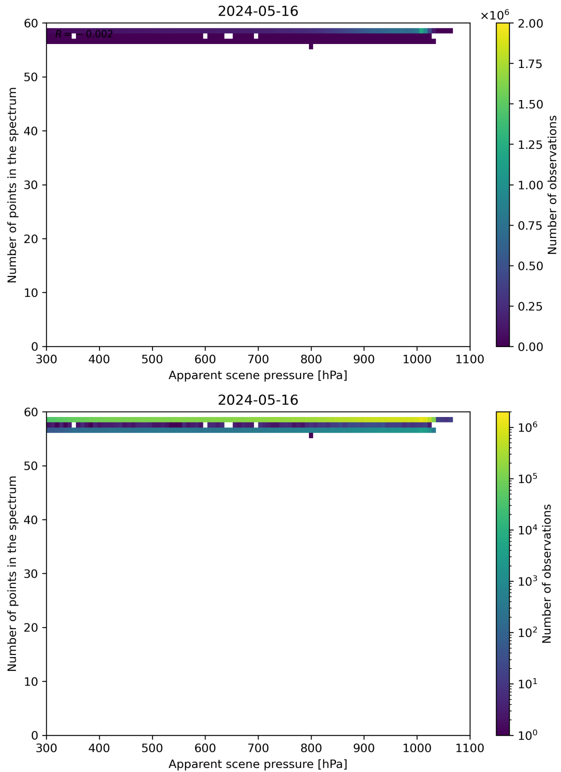
Figure 66: Scatter density plot of “Apparent scene pressure” against “Number of points in the spectrum” for 2024-05-15 to 2024-05-17.
