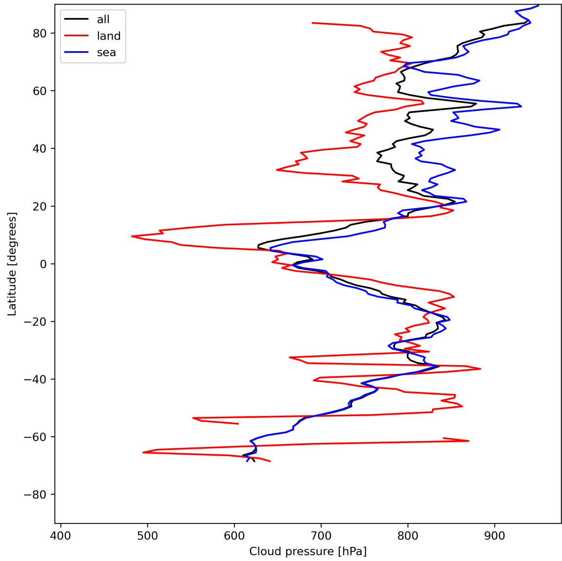
Figure 13: Zonal average of “Cloud pressure” for 2024-05-15 to 2024-05-17.
