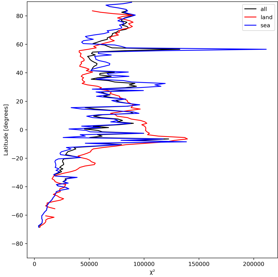
Figure 21: Zonal average of “ \chi^2 ” for 2024-05-15 to 2024-05-17.
