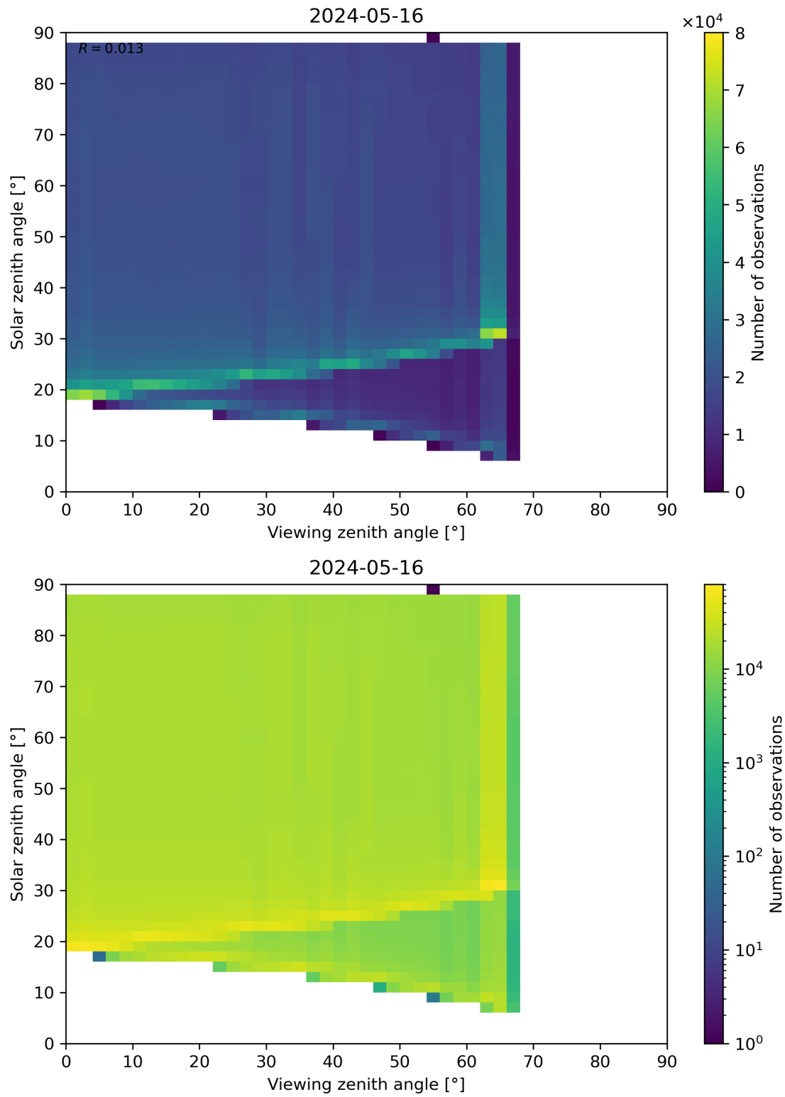
Figure 127: Scatter density plot of “Viewing zenith angle” against “Solar zenith angle” for 2024-05-15 to 2024-05-17.
