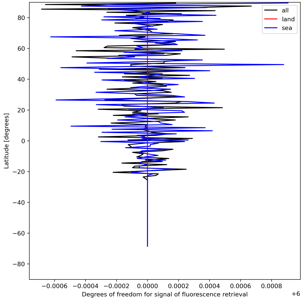
Figure 26: Zonal average of “Degrees of freedom for signal of fluorescence retrieval” for 2024-05-15 to 2024-05-17.
