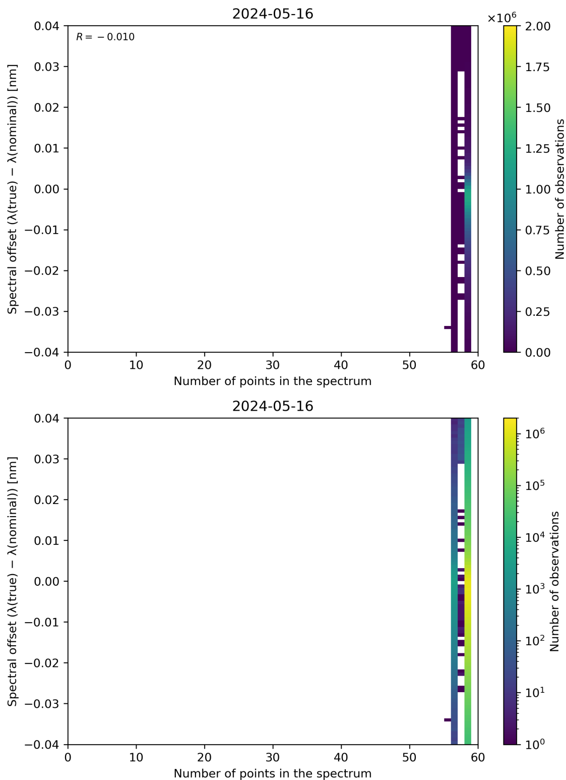
Figure 101: Scatter density plot of “Number of points in the spectrum” against “Spectral offset ( \lambda(\text{true}) - \lambda(\text{nominal}) )” for 2024-05-15 to 2024-05-17.
