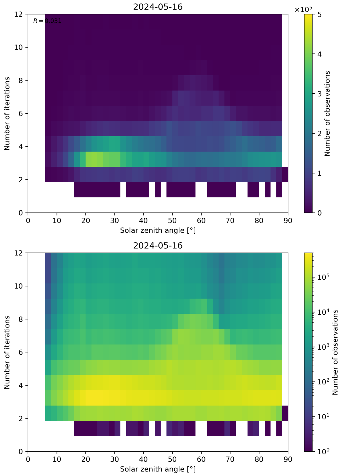
Figure 114: Scatter density plot of “Solar zenith angle” against “Number of iterations” for 2024-05-15 to 2024-05-17.
