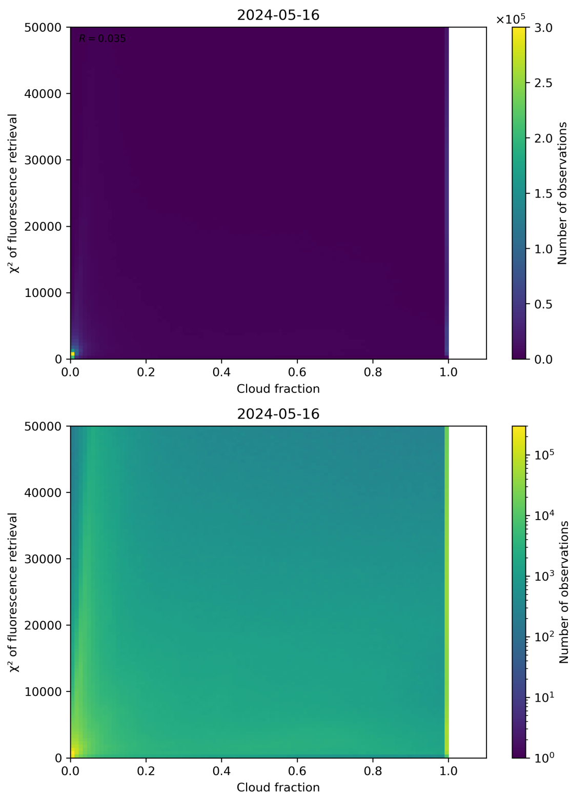
Figure 71: Scatter density plot of “Cloud fraction” against “ \chi^2 of fluorescence retrieval” for 2024-05-15 to 2024-05-17.
