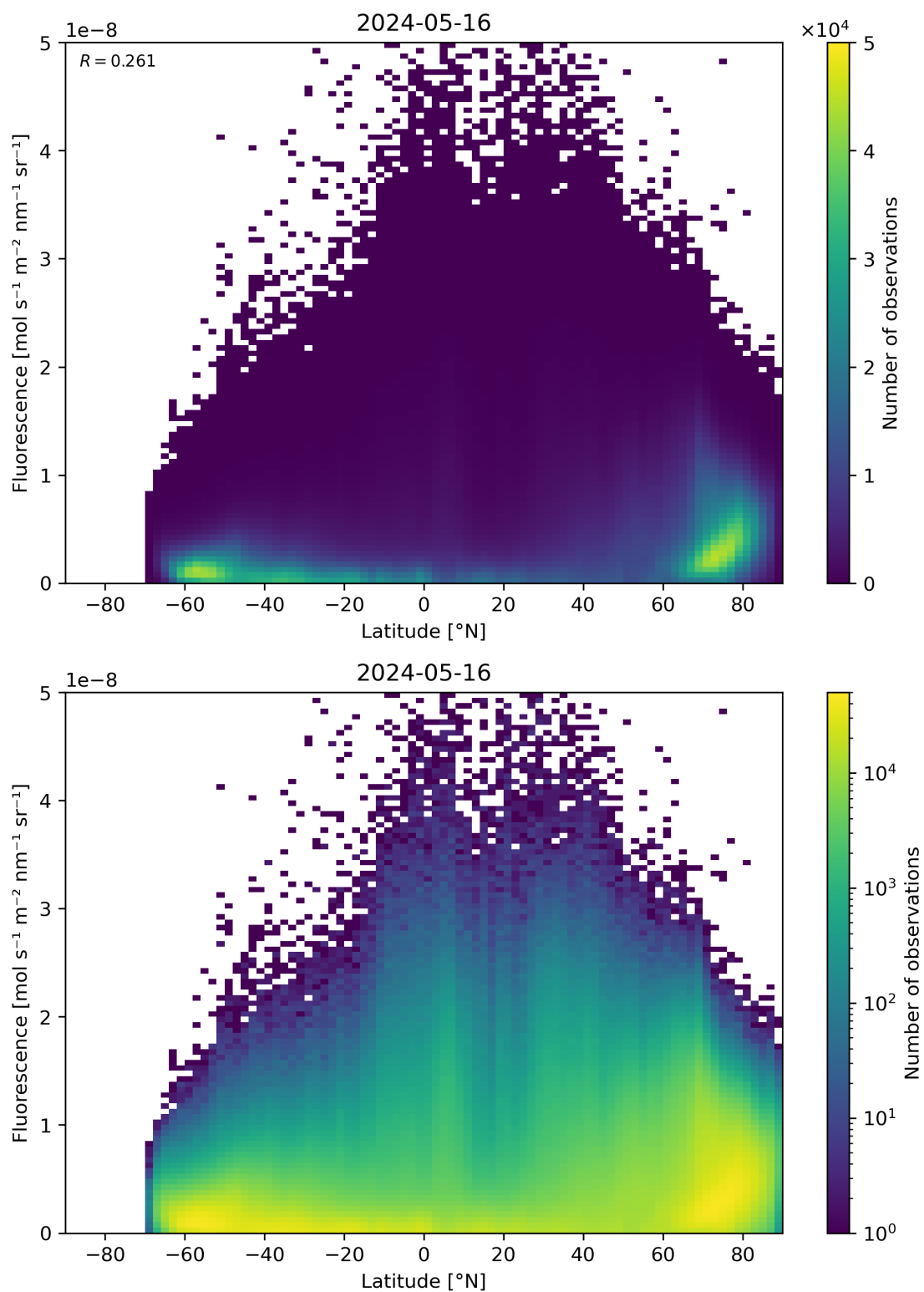
Figure 92: Scatter density plot of “Latitude” against “Fluorescence” for 2024-05-15 to 2024-05-17.
