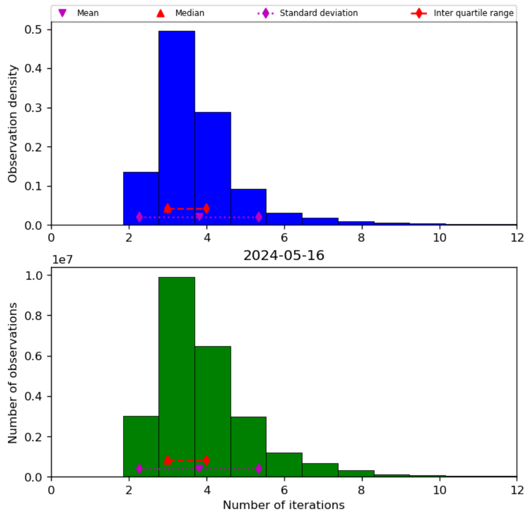
Figure 39: Histogram of “Number of iterations” for 2024-05-15 to 2024-05-17
