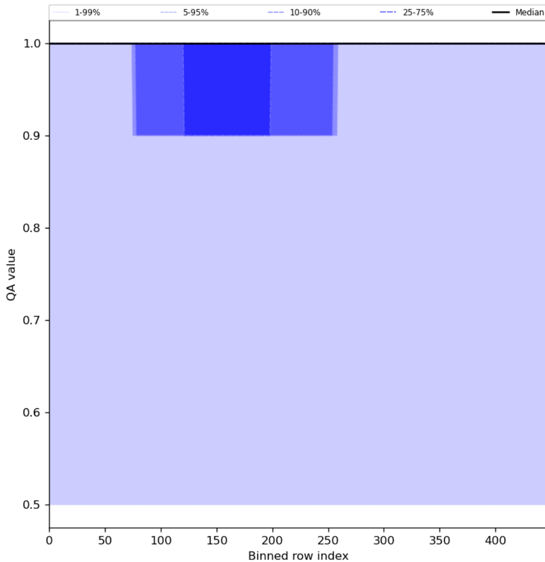
Figure 46: Along track statistics of “QA value” for 2024-05-15 to 2024-05-17
