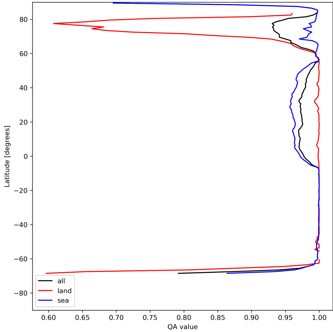
Figure 12: Zonal average of “QA value” for 2024-05-15 to 2024-05-17.
