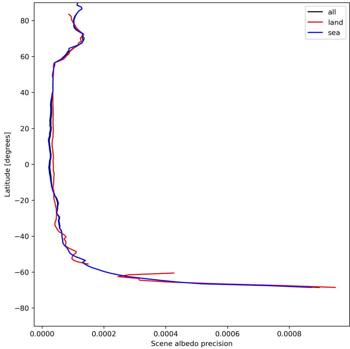
Figure 18: Zonal average of “Scene albedo precision” for 2024-05-15 to 2024-05-17.
