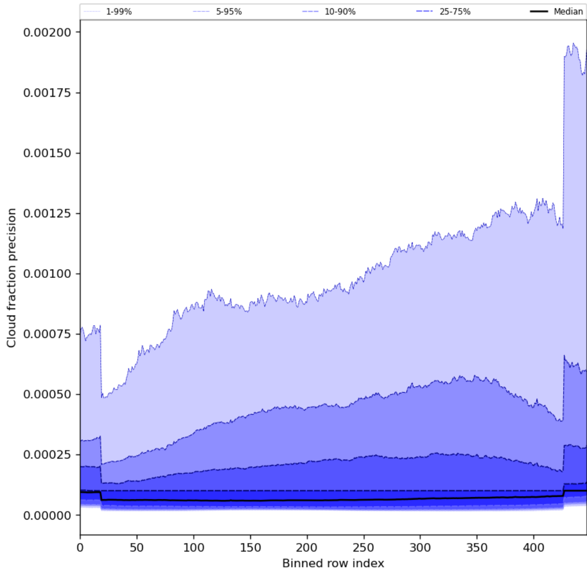
Figure 50: Along track statistics of “Cloud fraction precision” for 2024-05-15 to 2024-05-17
