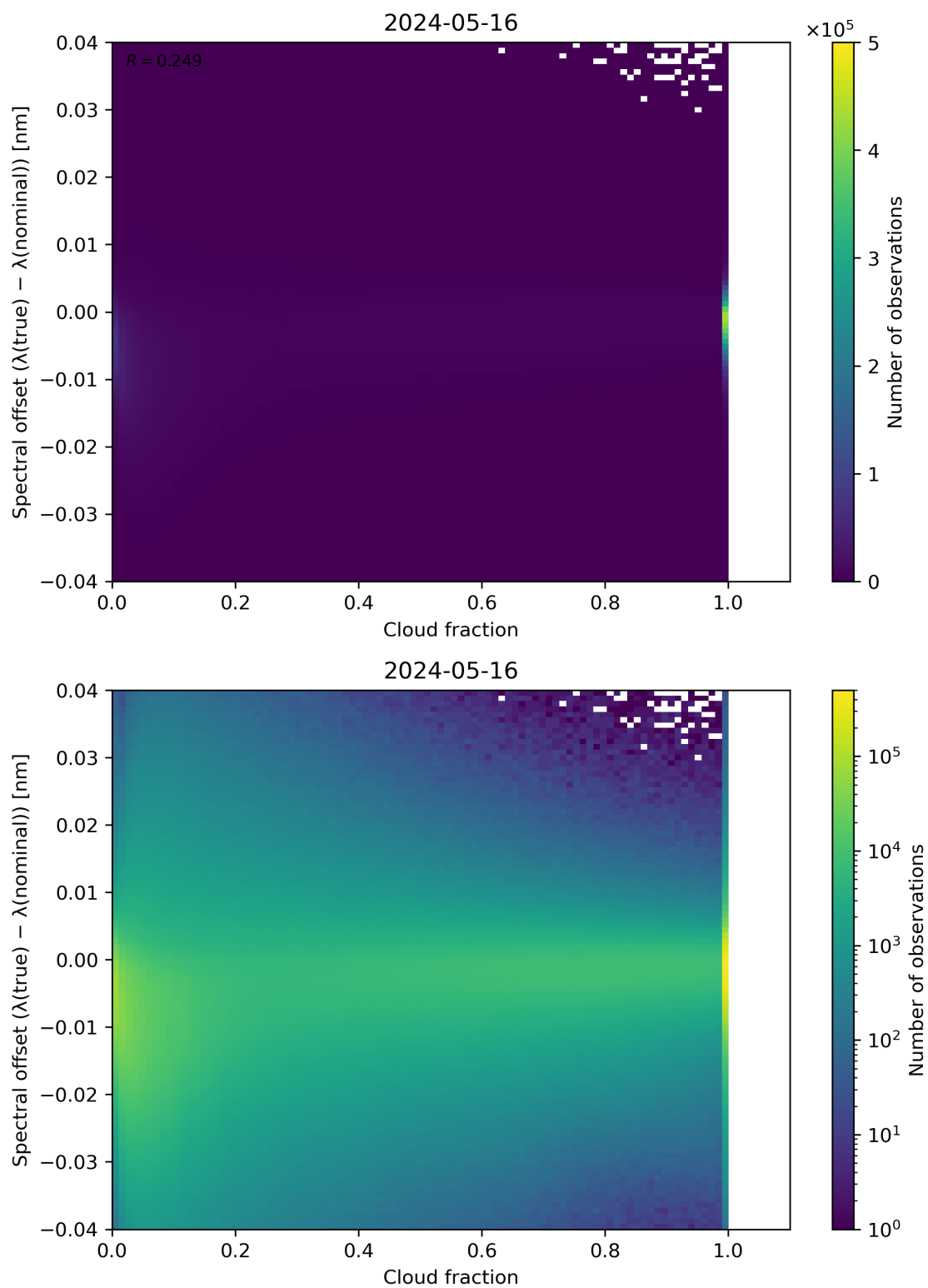
Figure 76: Scatter density plot of “Cloud fraction” against “Spectral offset ( \lambda(\text{true}) - \lambda(\text{nominal}) )” for 2024-05-15 to 2024-05-17.
