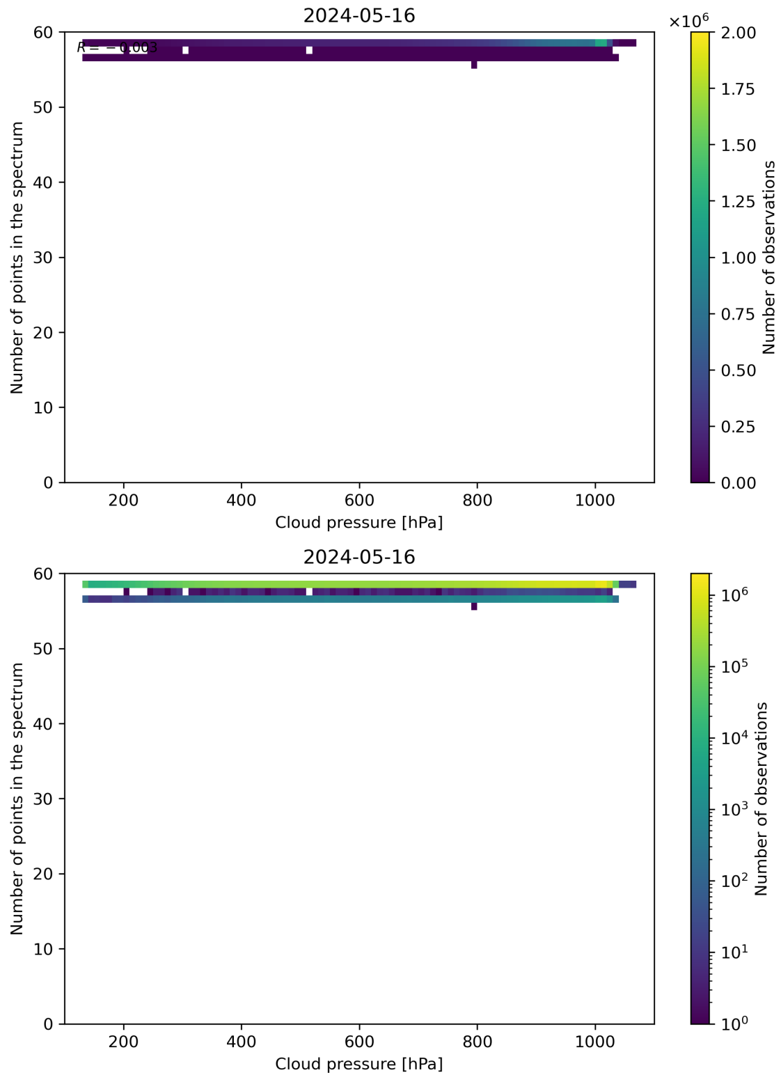
Figure 82: Scatter density plot of “Cloud pressure” against “Number of points in the spectrum” for 2024-05-15 to 2024-05-17.
