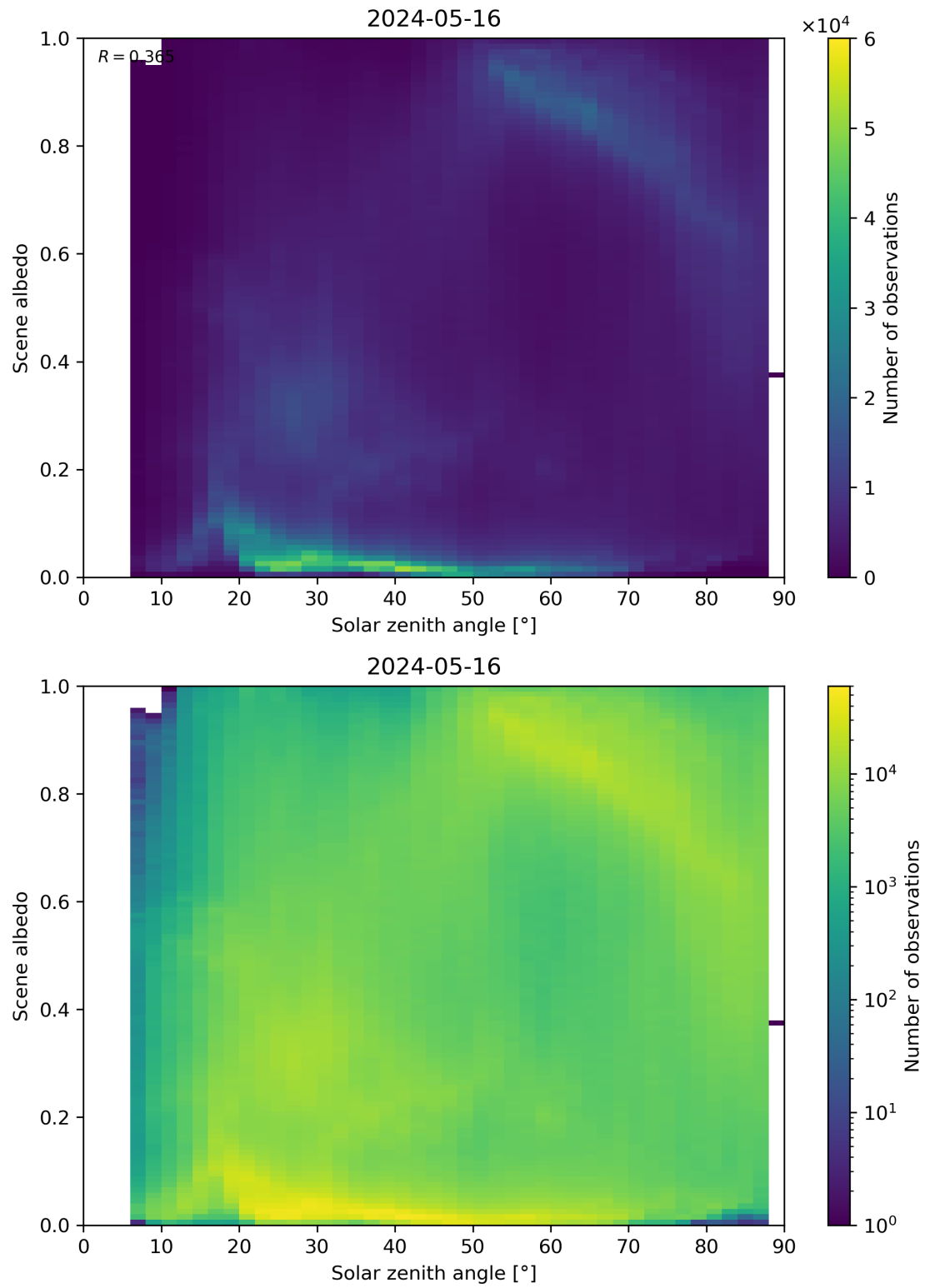
Figure 116: Scatter density plot of “Solar zenith angle” against “Scene albedo” for 2024-05-15 to 2024-05-17.
