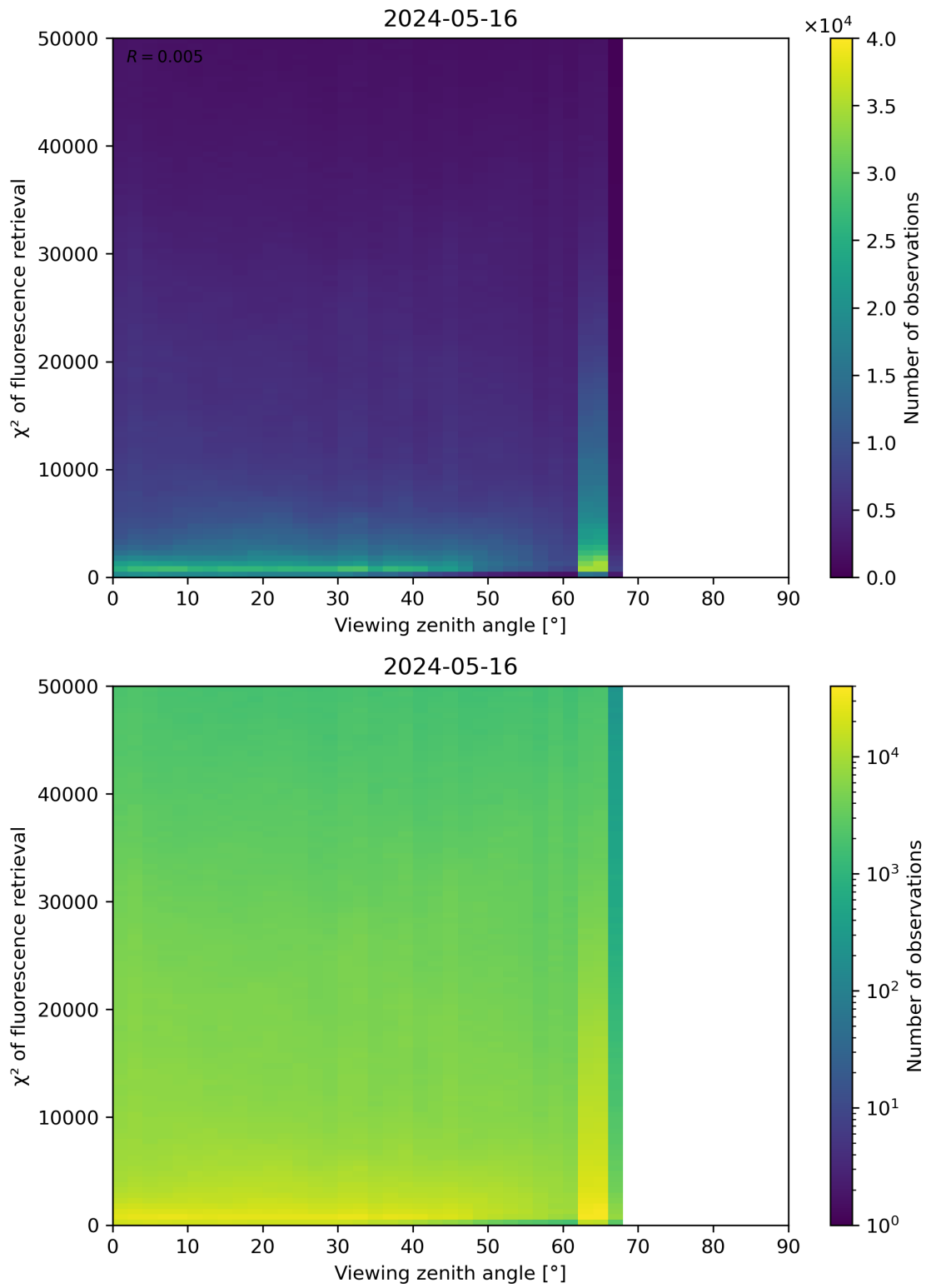
Figure 119: Scatter density plot of “Viewing zenith angle” against “ \chi^2 of fluorescence retrieval” for 2024-05-15 to 2024-05-17.
