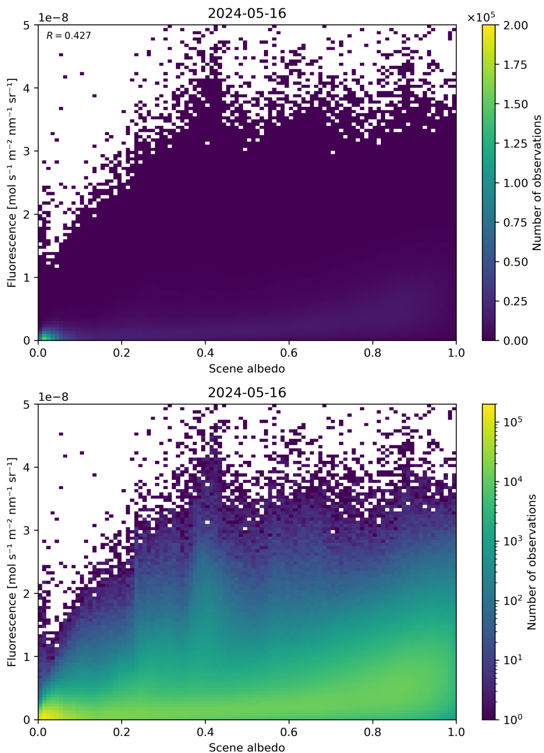
Figure 104: Scatter density plot of “Scene albedo” against “Fluorescence” for 2024-05-15 to 2024-05-17.
