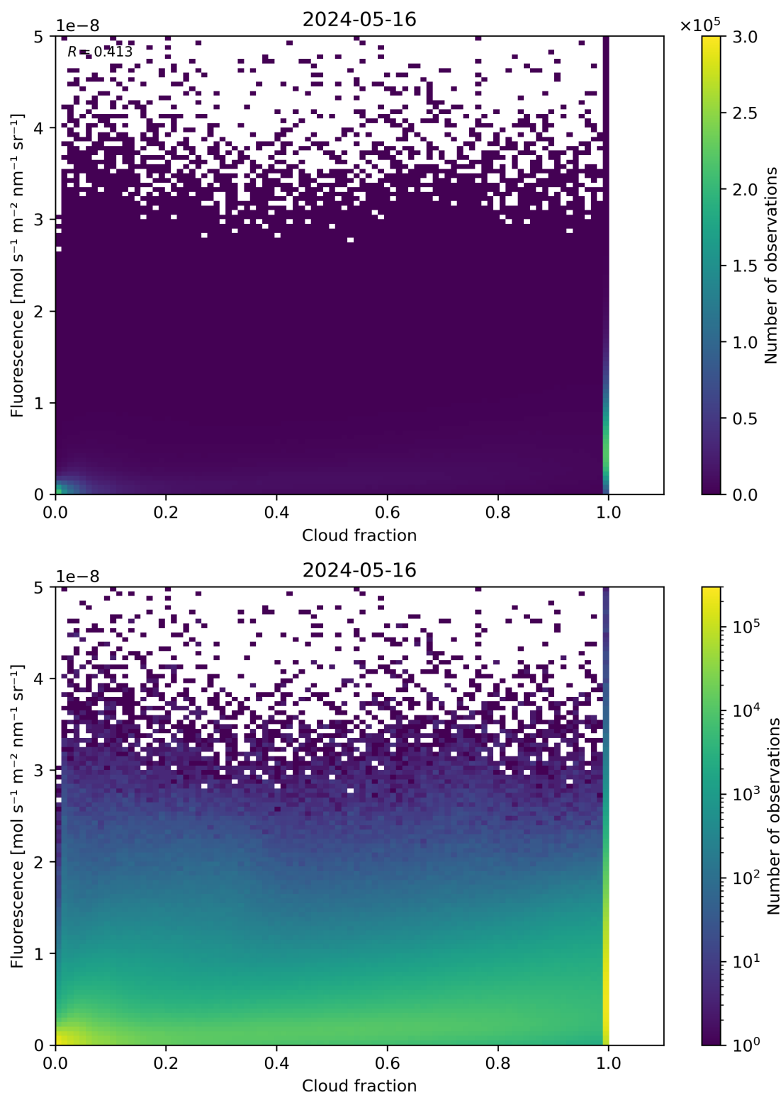
Figure 72: Scatter density plot of “Cloud fraction” against “Fluorescence” for 2024-05-15 to 2024-05-17.
