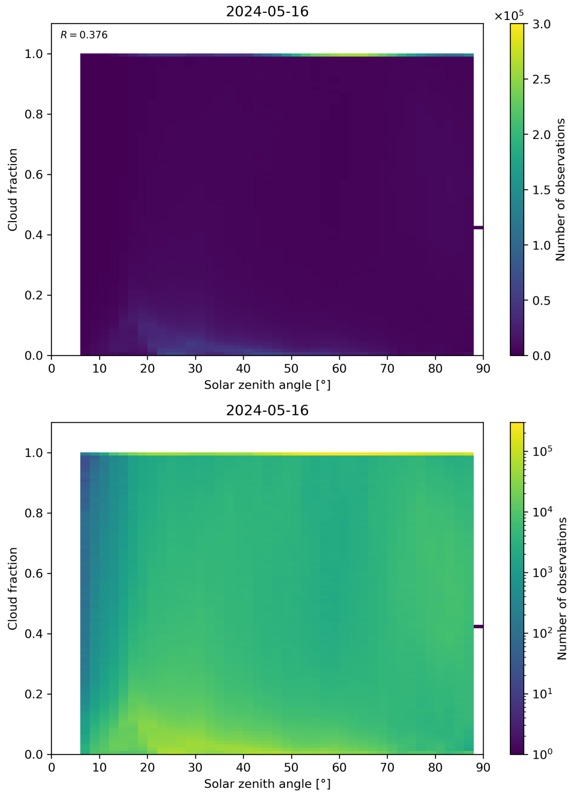
Figure 110: Scatter density plot of “Solar zenith angle” against “Cloud fraction” for 2024-05-15 to 2024-05-17.
