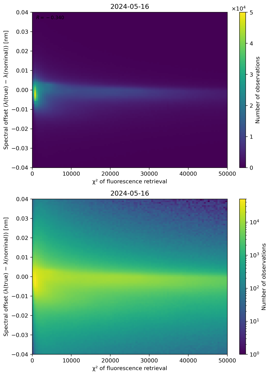
Figure 69: Scatter density plot of " \chi^2 of fluorescence retrieval" against "Spectral offset ( \lambda(\text{true}) - \lambda(\text{nominal}) )" for 2024-05-15 to 2024-05-17.
