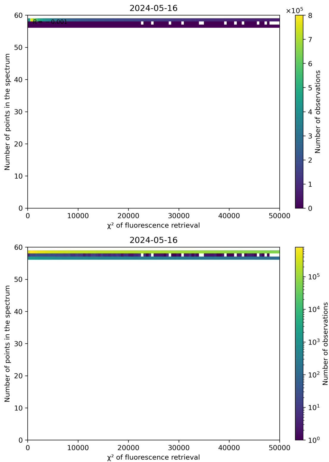
Figure 68: Scatter density plot of " \chi^2 of fluorescence retrieval" against "Number of points in the spectrum" for 2024-05-15 to 2024-05-17.
