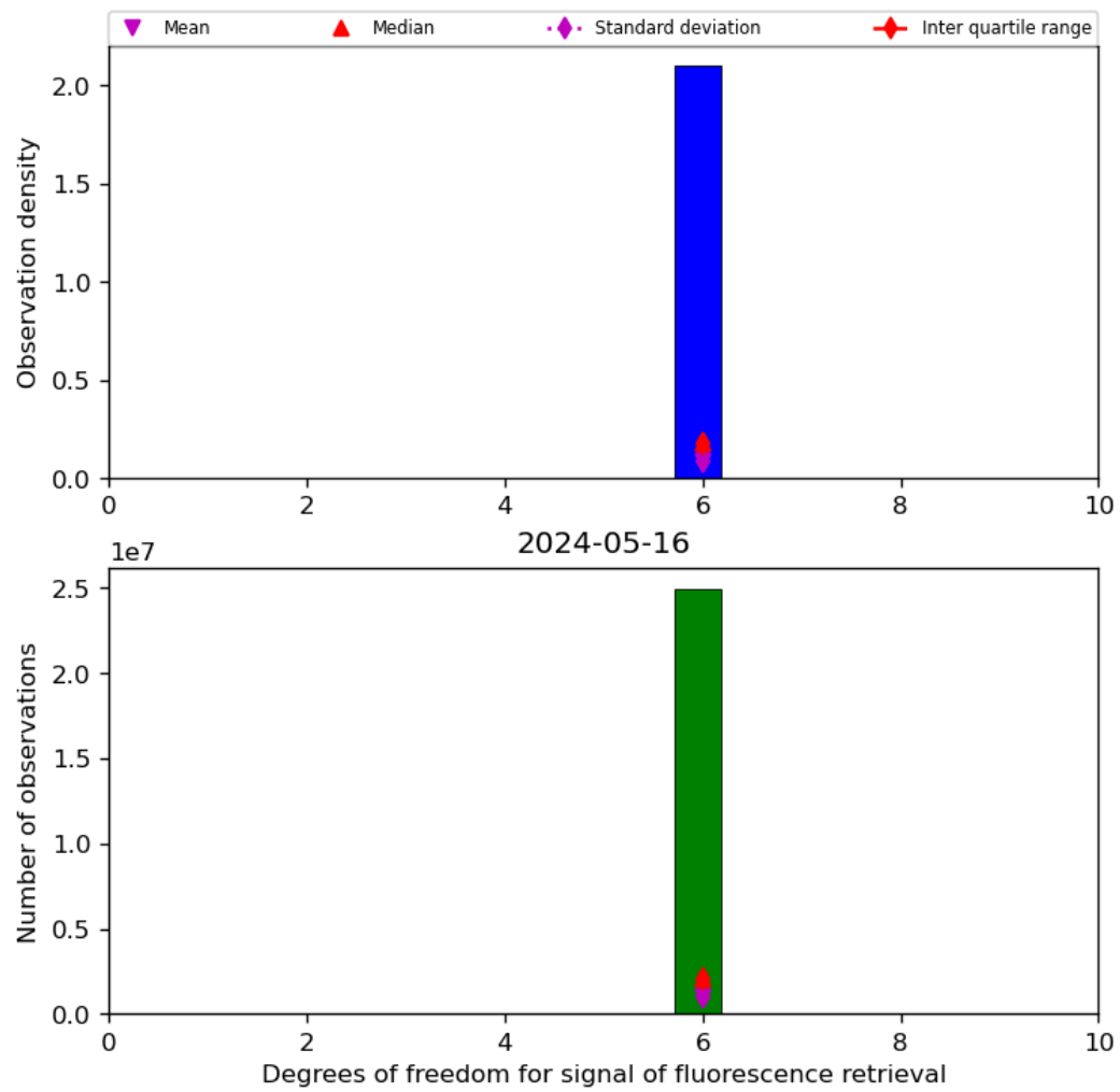
Figure 43: Histogram of “Degrees of freedom for signal of fluorescence retrieval” for 2024-05-15 to 2024-05-17
