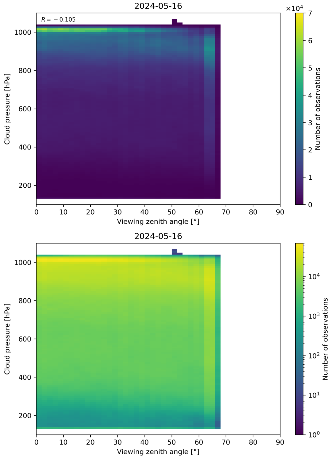
Figure 121: Scatter density plot of “Viewing zenith angle” against “Cloud pressure” for 2024-05-15 to 2024-05-17.
