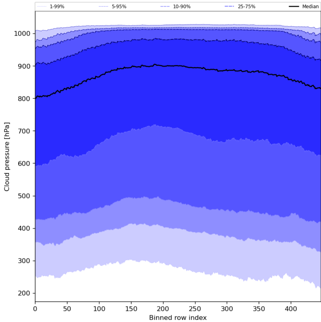
Figure 47: Along track statistics of “Cloud pressure” for 2024-05-16 to 2024-05-18
