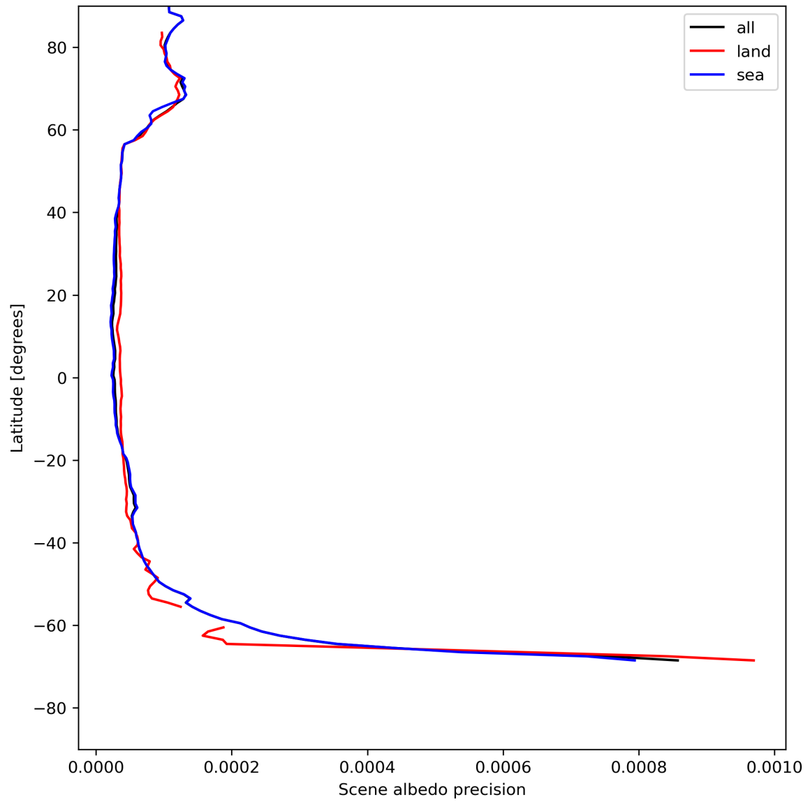
Figure 18: Zonal average of “Scene albedo precision” for 2024-05-16 to 2024-05-18.
