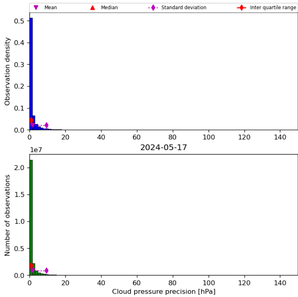
Figure 31: Histogram of “Cloud pressure precision” for 2024-05-16 to 2024-05-18
