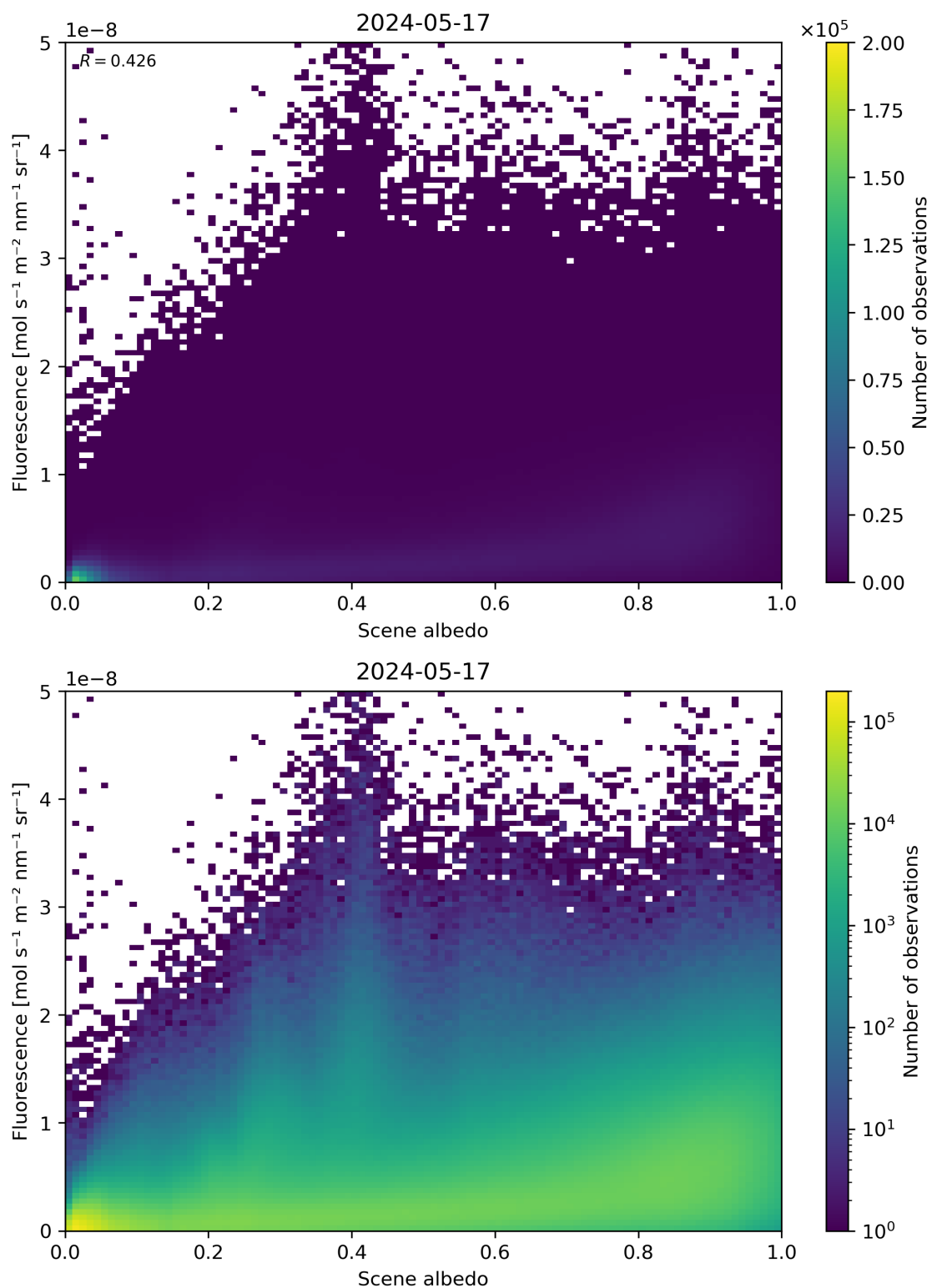
Figure 104: Scatter density plot of “Scene albedo” against “Fluorescence” for 2024-05-16 to 2024-05-18.
