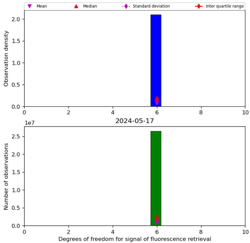
Figure 43: Histogram of “Degrees of freedom for signal of fluorescence retrieval” for 2024-05-16 to 2024-05-18
