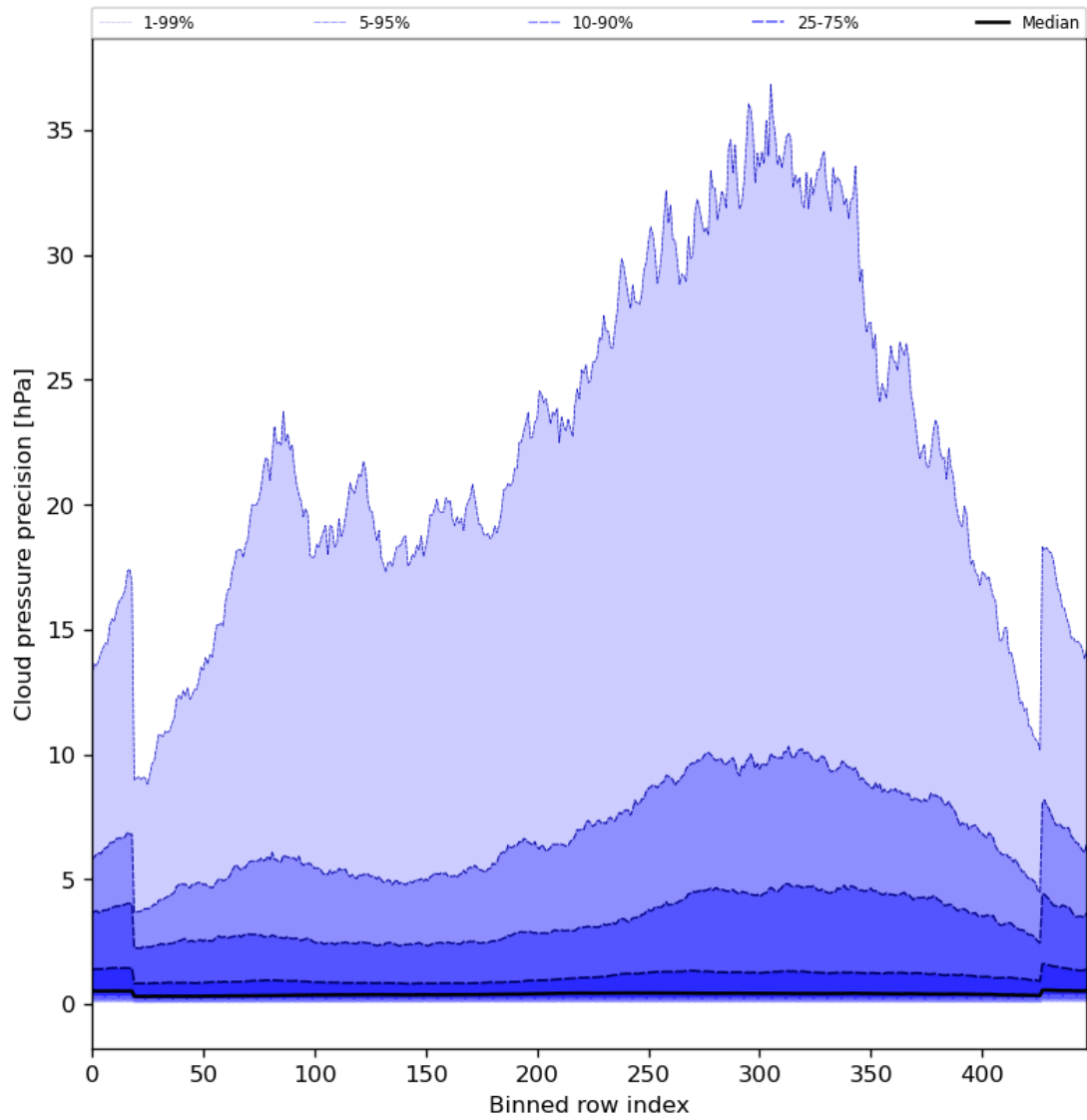
Figure 48: Along track statistics of “Cloud pressure precision” for 2024-05-16 to 2024-05-18
