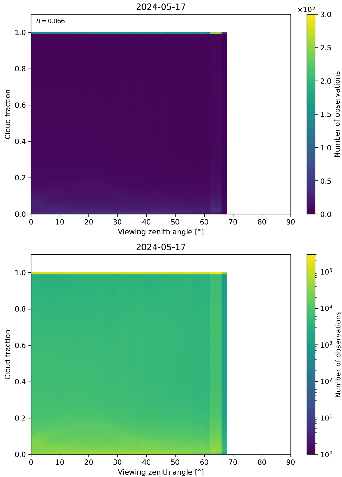
Figure 120: Scatter density plot of “Viewing zenith angle” against “Cloud fraction” for 2024-05-16 to 2024-05-18.
