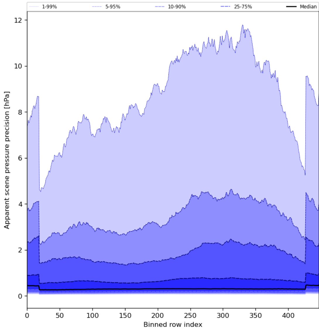
Figure 54: Along track statistics of “Apparent scene pressure precision” for 2024-05-16 to 2024-05-18
