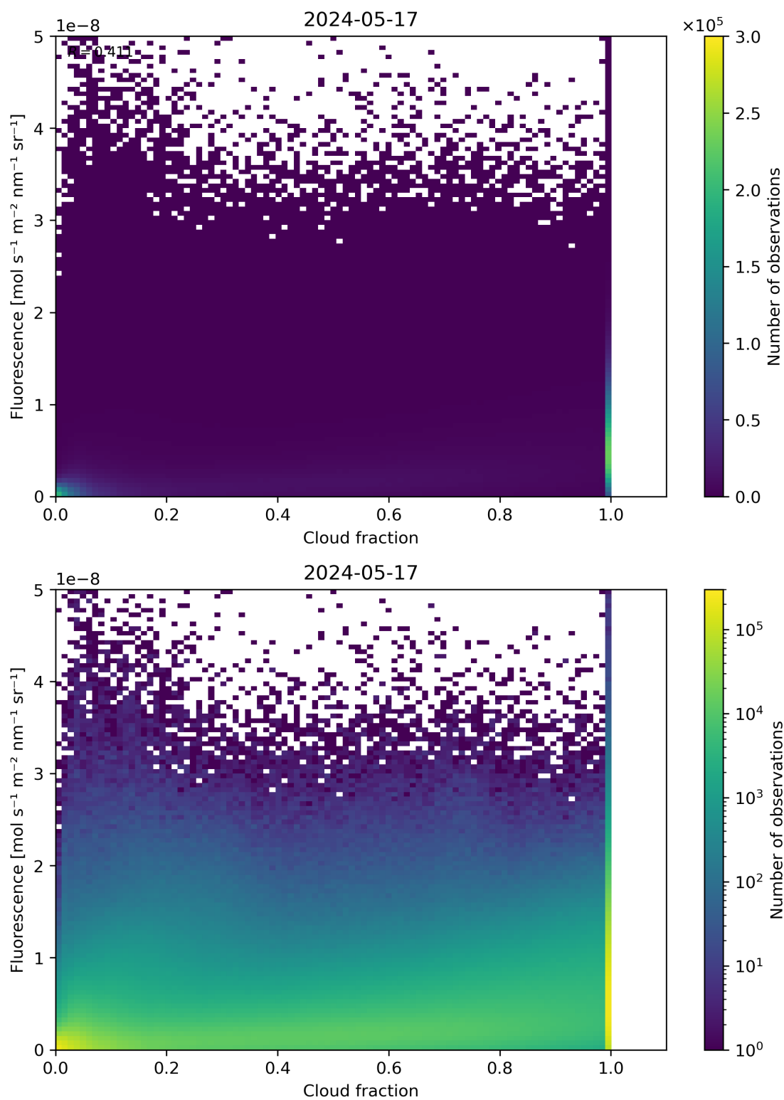
Figure 72: Scatter density plot of "Cloud fraction" against "Fluorescence" for 2024-05-16 to 2024-05-18.
