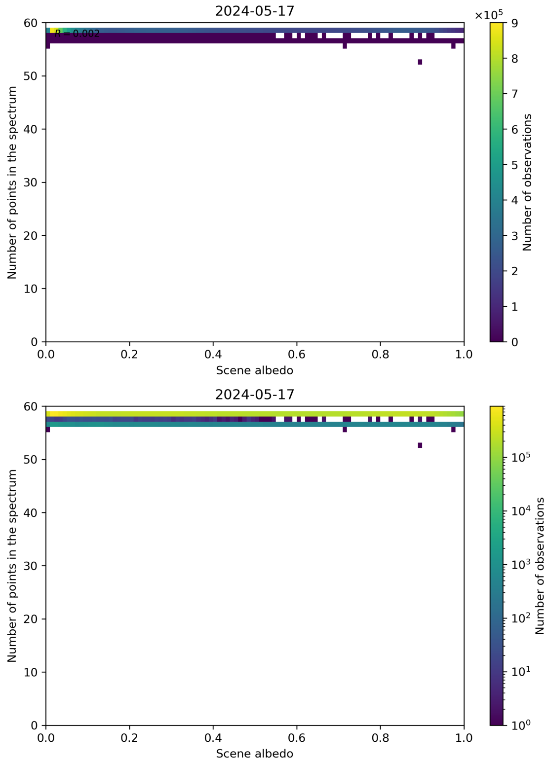
Figure 106: Scatter density plot of “Scene albedo” against “Number of points in the spectrum” for 2024-05-16 to 2024-05-18.
