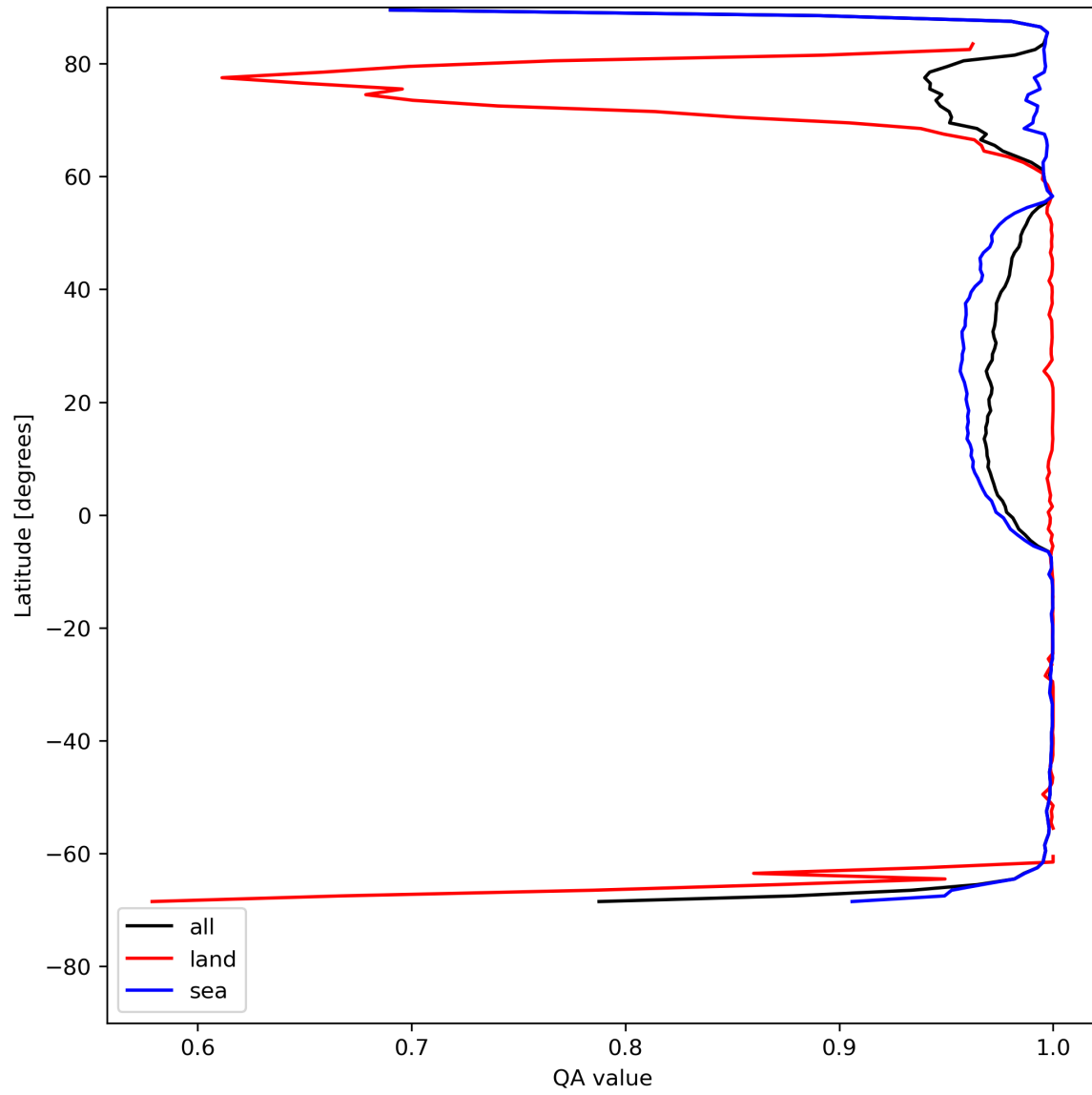
Figure 12: Zonal average of “QA value” for 2024-05-16 to 2024-05-18.
