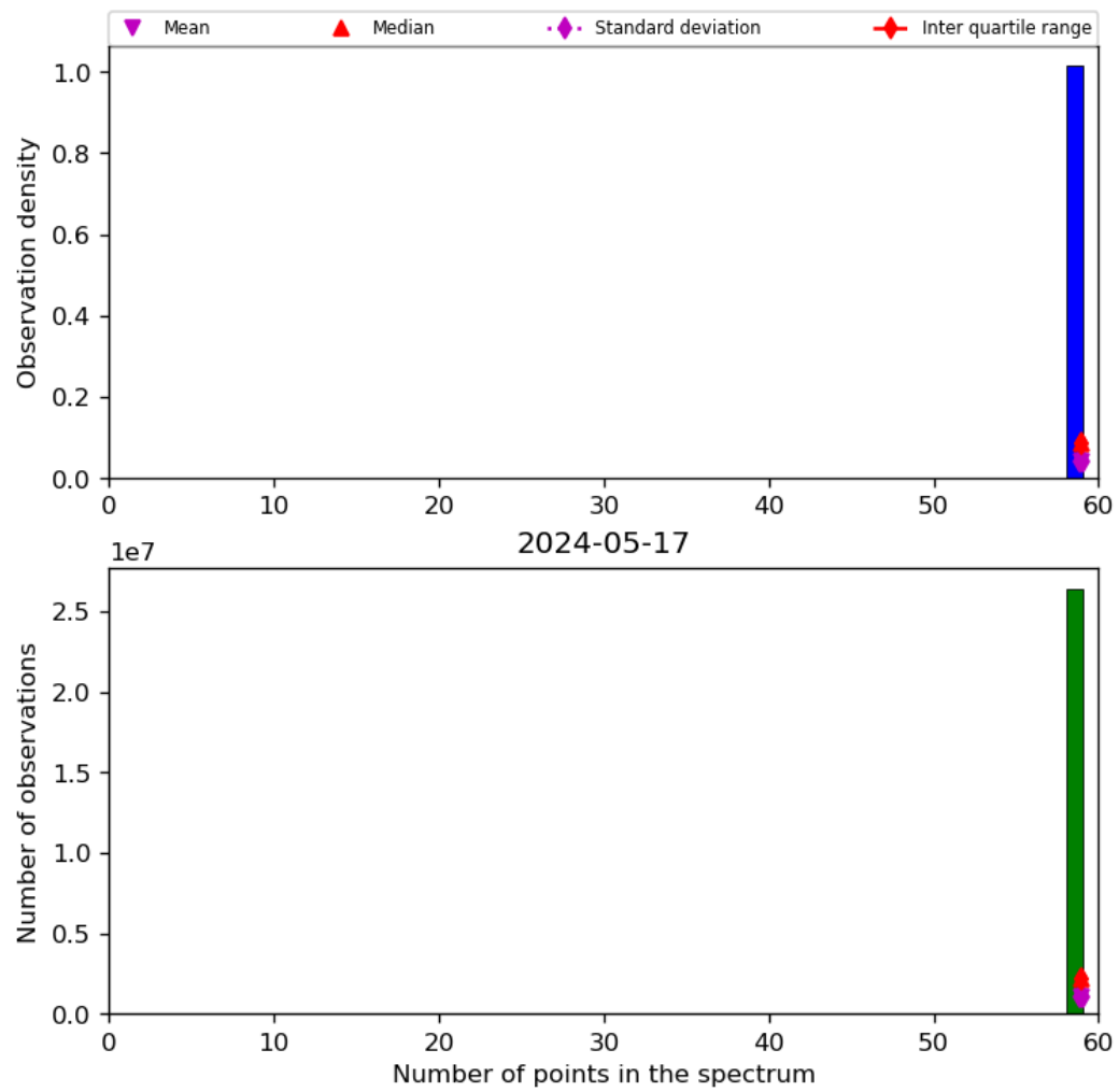
Figure 44: Histogram of “Number of points in the spectrum” for 2024-05-16 to 2024-05-18
