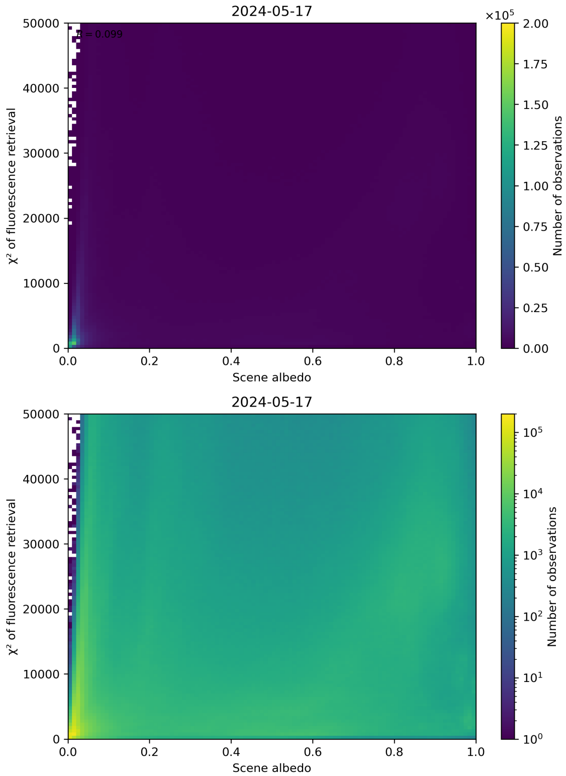
Figure 103: Scatter density plot of “Scene albedo” against “ \chi^2 of fluorescence retrieval” for 2024-05-16 to 2024-05-18.
