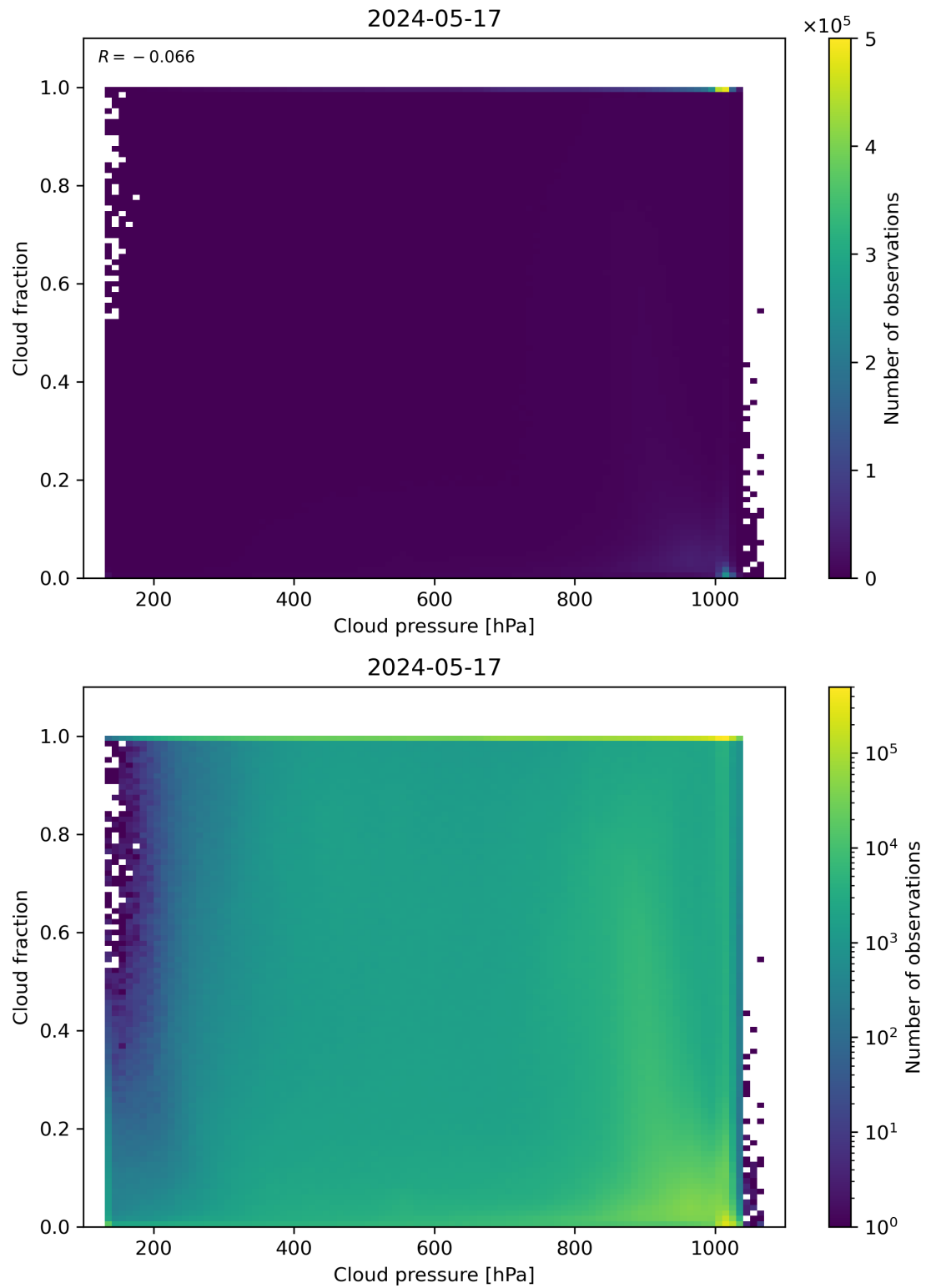
Figure 79: Scatter density plot of “Cloud pressure” against “Cloud fraction” for 2024-05-16 to 2024-05-18.
