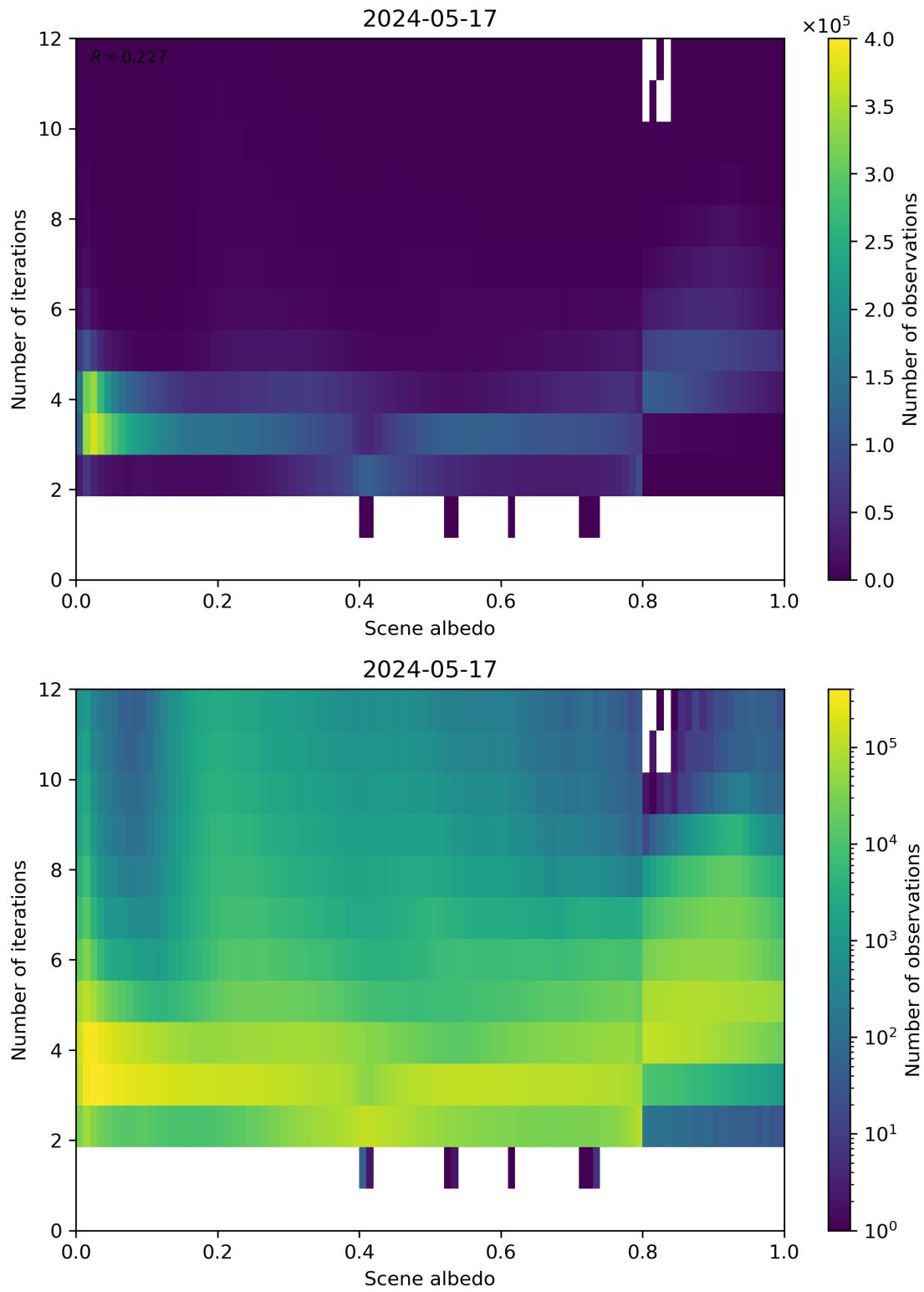
Figure 105: Scatter density plot of “Scene albedo” against “Number of iterations” for 2024-05-16 to 2024-05-18.
