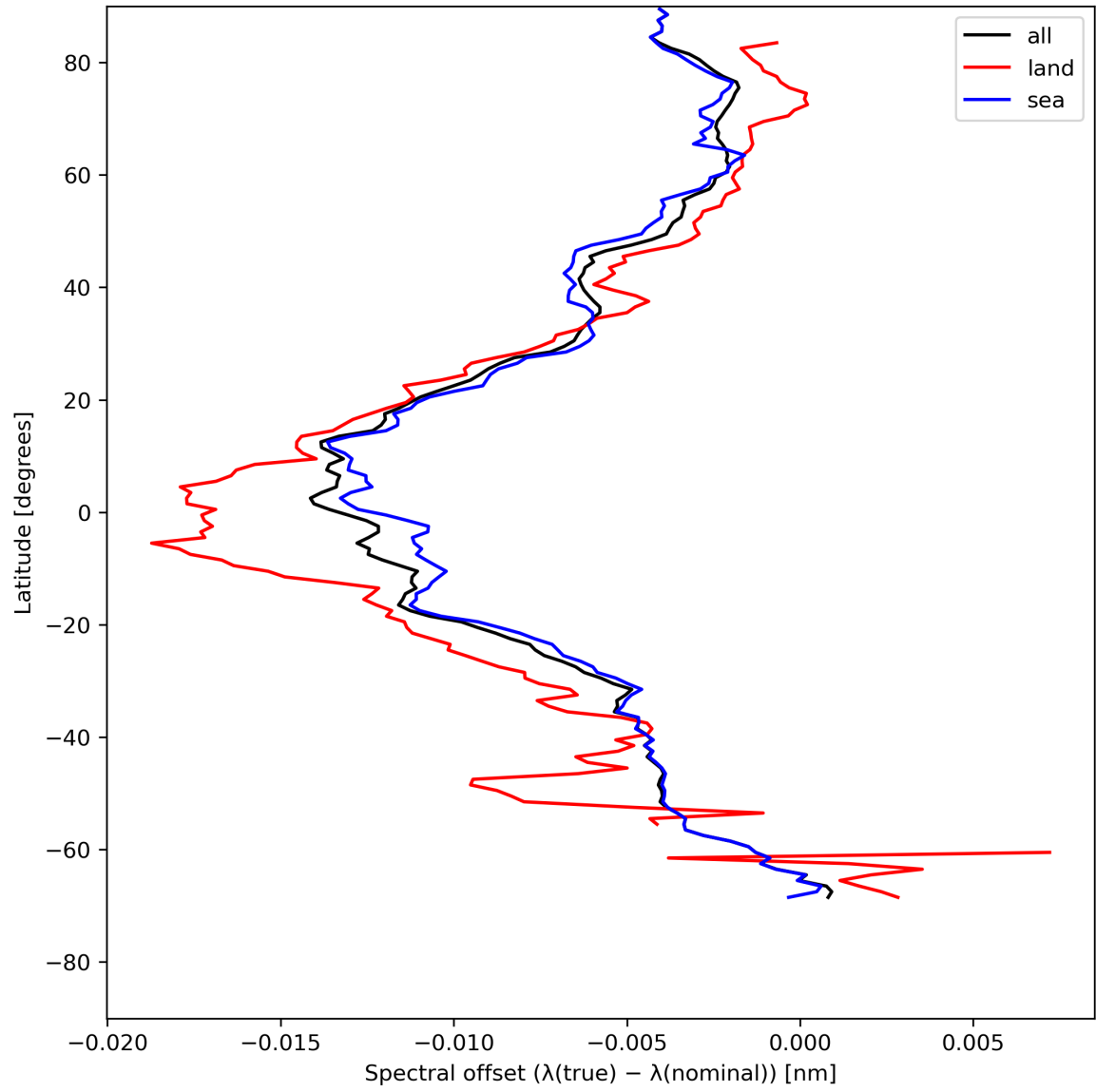
Figure 28: Zonal average of “Spectral offset ( \lambda(\text{true}) - \lambda(\text{nominal}) )” for 2024-05-16 to 2024-05-18.
