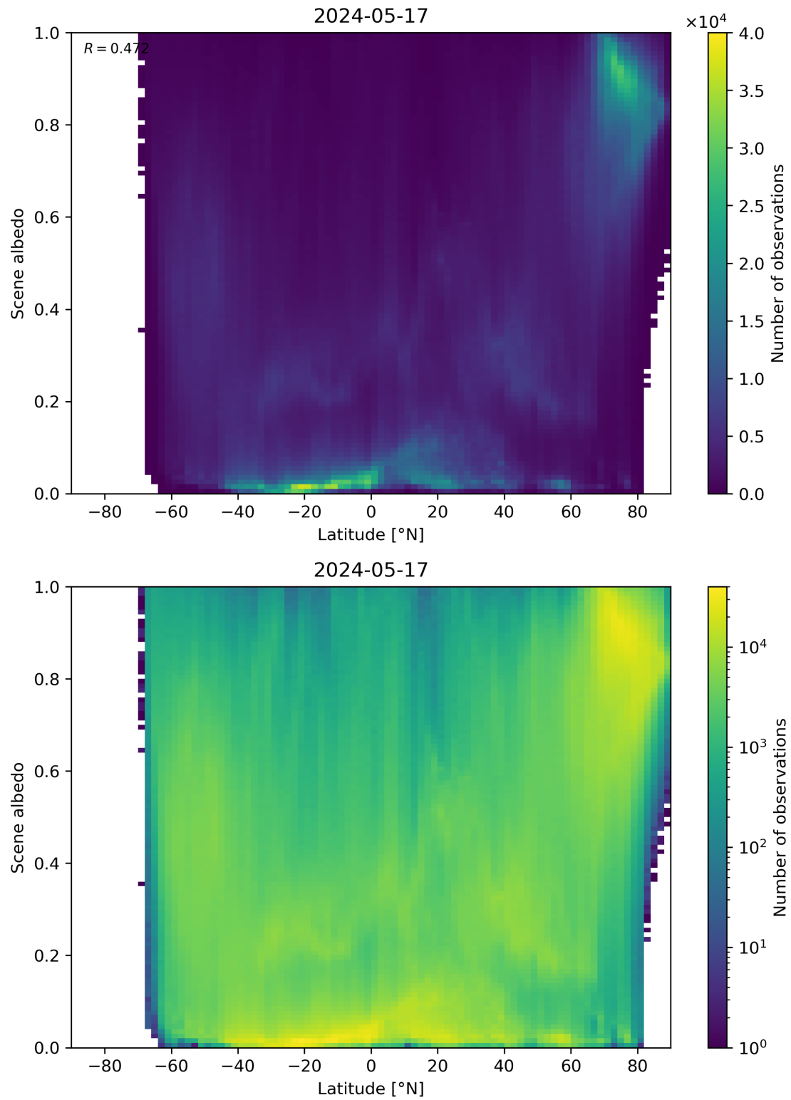
Figure 95: Scatter density plot of “Latitude” against “Scene albedo” for 2024-05-16 to 2024-05-18.
