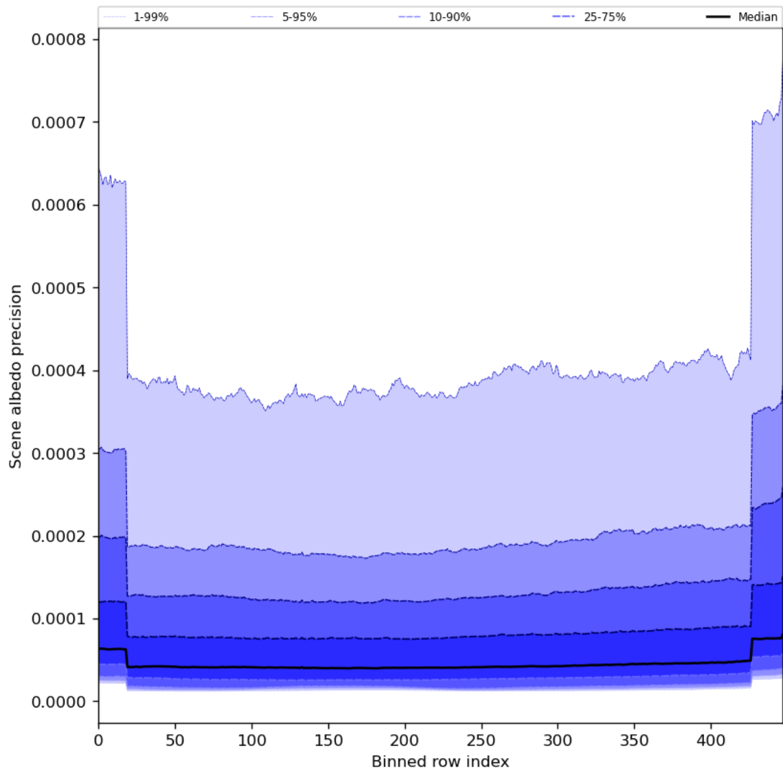
Figure 52: Along track statistics of “Scene albedo precision” for 2024-05-16 to 2024-05-18
