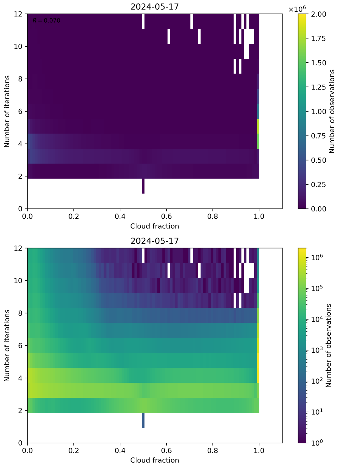
Figure 73: Scatter density plot of “Cloud fraction” against “Number of iterations” for 2024-05-16 to 2024-05-18.
