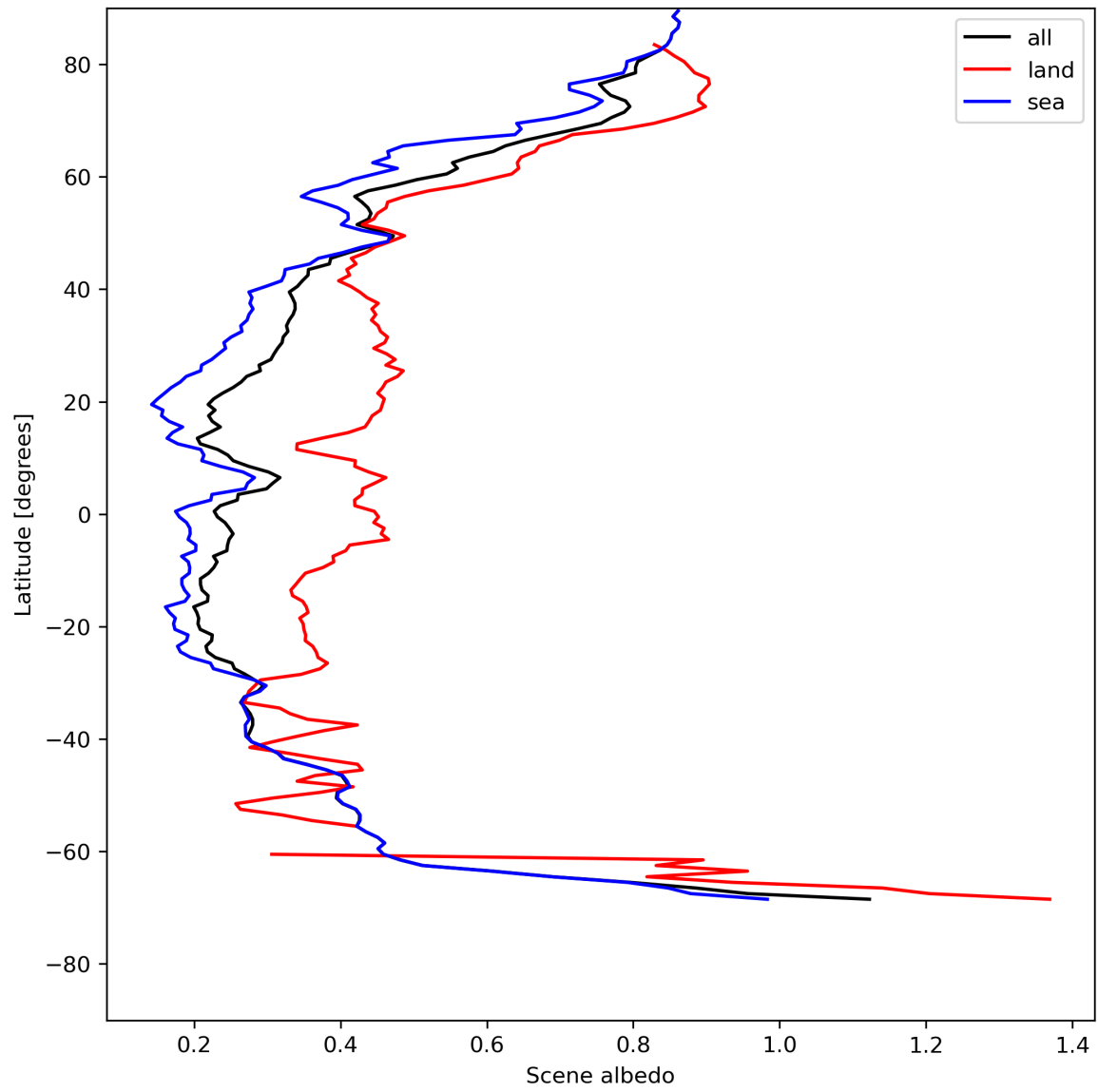
Figure 17: Zonal average of “Scene albedo” for 2024-05-16 to 2024-05-18.
