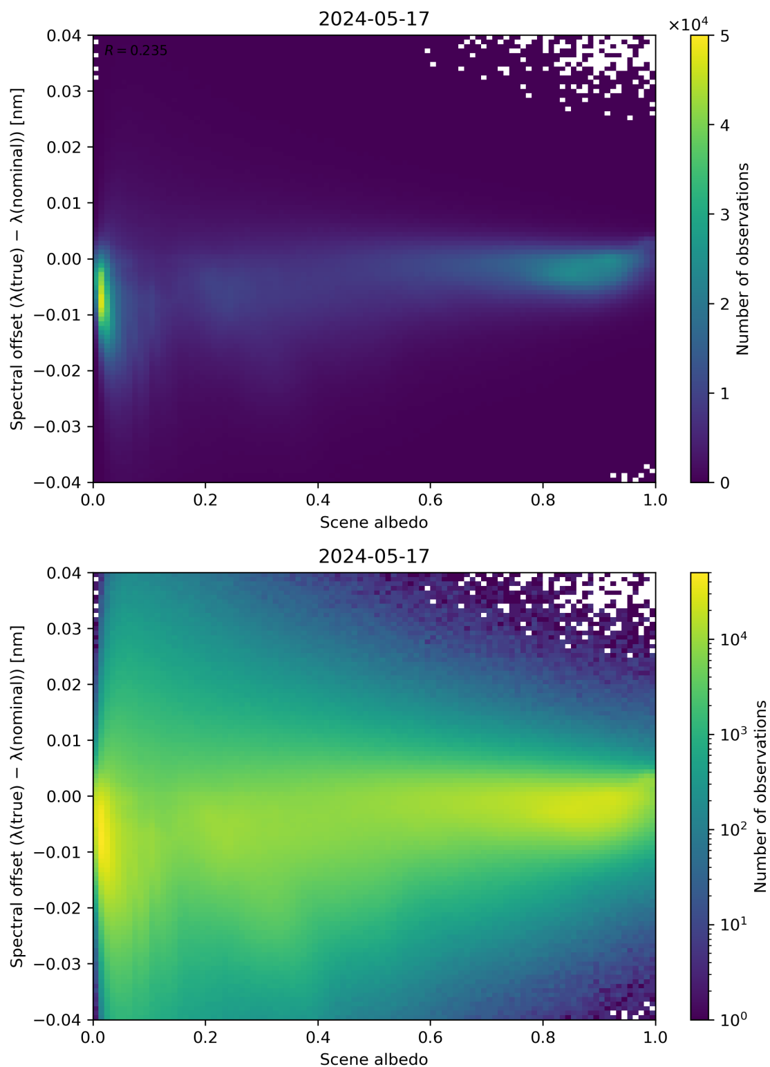
Figure 107: Scatter density plot of “Scene albedo” against “Spectral offset ( \lambda(\text{true}) - \lambda(\text{nominal}) )” for 2024-05-16 to 2024-05-18.
