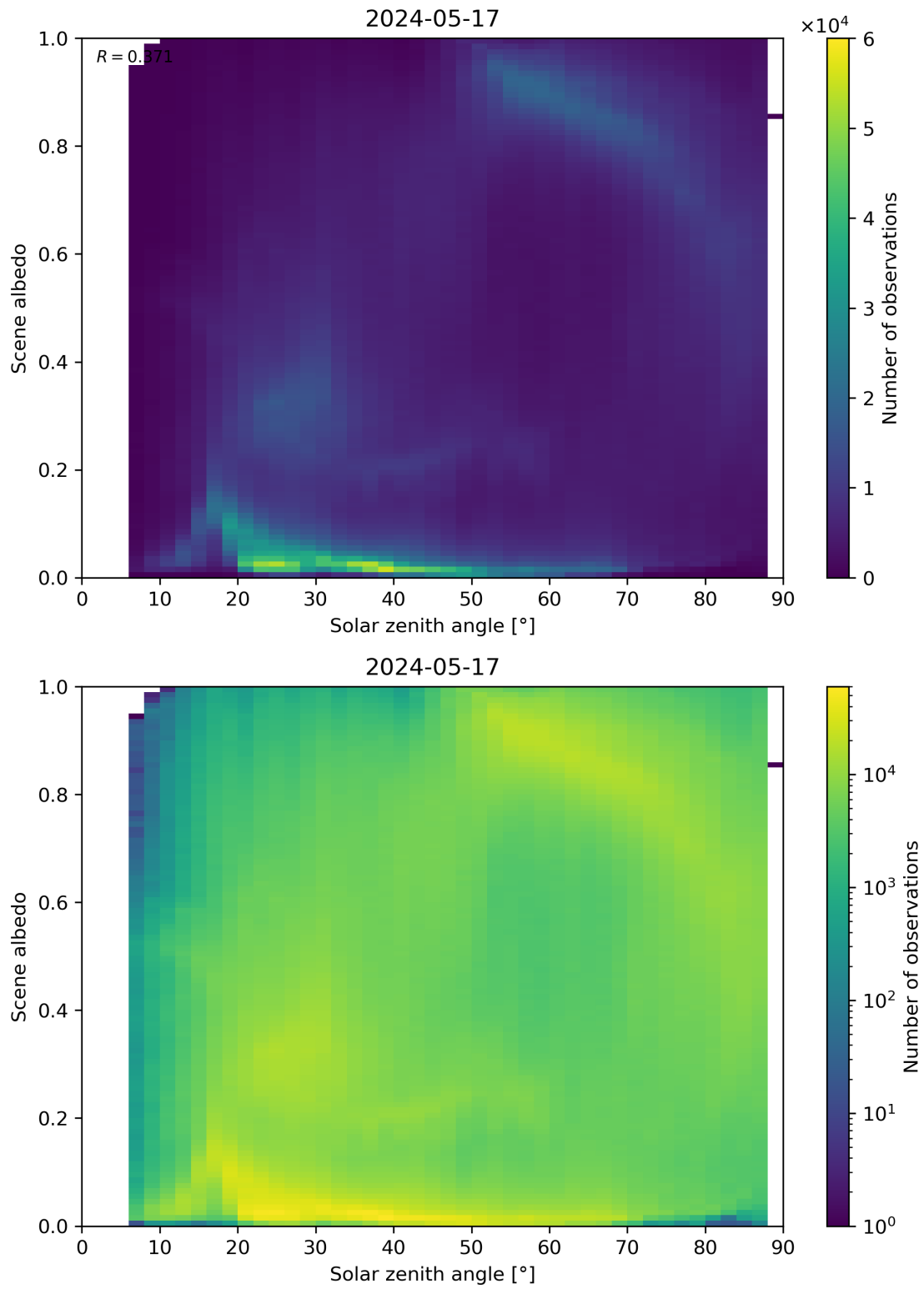
Figure 116: Scatter density plot of “Solar zenith angle” against “Scene albedo” for 2024-05-16 to 2024-05-18.
