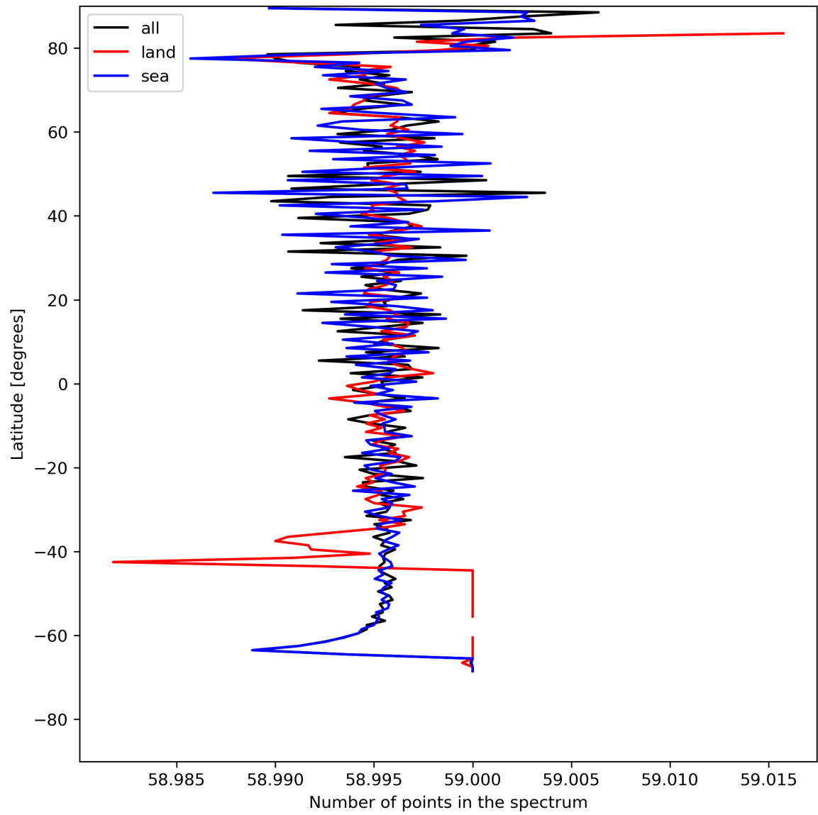
Figure 27: Zonal average of “Number of points in the spectrum” for 2024-05-16 to 2024-05-18.
