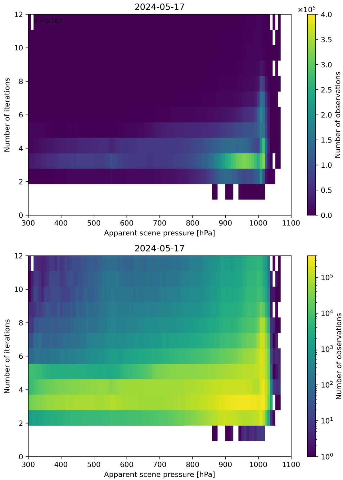
Figure 65: Scatter density plot of “Apparent scene pressure” against “Number of iterations” for 2024-05-16 to 2024-05-18.
