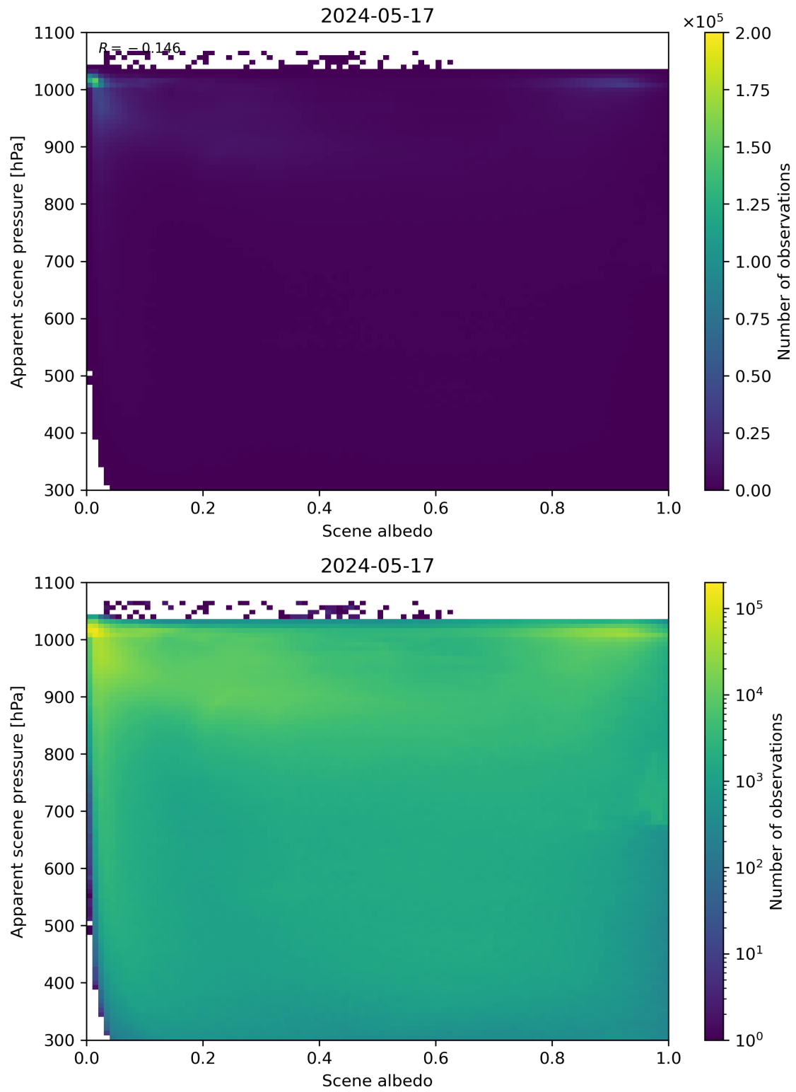
Figure 102: Scatter density plot of “Scene albedo” against “Apparent scene pressure” for 2024-05-16 to 2024-05-18.
