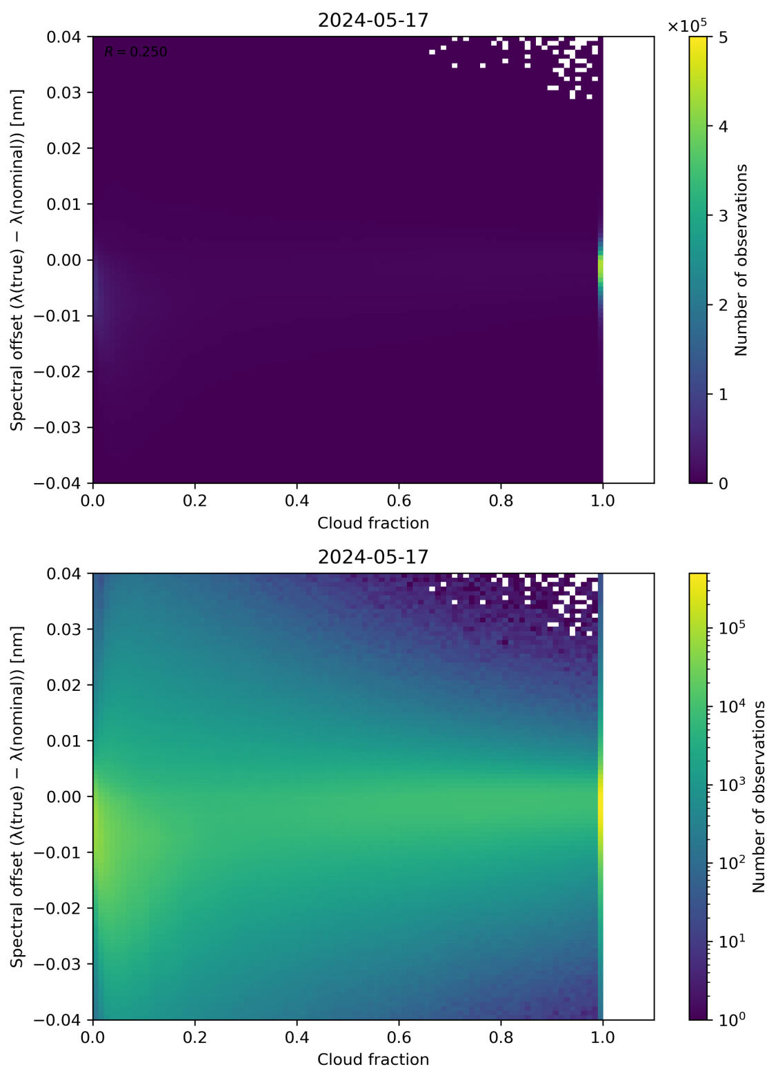
Figure 76: Scatter density plot of “Cloud fraction” against “Spectral offset ( \lambda(\text{true}) - \lambda(\text{nominal}) )” for 2024-05-16 to 2024-05-18.
