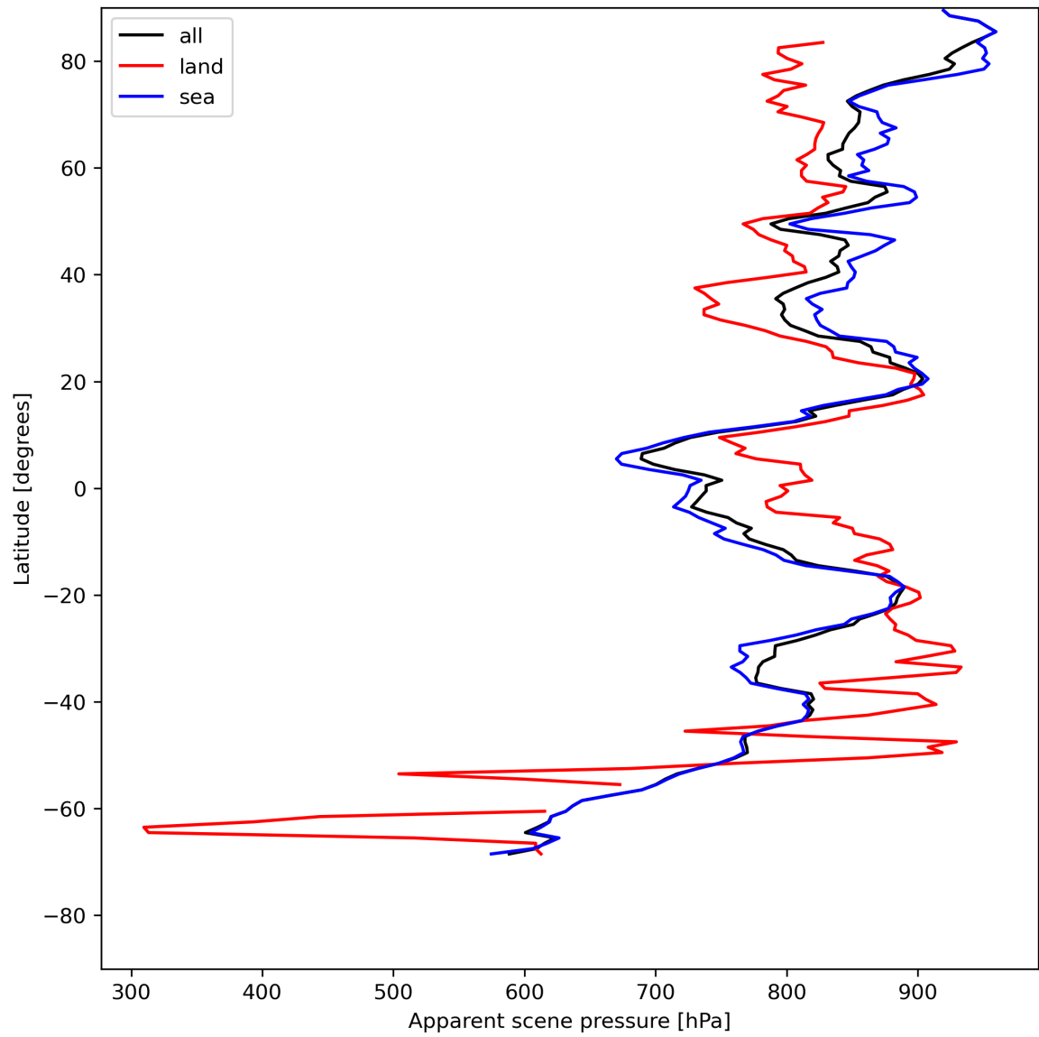
Figure 19: Zonal average of “Apparent scene pressure” for 2024-05-16 to 2024-05-18.
