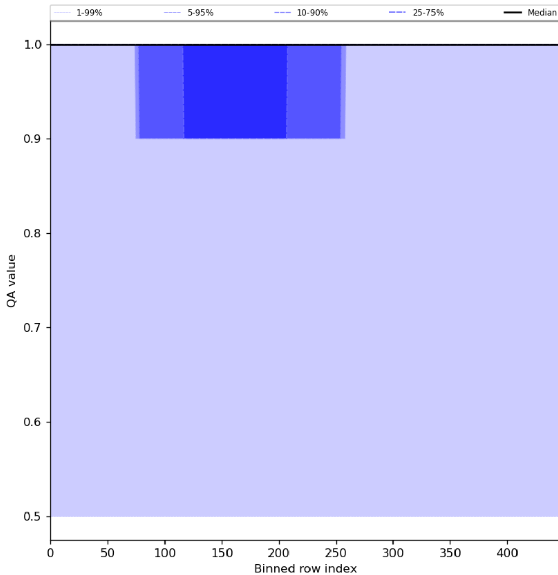
Figure 46: Along track statistics of “QA value” for 2024-05-16 to 2024-05-18
