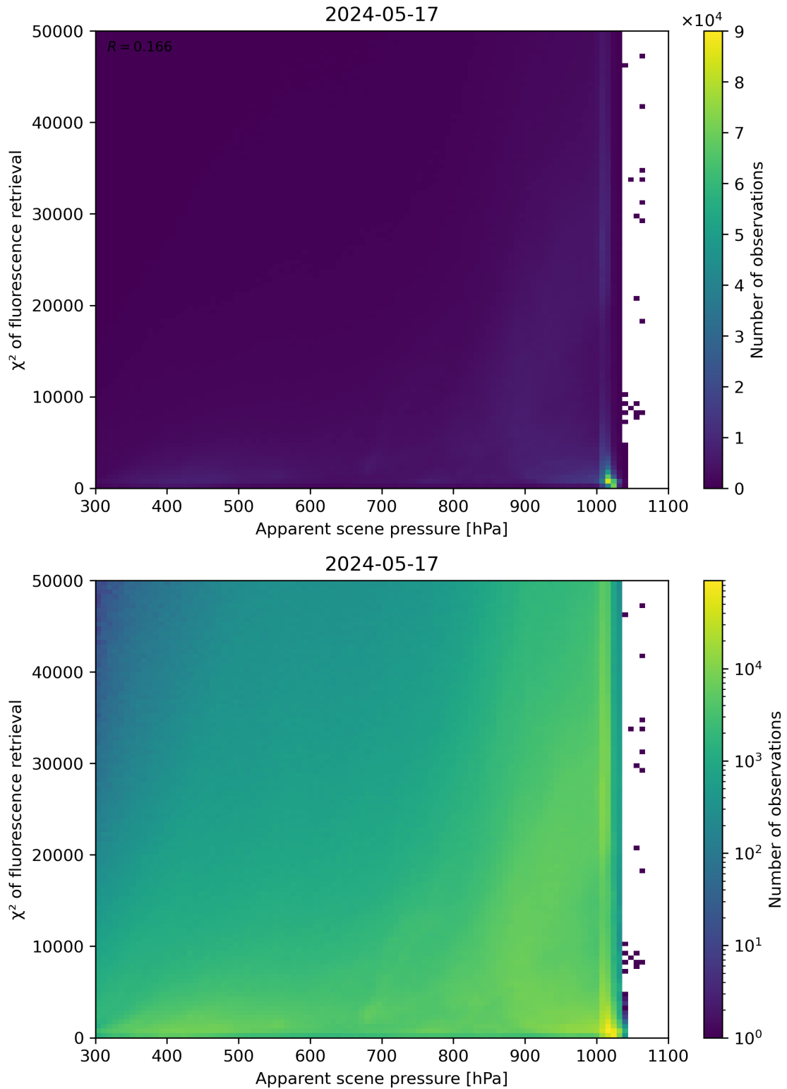
Figure 63: Scatter density plot of “Apparent scene pressure” against “ \chi^2 of fluorescence retrieval” for 2024-05-16 to 2024-05-18.
