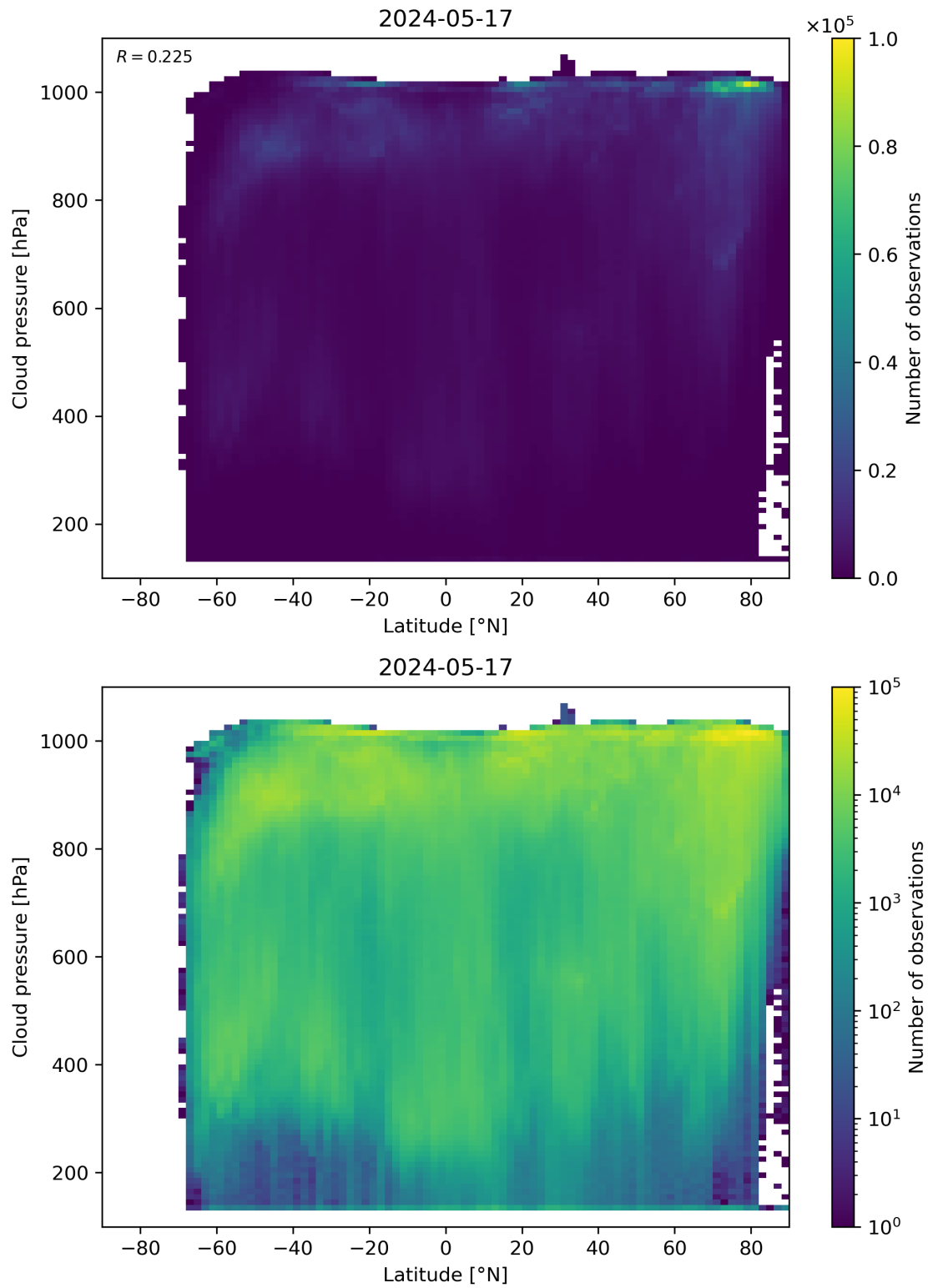
Figure 91: Scatter density plot of “Latitude” against “Cloud pressure” for 2024-05-16 to 2024-05-18.
