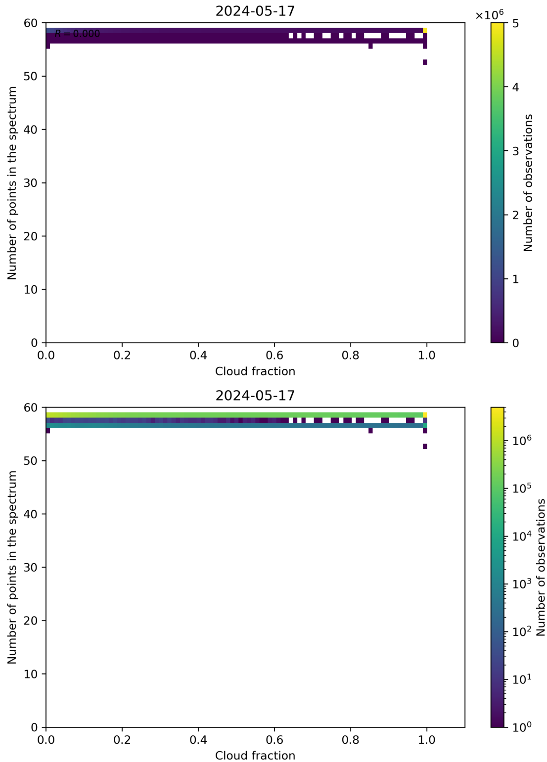
Figure 74: Scatter density plot of “Cloud fraction” against “Number of points in the spectrum” for 2024-05-16 to 2024-05-18.
