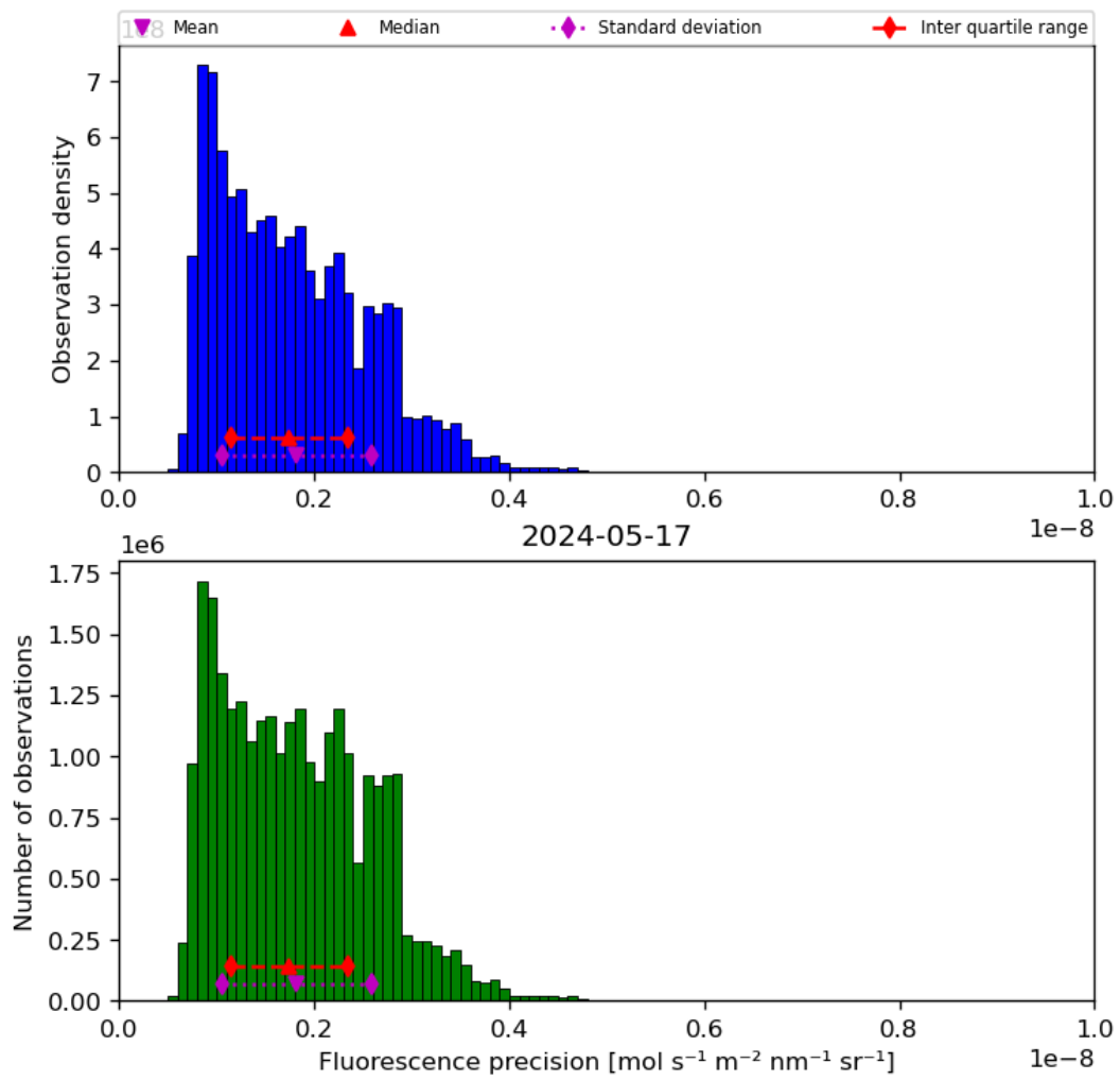
Figure 41: Histogram of “Fluorescence precision” for 2024-05-16 to 2024-05-18
