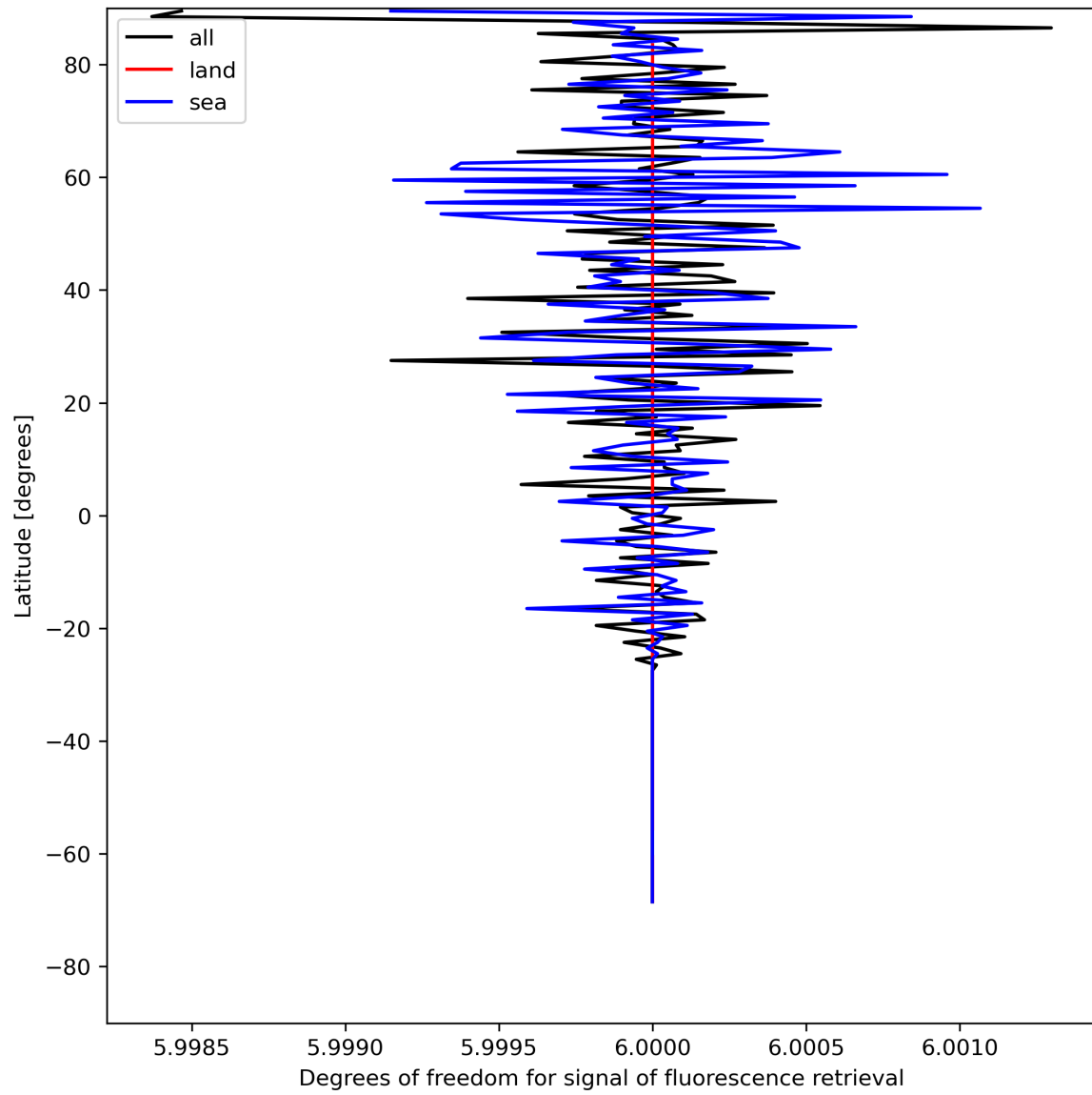
Figure 26: Zonal average of “Degrees of freedom for signal of fluorescence retrieval” for 2024-05-16 to 2024-05-18.
