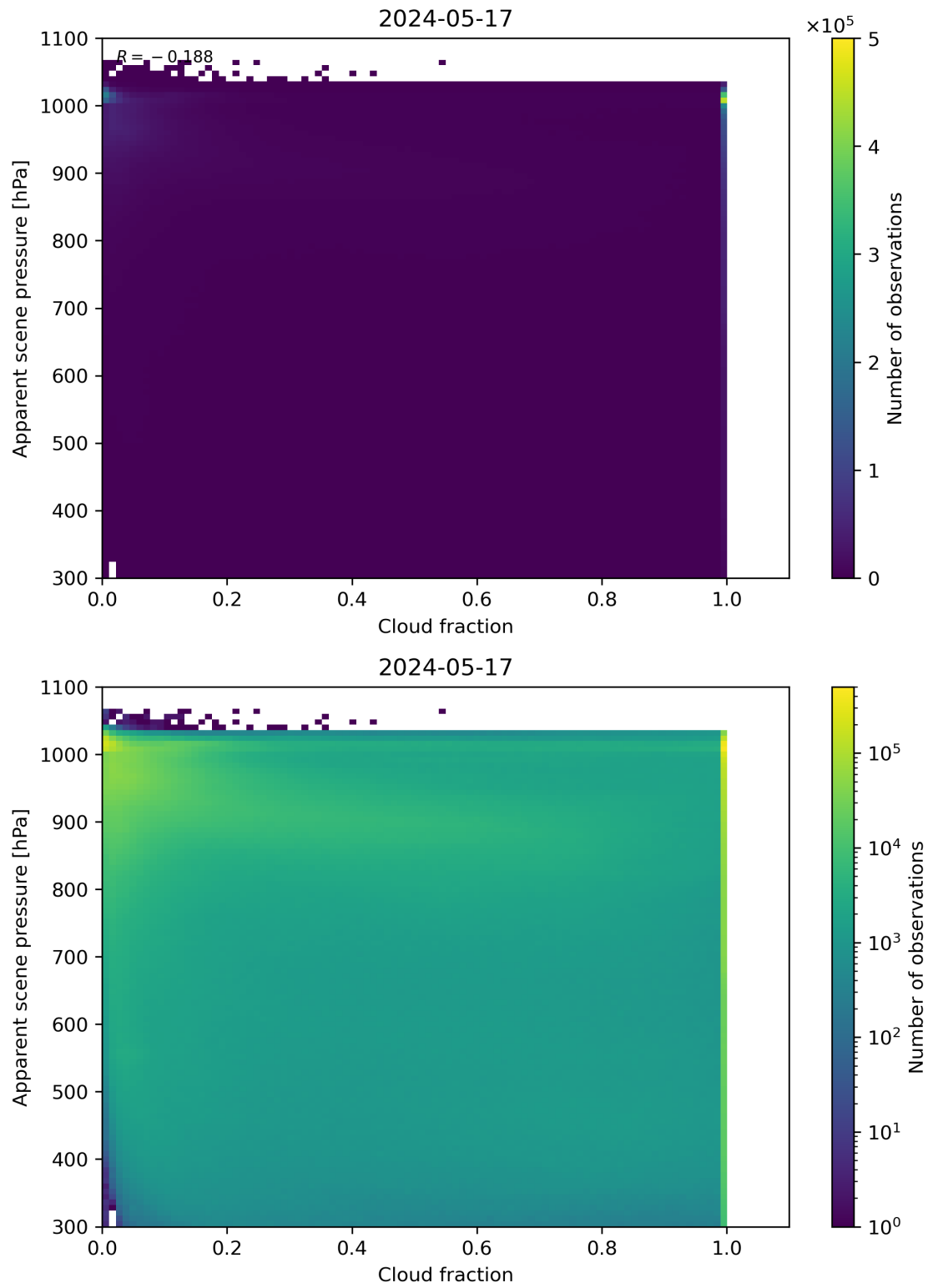
Figure 70: Scatter density plot of “Cloud fraction” against “Apparent scene pressure” for 2024-05-16 to 2024-05-18.
