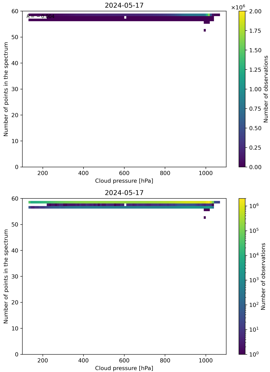
Figure 82: Scatter density plot of “Cloud pressure” against “Number of points in the spectrum” for 2024-05-16 to 2024-05-18.
