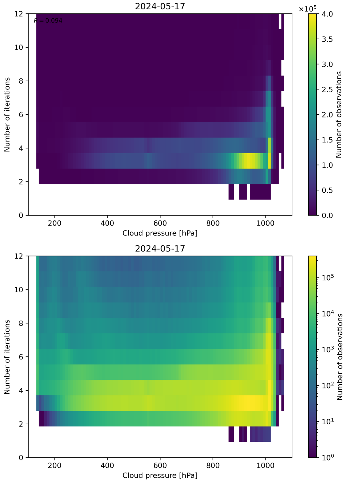
Figure 81: Scatter density plot of “Cloud pressure” against “Number of iterations” for 2024-05-16 to 2024-05-18.
