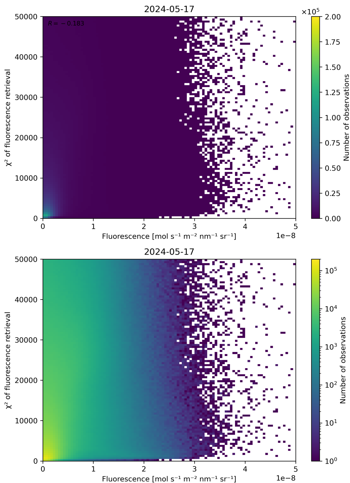
Figure 85: Scatter density plot of “Fluorescence” against “ \chi^2 of fluorescence retrieval” for 2024-05-16 to 2024-05-18.
