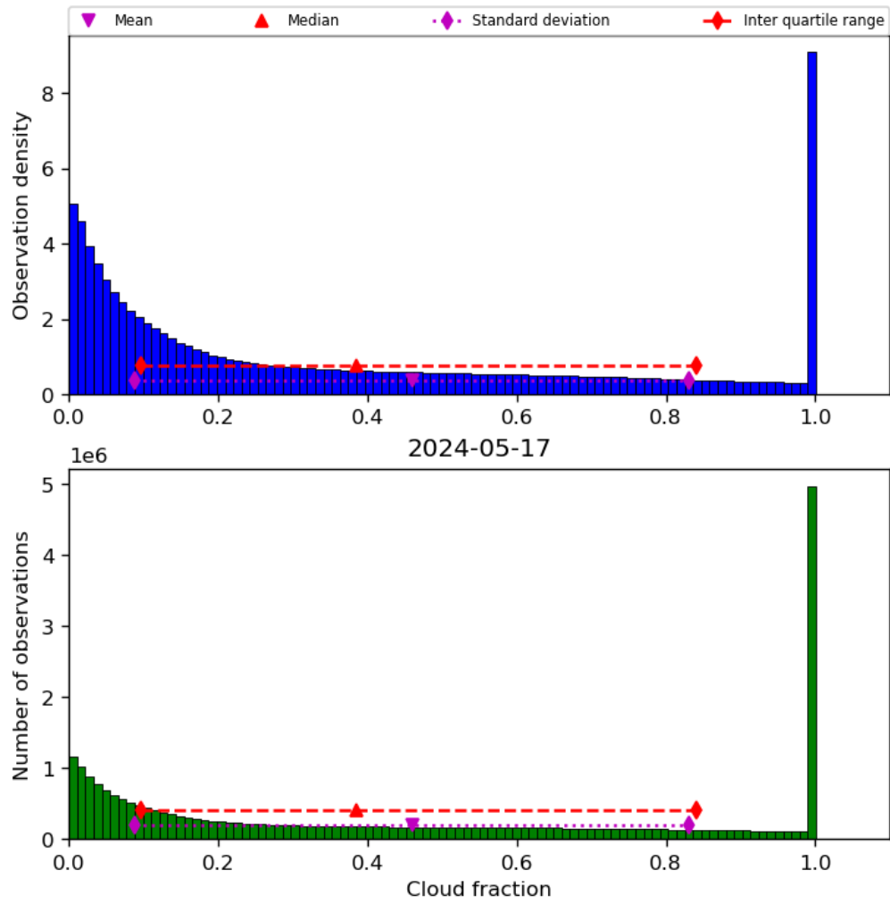
Figure 32: Histogram of “Cloud fraction” for 2024-05-16 to 2024-05-18
