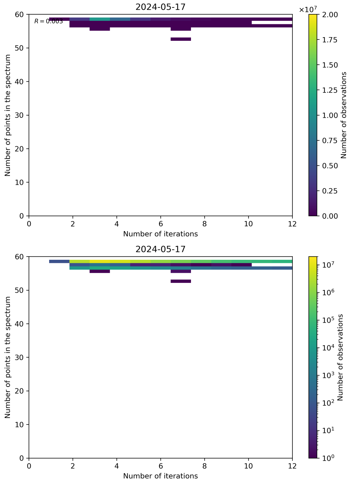
Figure 99: Scatter density plot of “Number of iterations” against “Number of points in the spectrum” for 2024-05-16 to 2024-05-18.
