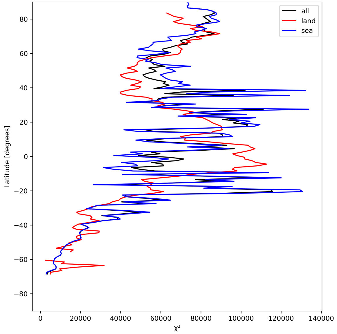
Figure 21: Zonal average of “ \chi^2 ” for 2024-05-16 to 2024-05-18.
