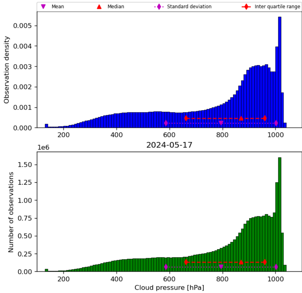
Figure 30: Histogram of “Cloud pressure” for 2024-05-16 to 2024-05-18
