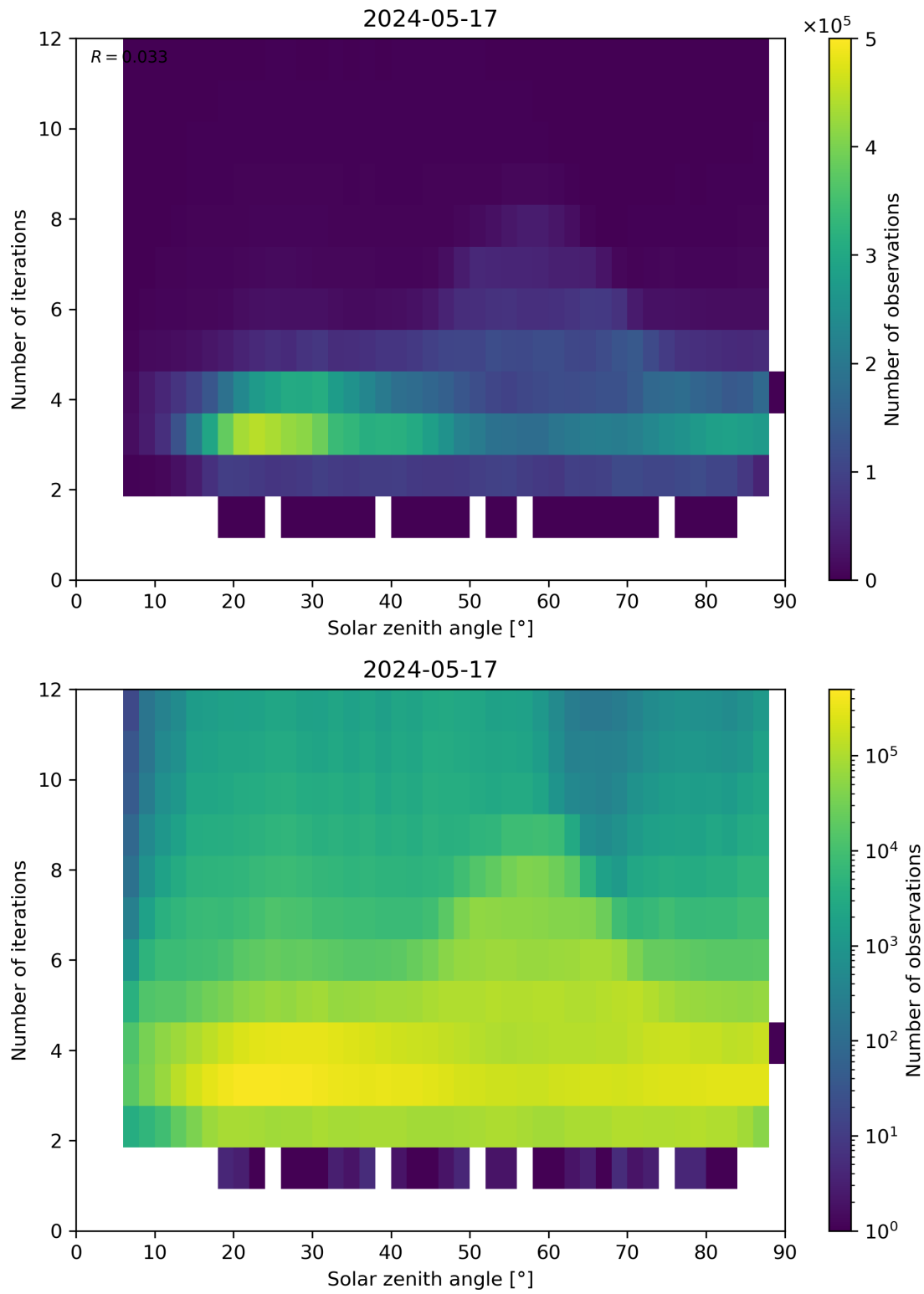
Figure 114: Scatter density plot of “Solar zenith angle” against “Number of iterations” for 2024-05-16 to 2024-05-18.
