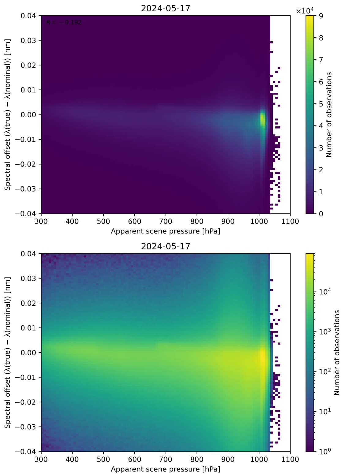
Figure 67: Scatter density plot of “Apparent scene pressure” against “Spectral offset ( \lambda(\text{true}) - \lambda(\text{nominal}) )” for 2024-05-16 to 2024-05-18.
