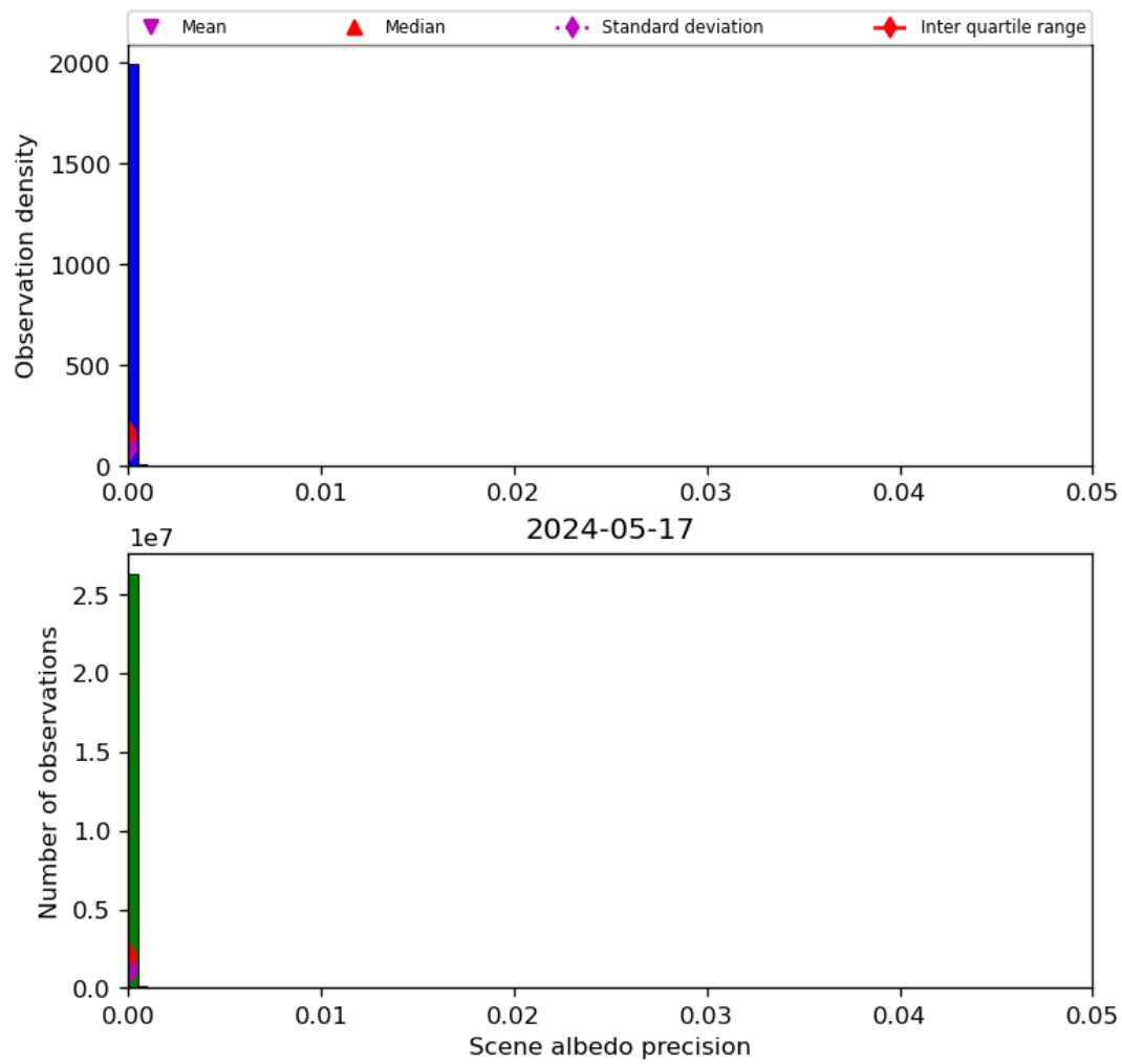
Figure 35: Histogram of “Scene albedo precision” for 2024-05-16 to 2024-05-18
