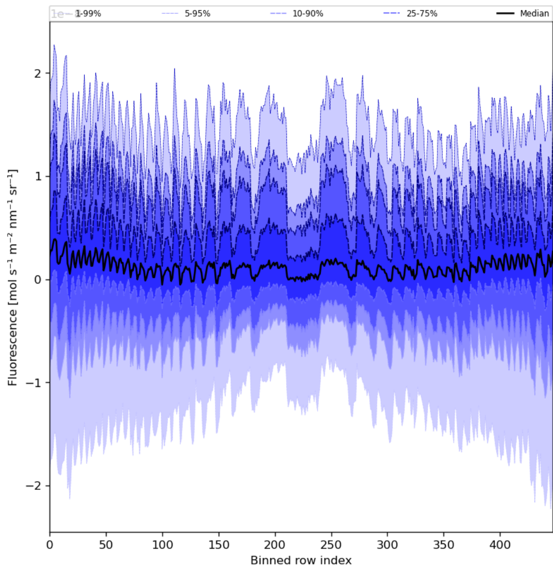
Figure 57: Along track statistics of “Fluorescence” for 2024-05-16 to 2024-05-18
