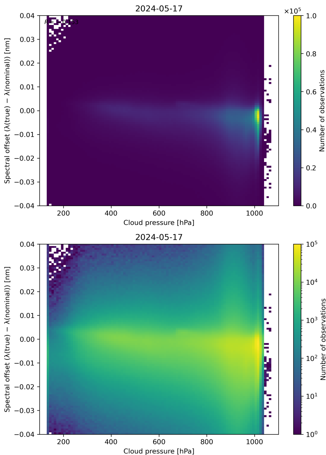
Figure 84: Scatter density plot of “Cloud pressure” against “Spectral offset ( \lambda(\text{true}) - \lambda(\text{nominal}) )” for 2024-05-16 to 2024-05-18.
