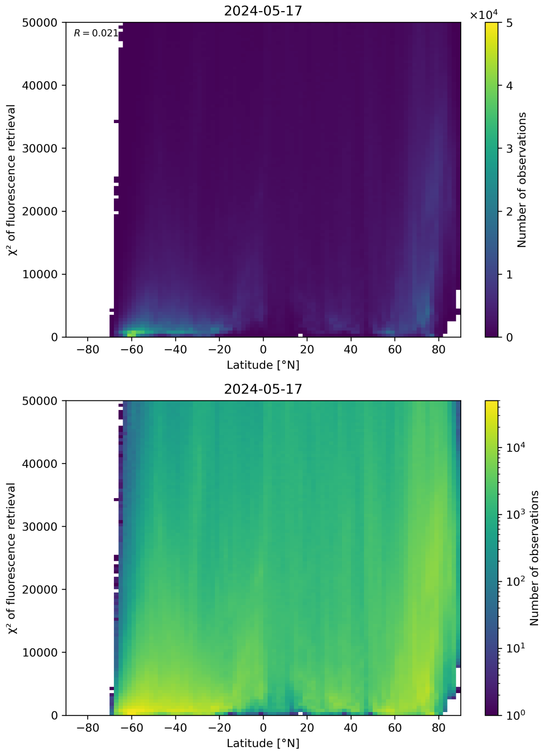
Figure 89: Scatter density plot of “Latitude” against “ \chi^2 of fluorescence retrieval” for 2024-05-16 to 2024-05-18.
