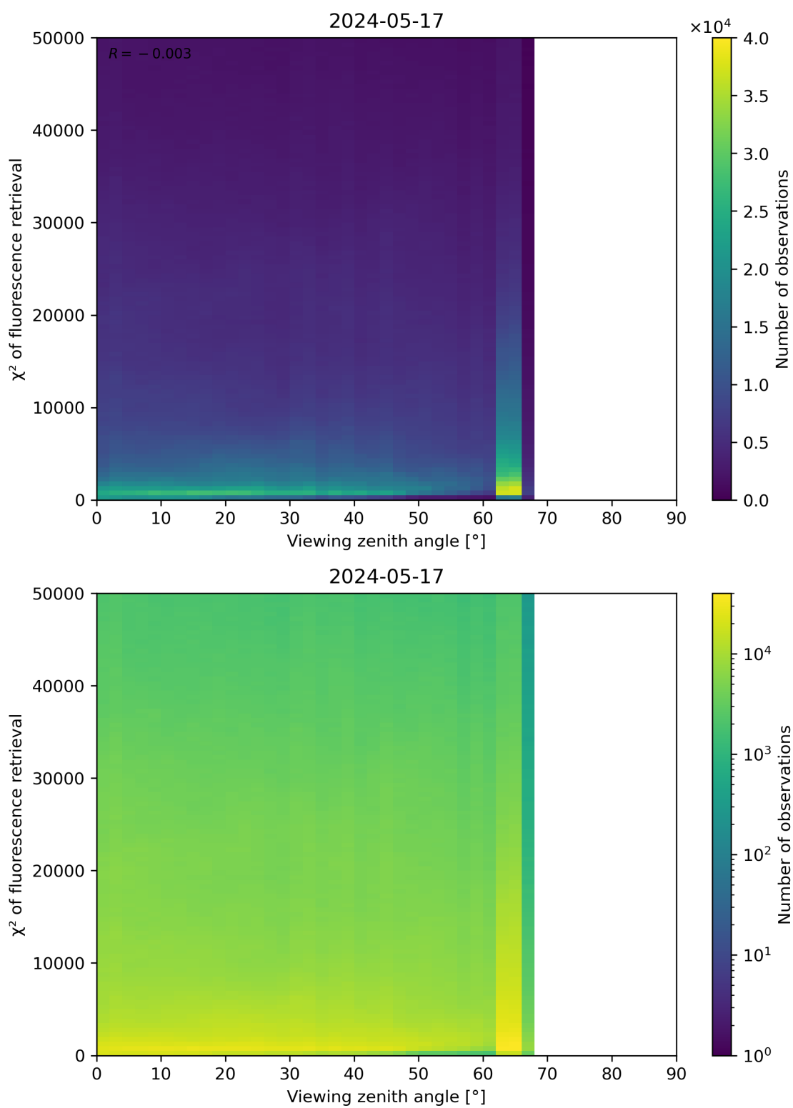
Figure 119: Scatter density plot of “Viewing zenith angle” against “ \chi^2 of fluorescence retrieval” for 2024-05-16 to 2024-05-18.
