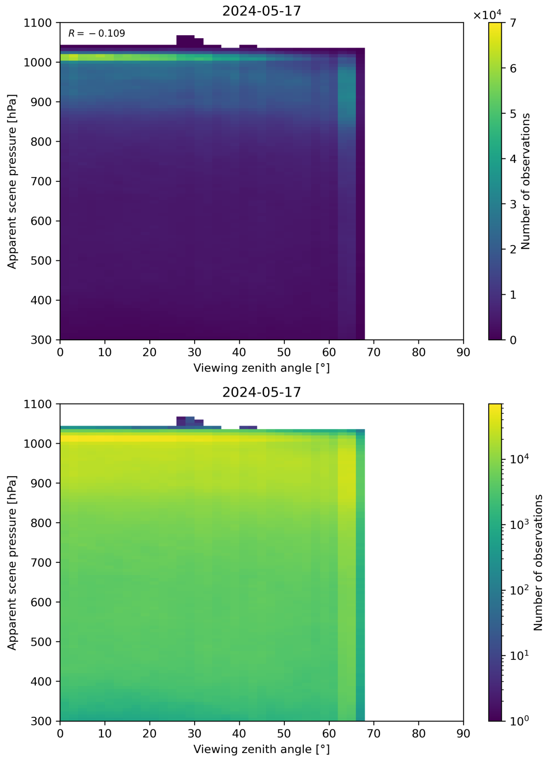
Figure 118: Scatter density plot of “Viewing zenith angle” against “Apparent scene pressure” for 2024-05-16 to 2024-05-18.
