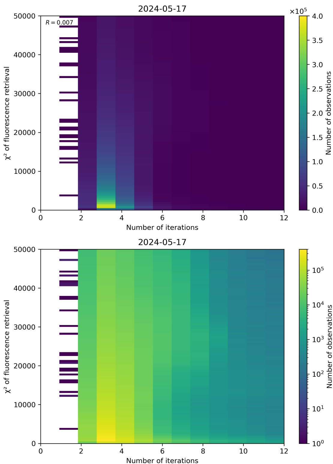
Figure 97: Scatter density plot of “Number of iterations” against “ \chi^2 of fluorescence retrieval” for 2024-05-16 to 2024-05-18.
