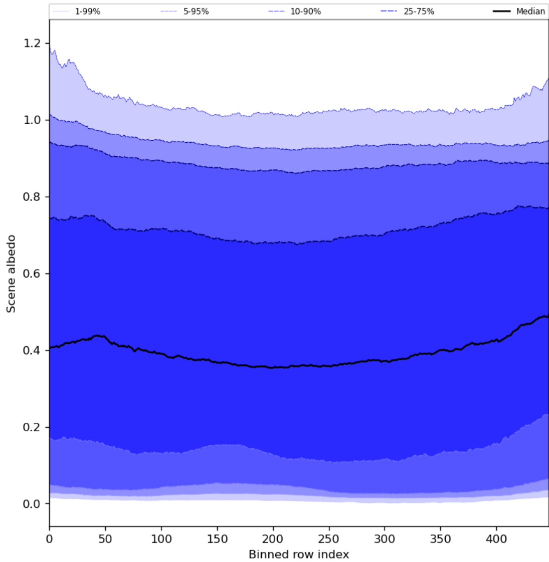
Figure 51: Along track statistics of “Scene albedo” for 2024-05-16 to 2024-05-18
