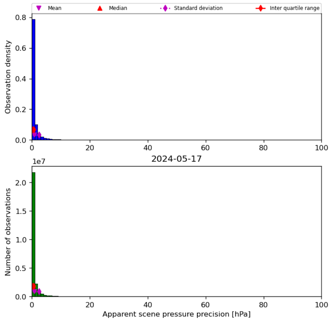
Figure 37: Histogram of “Apparent scene pressure precision” for 2024-05-16 to 2024-05-18
