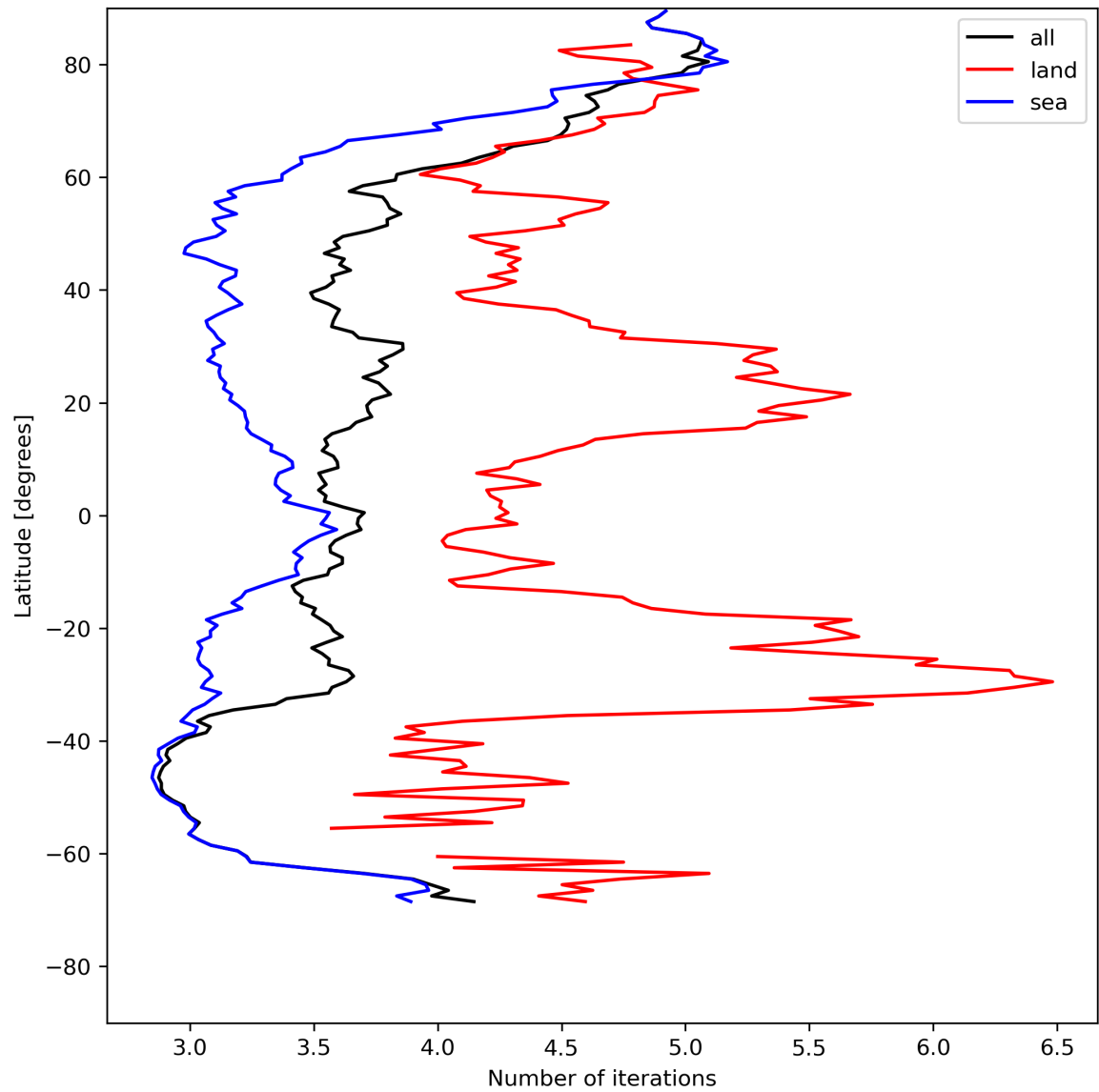
Figure 22: Zonal average of “Number of iterations” for 2024-05-16 to 2024-05-18.
