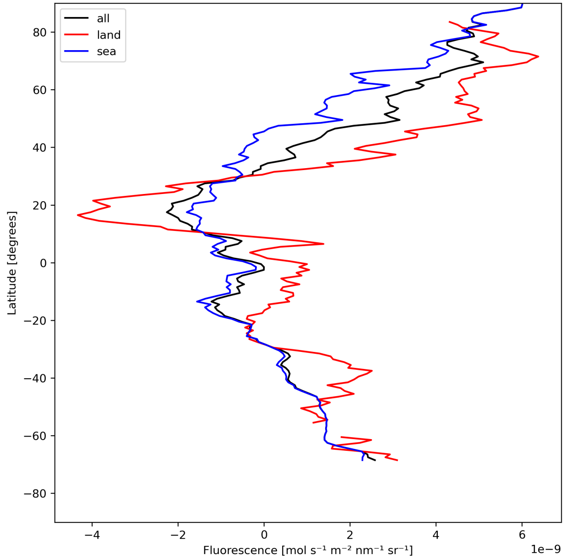
Figure 23: Zonal average of “Fluorescence” for 2024-05-16 to 2024-05-18.
