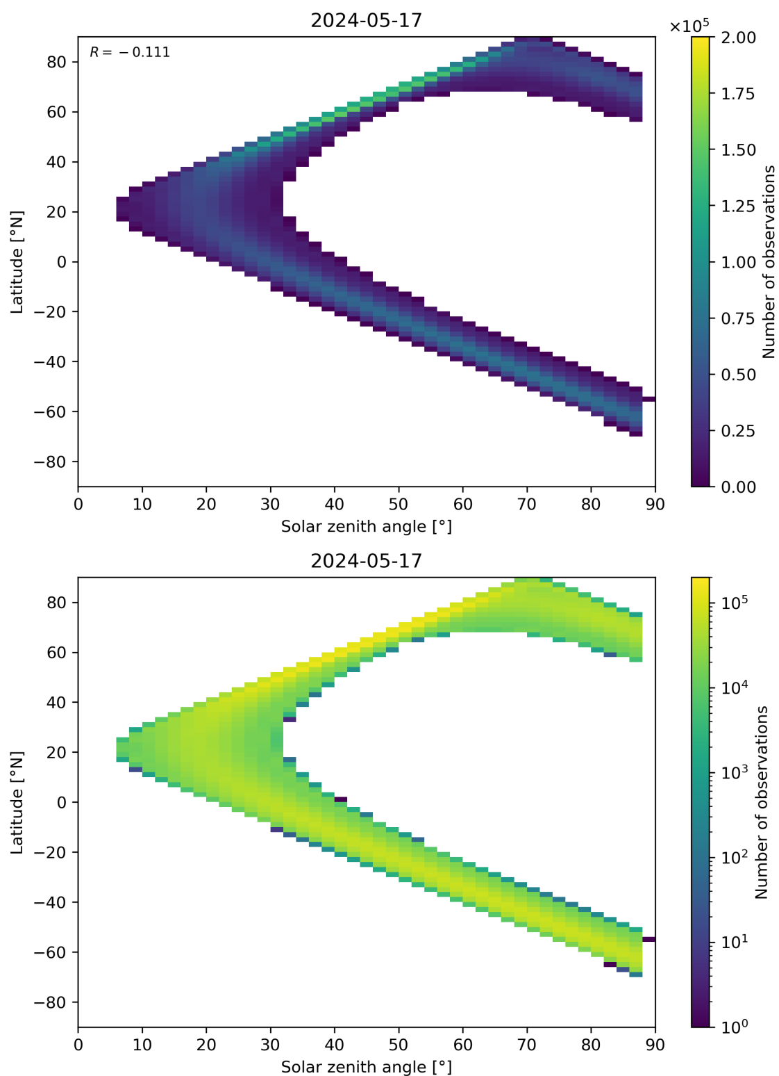
Figure 113: Scatter density plot of “Solar zenith angle” against “Latitude” for 2024-05-16 to 2024-05-18.
