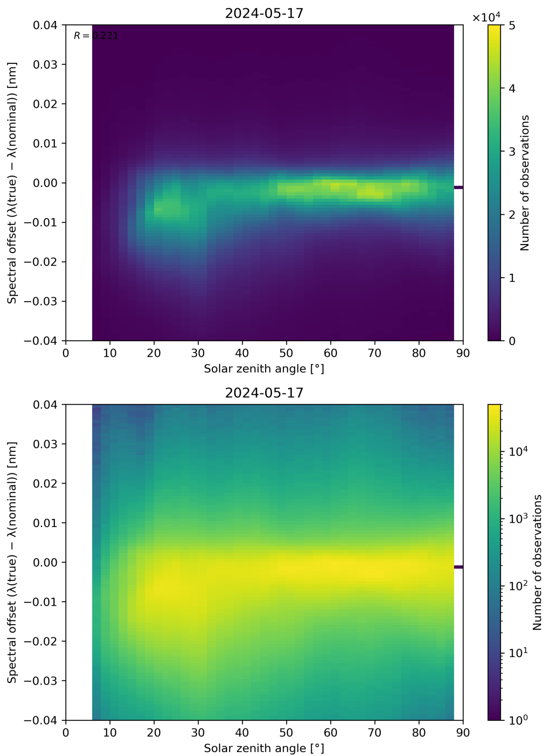
Figure 117: Scatter density plot of “Solar zenith angle” against “Spectral offset ( \lambda(\text{true}) - \lambda(\text{nominal}) )” for 2024-05-16 to 2024-05-18.
