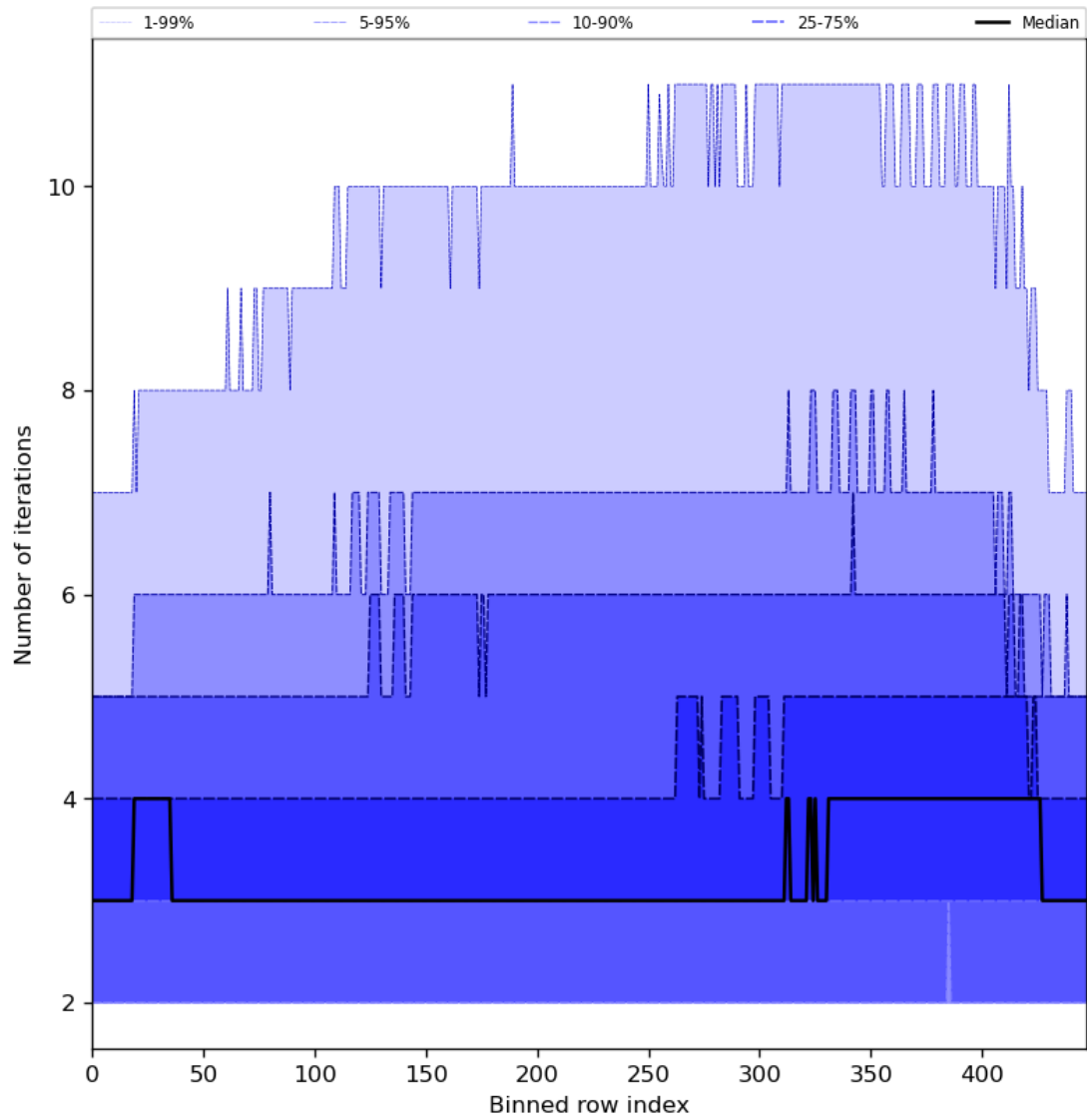
Figure 56: Along track statistics of “Number of iterations” for 2024-05-16 to 2024-05-18
