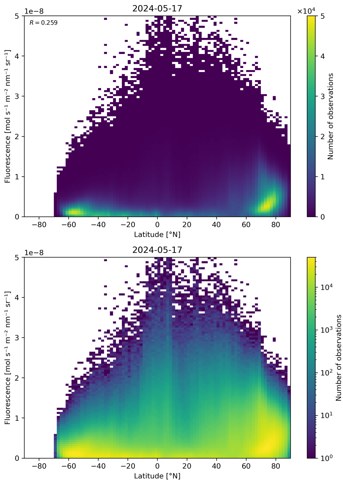
Figure 92: Scatter density plot of “Latitude” against “Fluorescence” for 2024-05-16 to 2024-05-18.
