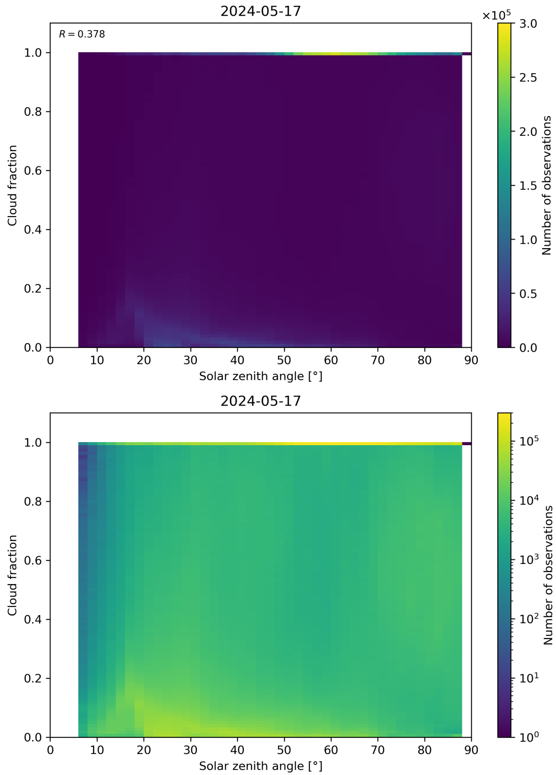
Figure 110: Scatter density plot of “Solar zenith angle” against “Cloud fraction” for 2024-05-16 to 2024-05-18.
