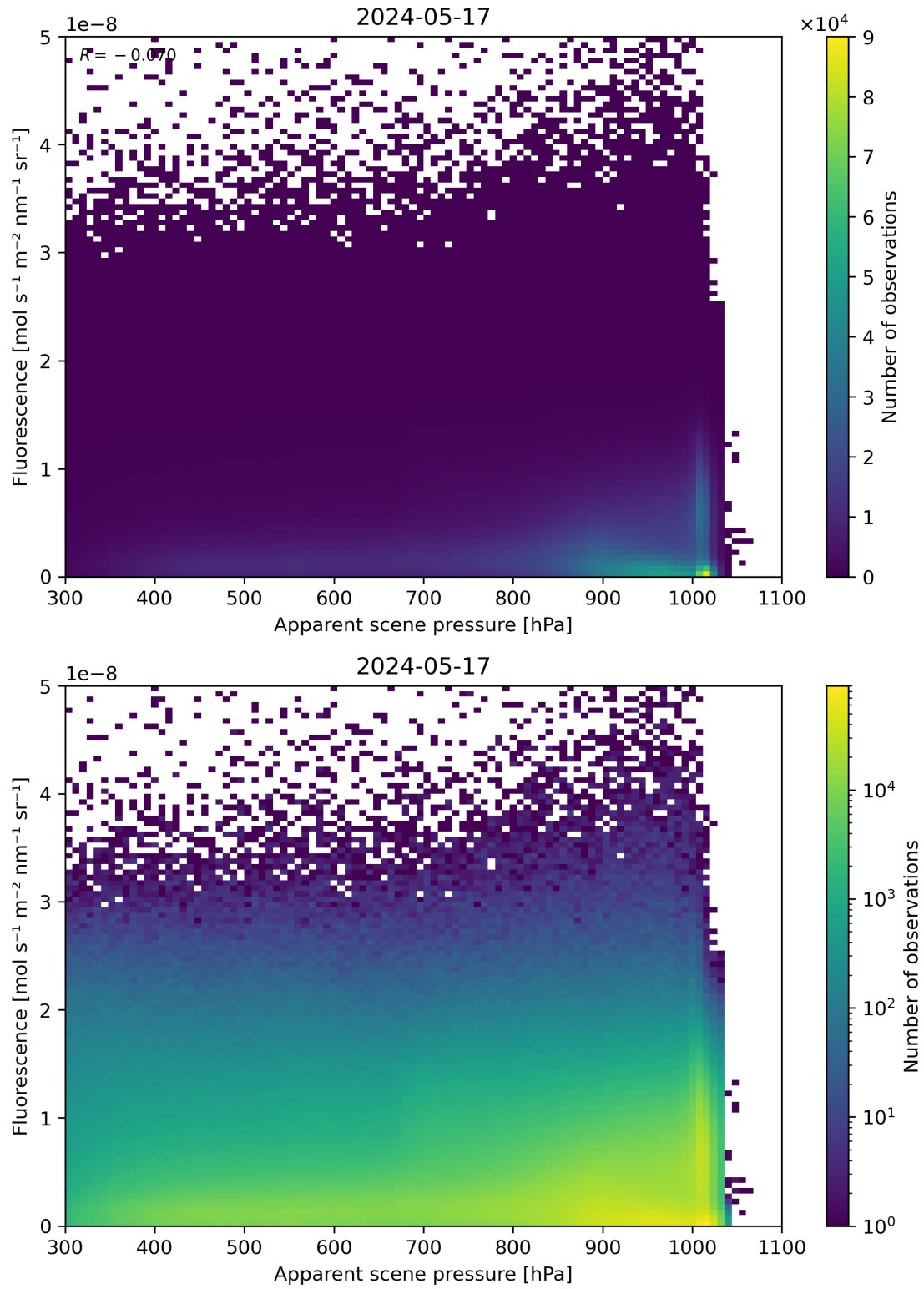
Figure 64: Scatter density plot of “Apparent scene pressure” against “Fluorescence” for 2024-05-16 to 2024-05-18.
