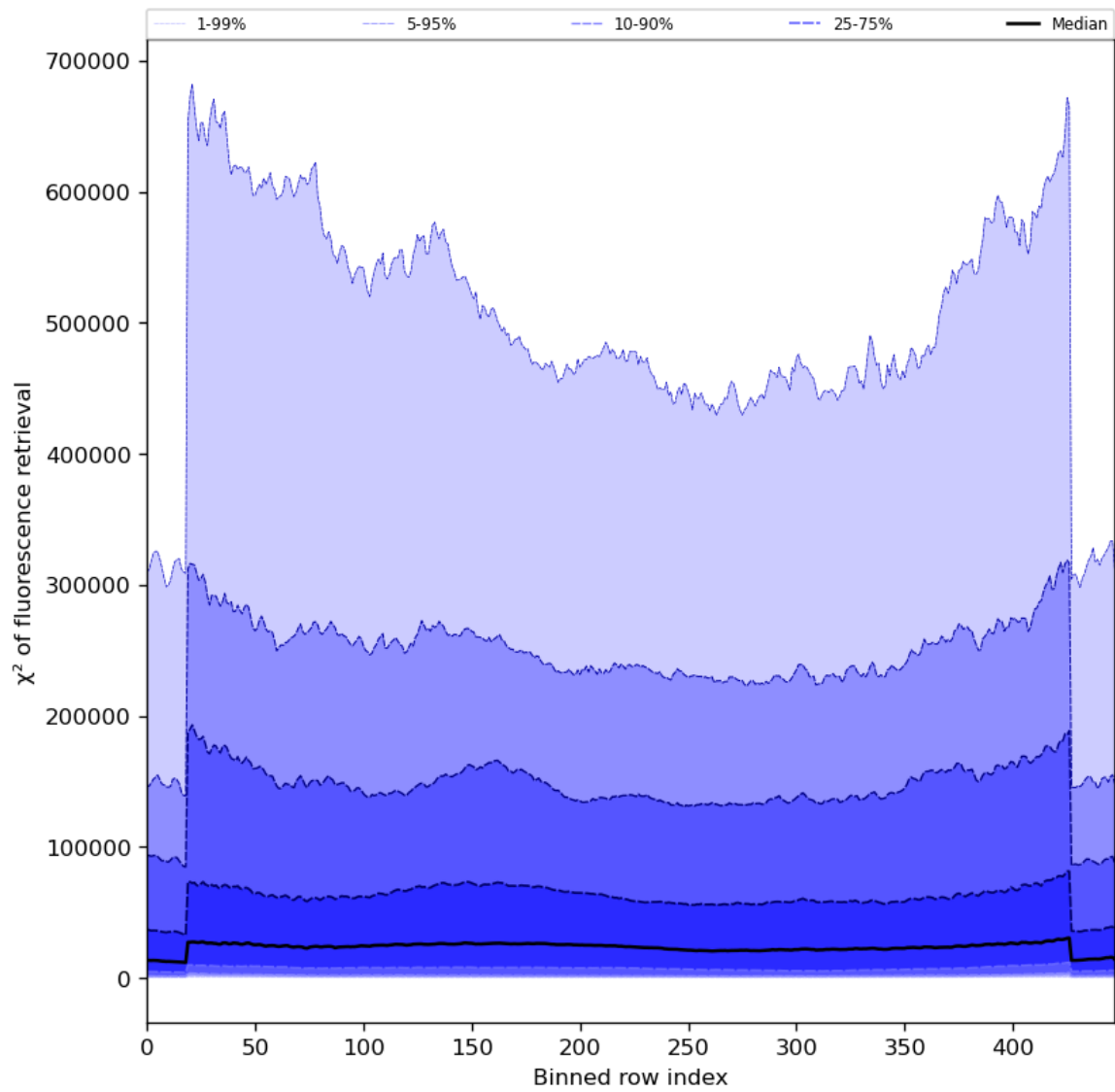
Figure 59: Along track statistics of “ \chi^2 of fluorescence retrieval” for 2024-05-16 to 2024-05-18
