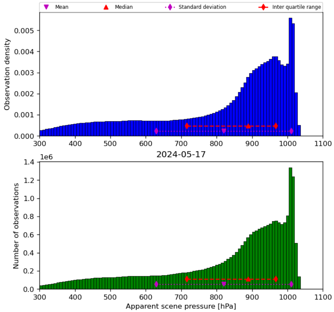
Figure 36: Histogram of “Apparent scene pressure” for 2024-05-16 to 2024-05-18
