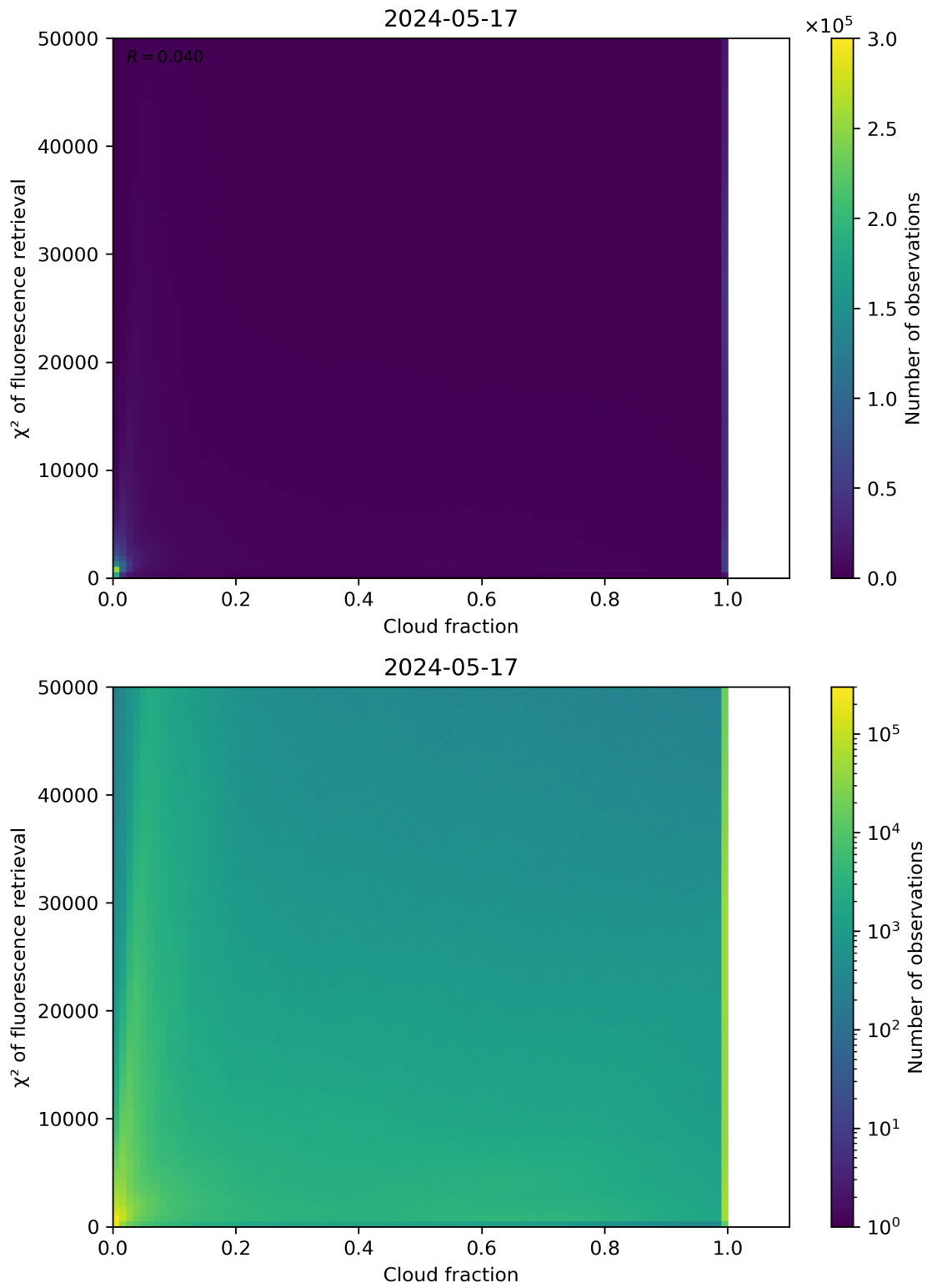
Figure 71: Scatter density plot of “Cloud fraction” against “ \chi^2 of fluorescence retrieval” for 2024-05-16 to 2024-05-18.
