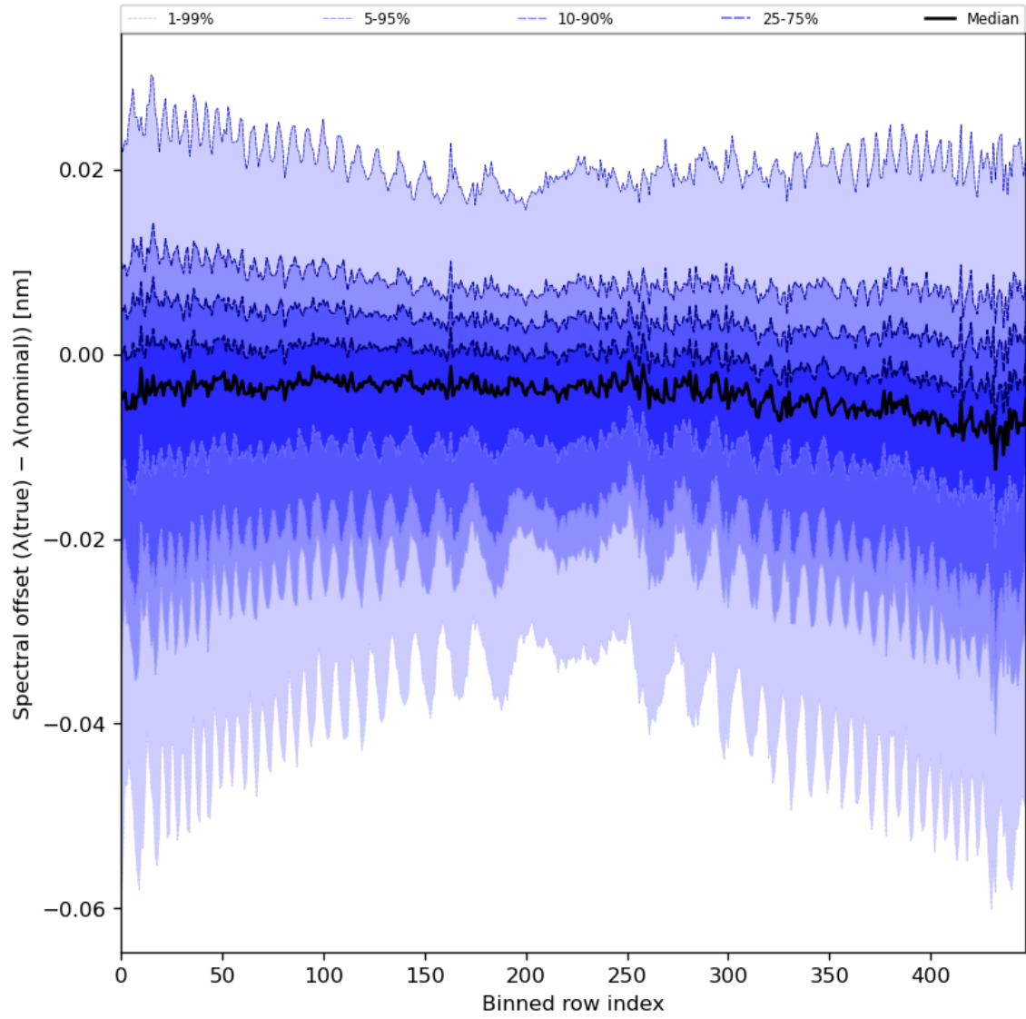
Figure 62: Along track statistics of “Spectral offset ( \lambda(\text{true}) - \lambda(\text{nominal}) )” for 2024-05-16 to 2024-05-18
