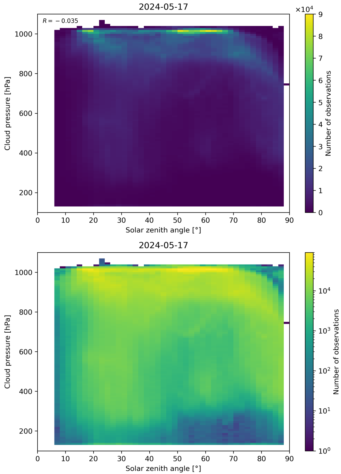
Figure 111: Scatter density plot of “Solar zenith angle” against “Cloud pressure” for 2024-05-16 to 2024-05-18.
