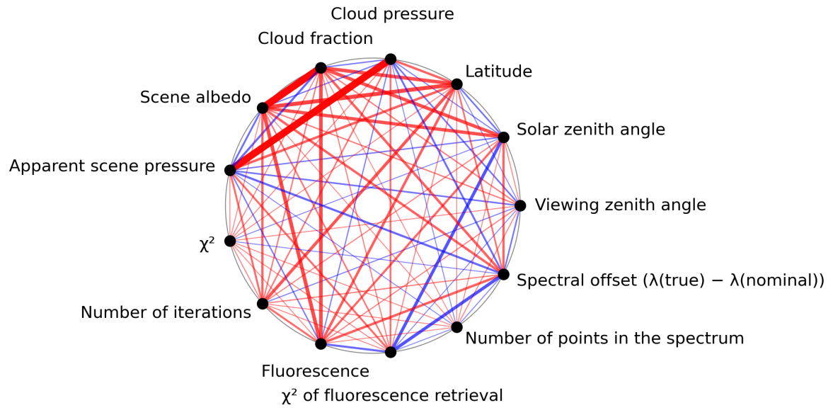
Figure 1: Map of correlation graph for 2024-05-16 to 2024-05-18.
