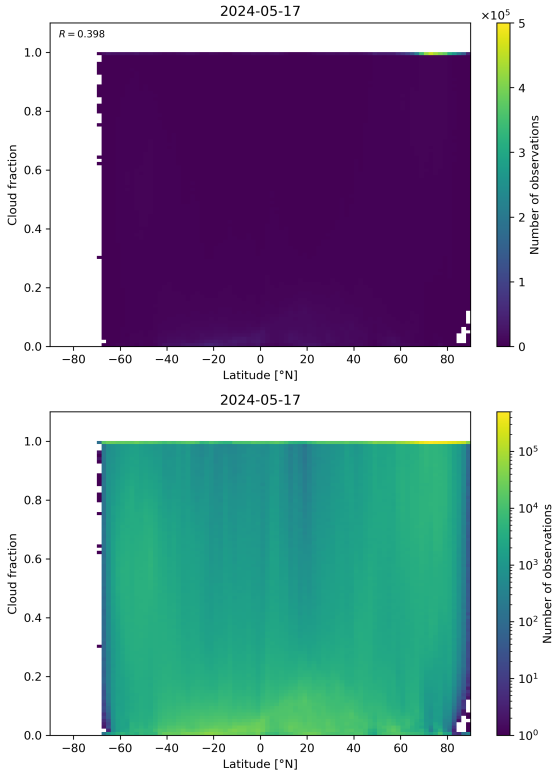
Figure 90: Scatter density plot of “Latitude” against “Cloud fraction” for 2024-05-16 to 2024-05-18.
