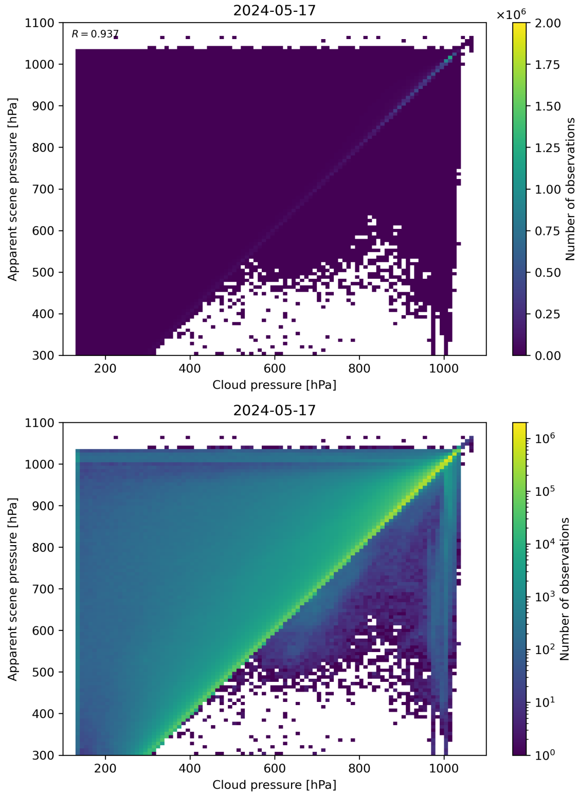
Figure 77: Scatter density plot of “Cloud pressure” against “Apparent scene pressure” for 2024-05-16 to 2024-05-18.
