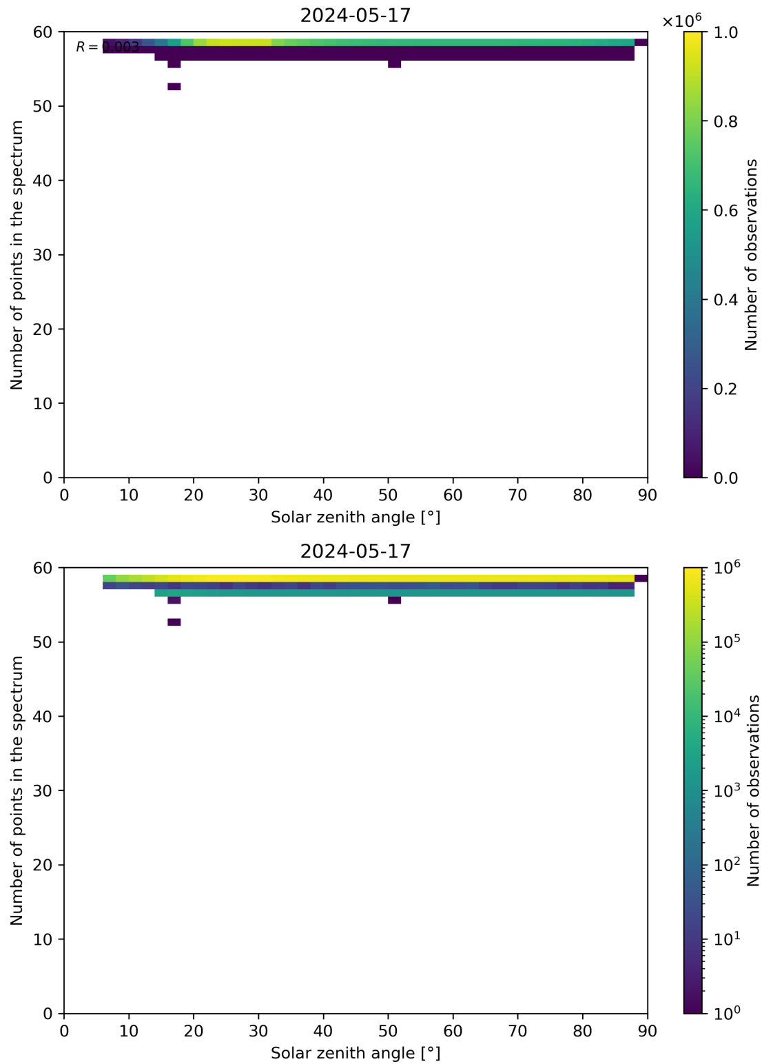
Figure 115: Scatter density plot of “Solar zenith angle” against “Number of points in the spectrum” for 2024-05-16 to 2024-05-18.
