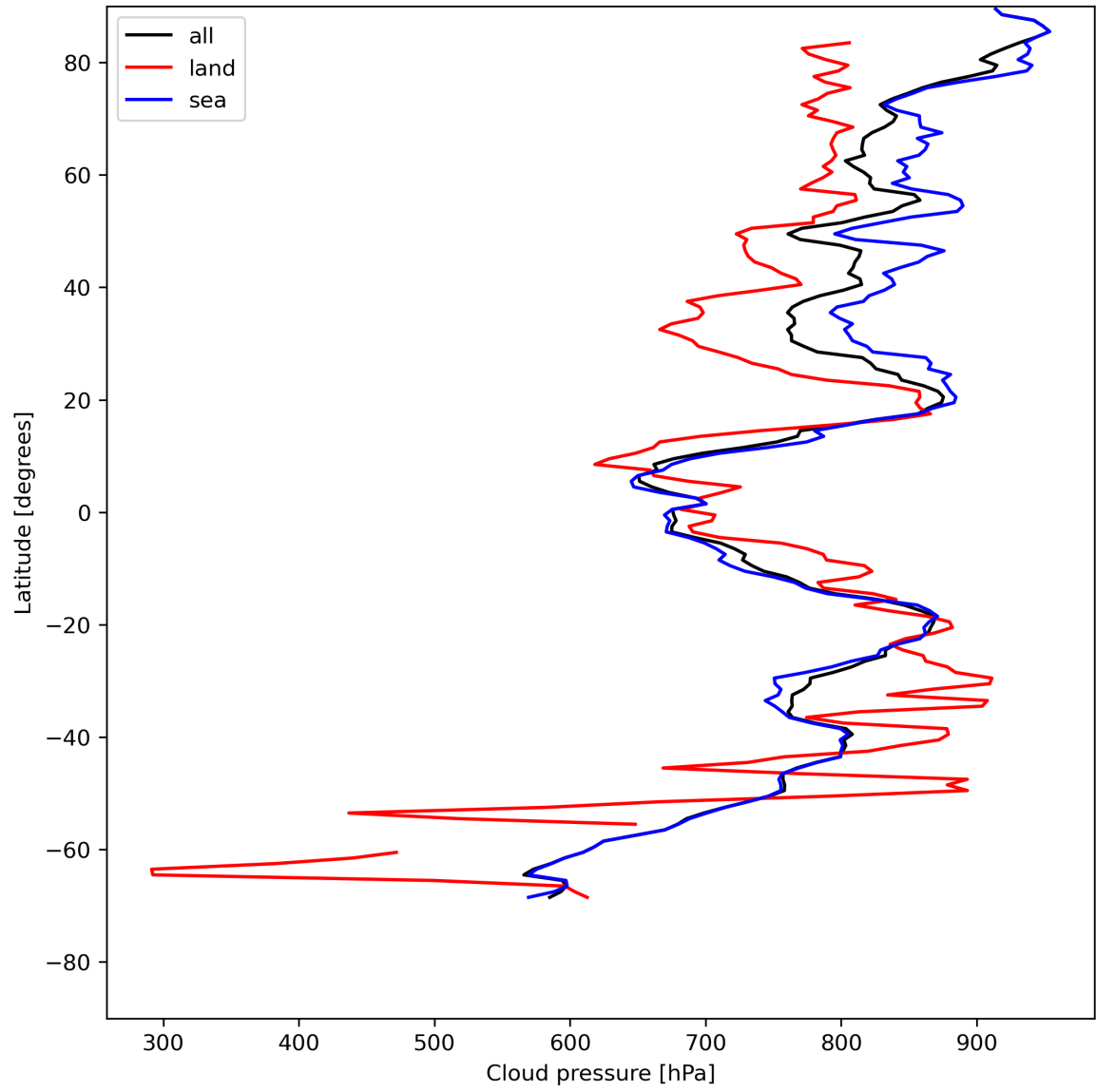
Figure 13: Zonal average of “Cloud pressure” for 2024-05-16 to 2024-05-18.
