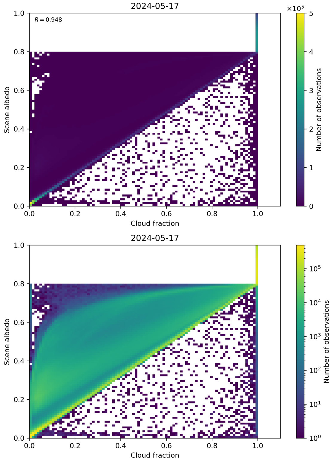
Figure 75: Scatter density plot of “Cloud fraction” against “Scene albedo” for 2024-05-16 to 2024-05-18.
