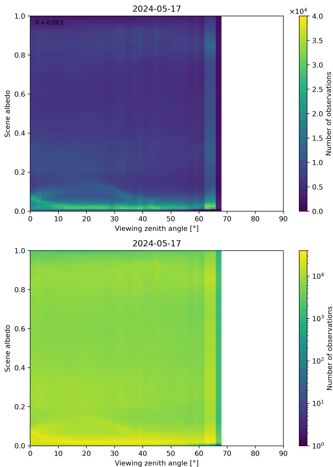
Figure 126: Scatter density plot of “Viewing zenith angle” against “Scene albedo” for 2024-05-16 to 2024-05-18.
