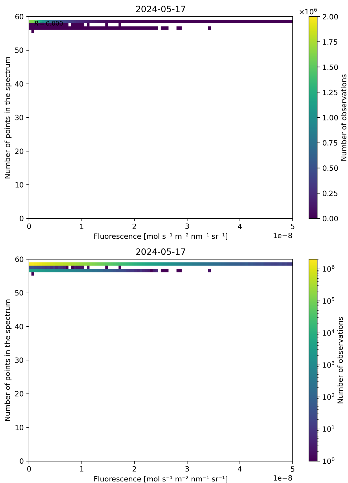
Figure 86: Scatter density plot of “Fluorescence” against “Number of points in the spectrum” for 2024-05-16 to 2024-05-18.
