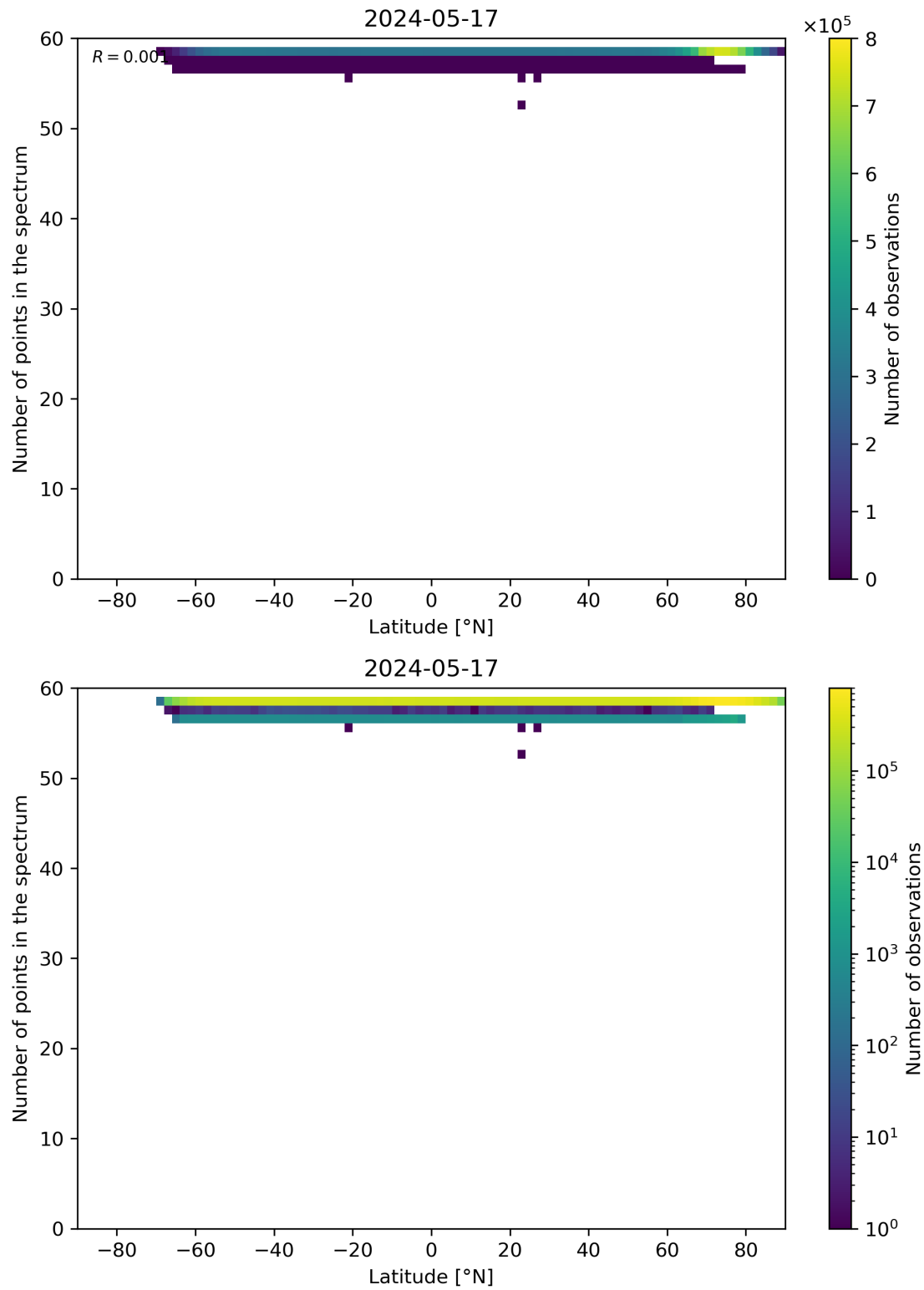
Figure 94: Scatter density plot of “Latitude” against “Number of points in the spectrum” for 2024-05-16 to 2024-05-18.
