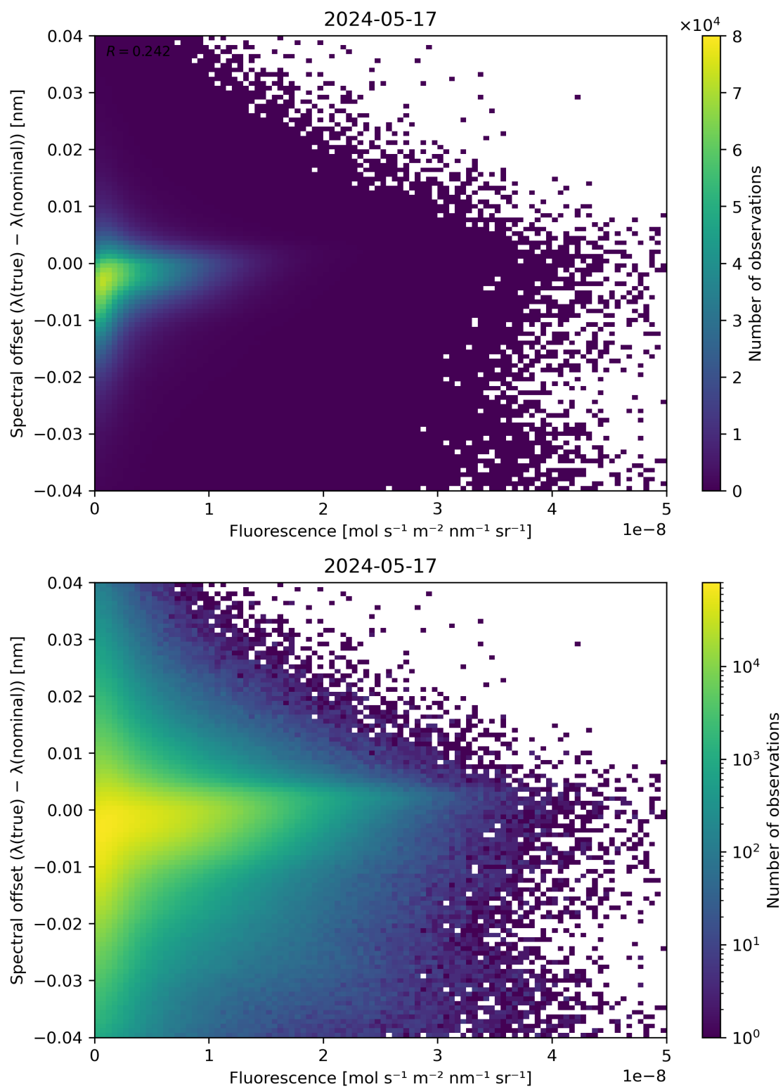
Figure 87: Scatter density plot of “Fluorescence” against “Spectral offset ( \lambda(\text{true}) - \lambda(\text{nominal}) )” for 2024-05-16 to 2024-05-18.
