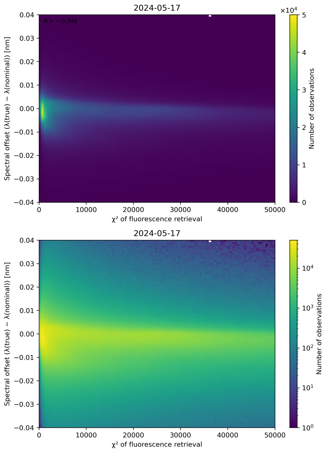
Figure 69: Scatter density plot of “ \chi^2 of fluorescence retrieval” against “Spectral offset ( \lambda(\text{true}) - \lambda(\text{nominal}) )” for 2024-05-16 to 2024-05-18.
