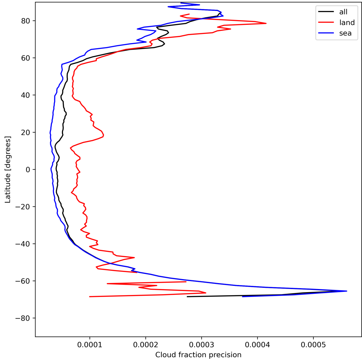
Figure 16: Zonal average of “Cloud fraction precision” for 2024-05-16 to 2024-05-18.
