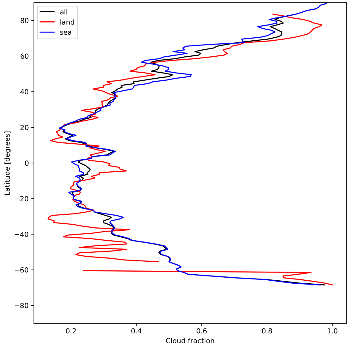
Figure 15: Zonal average of “Cloud fraction” for 2024-05-16 to 2024-05-18.
