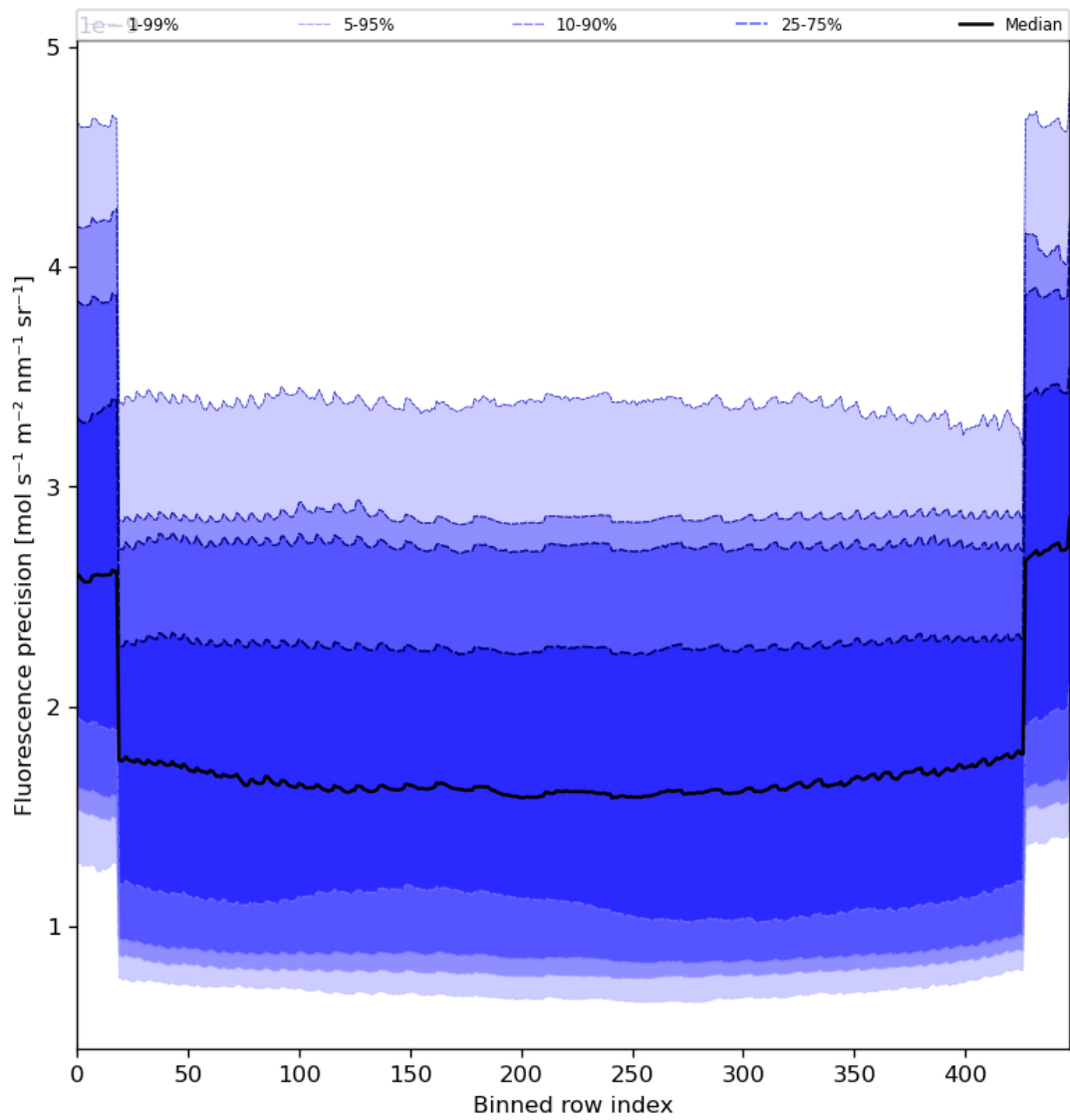
Figure 58: Along track statistics of “Fluorescence precision” for 2024-05-16 to 2024-05-18
