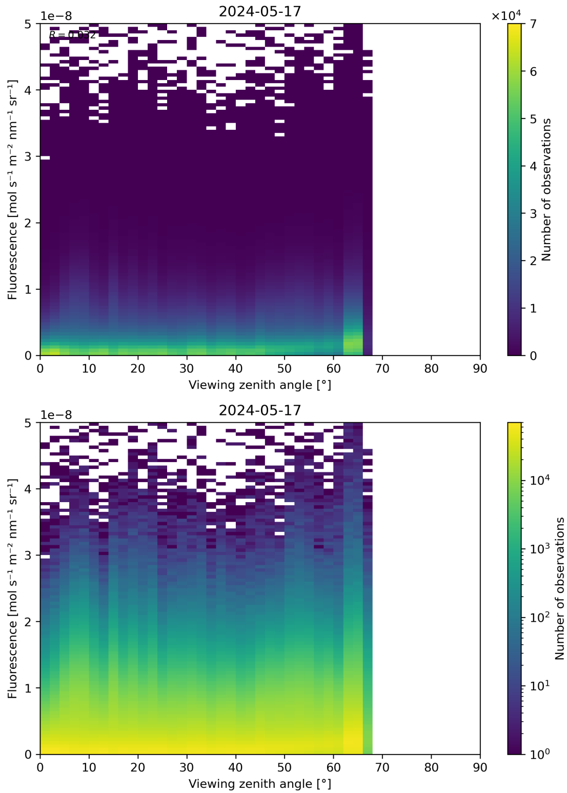
Figure 122: Scatter density plot of “Viewing zenith angle” against “Fluorescence” for 2024-05-16 to 2024-05-18.
