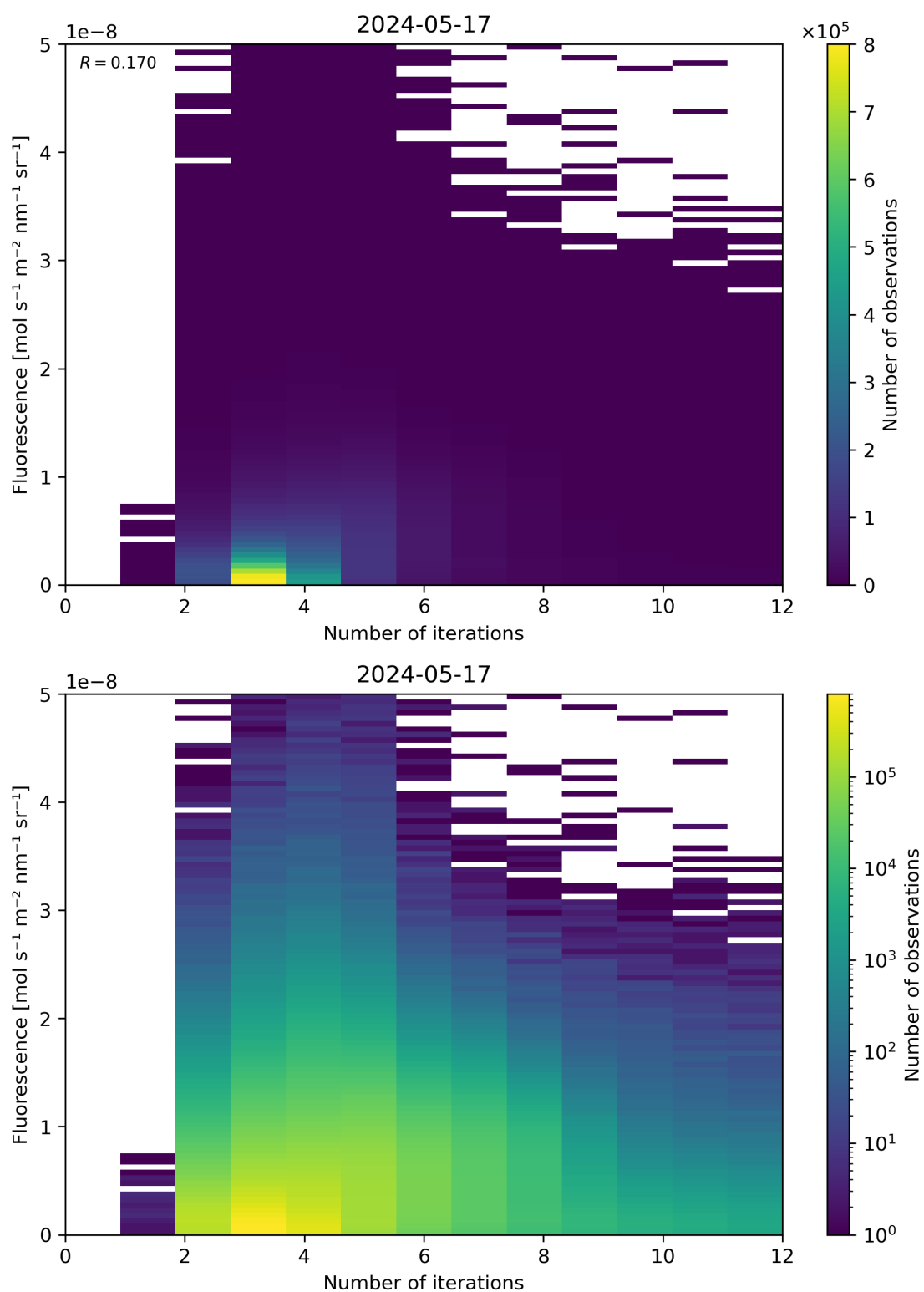
Figure 98: Scatter density plot of “Number of iterations” against “Fluorescence” for 2024-05-16 to 2024-05-18.
