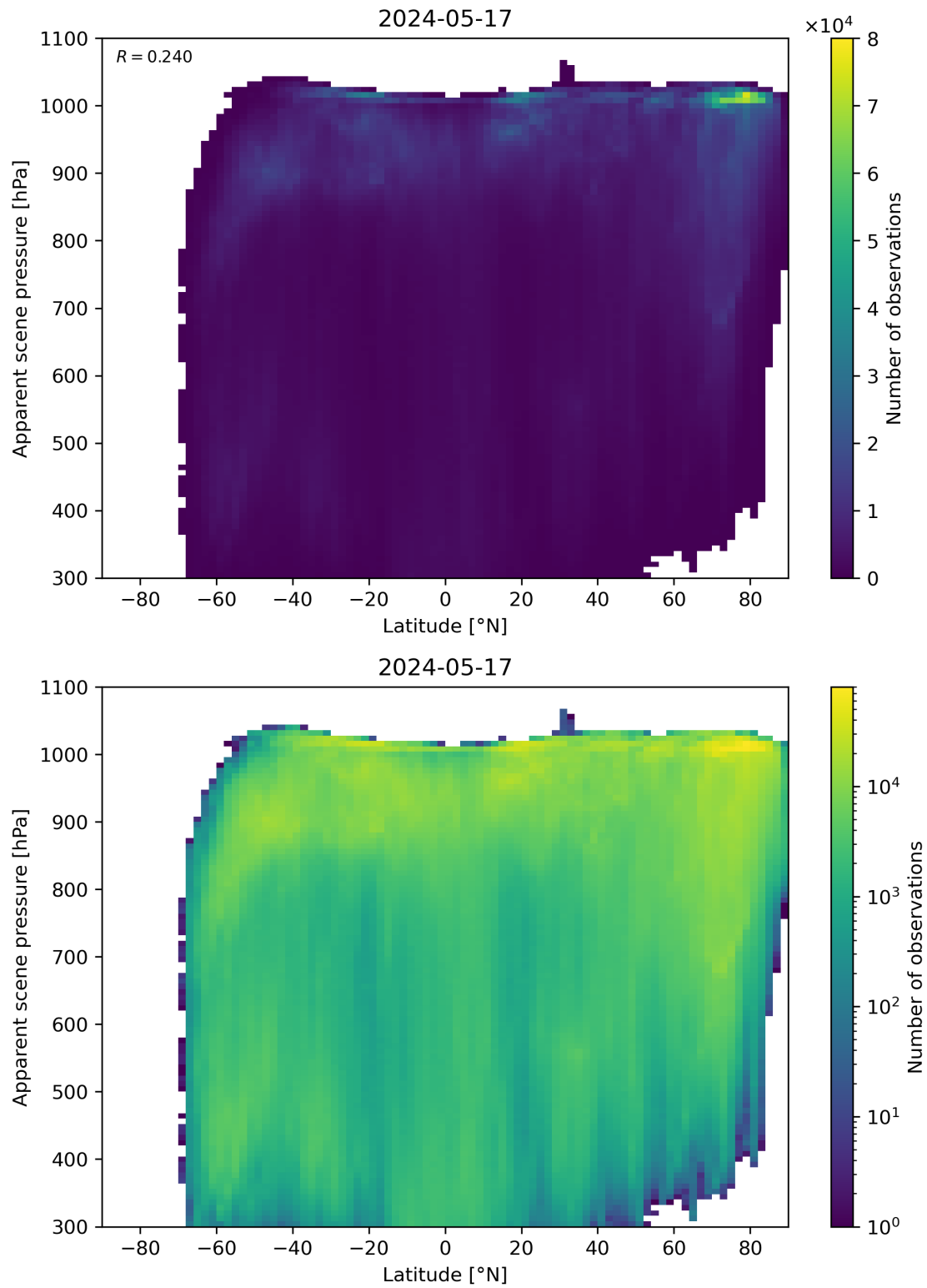
Figure 88: Scatter density plot of “Latitude” against “Apparent scene pressure” for 2024-05-16 to 2024-05-18.
