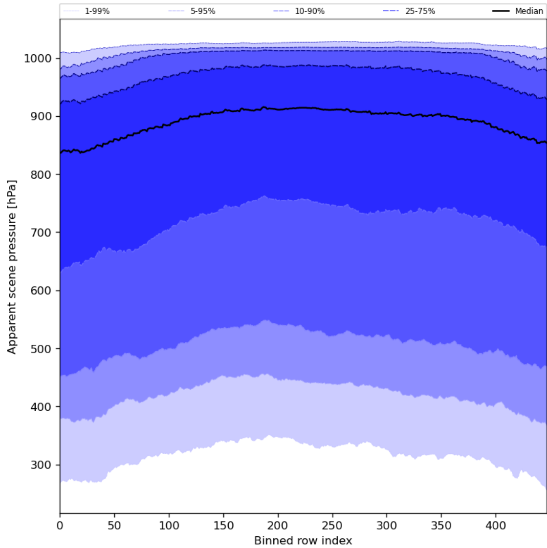
Figure 53: Along track statistics of “Apparent scene pressure” for 2024-05-16 to 2024-05-18
