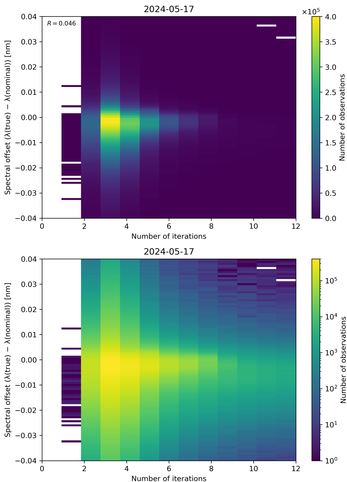
Figure 100: Scatter density plot of “Number of iterations” against “Spectral offset ( \lambda(\text{true}) - \lambda(\text{nominal}) )” for 2024-05-16 to 2024-05-18.
