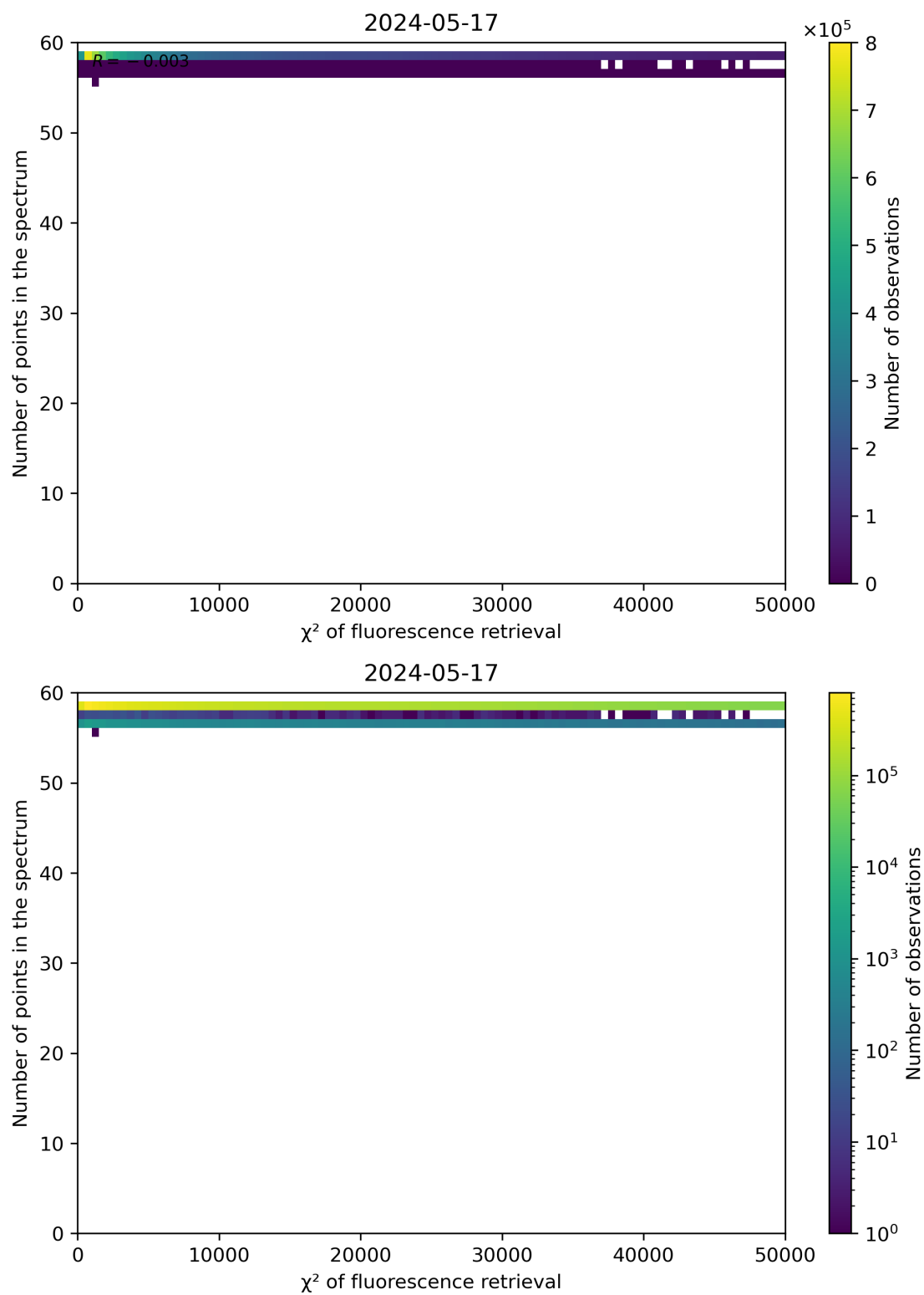
Figure 68: Scatter density plot of " \chi^2 of fluorescence retrieval" against "Number of points in the spectrum" for 2024-05-16 to 2024-05-18.
