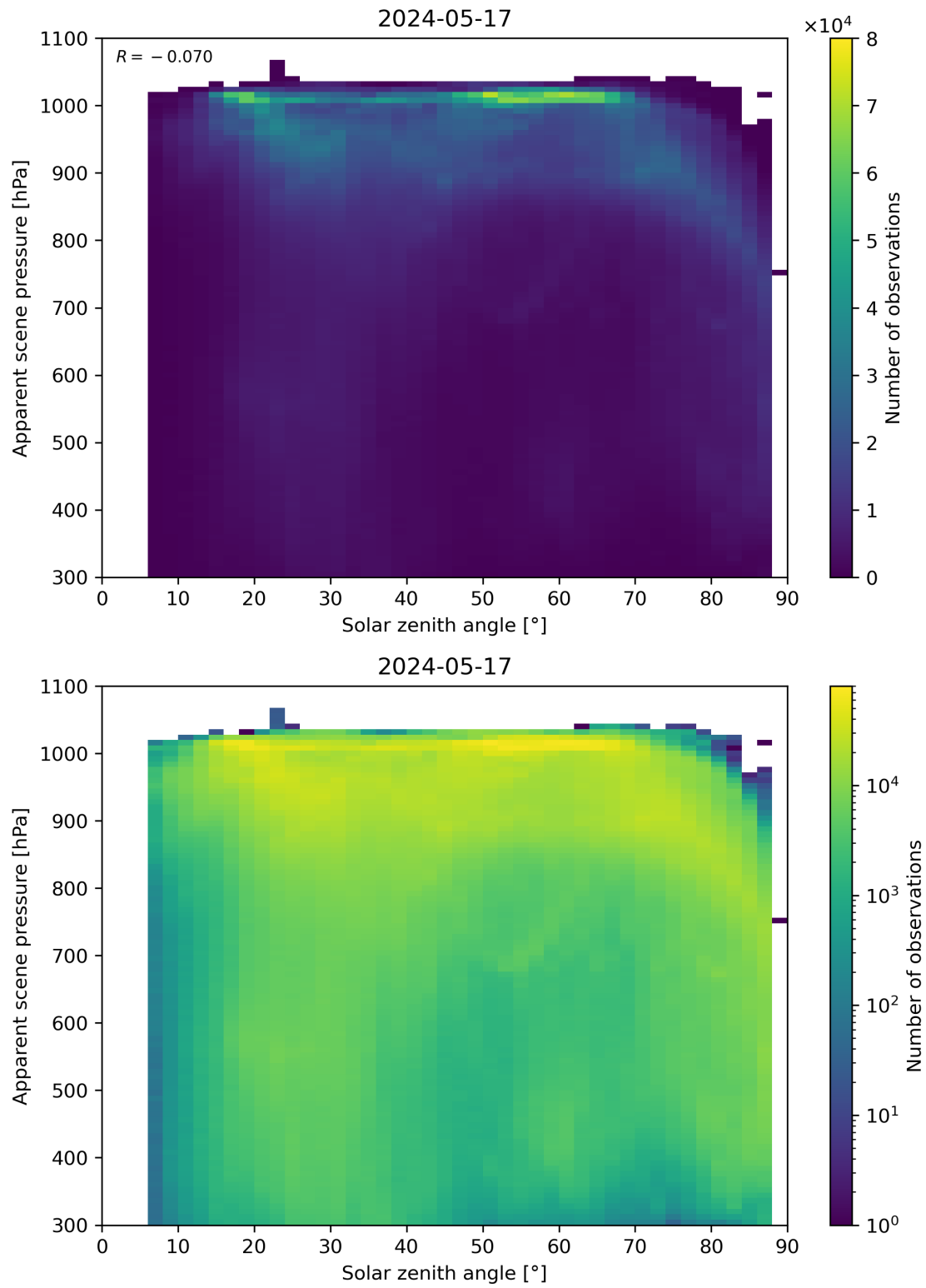
Figure 108: Scatter density plot of “Solar zenith angle” against “Apparent scene pressure” for 2024-05-16 to 2024-05-18.
