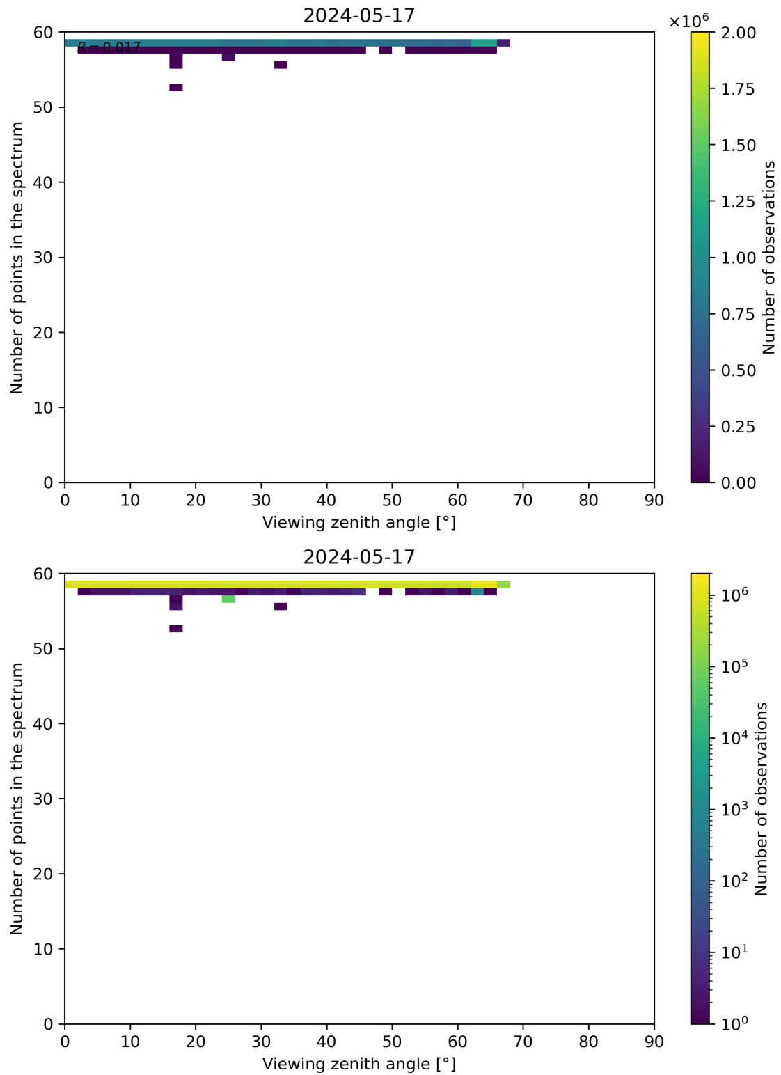
Figure 125: Scatter density plot of “Viewing zenith angle” against “Number of points in the spectrum” for 2024-05-16 to 2024-05-18.
