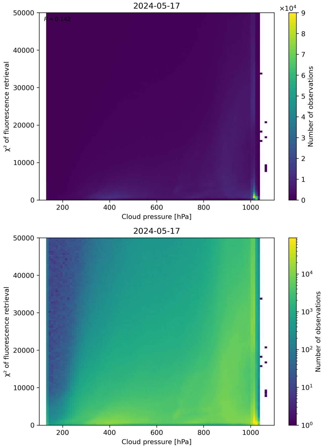
Figure 78: Scatter density plot of “Cloud pressure” against “ \chi^2 of fluorescence retrieval” for 2024-05-16 to 2024-05-18.
