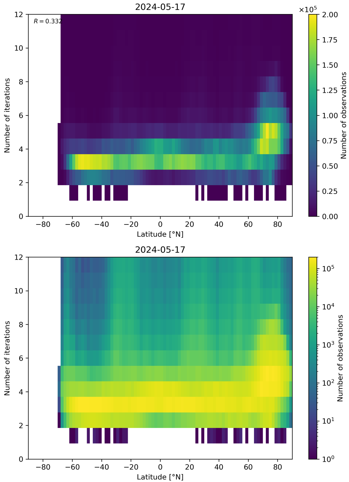
Figure 93: Scatter density plot of “Latitude” against “Number of iterations” for 2024-05-16 to 2024-05-18.
