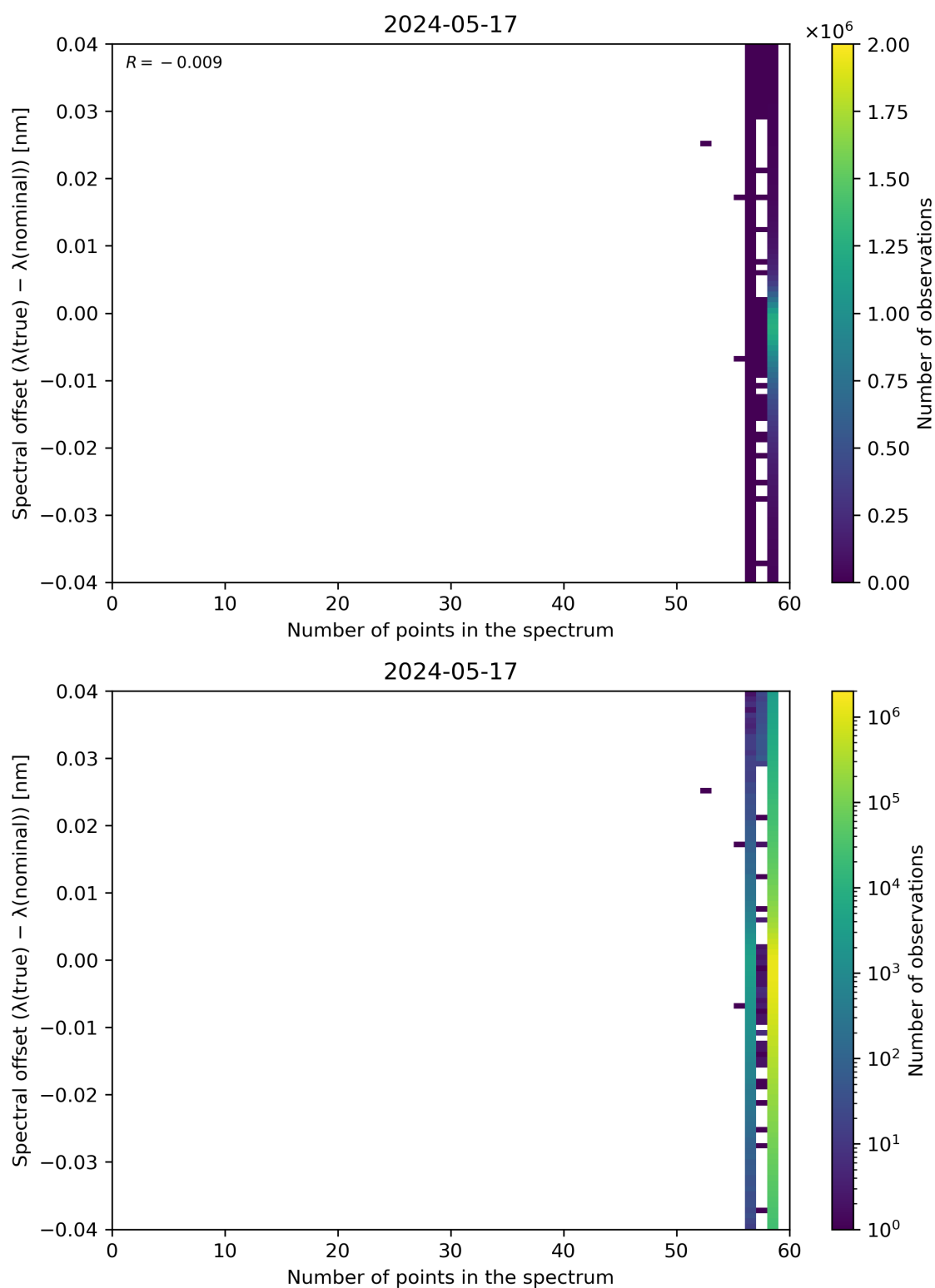
Figure 101: Scatter density plot of “Number of points in the spectrum” against “Spectral offset ( \lambda(\text{true}) - \lambda(\text{nominal}) )” for 2024-05-16 to 2024-05-18.
