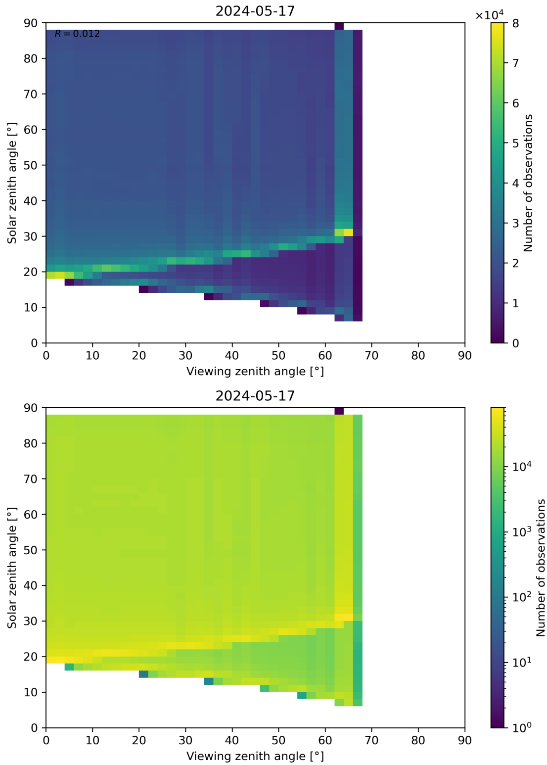
Figure 127: Scatter density plot of “Viewing zenith angle” against “Solar zenith angle” for 2024-05-16 to 2024-05-18.
