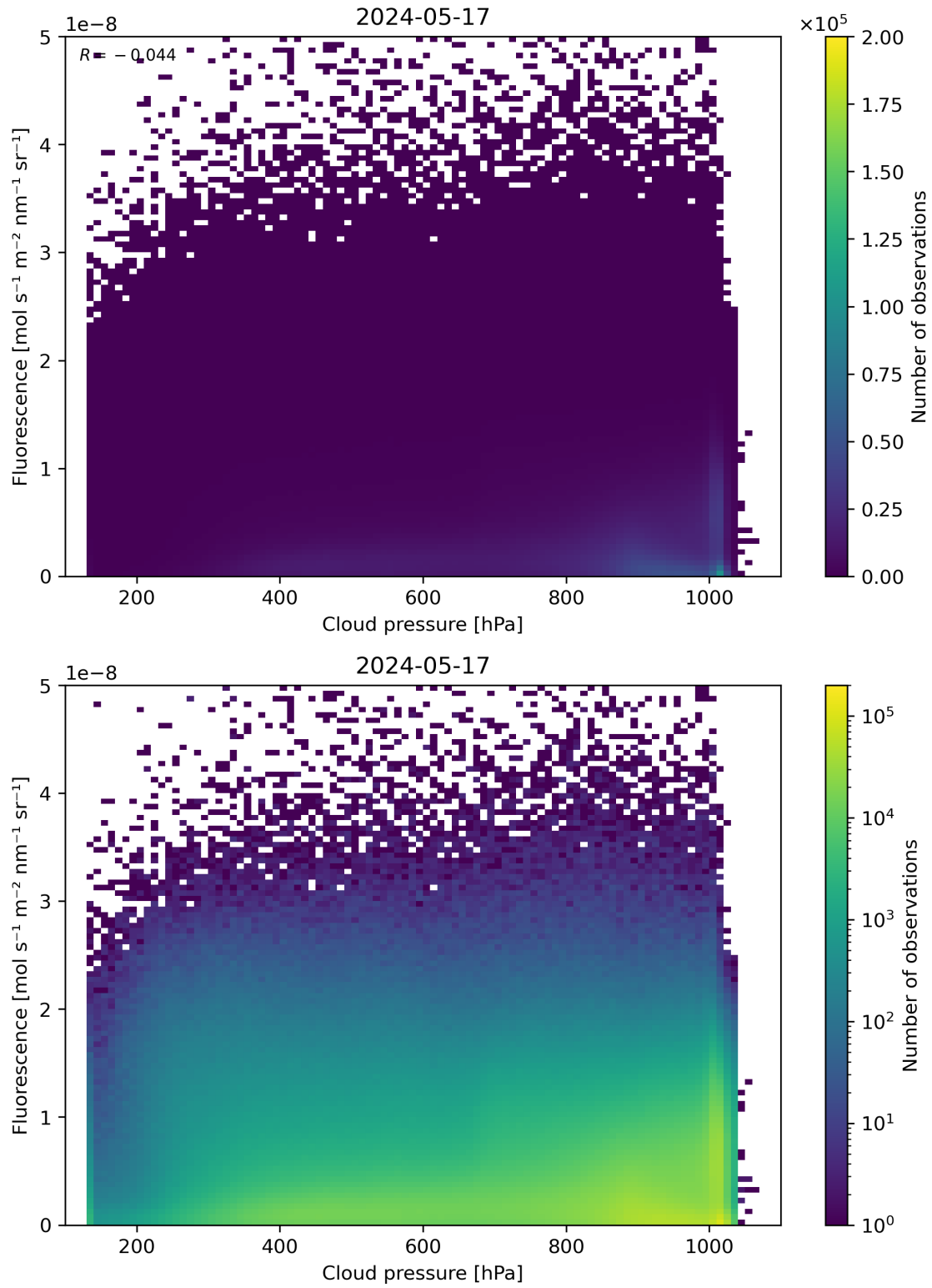
Figure 80: Scatter density plot of “Cloud pressure” against “Fluorescence” for 2024-05-16 to 2024-05-18.
