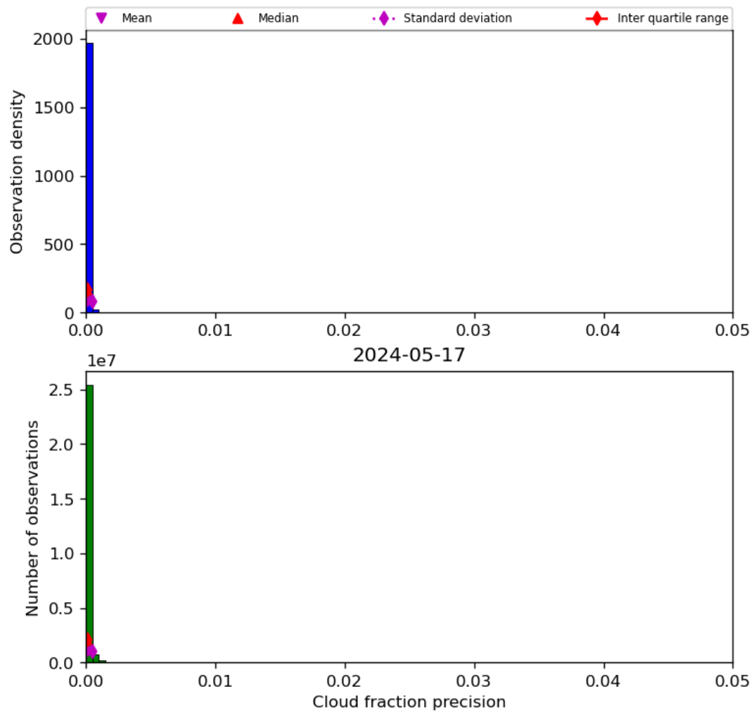
Figure 33: Histogram of “Cloud fraction precision” for 2024-05-16 to 2024-05-18
