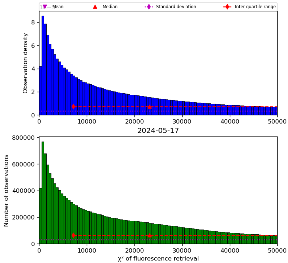
Figure 42: Histogram of “ \chi^2 of fluorescence retrieval” for 2024-05-16 to 2024-05-18
