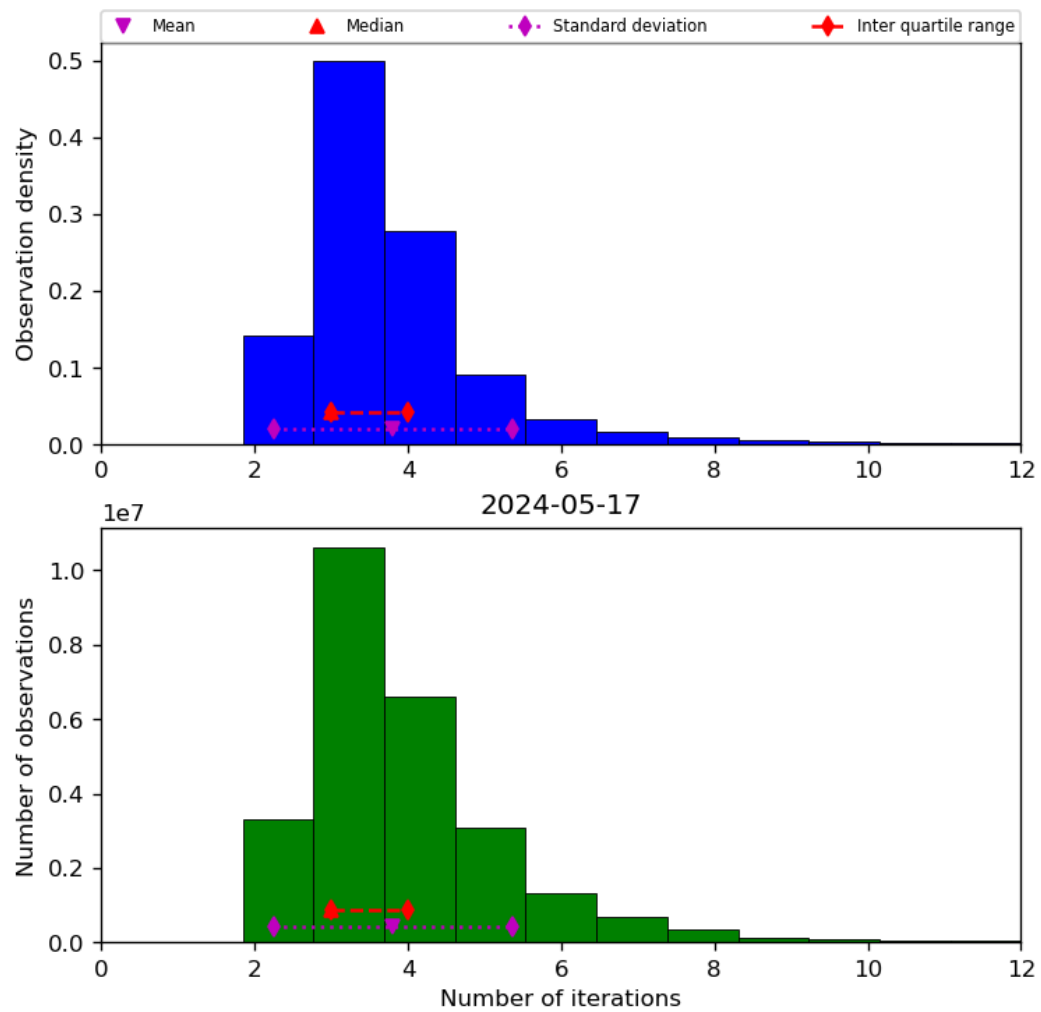
Figure 39: Histogram of “Number of iterations” for 2024-05-16 to 2024-05-18
