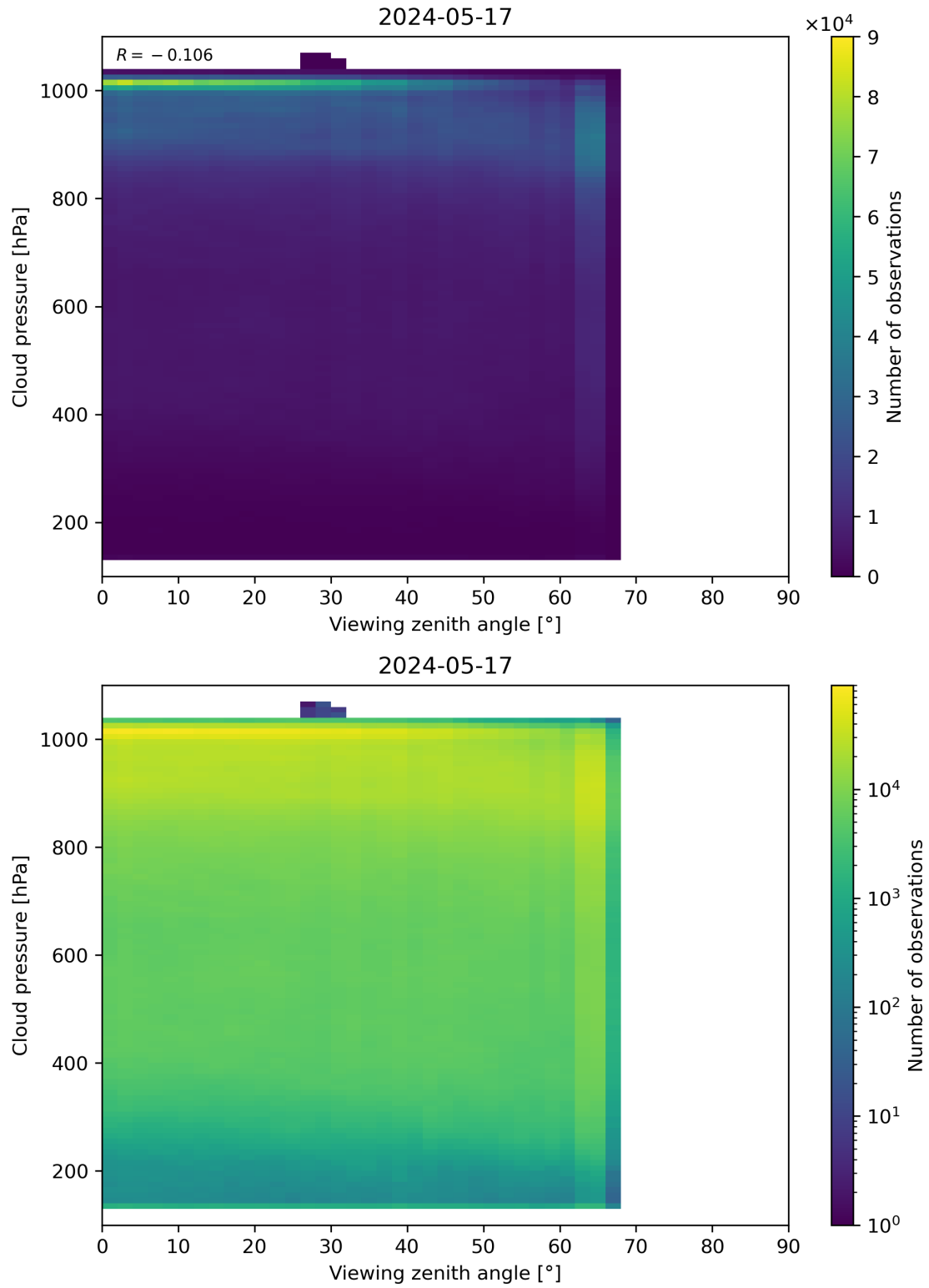
Figure 121: Scatter density plot of “Viewing zenith angle” against “Cloud pressure” for 2024-05-16 to 2024-05-18.
