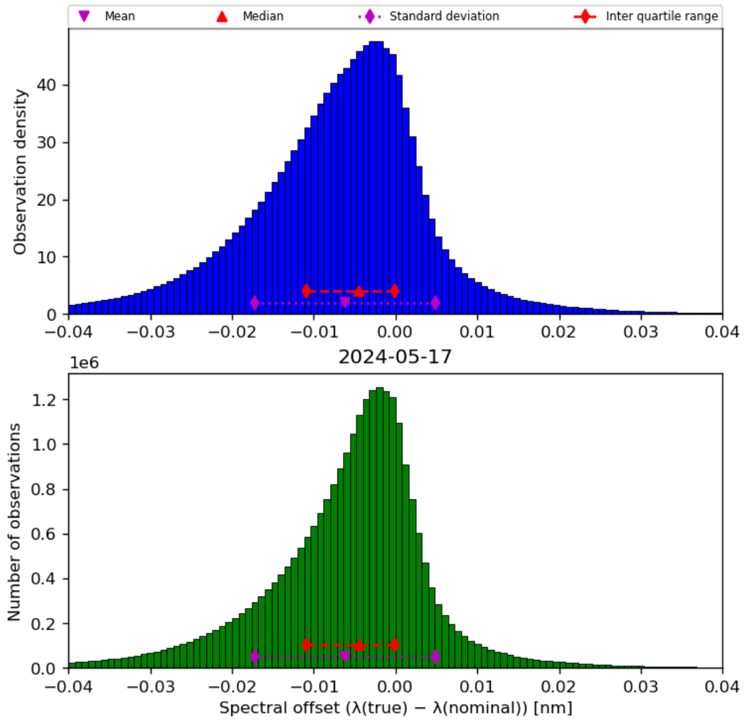
Figure 45: Histogram of “Spectral offset ( \lambda(\text{true}) - \lambda(\text{nominal}) )” for 2024-05-16 to 2024-05-18
