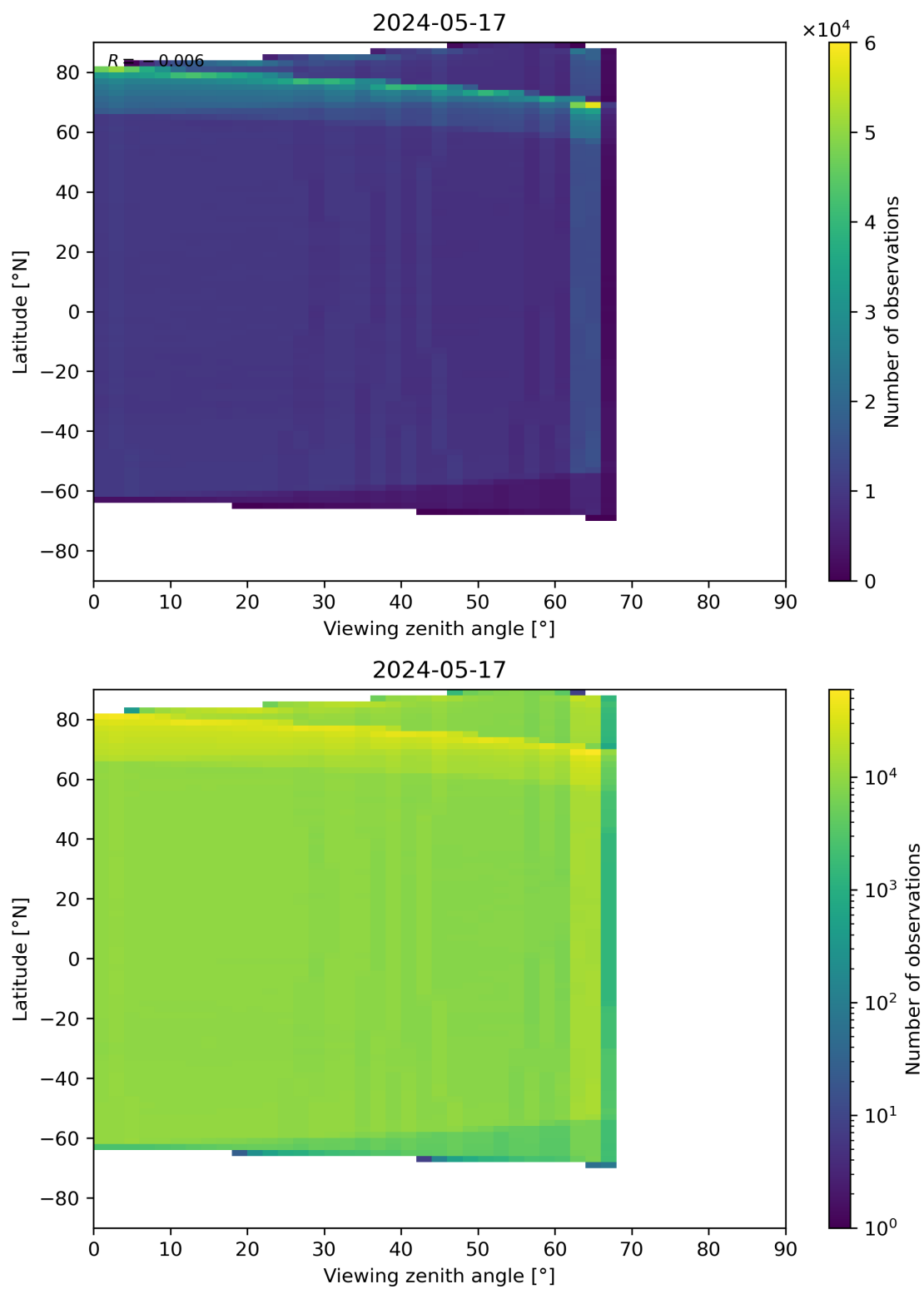
Figure 123: Scatter density plot of “Viewing zenith angle” against “Latitude” for 2024-05-16 to 2024-05-18.
