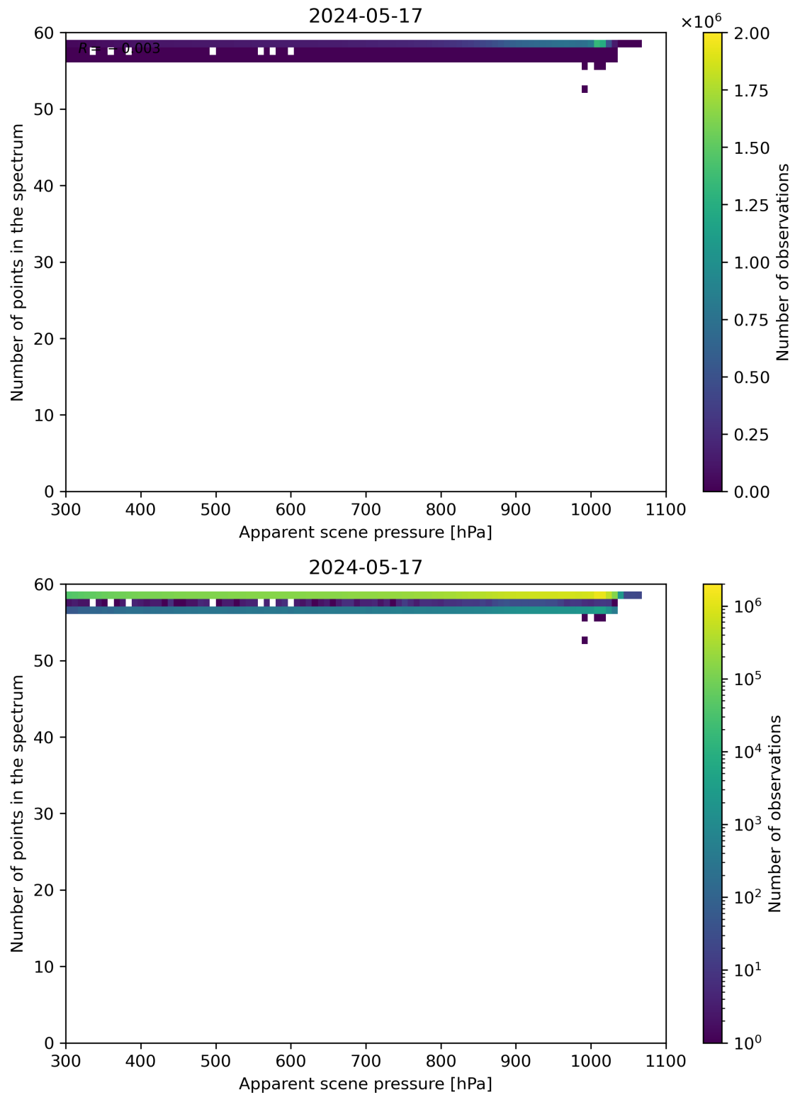
Figure 66: Scatter density plot of “Apparent scene pressure” against “Number of points in the spectrum” for 2024-05-16 to 2024-05-18.
