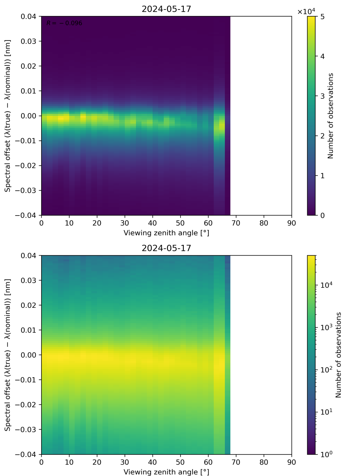
Figure 128: Scatter density plot of “Viewing zenith angle” against “Spectral offset ( \lambda(\text{true}) - \lambda(\text{nominal}) )” for 2024-05-16 to 2024-05-18.
