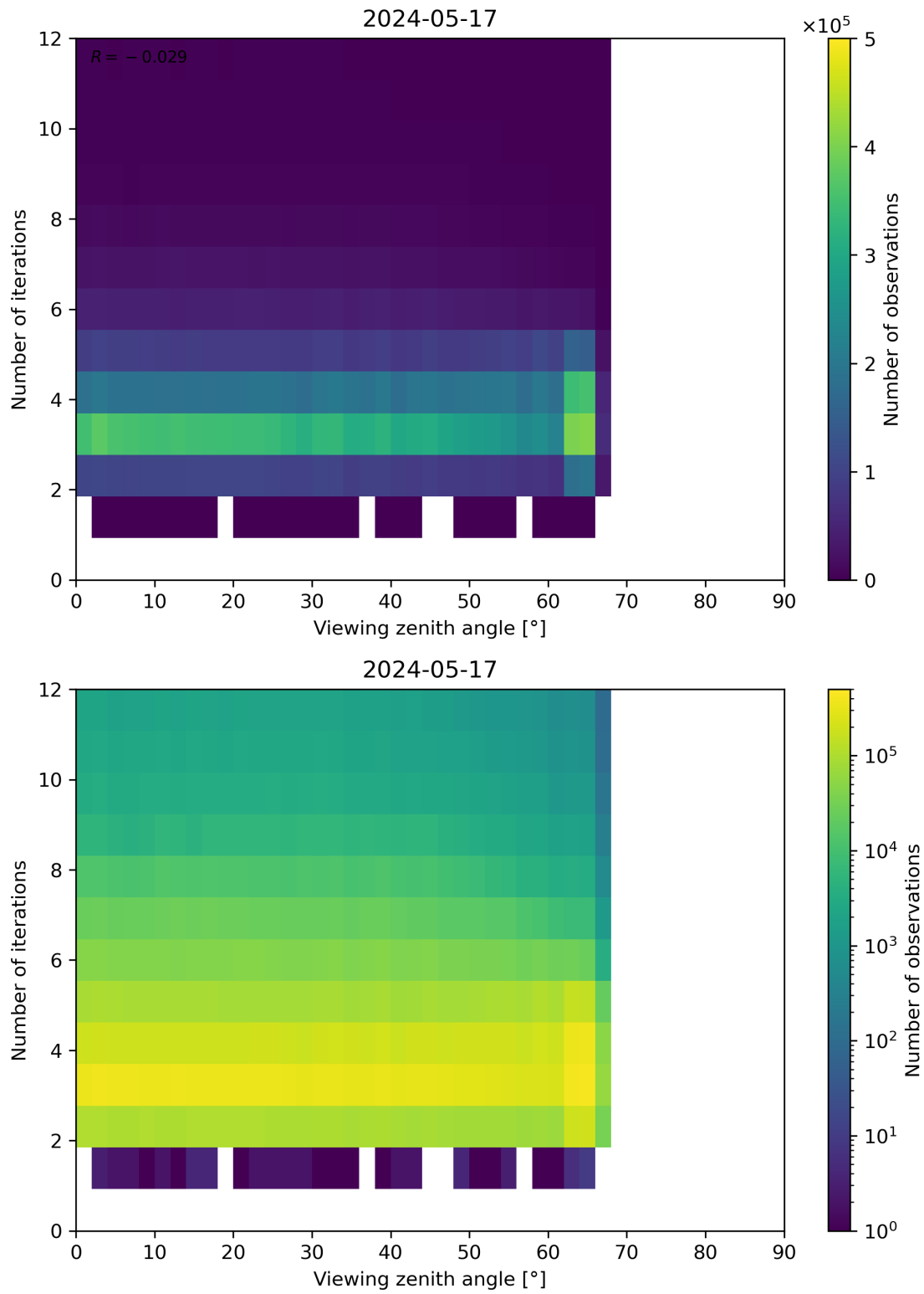
Figure 124: Scatter density plot of “Viewing zenith angle” against “Number of iterations” for 2024-05-16 to 2024-05-18.
