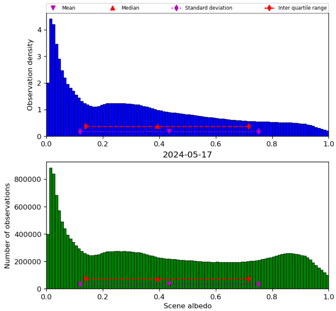
Figure 34: Histogram of “Scene albedo” for 2024-05-16 to 2024-05-18
