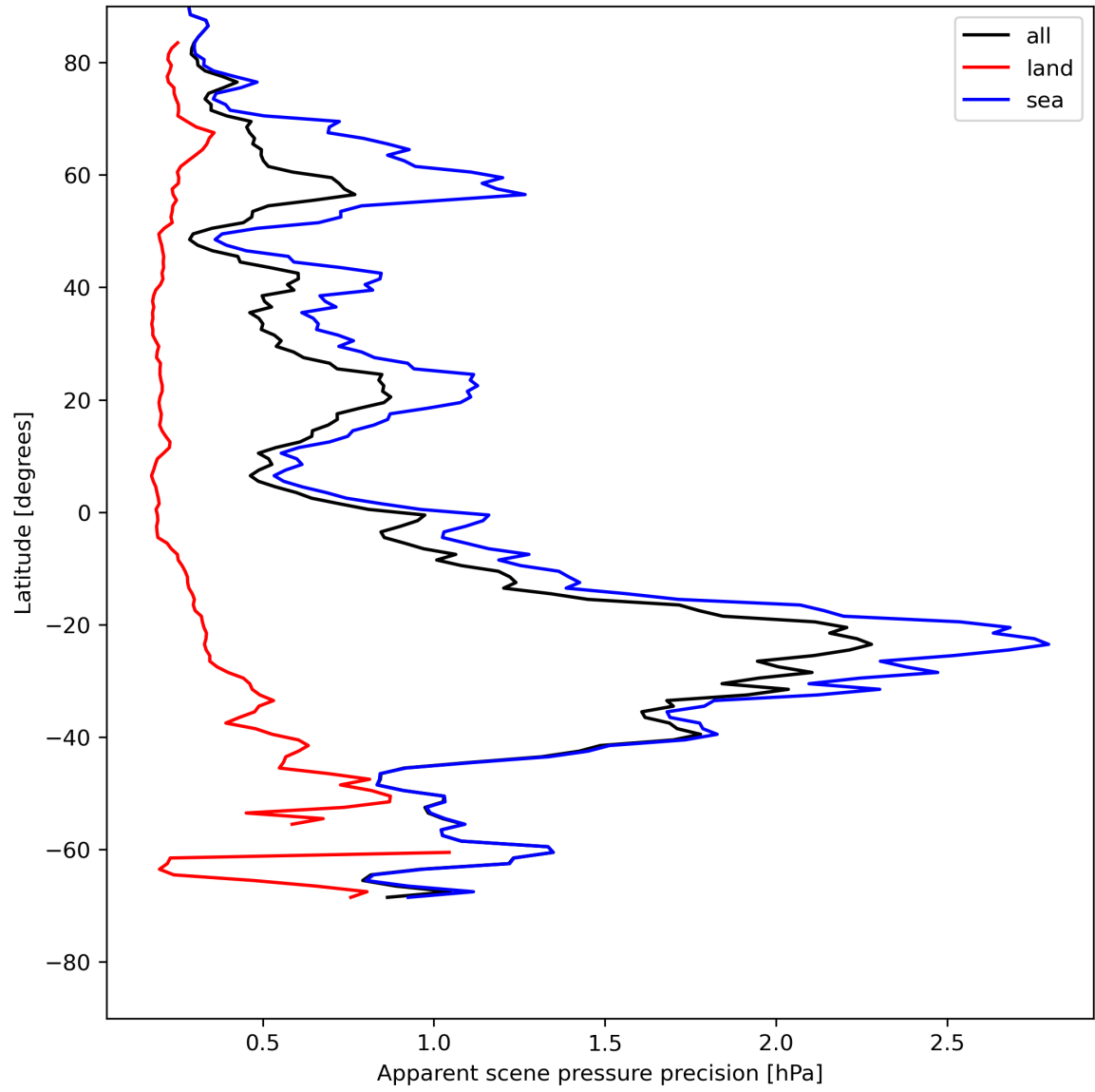
Figure 20: Zonal average of “Apparent scene pressure precision” for 2024-05-16 to 2024-05-18.
