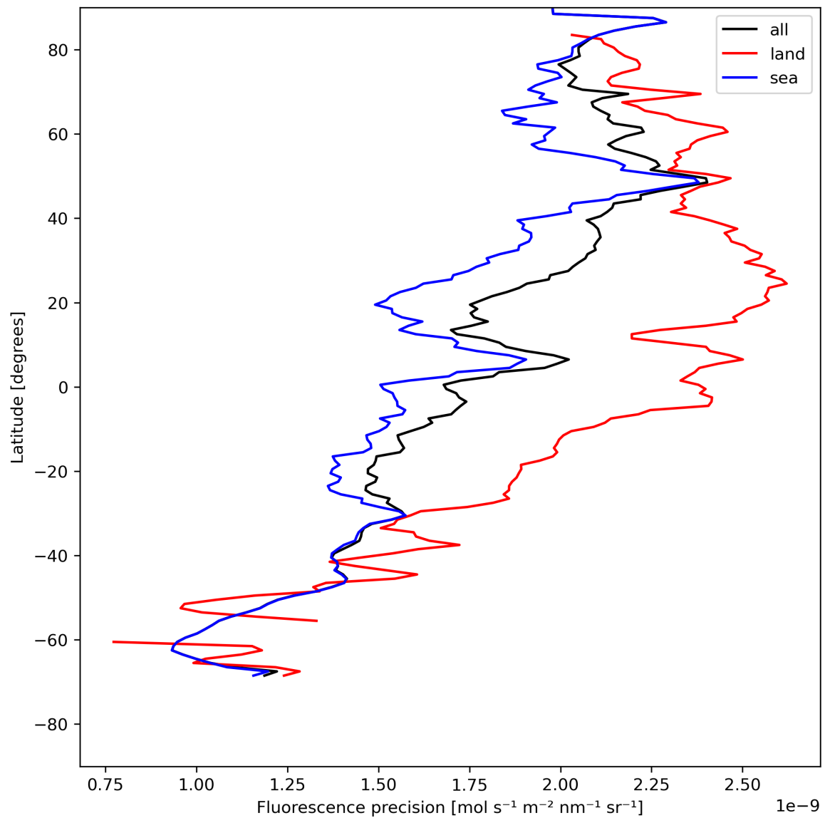
Figure 24: Zonal average of “Fluorescence precision” for 2024-05-16 to 2024-05-18.
