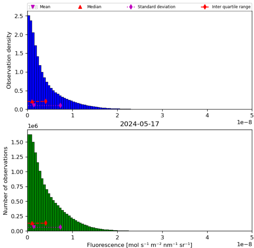
Figure 40: Histogram of “Fluorescence” for 2024-05-16 to 2024-05-18
