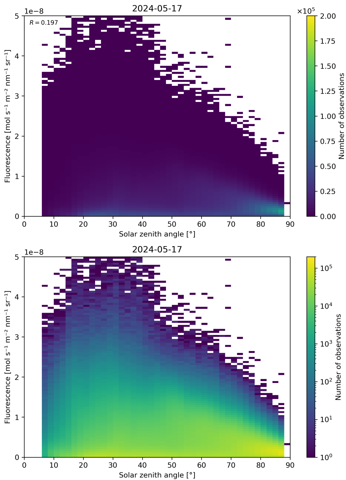
Figure 112: Scatter density plot of “Solar zenith angle” against “Fluorescence” for 2024-05-16 to 2024-05-18.
