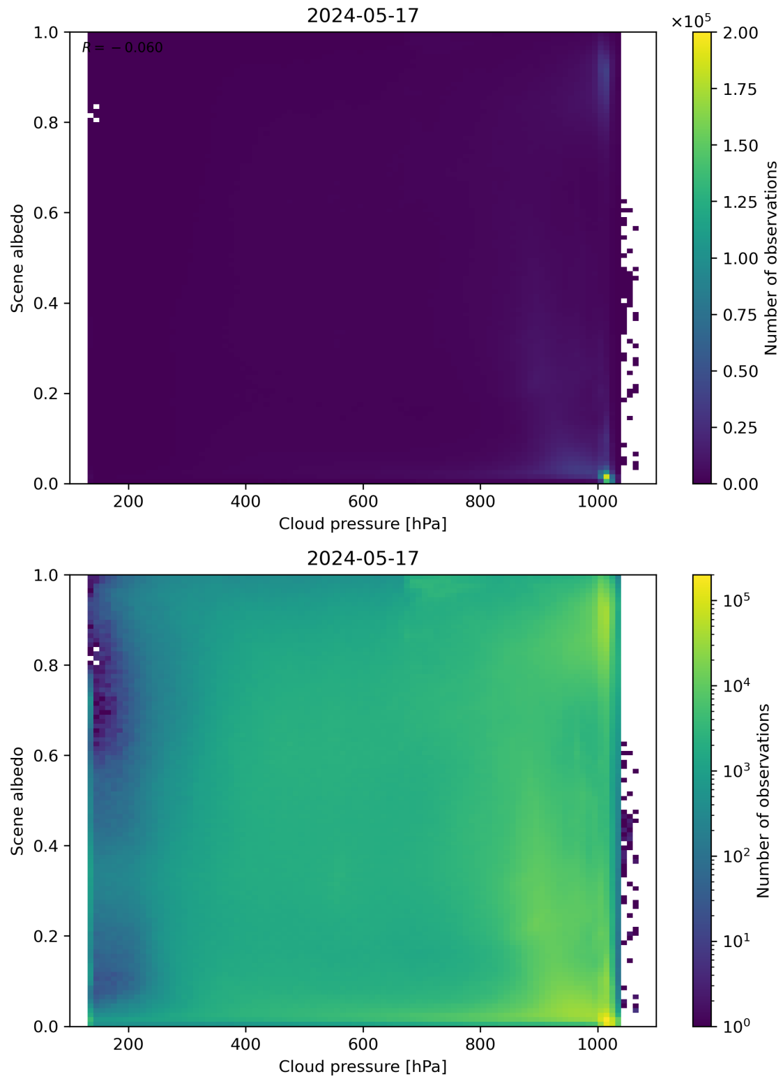
Figure 83: Scatter density plot of “Cloud pressure” against “Scene albedo” for 2024-05-16 to 2024-05-18.
