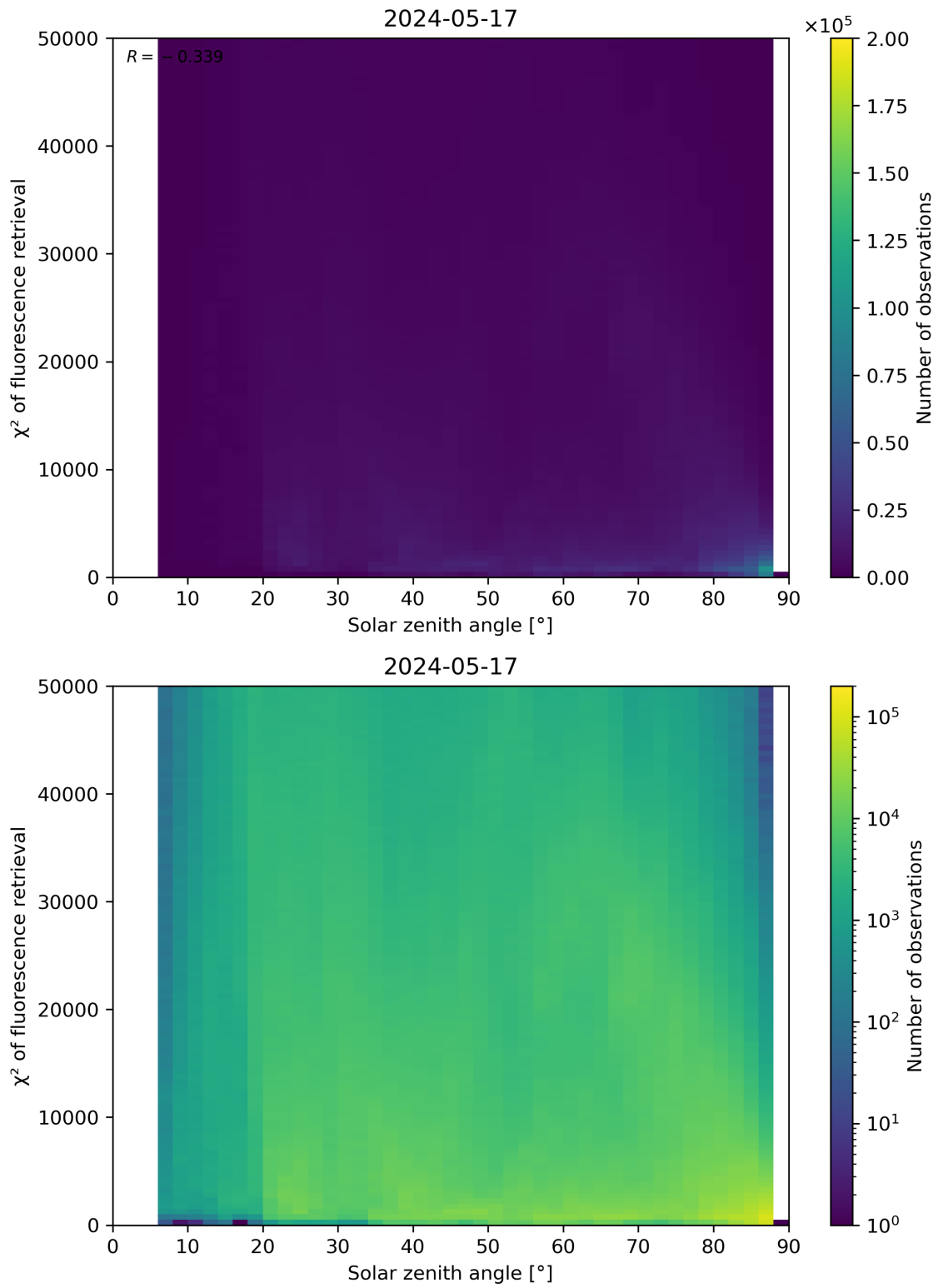
Figure 109: Scatter density plot of “Solar zenith angle” against “ \chi^2 of fluorescence retrieval” for 2024-05-16 to 2024-05-18.
