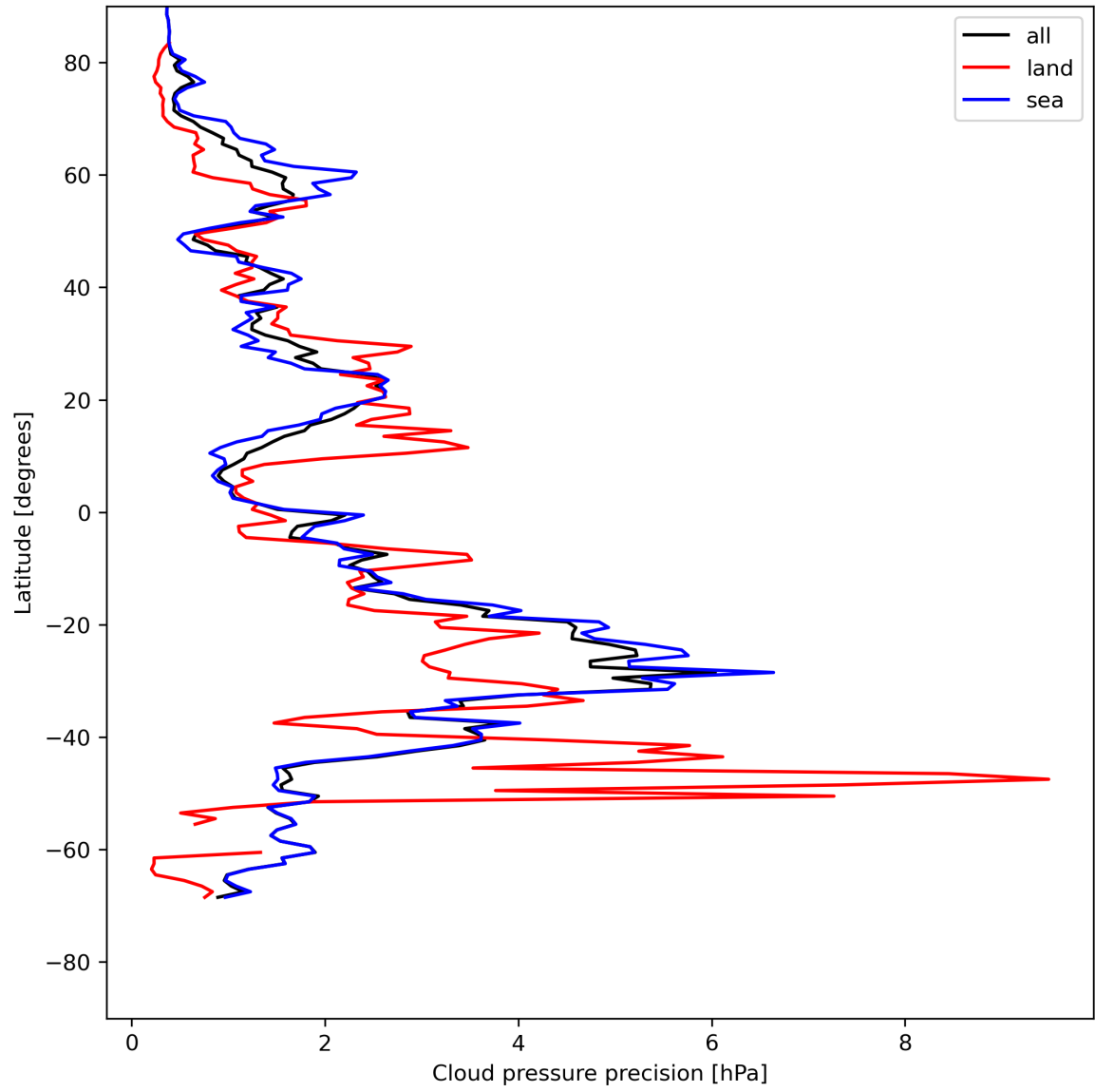
Figure 14: Zonal average of “Cloud pressure precision” for 2024-05-16 to 2024-05-18.
