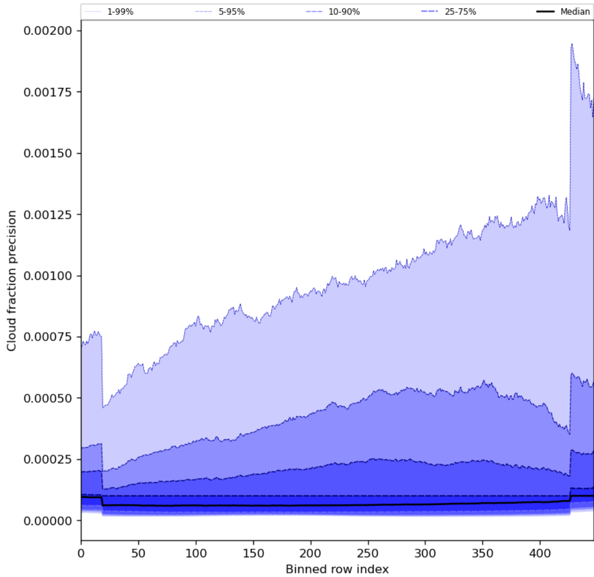
Figure 50: Along track statistics of “Cloud fraction precision” for 2024-05-16 to 2024-05-18
