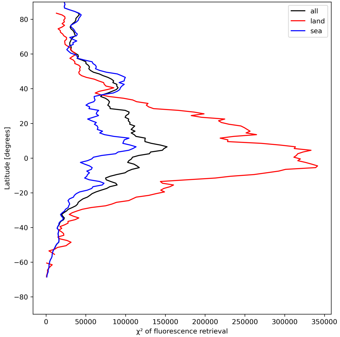
Figure 25: Zonal average of “ \chi^2 of fluorescence retrieval” for 2024-05-16 to 2024-05-18.
