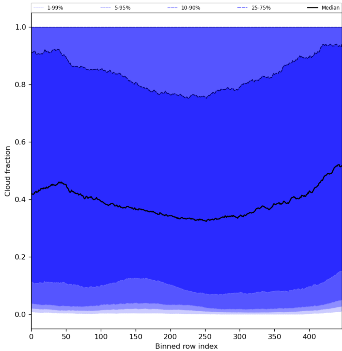
Figure 49: Along track statistics of “Cloud fraction” for 2024-05-16 to 2024-05-18
