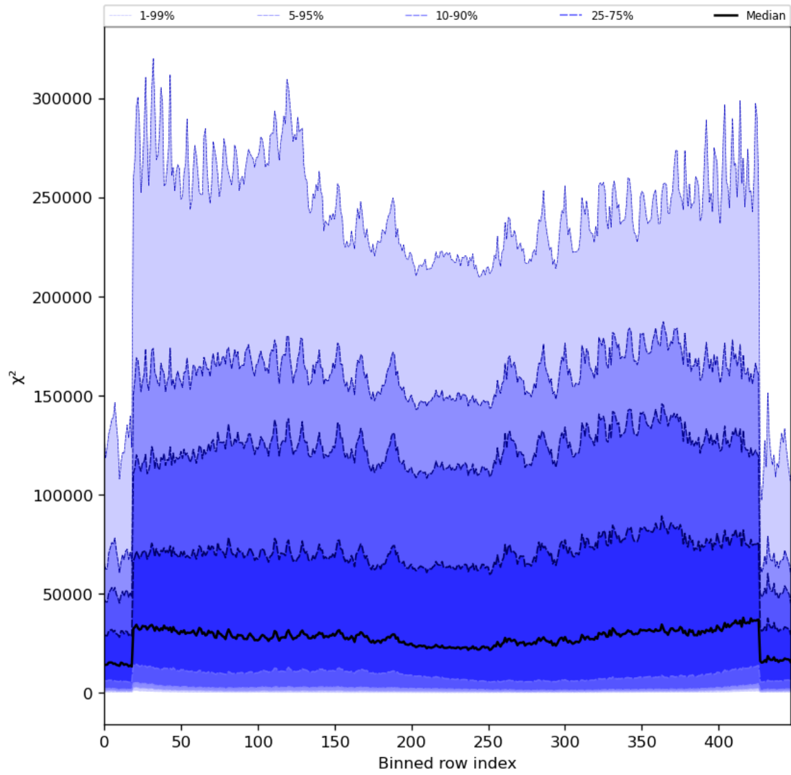
Figure 55: Along track statistics of “ \chi^2 ” for 2024-05-16 to 2024-05-18
