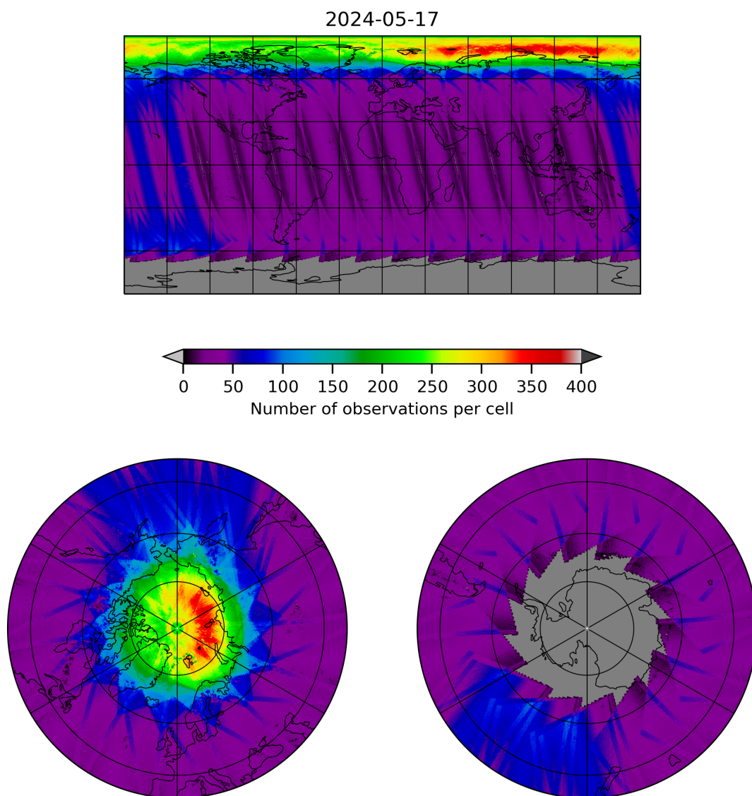
Figure 11: Map of the number of observations for 2024-05-16 to 2024-05-18
