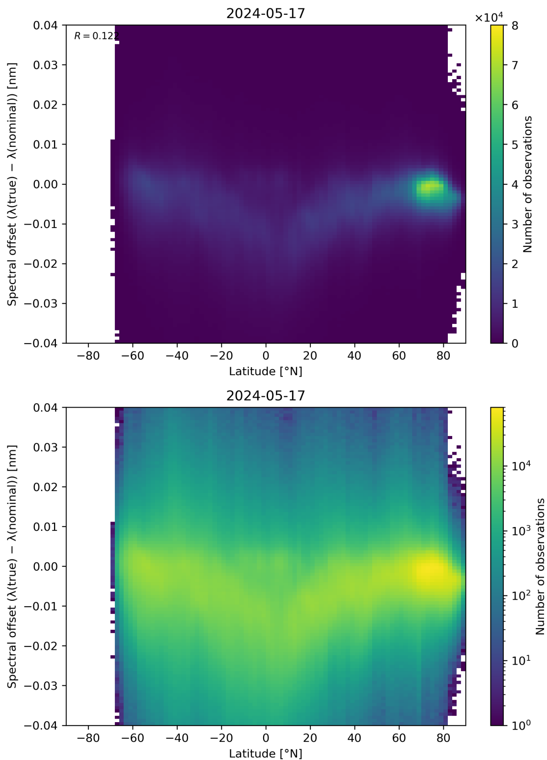
Figure 96: Scatter density plot of “Latitude” against “Spectral offset ( \lambda(\text{true}) - \lambda(\text{nominal}) )” for 2024-05-16 to 2024-05-18.
