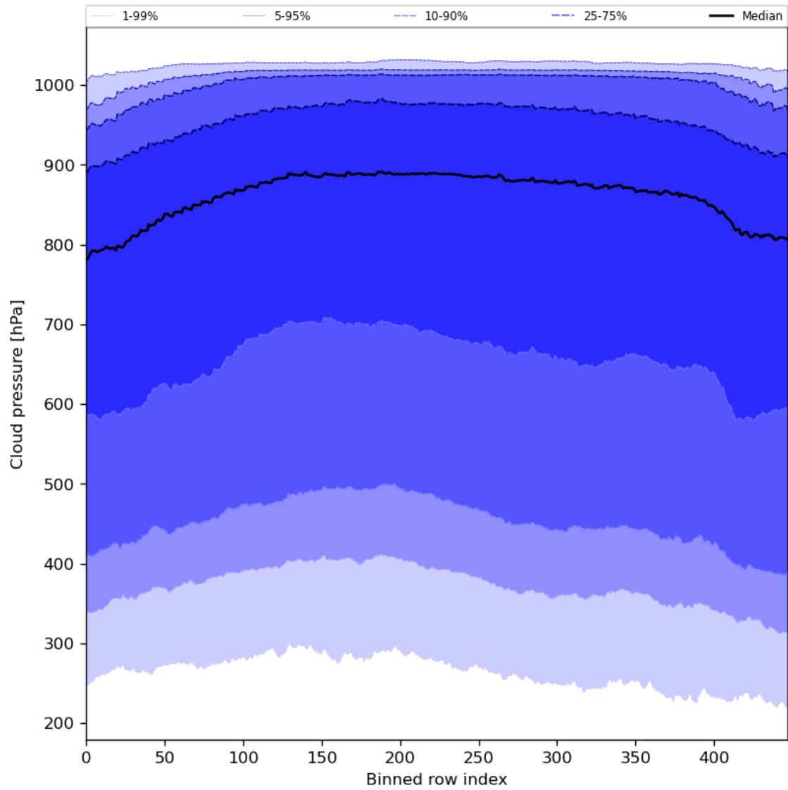
Figure 47: Along track statistics of “Cloud pressure” for 2024-05-18 to 2024-05-19
