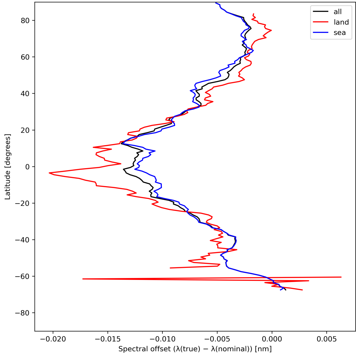
Figure 28: Zonal average of “Spectral offset ( \lambda(\text{true}) - \lambda(\text{nominal}) )” for 2024-05-18 to 2024-05-19.
