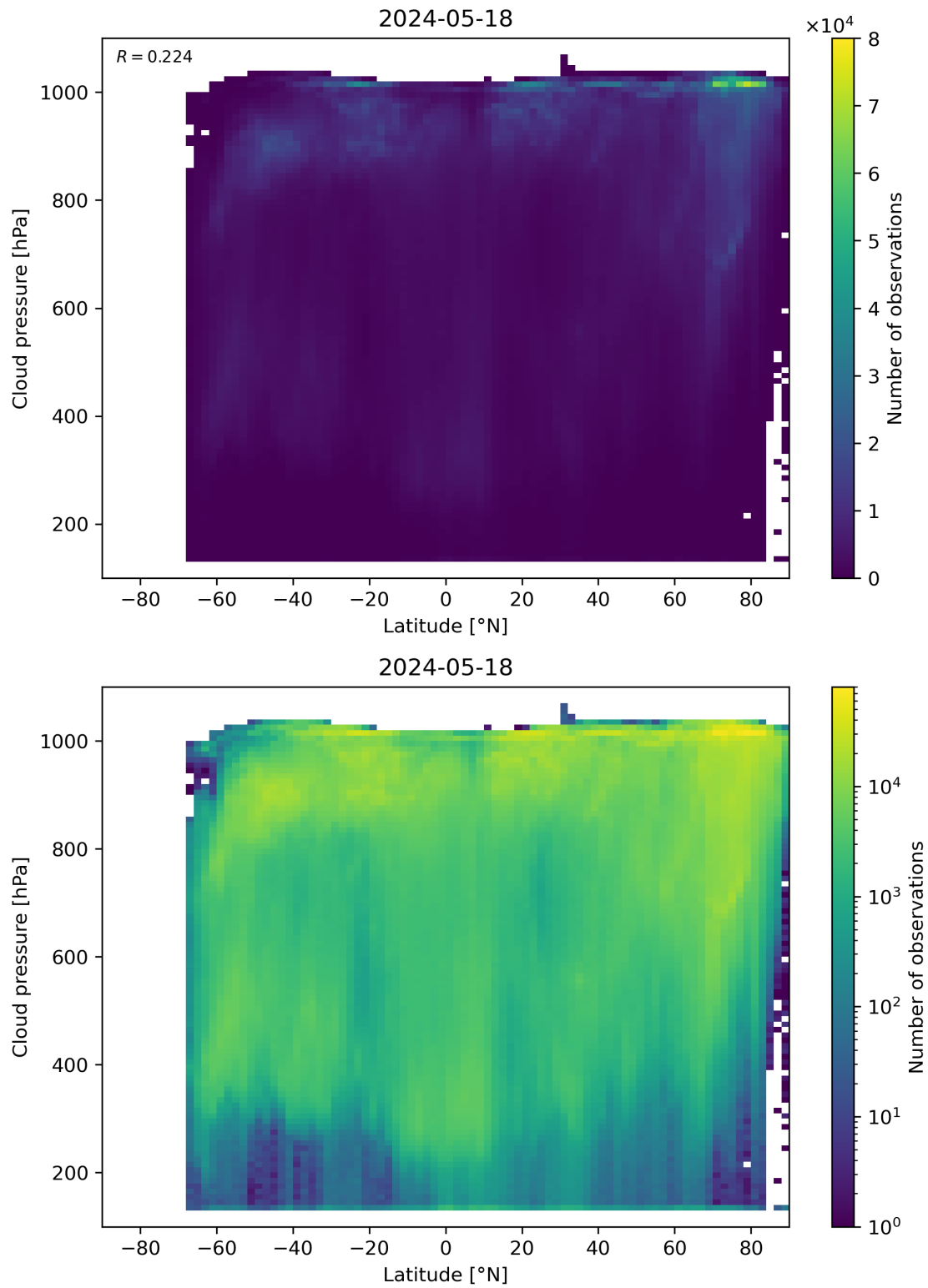
Figure 91: Scatter density plot of “Latitude” against “Cloud pressure” for 2024-05-18 to 2024-05-19.
