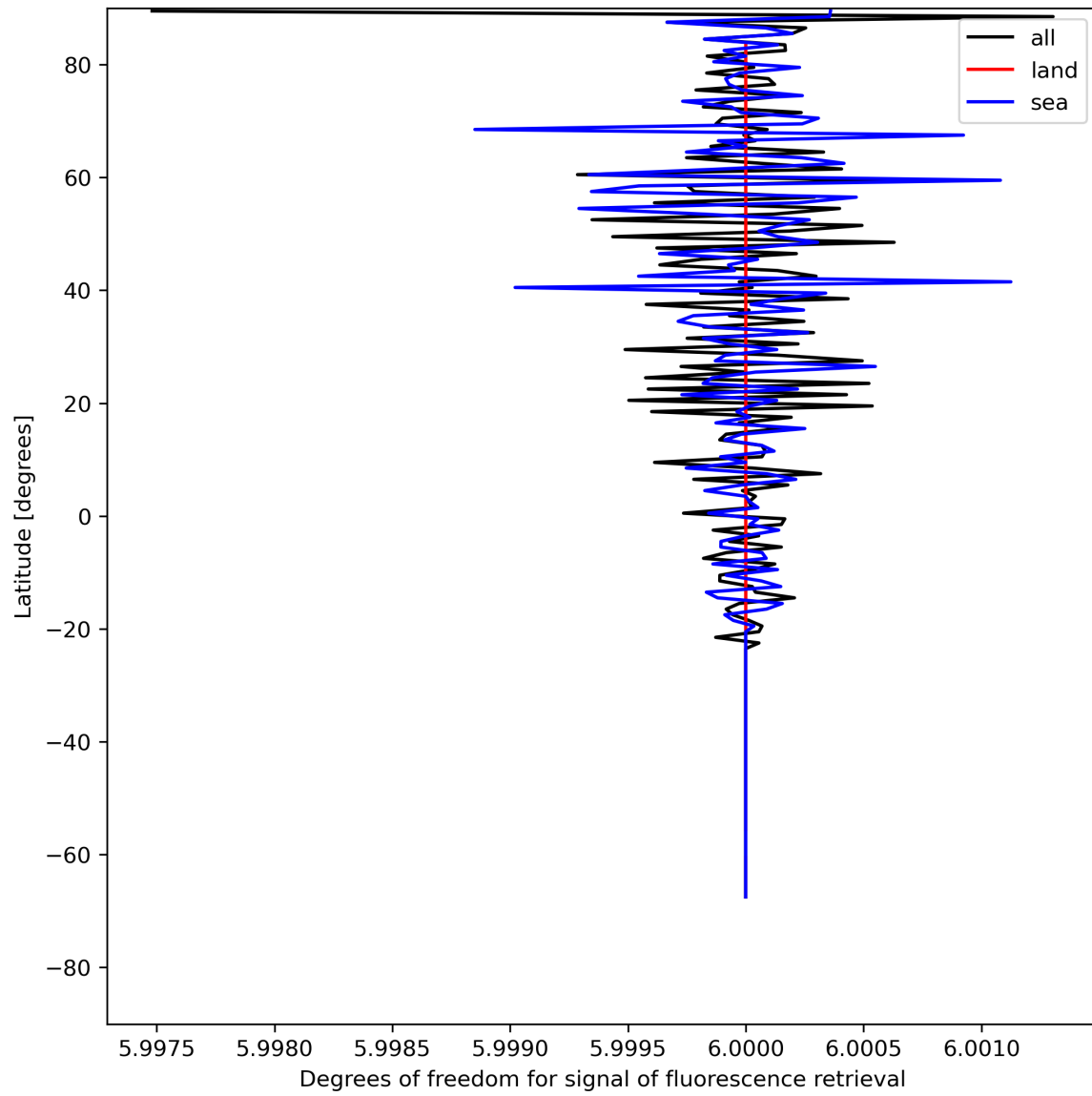
Figure 26: Zonal average of “Degrees of freedom for signal of fluorescence retrieval” for 2024-05-18 to 2024-05-19.
