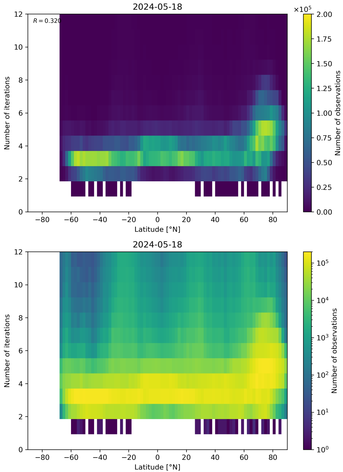
Figure 93: Scatter density plot of “Latitude” against “Number of iterations” for 2024-05-18 to 2024-05-19.
