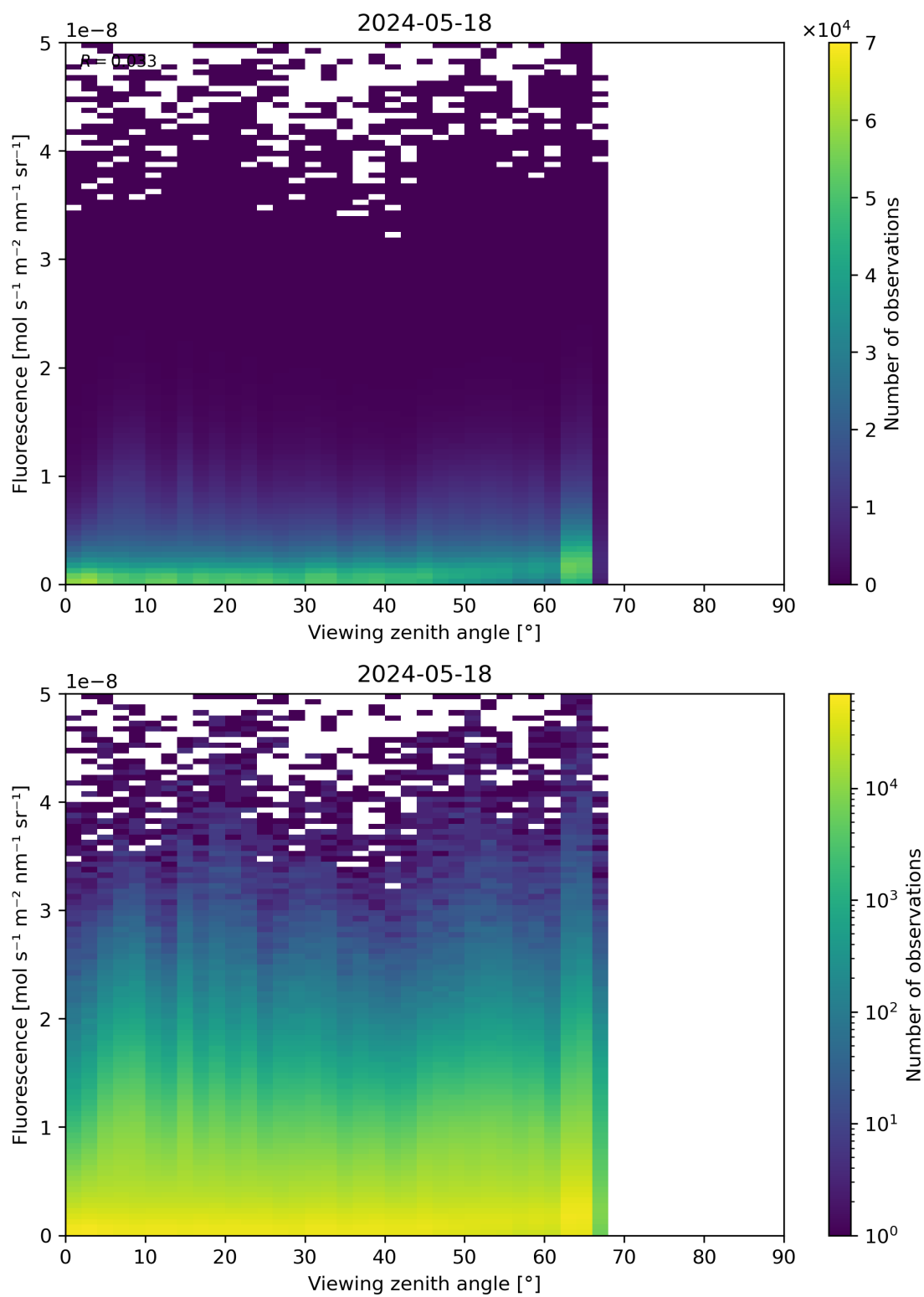
Figure 122: Scatter density plot of “Viewing zenith angle” against “Fluorescence” for 2024-05-18 to 2024-05-19.
