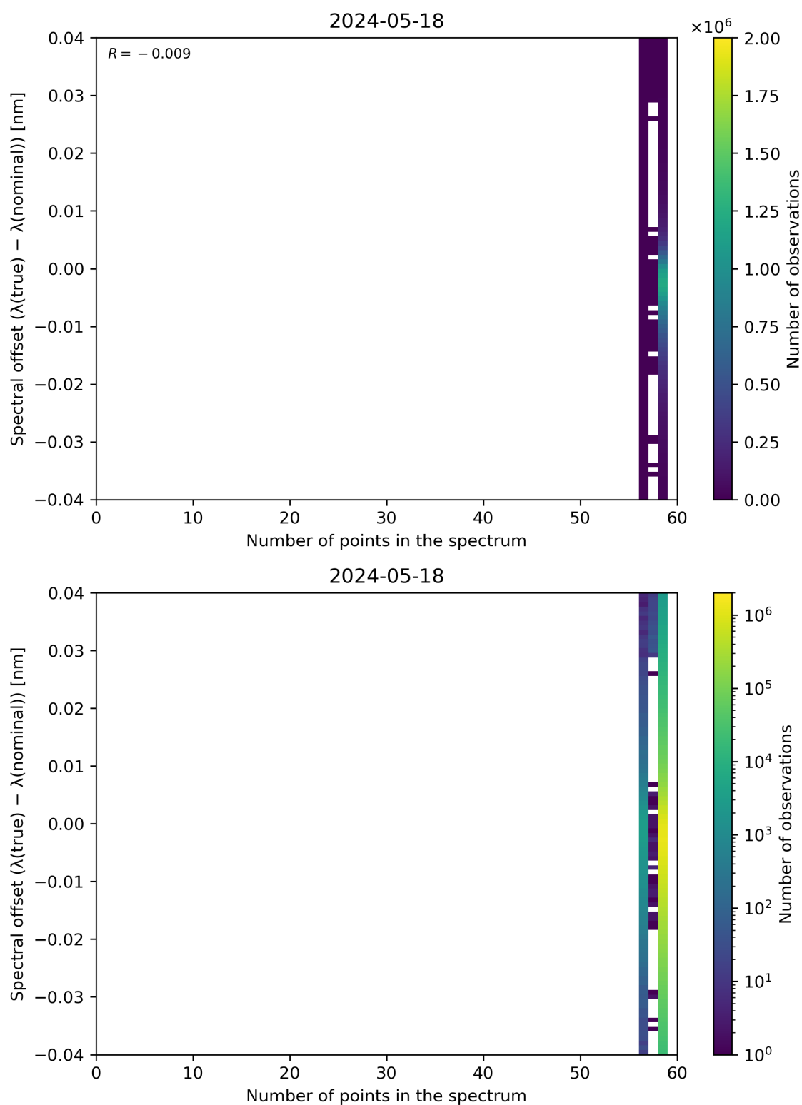
Figure 101: Scatter density plot of “Number of points in the spectrum” against “Spectral offset ( \lambda(\text{true}) - \lambda(\text{nominal}) )” for 2024-05-18 to 2024-05-19.
