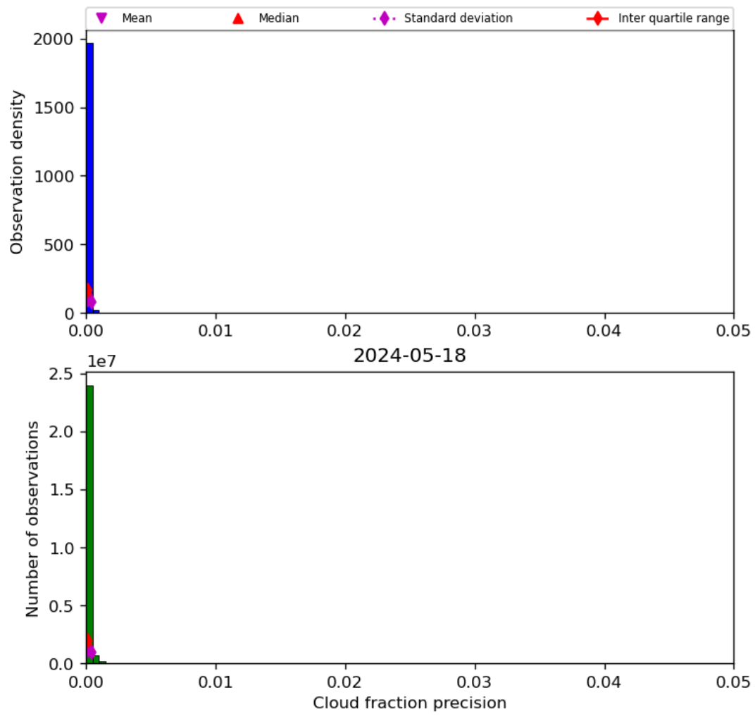
Figure 33: Histogram of “Cloud fraction precision” for 2024-05-18 to 2024-05-19
