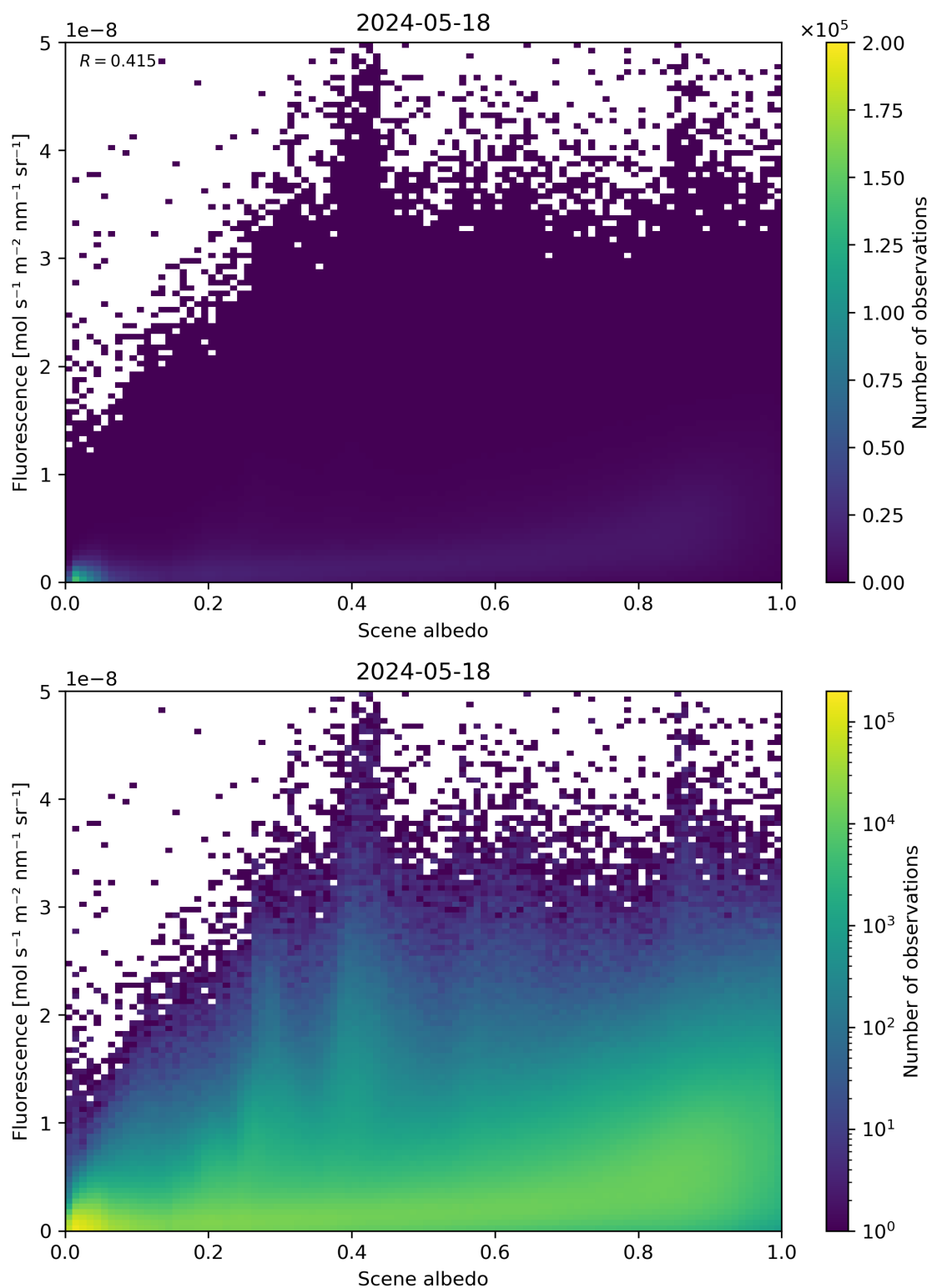
Figure 104: Scatter density plot of “Scene albedo” against “Fluorescence” for 2024-05-18 to 2024-05-19.
