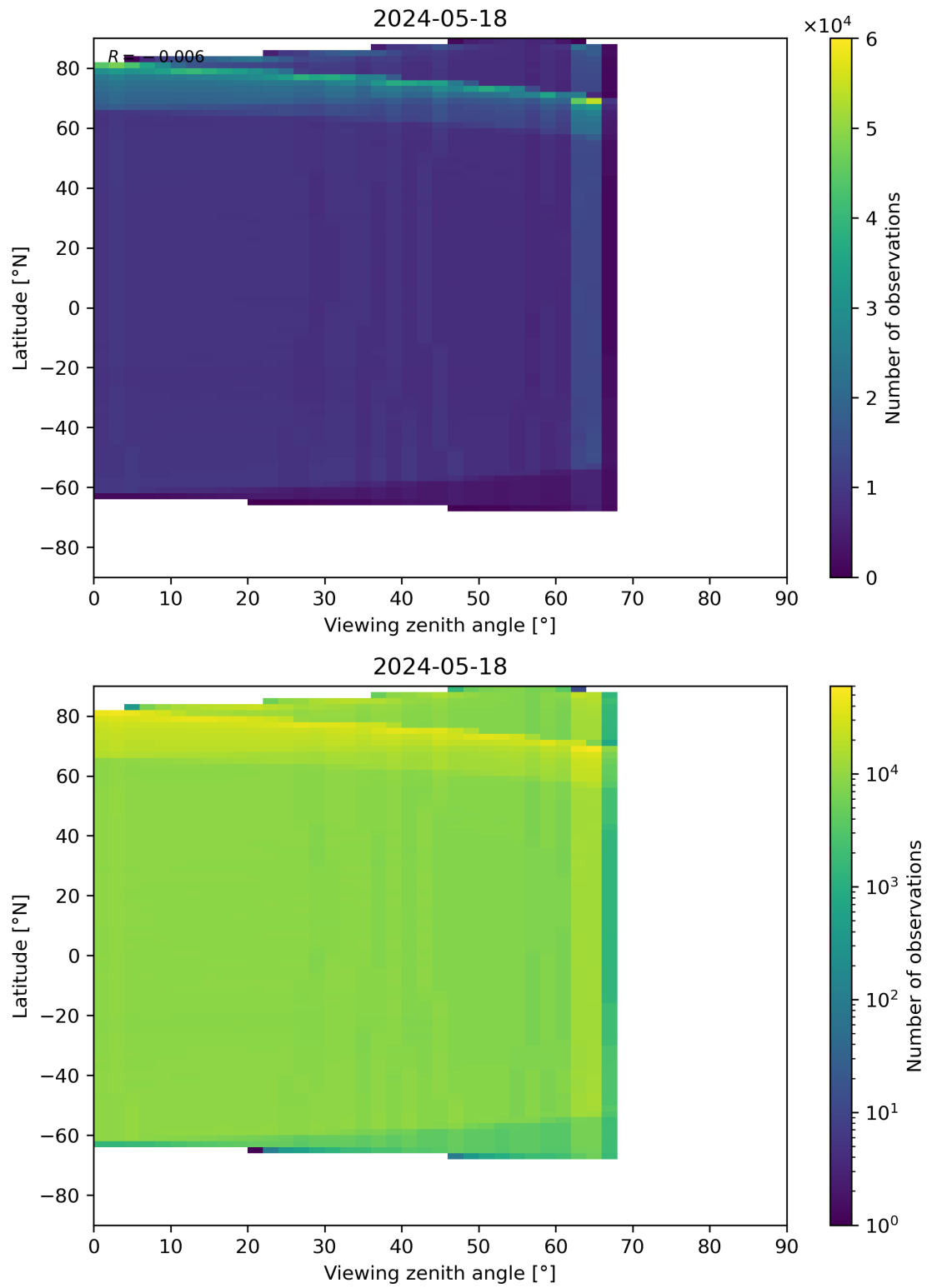
Figure 123: Scatter density plot of “Viewing zenith angle” against “Latitude” for 2024-05-18 to 2024-05-19.
