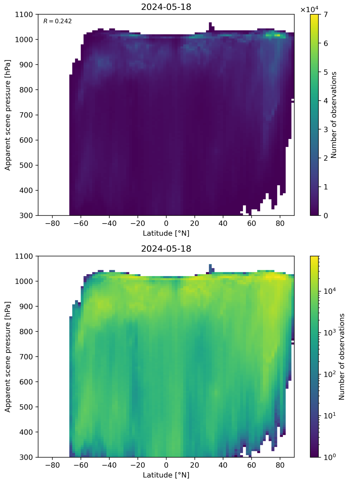
Figure 88: Scatter density plot of “Latitude” against “Apparent scene pressure” for 2024-05-18 to 2024-05-19.
