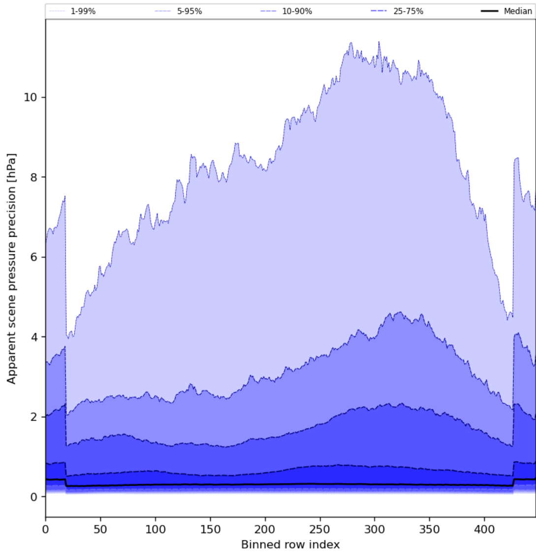
Figure 54: Along track statistics of “Apparent scene pressure precision” for 2024-05-18 to 2024-05-19
