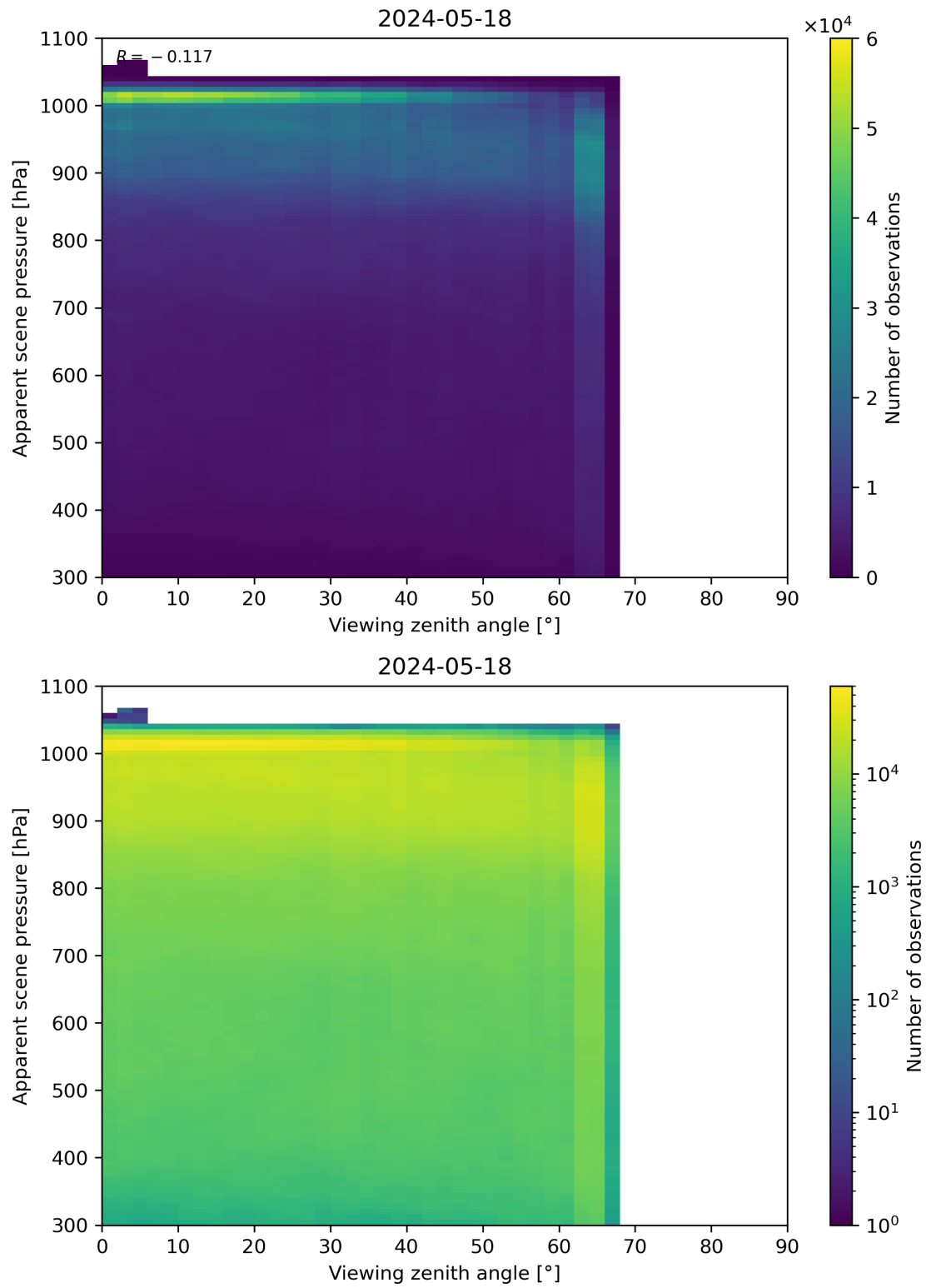
Figure 118: Scatter density plot of “Viewing zenith angle” against “Apparent scene pressure” for 2024-05-18 to 2024-05-19.
