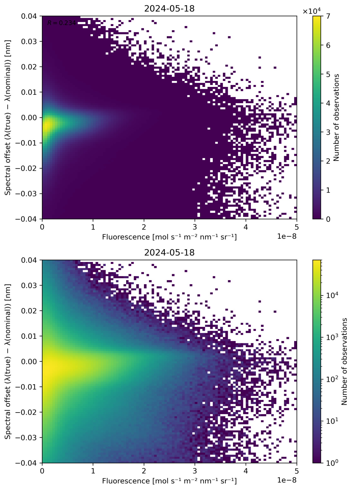
Figure 87: Scatter density plot of “Fluorescence” against “Spectral offset ( \lambda(\text{true}) - \lambda(\text{nominal}) )” for 2024-05-18 to 2024-05-19.
