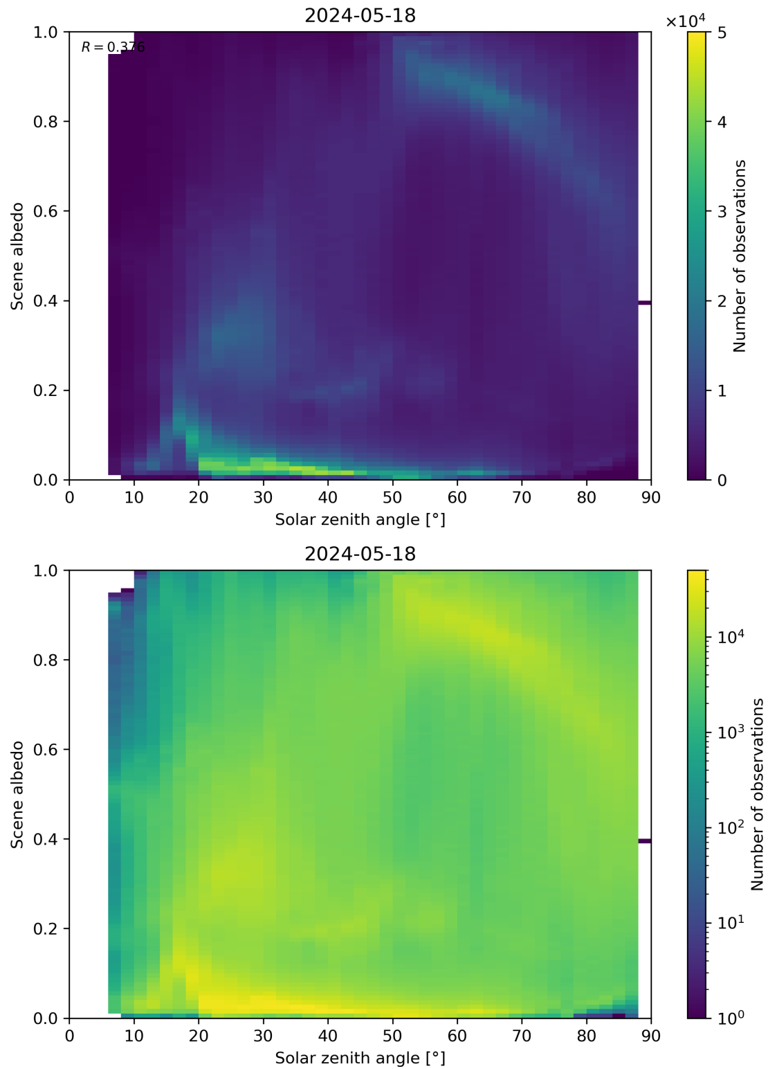
Figure 116: Scatter density plot of “Solar zenith angle” against “Scene albedo” for 2024-05-18 to 2024-05-19.
