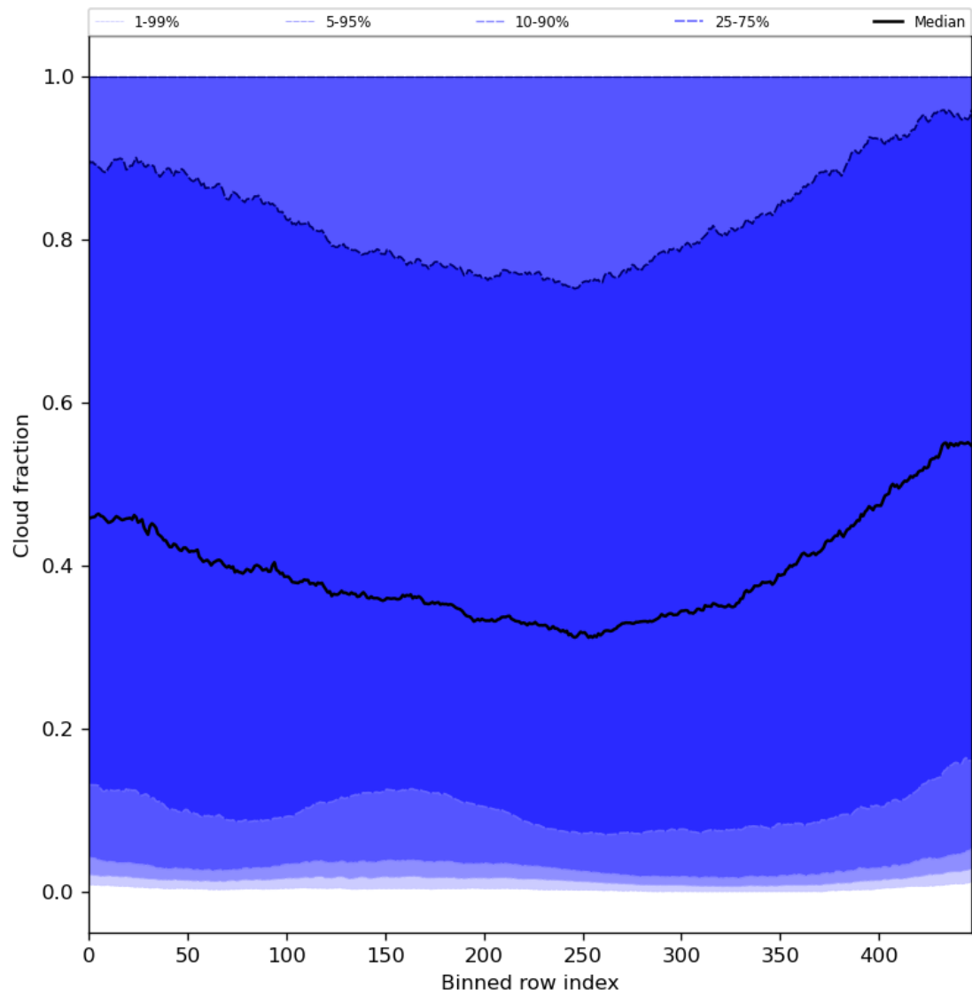
Figure 49: Along track statistics of “Cloud fraction” for 2024-05-18 to 2024-05-19
