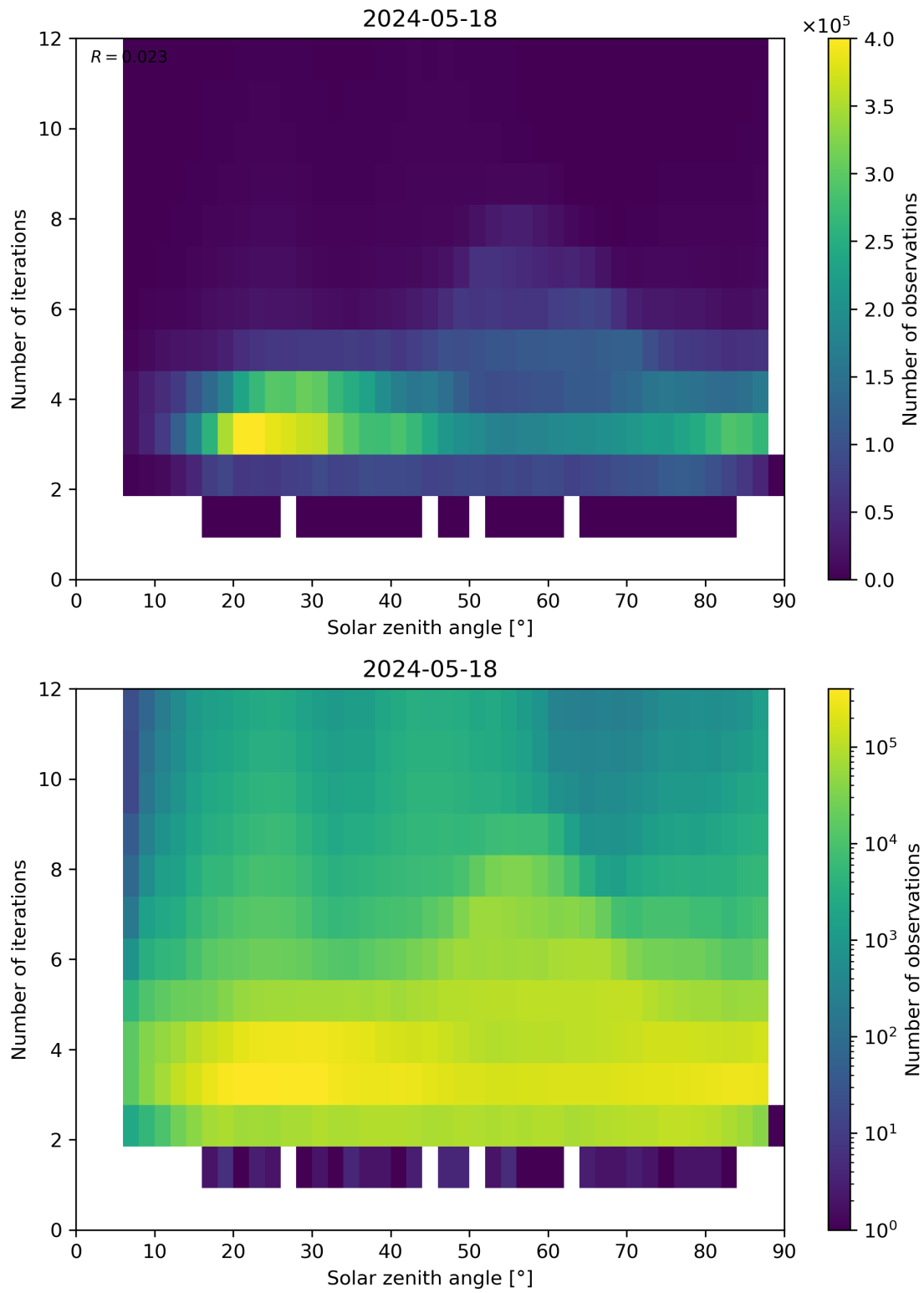
Figure 114: Scatter density plot of “Solar zenith angle” against “Number of iterations” for 2024-05-18 to 2024-05-19.
