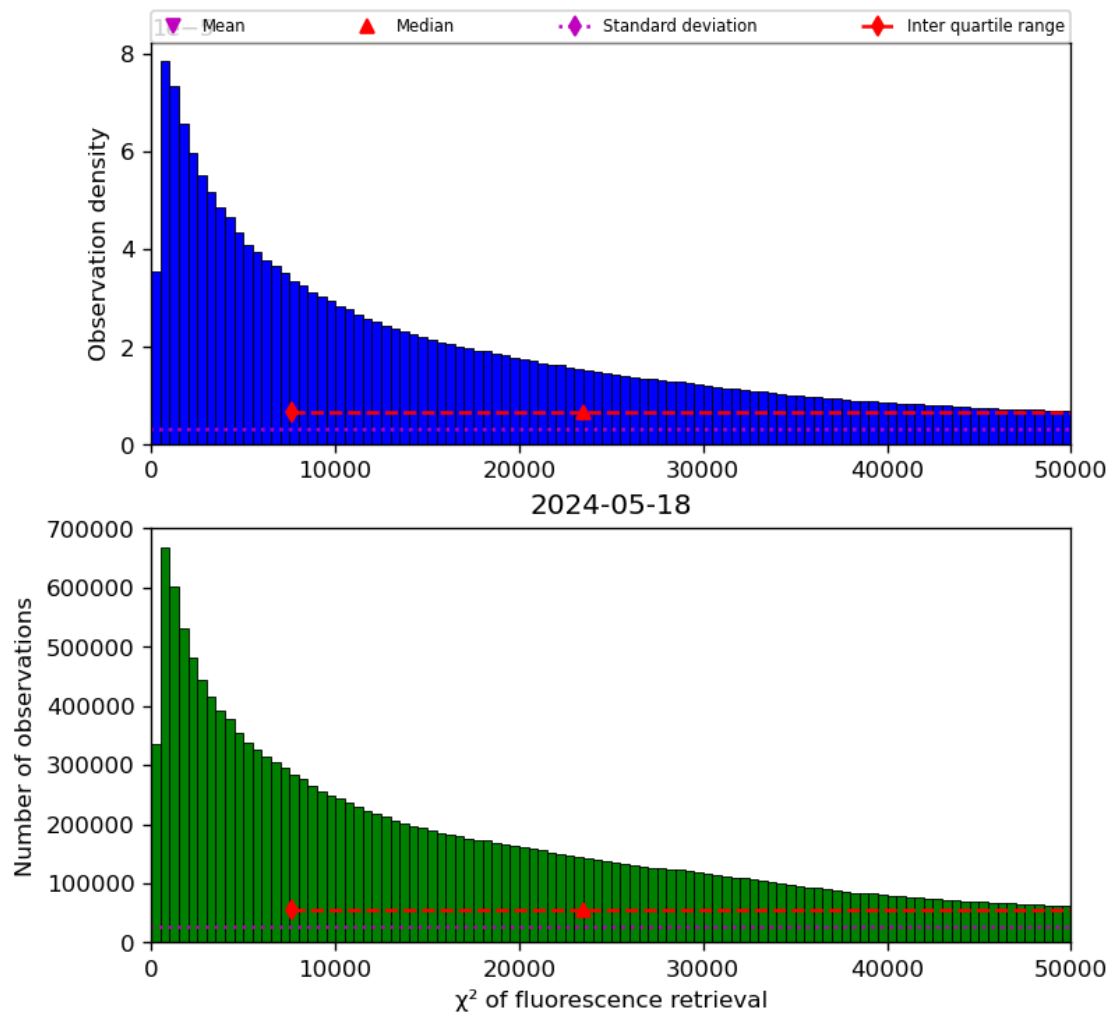
Figure 42: Histogram of “ \chi^2 of fluorescence retrieval” for 2024-05-18 to 2024-05-19
