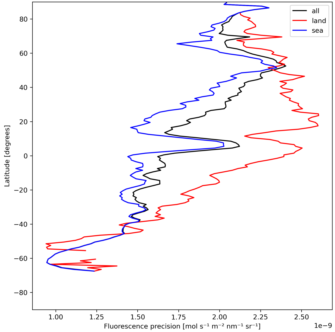
Figure 24: Zonal average of “Fluorescence precision” for 2024-05-18 to 2024-05-19.
