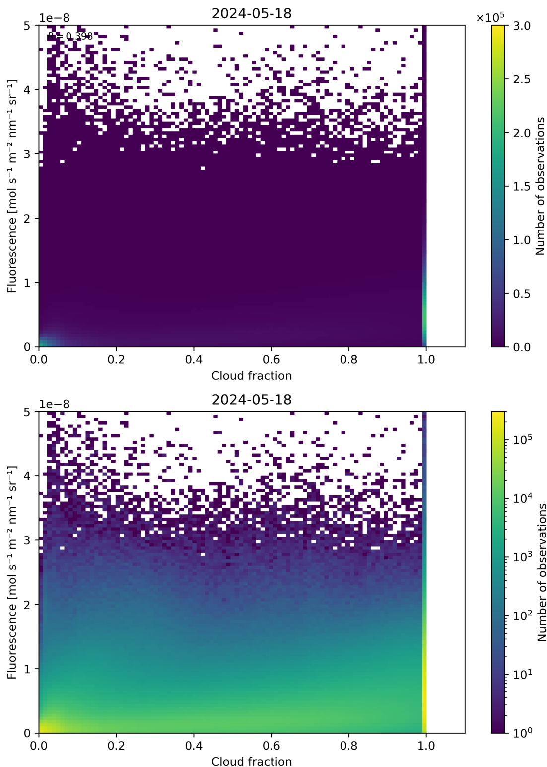
Figure 72: Scatter density plot of “Cloud fraction” against “Fluorescence” for 2024-05-18 to 2024-05-19.
