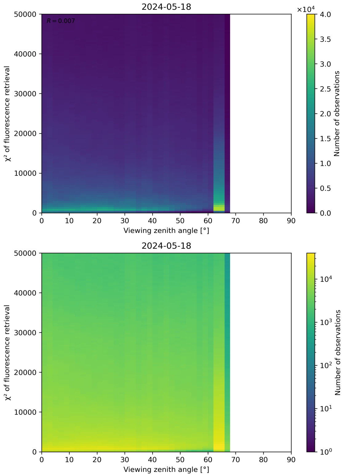
Figure 119: Scatter density plot of “Viewing zenith angle” against “ \chi^2 of fluorescence retrieval” for 2024-05-18 to 2024-05-19.
