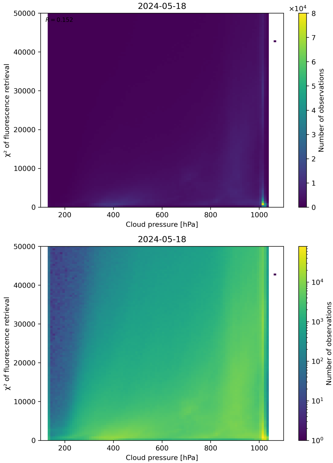
Figure 78: Scatter density plot of “Cloud pressure” against “ \chi^2 of fluorescence retrieval” for 2024-05-18 to 2024-05-19.
