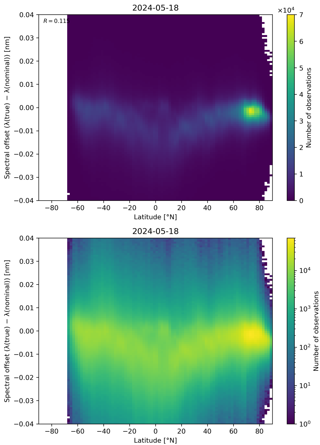
Figure 96: Scatter density plot of “Latitude” against “Spectral offset ( \lambda(\text{true}) - \lambda(\text{nominal}) )” for 2024-05-18 to 2024-05-19.
