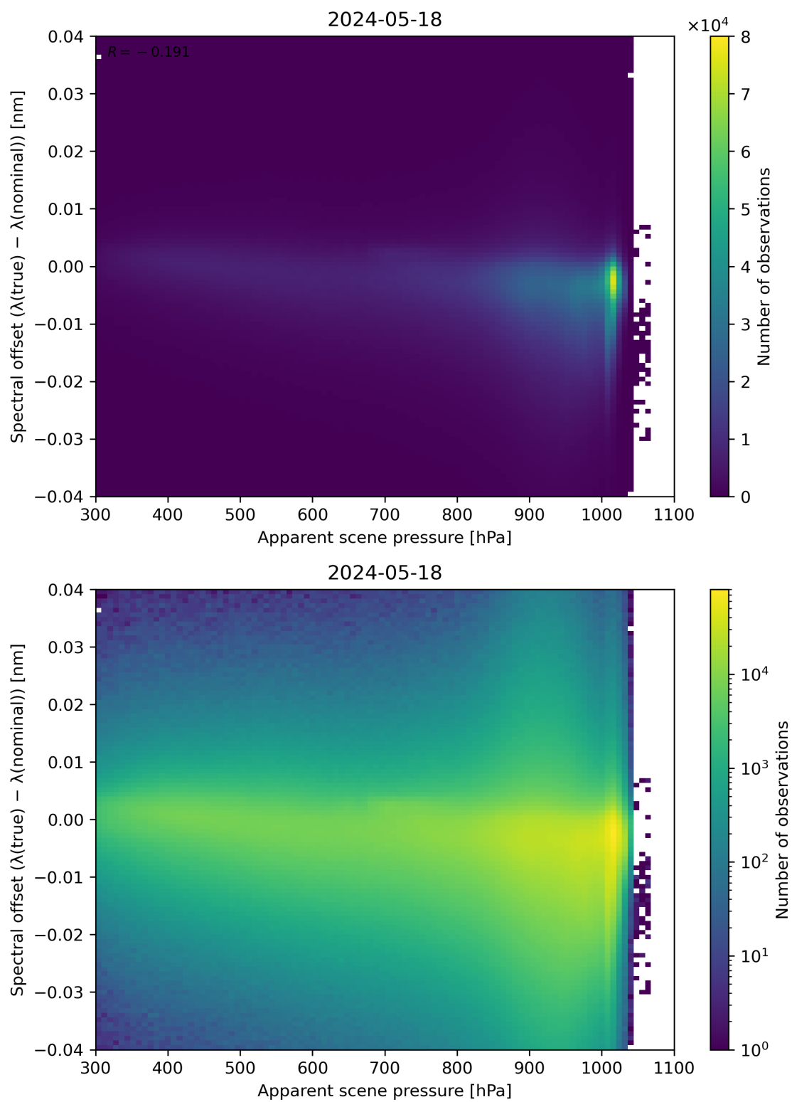
Figure 67: Scatter density plot of “Apparent scene pressure” against “Spectral offset ( \lambda(\text{true}) - \lambda(\text{nominal}) )” for 2024-05-18 to 2024-05-19.
