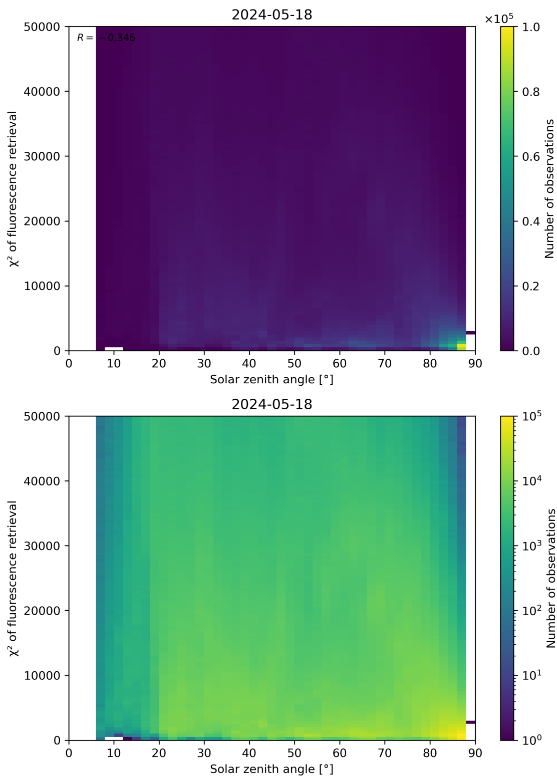
Figure 109: Scatter density plot of “Solar zenith angle” against “ \chi^2 of fluorescence retrieval” for 2024-05-18 to 2024-05-19.
