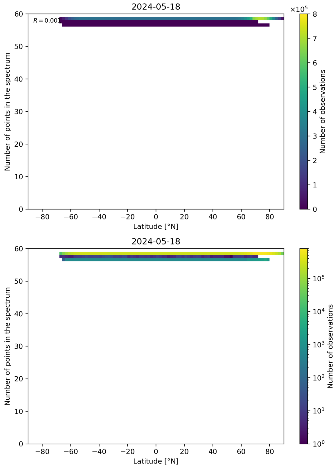
Figure 94: Scatter density plot of “Latitude” against “Number of points in the spectrum” for 2024-05-18 to 2024-05-19.
