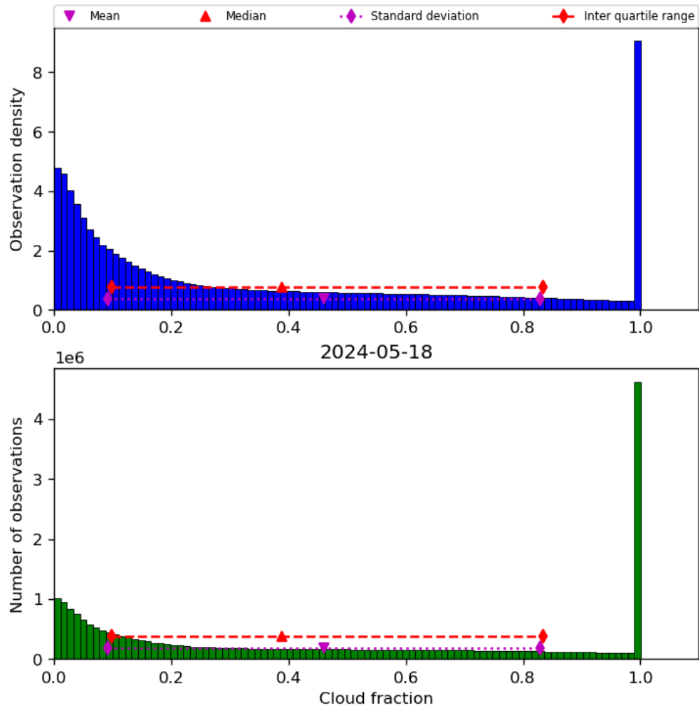
Figure 32: Histogram of “Cloud fraction” for 2024-05-18 to 2024-05-19
