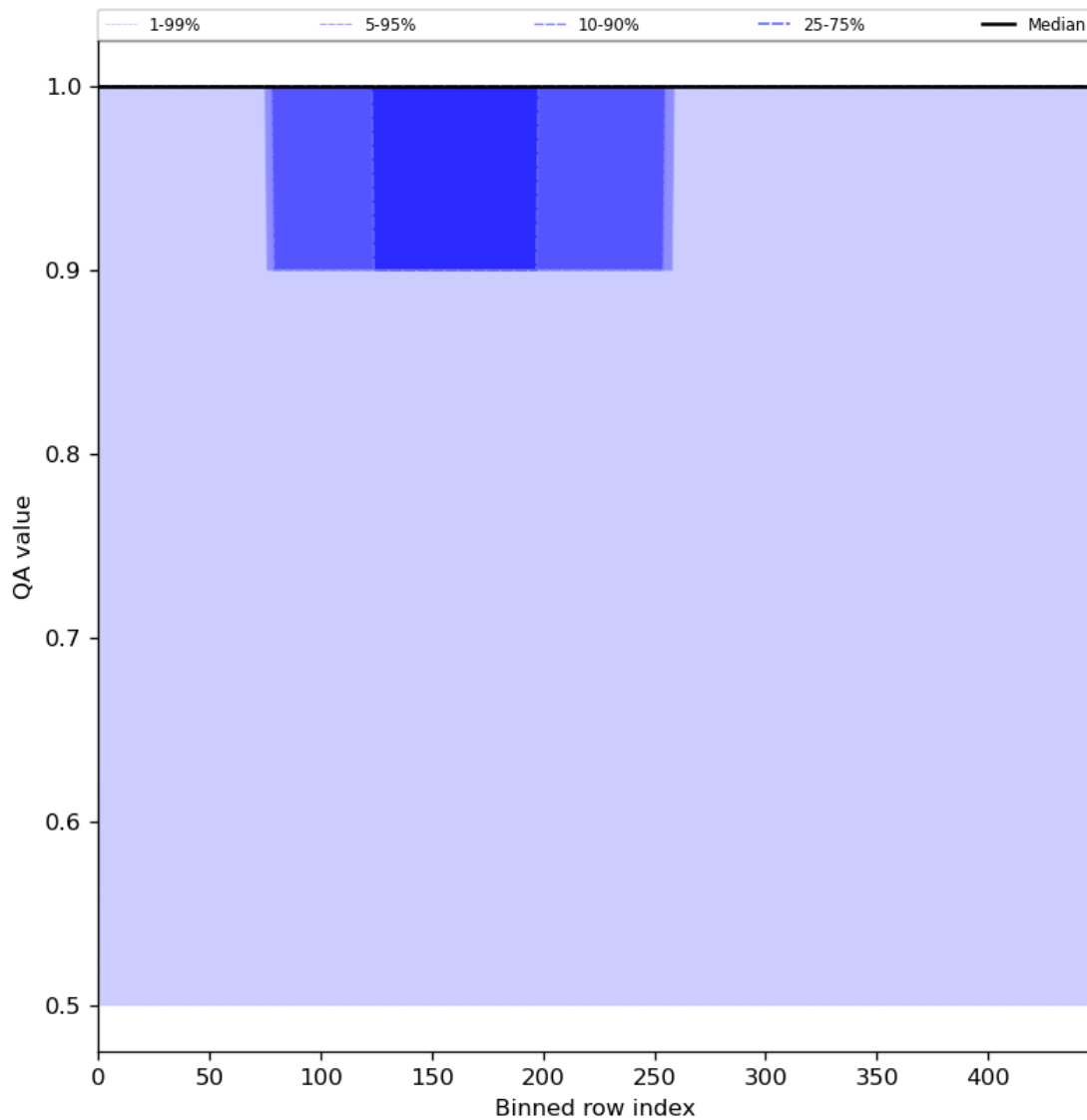
Figure 46: Along track statistics of “QA value” for 2024-05-18 to 2024-05-19
