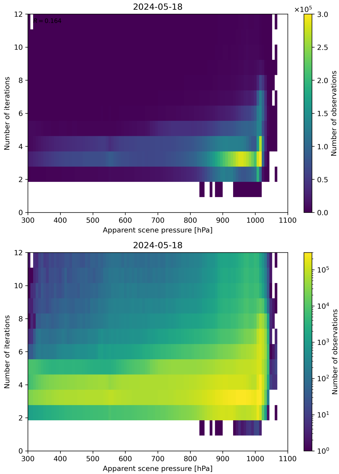
Figure 65: Scatter density plot of “Apparent scene pressure” against “Number of iterations” for 2024-05-18 to 2024-05-19.
