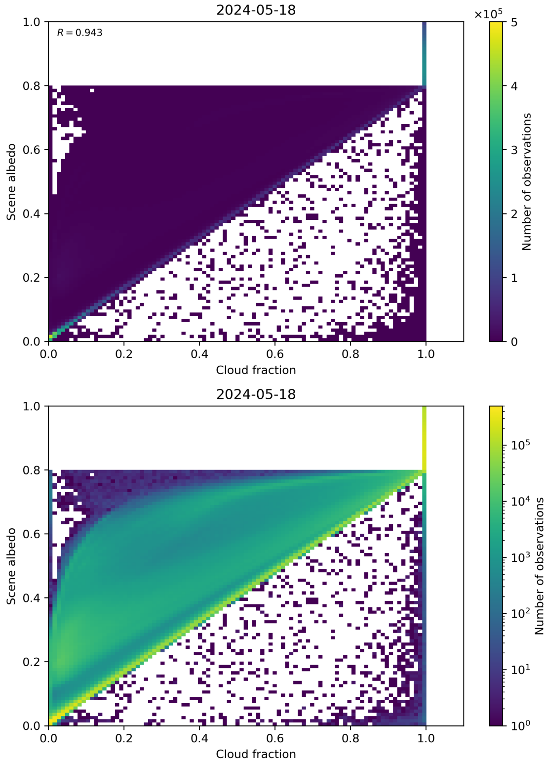
Figure 75: Scatter density plot of “Cloud fraction” against “Scene albedo” for 2024-05-18 to 2024-05-19.
