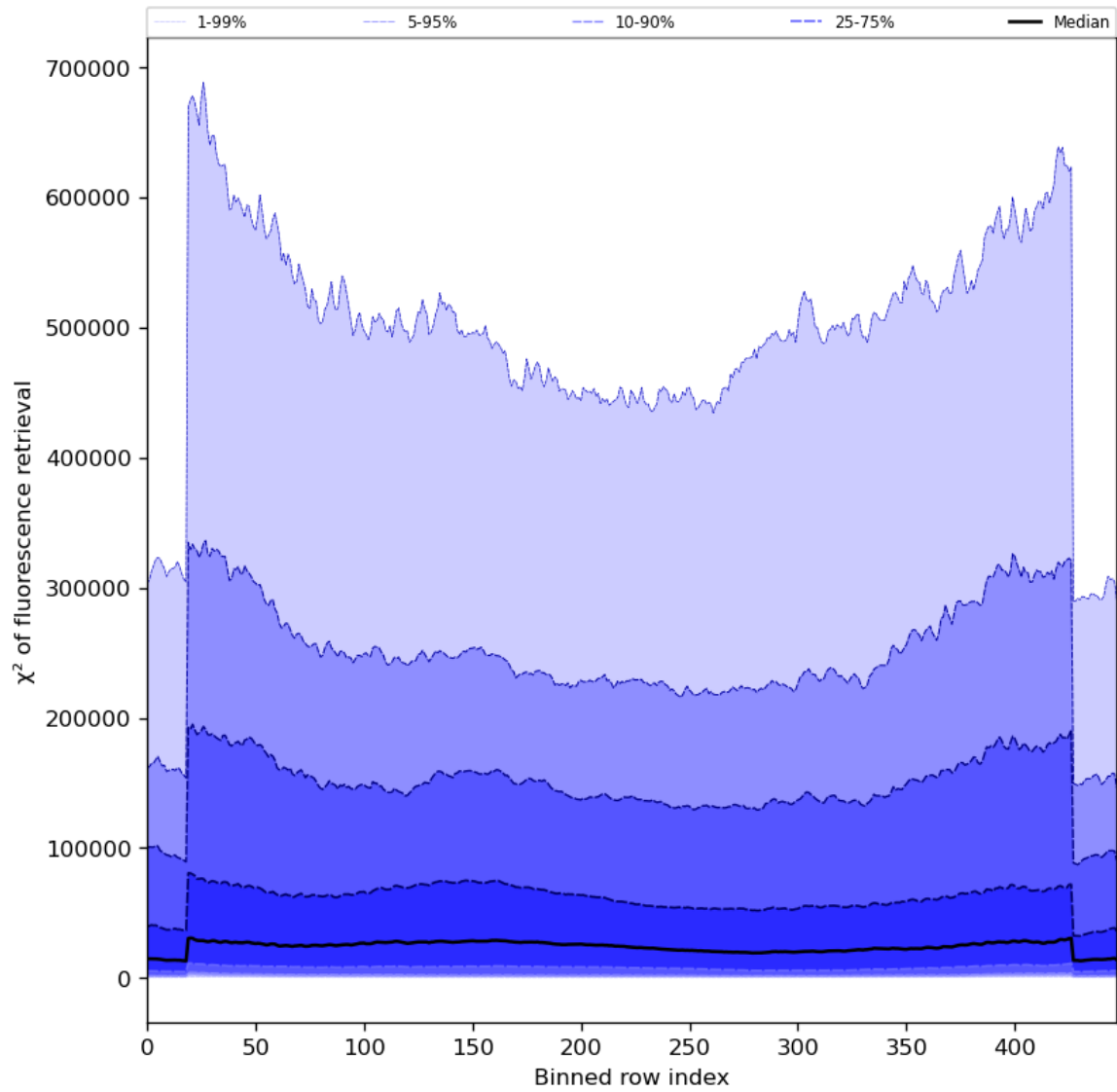
Figure 59: Along track statistics of “ \chi^2 of fluorescence retrieval” for 2024-05-18 to 2024-05-19
