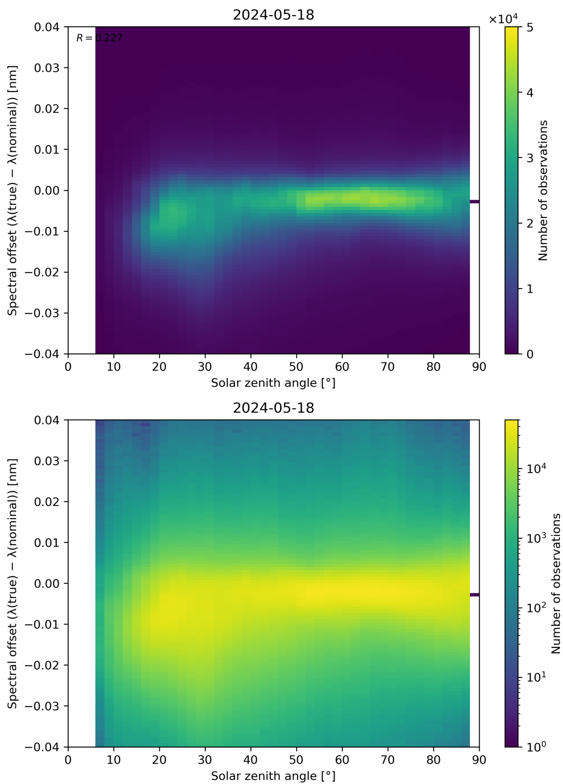
Figure 117: Scatter density plot of “Solar zenith angle” against “Spectral offset ( \lambda(\text{true}) - \lambda(\text{nominal}) )” for 2024-05-18 to 2024-05-19.
