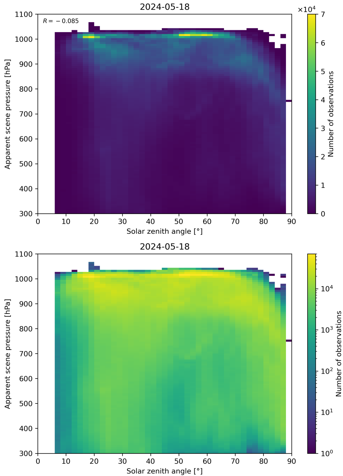
Figure 108: Scatter density plot of “Solar zenith angle” against “Apparent scene pressure” for 2024-05-18 to 2024-05-19.
