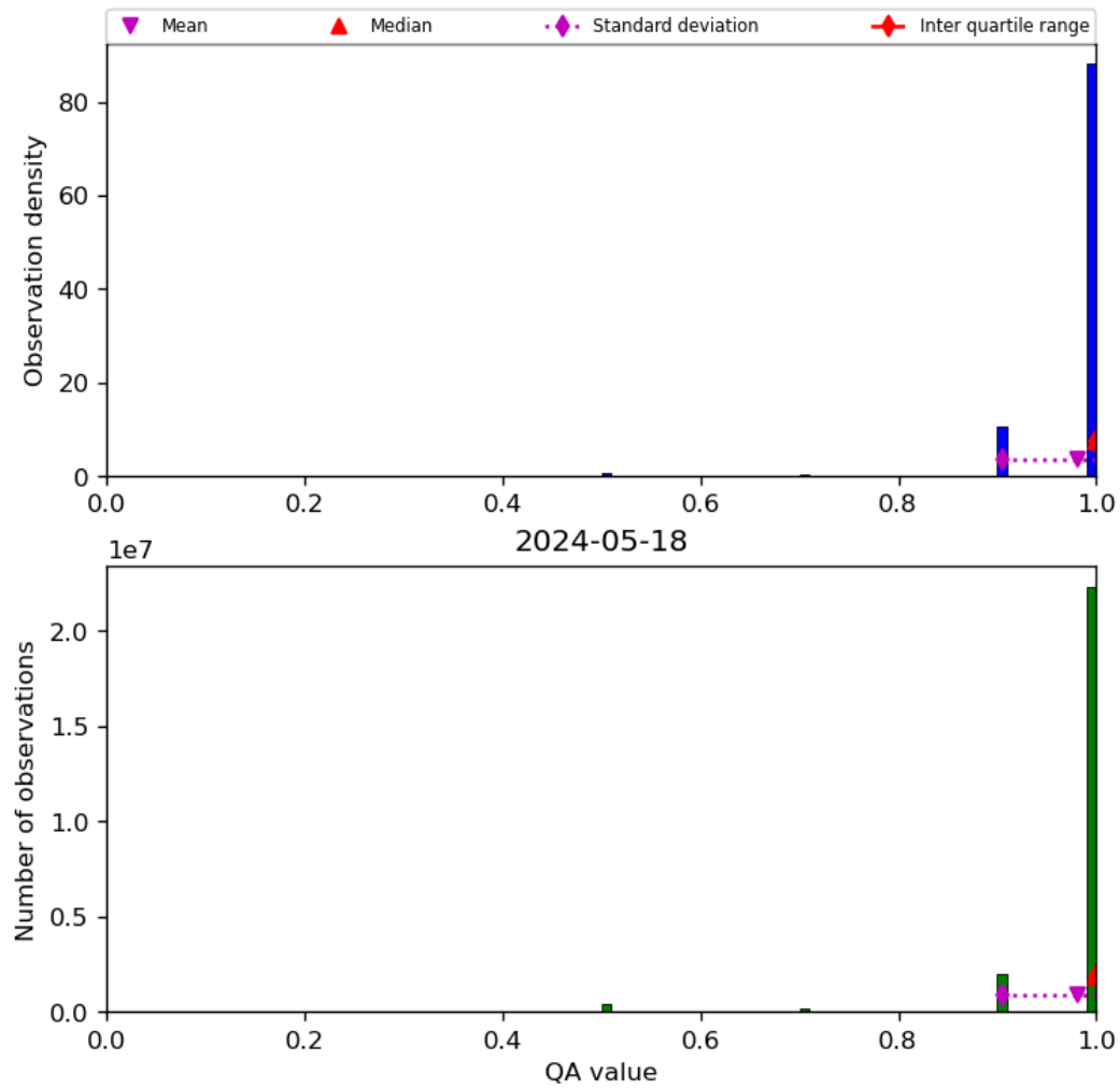
Figure 29: Histogram of “QA value” for 2024-05-18 to 2024-05-19
