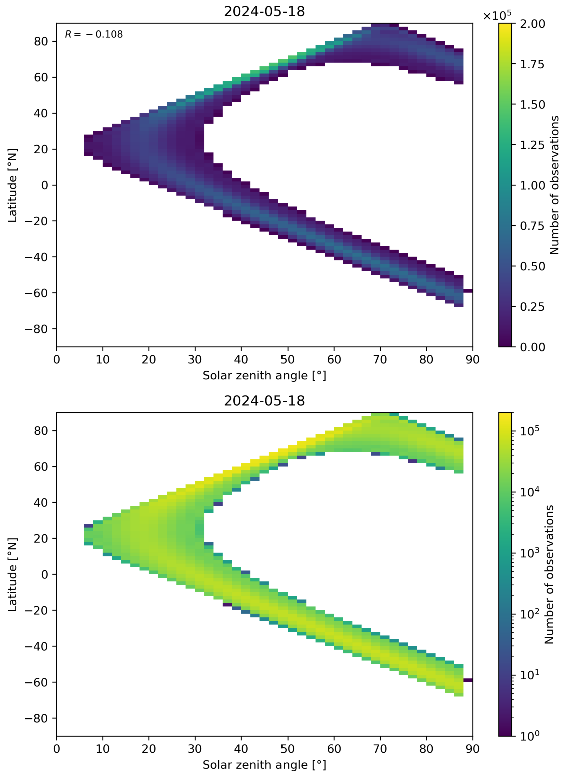
Figure 113: Scatter density plot of “Solar zenith angle” against “Latitude” for 2024-05-18 to 2024-05-19.
