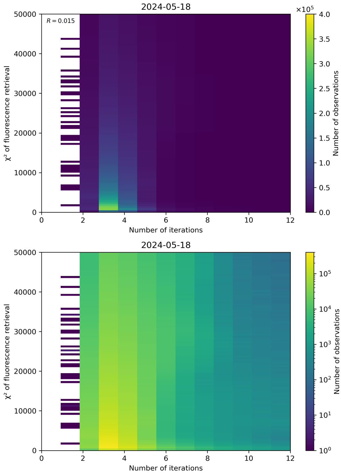
Figure 97: Scatter density plot of “Number of iterations” against “ \chi^2 of fluorescence retrieval” for 2024-05-18 to 2024-05-19.
