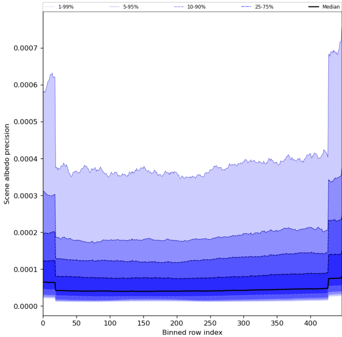
Figure 52: Along track statistics of “Scene albedo precision” for 2024-05-18 to 2024-05-19
