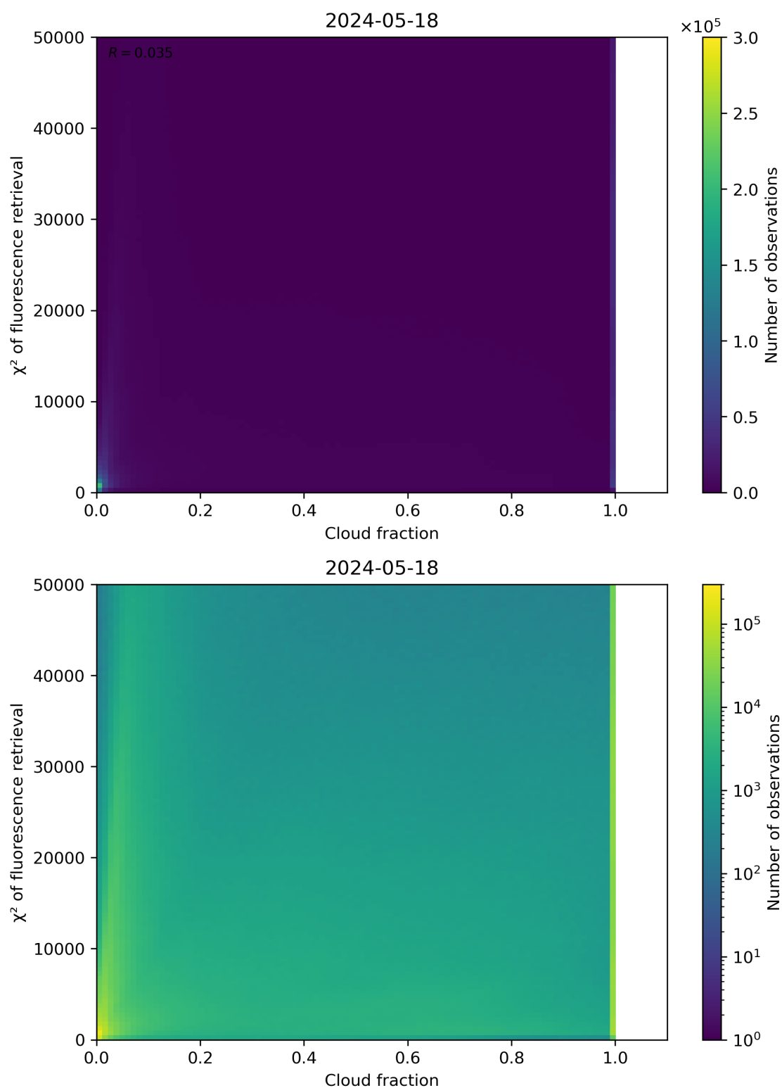
Figure 71: Scatter density plot of “Cloud fraction” against “ \chi^2 of fluorescence retrieval” for 2024-05-18 to 2024-05-19.
