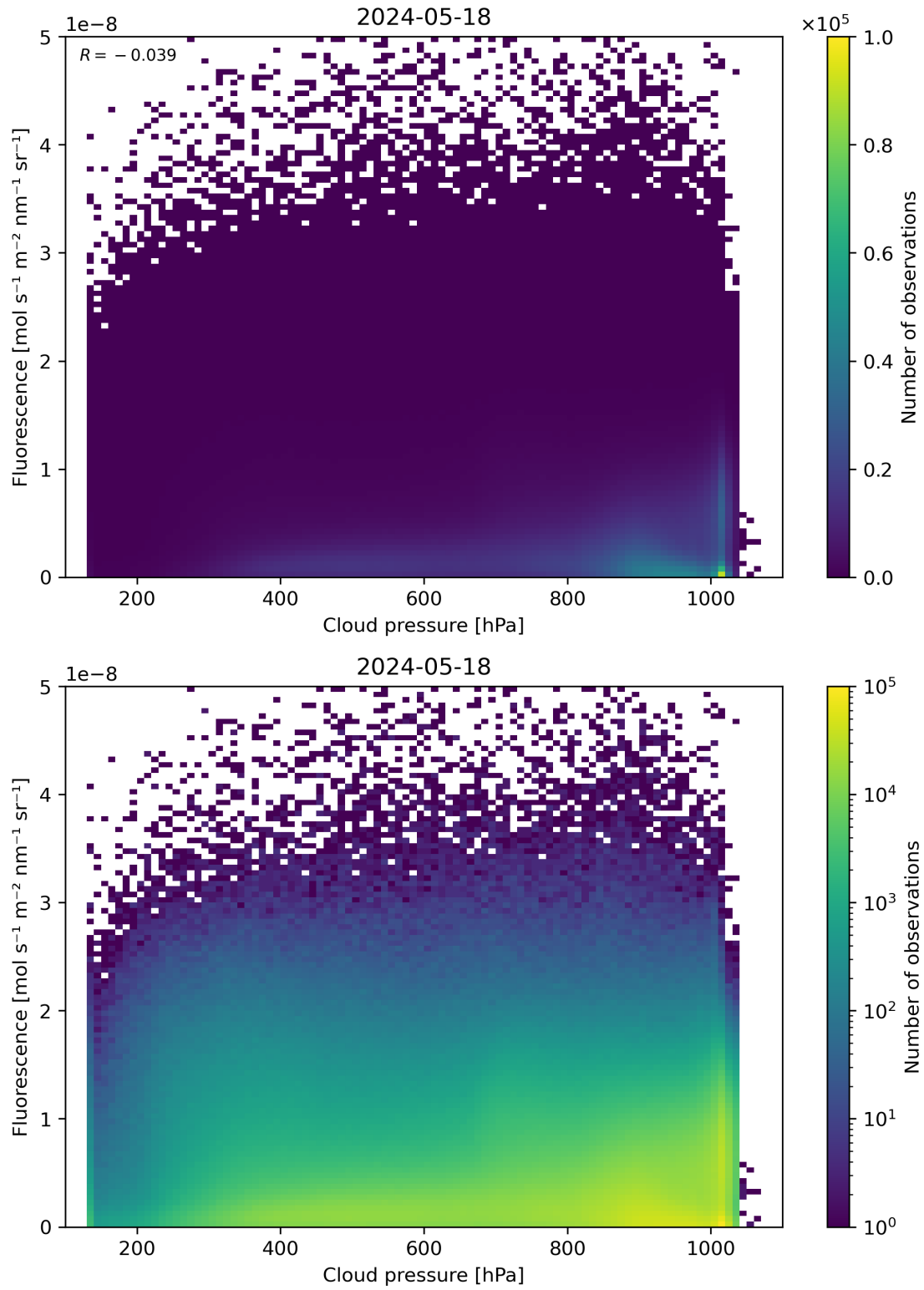
Figure 80: Scatter density plot of “Cloud pressure” against “Fluorescence” for 2024-05-18 to 2024-05-19.
