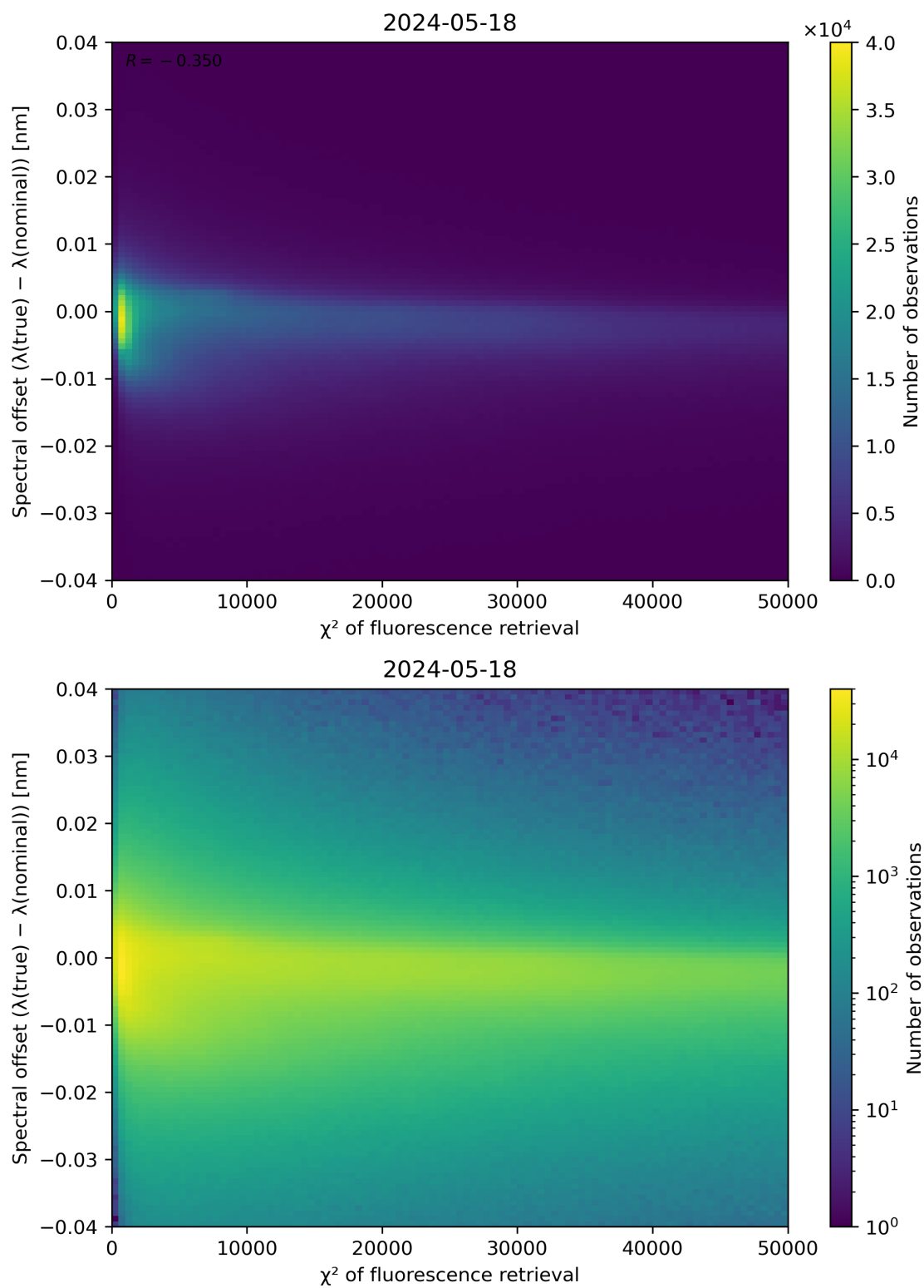
Figure 69: Scatter density plot of " \chi^2 of fluorescence retrieval" against "Spectral offset ( \lambda(\text{true}) - \lambda(\text{nominal}) )" for 2024-05-18 to 2024-05-19.
