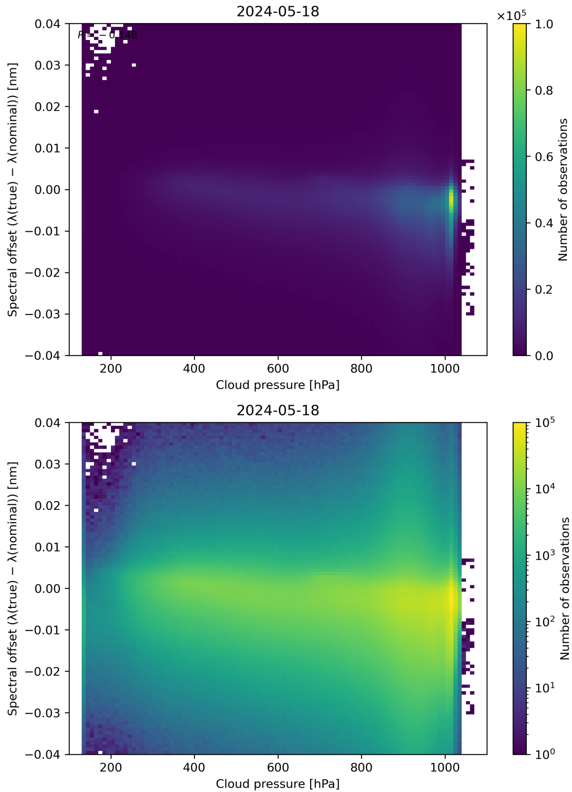
Figure 84: Scatter density plot of “Cloud pressure” against “Spectral offset ( \lambda(\text{true}) - \lambda(\text{nominal}) )” for 2024-05-18 to 2024-05-19.
