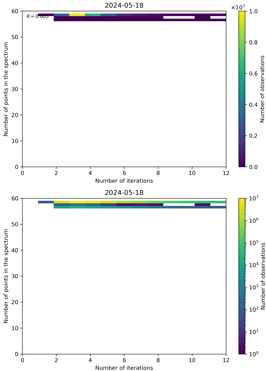
Figure 99: Scatter density plot of “Number of iterations” against “Number of points in the spectrum” for 2024-05-18 to 2024-05-19.
