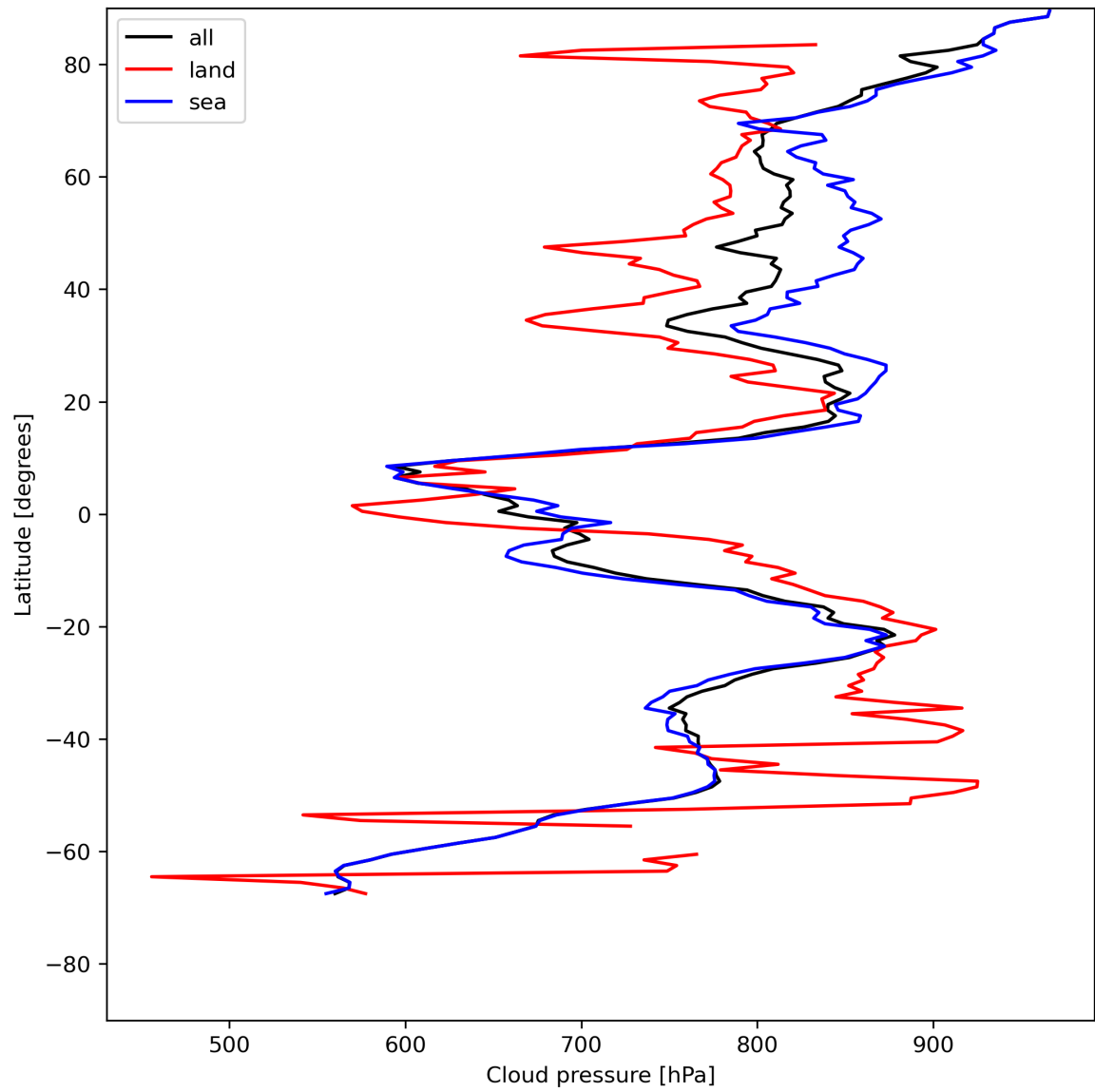
Figure 13: Zonal average of “Cloud pressure” for 2024-05-18 to 2024-05-19.
