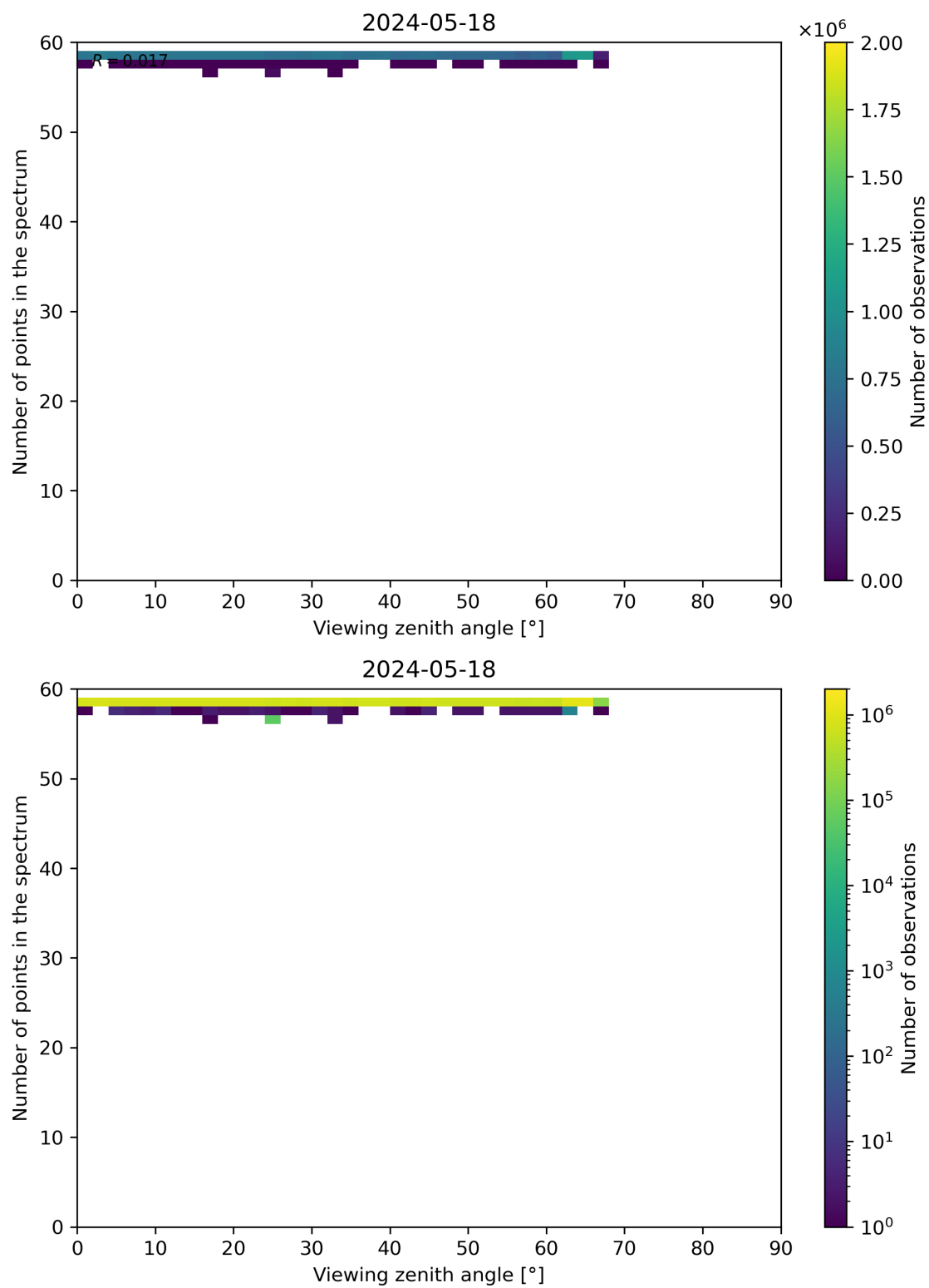
Figure 125: Scatter density plot of “Viewing zenith angle” against “Number of points in the spectrum” for 2024-05-18 to 2024-05-19.
