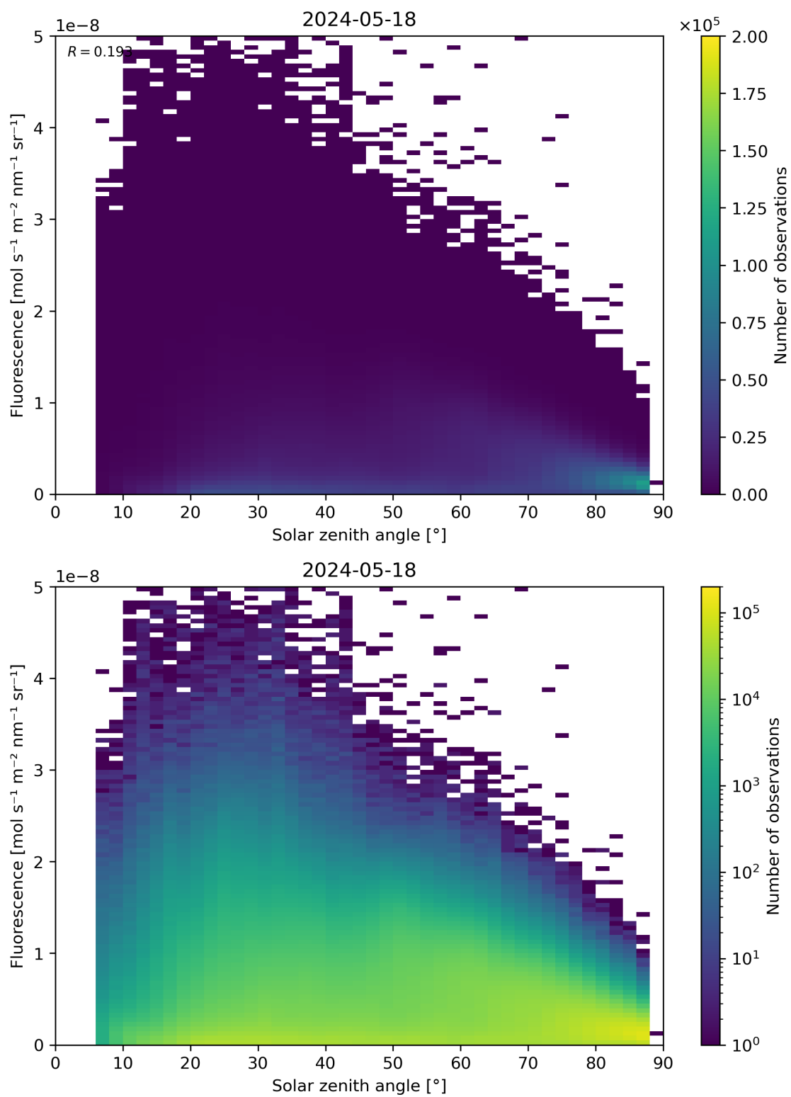
Figure 112: Scatter density plot of “Solar zenith angle” against “Fluorescence” for 2024-05-18 to 2024-05-19.
