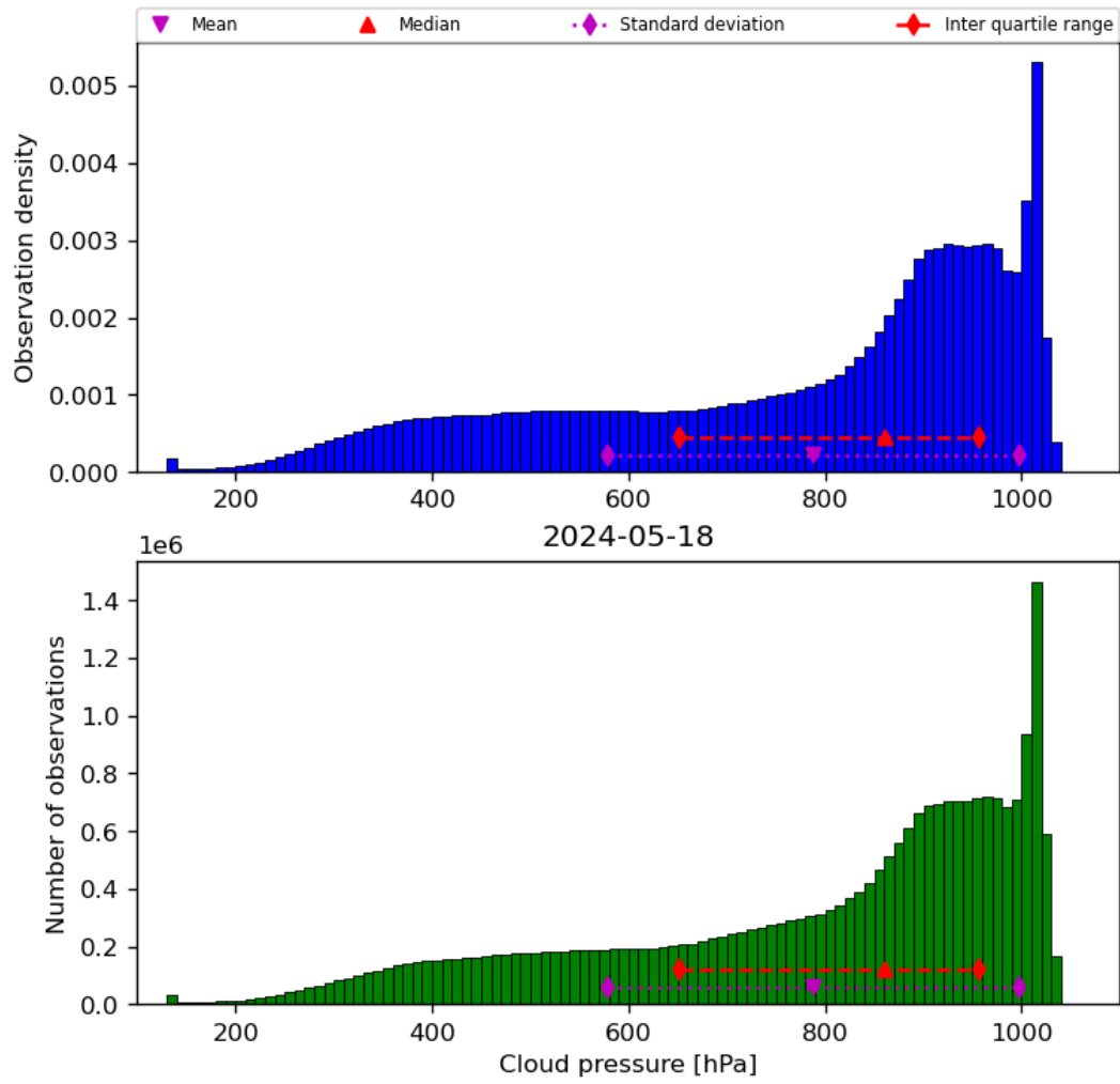
Figure 30: Histogram of “Cloud pressure” for 2024-05-18 to 2024-05-19
