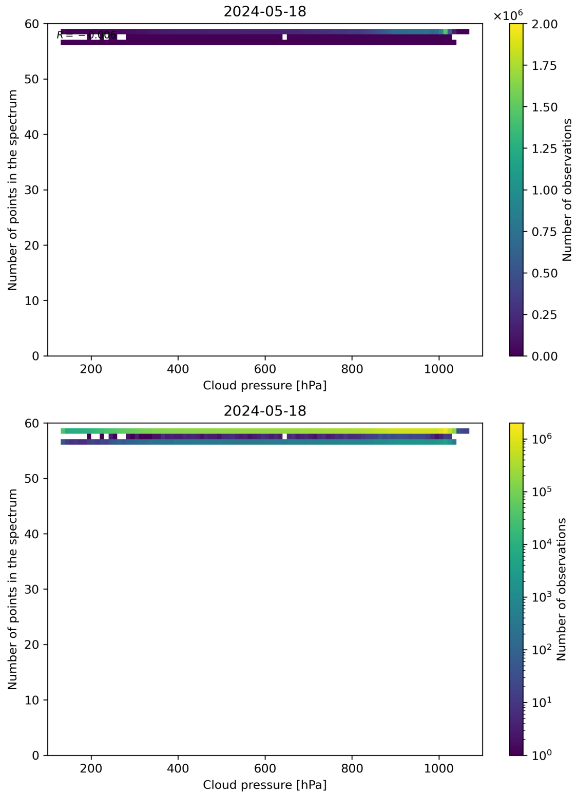
Figure 82: Scatter density plot of “Cloud pressure” against “Number of points in the spectrum” for 2024-05-18 to 2024-05-19.
