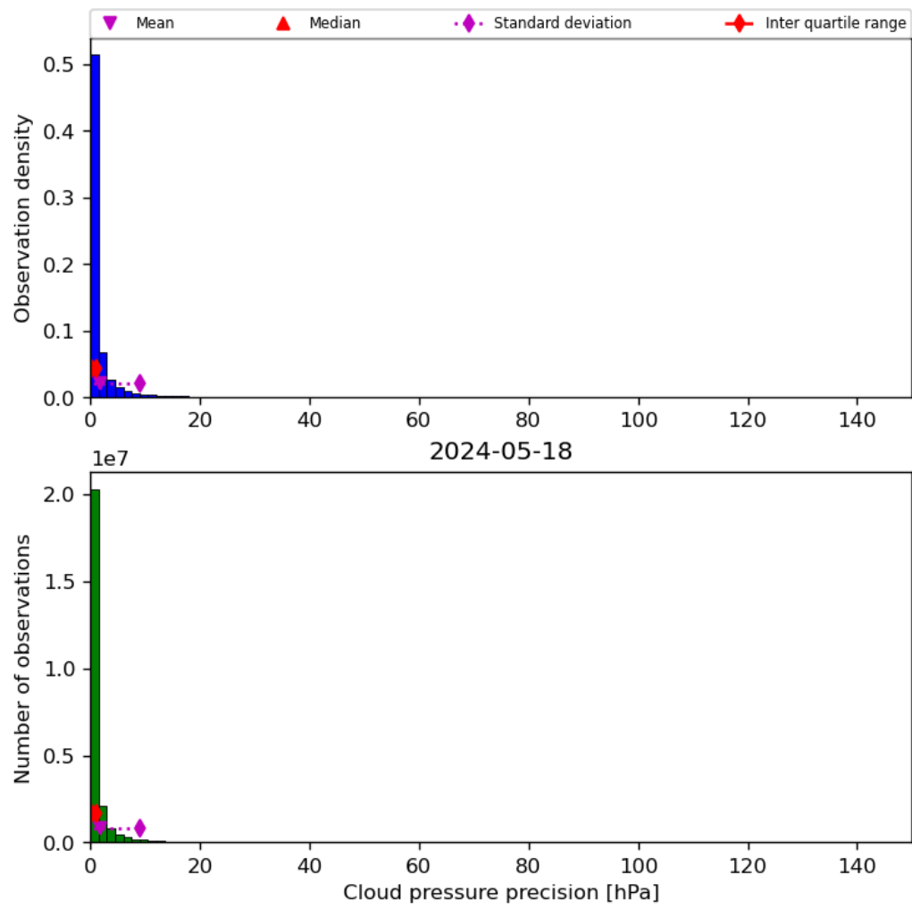
Figure 31: Histogram of “Cloud pressure precision” for 2024-05-18 to 2024-05-19
