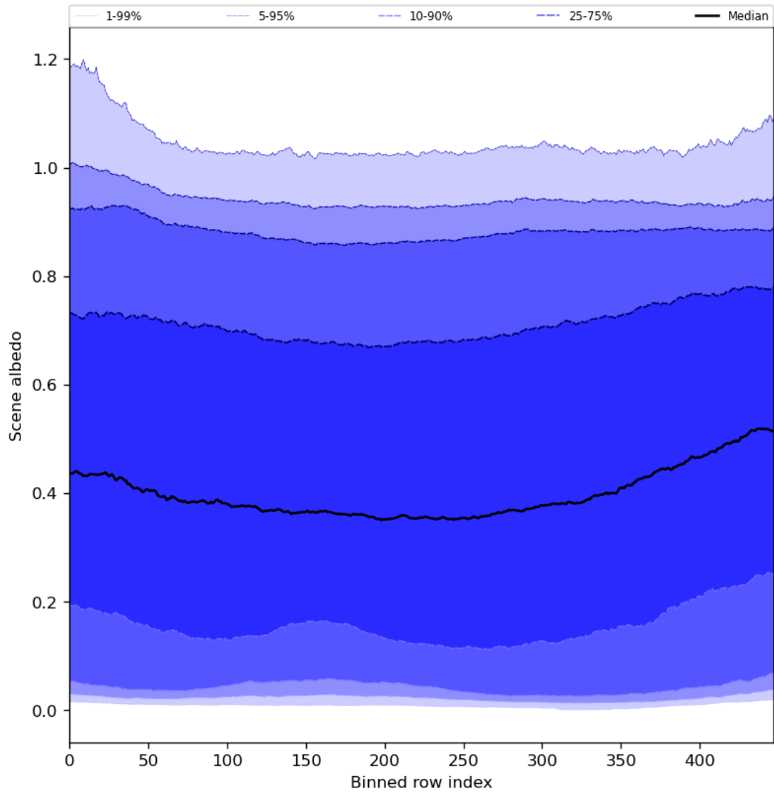
Figure 51: Along track statistics of “Scene albedo” for 2024-05-18 to 2024-05-19
