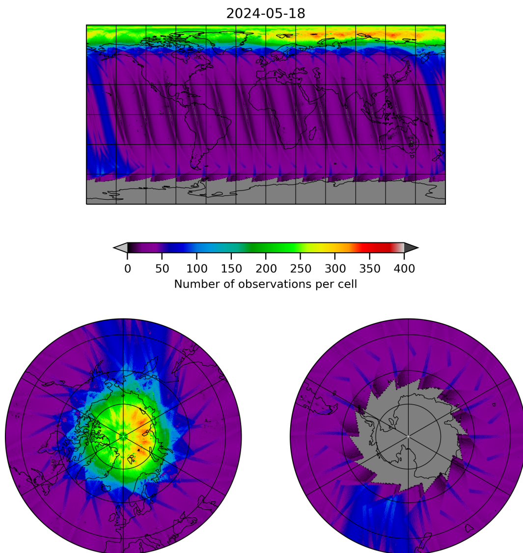
Figure 11: Map of the number of observations for 2024-05-18 to 2024-05-19
