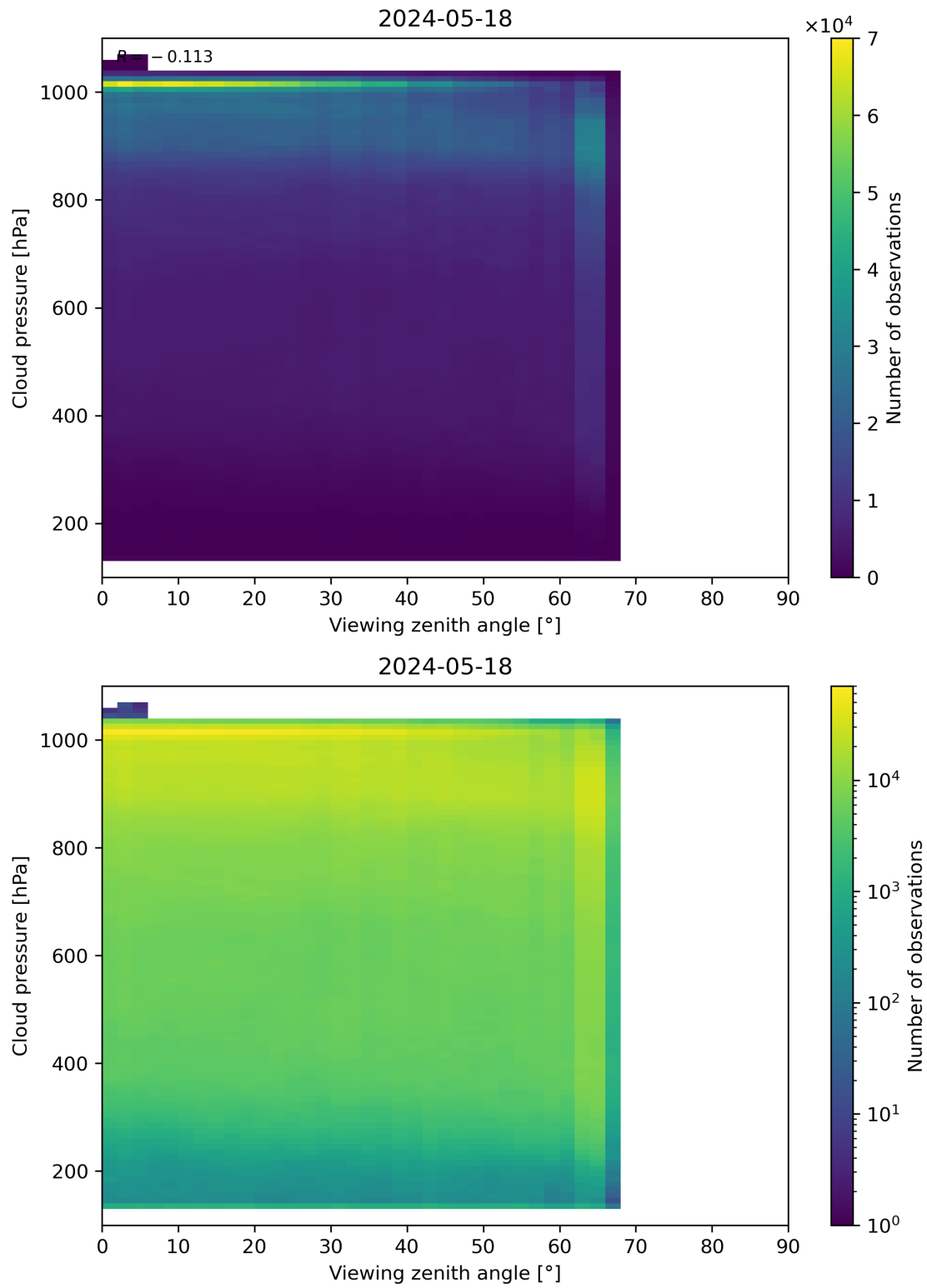
Figure 121: Scatter density plot of “Viewing zenith angle” against “Cloud pressure” for 2024-05-18 to 2024-05-19.
