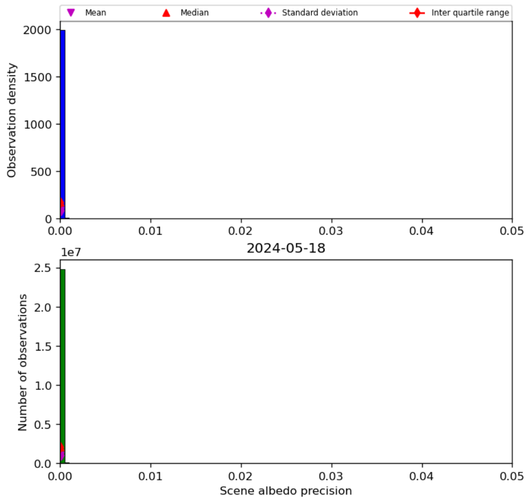
Figure 35: Histogram of “Scene albedo precision” for 2024-05-18 to 2024-05-19
