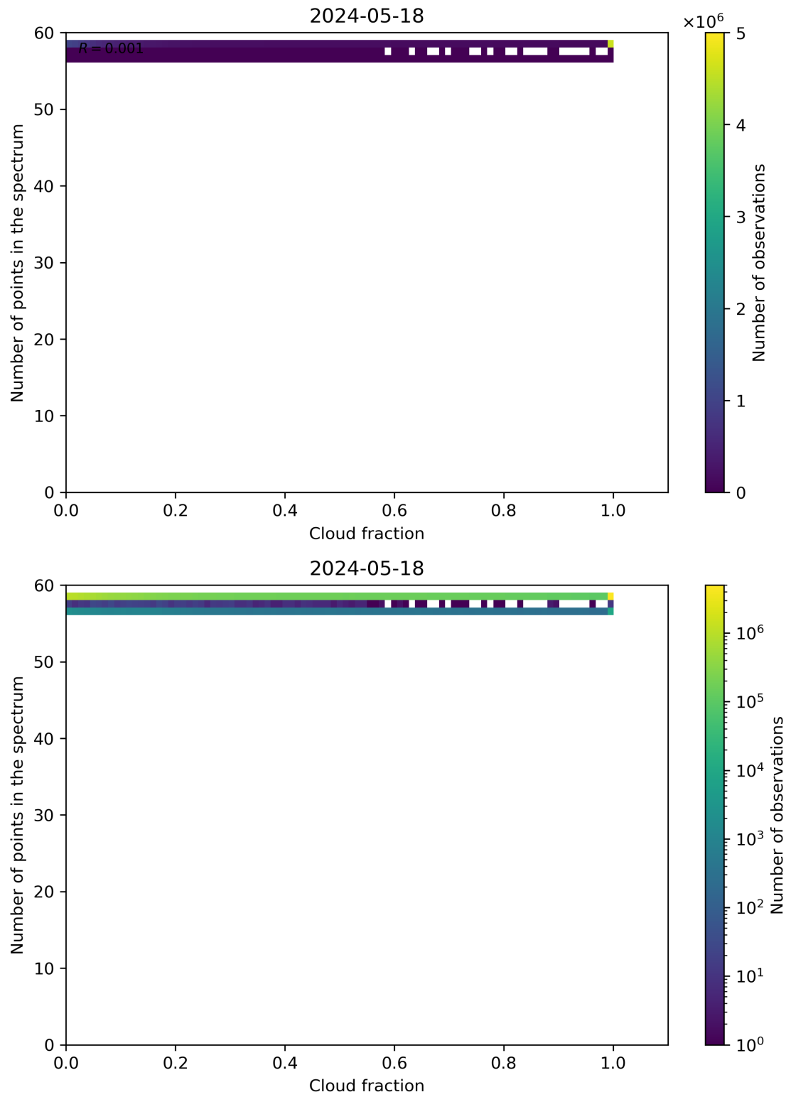
Figure 74: Scatter density plot of “Cloud fraction” against “Number of points in the spectrum” for 2024-05-18 to 2024-05-19.
