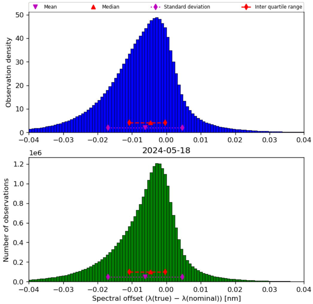
Figure 45: Histogram of “Spectral offset ( \lambda(\text{true}) - \lambda(\text{nominal}) )” for 2024-05-18 to 2024-05-19
