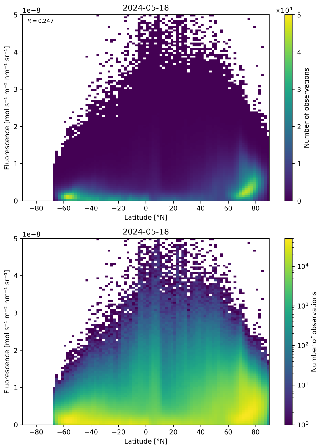
Figure 92: Scatter density plot of “Latitude” against “Fluorescence” for 2024-05-18 to 2024-05-19.
