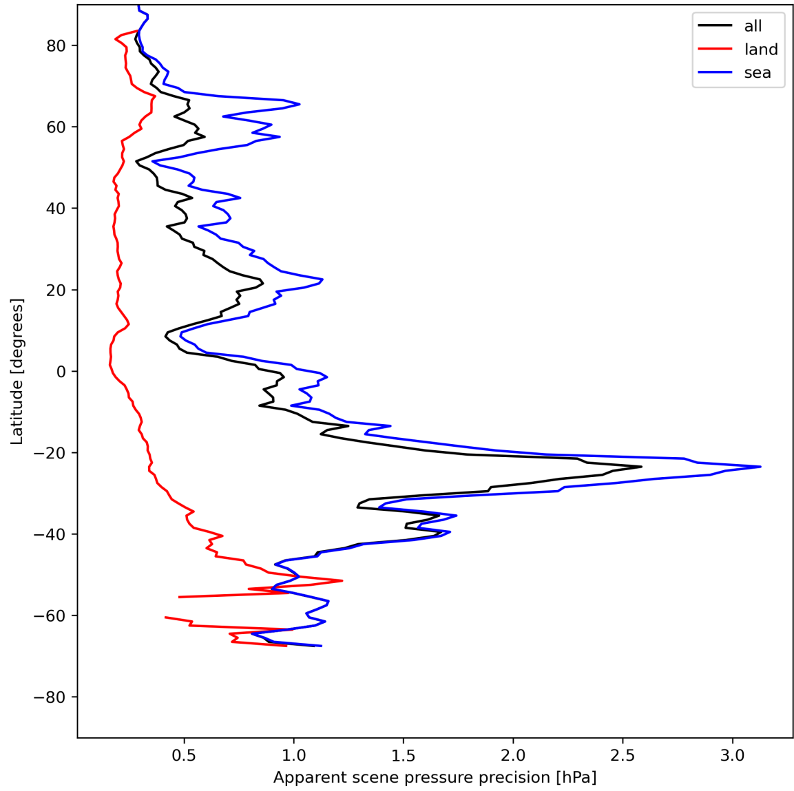
Figure 20: Zonal average of “Apparent scene pressure precision” for 2024-05-18 to 2024-05-19.
