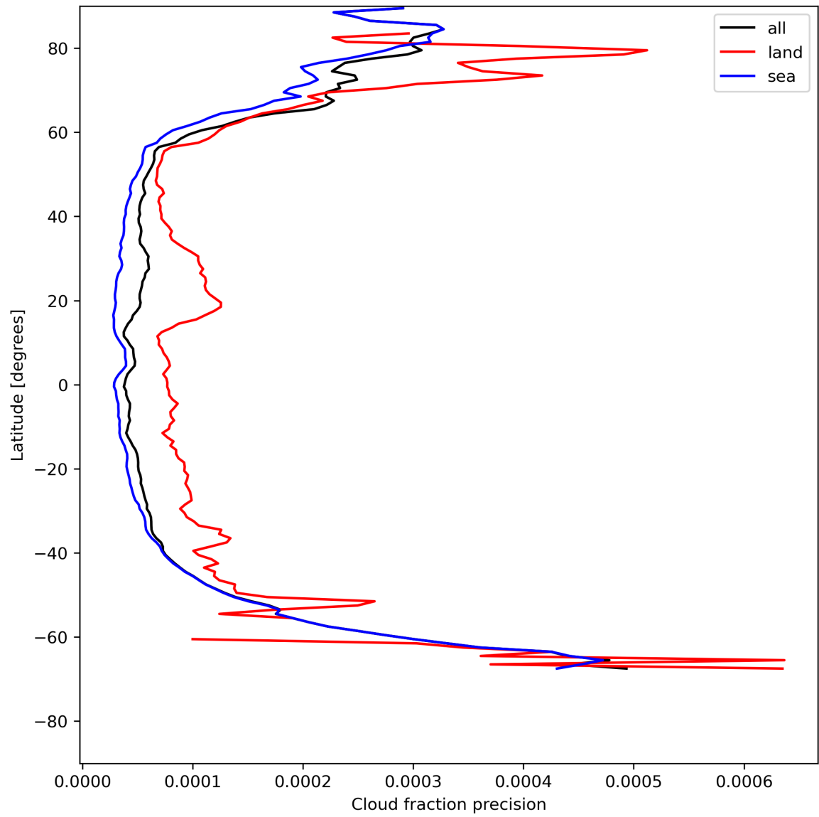
Figure 16: Zonal average of “Cloud fraction precision” for 2024-05-18 to 2024-05-19.
