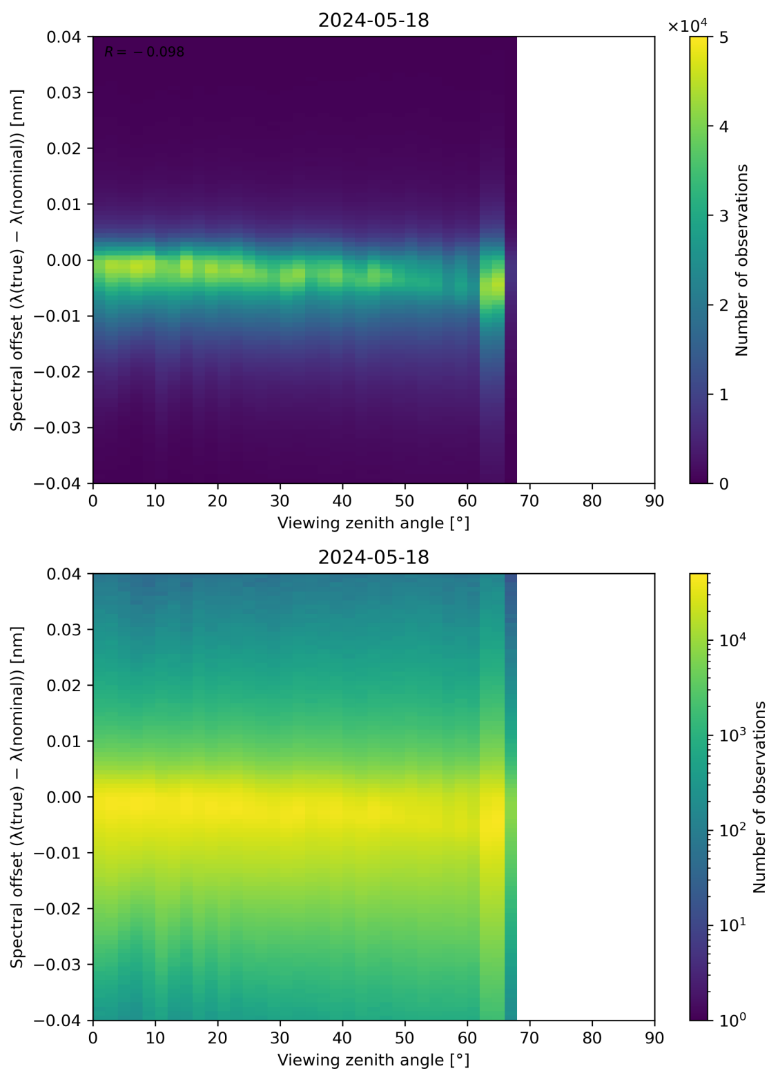
Figure 128: Scatter density plot of “Viewing zenith angle” against “Spectral offset ( \lambda(\text{true}) - \lambda(\text{nominal}) )” for 2024-05-18 to 2024-05-19.
