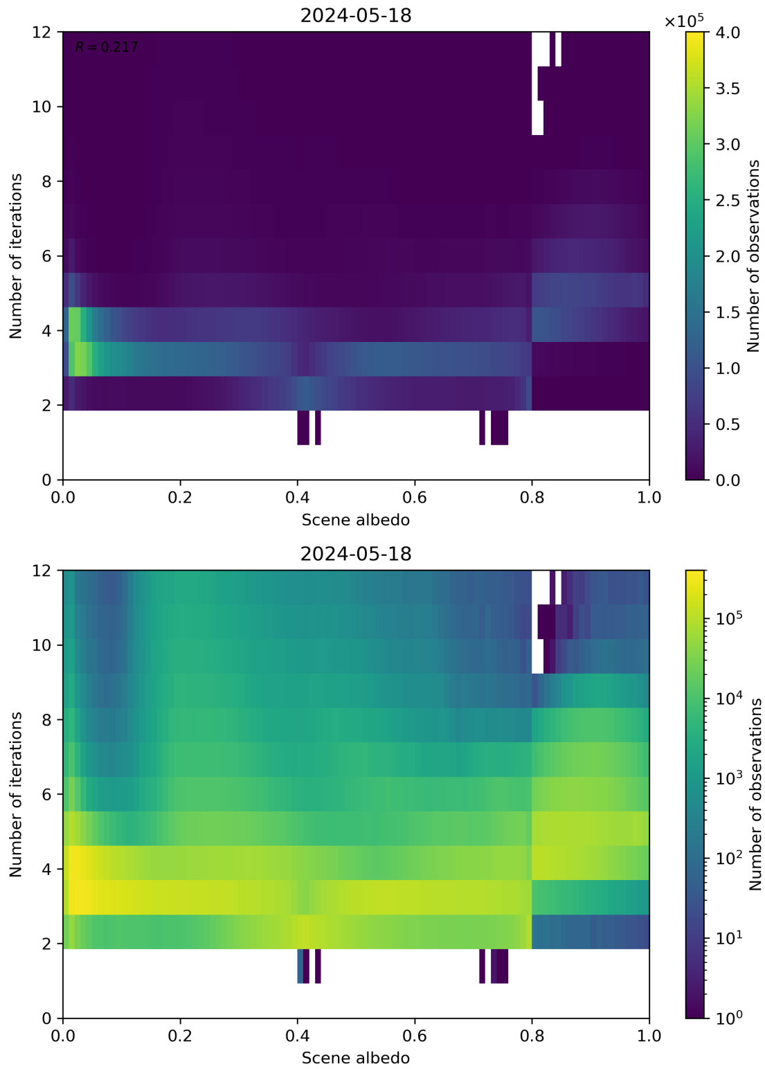
Figure 105: Scatter density plot of “Scene albedo” against “Number of iterations” for 2024-05-18 to 2024-05-19.
