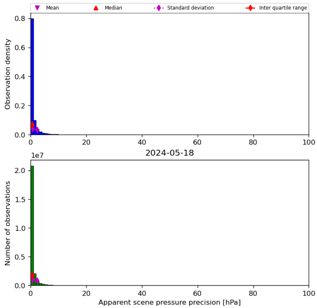
Figure 37: Histogram of “Apparent scene pressure precision” for 2024-05-18 to 2024-05-19
