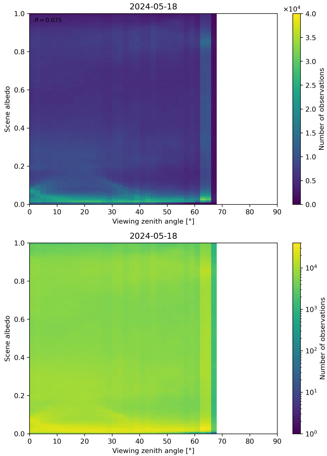
Figure 126: Scatter density plot of “Viewing zenith angle” against “Scene albedo” for 2024-05-18 to 2024-05-19.
