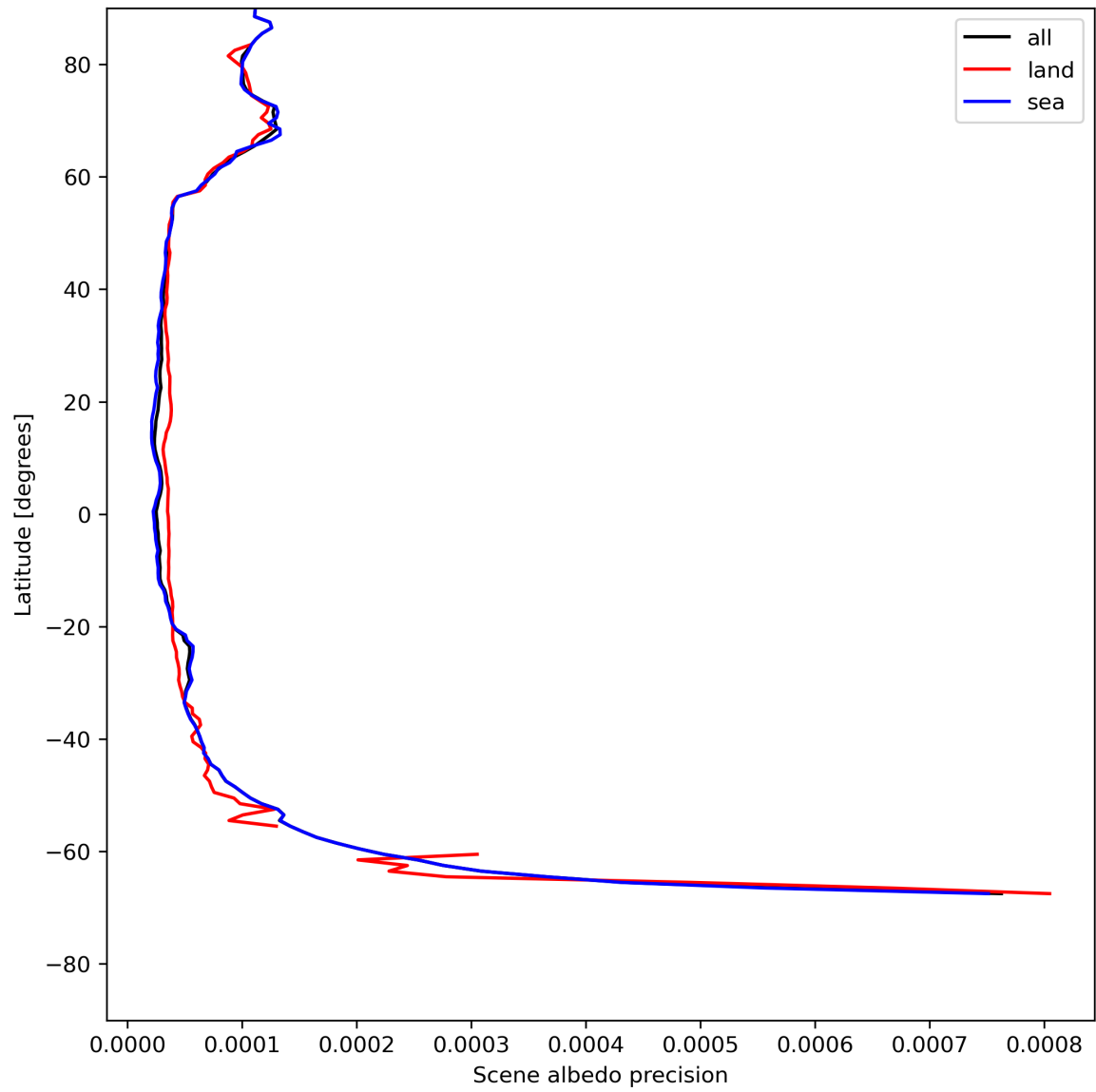
Figure 18: Zonal average of “Scene albedo precision” for 2024-05-18 to 2024-05-19.
