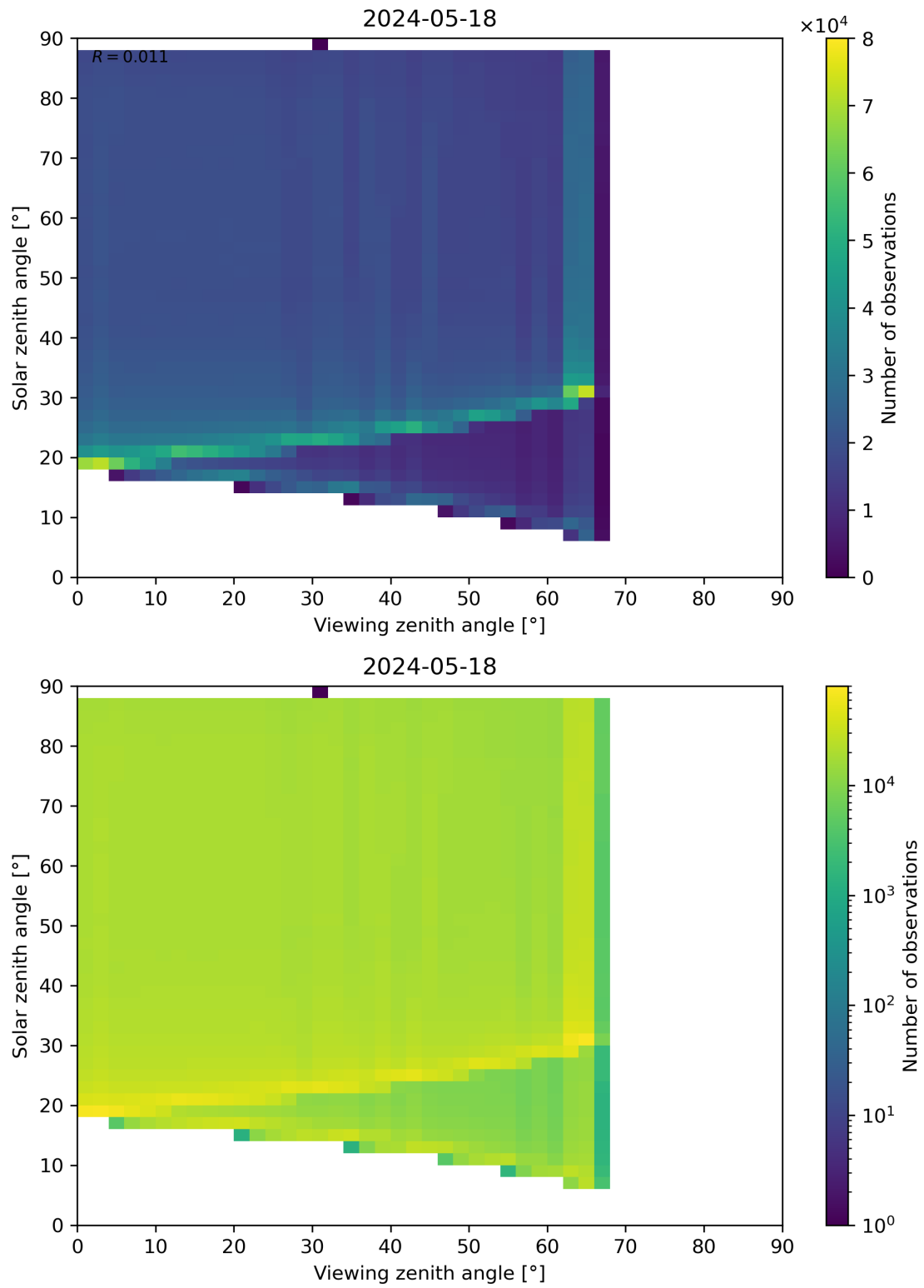
Figure 127: Scatter density plot of “Viewing zenith angle” against “Solar zenith angle” for 2024-05-18 to 2024-05-19.
