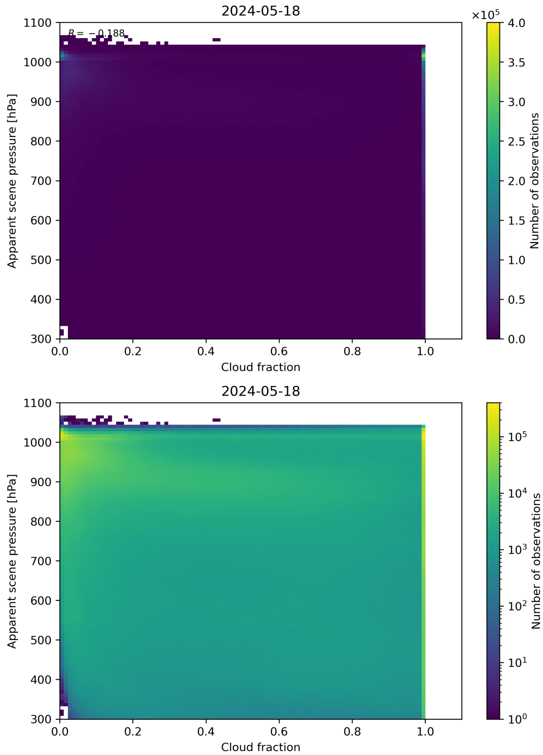
Figure 70: Scatter density plot of “Cloud fraction” against “Apparent scene pressure” for 2024-05-18 to 2024-05-19.
