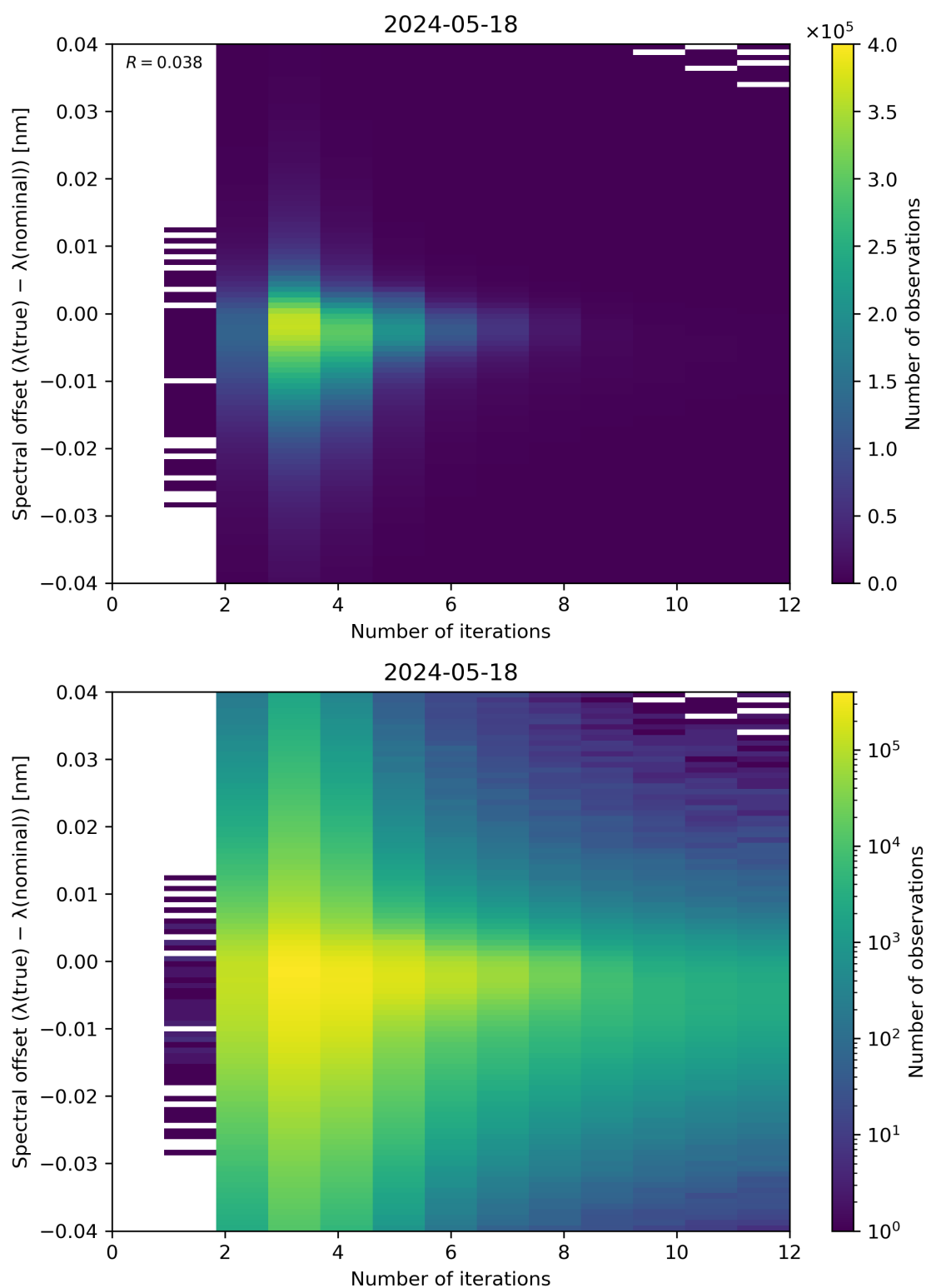
Figure 100: Scatter density plot of “Number of iterations” against “Spectral offset ( \lambda(\text{true}) - \lambda(\text{nominal}) )” for 2024-05-18 to 2024-05-19.
