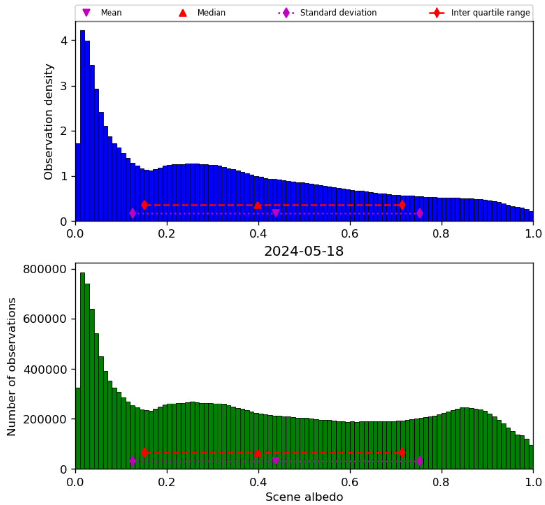
Figure 34: Histogram of “Scene albedo” for 2024-05-18 to 2024-05-19
