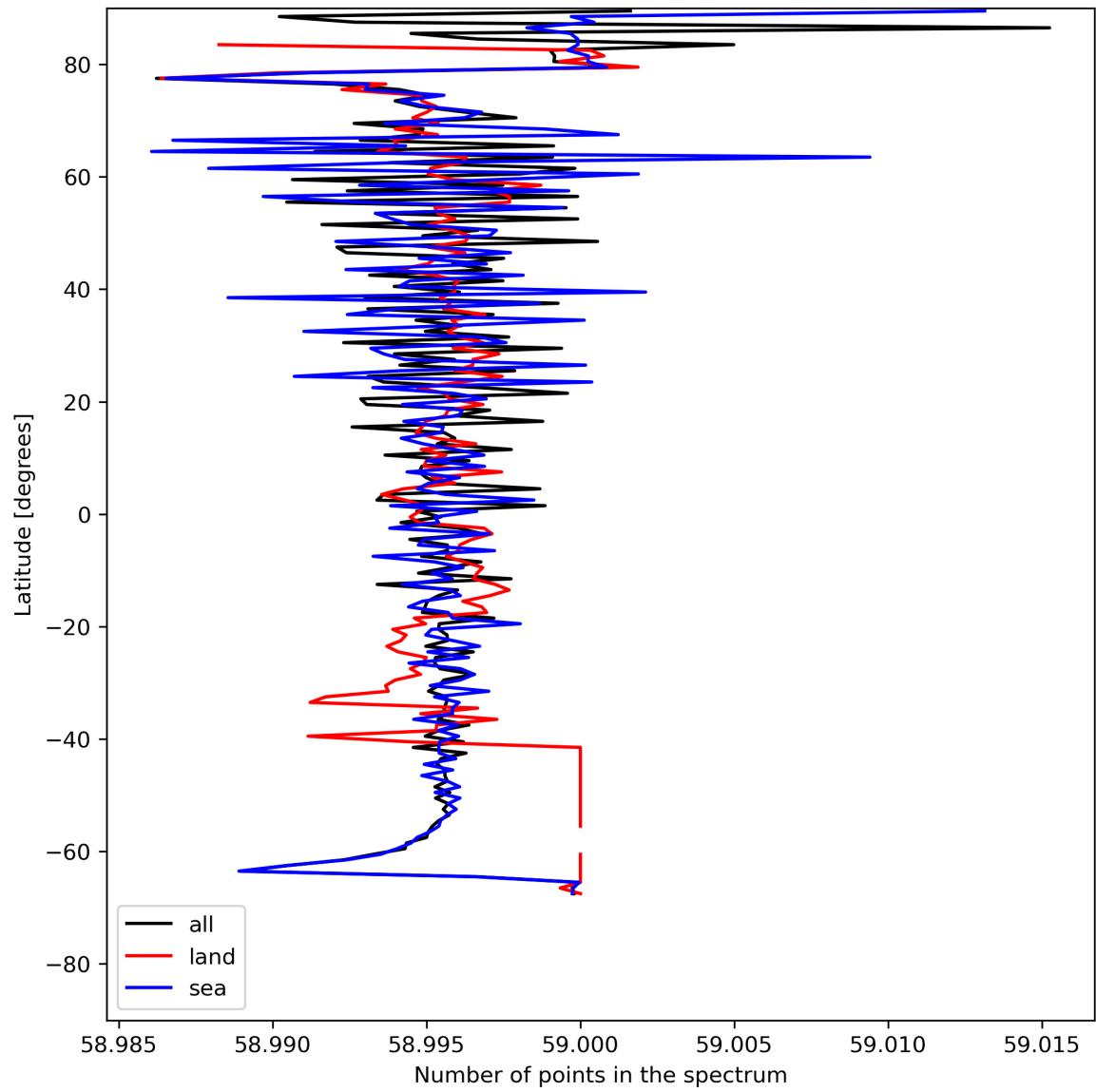
Figure 27: Zonal average of "Number of points in the spectrum" for 2024-05-18 to 2024-05-19.
