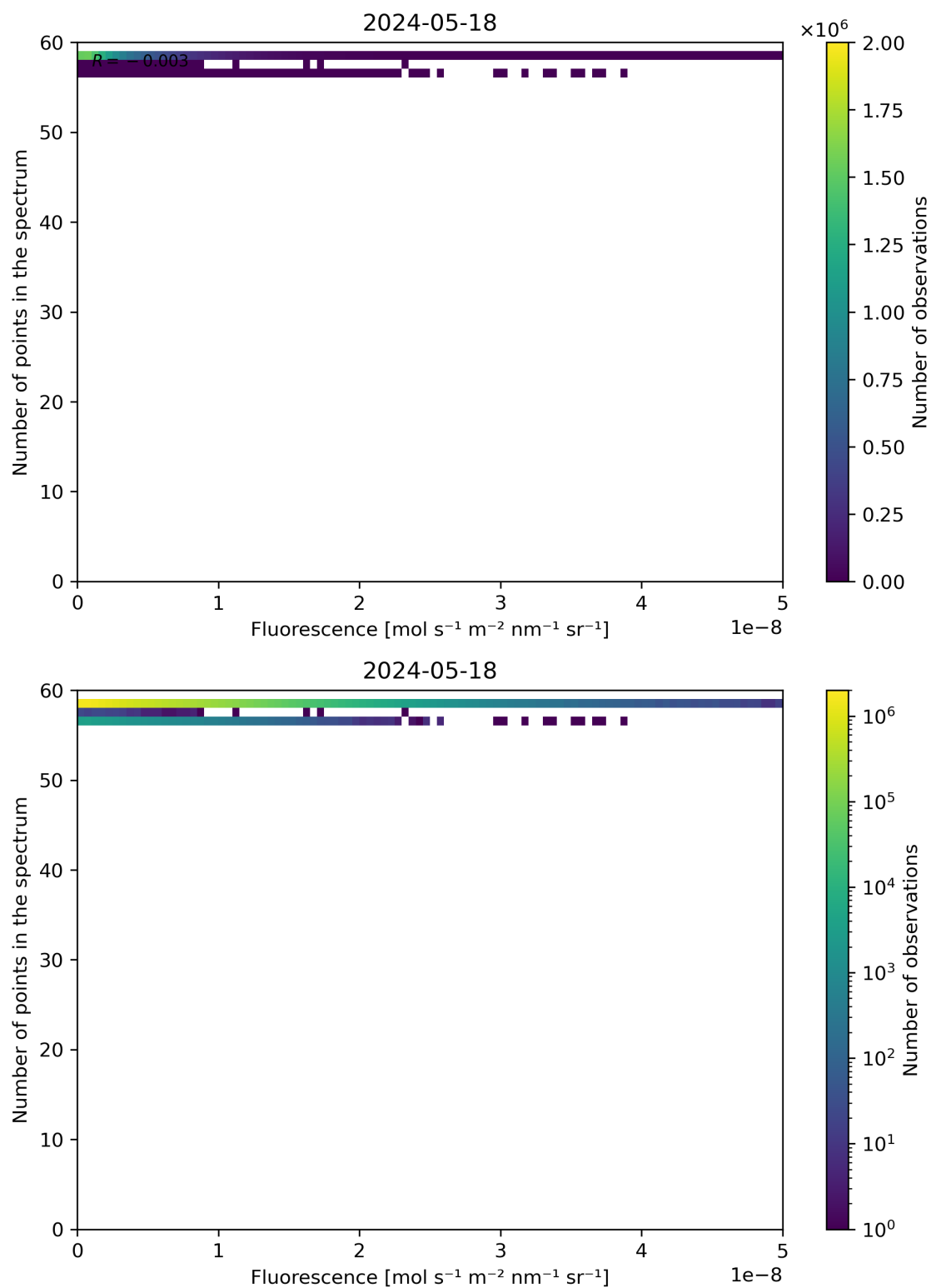
Figure 86: Scatter density plot of “Fluorescence” against “Number of points in the spectrum” for 2024-05-18 to 2024-05-19.
