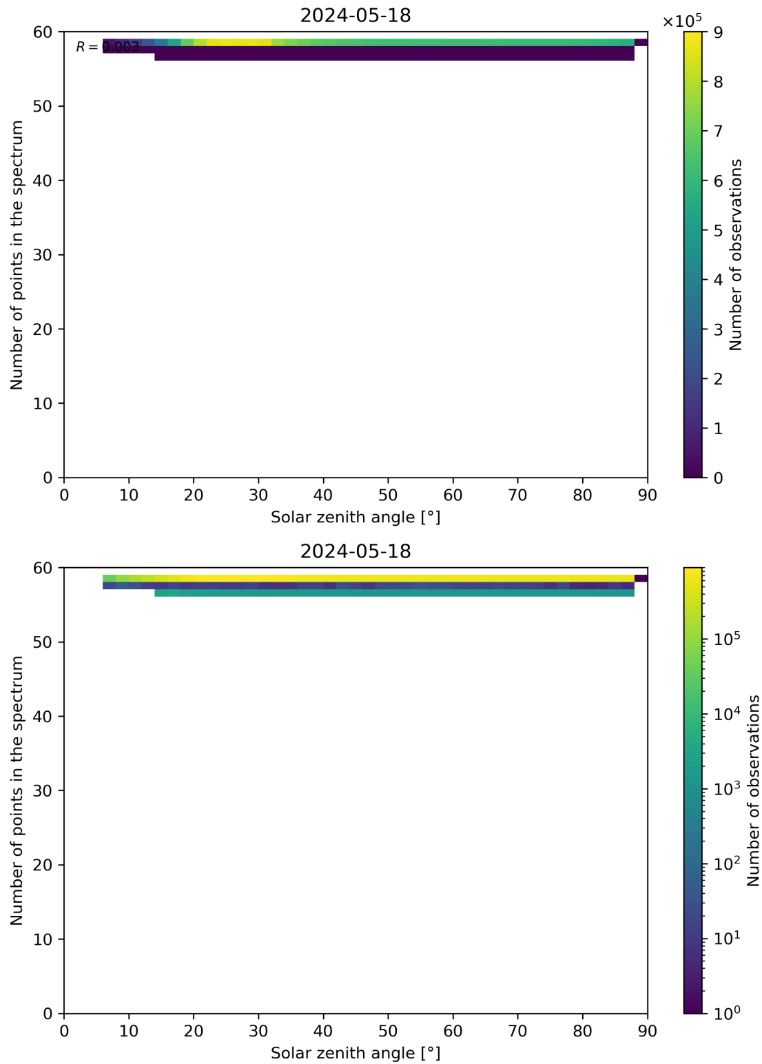
Figure 115: Scatter density plot of “Solar zenith angle” against “Number of points in the spectrum” for 2024-05-18 to 2024-05-19.
