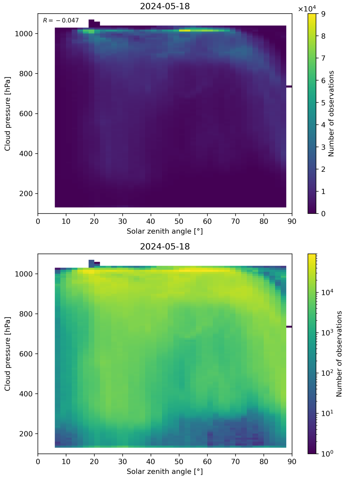
Figure 111: Scatter density plot of “Solar zenith angle” against “Cloud pressure” for 2024-05-18 to 2024-05-19.
