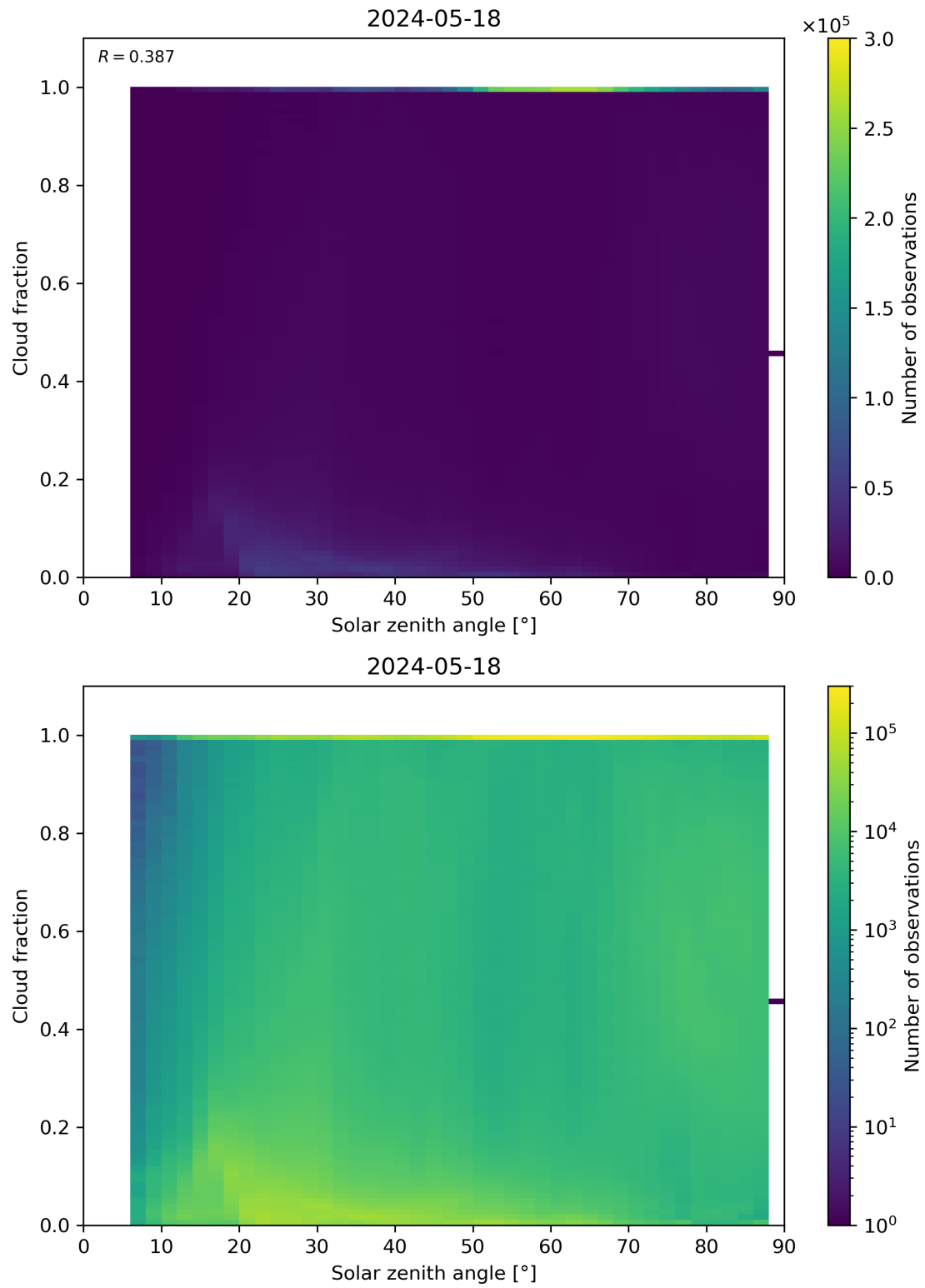
Figure 110: Scatter density plot of “Solar zenith angle” against “Cloud fraction” for 2024-05-18 to 2024-05-19.
