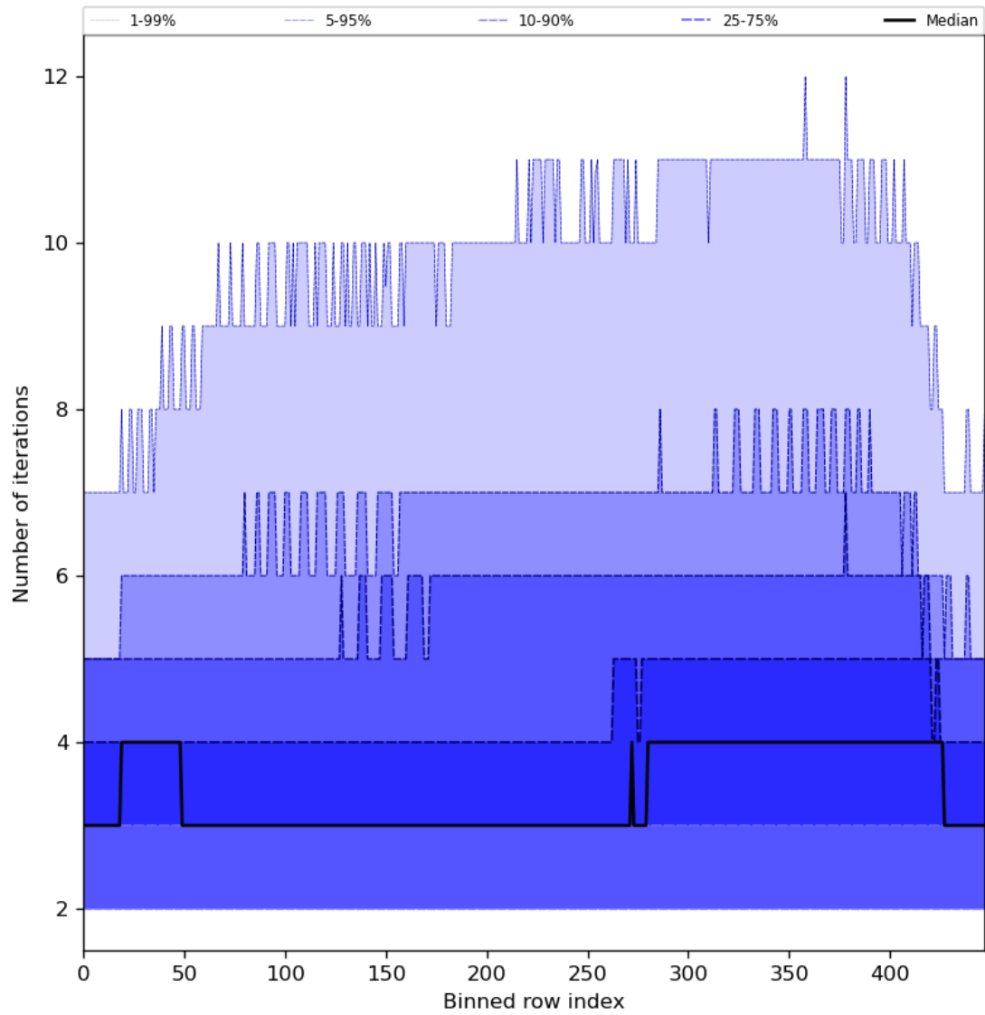
Figure 56: Along track statistics of “Number of iterations” for 2024-05-18 to 2024-05-19
