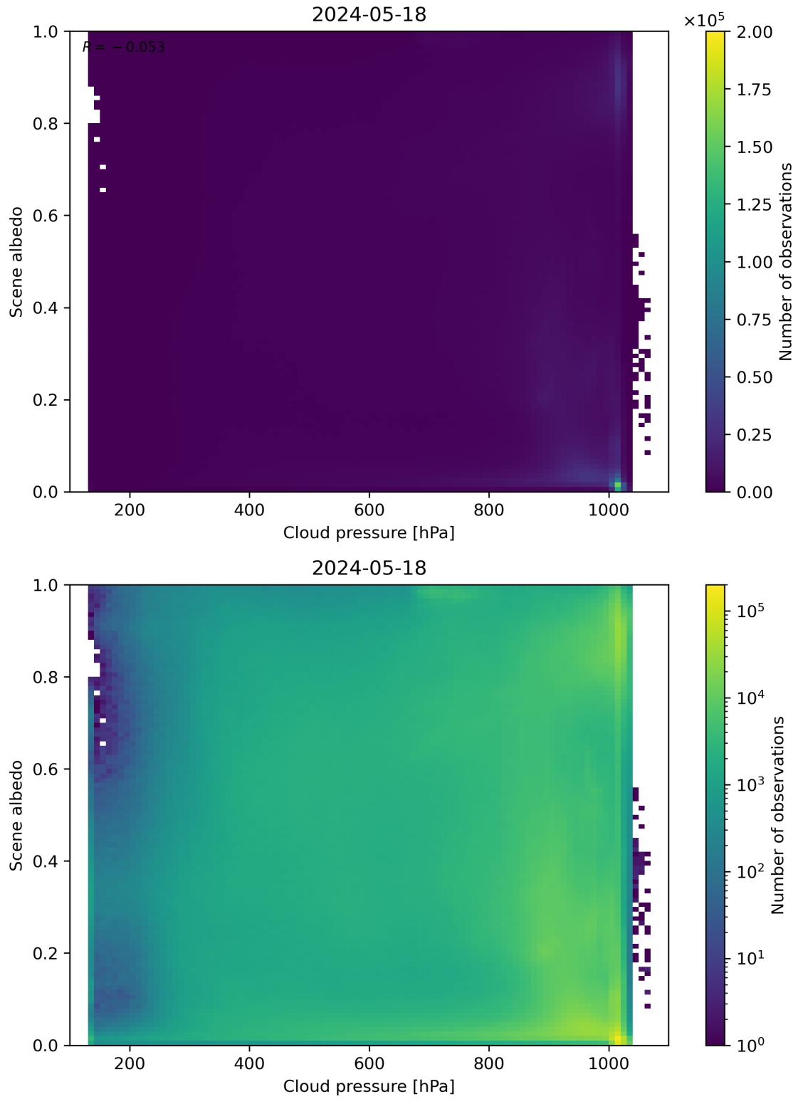
Figure 83: Scatter density plot of “Cloud pressure” against “Scene albedo” for 2024-05-18 to 2024-05-19.
