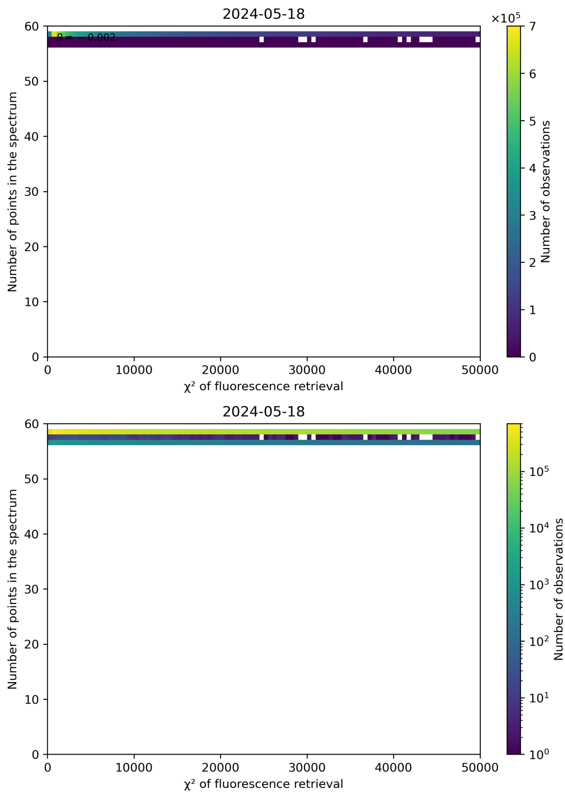
Figure 68: Scatter density plot of “ \chi^2 of fluorescence retrieval” against “Number of points in the spectrum” for 2024-05-18 to 2024-05-19.
