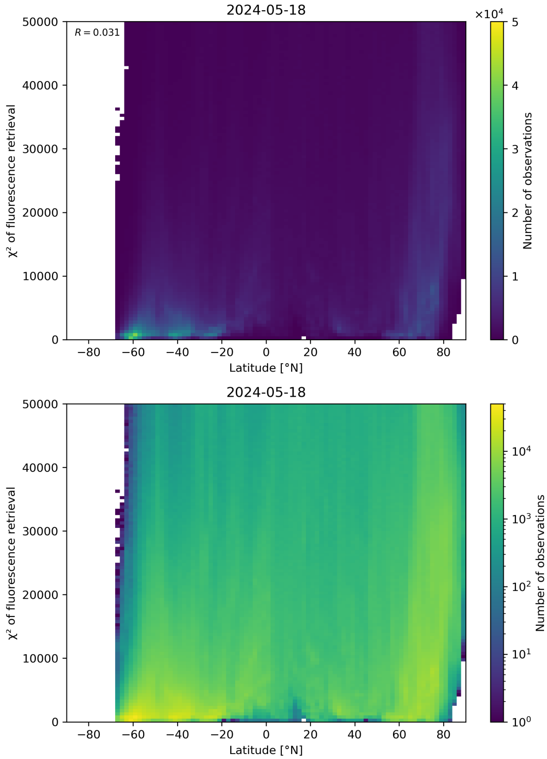
Figure 89: Scatter density plot of “Latitude” against “ \chi^2 of fluorescence retrieval” for 2024-05-18 to 2024-05-19.
