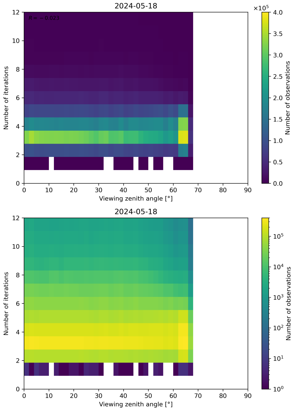
Figure 124: Scatter density plot of “Viewing zenith angle” against “Number of iterations” for 2024-05-18 to 2024-05-19.
