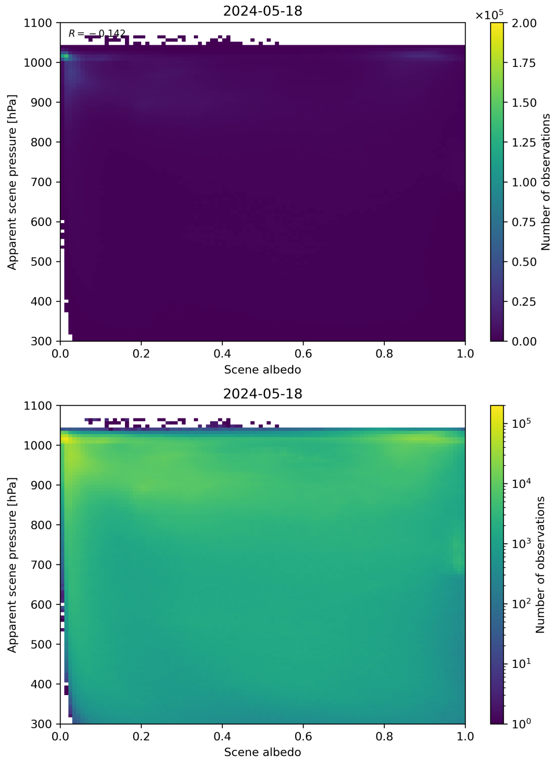
Figure 102: Scatter density plot of “Scene albedo” against “Apparent scene pressure” for 2024-05-18 to 2024-05-19.
