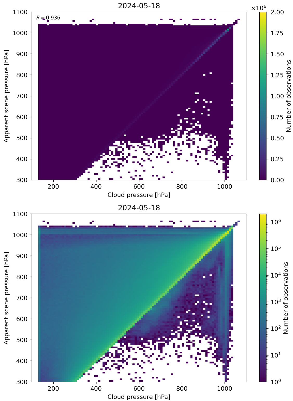
Figure 77: Scatter density plot of “Cloud pressure” against “Apparent scene pressure” for 2024-05-18 to 2024-05-19.
