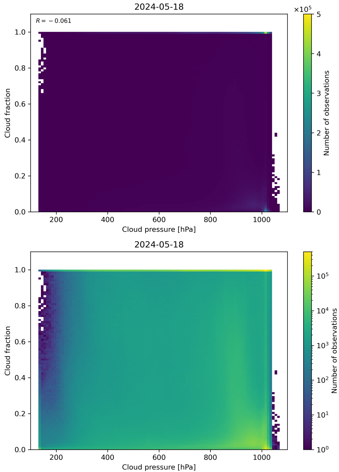
Figure 79: Scatter density plot of “Cloud pressure” against “Cloud fraction” for 2024-05-18 to 2024-05-19.
