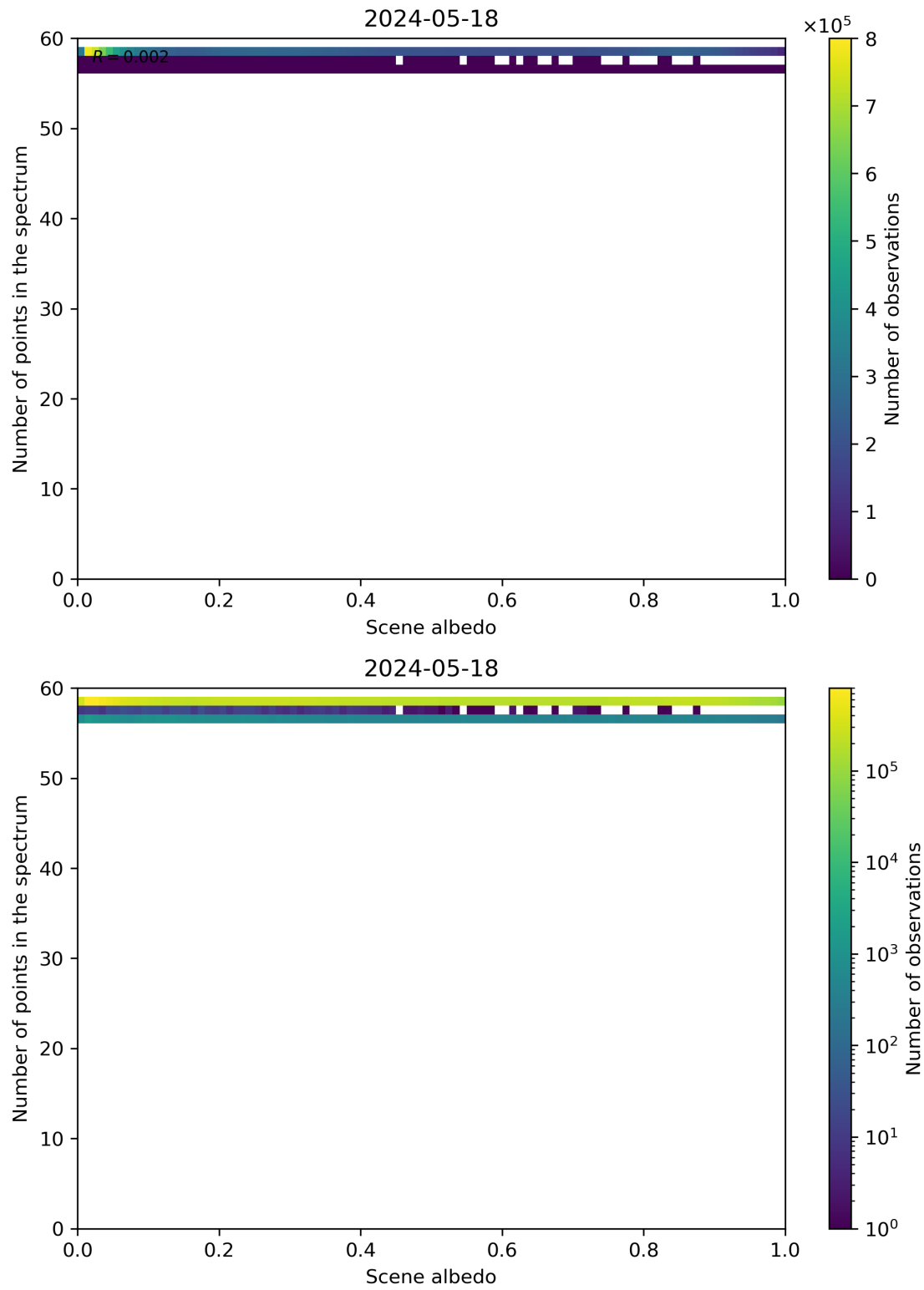
Figure 106: Scatter density plot of “Scene albedo” against “Number of points in the spectrum” for 2024-05-18 to 2024-05-19.
