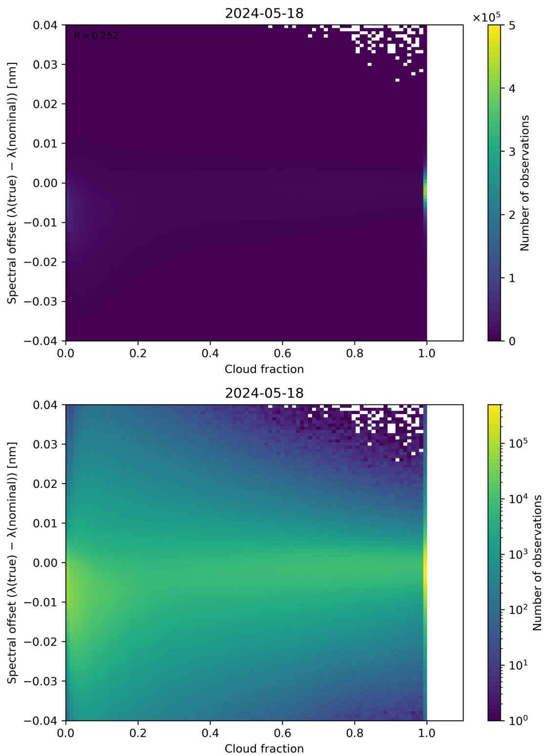
Figure 76: Scatter density plot of “Cloud fraction” against “Spectral offset ( \lambda(\text{true}) - \lambda(\text{nominal}) )” for 2024-05-18 to 2024-05-19.
