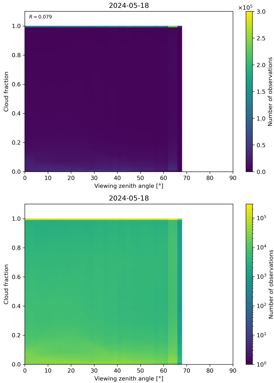
Figure 120: Scatter density plot of “Viewing zenith angle” against “Cloud fraction” for 2024-05-18 to 2024-05-19.
