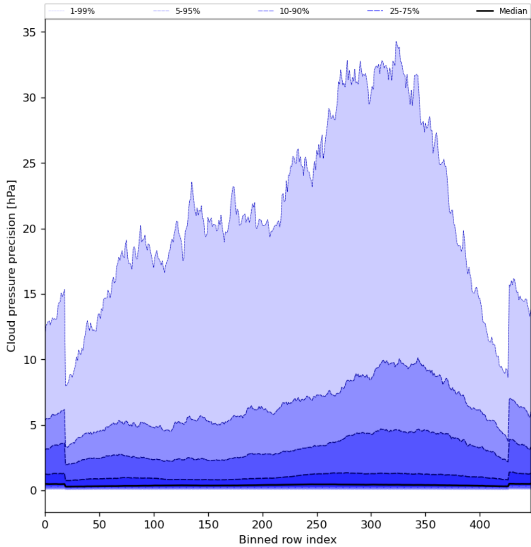
Figure 48: Along track statistics of “Cloud pressure precision” for 2024-05-18 to 2024-05-19
