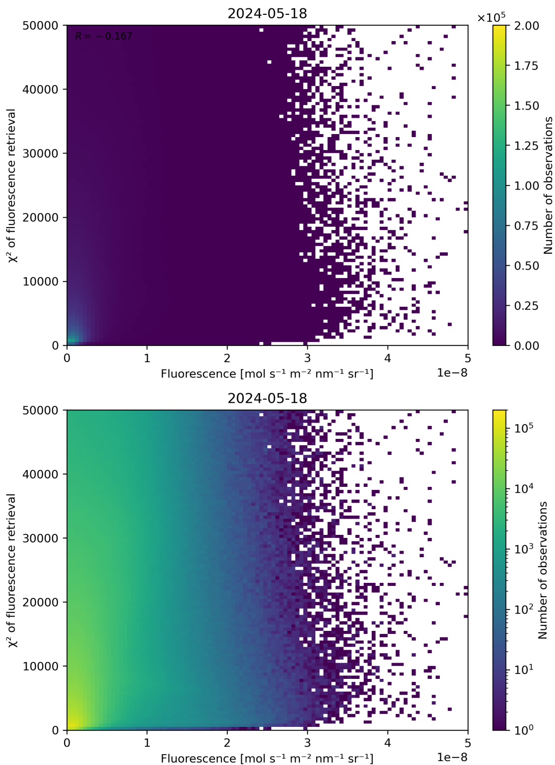
Figure 85: Scatter density plot of “Fluorescence” against “ \chi^2 of fluorescence retrieval” for 2024-05-18 to 2024-05-19.
