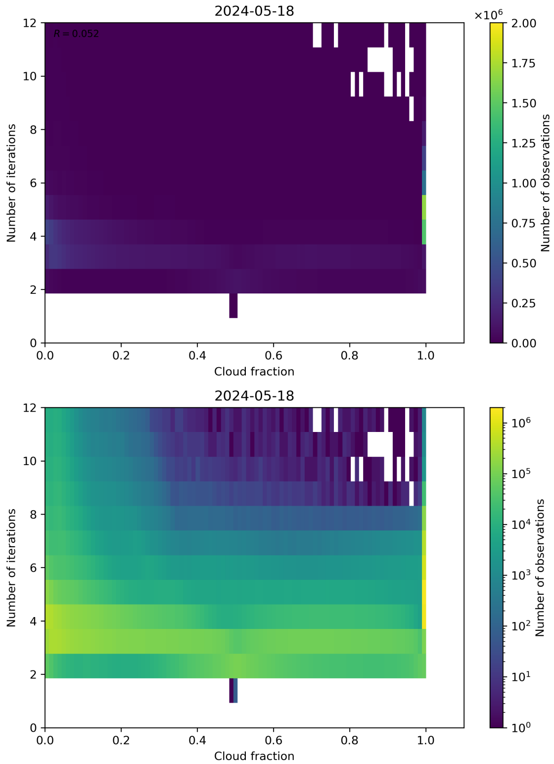
Figure 73: Scatter density plot of “Cloud fraction” against “Number of iterations” for 2024-05-18 to 2024-05-19.
