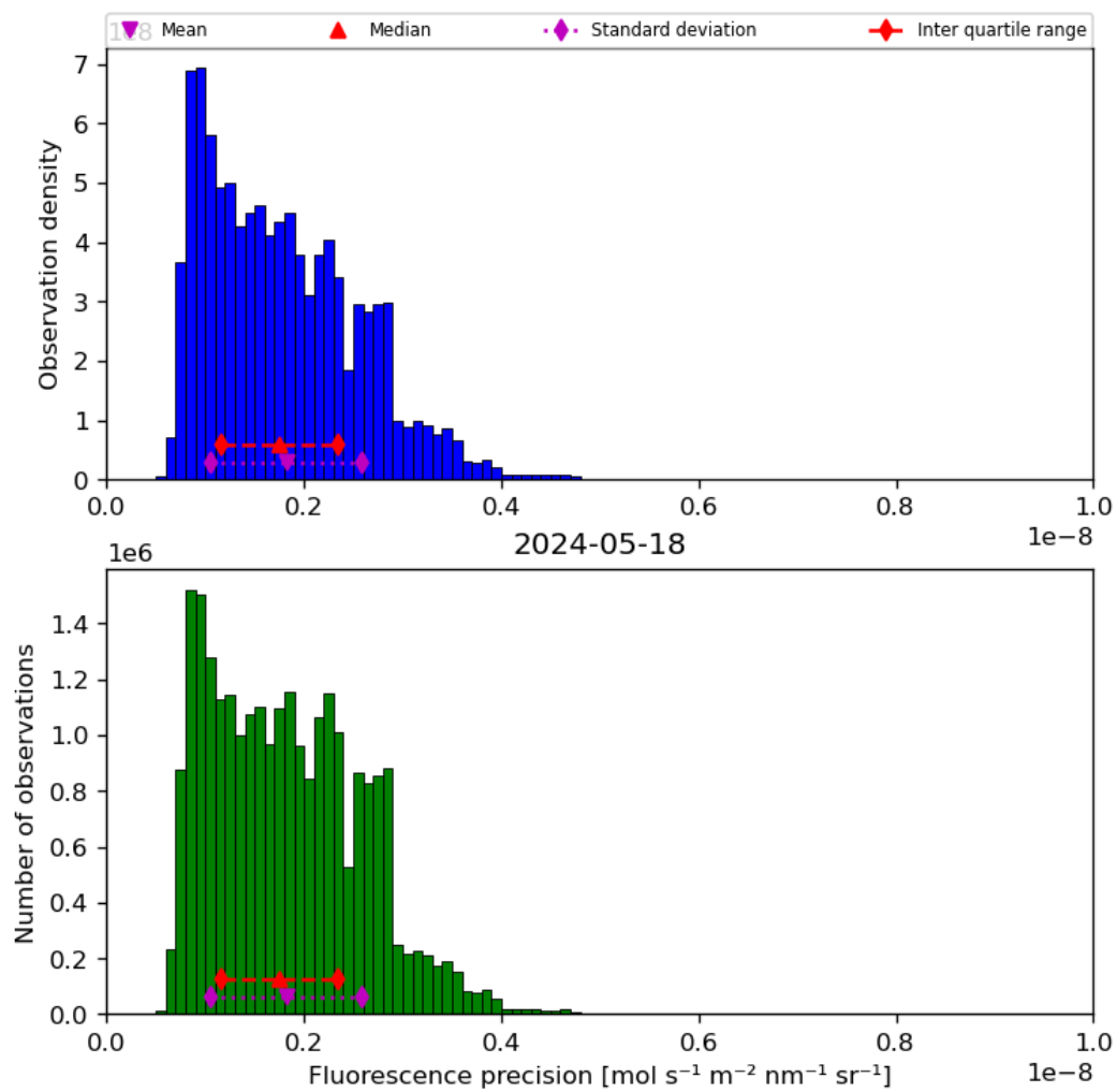
Figure 41: Histogram of “Fluorescence precision” for 2024-05-18 to 2024-05-19
