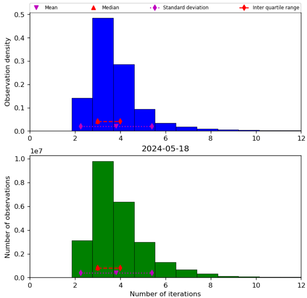
Figure 39: Histogram of “Number of iterations” for 2024-05-18 to 2024-05-19
