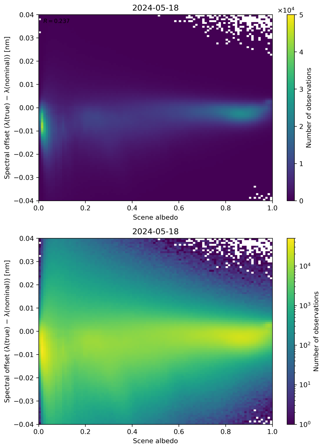
Figure 107: Scatter density plot of “Scene albedo” against “Spectral offset ( \lambda(\text{true}) - \lambda(\text{nominal}) )” for 2024-05-18 to 2024-05-19.
