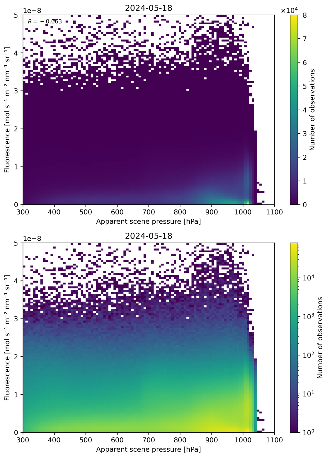
Figure 64: Scatter density plot of “Apparent scene pressure” against “Fluorescence” for 2024-05-18 to 2024-05-19.
