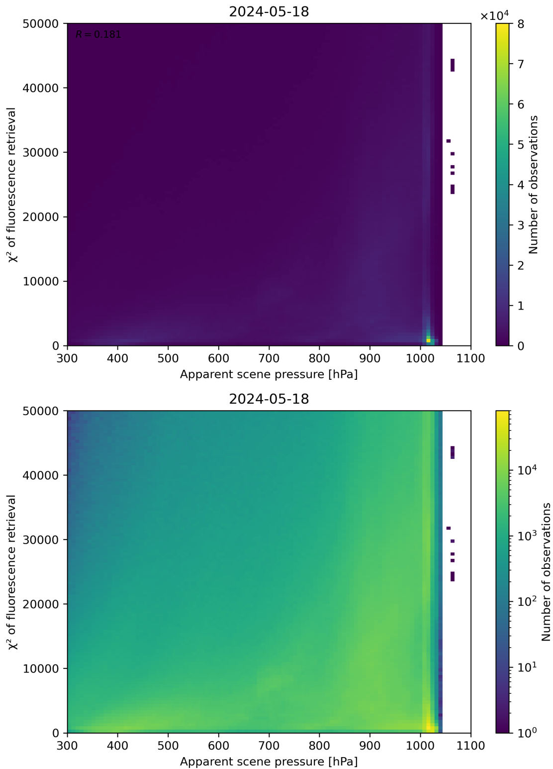
Figure 63: Scatter density plot of “Apparent scene pressure” against “ \chi^2 of fluorescence retrieval” for 2024-05-18 to 2024-05-19.
