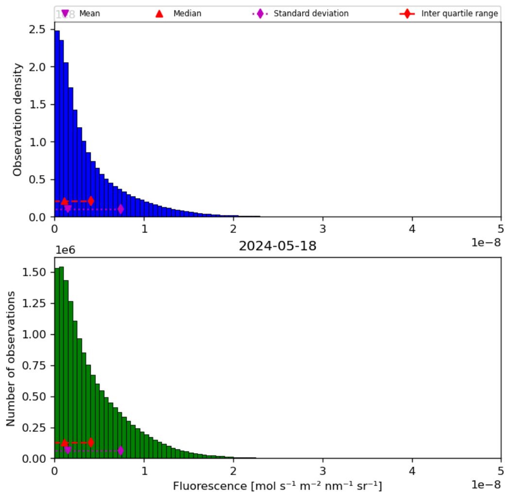
Figure 40: Histogram of “Fluorescence” for 2024-05-18 to 2024-05-19
