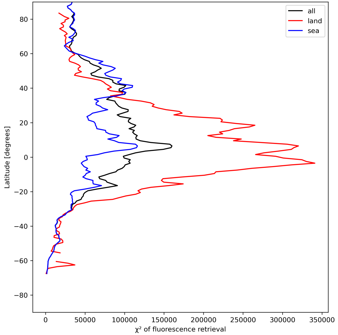
Figure 25: Zonal average of “ \chi^2 of fluorescence retrieval” for 2024-05-18 to 2024-05-19.
