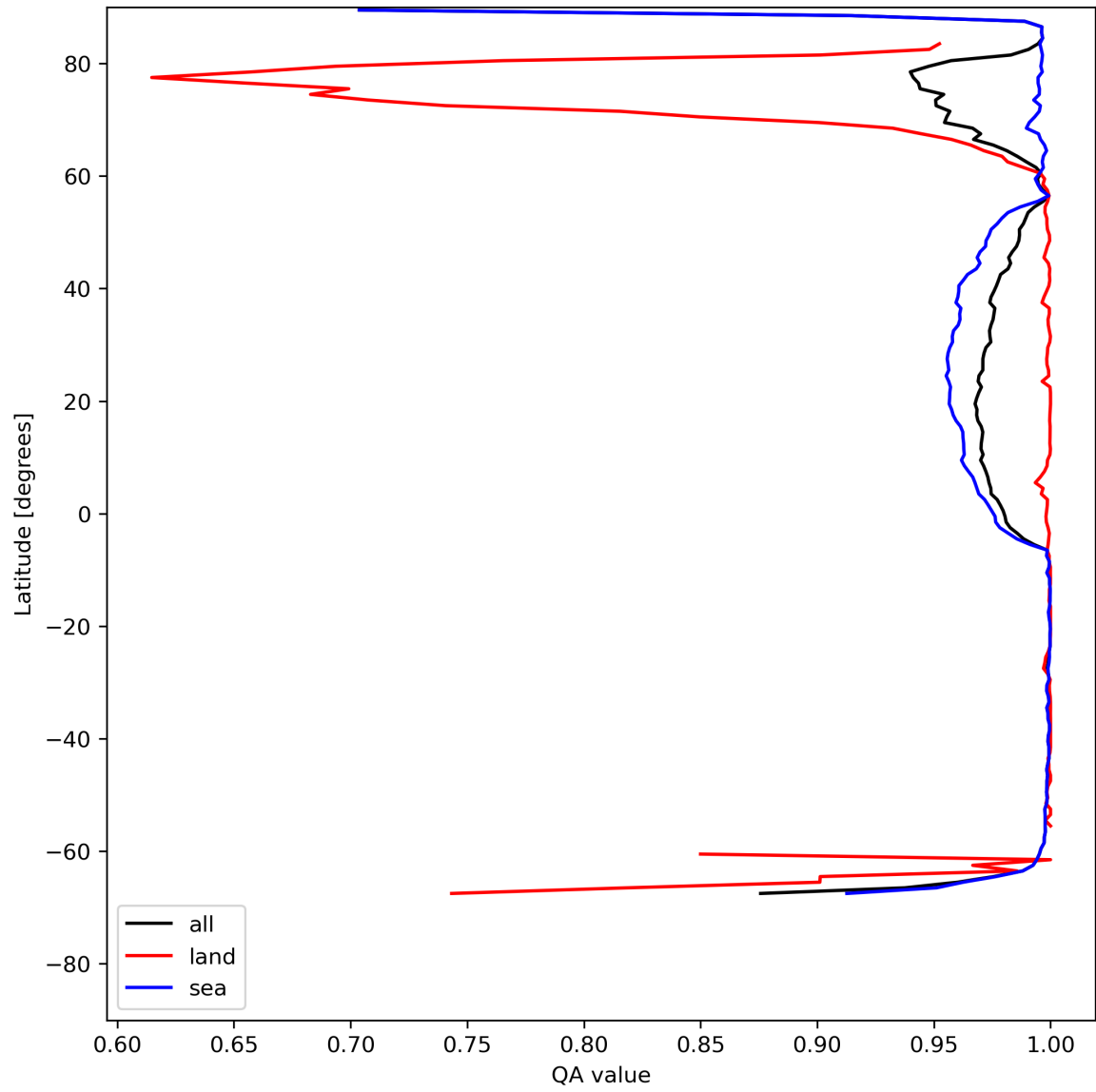
Figure 12: Zonal average of “QA value” for 2024-05-18 to 2024-05-19.
