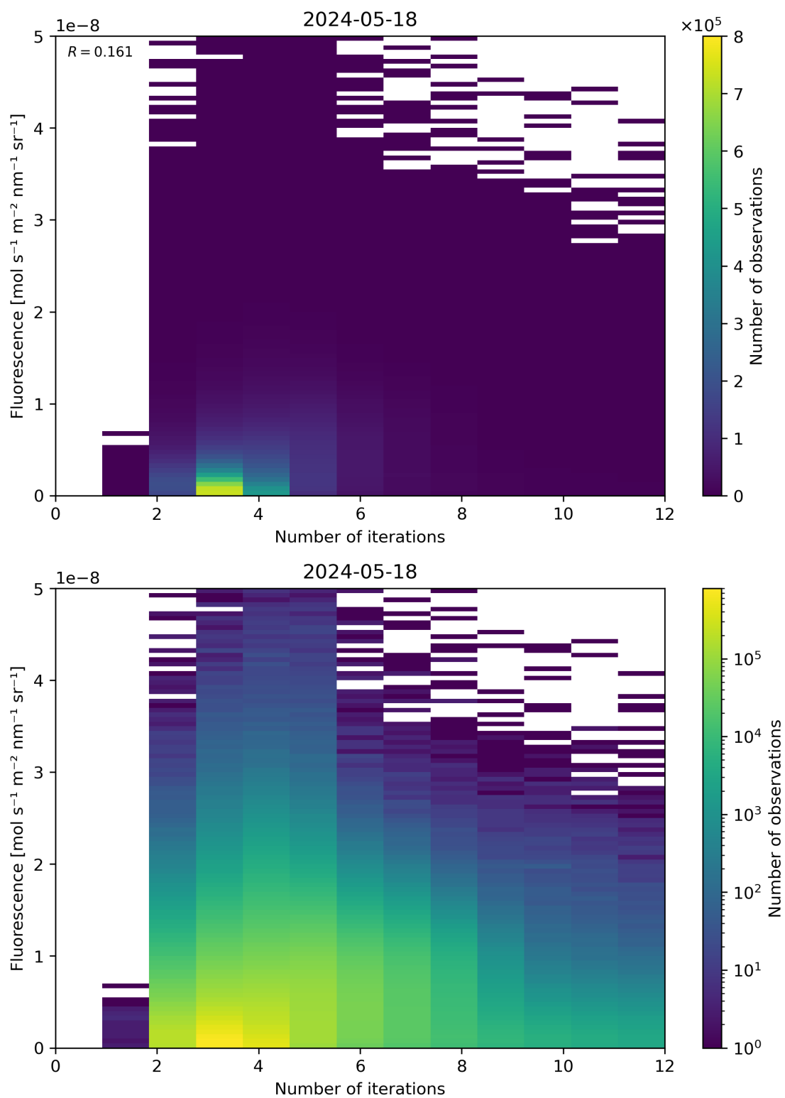
Figure 98: Scatter density plot of “Number of iterations” against “Fluorescence” for 2024-05-18 to 2024-05-19.
