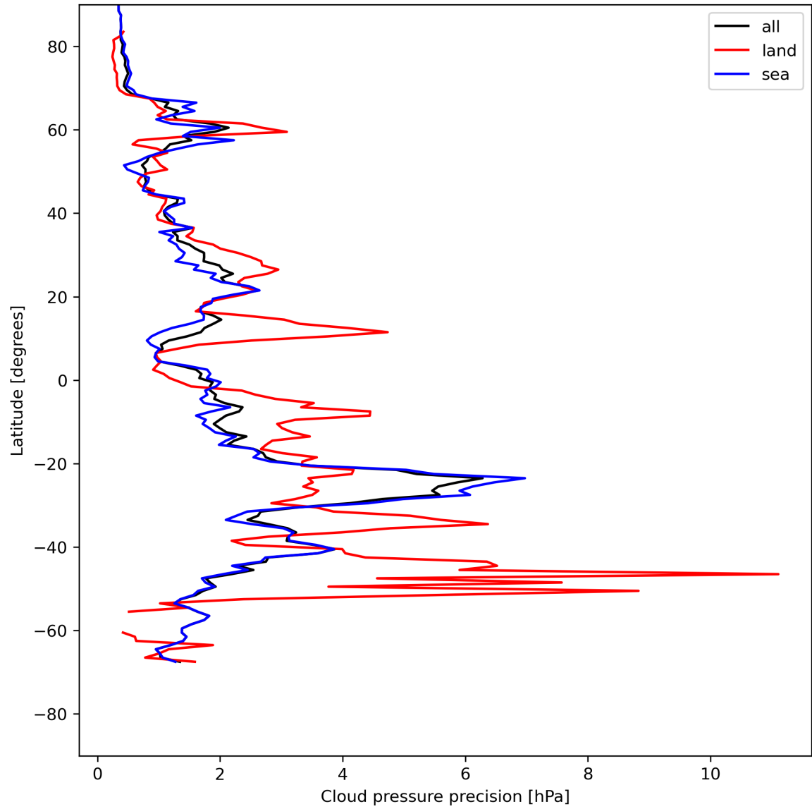
Figure 14: Zonal average of “Cloud pressure precision” for 2024-05-18 to 2024-05-19.
