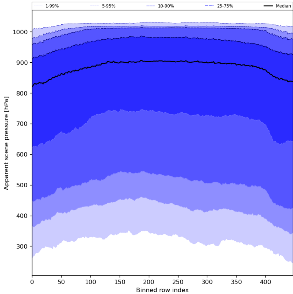
Figure 53: Along track statistics of “Apparent scene pressure” for 2024-05-18 to 2024-05-19
