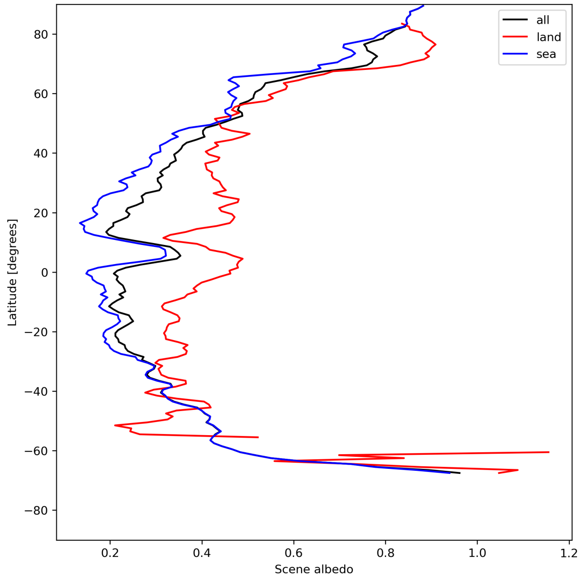
Figure 17: Zonal average of “Scene albedo” for 2024-05-18 to 2024-05-19.
