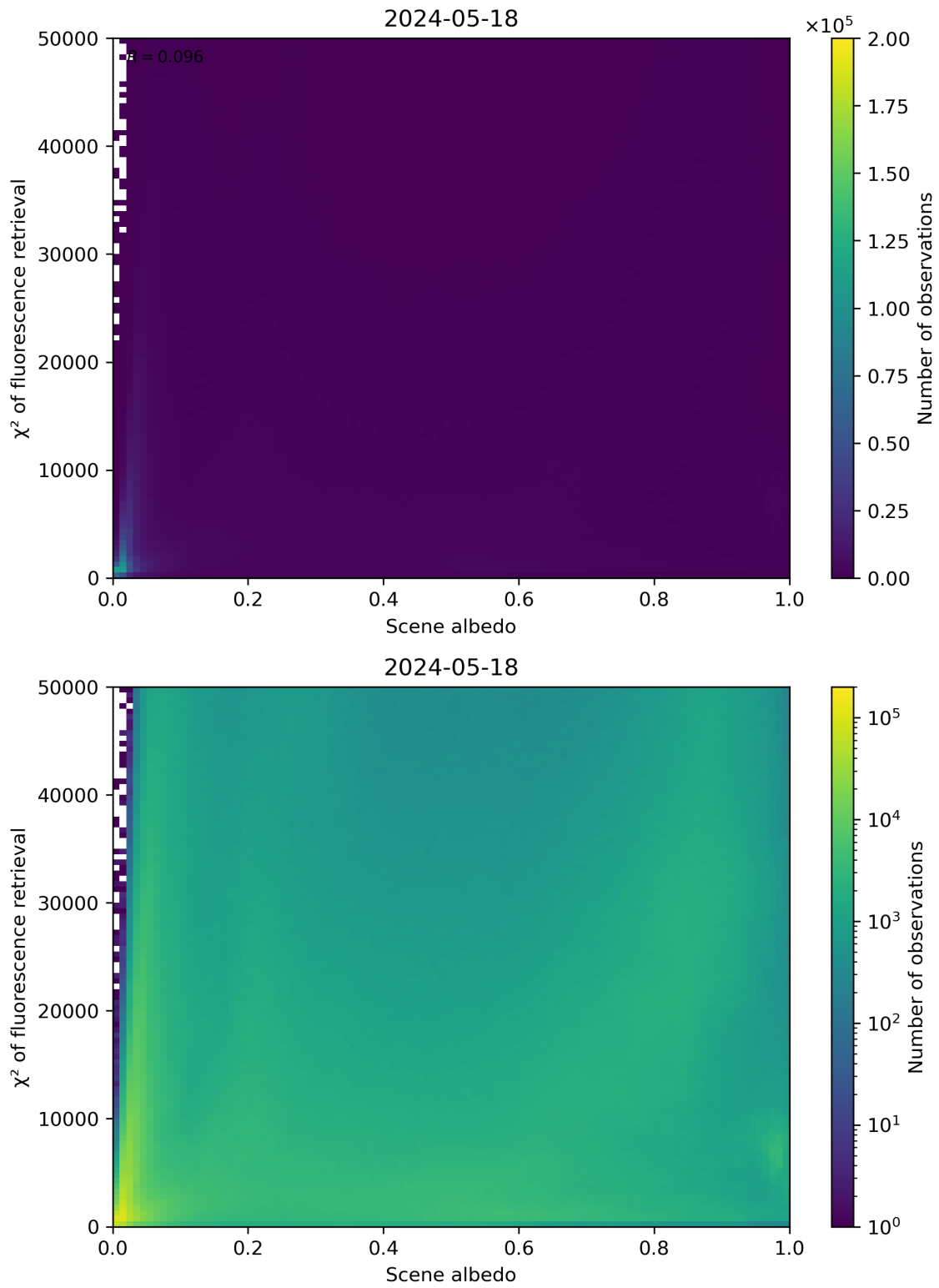
Figure 103: Scatter density plot of “Scene albedo” against “ \chi^2 of fluorescence retrieval” for 2024-05-18 to 2024-05-19.
