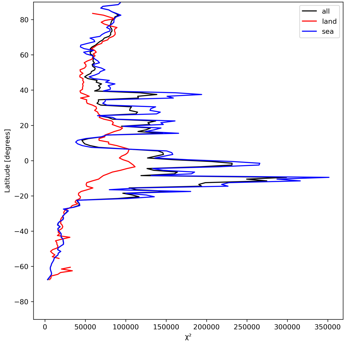
Figure 21: Zonal average of “ \chi^2 ” for 2024-05-18 to 2024-05-19.
