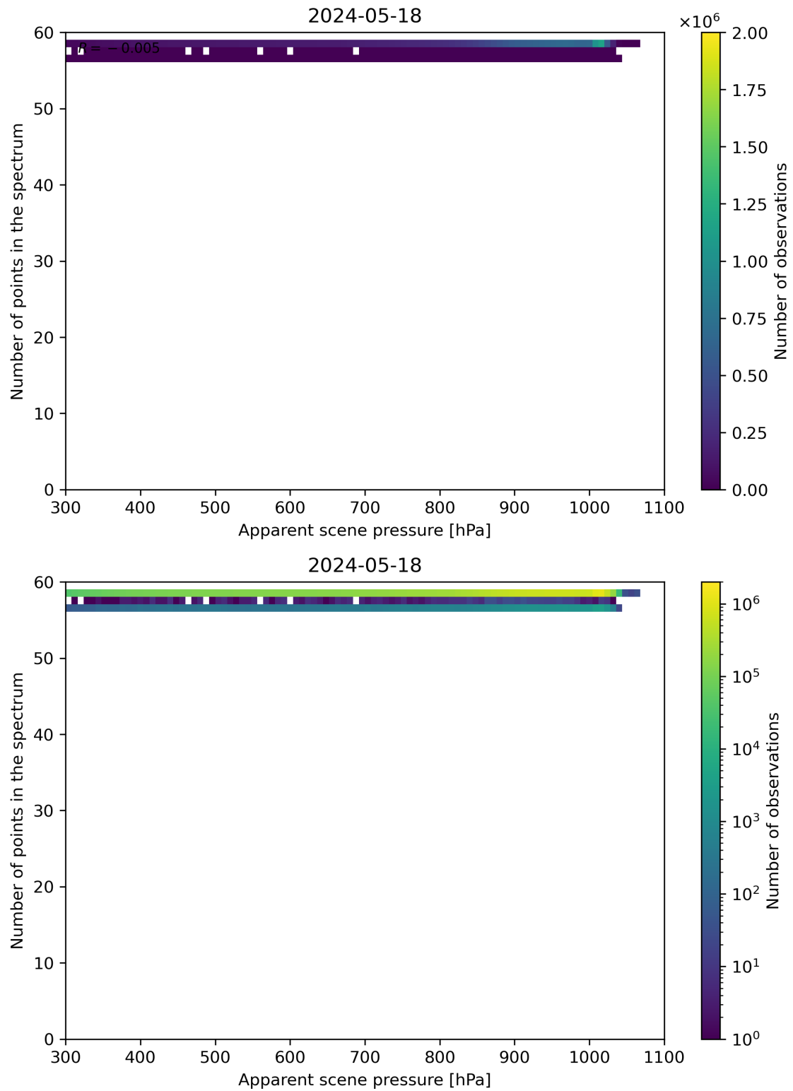
Figure 66: Scatter density plot of “Apparent scene pressure” against “Number of points in the spectrum” for 2024-05-18 to 2024-05-19.
