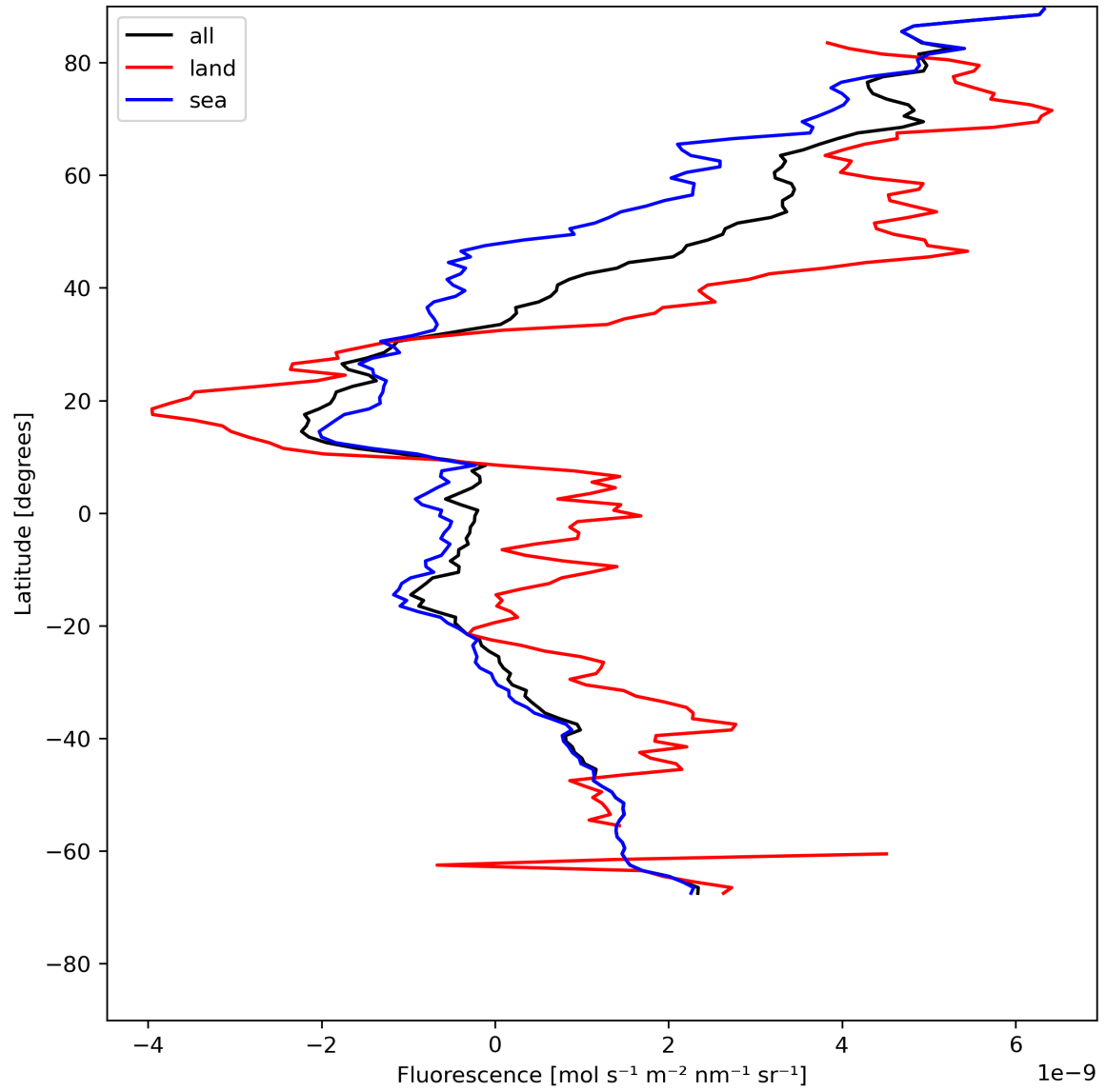
Figure 23: Zonal average of “Fluorescence” for 2024-05-18 to 2024-05-19.
