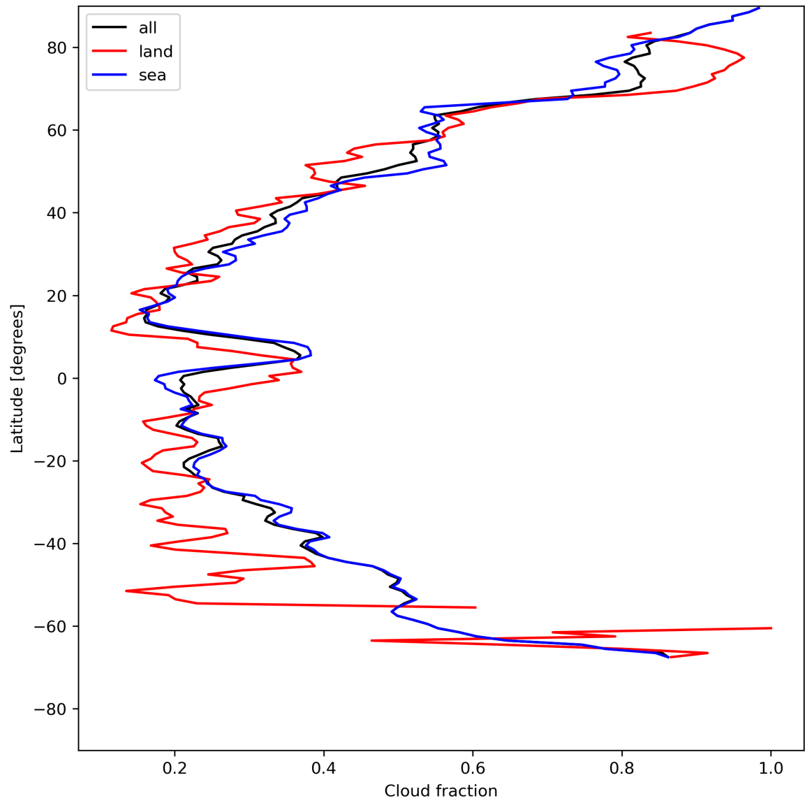
Figure 15: Zonal average of “Cloud fraction” for 2024-05-18 to 2024-05-19.
