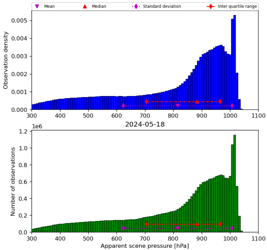
Figure 36: Histogram of “Apparent scene pressure” for 2024-05-18 to 2024-05-19
