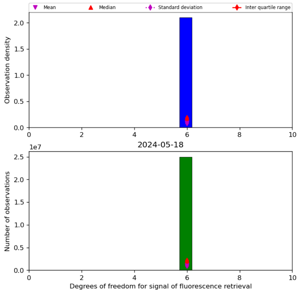
Figure 43: Histogram of “Degrees of freedom for signal of fluorescence retrieval” for 2024-05-18 to 2024-05-19
