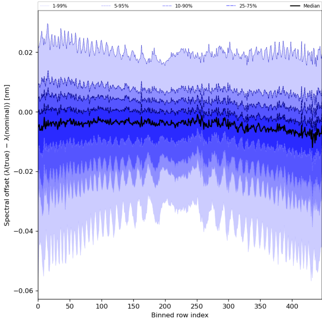
Figure 62: Along track statistics of “Spectral offset ( \lambda(\text{true}) - \lambda(\text{nominal}) )” for 2024-05-18 to 2024-05-19
