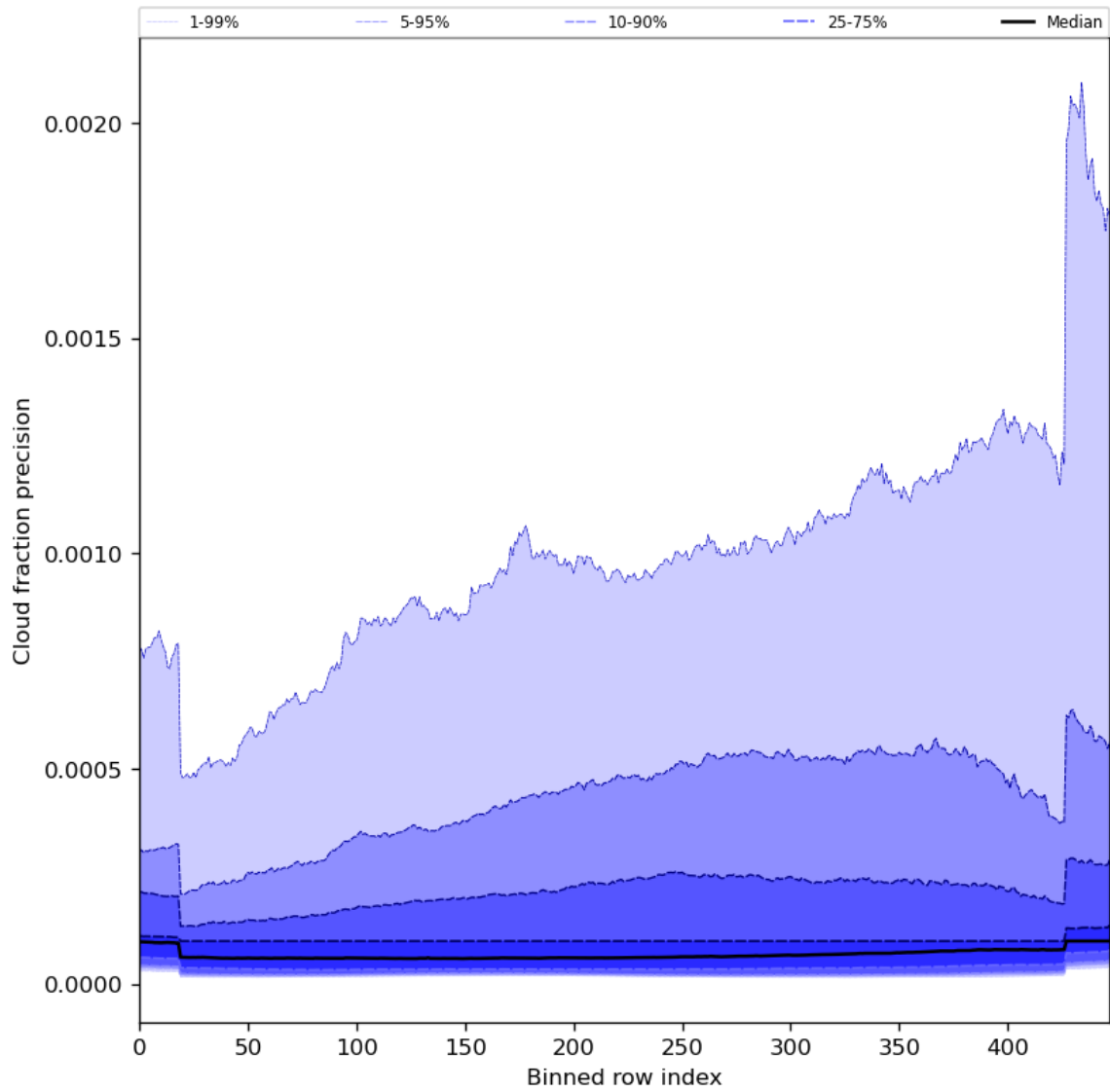
Figure 50: Along track statistics of “Cloud fraction precision” for 2024-05-18 to 2024-05-19
