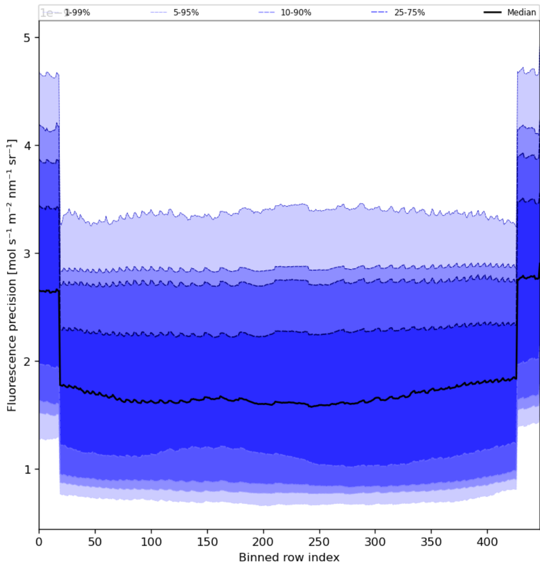
Figure 58: Along track statistics of “Fluorescence precision” for 2024-05-18 to 2024-05-19
