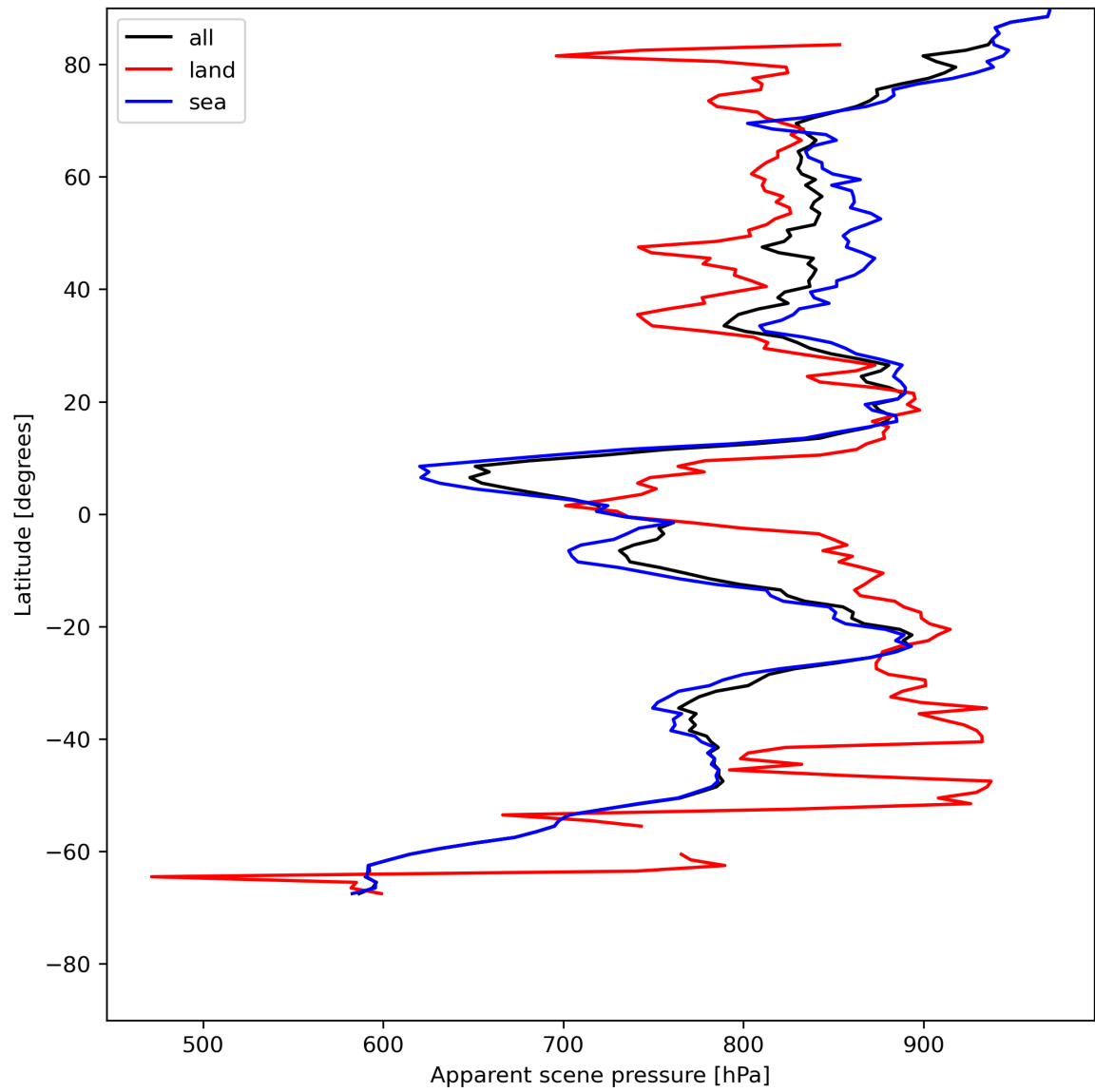
Figure 19: Zonal average of “Apparent scene pressure” for 2024-05-18 to 2024-05-19.
