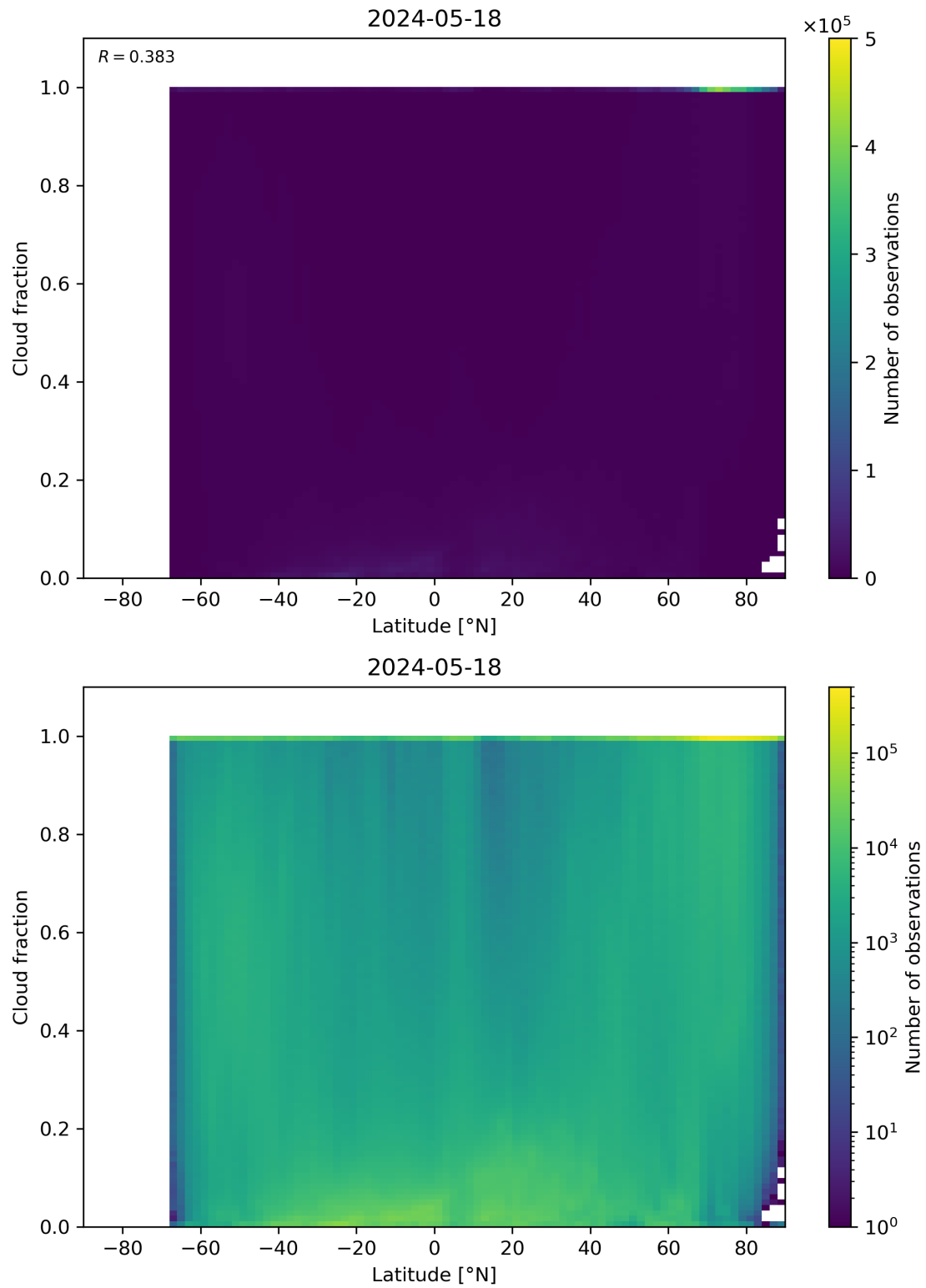
Figure 90: Scatter density plot of “Latitude” against “Cloud fraction” for 2024-05-18 to 2024-05-19.
