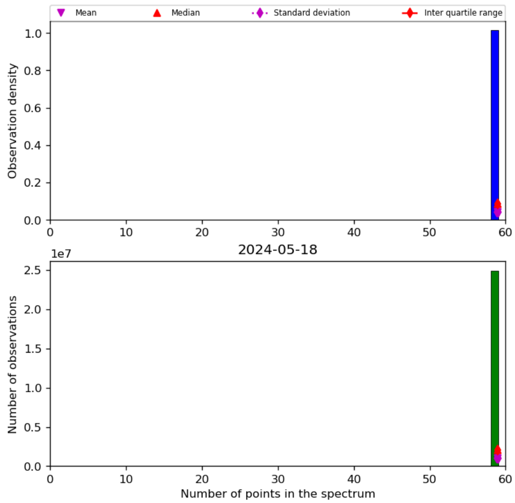
Figure 44: Histogram of “Number of points in the spectrum” for 2024-05-18 to 2024-05-19
