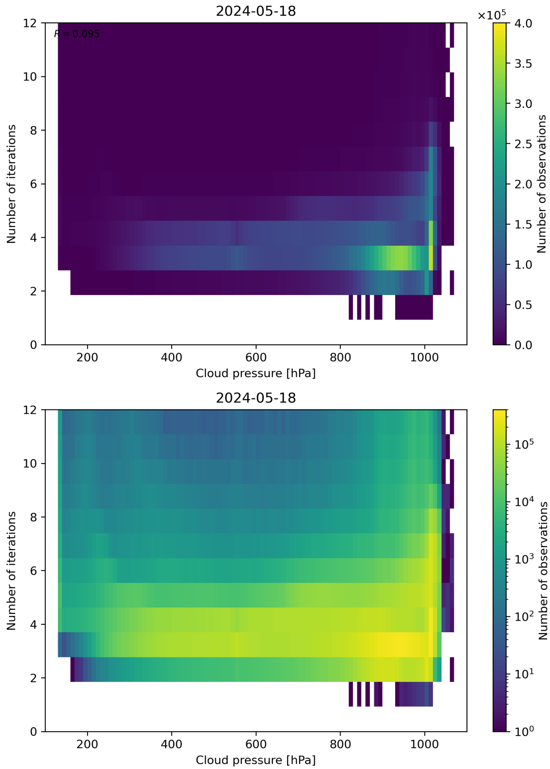
Figure 81: Scatter density plot of “Cloud pressure” against “Number of iterations” for 2024-05-18 to 2024-05-19.
