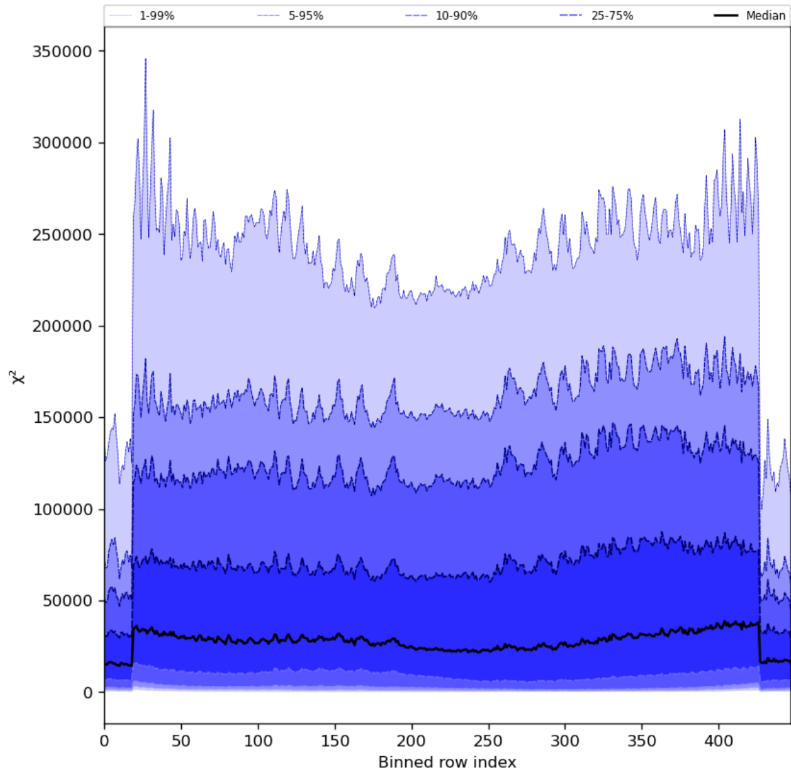
Figure 55: Along track statistics of “ \chi^2 ” for 2024-05-18 to 2024-05-19
