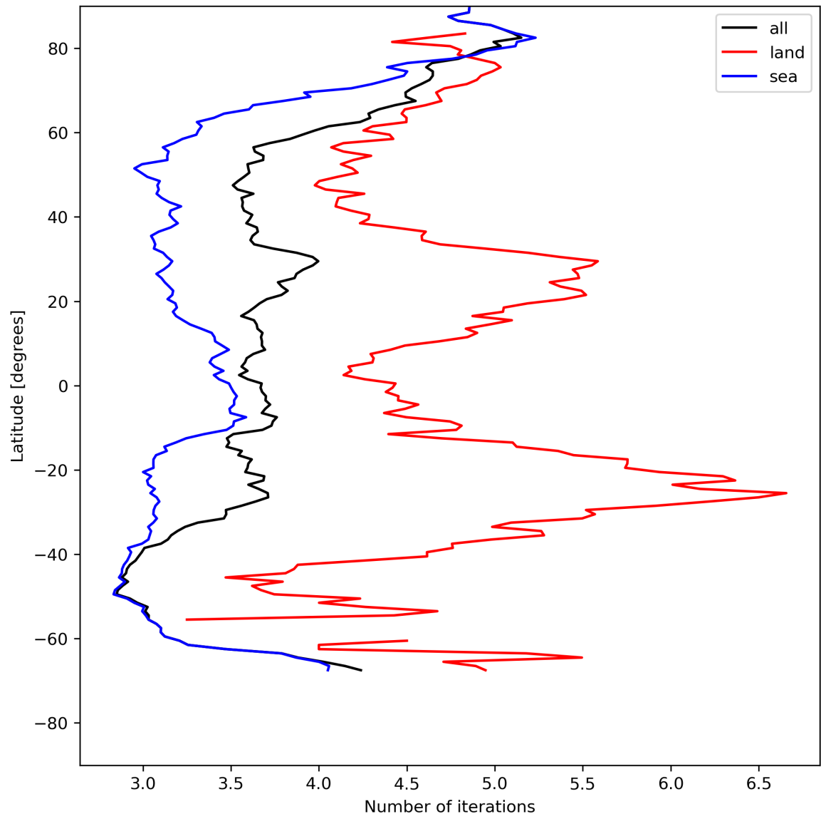
Figure 22: Zonal average of “Number of iterations” for 2024-05-18 to 2024-05-19.
