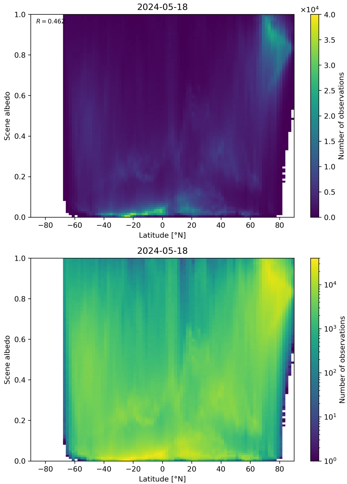
Figure 95: Scatter density plot of “Latitude” against “Scene albedo” for 2024-05-18 to 2024-05-19.
