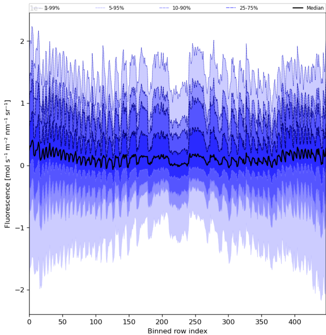
Figure 57: Along track statistics of “Fluorescence” for 2024-05-18 to 2024-05-19
