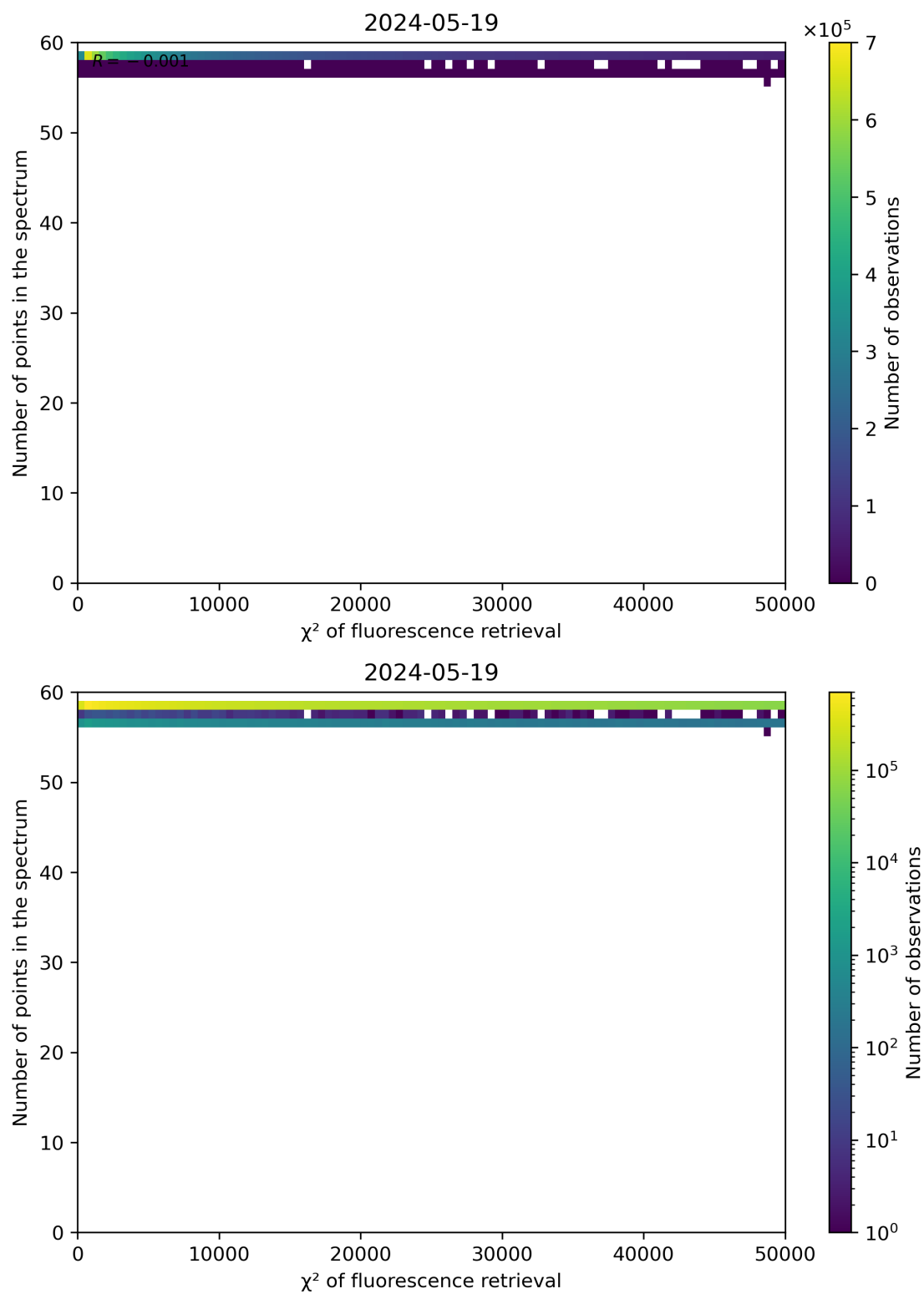
Figure 68: Scatter density plot of “ \chi^2 of fluorescence retrieval” against “Number of points in the spectrum” for 2024-05-18 to 2024-05-20.
