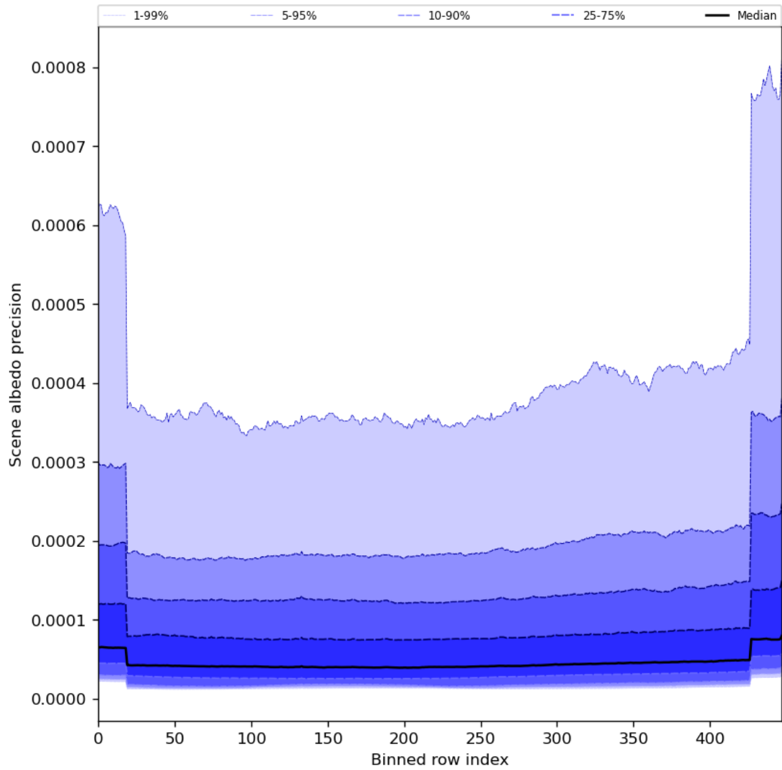
Figure 52: Along track statistics of “Scene albedo precision” for 2024-05-18 to 2024-05-20
