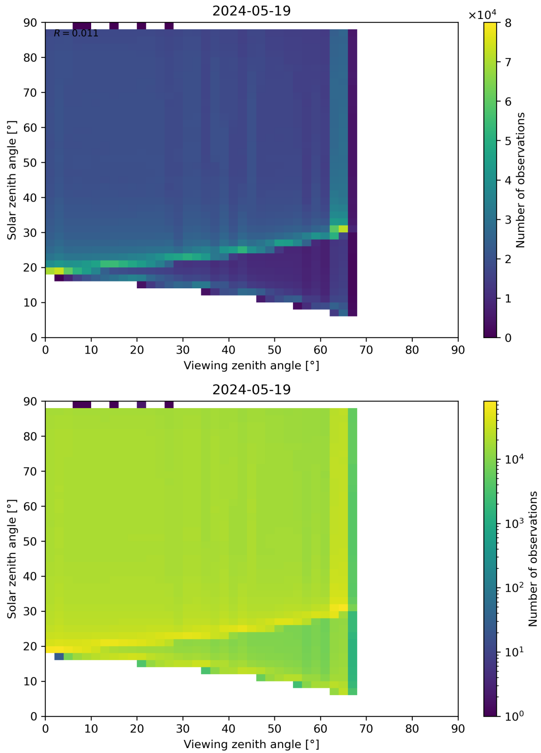
Figure 127: Scatter density plot of “Viewing zenith angle” against “Solar zenith angle” for 2024-05-18 to 2024-05-20.
