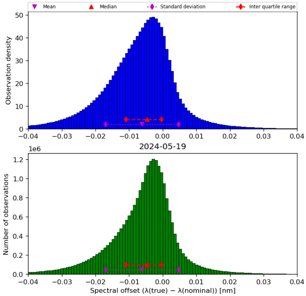
Figure 45: Histogram of “Spectral offset ( \lambda(\text{true}) - \lambda(\text{nominal}) )” for 2024-05-18 to 2024-05-20
