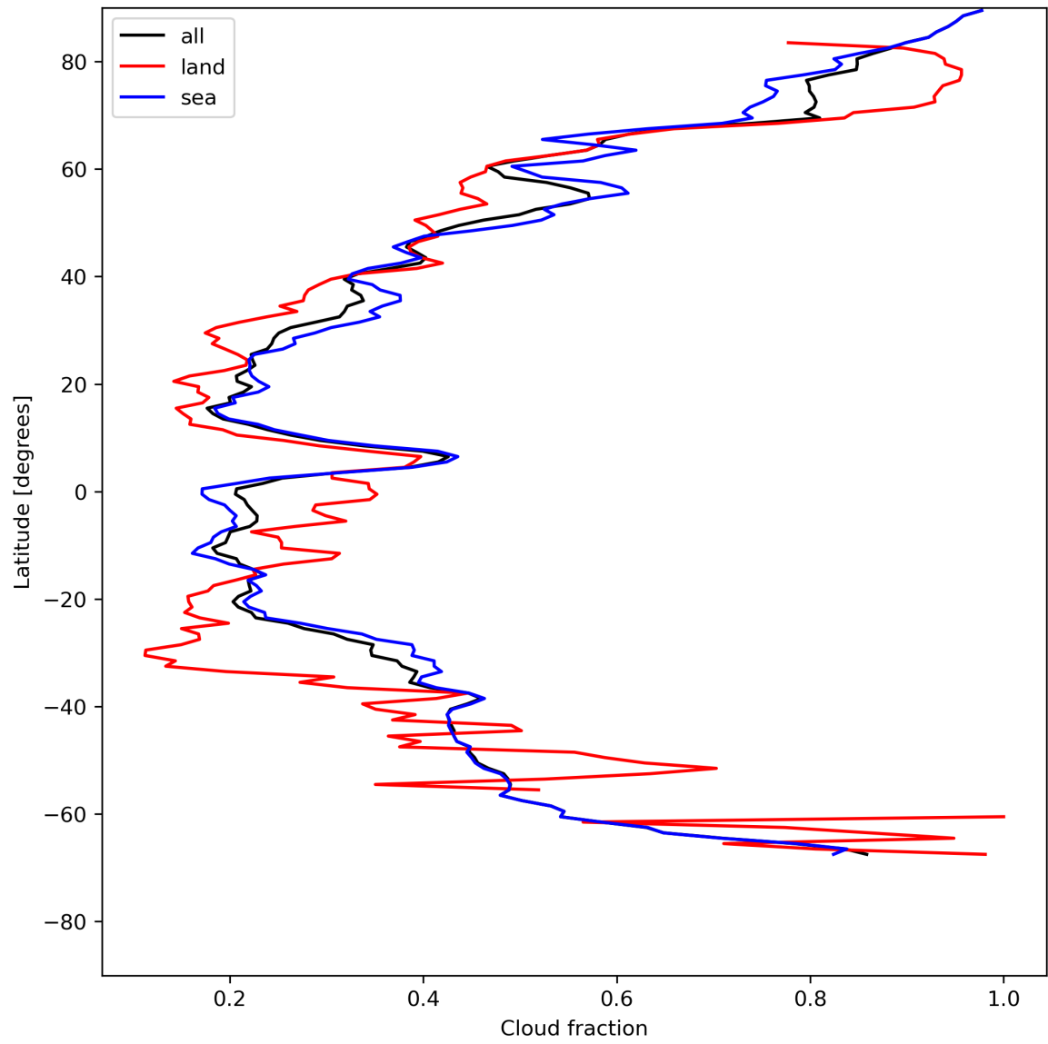
Figure 15: Zonal average of “Cloud fraction” for 2024-05-18 to 2024-05-20.
