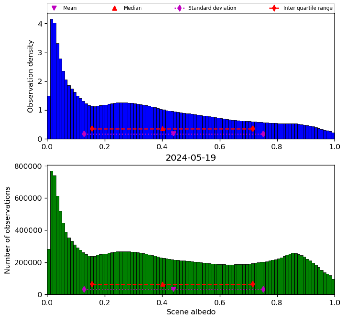
Figure 34: Histogram of “Scene albedo” for 2024-05-18 to 2024-05-20
