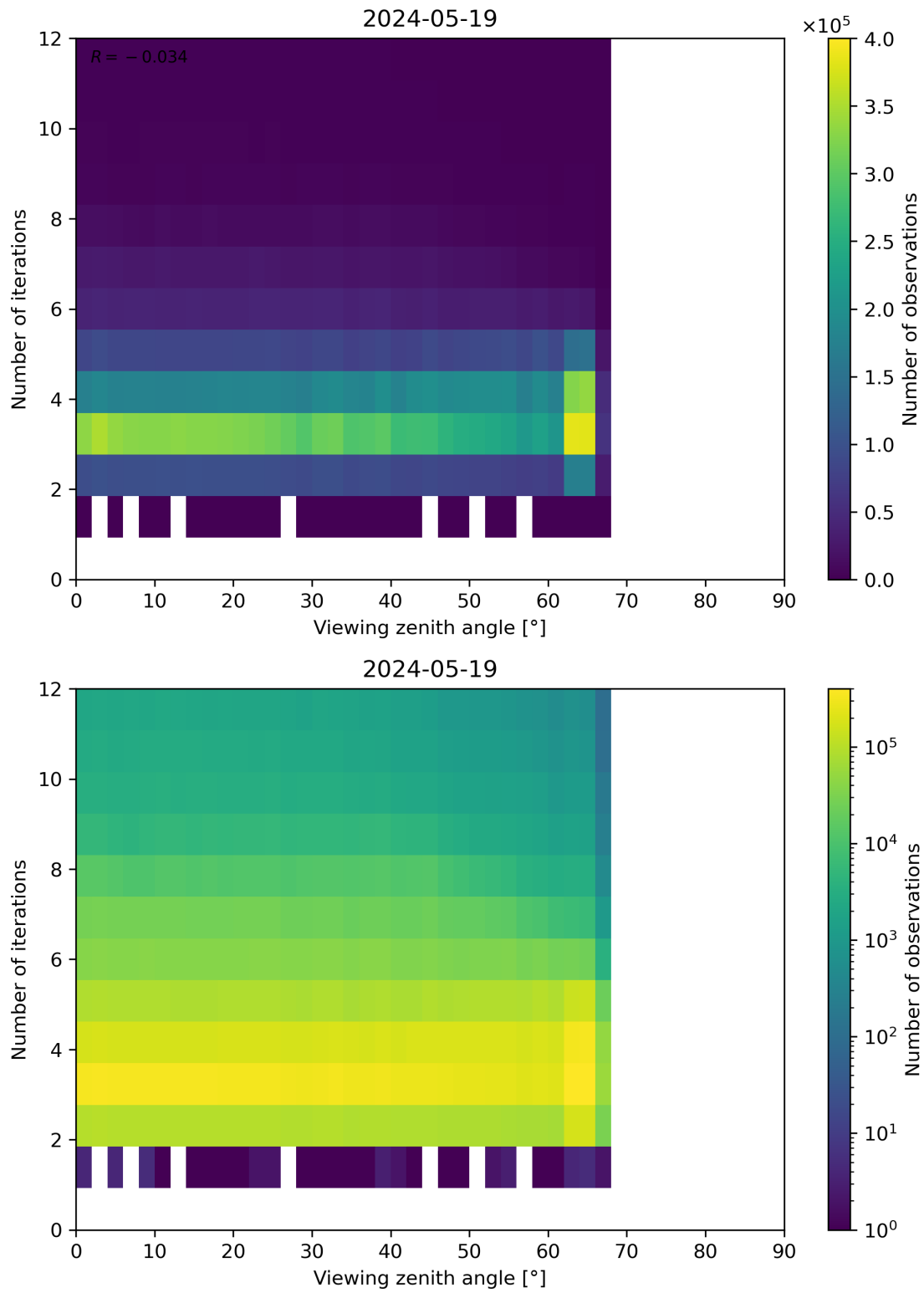
Figure 124: Scatter density plot of “Viewing zenith angle” against “Number of iterations” for 2024-05-18 to 2024-05-20.
