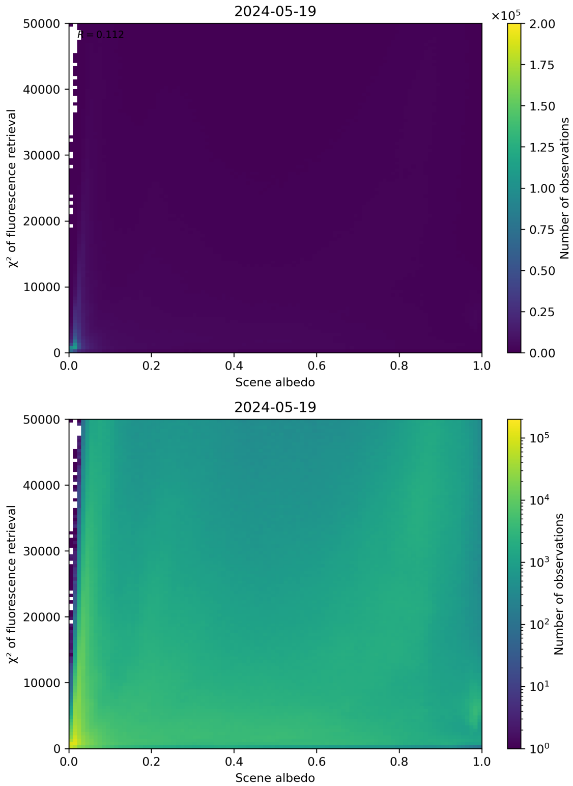
Figure 103: Scatter density plot of “Scene albedo” against “ \chi^2 of fluorescence retrieval” for 2024-05-18 to 2024-05-20.
