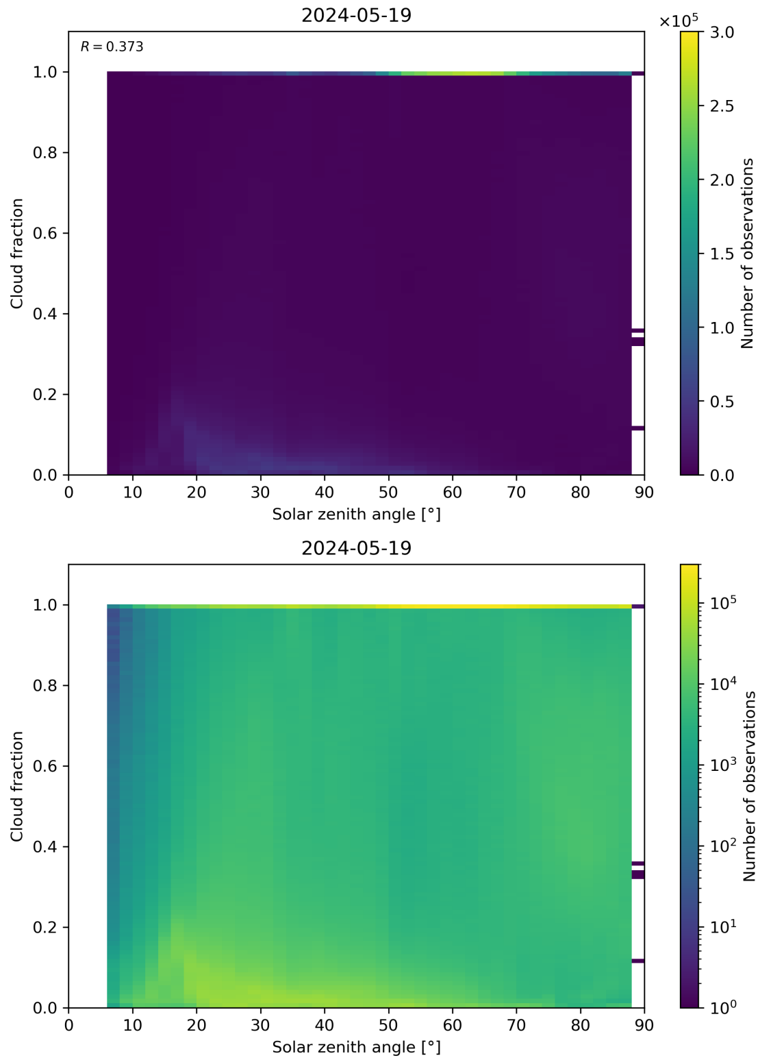
Figure 110: Scatter density plot of “Solar zenith angle” against “Cloud fraction” for 2024-05-18 to 2024-05-20.
