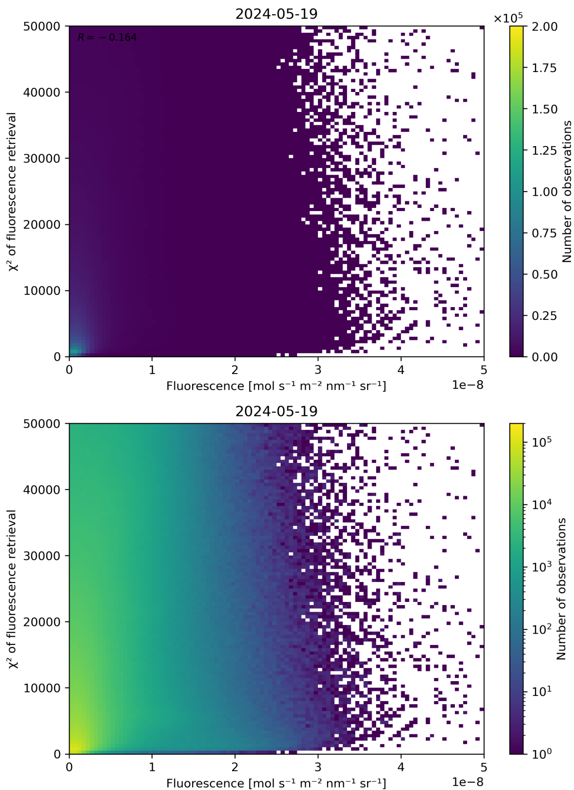
Figure 85: Scatter density plot of “Fluorescence” against “ \chi^2 of fluorescence retrieval” for 2024-05-18 to 2024-05-20.
