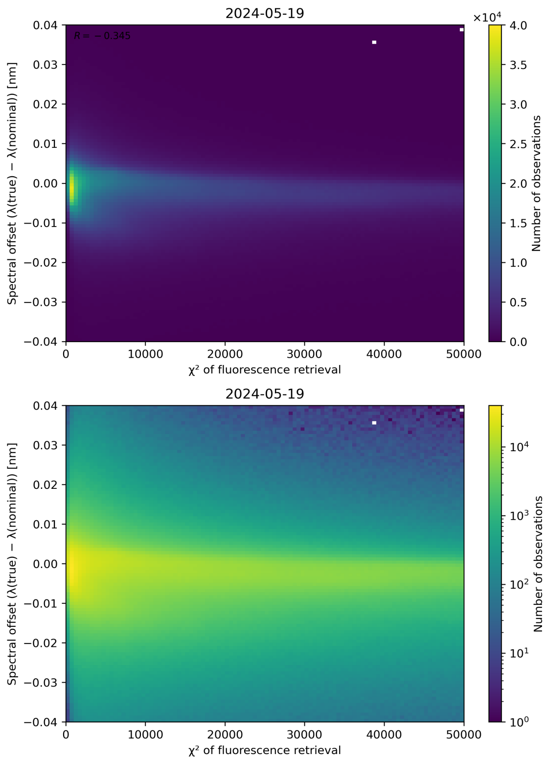
Figure 69: Scatter density plot of " \chi^2 of fluorescence retrieval" against "Spectral offset ( \lambda(\text{true}) - \lambda(\text{nominal}) )" for 2024-05-18 to 2024-05-20.
