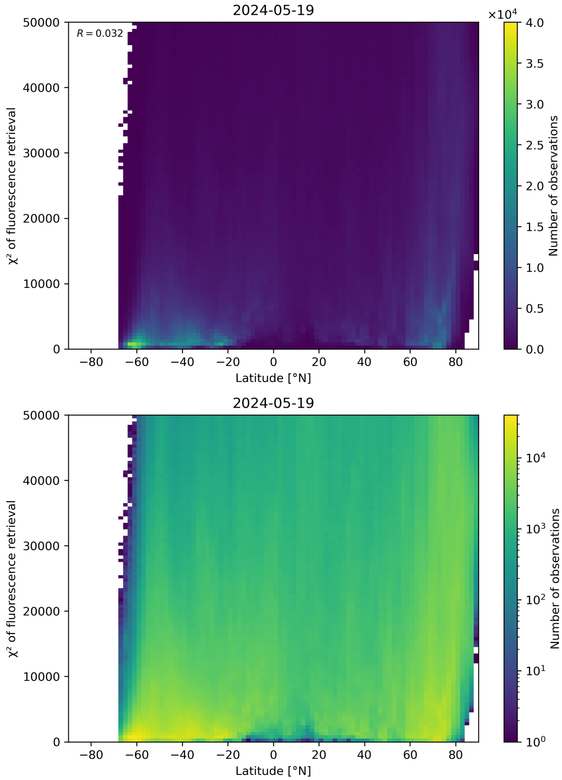
Figure 89: Scatter density plot of “Latitude” against “ \chi^2 of fluorescence retrieval” for 2024-05-18 to 2024-05-20.
