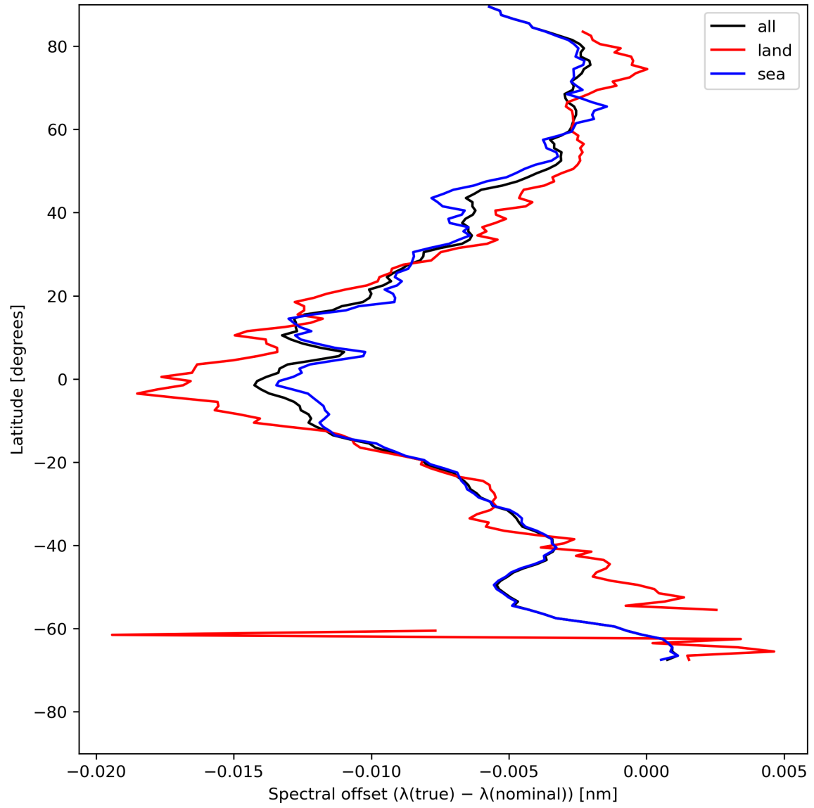
Figure 28: Zonal average of “Spectral offset ( \lambda(\text{true}) - \lambda(\text{nominal}) )” for 2024-05-18 to 2024-05-20.
