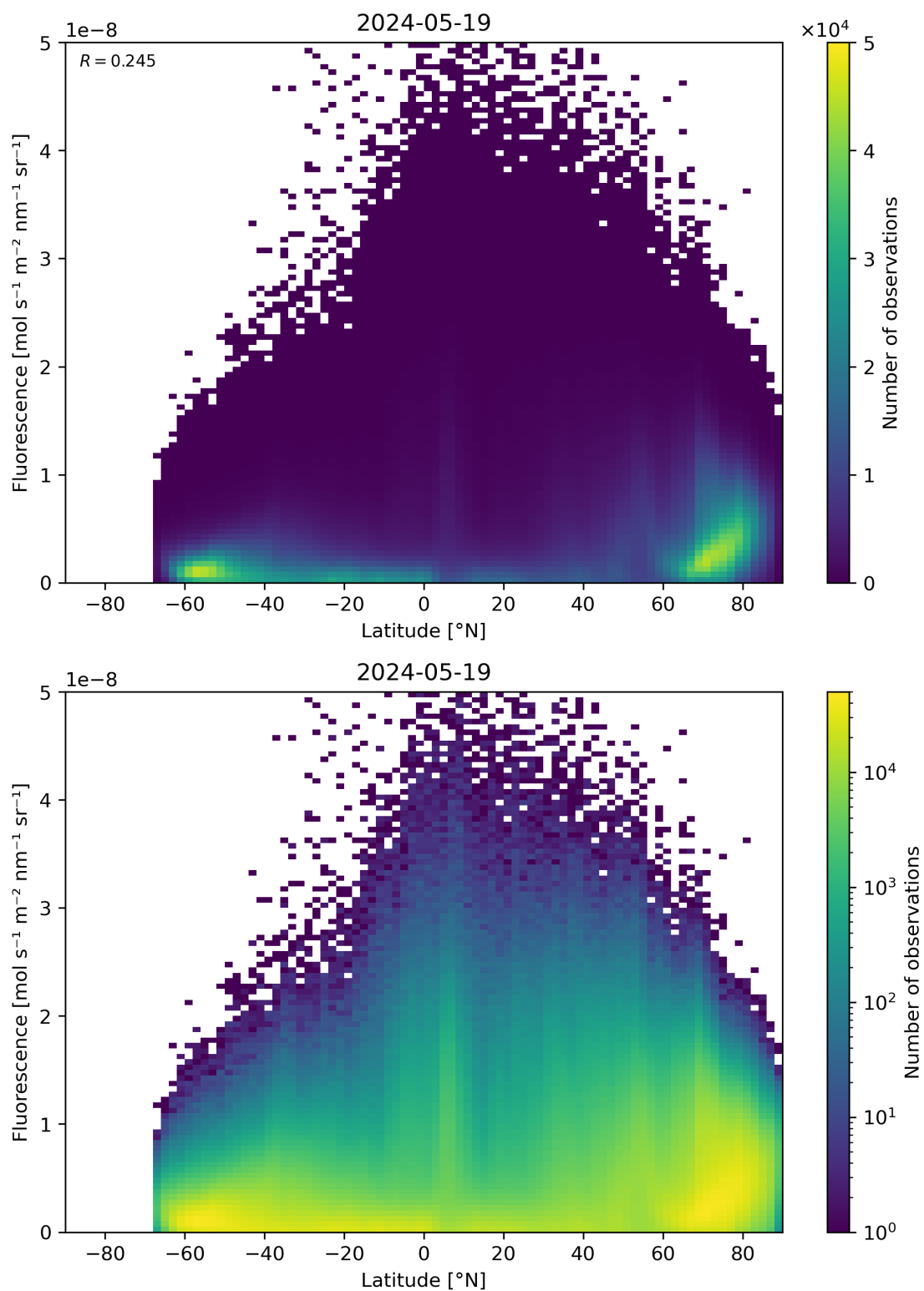
Figure 92: Scatter density plot of “Latitude” against “Fluorescence” for 2024-05-18 to 2024-05-20.
