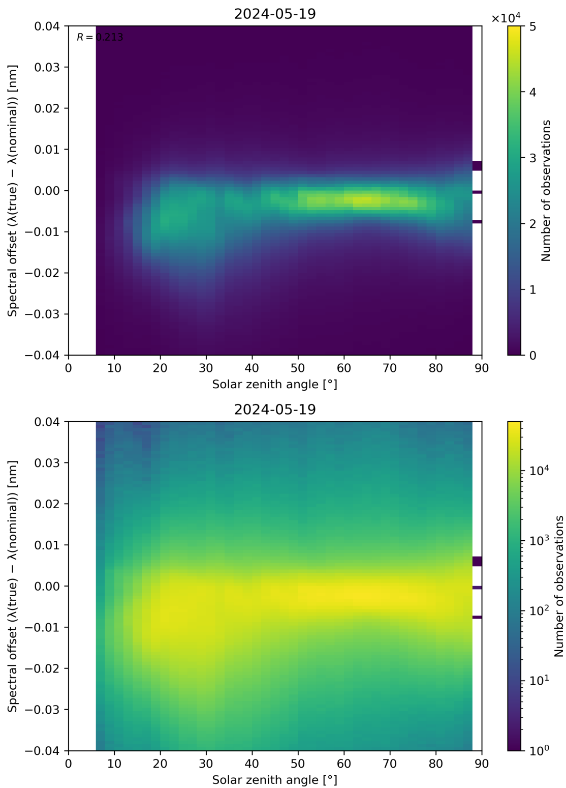
Figure 117: Scatter density plot of “Solar zenith angle” against “Spectral offset ( \lambda(\text{true}) - \lambda(\text{nominal}) )” for 2024-05-18 to 2024-05-20.
