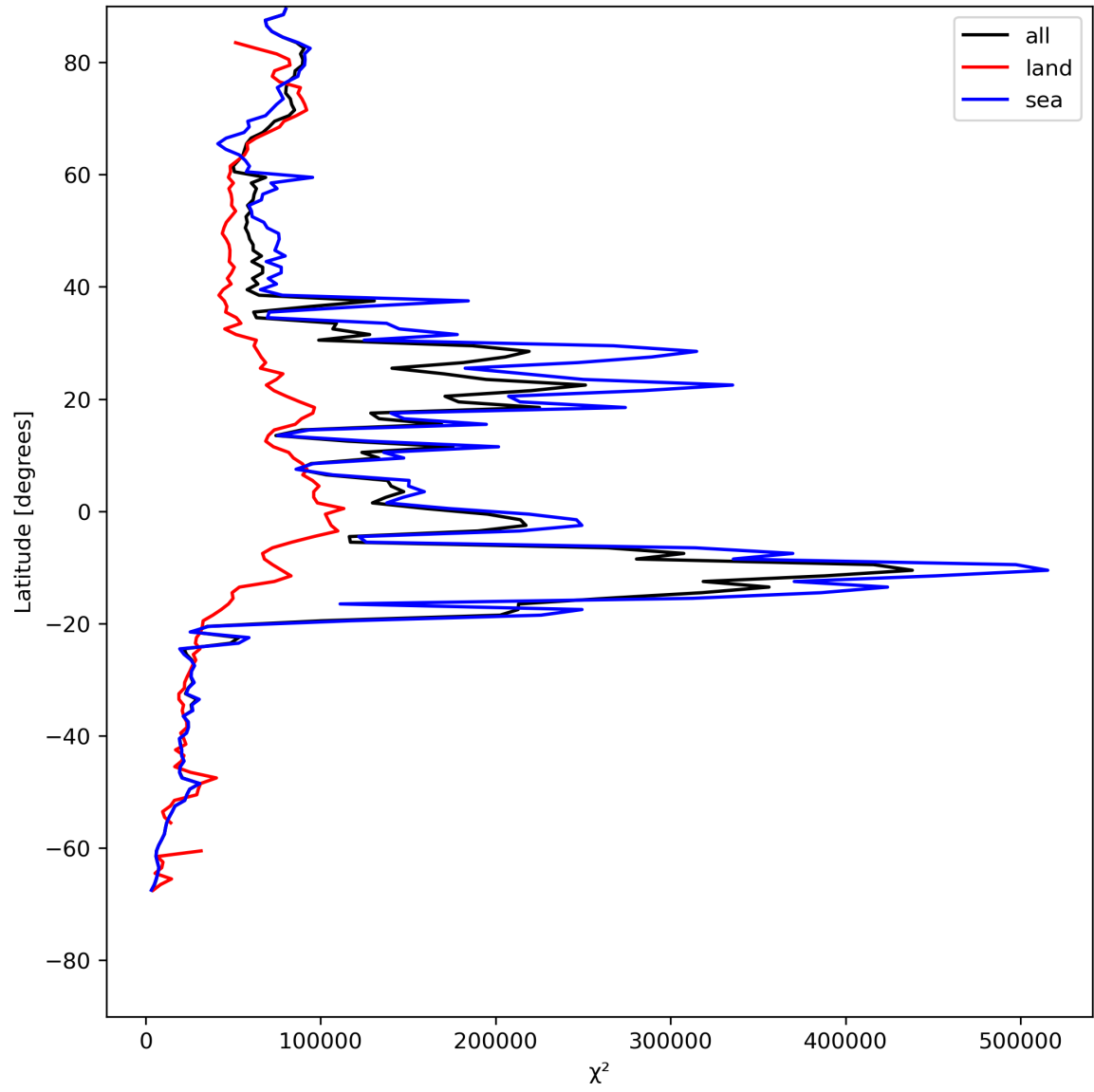
Figure 21: Zonal average of “ \chi^2 ” for 2024-05-18 to 2024-05-20.
