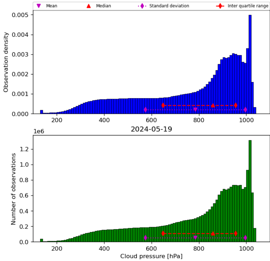
Figure 30: Histogram of “Cloud pressure” for 2024-05-18 to 2024-05-20
