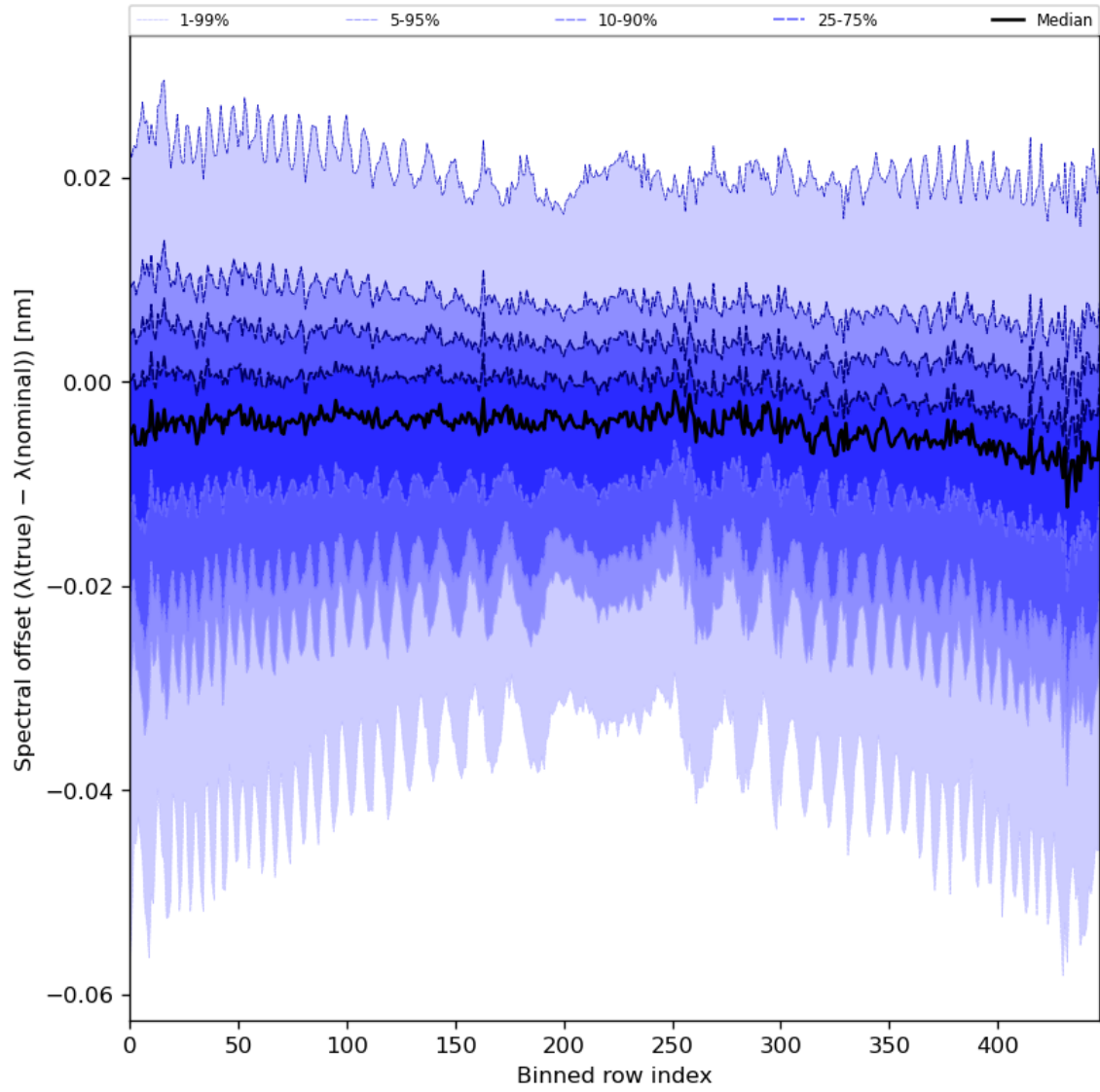
Figure 62: Along track statistics of “Spectral offset ( \lambda(\text{true}) - \lambda(\text{nominal}) )” for 2024-05-18 to 2024-05-20
