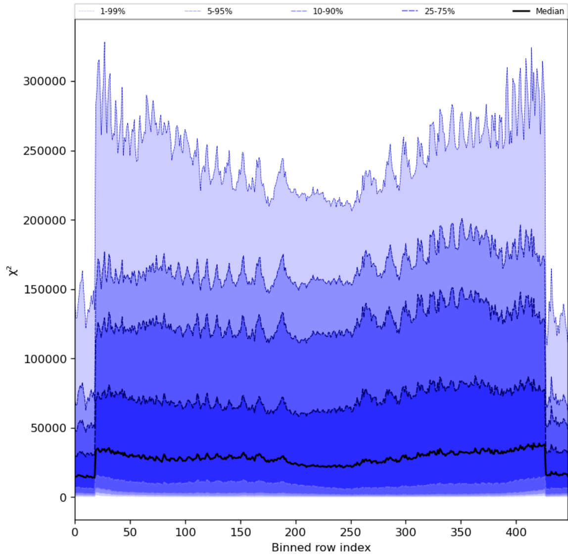
Figure 55: Along track statistics of “ \chi^2 ” for 2024-05-18 to 2024-05-20
