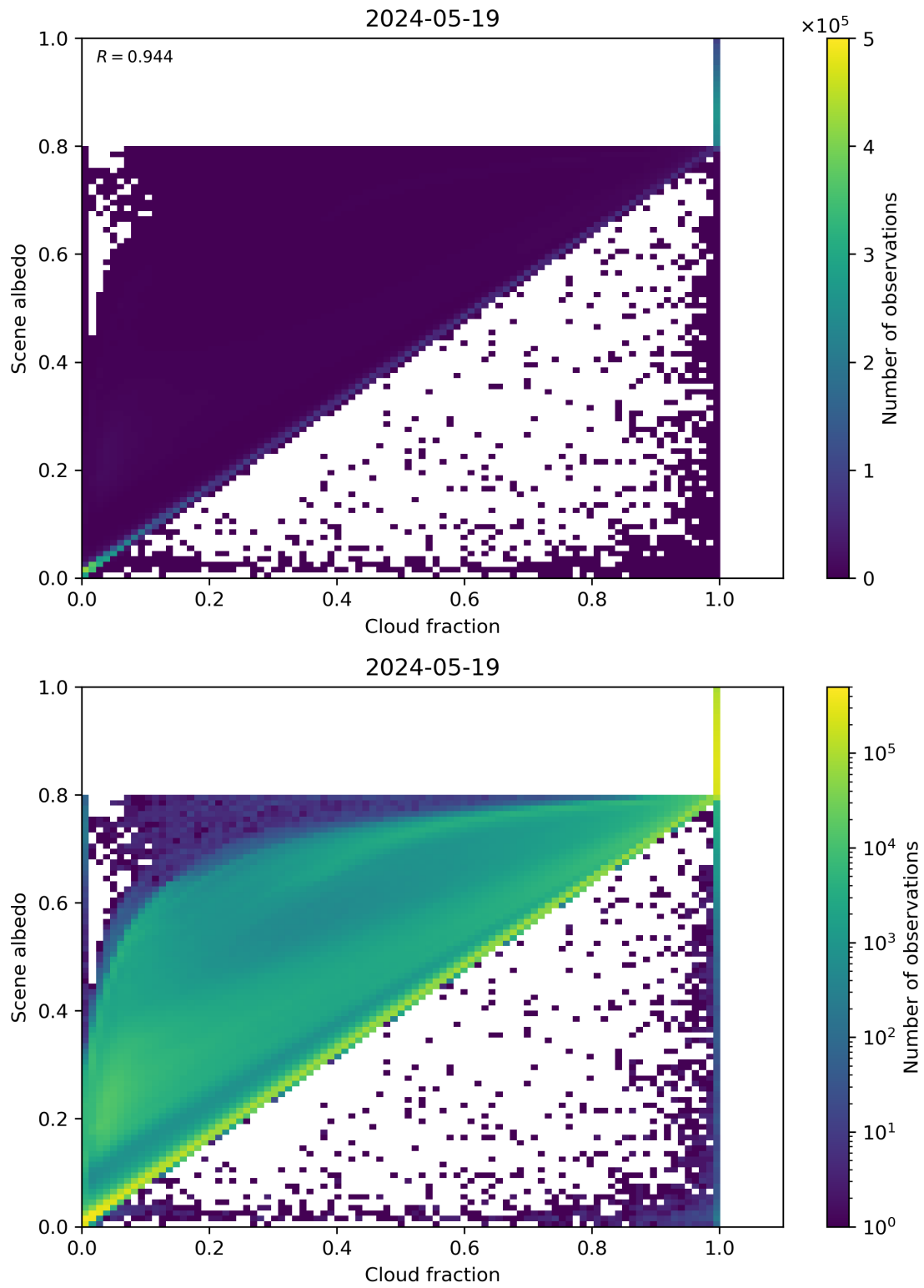
Figure 75: Scatter density plot of “Cloud fraction” against “Scene albedo” for 2024-05-18 to 2024-05-20.
