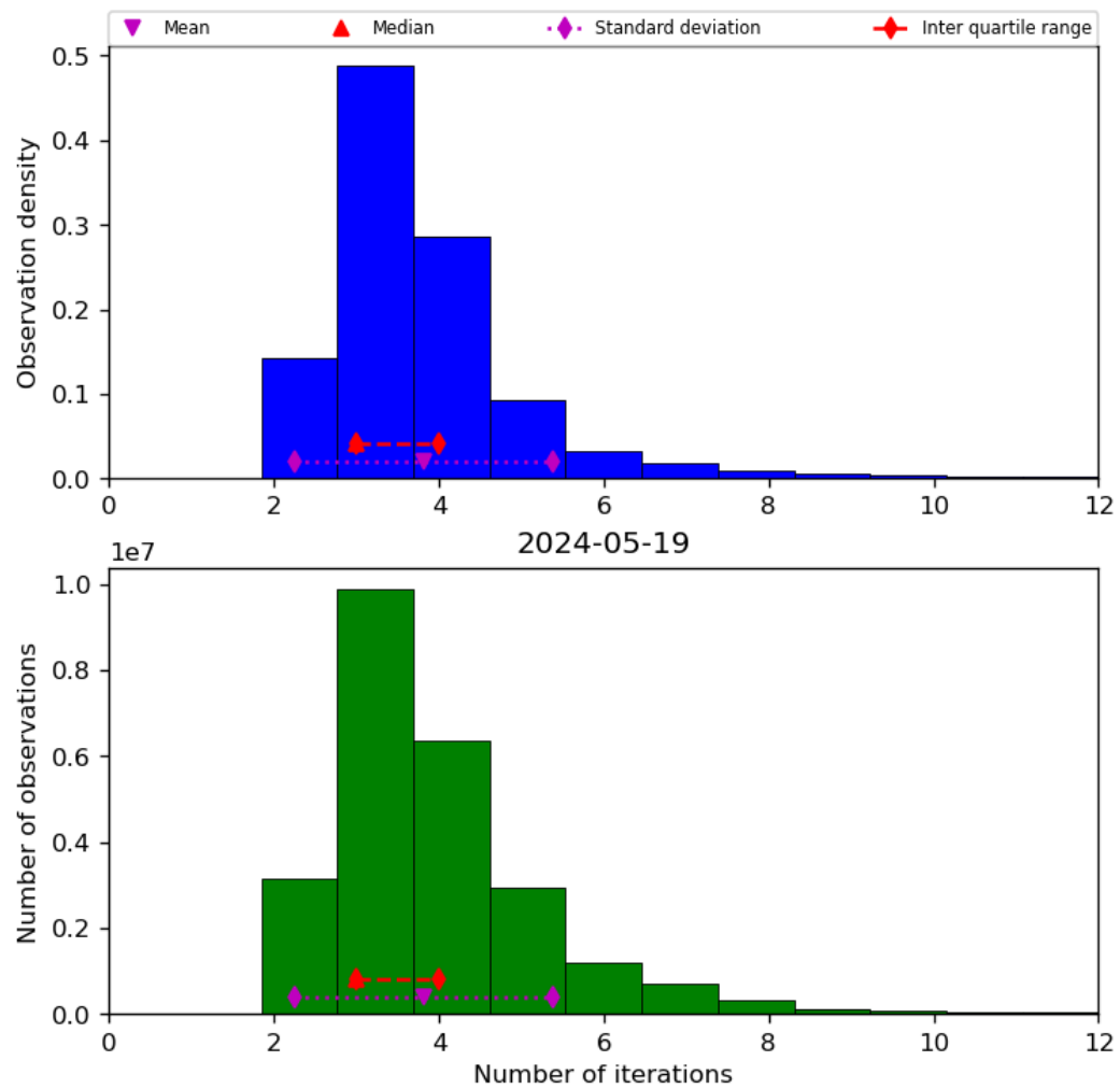
Figure 39: Histogram of “Number of iterations” for 2024-05-18 to 2024-05-20
