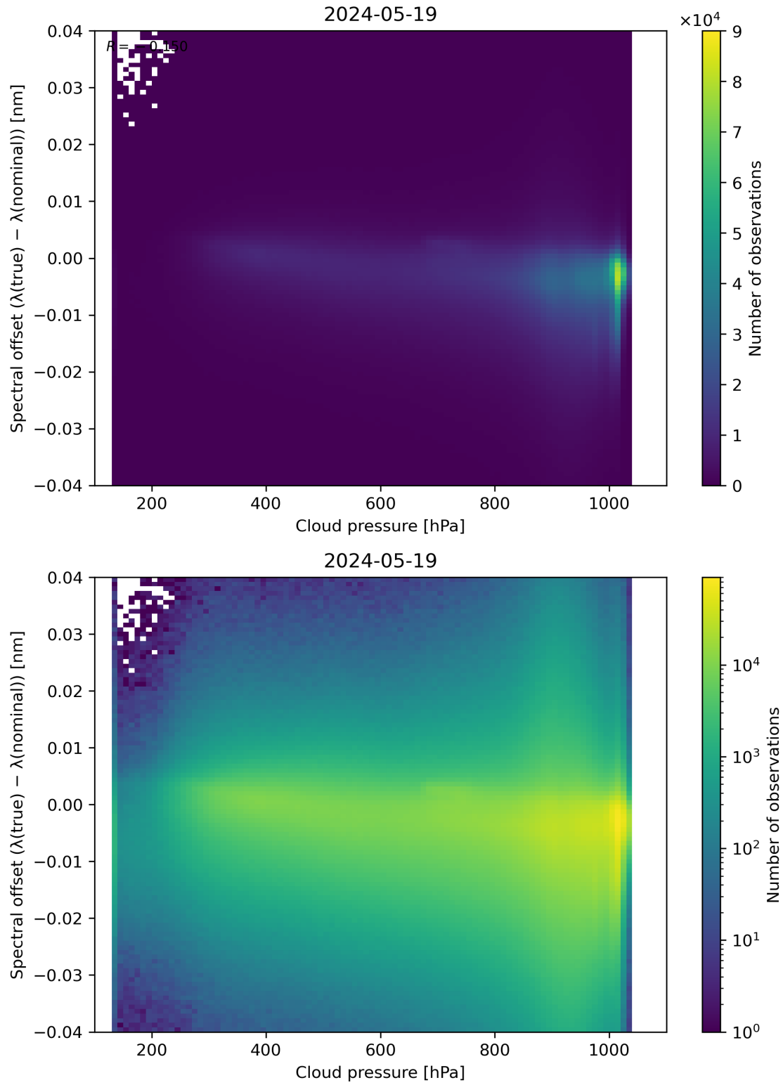
Figure 84: Scatter density plot of “Cloud pressure” against “Spectral offset ( \lambda(\text{true}) - \lambda(\text{nominal}) )” for 2024-05-18 to 2024-05-20.
