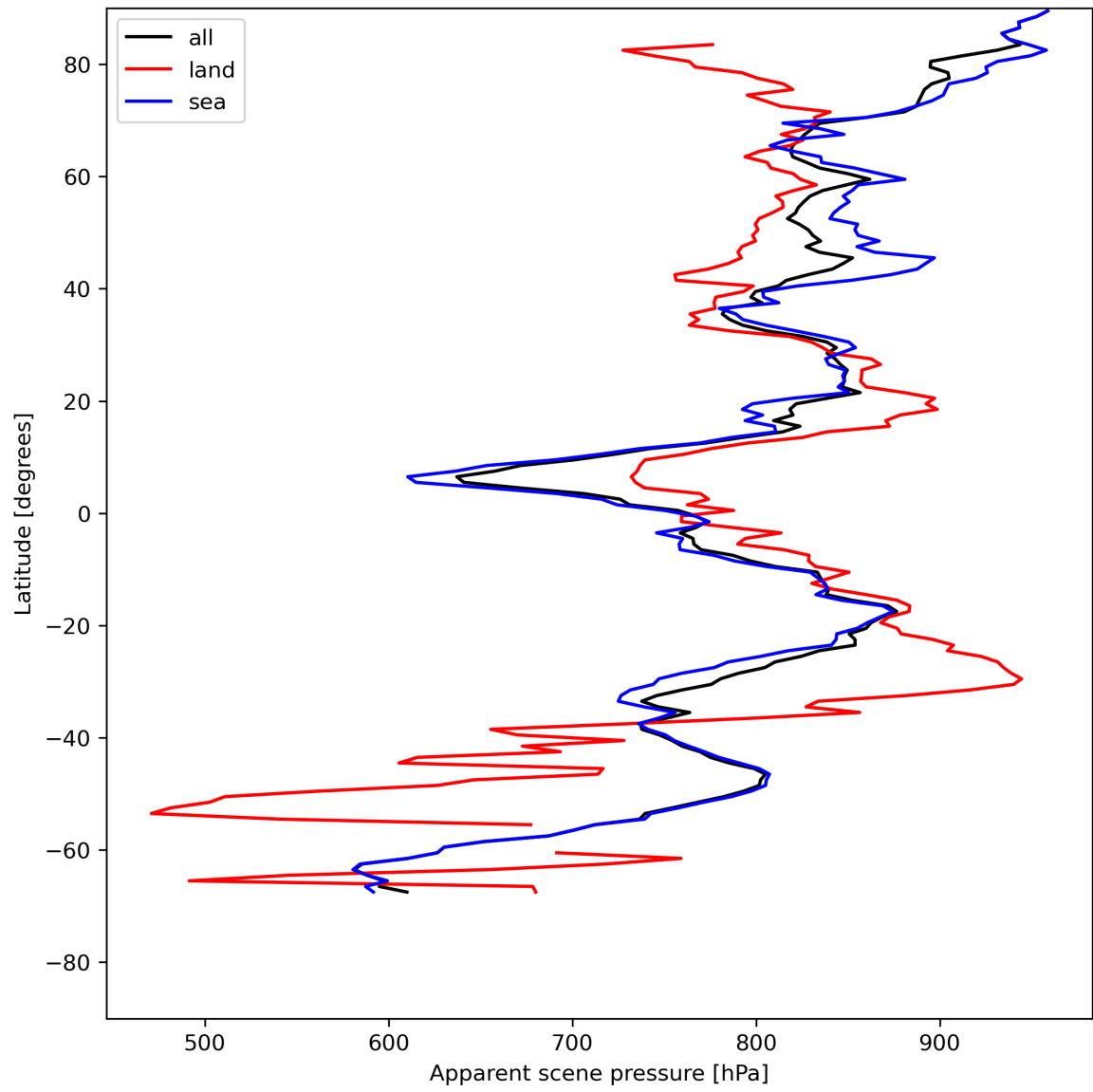
Figure 19: Zonal average of “Apparent scene pressure” for 2024-05-18 to 2024-05-20.
