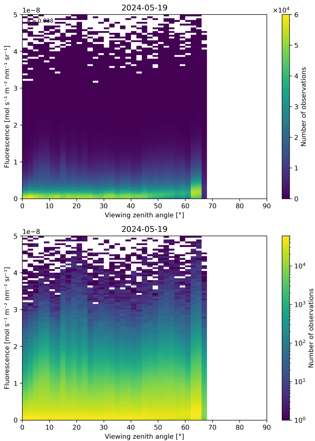
Figure 122: Scatter density plot of “Viewing zenith angle” against “Fluorescence” for 2024-05-18 to 2024-05-20.
