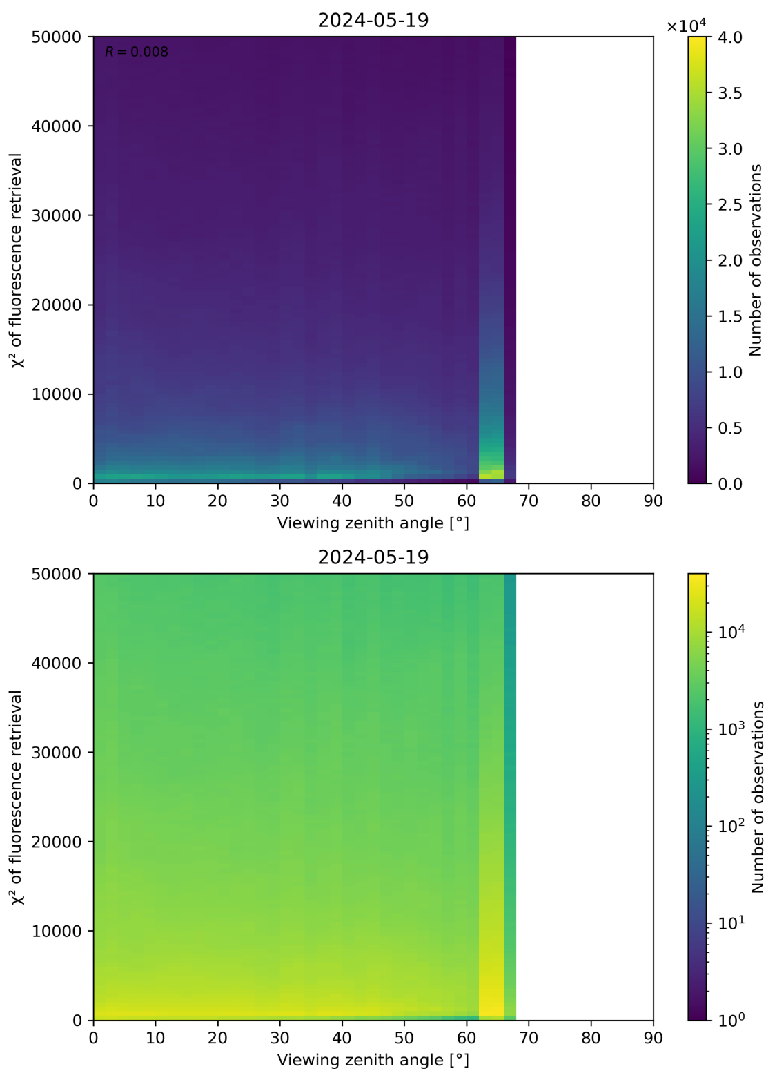
Figure 119: Scatter density plot of “Viewing zenith angle” against “ \chi^2 of fluorescence retrieval” for 2024-05-18 to 2024-05-20.
