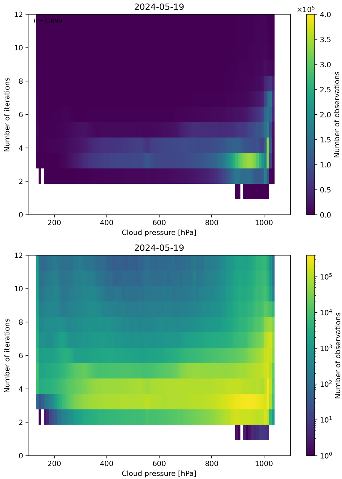
Figure 81: Scatter density plot of “Cloud pressure” against “Number of iterations” for 2024-05-18 to 2024-05-20.
