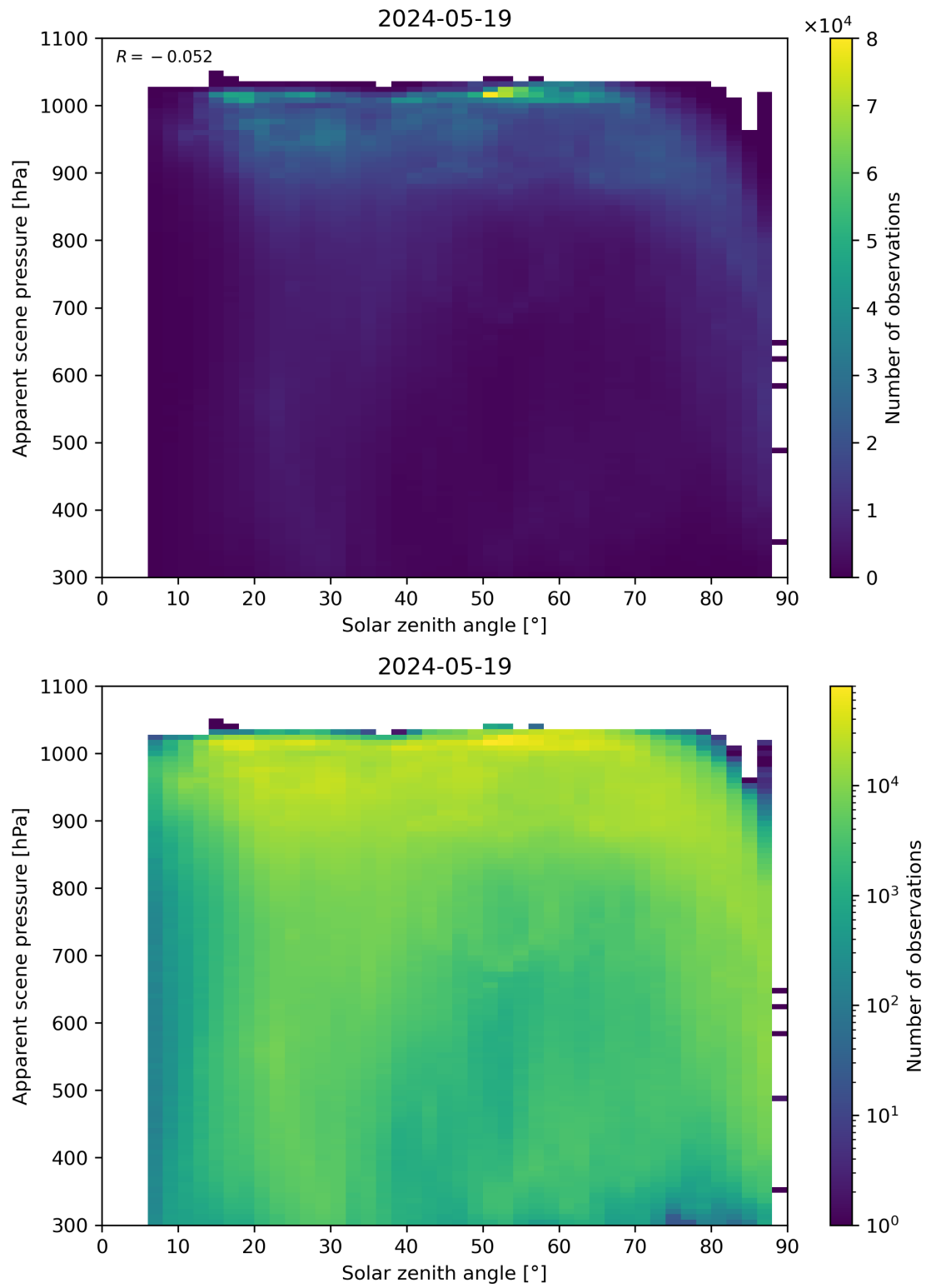
Figure 108: Scatter density plot of “Solar zenith angle” against “Apparent scene pressure” for 2024-05-18 to 2024-05-20.
