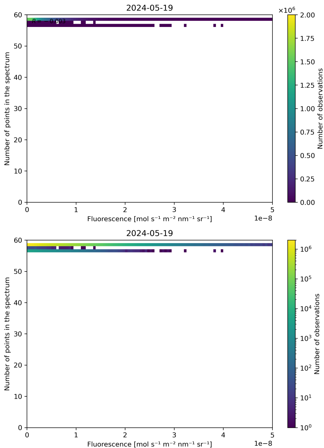
Figure 86: Scatter density plot of “Fluorescence” against “Number of points in the spectrum” for 2024-05-18 to 2024-05-20.
