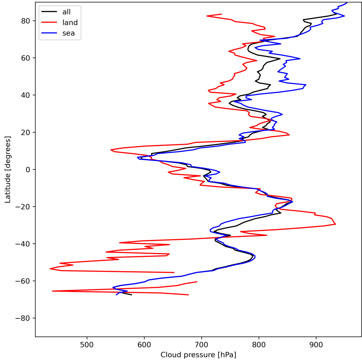
Figure 13: Zonal average of “Cloud pressure” for 2024-05-18 to 2024-05-20.
