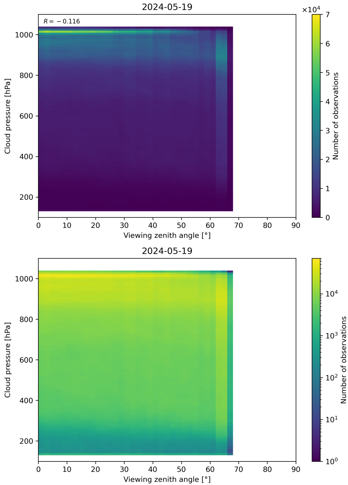
Figure 121: Scatter density plot of “Viewing zenith angle” against “Cloud pressure” for 2024-05-18 to 2024-05-20.
