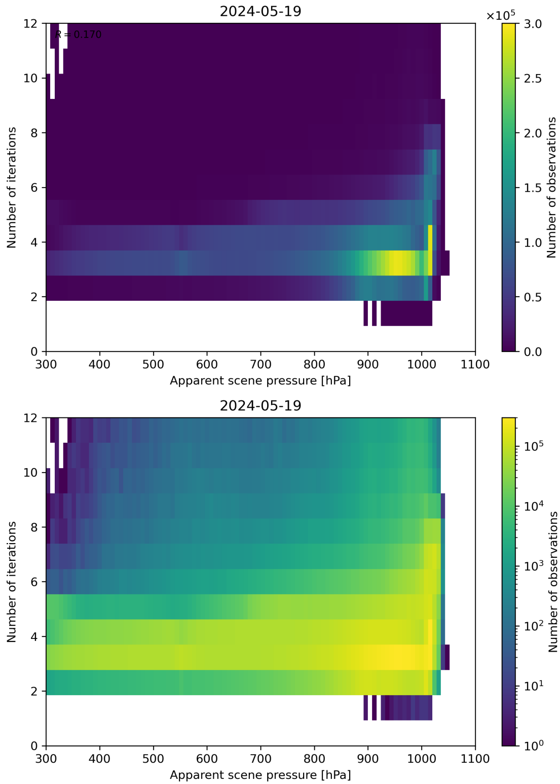
Figure 65: Scatter density plot of “Apparent scene pressure” against “Number of iterations” for 2024-05-18 to 2024-05-20.
