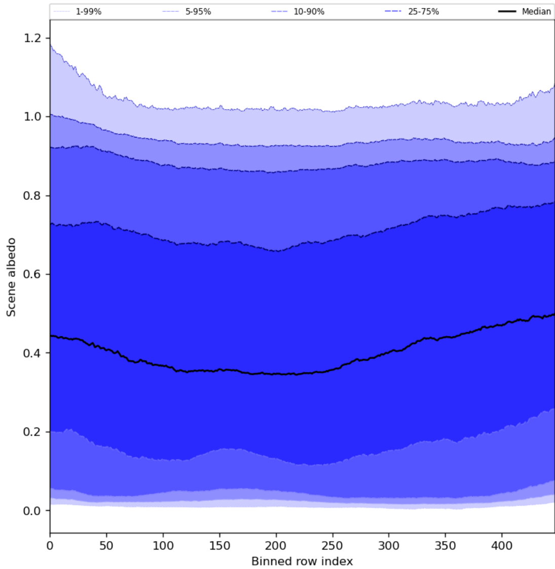
Figure 51: Along track statistics of “Scene albedo” for 2024-05-18 to 2024-05-20
