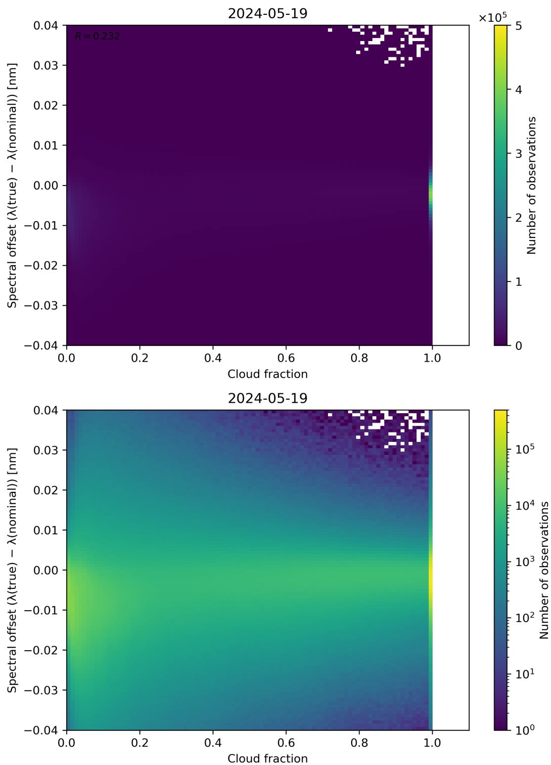
Figure 76: Scatter density plot of “Cloud fraction” against “Spectral offset ( \lambda(\text{true}) - \lambda(\text{nominal}) )” for 2024-05-18 to 2024-05-20.
