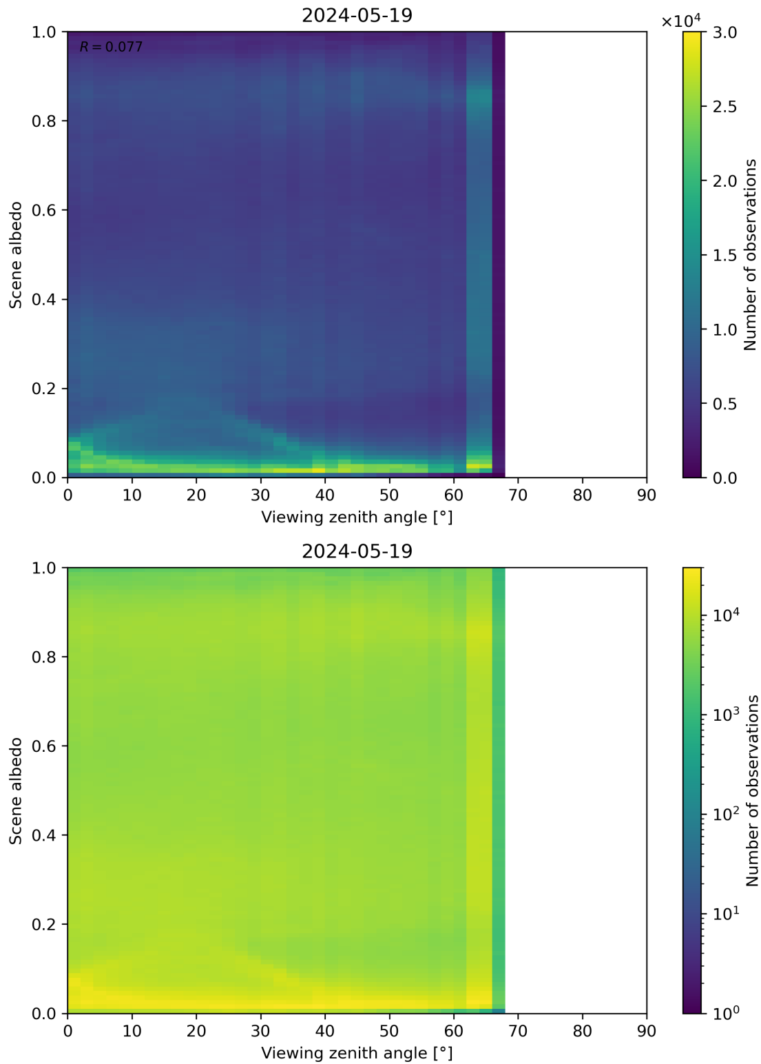
Figure 126: Scatter density plot of “Viewing zenith angle” against “Scene albedo” for 2024-05-18 to 2024-05-20.
