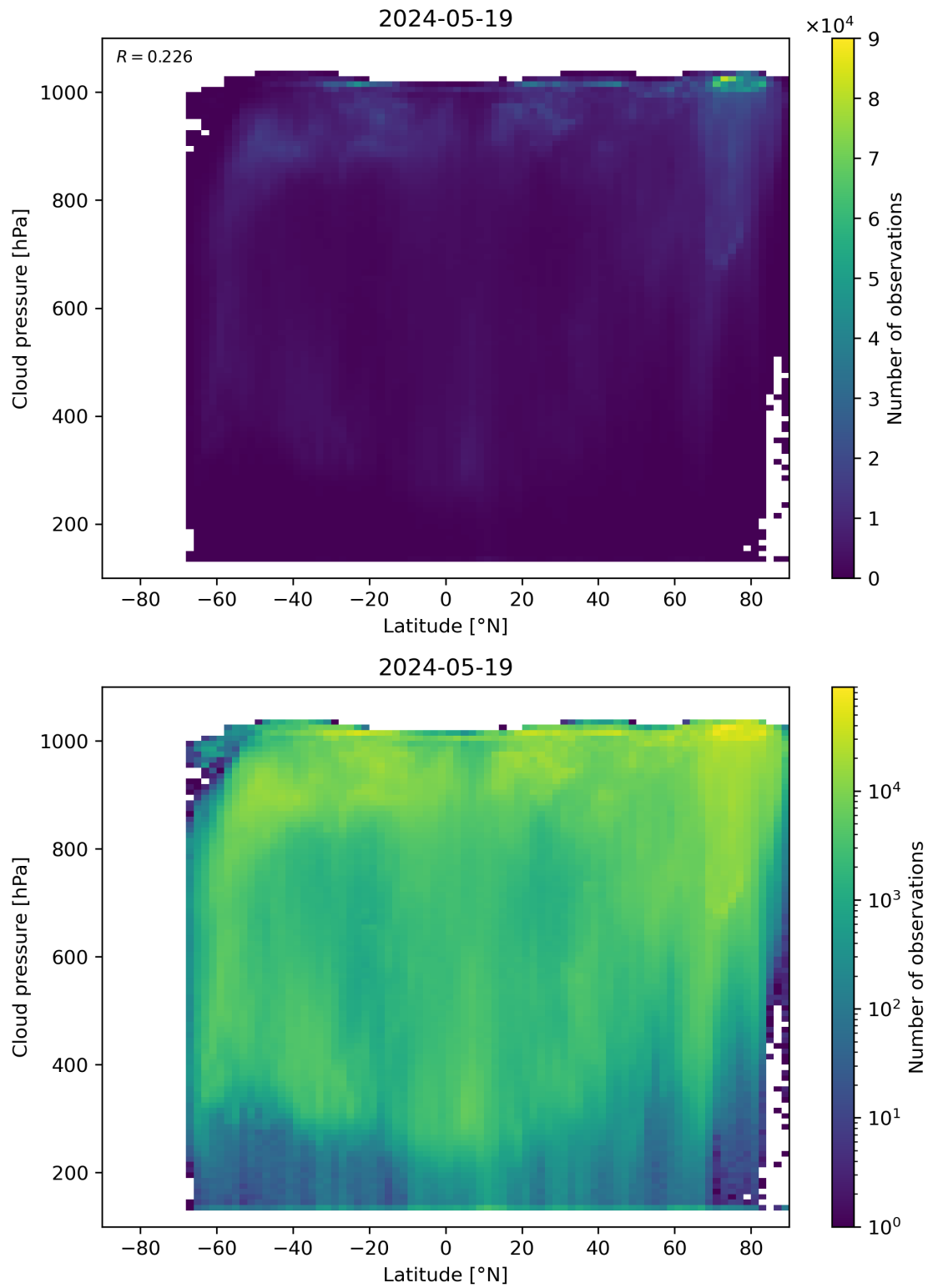
Figure 91: Scatter density plot of “Latitude” against “Cloud pressure” for 2024-05-18 to 2024-05-20.
