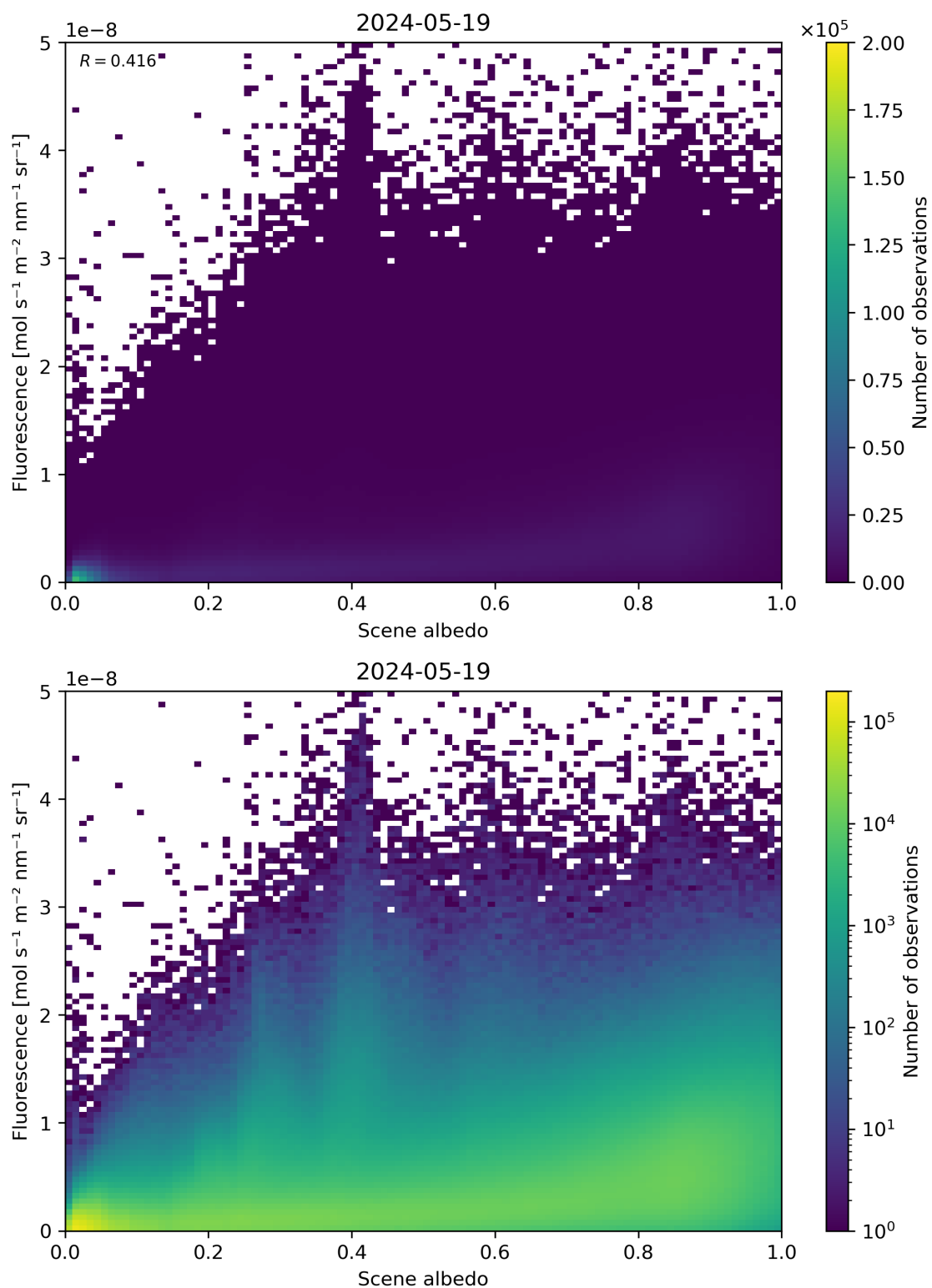
Figure 104: Scatter density plot of “Scene albedo” against “Fluorescence” for 2024-05-18 to 2024-05-20.
