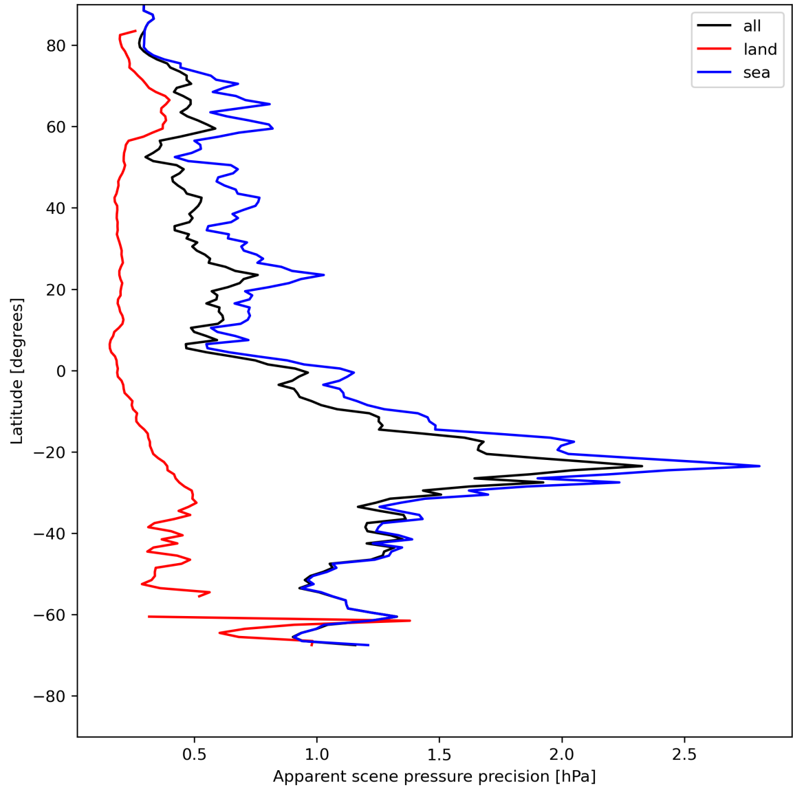
Figure 20: Zonal average of “Apparent scene pressure precision” for 2024-05-18 to 2024-05-20.
