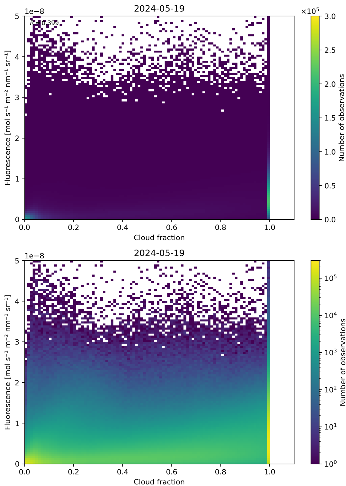
Figure 72: Scatter density plot of “Cloud fraction” against “Fluorescence” for 2024-05-18 to 2024-05-20.
