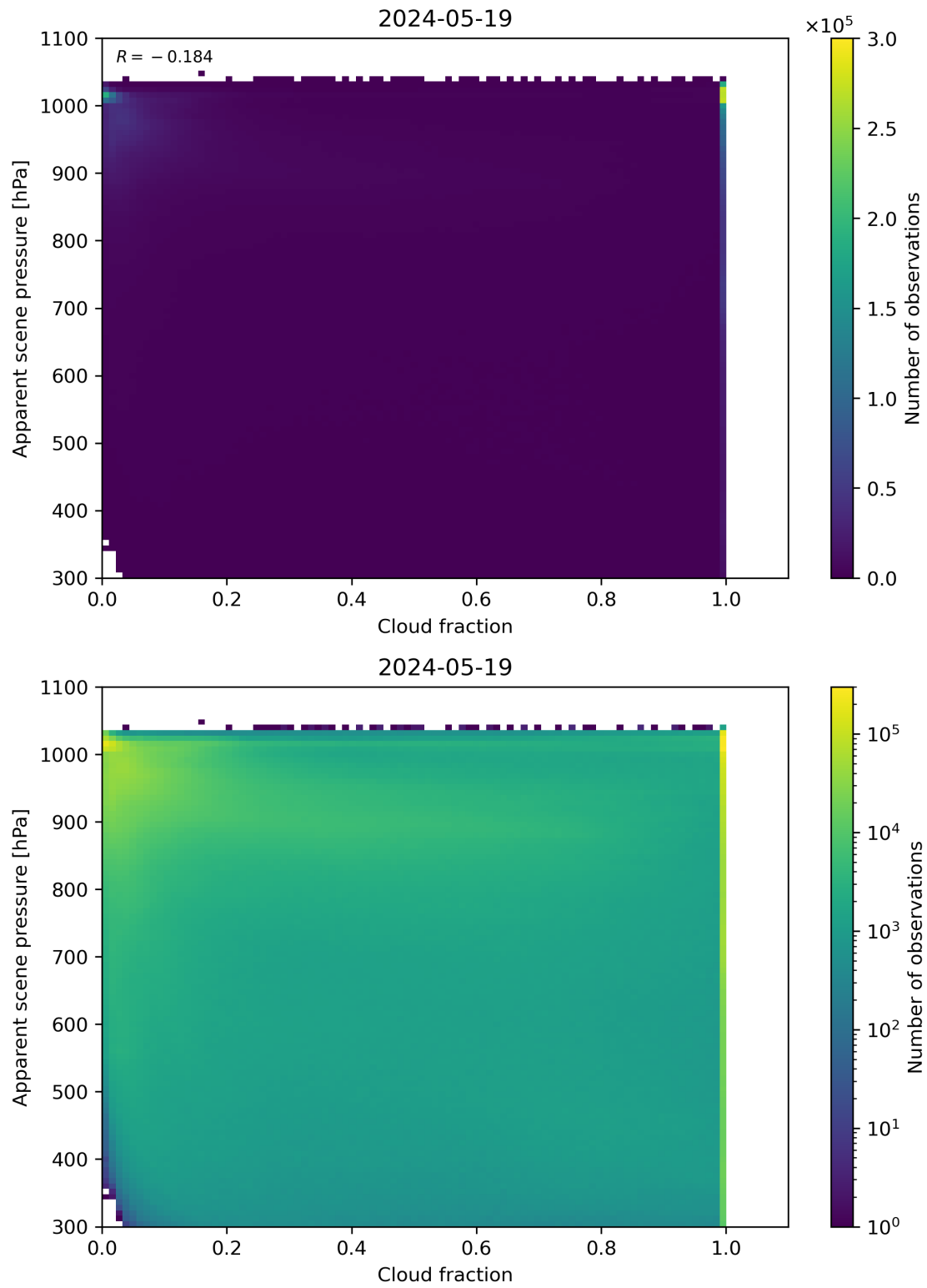
Figure 70: Scatter density plot of “Cloud fraction” against “Apparent scene pressure” for 2024-05-18 to 2024-05-20.
