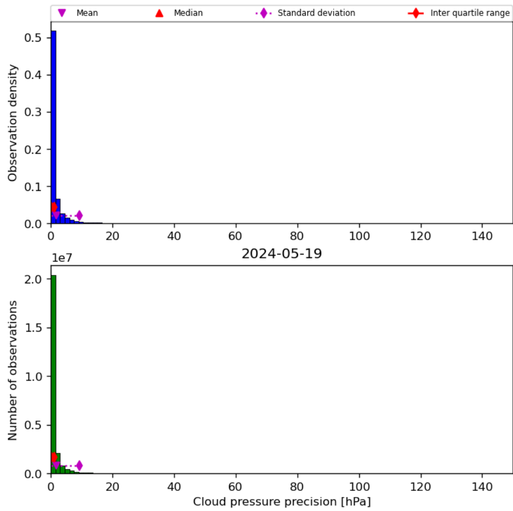
Figure 31: Histogram of “Cloud pressure precision” for 2024-05-18 to 2024-05-20
