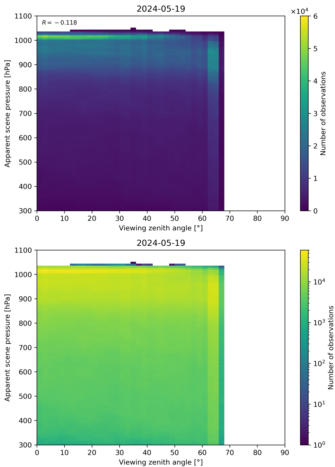
Figure 118: Scatter density plot of “Viewing zenith angle” against “Apparent scene pressure” for 2024-05-18 to 2024-05-20.
