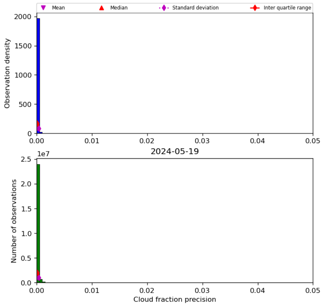
Figure 33: Histogram of “Cloud fraction precision” for 2024-05-18 to 2024-05-20
