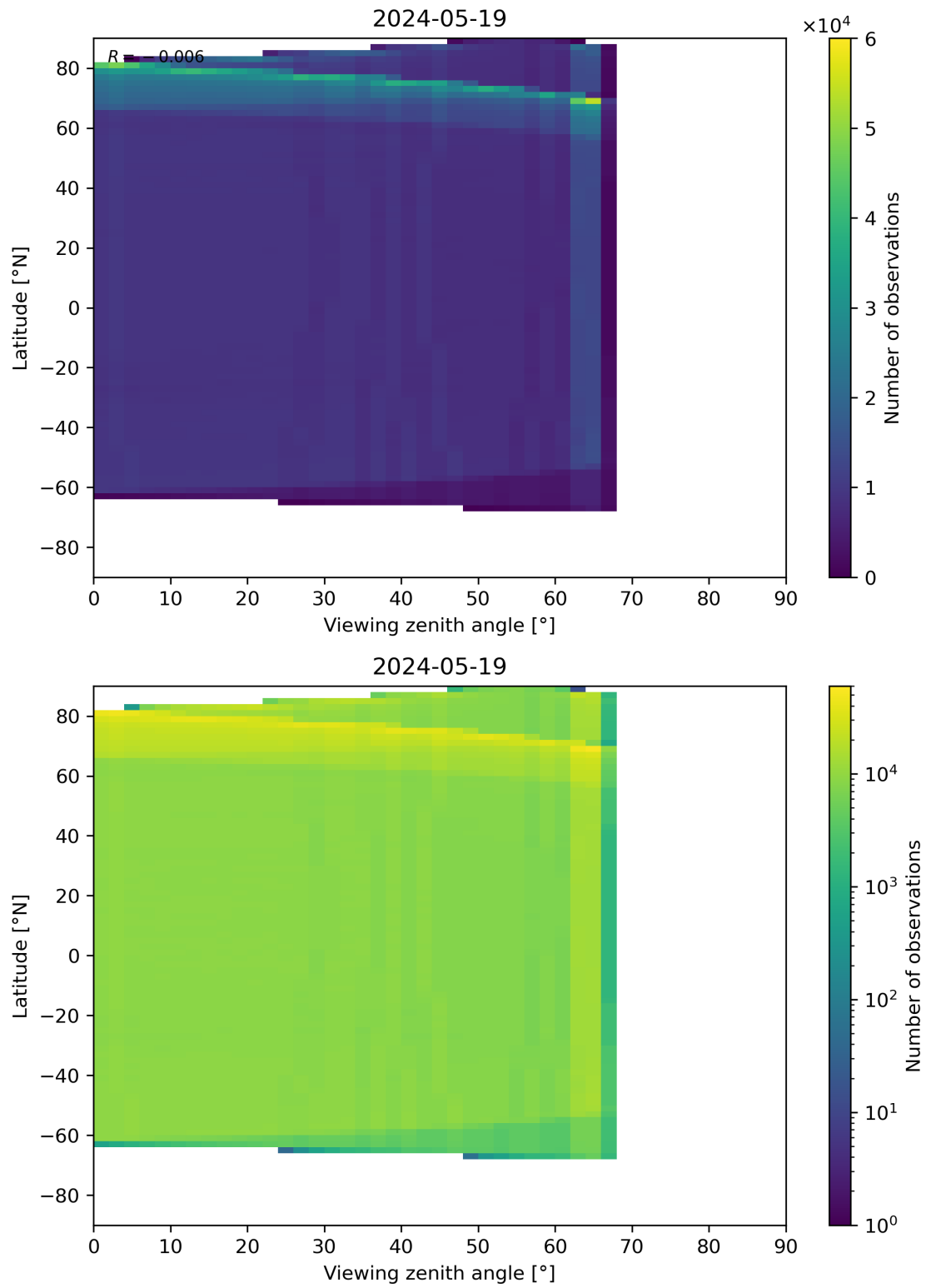
Figure 123: Scatter density plot of “Viewing zenith angle” against “Latitude” for 2024-05-18 to 2024-05-20.
