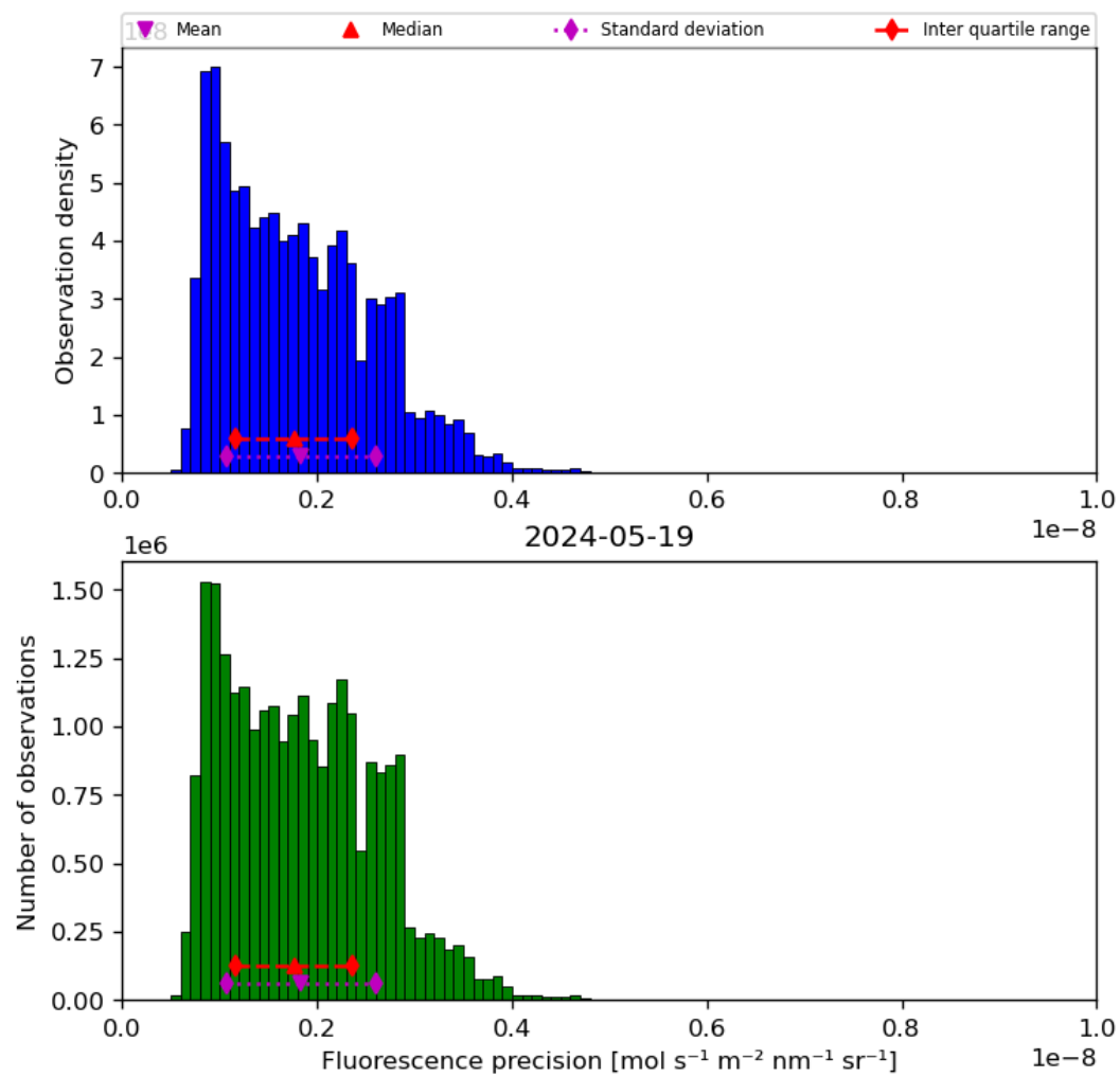
Figure 41: Histogram of “Fluorescence precision” for 2024-05-18 to 2024-05-20
