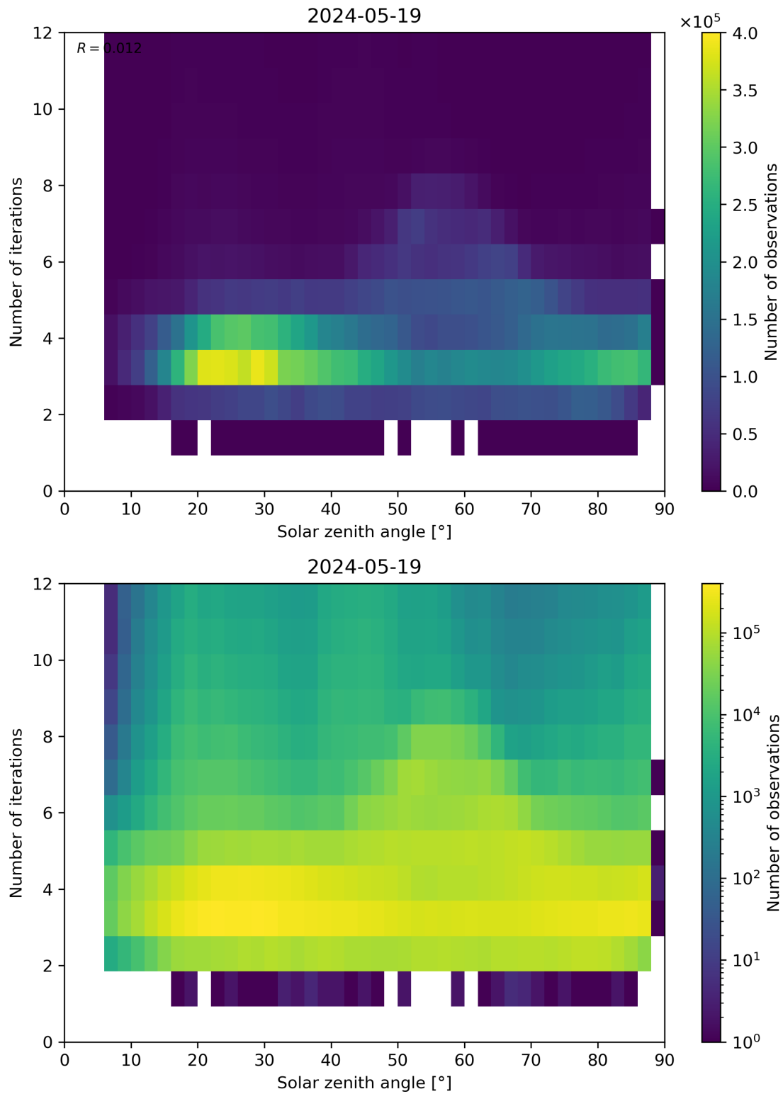
Figure 114: Scatter density plot of “Solar zenith angle” against “Number of iterations” for 2024-05-18 to 2024-05-20.
