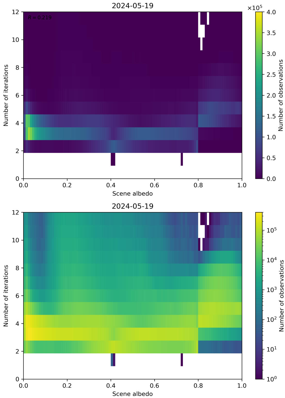
Figure 105: Scatter density plot of “Scene albedo” against “Number of iterations” for 2024-05-18 to 2024-05-20.
