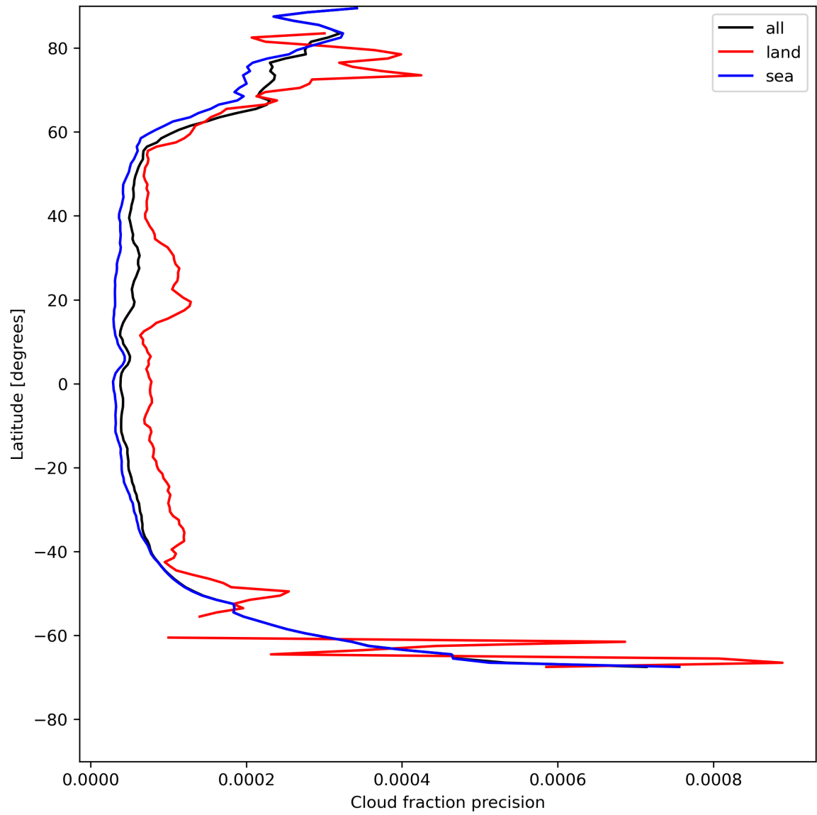
Figure 16: Zonal average of “Cloud fraction precision” for 2024-05-18 to 2024-05-20.
