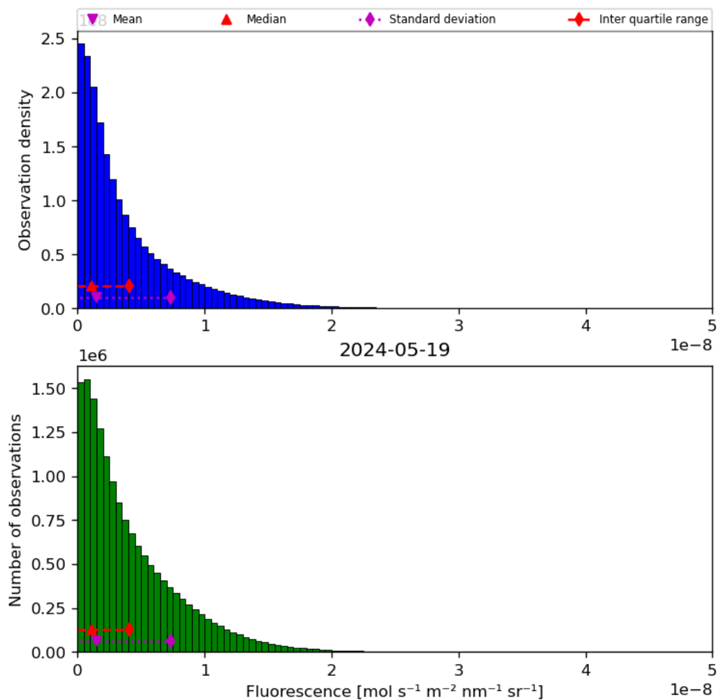
Figure 40: Histogram of “Fluorescence” for 2024-05-18 to 2024-05-20
