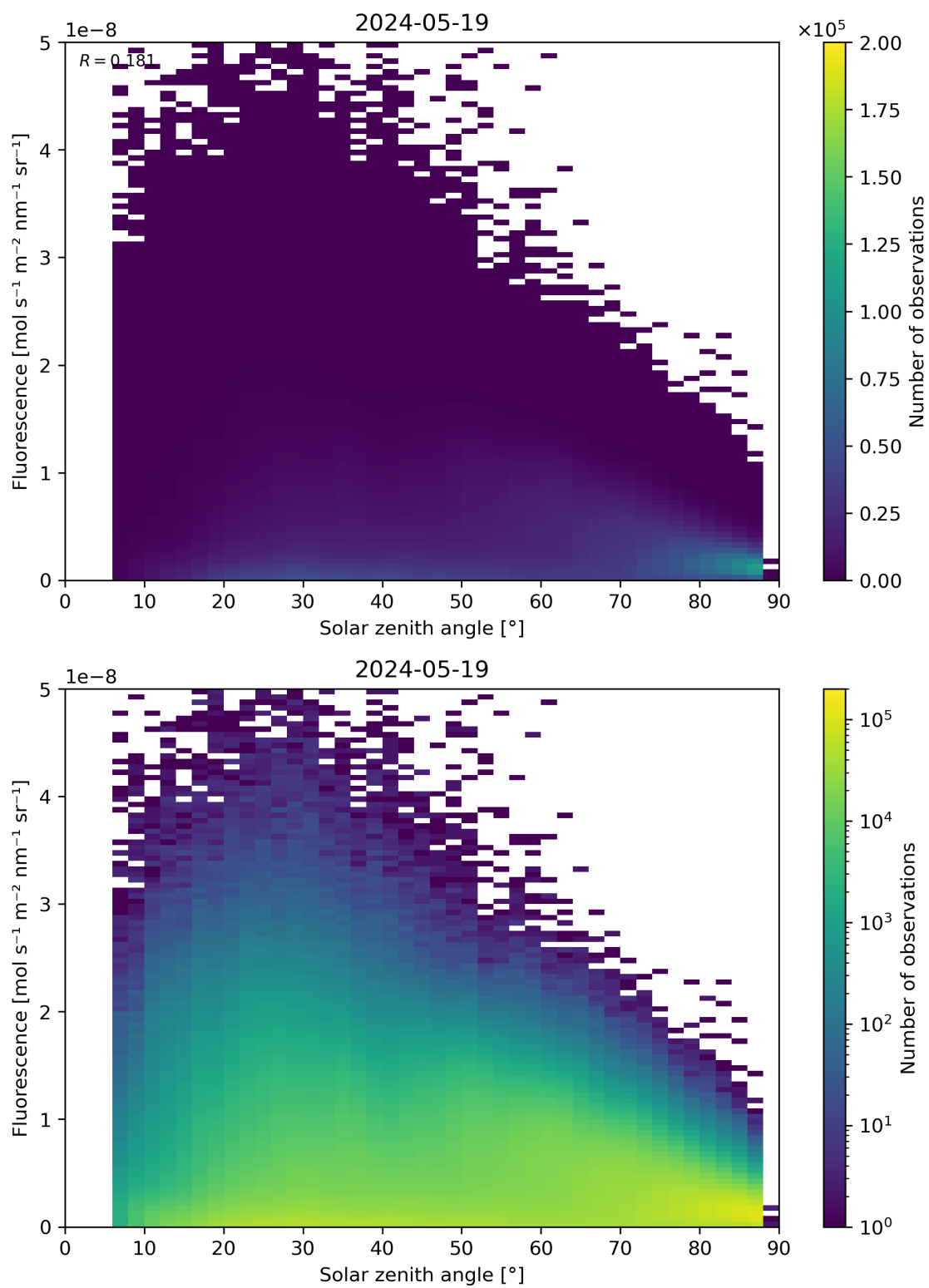
Figure 112: Scatter density plot of “Solar zenith angle” against “Fluorescence” for 2024-05-18 to 2024-05-20.
