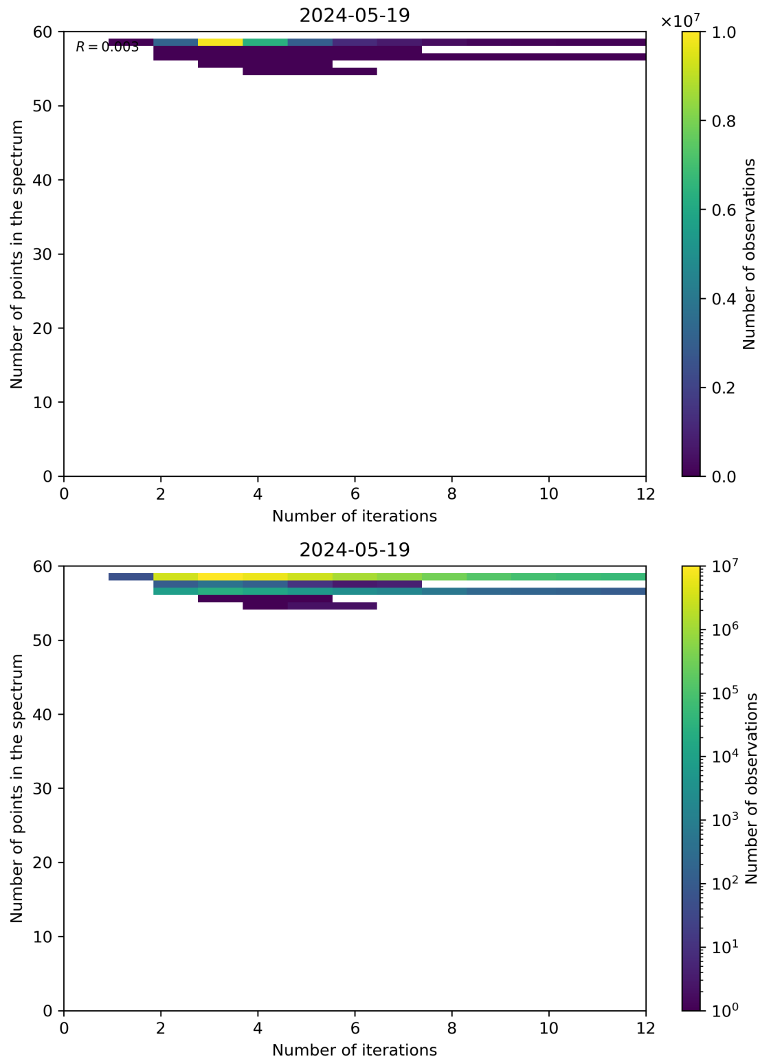
Figure 99: Scatter density plot of “Number of iterations” against “Number of points in the spectrum” for 2024-05-18 to 2024-05-20.
