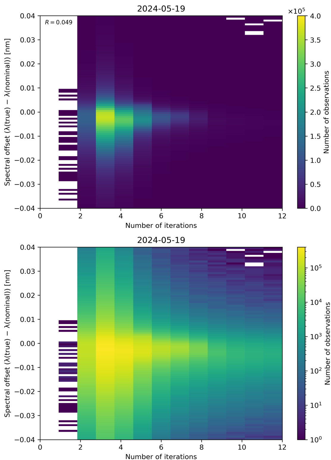
Figure 100: Scatter density plot of “Number of iterations” against “Spectral offset ( \lambda(\text{true}) - \lambda(\text{nominal}) )” for 2024-05-18 to 2024-05-20.
