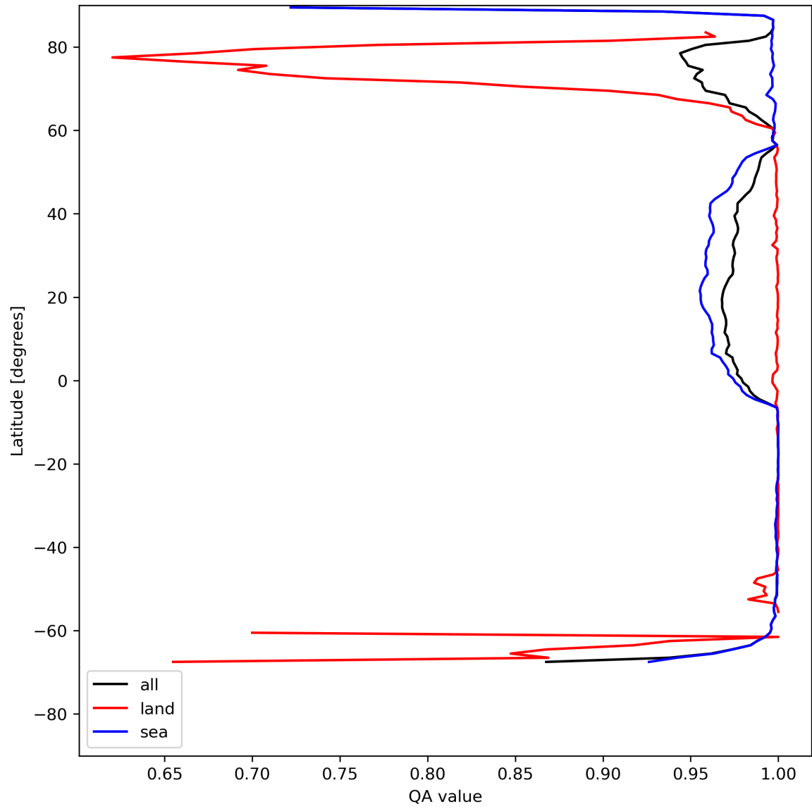
Figure 12: Zonal average of “QA value” for 2024-05-18 to 2024-05-20.
