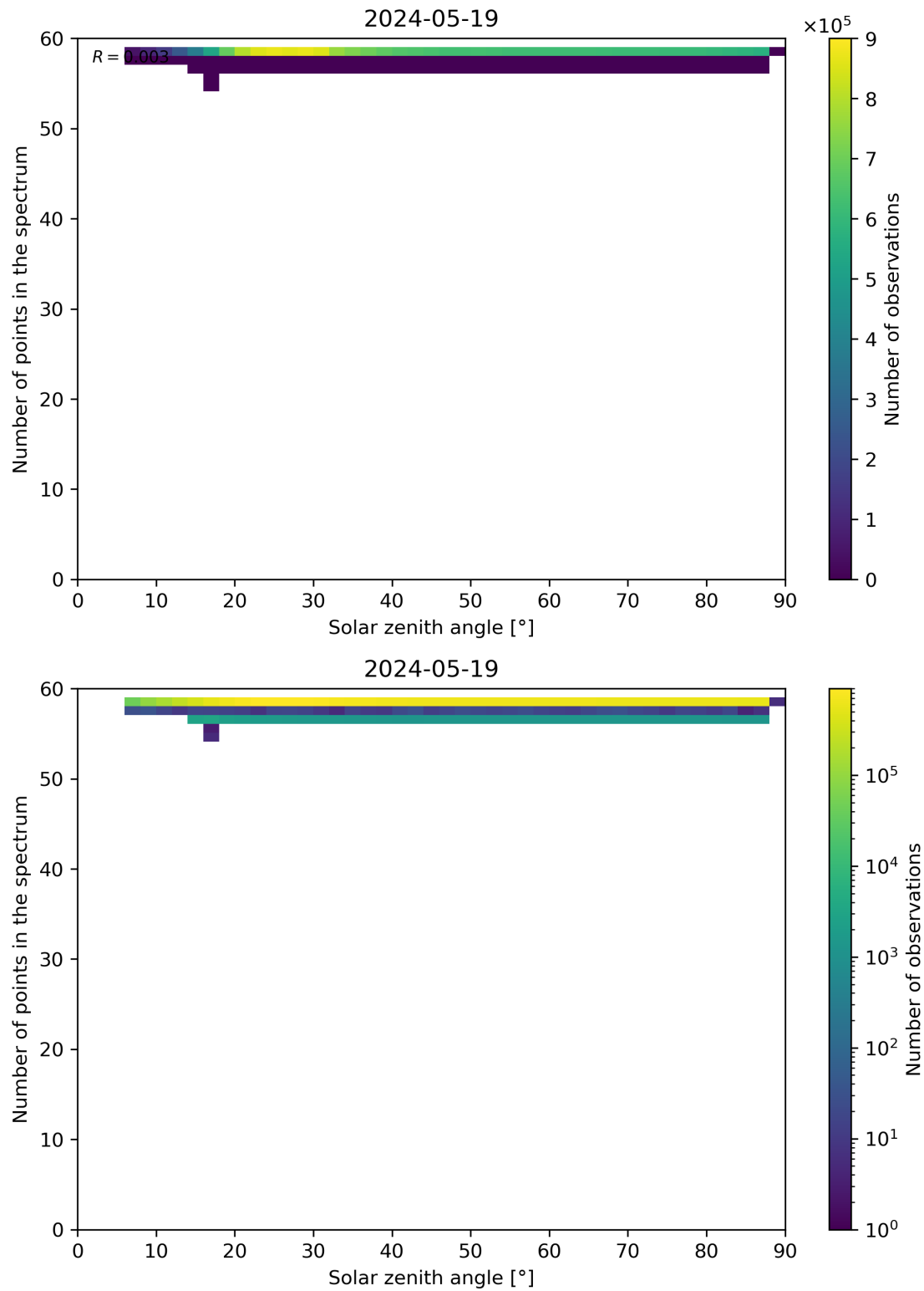
Figure 115: Scatter density plot of “Solar zenith angle” against “Number of points in the spectrum” for 2024-05-18 to 2024-05-20.
