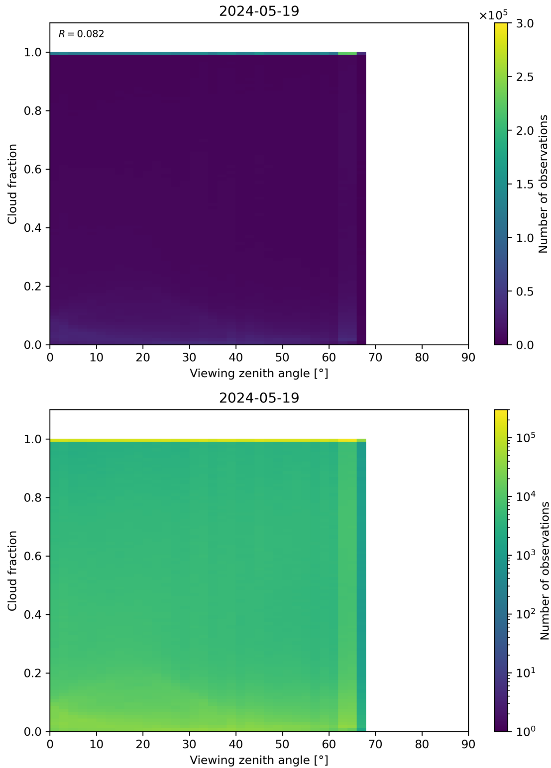
Figure 120: Scatter density plot of “Viewing zenith angle” against “Cloud fraction” for 2024-05-18 to 2024-05-20.
