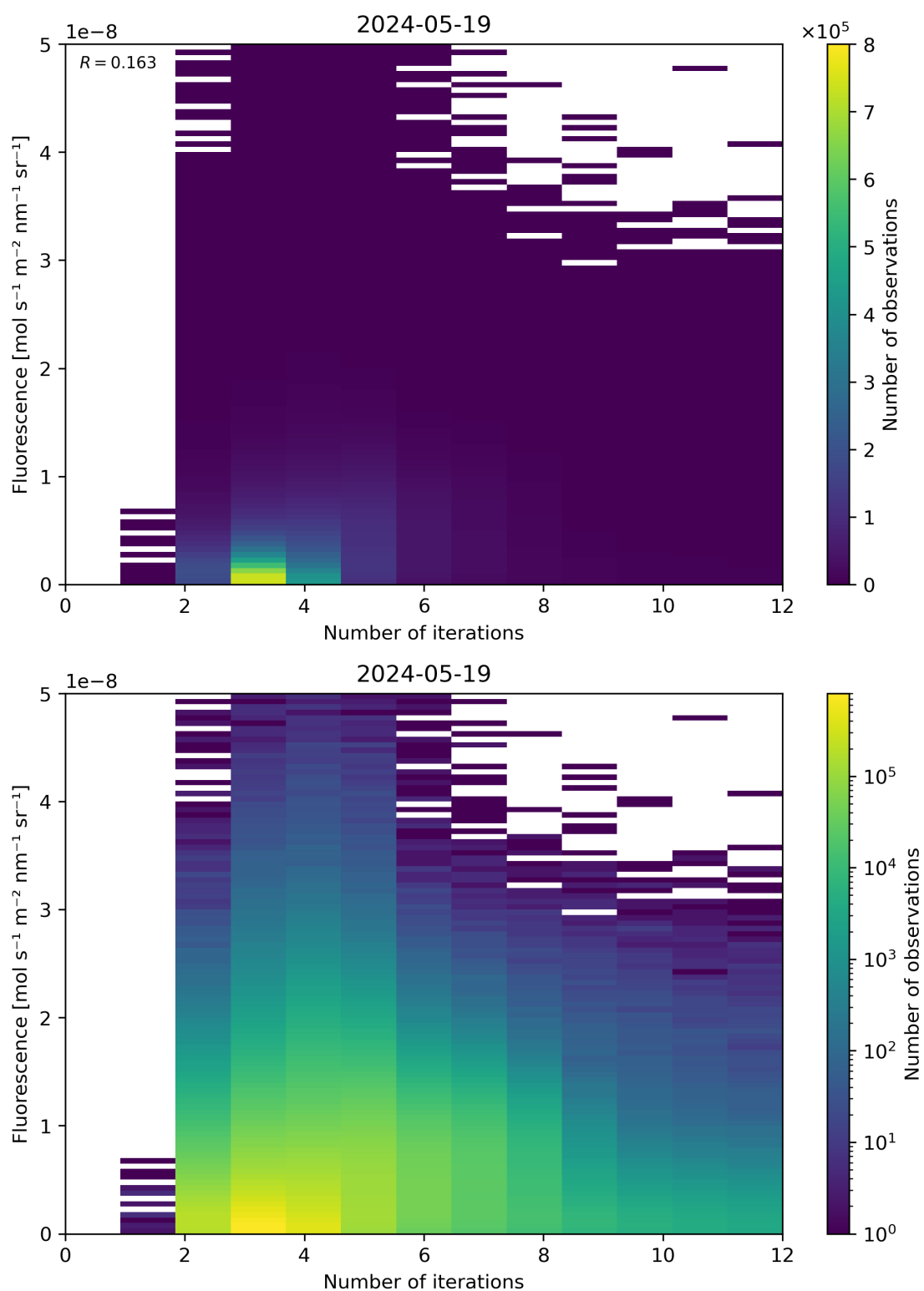
Figure 98: Scatter density plot of “Number of iterations” against “Fluorescence” for 2024-05-18 to 2024-05-20.
