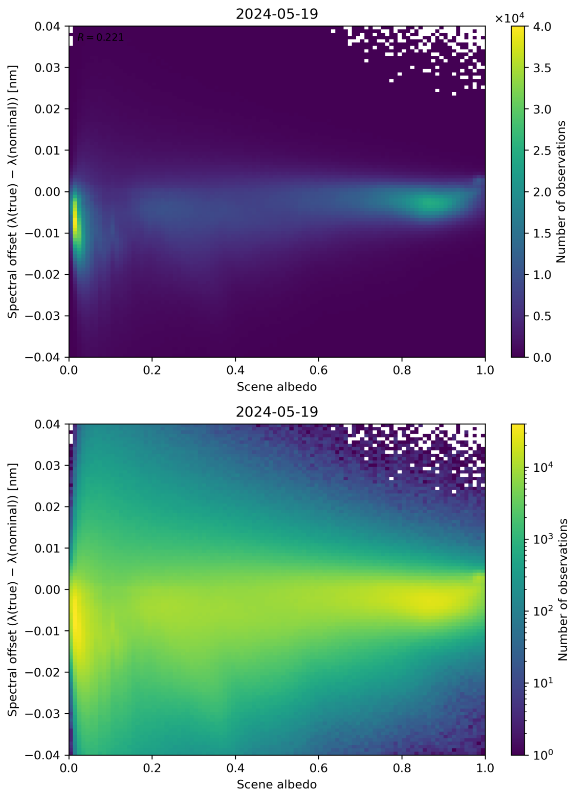
Figure 107: Scatter density plot of “Scene albedo” against “Spectral offset ( \lambda(\text{true}) - \lambda(\text{nominal}) )” for 2024-05-18 to 2024-05-20.
