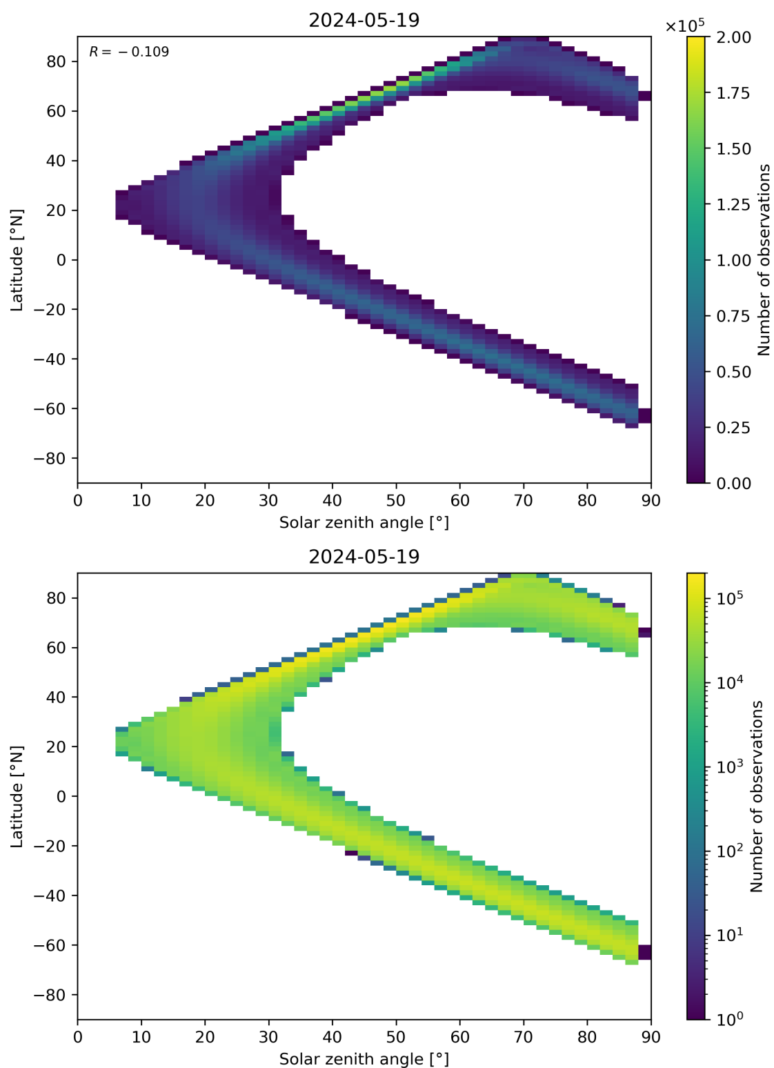
Figure 113: Scatter density plot of “Solar zenith angle” against “Latitude” for 2024-05-18 to 2024-05-20.
