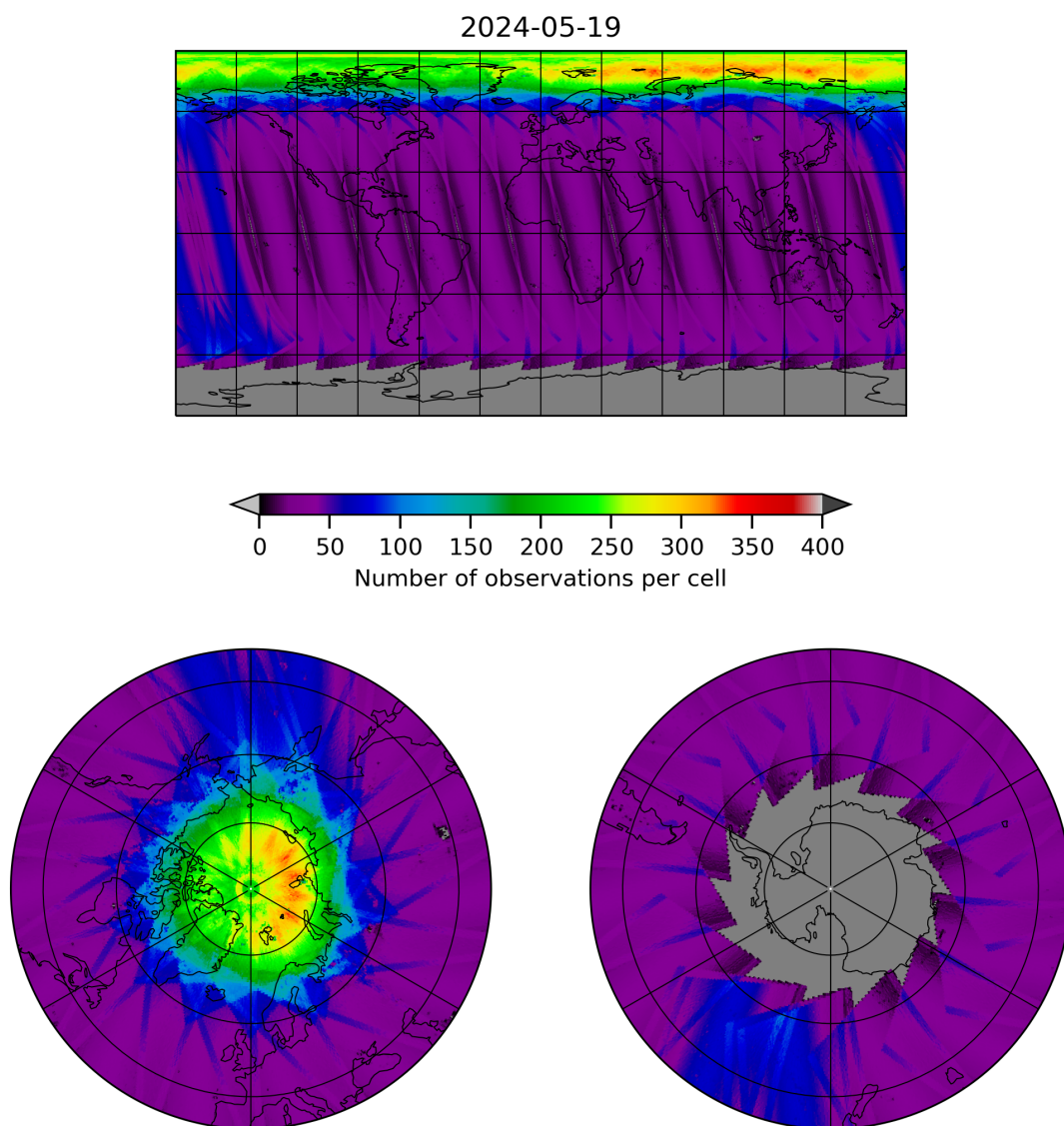
Figure 11: Map of the number of observations for 2024-05-18 to 2024-05-20
