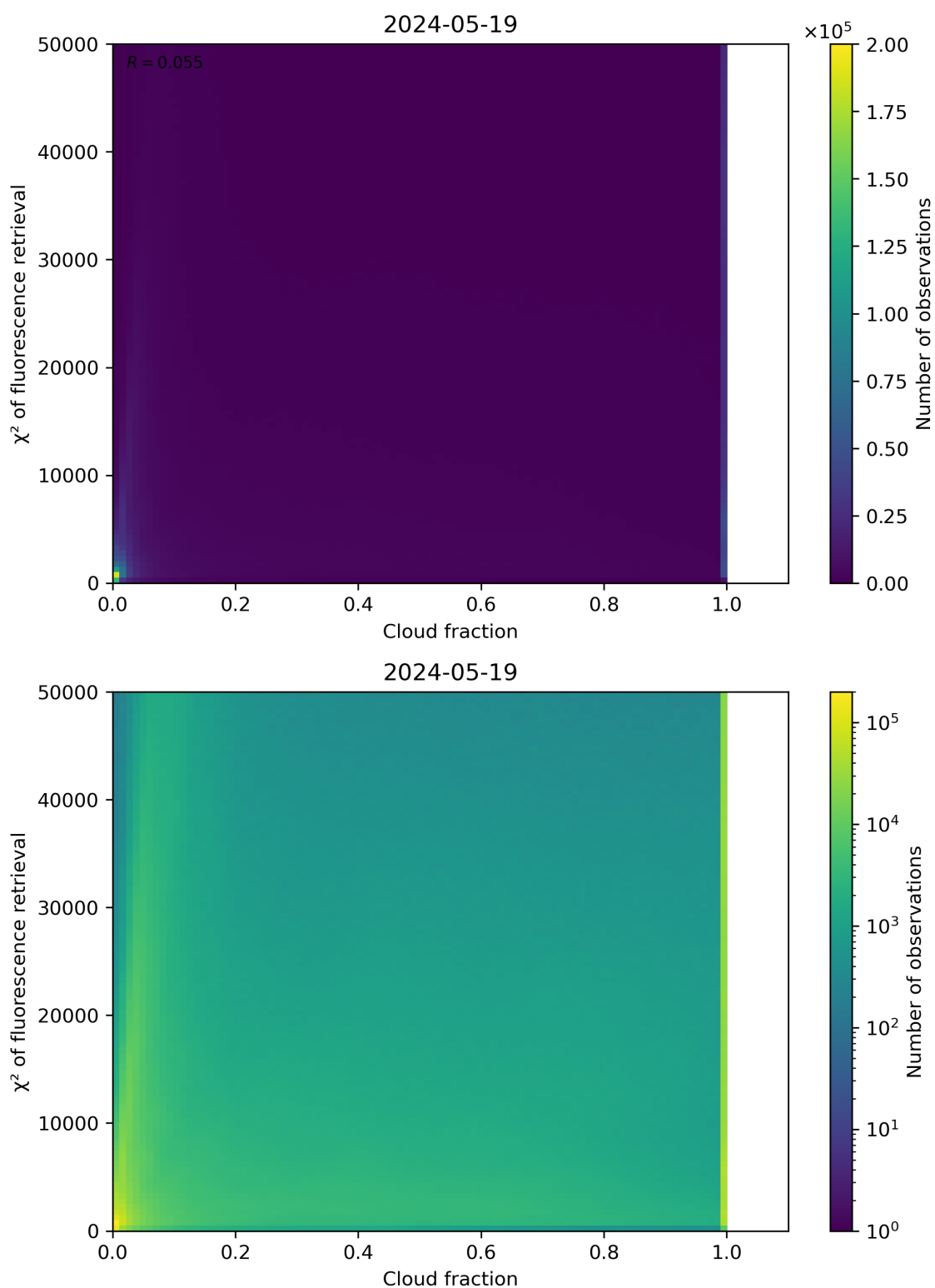
Figure 71: Scatter density plot of “Cloud fraction” against “ \chi^2 of fluorescence retrieval” for 2024-05-18 to 2024-05-20.
