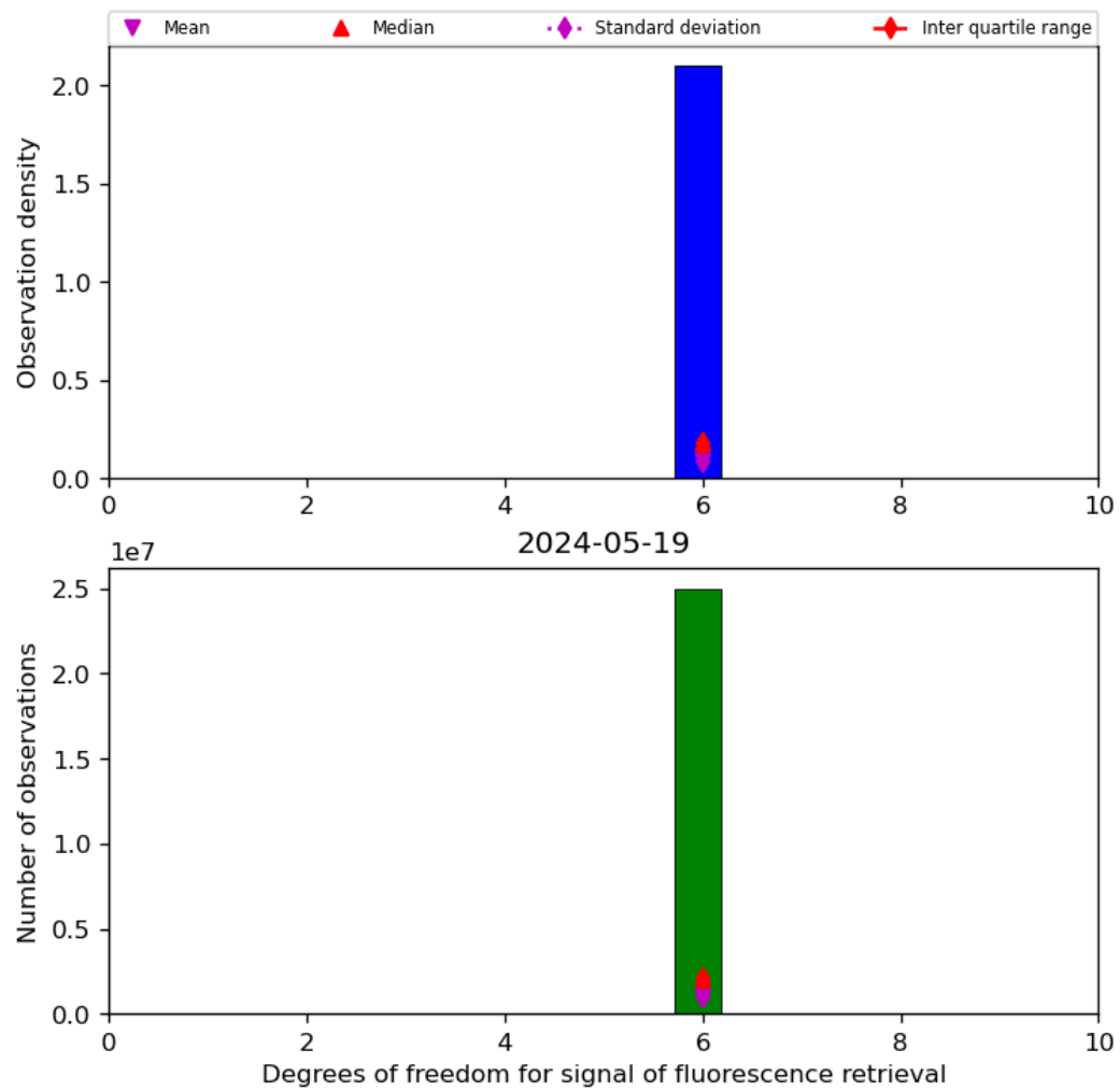
Figure 43: Histogram of “Degrees of freedom for signal of fluorescence retrieval” for 2024-05-18 to 2024-05-20
