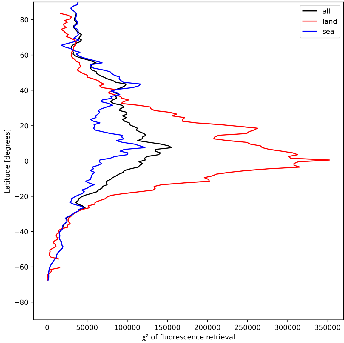
Figure 25: Zonal average of “ \chi^2 of fluorescence retrieval” for 2024-05-18 to 2024-05-20.
