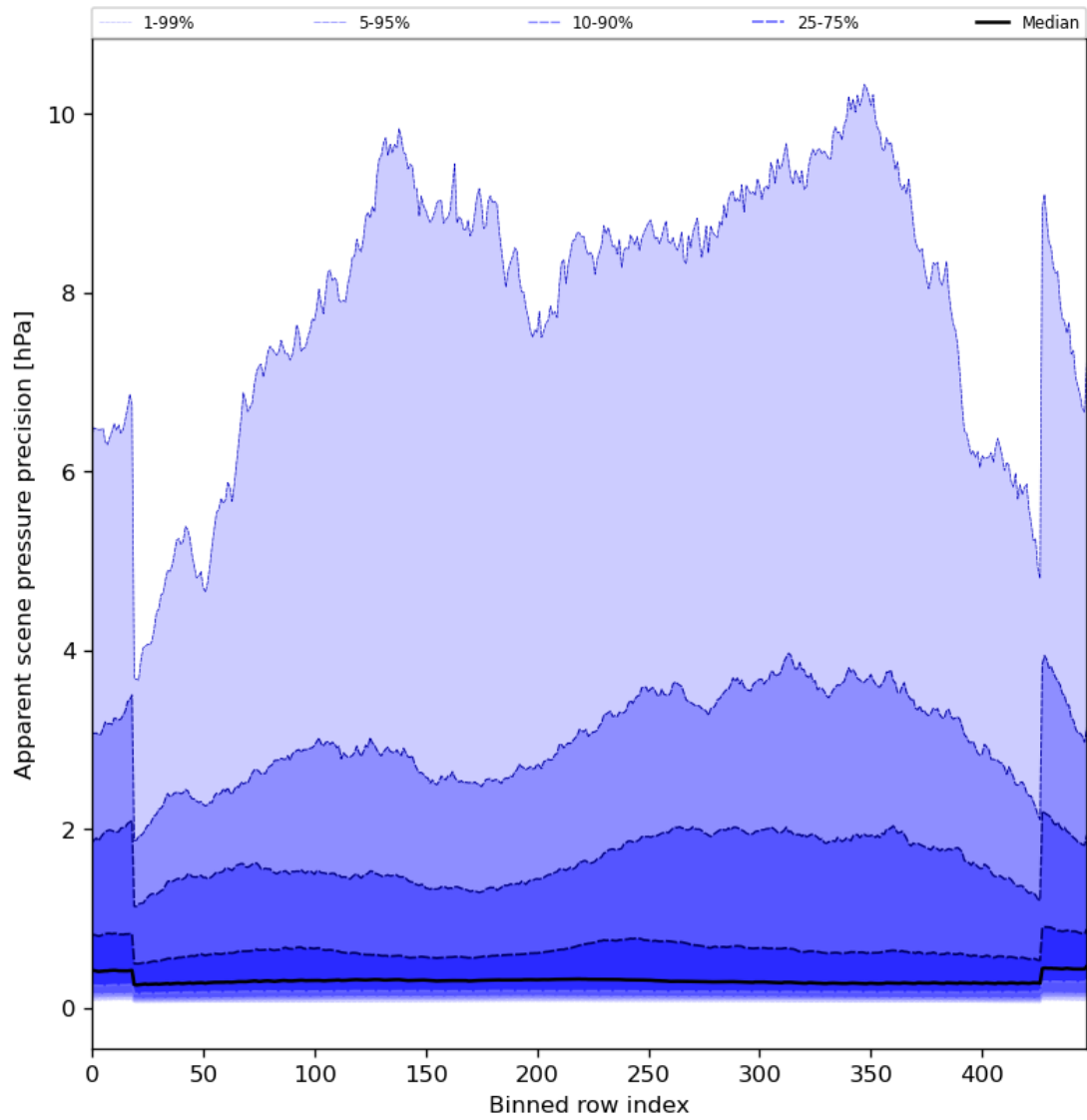
Figure 54: Along track statistics of “Apparent scene pressure precision” for 2024-05-18 to 2024-05-20
