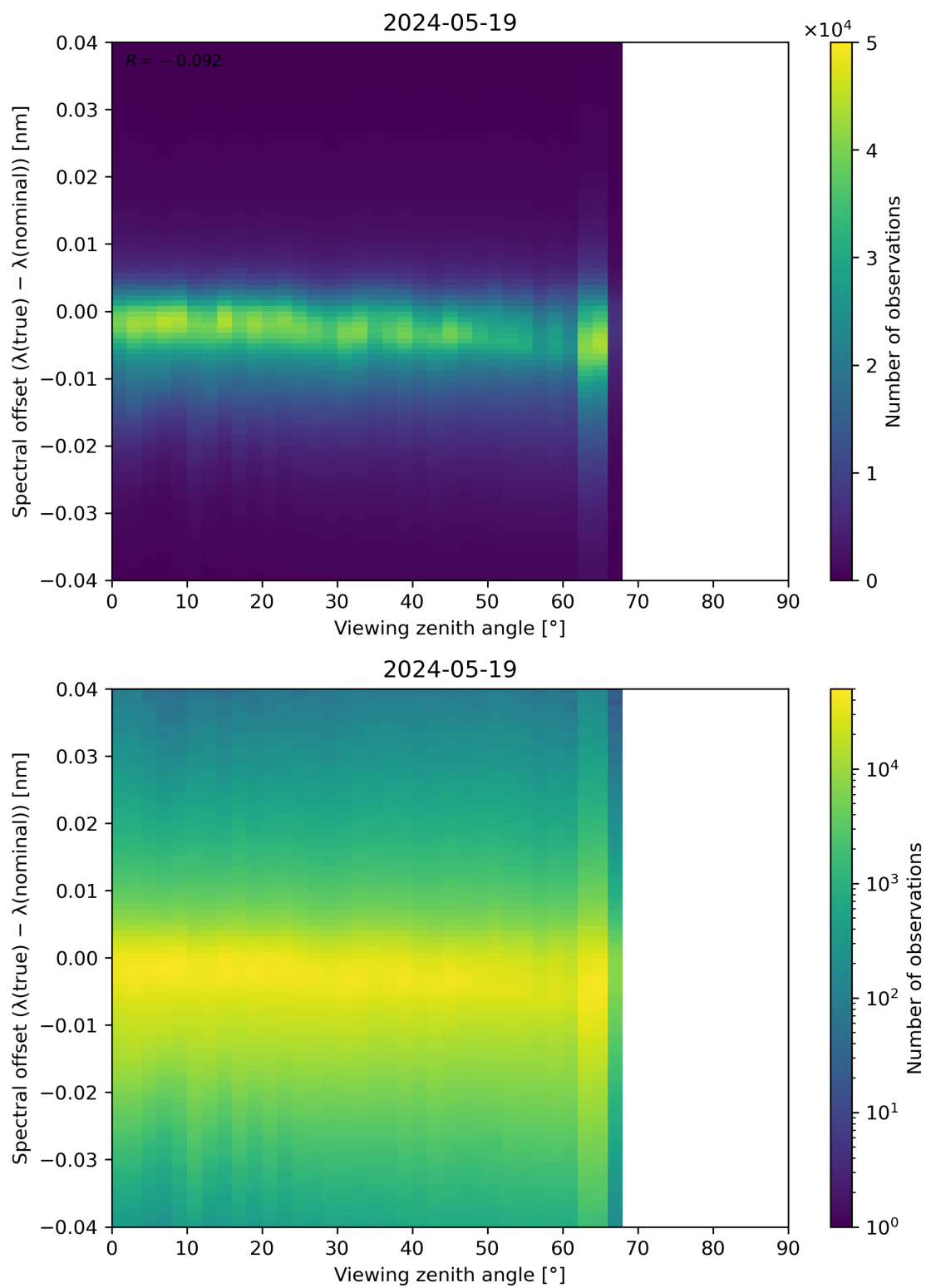
Figure 128: Scatter density plot of “Viewing zenith angle” against “Spectral offset ( \lambda(\text{true}) - \lambda(\text{nominal}) )” for 2024-05-18 to 2024-05-20.
