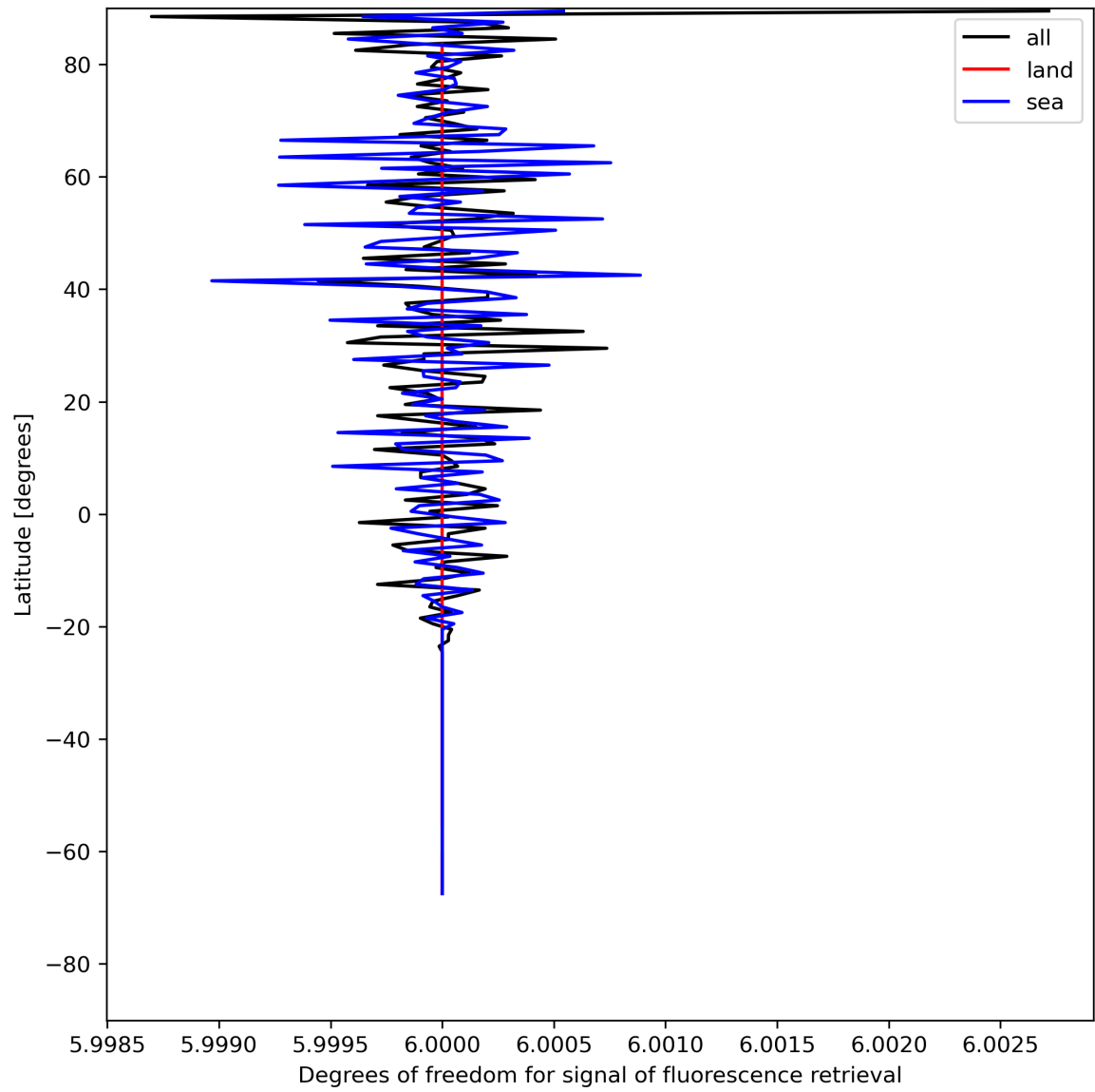
Figure 26: Zonal average of “Degrees of freedom for signal of fluorescence retrieval” for 2024-05-18 to 2024-05-20.
