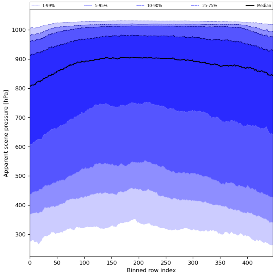
Figure 53: Along track statistics of “Apparent scene pressure” for 2024-05-18 to 2024-05-20
