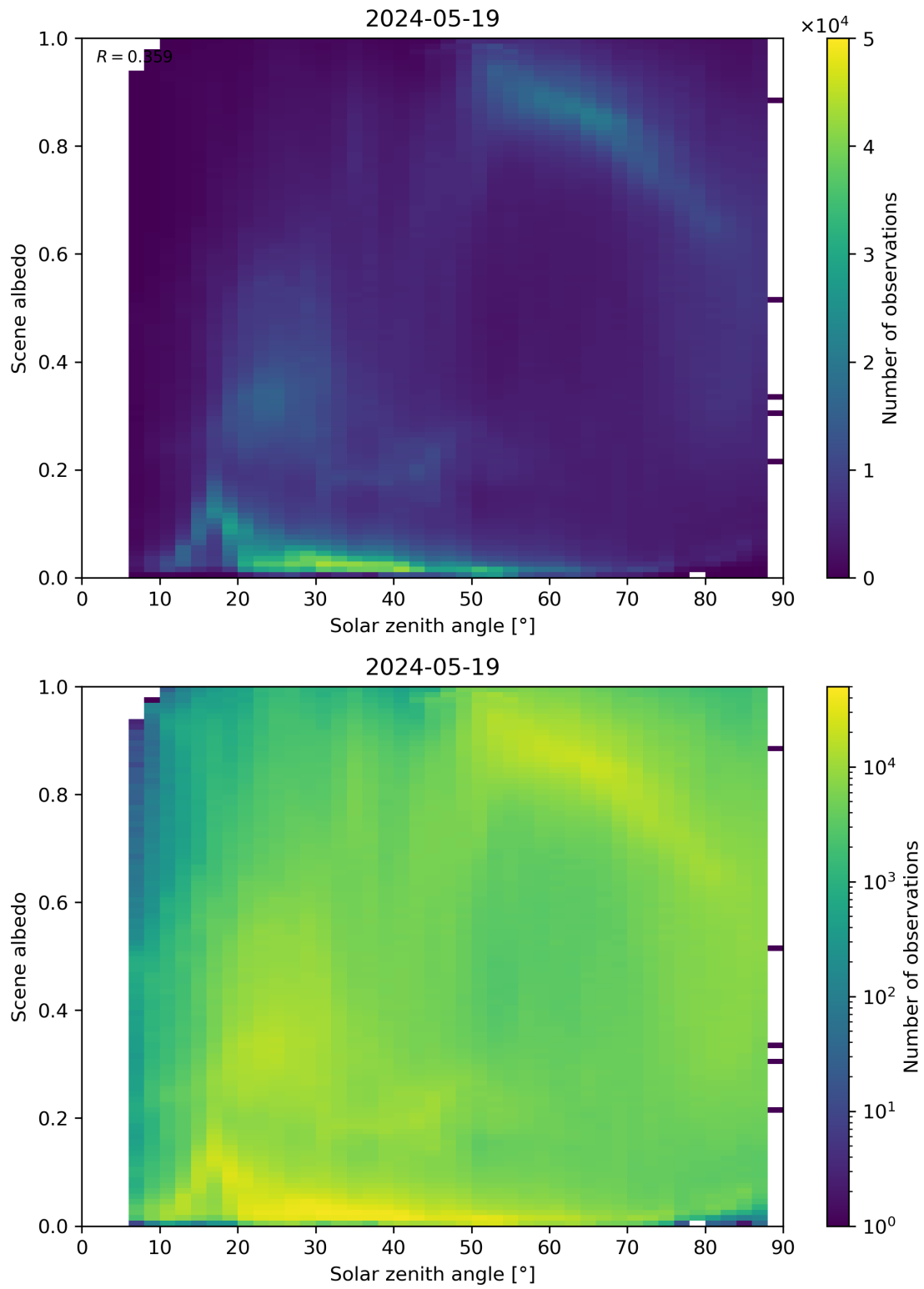
Figure 116: Scatter density plot of “Solar zenith angle” against “Scene albedo” for 2024-05-18 to 2024-05-20.
