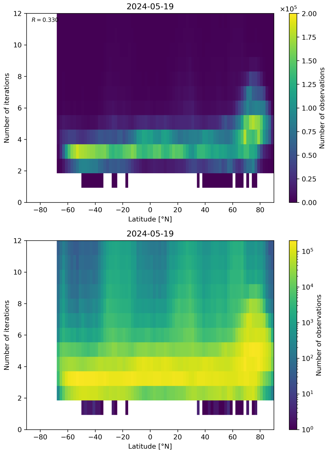
Figure 93: Scatter density plot of “Latitude” against “Number of iterations” for 2024-05-18 to 2024-05-20.
