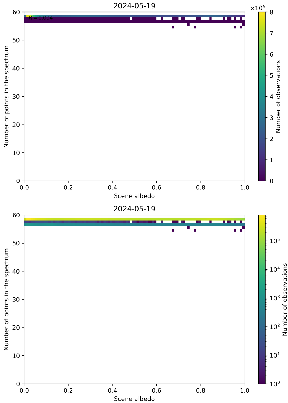
Figure 106: Scatter density plot of “Scene albedo” against “Number of points in the spectrum” for 2024-05-18 to 2024-05-20.
