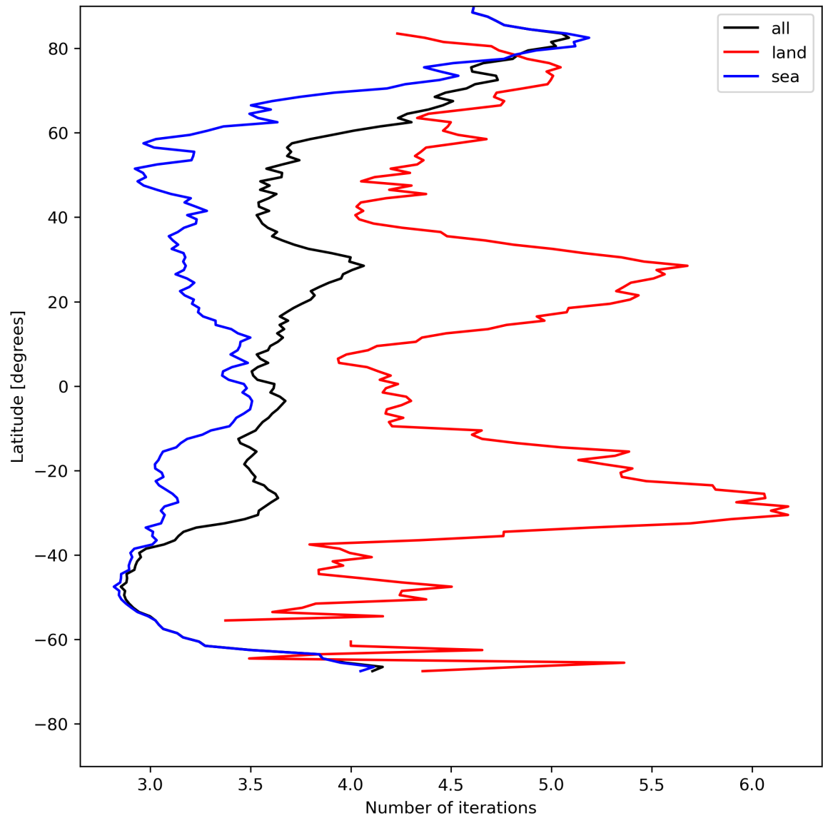
Figure 22: Zonal average of “Number of iterations” for 2024-05-18 to 2024-05-20.
