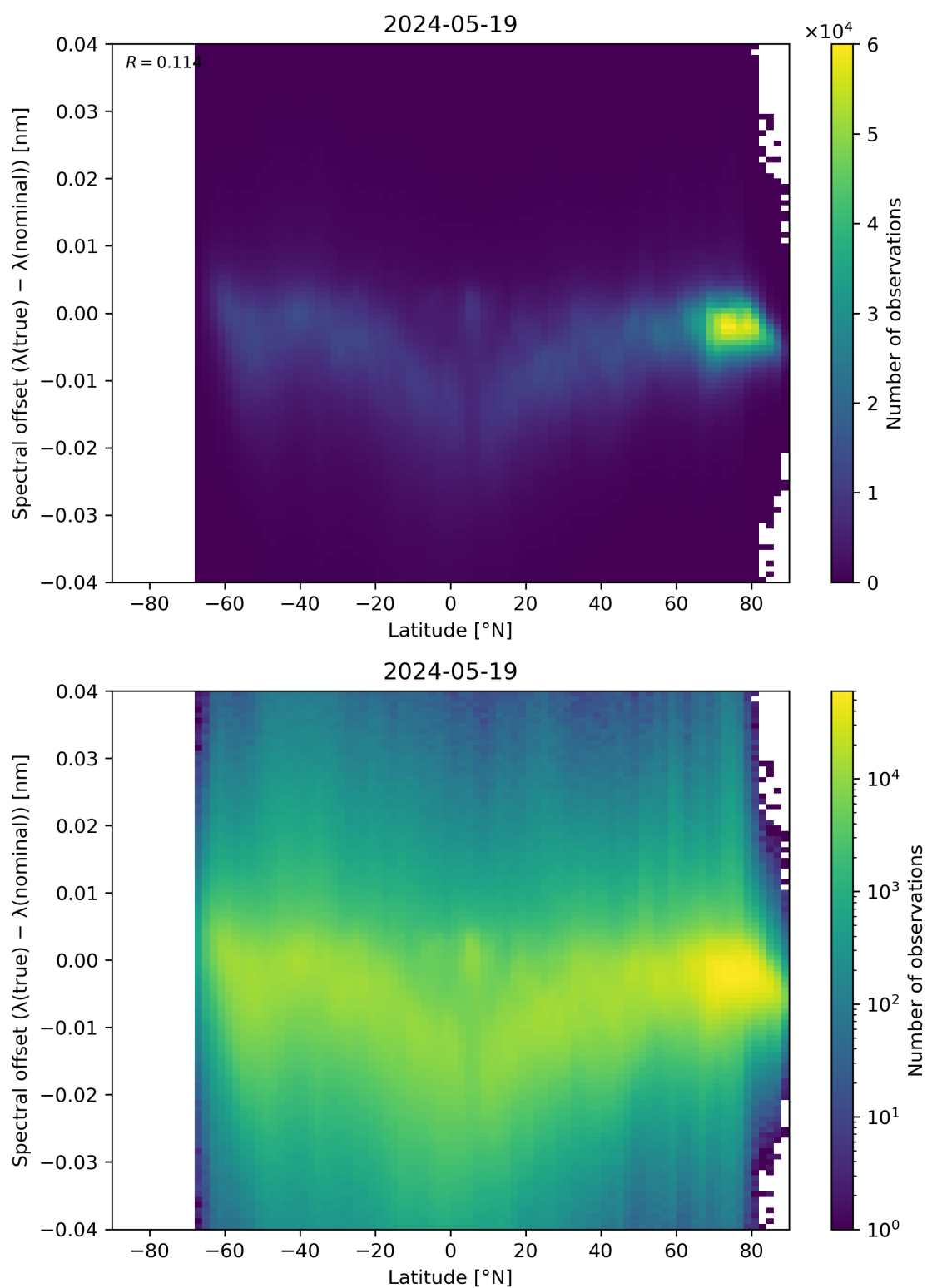
Figure 96: Scatter density plot of “Latitude” against “Spectral offset ( \lambda(\text{true}) - \lambda(\text{nominal}) )” for 2024-05-18 to 2024-05-20.
