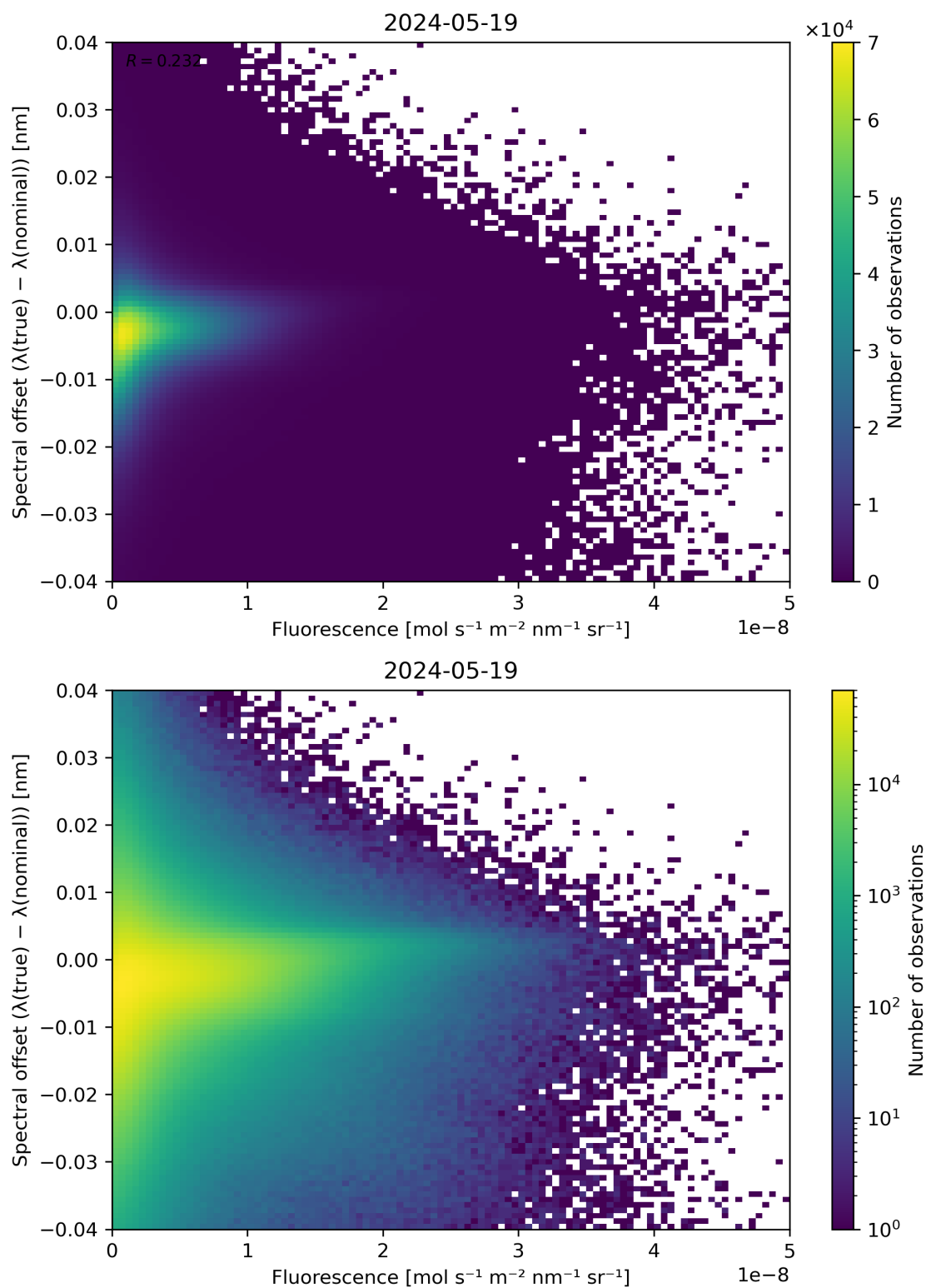
Figure 87: Scatter density plot of “Fluorescence” against “Spectral offset ( \lambda(\text{true}) - \lambda(\text{nominal}) )” for 2024-05-18 to 2024-05-20.
