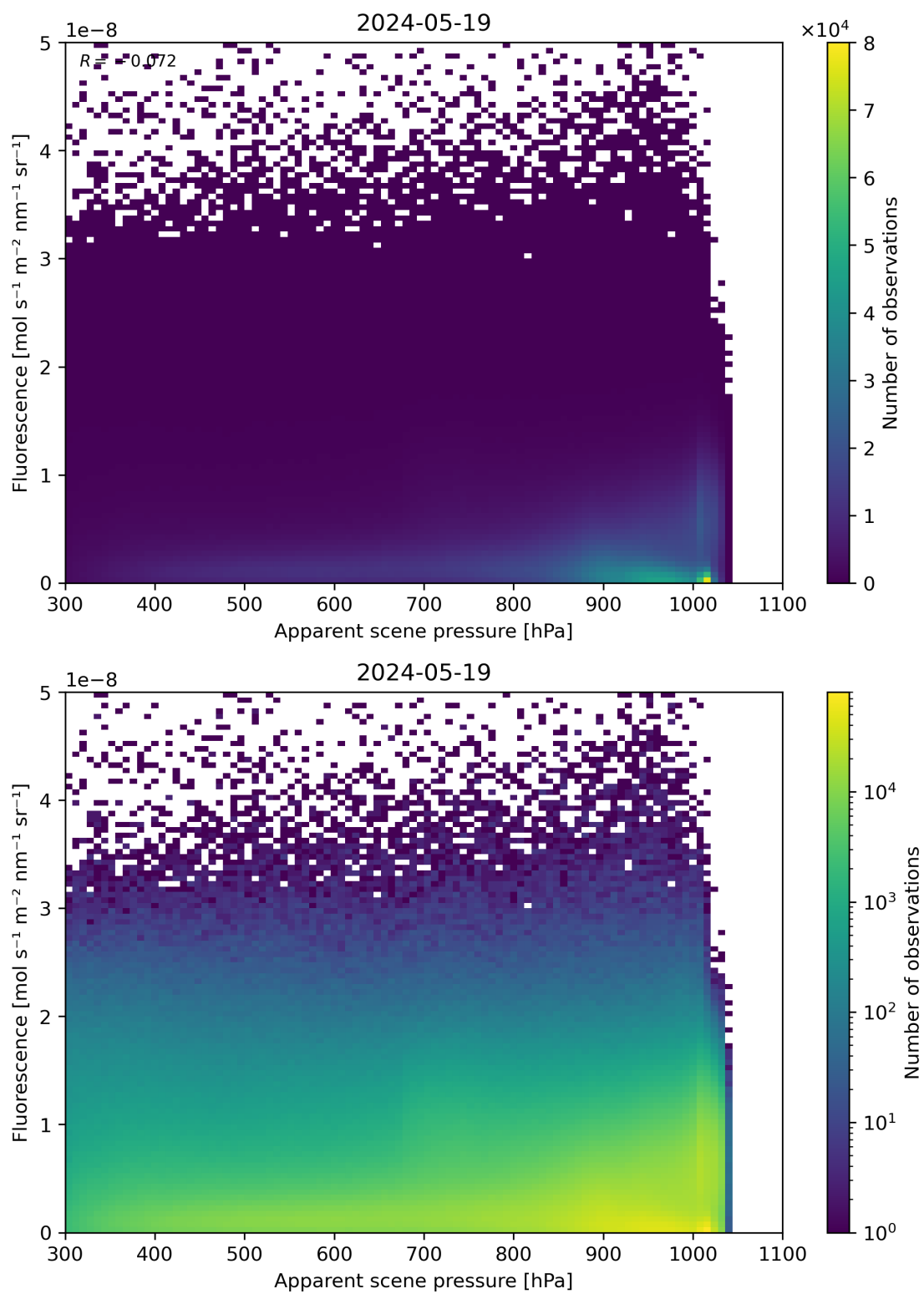
Figure 64: Scatter density plot of “Apparent scene pressure” against “Fluorescence” for 2024-05-18 to 2024-05-20.
