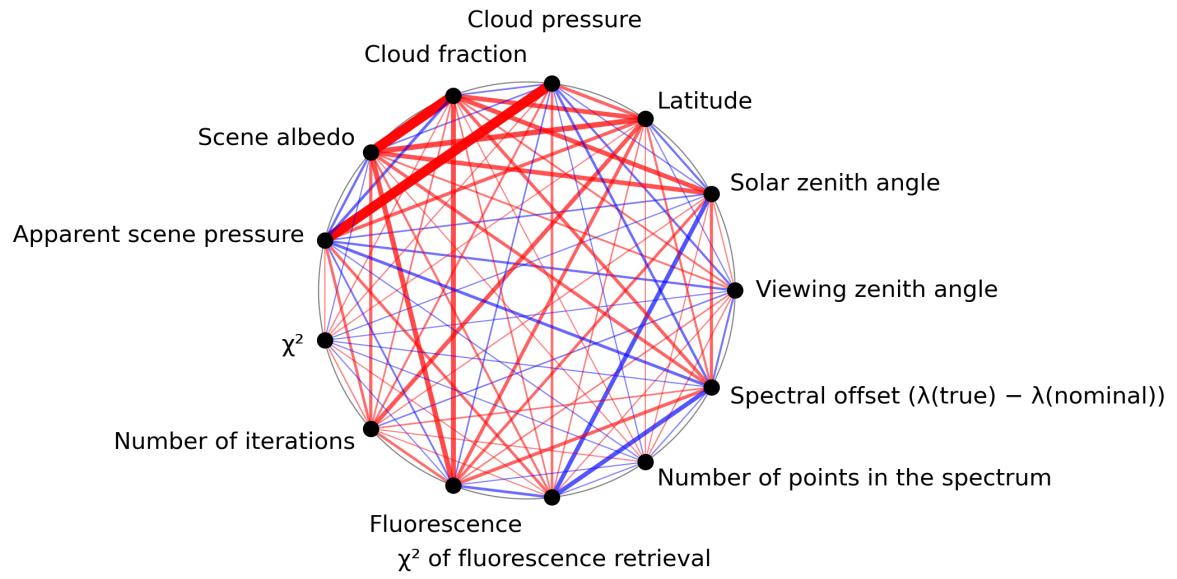
Figure 1: Map of correlation graph for 2024-05-18 to 2024-05-20.
