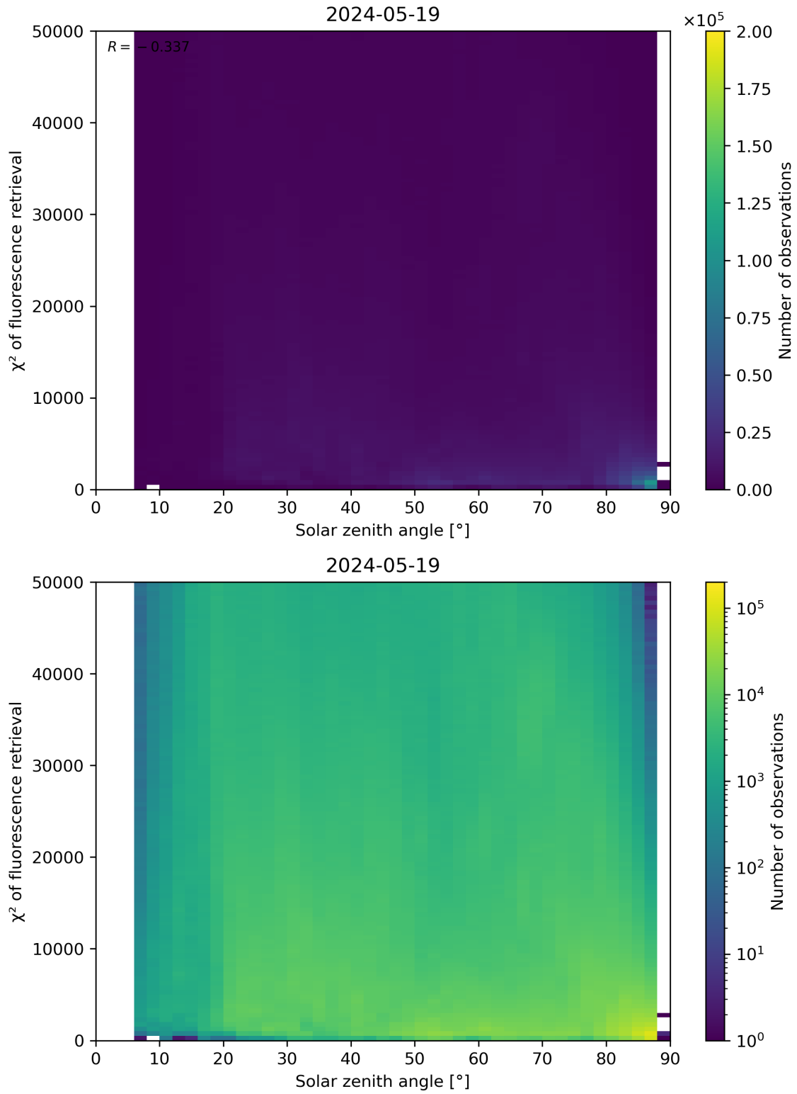
Figure 109: Scatter density plot of “Solar zenith angle” against “ \chi^2 of fluorescence retrieval” for 2024-05-18 to 2024-05-20.
