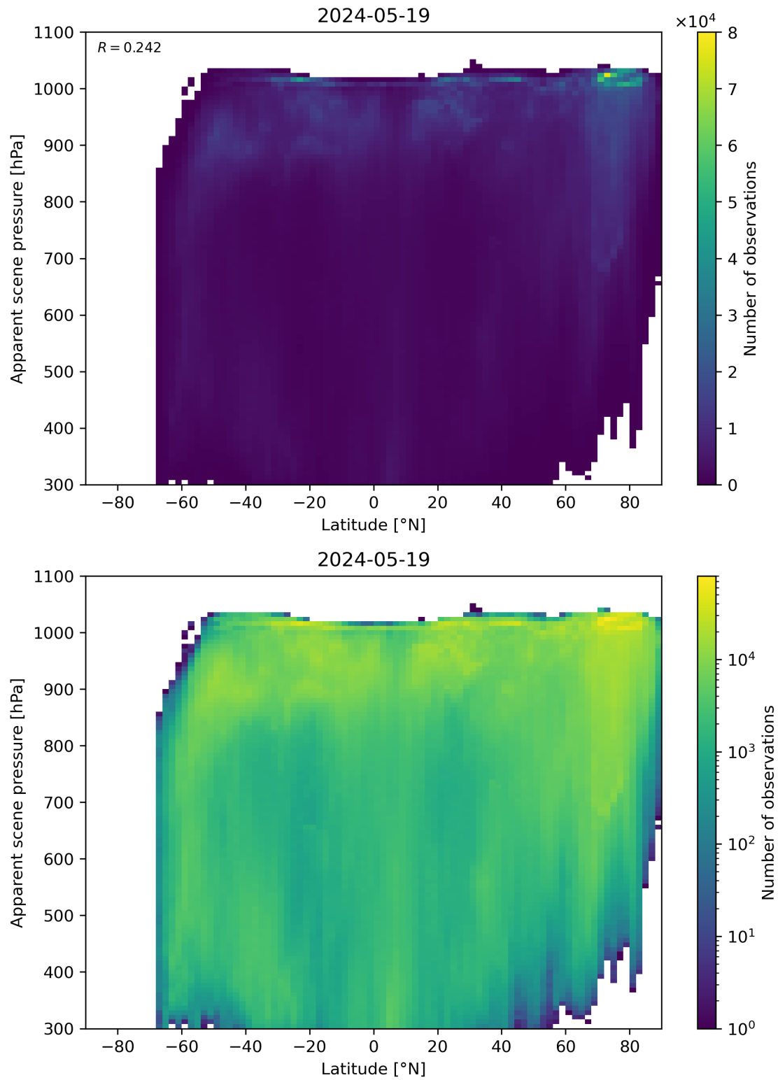
Figure 88: Scatter density plot of “Latitude” against “Apparent scene pressure” for 2024-05-18 to 2024-05-20.
