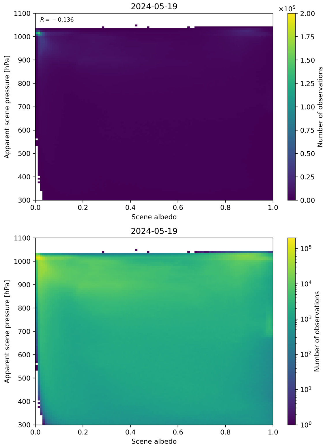
Figure 102: Scatter density plot of “Scene albedo” against “Apparent scene pressure” for 2024-05-18 to 2024-05-20.
