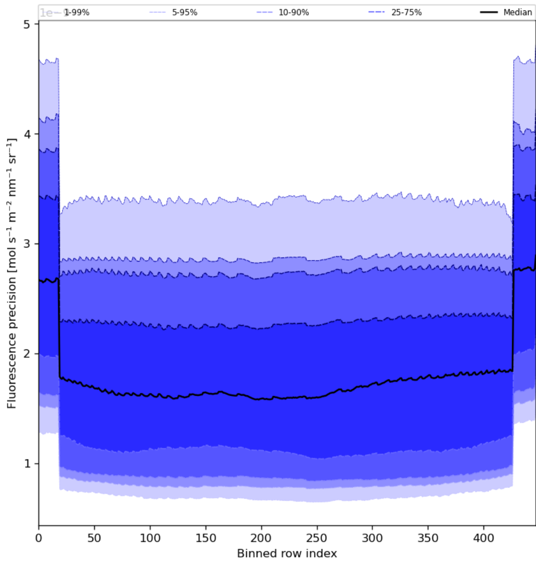
Figure 58: Along track statistics of “Fluorescence precision” for 2024-05-18 to 2024-05-20
