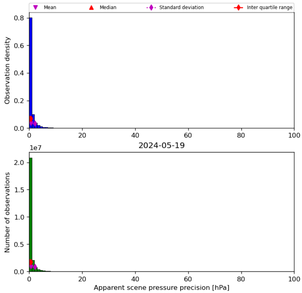
Figure 37: Histogram of “Apparent scene pressure precision” for 2024-05-18 to 2024-05-20
