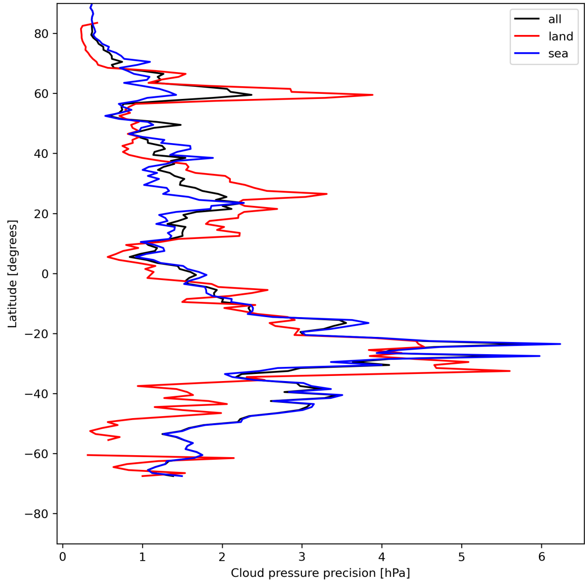
Figure 14: Zonal average of “Cloud pressure precision” for 2024-05-18 to 2024-05-20.
