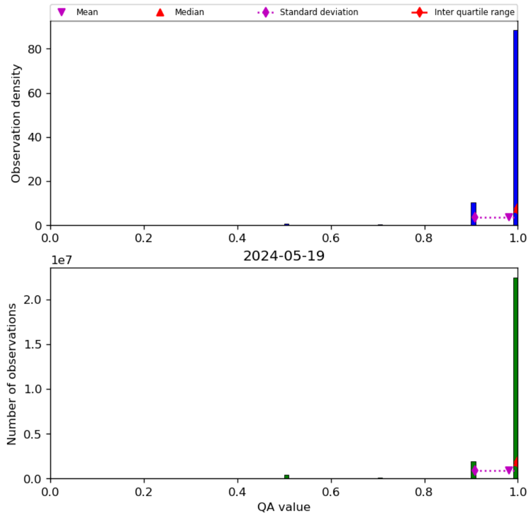
Figure 29: Histogram of “QA value” for 2024-05-18 to 2024-05-20
