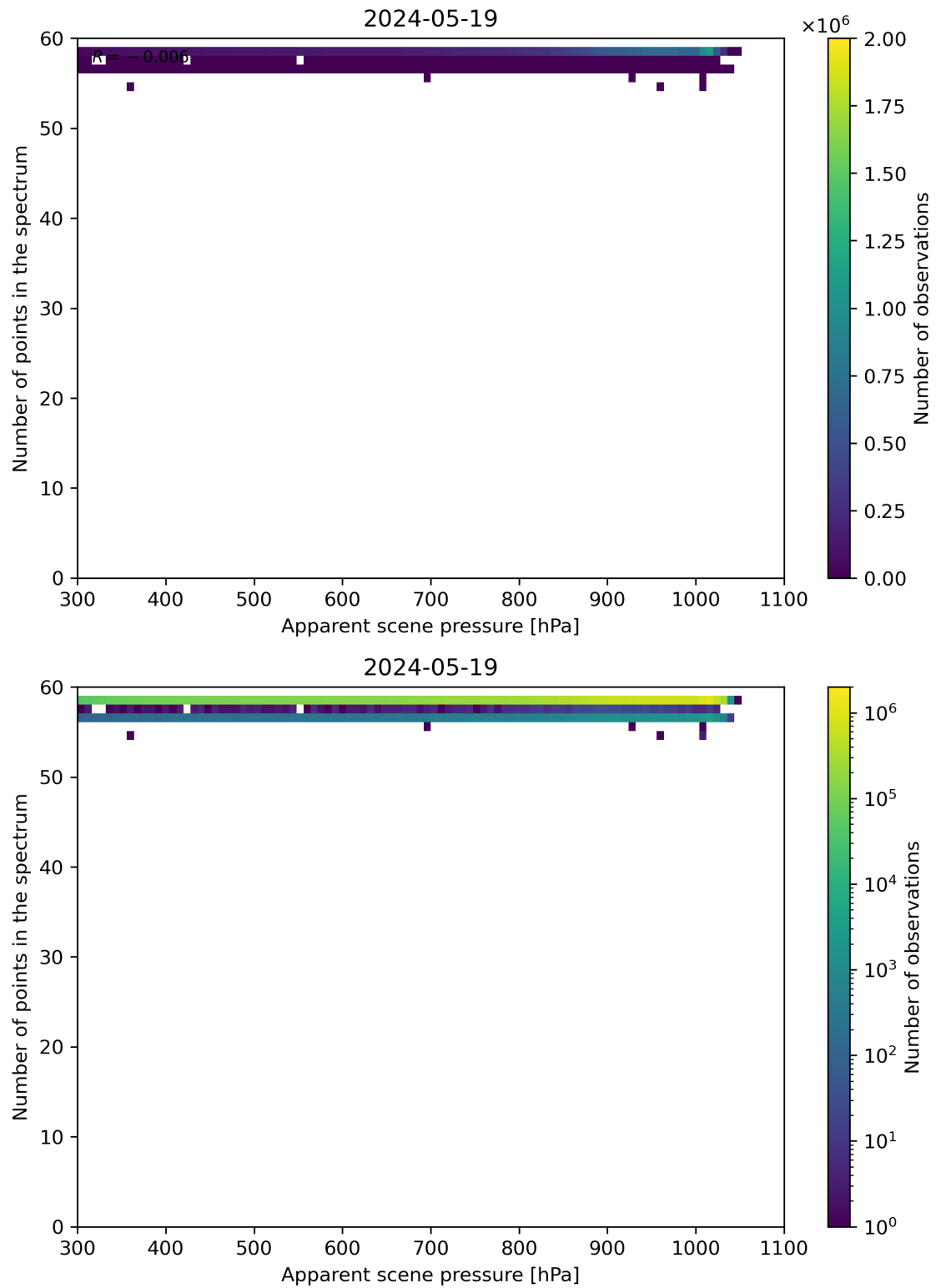
Figure 66: Scatter density plot of “Apparent scene pressure” against “Number of points in the spectrum” for 2024-05-18 to 2024-05-20.
