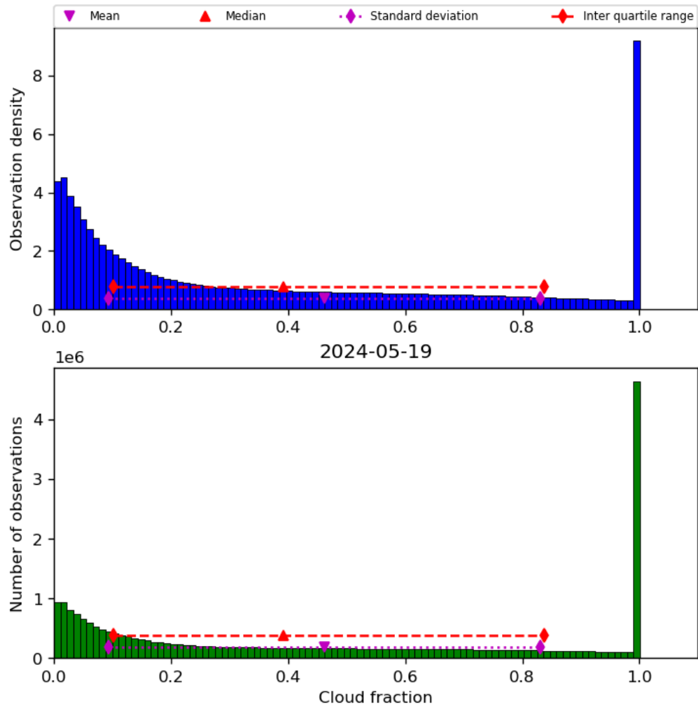
Figure 32: Histogram of “Cloud fraction” for 2024-05-18 to 2024-05-20
