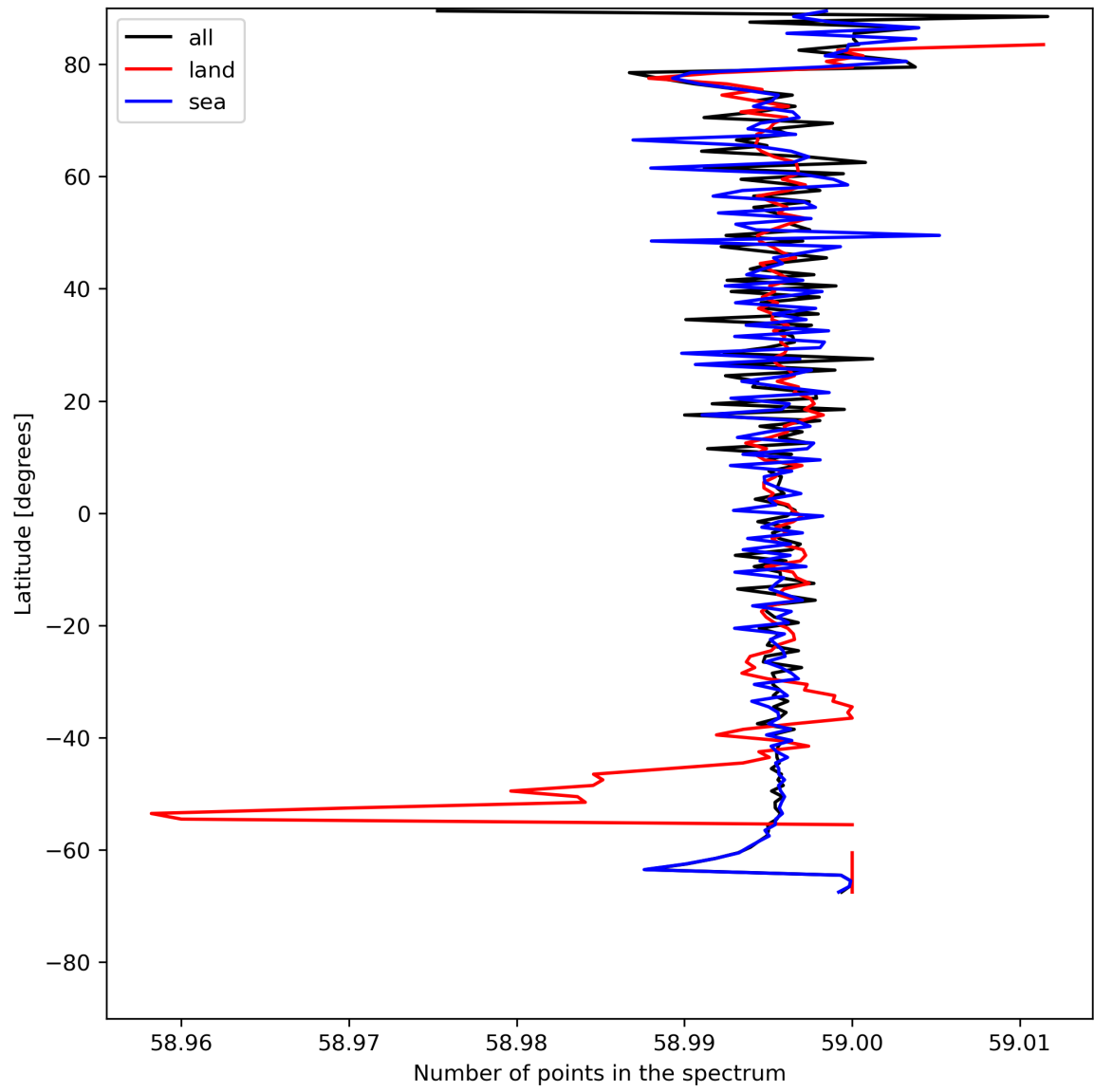
Figure 27: Zonal average of “Number of points in the spectrum” for 2024-05-18 to 2024-05-20.
