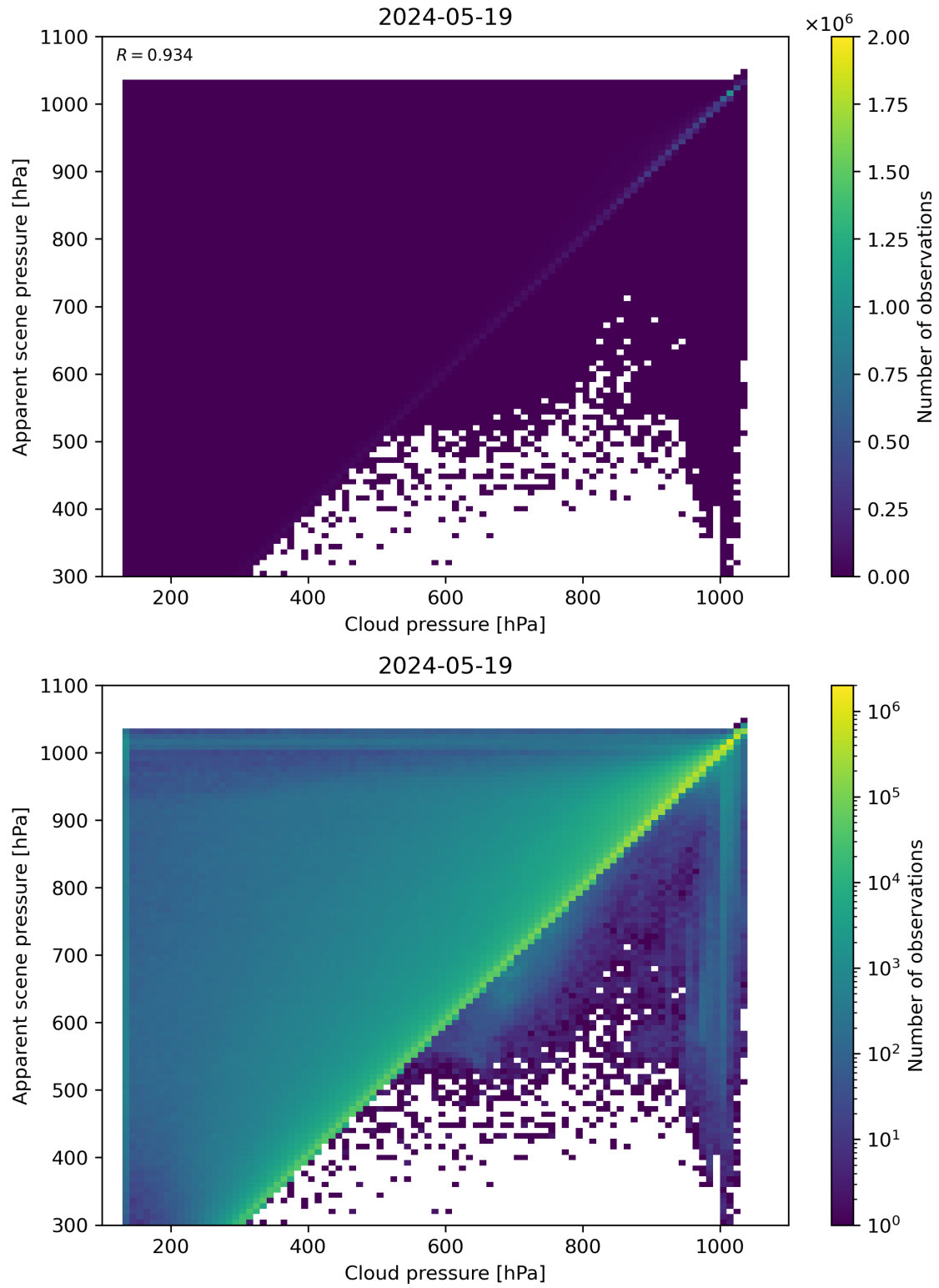
Figure 77: Scatter density plot of “Cloud pressure” against “Apparent scene pressure” for 2024-05-18 to 2024-05-20.
