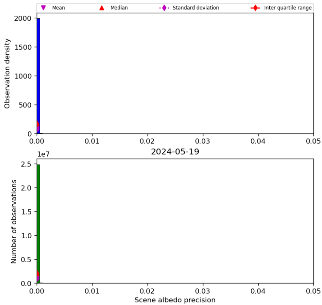
Figure 35: Histogram of “Scene albedo precision” for 2024-05-18 to 2024-05-20
