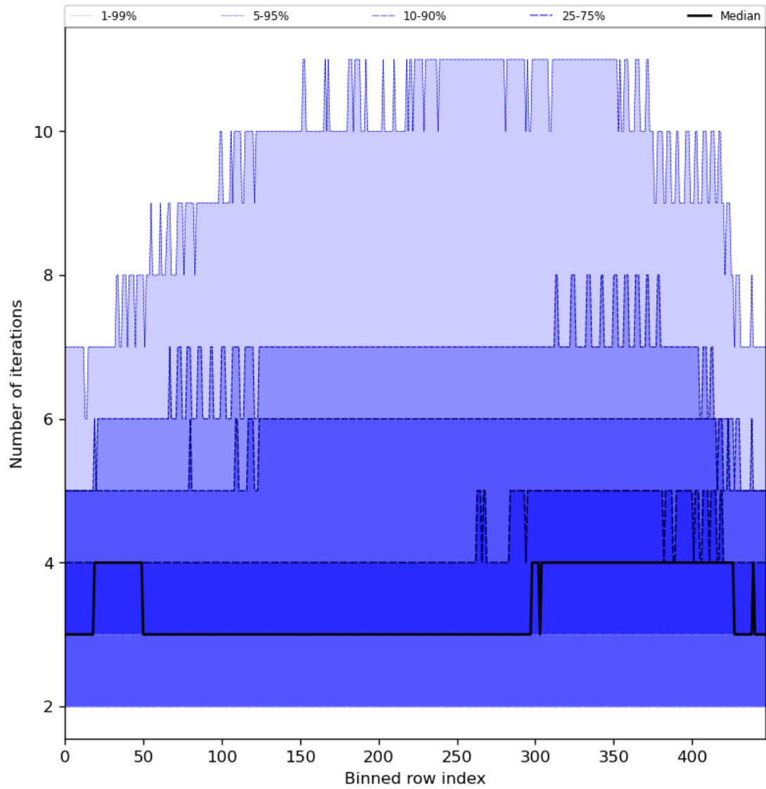
Figure 56: Along track statistics of “Number of iterations” for 2024-05-18 to 2024-05-20
