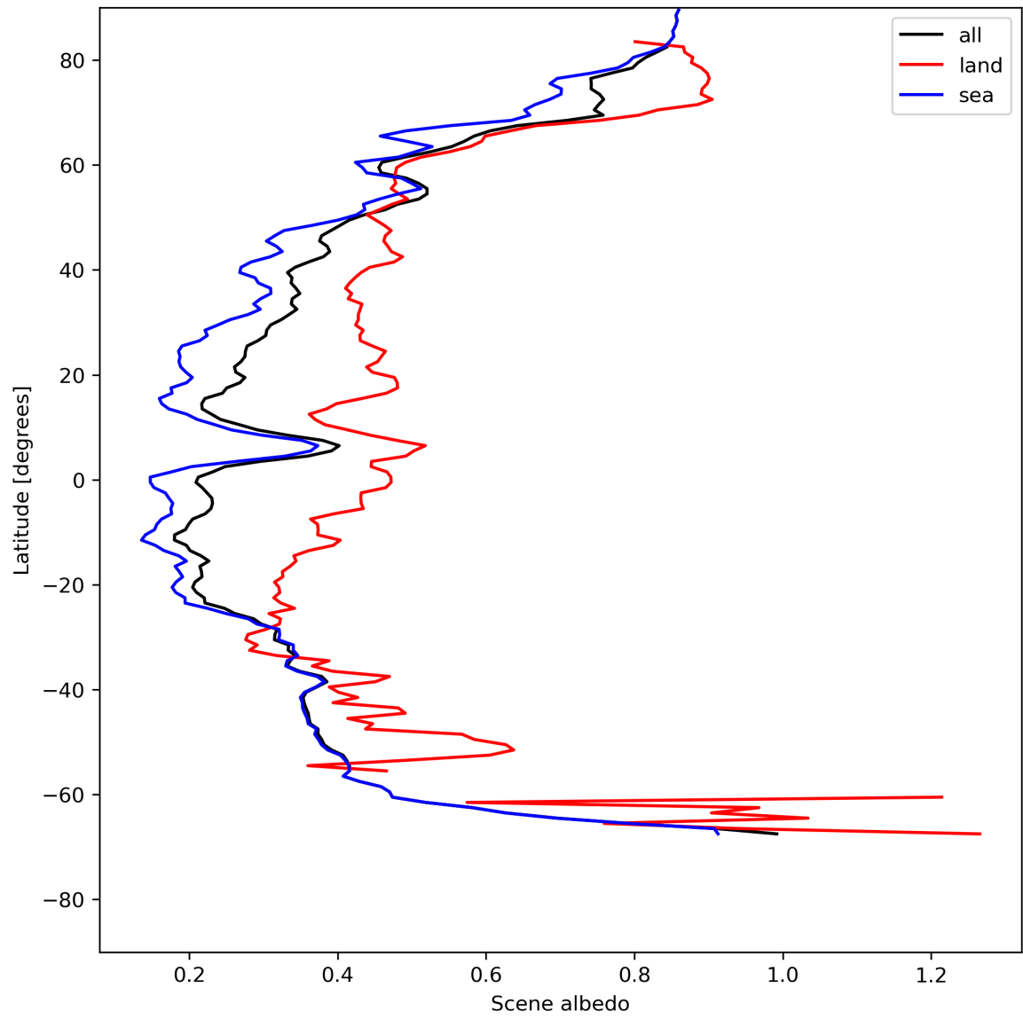
Figure 17: Zonal average of “Scene albedo” for 2024-05-18 to 2024-05-20.
