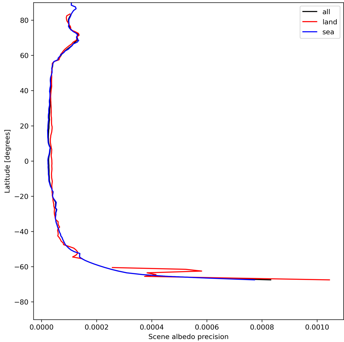
Figure 18: Zonal average of “Scene albedo precision” for 2024-05-18 to 2024-05-20.
