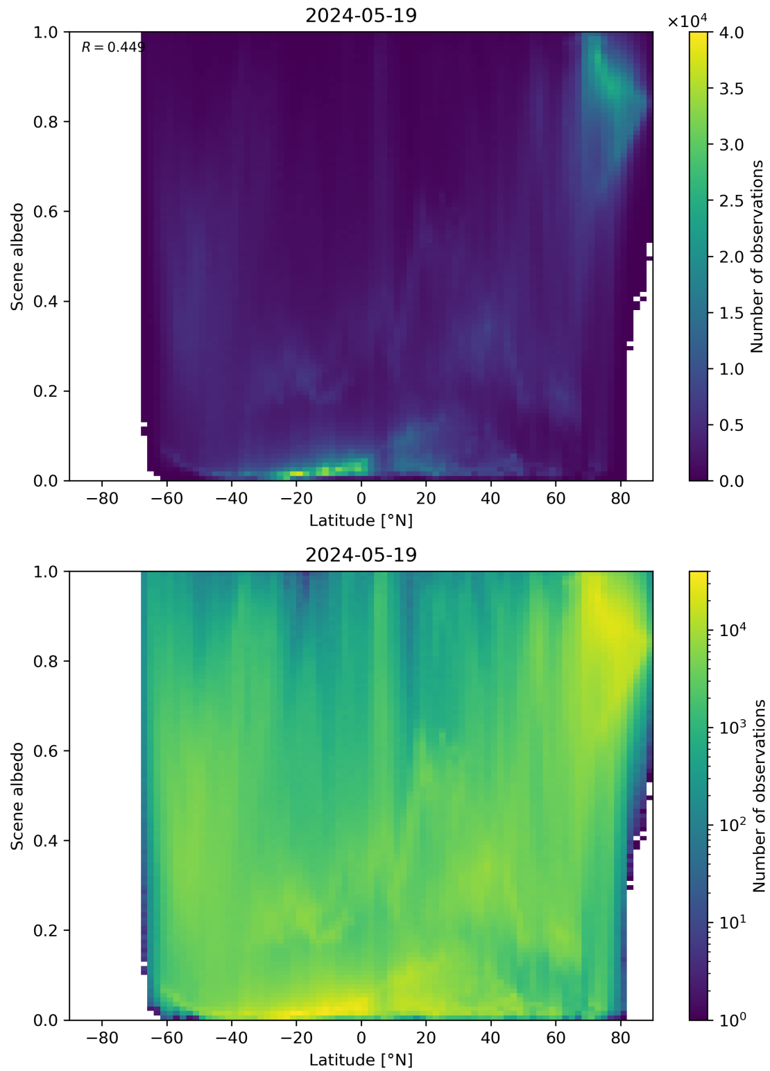
Figure 95: Scatter density plot of “Latitude” against “Scene albedo” for 2024-05-18 to 2024-05-20.
