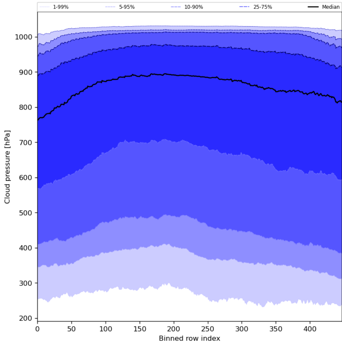
Figure 47: Along track statistics of “Cloud pressure” for 2024-05-18 to 2024-05-20
