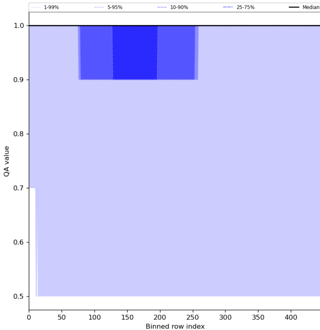
Figure 46: Along track statistics of “QA value” for 2024-05-18 to 2024-05-20
