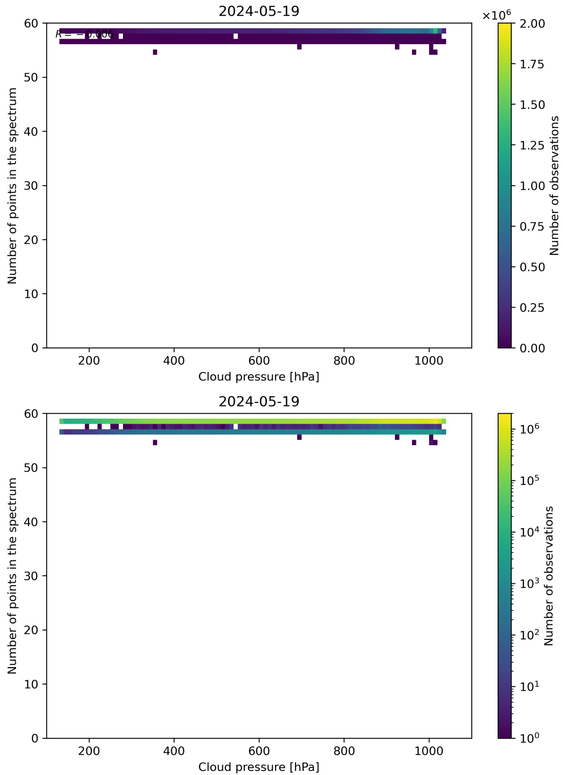
Figure 82: Scatter density plot of “Cloud pressure” against “Number of points in the spectrum” for 2024-05-18 to 2024-05-20.
