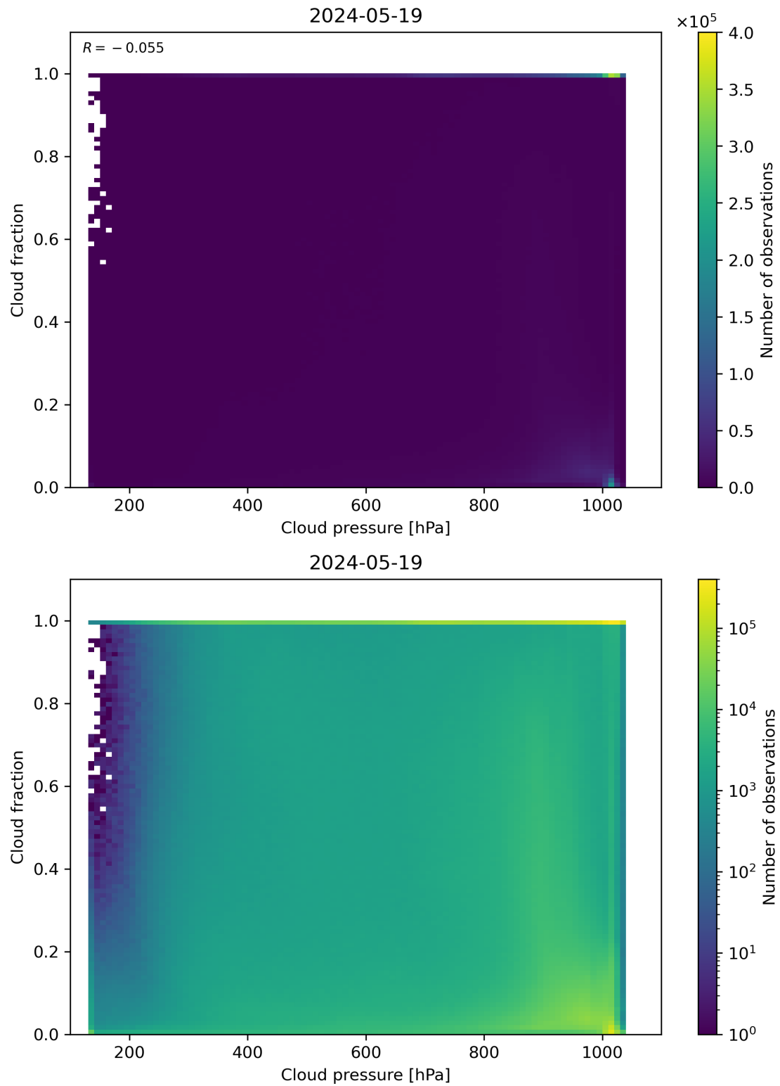
Figure 79: Scatter density plot of “Cloud pressure” against “Cloud fraction” for 2024-05-18 to 2024-05-20.
