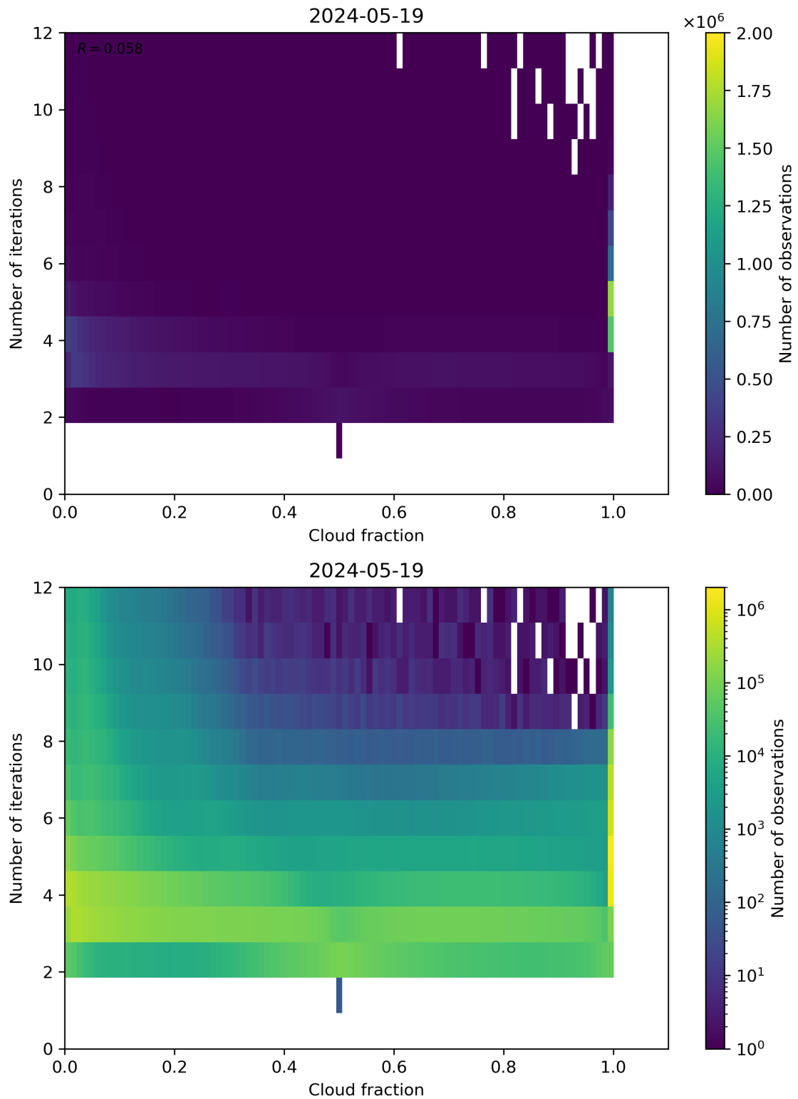
Figure 73: Scatter density plot of “Cloud fraction” against “Number of iterations” for 2024-05-18 to 2024-05-20.
