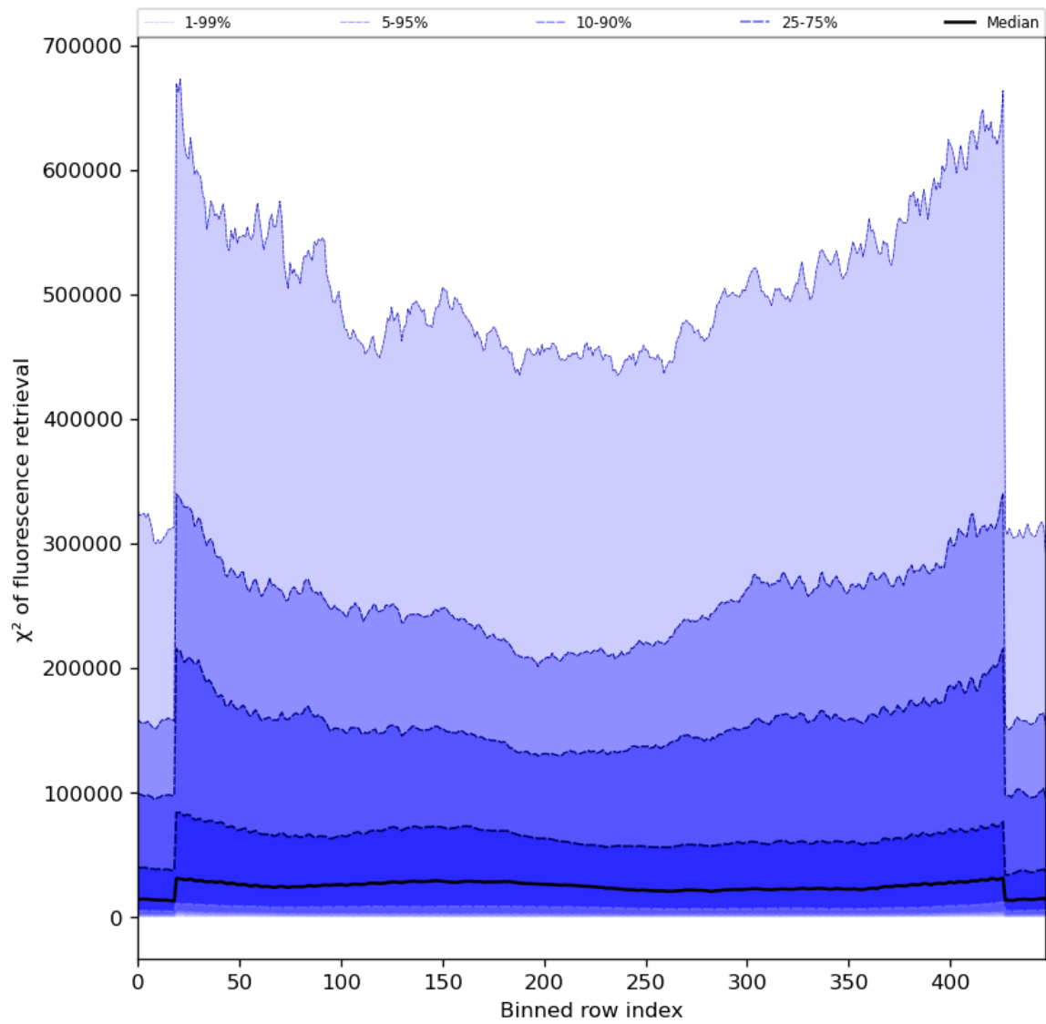
Figure 59: Along track statistics of “ \chi^2 of fluorescence retrieval” for 2024-05-18 to 2024-05-20
