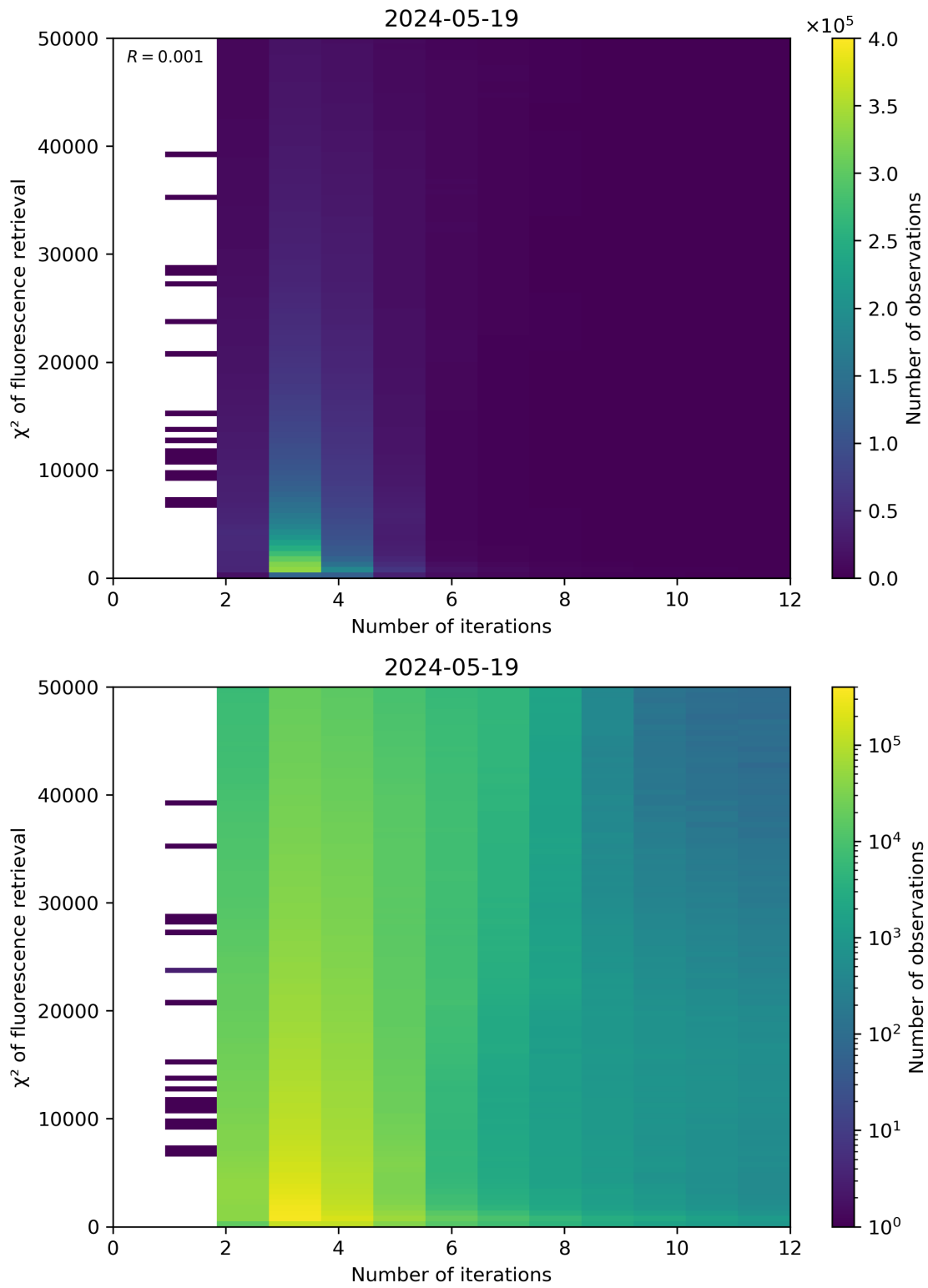
Figure 97: Scatter density plot of “Number of iterations” against “ \chi^2 of fluorescence retrieval” for 2024-05-18 to 2024-05-20.
