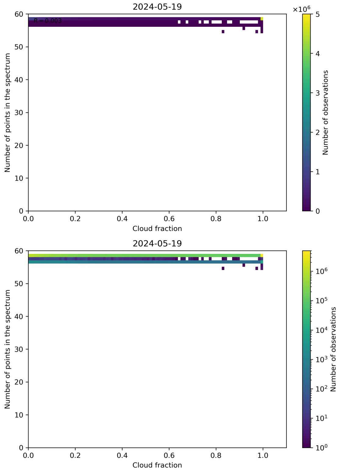
Figure 74: Scatter density plot of “Cloud fraction” against “Number of points in the spectrum” for 2024-05-18 to 2024-05-20.
