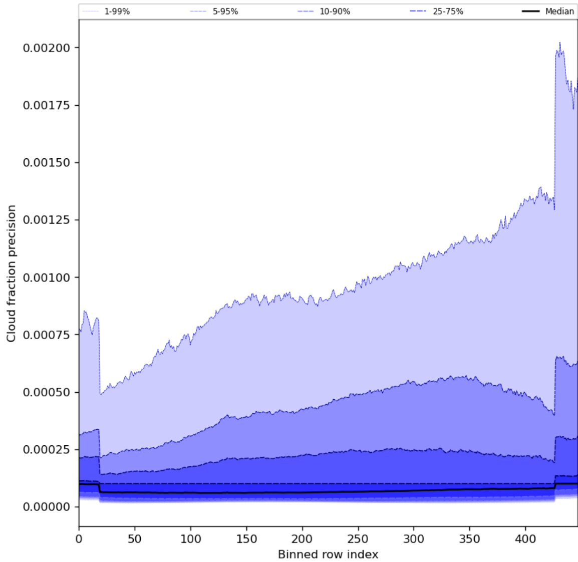
Figure 50: Along track statistics of “Cloud fraction precision” for 2024-05-18 to 2024-05-20
