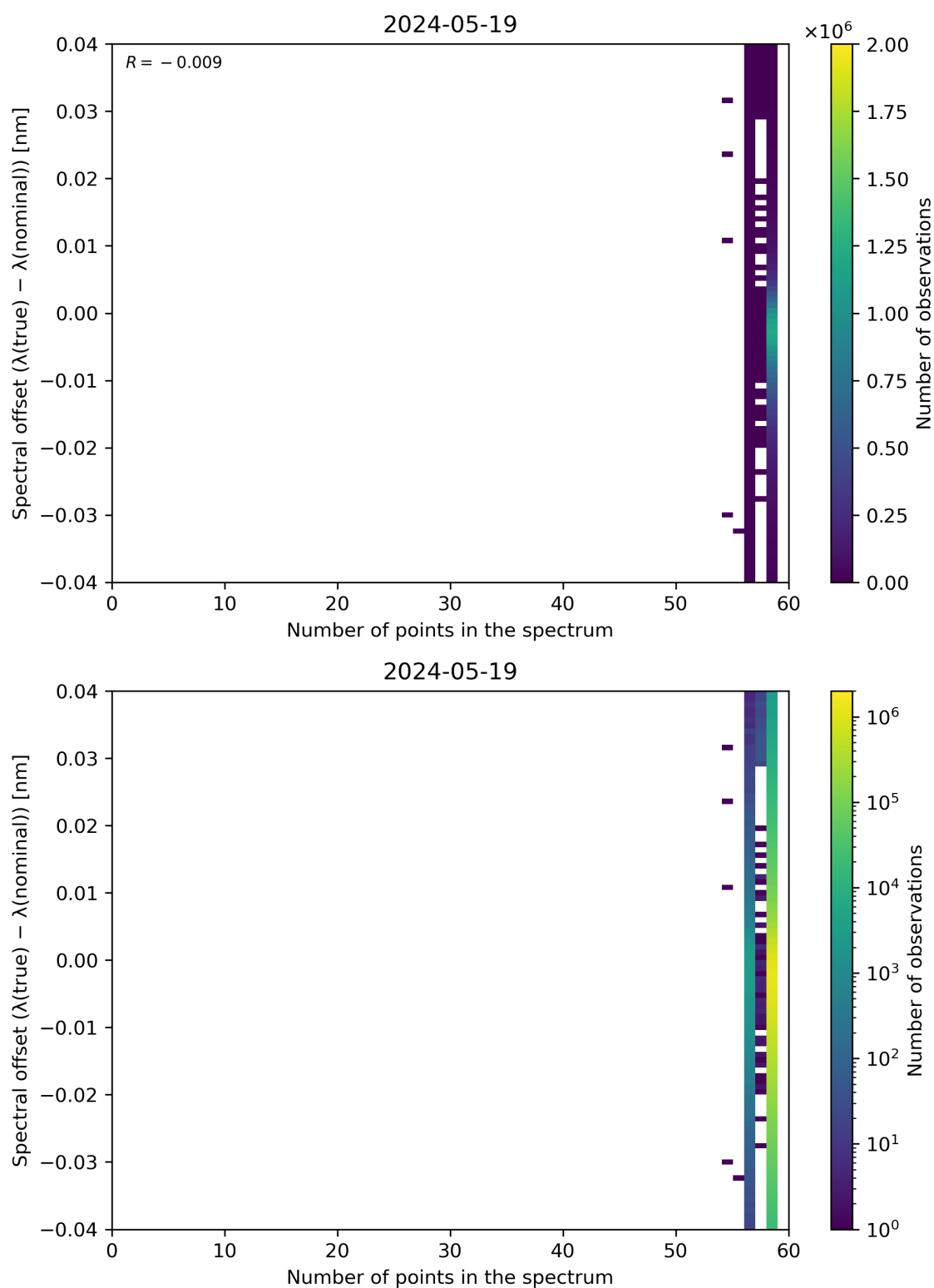
Figure 101: Scatter density plot of “Number of points in the spectrum” against “Spectral offset ( \lambda(\text{true}) - \lambda(\text{nominal}) )” for 2024-05-18 to 2024-05-20.
