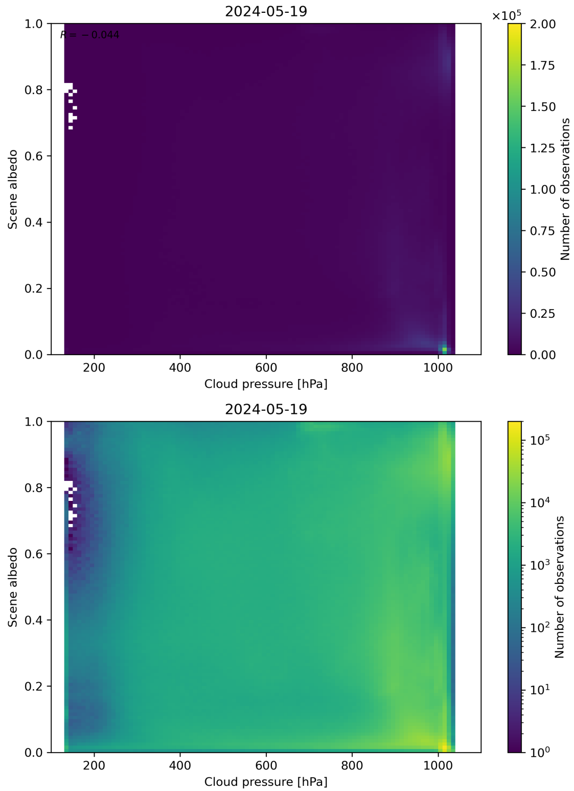
Figure 83: Scatter density plot of “Cloud pressure” against “Scene albedo” for 2024-05-18 to 2024-05-20.
