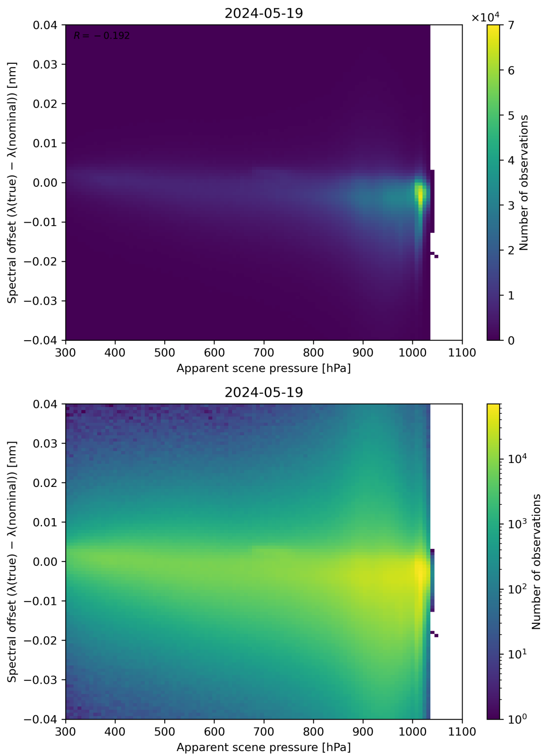
Figure 67: Scatter density plot of “Apparent scene pressure” against “Spectral offset ( \lambda(\text{true}) - \lambda(\text{nominal}) )” for 2024-05-18 to 2024-05-20.
