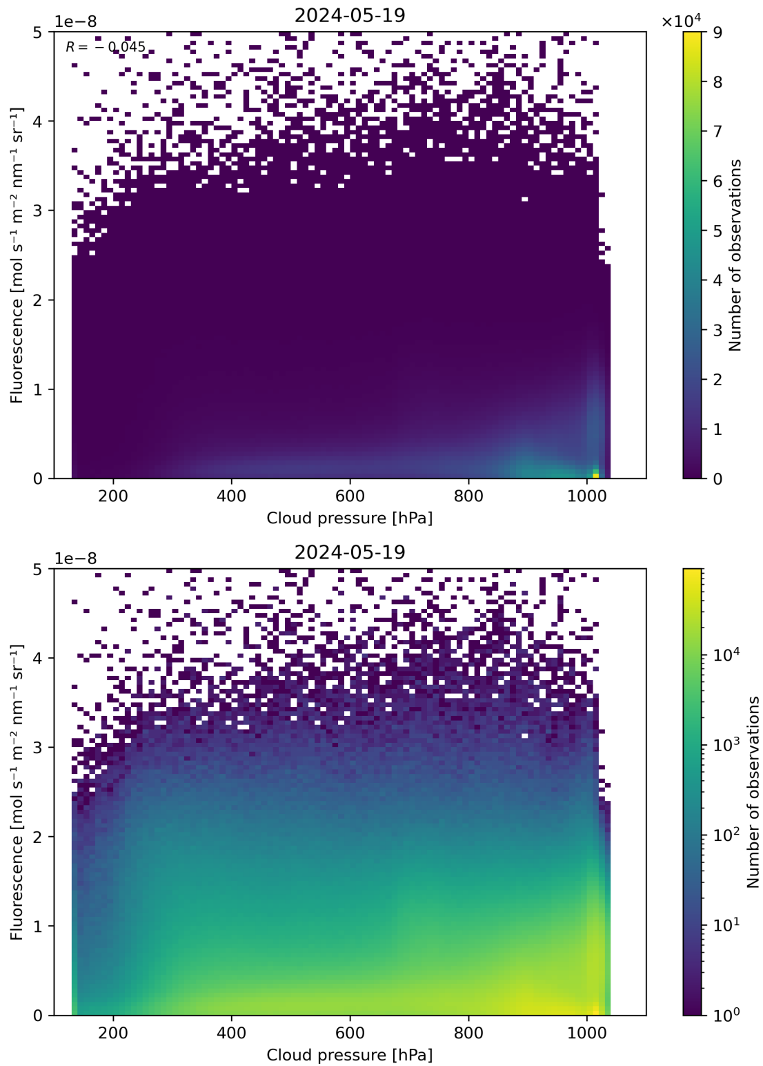
Figure 80: Scatter density plot of “Cloud pressure” against “Fluorescence” for 2024-05-18 to 2024-05-20.
