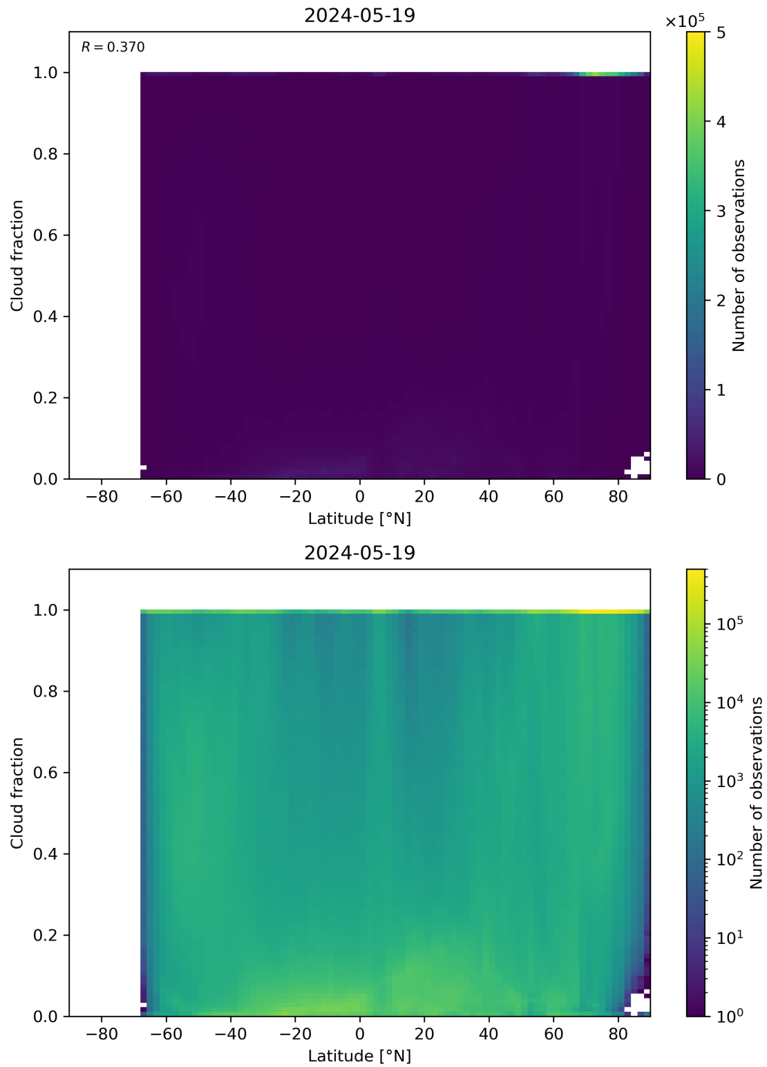
Figure 90: Scatter density plot of “Latitude” against “Cloud fraction” for 2024-05-18 to 2024-05-20.
