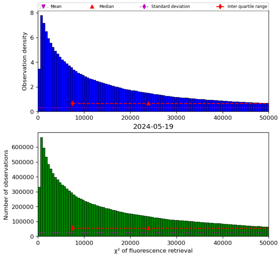
Figure 42: Histogram of “ \chi^2 of fluorescence retrieval” for 2024-05-18 to 2024-05-20
