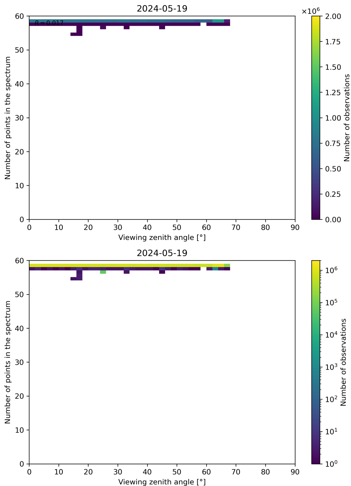
Figure 125: Scatter density plot of “Viewing zenith angle” against “Number of points in the spectrum” for 2024-05-18 to 2024-05-20.
