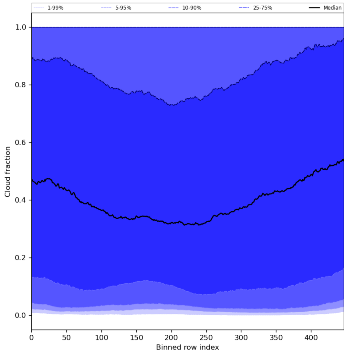
Figure 49: Along track statistics of “Cloud fraction” for 2024-05-18 to 2024-05-20
