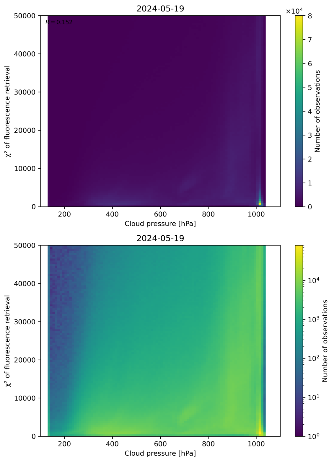
Figure 78: Scatter density plot of “Cloud pressure” against “ \chi^2 of fluorescence retrieval” for 2024-05-18 to 2024-05-20.
