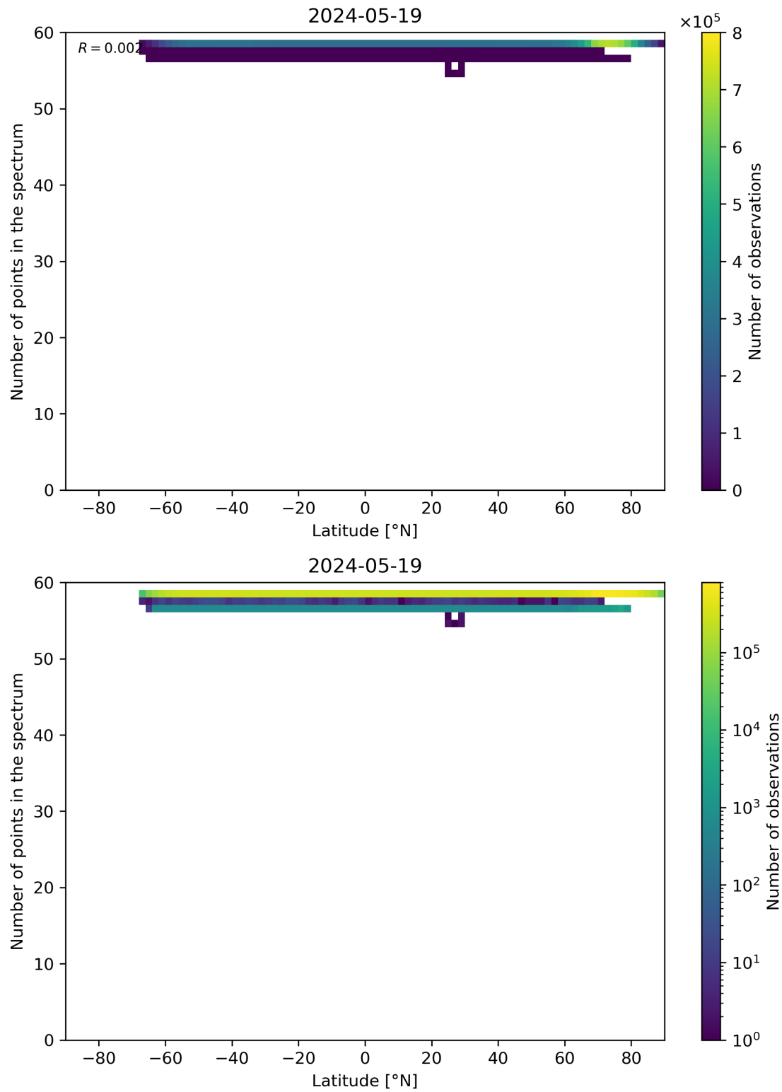
Figure 94: Scatter density plot of “Latitude” against “Number of points in the spectrum” for 2024-05-18 to 2024-05-20.
