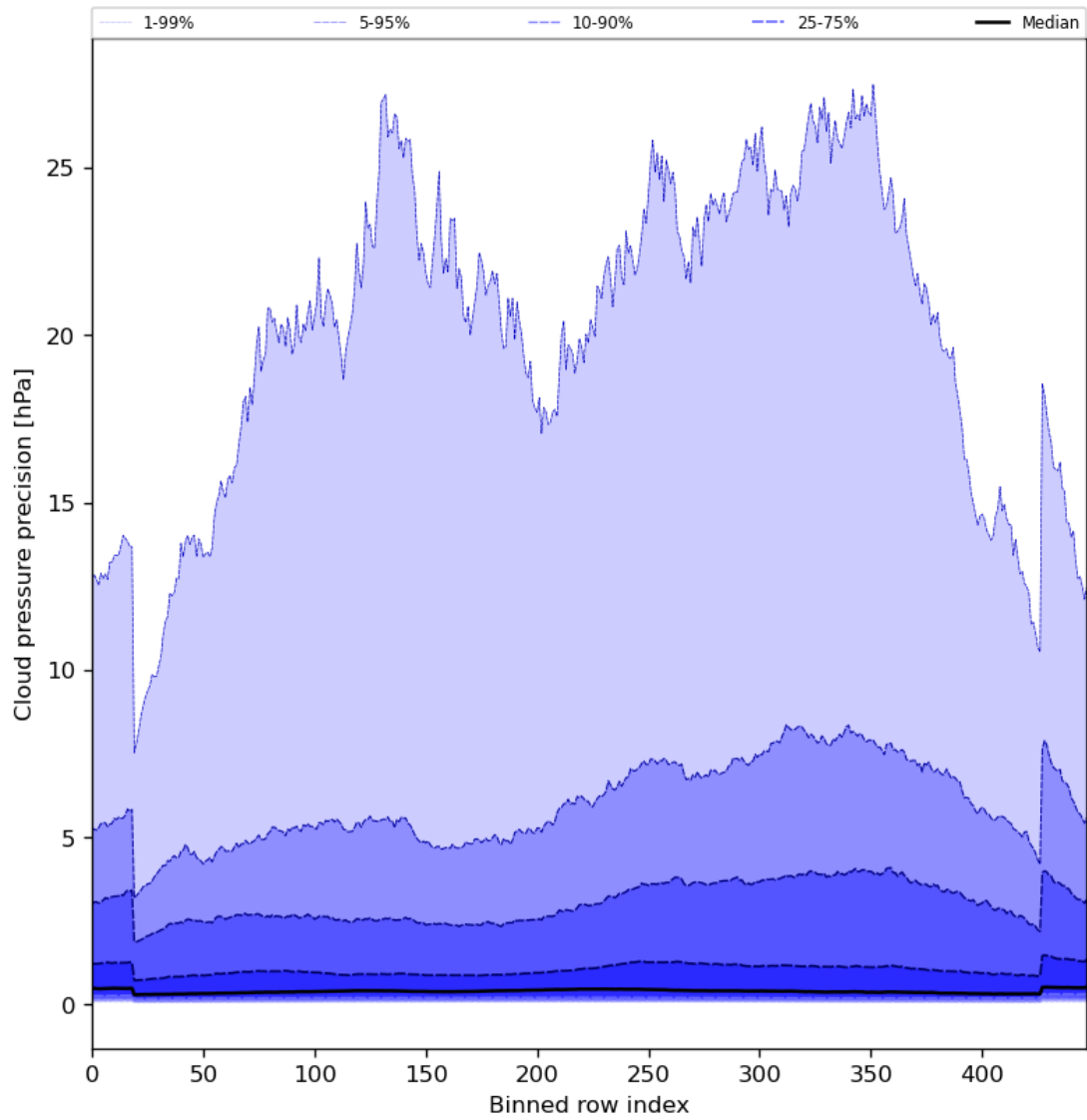
Figure 48: Along track statistics of “Cloud pressure precision” for 2024-05-18 to 2024-05-20
