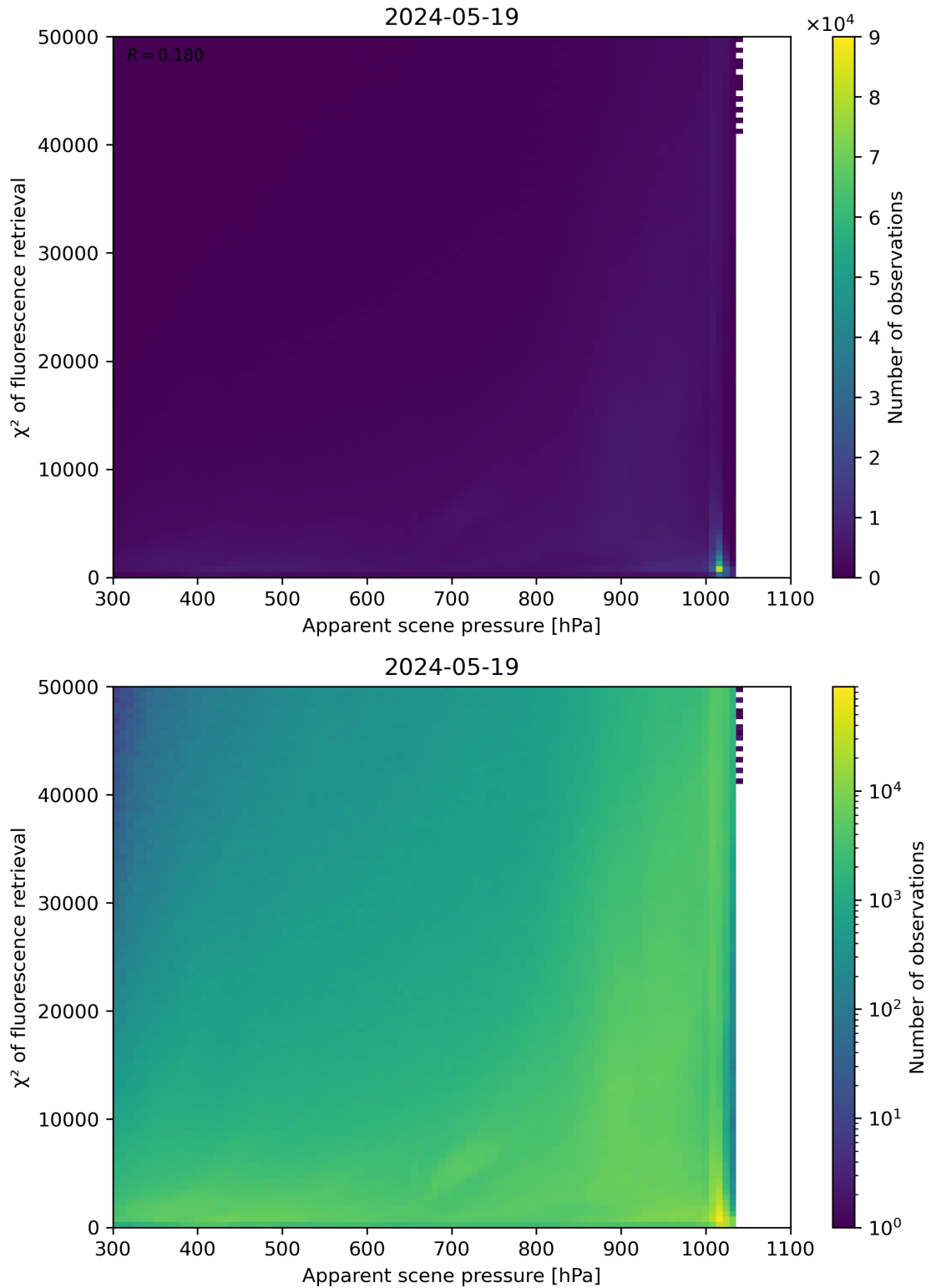
Figure 63: Scatter density plot of “Apparent scene pressure” against “ \chi^2 of fluorescence retrieval” for 2024-05-18 to 2024-05-20.
