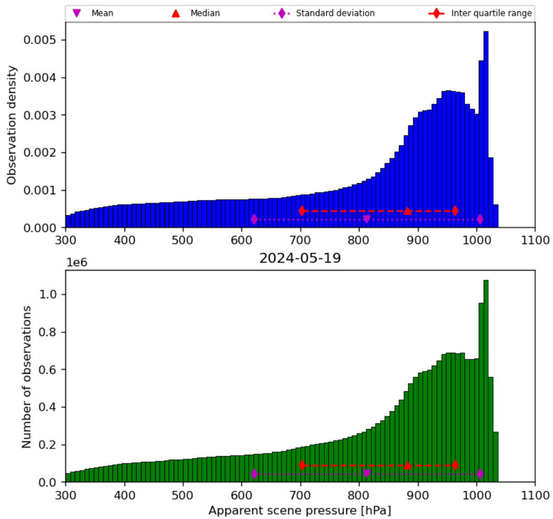
Figure 36: Histogram of “Apparent scene pressure” for 2024-05-18 to 2024-05-20
