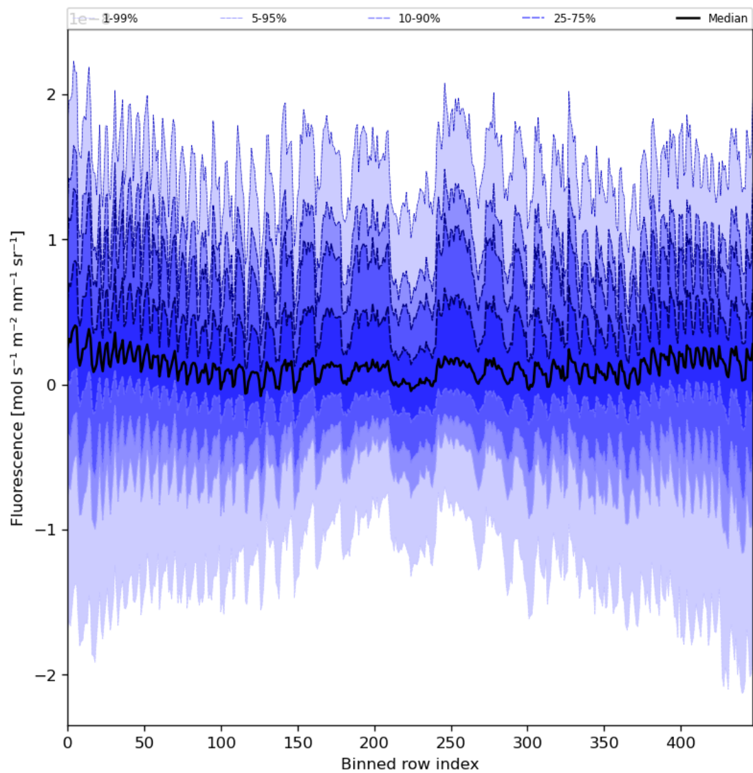
Figure 57: Along track statistics of “Fluorescence” for 2024-05-18 to 2024-05-20
