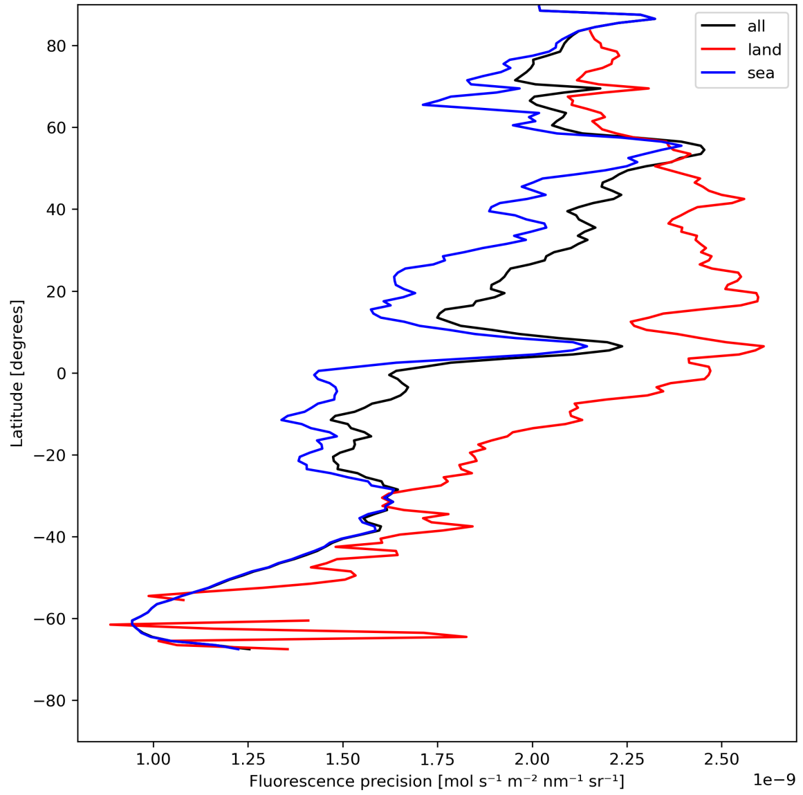
Figure 24: Zonal average of “Fluorescence precision” for 2024-05-18 to 2024-05-20.
