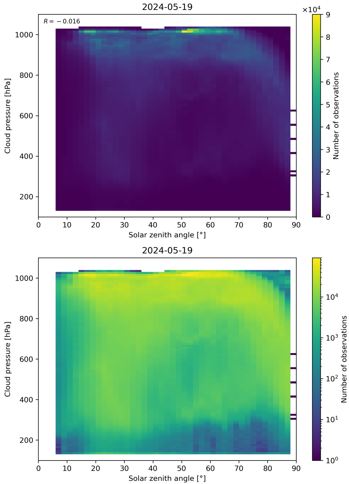
Figure 111: Scatter density plot of “Solar zenith angle” against “Cloud pressure” for 2024-05-18 to 2024-05-20.
