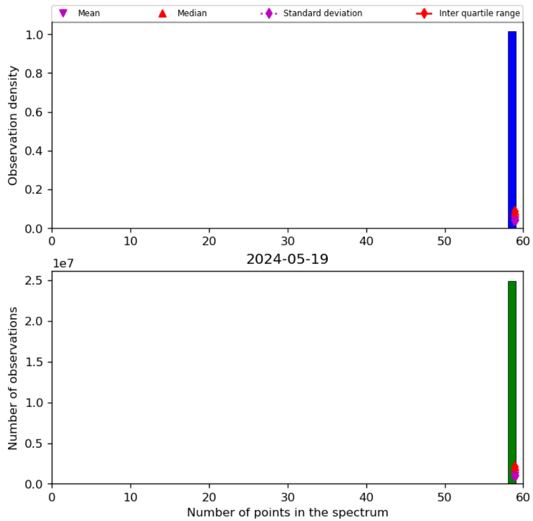
Figure 44: Histogram of “Number of points in the spectrum” for 2024-05-18 to 2024-05-20
