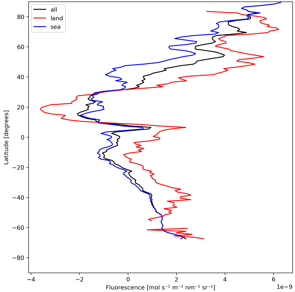
Figure 23: Zonal average of “Fluorescence” for 2024-05-18 to 2024-05-20.
