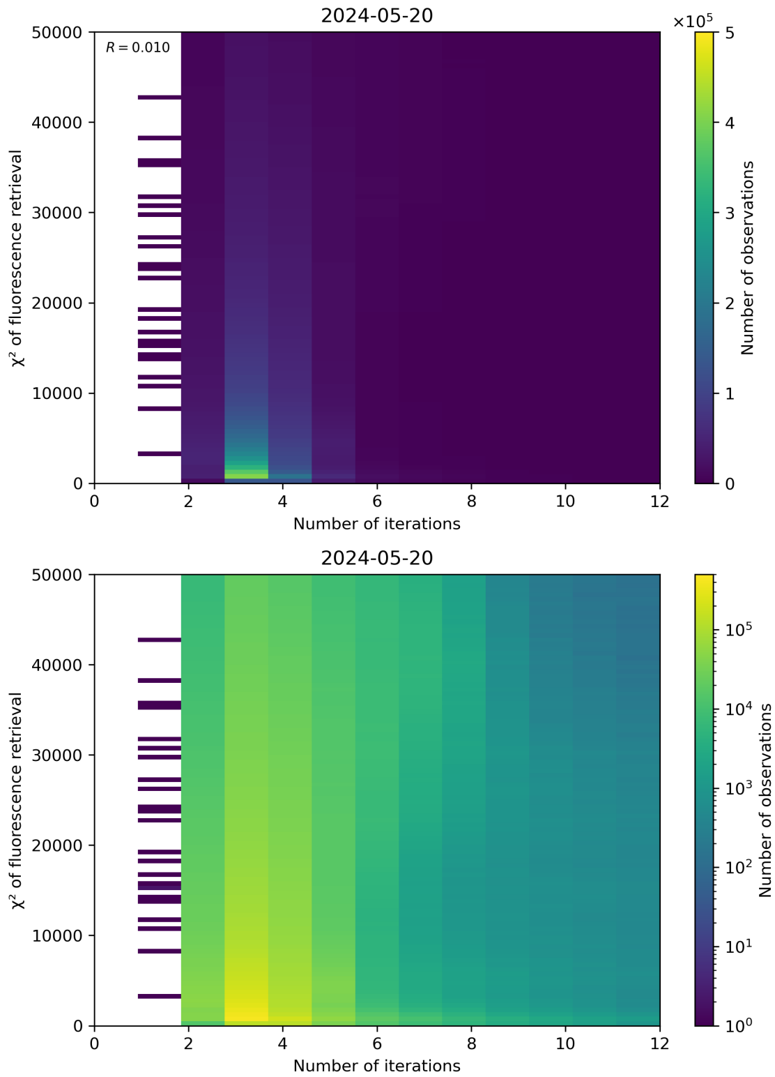
Figure 97: Scatter density plot of “Number of iterations” against “ \chi^2 of fluorescence retrieval” for 2024-05-19 to 2024-05-21.
