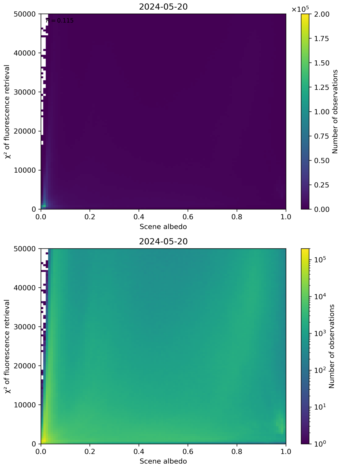
Figure 103: Scatter density plot of “Scene albedo” against “ \chi^2 of fluorescence retrieval” for 2024-05-19 to 2024-05-21.
