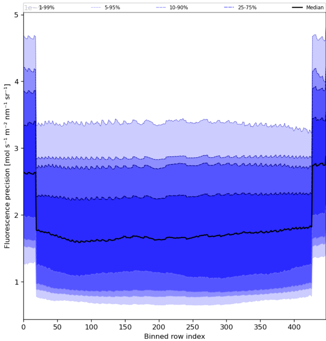
Figure 58: Along track statistics of “Fluorescence precision” for 2024-05-19 to 2024-05-21
