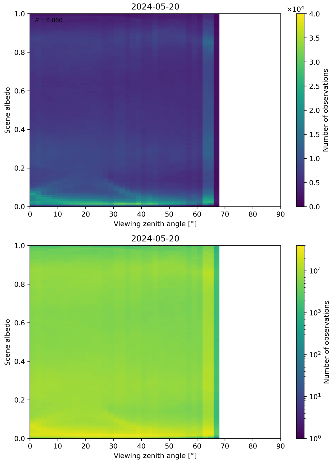
Figure 126: Scatter density plot of “Viewing zenith angle” against “Scene albedo” for 2024-05-19 to 2024-05-21.
