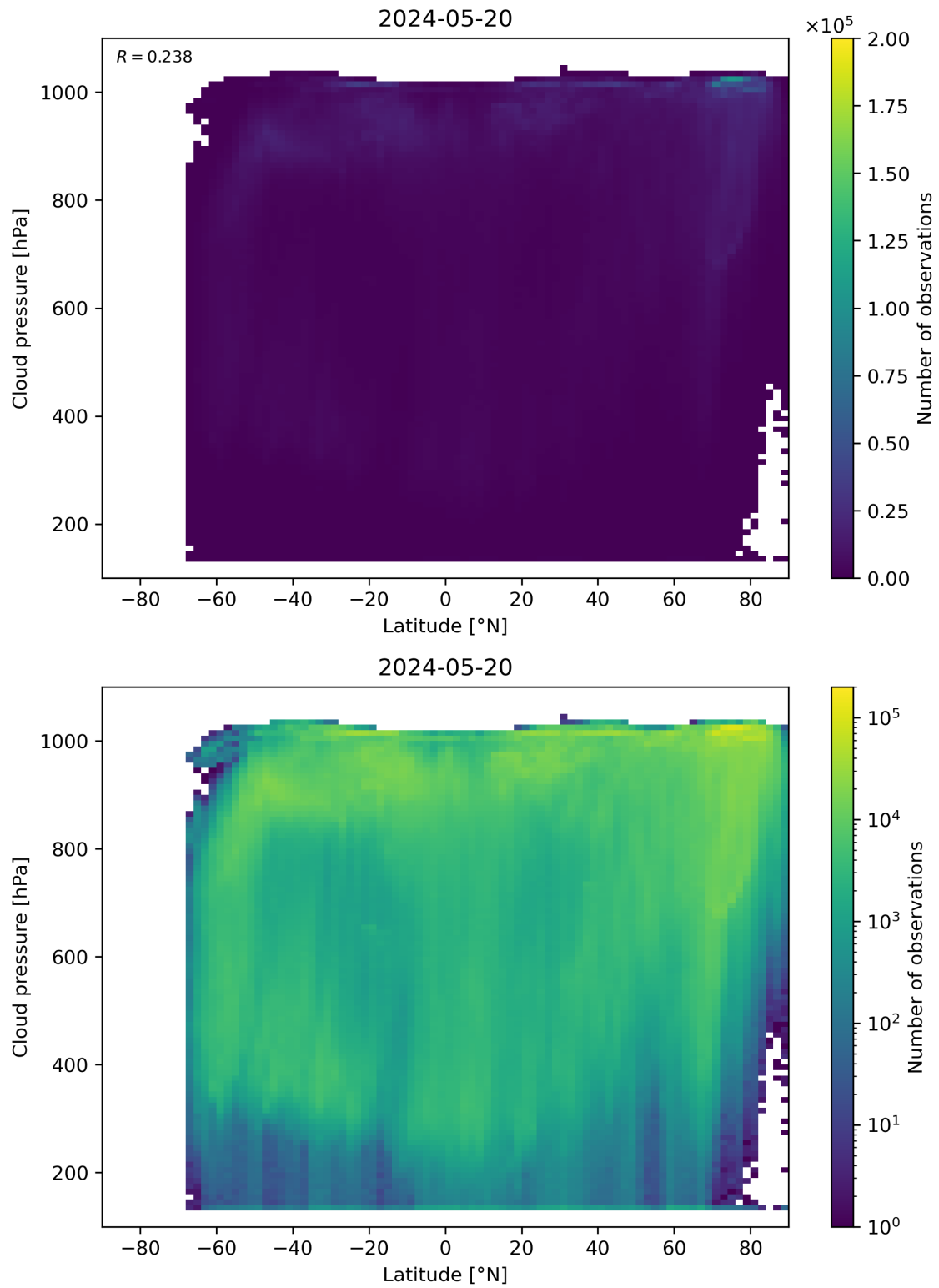
Figure 91: Scatter density plot of “Latitude” against “Cloud pressure” for 2024-05-19 to 2024-05-21.
