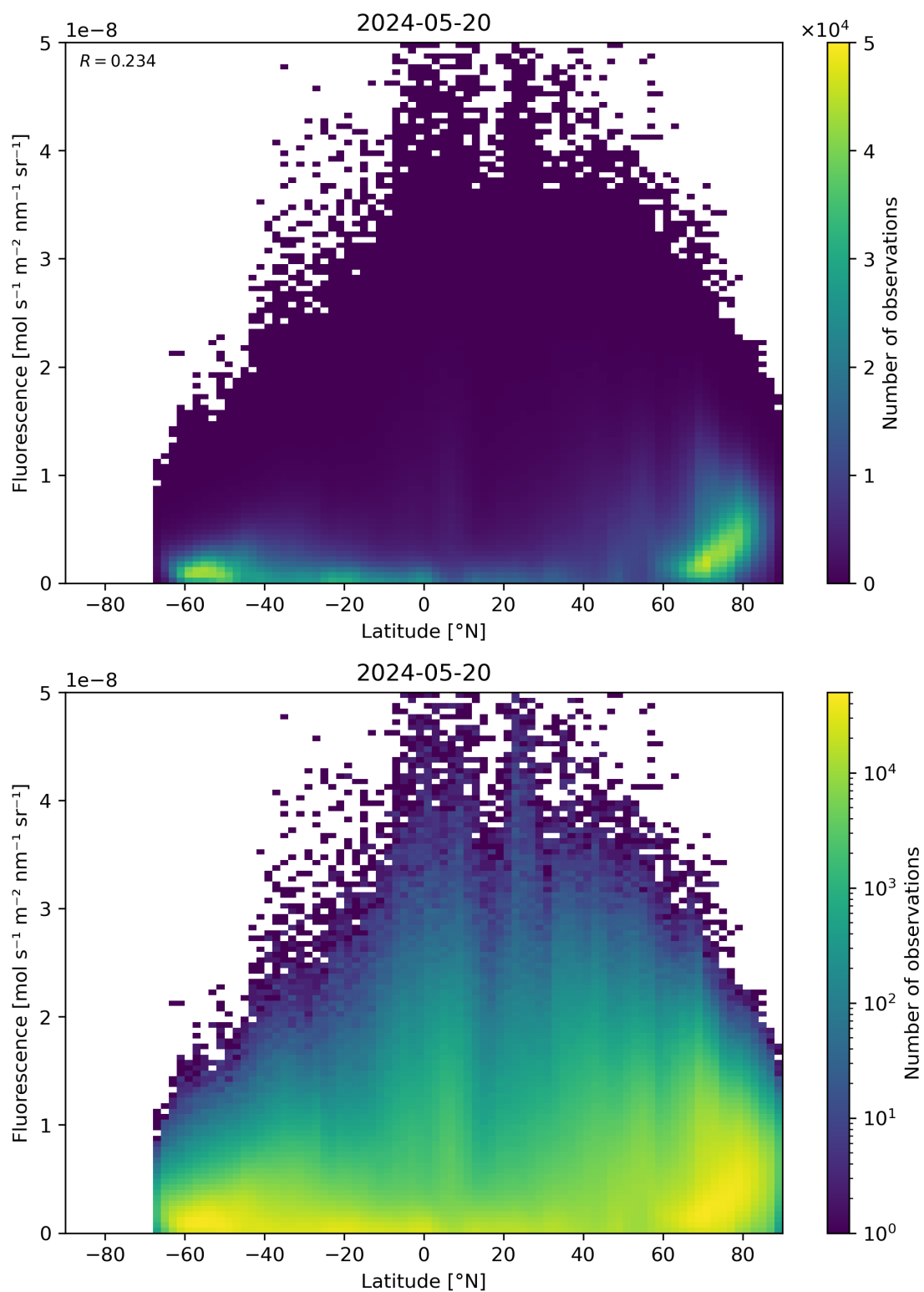
Figure 92: Scatter density plot of “Latitude” against “Fluorescence” for 2024-05-19 to 2024-05-21.
