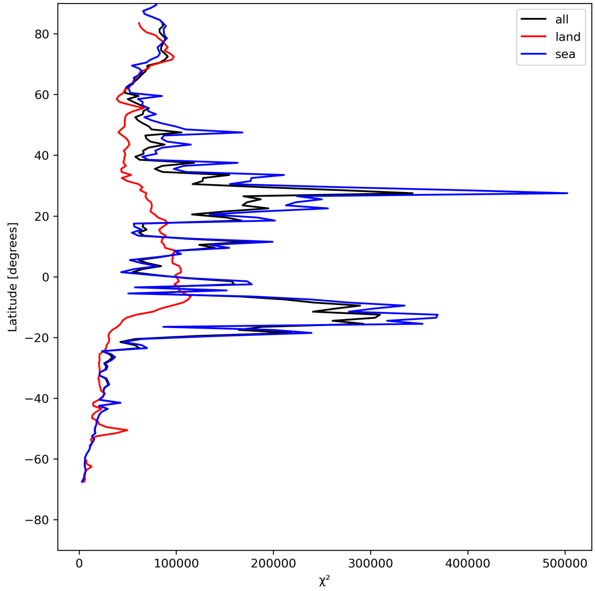
Figure 21: Zonal average of “ \chi^2 ” for 2024-05-19 to 2024-05-21.
