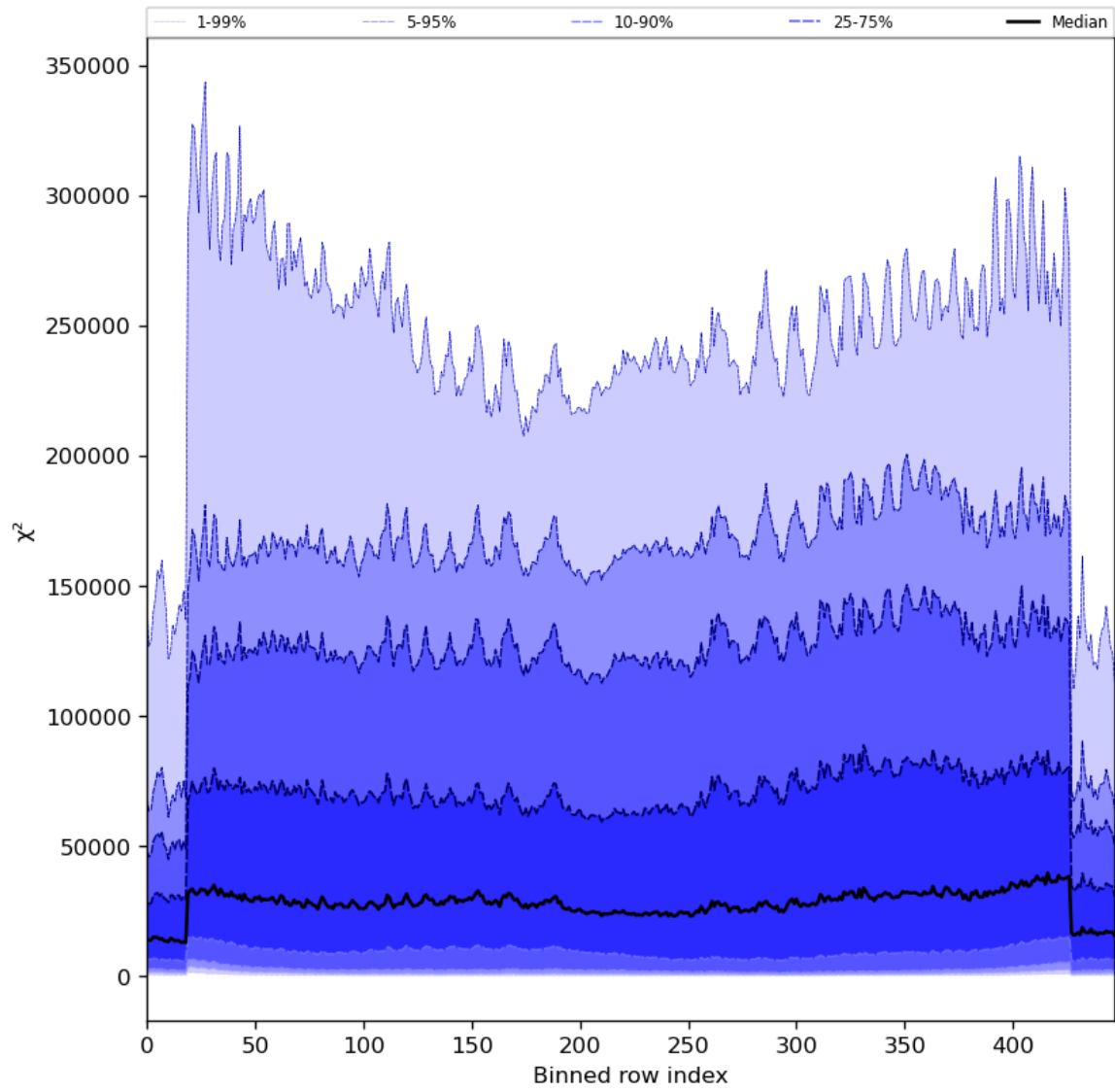
Figure 55: Along track statistics of “ \chi^2 ” for 2024-05-19 to 2024-05-21
