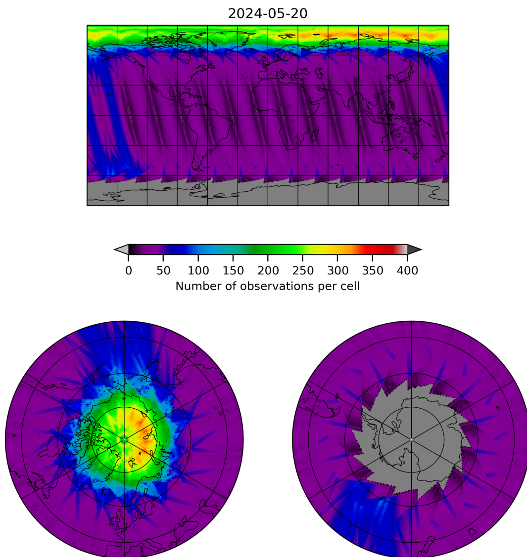
Figure 11: Map of the number of observations for 2024-05-19 to 2024-05-21
