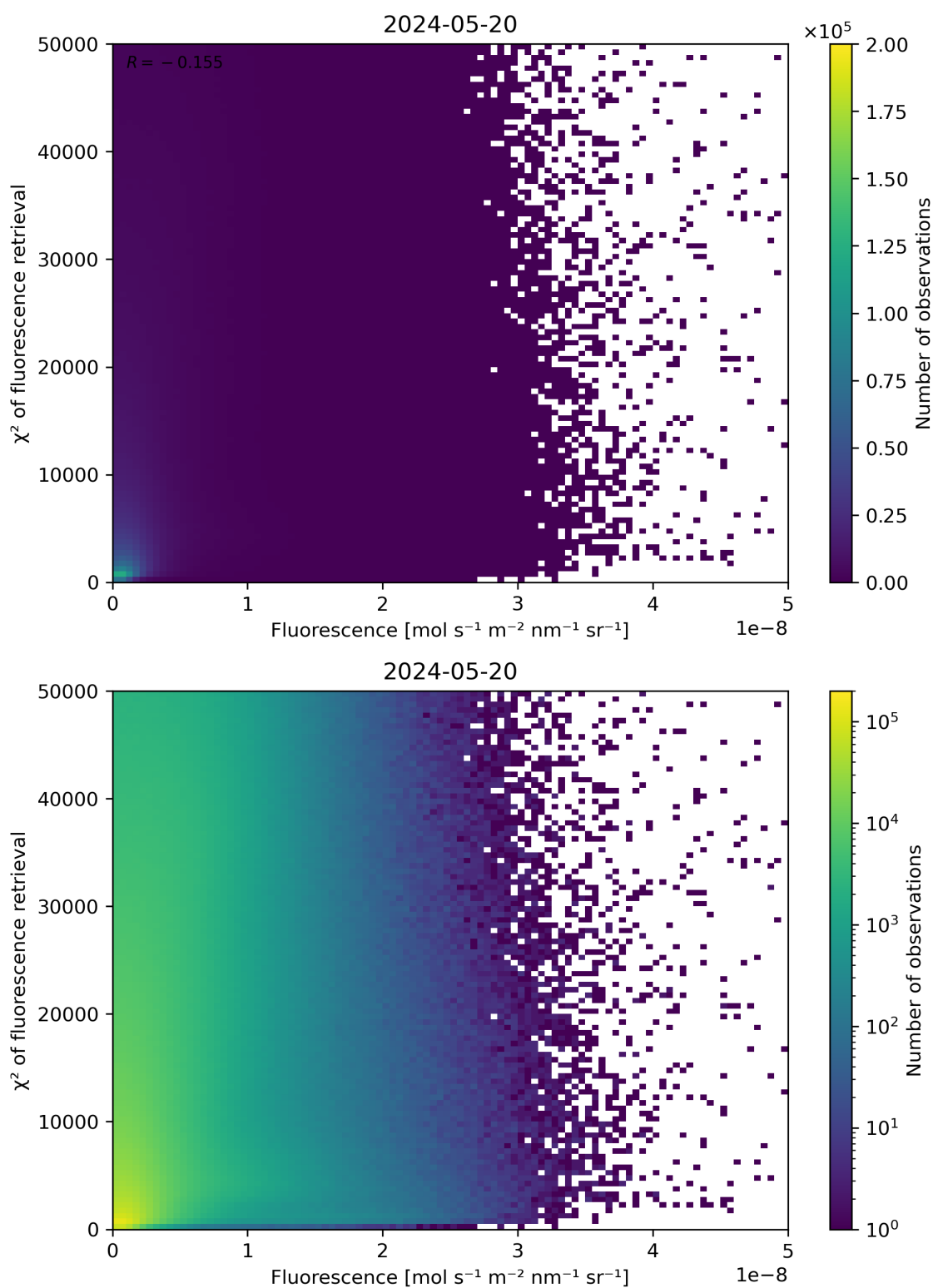
Figure 85: Scatter density plot of “Fluorescence” against “ \chi^2 of fluorescence retrieval” for 2024-05-19 to 2024-05-21.
