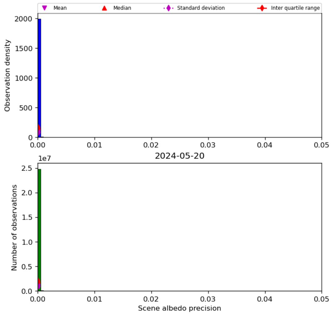
Figure 35: Histogram of “Scene albedo precision” for 2024-05-19 to 2024-05-21
