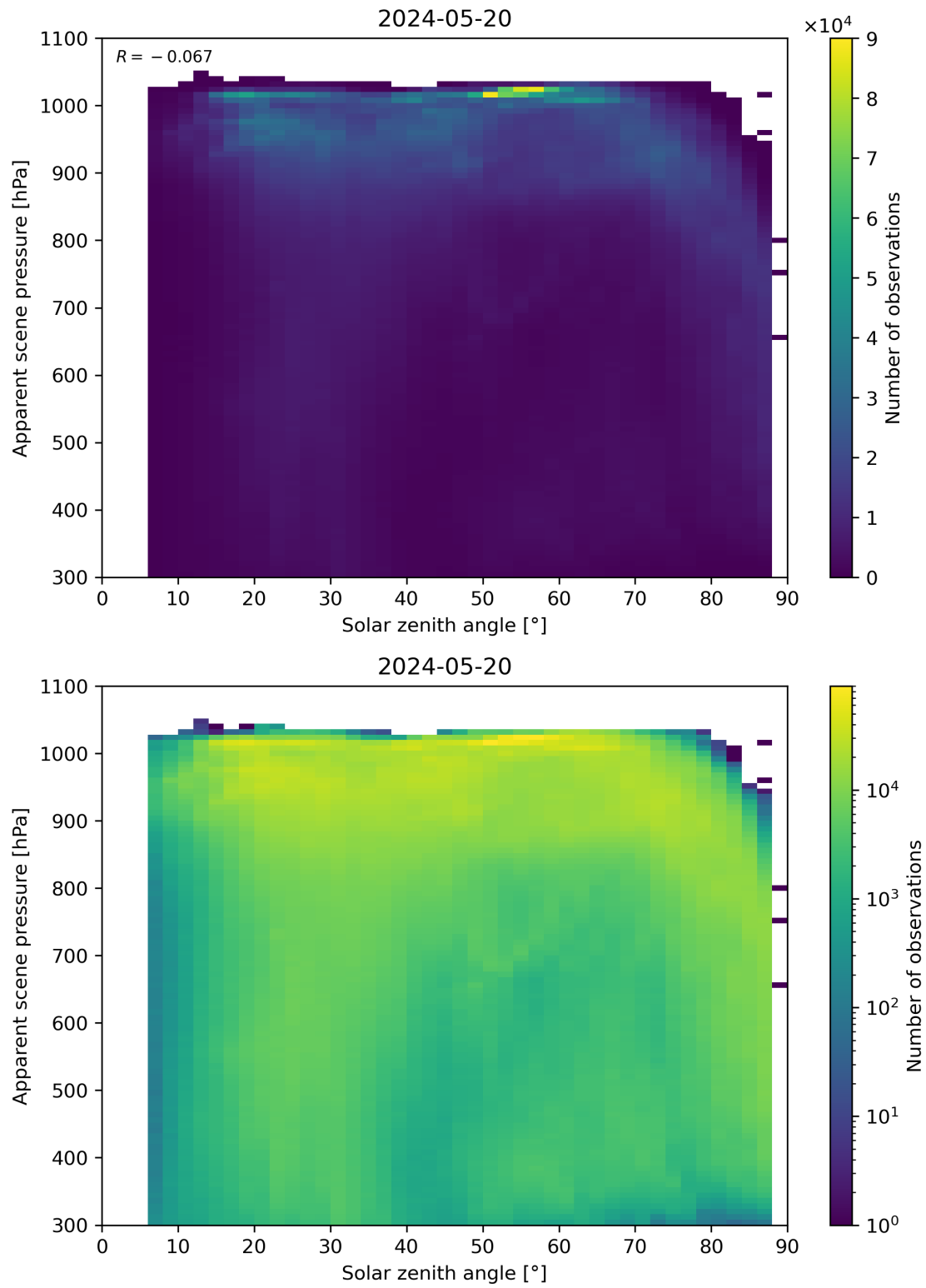
Figure 108: Scatter density plot of “Solar zenith angle” against “Apparent scene pressure” for 2024-05-19 to 2024-05-21.
