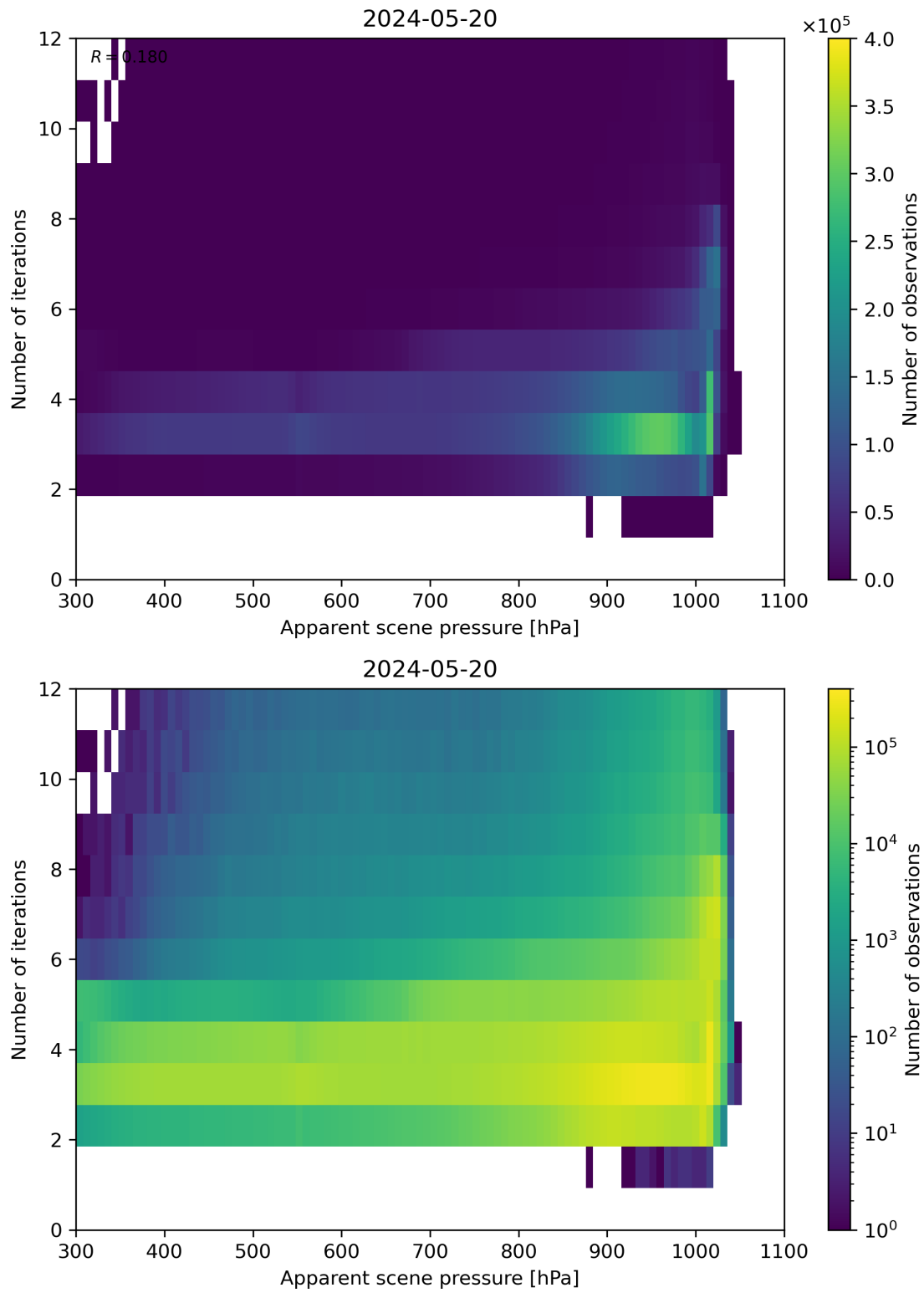
Figure 65: Scatter density plot of “Apparent scene pressure” against “Number of iterations” for 2024-05-19 to 2024-05-21.
