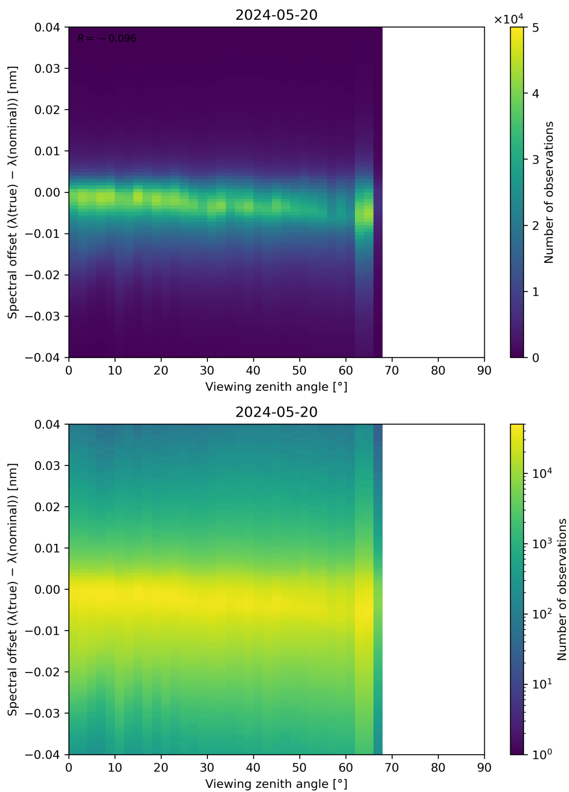
Figure 128: Scatter density plot of “Viewing zenith angle” against “Spectral offset ( \lambda(\text{true}) - \lambda(\text{nominal}) )” for 2024-05-19 to 2024-05-21.
