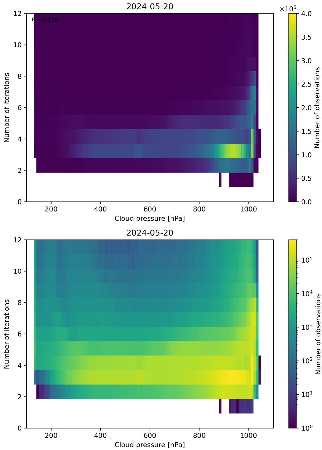
Figure 81: Scatter density plot of “Cloud pressure” against “Number of iterations” for 2024-05-19 to 2024-05-21.
