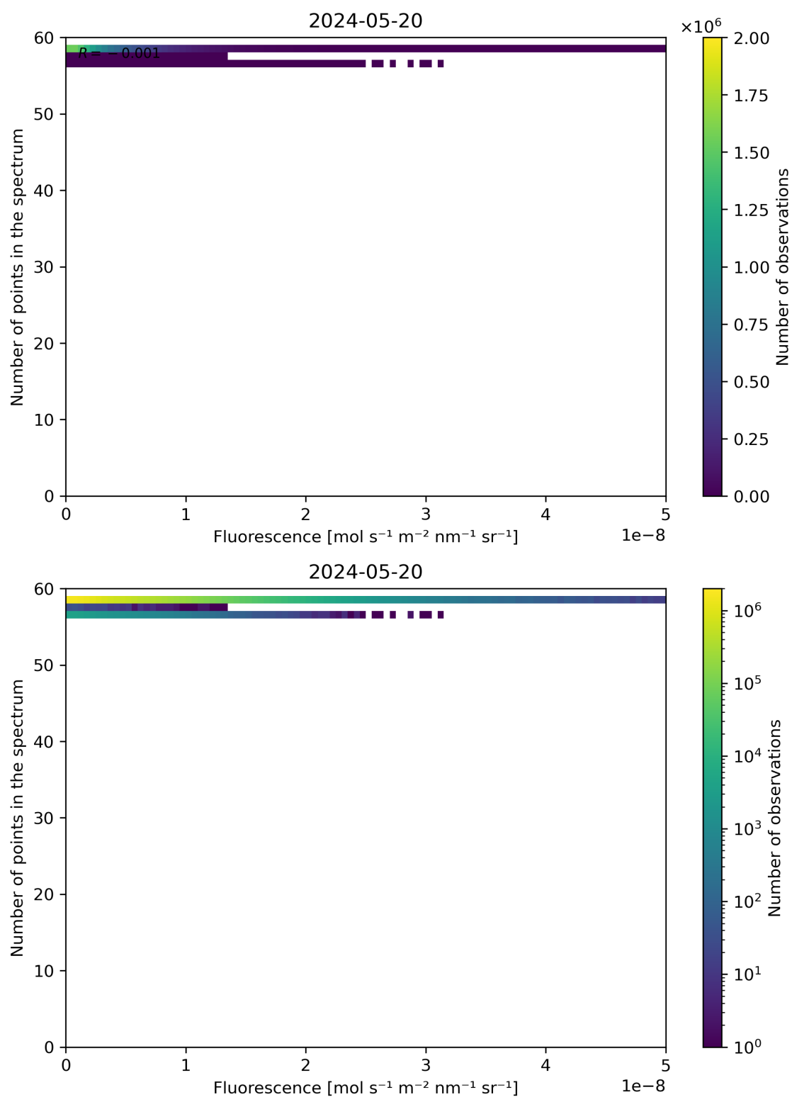
Figure 86: Scatter density plot of “Fluorescence” against “Number of points in the spectrum” for 2024-05-19 to 2024-05-21.
