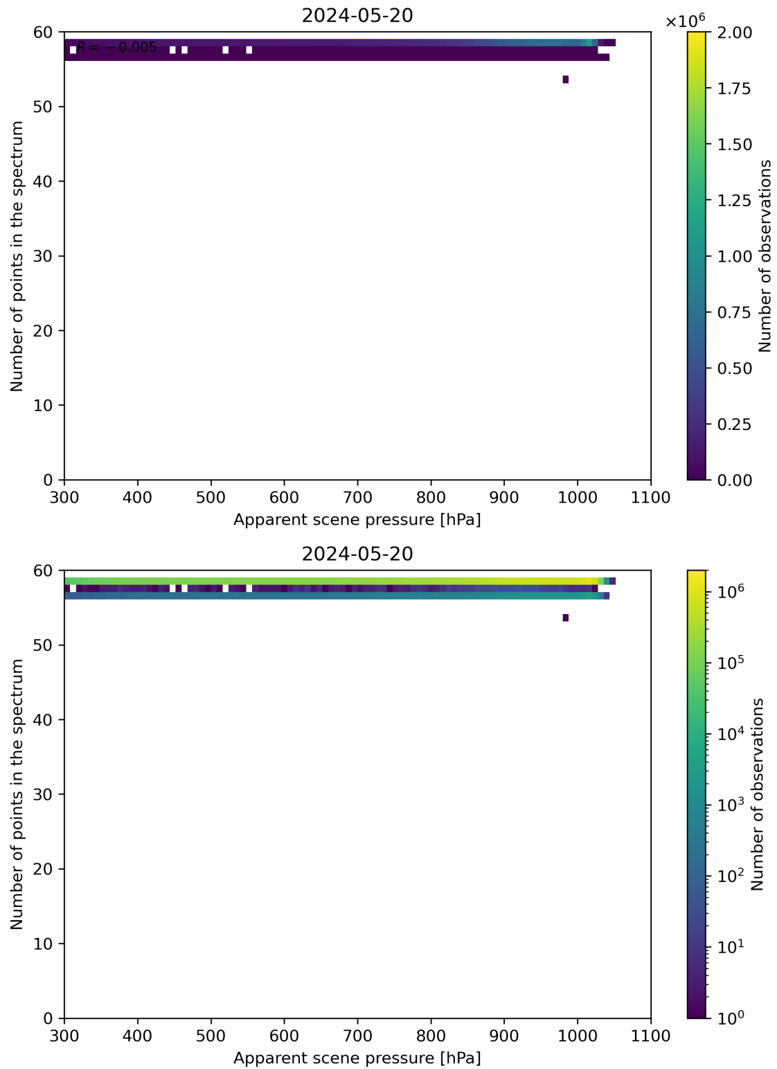
Figure 66: Scatter density plot of “Apparent scene pressure” against “Number of points in the spectrum” for 2024-05-19 to 2024-05-21.
