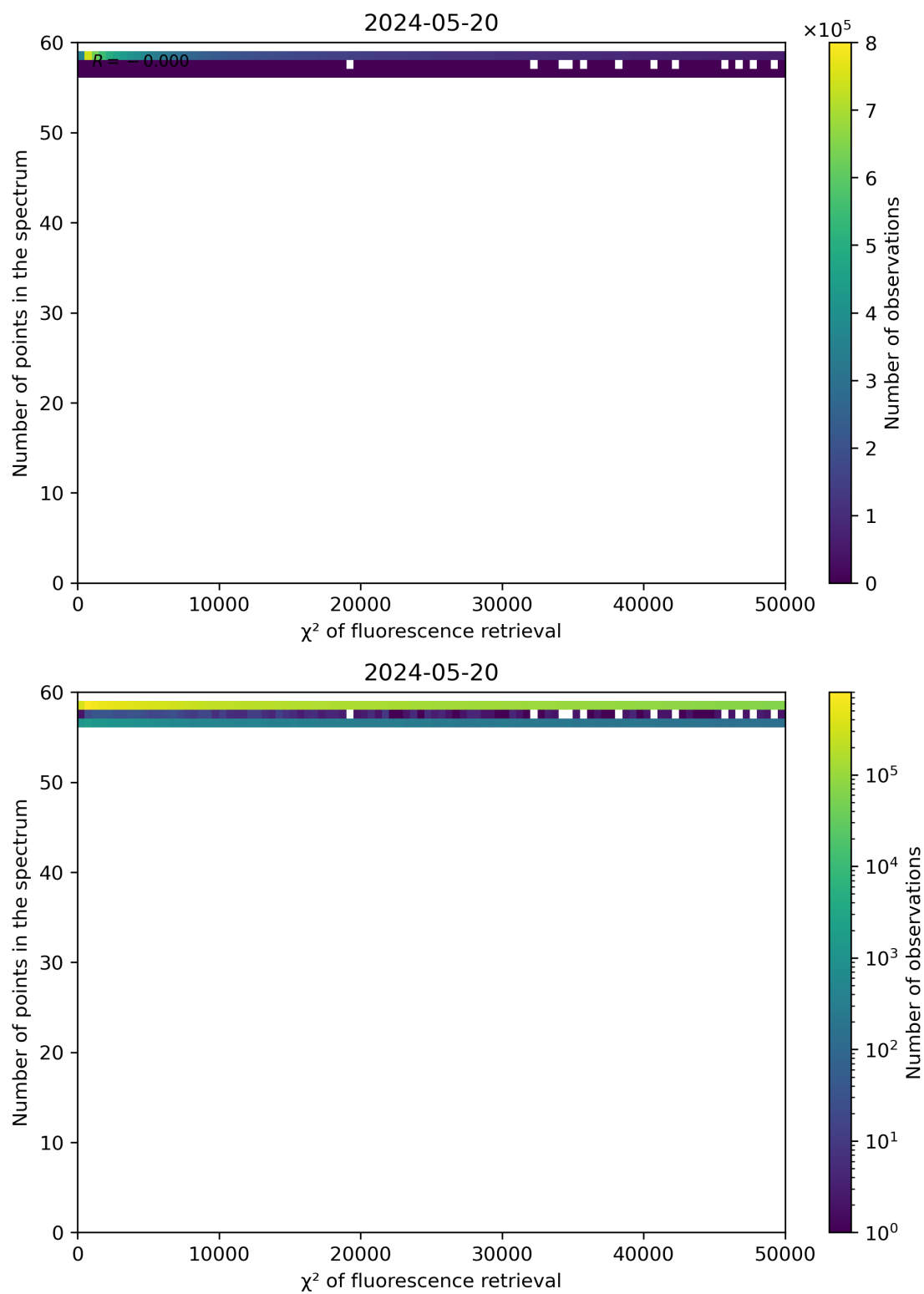
Figure 68: Scatter density plot of " \chi^2 of fluorescence retrieval" against "Number of points in the spectrum" for 2024-05-19 to 2024-05-21.
