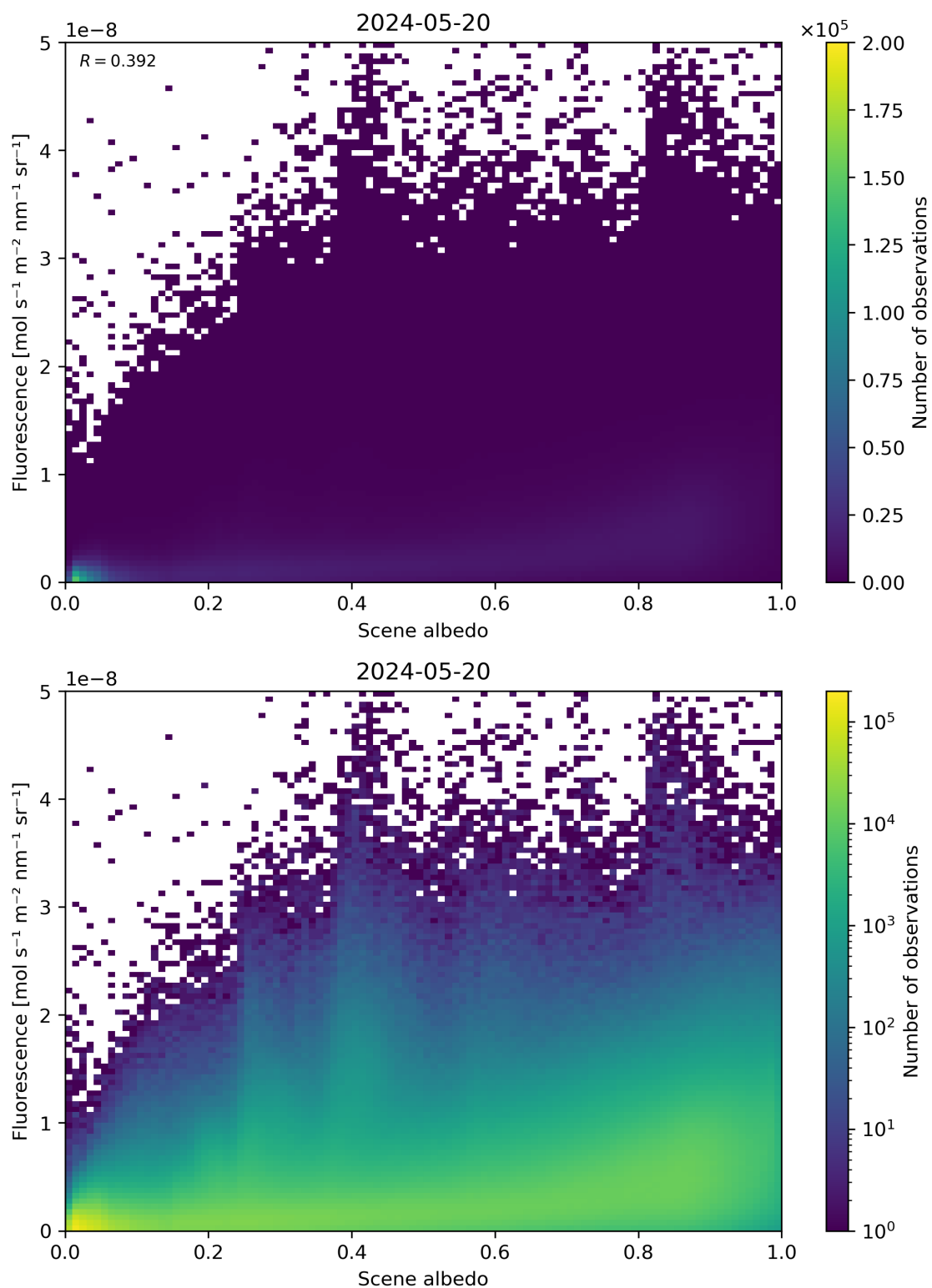
Figure 104: Scatter density plot of “Scene albedo” against “Fluorescence” for 2024-05-19 to 2024-05-21.
