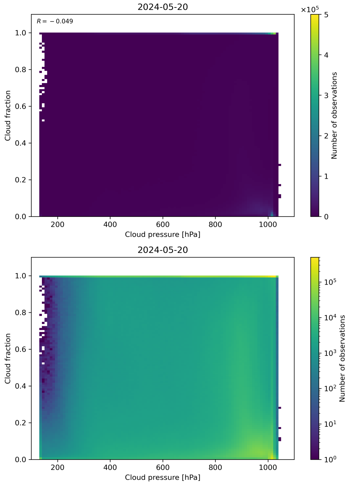
Figure 79: Scatter density plot of “Cloud pressure” against “Cloud fraction” for 2024-05-19 to 2024-05-21.
