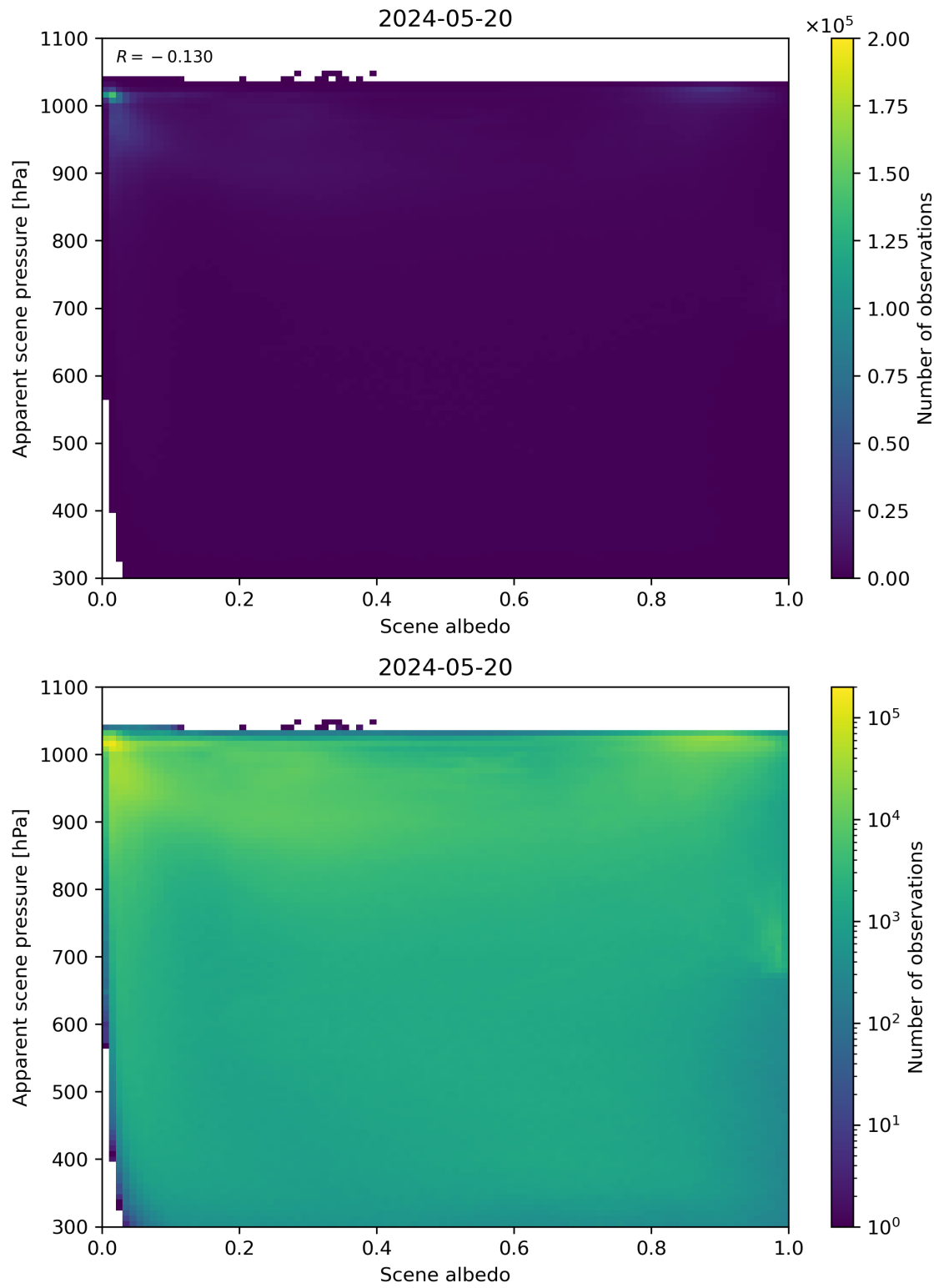
Figure 102: Scatter density plot of “Scene albedo” against “Apparent scene pressure” for 2024-05-19 to 2024-05-21.
