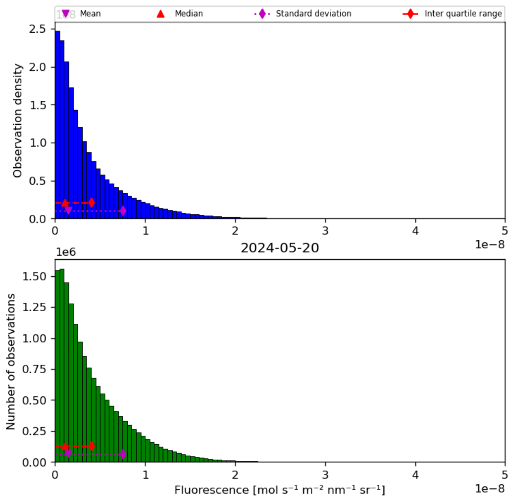
Figure 40: Histogram of “Fluorescence” for 2024-05-19 to 2024-05-21
