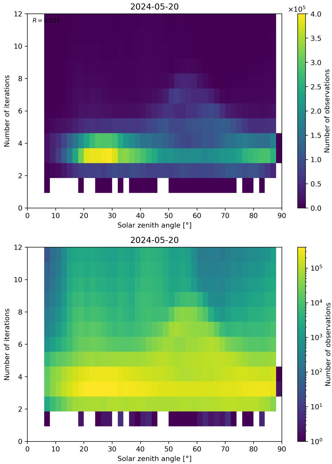
Figure 114: Scatter density plot of “Solar zenith angle” against “Number of iterations” for 2024-05-19 to 2024-05-21.
