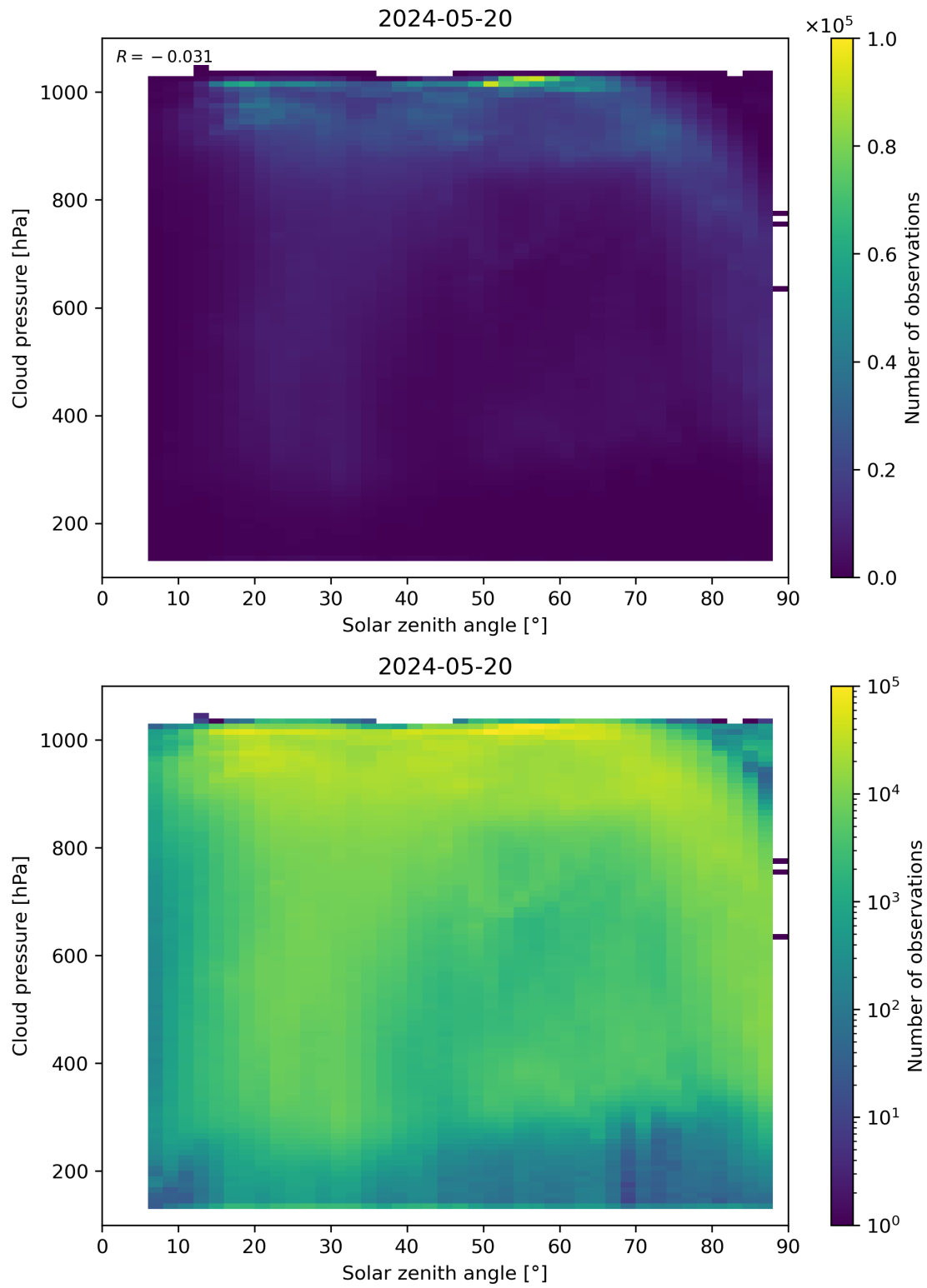
Figure 111: Scatter density plot of “Solar zenith angle” against “Cloud pressure” for 2024-05-19 to 2024-05-21.
