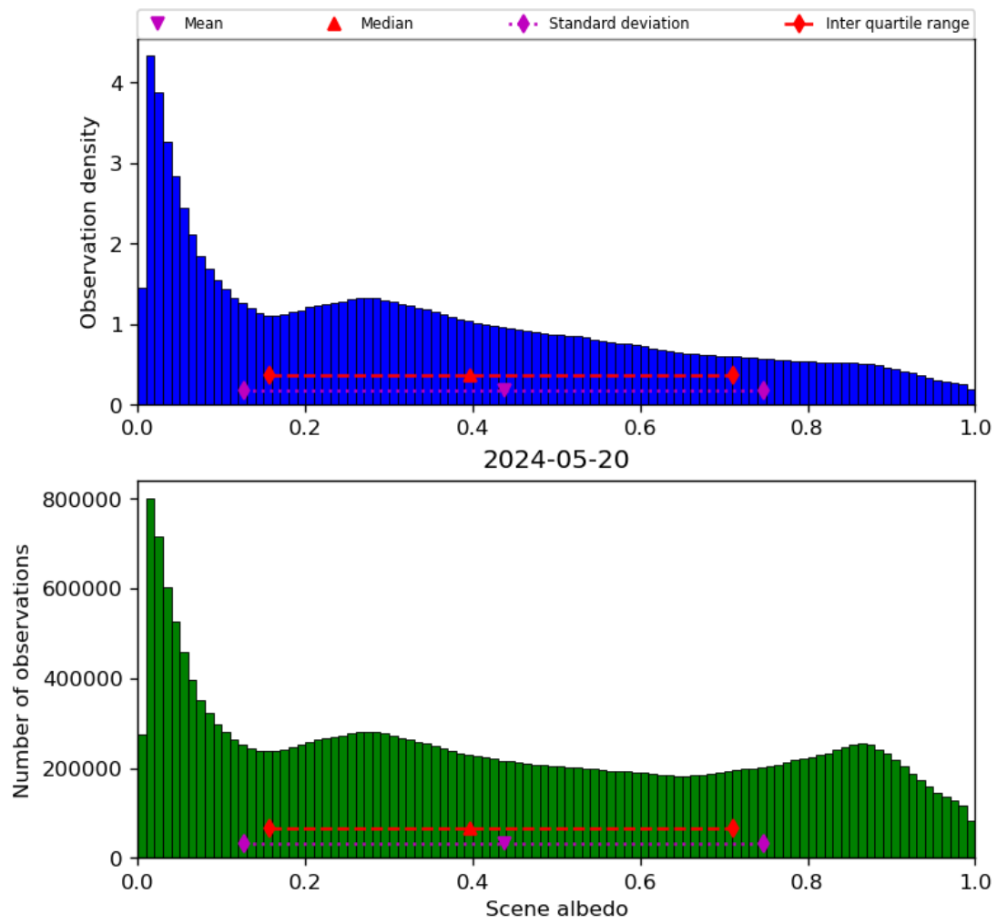
Figure 34: Histogram of “Scene albedo” for 2024-05-19 to 2024-05-21
