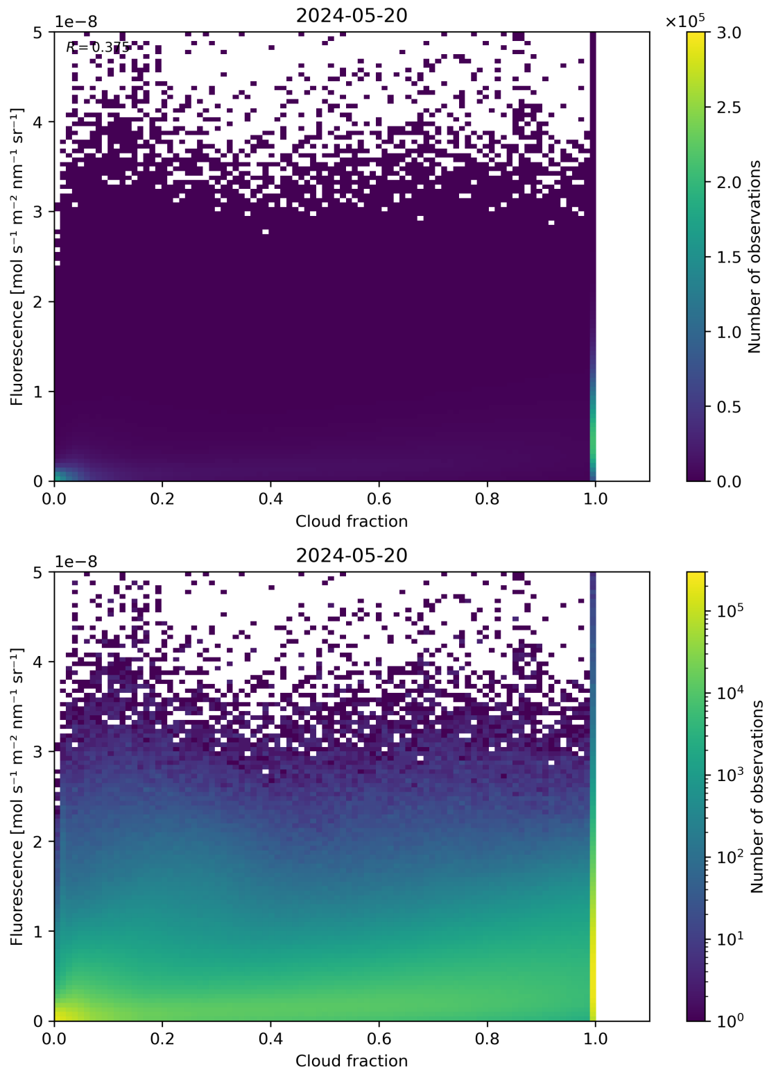
Figure 72: Scatter density plot of “Cloud fraction” against “Fluorescence” for 2024-05-19 to 2024-05-21.
