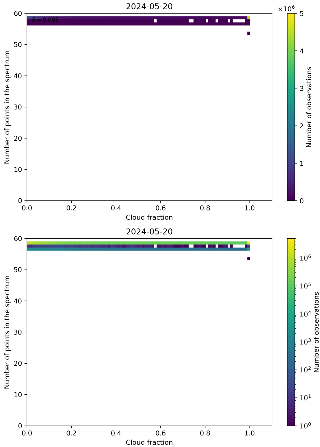
Figure 74: Scatter density plot of “Cloud fraction” against “Number of points in the spectrum” for 2024-05-19 to 2024-05-21.
