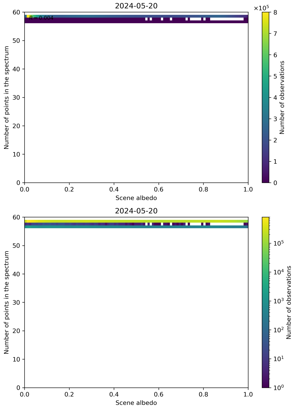
Figure 106: Scatter density plot of “Scene albedo” against “Number of points in the spectrum” for 2024-05-19 to 2024-05-21.
