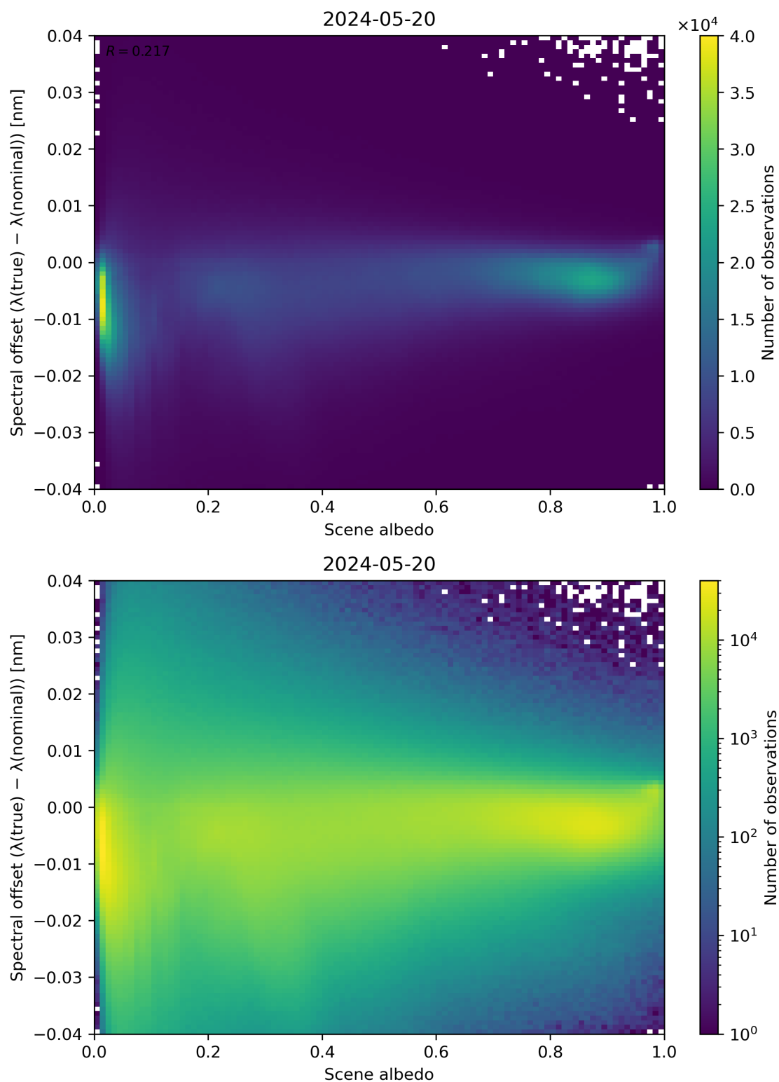
Figure 107: Scatter density plot of “Scene albedo” against “Spectral offset ( \lambda(\text{true}) - \lambda(\text{nominal}) )” for 2024-05-19 to 2024-05-21.
