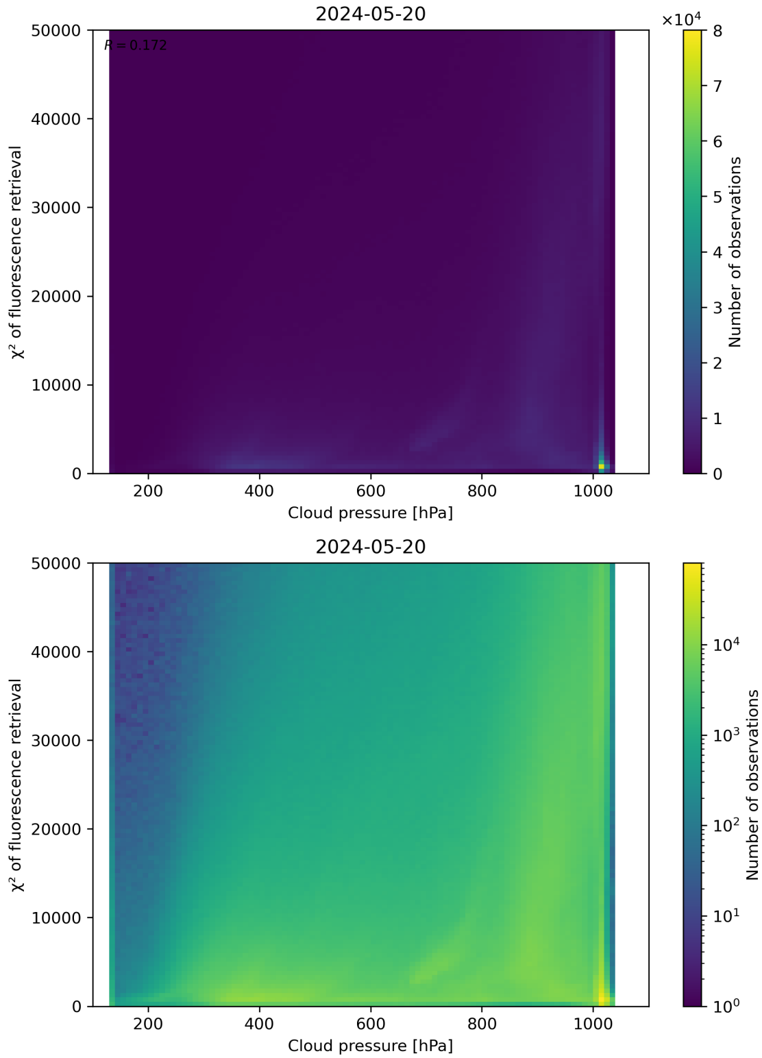
Figure 78: Scatter density plot of “Cloud pressure” against “ \chi^2 of fluorescence retrieval” for 2024-05-19 to 2024-05-21.
