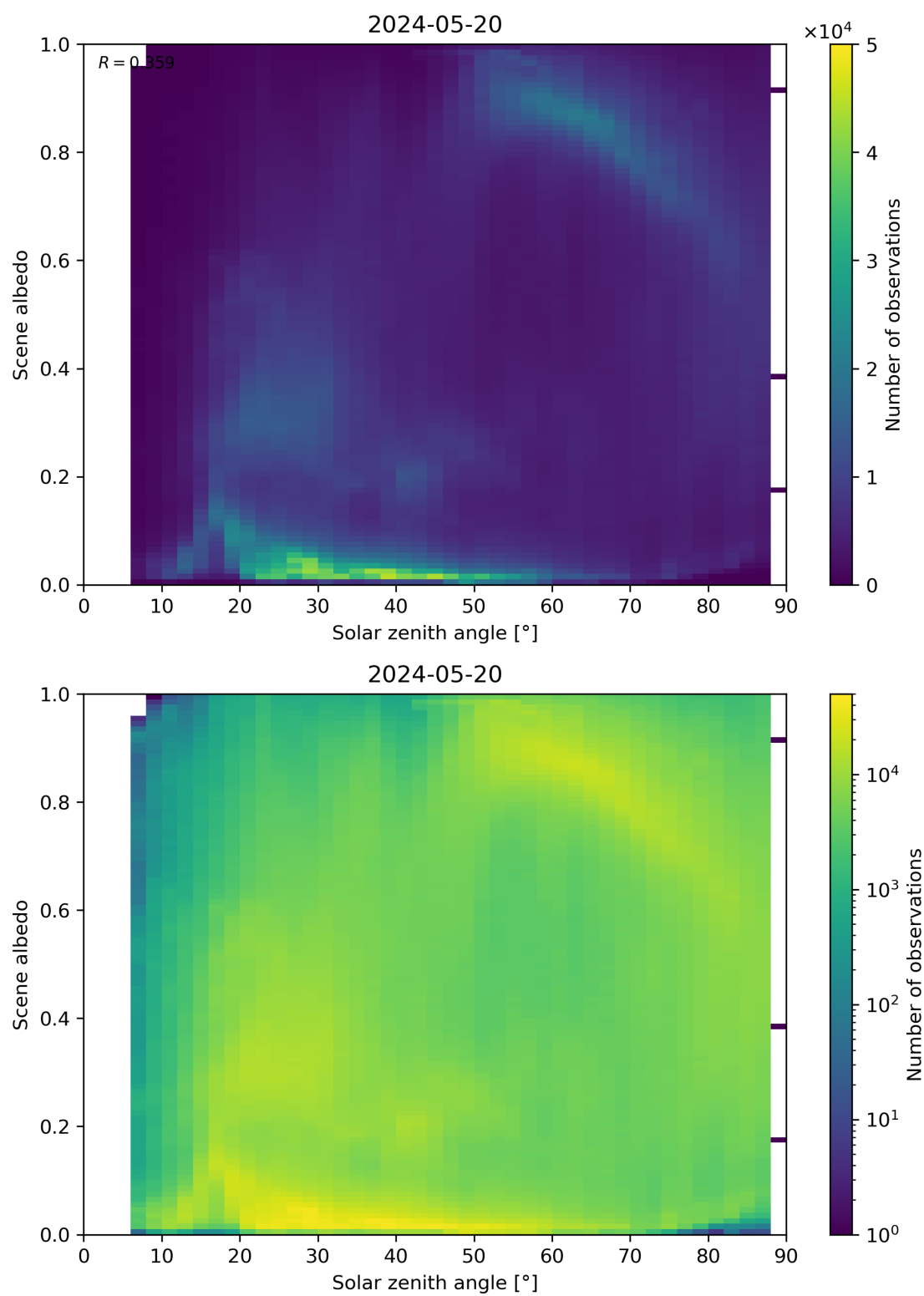
Figure 116: Scatter density plot of “Solar zenith angle” against “Scene albedo” for 2024-05-19 to 2024-05-21.
