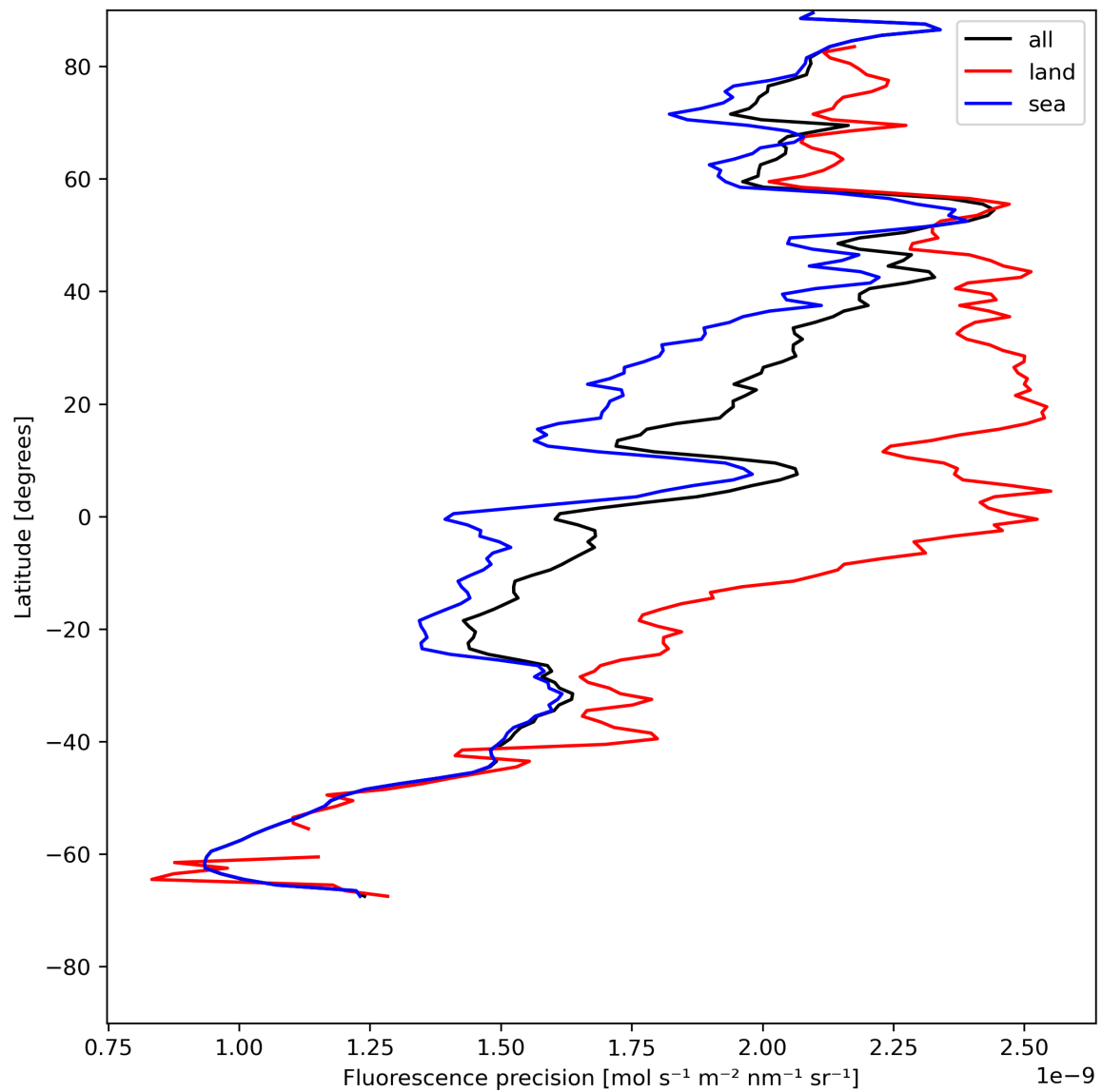
Figure 24: Zonal average of “Fluorescence precision” for 2024-05-19 to 2024-05-21.
