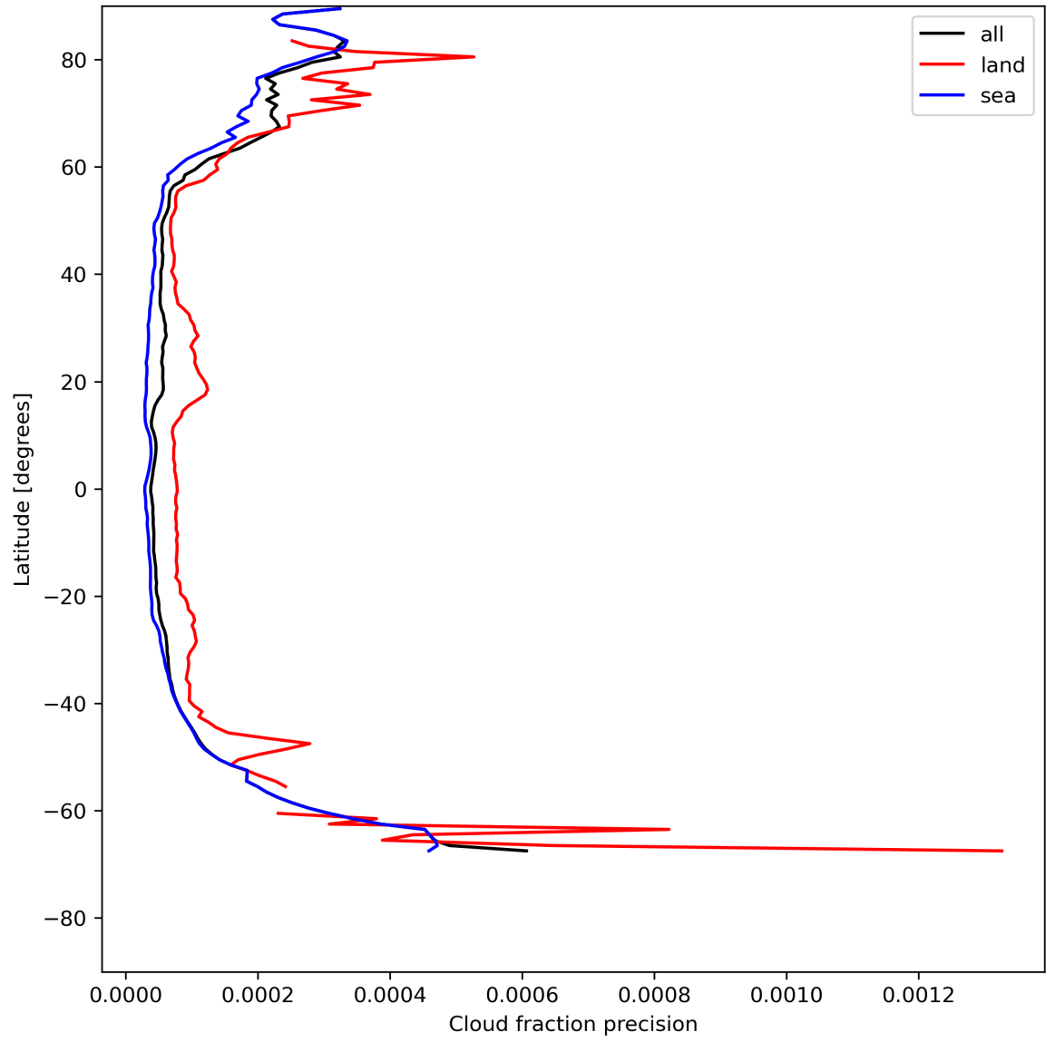
Figure 16: Zonal average of “Cloud fraction precision” for 2024-05-19 to 2024-05-21.
