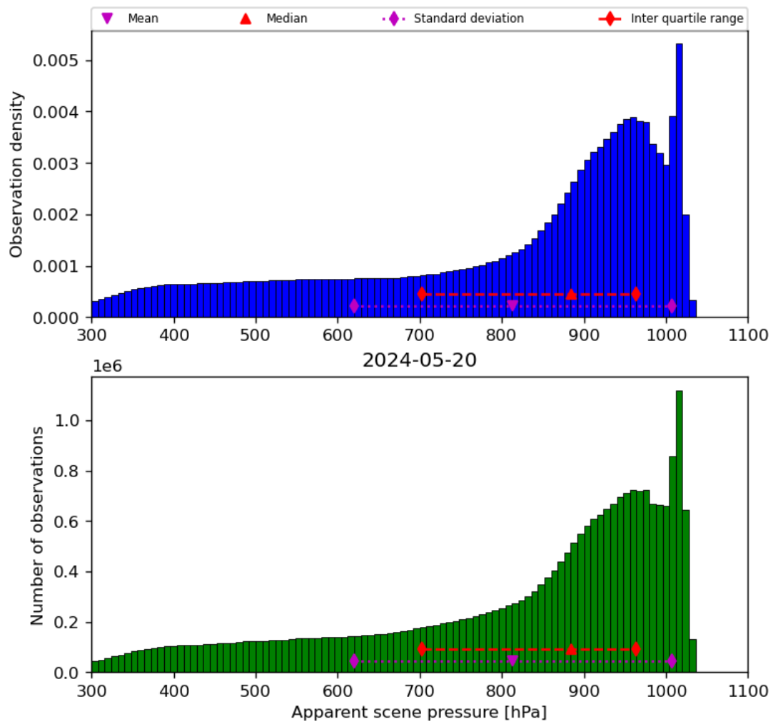
Figure 36: Histogram of “Apparent scene pressure” for 2024-05-19 to 2024-05-21
