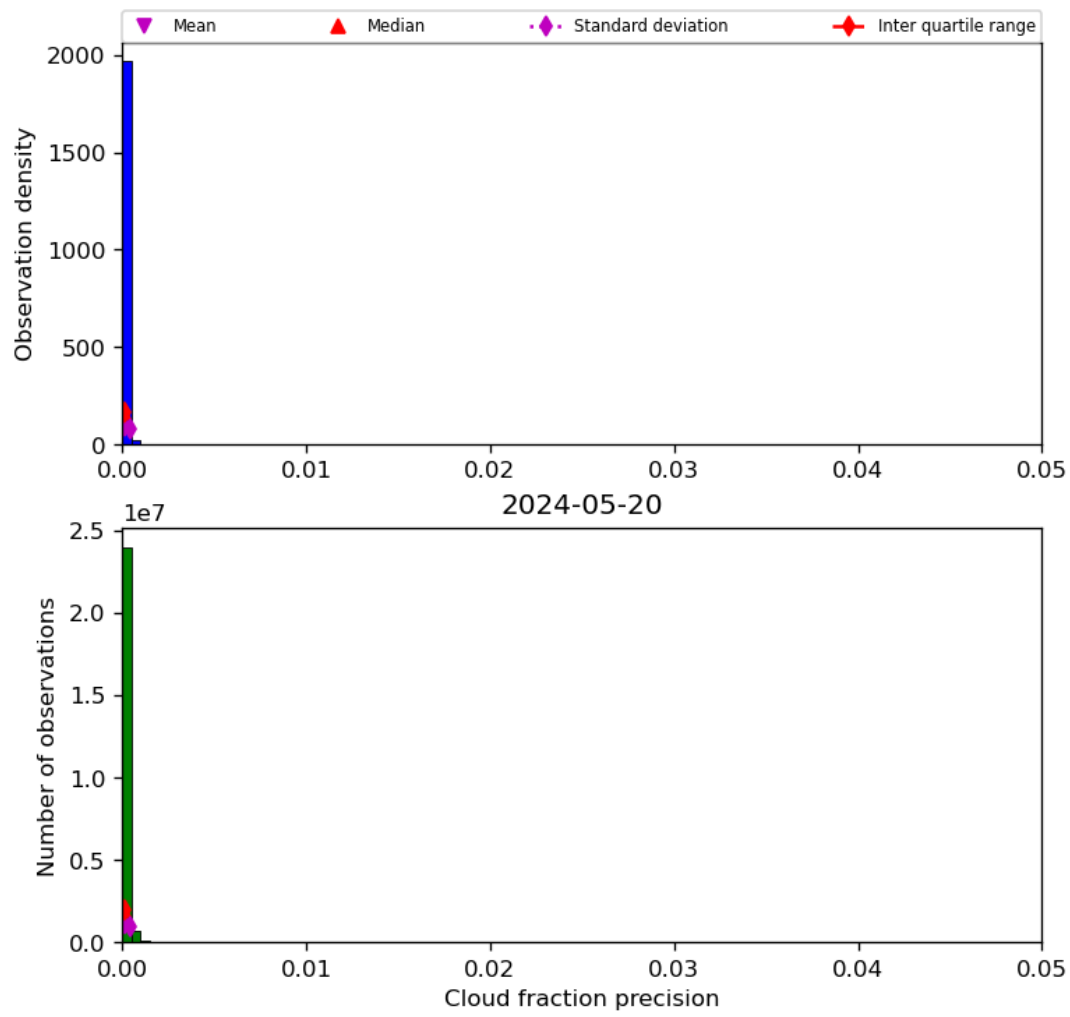
Figure 33: Histogram of “Cloud fraction precision” for 2024-05-19 to 2024-05-21
