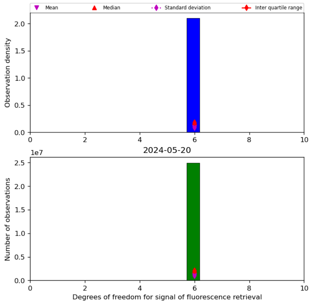
Figure 43: Histogram of “Degrees of freedom for signal of fluorescence retrieval” for 2024-05-19 to 2024-05-21
