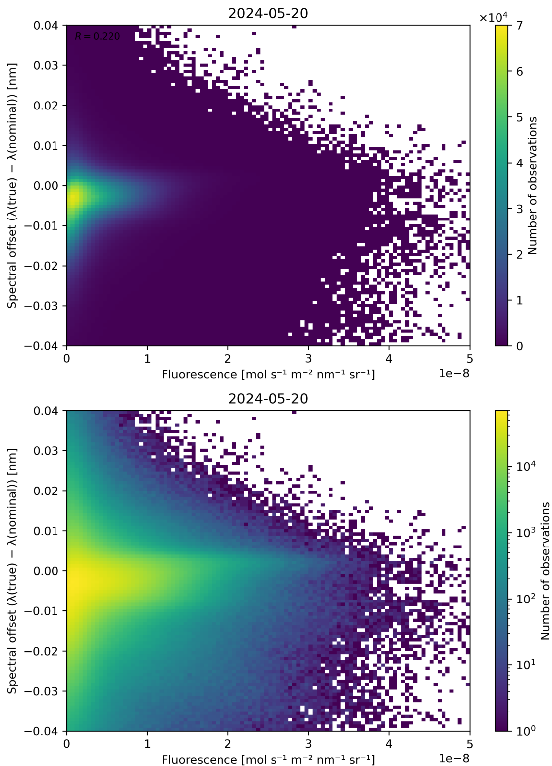
Figure 87: Scatter density plot of “Fluorescence” against “Spectral offset ( \lambda(\text{true}) - \lambda(\text{nominal}) )” for 2024-05-19 to 2024-05-21.
