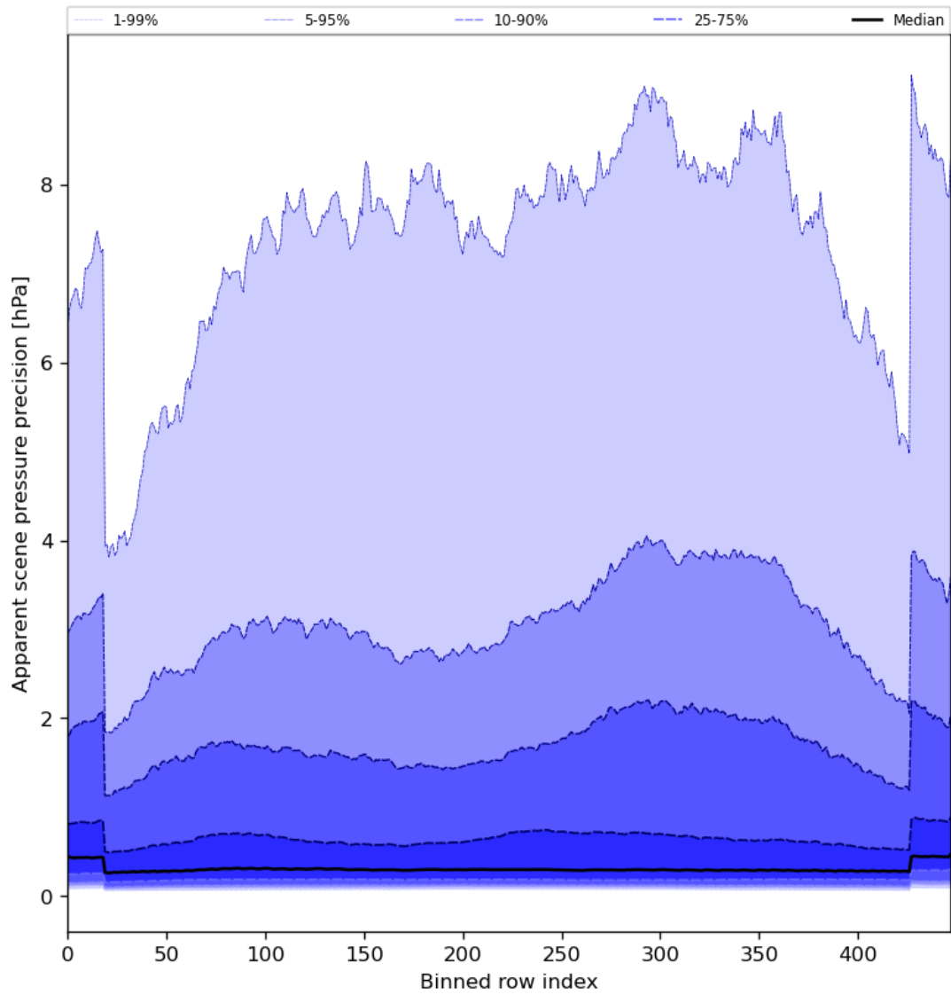
Figure 54: Along track statistics of “Apparent scene pressure precision” for 2024-05-19 to 2024-05-21
