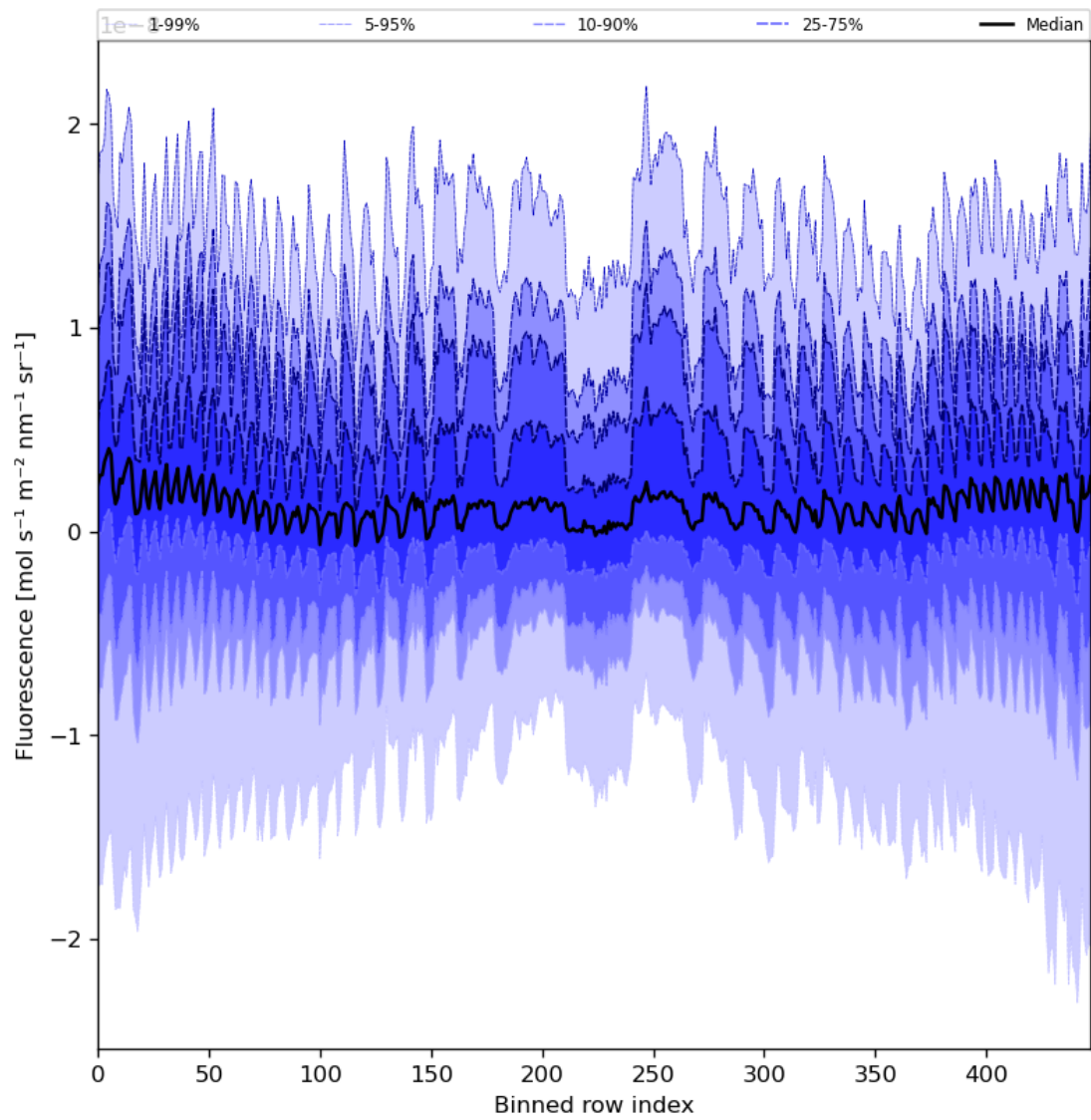
Figure 57: Along track statistics of “Fluorescence” for 2024-05-19 to 2024-05-21
