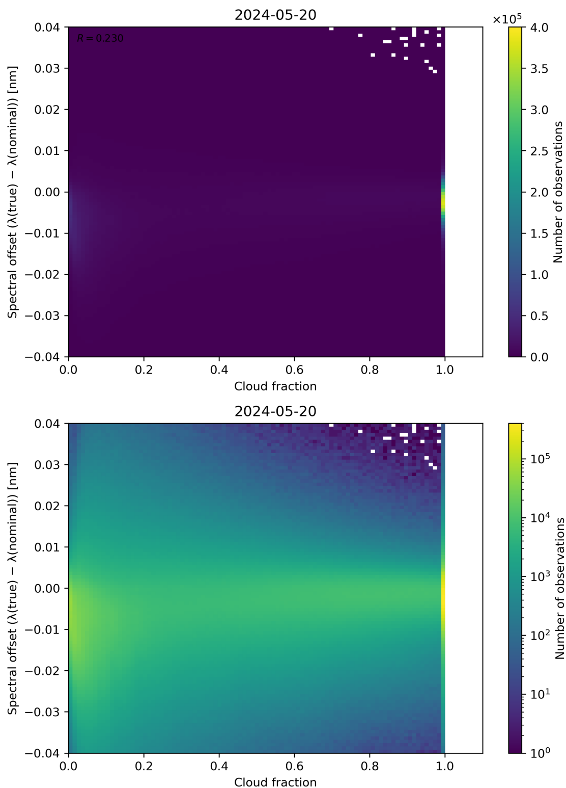
Figure 76: Scatter density plot of “Cloud fraction” against “Spectral offset ( \lambda(\text{true}) - \lambda(\text{nominal}) )” for 2024-05-19 to 2024-05-21.
