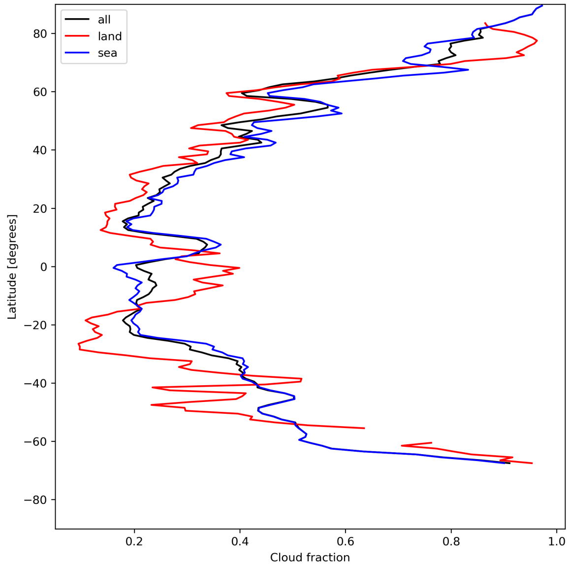
Figure 15: Zonal average of “Cloud fraction” for 2024-05-19 to 2024-05-21.
