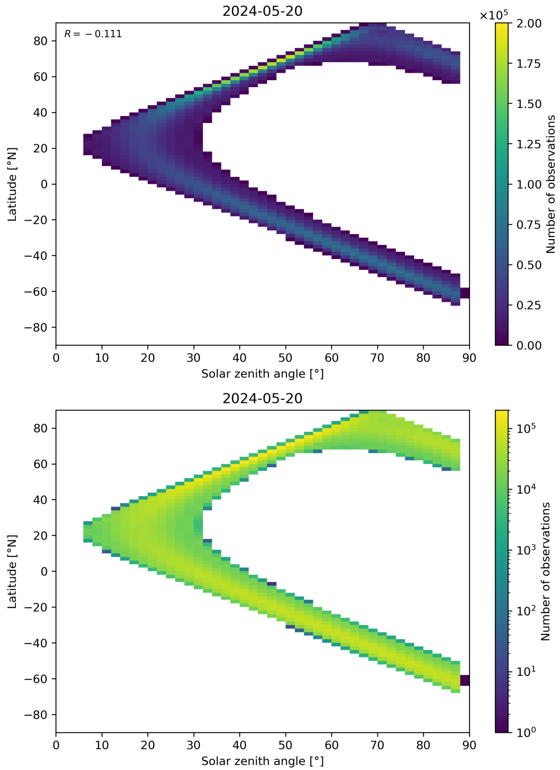
Figure 113: Scatter density plot of “Solar zenith angle” against “Latitude” for 2024-05-19 to 2024-05-21.
