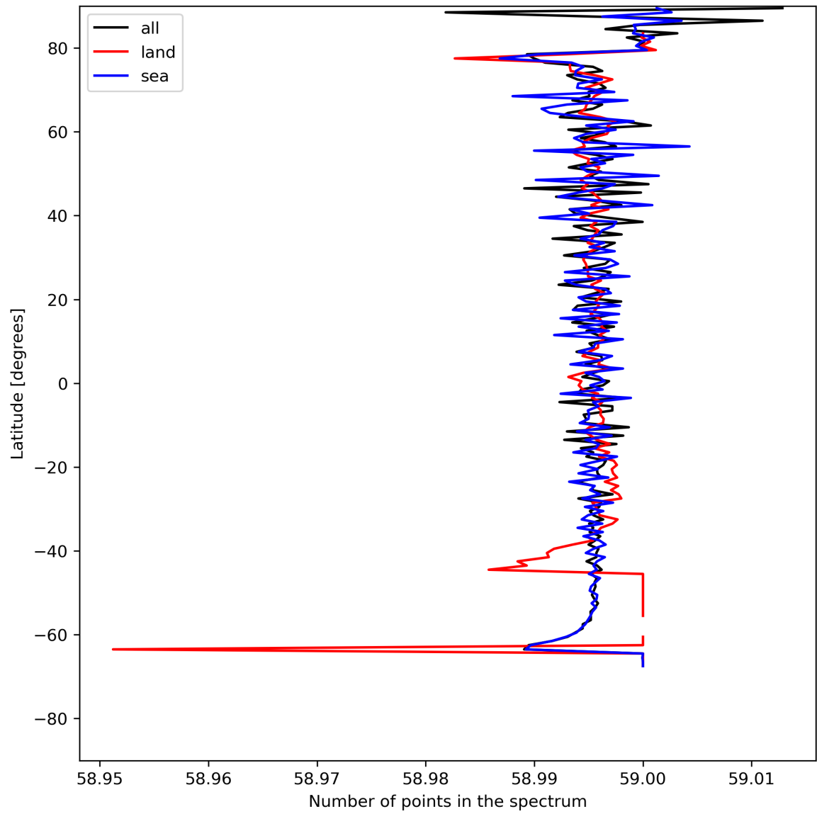
Figure 27: Zonal average of “Number of points in the spectrum” for 2024-05-19 to 2024-05-21.
