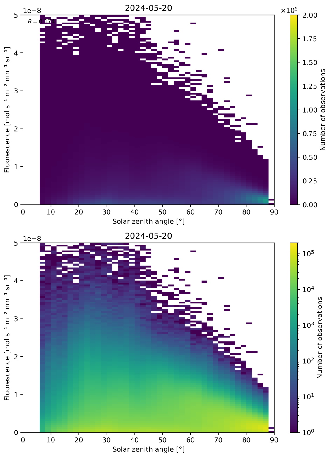
Figure 112: Scatter density plot of “Solar zenith angle” against “Fluorescence” for 2024-05-19 to 2024-05-21.
