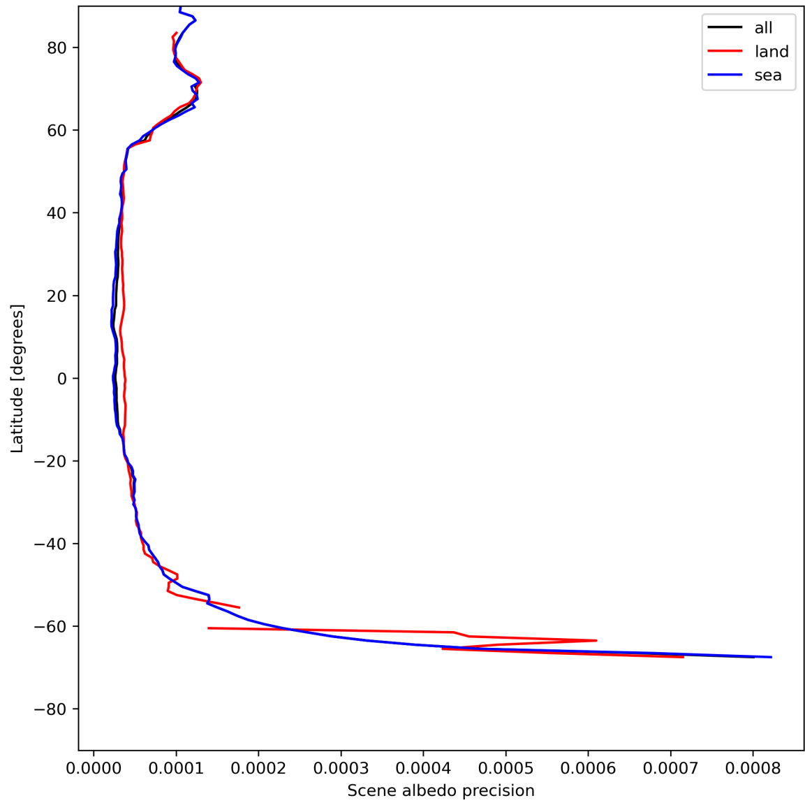
Figure 18: Zonal average of “Scene albedo precision” for 2024-05-19 to 2024-05-21.
