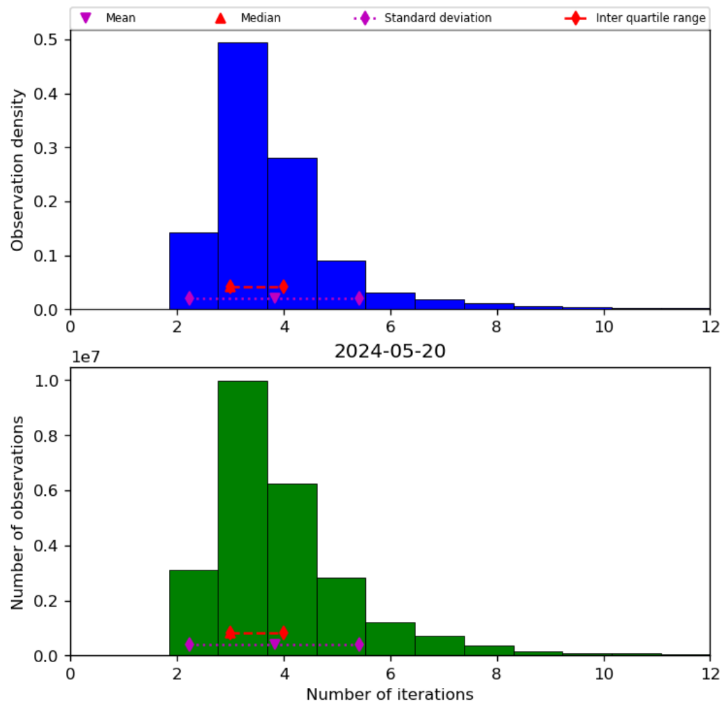
Figure 39: Histogram of “Number of iterations” for 2024-05-19 to 2024-05-21
