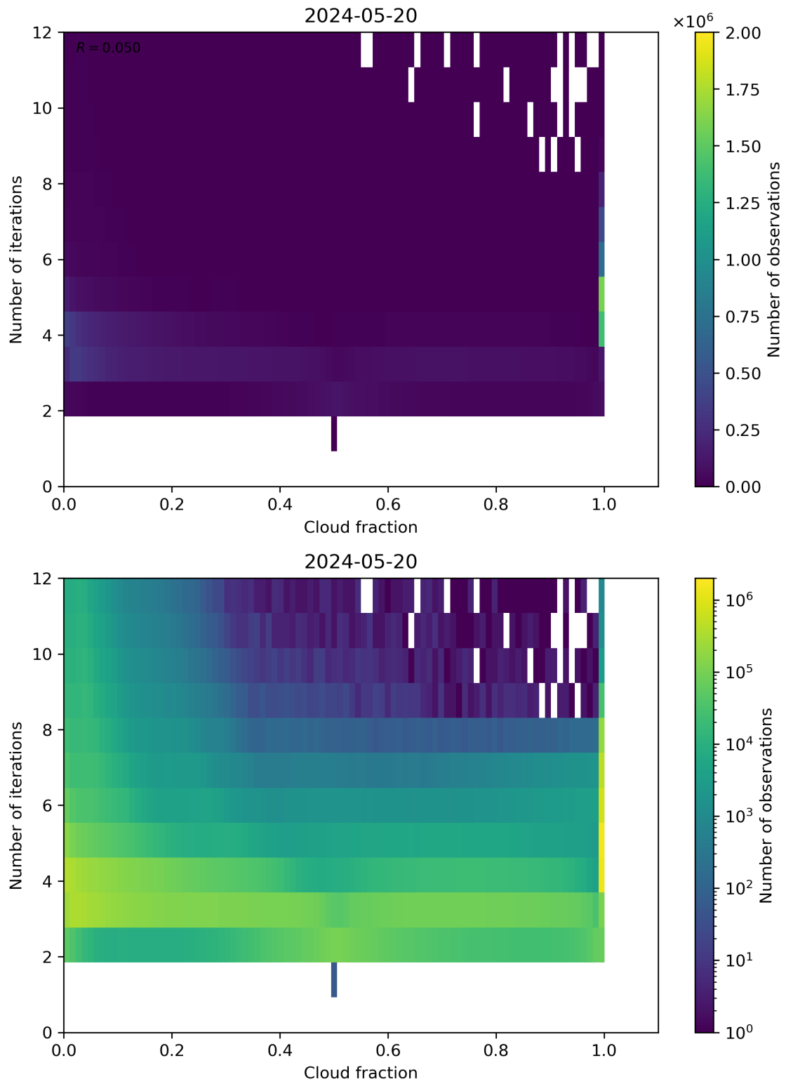
Figure 73: Scatter density plot of “Cloud fraction” against “Number of iterations” for 2024-05-19 to 2024-05-21.
