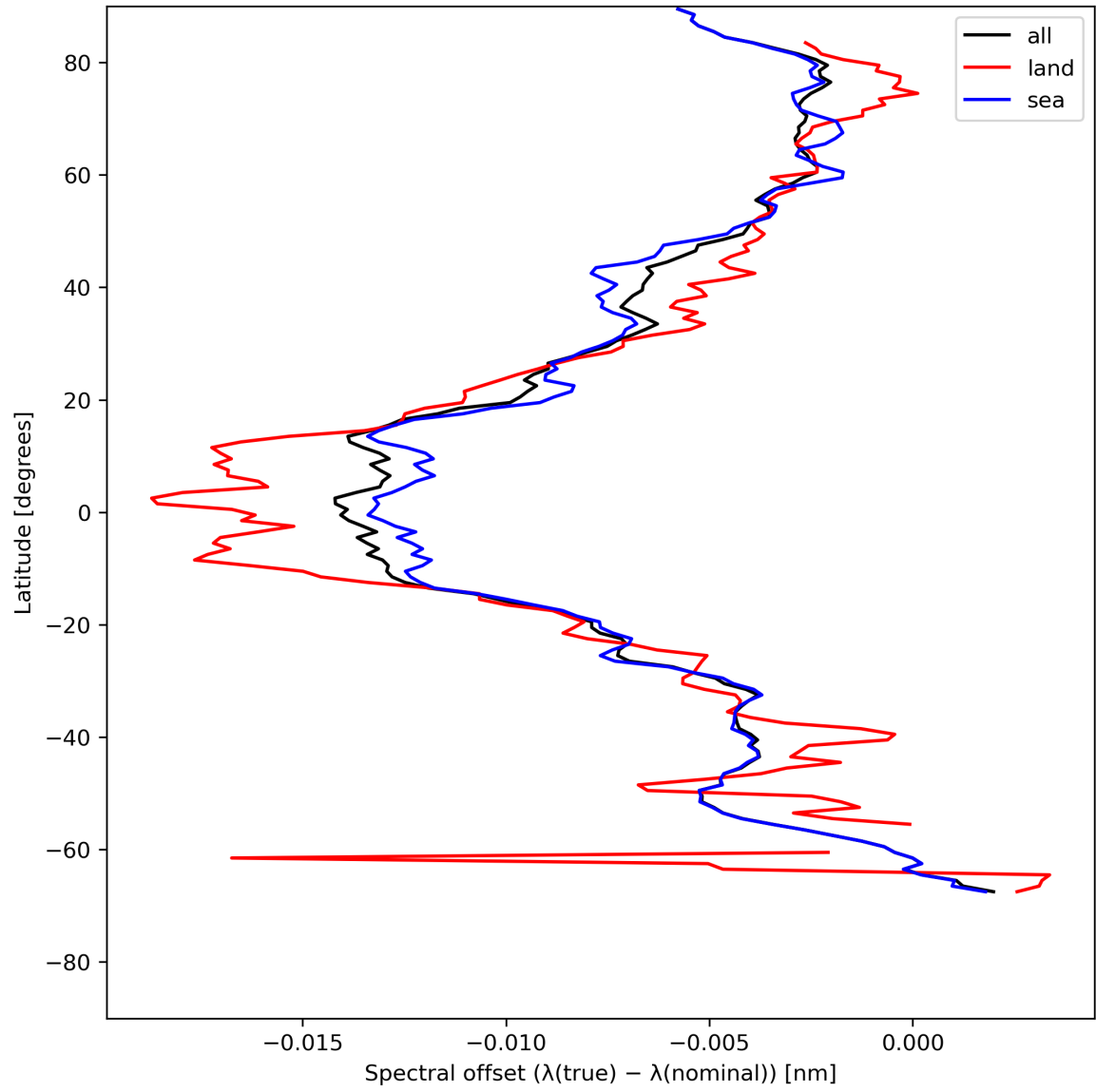
Figure 28: Zonal average of “Spectral offset ( \lambda(\text{true}) - \lambda(\text{nominal}) )” for 2024-05-19 to 2024-05-21.
