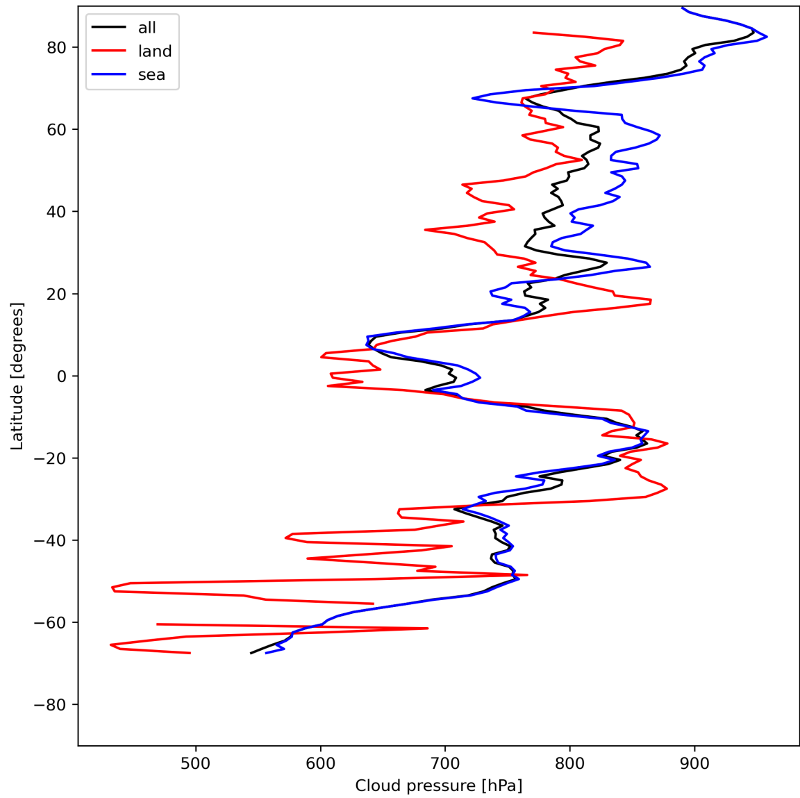
Figure 13: Zonal average of “Cloud pressure” for 2024-05-19 to 2024-05-21.
