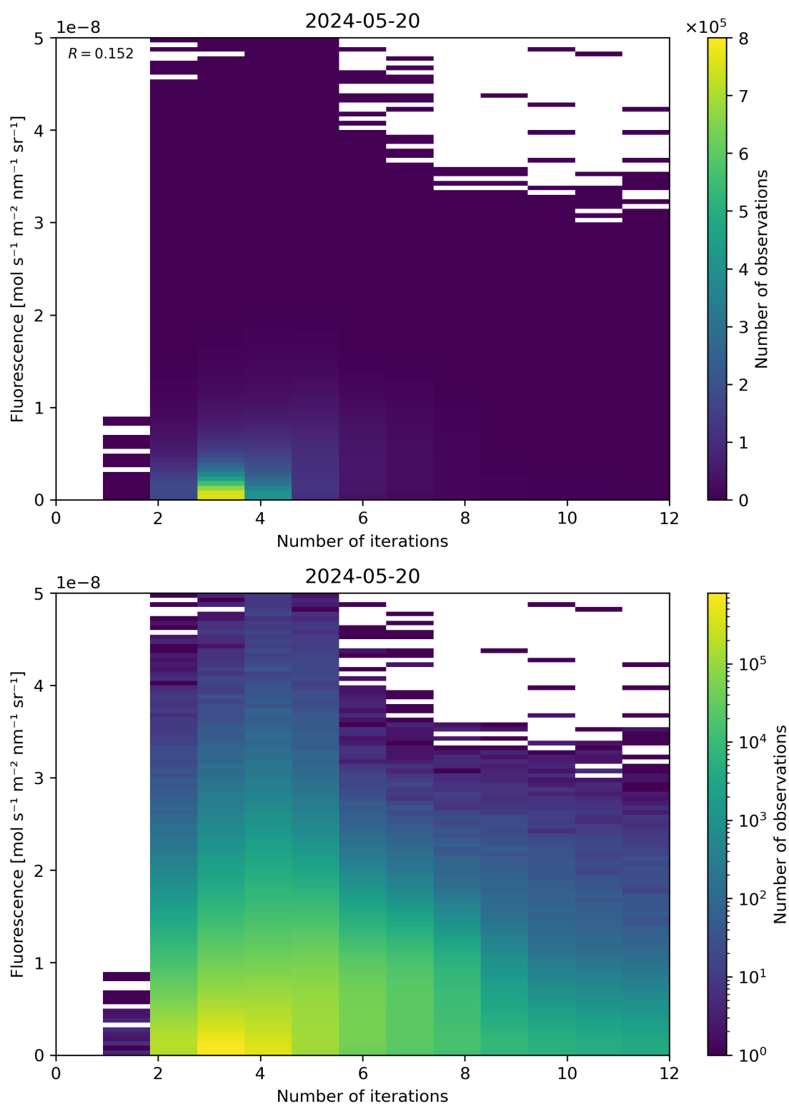
Figure 98: Scatter density plot of “Number of iterations” against “Fluorescence” for 2024-05-19 to 2024-05-21.
