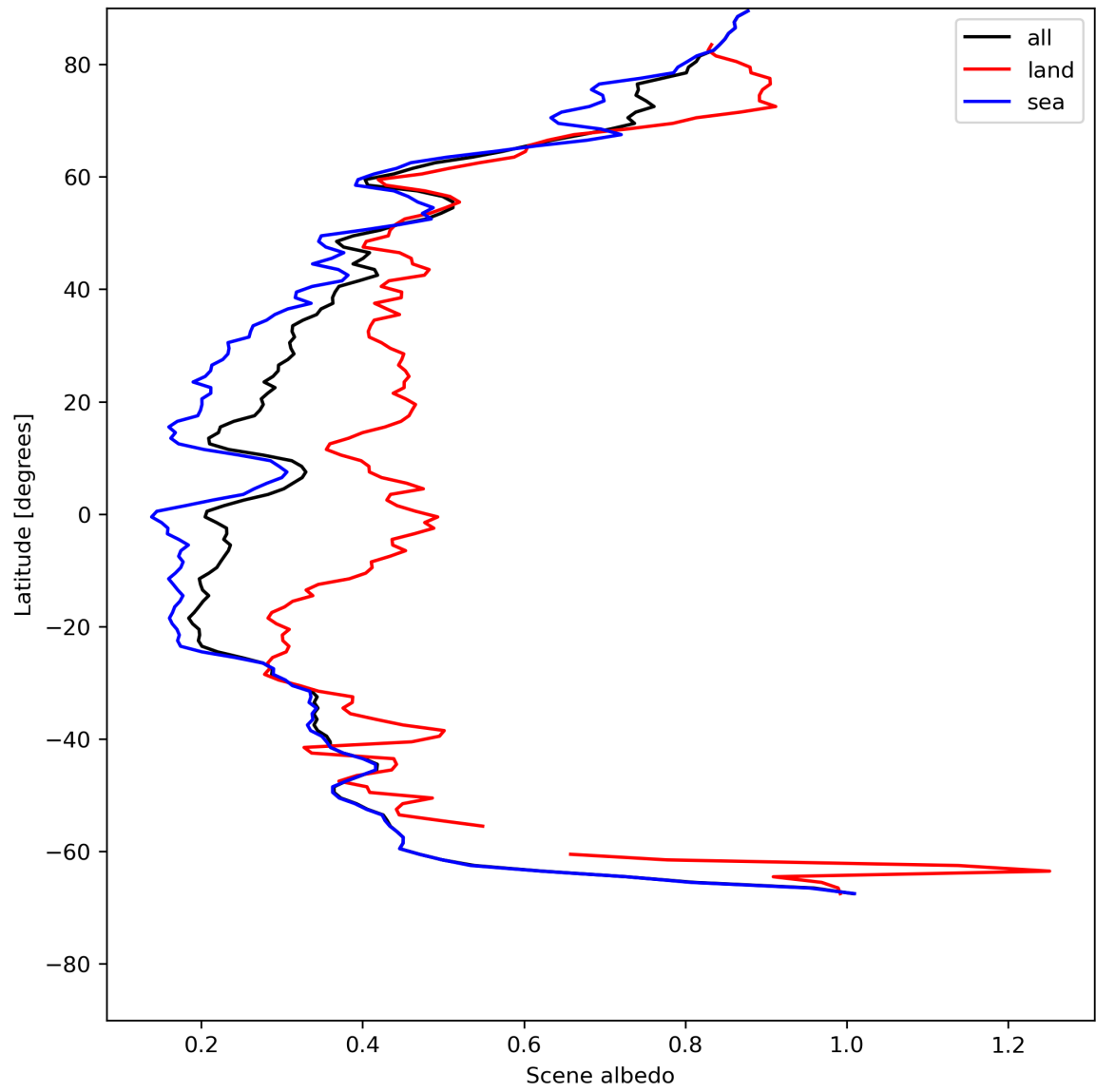
Figure 17: Zonal average of “Scene albedo” for 2024-05-19 to 2024-05-21.
