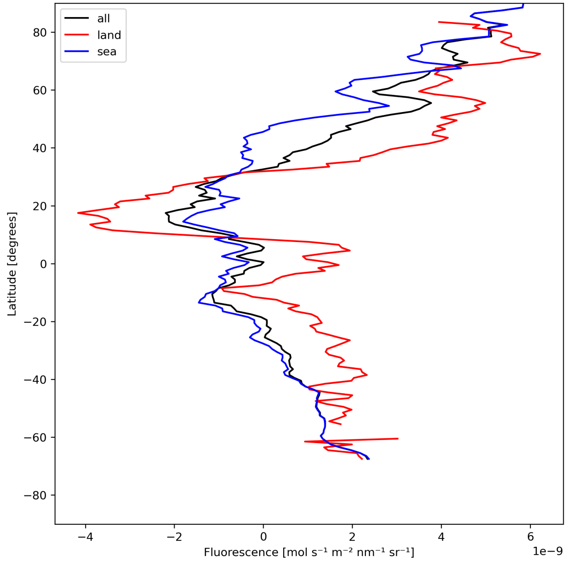
Figure 23: Zonal average of “Fluorescence” for 2024-05-19 to 2024-05-21.
