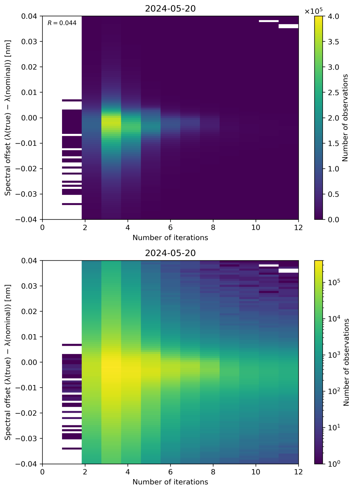
Figure 100: Scatter density plot of “Number of iterations” against “Spectral offset ( \lambda(\text{true}) - \lambda(\text{nominal}) )” for 2024-05-19 to 2024-05-21.
