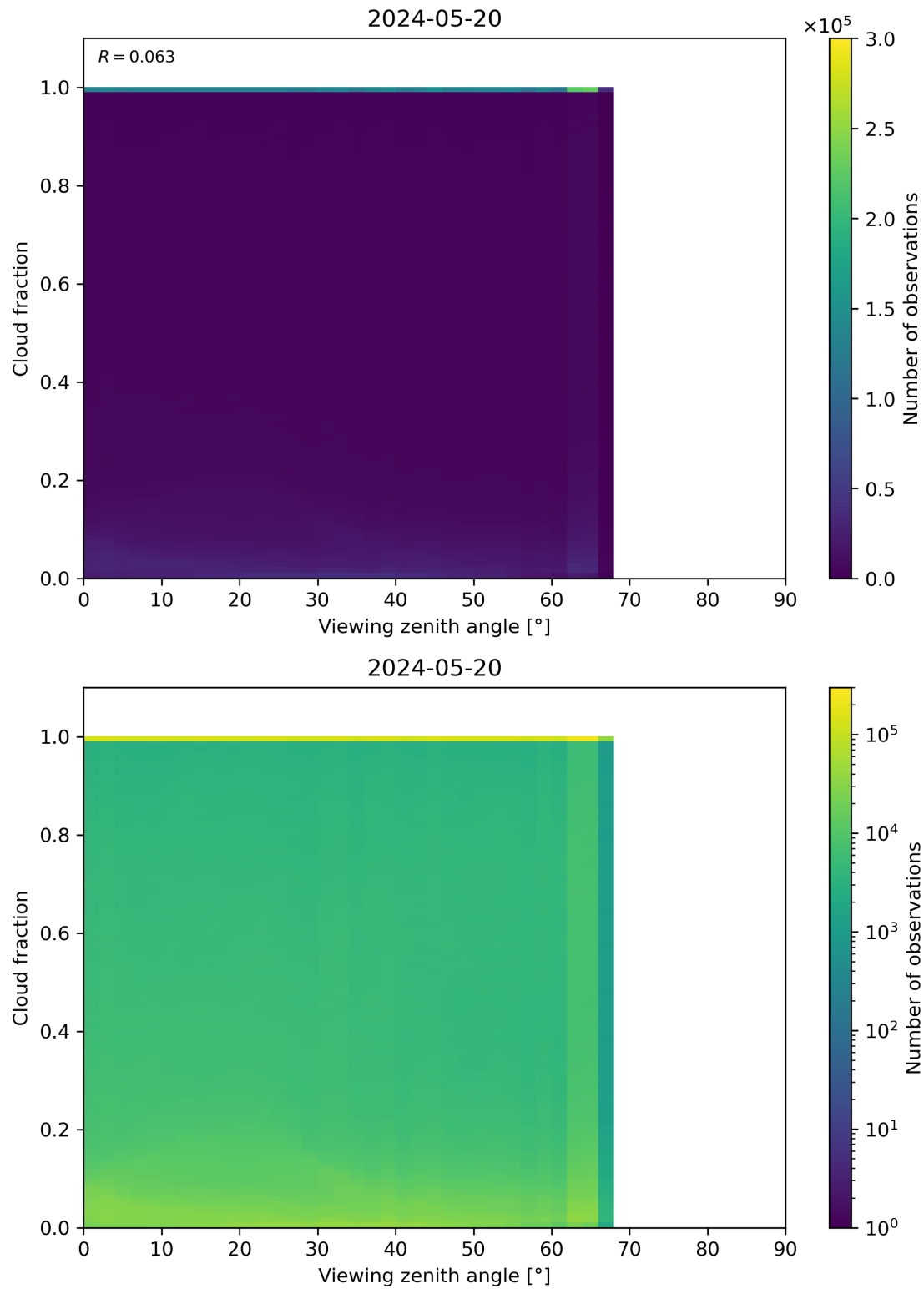
Figure 120: Scatter density plot of “Viewing zenith angle” against “Cloud fraction” for 2024-05-19 to 2024-05-21.
