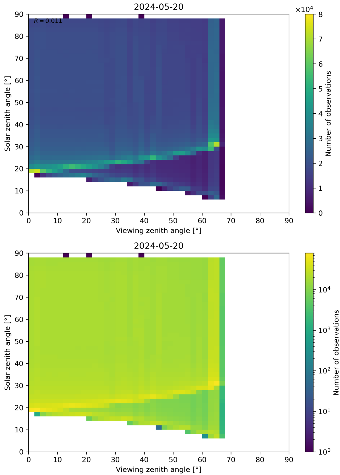
Figure 127: Scatter density plot of “Viewing zenith angle” against “Solar zenith angle” for 2024-05-19 to 2024-05-21.
