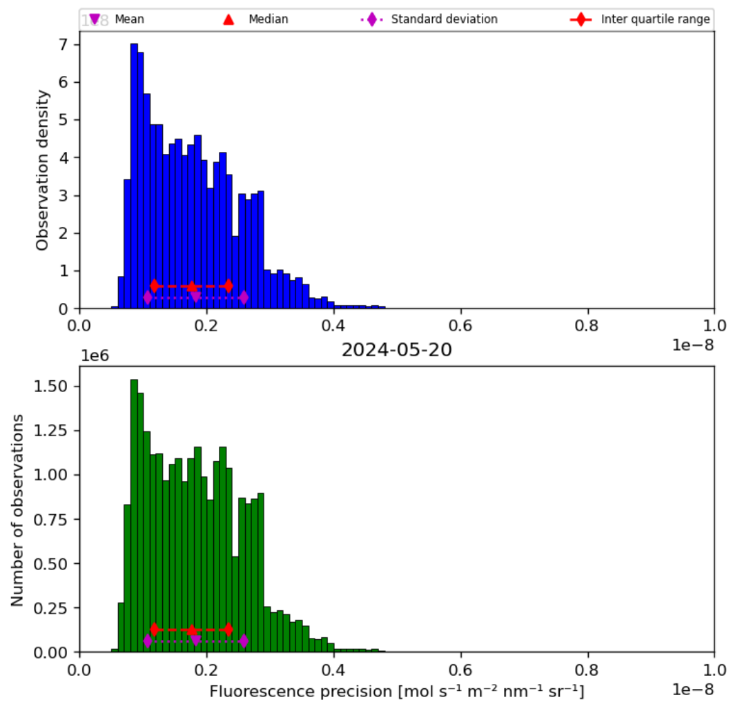
Figure 41: Histogram of “Fluorescence precision” for 2024-05-19 to 2024-05-21
