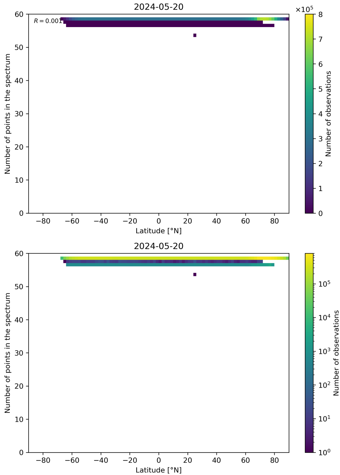
Figure 94: Scatter density plot of “Latitude” against “Number of points in the spectrum” for 2024-05-19 to 2024-05-21.
