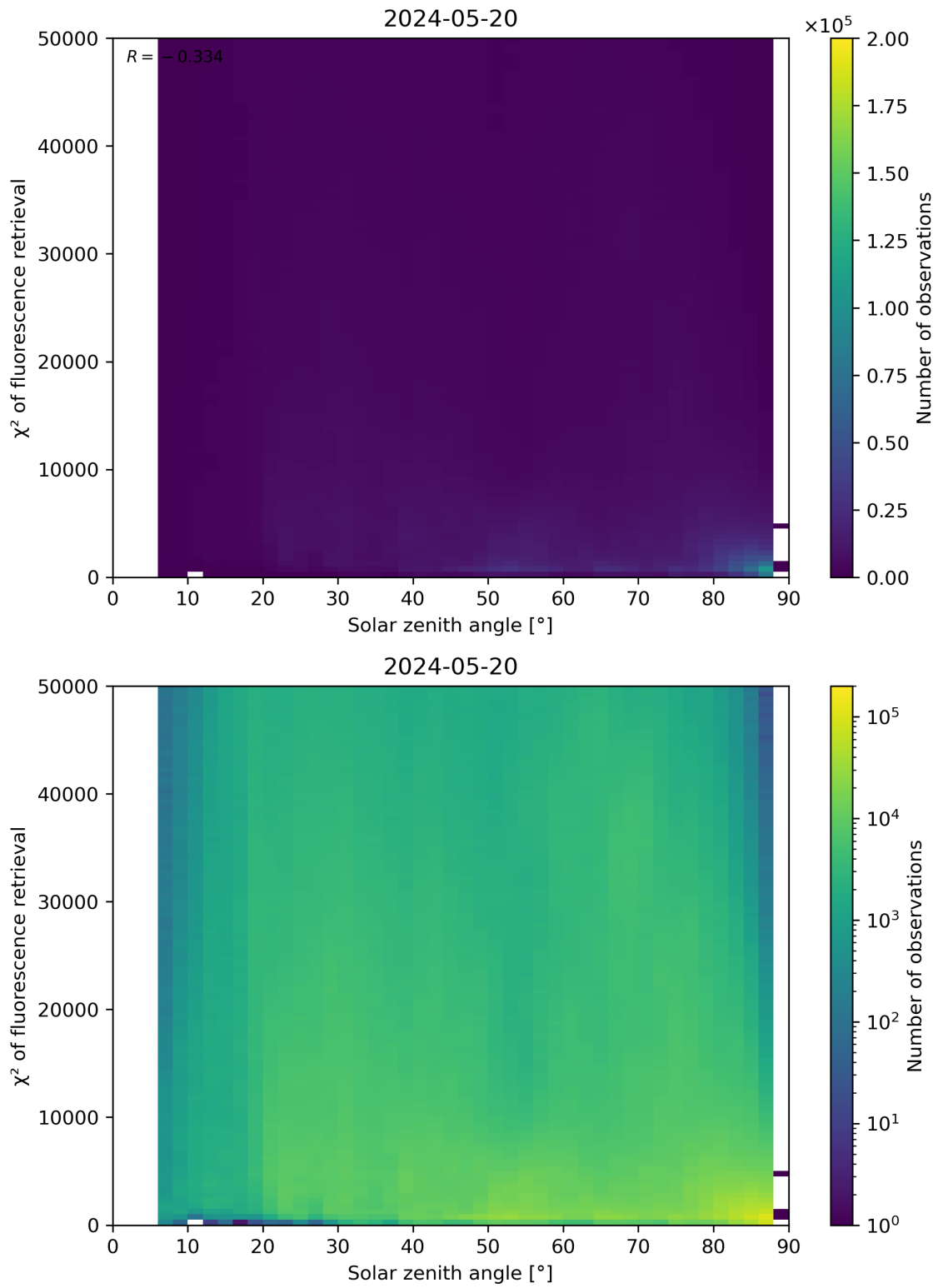
Figure 109: Scatter density plot of “Solar zenith angle” against “ \chi^2 of fluorescence retrieval” for 2024-05-19 to 2024-05-21.
