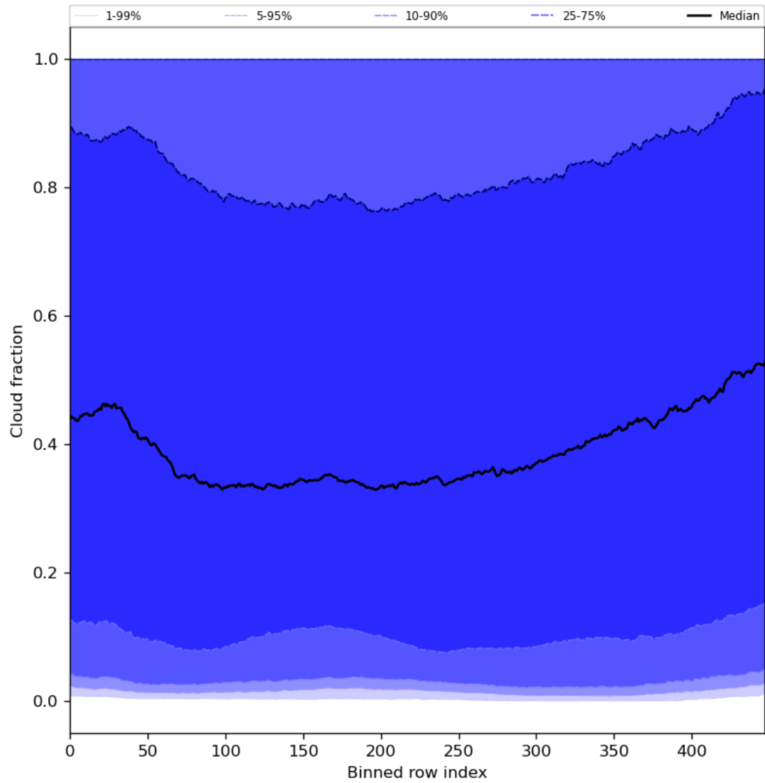
Figure 49: Along track statistics of “Cloud fraction” for 2024-05-19 to 2024-05-21
