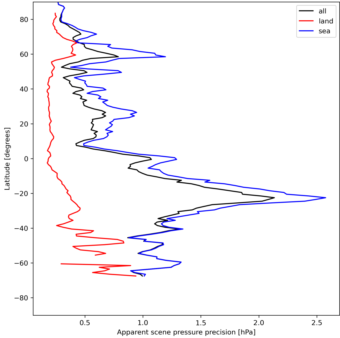
Figure 20: Zonal average of “Apparent scene pressure precision” for 2024-05-19 to 2024-05-21.
