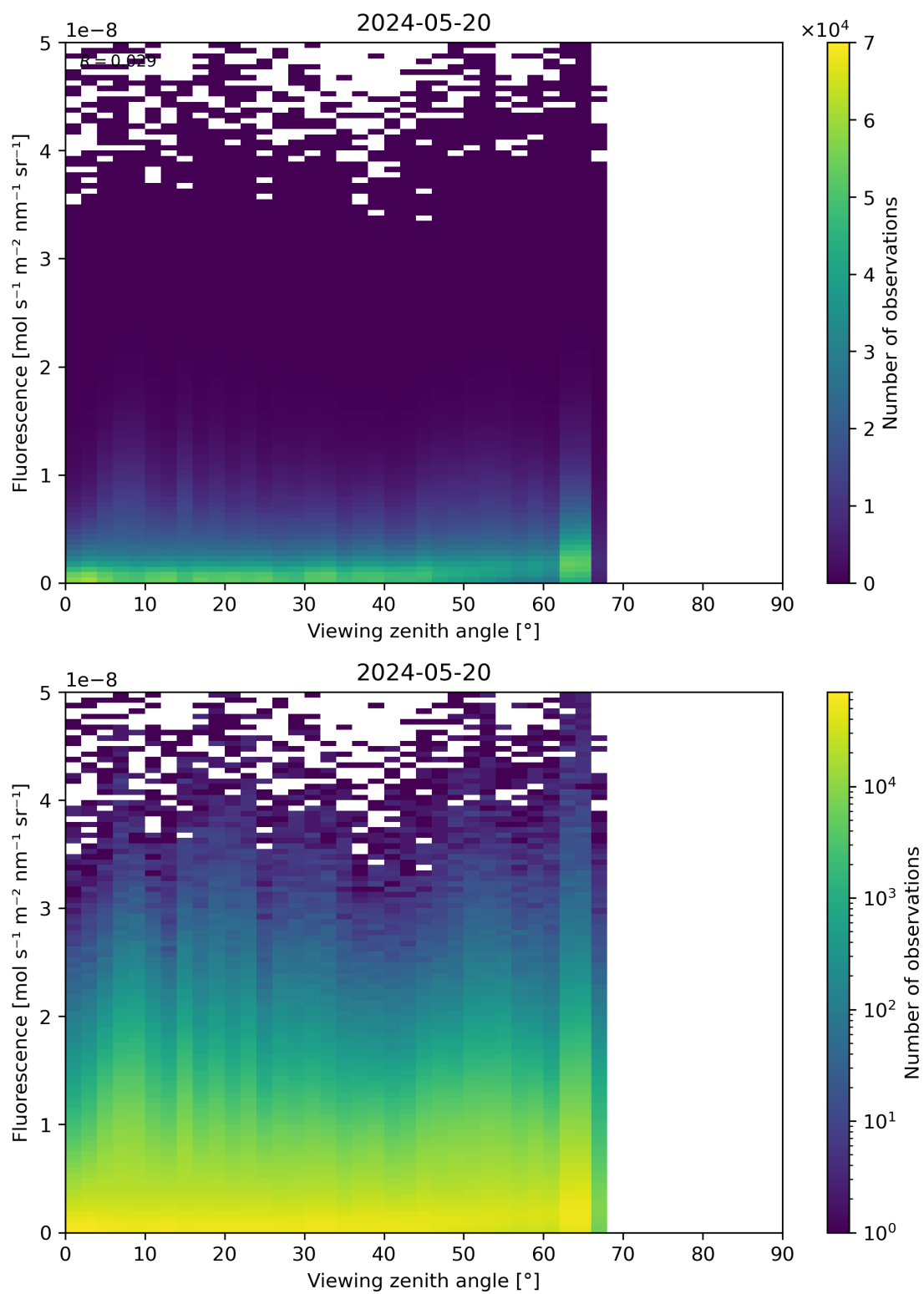
Figure 122: Scatter density plot of “Viewing zenith angle” against “Fluorescence” for 2024-05-19 to 2024-05-21.
