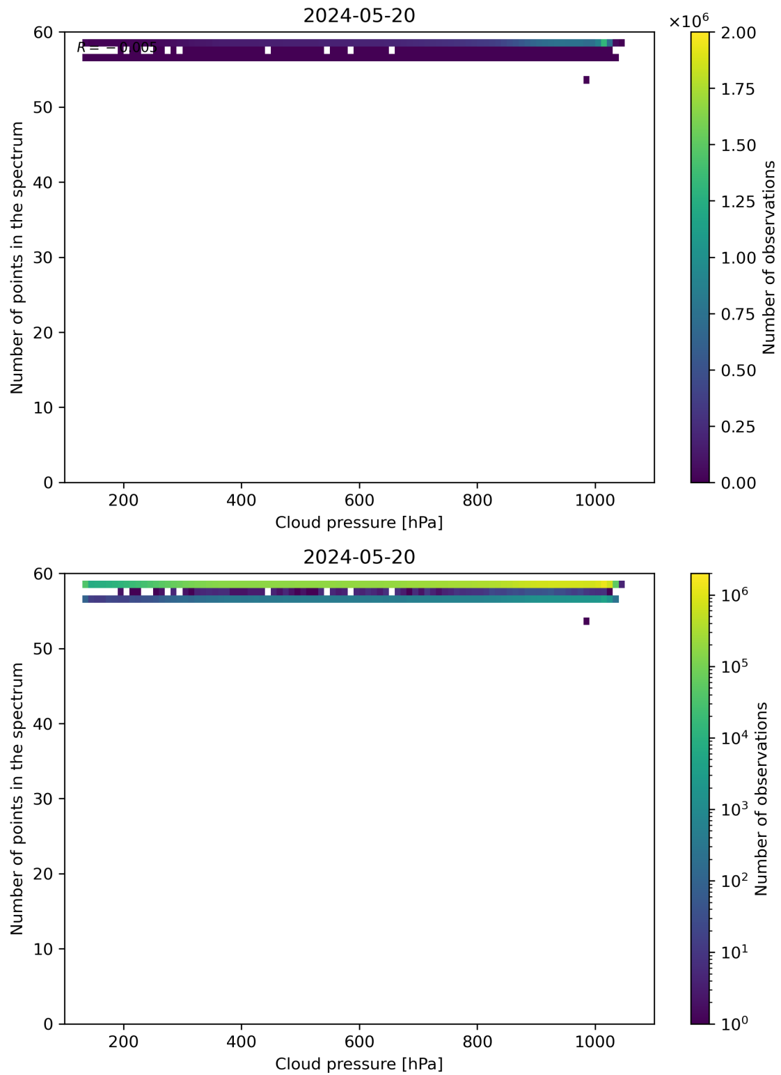
Figure 82: Scatter density plot of “Cloud pressure” against “Number of points in the spectrum” for 2024-05-19 to 2024-05-21.
