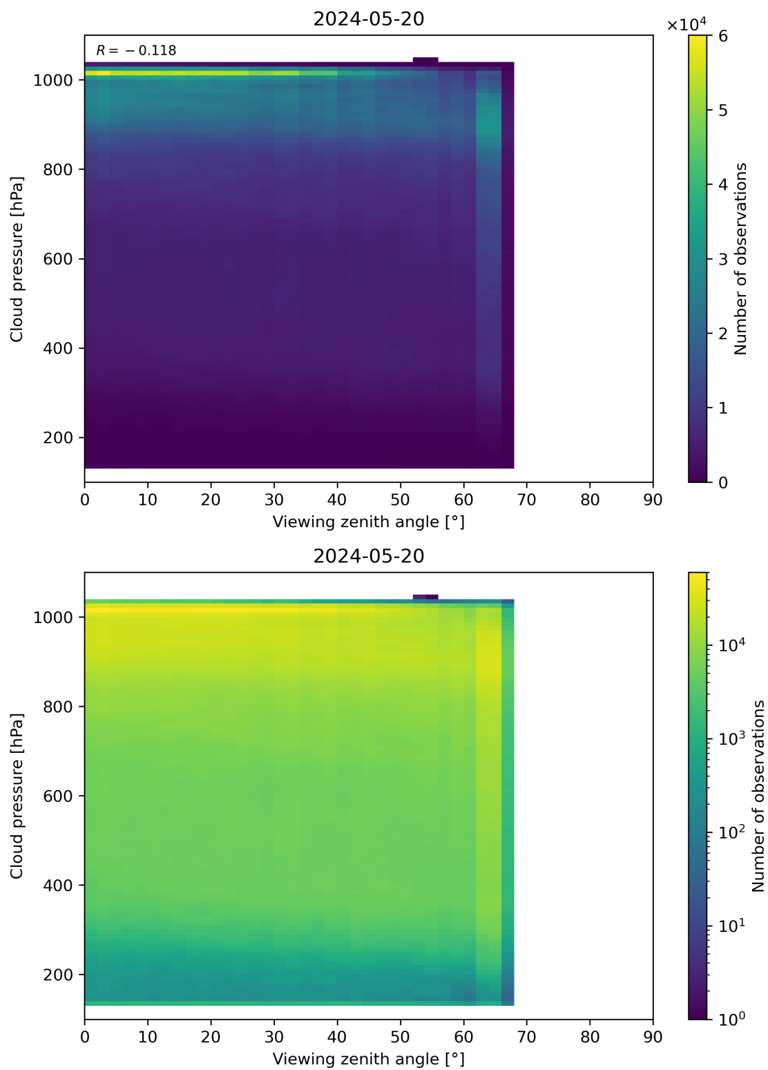
Figure 121: Scatter density plot of “Viewing zenith angle” against “Cloud pressure” for 2024-05-19 to 2024-05-21.
