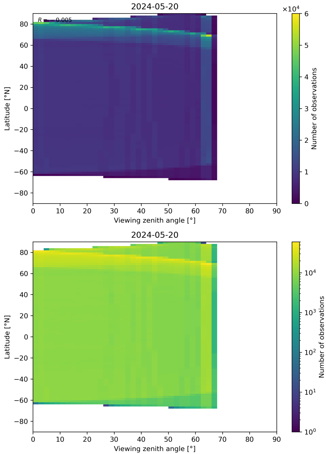
Figure 123: Scatter density plot of “Viewing zenith angle” against “Latitude” for 2024-05-19 to 2024-05-21.
