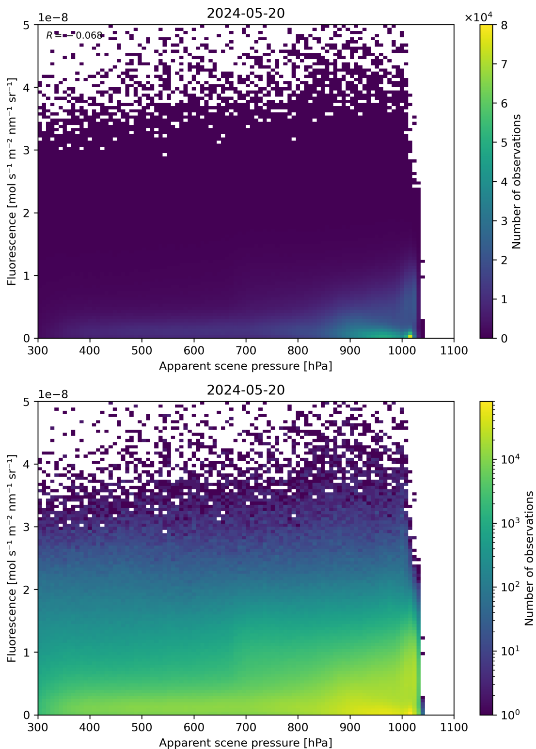
Figure 64: Scatter density plot of “Apparent scene pressure” against “Fluorescence” for 2024-05-19 to 2024-05-21.
