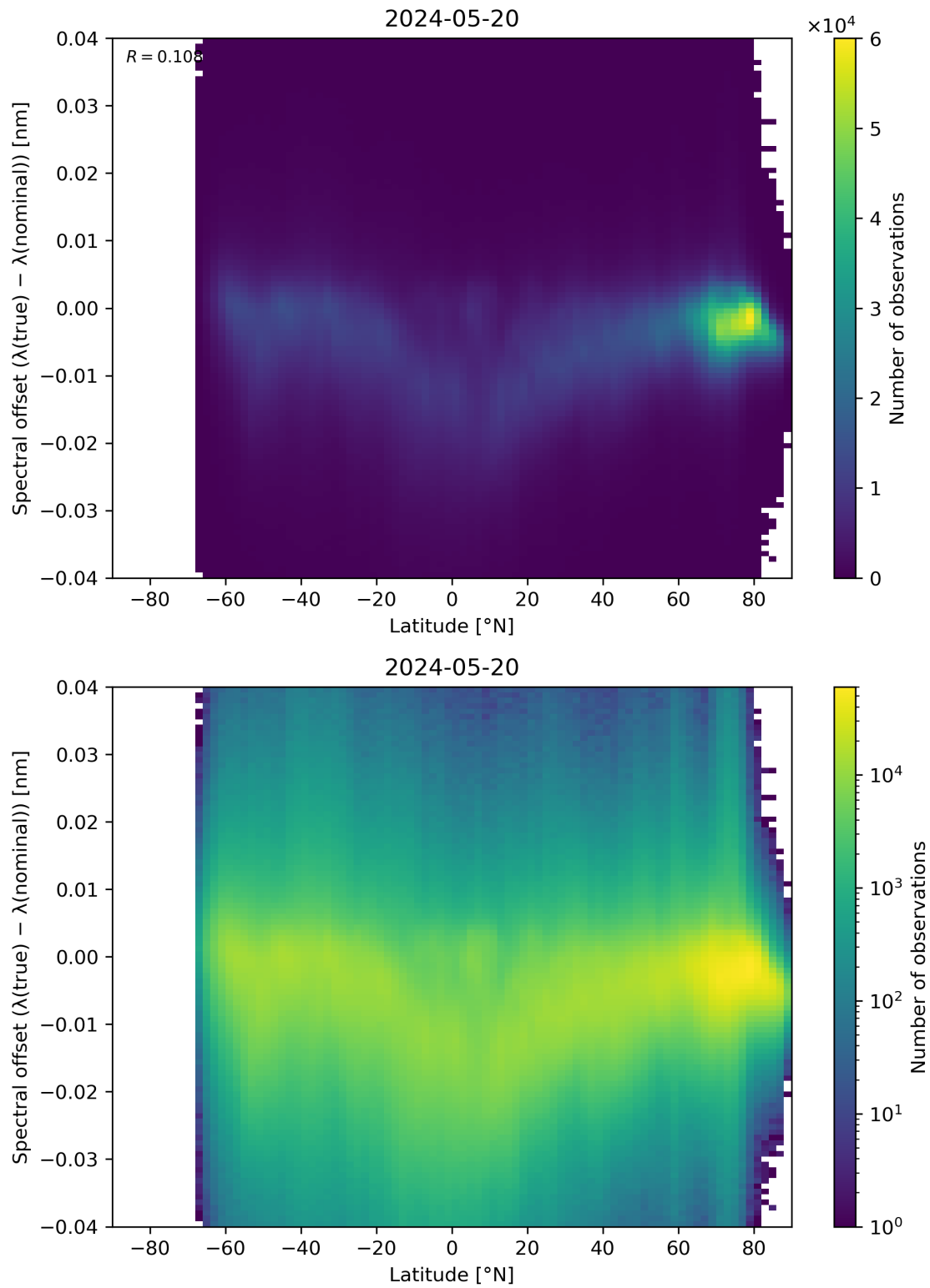
Figure 96: Scatter density plot of “Latitude” against “Spectral offset ( \lambda(\text{true}) - \lambda(\text{nominal}) )” for 2024-05-19 to 2024-05-21.
