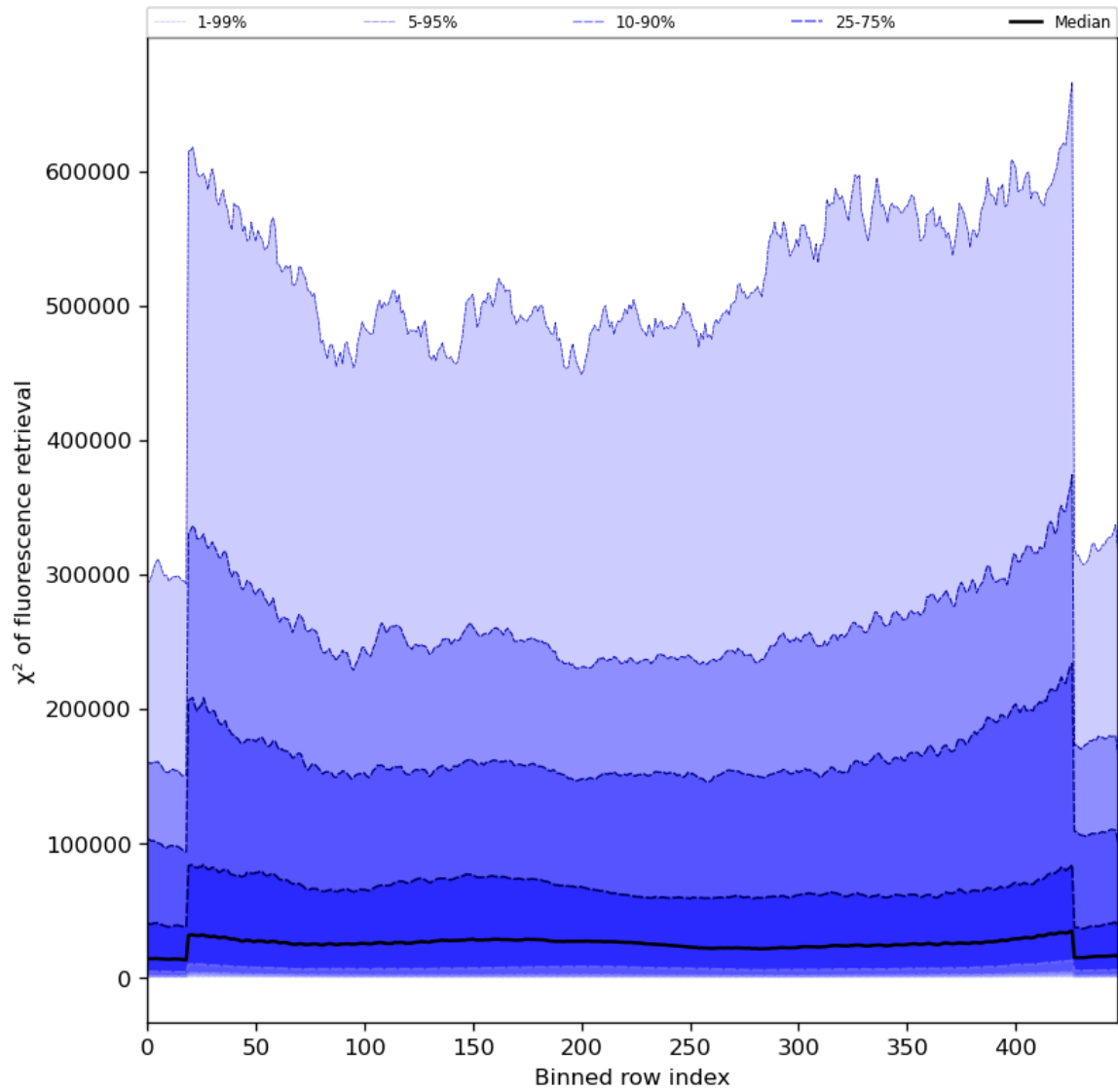
Figure 59: Along track statistics of “ \chi^2 of fluorescence retrieval” for 2024-05-19 to 2024-05-21
