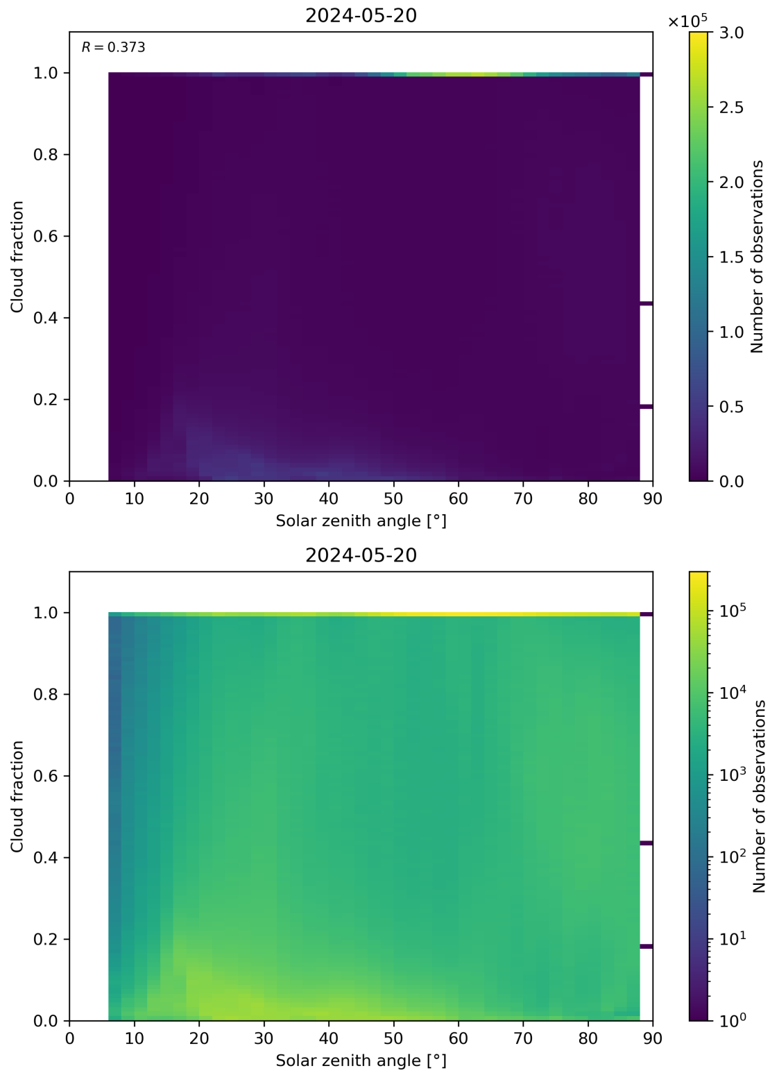
Figure 110: Scatter density plot of “Solar zenith angle” against “Cloud fraction” for 2024-05-19 to 2024-05-21.
