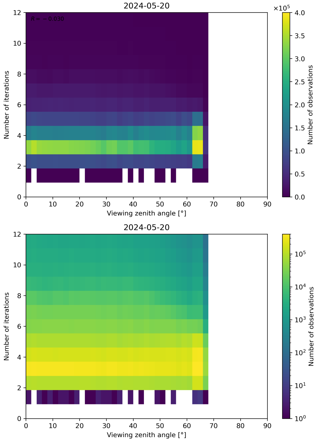
Figure 124: Scatter density plot of “Viewing zenith angle” against “Number of iterations” for 2024-05-19 to 2024-05-21.
