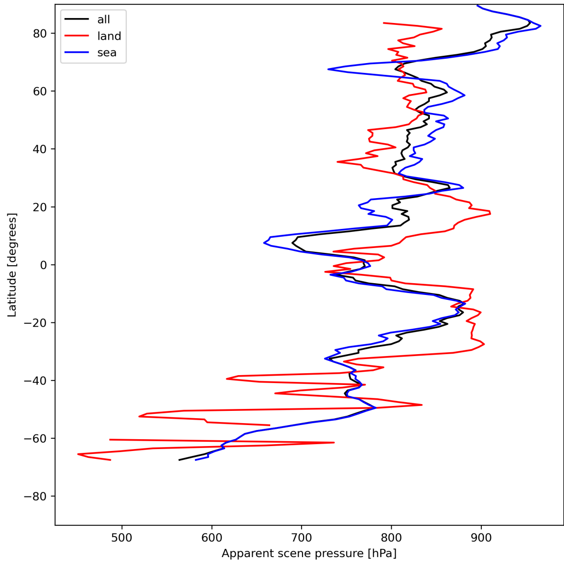
Figure 19: Zonal average of “Apparent scene pressure” for 2024-05-19 to 2024-05-21.
