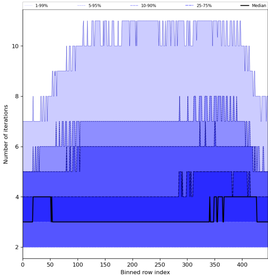
Figure 56: Along track statistics of “Number of iterations” for 2024-05-19 to 2024-05-21
