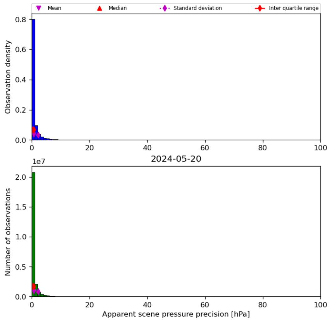
Figure 37: Histogram of “Apparent scene pressure precision” for 2024-05-19 to 2024-05-21
