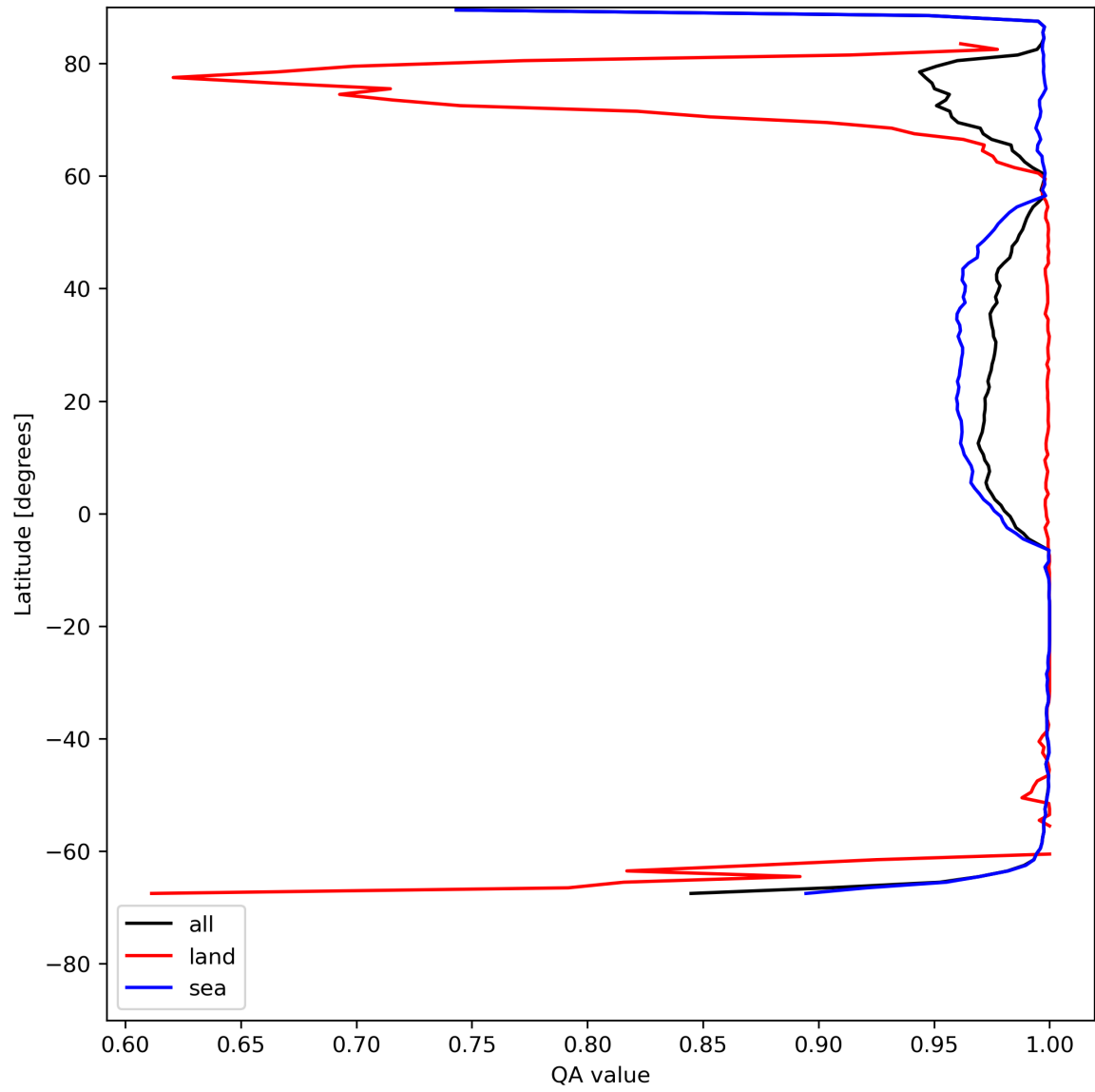
Figure 12: Zonal average of “QA value” for 2024-05-19 to 2024-05-21.
