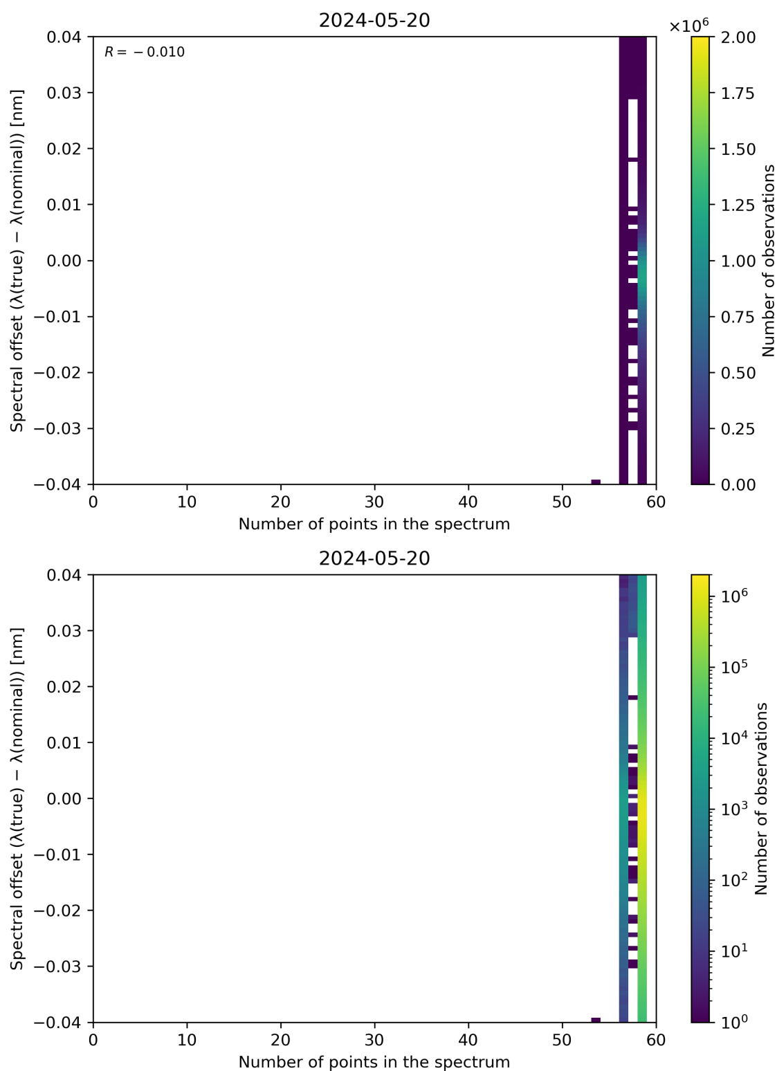
Figure 101: Scatter density plot of “Number of points in the spectrum” against “Spectral offset ( \lambda(\text{true}) - \lambda(\text{nominal}) )” for 2024-05-19 to 2024-05-21.
