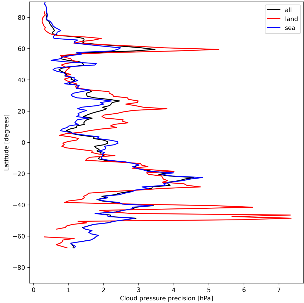
Figure 14: Zonal average of “Cloud pressure precision” for 2024-05-19 to 2024-05-21.
