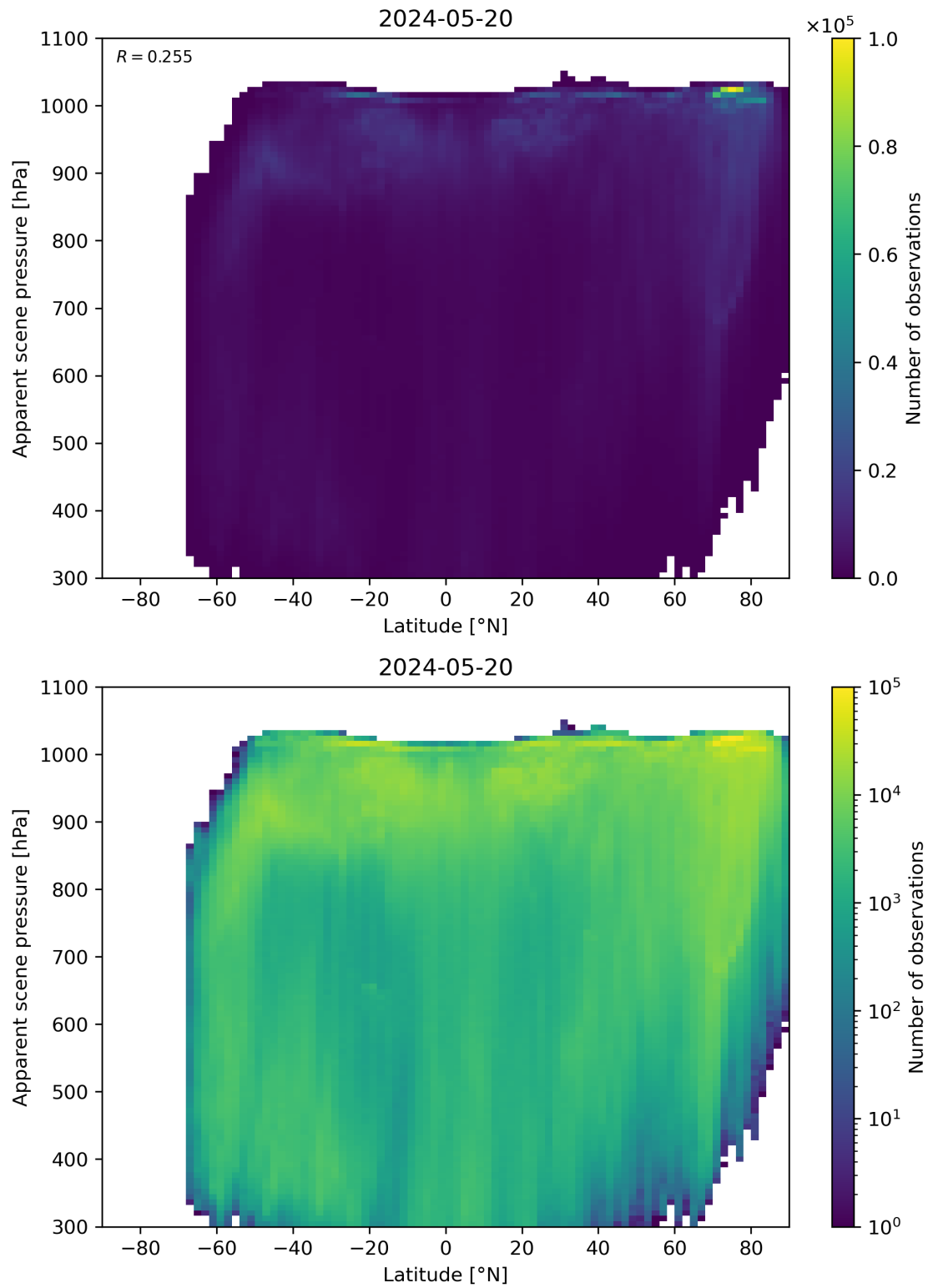
Figure 88: Scatter density plot of “Latitude” against “Apparent scene pressure” for 2024-05-19 to 2024-05-21.
