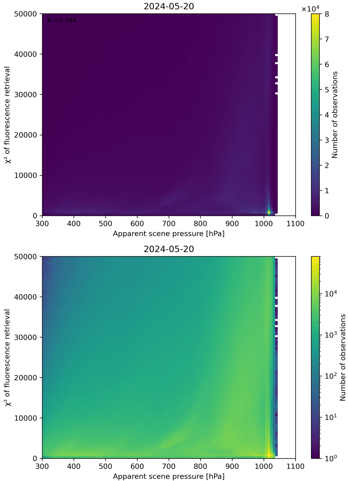
Figure 63: Scatter density plot of “Apparent scene pressure” against “ \chi^2 of fluorescence retrieval” for 2024-05-19 to 2024-05-21.
