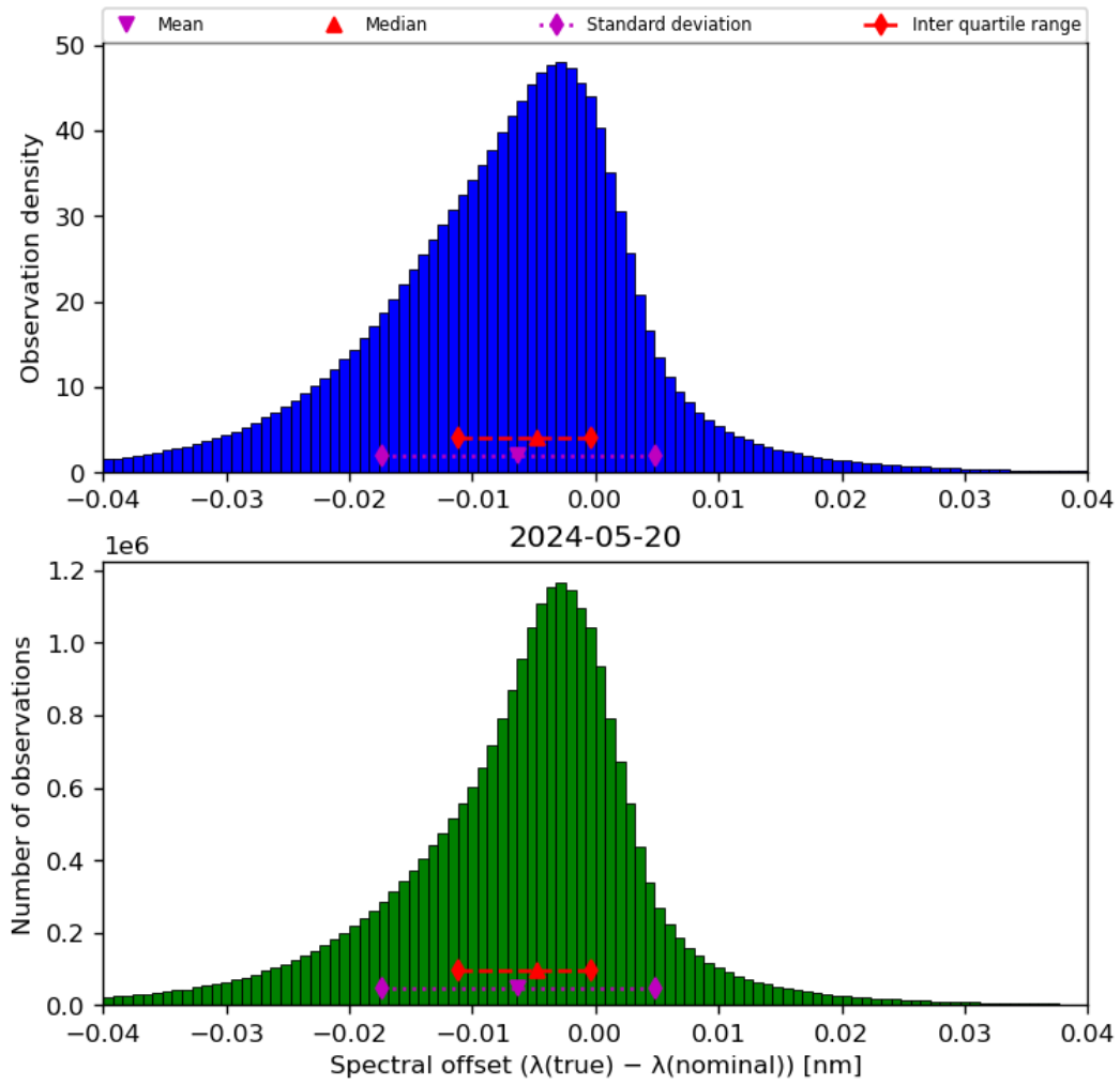
Figure 45: Histogram of “Spectral offset ( \lambda(\text{true}) - \lambda(\text{nominal}) )” for 2024-05-19 to 2024-05-21
