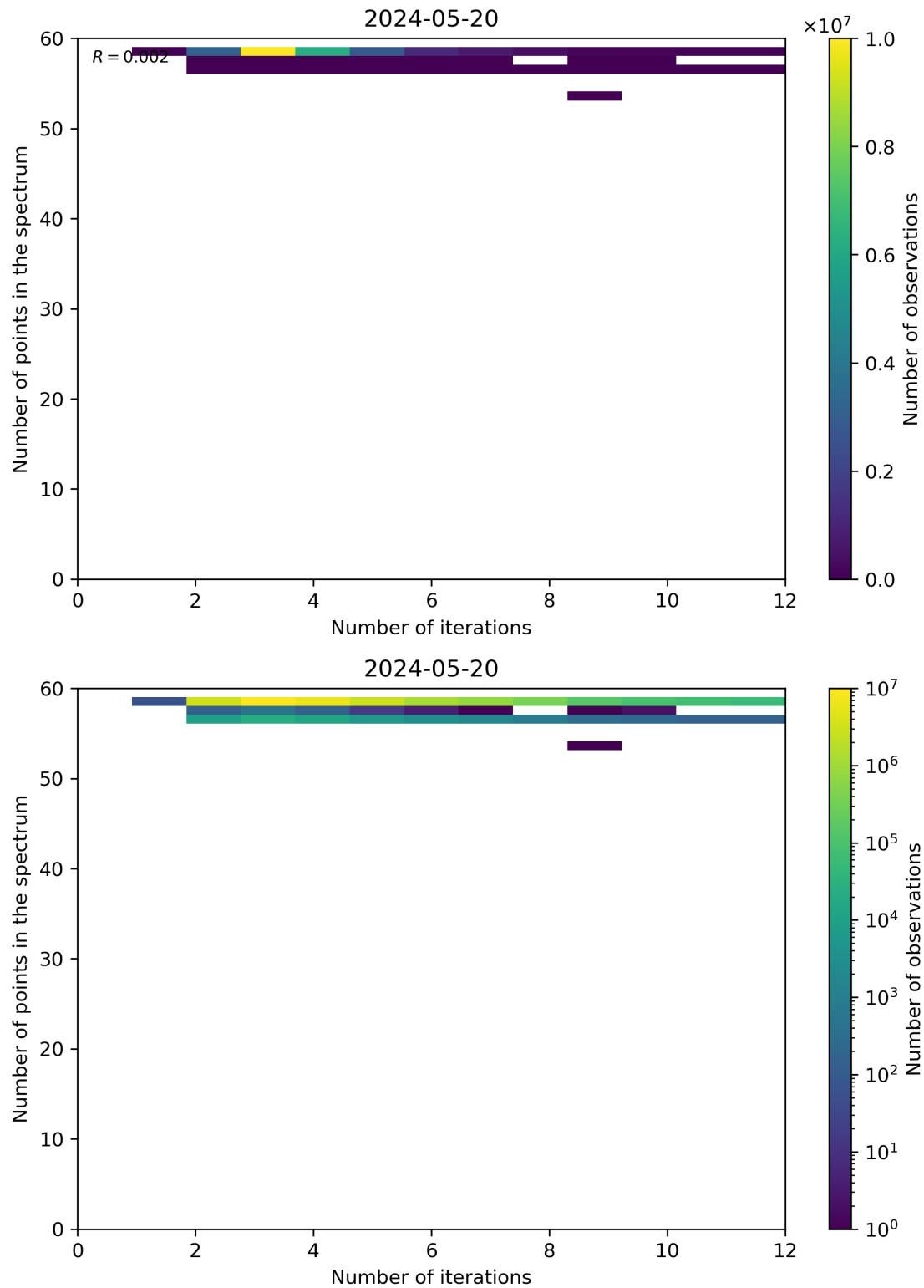
Figure 99: Scatter density plot of “Number of iterations” against “Number of points in the spectrum” for 2024-05-19 to 2024-05-21.
