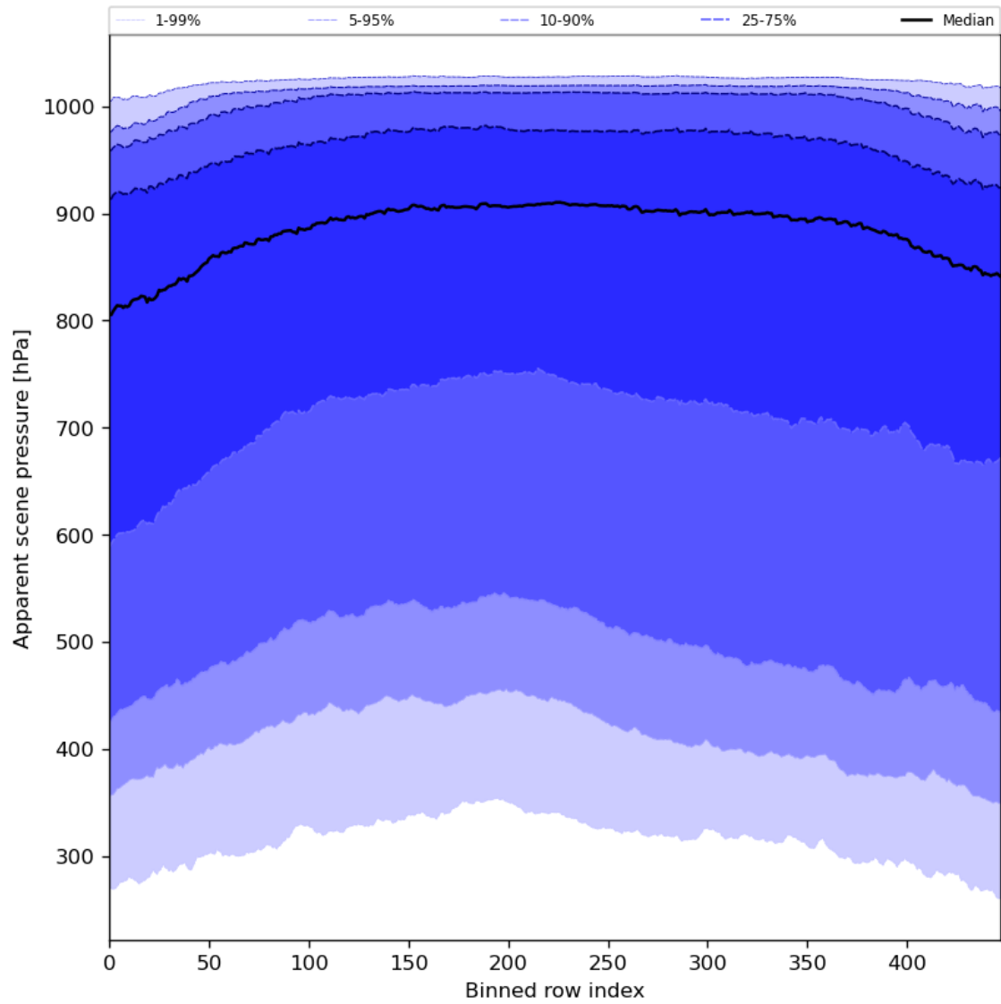
Figure 53: Along track statistics of “Apparent scene pressure” for 2024-05-19 to 2024-05-21
