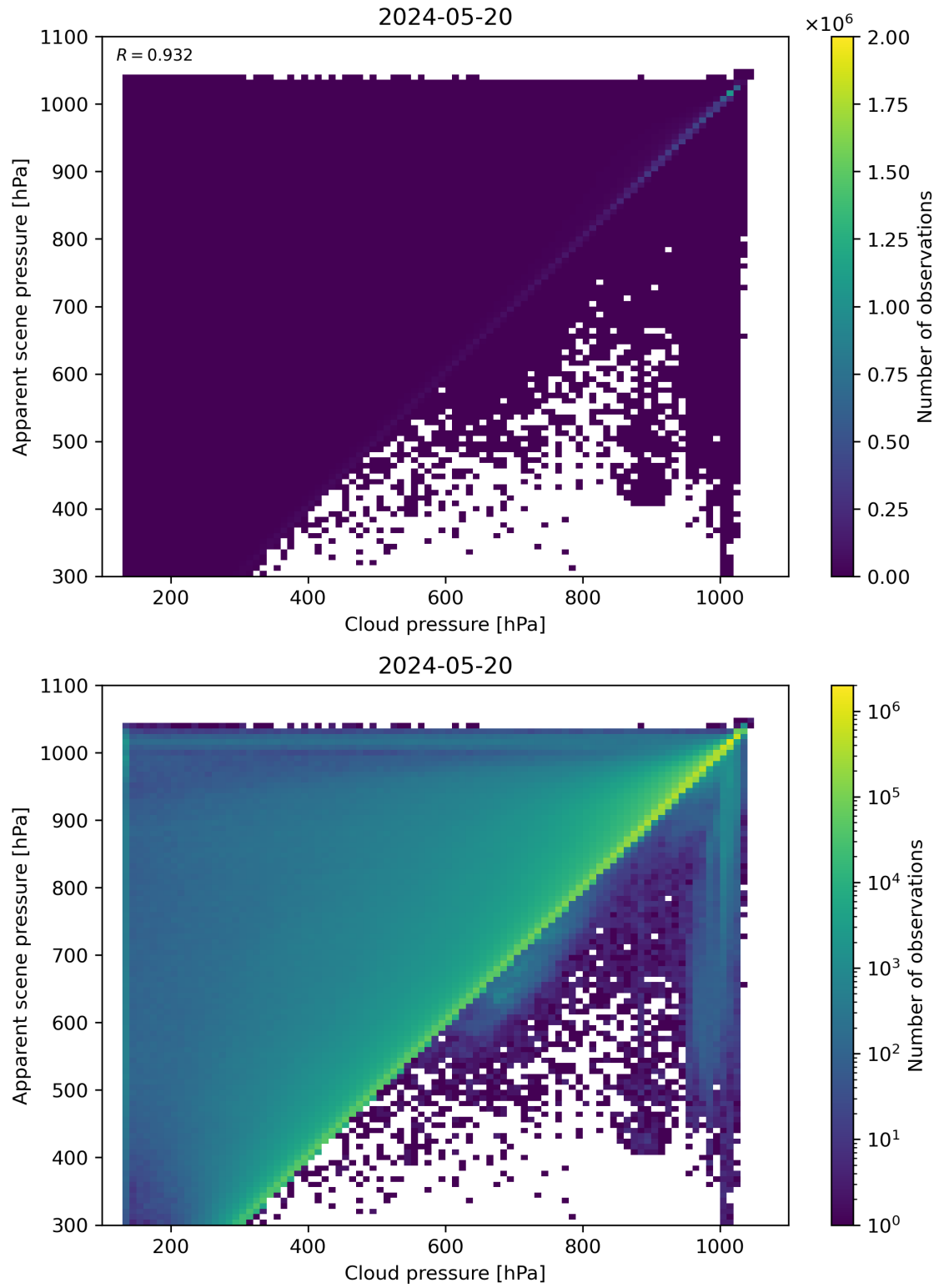
Figure 77: Scatter density plot of “Cloud pressure” against “Apparent scene pressure” for 2024-05-19 to 2024-05-21.
