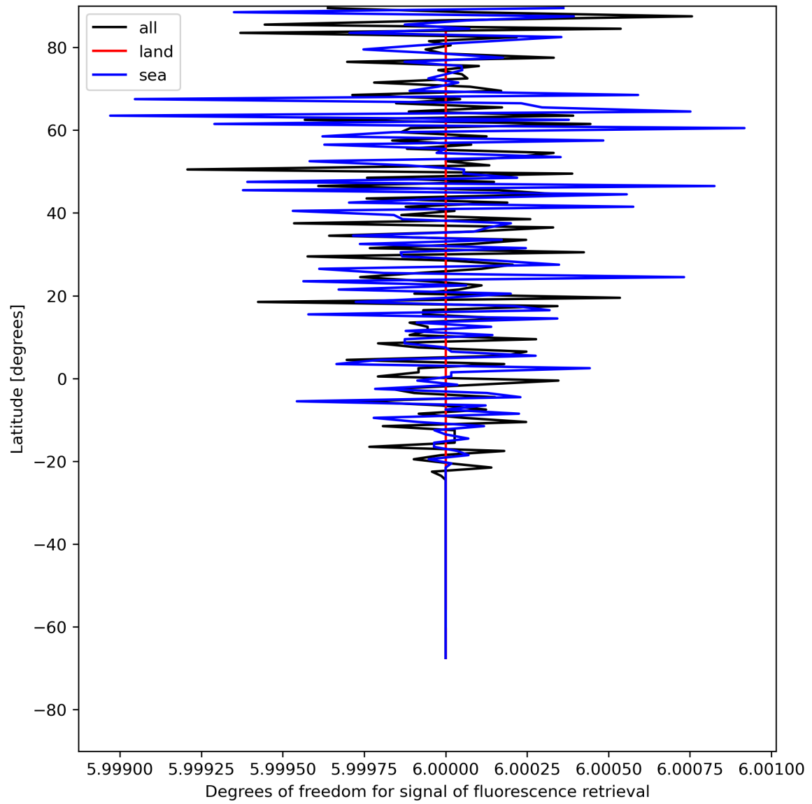
Figure 26: Zonal average of “Degrees of freedom for signal of fluorescence retrieval” for 2024-05-19 to 2024-05-21.
