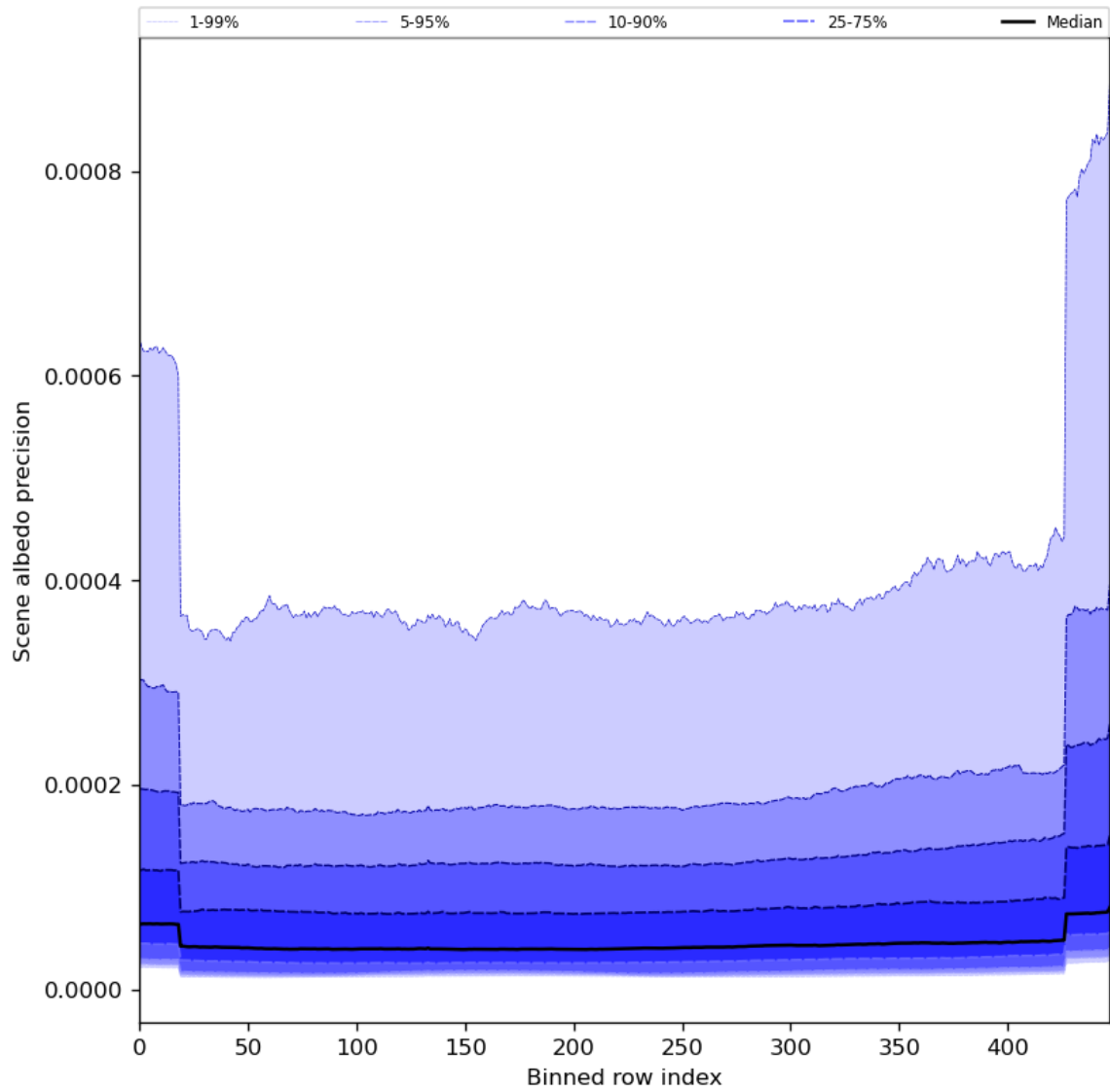
Figure 52: Along track statistics of “Scene albedo precision” for 2024-05-19 to 2024-05-21
