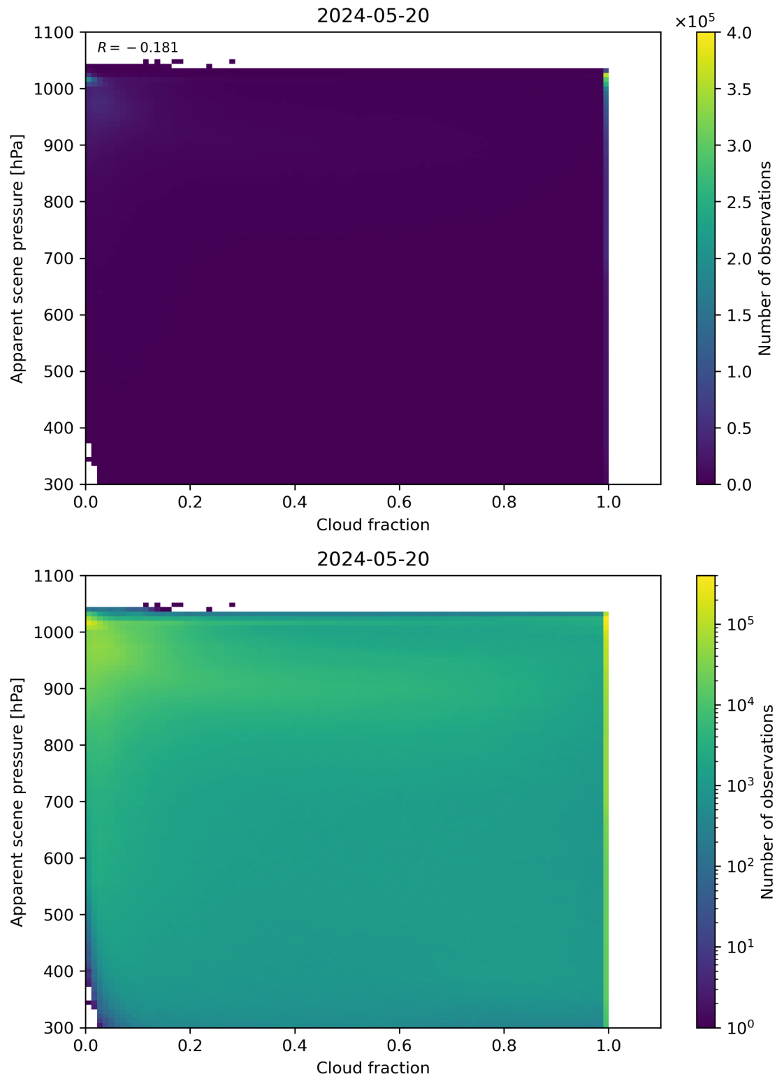
Figure 70: Scatter density plot of “Cloud fraction” against “Apparent scene pressure” for 2024-05-19 to 2024-05-21.
