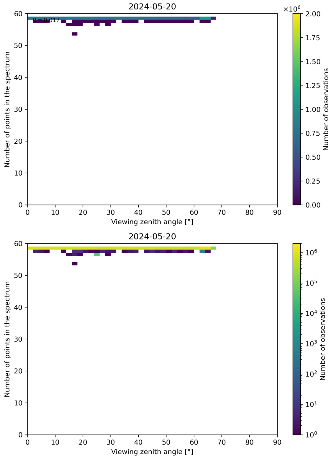
Figure 125: Scatter density plot of “Viewing zenith angle” against “Number of points in the spectrum” for 2024-05-19 to 2024-05-21.
