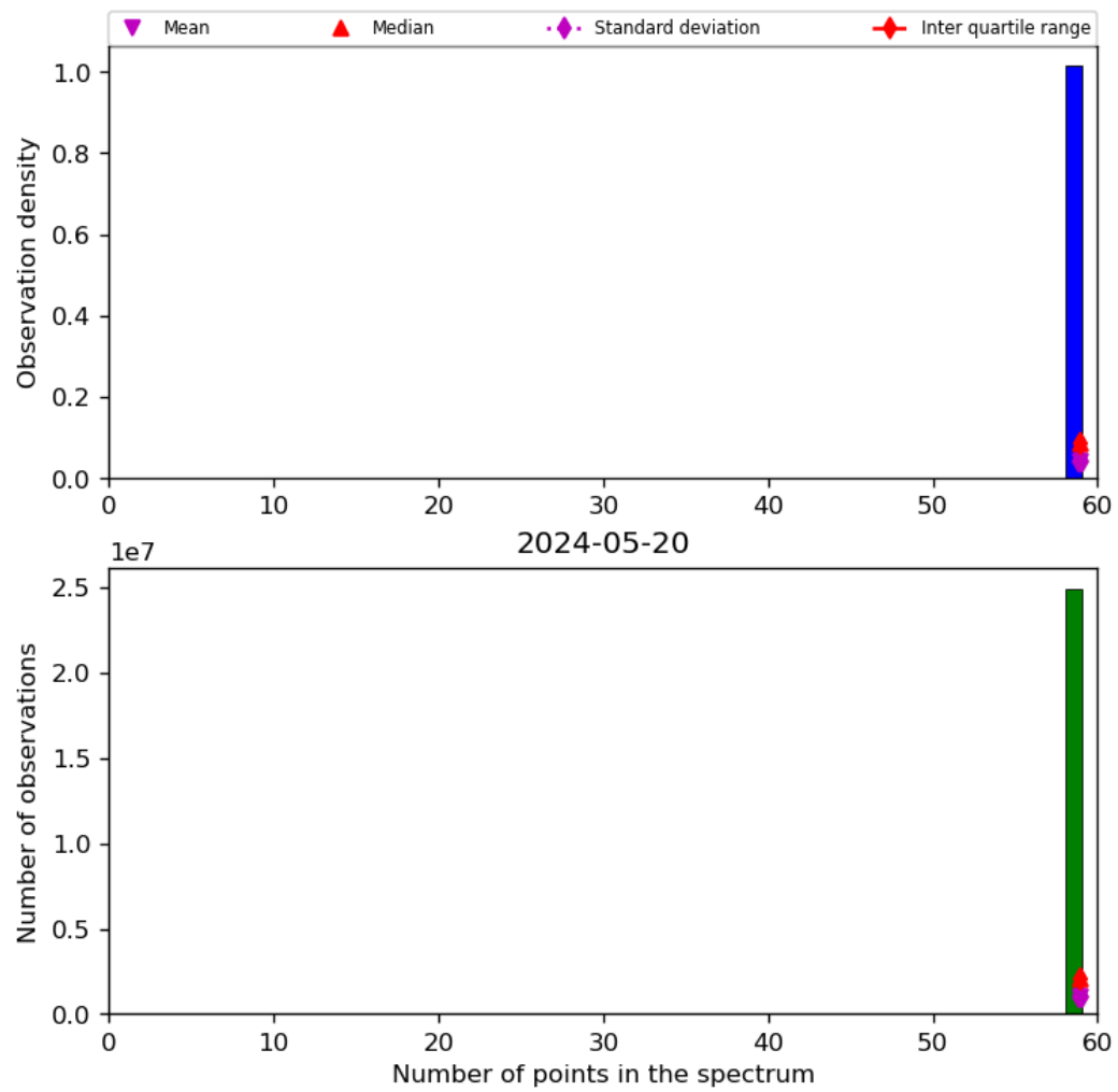
Figure 44: Histogram of "Number of points in the spectrum" for 2024-05-19 to 2024-05-21
