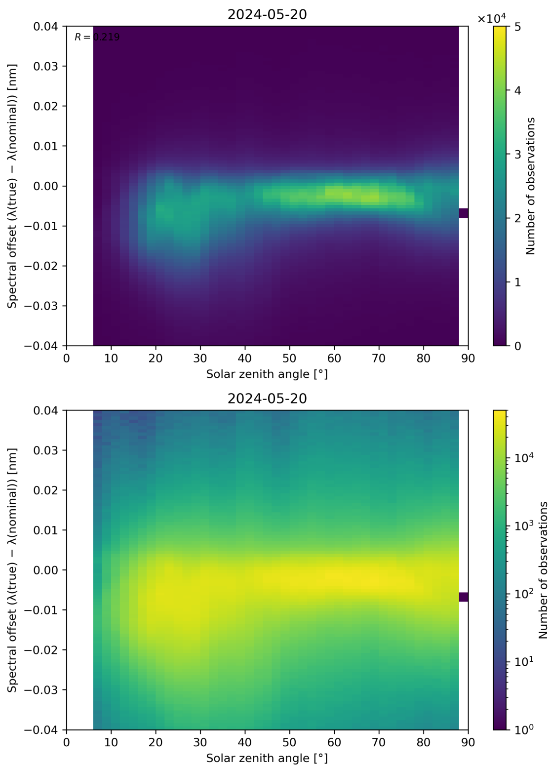
Figure 117: Scatter density plot of “Solar zenith angle” against “Spectral offset ( \lambda(\text{true}) - \lambda(\text{nominal}) )” for 2024-05-19 to 2024-05-21.
