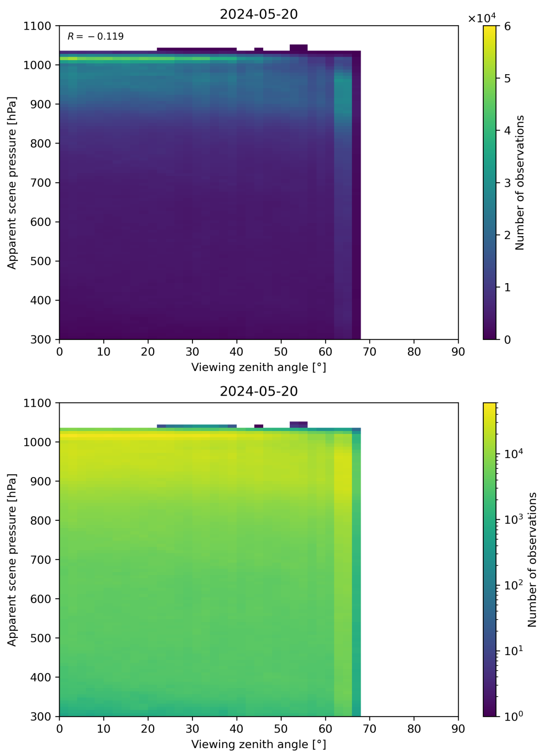
Figure 118: Scatter density plot of “Viewing zenith angle” against “Apparent scene pressure” for 2024-05-19 to 2024-05-21.
