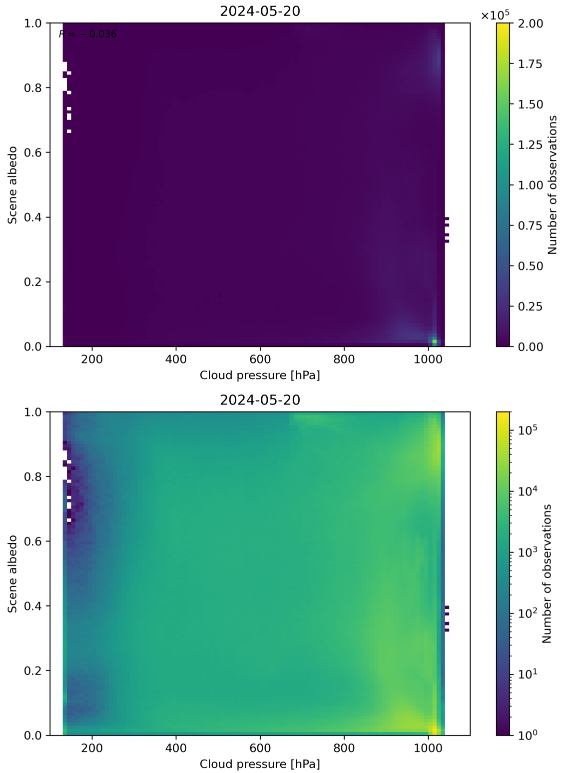
Figure 83: Scatter density plot of “Cloud pressure” against “Scene albedo” for 2024-05-19 to 2024-05-21.
