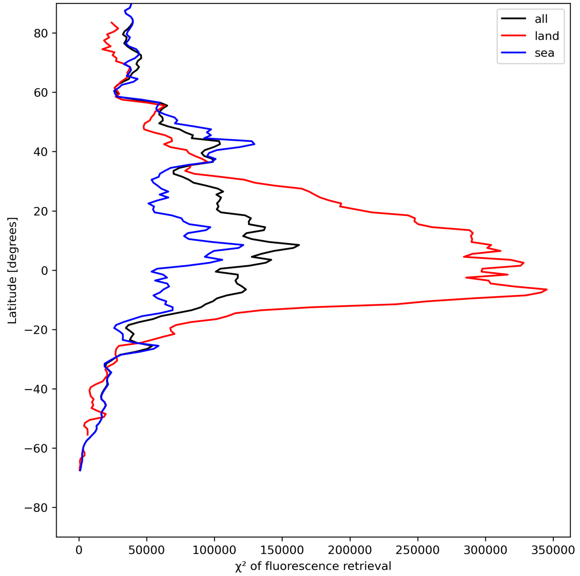
Figure 25: Zonal average of “ \chi^2 of fluorescence retrieval” for 2024-05-19 to 2024-05-21.
