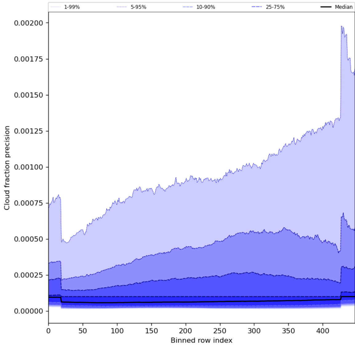
Figure 50: Along track statistics of “Cloud fraction precision” for 2024-05-19 to 2024-05-21
