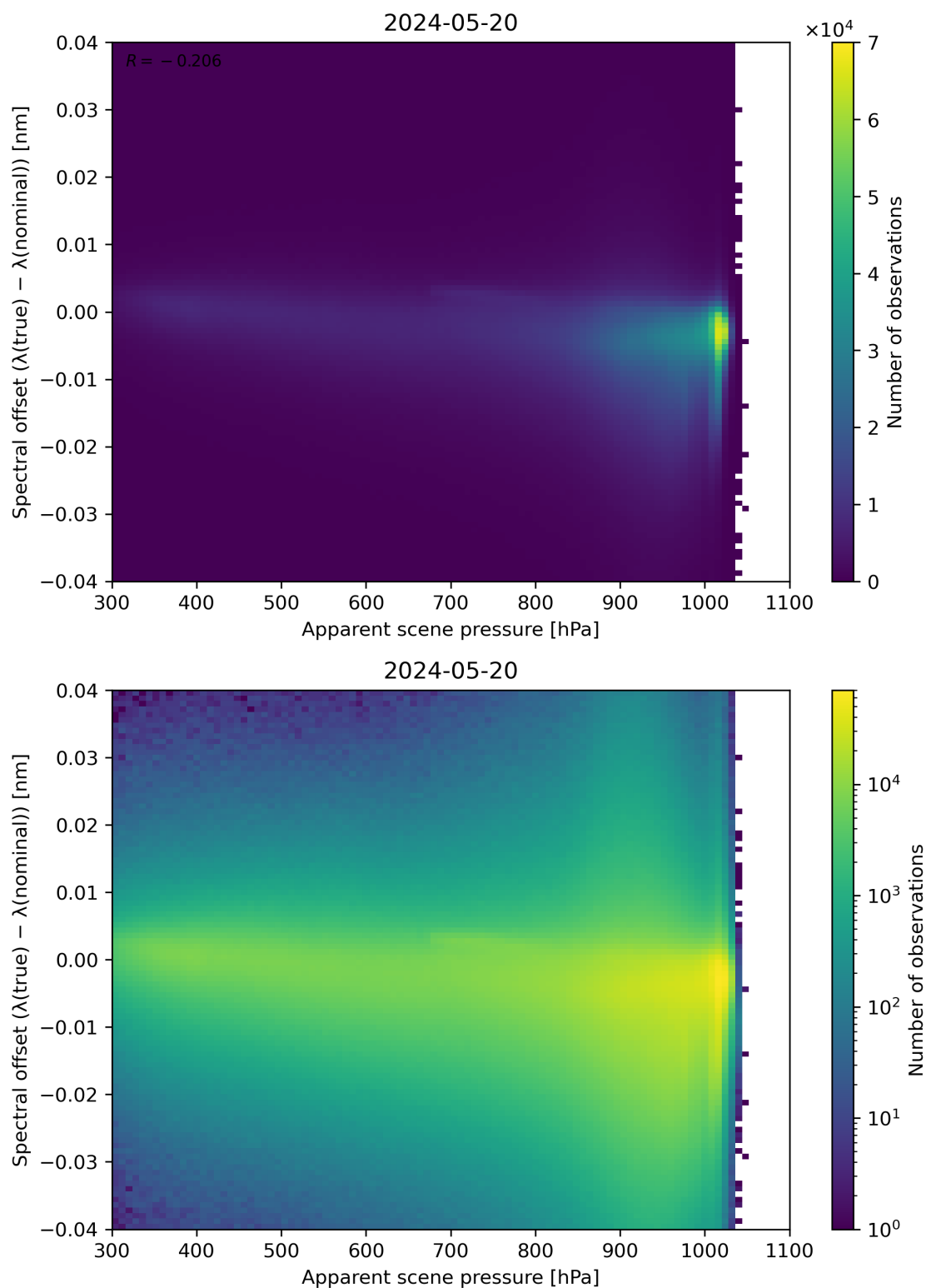
Figure 67: Scatter density plot of “Apparent scene pressure” against “Spectral offset ( \lambda(\text{true}) - \lambda(\text{nominal}) )” for 2024-05-19 to 2024-05-21.
