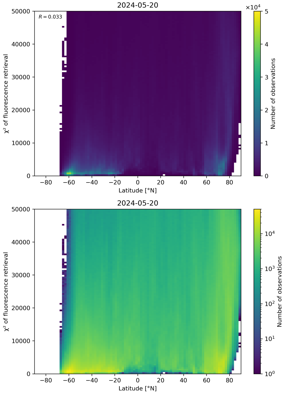
Figure 89: Scatter density plot of “Latitude” against “ \chi^2 of fluorescence retrieval” for 2024-05-19 to 2024-05-21.
