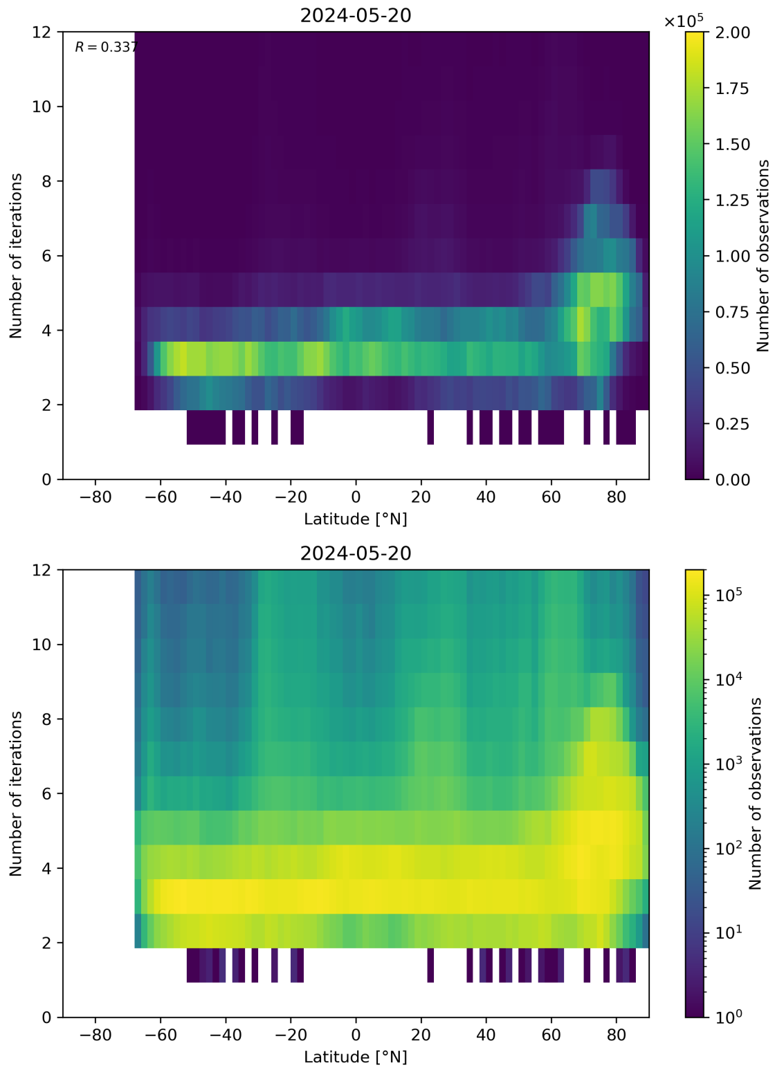
Figure 93: Scatter density plot of “Latitude” against “Number of iterations” for 2024-05-19 to 2024-05-21.
