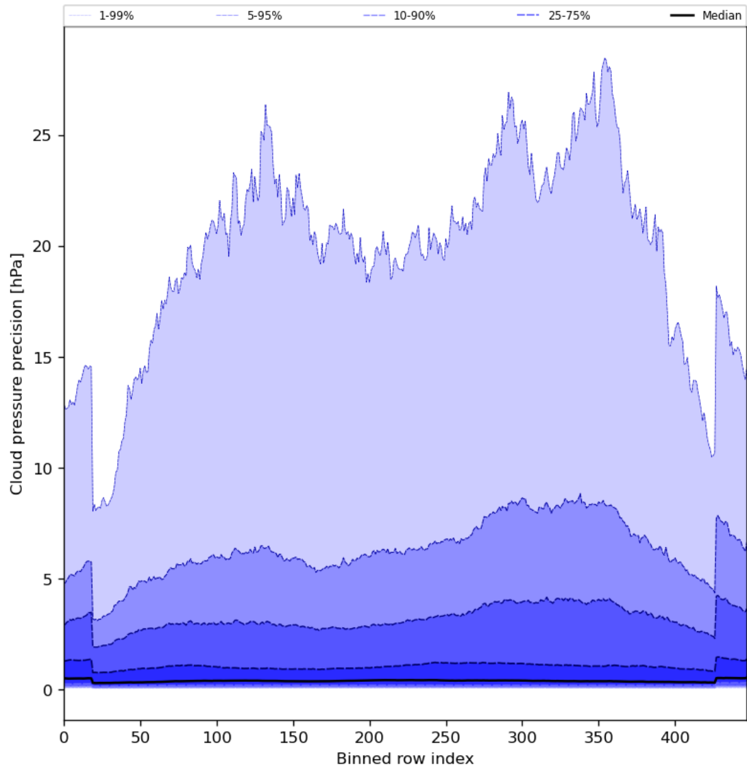
Figure 48: Along track statistics of “Cloud pressure precision” for 2024-05-19 to 2024-05-21
