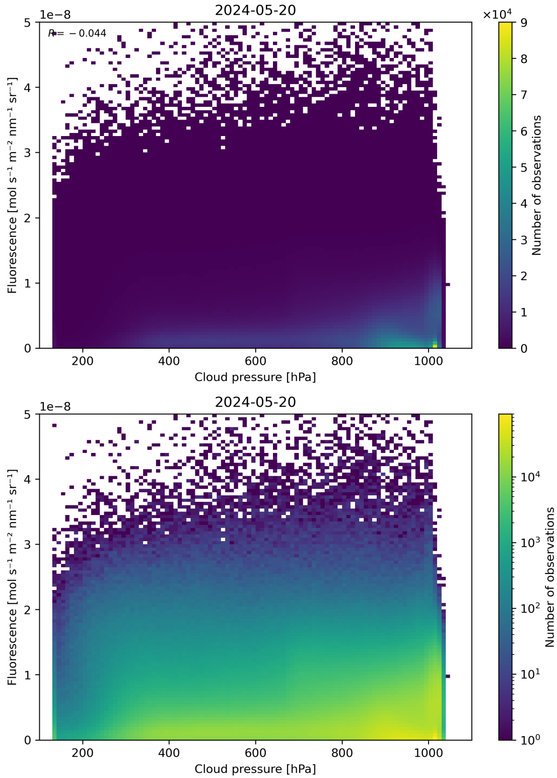
Figure 80: Scatter density plot of “Cloud pressure” against “Fluorescence” for 2024-05-19 to 2024-05-21.
