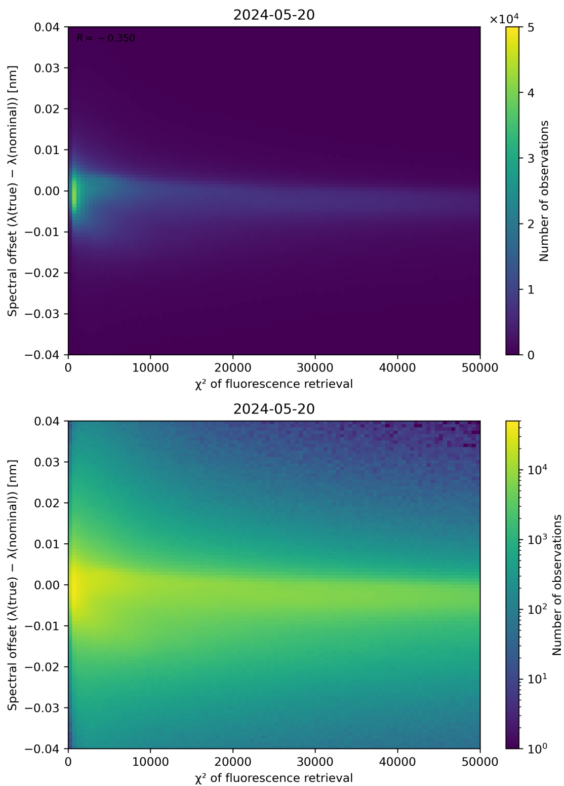
Figure 69: Scatter density plot of " \chi^2 of fluorescence retrieval" against "Spectral offset ( \lambda(\text{true}) - \lambda(\text{nominal}) )" for 2024-05-19 to 2024-05-21.
