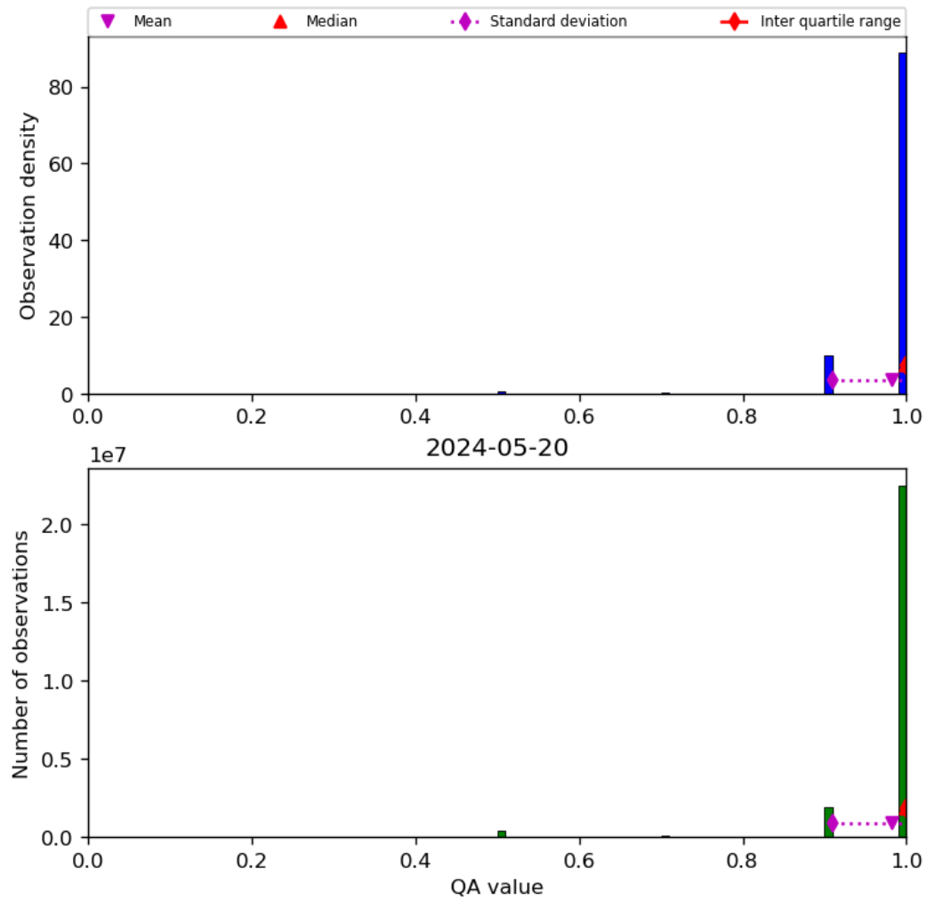
Figure 29: Histogram of “QA value” for 2024-05-19 to 2024-05-21
