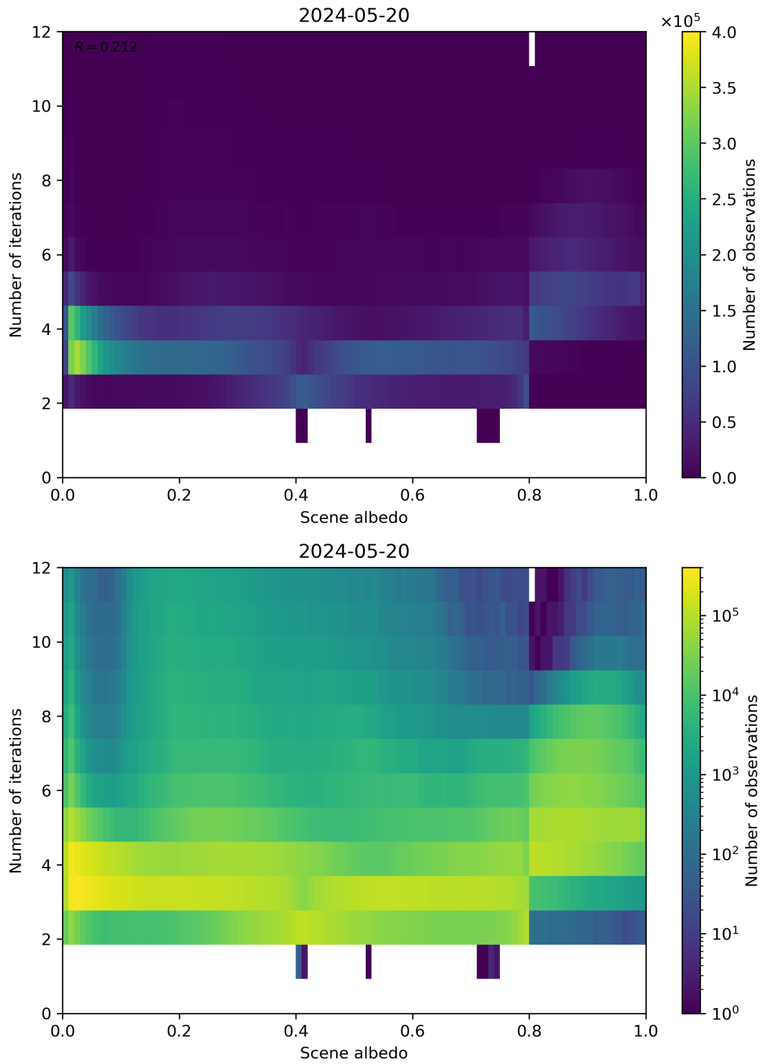
Figure 105: Scatter density plot of “Scene albedo” against “Number of iterations” for 2024-05-19 to 2024-05-21.
