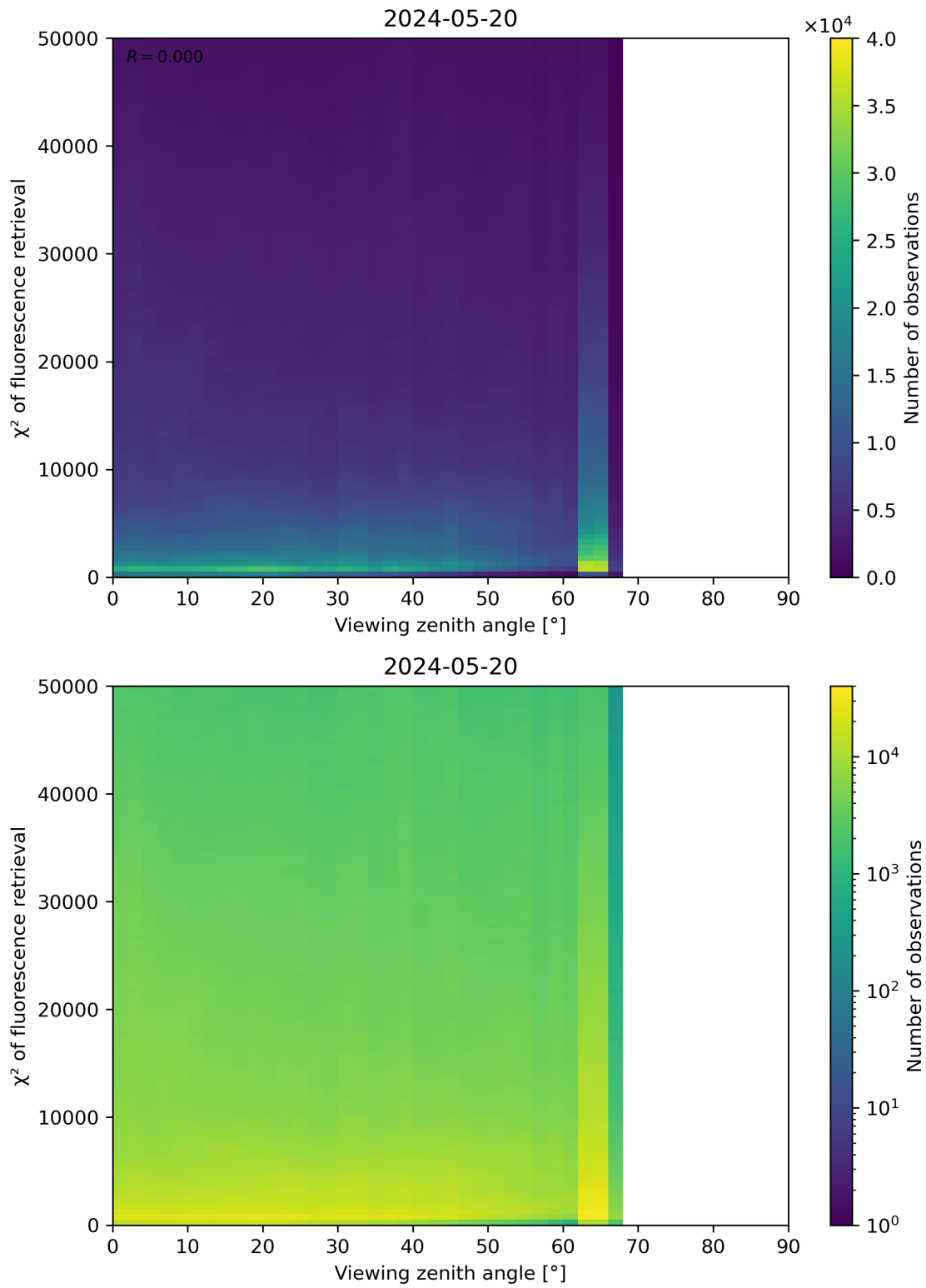
Figure 119: Scatter density plot of “Viewing zenith angle” against “ \chi^2 of fluorescence retrieval” for 2024-05-19 to 2024-05-21.
