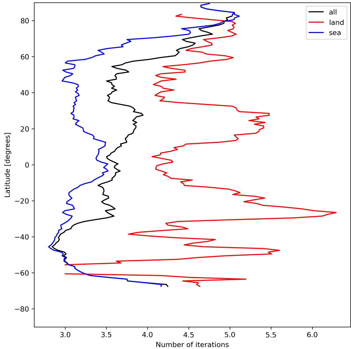
Figure 22: Zonal average of “Number of iterations” for 2024-05-19 to 2024-05-21.
