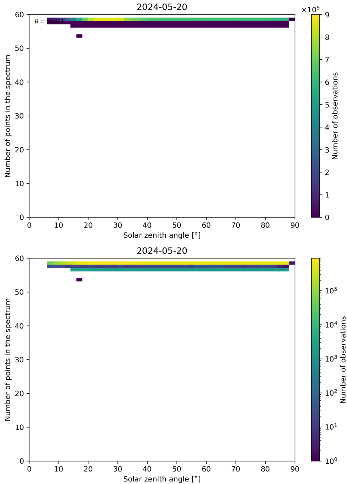
Figure 115: Scatter density plot of “Solar zenith angle” against “Number of points in the spectrum” for 2024-05-19 to 2024-05-21.
