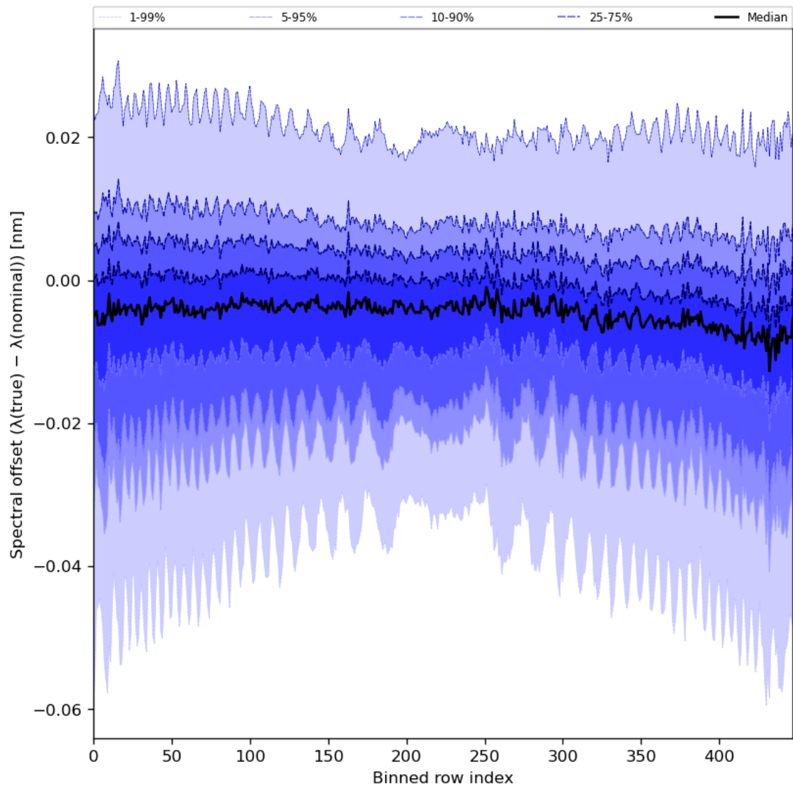
Figure 62: Along track statistics of “Spectral offset ( \lambda(\text{true}) - \lambda(\text{nominal}) )” for 2024-05-19 to 2024-05-21
