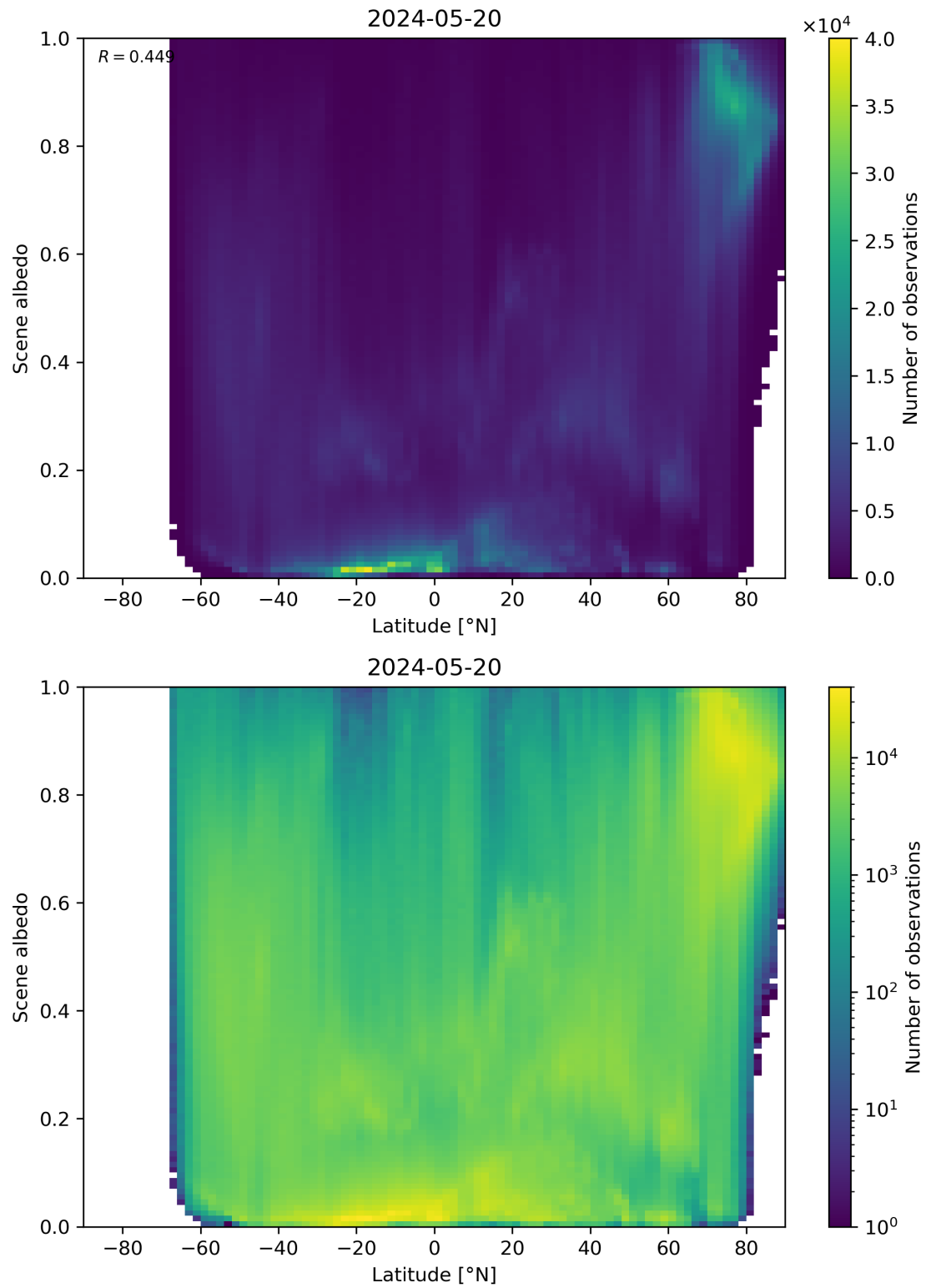
Figure 95: Scatter density plot of “Latitude” against “Scene albedo” for 2024-05-19 to 2024-05-21.
