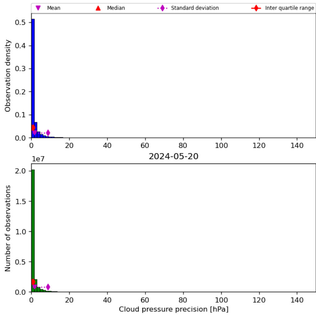
Figure 31: Histogram of “Cloud pressure precision” for 2024-05-19 to 2024-05-21
