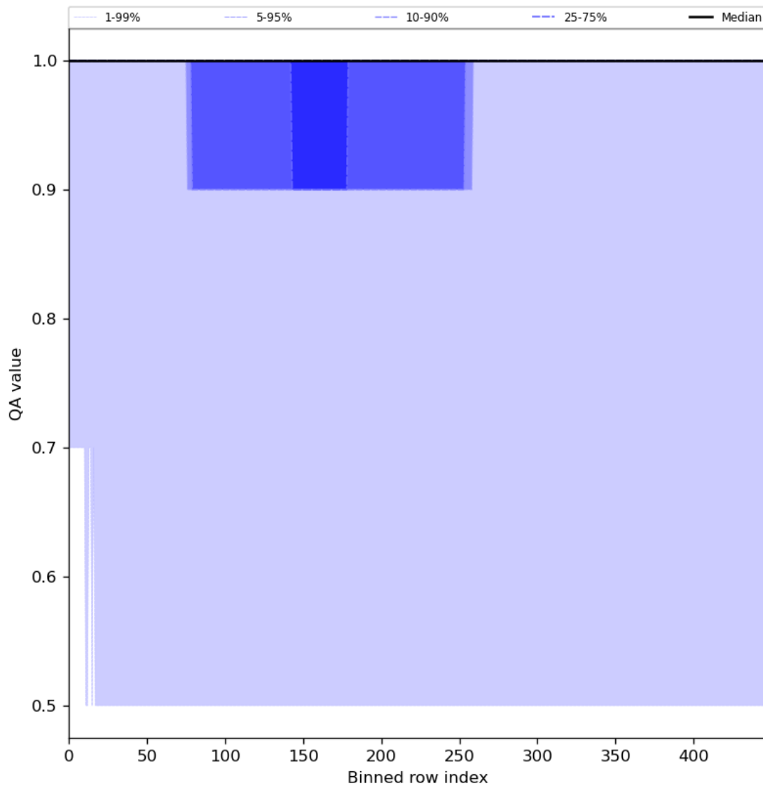
Figure 46: Along track statistics of “QA value” for 2024-05-19 to 2024-05-21
