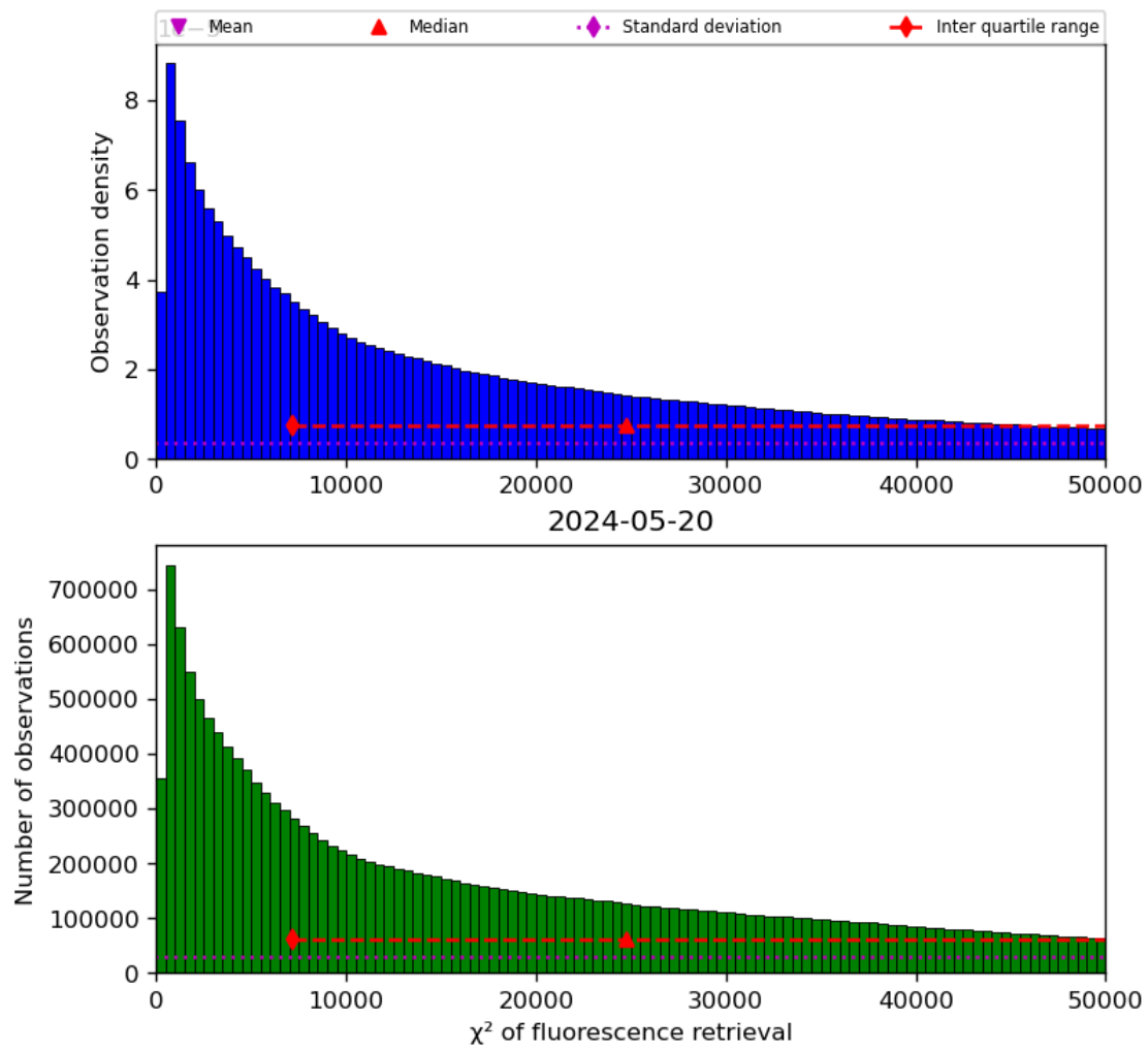
Figure 42: Histogram of “ \chi^2 of fluorescence retrieval” for 2024-05-19 to 2024-05-21
