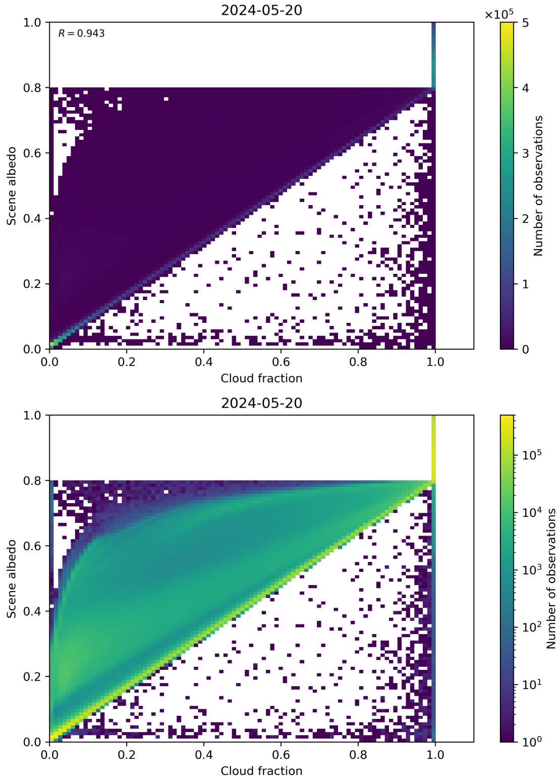
Figure 75: Scatter density plot of “Cloud fraction” against “Scene albedo” for 2024-05-19 to 2024-05-21.
