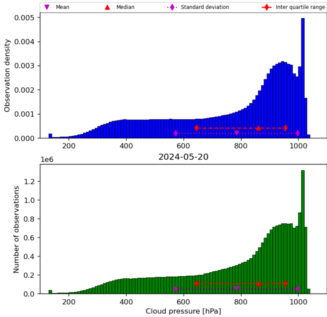
Figure 30: Histogram of “Cloud pressure” for 2024-05-19 to 2024-05-21
