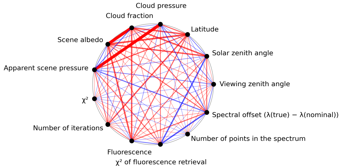
Figure 1: Map of correlation graph for 2024-05-19 to 2024-05-21.
