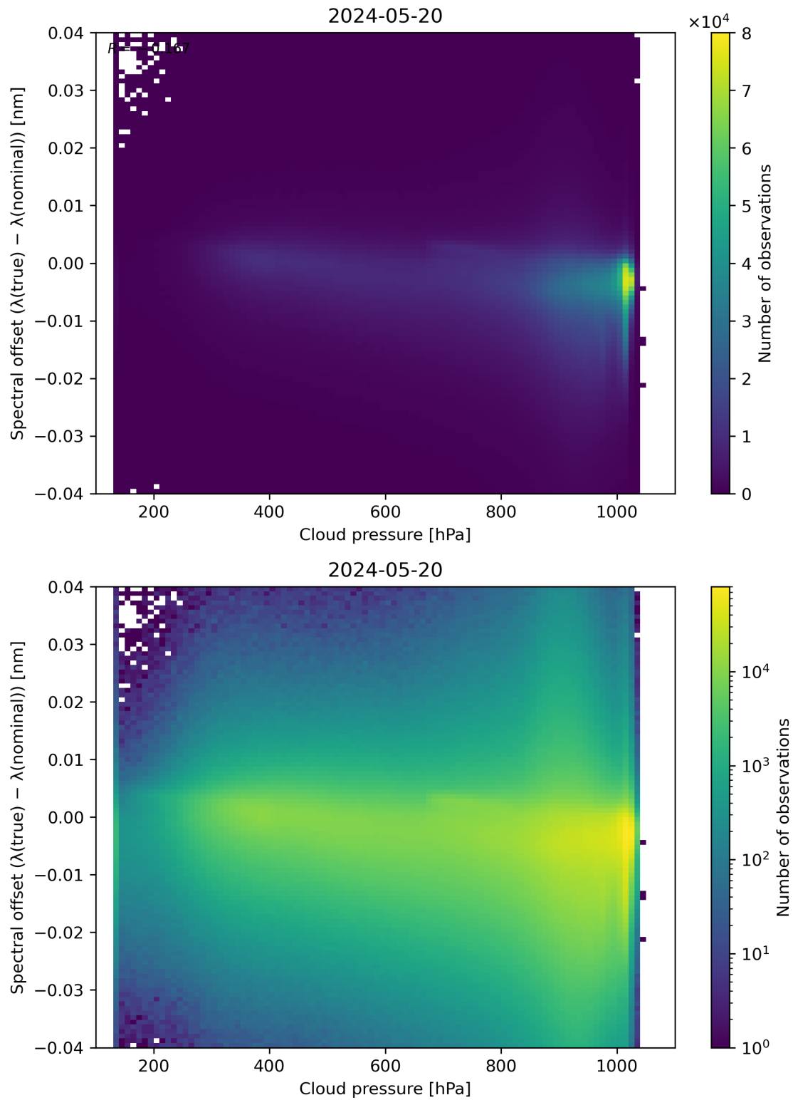
Figure 84: Scatter density plot of “Cloud pressure” against “Spectral offset ( \lambda(\text{true}) - \lambda(\text{nominal}) )” for 2024-05-19 to 2024-05-21.
