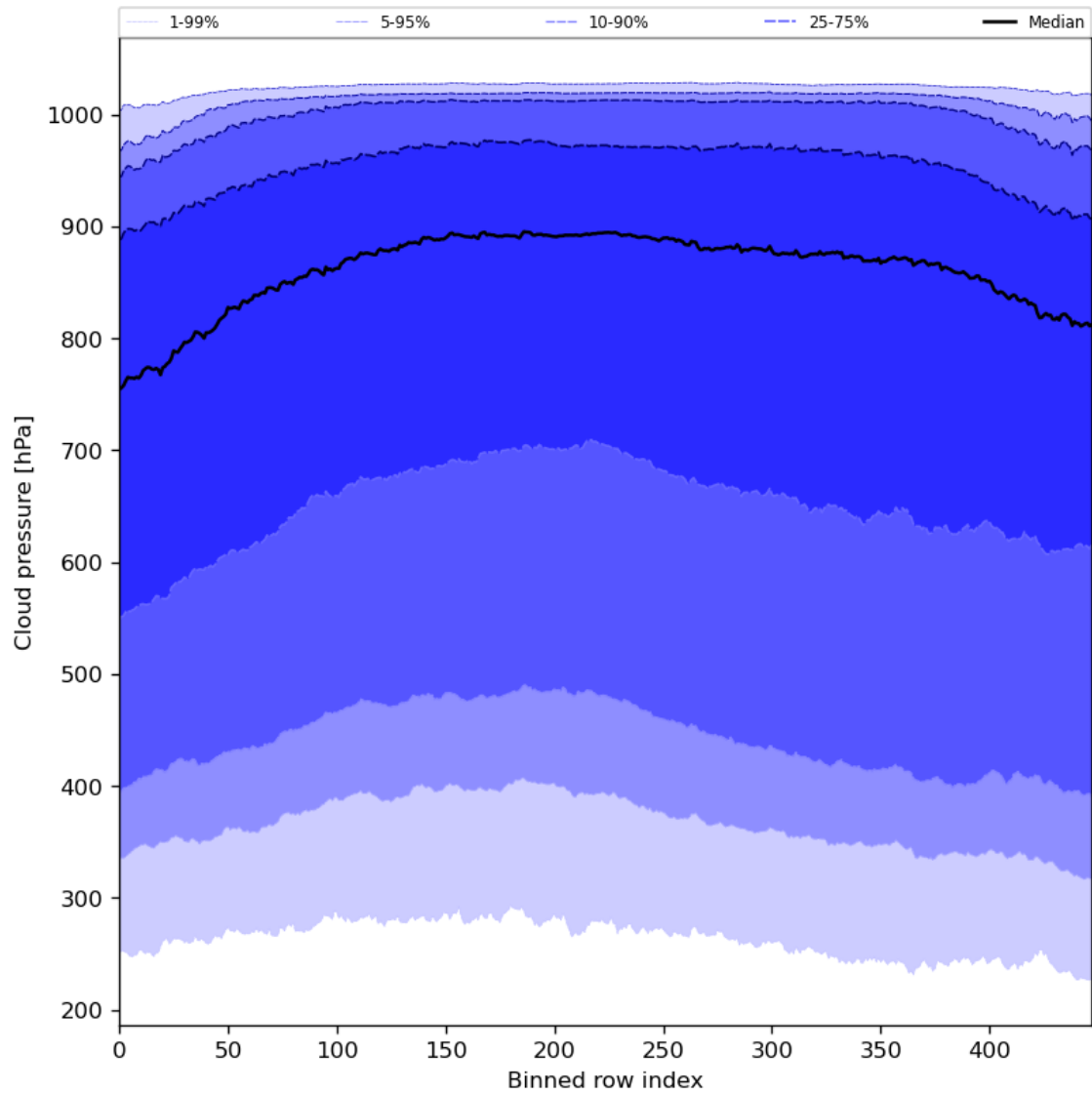
Figure 47: Along track statistics of “Cloud pressure” for 2024-05-19 to 2024-05-21
