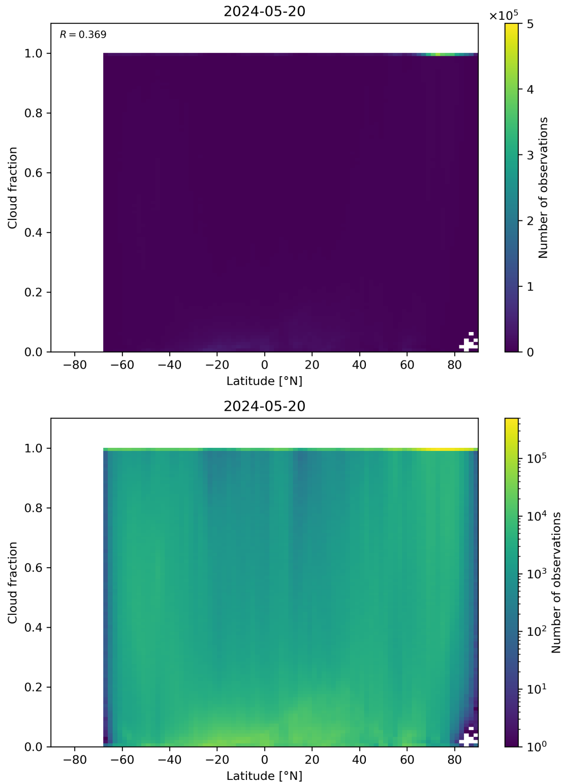
Figure 90: Scatter density plot of “Latitude” against “Cloud fraction” for 2024-05-19 to 2024-05-21.
