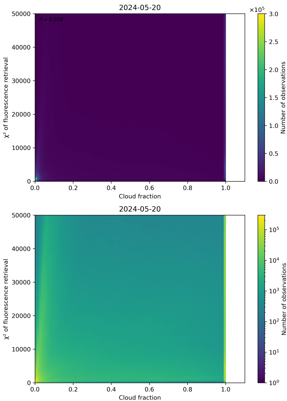
Figure 71: Scatter density plot of “Cloud fraction” against “ \chi^2 of fluorescence retrieval” for 2024-05-19 to 2024-05-21.
