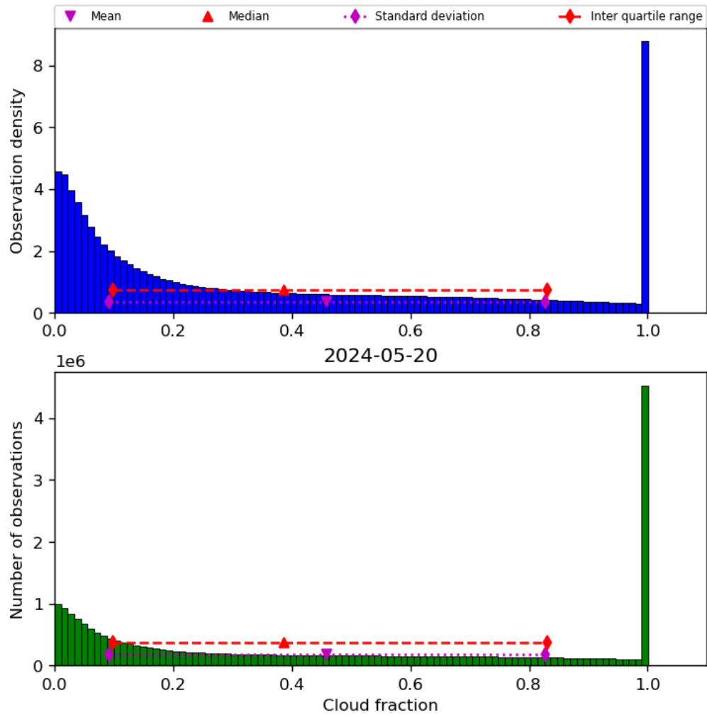
Figure 32: Histogram of “Cloud fraction” for 2024-05-19 to 2024-05-21
