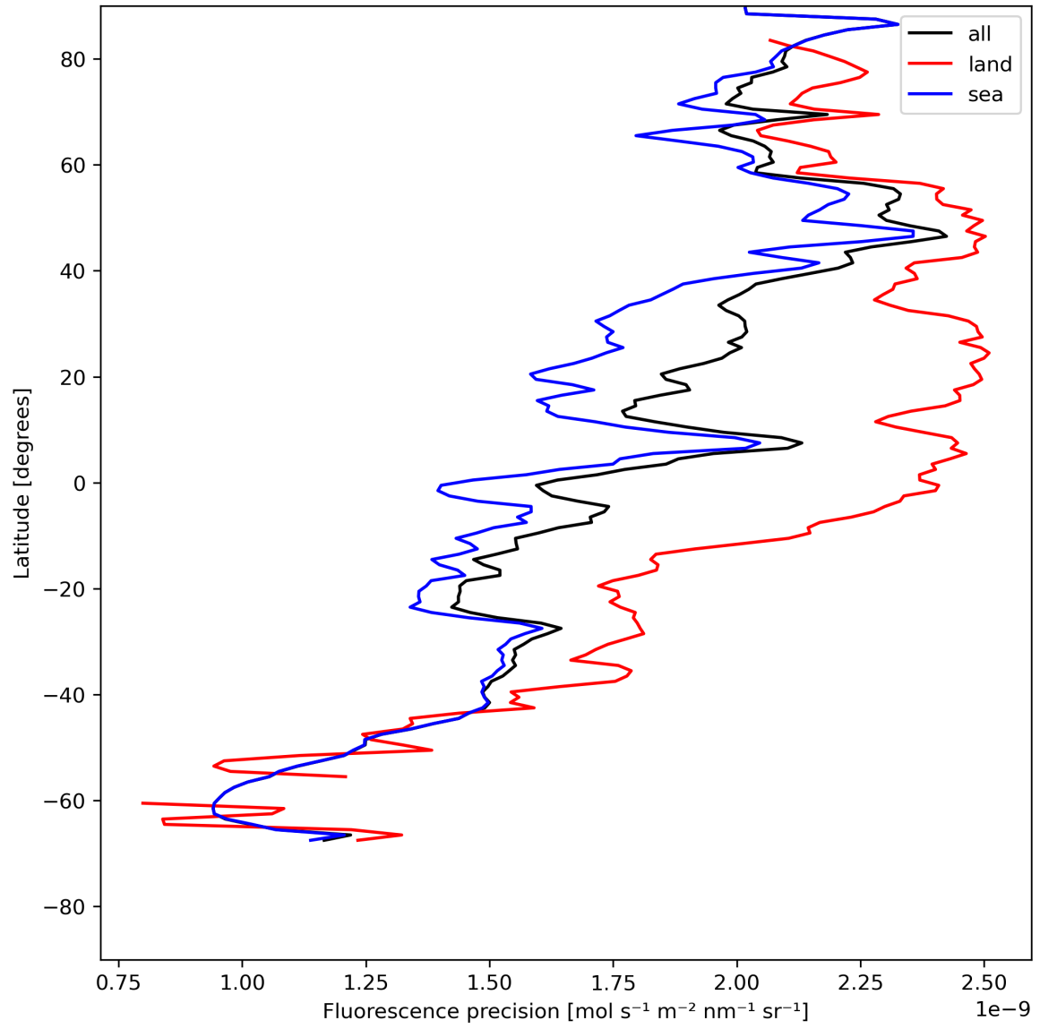
Figure 24: Zonal average of “Fluorescence precision” for 2024-05-20 to 2024-05-22.
