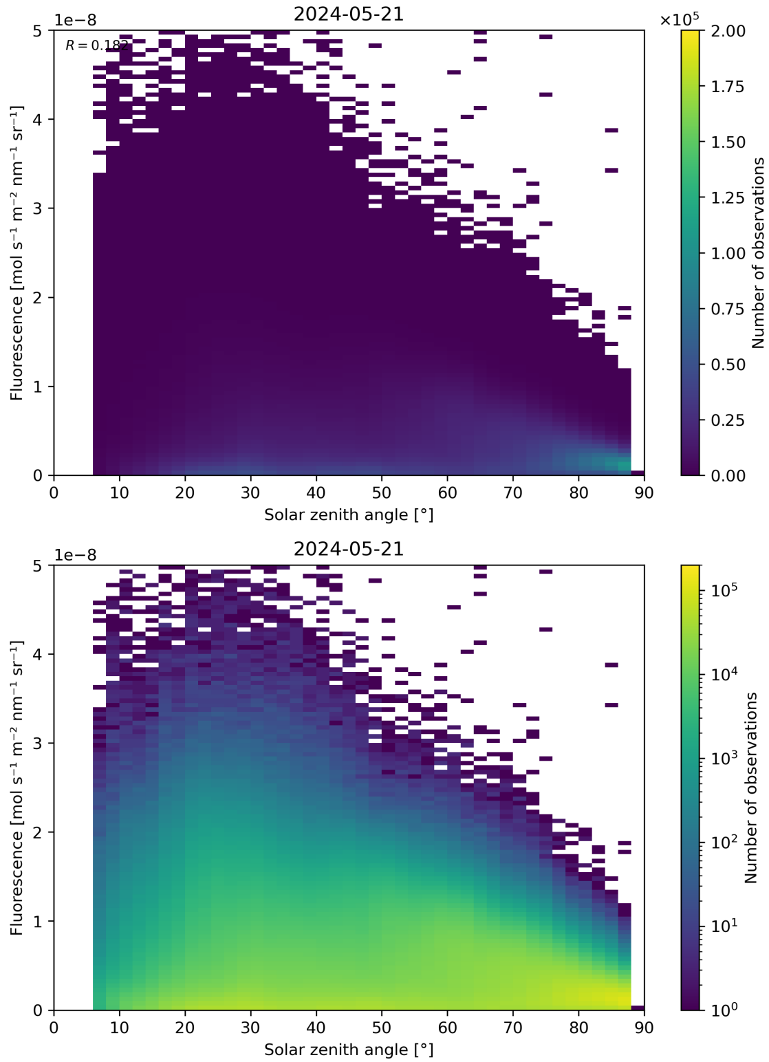
Figure 112: Scatter density plot of “Solar zenith angle” against “Fluorescence” for 2024-05-20 to 2024-05-22.
