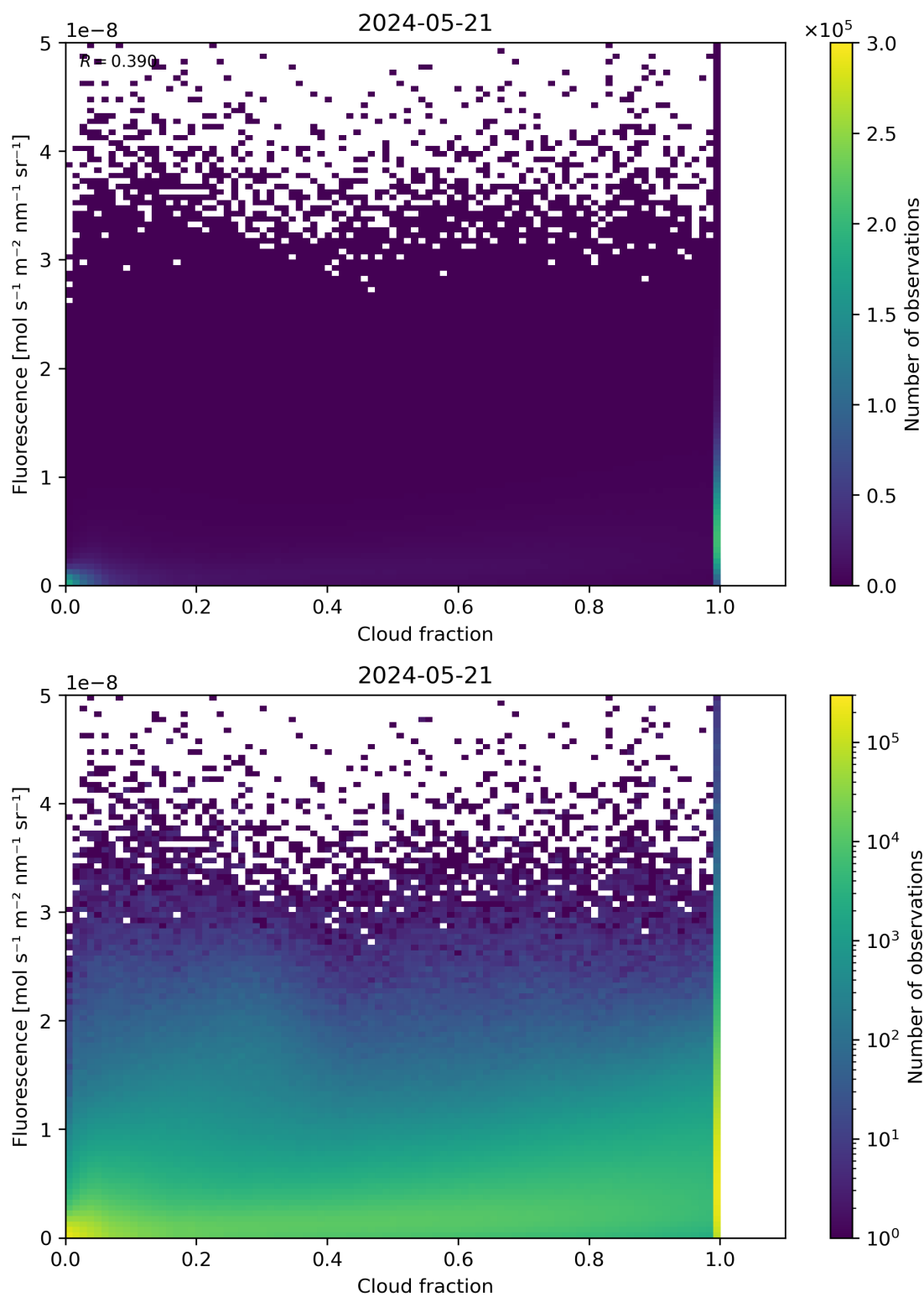
Figure 72: Scatter density plot of “Cloud fraction” against “Fluorescence” for 2024-05-20 to 2024-05-22.
