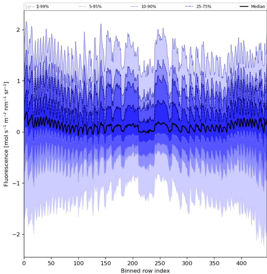
Figure 57: Along track statistics of "Fluorescence" for 2024-05-20 to 2024-05-22
