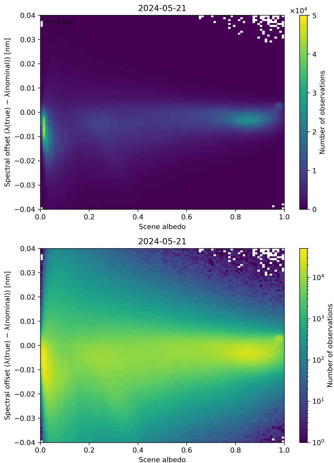
Figure 107: Scatter density plot of “Scene albedo” against “Spectral offset ( \lambda(\text{true}) - \lambda(\text{nominal}) )” for 2024-05-20 to 2024-05-22.
