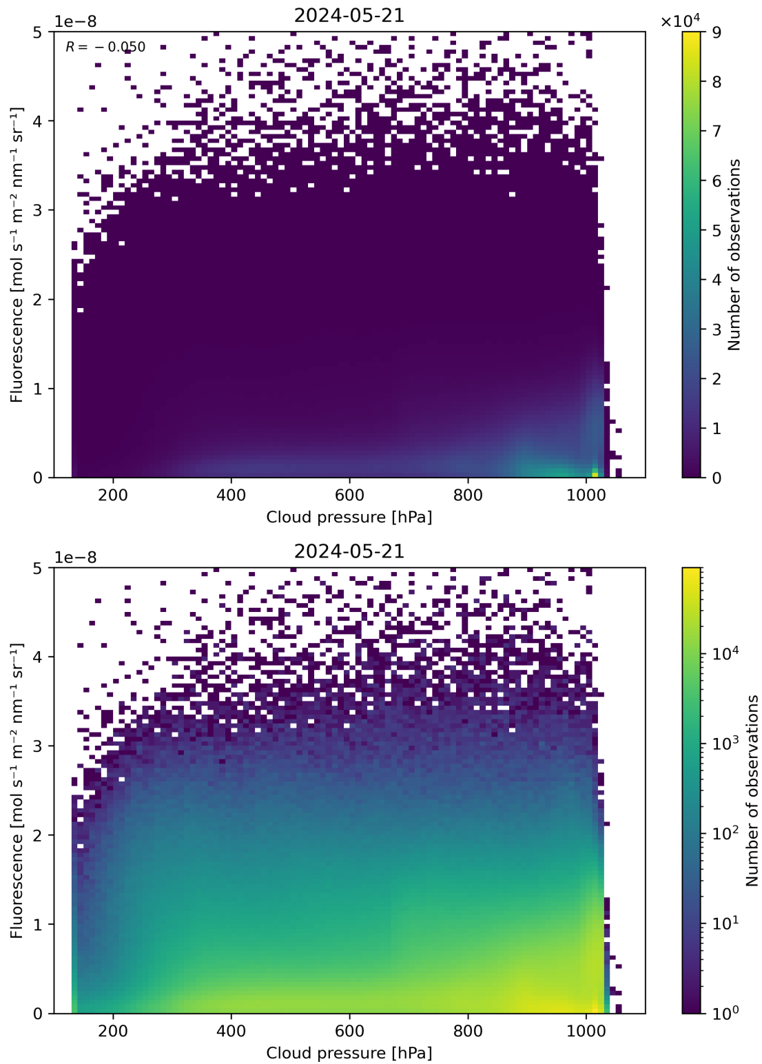
Figure 80: Scatter density plot of “Cloud pressure” against “Fluorescence” for 2024-05-20 to 2024-05-22.
