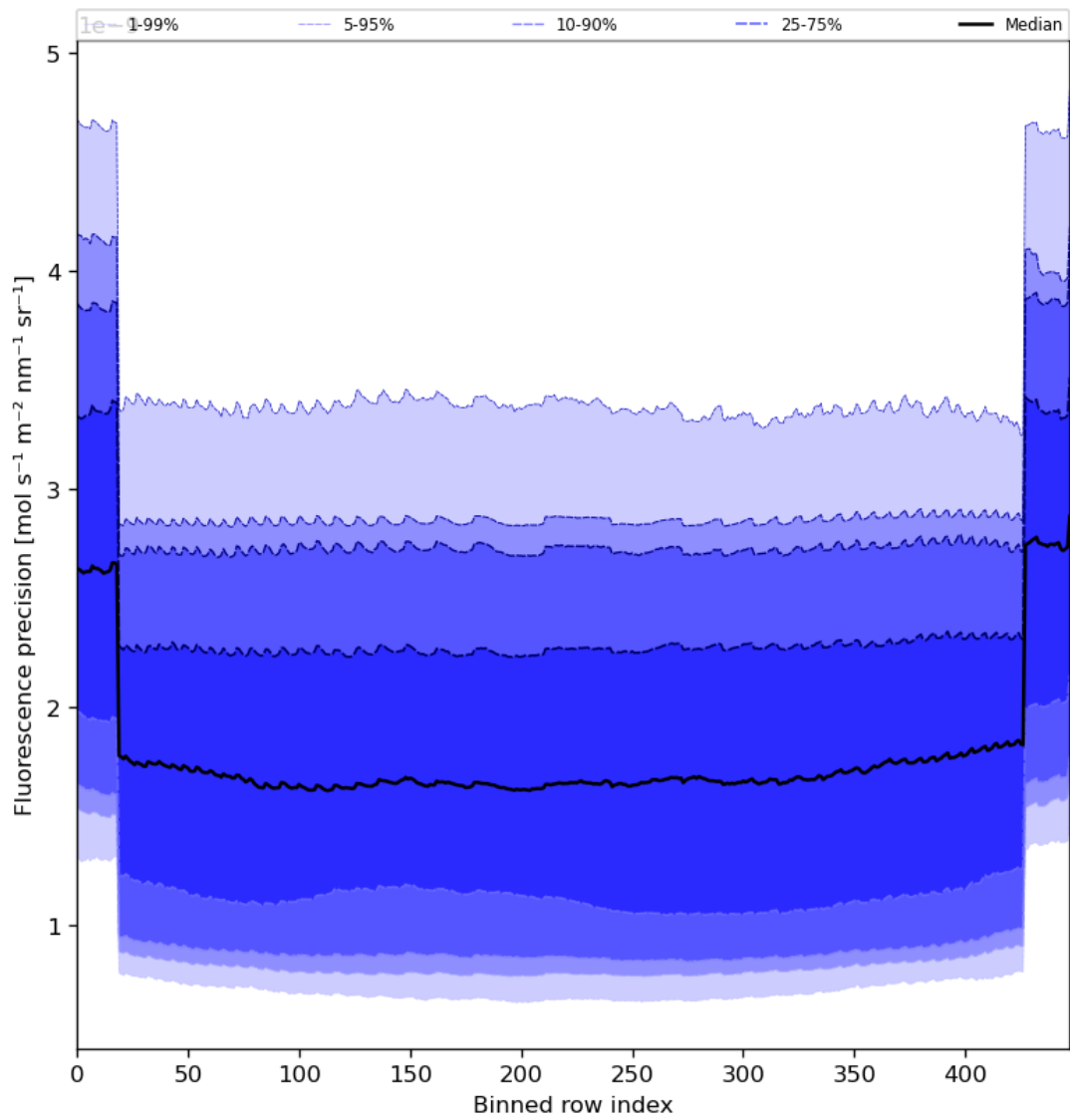
Figure 58: Along track statistics of “Fluorescence precision” for 2024-05-20 to 2024-05-22
