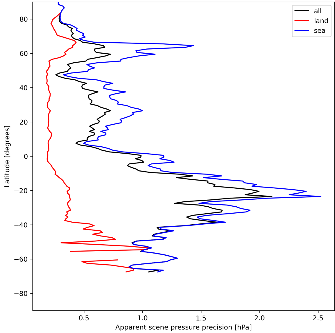
Figure 20: Zonal average of “Apparent scene pressure precision” for 2024-05-20 to 2024-05-22.
