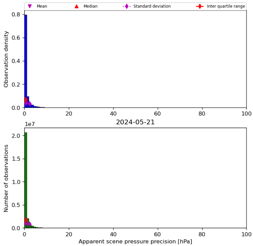
Figure 37: Histogram of “Apparent scene pressure precision” for 2024-05-20 to 2024-05-22
