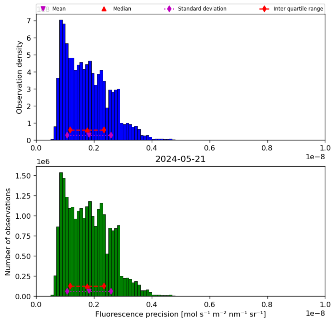
Figure 41: Histogram of “Fluorescence precision” for 2024-05-20 to 2024-05-22
