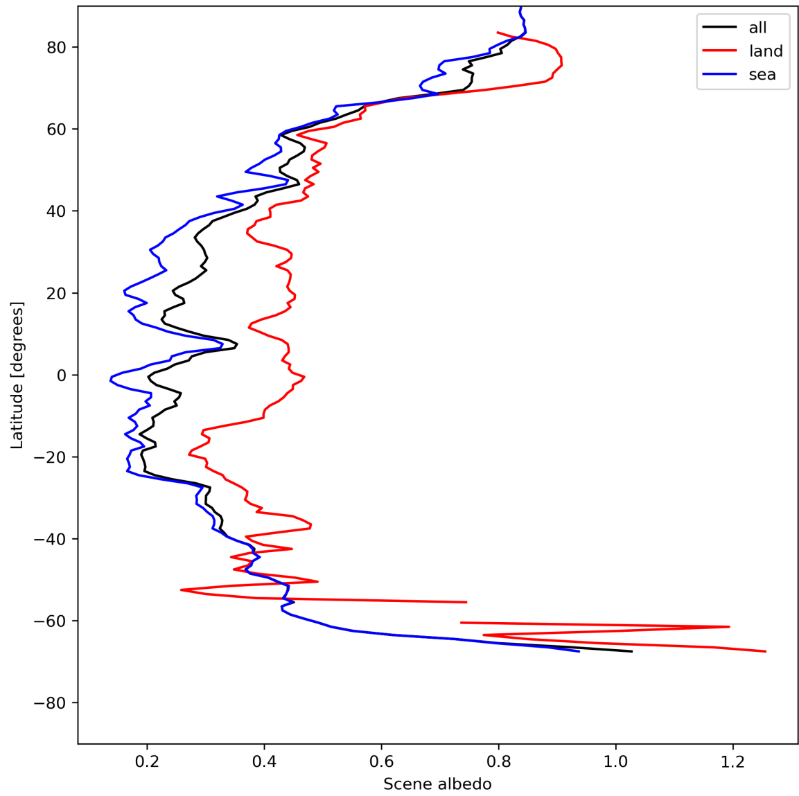
Figure 17: Zonal average of “Scene albedo” for 2024-05-20 to 2024-05-22.
