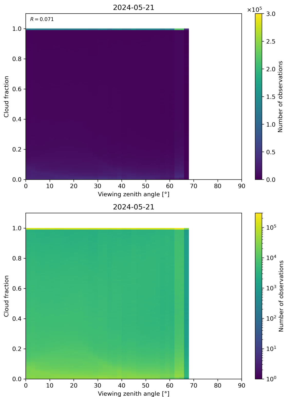
Figure 120: Scatter density plot of “Viewing zenith angle” against “Cloud fraction” for 2024-05-20 to 2024-05-22.
