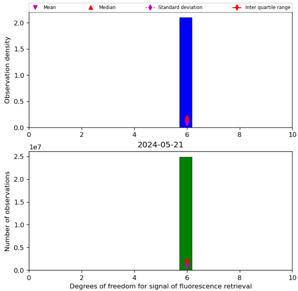
Figure 43: Histogram of “Degrees of freedom for signal of fluorescence retrieval” for 2024-05-20 to 2024-05-22
