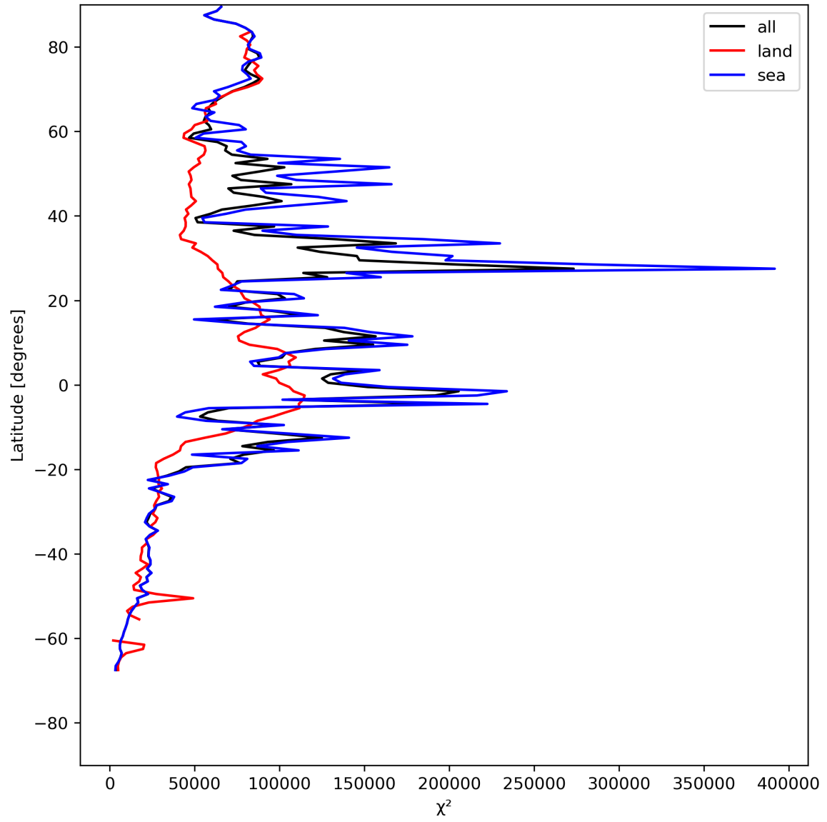
Figure 21: Zonal average of “ \chi^2 ” for 2024-05-20 to 2024-05-22.
