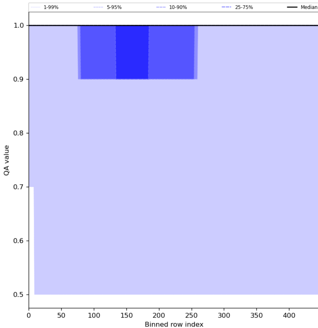
Figure 46: Along track statistics of “QA value” for 2024-05-20 to 2024-05-22
