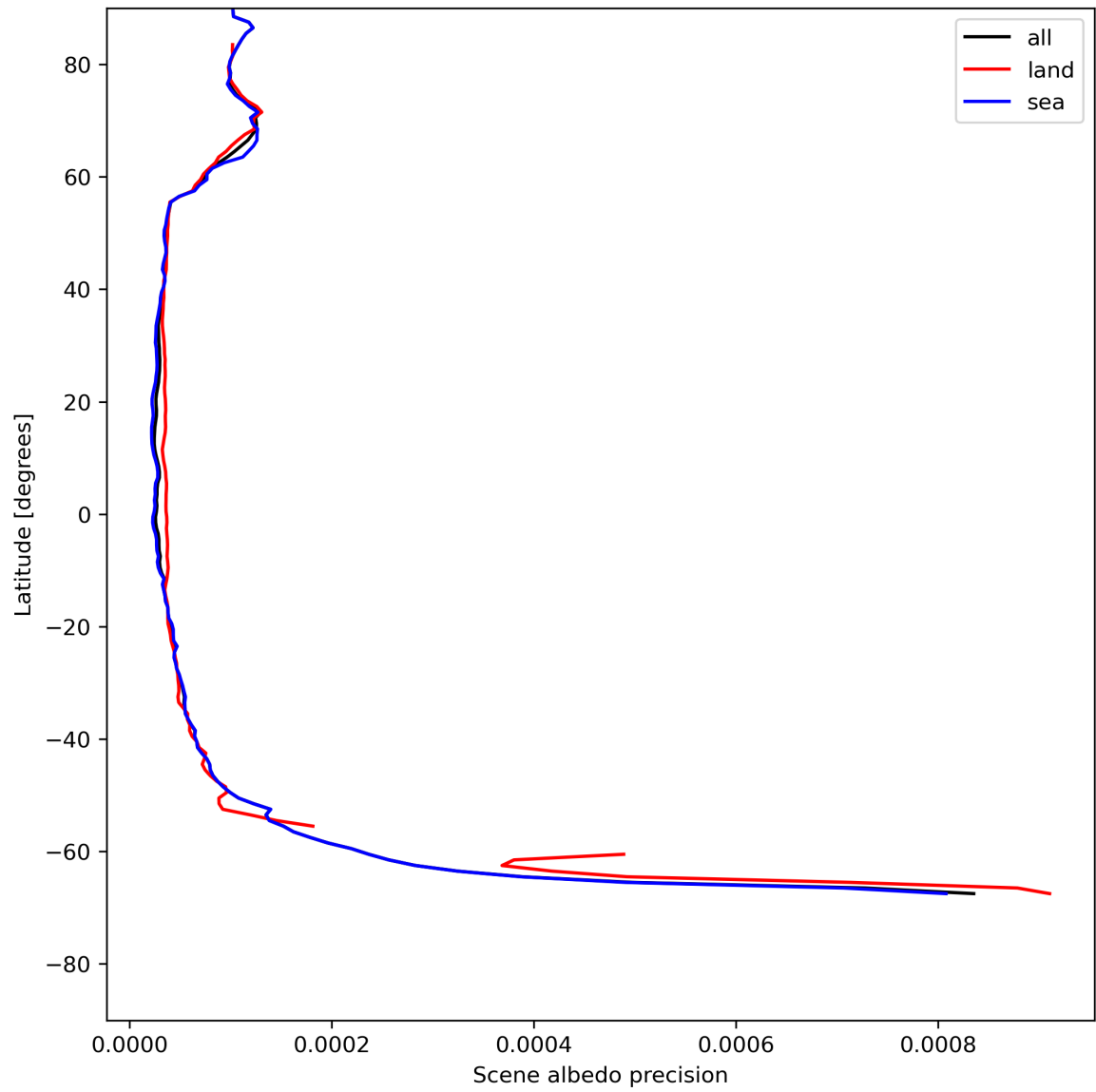
Figure 18: Zonal average of “Scene albedo precision” for 2024-05-20 to 2024-05-22.
