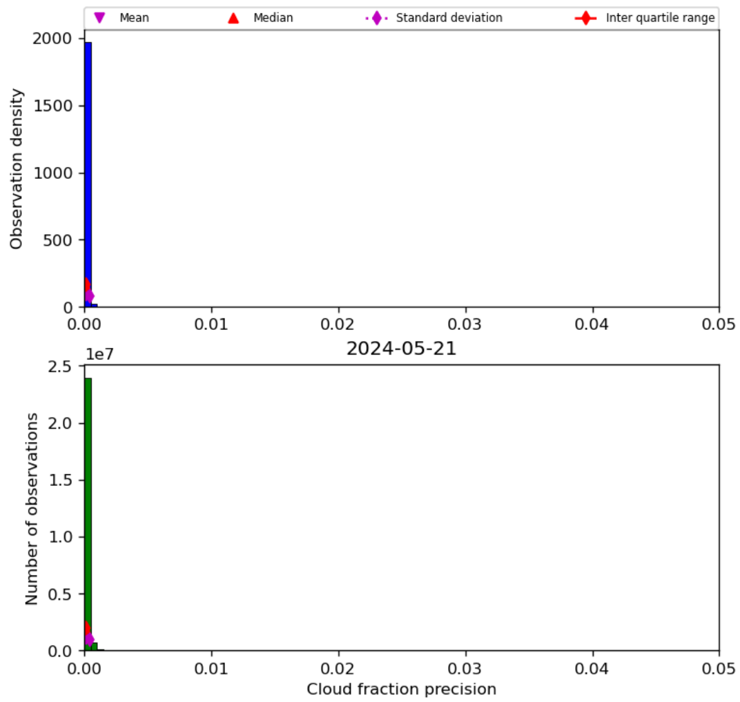
Figure 33: Histogram of “Cloud fraction precision” for 2024-05-20 to 2024-05-22
