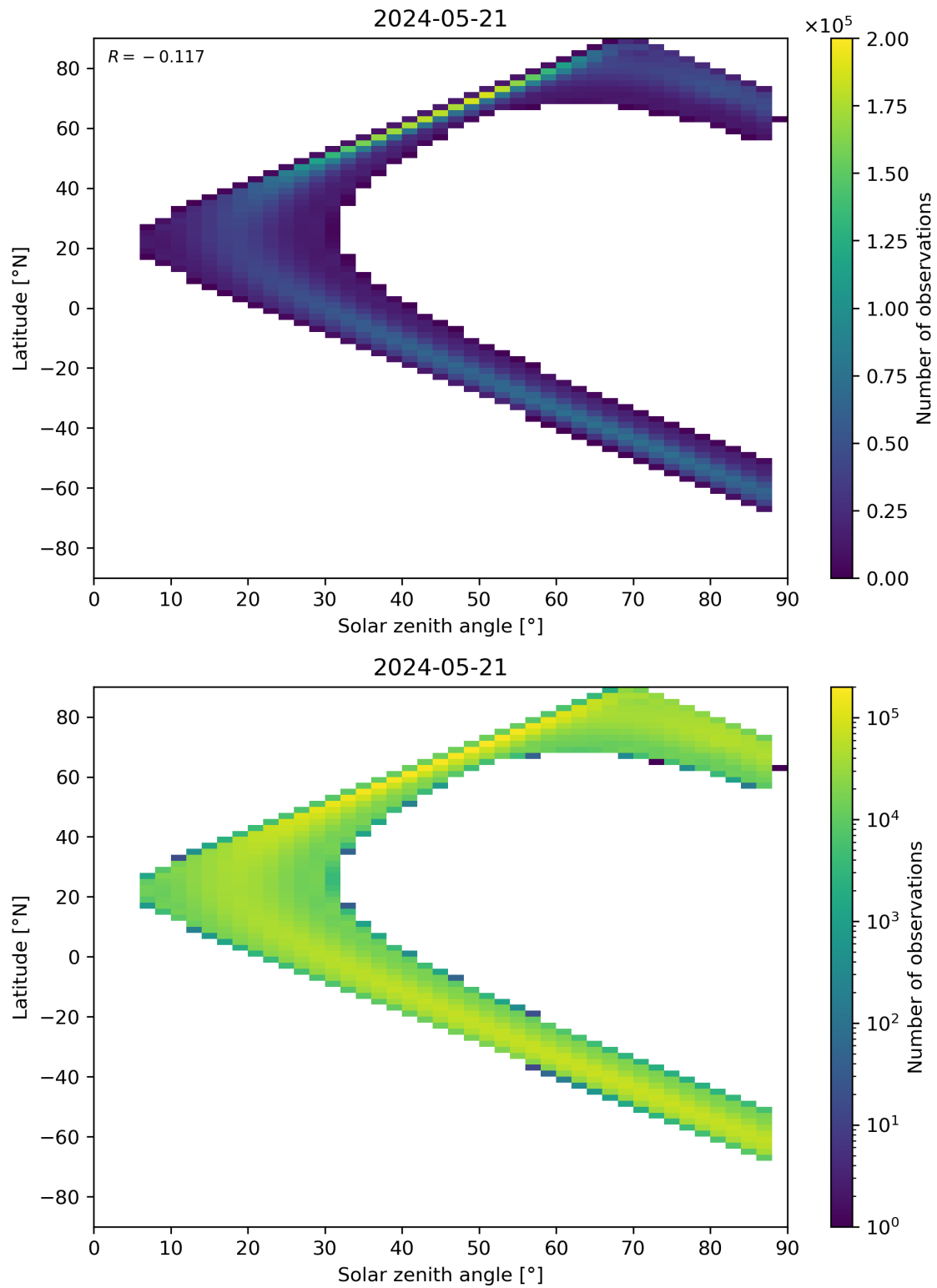
Figure 113: Scatter density plot of “Solar zenith angle” against “Latitude” for 2024-05-20 to 2024-05-22.
