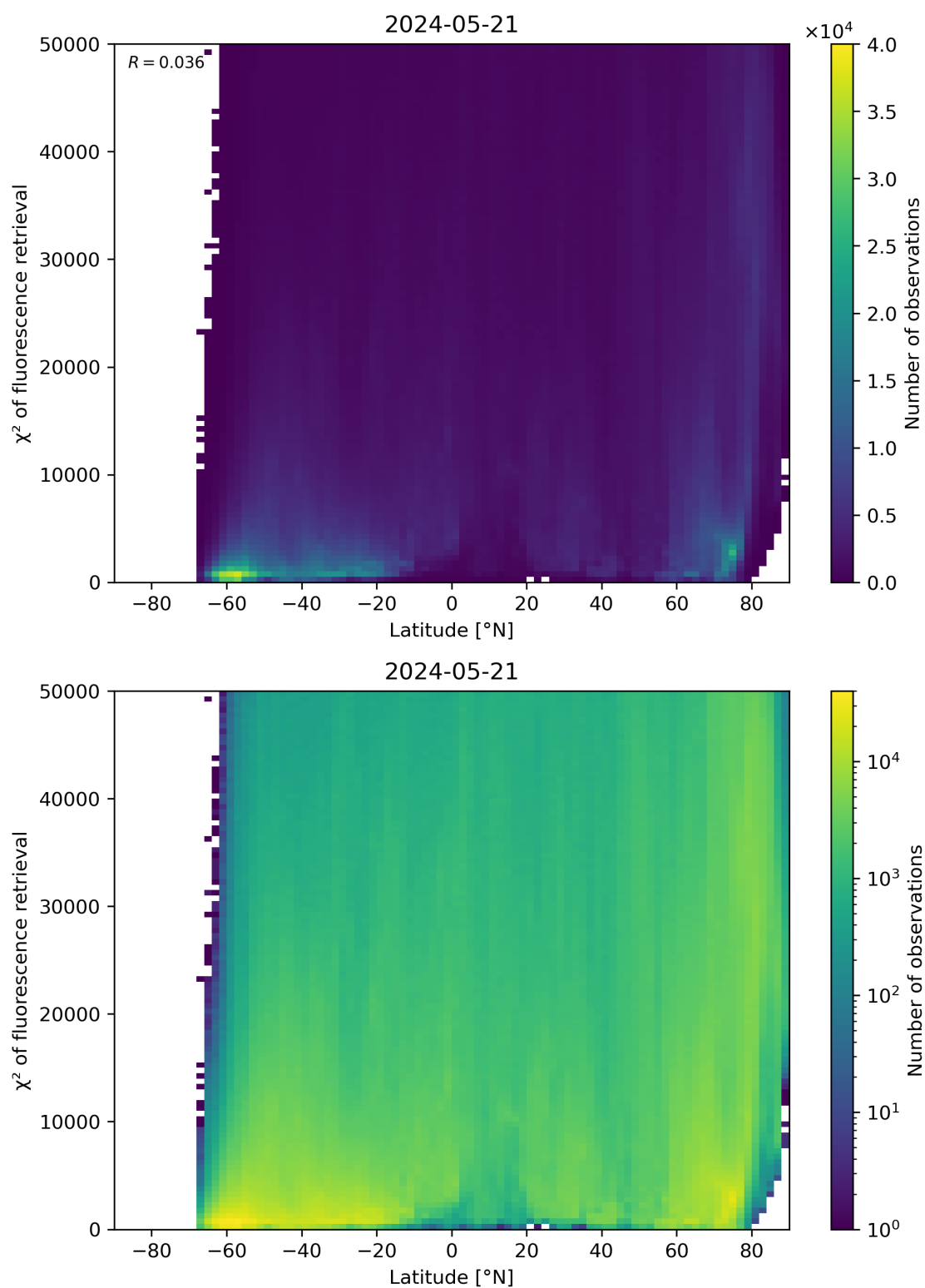
Figure 89: Scatter density plot of “Latitude” against “ \chi^2 of fluorescence retrieval” for 2024-05-20 to 2024-05-22.
