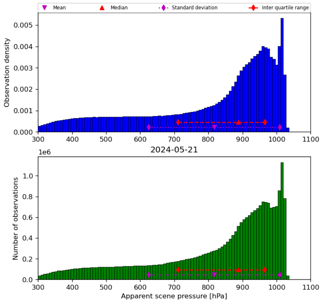
Figure 36: Histogram of “Apparent scene pressure” for 2024-05-20 to 2024-05-22
