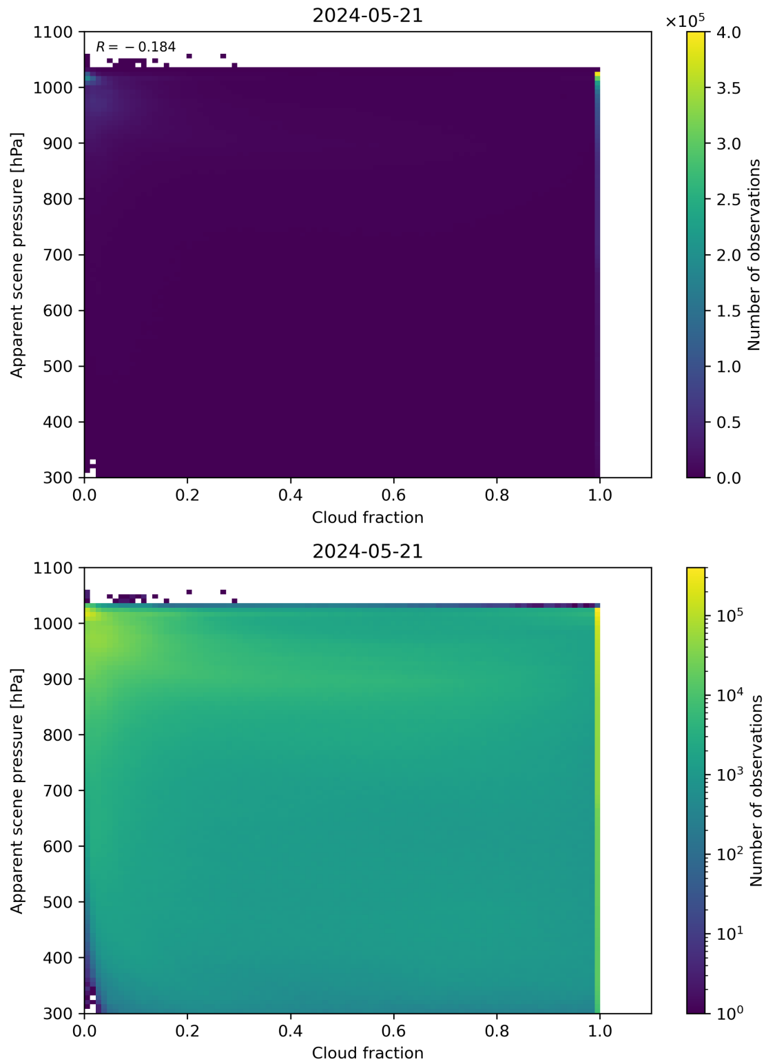
Figure 70: Scatter density plot of “Cloud fraction” against “Apparent scene pressure” for 2024-05-20 to 2024-05-22.
