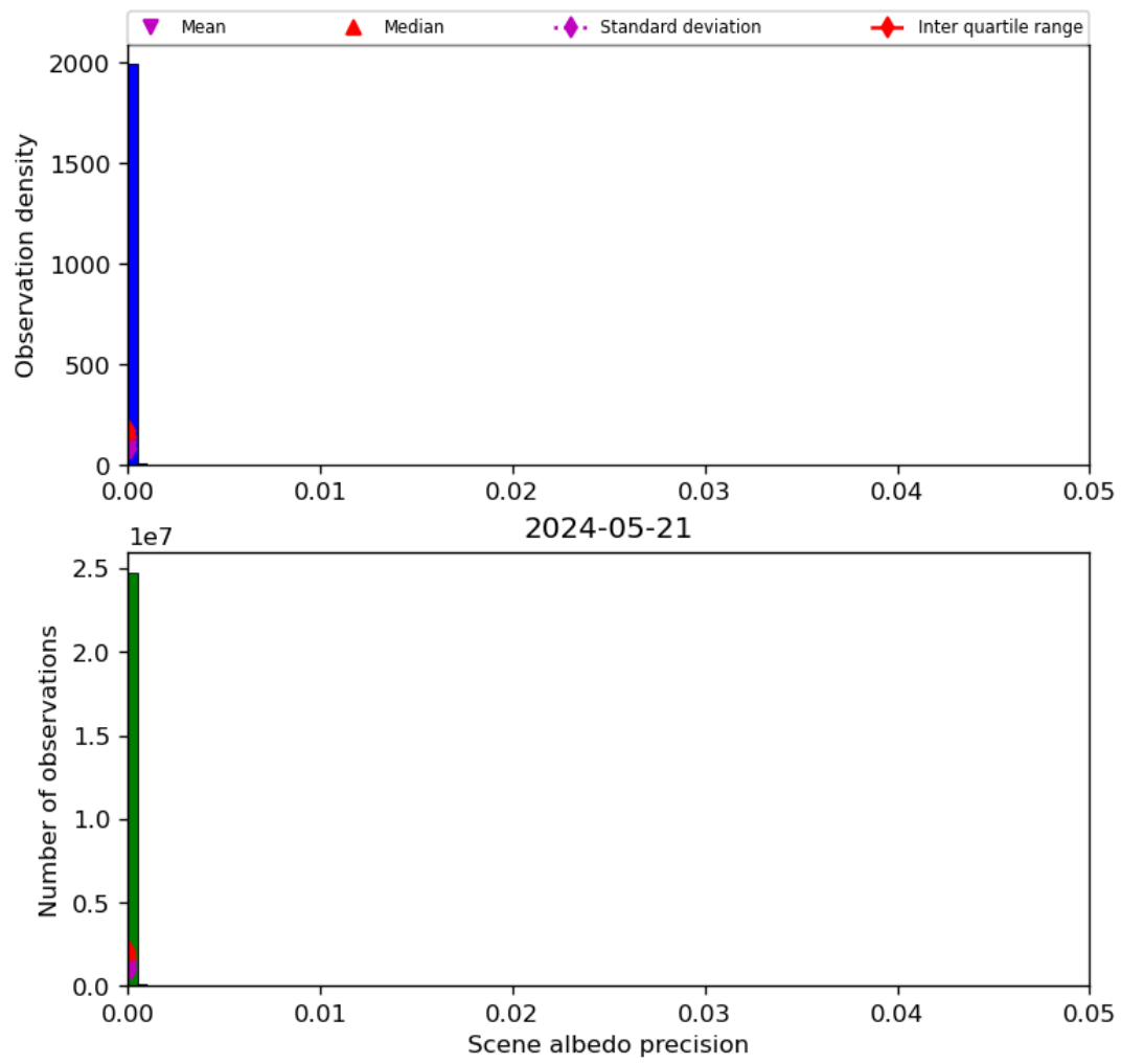
Figure 35: Histogram of “Scene albedo precision” for 2024-05-20 to 2024-05-22
