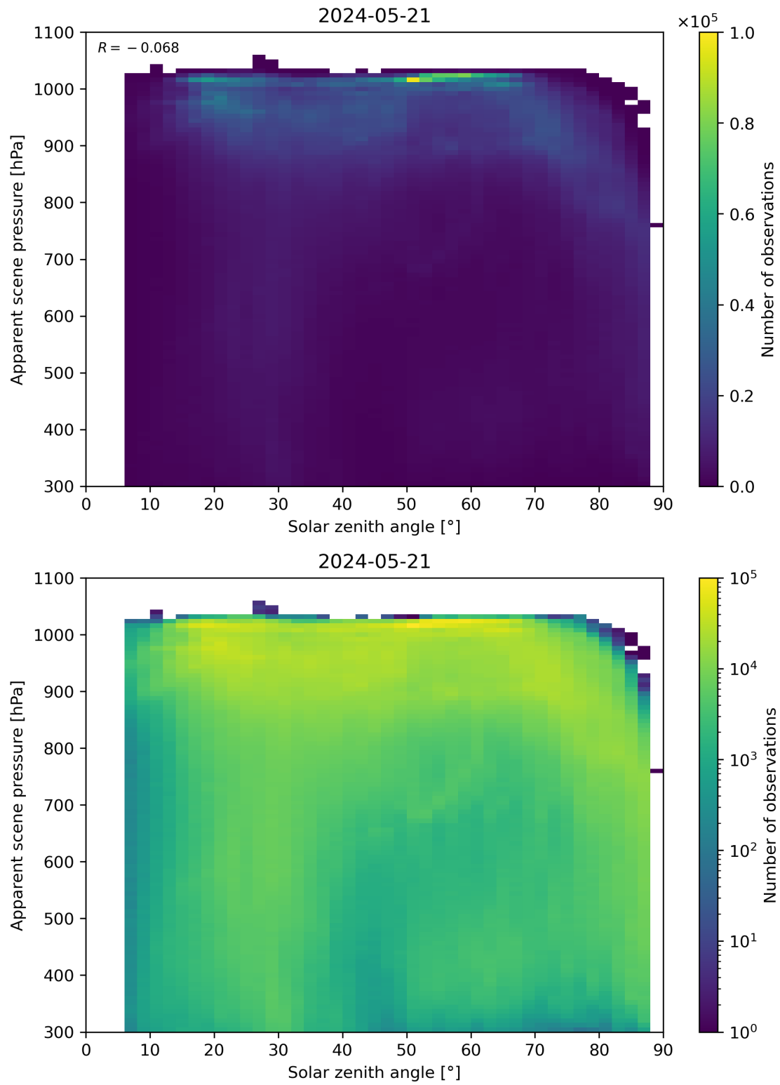
Figure 108: Scatter density plot of “Solar zenith angle” against “Apparent scene pressure” for 2024-05-20 to 2024-05-22.
