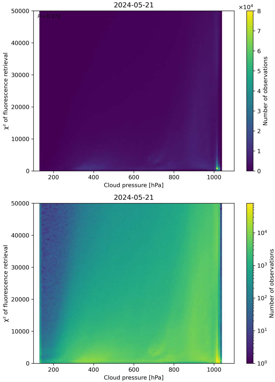
Figure 78: Scatter density plot of “Cloud pressure” against “ \chi^2 of fluorescence retrieval” for 2024-05-20 to 2024-05-22.
