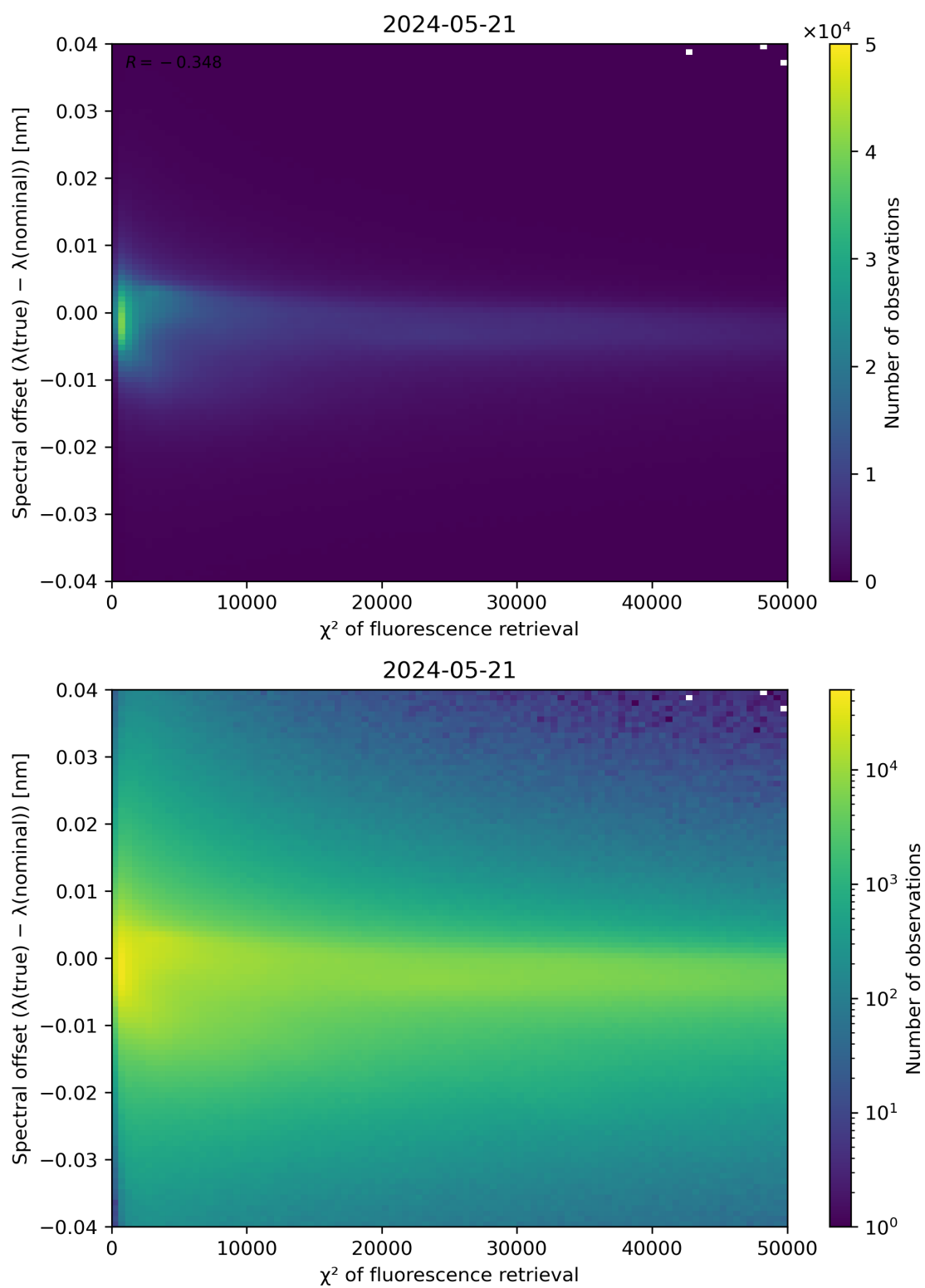
Figure 69: Scatter density plot of " \chi^2 of fluorescence retrieval" against "Spectral offset ( \lambda(\text{true}) - \lambda(\text{nominal}) )" for 2024-05-20 to 2024-05-22.
