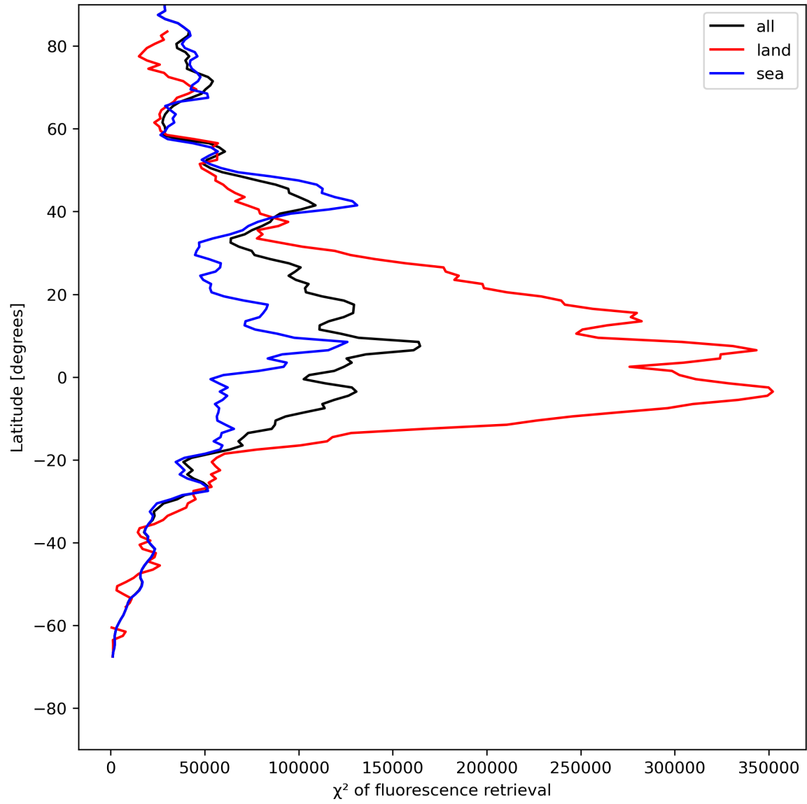
Figure 25: Zonal average of “ \chi^2 of fluorescence retrieval” for 2024-05-20 to 2024-05-22.
