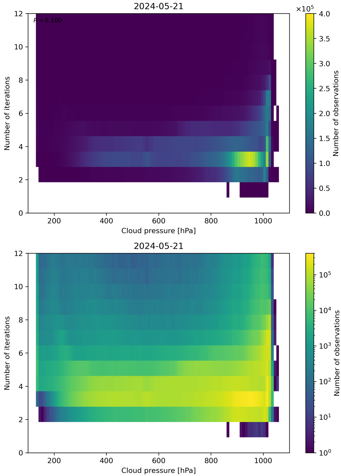
Figure 81: Scatter density plot of “Cloud pressure” against “Number of iterations” for 2024-05-20 to 2024-05-22.
