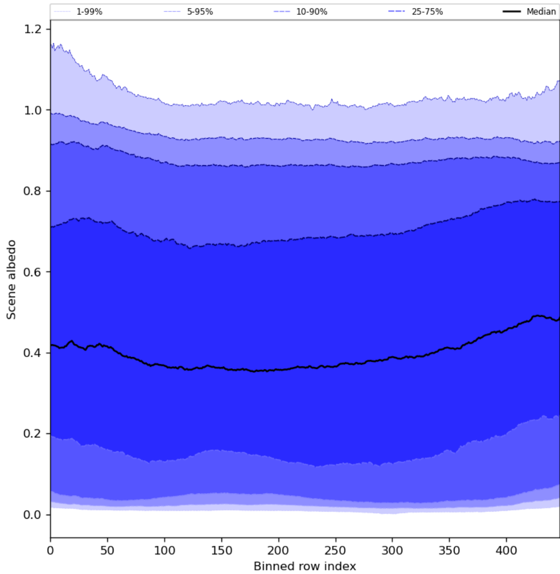
Figure 51: Along track statistics of “Scene albedo” for 2024-05-20 to 2024-05-22
