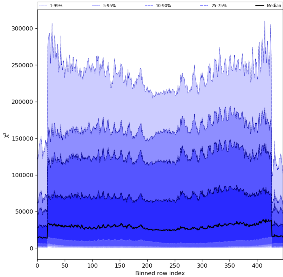
Figure 55: Along track statistics of “ \chi^2 ” for 2024-05-20 to 2024-05-22
