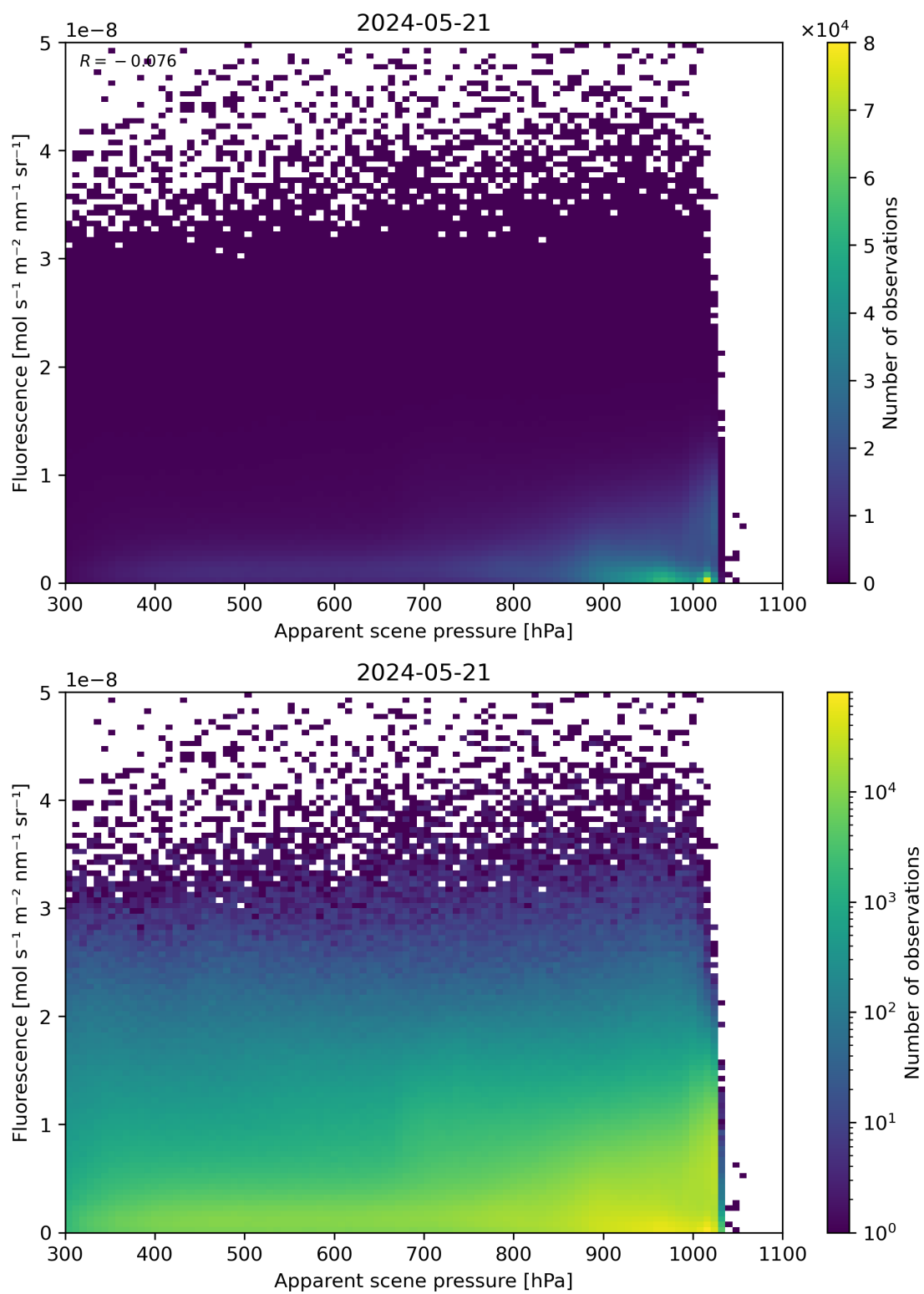
Figure 64: Scatter density plot of “Apparent scene pressure” against “Fluorescence” for 2024-05-20 to 2024-05-22.
