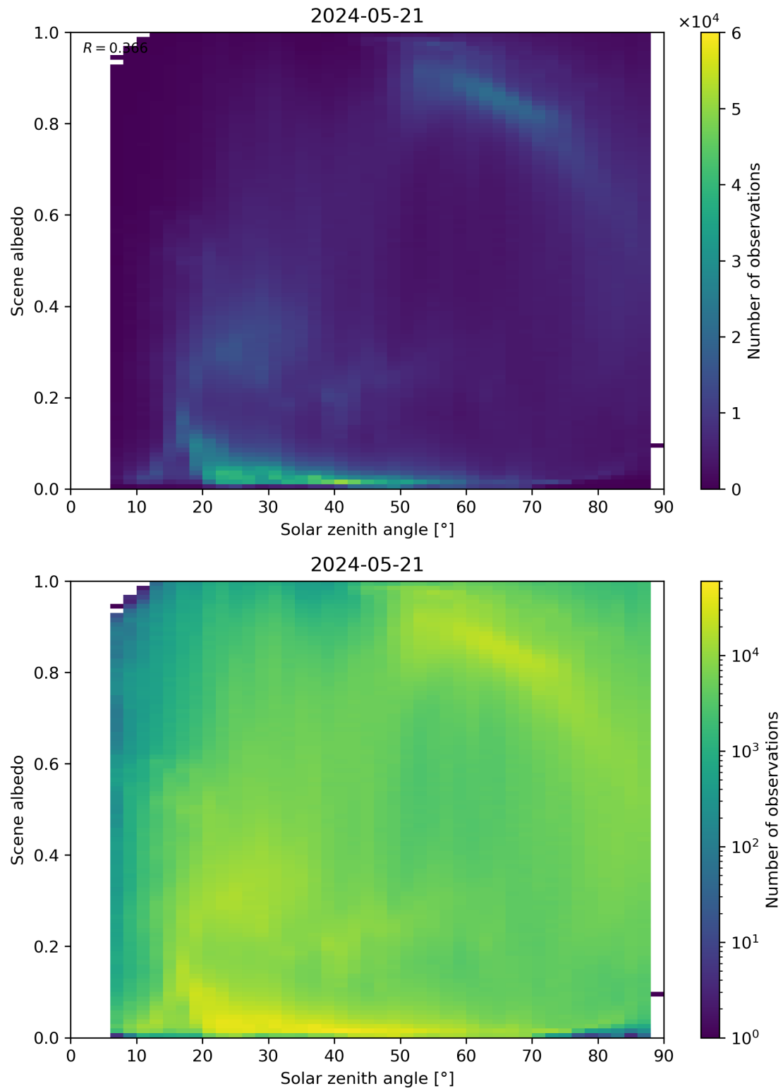
Figure 116: Scatter density plot of “Solar zenith angle” against “Scene albedo” for 2024-05-20 to 2024-05-22.
