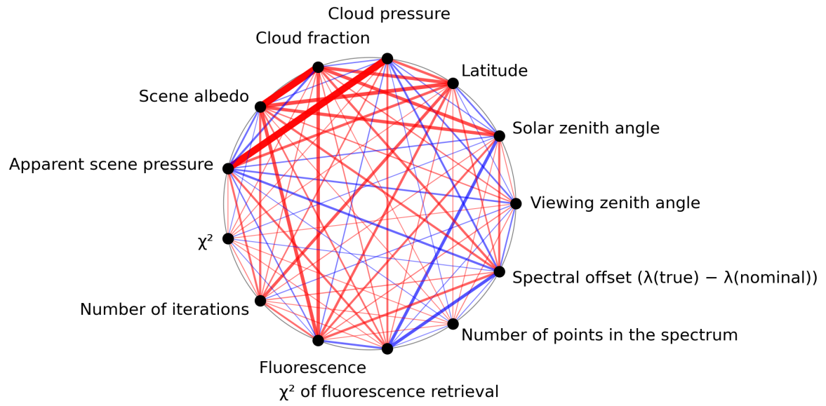
Figure 1: Map of correlation graph for 2024-05-20 to 2024-05-22.
