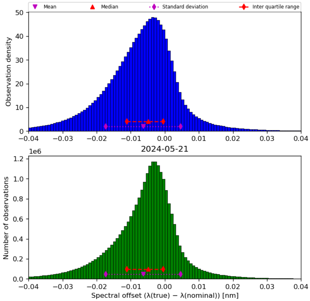
Figure 45: Histogram of “Spectral offset ( \lambda(\text{true}) - \lambda(\text{nominal}) )” for 2024-05-20 to 2024-05-22
