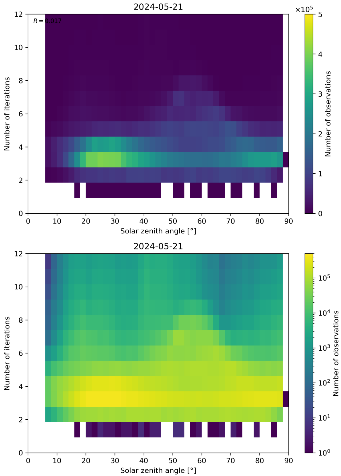
Figure 114: Scatter density plot of “Solar zenith angle” against “Number of iterations” for 2024-05-20 to 2024-05-22.
