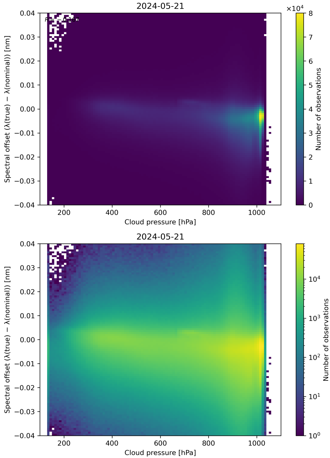
Figure 84: Scatter density plot of “Cloud pressure” against “Spectral offset ( \lambda(\text{true}) - \lambda(\text{nominal}) )” for 2024-05-20 to 2024-05-22.
