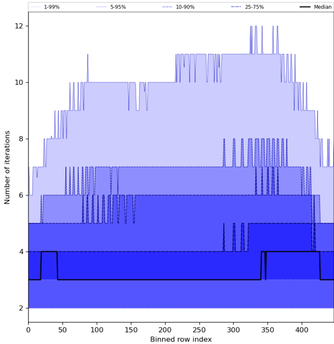
Figure 56: Along track statistics of “Number of iterations” for 2024-05-20 to 2024-05-22
