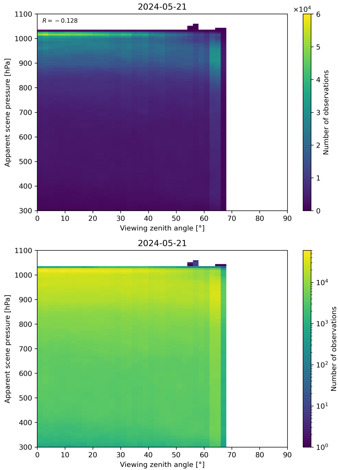
Figure 118: Scatter density plot of “Viewing zenith angle” against “Apparent scene pressure” for 2024-05-20 to 2024-05-22.
