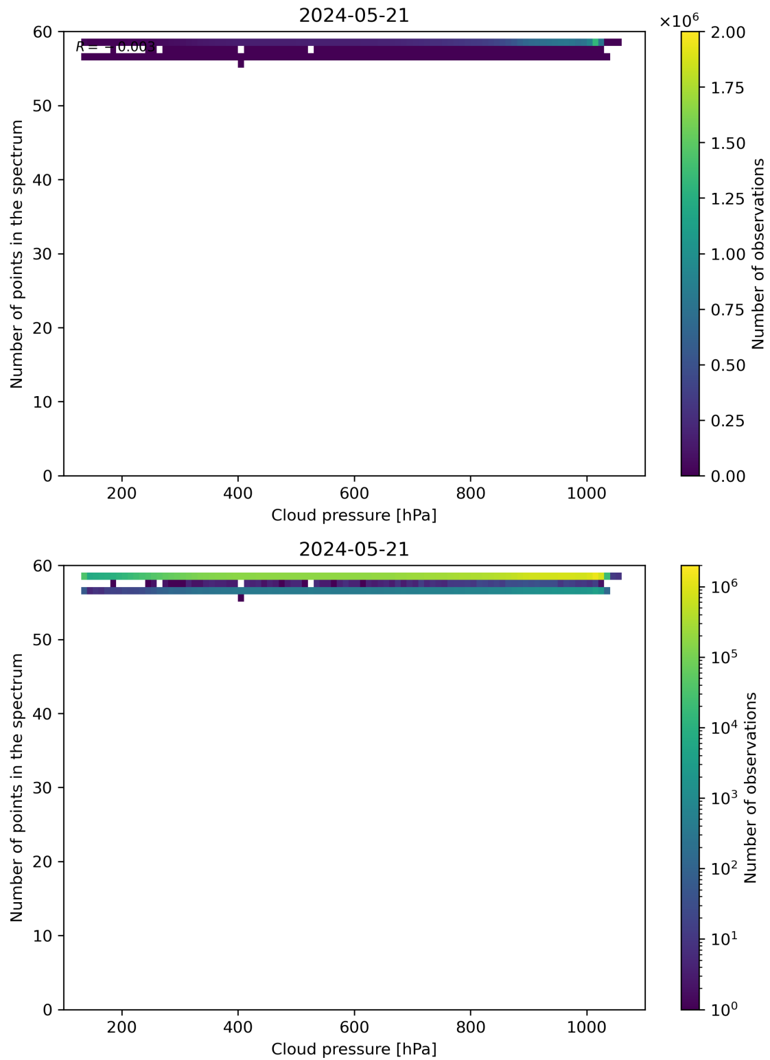
Figure 82: Scatter density plot of “Cloud pressure” against “Number of points in the spectrum” for 2024-05-20 to 2024-05-22.
