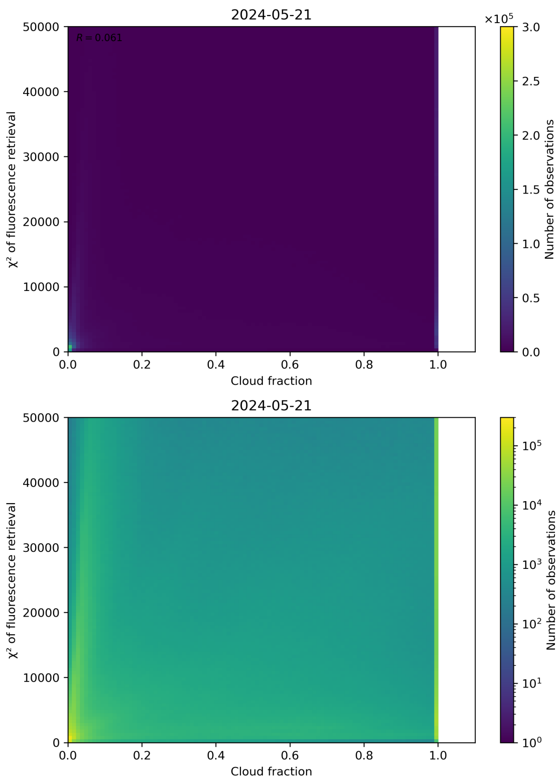
Figure 71: Scatter density plot of “Cloud fraction” against “ \chi^2 of fluorescence retrieval” for 2024-05-20 to 2024-05-22.
