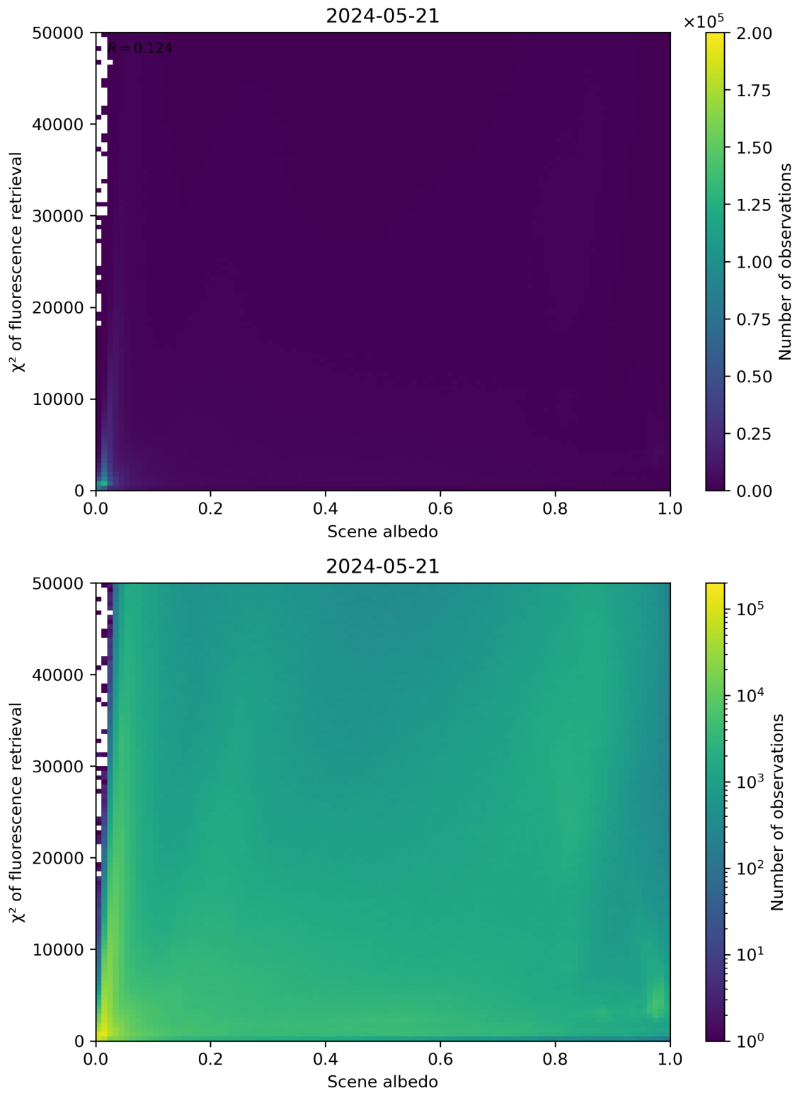
Figure 103: Scatter density plot of “Scene albedo” against “ \chi^2 of fluorescence retrieval” for 2024-05-20 to 2024-05-22.
