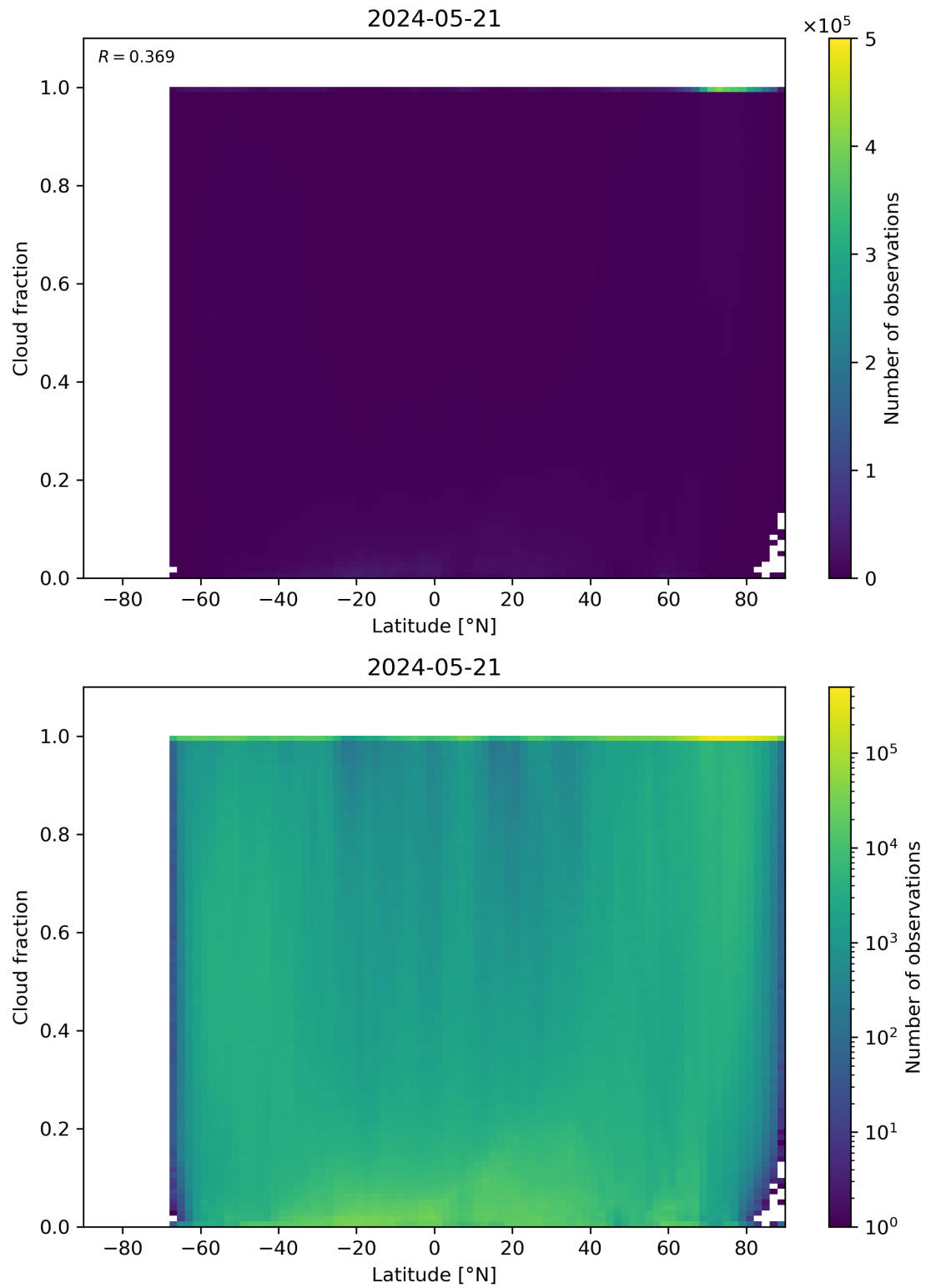
Figure 90: Scatter density plot of “Latitude” against “Cloud fraction” for 2024-05-20 to 2024-05-22.
