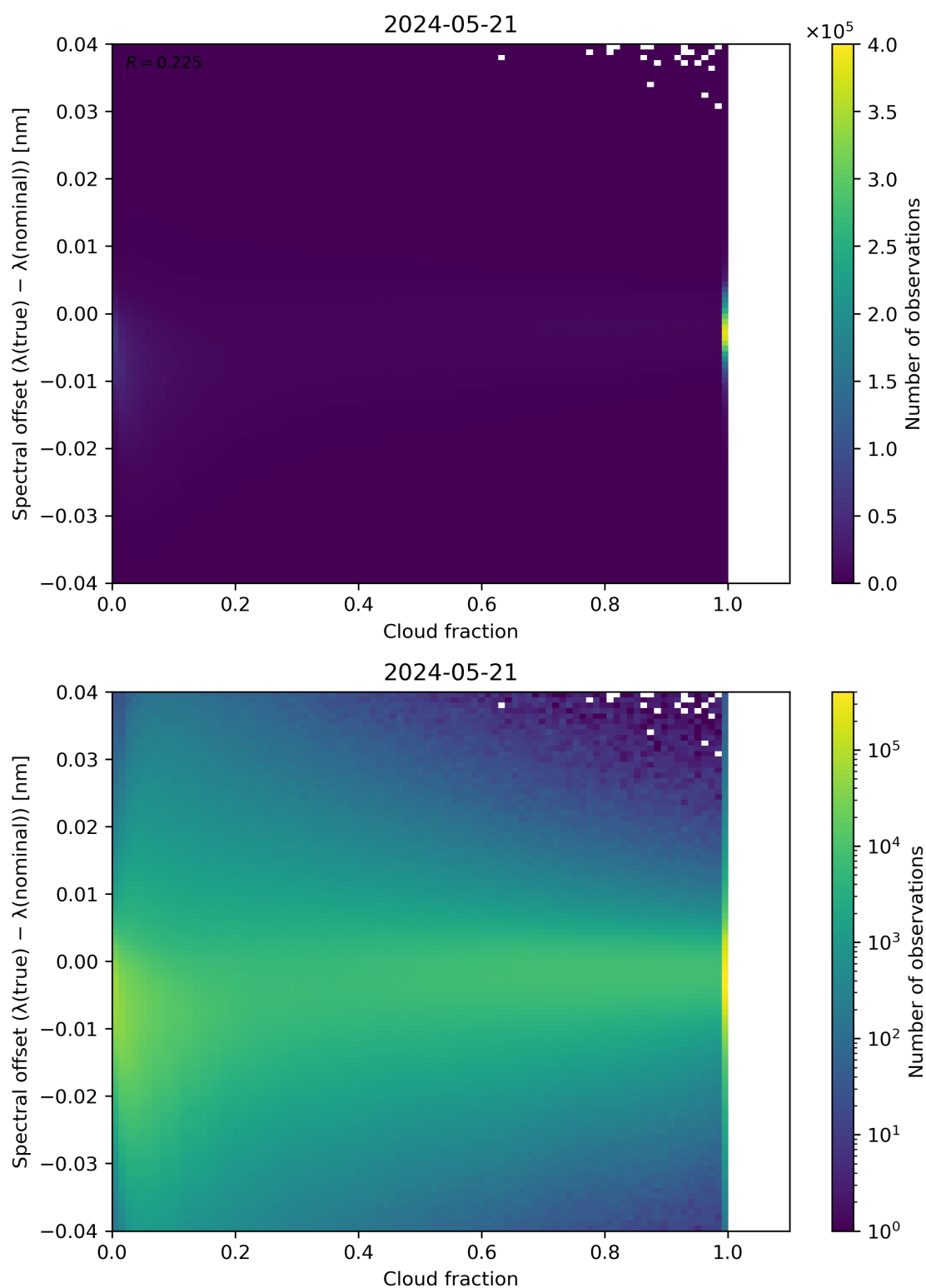
Figure 76: Scatter density plot of “Cloud fraction” against “Spectral offset ( \lambda(\text{true}) - \lambda(\text{nominal}) )” for 2024-05-20 to 2024-05-22.
