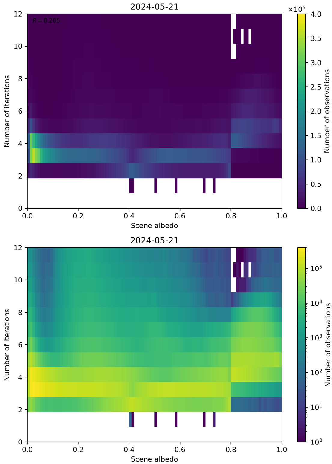
Figure 105: Scatter density plot of “Scene albedo” against “Number of iterations” for 2024-05-20 to 2024-05-22.
