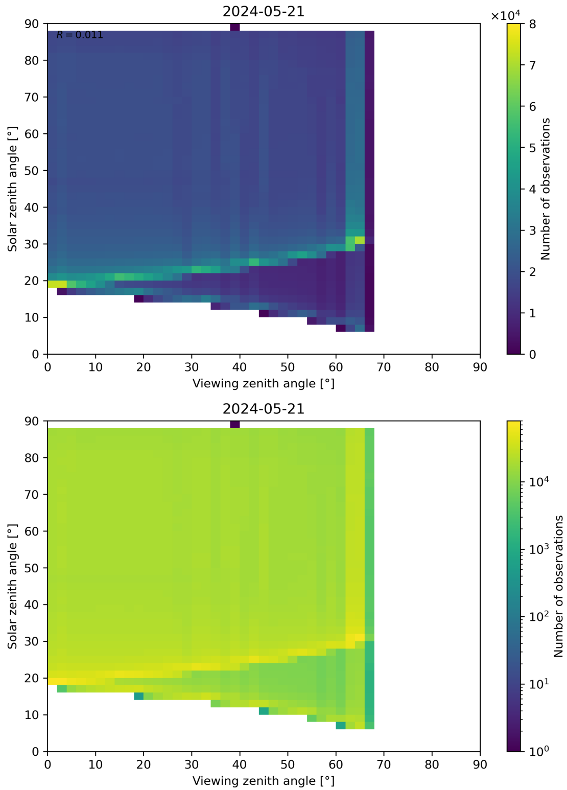
Figure 127: Scatter density plot of “Viewing zenith angle” against “Solar zenith angle” for 2024-05-20 to 2024-05-22.
