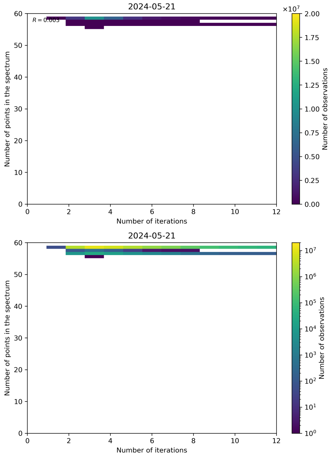
Figure 99: Scatter density plot of “Number of iterations” against “Number of points in the spectrum” for 2024-05-20 to 2024-05-22.
