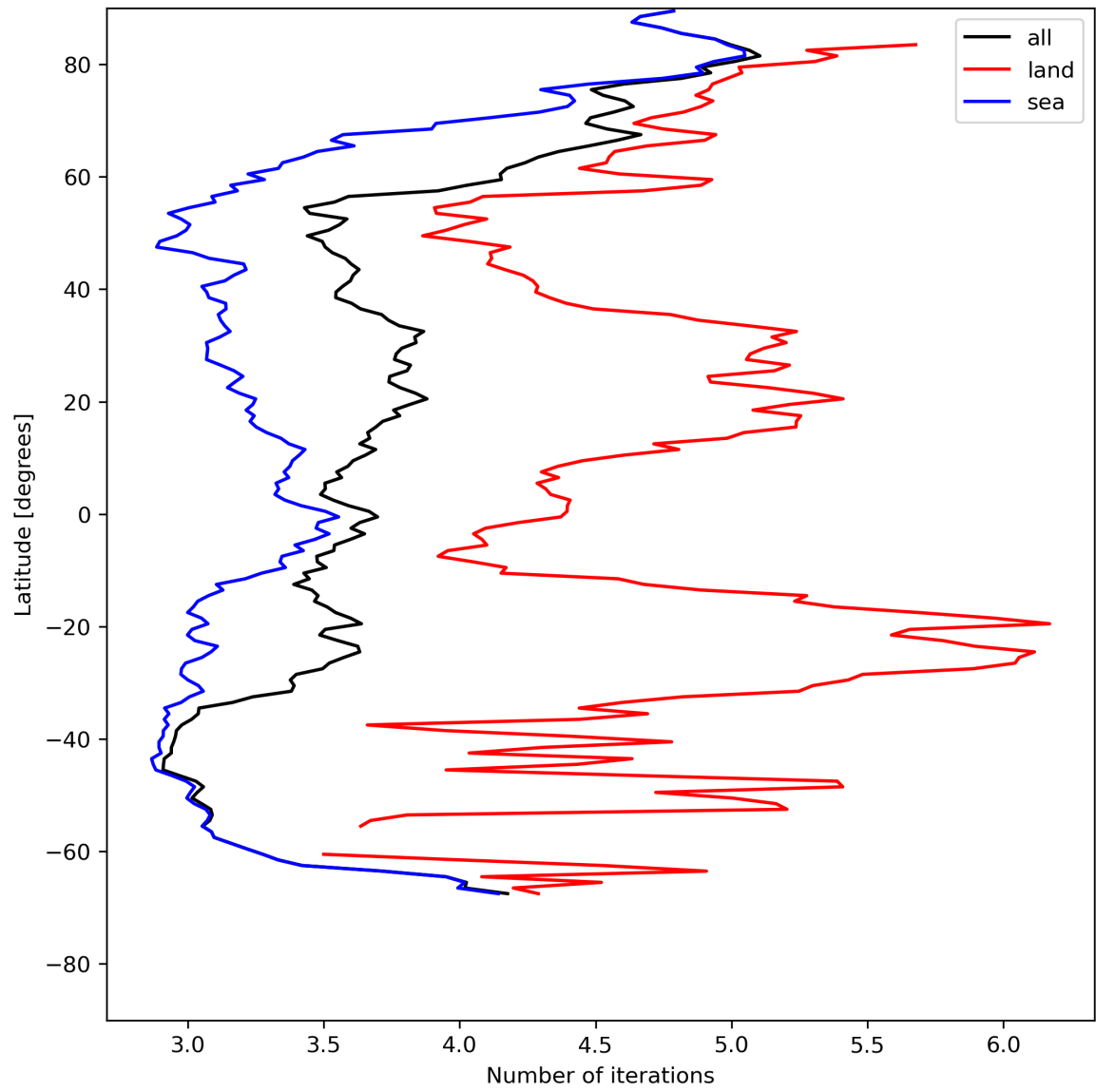
Figure 22: Zonal average of “Number of iterations” for 2024-05-20 to 2024-05-22.
