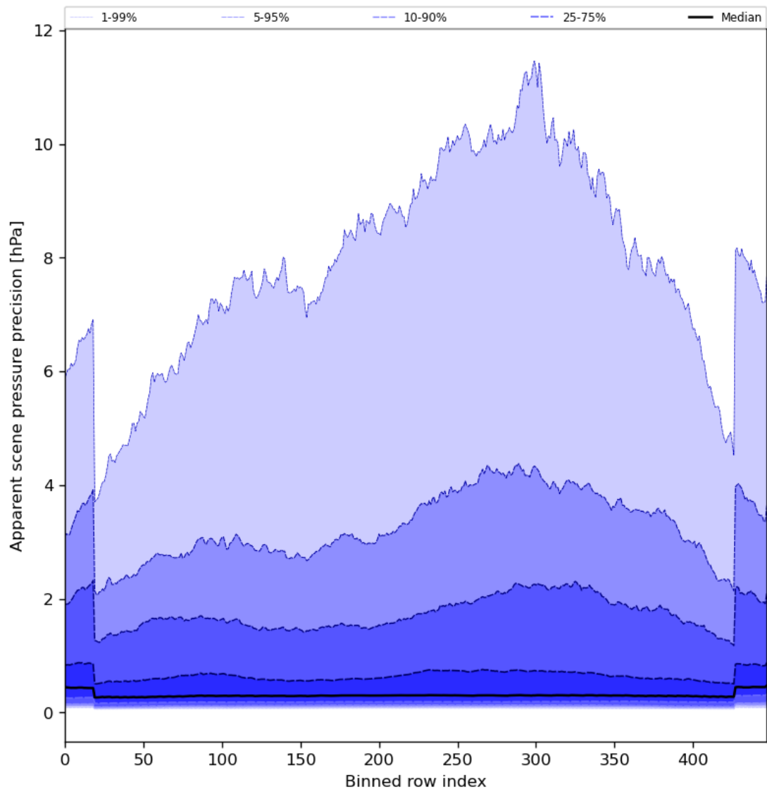
Figure 54: Along track statistics of “Apparent scene pressure precision” for 2024-05-20 to 2024-05-22
