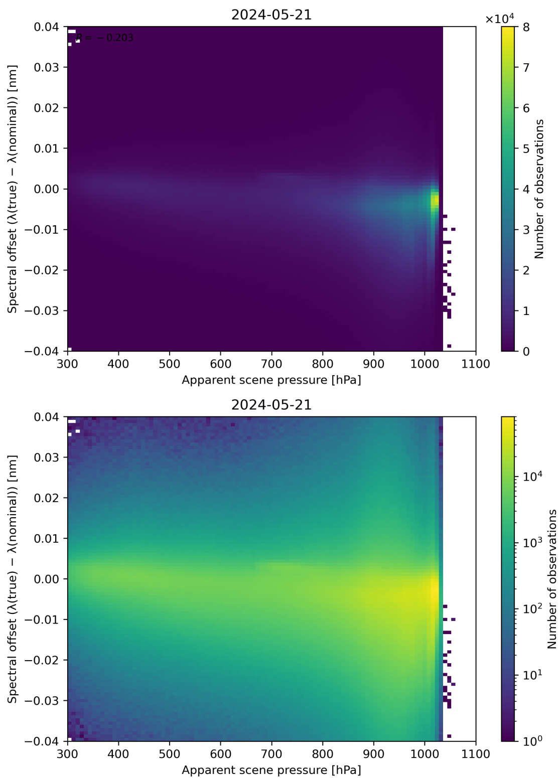
Figure 67: Scatter density plot of “Apparent scene pressure” against “Spectral offset ( \lambda(\text{true}) - \lambda(\text{nominal}) )” for 2024-05-20 to 2024-05-22.
