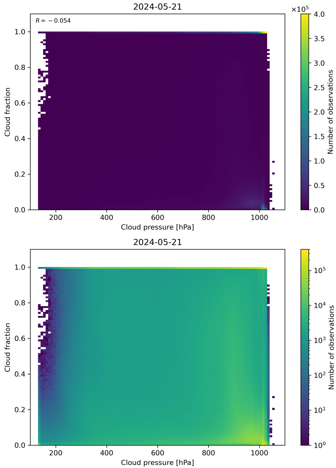
Figure 79: Scatter density plot of “Cloud pressure” against “Cloud fraction” for 2024-05-20 to 2024-05-22.
