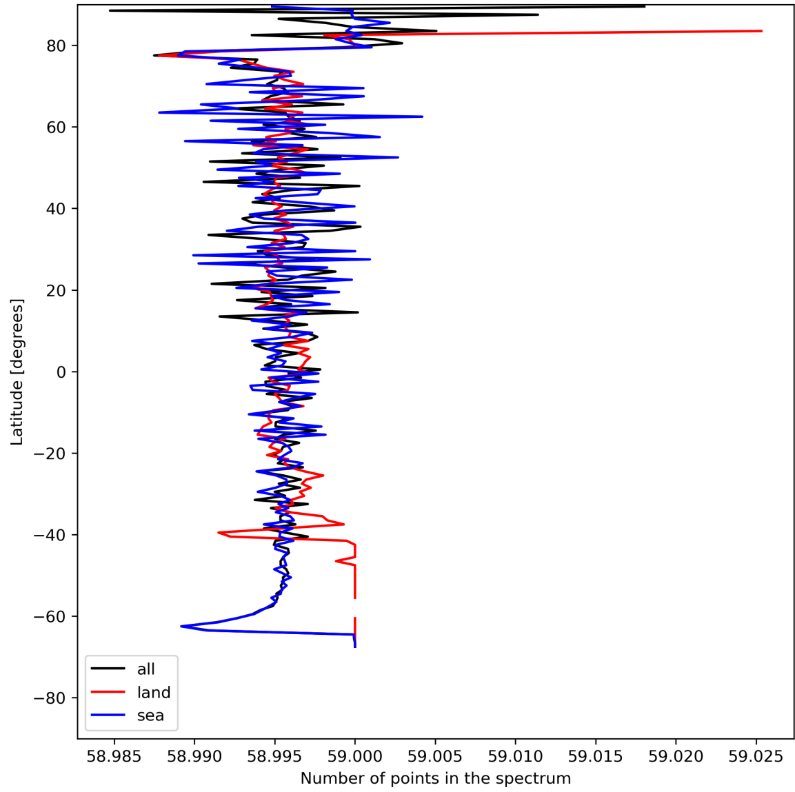
Figure 27: Zonal average of “Number of points in the spectrum” for 2024-05-20 to 2024-05-22.
