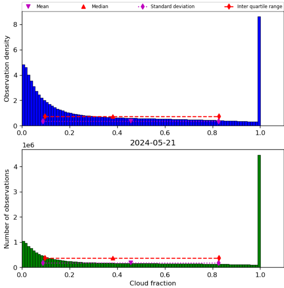
Figure 32: Histogram of “Cloud fraction” for 2024-05-20 to 2024-05-22
