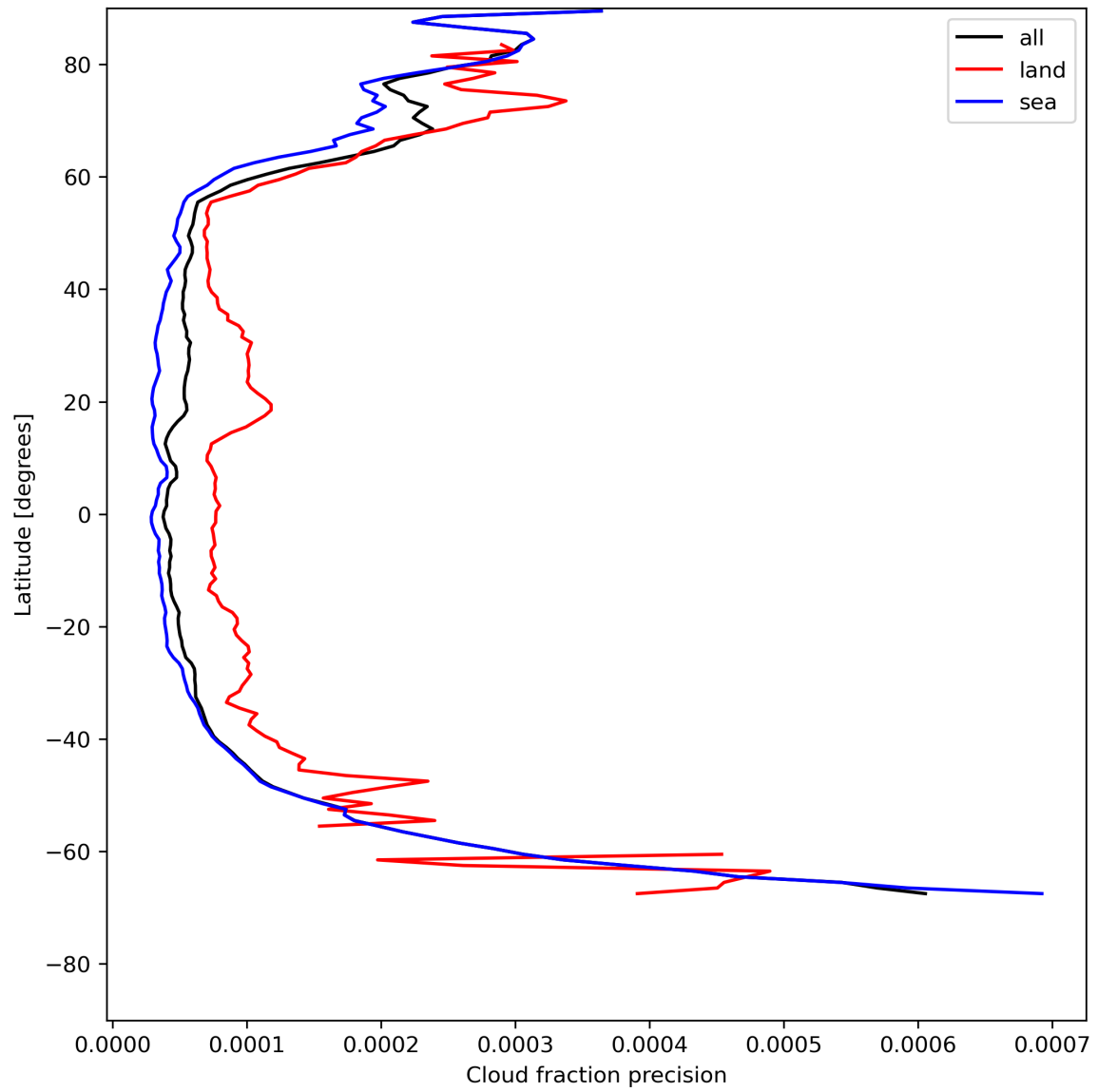
Figure 16: Zonal average of “Cloud fraction precision” for 2024-05-20 to 2024-05-22.
