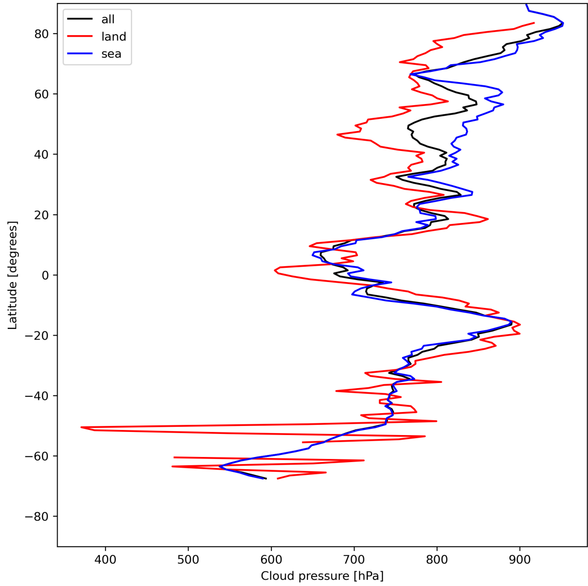
Figure 13: Zonal average of “Cloud pressure” for 2024-05-20 to 2024-05-22.
