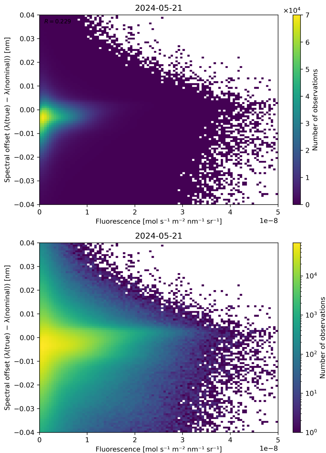
Figure 87: Scatter density plot of “Fluorescence” against “Spectral offset ( \lambda(\text{true}) - \lambda(\text{nominal}) )” for 2024-05-20 to 2024-05-22.
