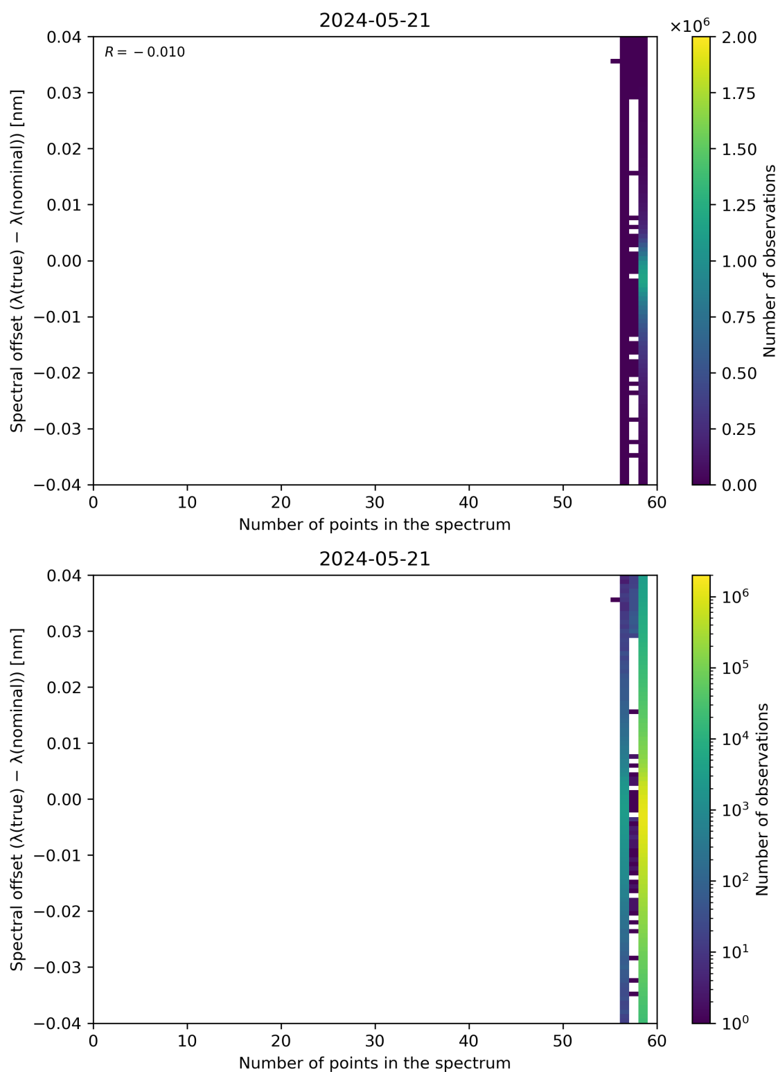
Figure 101: Scatter density plot of “Number of points in the spectrum” against “Spectral offset ( \lambda(\text{true}) - \lambda(\text{nominal}) )” for 2024-05-20 to 2024-05-22.
