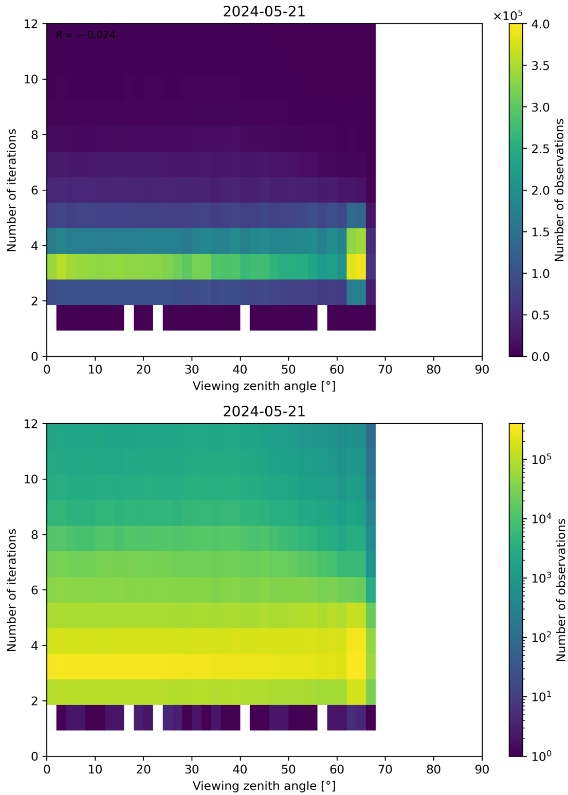
Figure 124: Scatter density plot of “Viewing zenith angle” against “Number of iterations” for 2024-05-20 to 2024-05-22.
