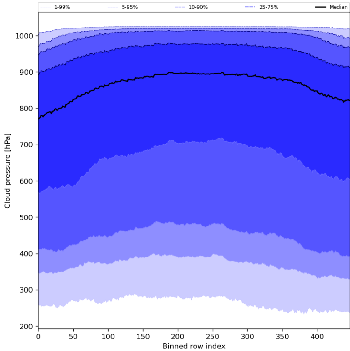
Figure 47: Along track statistics of “Cloud pressure” for 2024-05-20 to 2024-05-22
