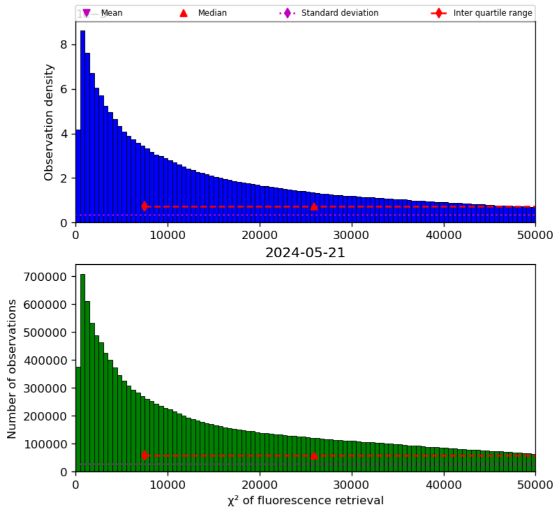
Figure 42: Histogram of “ \chi^2 of fluorescence retrieval” for 2024-05-20 to 2024-05-22
