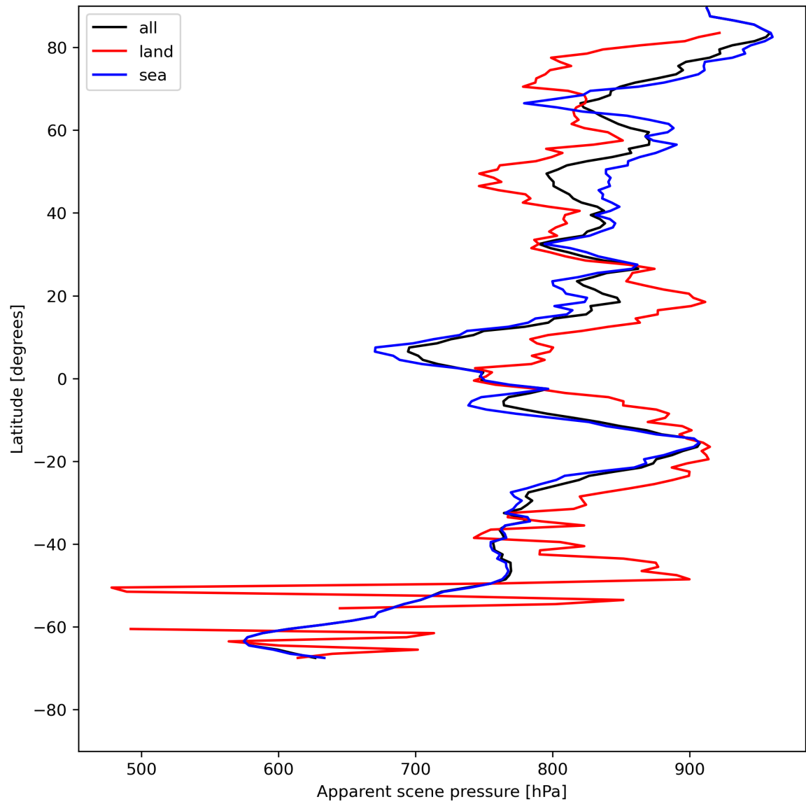
Figure 19: Zonal average of “Apparent scene pressure” for 2024-05-20 to 2024-05-22.
