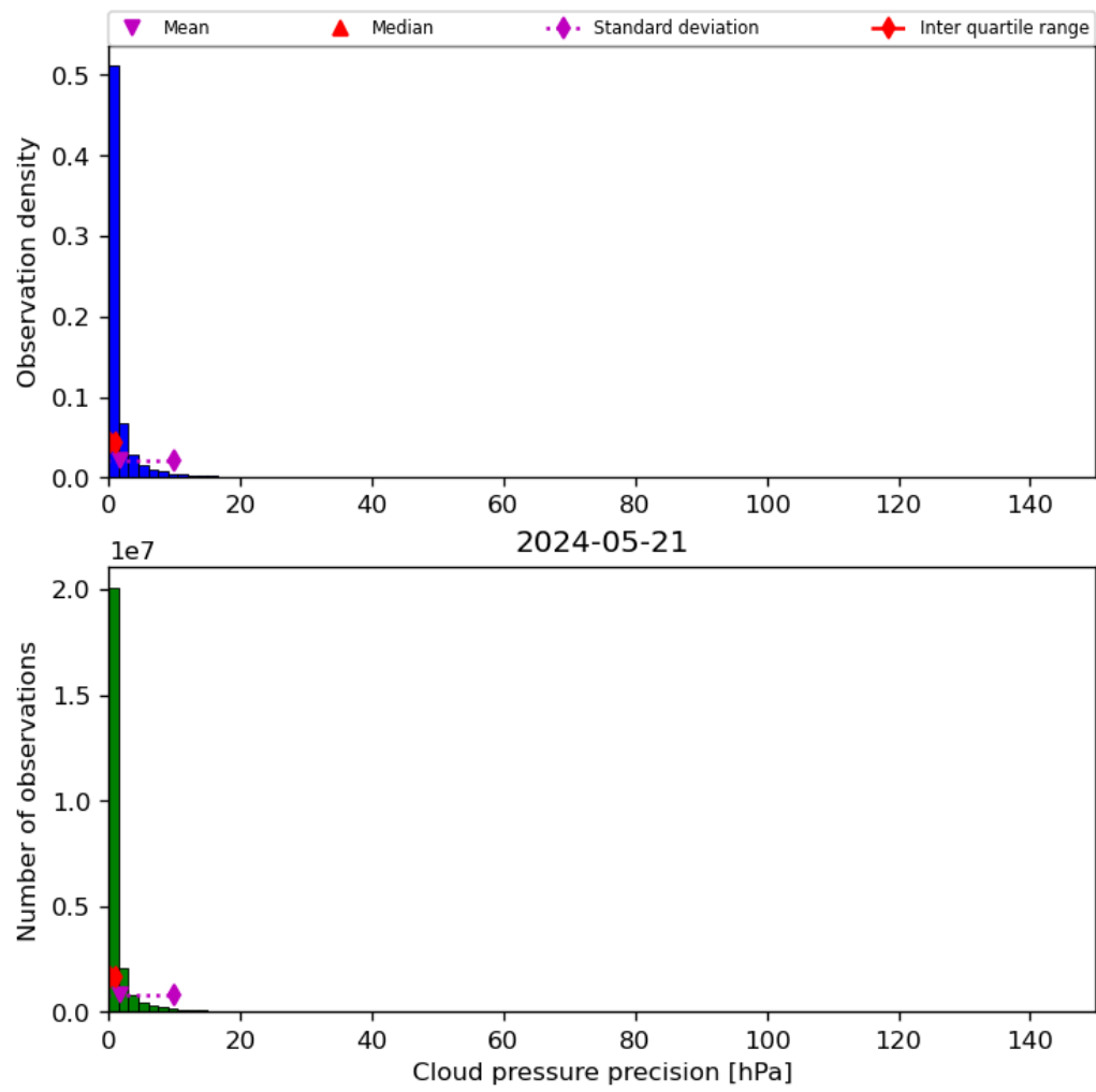
Figure 31: Histogram of “Cloud pressure precision” for 2024-05-20 to 2024-05-22
