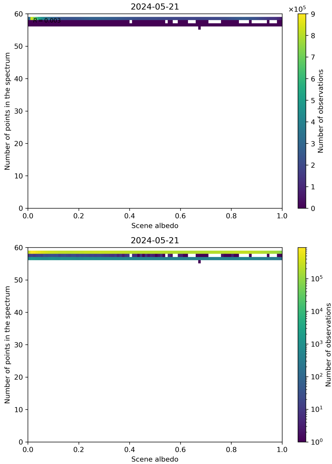
Figure 106: Scatter density plot of “Scene albedo” against “Number of points in the spectrum” for 2024-05-20 to 2024-05-22.
