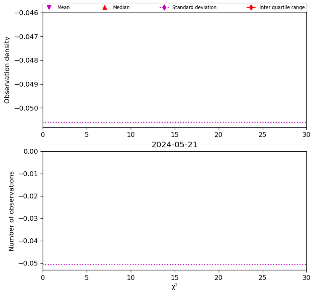
Figure 38: Histogram of “ \chi^2 ” for 2024-05-20 to 2024-05-22
