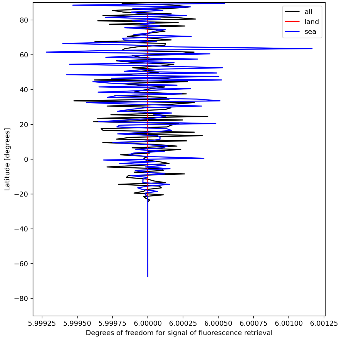
Figure 26: Zonal average of “Degrees of freedom for signal of fluorescence retrieval” for 2024-05-20 to 2024-05-22.
