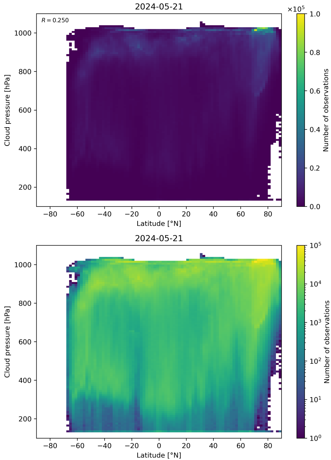
Figure 91: Scatter density plot of “Latitude” against “Cloud pressure” for 2024-05-20 to 2024-05-22.
