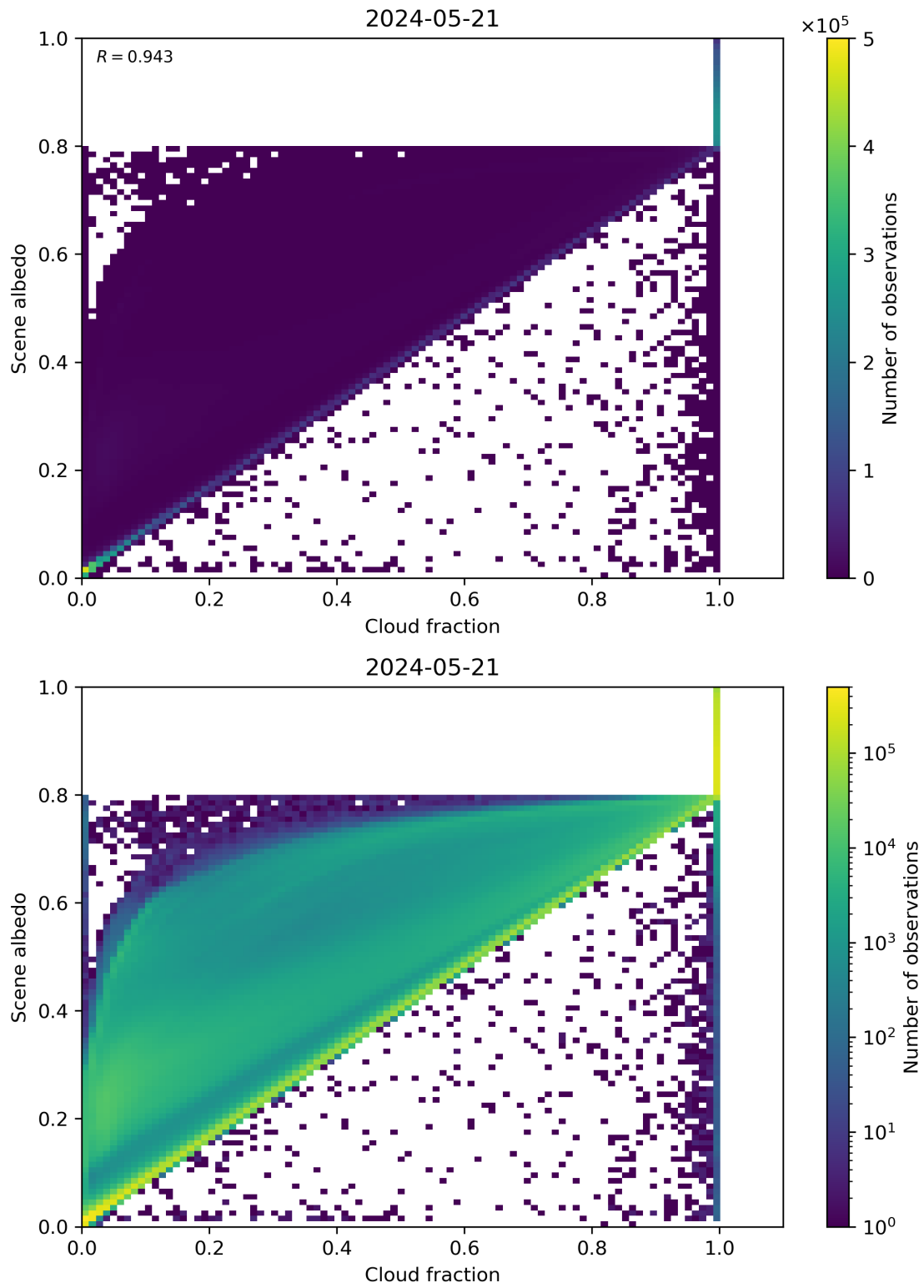
Figure 75: Scatter density plot of “Cloud fraction” against “Scene albedo” for 2024-05-20 to 2024-05-22.
