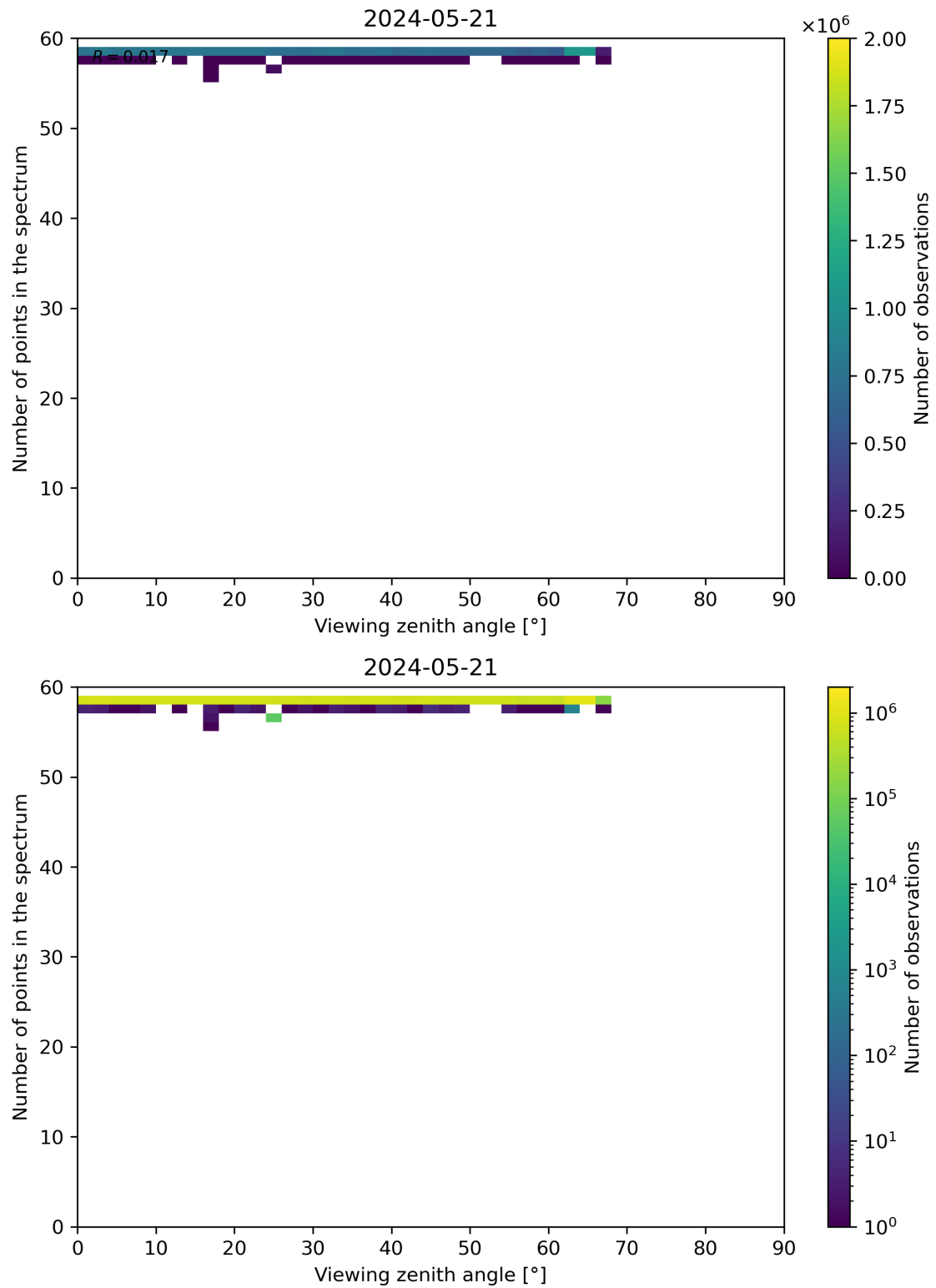
Figure 125: Scatter density plot of “Viewing zenith angle” against “Number of points in the spectrum” for 2024-05-20 to 2024-05-22.
