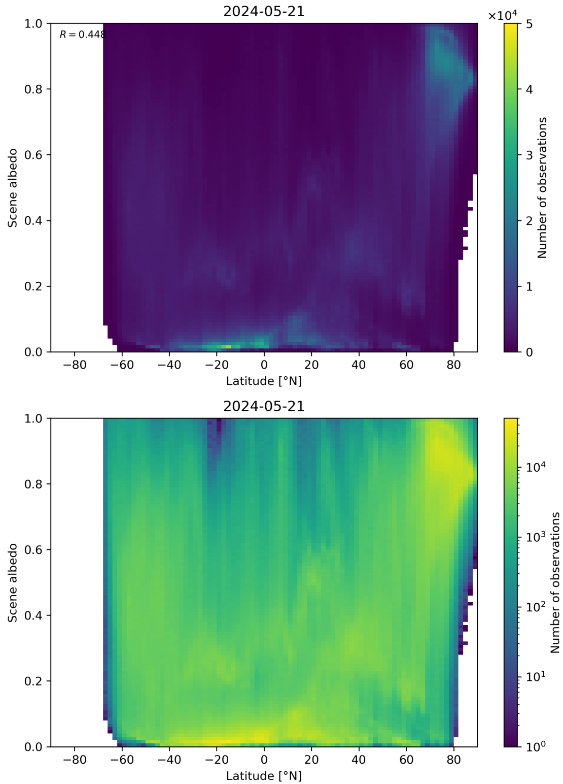
Figure 95: Scatter density plot of “Latitude” against “Scene albedo” for 2024-05-20 to 2024-05-22.
