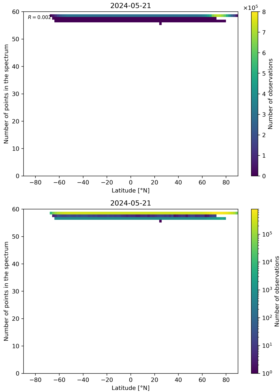
Figure 94: Scatter density plot of “Latitude” against “Number of points in the spectrum” for 2024-05-20 to 2024-05-22.
