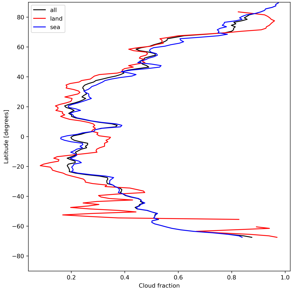
Figure 15: Zonal average of “Cloud fraction” for 2024-05-20 to 2024-05-22.
