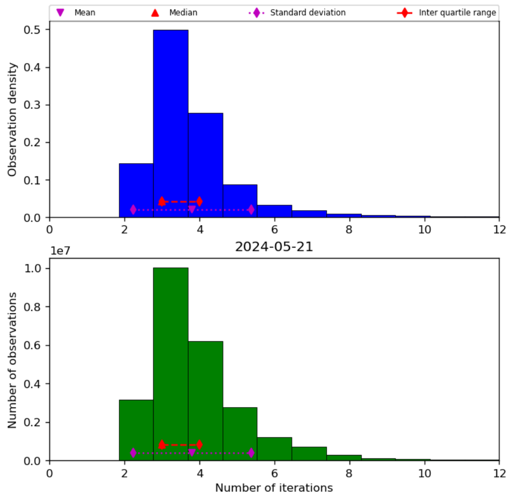
Figure 39: Histogram of “Number of iterations” for 2024-05-20 to 2024-05-22
