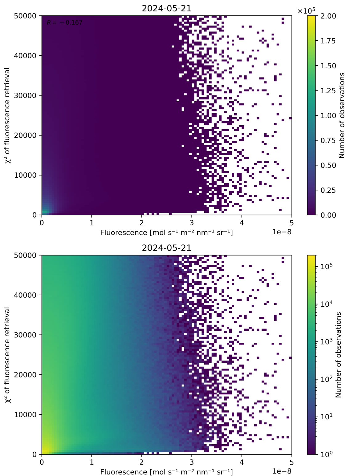
Figure 85: Scatter density plot of “Fluorescence” against “ \chi^2 of fluorescence retrieval” for 2024-05-20 to 2024-05-22.
