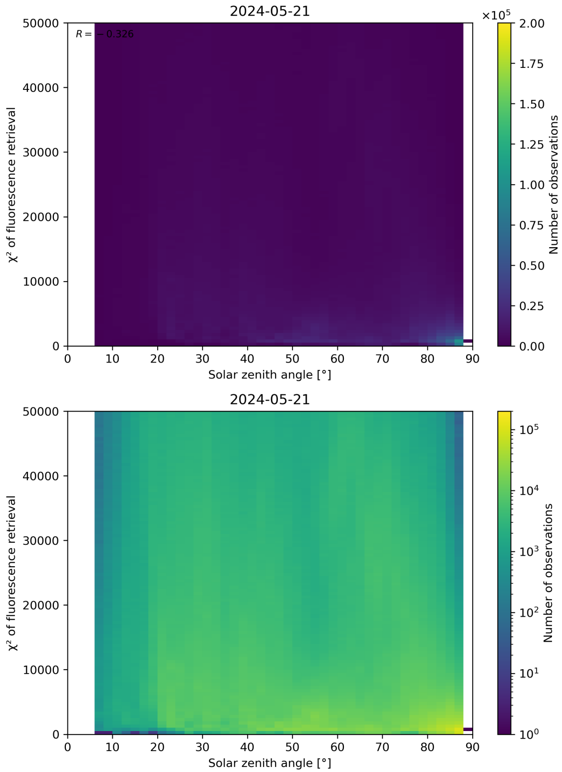
Figure 109: Scatter density plot of “Solar zenith angle” against “ \chi^2 of fluorescence retrieval” for 2024-05-20 to 2024-05-22.
