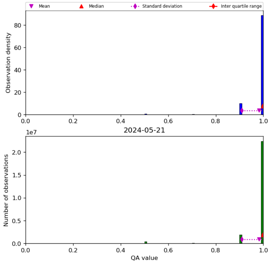
Figure 29: Histogram of “QA value” for 2024-05-20 to 2024-05-22
