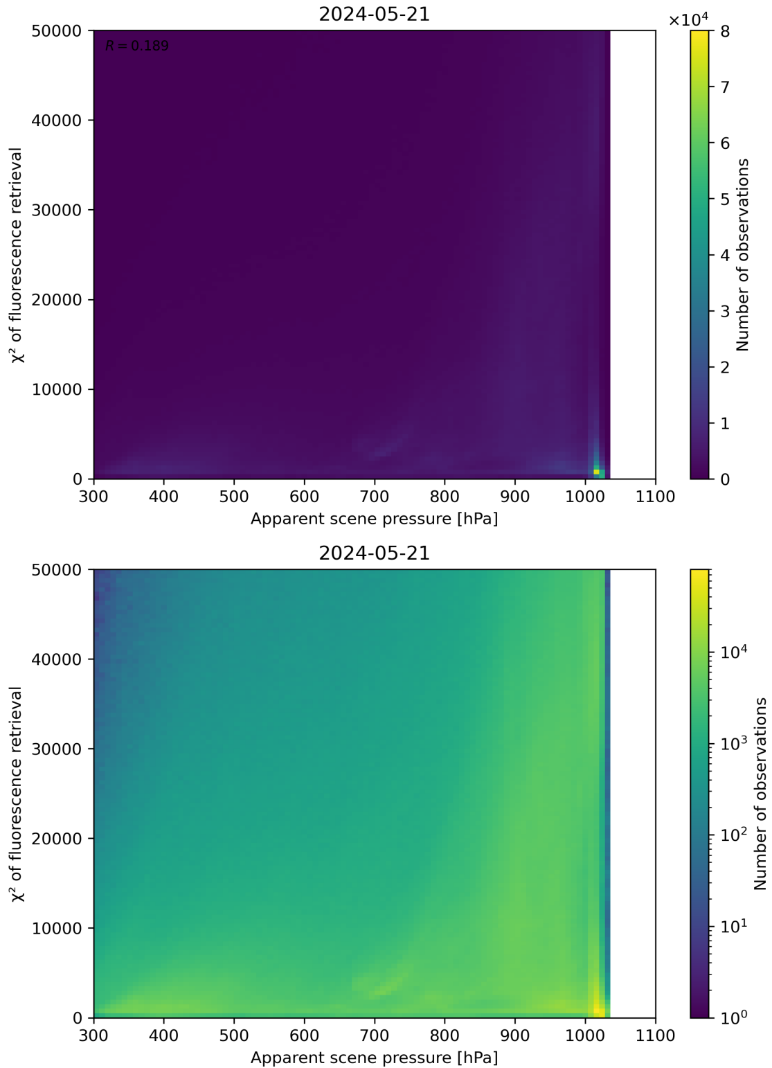
Figure 63: Scatter density plot of “Apparent scene pressure” against “ \chi^2 of fluorescence retrieval” for 2024-05-20 to 2024-05-22.
