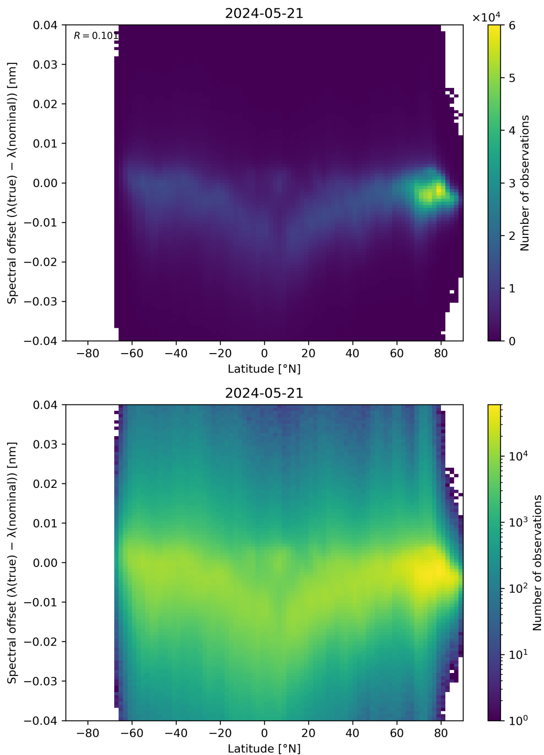
Figure 96: Scatter density plot of “Latitude” against “Spectral offset ( \lambda(\text{true}) - \lambda(\text{nominal}) )” for 2024-05-20 to 2024-05-22.
