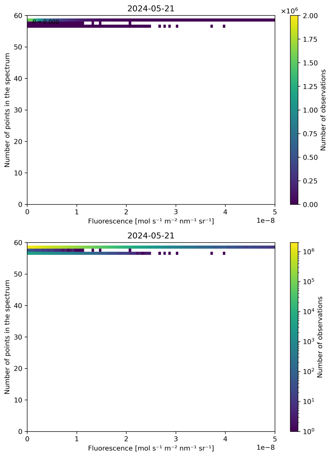
Figure 86: Scatter density plot of “Fluorescence” against “Number of points in the spectrum” for 2024-05-20 to 2024-05-22.
