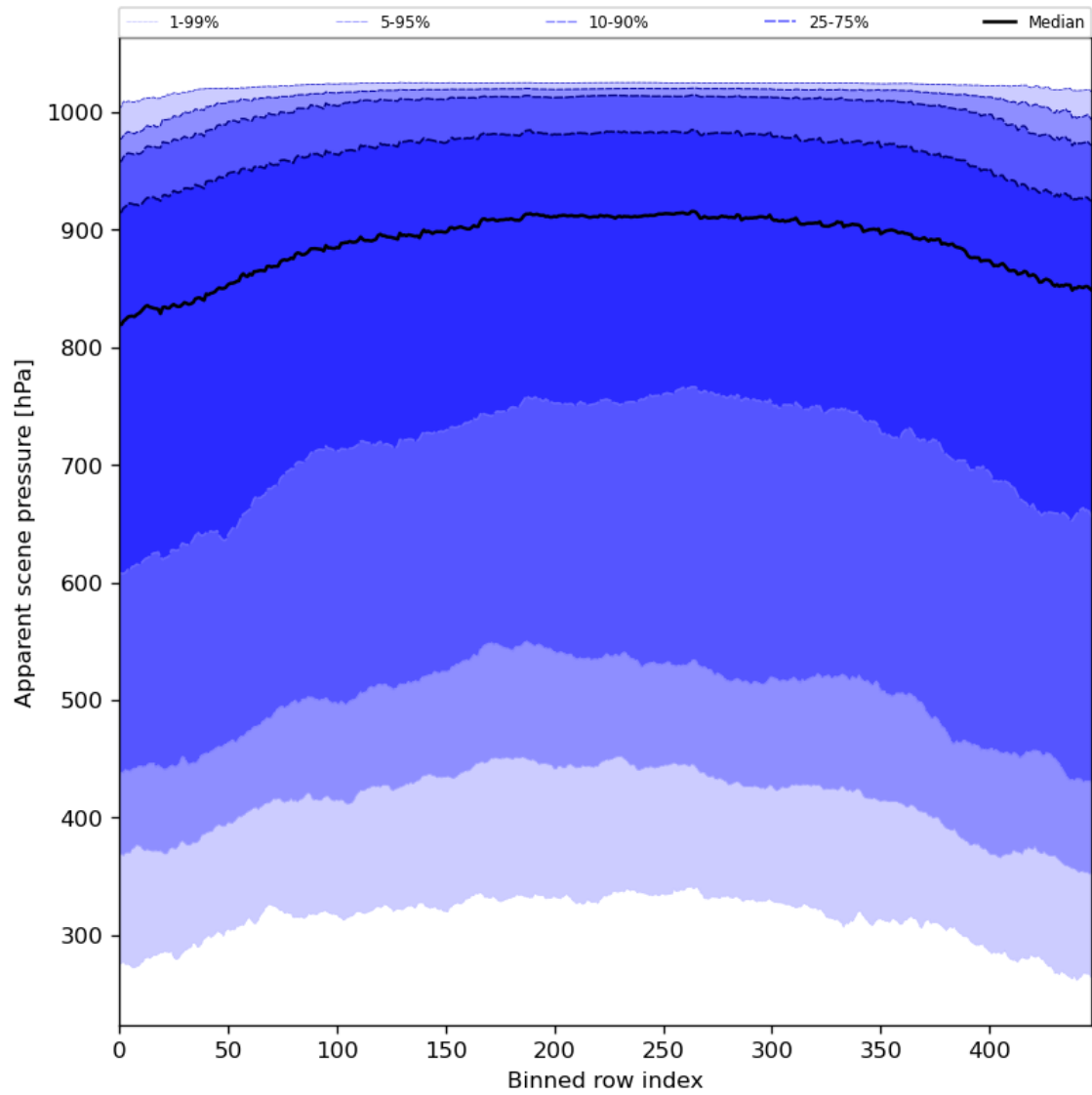
Figure 53: Along track statistics of “Apparent scene pressure” for 2024-05-20 to 2024-05-22
