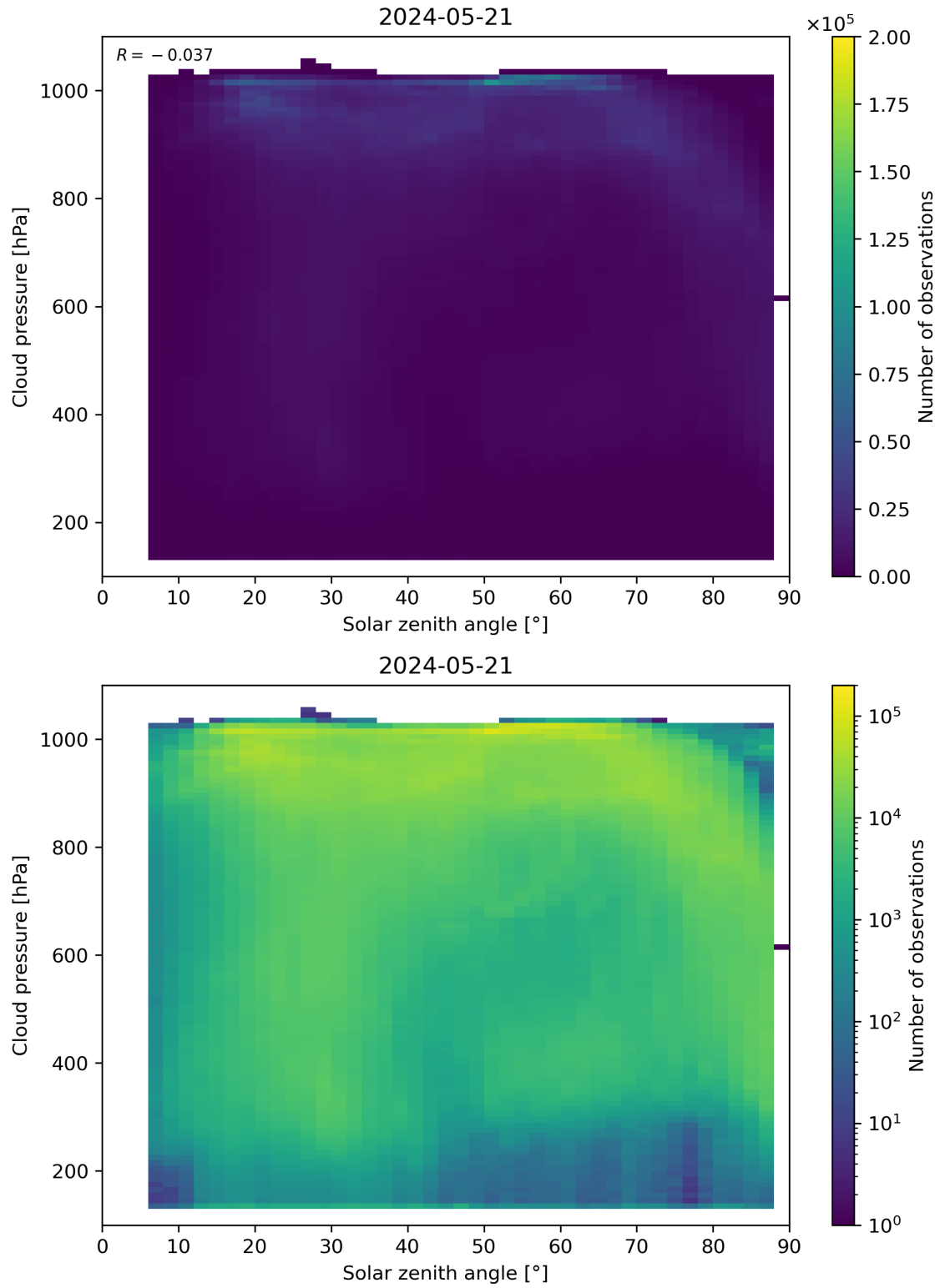
Figure 111: Scatter density plot of “Solar zenith angle” against “Cloud pressure” for 2024-05-20 to 2024-05-22.
