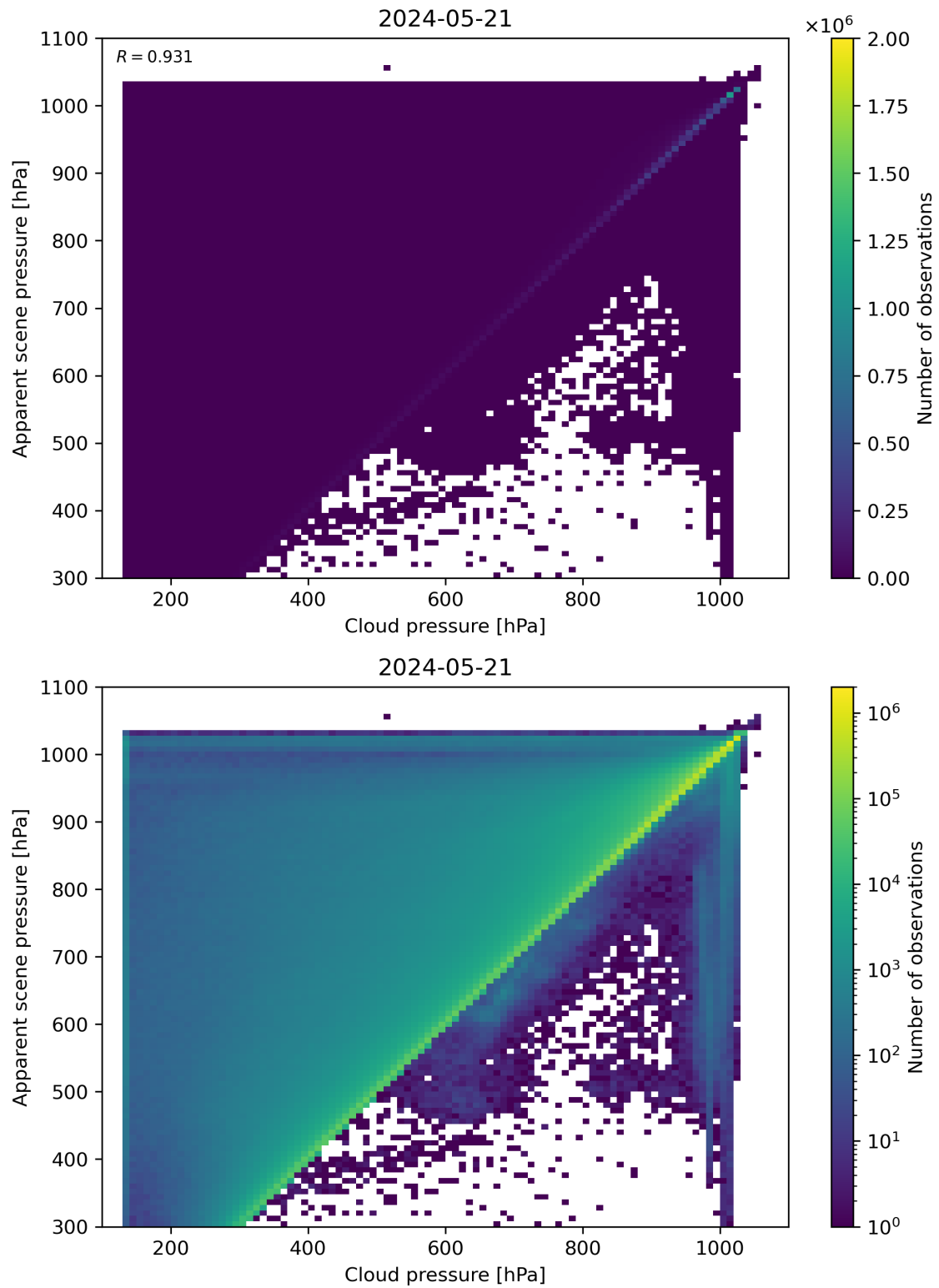
Figure 77: Scatter density plot of “Cloud pressure” against “Apparent scene pressure” for 2024-05-20 to 2024-05-22.
