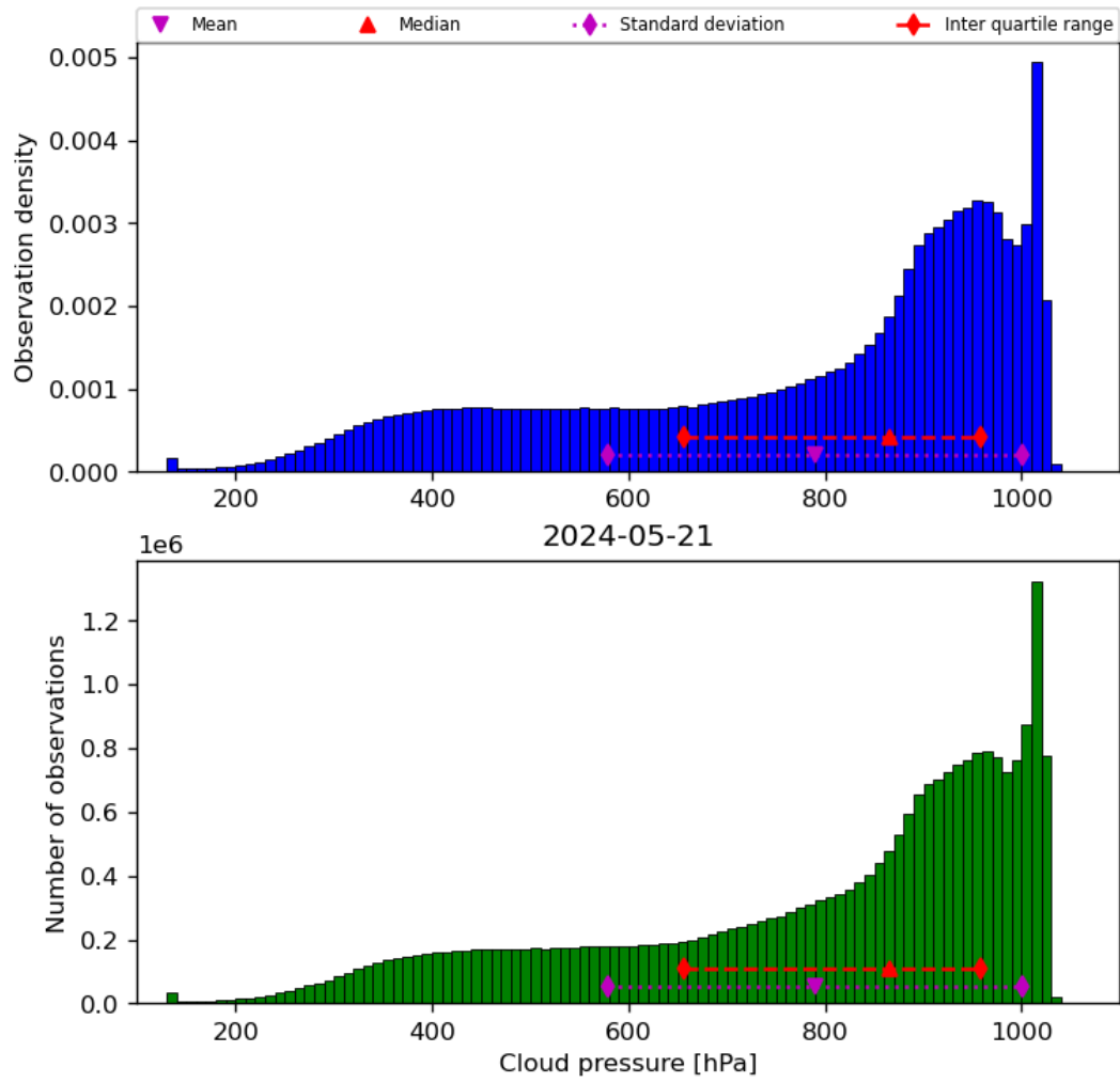
Figure 30: Histogram of “Cloud pressure” for 2024-05-20 to 2024-05-22
