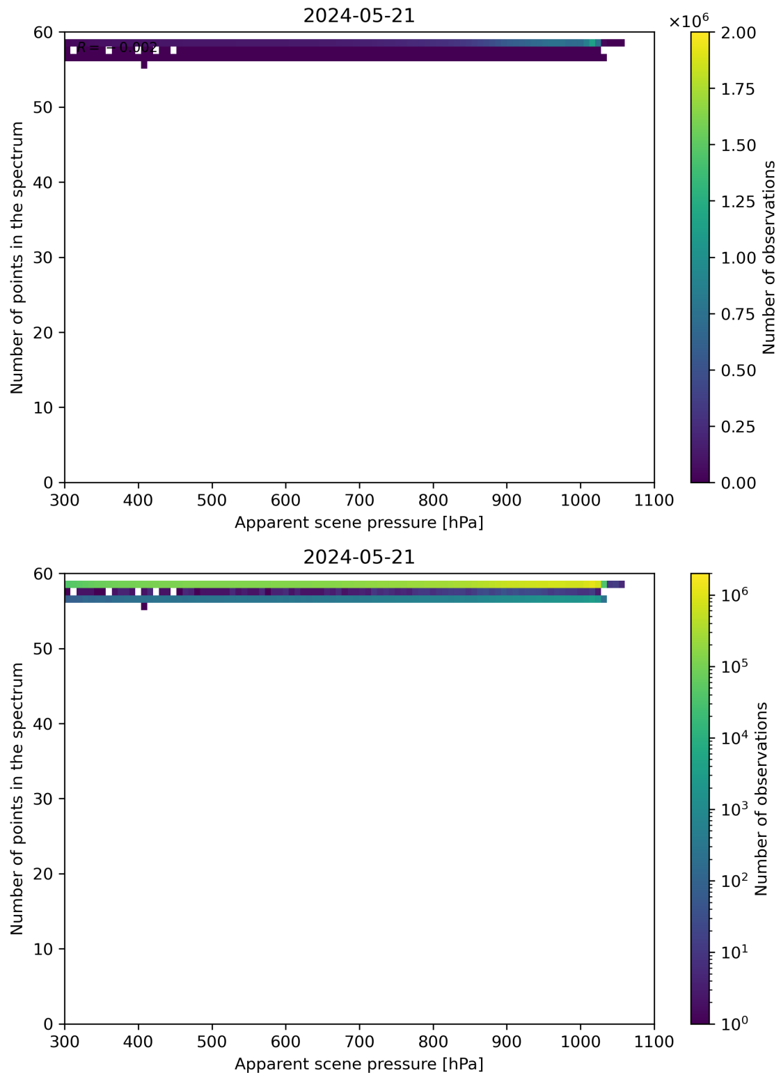
Figure 66: Scatter density plot of “Apparent scene pressure” against “Number of points in the spectrum” for 2024-05-20 to 2024-05-22.
