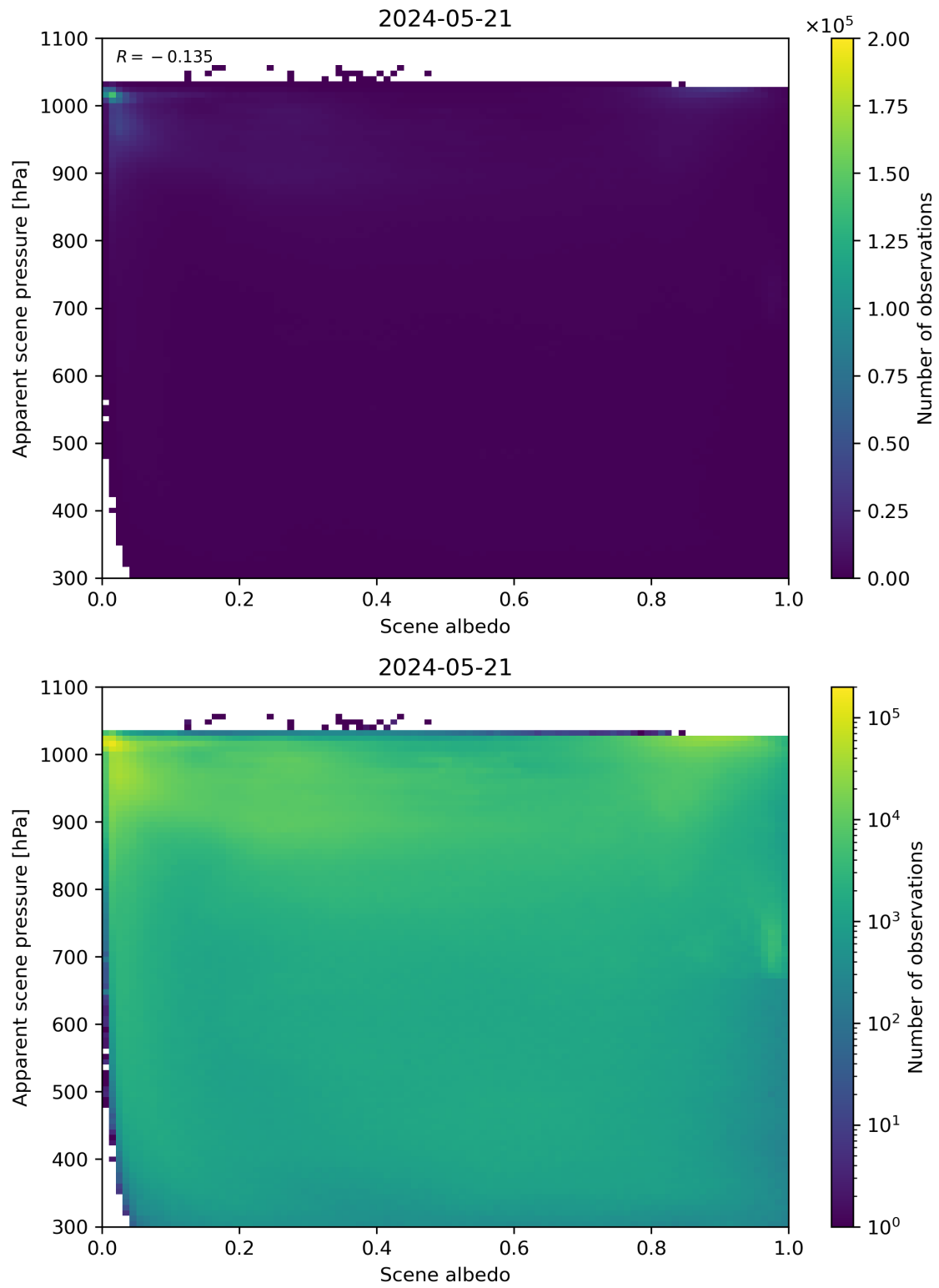
Figure 102: Scatter density plot of “Scene albedo” against “Apparent scene pressure” for 2024-05-20 to 2024-05-22.
