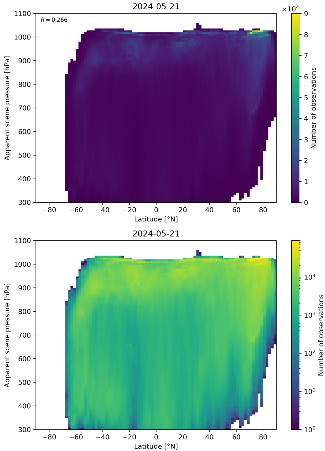
Figure 88: Scatter density plot of “Latitude” against “Apparent scene pressure” for 2024-05-20 to 2024-05-22.
