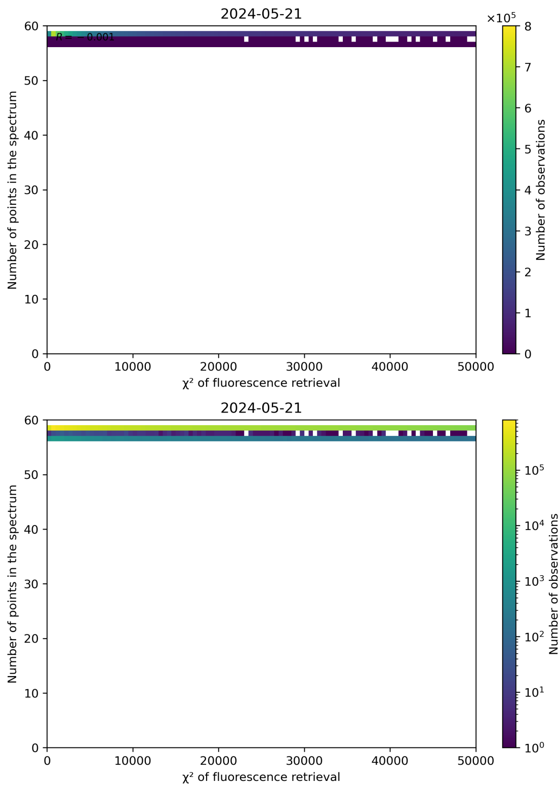
Figure 68: Scatter density plot of " \chi^2 of fluorescence retrieval" against "Number of points in the spectrum" for 2024-05-20 to 2024-05-22.
