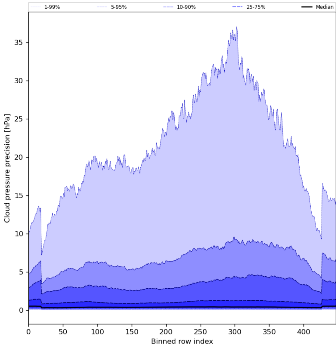
Figure 48: Along track statistics of “Cloud pressure precision” for 2024-05-20 to 2024-05-22
