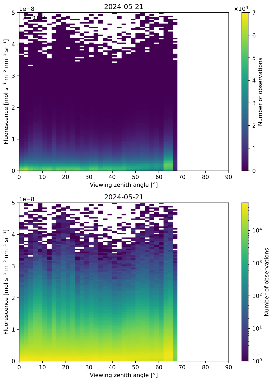
Figure 122: Scatter density plot of “Viewing zenith angle” against “Fluorescence” for 2024-05-20 to 2024-05-22.
