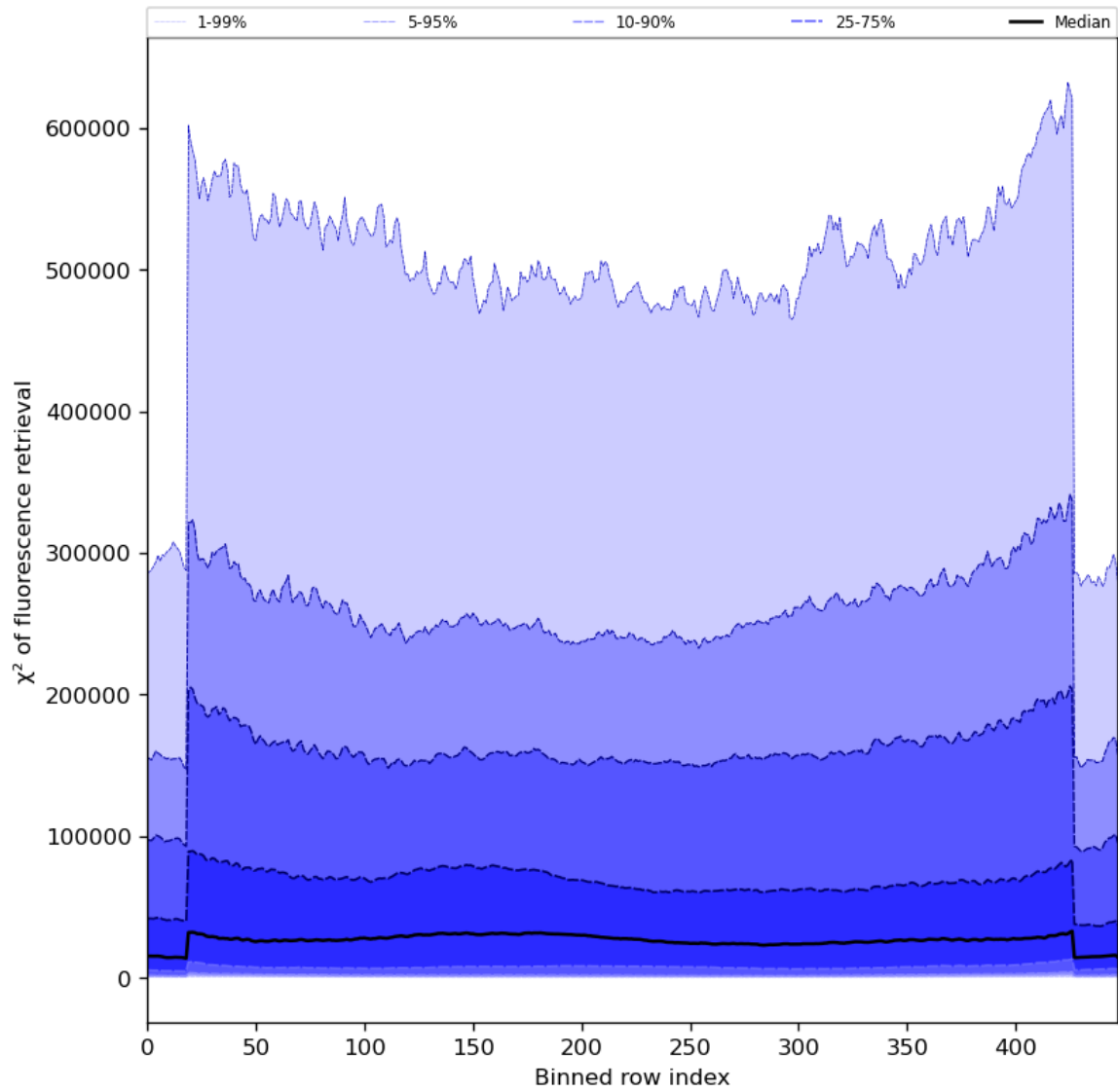
Figure 59: Along track statistics of “ \chi^2 of fluorescence retrieval” for 2024-05-20 to 2024-05-22
