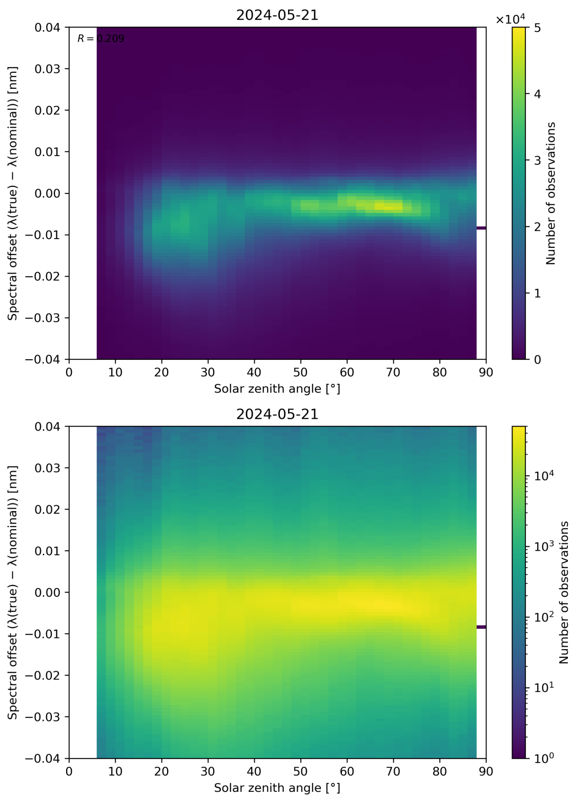
Figure 117: Scatter density plot of “Solar zenith angle” against “Spectral offset ( \lambda(\text{true}) - \lambda(\text{nominal}) )” for 2024-05-20 to 2024-05-22.
