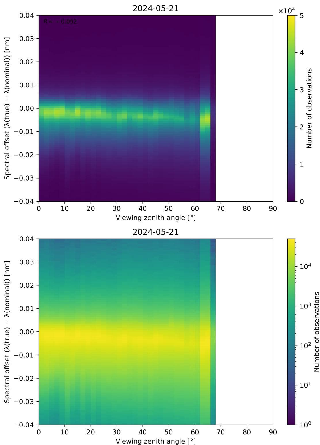
Figure 128: Scatter density plot of “Viewing zenith angle” against “Spectral offset ( \lambda(\text{true}) - \lambda(\text{nominal}) )” for 2024-05-20 to 2024-05-22.
