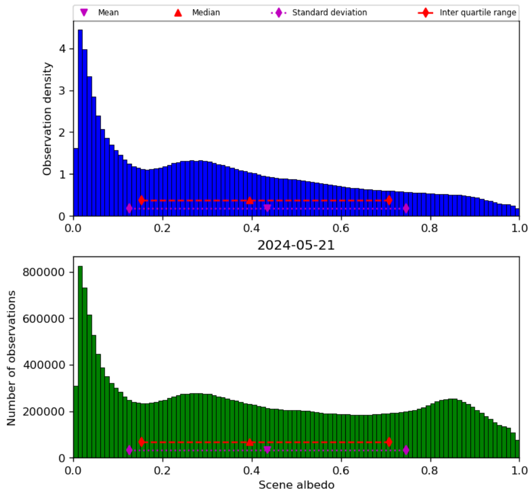
Figure 34: Histogram of “Scene albedo” for 2024-05-20 to 2024-05-22
