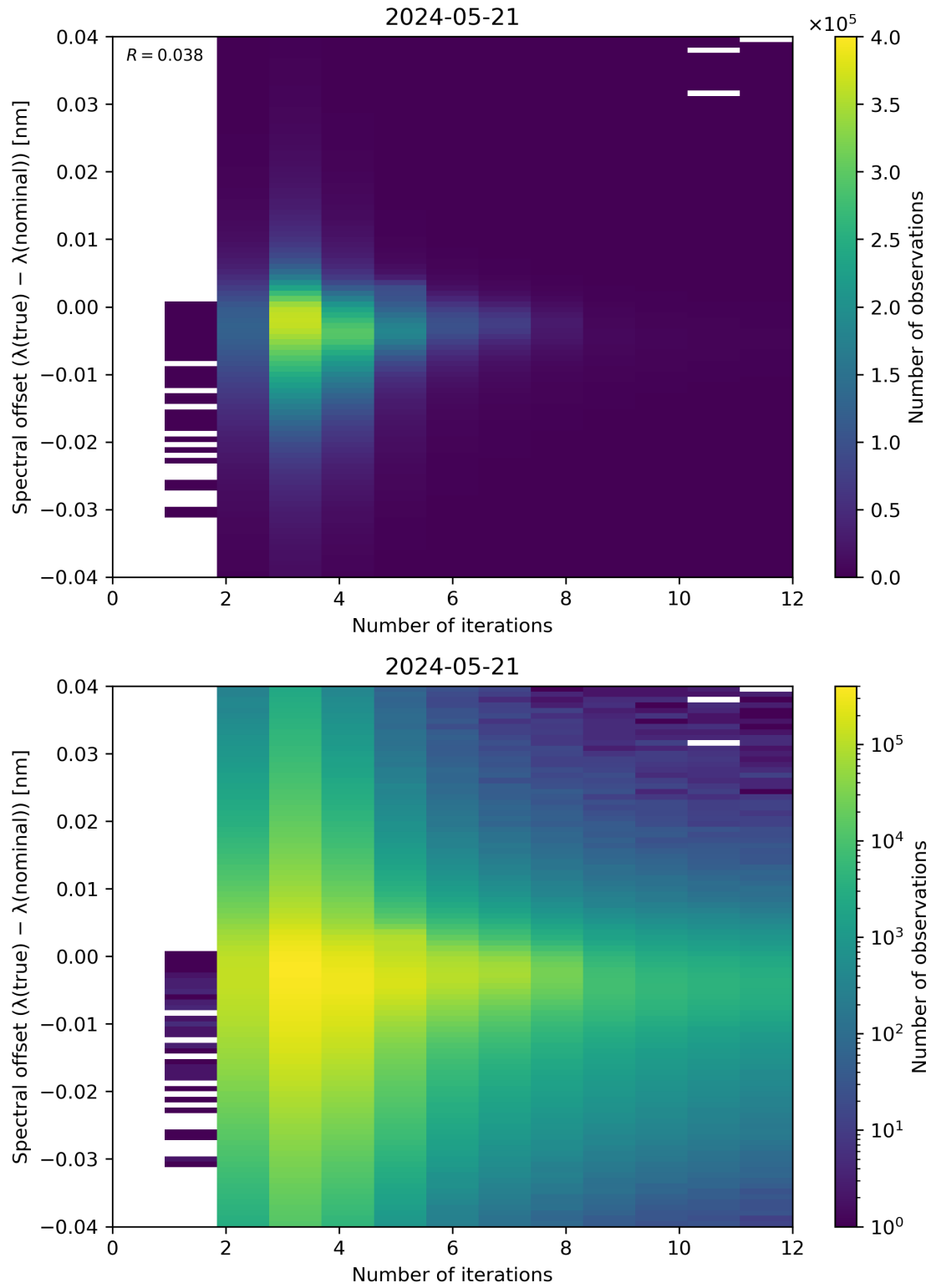
Figure 100: Scatter density plot of “Number of iterations” against “Spectral offset ( \lambda(\text{true}) - \lambda(\text{nominal}) )” for 2024-05-20 to 2024-05-22.
