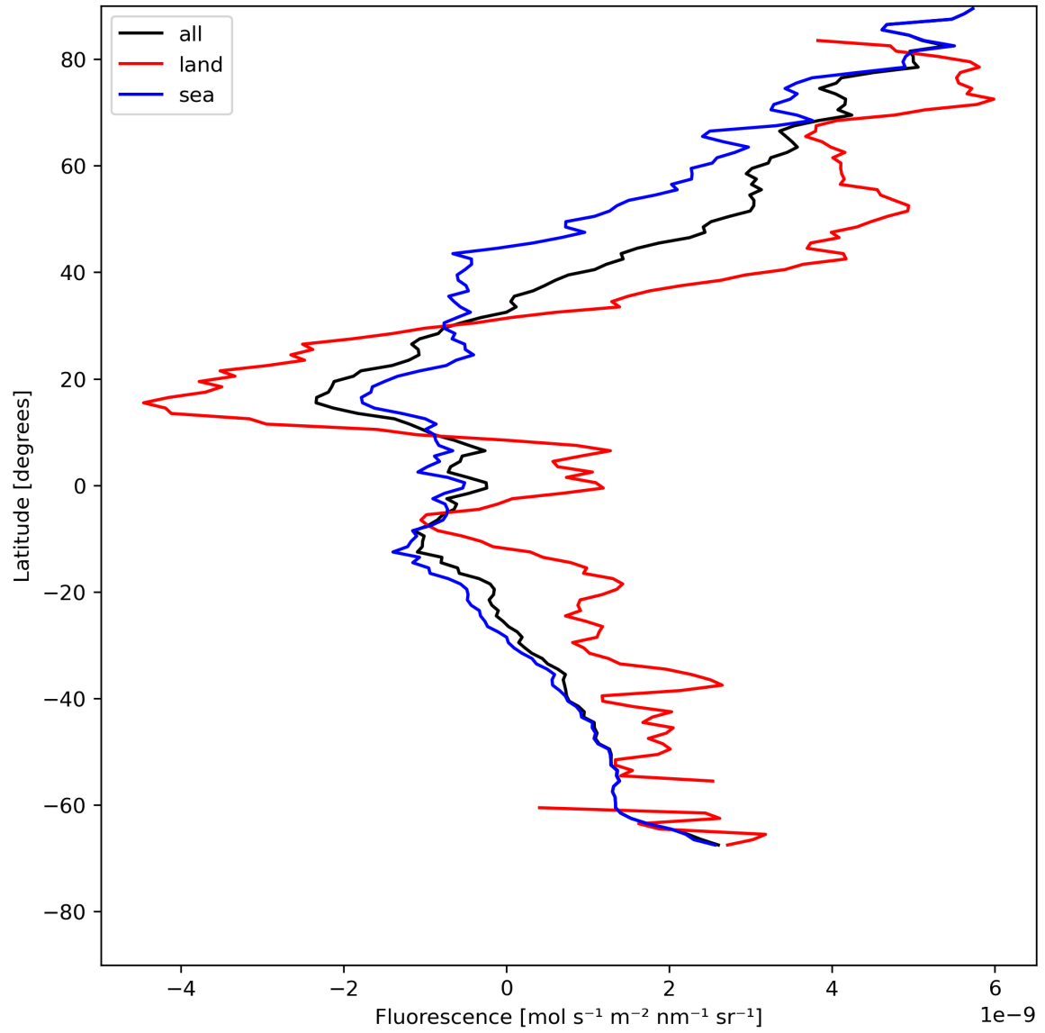
Figure 23: Zonal average of “Fluorescence” for 2024-05-20 to 2024-05-22.
