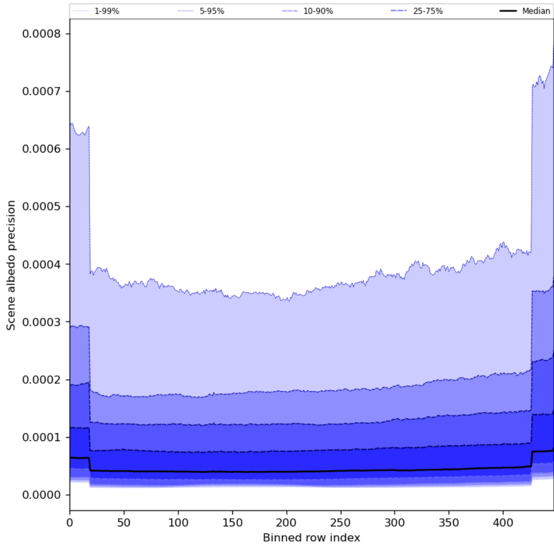
Figure 52: Along track statistics of “Scene albedo precision” for 2024-05-20 to 2024-05-22
