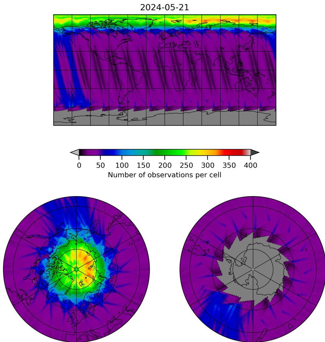
Figure 11: Map of the number of observations for 2024-05-20 to 2024-05-22
