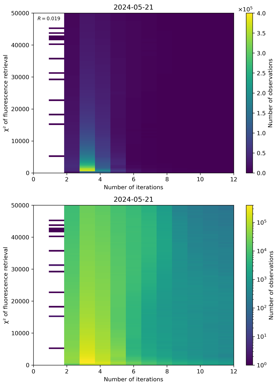
Figure 97: Scatter density plot of “Number of iterations” against “ \chi^2 of fluorescence retrieval” for 2024-05-20 to 2024-05-22.
