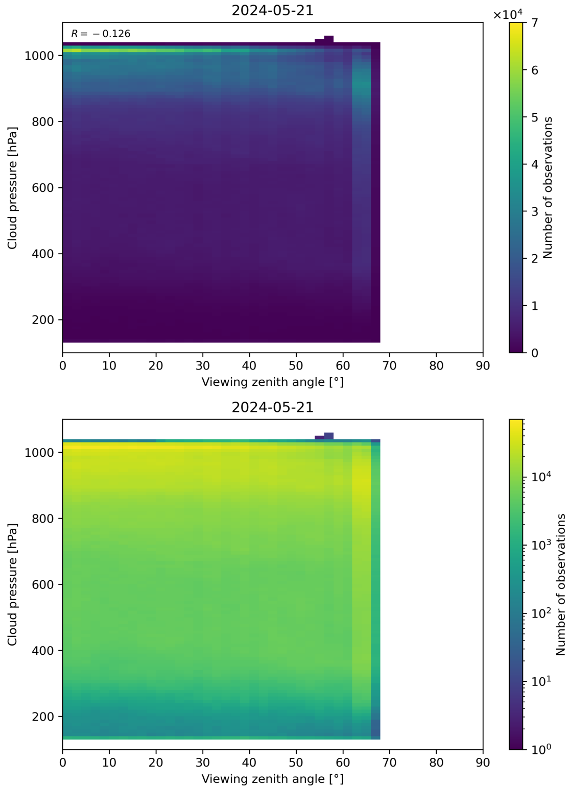
Figure 121: Scatter density plot of “Viewing zenith angle” against “Cloud pressure” for 2024-05-20 to 2024-05-22.
