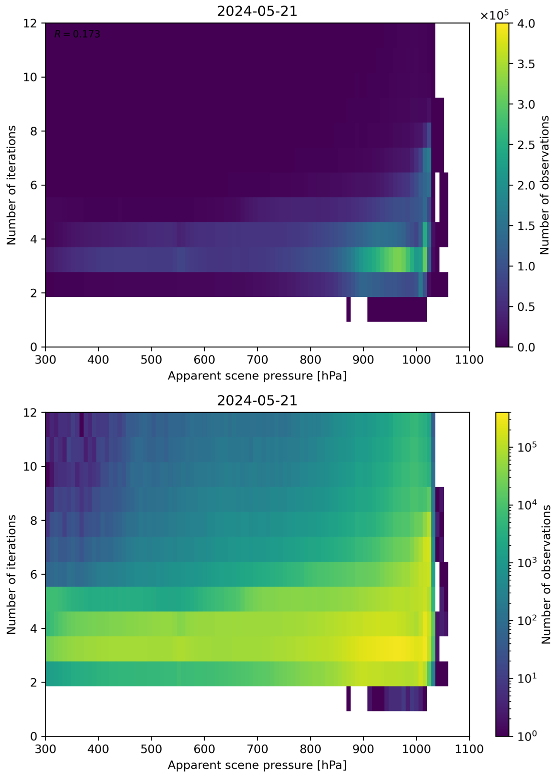
Figure 65: Scatter density plot of “Apparent scene pressure” against “Number of iterations” for 2024-05-20 to 2024-05-22.
