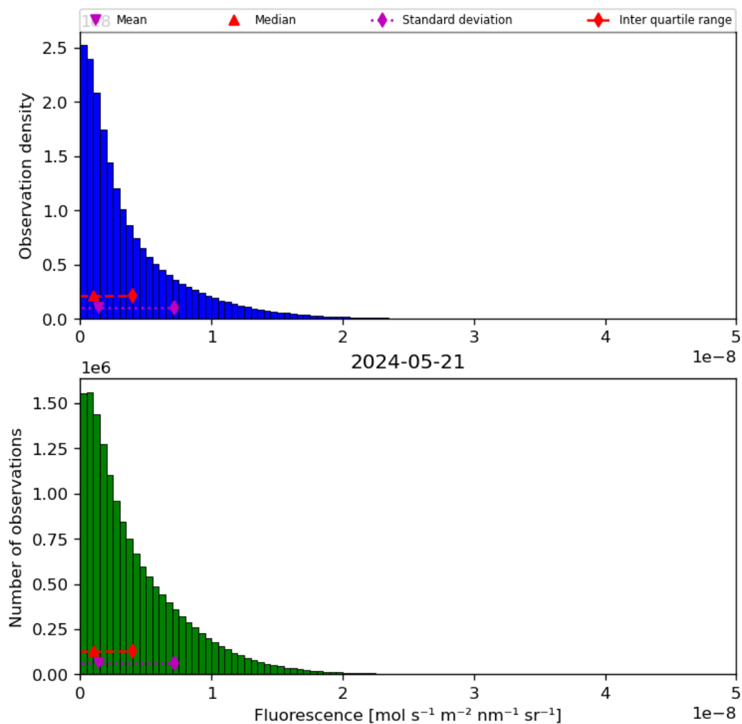
Figure 40: Histogram of “Fluorescence” for 2024-05-20 to 2024-05-22
