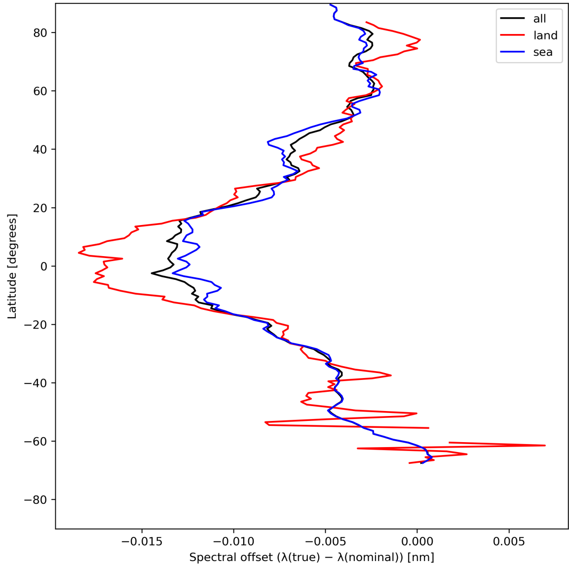
Figure 28: Zonal average of “Spectral offset ( \lambda(\text{true}) - \lambda(\text{nominal}) )” for 2024-05-20 to 2024-05-22.
