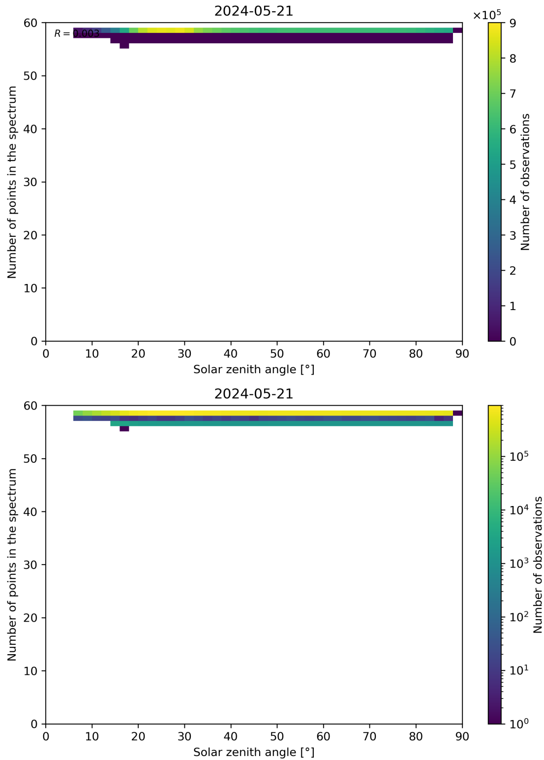
Figure 115: Scatter density plot of “Solar zenith angle” against “Number of points in the spectrum” for 2024-05-20 to 2024-05-22.
