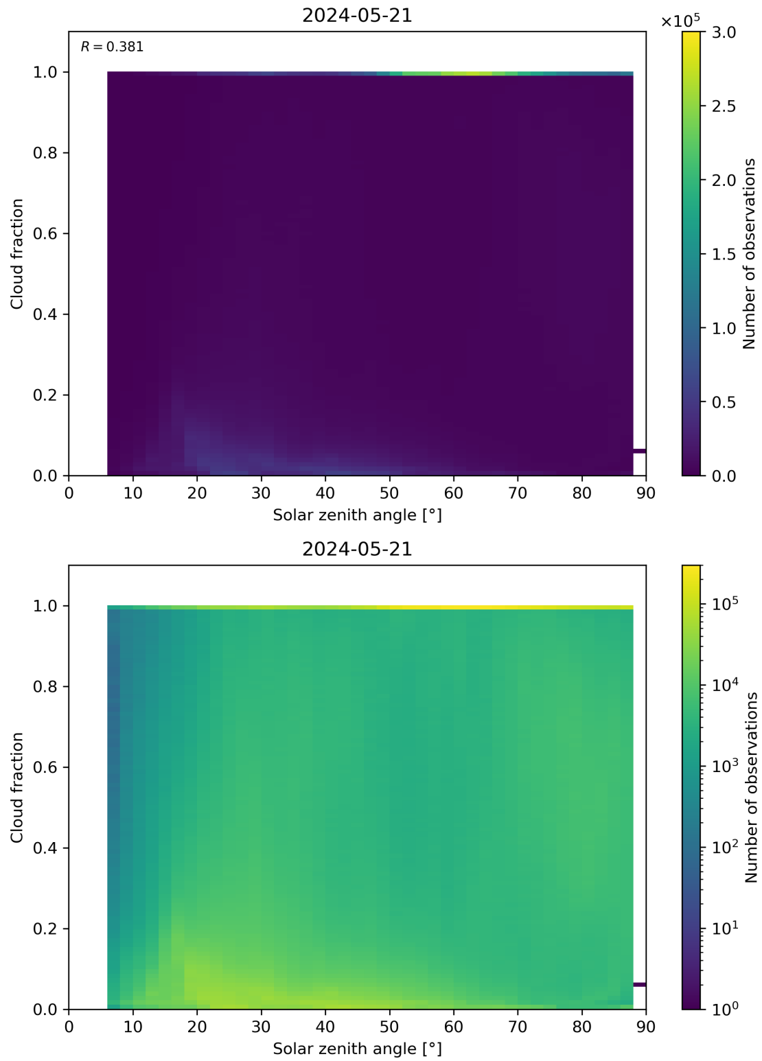
Figure 110: Scatter density plot of “Solar zenith angle” against “Cloud fraction” for 2024-05-20 to 2024-05-22.
