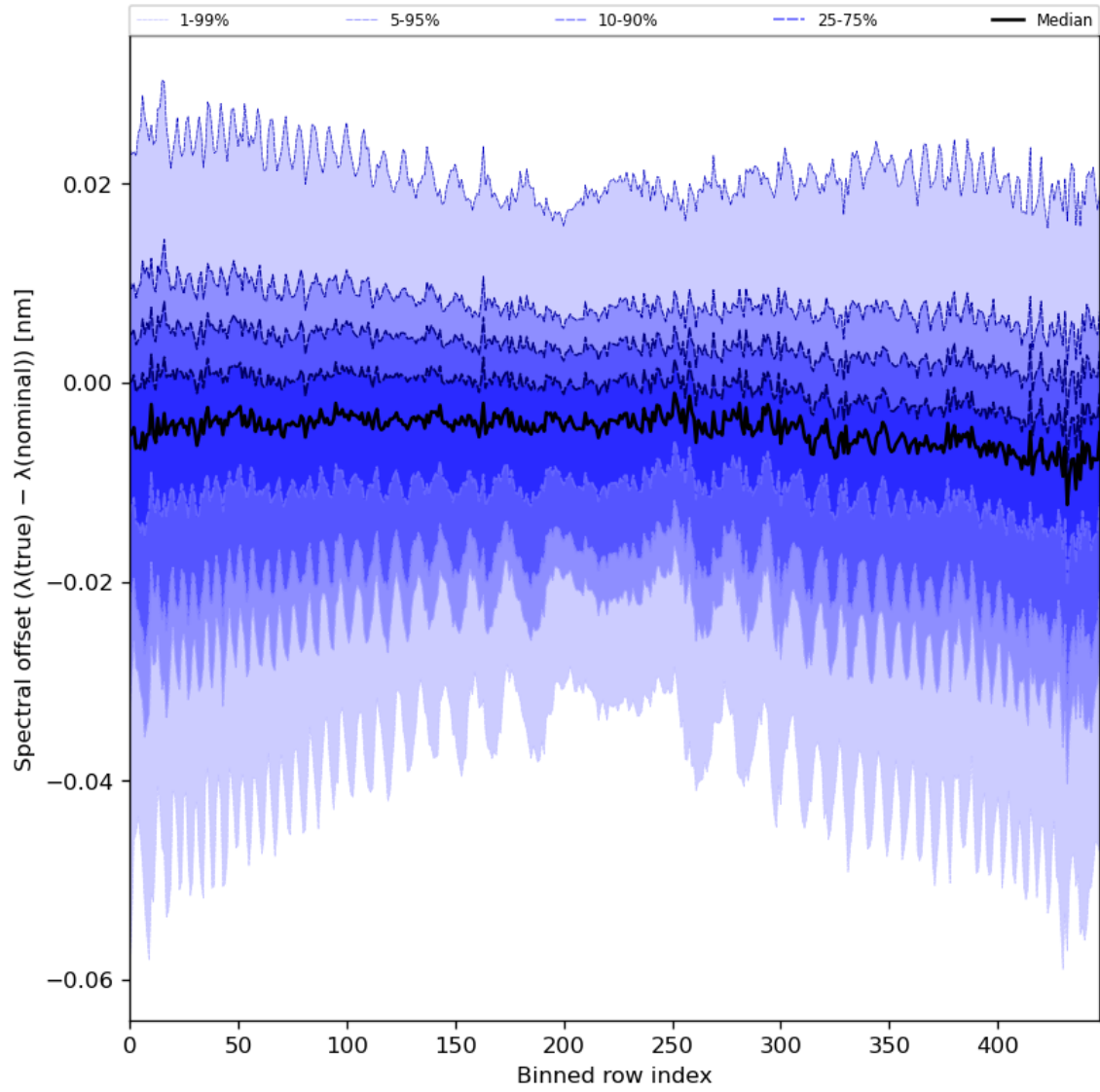
Figure 62: Along track statistics of “Spectral offset ( \lambda(\text{true}) - \lambda(\text{nominal}) )” for 2024-05-20 to 2024-05-22
