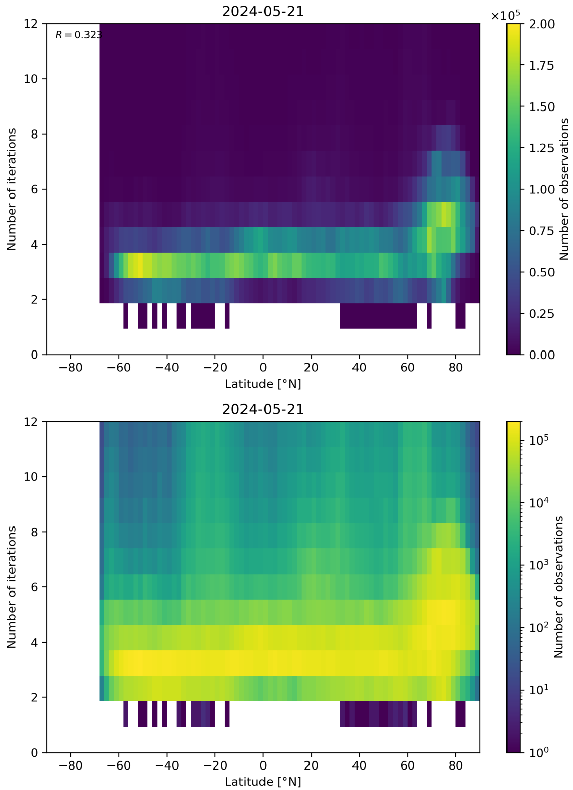
Figure 93: Scatter density plot of “Latitude” against “Number of iterations” for 2024-05-20 to 2024-05-22.
