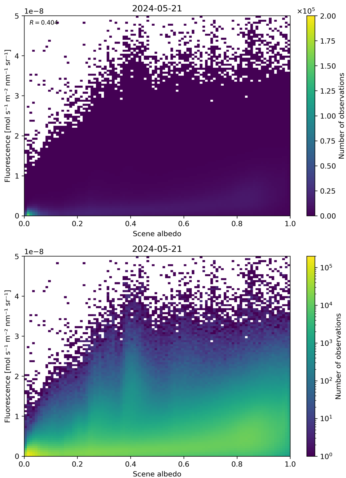
Figure 104: Scatter density plot of “Scene albedo” against “Fluorescence” for 2024-05-20 to 2024-05-22.
