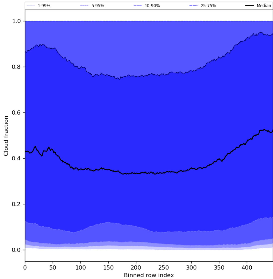
Figure 49: Along track statistics of “Cloud fraction” for 2024-05-20 to 2024-05-22
