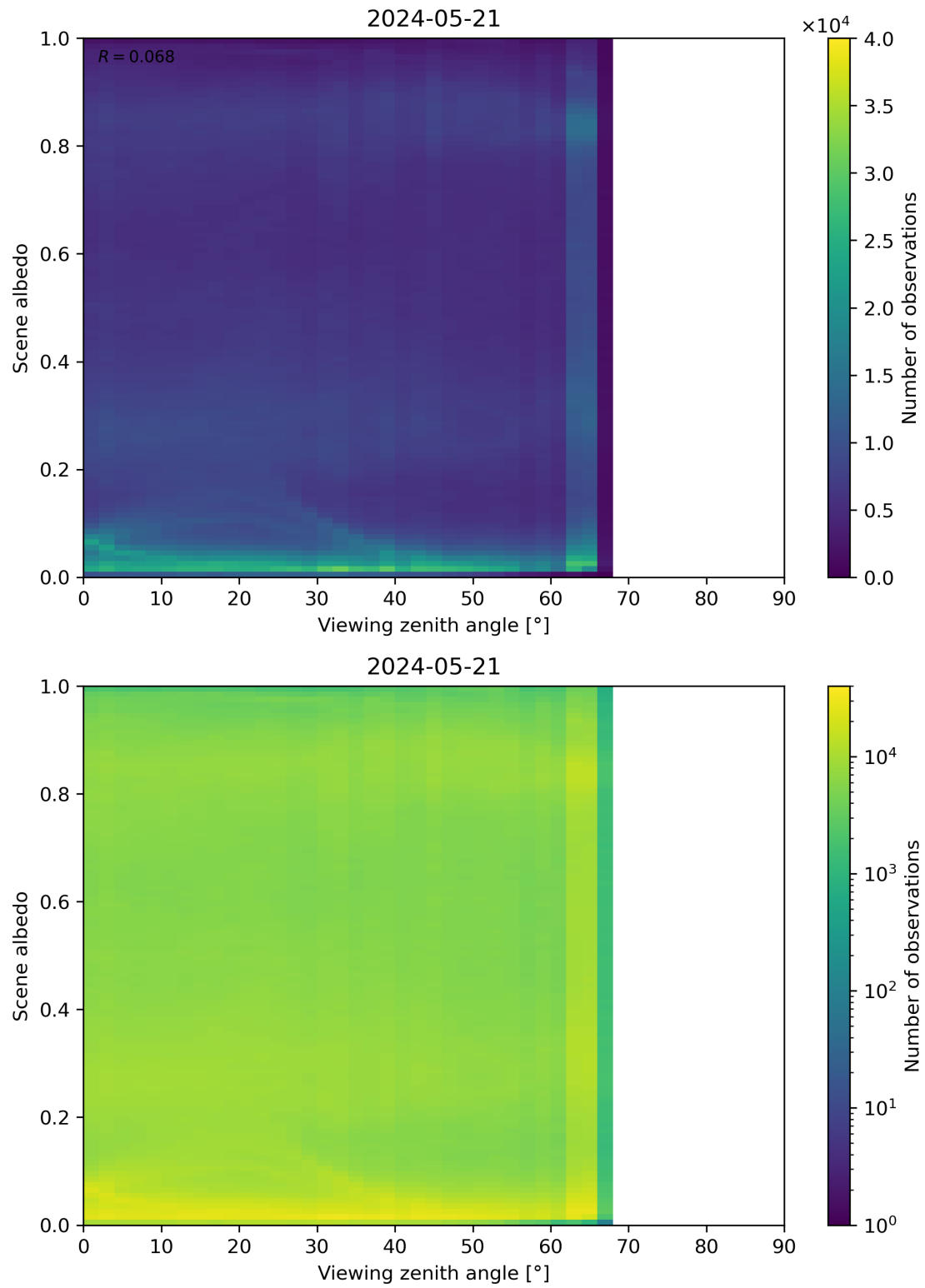
Figure 126: Scatter density plot of “Viewing zenith angle” against “Scene albedo” for 2024-05-20 to 2024-05-22.
