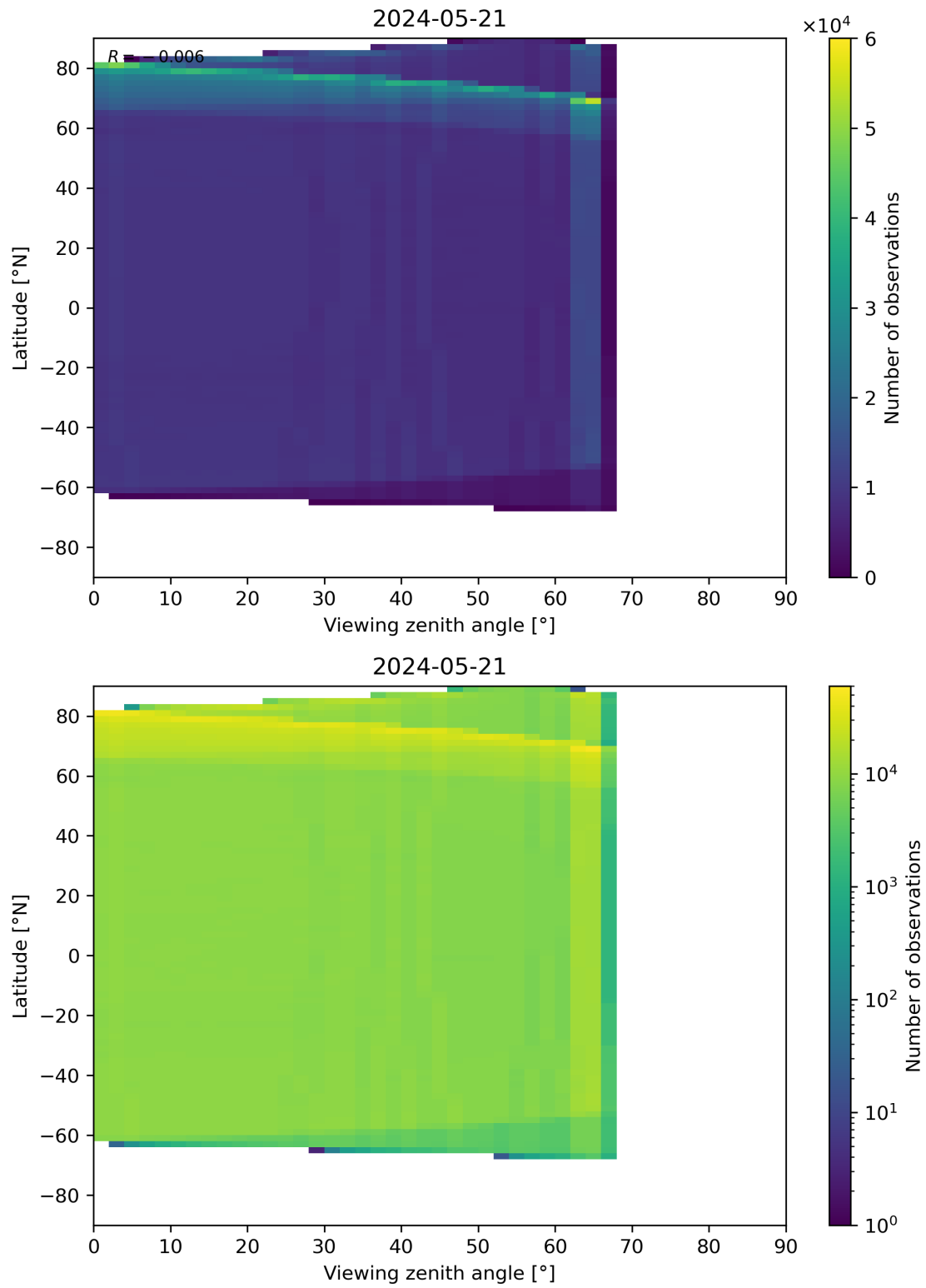
Figure 123: Scatter density plot of “Viewing zenith angle” against “Latitude” for 2024-05-20 to 2024-05-22.
