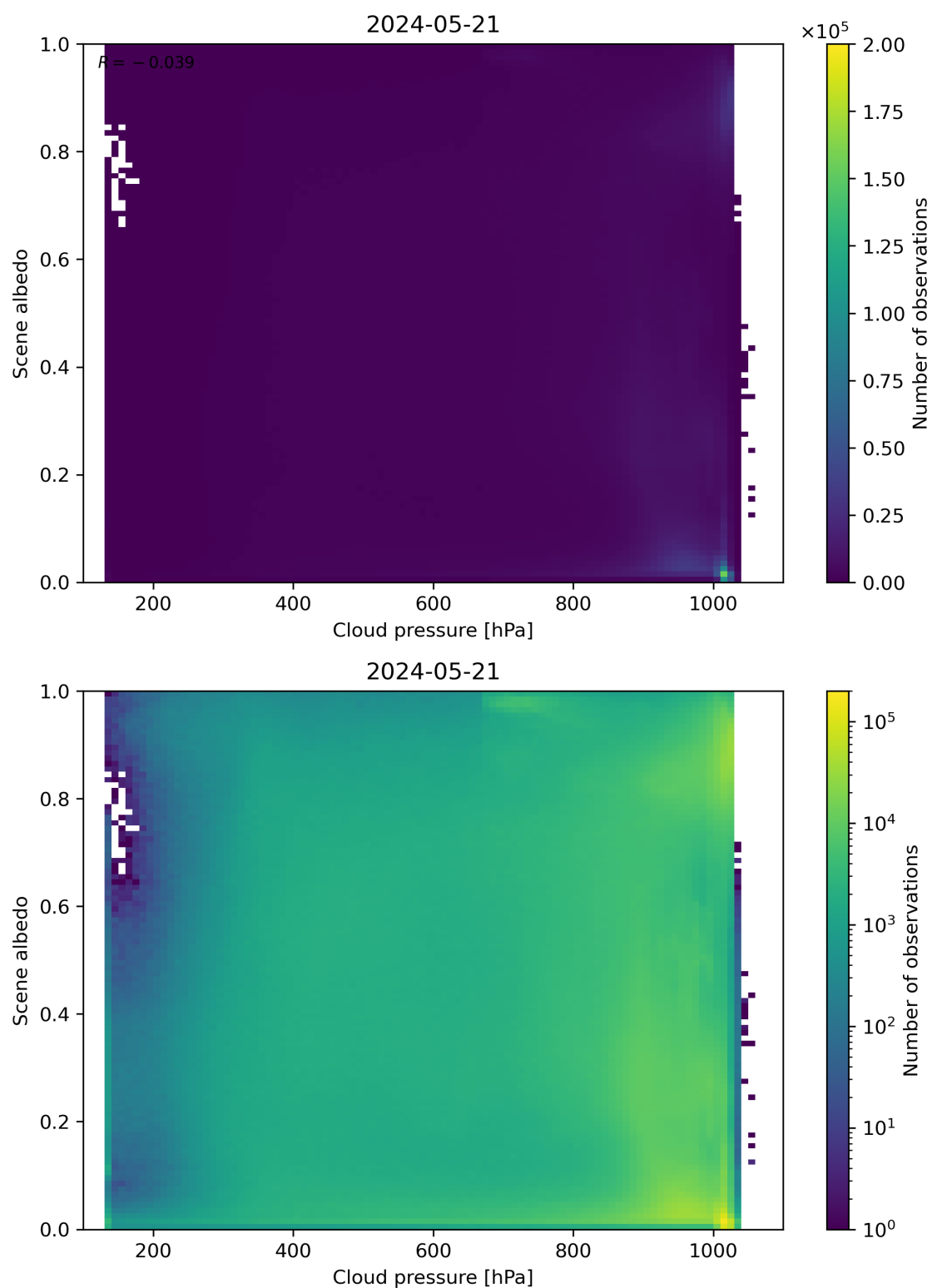
Figure 83: Scatter density plot of “Cloud pressure” against “Scene albedo” for 2024-05-20 to 2024-05-22.
