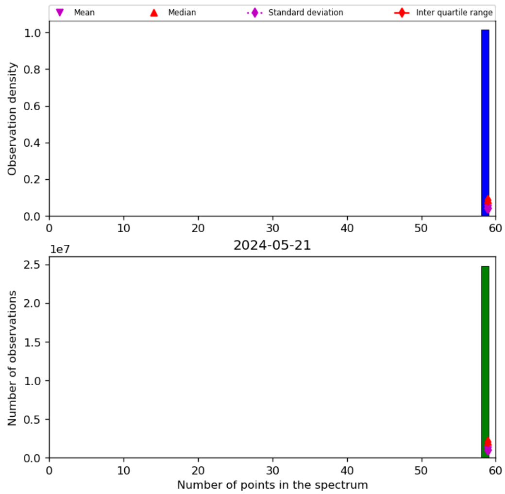
Figure 44: Histogram of “Number of points in the spectrum” for 2024-05-20 to 2024-05-22
