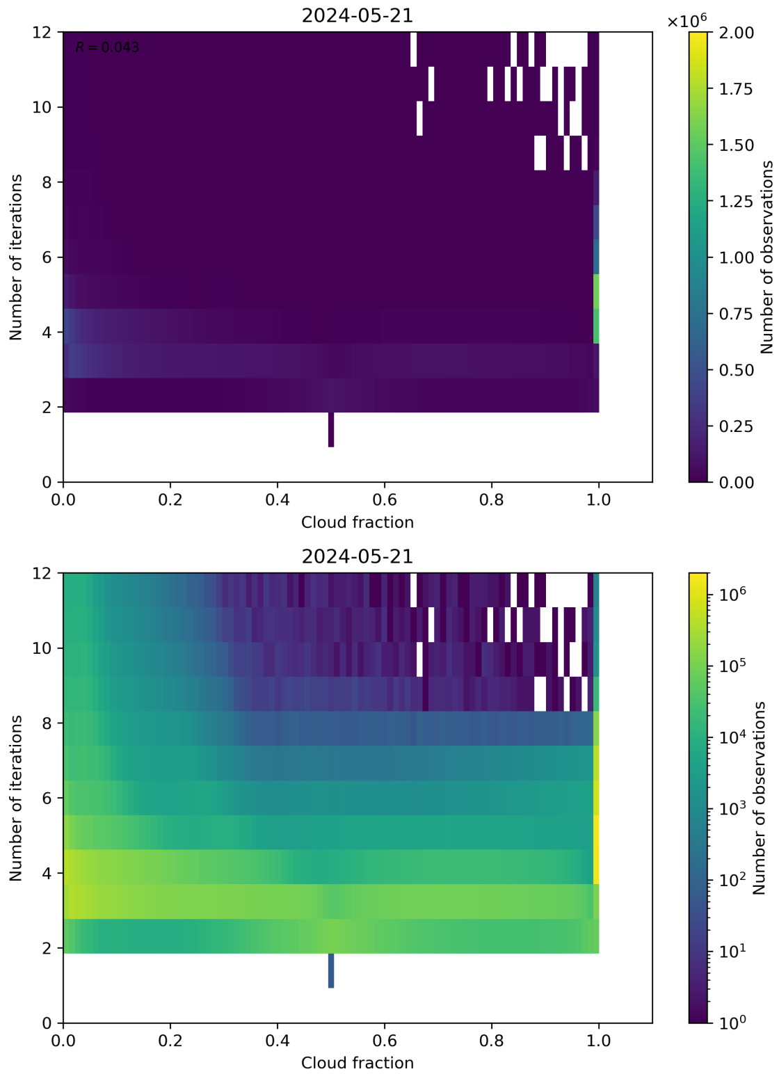
Figure 73: Scatter density plot of “Cloud fraction” against “Number of iterations” for 2024-05-20 to 2024-05-22.
