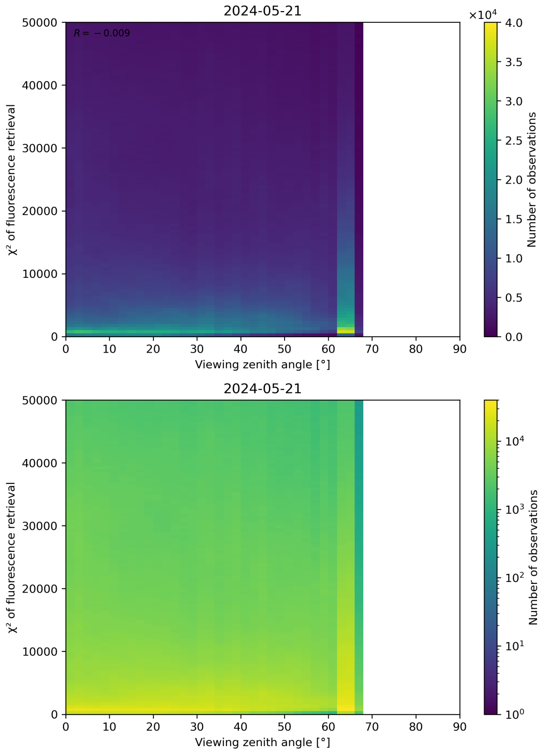
Figure 119: Scatter density plot of “Viewing zenith angle” against “ \chi^2 of fluorescence retrieval” for 2024-05-20 to 2024-05-22.
