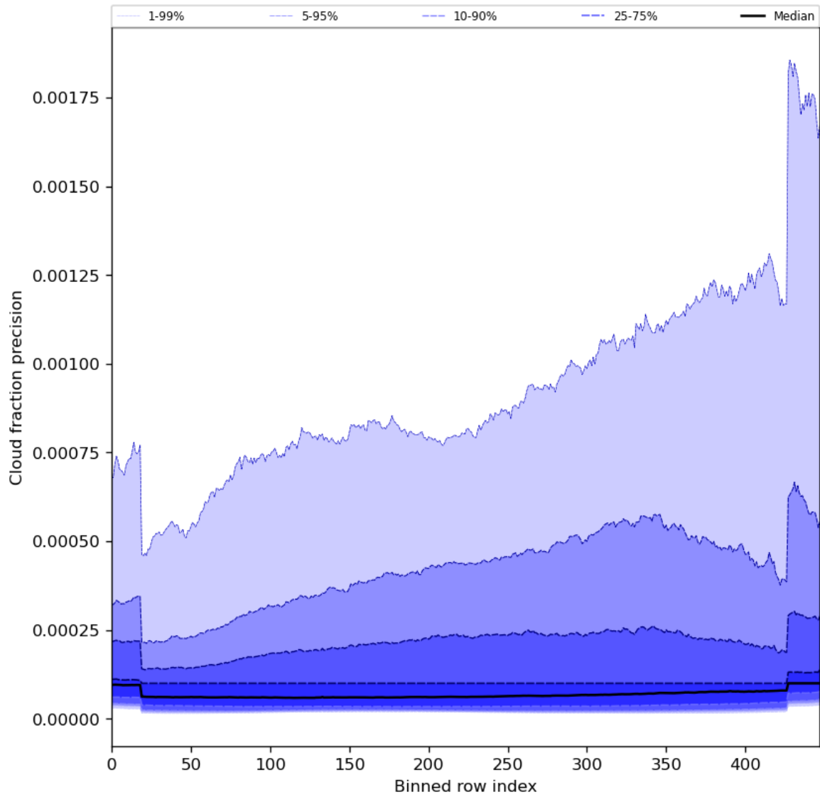
Figure 50: Along track statistics of “Cloud fraction precision” for 2024-05-20 to 2024-05-22
