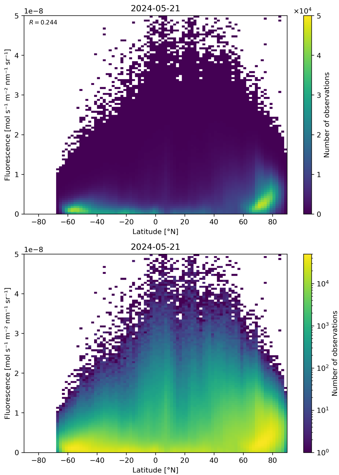
Figure 92: Scatter density plot of “Latitude” against “Fluorescence” for 2024-05-20 to 2024-05-22.
