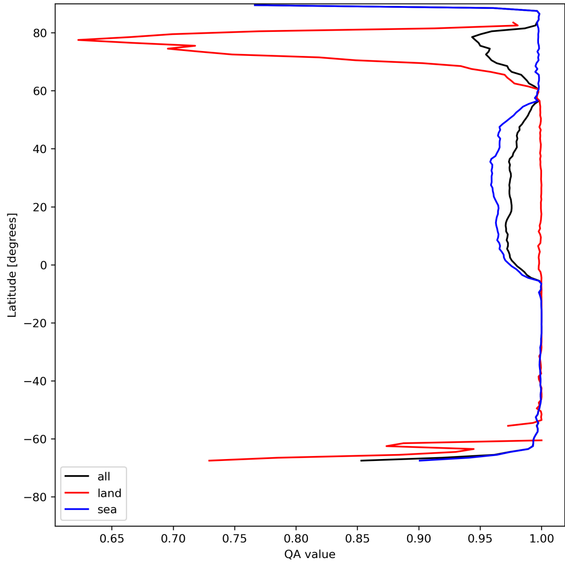
Figure 12: Zonal average of “QA value” for 2024-05-20 to 2024-05-22.
