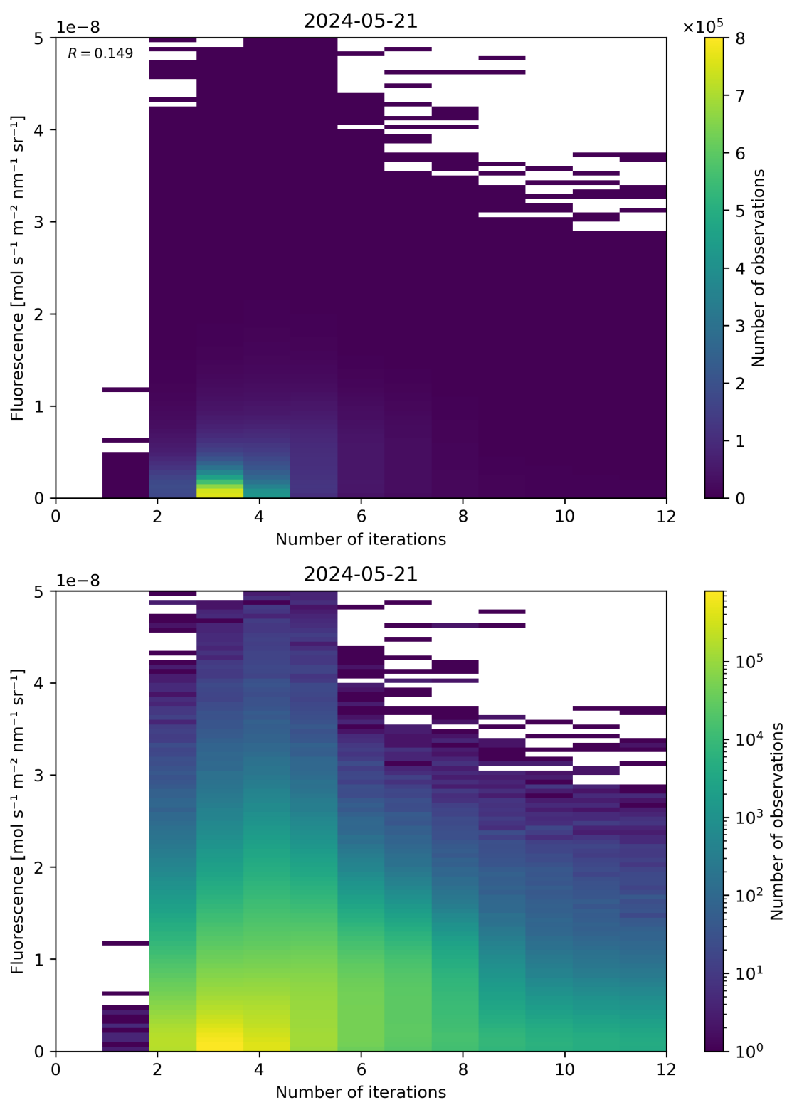
Figure 98: Scatter density plot of “Number of iterations” against “Fluorescence” for 2024-05-20 to 2024-05-22.
