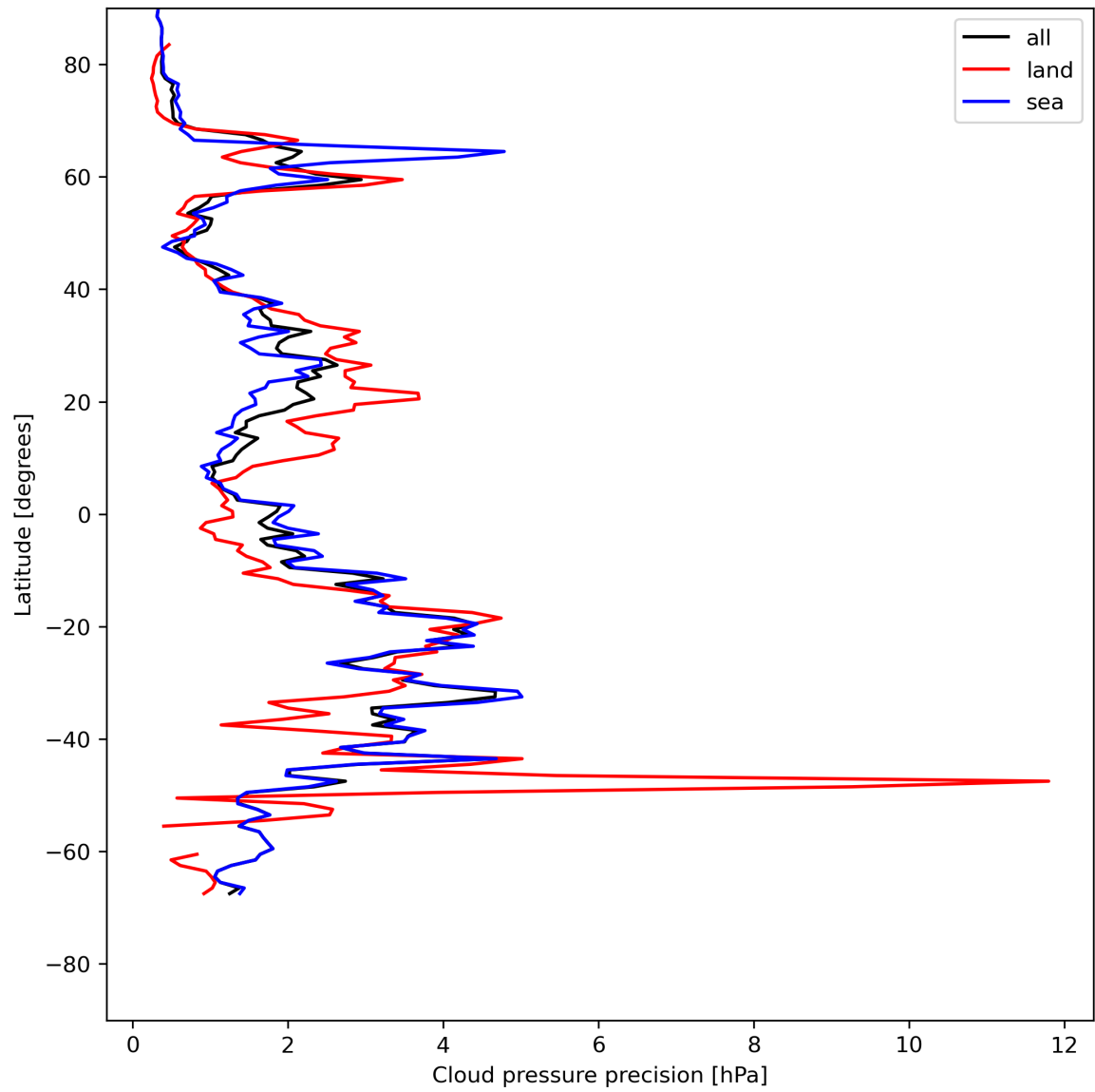
Figure 14: Zonal average of “Cloud pressure precision” for 2024-05-20 to 2024-05-22.
