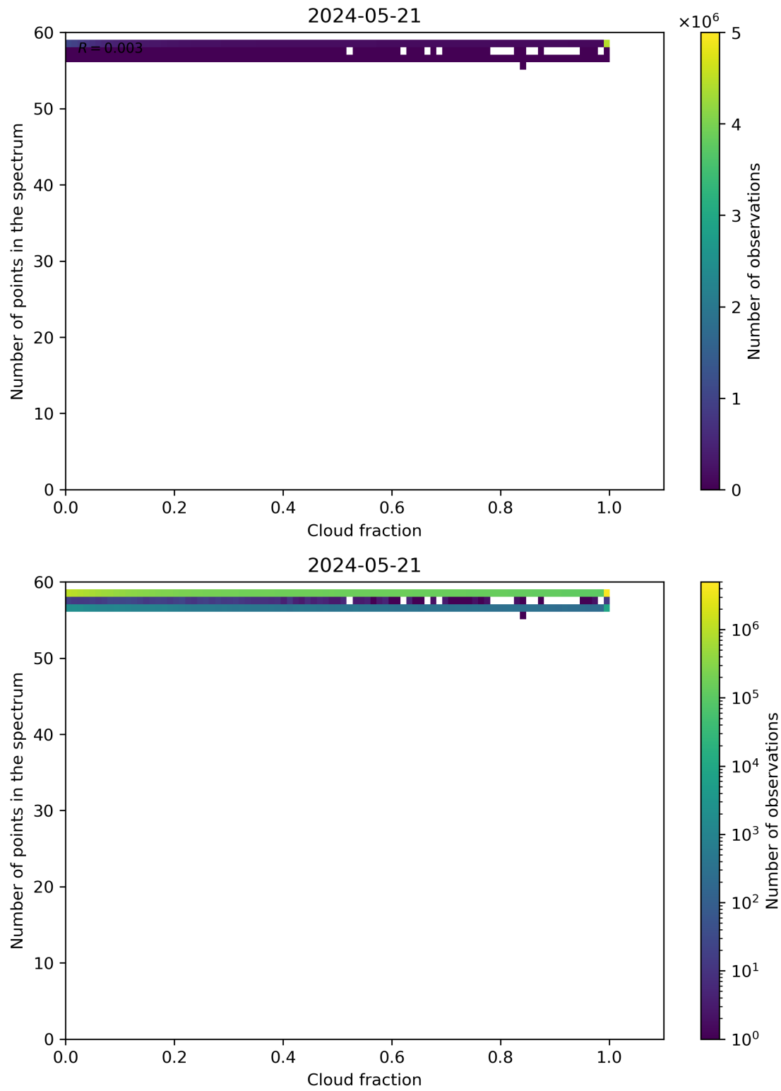
Figure 74: Scatter density plot of “Cloud fraction” against “Number of points in the spectrum” for 2024-05-20 to 2024-05-22.
