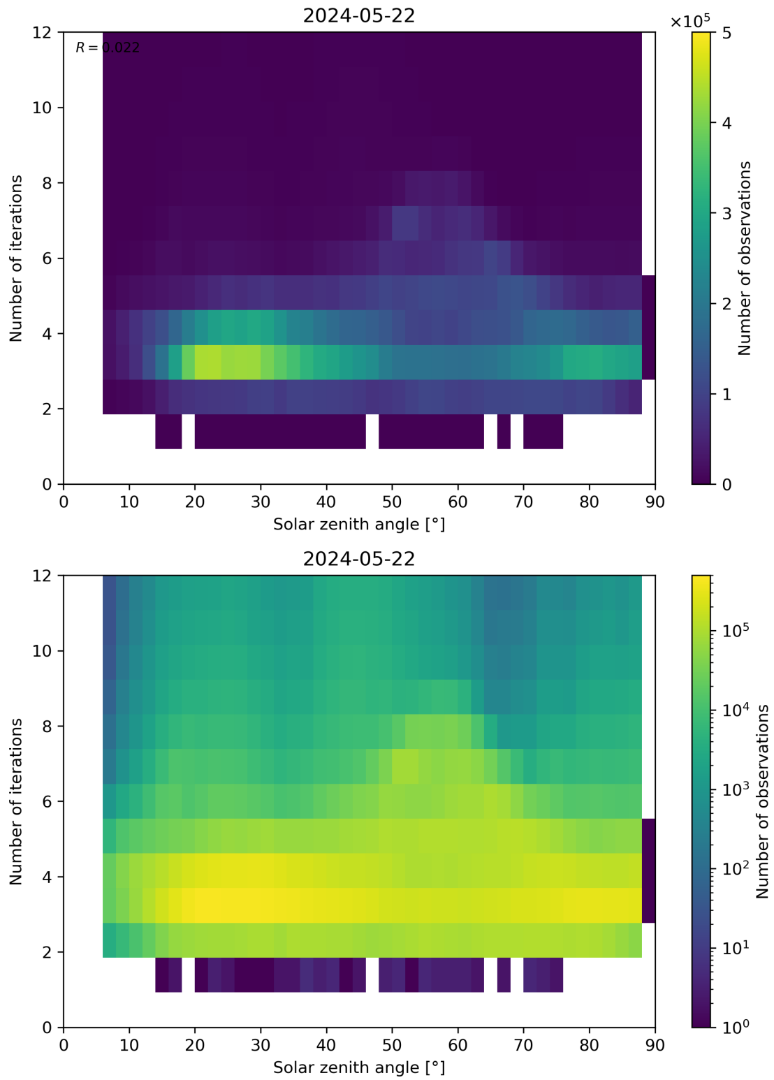
Figure 114: Scatter density plot of “Solar zenith angle” against “Number of iterations” for 2024-05-21 to 2024-05-23.
