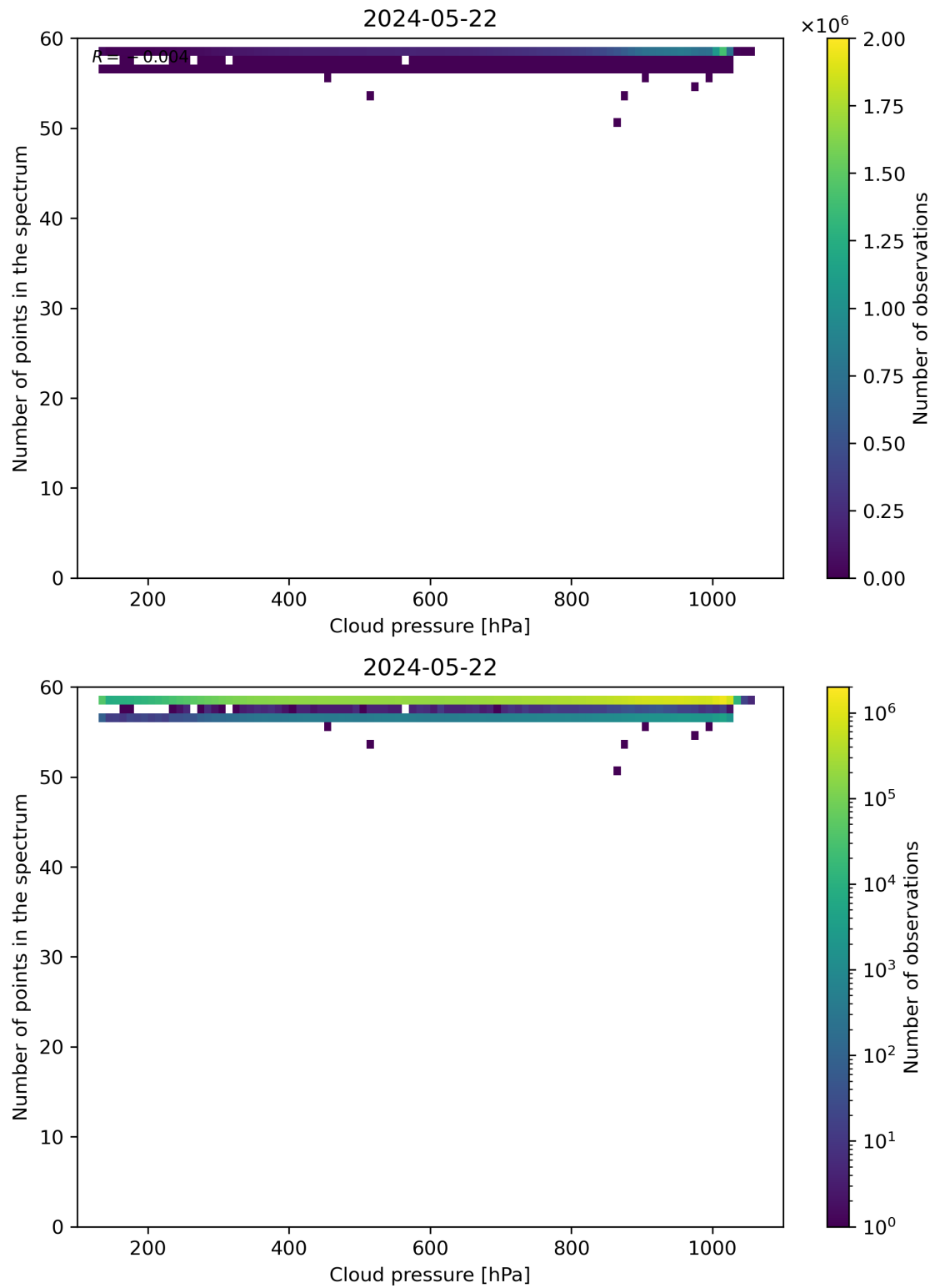
Figure 82: Scatter density plot of “Cloud pressure” against “Number of points in the spectrum” for 2024-05-21 to 2024-05-23.
