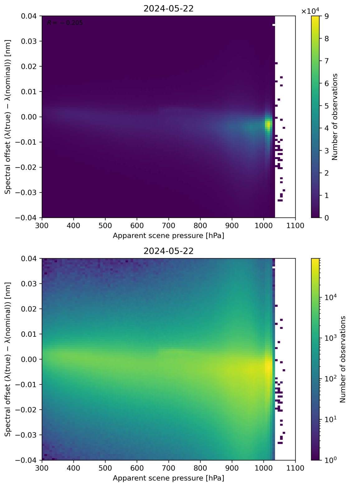
Figure 67: Scatter density plot of “Apparent scene pressure” against “Spectral offset ( \lambda(\text{true}) - \lambda(\text{nominal}) )” for 2024-05-21 to 2024-05-23.
