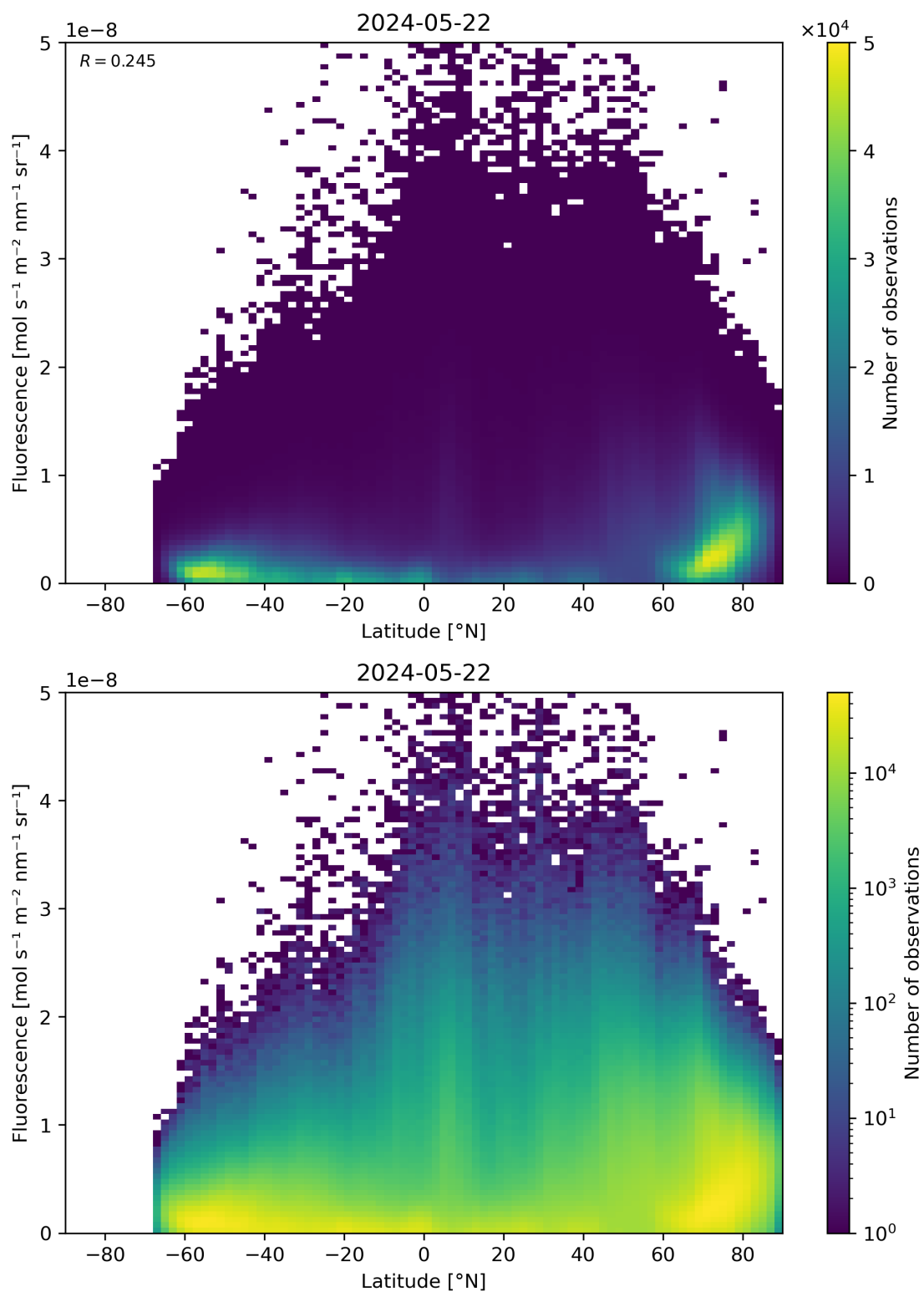
Figure 92: Scatter density plot of “Latitude” against “Fluorescence” for 2024-05-21 to 2024-05-23.
