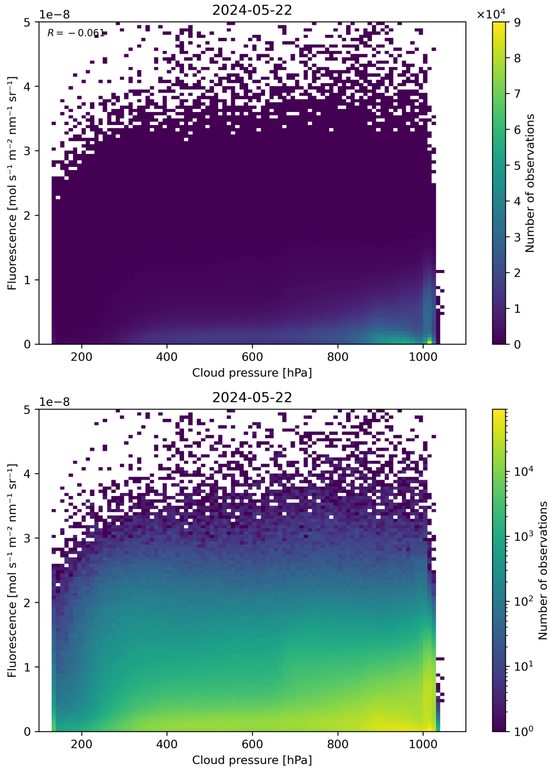
Figure 80: Scatter density plot of “Cloud pressure” against “Fluorescence” for 2024-05-21 to 2024-05-23.
