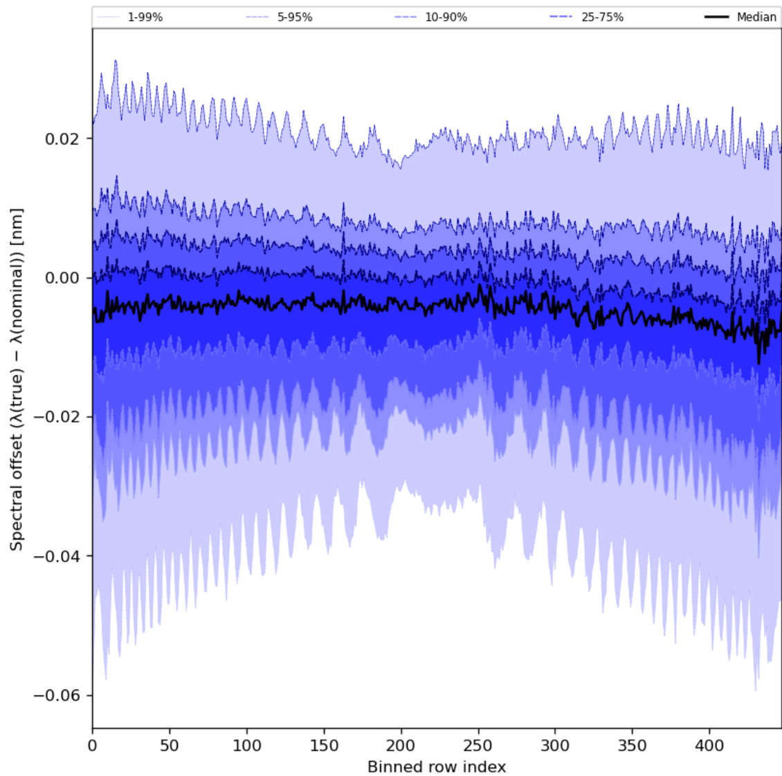
Figure 62: Along track statistics of “Spectral offset ( \lambda(\text{true}) - \lambda(\text{nominal}) )” for 2024-05-21 to 2024-05-23
