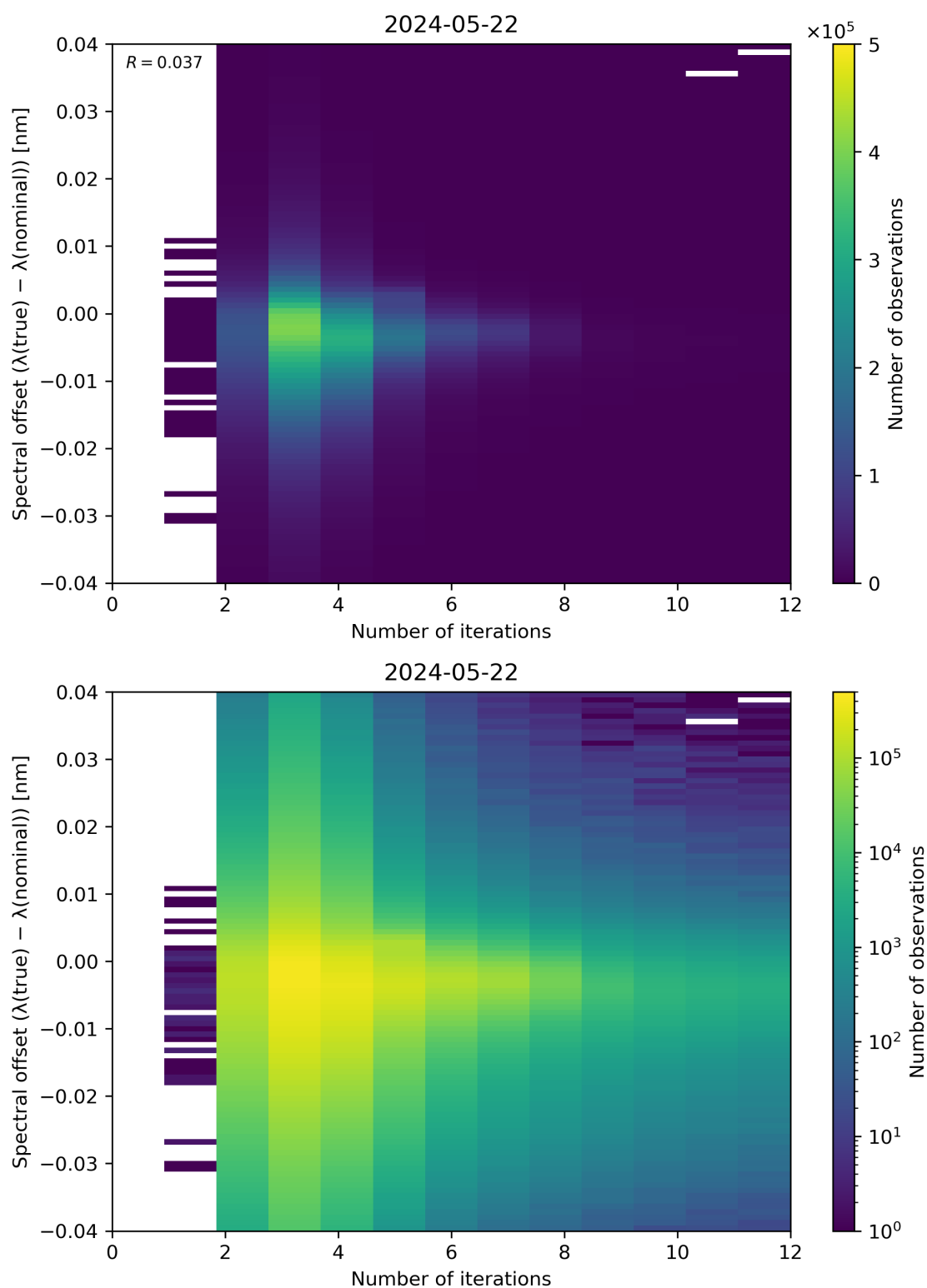
Figure 100: Scatter density plot of “Number of iterations” against “Spectral offset ( \lambda(\text{true}) - \lambda(\text{nominal}) )” for 2024-05-21 to 2024-05-23.
