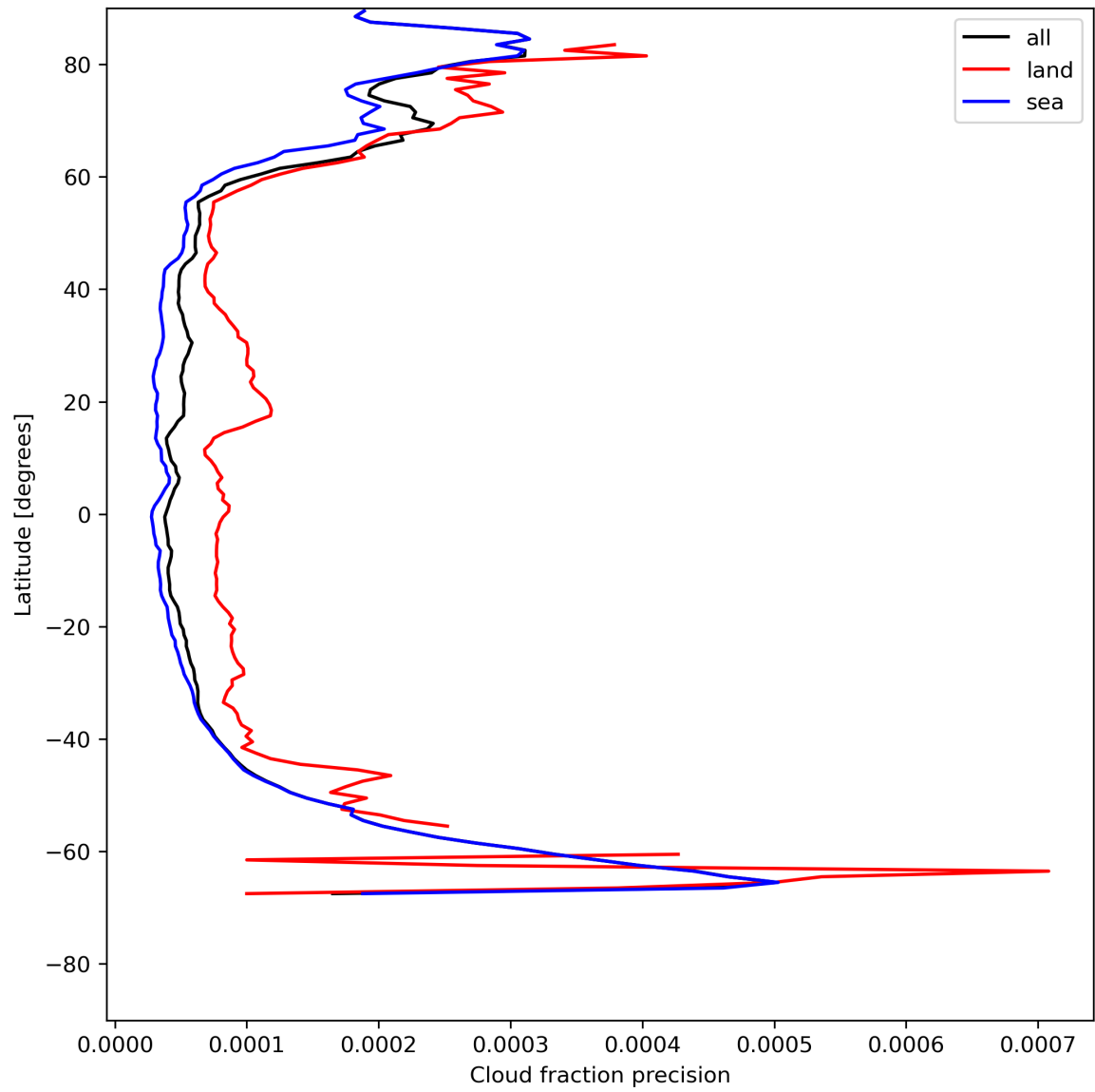
Figure 16: Zonal average of “Cloud fraction precision” for 2024-05-21 to 2024-05-23.
