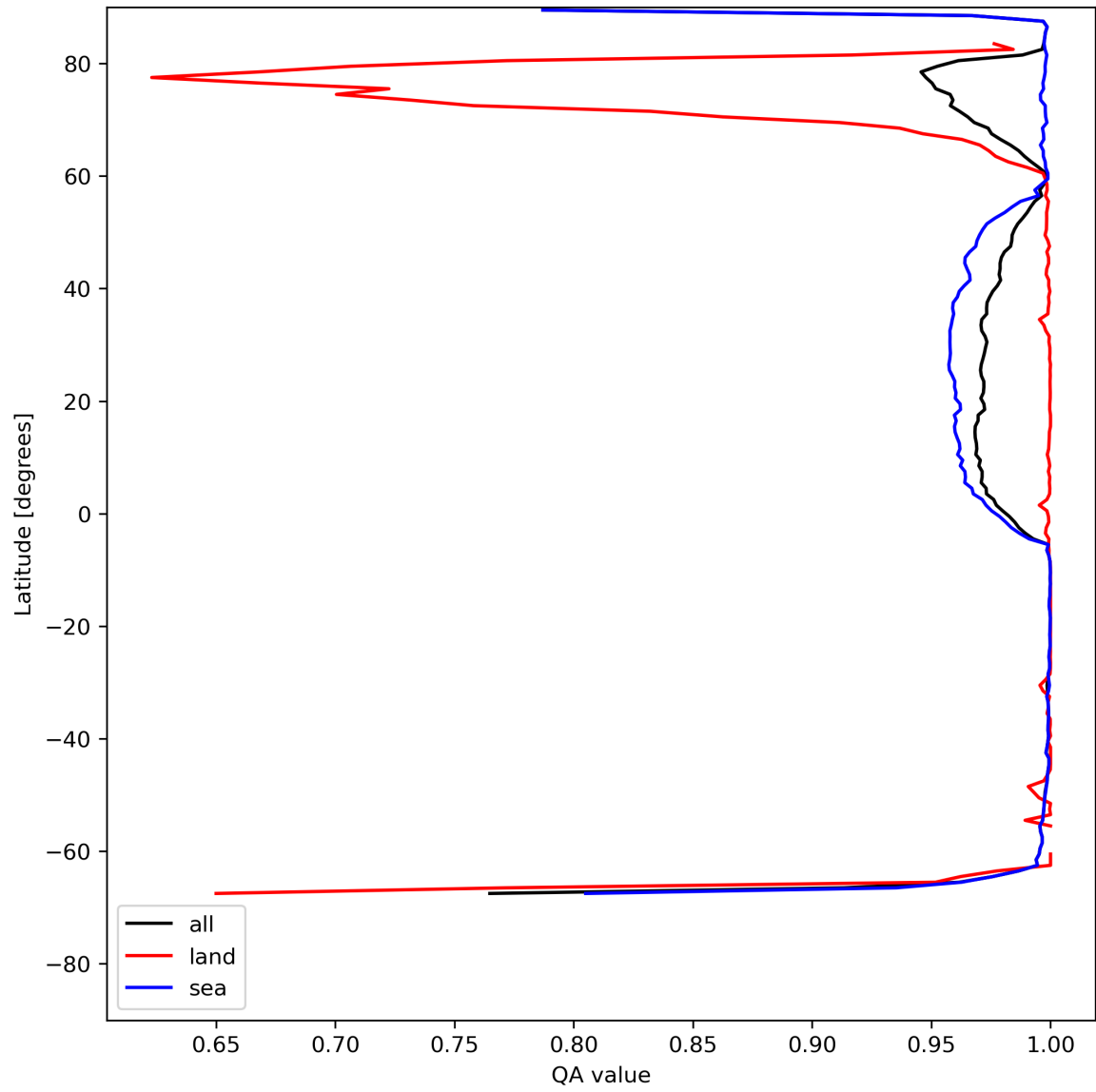
Figure 12: Zonal average of “QA value” for 2024-05-21 to 2024-05-23.
