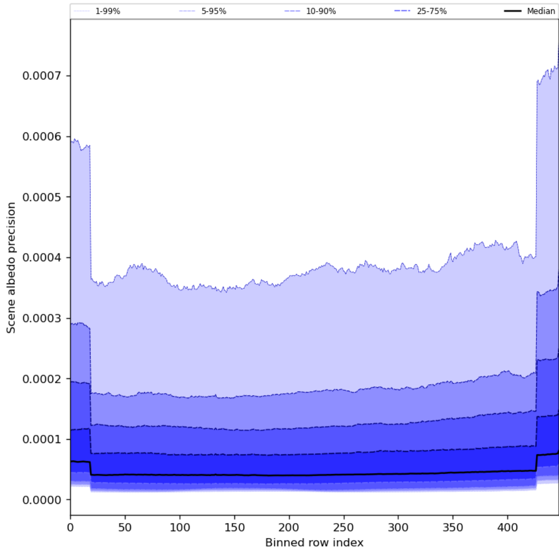
Figure 52: Along track statistics of “Scene albedo precision” for 2024-05-21 to 2024-05-23
