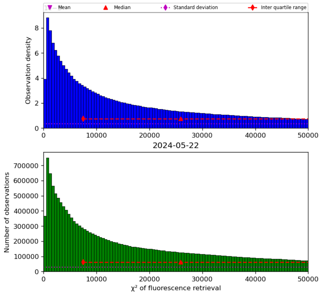
Figure 42: Histogram of “ \chi^2 of fluorescence retrieval” for 2024-05-21 to 2024-05-23
