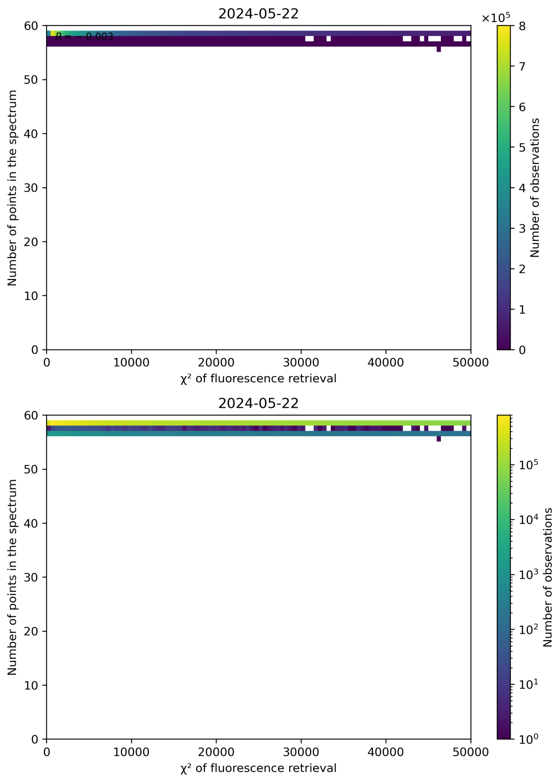
Figure 68: Scatter density plot of “ \chi^2 of fluorescence retrieval” against “Number of points in the spectrum” for 2024-05-21 to 2024-05-23.
