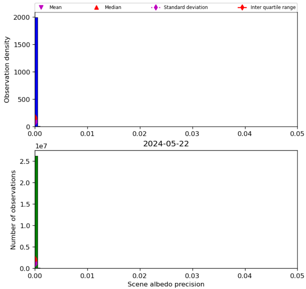
Figure 35: Histogram of “Scene albedo precision” for 2024-05-21 to 2024-05-23
