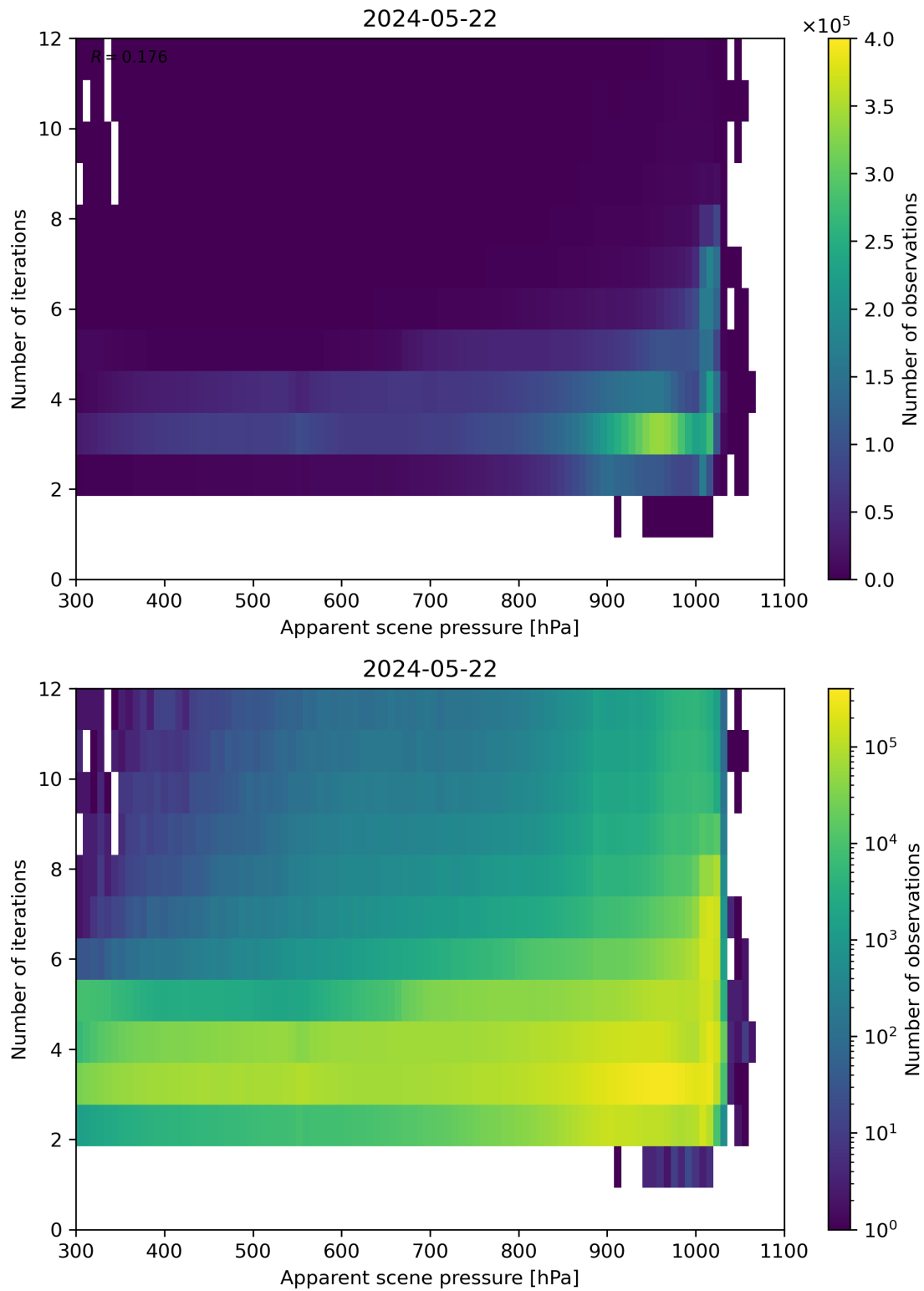
Figure 65: Scatter density plot of “Apparent scene pressure” against “Number of iterations” for 2024-05-21 to 2024-05-23.
