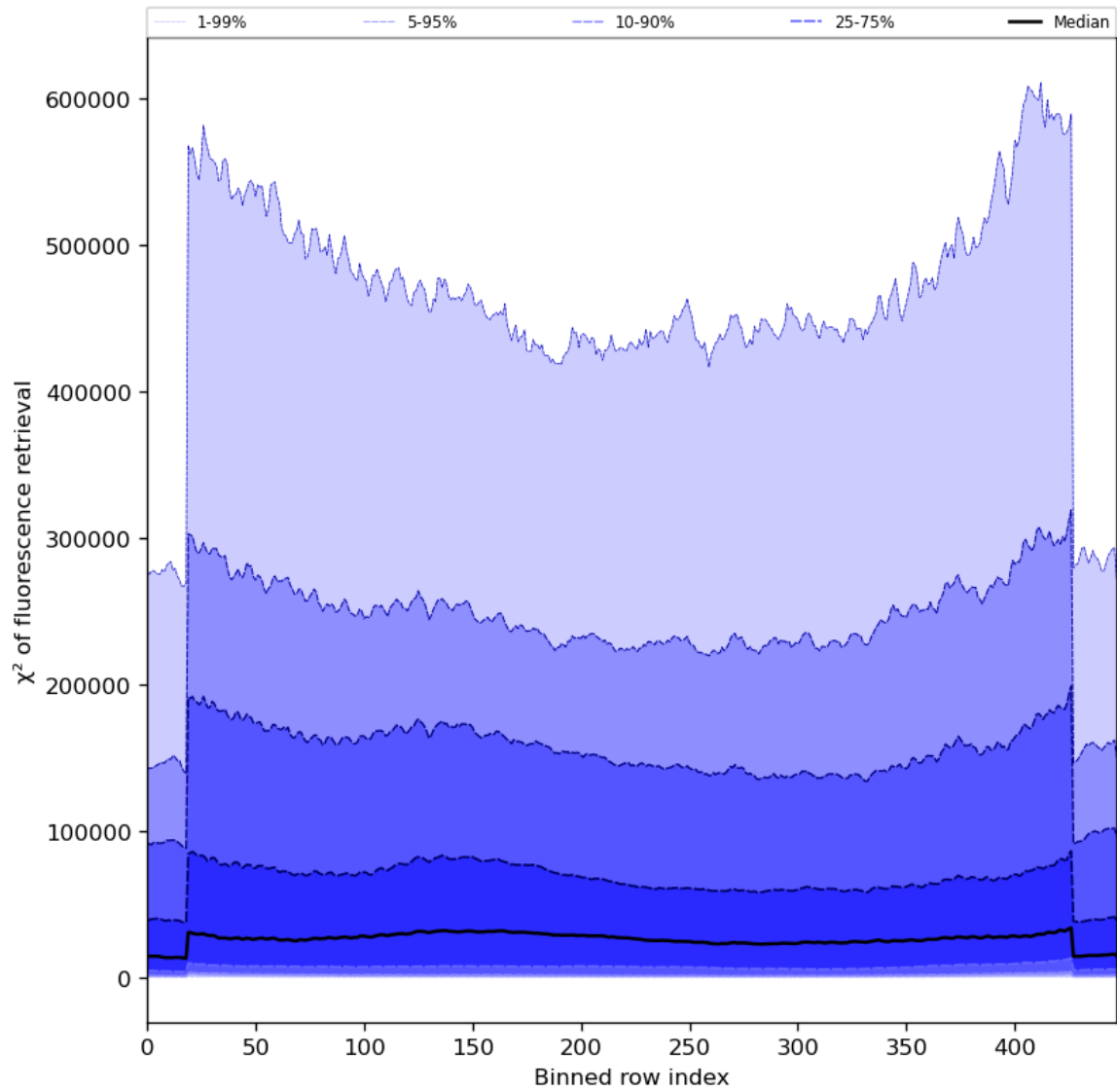
Figure 59: Along track statistics of “ \chi^2 of fluorescence retrieval” for 2024-05-21 to 2024-05-23
