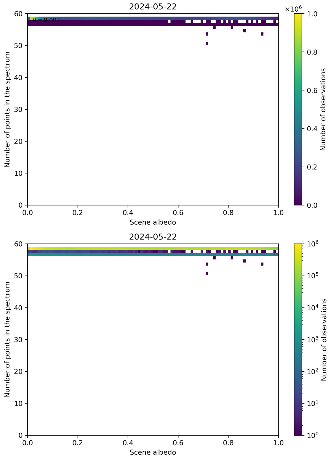
Figure 106: Scatter density plot of “Scene albedo” against “Number of points in the spectrum” for 2024-05-21 to 2024-05-23.
