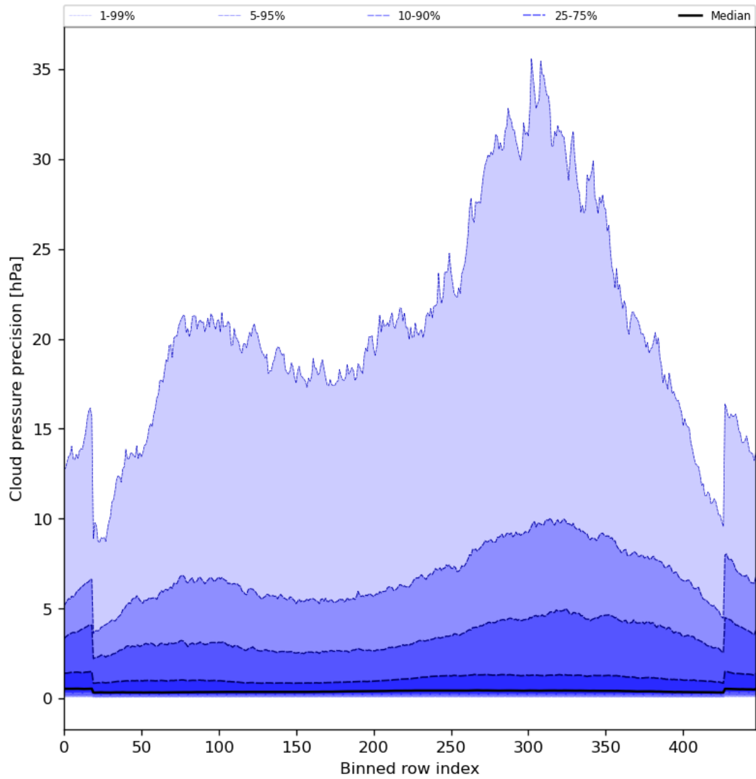
Figure 48: Along track statistics of “Cloud pressure precision” for 2024-05-21 to 2024-05-23
