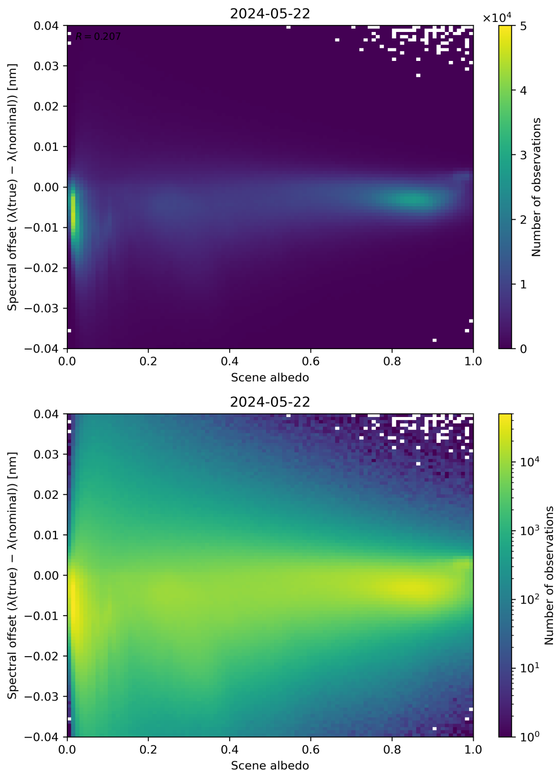
Figure 107: Scatter density plot of “Scene albedo” against “Spectral offset ( \lambda(\text{true}) - \lambda(\text{nominal}) )” for 2024-05-21 to 2024-05-23.
