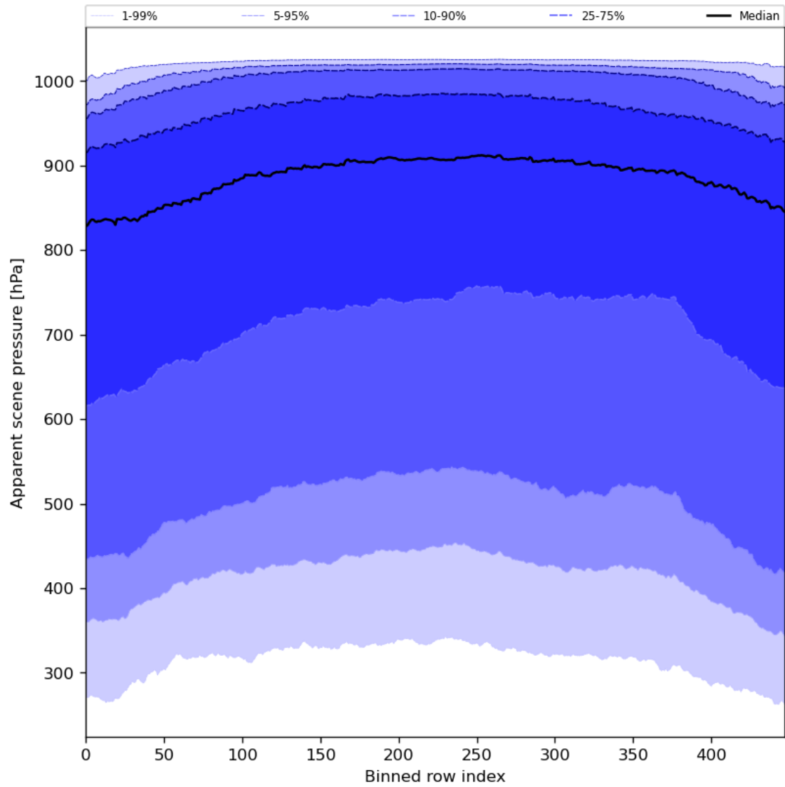
Figure 53: Along track statistics of “Apparent scene pressure” for 2024-05-21 to 2024-05-23
