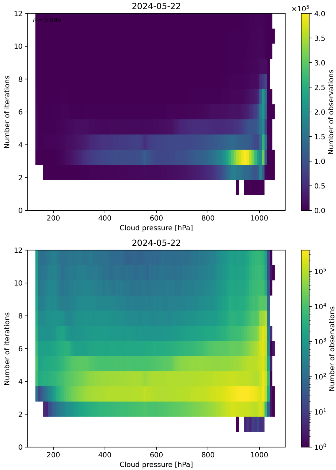
Figure 81: Scatter density plot of “Cloud pressure” against “Number of iterations” for 2024-05-21 to 2024-05-23.
