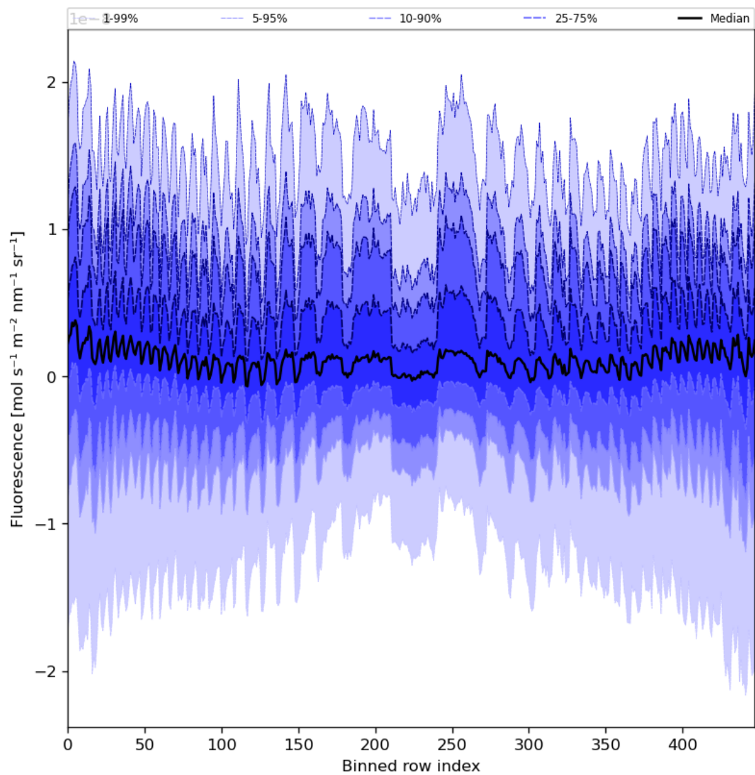
Figure 57: Along track statistics of “Fluorescence” for 2024-05-21 to 2024-05-23
