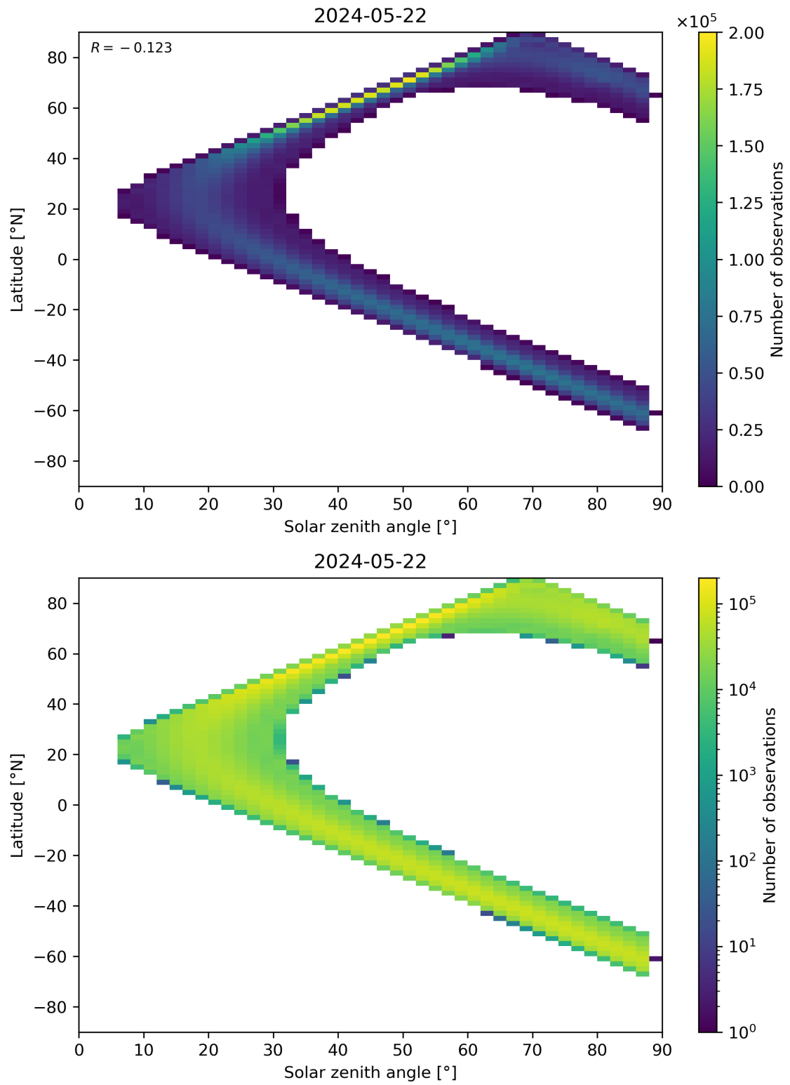
Figure 113: Scatter density plot of “Solar zenith angle” against “Latitude” for 2024-05-21 to 2024-05-23.
