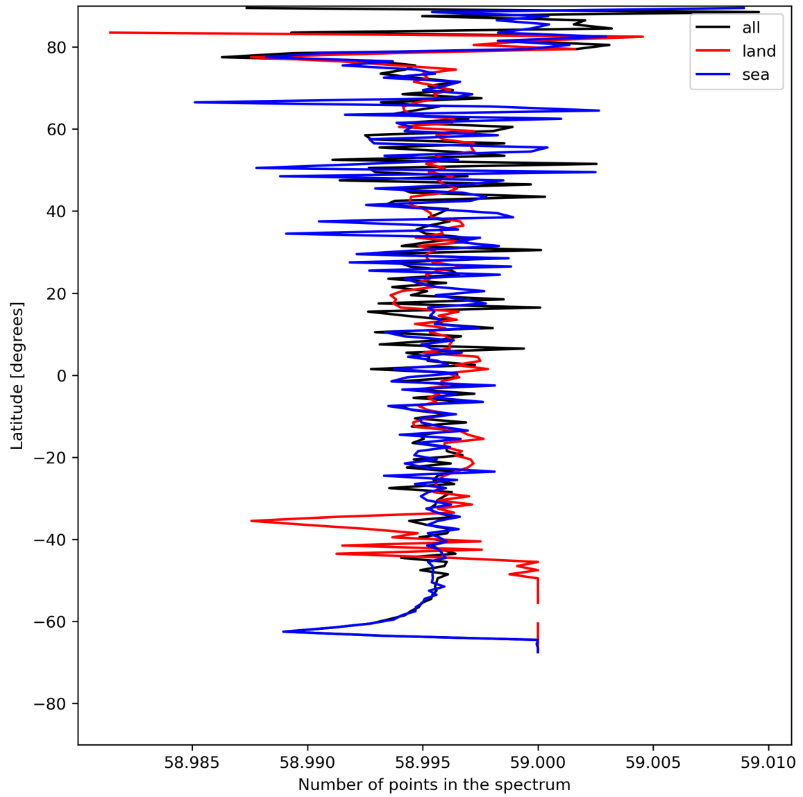
Figure 27: Zonal average of “Number of points in the spectrum” for 2024-05-21 to 2024-05-23.
