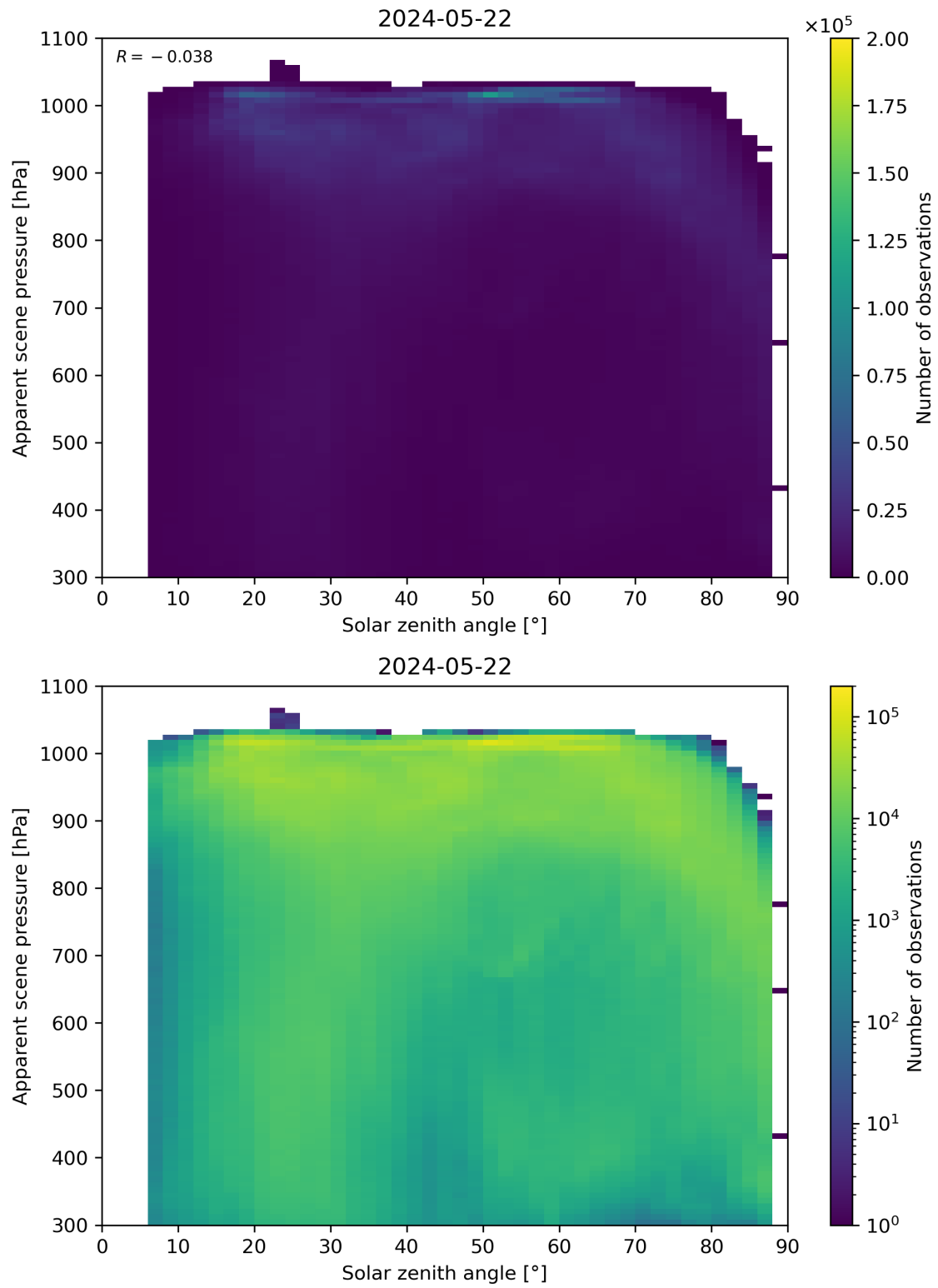
Figure 108: Scatter density plot of “Solar zenith angle” against “Apparent scene pressure” for 2024-05-21 to 2024-05-23.
