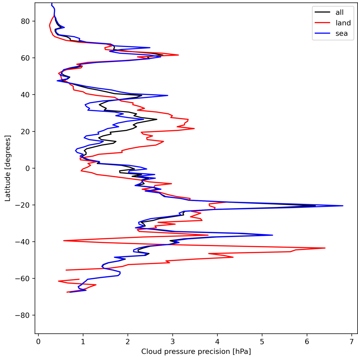
Figure 14: Zonal average of “Cloud pressure precision” for 2024-05-21 to 2024-05-23.
