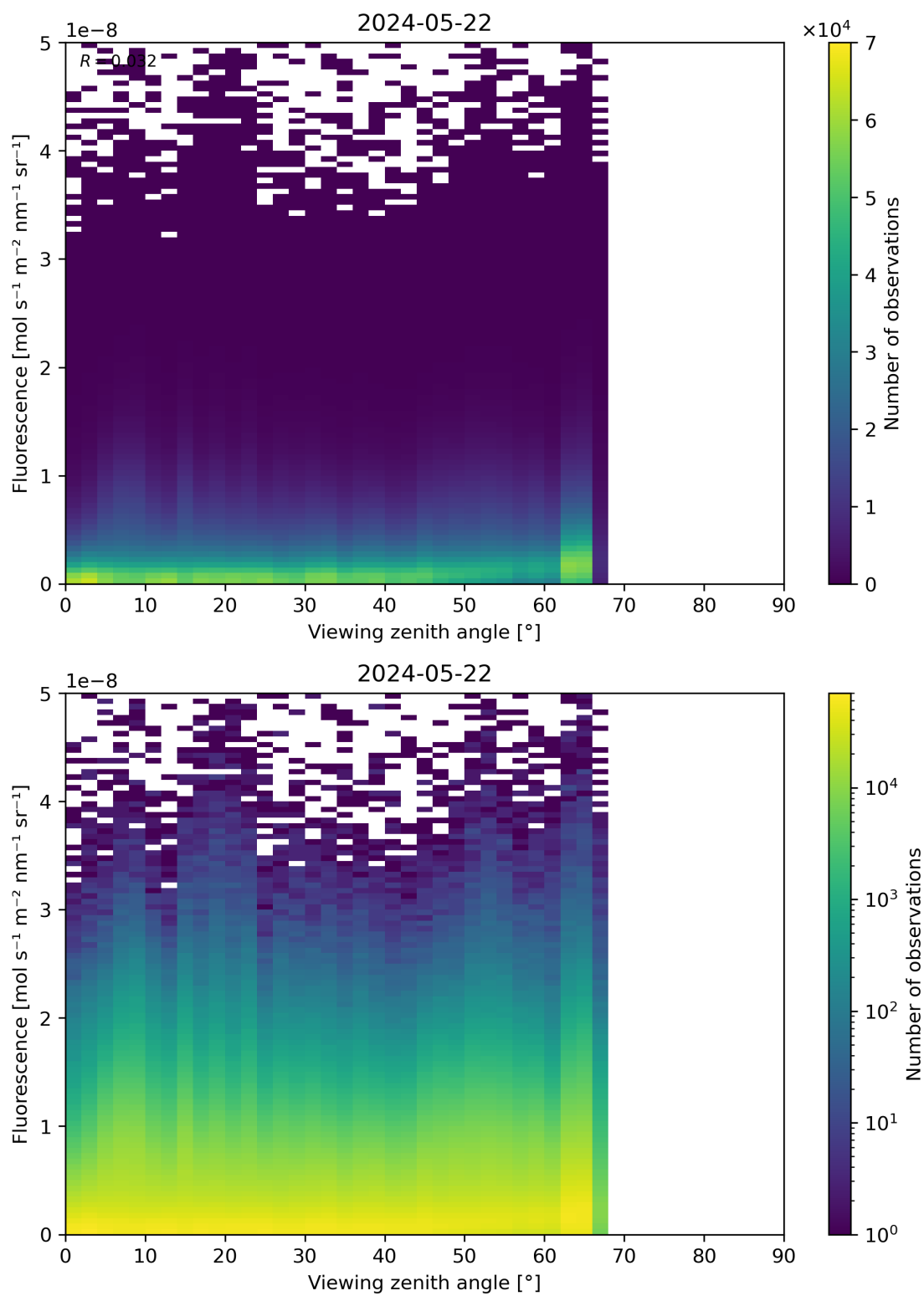
Figure 122: Scatter density plot of “Viewing zenith angle” against “Fluorescence” for 2024-05-21 to 2024-05-23.
