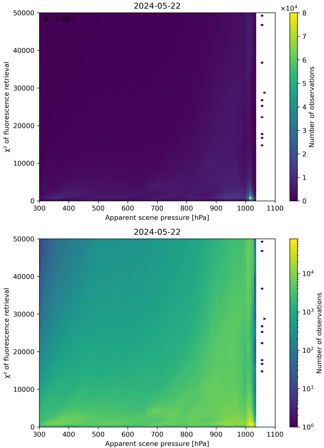
Figure 63: Scatter density plot of “Apparent scene pressure” against “ \chi^2 of fluorescence retrieval” for 2024-05-21 to 2024-05-23.
