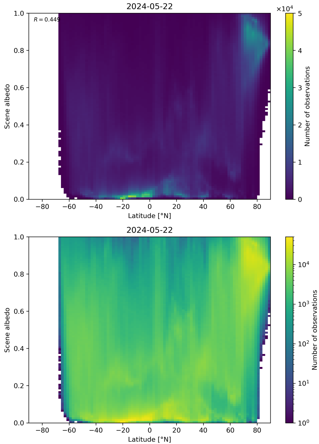
Figure 95: Scatter density plot of “Latitude” against “Scene albedo” for 2024-05-21 to 2024-05-23.
