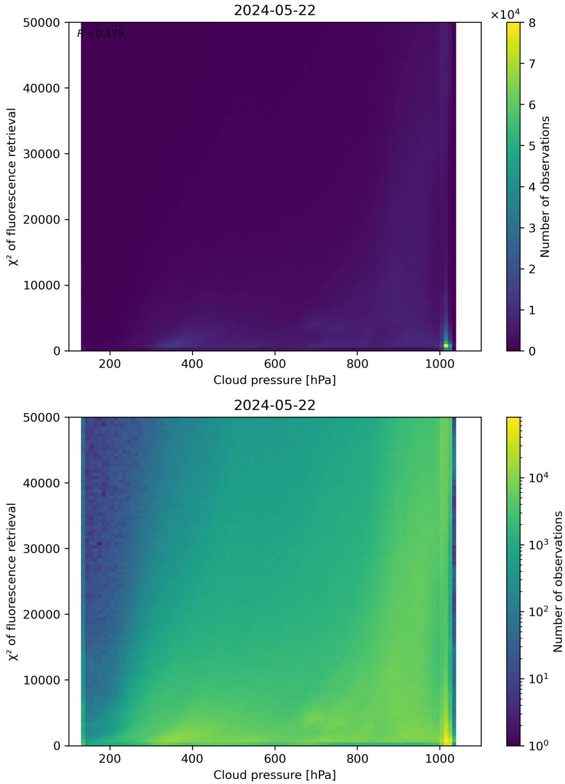
Figure 78: Scatter density plot of “Cloud pressure” against “ \chi^2 of fluorescence retrieval” for 2024-05-21 to 2024-05-23.
