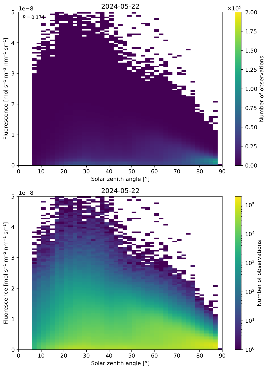
Figure 112: Scatter density plot of “Solar zenith angle” against “Fluorescence” for 2024-05-21 to 2024-05-23.
