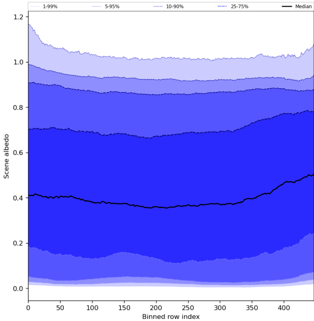
Figure 51: Along track statistics of “Scene albedo” for 2024-05-21 to 2024-05-23
