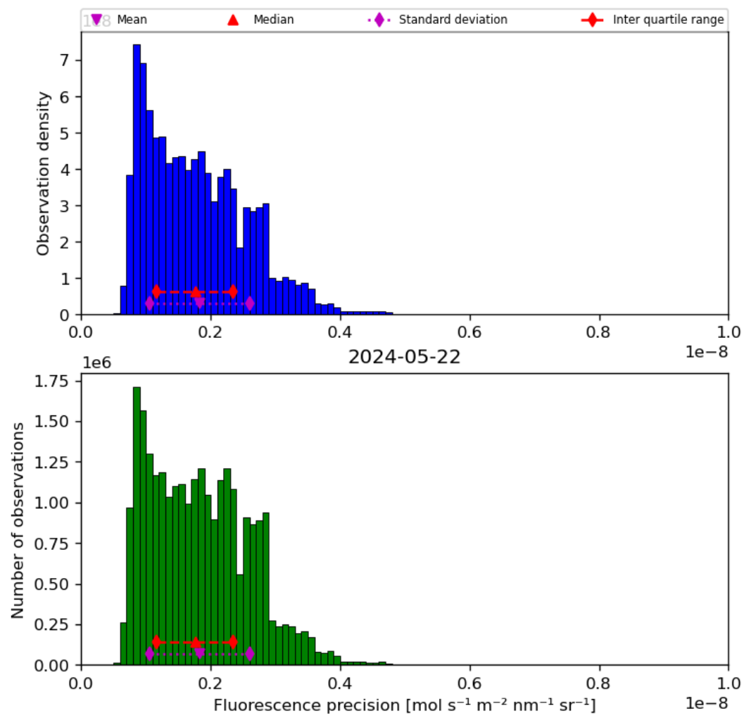
Figure 41: Histogram of “Fluorescence precision” for 2024-05-21 to 2024-05-23
