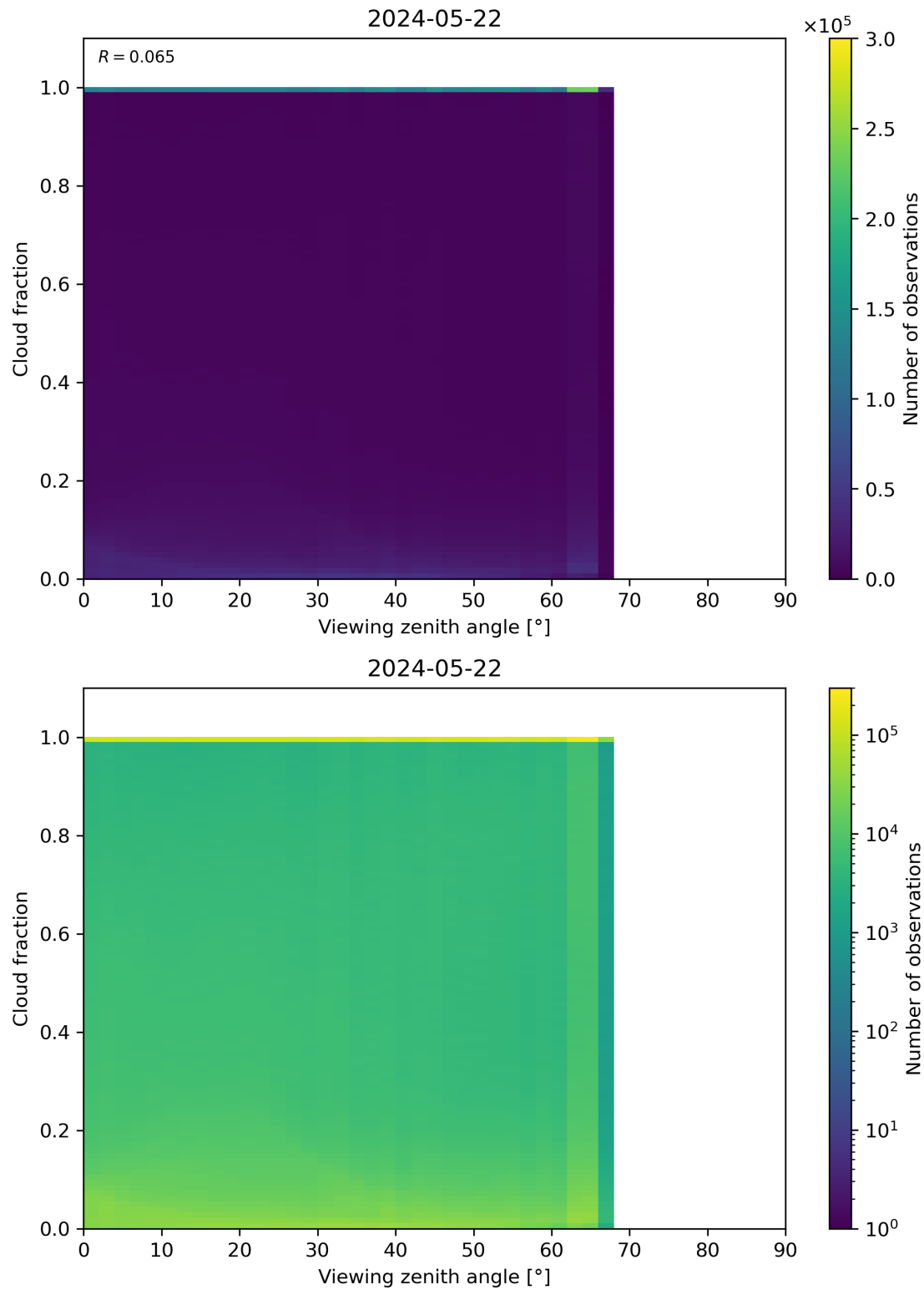
Figure 120: Scatter density plot of “Viewing zenith angle” against “Cloud fraction” for 2024-05-21 to 2024-05-23.
