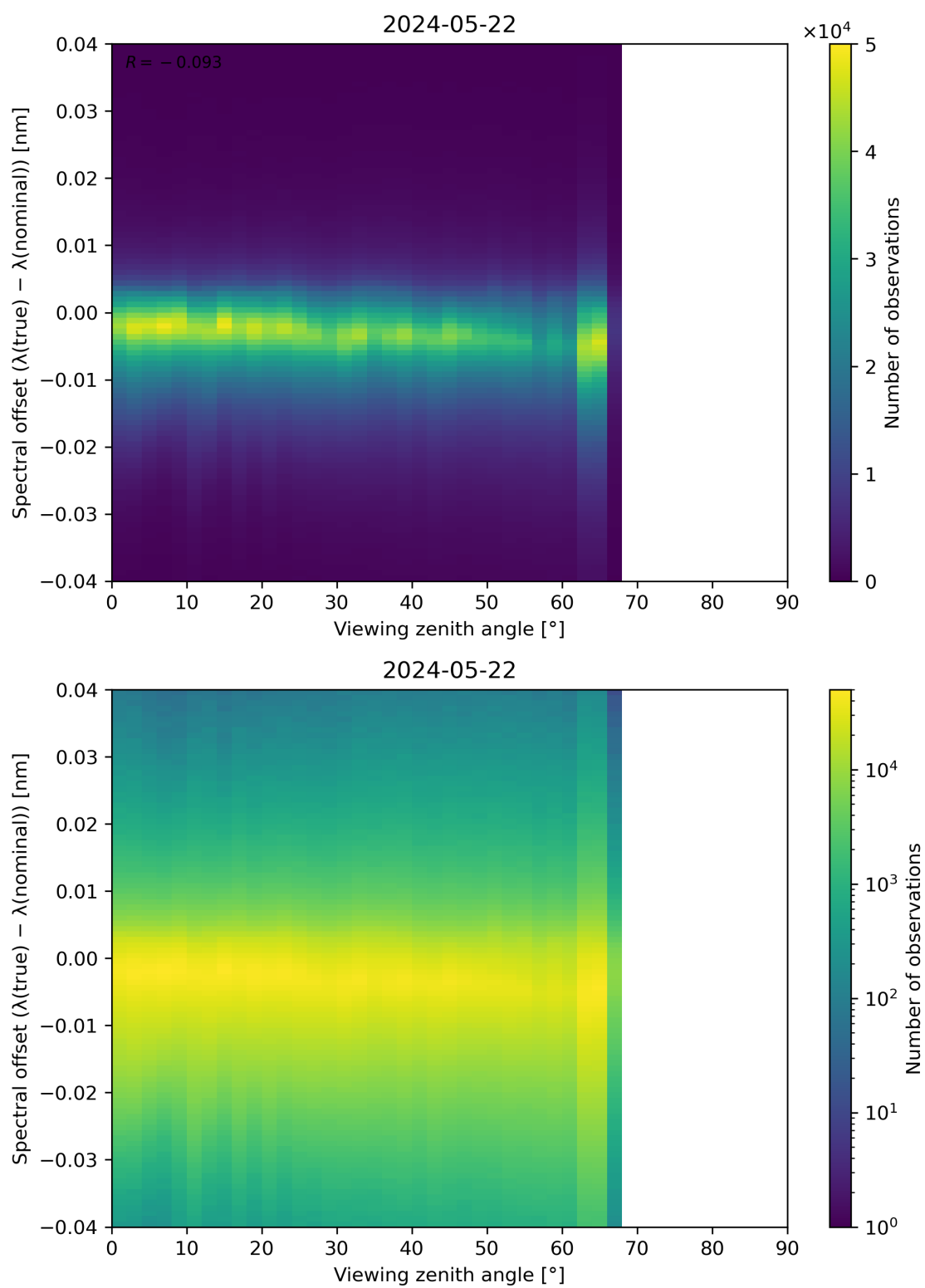
Figure 128: Scatter density plot of “Viewing zenith angle” against “Spectral offset ( \lambda(\text{true}) - \lambda(\text{nominal}) )” for 2024-05-21 to 2024-05-23.
