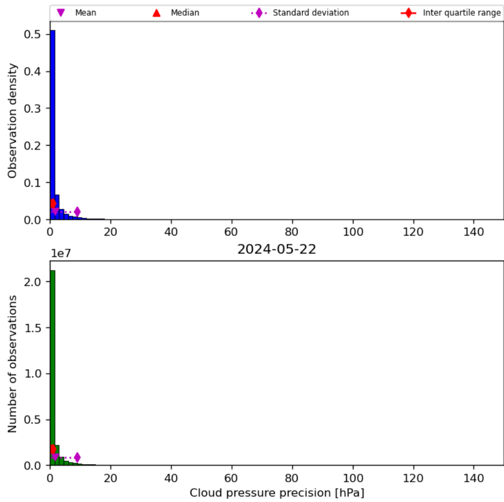
Figure 31: Histogram of “Cloud pressure precision” for 2024-05-21 to 2024-05-23
