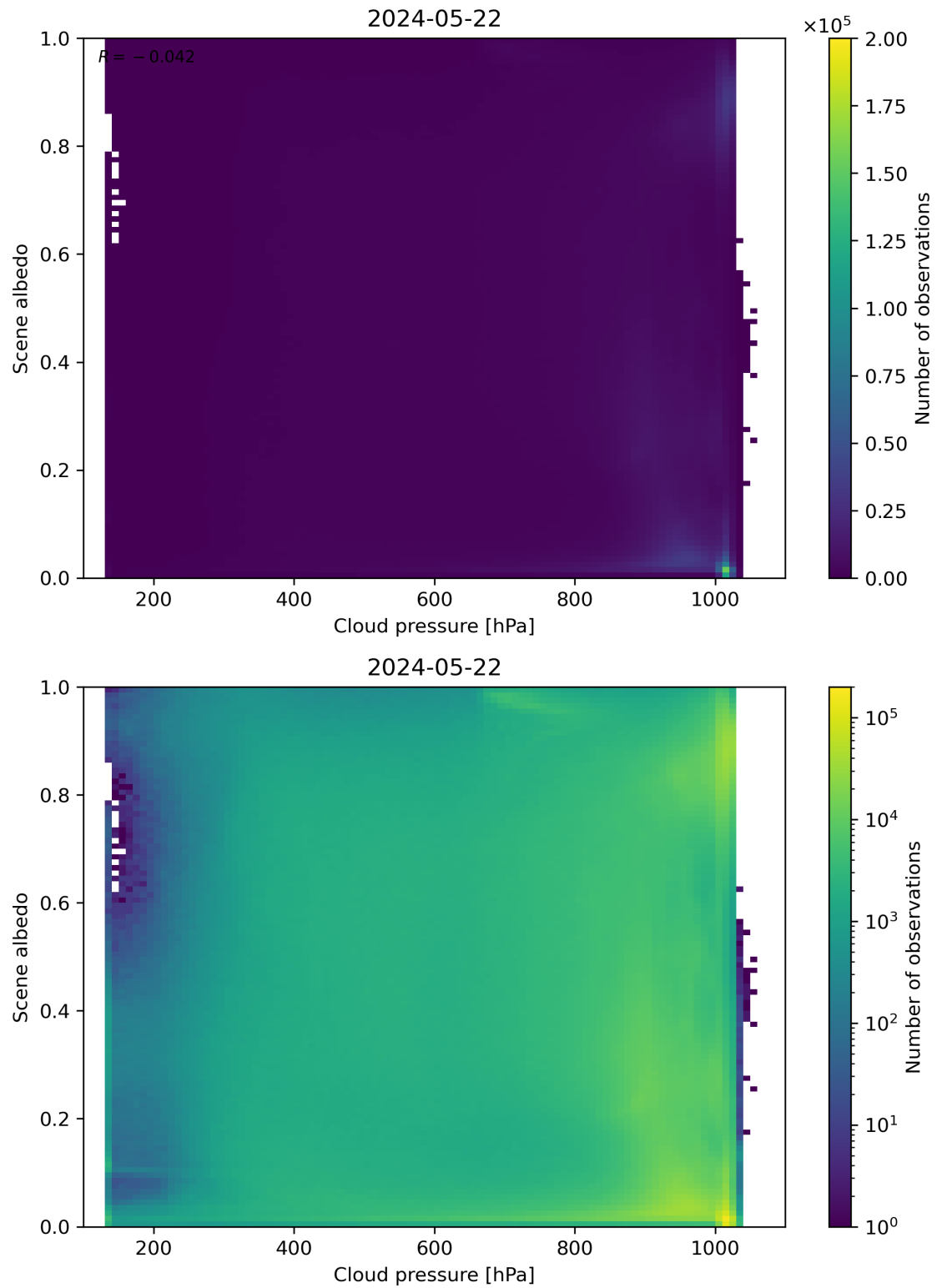
Figure 83: Scatter density plot of “Cloud pressure” against “Scene albedo” for 2024-05-21 to 2024-05-23.
