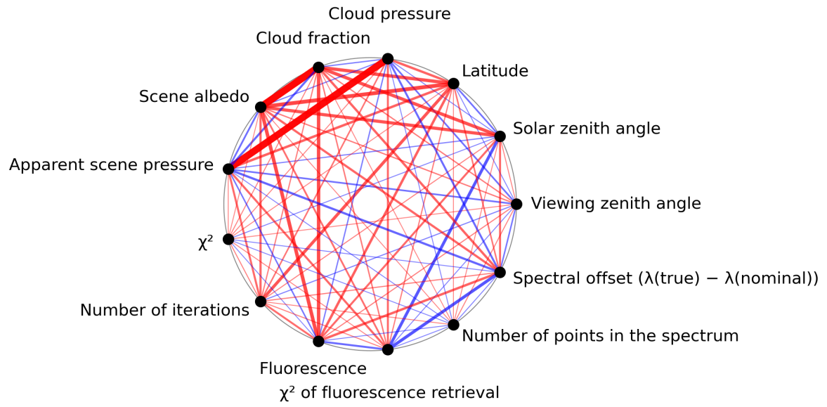
Figure 1: Map of correlation graph for 2024-05-21 to 2024-05-23.
