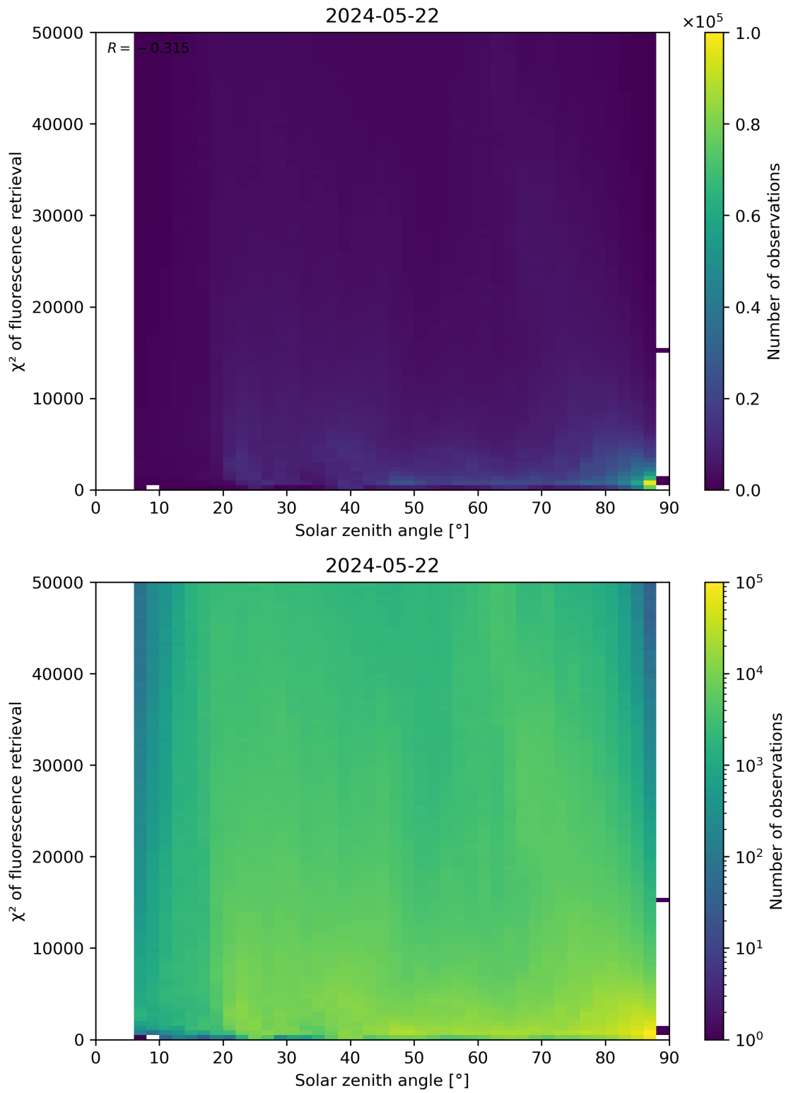
Figure 109: Scatter density plot of “Solar zenith angle” against “ \chi^2 of fluorescence retrieval” for 2024-05-21 to 2024-05-23.
