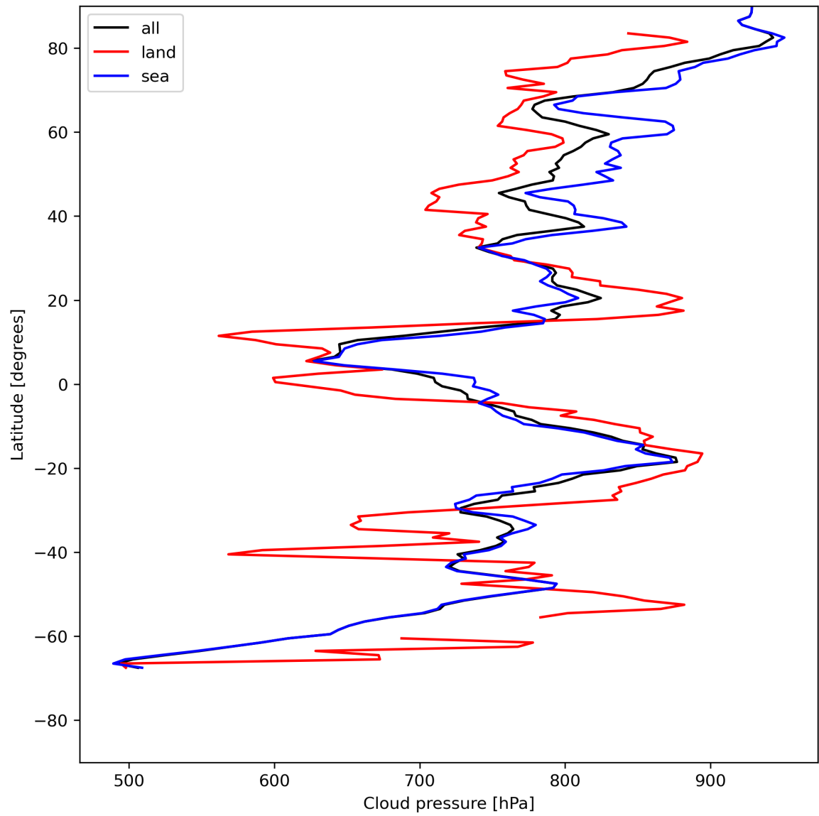
Figure 13: Zonal average of “Cloud pressure” for 2024-05-21 to 2024-05-23.
