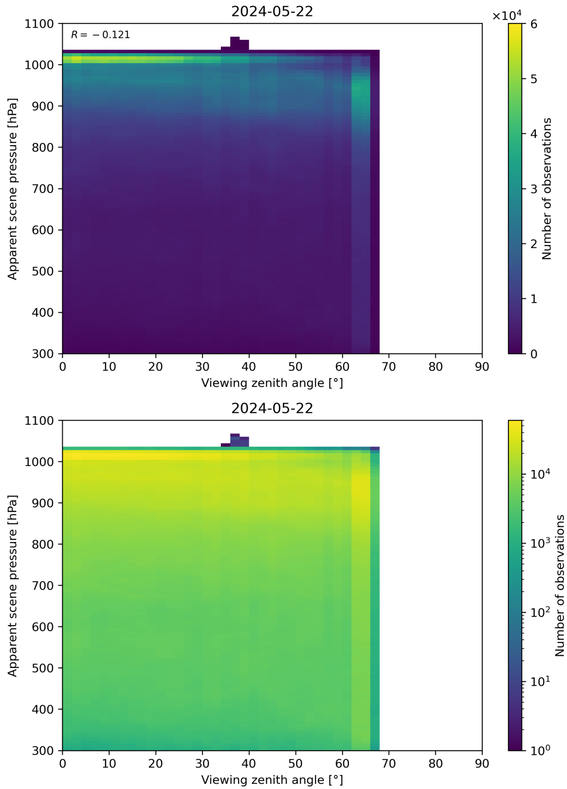
Figure 118: Scatter density plot of “Viewing zenith angle” against “Apparent scene pressure” for 2024-05-21 to 2024-05-23.
