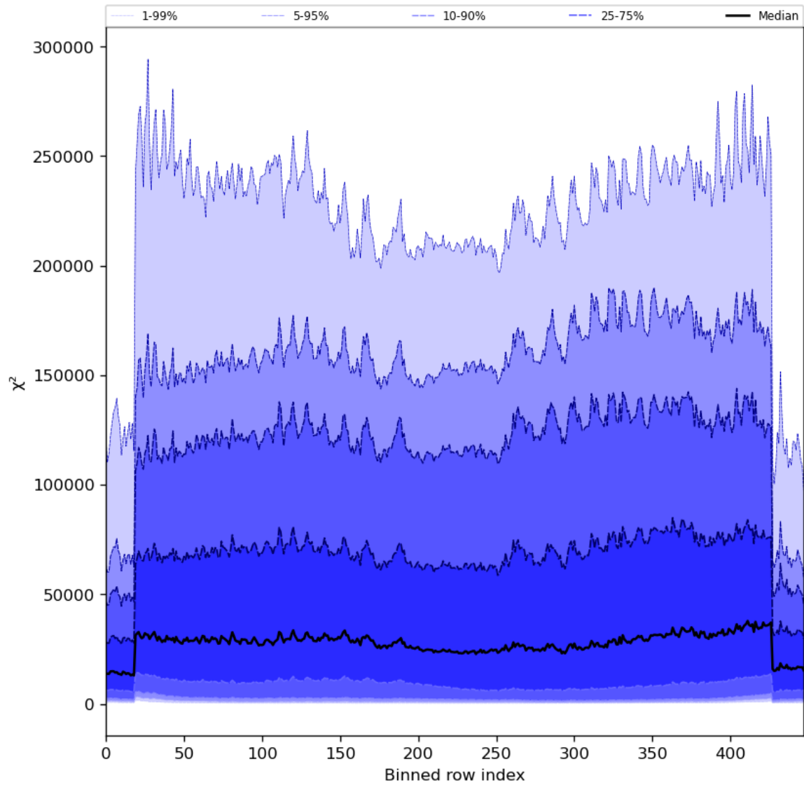
Figure 55: Along track statistics of “ \chi^2 ” for 2024-05-21 to 2024-05-23
