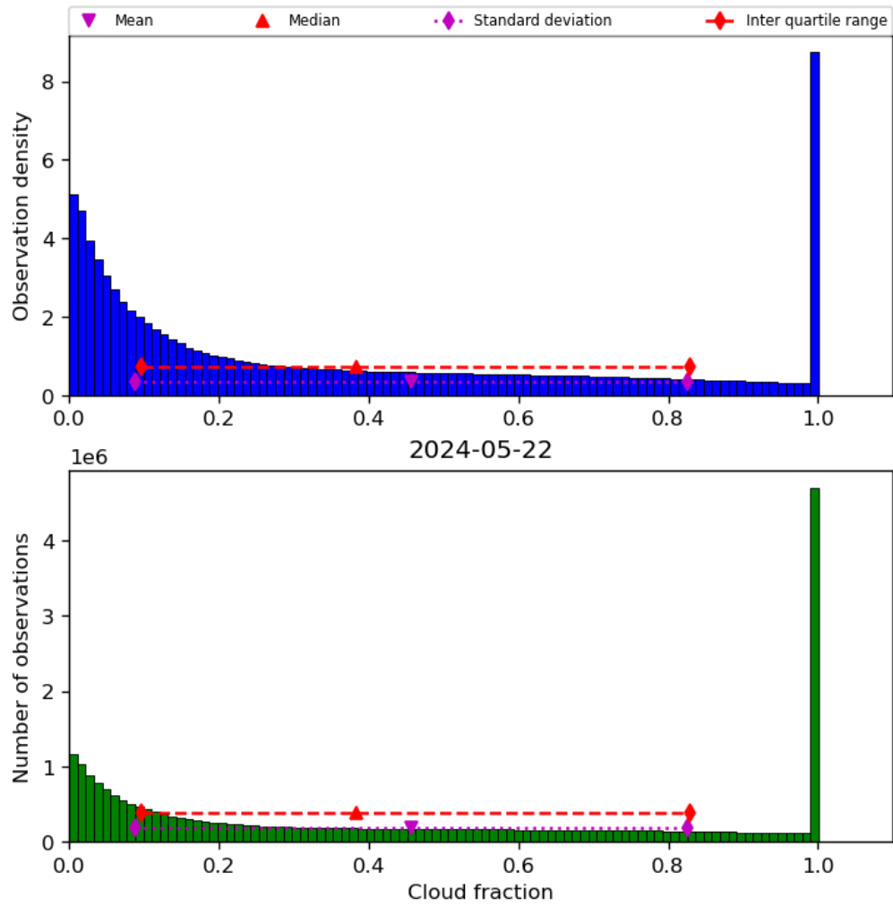
Figure 32: Histogram of “Cloud fraction” for 2024-05-21 to 2024-05-23
