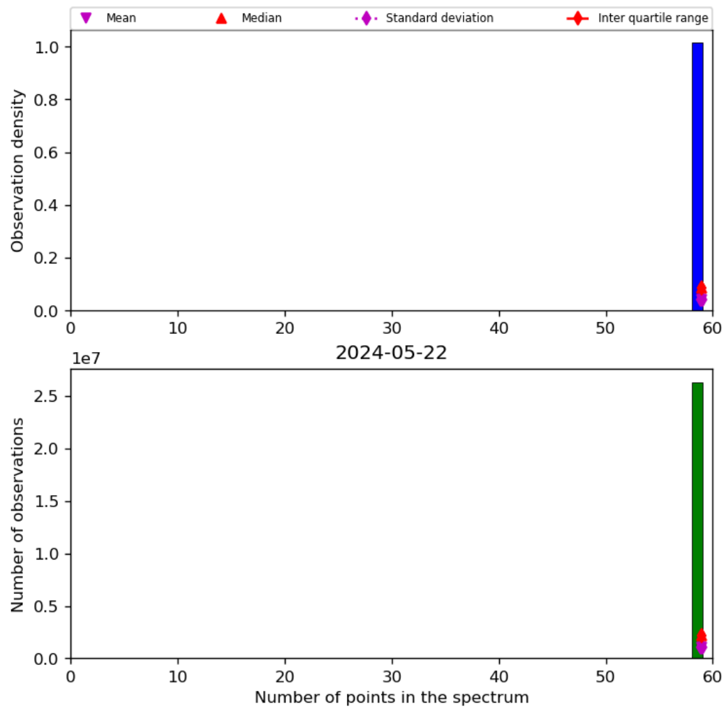
Figure 44: Histogram of “Number of points in the spectrum” for 2024-05-21 to 2024-05-23
