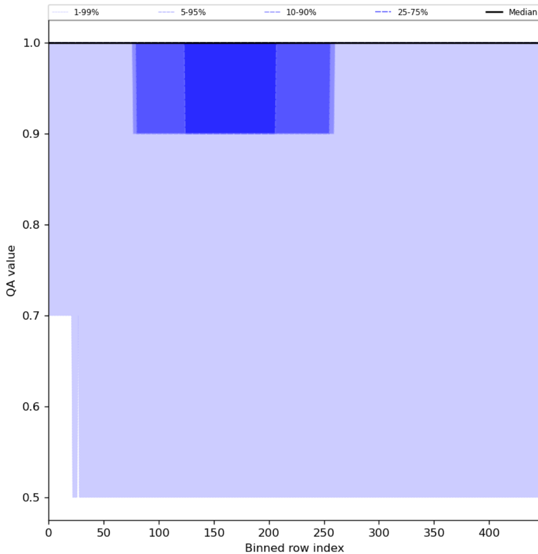
Figure 46: Along track statistics of “QA value” for 2024-05-21 to 2024-05-23
