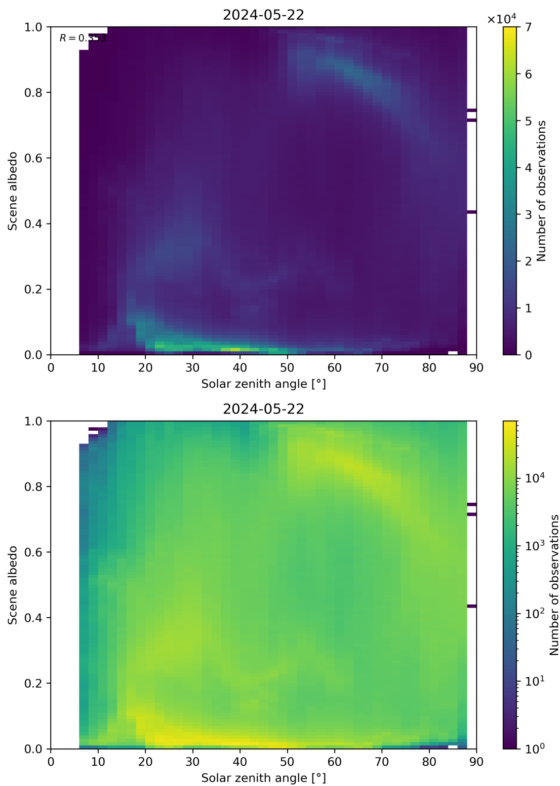
Figure 116: Scatter density plot of “Solar zenith angle” against “Scene albedo” for 2024-05-21 to 2024-05-23.
