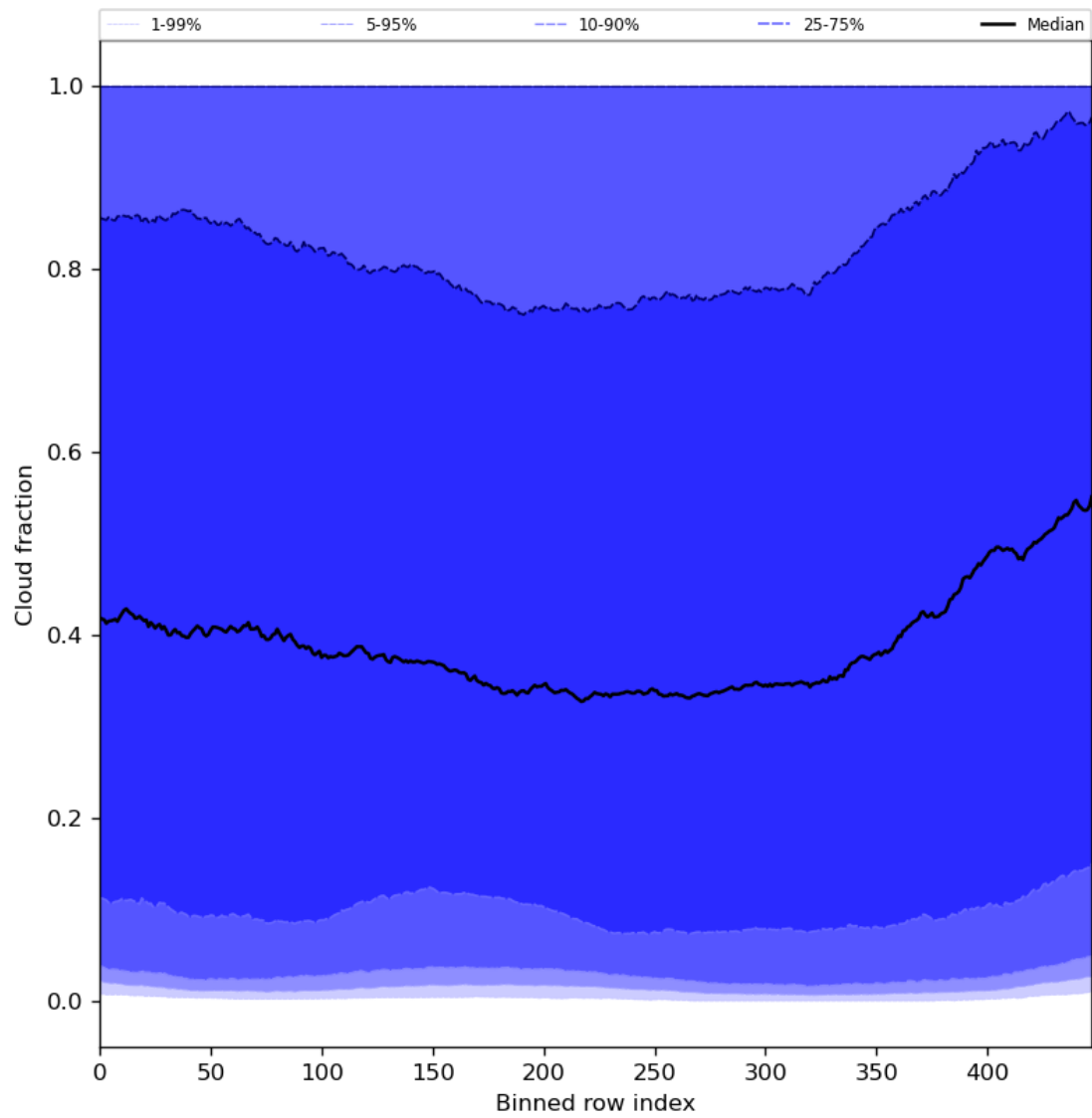
Figure 49: Along track statistics of “Cloud fraction” for 2024-05-21 to 2024-05-23
