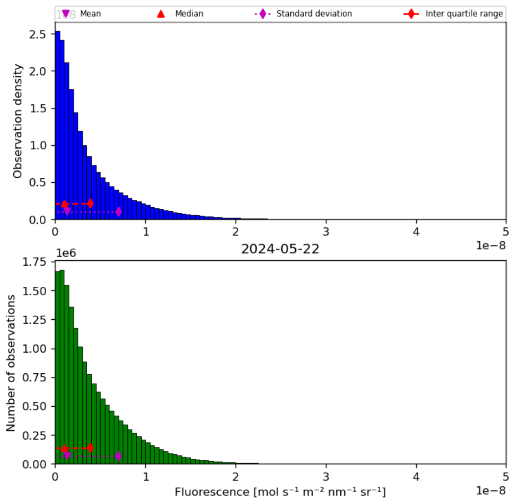
Figure 40: Histogram of “Fluorescence” for 2024-05-21 to 2024-05-23
