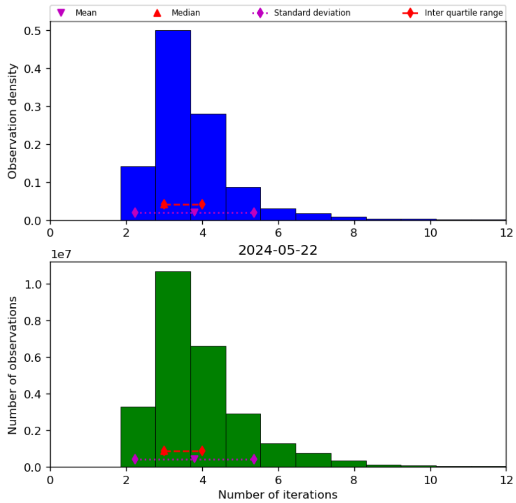
Figure 39: Histogram of “Number of iterations” for 2024-05-21 to 2024-05-23
