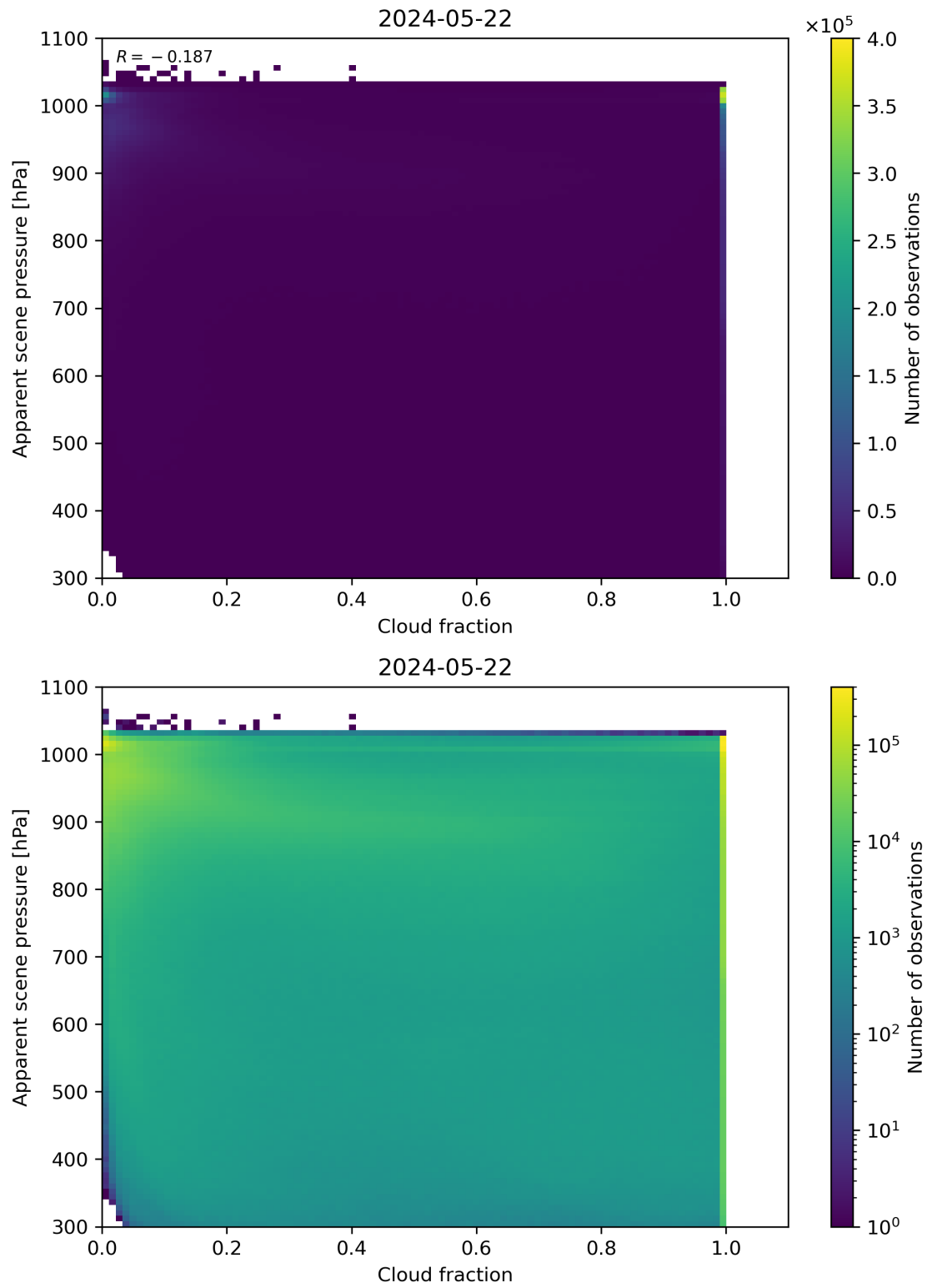
Figure 70: Scatter density plot of “Cloud fraction” against “Apparent scene pressure” for 2024-05-21 to 2024-05-23.
