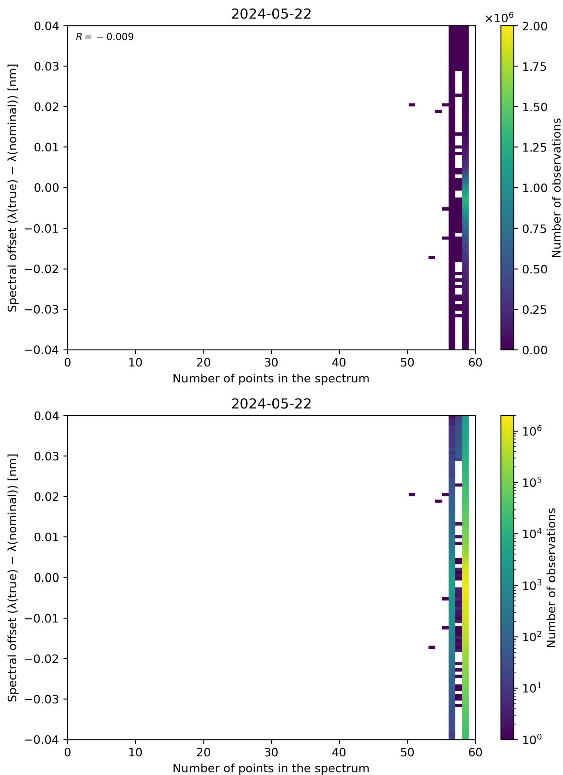
Figure 101: Scatter density plot of “Number of points in the spectrum” against “Spectral offset ( \lambda(\text{true}) - \lambda(\text{nominal}) )” for 2024-05-21 to 2024-05-23.
