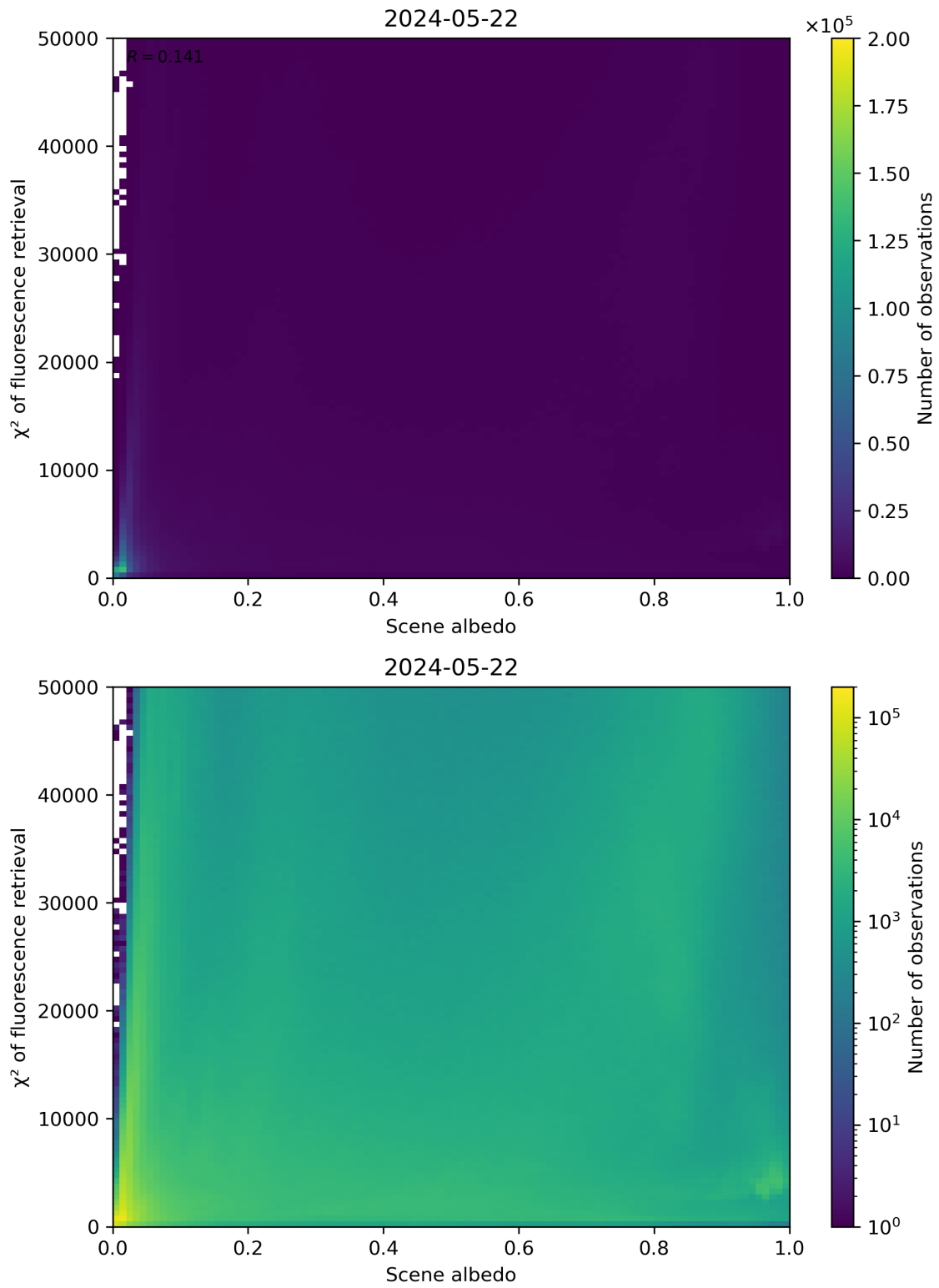
Figure 103: Scatter density plot of “Scene albedo” against “ \chi^2 of fluorescence retrieval” for 2024-05-21 to 2024-05-23.
