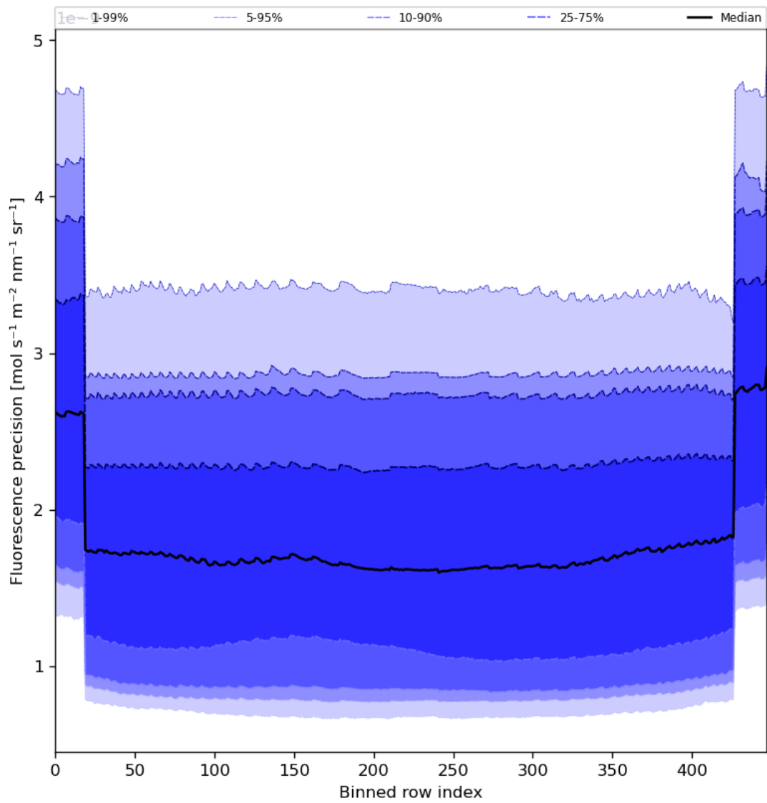
Figure 58: Along track statistics of “Fluorescence precision” for 2024-05-21 to 2024-05-23
