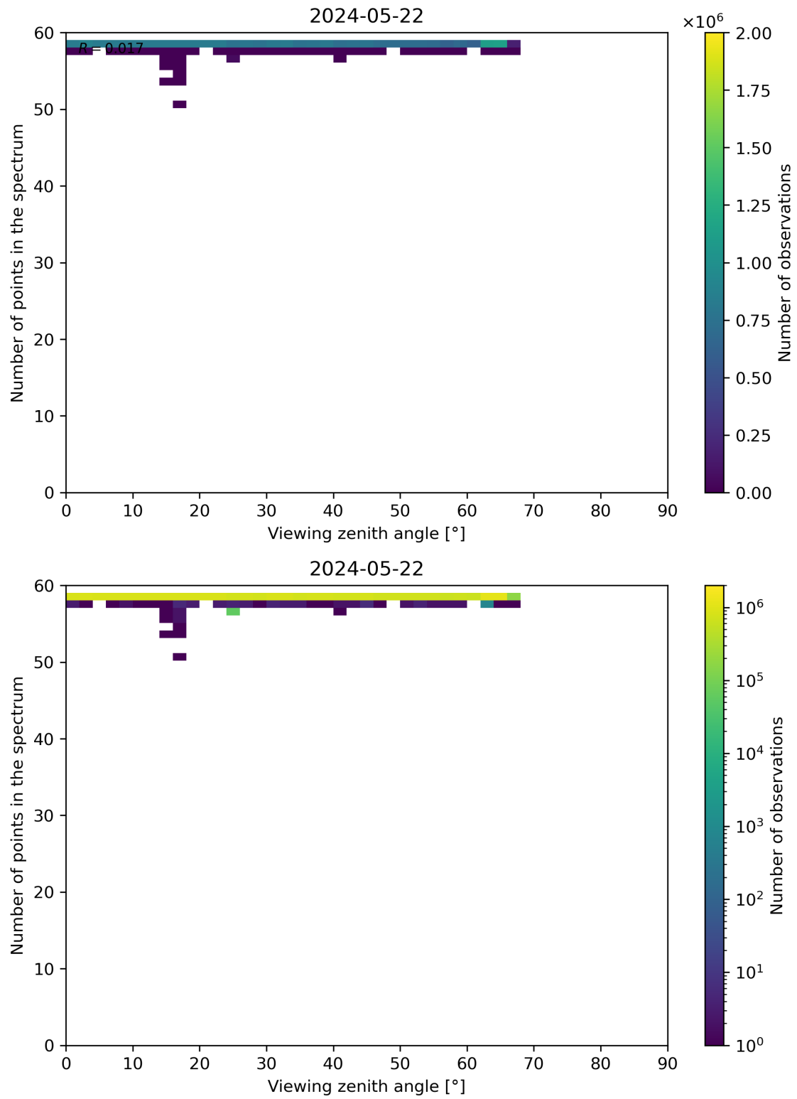
Figure 125: Scatter density plot of “Viewing zenith angle” against “Number of points in the spectrum” for 2024-05-21 to 2024-05-23.
