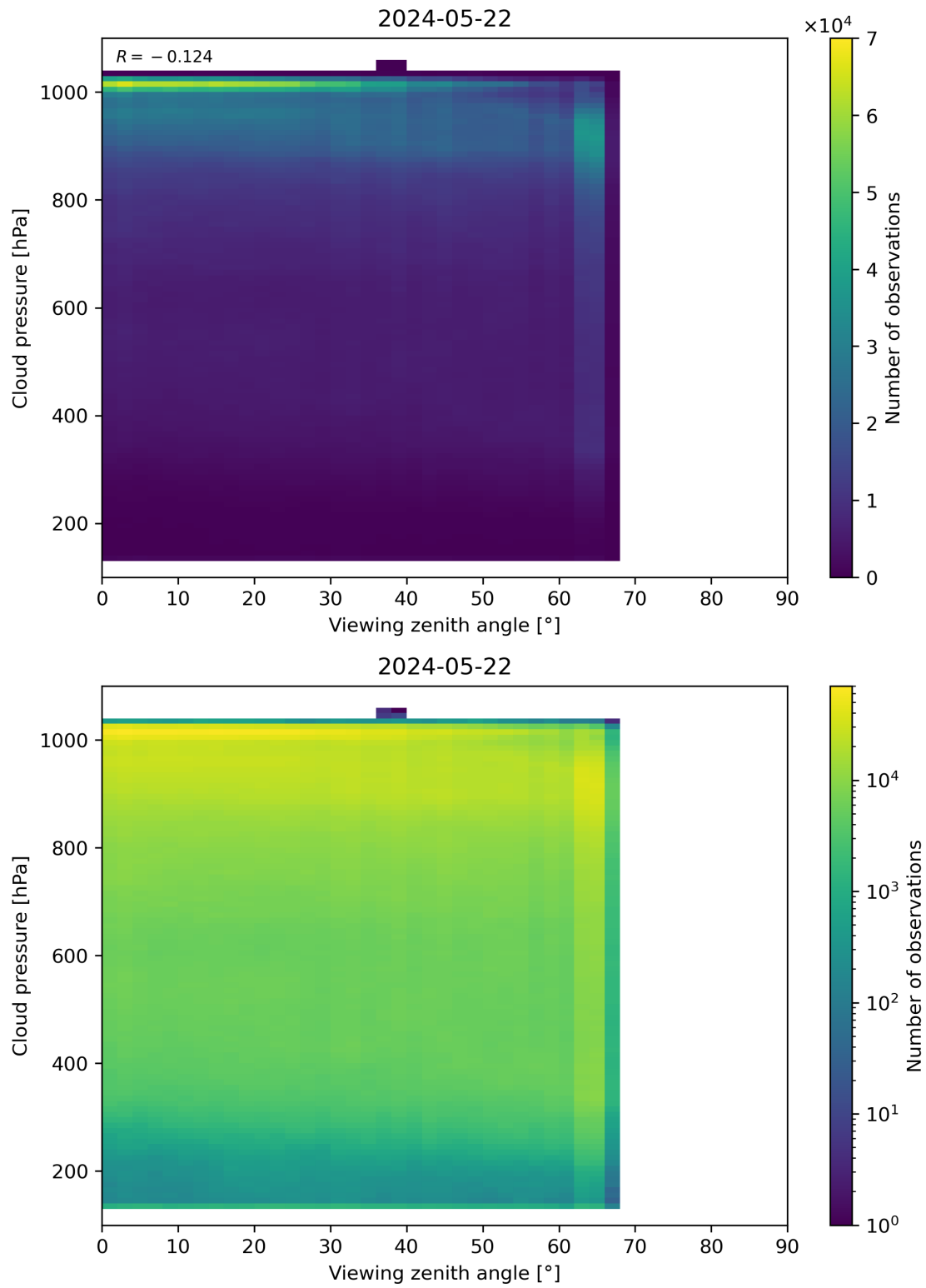
Figure 121: Scatter density plot of “Viewing zenith angle” against “Cloud pressure” for 2024-05-21 to 2024-05-23.
