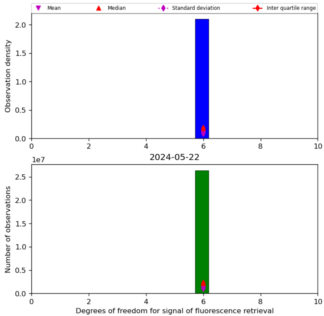
Figure 43: Histogram of “Degrees of freedom for signal of fluorescence retrieval” for 2024-05-21 to 2024-05-23
