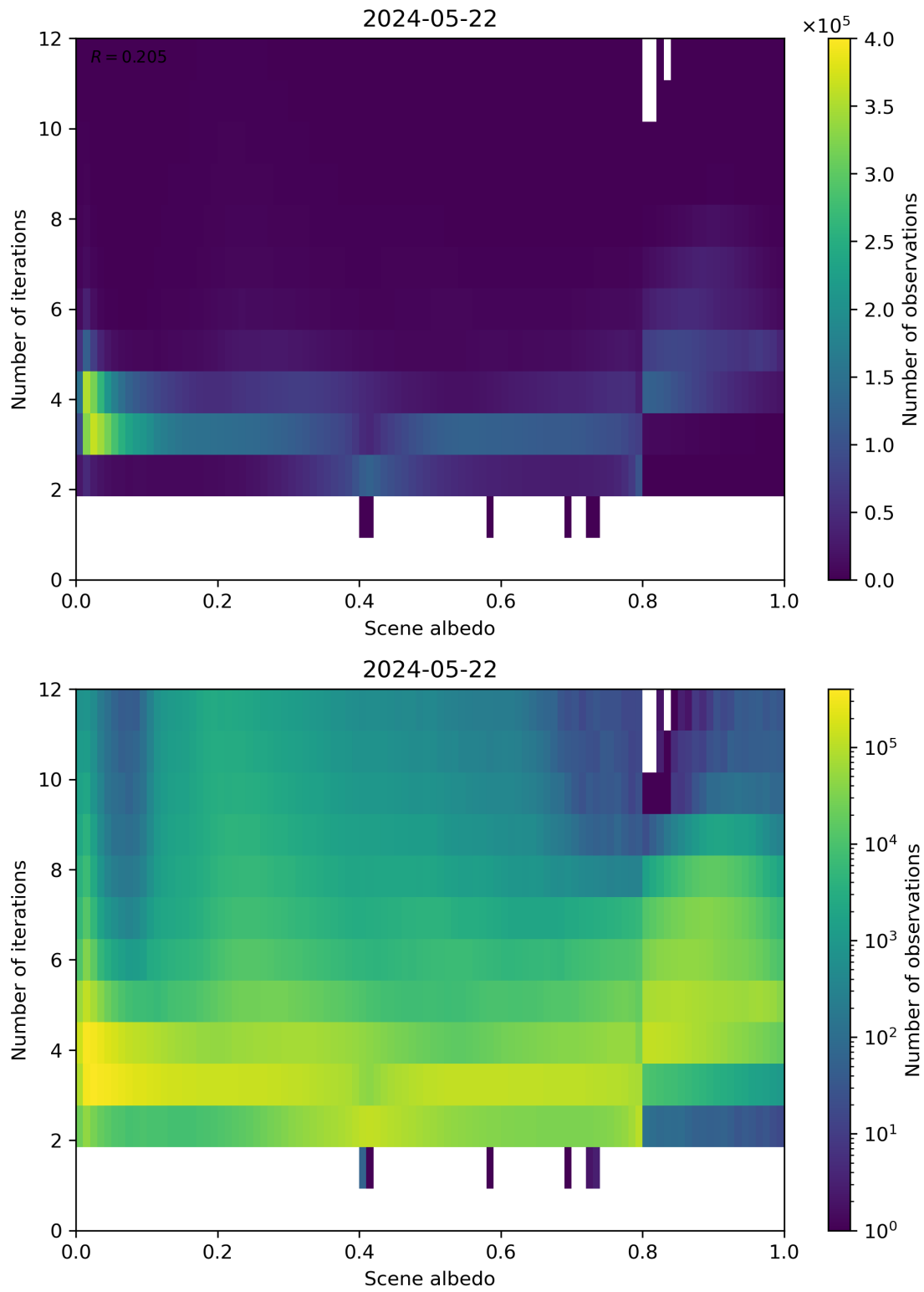
Figure 105: Scatter density plot of “Scene albedo” against “Number of iterations” for 2024-05-21 to 2024-05-23.
