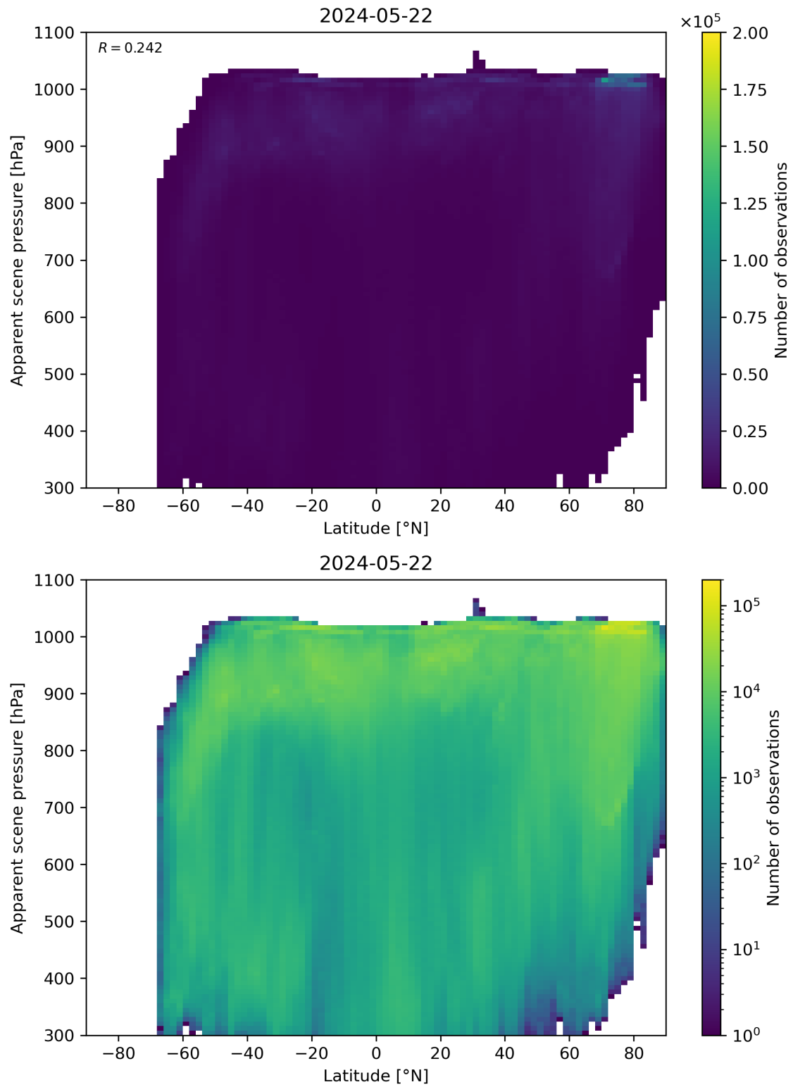
Figure 88: Scatter density plot of “Latitude” against “Apparent scene pressure” for 2024-05-21 to 2024-05-23.
