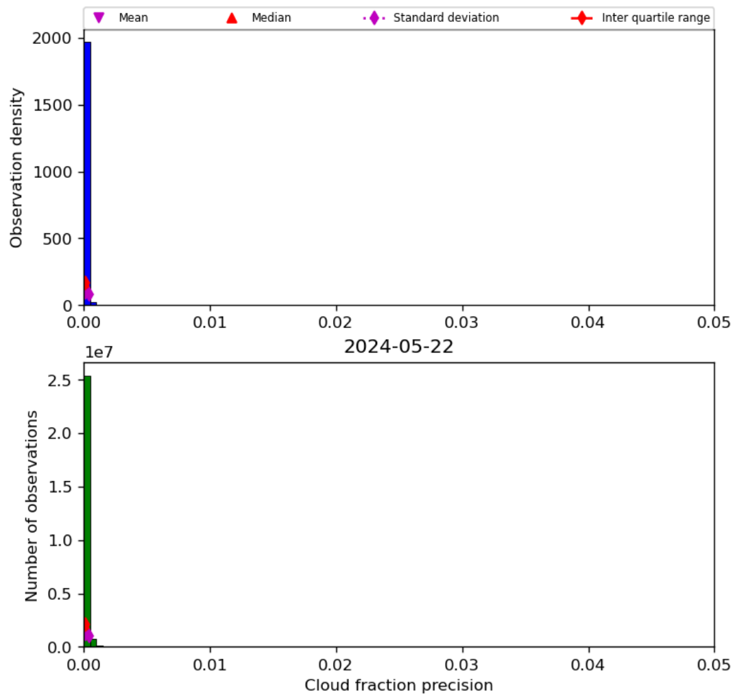
Figure 33: Histogram of “Cloud fraction precision” for 2024-05-21 to 2024-05-23
