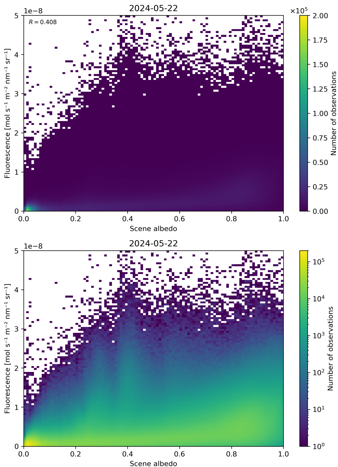
Figure 104: Scatter density plot of “Scene albedo” against “Fluorescence” for 2024-05-21 to 2024-05-23.
