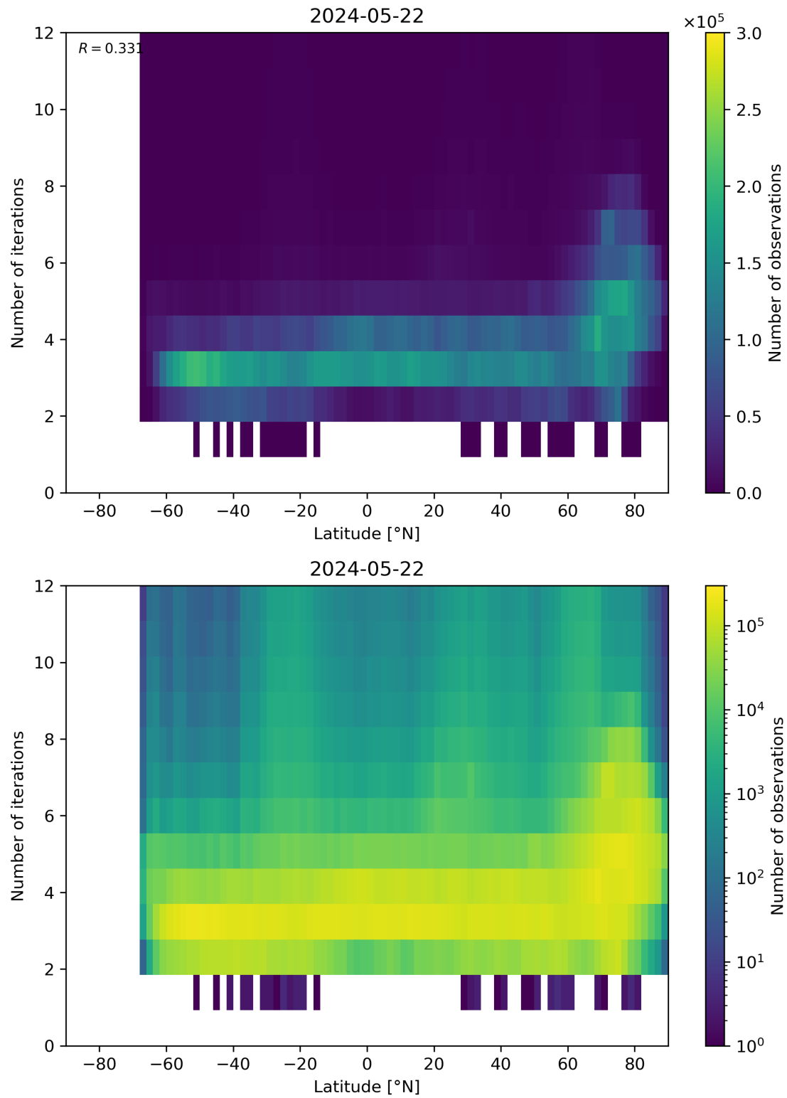
Figure 93: Scatter density plot of “Latitude” against “Number of iterations” for 2024-05-21 to 2024-05-23.
