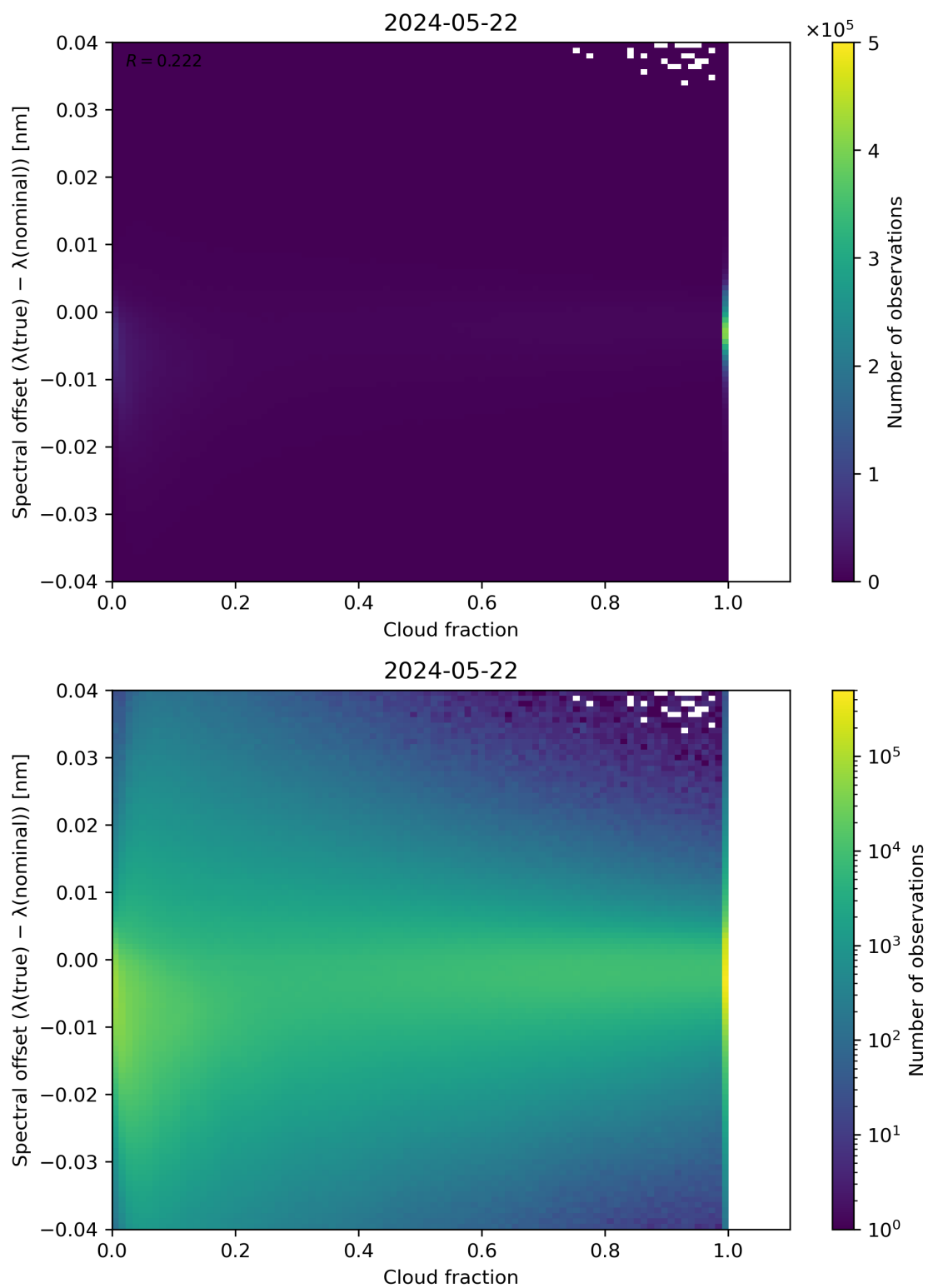
Figure 76: Scatter density plot of “Cloud fraction” against “Spectral offset ( \lambda(\text{true}) - \lambda(\text{nominal}) )” for 2024-05-21 to 2024-05-23.
