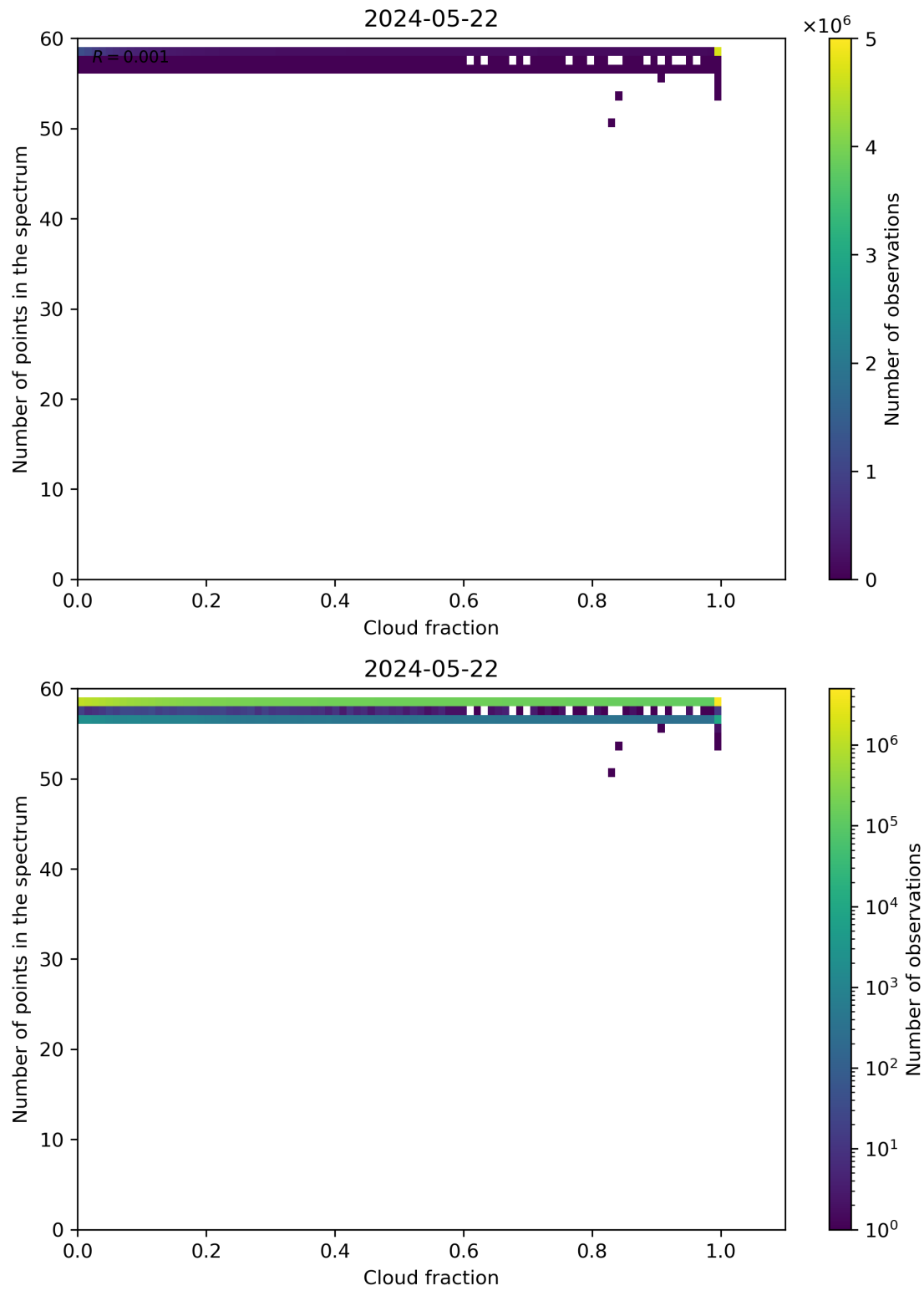
Figure 74: Scatter density plot of “Cloud fraction” against “Number of points in the spectrum” for 2024-05-21 to 2024-05-23.
