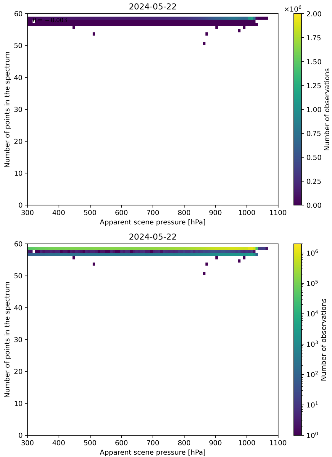
Figure 66: Scatter density plot of “Apparent scene pressure” against “Number of points in the spectrum” for 2024-05-21 to 2024-05-23.
