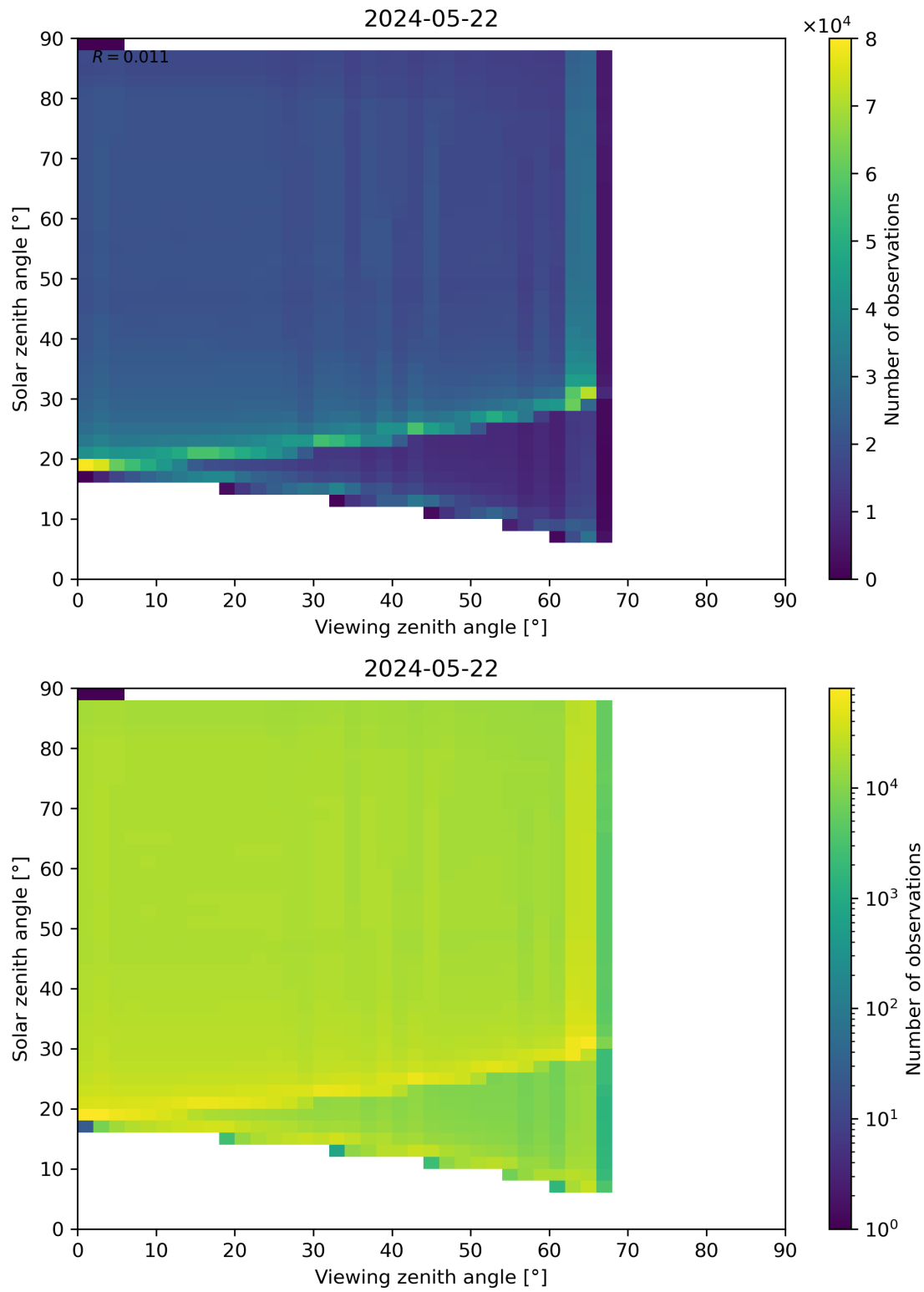
Figure 127: Scatter density plot of “Viewing zenith angle” against “Solar zenith angle” for 2024-05-21 to 2024-05-23.
