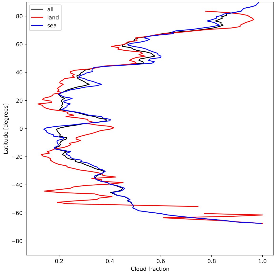
Figure 15: Zonal average of “Cloud fraction” for 2024-05-21 to 2024-05-23.
