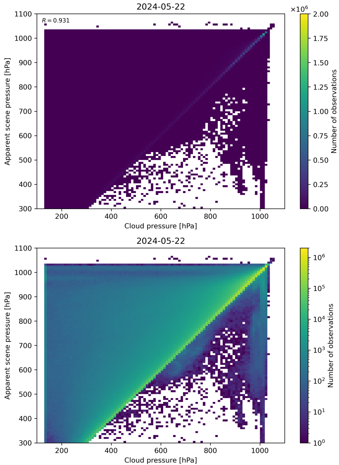
Figure 77: Scatter density plot of “Cloud pressure” against “Apparent scene pressure” for 2024-05-21 to 2024-05-23.
