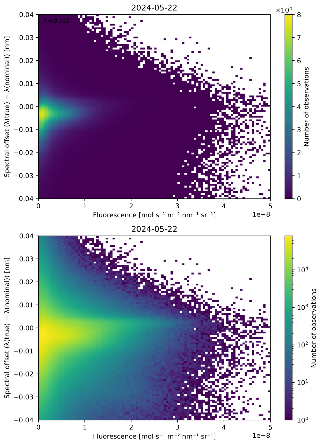
Figure 87: Scatter density plot of “Fluorescence” against “Spectral offset ( \lambda(\text{true}) - \lambda(\text{nominal}) )” for 2024-05-21 to 2024-05-23.
