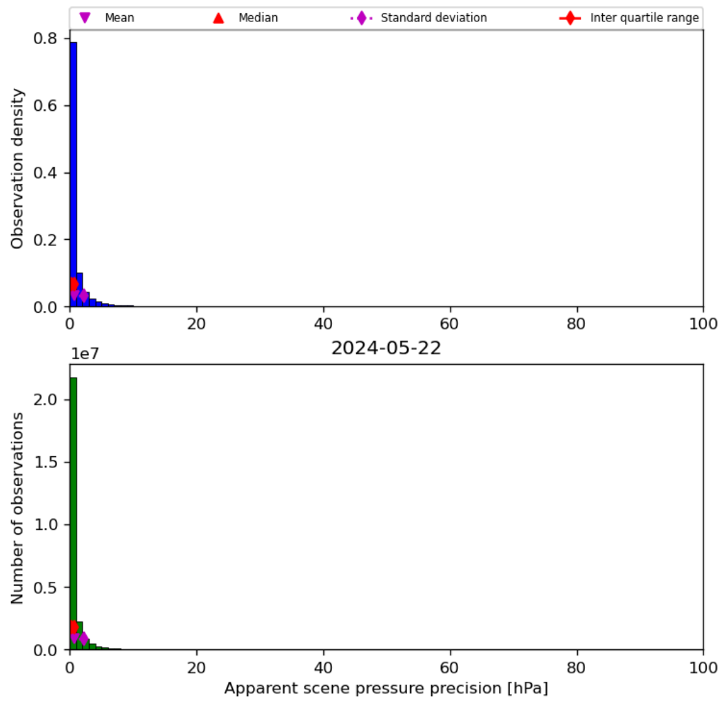
Figure 37: Histogram of “Apparent scene pressure precision” for 2024-05-21 to 2024-05-23
