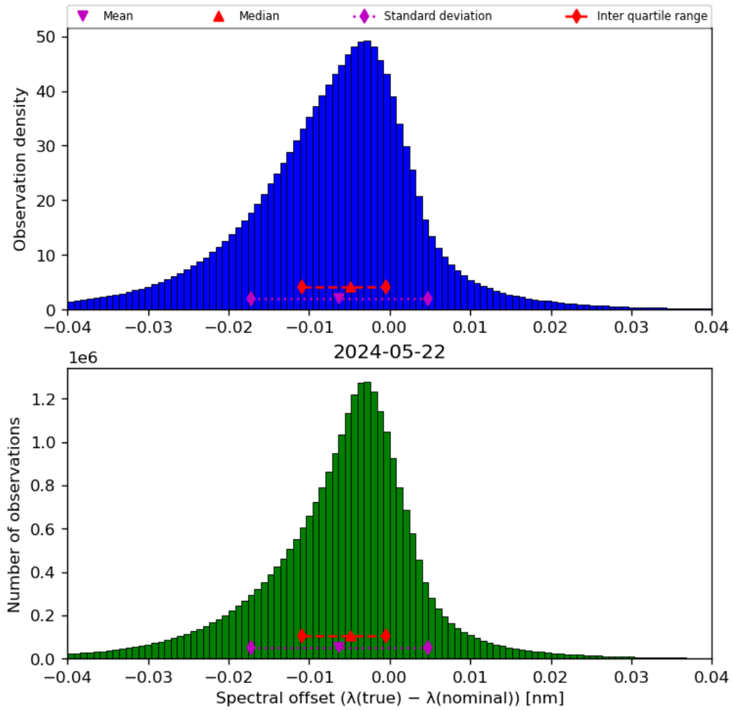
Figure 45: Histogram of “Spectral offset ( \lambda(\text{true}) - \lambda(\text{nominal}) )” for 2024-05-21 to 2024-05-23
