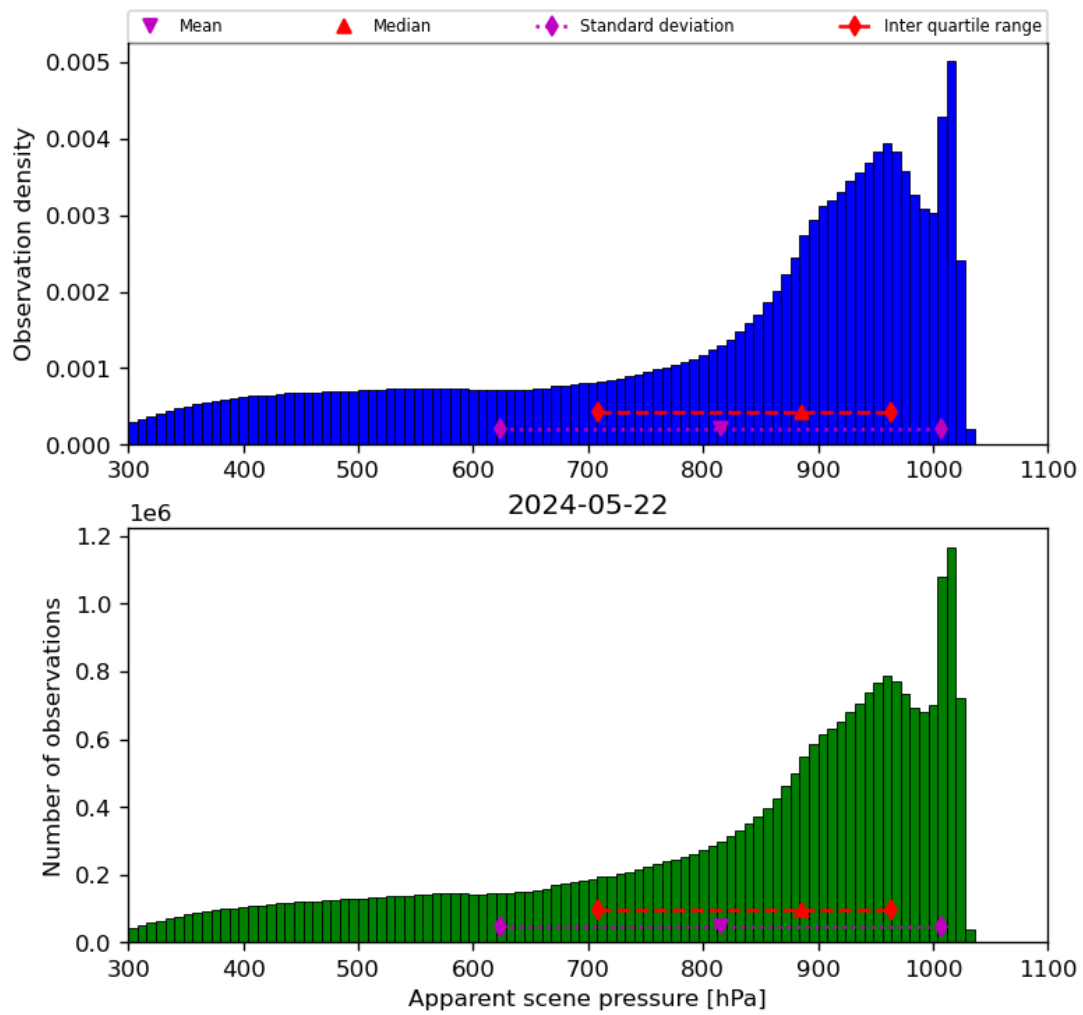
Figure 36: Histogram of “Apparent scene pressure” for 2024-05-21 to 2024-05-23
