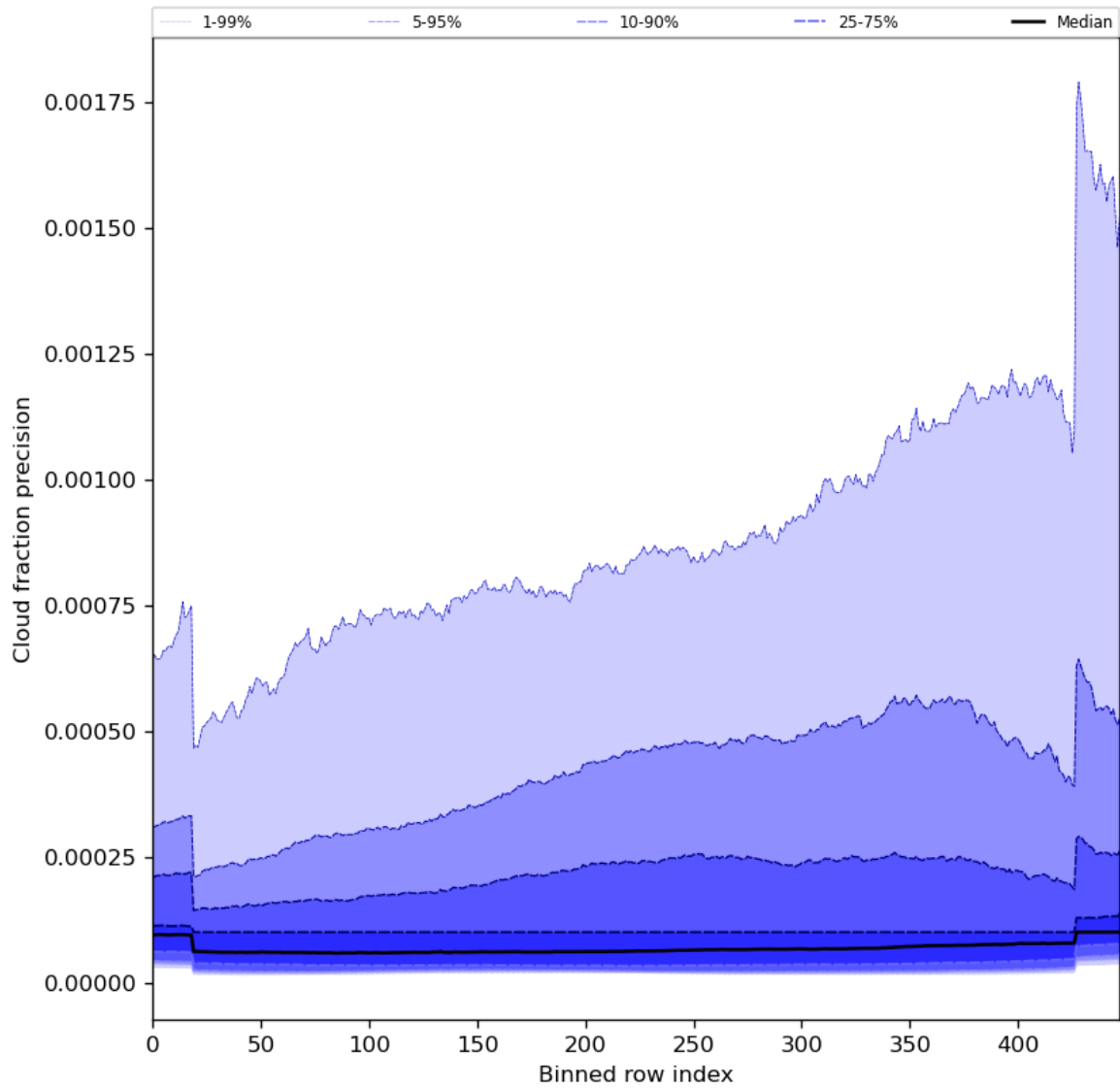
Figure 50: Along track statistics of “Cloud fraction precision” for 2024-05-21 to 2024-05-23
