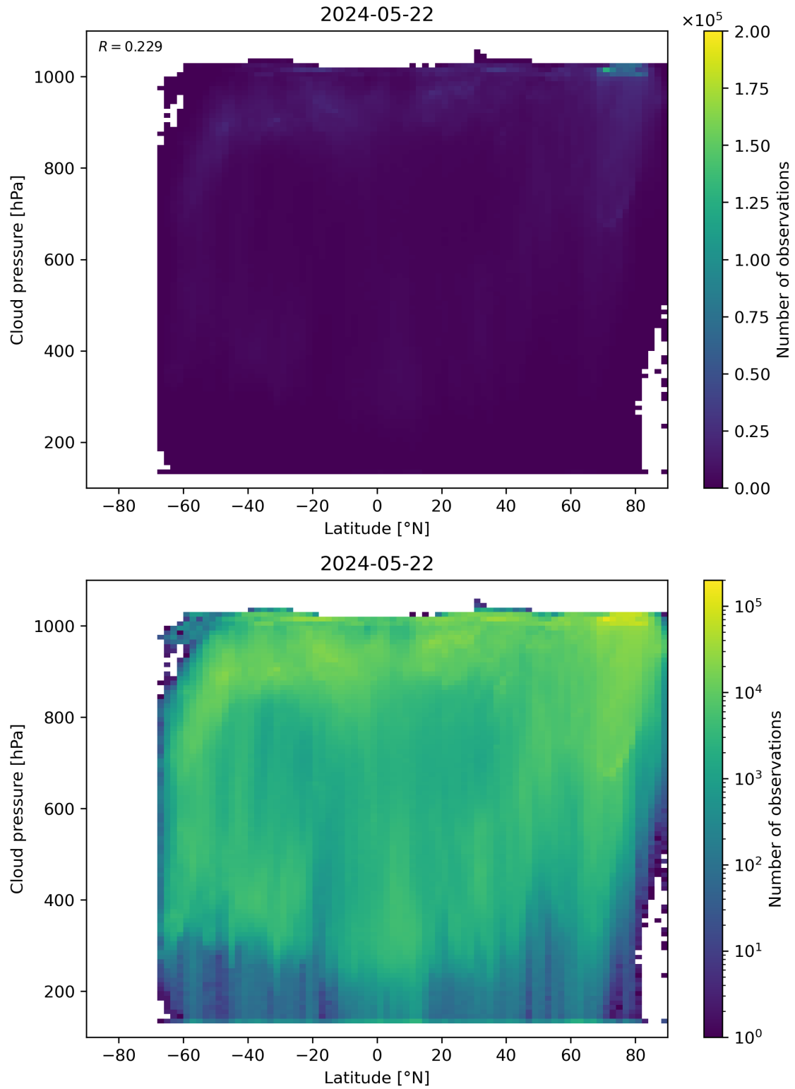
Figure 91: Scatter density plot of “Latitude” against “Cloud pressure” for 2024-05-21 to 2024-05-23.
