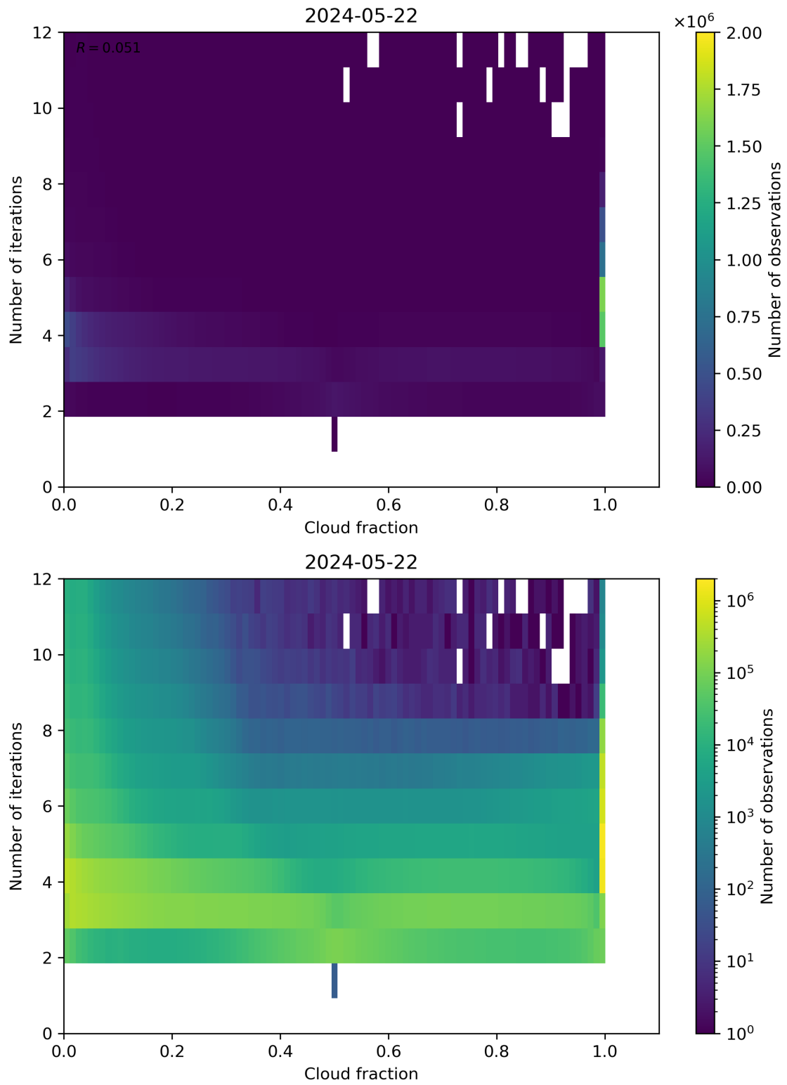
Figure 73: Scatter density plot of “Cloud fraction” against “Number of iterations” for 2024-05-21 to 2024-05-23.
