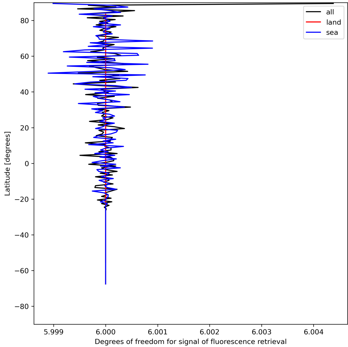
Figure 26: Zonal average of “Degrees of freedom for signal of fluorescence retrieval” for 2024-05-21 to 2024-05-23.
