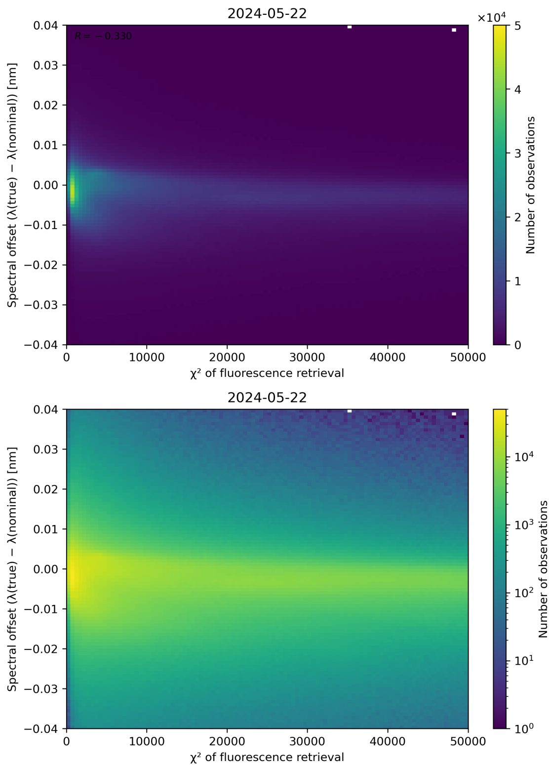
Figure 69: Scatter density plot of “ \chi^2 of fluorescence retrieval” against “Spectral offset ( \lambda(\text{true}) - \lambda(\text{nominal})) ” for 2024-05-21 to 2024-05-23.
