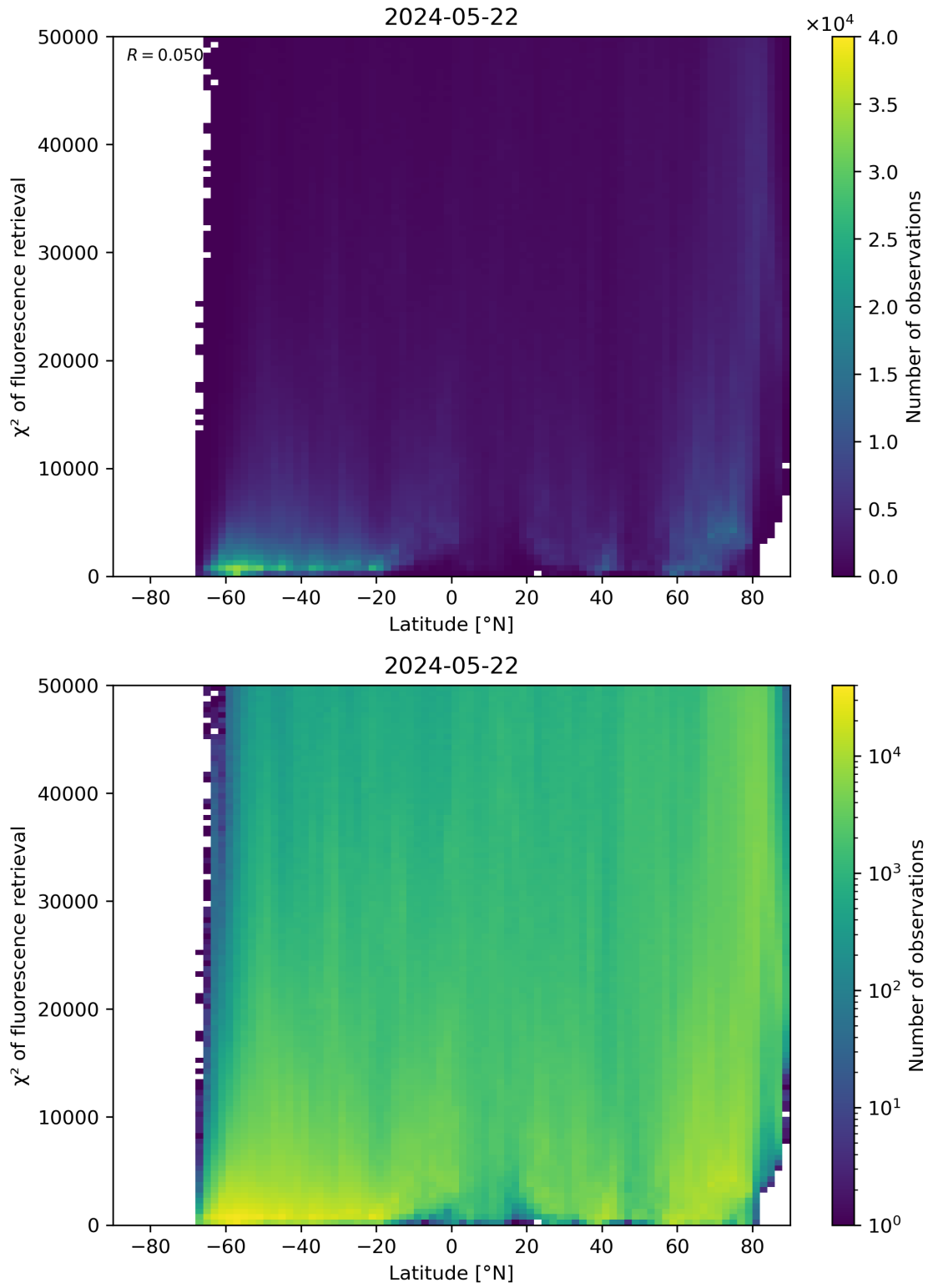
Figure 89: Scatter density plot of “Latitude” against “ \chi^2 of fluorescence retrieval” for 2024-05-21 to 2024-05-23.
