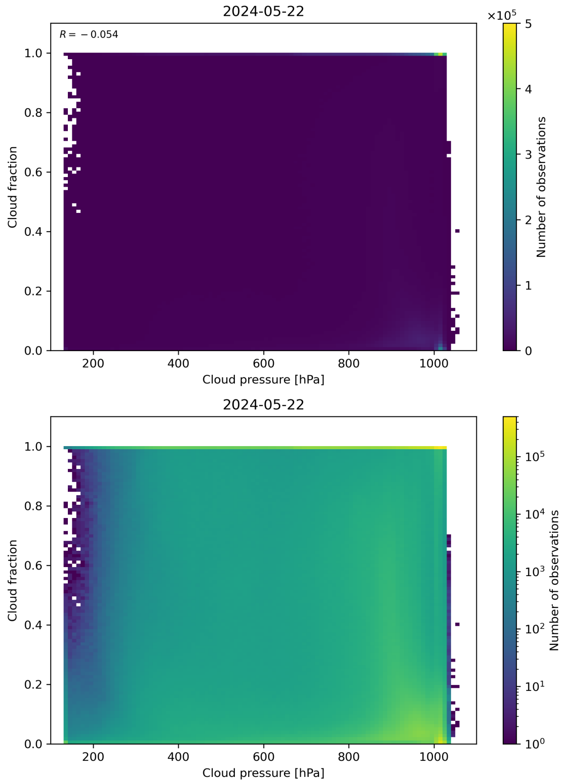
Figure 79: Scatter density plot of “Cloud pressure” against “Cloud fraction” for 2024-05-21 to 2024-05-23.
