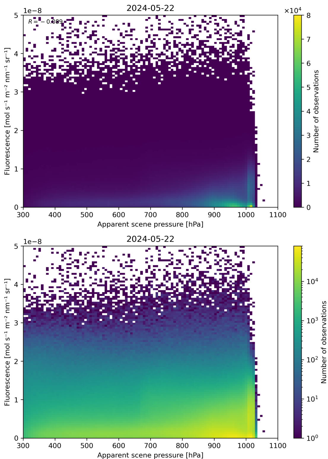
Figure 64: Scatter density plot of “Apparent scene pressure” against “Fluorescence” for 2024-05-21 to 2024-05-23.
