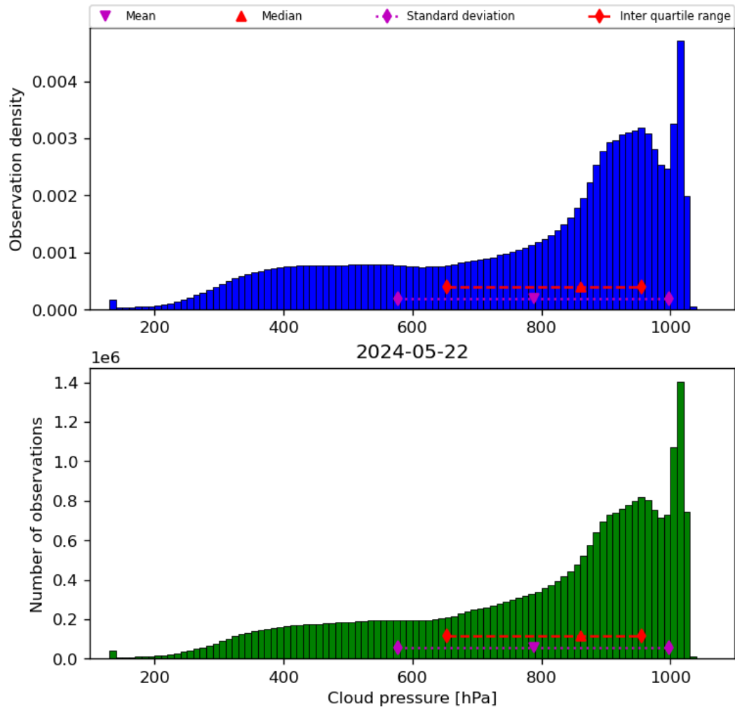
Figure 30: Histogram of “Cloud pressure” for 2024-05-21 to 2024-05-23
