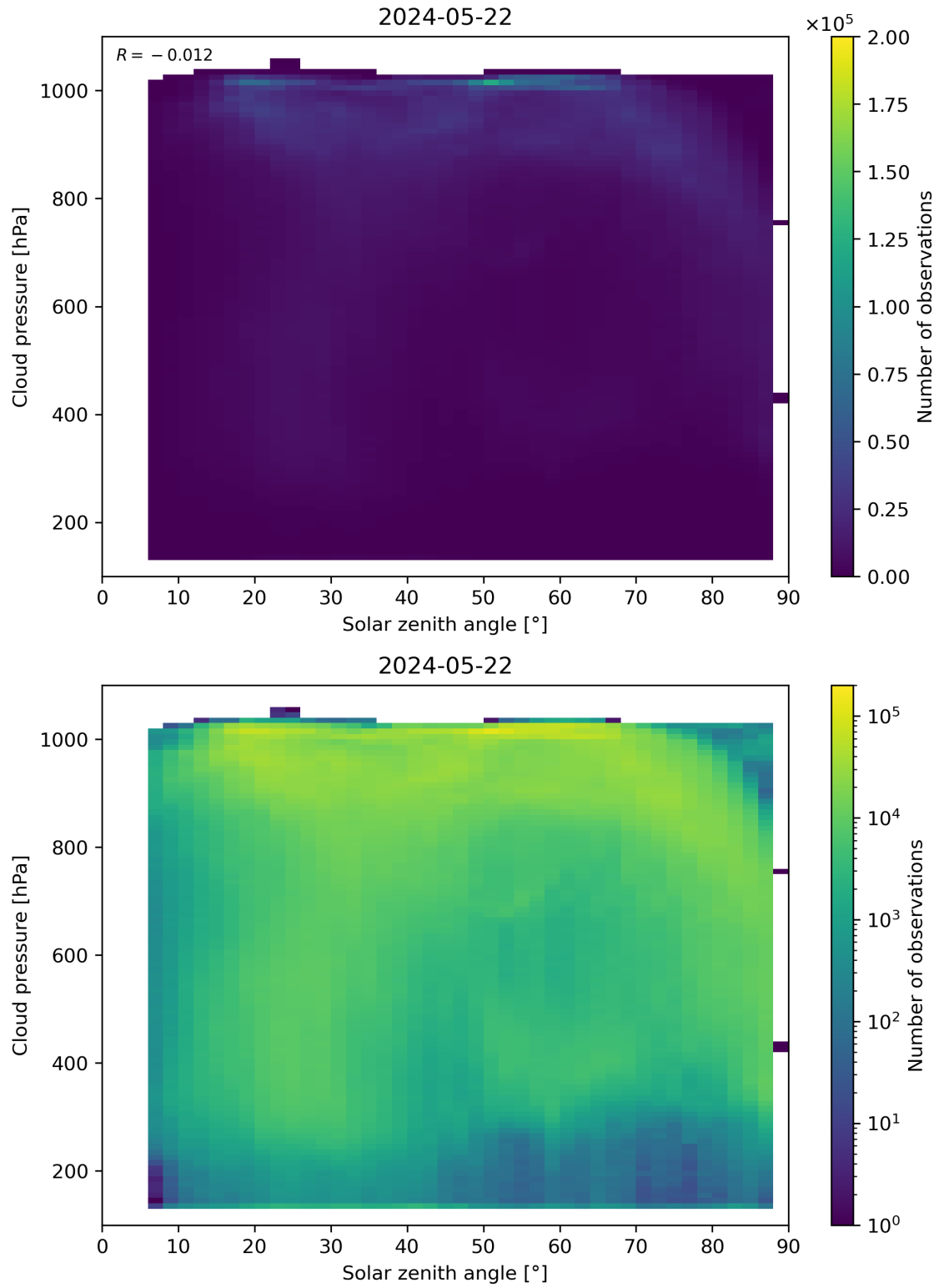
Figure 111: Scatter density plot of “Solar zenith angle” against “Cloud pressure” for 2024-05-21 to 2024-05-23.
