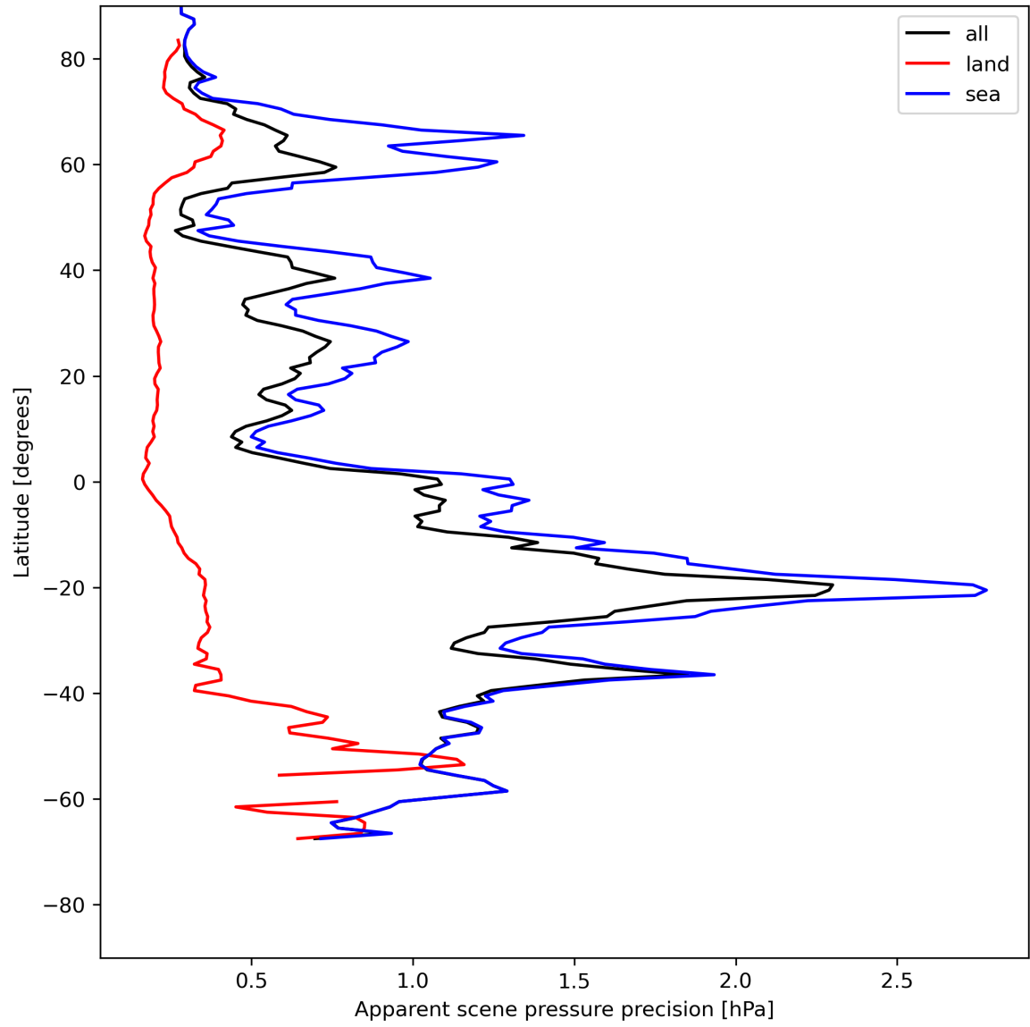
Figure 20: Zonal average of “Apparent scene pressure precision” for 2024-05-21 to 2024-05-23.
