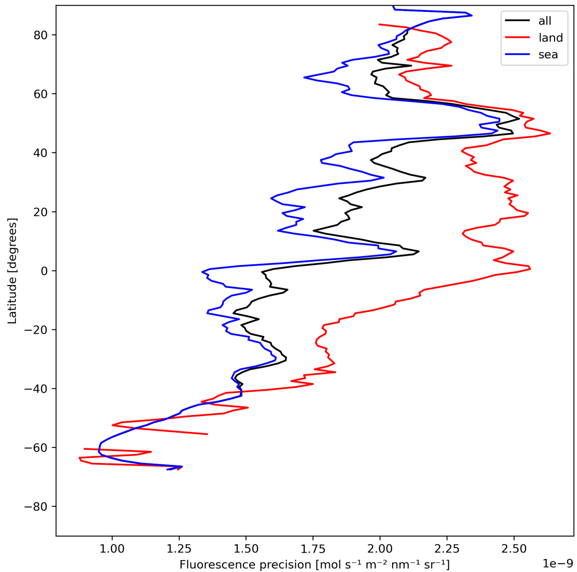
Figure 24: Zonal average of “Fluorescence precision” for 2024-05-21 to 2024-05-23.
