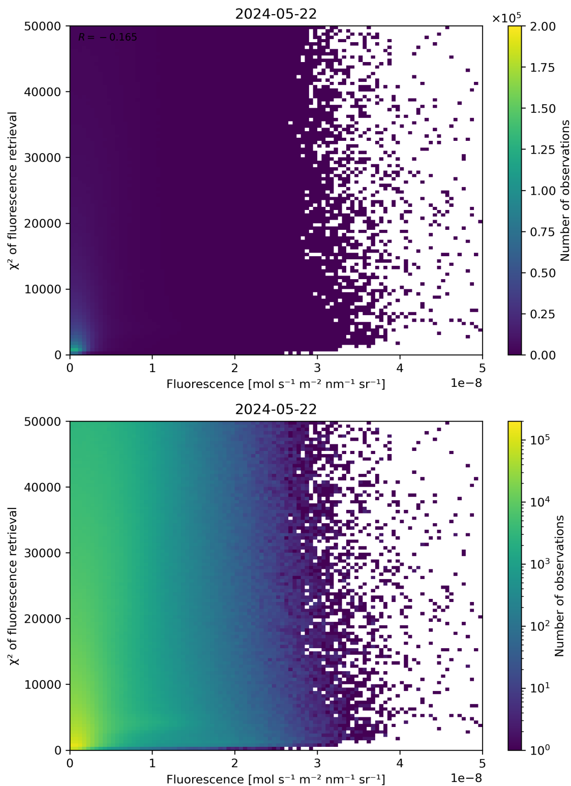
Figure 85: Scatter density plot of “Fluorescence” against “ \chi^2 of fluorescence retrieval” for 2024-05-21 to 2024-05-23.
