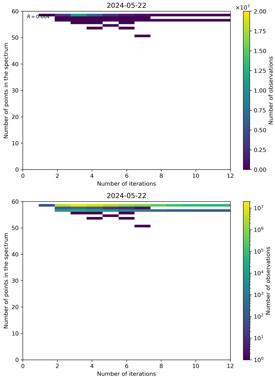
Figure 99: Scatter density plot of “Number of iterations” against “Number of points in the spectrum” for 2024-05-21 to 2024-05-23.
