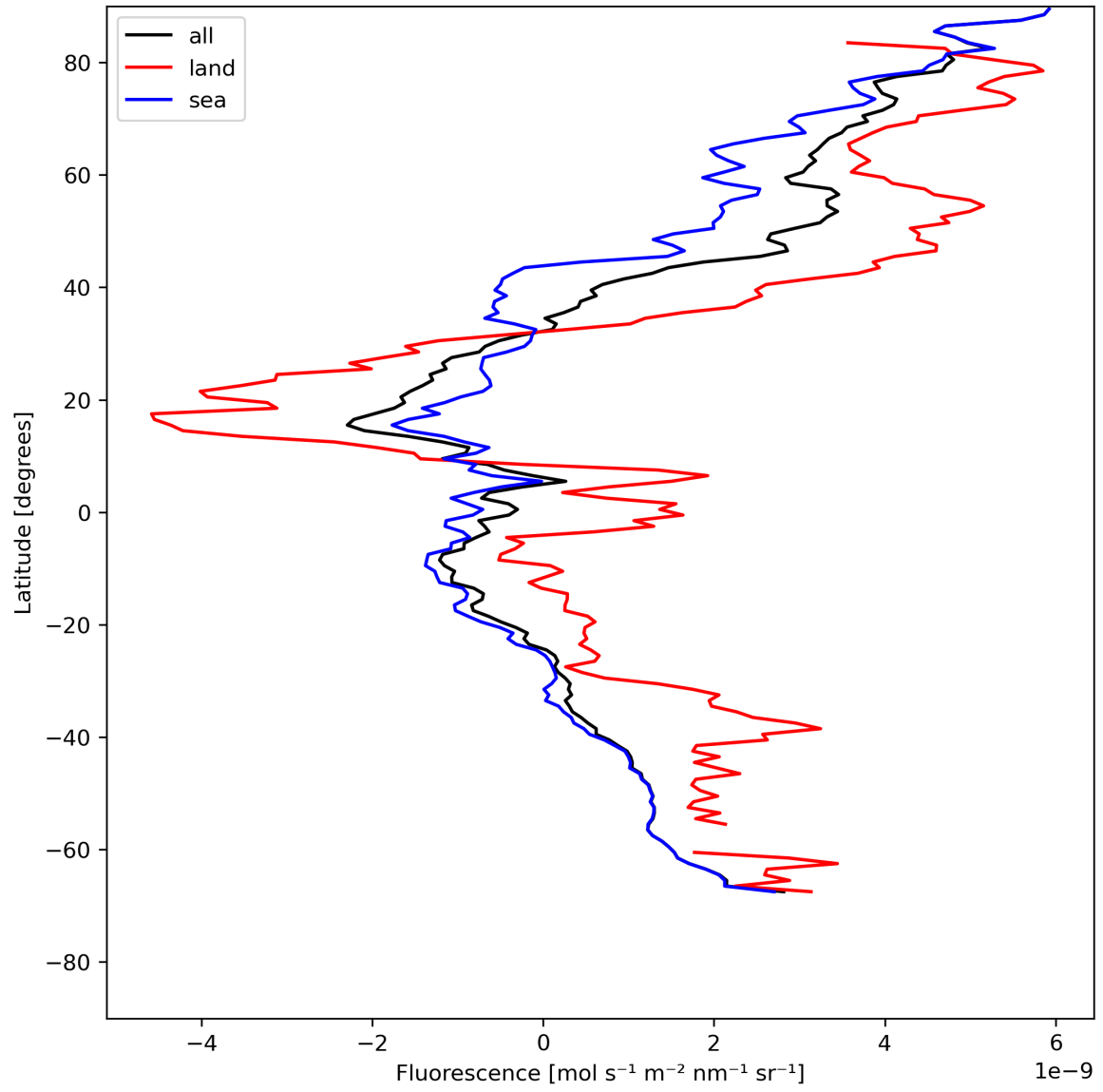
Figure 23: Zonal average of “Fluorescence” for 2024-05-21 to 2024-05-23.
