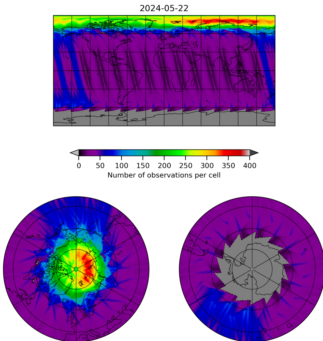
Figure 11: Map of the number of observations for 2024-05-21 to 2024-05-23
