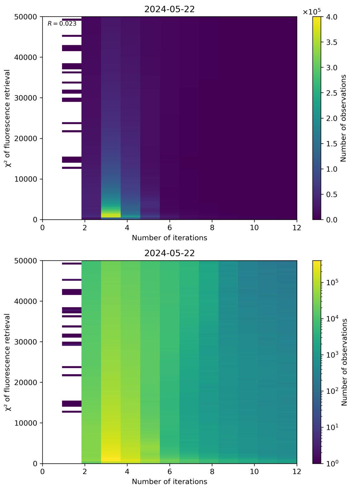
Figure 97: Scatter density plot of “Number of iterations” against “ \chi^2 of fluorescence retrieval” for 2024-05-21 to 2024-05-23.
