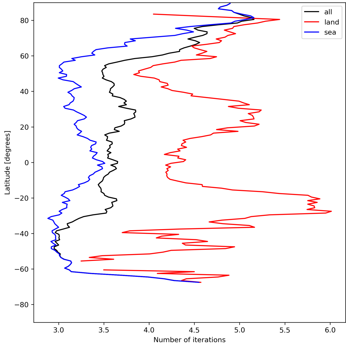
Figure 22: Zonal average of “Number of iterations” for 2024-05-21 to 2024-05-23.
