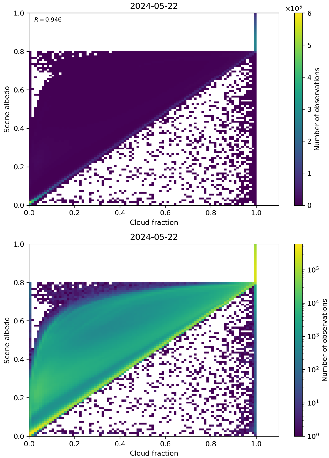
Figure 75: Scatter density plot of “Cloud fraction” against “Scene albedo” for 2024-05-21 to 2024-05-23.
