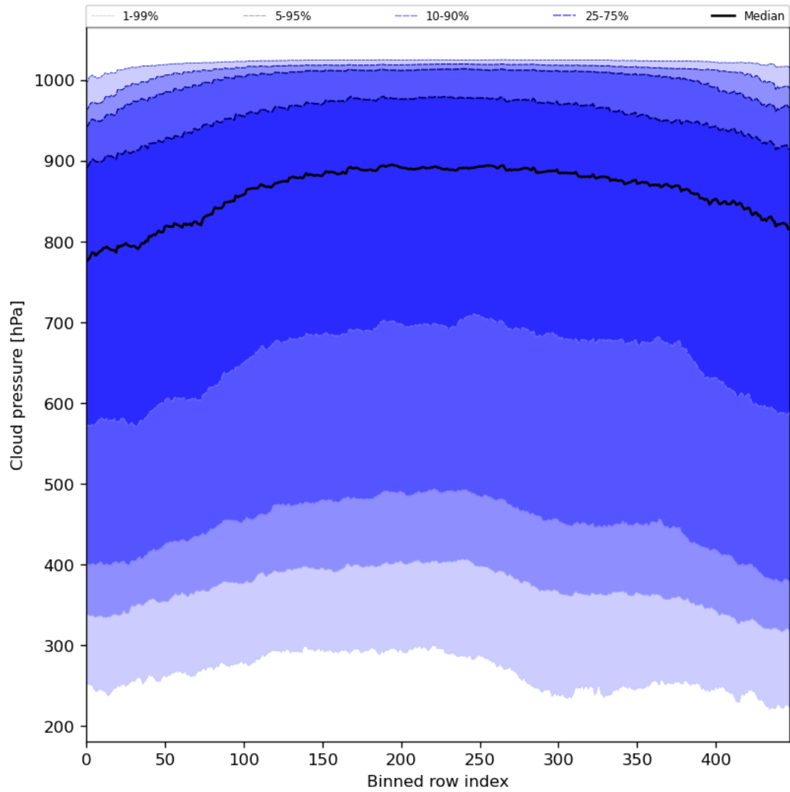
Figure 47: Along track statistics of “Cloud pressure” for 2024-05-21 to 2024-05-23
