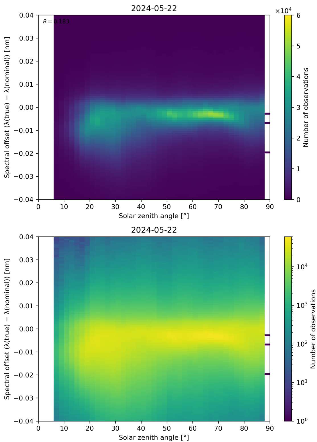
Figure 117: Scatter density plot of “Solar zenith angle” against “Spectral offset ( \lambda(\text{true}) - \lambda(\text{nominal}) )” for 2024-05-21 to 2024-05-23.
