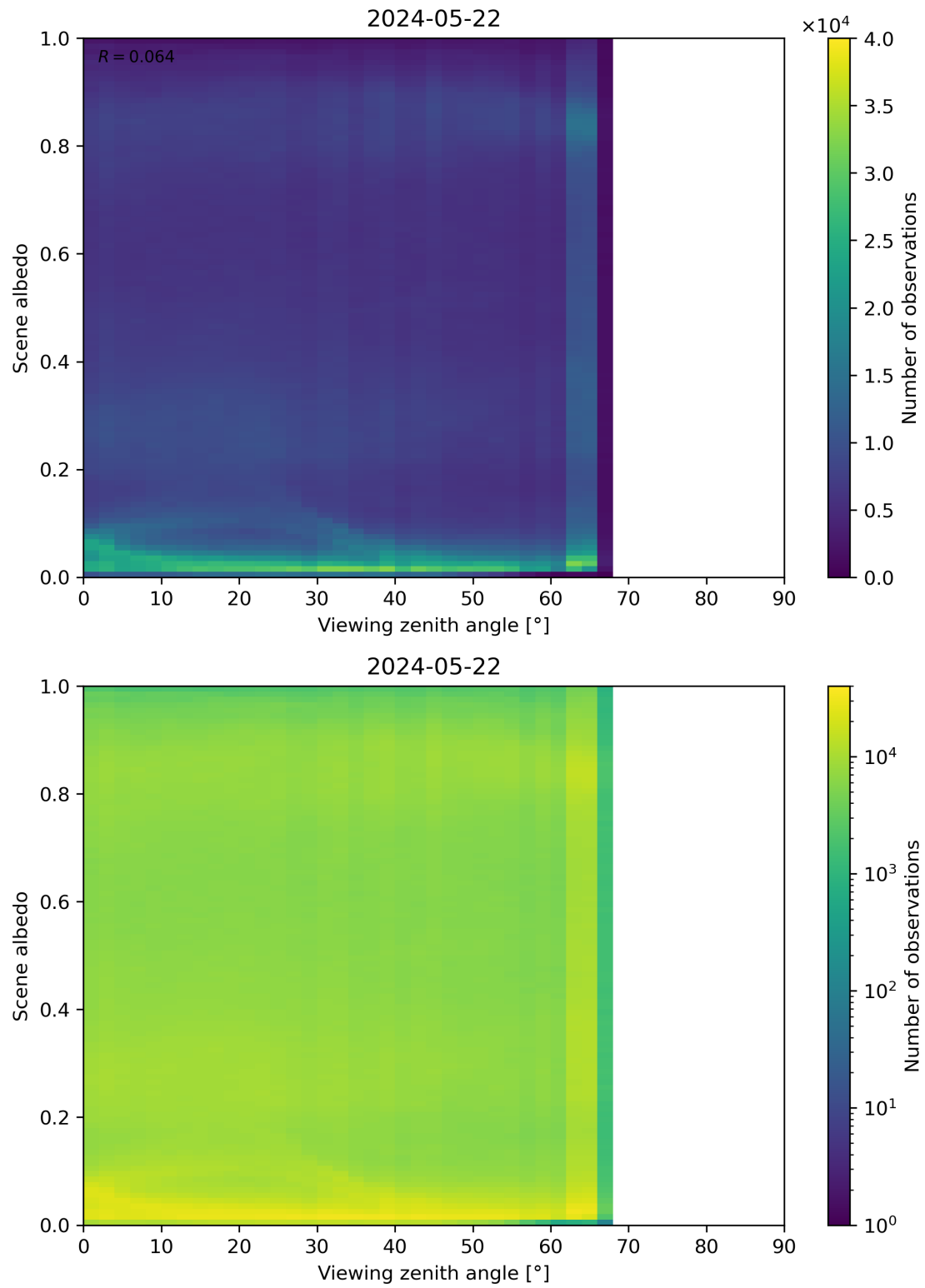
Figure 126: Scatter density plot of “Viewing zenith angle” against “Scene albedo” for 2024-05-21 to 2024-05-23.
