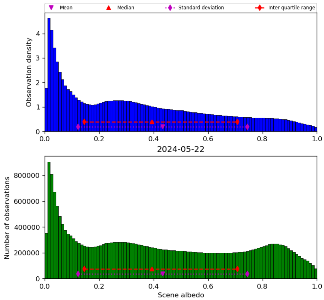
Figure 34: Histogram of “Scene albedo” for 2024-05-21 to 2024-05-23
