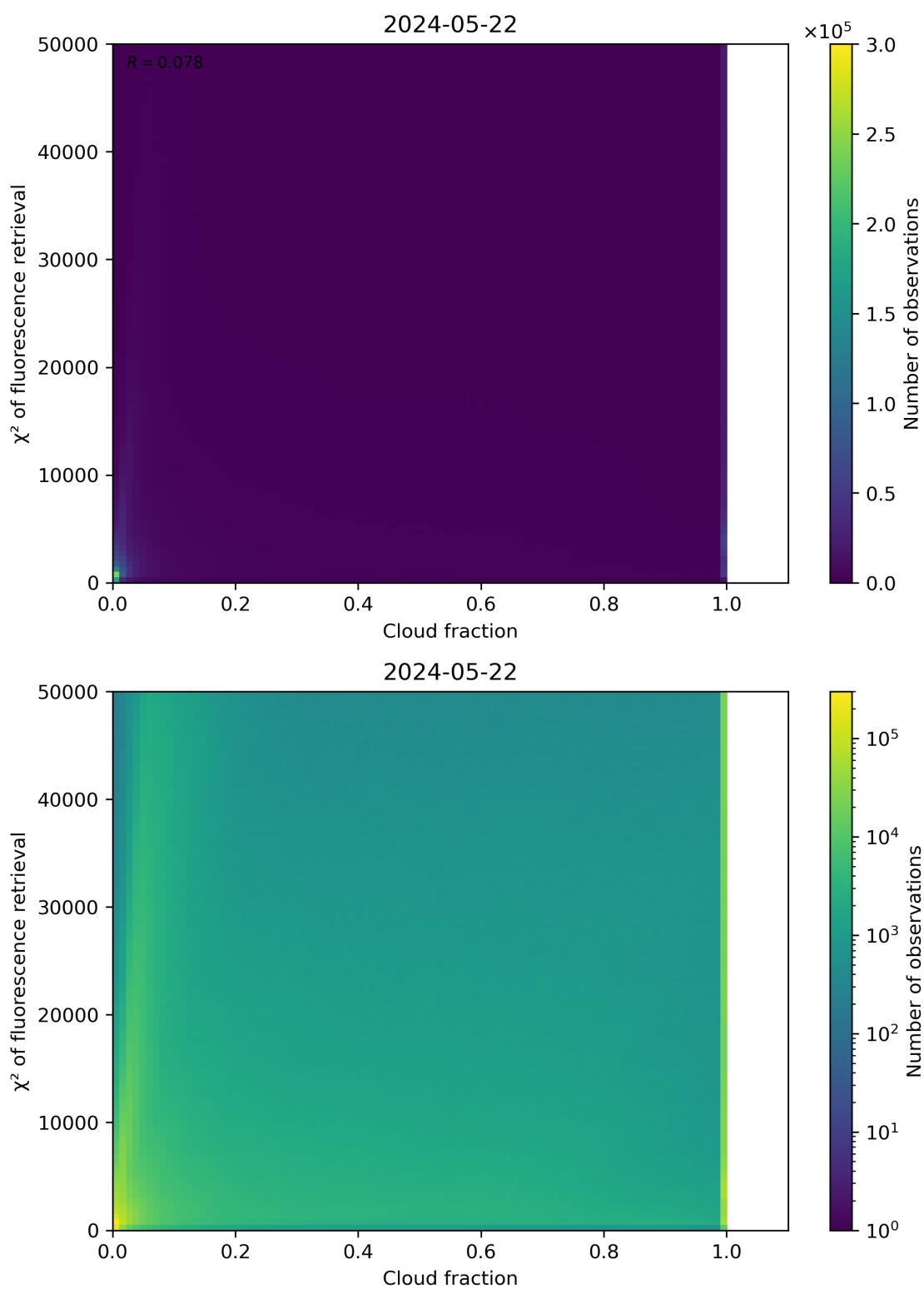
Figure 71: Scatter density plot of “Cloud fraction” against “ \chi^2 of fluorescence retrieval” for 2024-05-21 to 2024-05-23.
