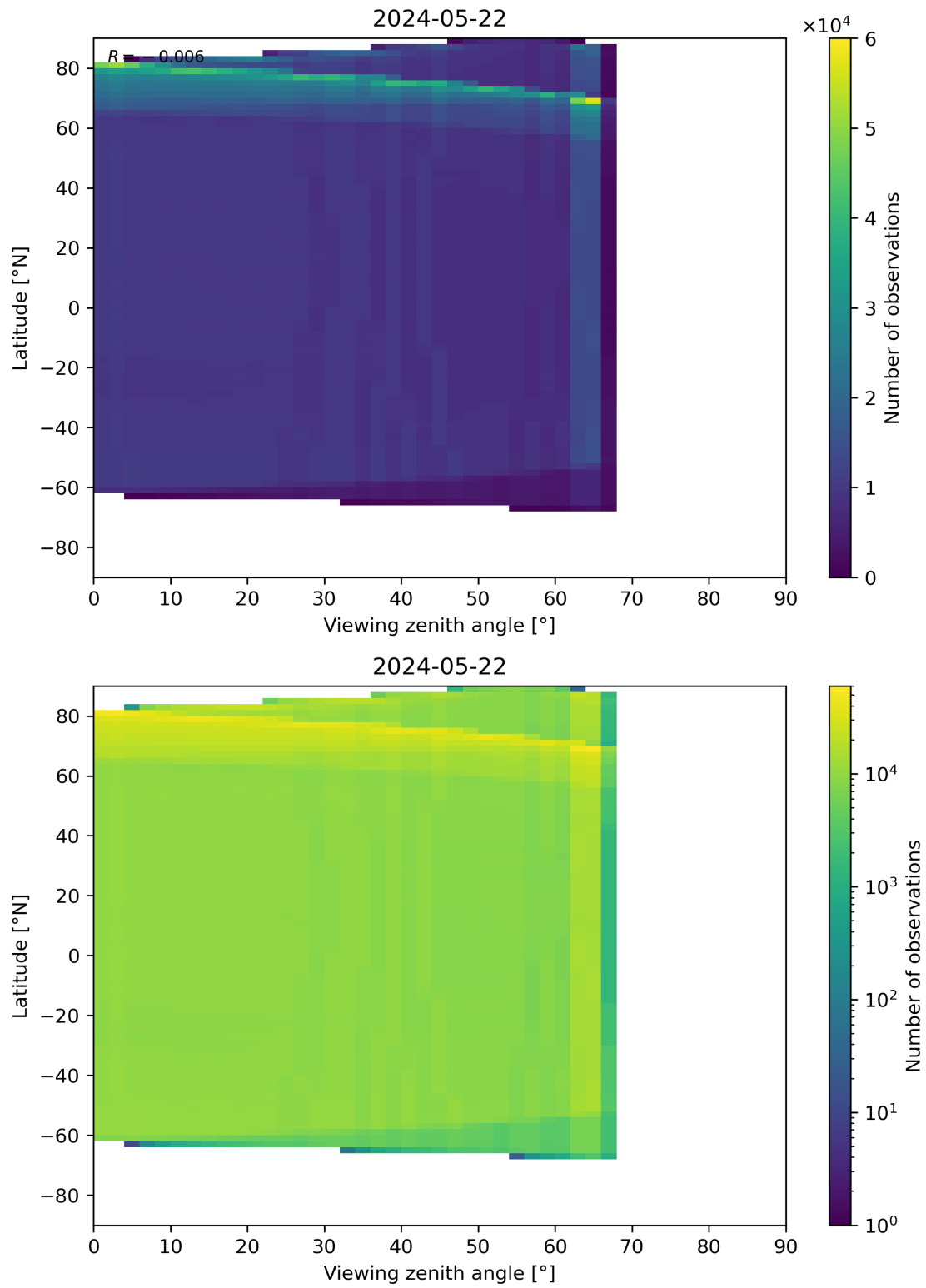
Figure 123: Scatter density plot of “Viewing zenith angle” against “Latitude” for 2024-05-21 to 2024-05-23.
