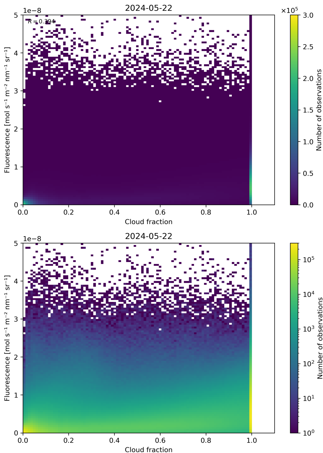
Figure 72: Scatter density plot of “Cloud fraction” against “Fluorescence” for 2024-05-21 to 2024-05-23.
