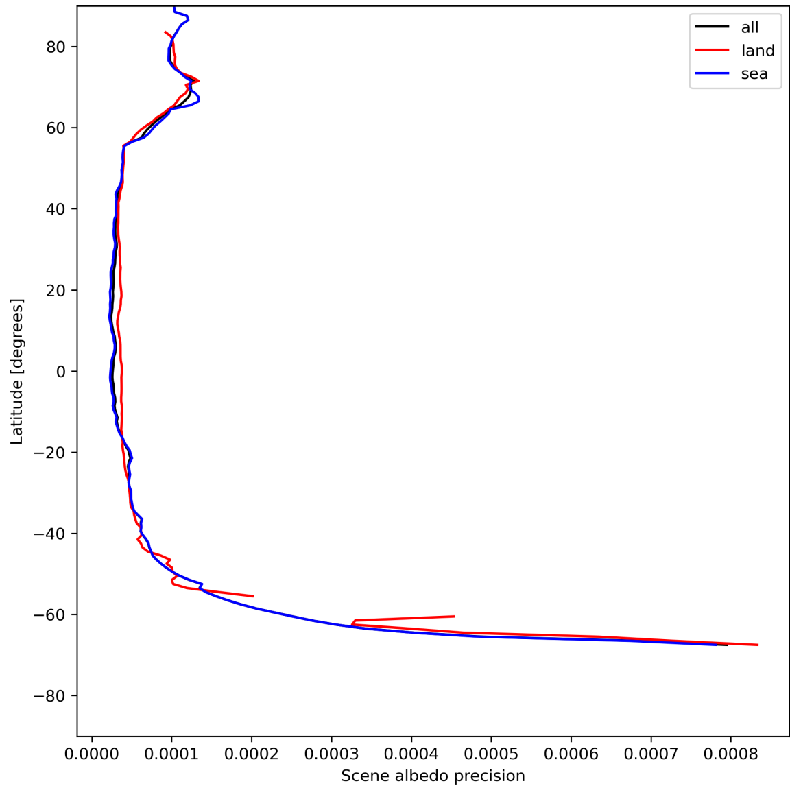
Figure 18: Zonal average of “Scene albedo precision” for 2024-05-21 to 2024-05-23.
