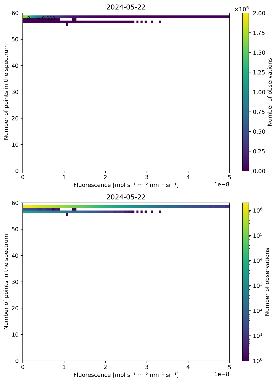
Figure 86: Scatter density plot of “Fluorescence” against “Number of points in the spectrum” for 2024-05-21 to 2024-05-23.
