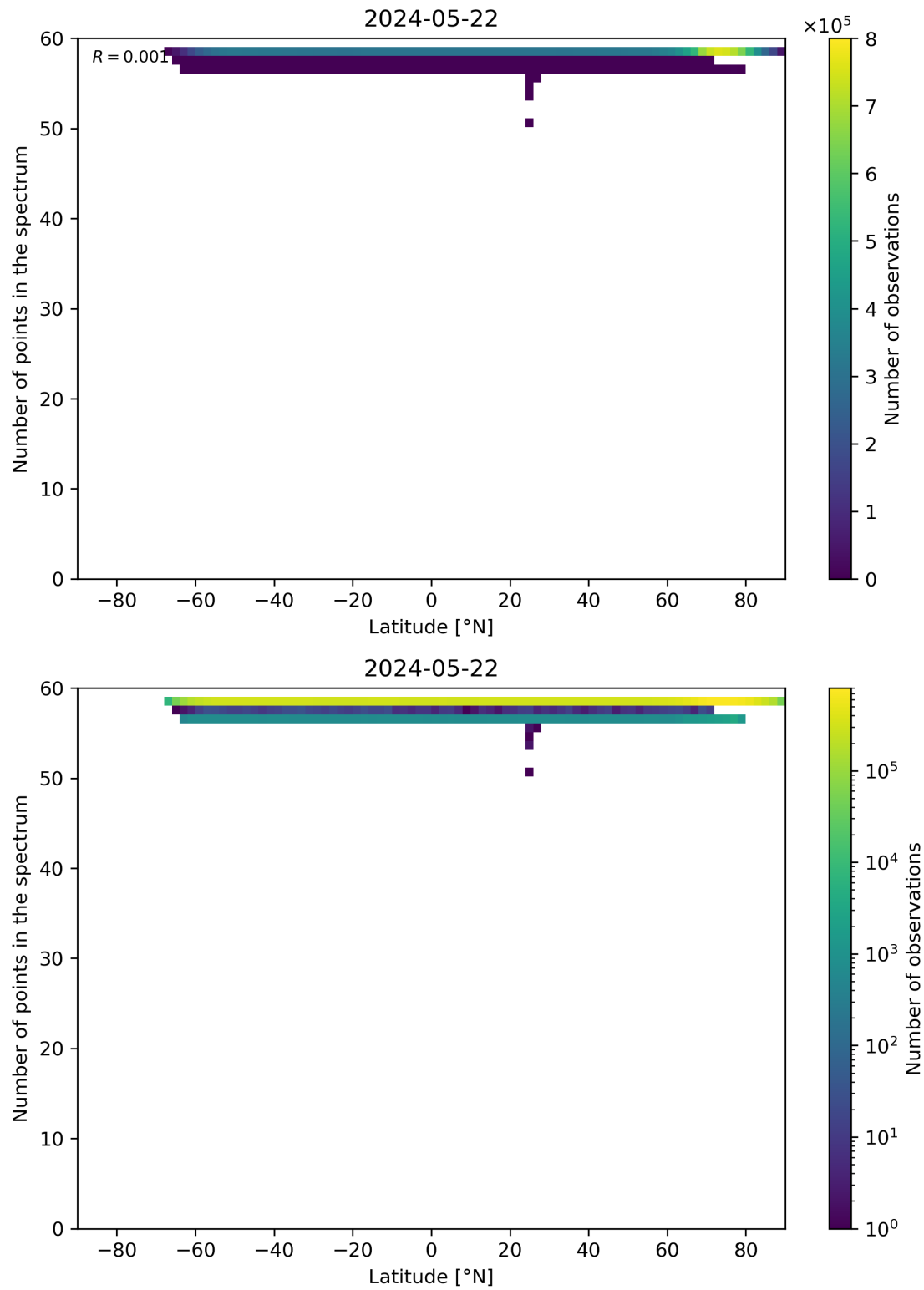
Figure 94: Scatter density plot of “Latitude” against “Number of points in the spectrum” for 2024-05-21 to 2024-05-23.
