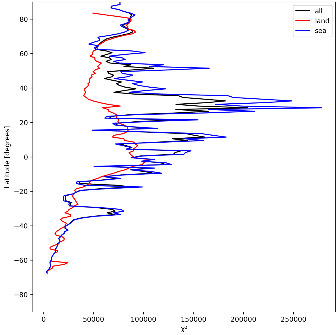
Figure 21: Zonal average of “ \chi^2 ” for 2024-05-21 to 2024-05-23.
