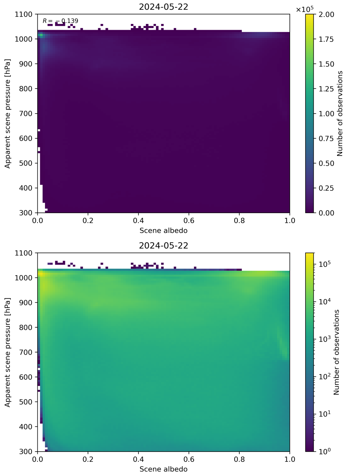
Figure 102: Scatter density plot of “Scene albedo” against “Apparent scene pressure” for 2024-05-21 to 2024-05-23.
