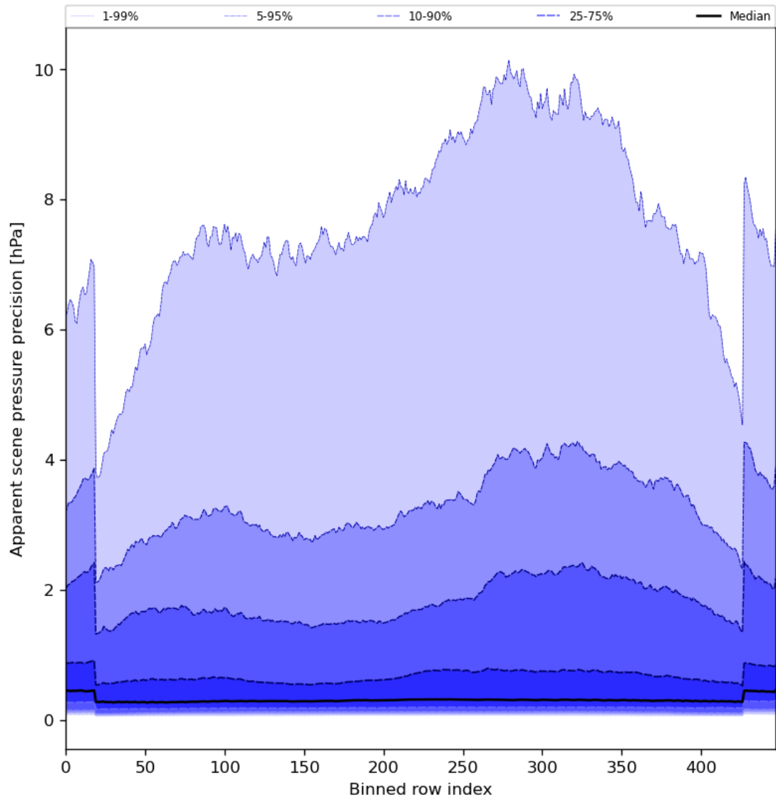
Figure 54: Along track statistics of “Apparent scene pressure precision” for 2024-05-21 to 2024-05-23
