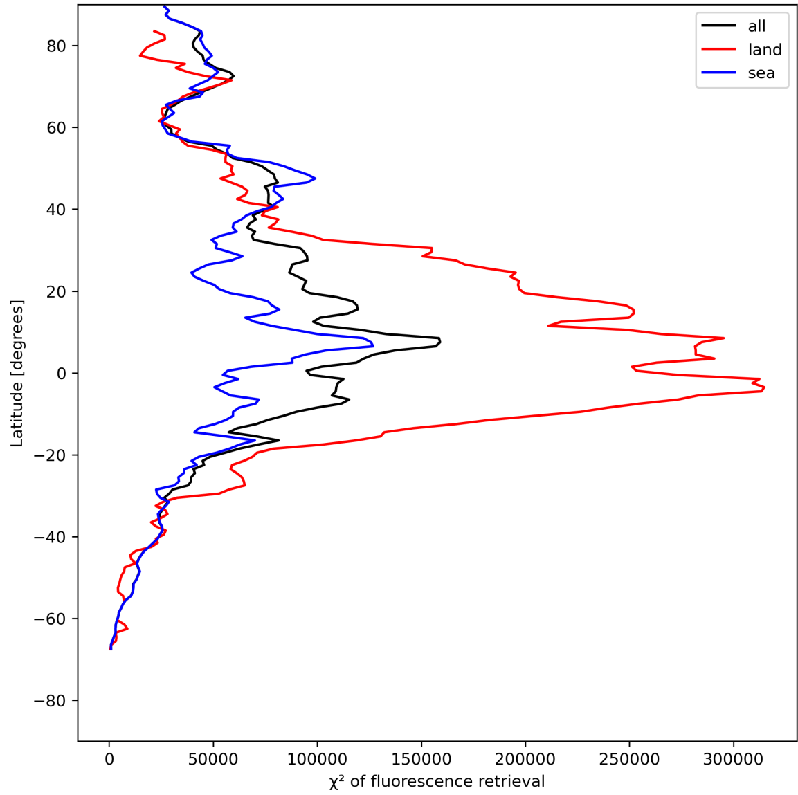
Figure 25: Zonal average of “ \chi^2 of fluorescence retrieval” for 2024-05-21 to 2024-05-23.
