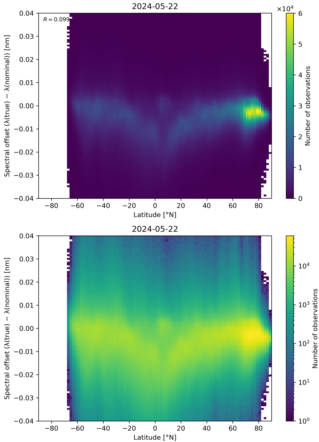
Figure 96: Scatter density plot of “Latitude” against “Spectral offset ( \lambda(\text{true}) - \lambda(\text{nominal}) )” for 2024-05-21 to 2024-05-23.
