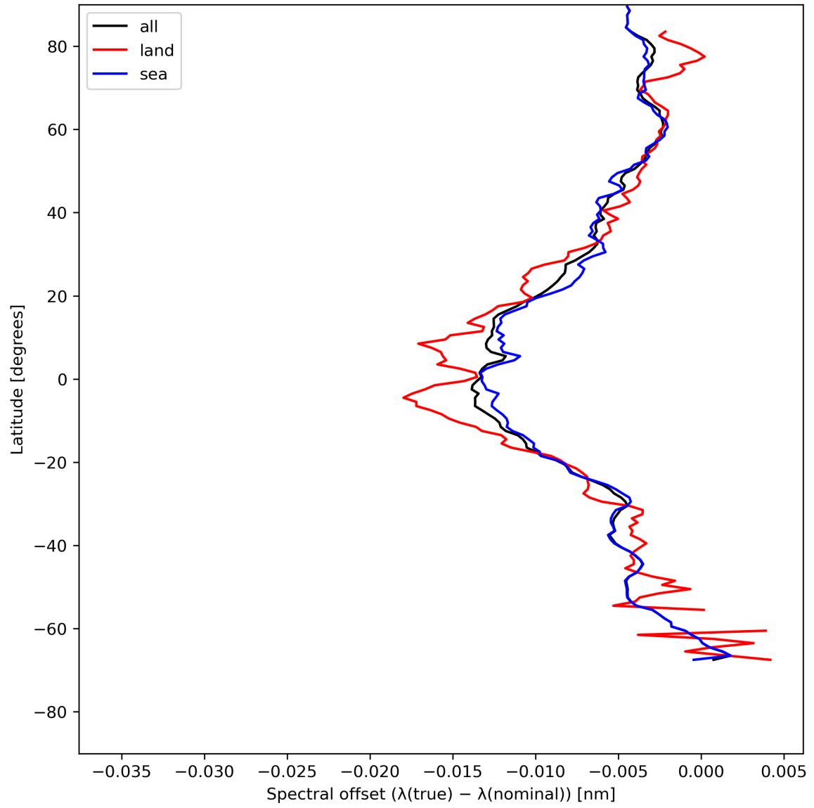
Figure 28: Zonal average of “Spectral offset ( \lambda(\text{true}) - \lambda(\text{nominal}) )” for 2024-05-21 to 2024-05-23.
