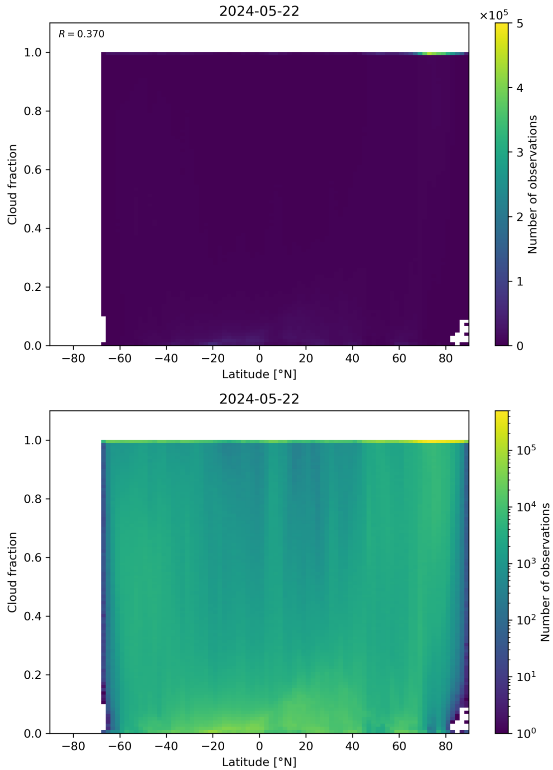
Figure 90: Scatter density plot of “Latitude” against “Cloud fraction” for 2024-05-21 to 2024-05-23.
