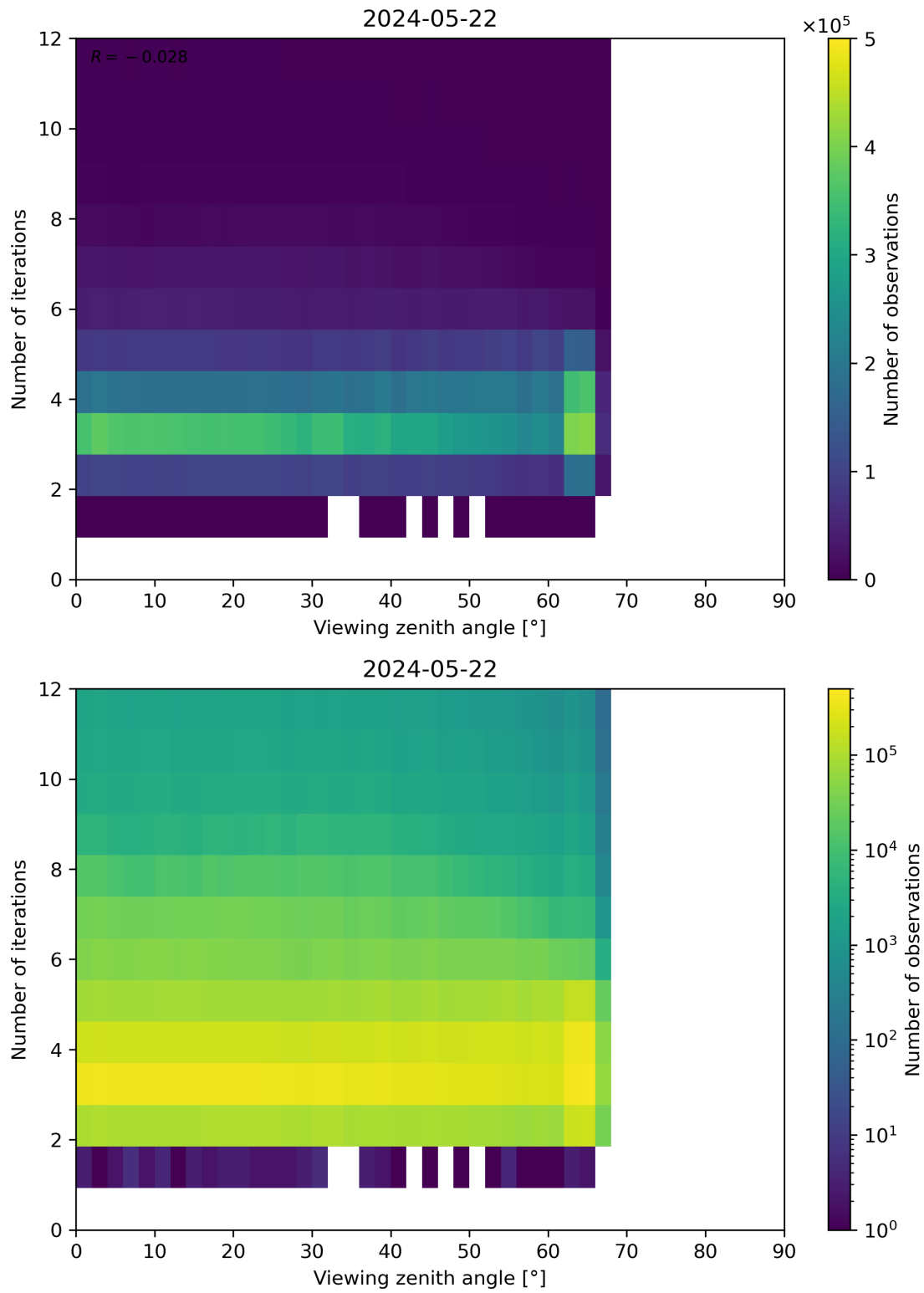
Figure 124: Scatter density plot of “Viewing zenith angle” against “Number of iterations” for 2024-05-21 to 2024-05-23.
