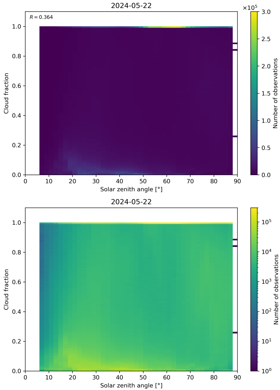
Figure 110: Scatter density plot of “Solar zenith angle” against “Cloud fraction” for 2024-05-21 to 2024-05-23.
