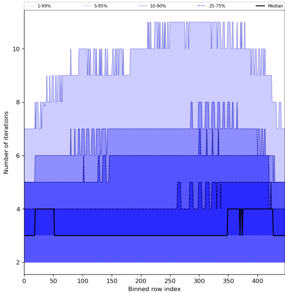
Figure 56: Along track statistics of “Number of iterations” for 2024-05-21 to 2024-05-23
