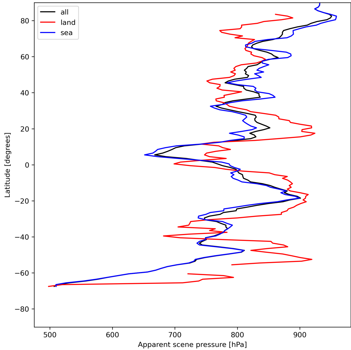
Figure 19: Zonal average of “Apparent scene pressure” for 2024-05-21 to 2024-05-23.
