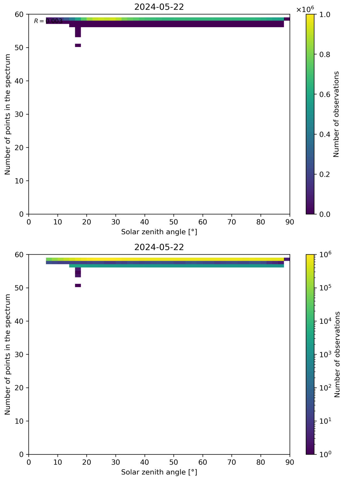
Figure 115: Scatter density plot of “Solar zenith angle” against “Number of points in the spectrum” for 2024-05-21 to 2024-05-23.
