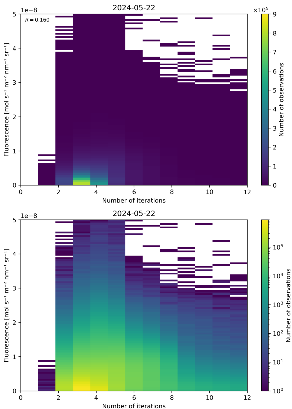
Figure 98: Scatter density plot of “Number of iterations” against “Fluorescence” for 2024-05-21 to 2024-05-23.
