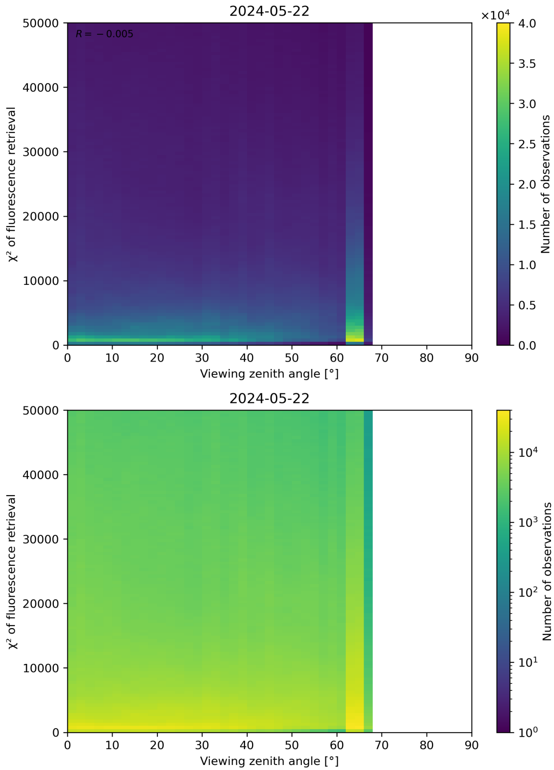
Figure 119: Scatter density plot of “Viewing zenith angle” against “ \chi^2 of fluorescence retrieval” for 2024-05-21 to 2024-05-23.
