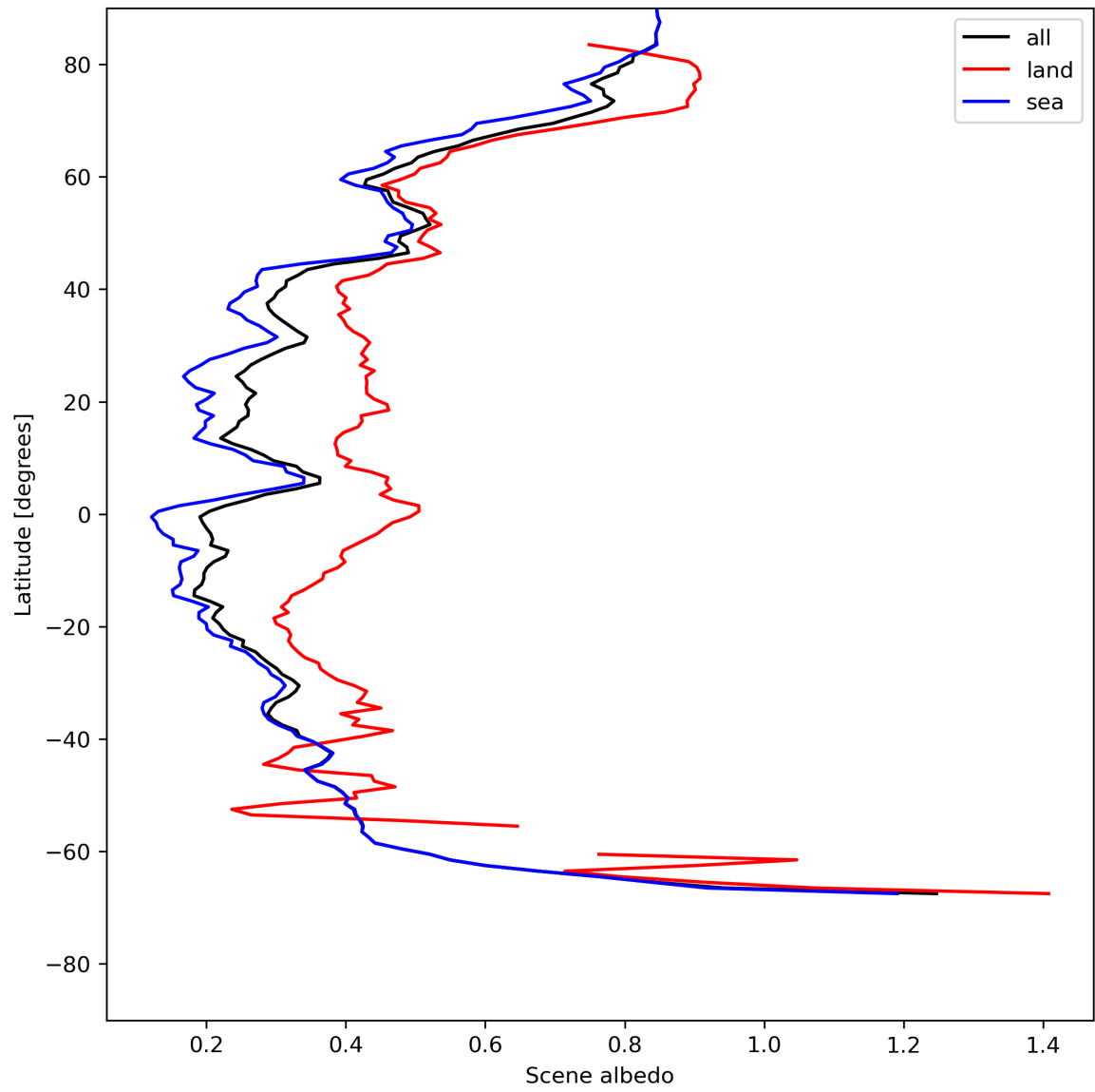
Figure 17: Zonal average of “Scene albedo” for 2024-05-21 to 2024-05-23.
