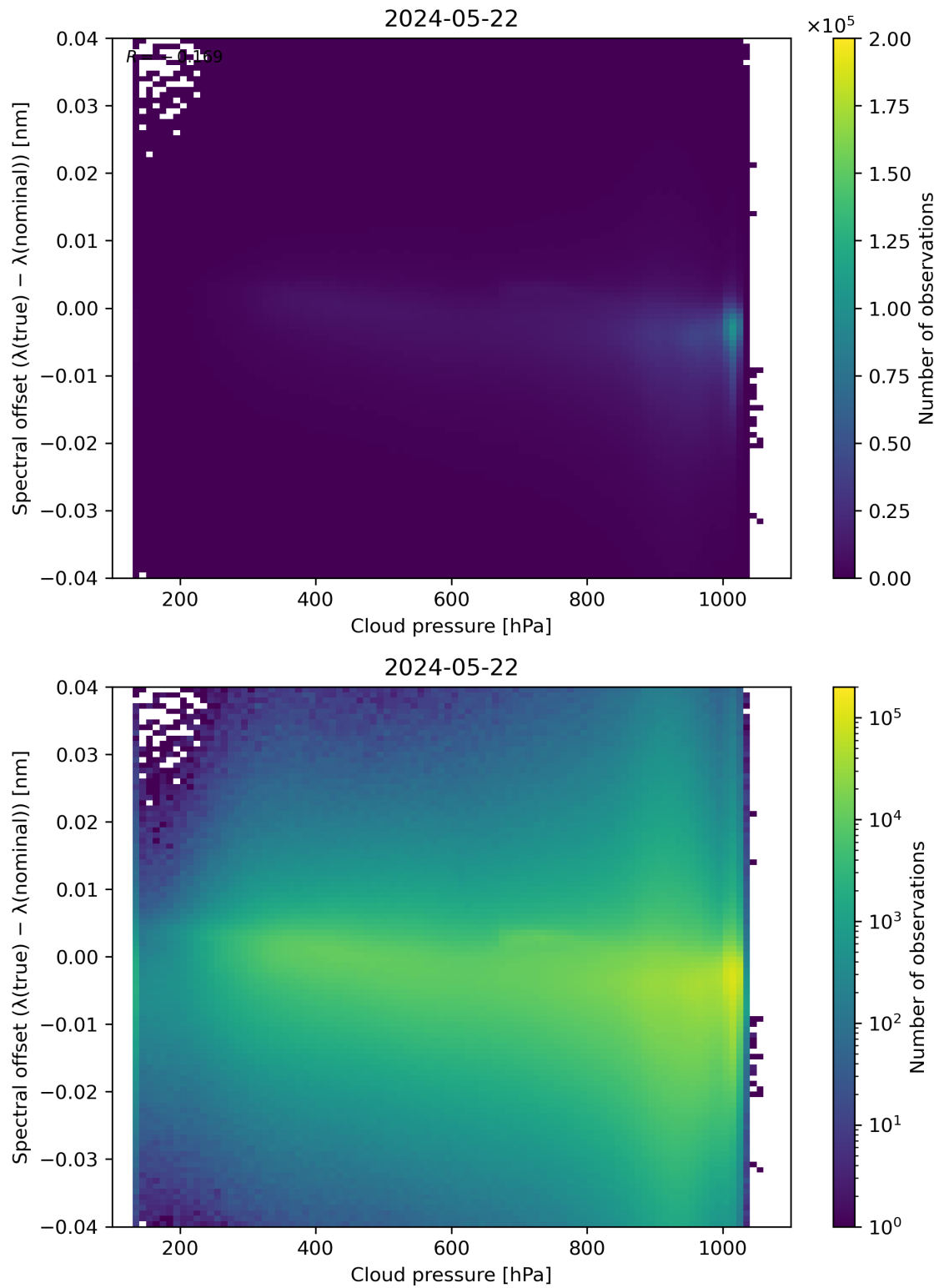
Figure 84: Scatter density plot of “Cloud pressure” against “Spectral offset ( \lambda(\text{true}) - \lambda(\text{nominal}) )” for 2024-05-21 to 2024-05-23.
