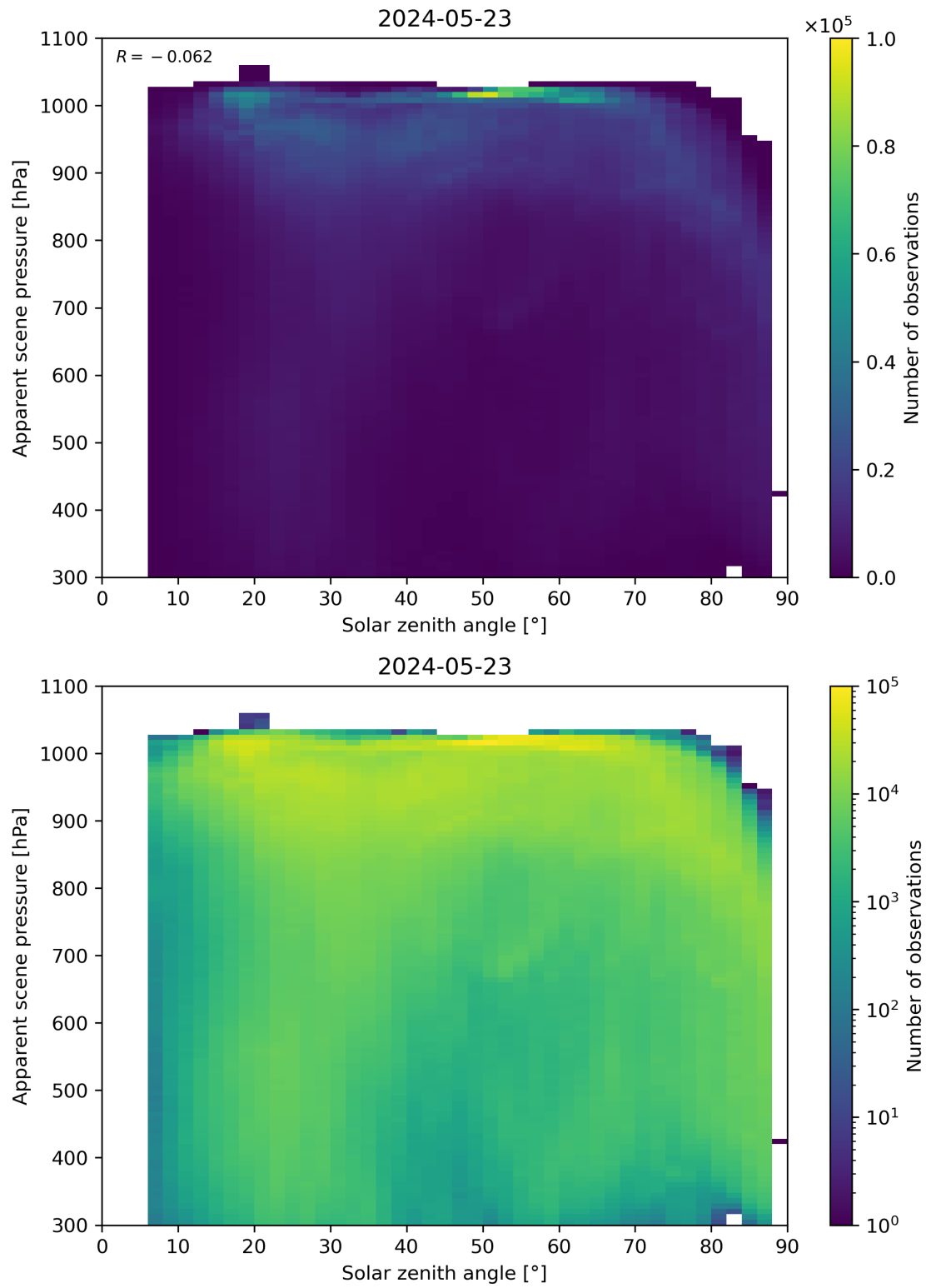
Figure 108: Scatter density plot of “Solar zenith angle” against “Apparent scene pressure” for 2024-05-23 to 2024-05-24.
