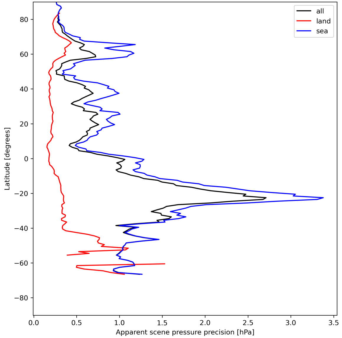
Figure 20: Zonal average of “Apparent scene pressure precision” for 2024-05-23 to 2024-05-24.
