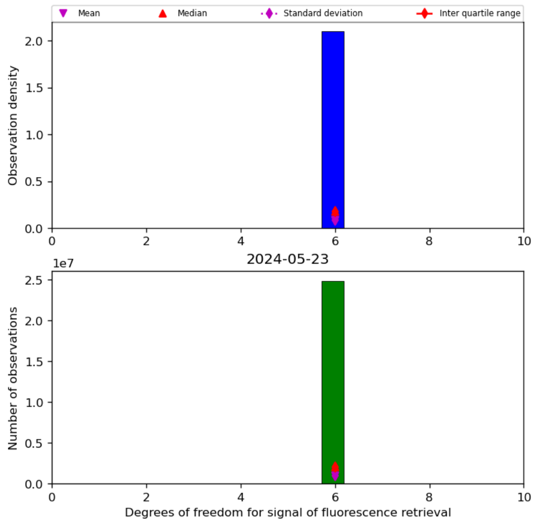
Figure 43: Histogram of “Degrees of freedom for signal of fluorescence retrieval” for 2024-05-23 to 2024-05-24
