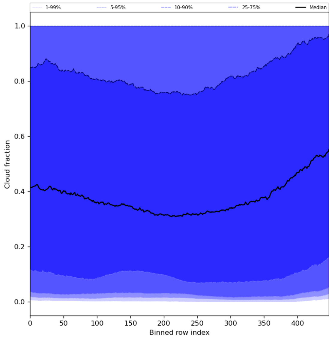
Figure 49: Along track statistics of “Cloud fraction” for 2024-05-23 to 2024-05-24
