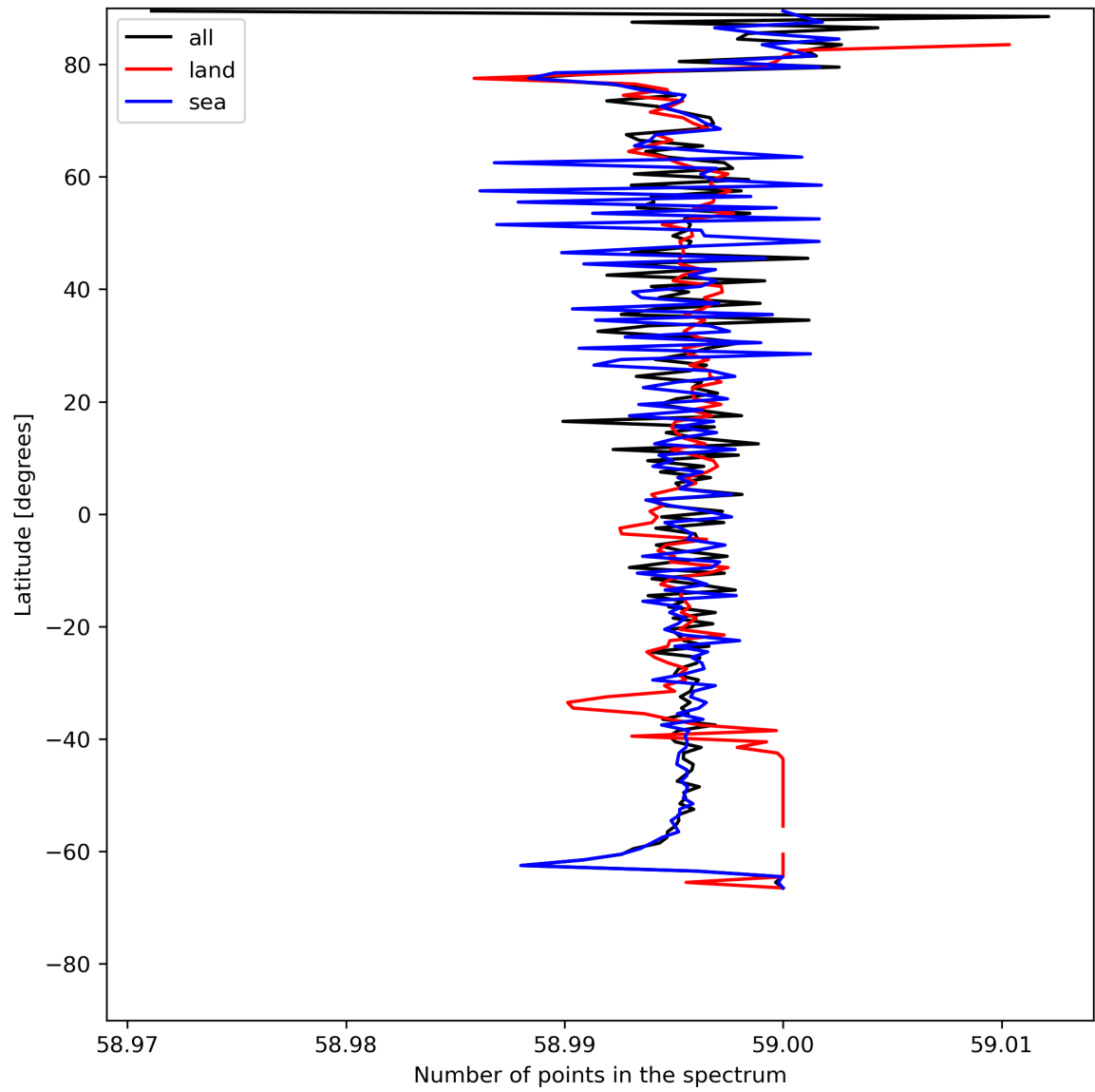
Figure 27: Zonal average of “Number of points in the spectrum” for 2024-05-23 to 2024-05-24.
