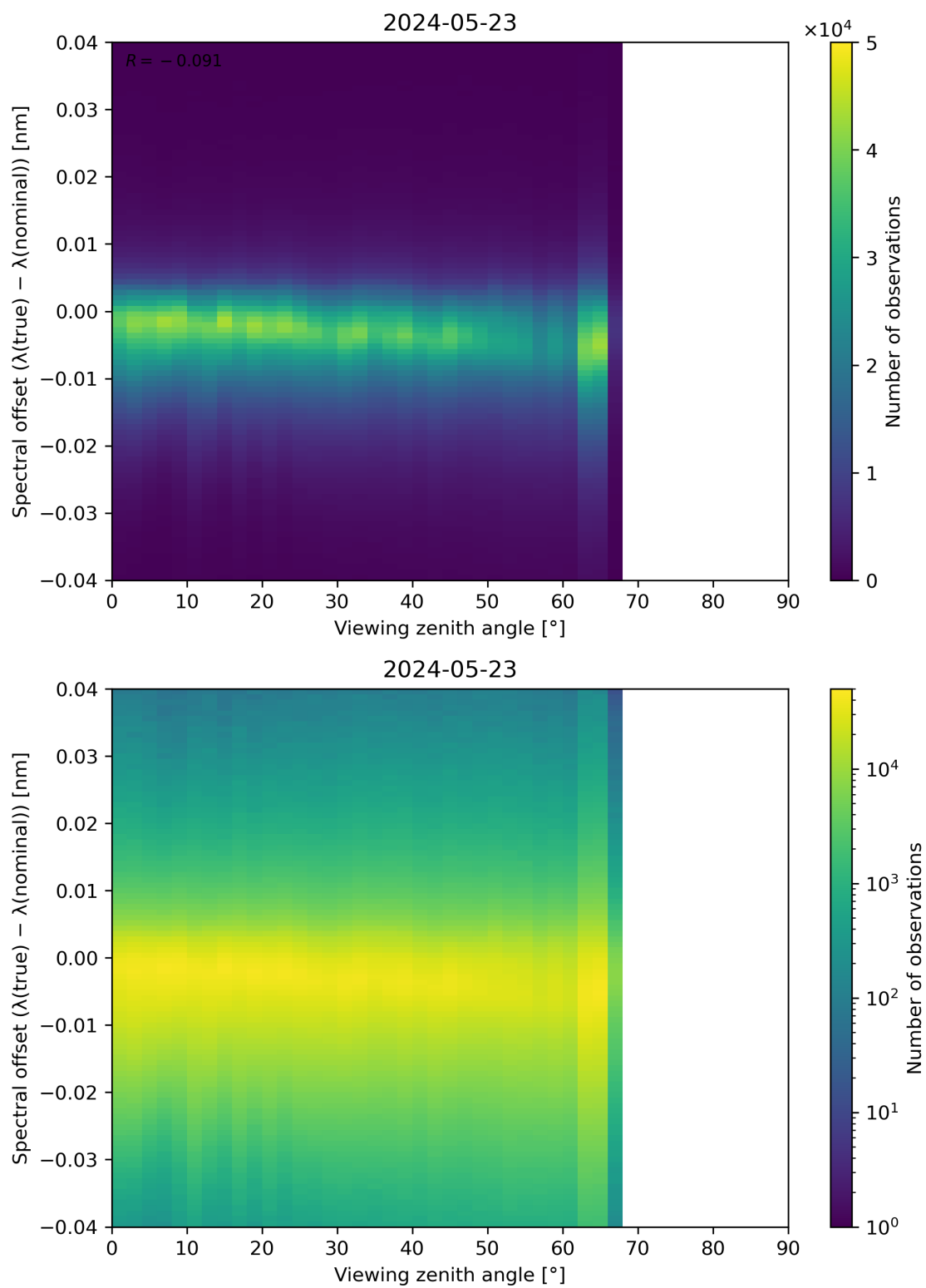
Figure 128: Scatter density plot of “Viewing zenith angle” against “Spectral offset ( \lambda(\text{true}) - \lambda(\text{nominal}) )” for 2024-05-23 to 2024-05-24.
