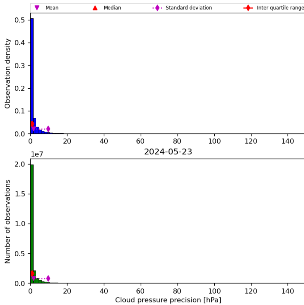
Figure 31: Histogram of “Cloud pressure precision” for 2024-05-23 to 2024-05-24
