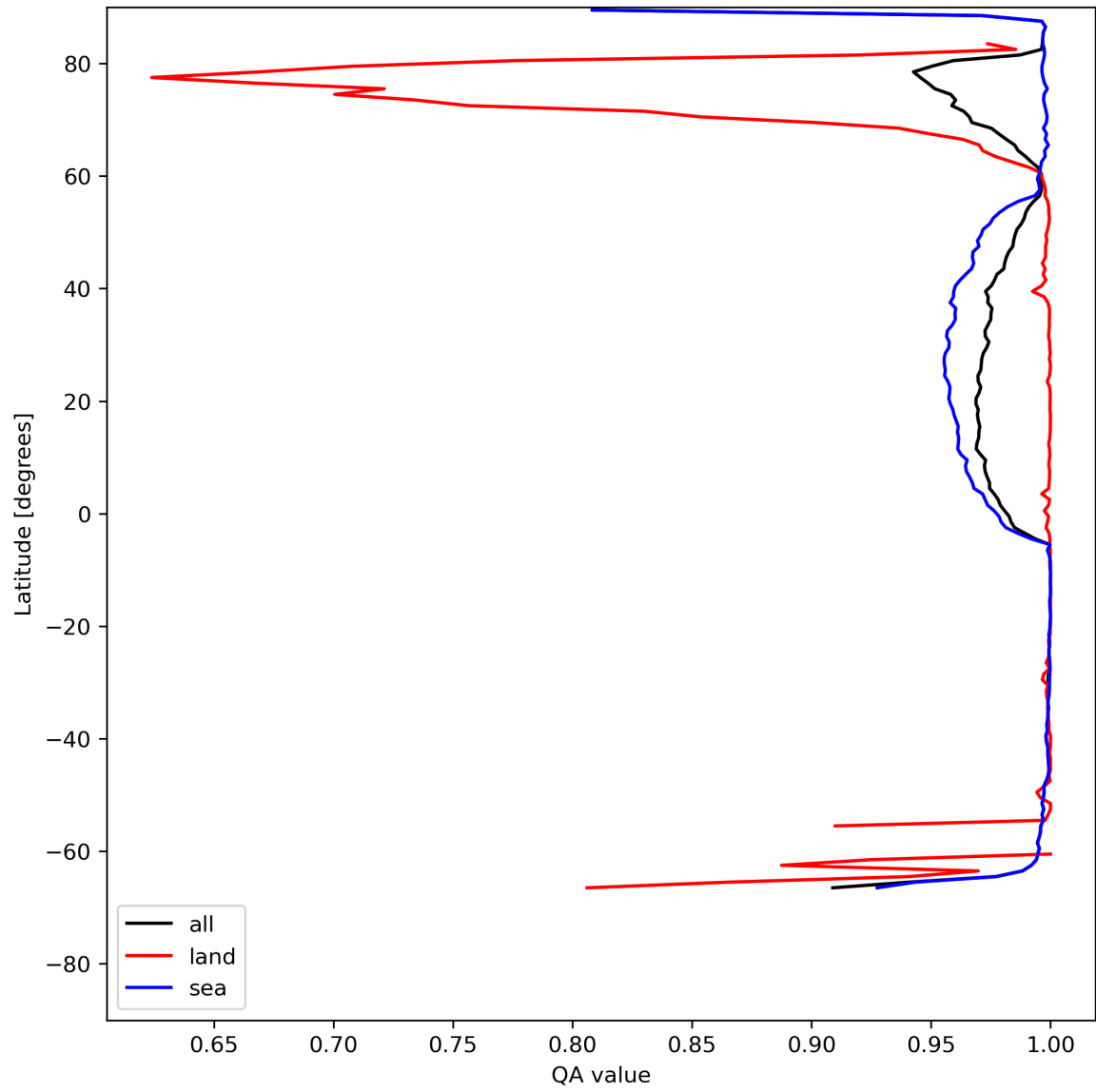
Figure 12: Zonal average of “QA value” for 2024-05-23 to 2024-05-24.
