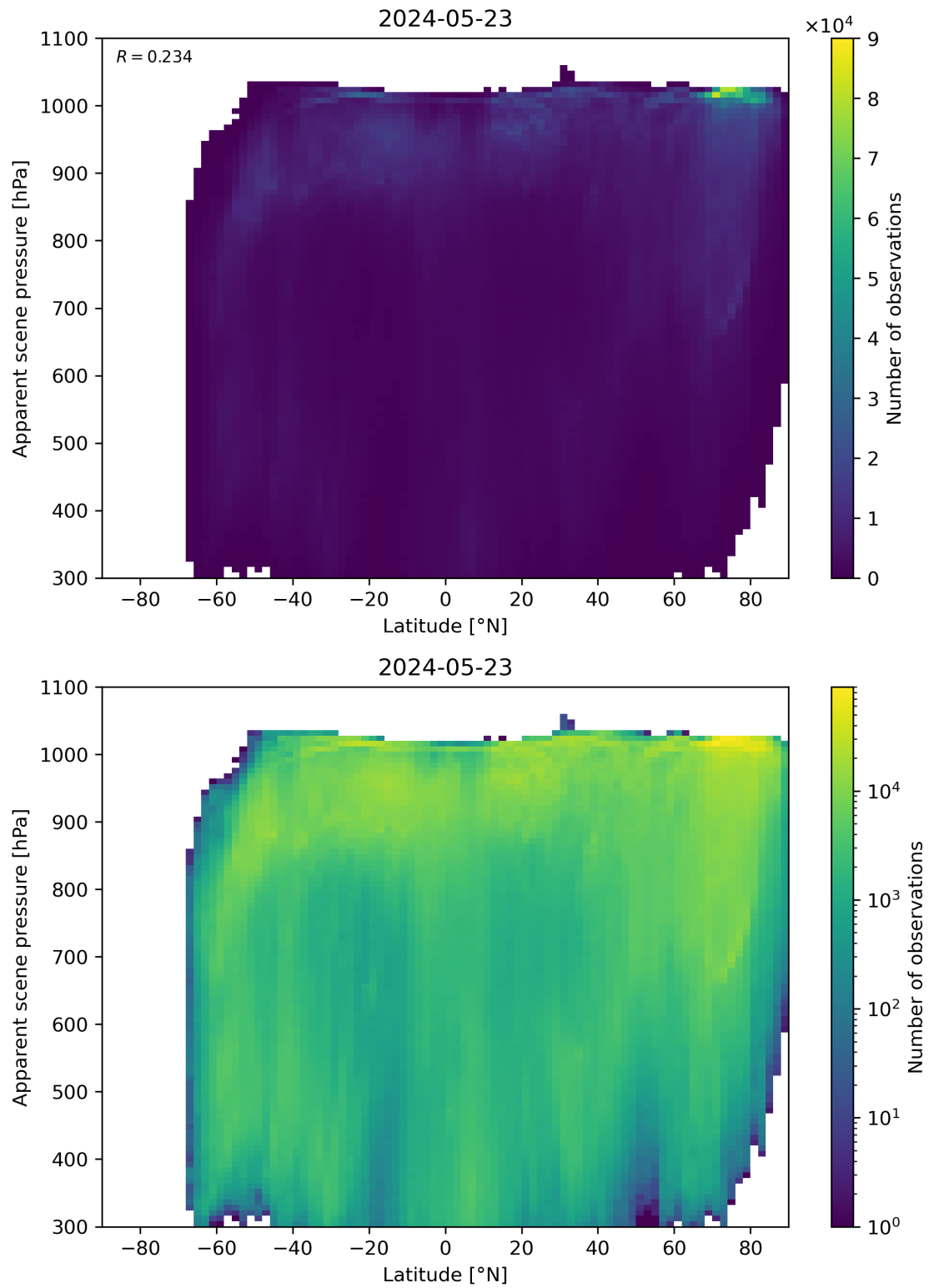
Figure 88: Scatter density plot of “Latitude” against “Apparent scene pressure” for 2024-05-23 to 2024-05-24.
