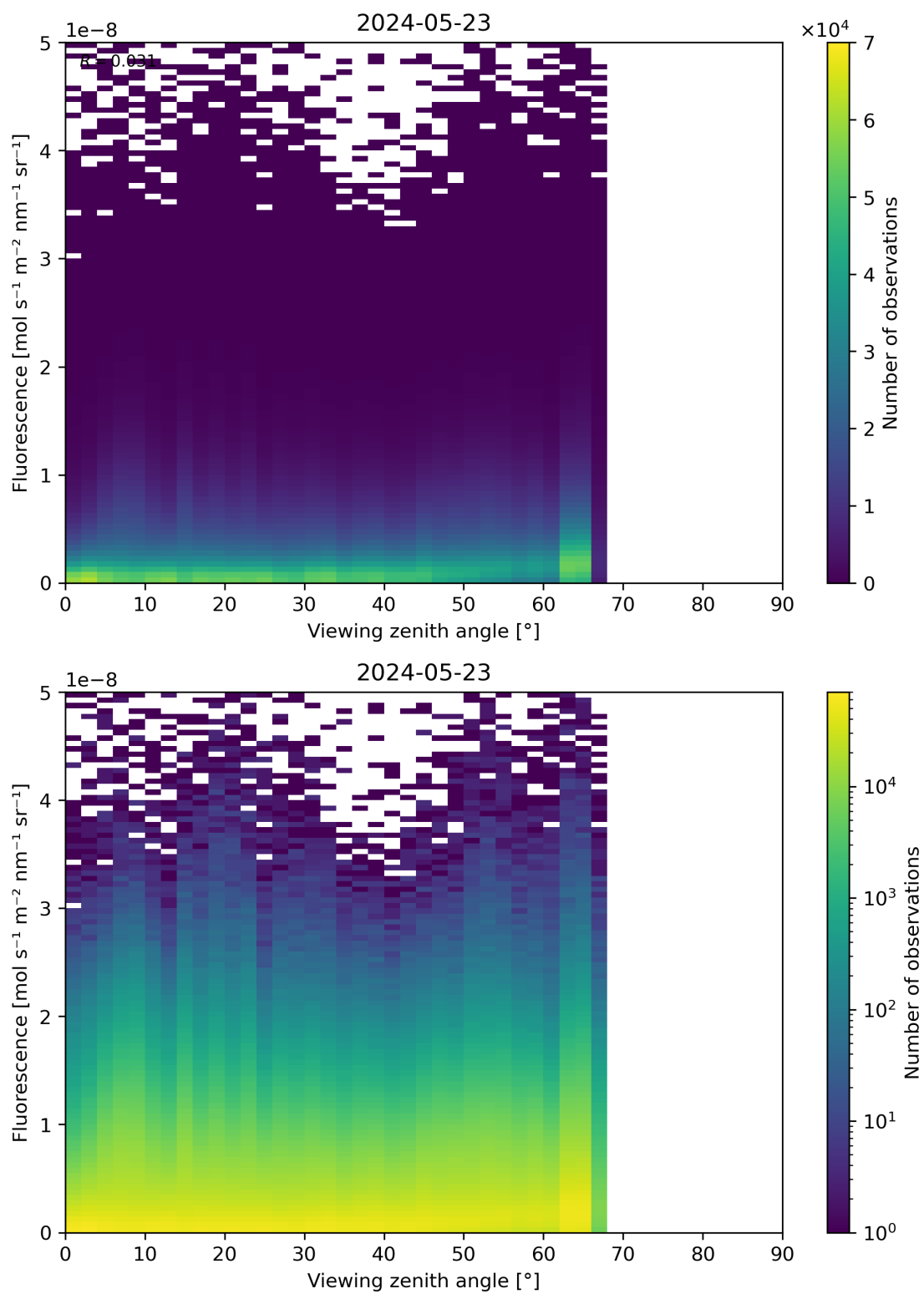
Figure 122: Scatter density plot of “Viewing zenith angle” against “Fluorescence” for 2024-05-23 to 2024-05-24.
