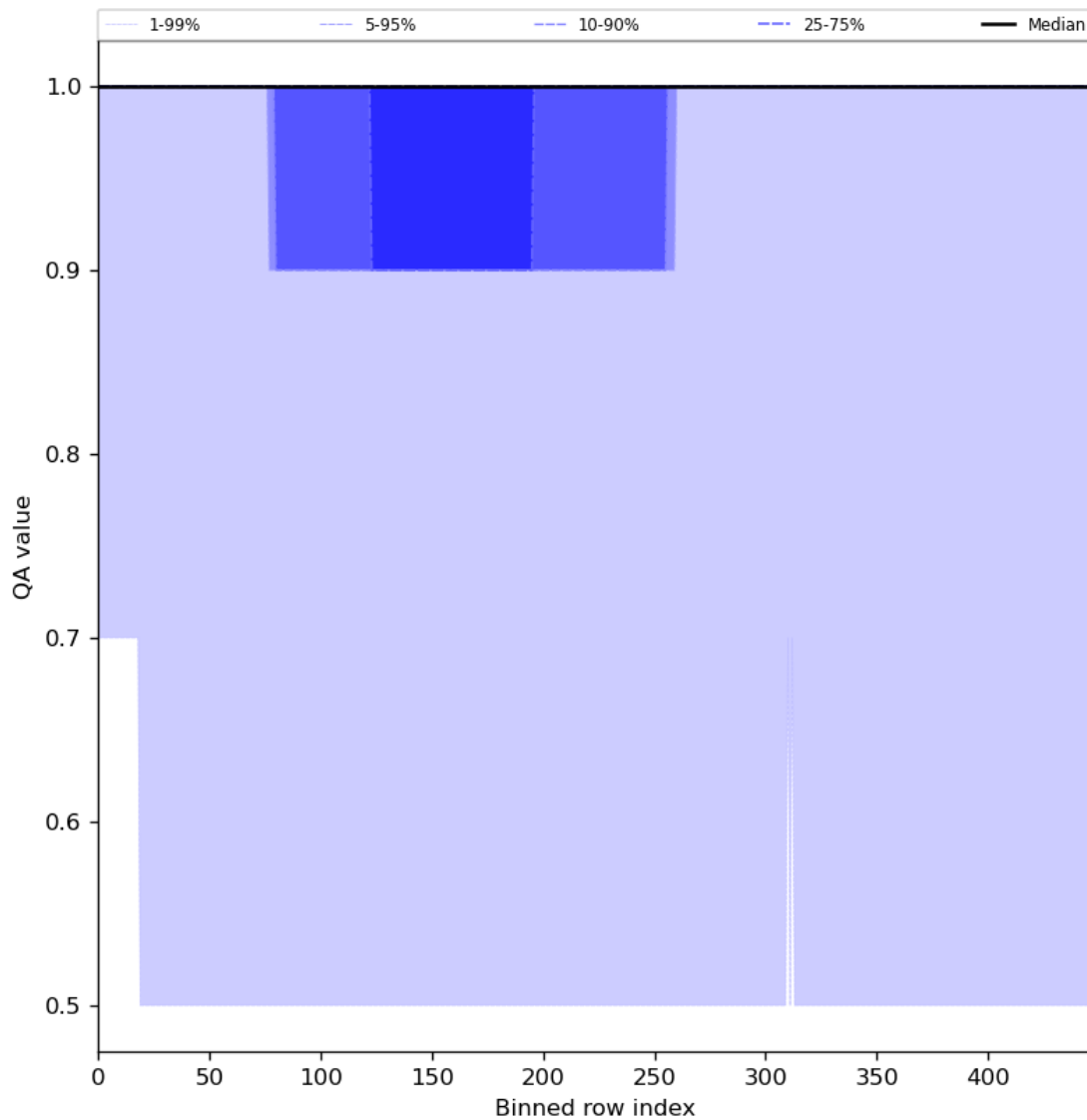
Figure 46: Along track statistics of “QA value” for 2024-05-23 to 2024-05-24
