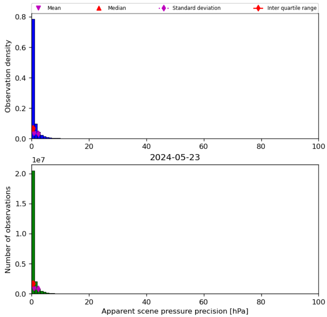
Figure 37: Histogram of “Apparent scene pressure precision” for 2024-05-23 to 2024-05-24
