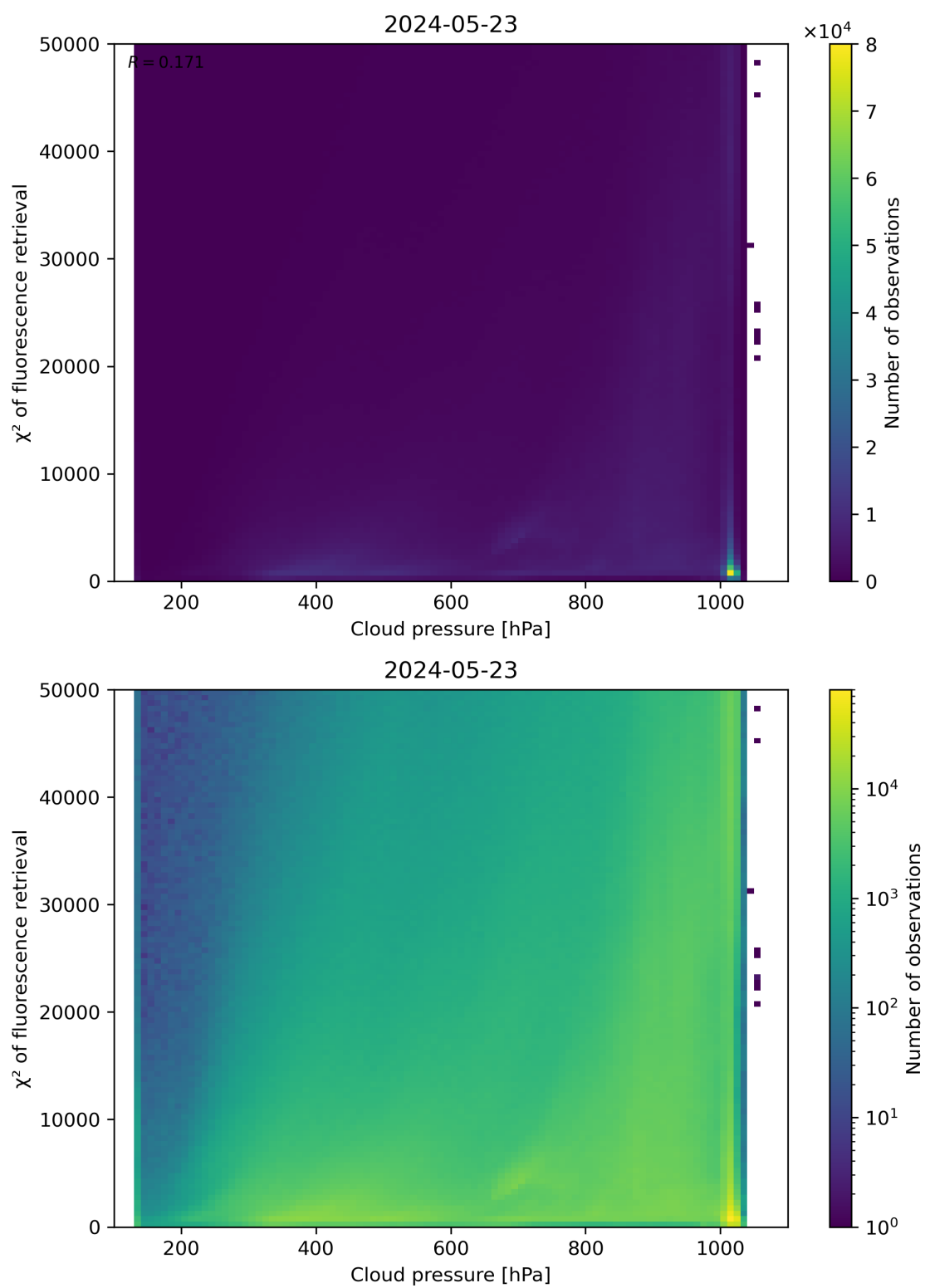
Figure 78: Scatter density plot of “Cloud pressure” against “ \chi^2 of fluorescence retrieval” for 2024-05-23 to 2024-05-24.
