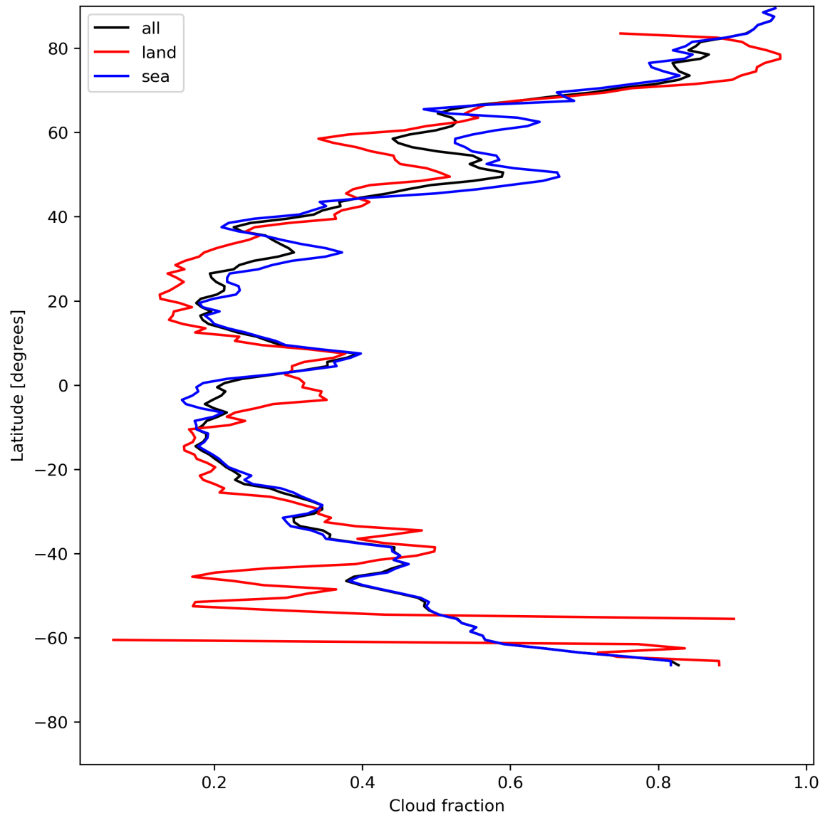
Figure 15: Zonal average of “Cloud fraction” for 2024-05-23 to 2024-05-24.
