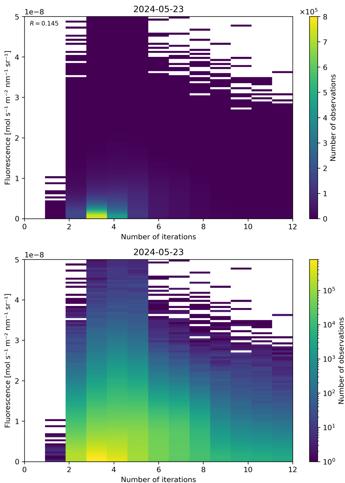
Figure 98: Scatter density plot of “Number of iterations” against “Fluorescence” for 2024-05-23 to 2024-05-24.
