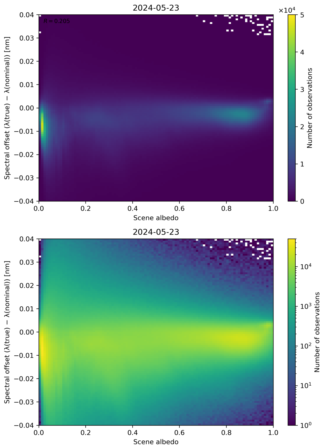
Figure 107: Scatter density plot of “Scene albedo” against “Spectral offset ( \lambda(\text{true}) - \lambda(\text{nominal}) )” for 2024-05-23 to 2024-05-24.
