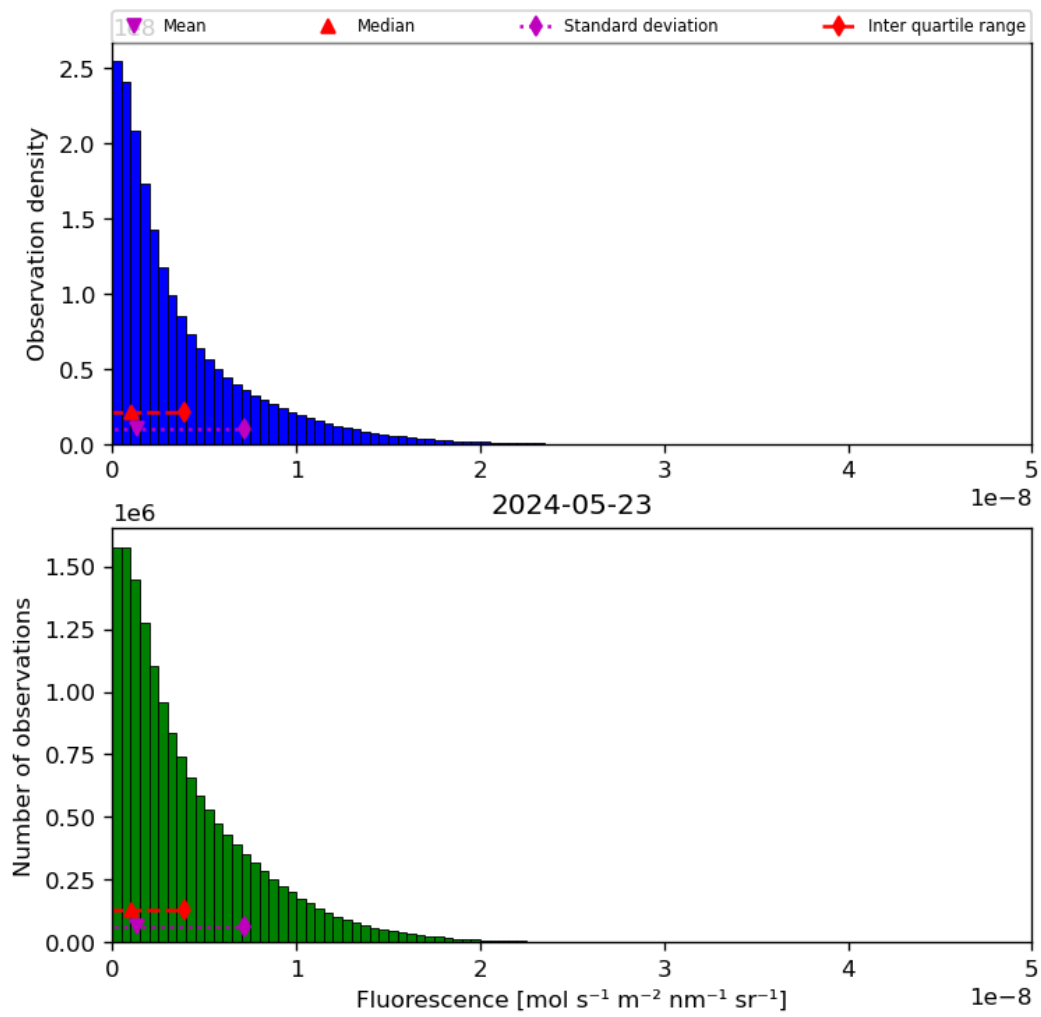
Figure 40: Histogram of “Fluorescence” for 2024-05-23 to 2024-05-24
