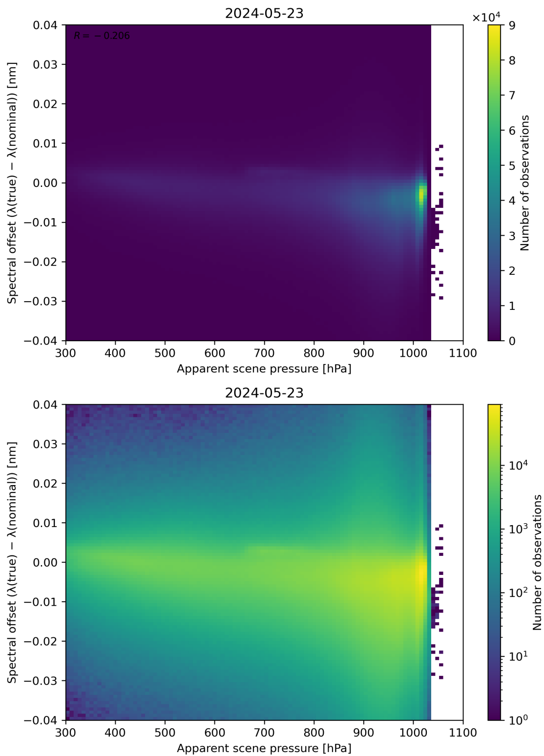
Figure 67: Scatter density plot of “Apparent scene pressure” against “Spectral offset ( \lambda(\text{true}) - \lambda(\text{nominal}) )” for 2024-05-23 to 2024-05-24.
