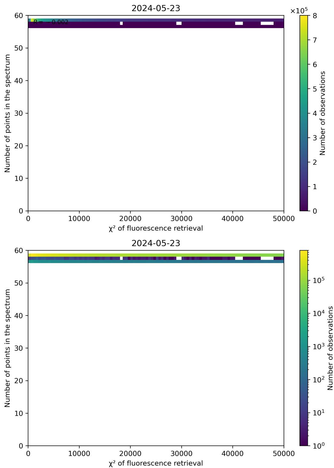
Figure 68: Scatter density plot of " \chi^2 of fluorescence retrieval" against "Number of points in the spectrum" for 2024-05-23 to 2024-05-24.
