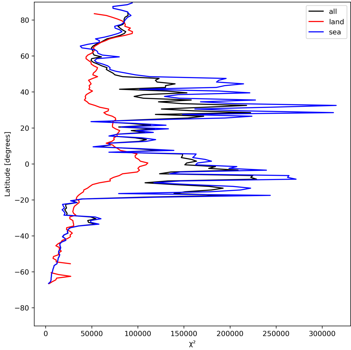
Figure 21: Zonal average of “ \chi^2 ” for 2024-05-23 to 2024-05-24.
