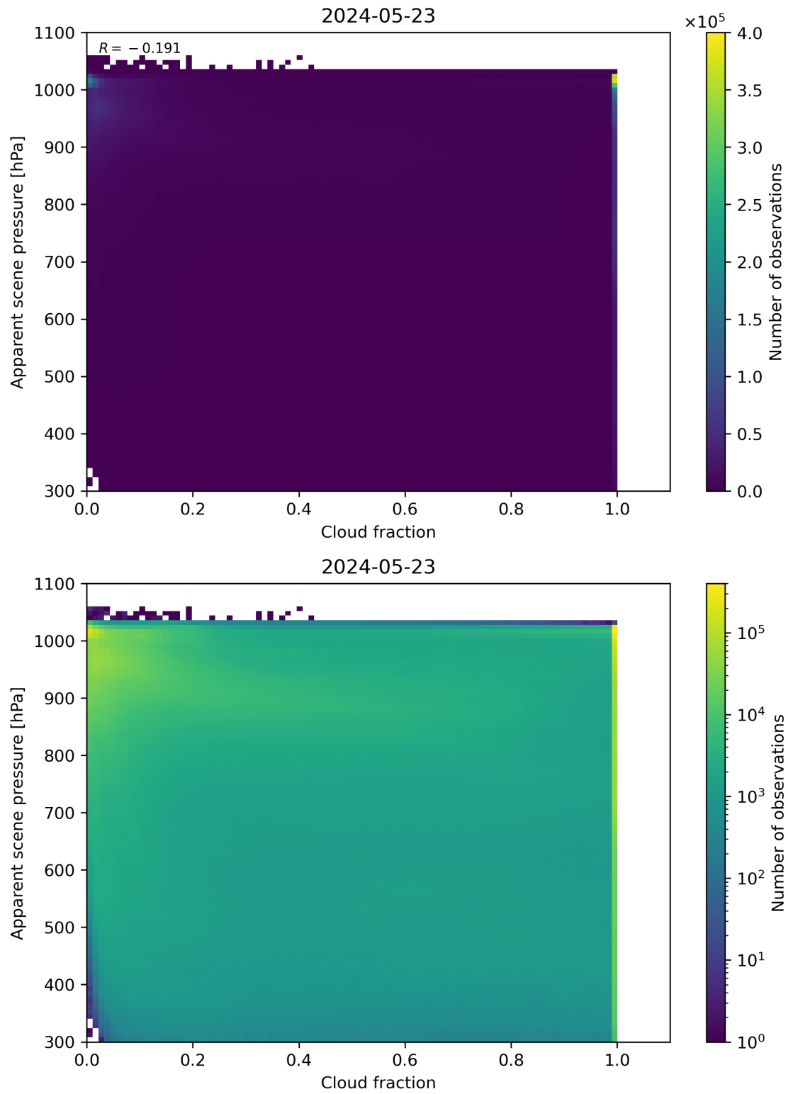
Figure 70: Scatter density plot of “Cloud fraction” against “Apparent scene pressure” for 2024-05-23 to 2024-05-24.
