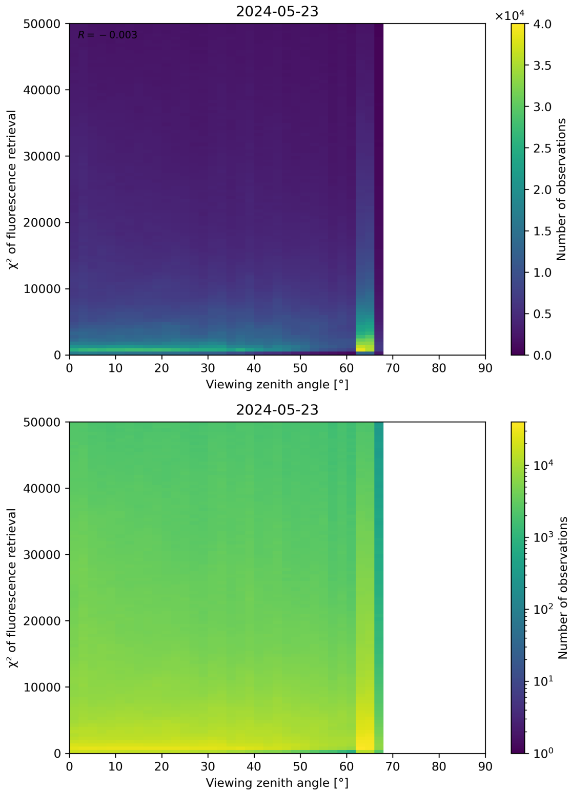
Figure 119: Scatter density plot of “Viewing zenith angle” against “ \chi^2 of fluorescence retrieval” for 2024-05-23 to 2024-05-24.
