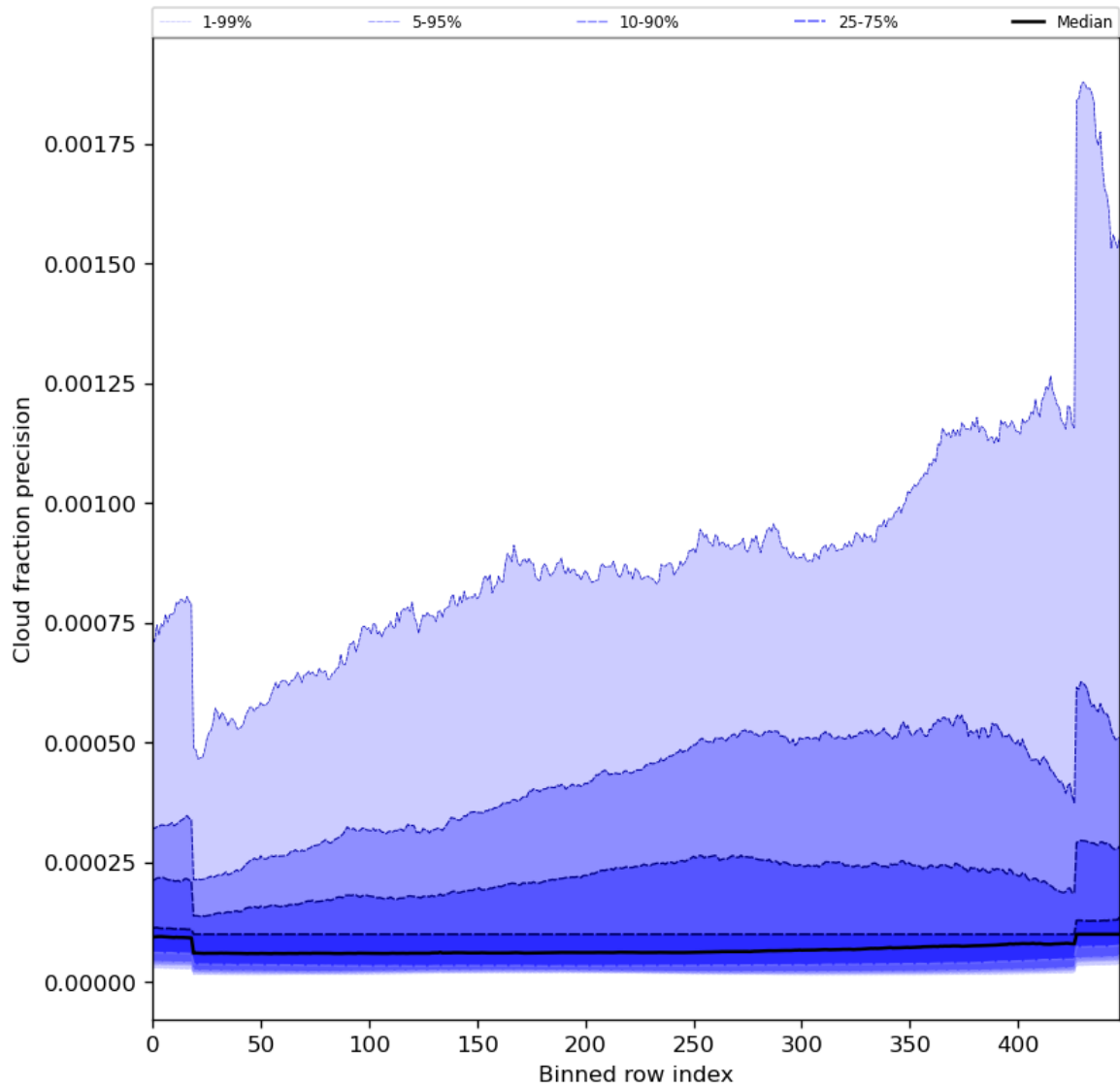
Figure 50: Along track statistics of “Cloud fraction precision” for 2024-05-23 to 2024-05-24
