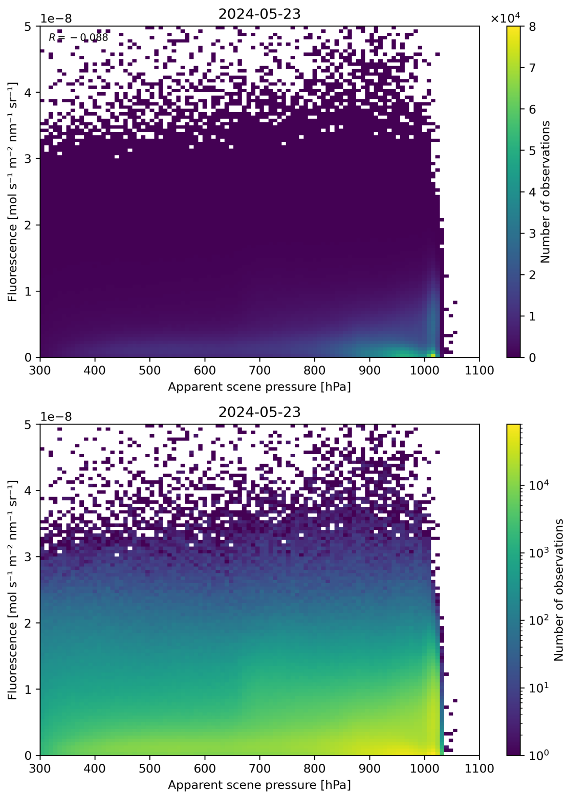
Figure 64: Scatter density plot of “Apparent scene pressure” against “Fluorescence” for 2024-05-23 to 2024-05-24.
