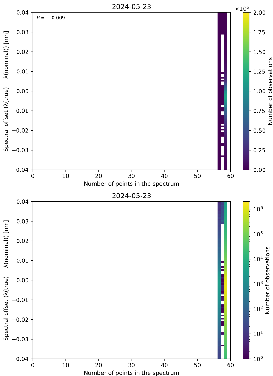
Figure 101: Scatter density plot of “Number of points in the spectrum” against “Spectral offset ( \lambda(\text{true}) - \lambda(\text{nominal}) )” for 2024-05-23 to 2024-05-24.
