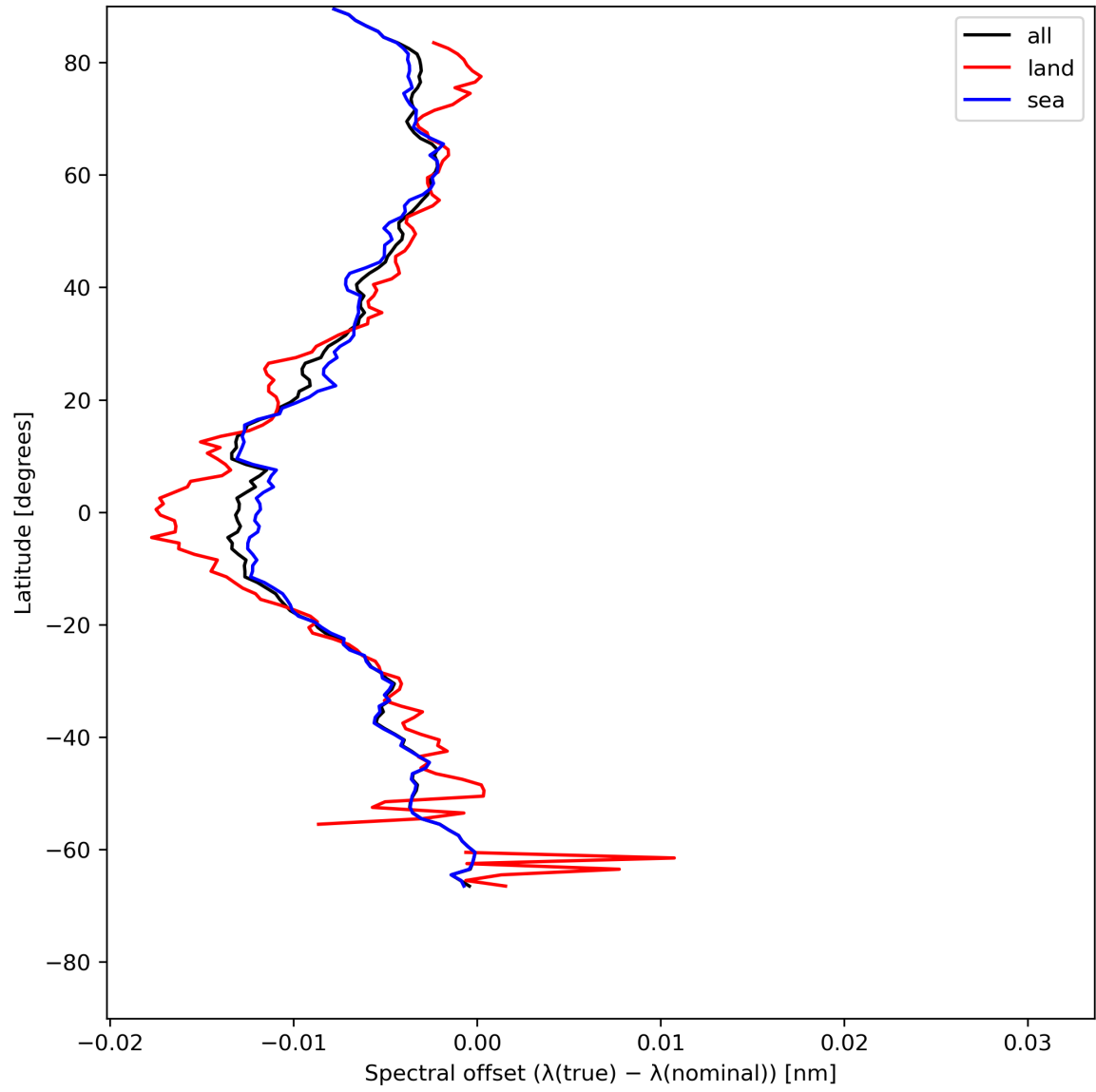
Figure 28: Zonal average of “Spectral offset ( \lambda(\text{true}) - \lambda(\text{nominal}) )” for 2024-05-23 to 2024-05-24.
