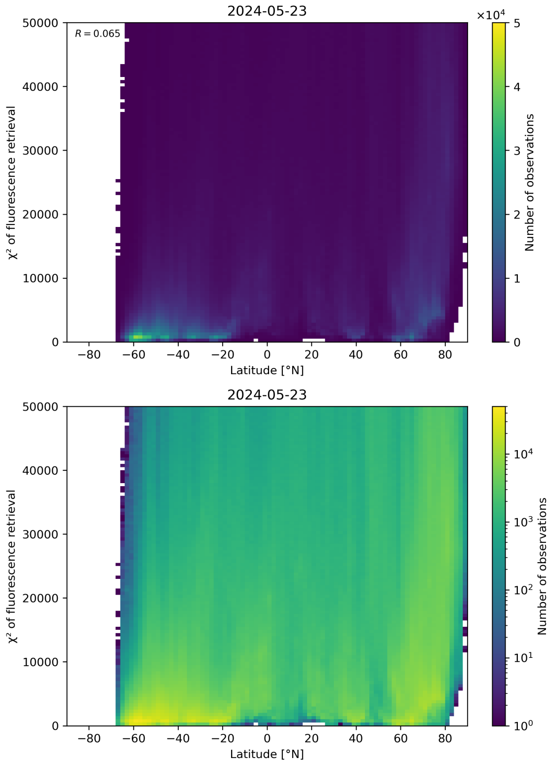
Figure 89: Scatter density plot of “Latitude” against “ \chi^2 of fluorescence retrieval” for 2024-05-23 to 2024-05-24.
