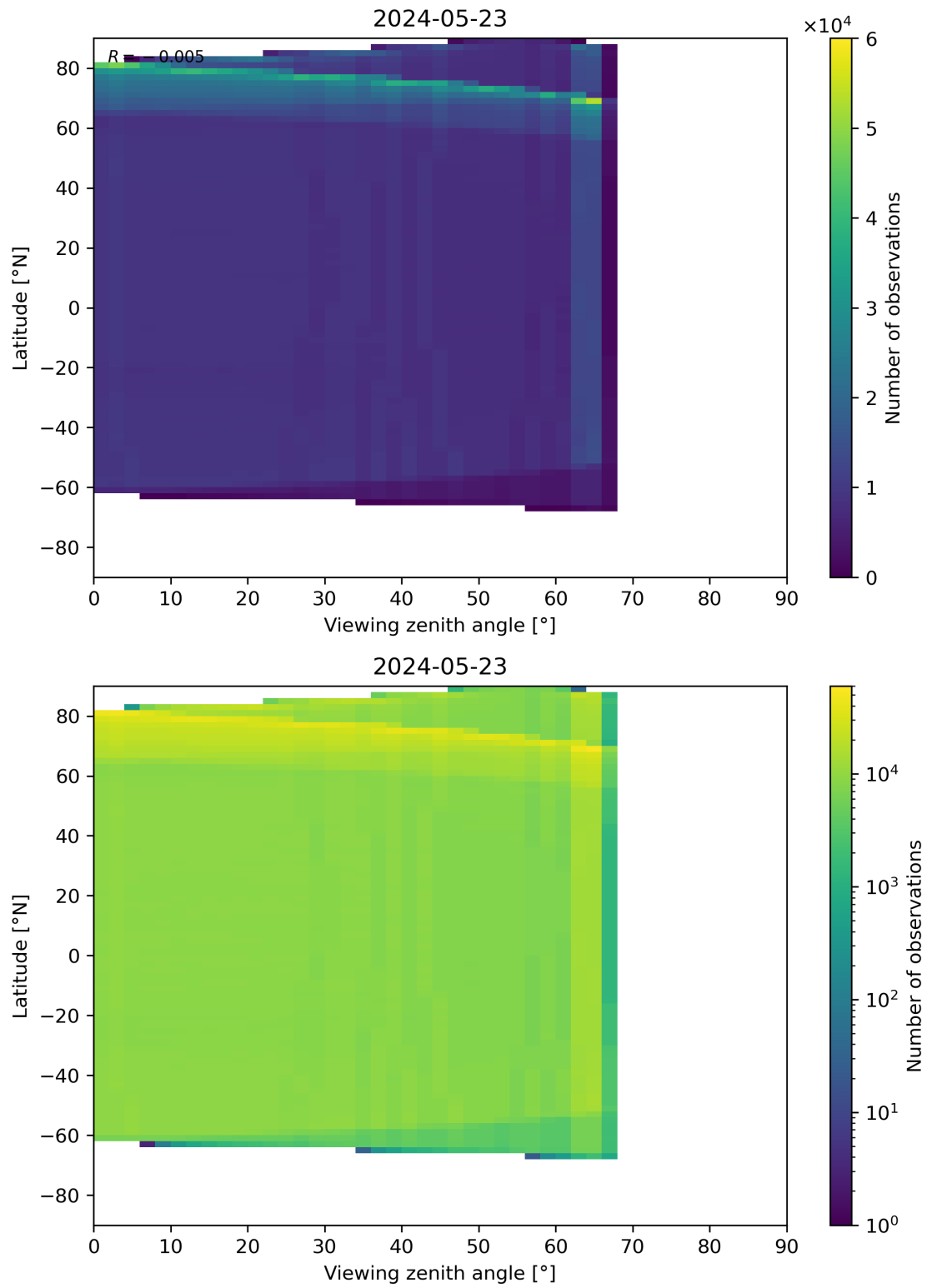
Figure 123: Scatter density plot of “Viewing zenith angle” against “Latitude” for 2024-05-23 to 2024-05-24.
