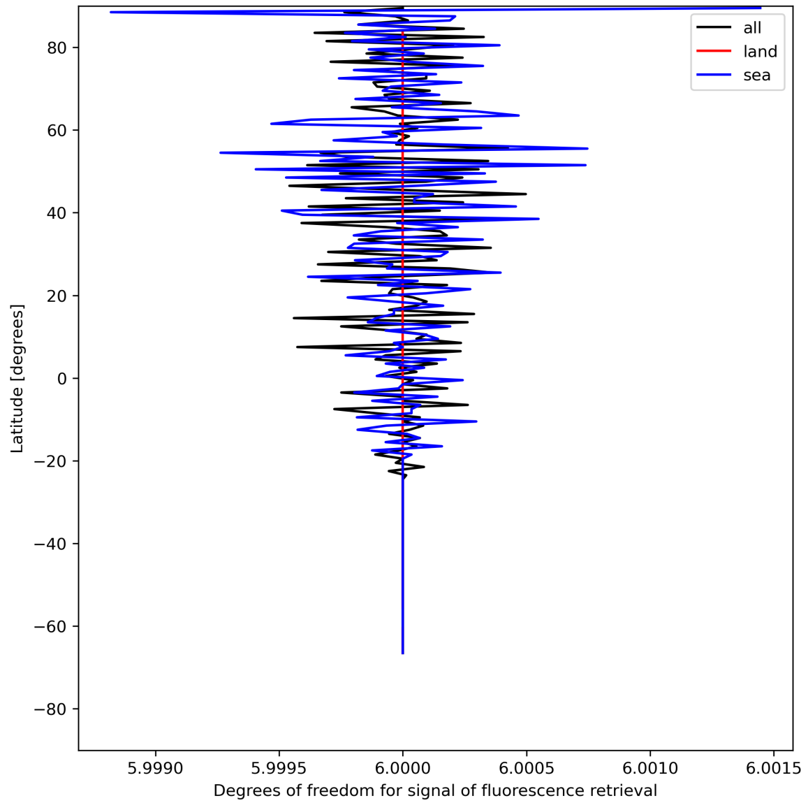
Figure 26: Zonal average of “Degrees of freedom for signal of fluorescence retrieval” for 2024-05-23 to 2024-05-24.
