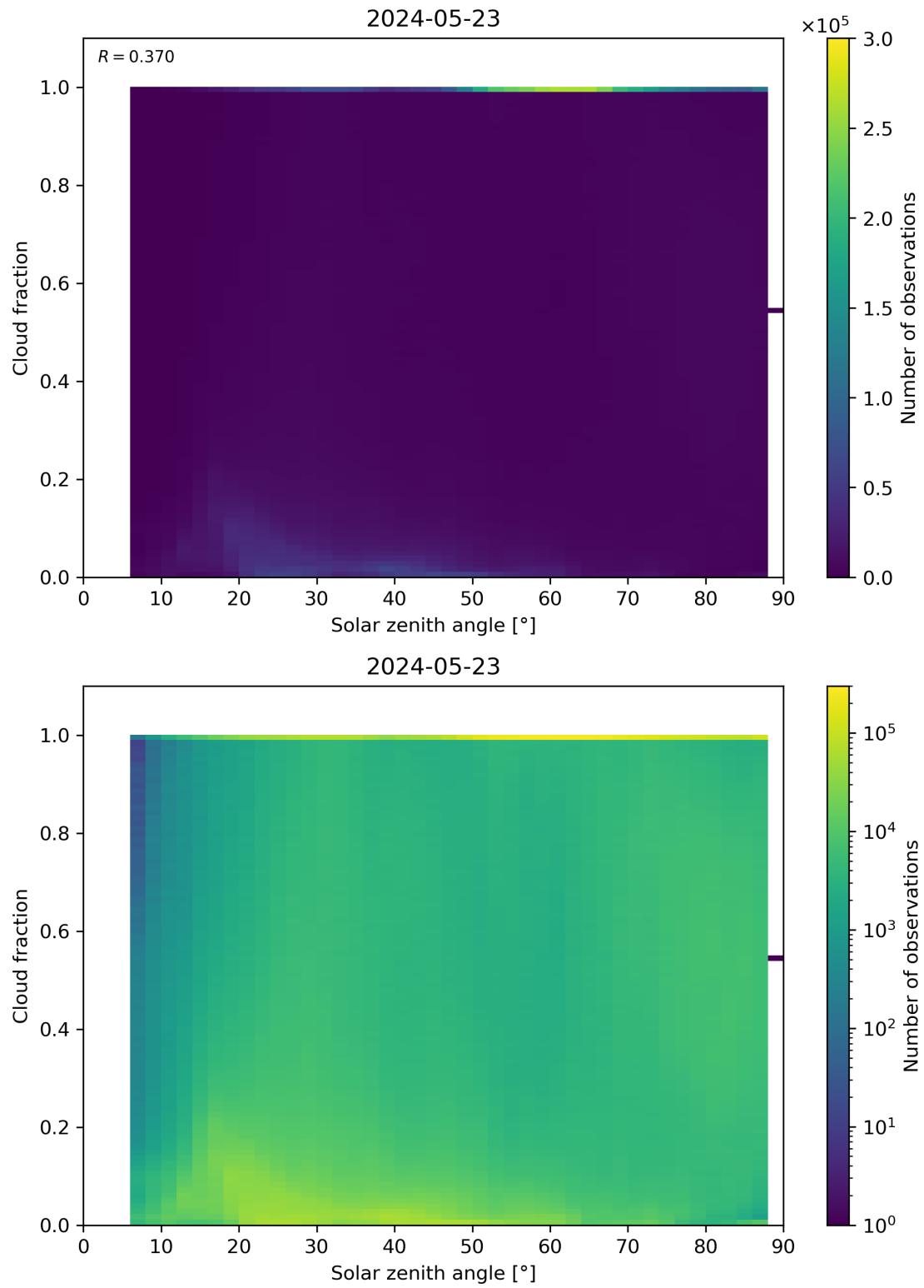
Figure 110: Scatter density plot of “Solar zenith angle” against “Cloud fraction” for 2024-05-23 to 2024-05-24.
