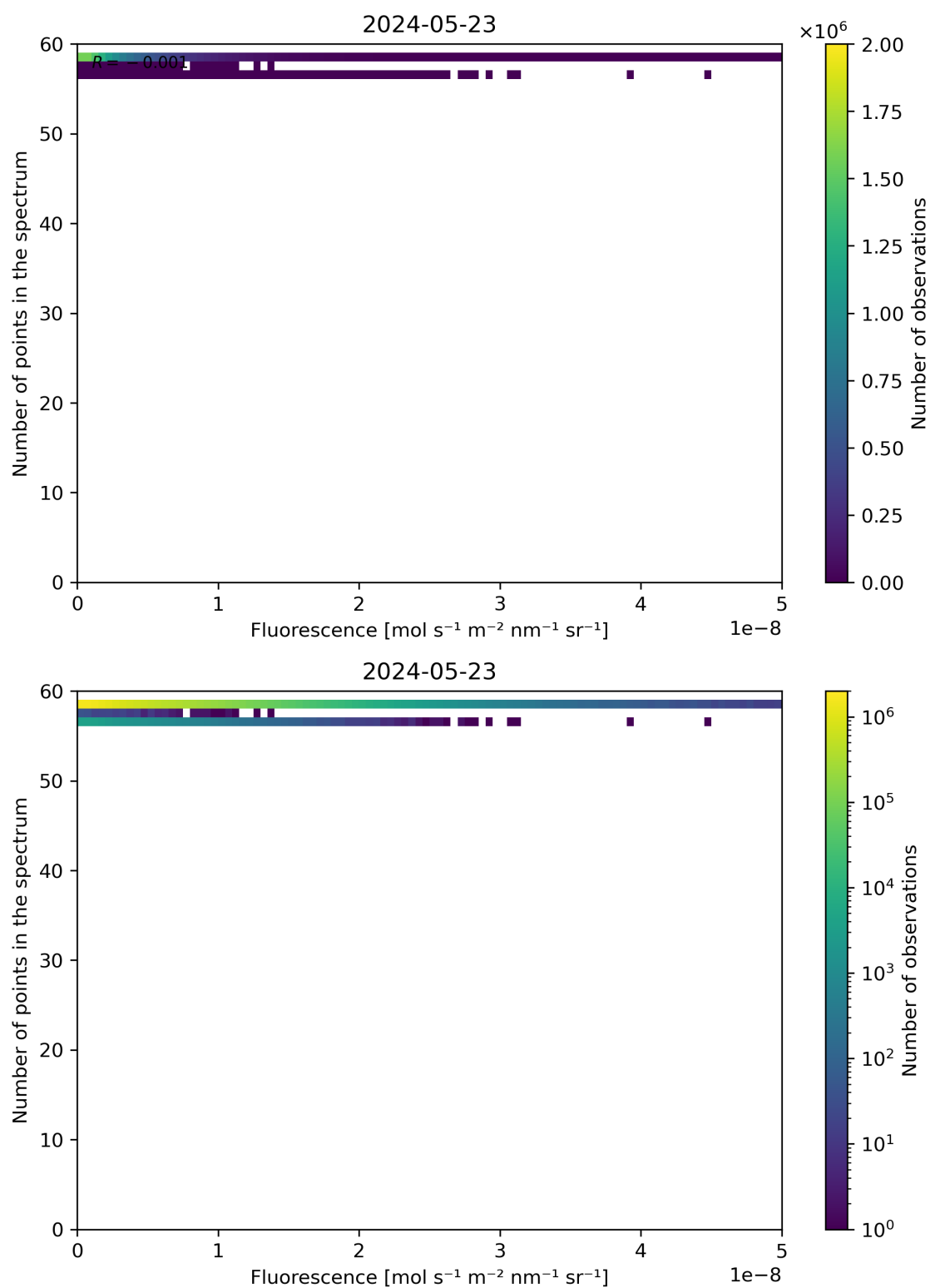
Figure 86: Scatter density plot of “Fluorescence” against “Number of points in the spectrum” for 2024-05-23 to 2024-05-24.
