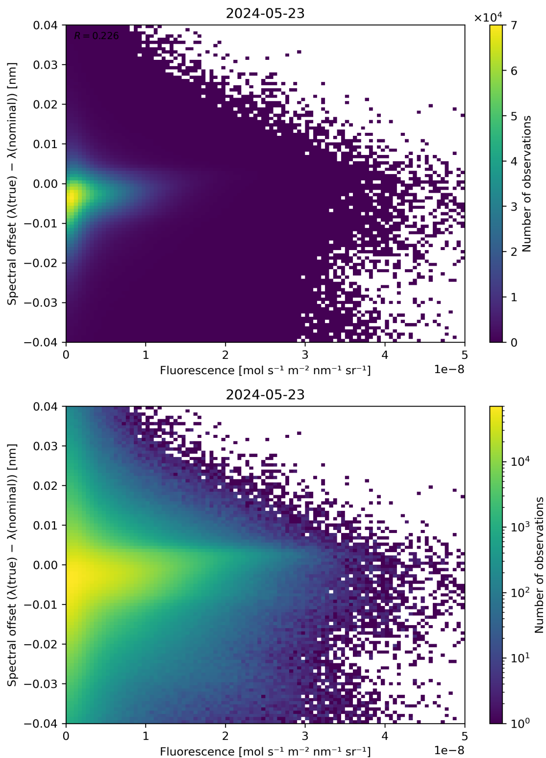
Figure 87: Scatter density plot of “Fluorescence” against “Spectral offset ( \lambda(\text{true}) - \lambda(\text{nominal}) )” for 2024-05-23 to 2024-05-24.
