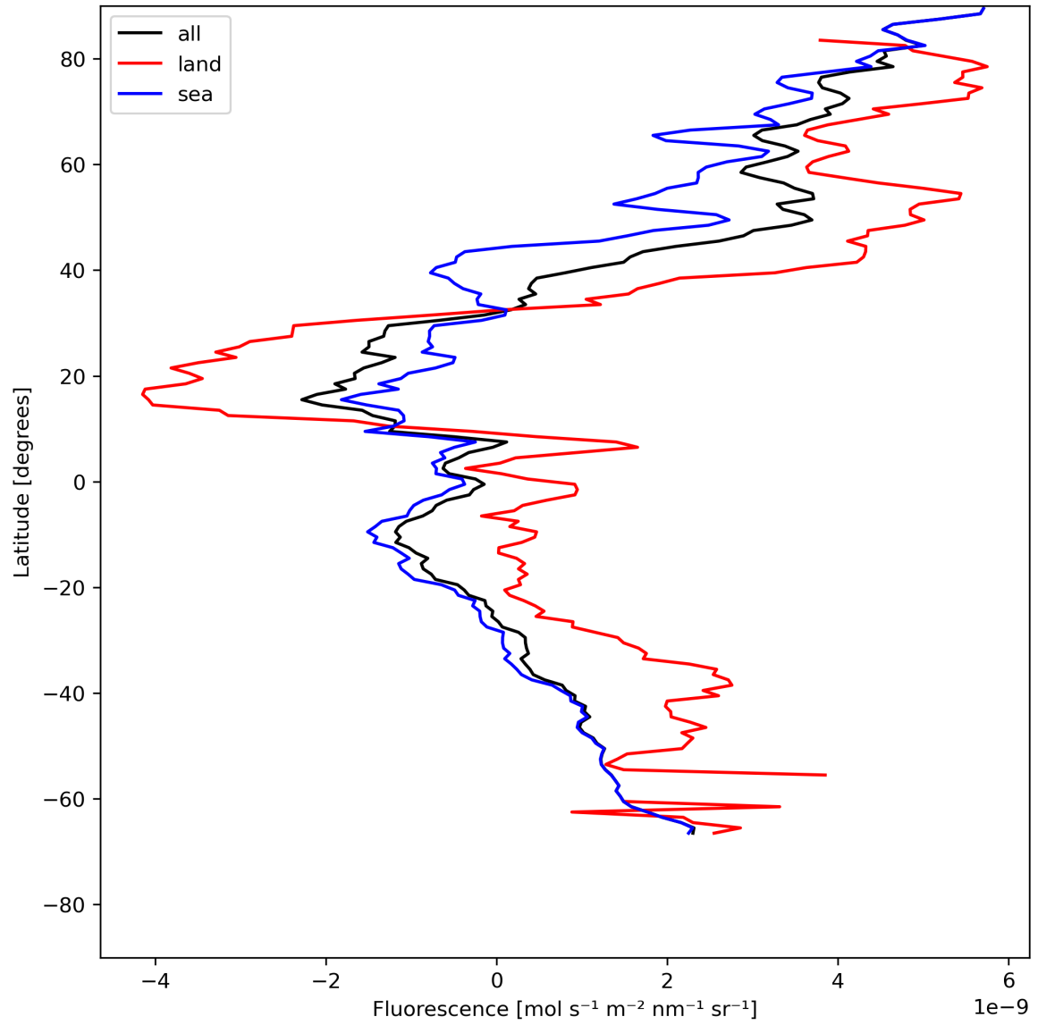
Figure 23: Zonal average of “Fluorescence” for 2024-05-23 to 2024-05-24.
