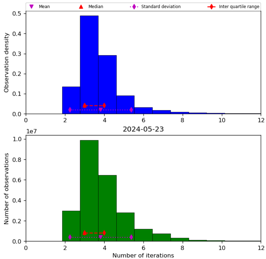
Figure 39: Histogram of “Number of iterations” for 2024-05-23 to 2024-05-24
