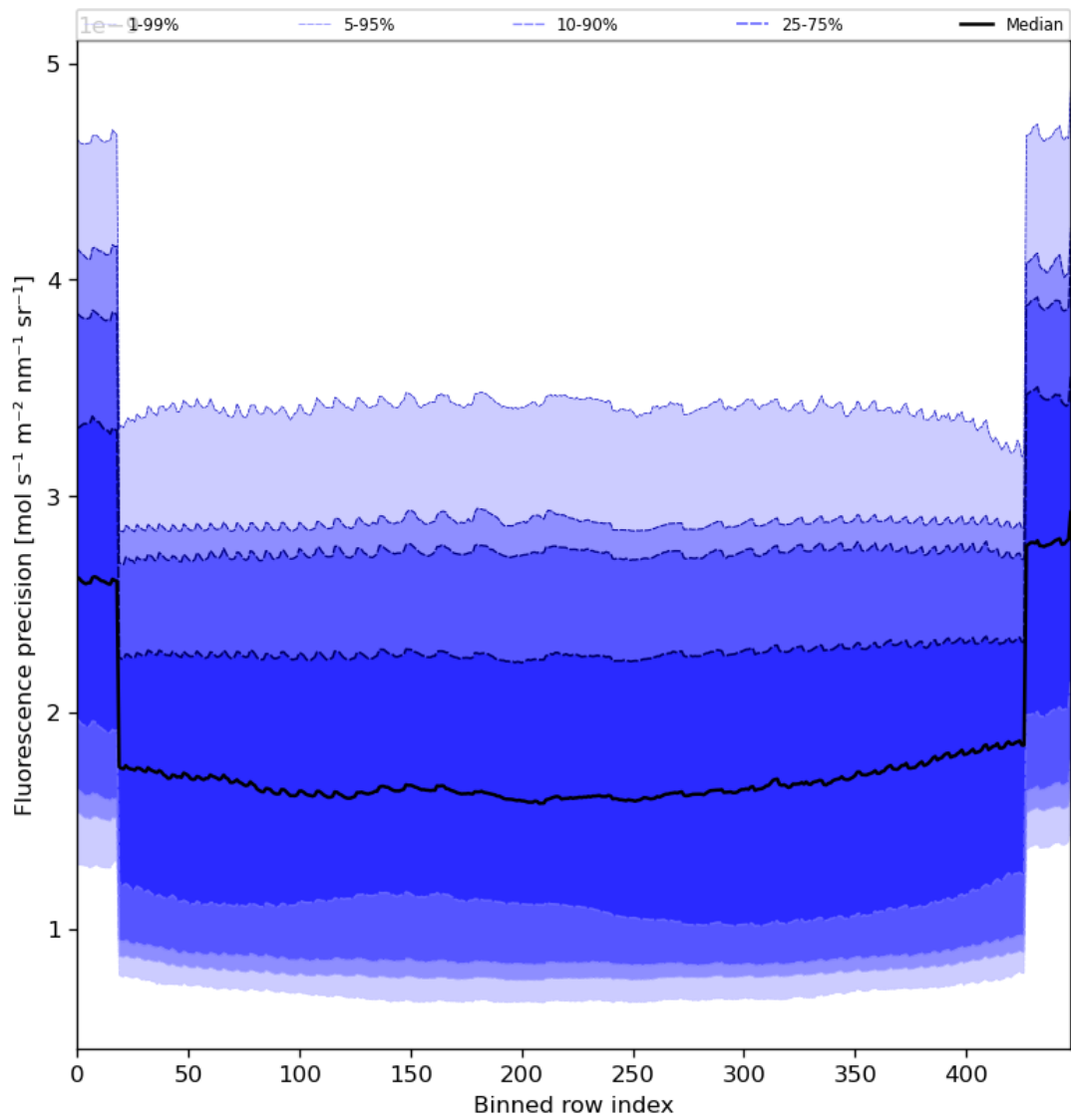
Figure 58: Along track statistics of “Fluorescence precision” for 2024-05-23 to 2024-05-24
