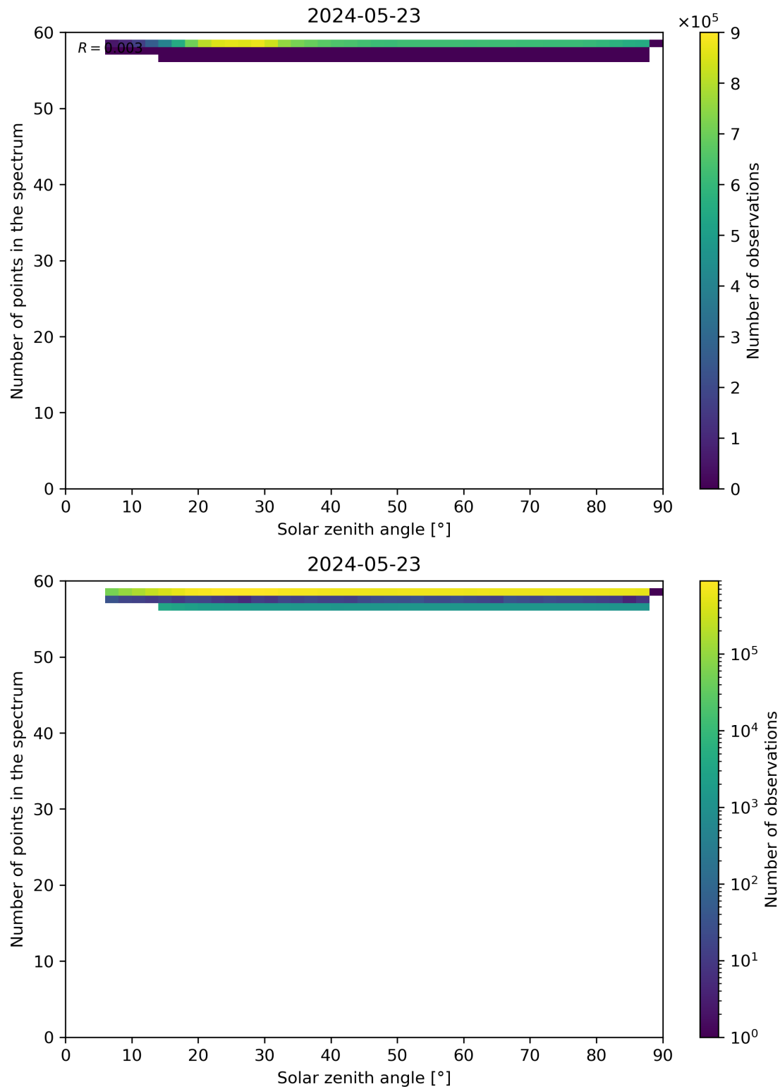
Figure 115: Scatter density plot of “Solar zenith angle” against “Number of points in the spectrum” for 2024-05-23 to 2024-05-24.
