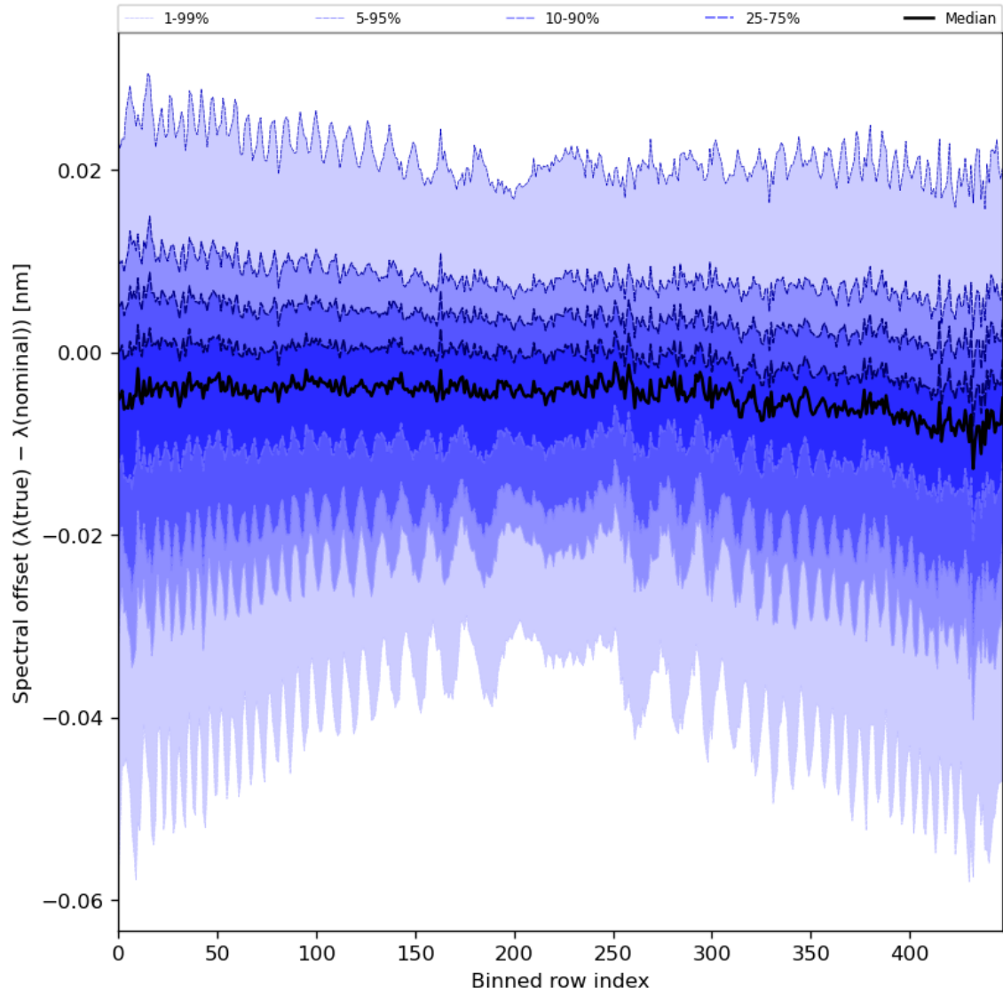
Figure 62: Along track statistics of “Spectral offset ( \lambda(\text{true}) - \lambda(\text{nominal}) )” for 2024-05-23 to 2024-05-24
