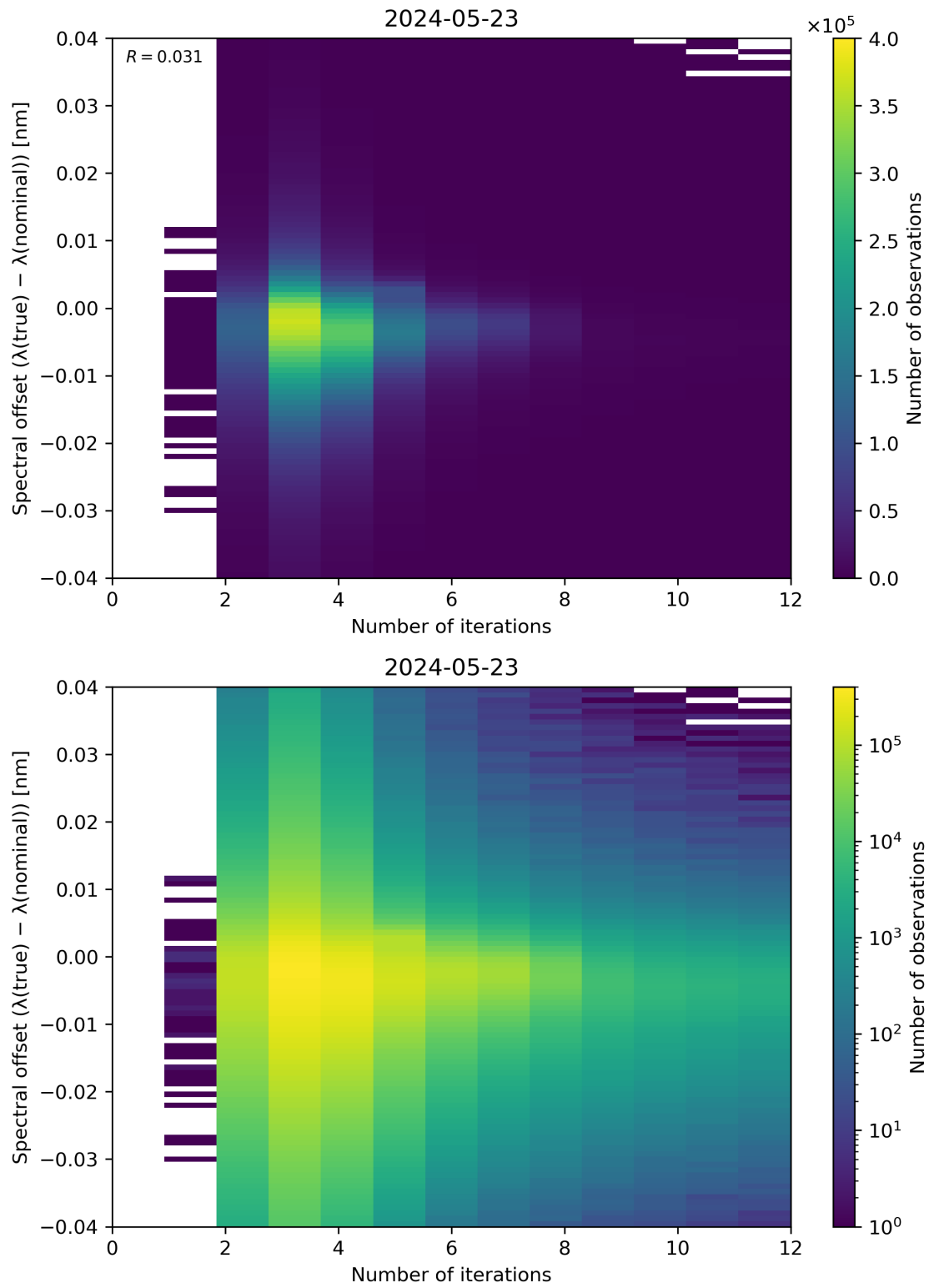
Figure 100: Scatter density plot of “Number of iterations” against “Spectral offset ( \lambda(\text{true}) - \lambda(\text{nominal}) )” for 2024-05-23 to 2024-05-24.
