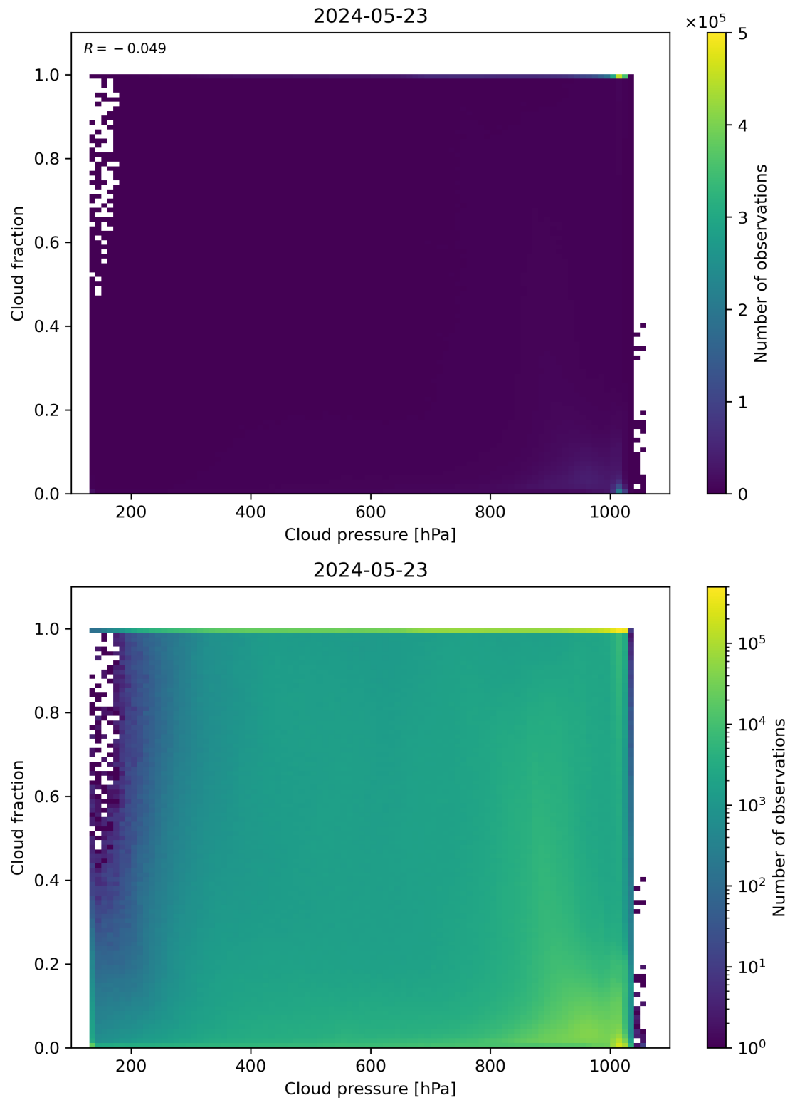
Figure 79: Scatter density plot of “Cloud pressure” against “Cloud fraction” for 2024-05-23 to 2024-05-24.
