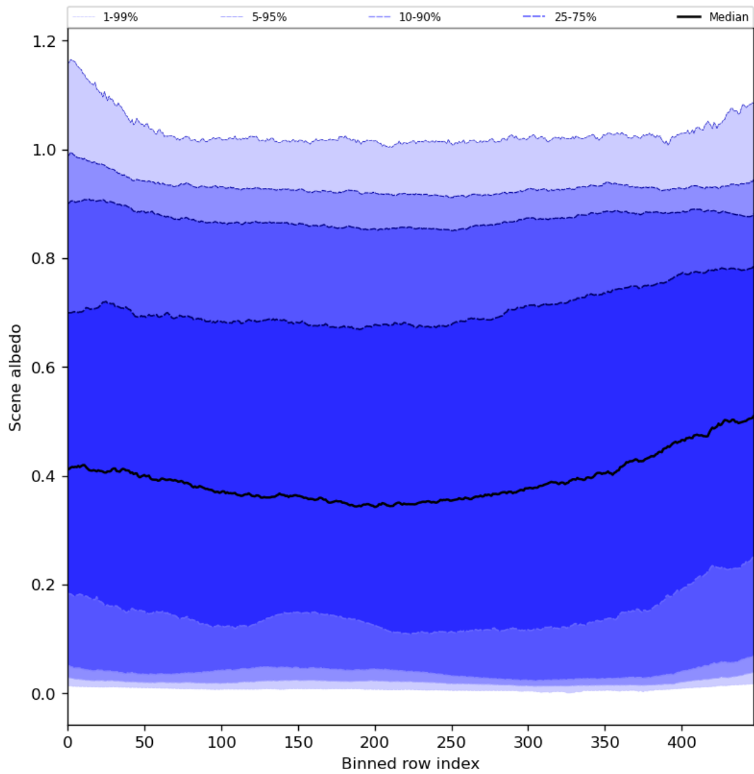
Figure 51: Along track statistics of “Scene albedo” for 2024-05-23 to 2024-05-24
