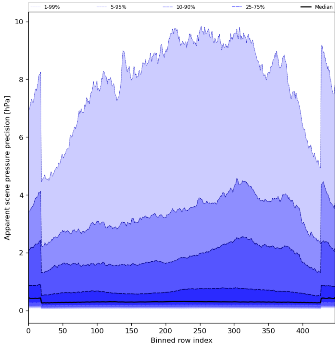
Figure 54: Along track statistics of “Apparent scene pressure precision” for 2024-05-23 to 2024-05-24
