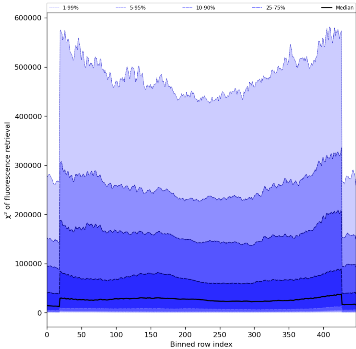
Figure 59: Along track statistics of “ \chi^2 of fluorescence retrieval” for 2024-05-23 to 2024-05-24
