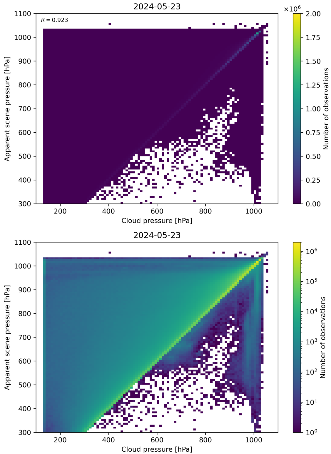
Figure 77: Scatter density plot of “Cloud pressure” against “Apparent scene pressure” for 2024-05-23 to 2024-05-24.
