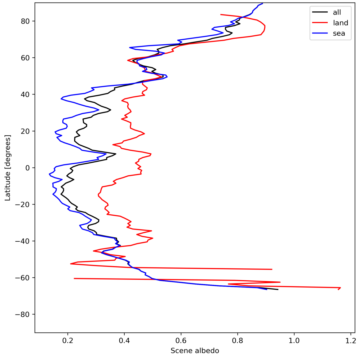
Figure 17: Zonal average of “Scene albedo” for 2024-05-23 to 2024-05-24.
