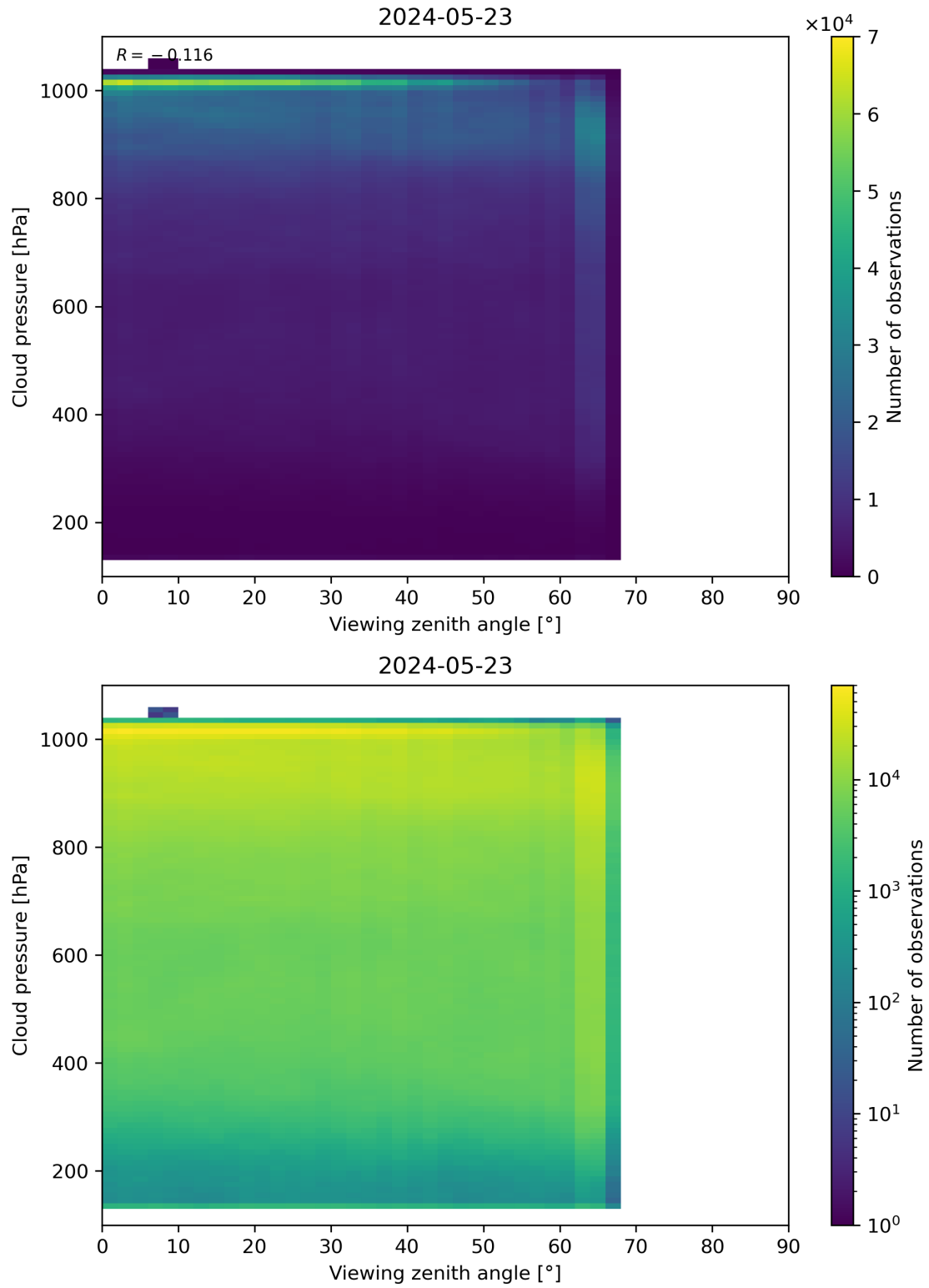
Figure 121: Scatter density plot of “Viewing zenith angle” against “Cloud pressure” for 2024-05-23 to 2024-05-24.
