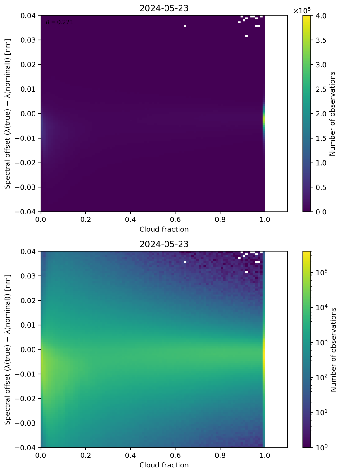
Figure 76: Scatter density plot of “Cloud fraction” against “Spectral offset ( \lambda(\text{true}) - \lambda(\text{nominal}) )” for 2024-05-23 to 2024-05-24.
