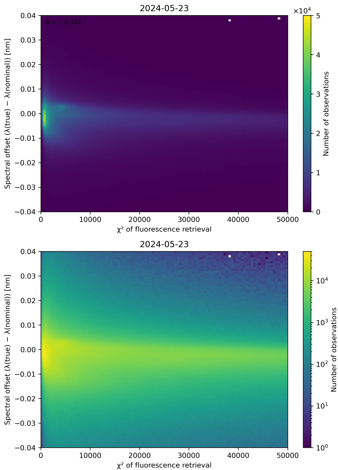
Figure 69: Scatter density plot of “ \chi^2 of fluorescence retrieval” against “Spectral offset ( \lambda(\text{true}) - \lambda(\text{nominal}) )” for 2024-05-23 to 2024-05-24.
