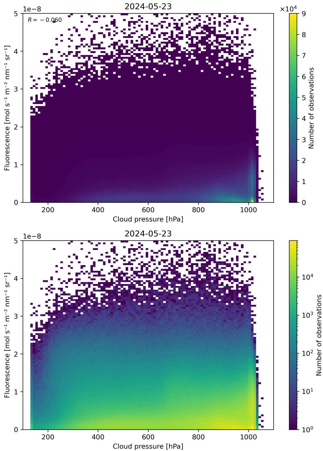
Figure 80: Scatter density plot of “Cloud pressure” against “Fluorescence” for 2024-05-23 to 2024-05-24.
