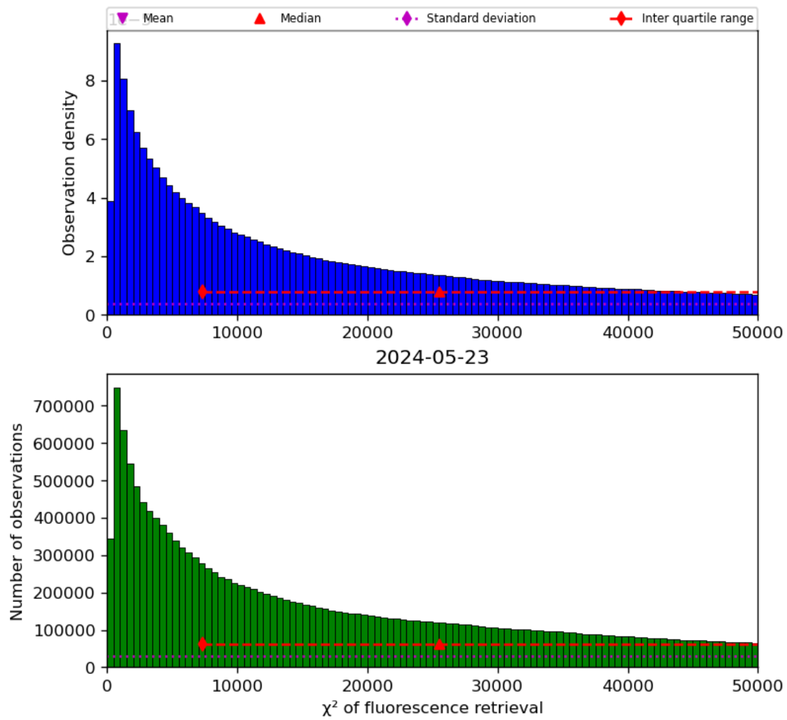
Figure 42: Histogram of “ \chi^2 of fluorescence retrieval” for 2024-05-23 to 2024-05-24
