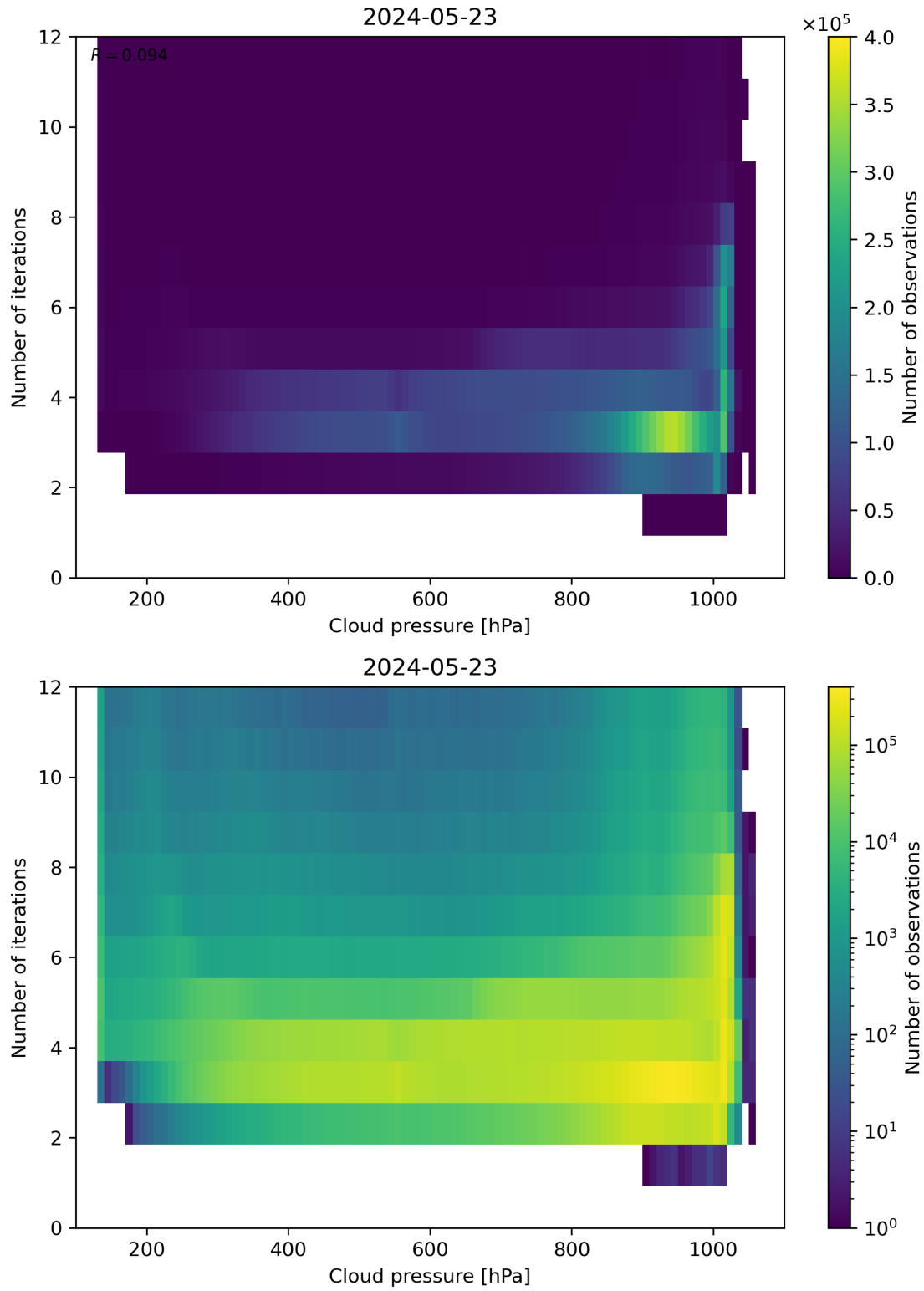
Figure 81: Scatter density plot of “Cloud pressure” against “Number of iterations” for 2024-05-23 to 2024-05-24.
