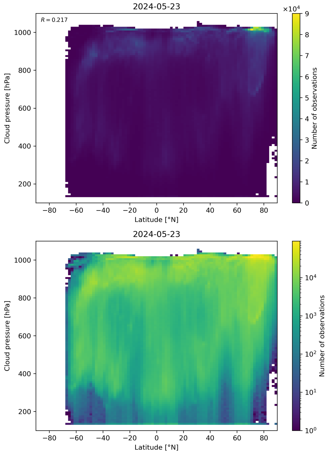
Figure 91: Scatter density plot of “Latitude” against “Cloud pressure” for 2024-05-23 to 2024-05-24.
