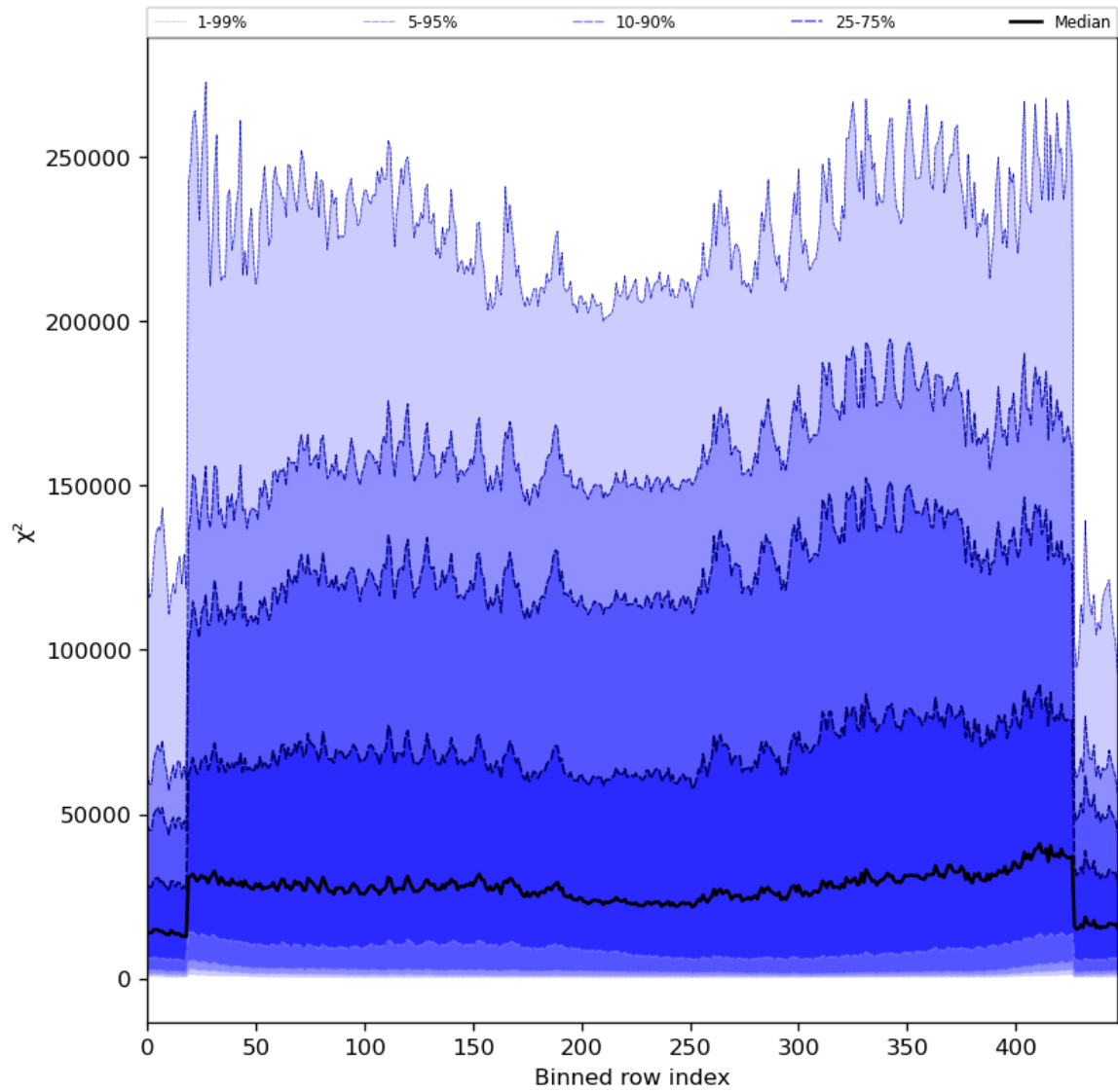
Figure 55: Along track statistics of “ \chi^2 ” for 2024-05-23 to 2024-05-24
