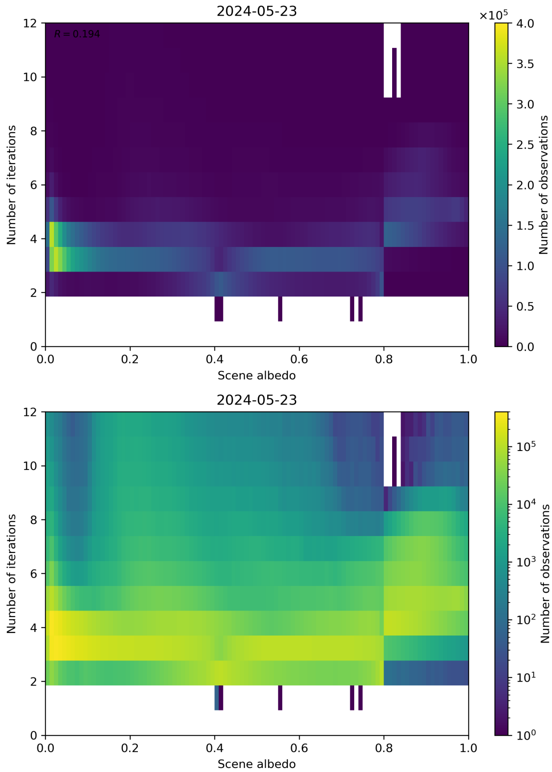
Figure 105: Scatter density plot of “Scene albedo” against “Number of iterations” for 2024-05-23 to 2024-05-24.
