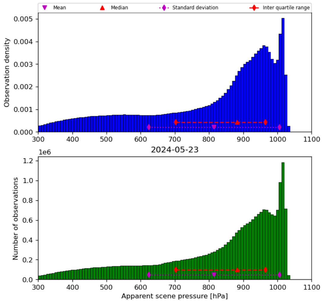
Figure 36: Histogram of “Apparent scene pressure” for 2024-05-23 to 2024-05-24
