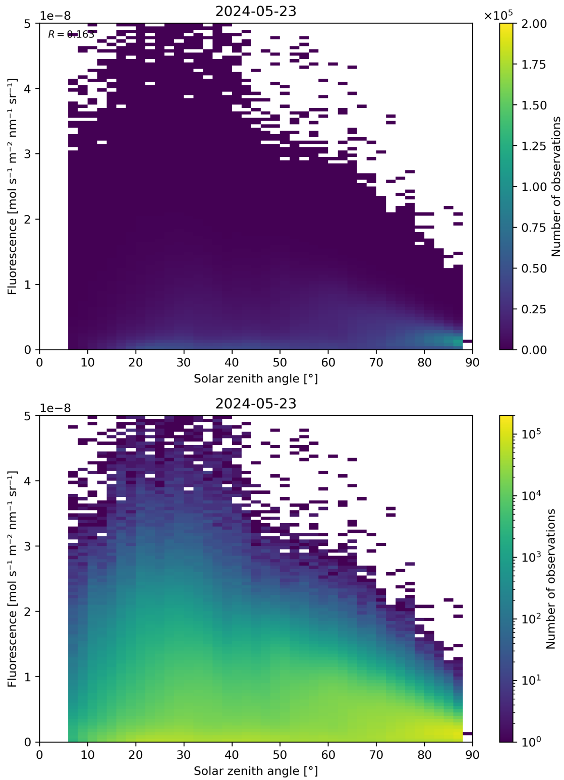
Figure 112: Scatter density plot of “Solar zenith angle” against “Fluorescence” for 2024-05-23 to 2024-05-24.
