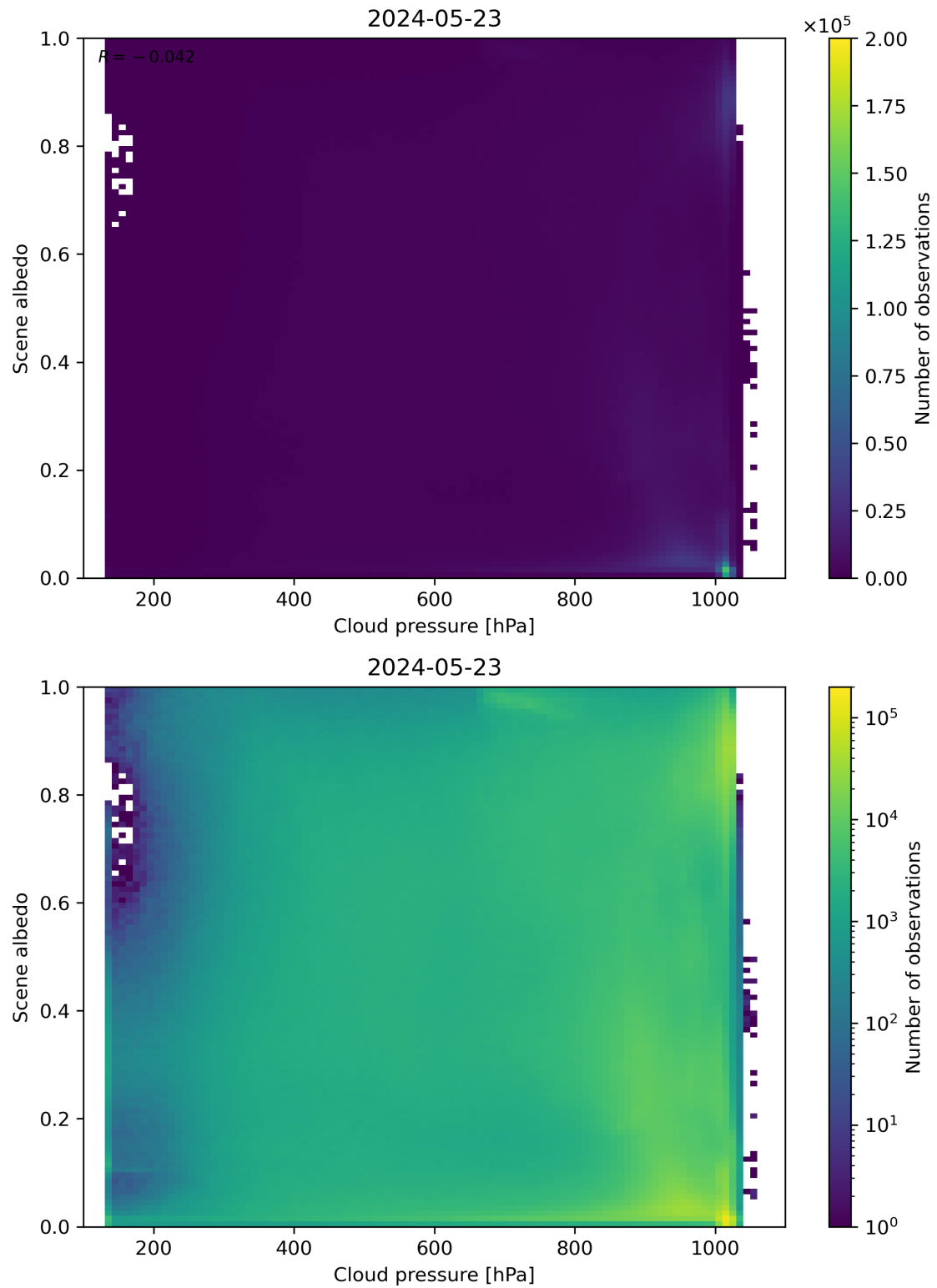
Figure 83: Scatter density plot of “Cloud pressure” against “Scene albedo” for 2024-05-23 to 2024-05-24.
