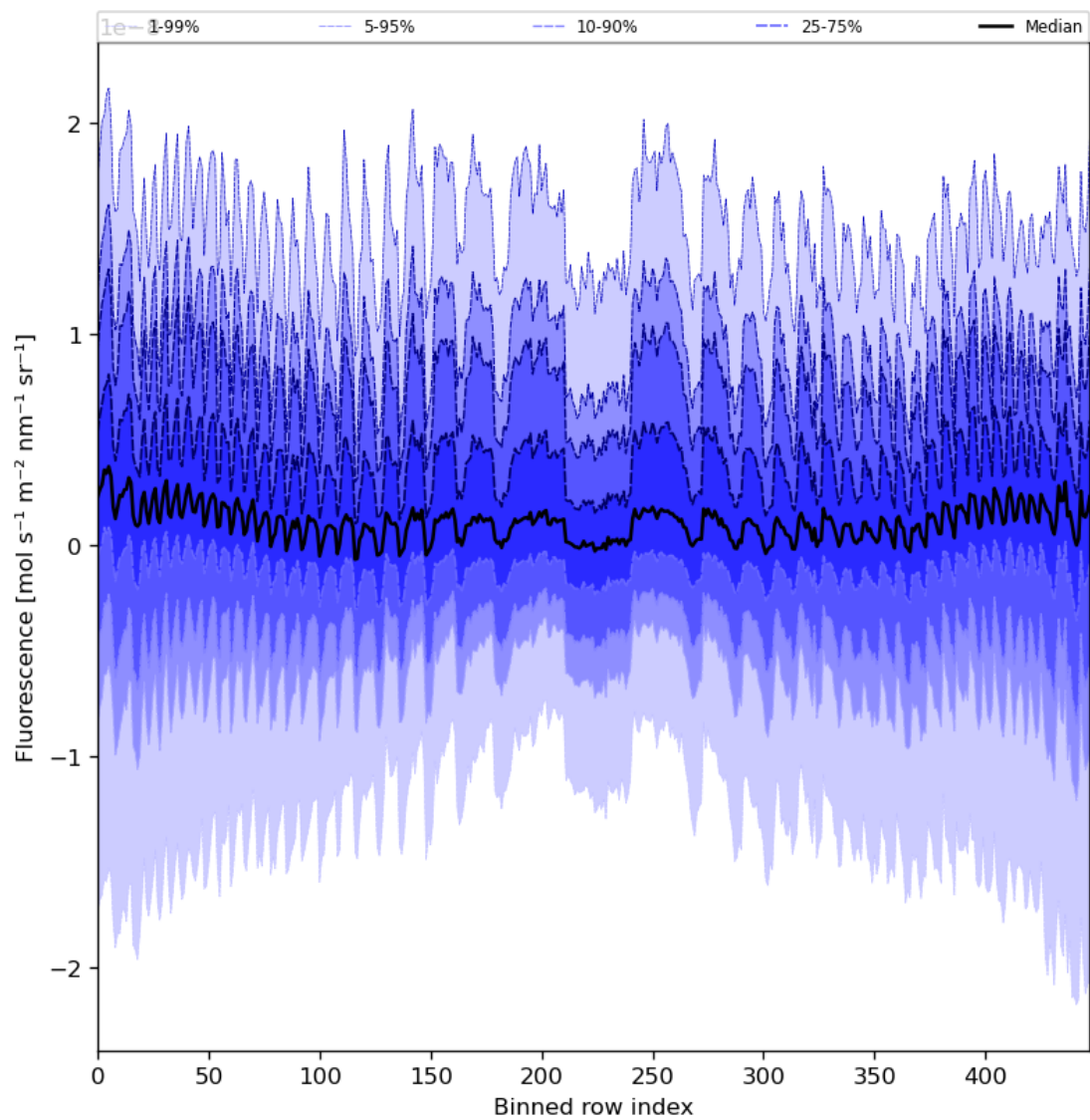
Figure 57: Along track statistics of “Fluorescence” for 2024-05-23 to 2024-05-24
