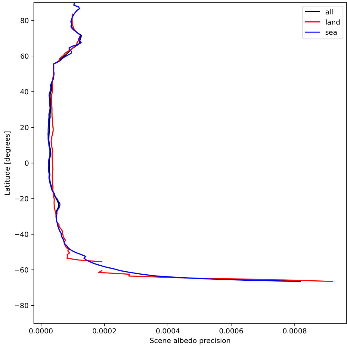
Figure 18: Zonal average of "Scene albedo precision" for 2024-05-23 to 2024-05-24.
