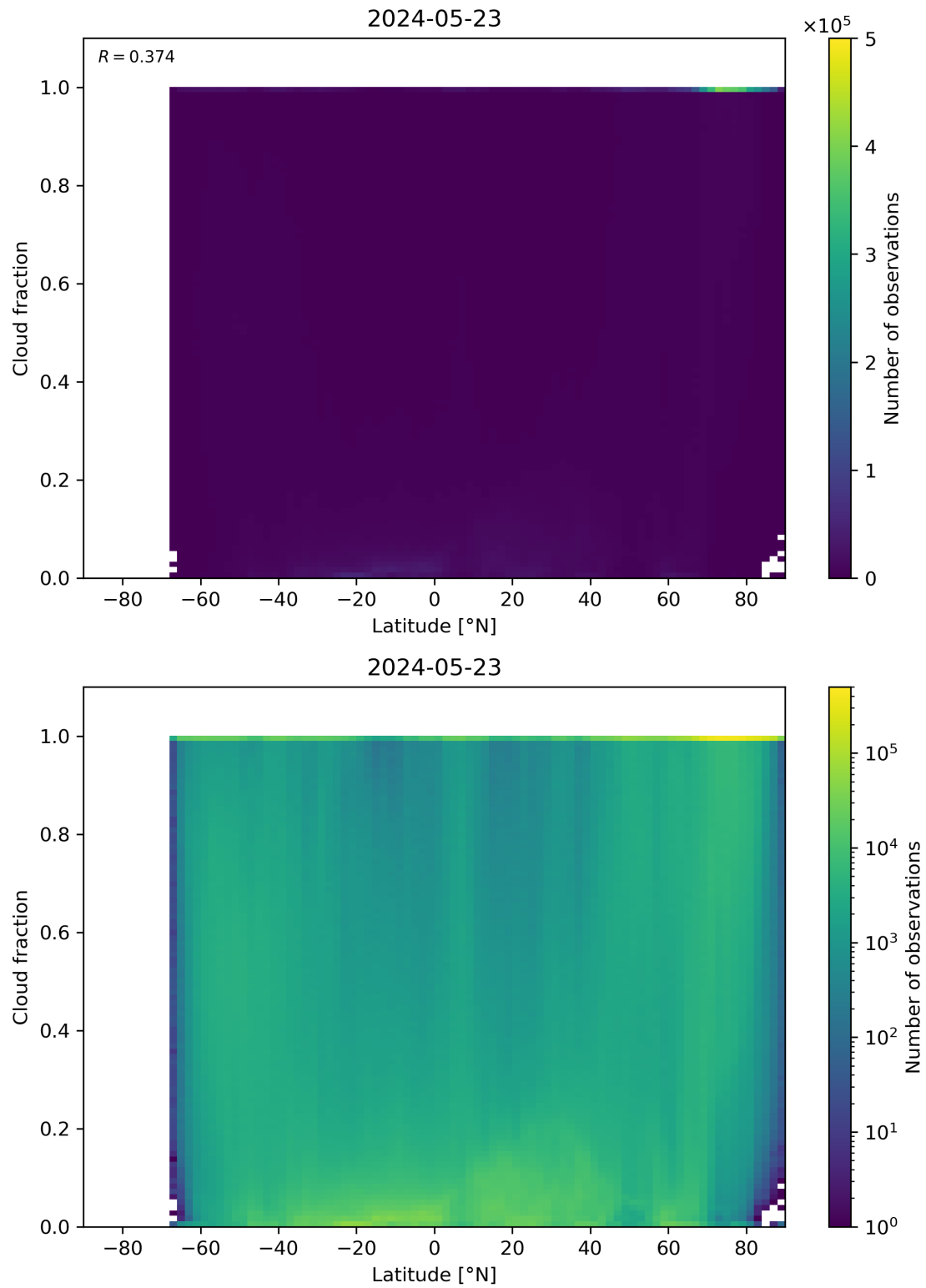
Figure 90: Scatter density plot of “Latitude” against “Cloud fraction” for 2024-05-23 to 2024-05-24.
