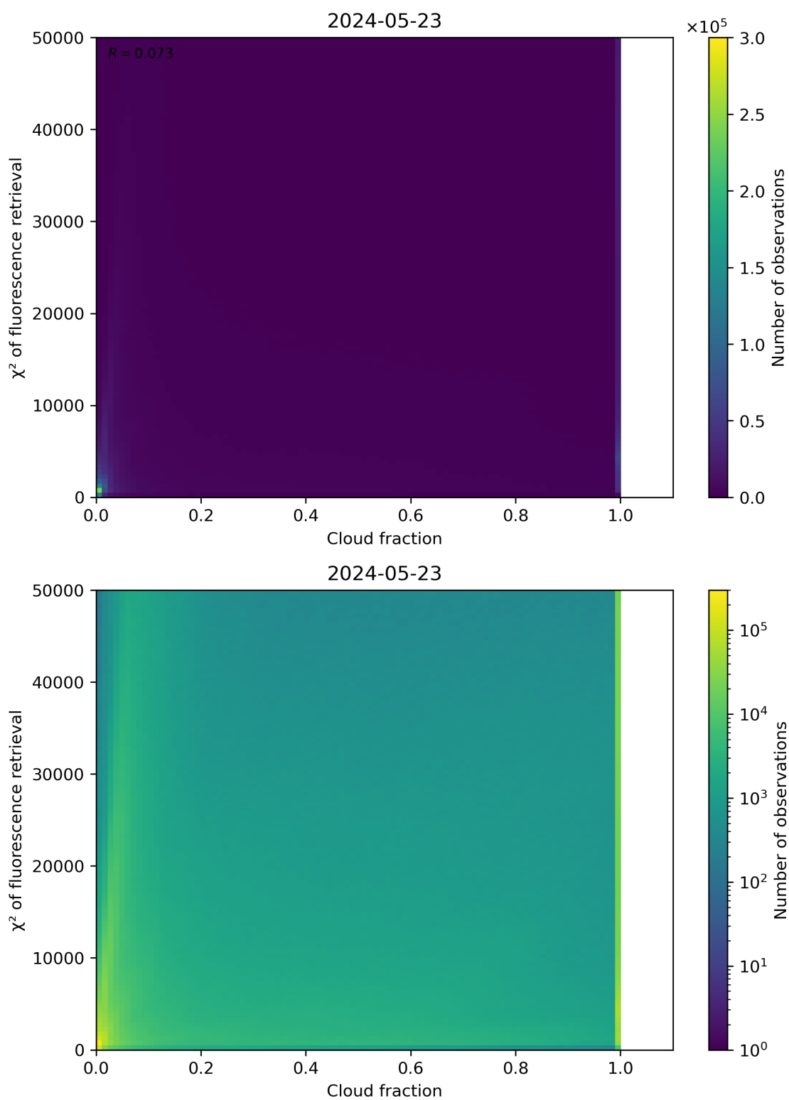
Figure 71: Scatter density plot of “Cloud fraction” against “ \chi^2 of fluorescence retrieval” for 2024-05-23 to 2024-05-24.
