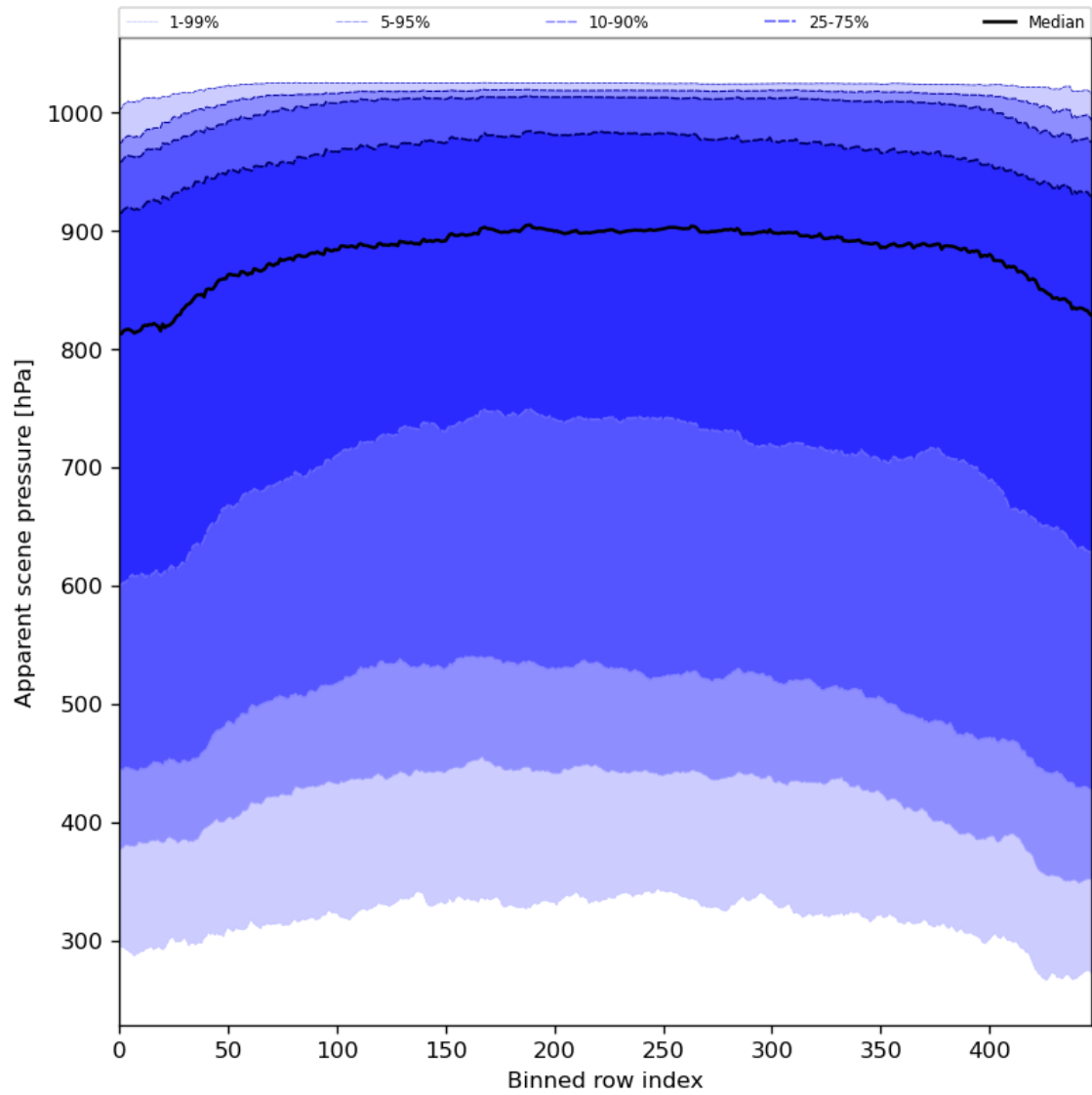
Figure 53: Along track statistics of “Apparent scene pressure” for 2024-05-23 to 2024-05-24
