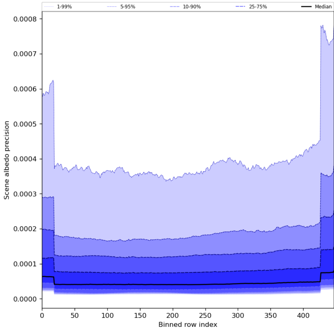
Figure 52: Along track statistics of “Scene albedo precision” for 2024-05-23 to 2024-05-24
