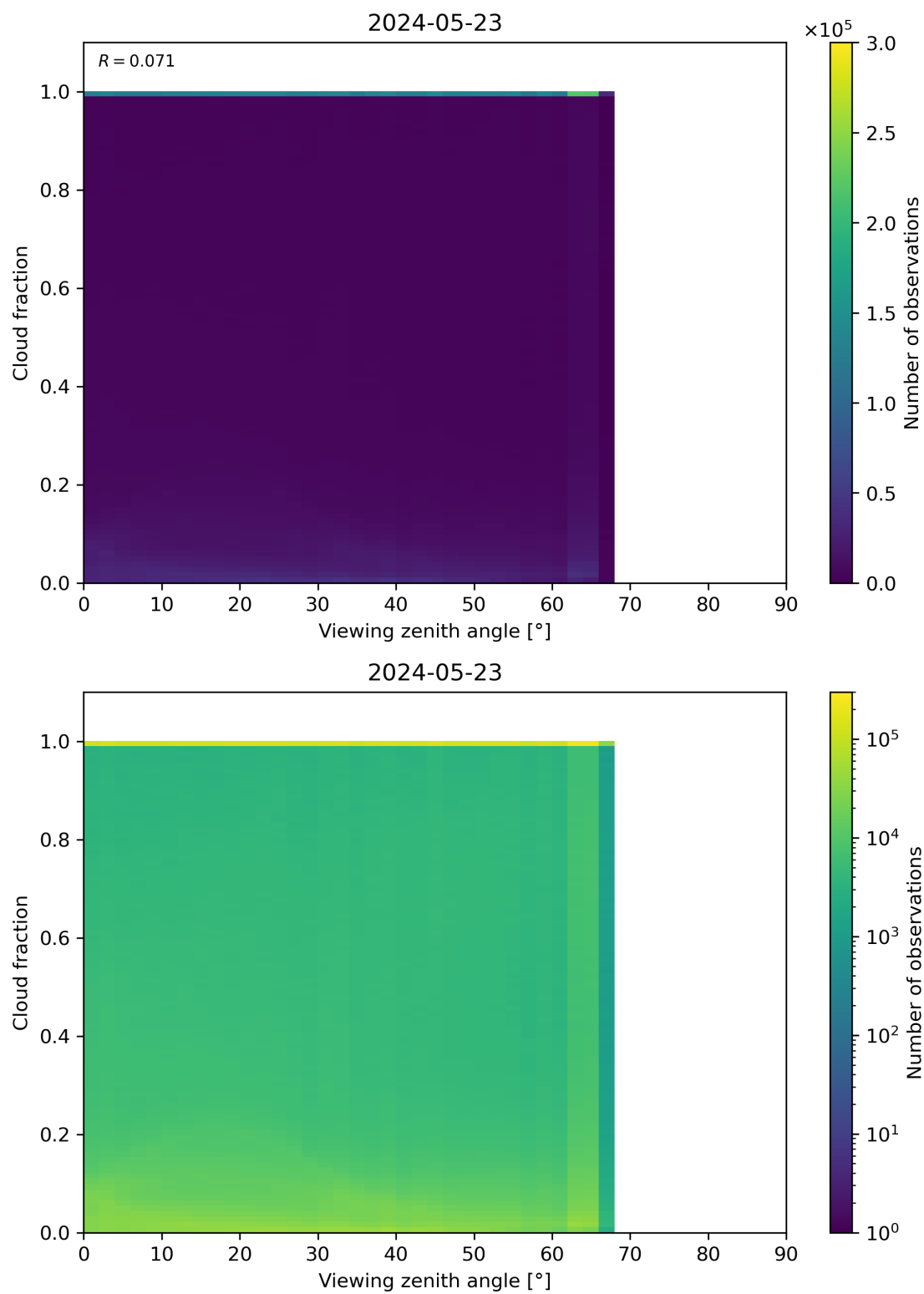
Figure 120: Scatter density plot of “Viewing zenith angle” against “Cloud fraction” for 2024-05-23 to 2024-05-24.
