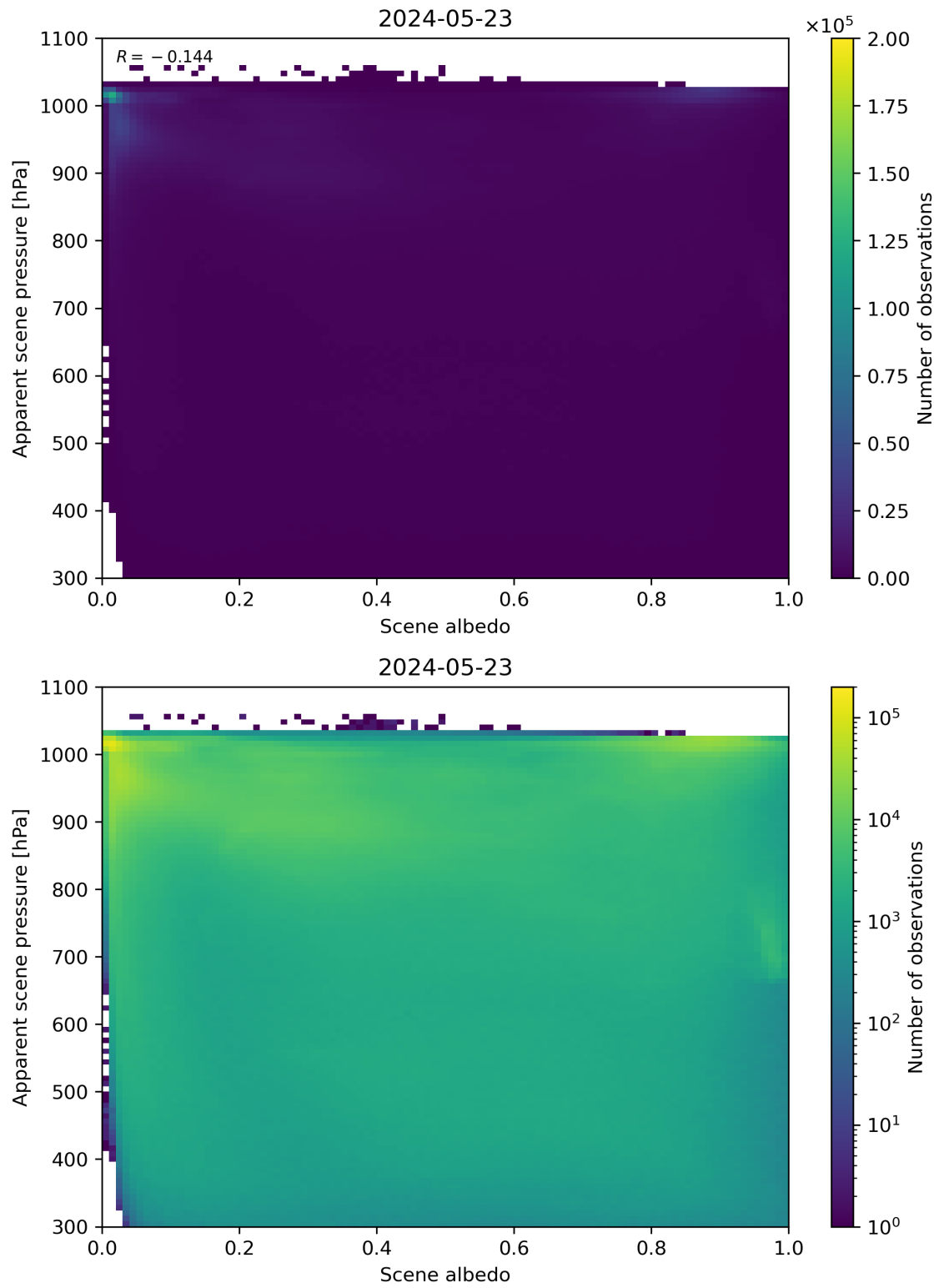
Figure 102: Scatter density plot of “Scene albedo” against “Apparent scene pressure” for 2024-05-23 to 2024-05-24.
