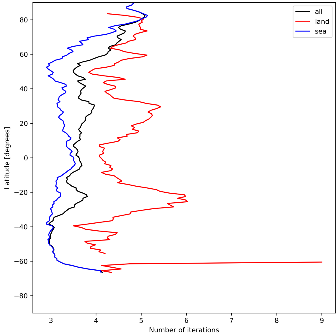
Figure 22: Zonal average of “Number of iterations” for 2024-05-23 to 2024-05-24.
