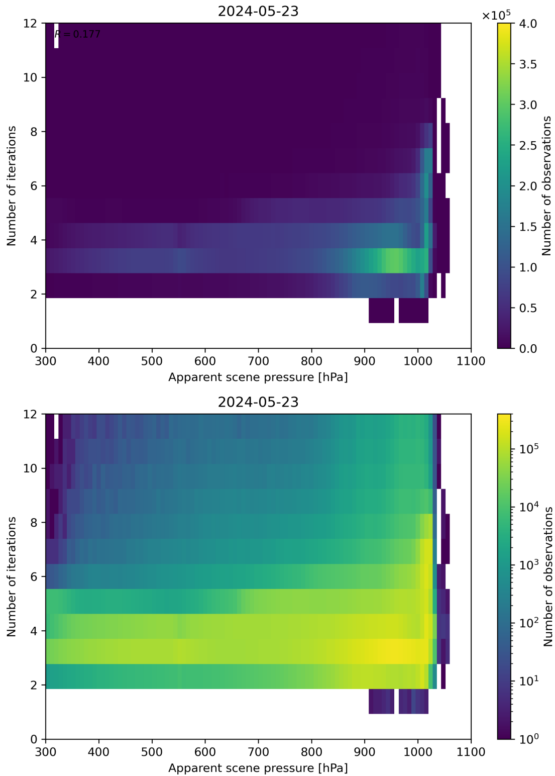
Figure 65: Scatter density plot of “Apparent scene pressure” against “Number of iterations” for 2024-05-23 to 2024-05-24.
