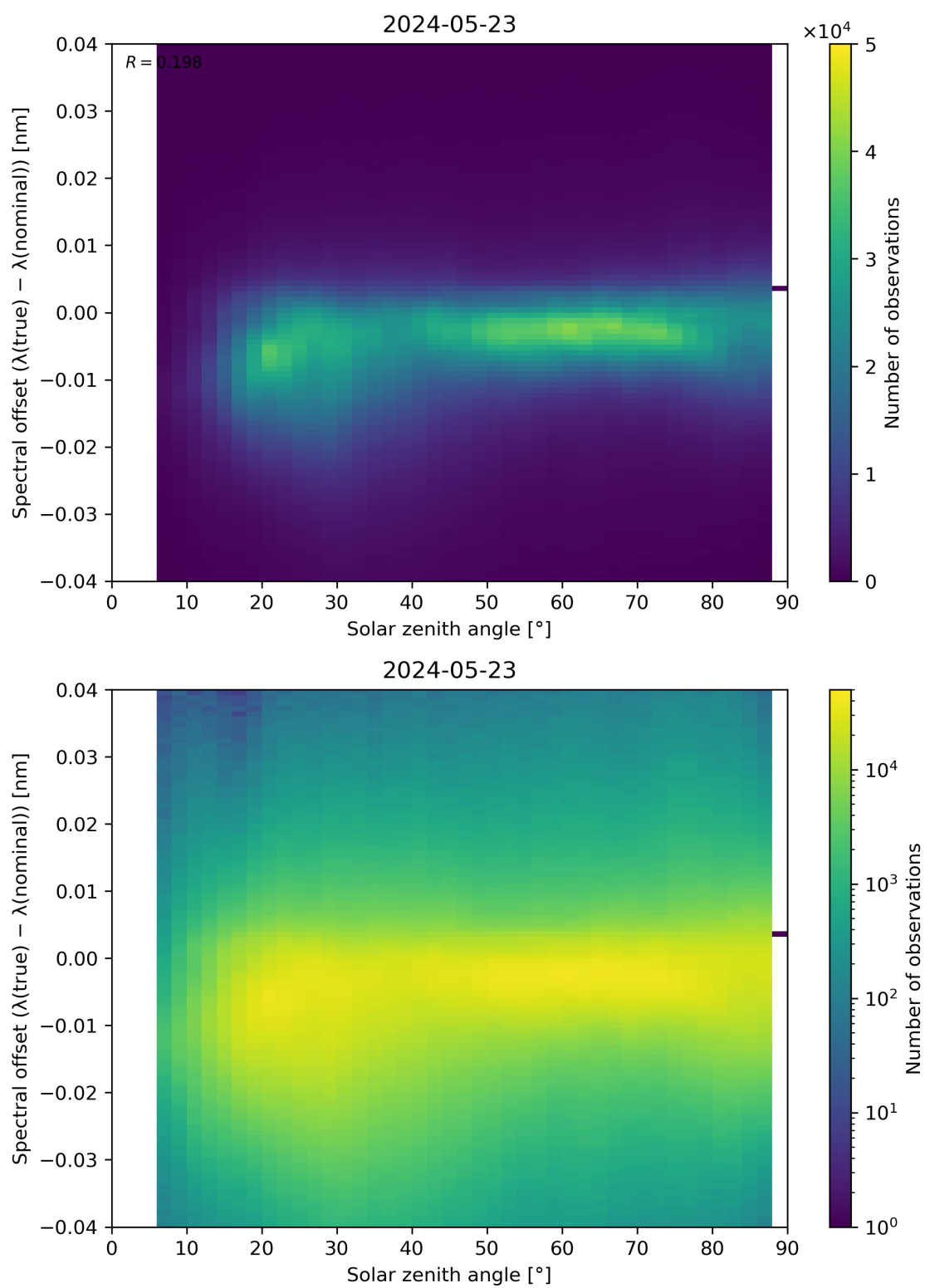
Figure 117: Scatter density plot of “Solar zenith angle” against “Spectral offset ( \lambda(\text{true}) - \lambda(\text{nominal}) )” for 2024-05-23 to 2024-05-24.
