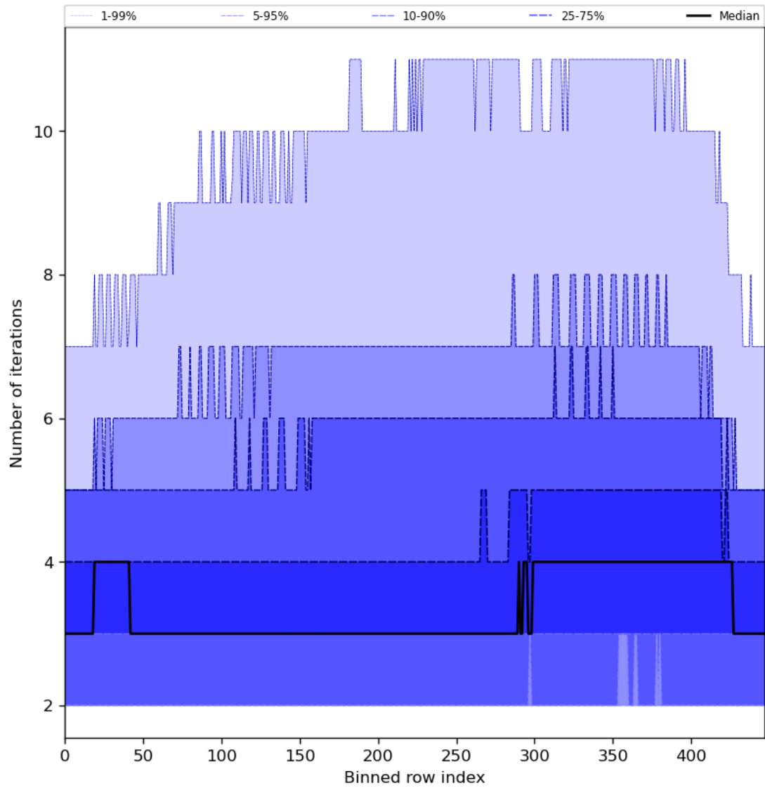
Figure 56: Along track statistics of “Number of iterations” for 2024-05-23 to 2024-05-24
