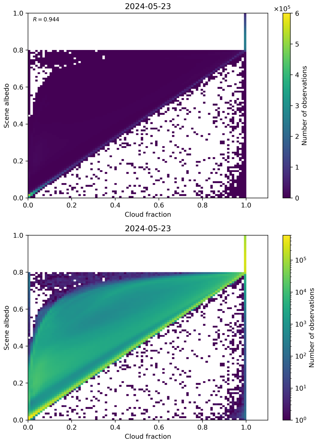
Figure 75: Scatter density plot of “Cloud fraction” against “Scene albedo” for 2024-05-23 to 2024-05-24.
