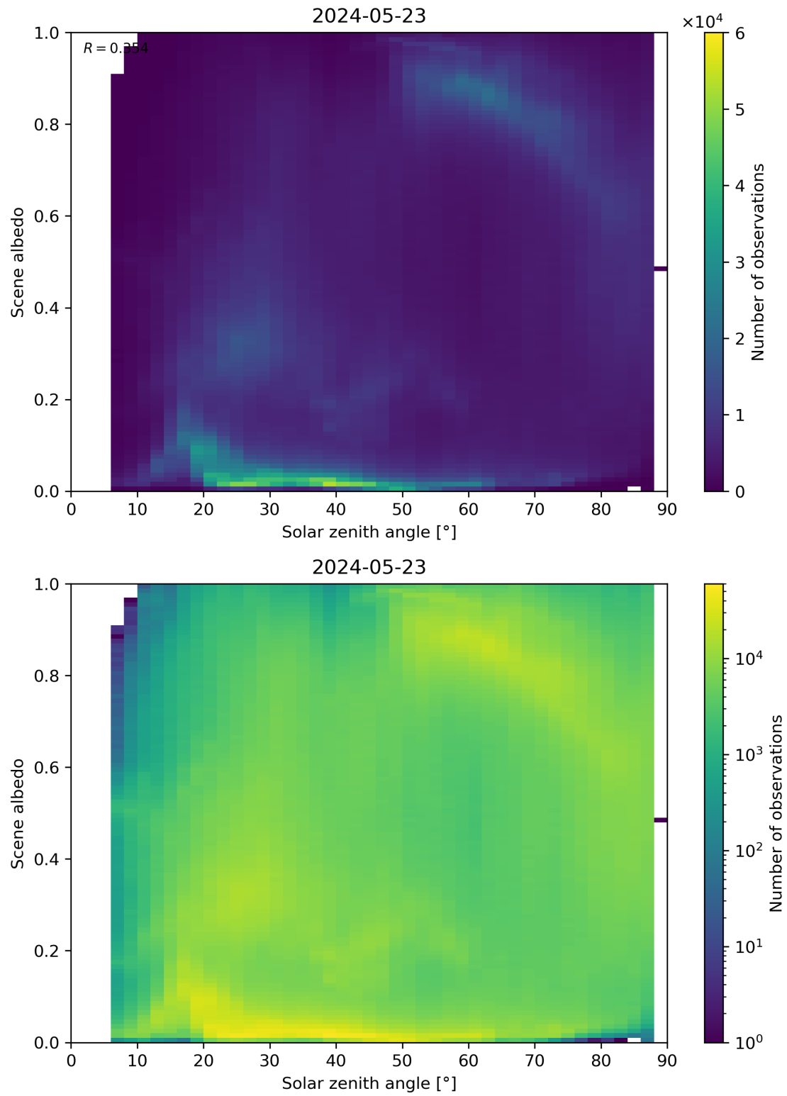
Figure 116: Scatter density plot of “Solar zenith angle” against “Scene albedo” for 2024-05-23 to 2024-05-24.
