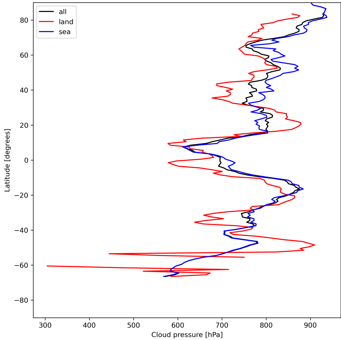
Figure 13: Zonal average of “Cloud pressure” for 2024-05-23 to 2024-05-24.
