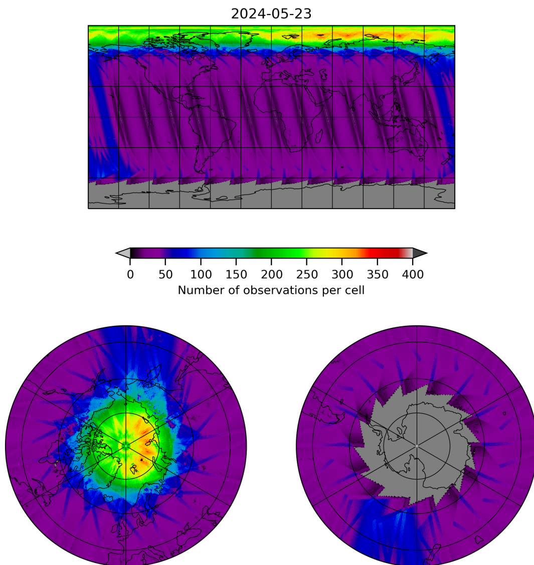
Figure 11: Map of the number of observations for 2024-05-23 to 2024-05-24
