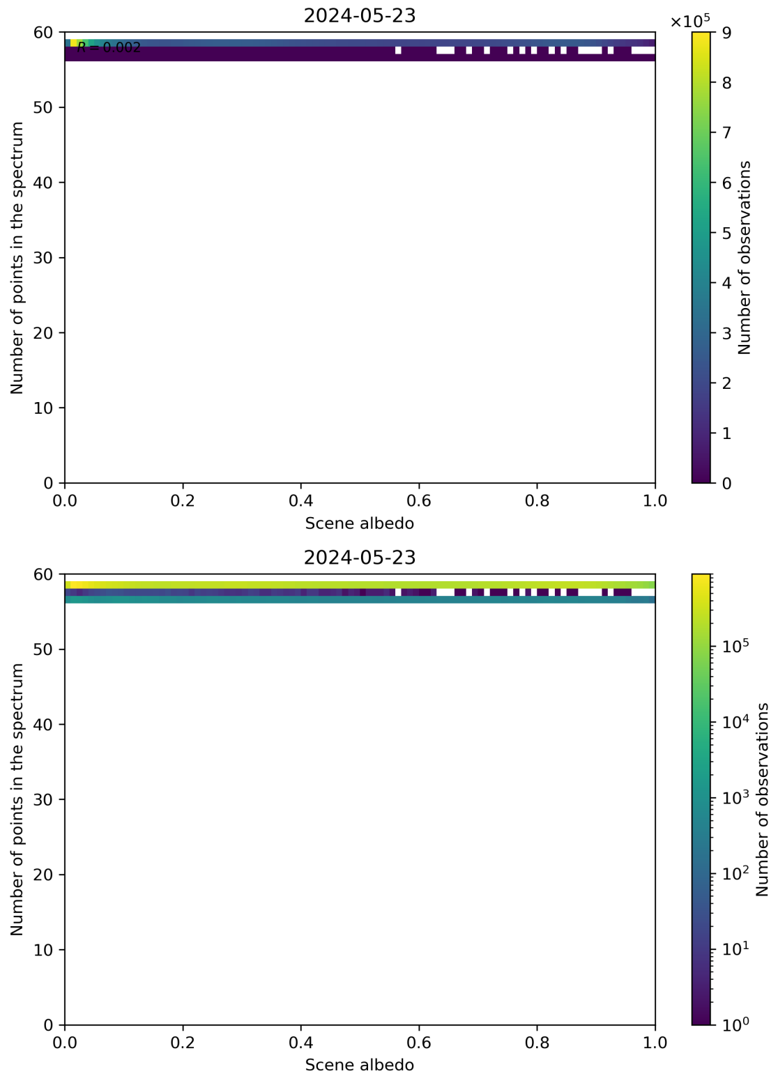
Figure 106: Scatter density plot of “Scene albedo” against “Number of points in the spectrum” for 2024-05-23 to 2024-05-24.
