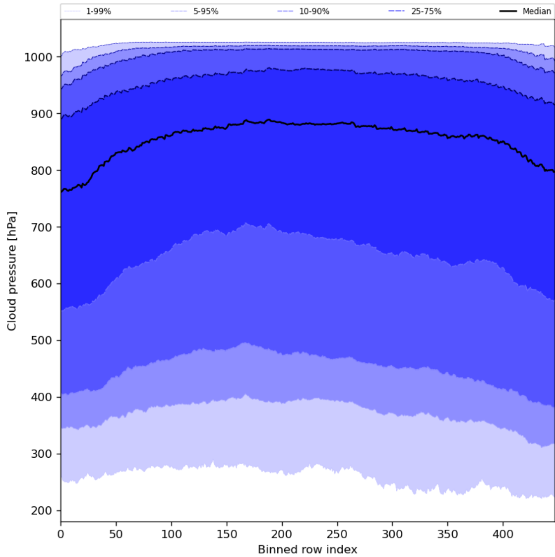
Figure 47: Along track statistics of “Cloud pressure” for 2024-05-23 to 2024-05-24
