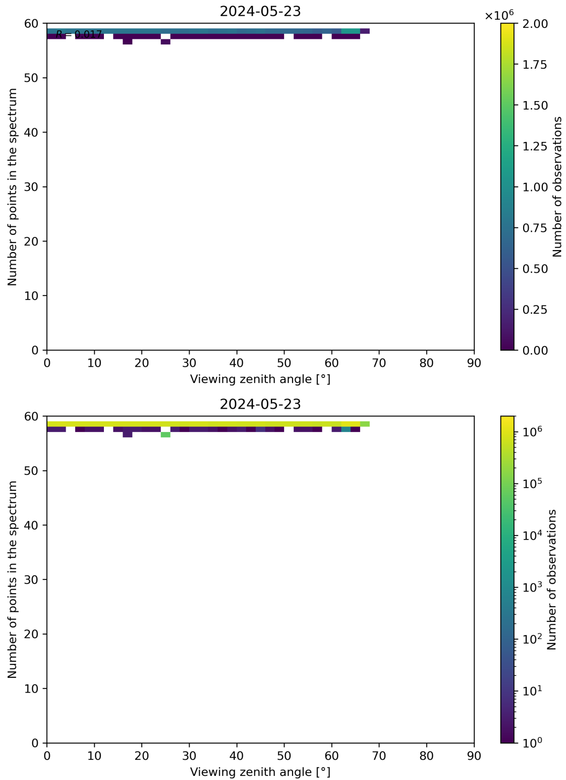
Figure 125: Scatter density plot of “Viewing zenith angle” against “Number of points in the spectrum” for 2024-05-23 to 2024-05-24.
