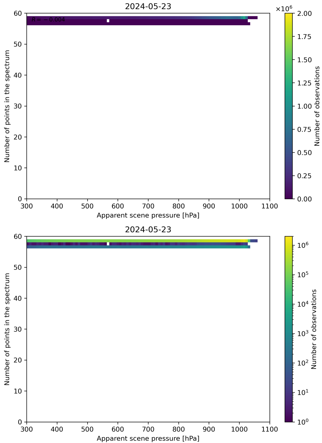
Figure 66: Scatter density plot of “Apparent scene pressure” against “Number of points in the spectrum” for 2024-05-23 to 2024-05-24.
