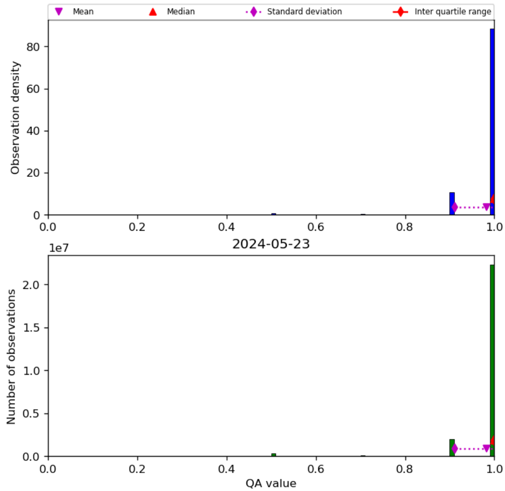
Figure 29: Histogram of “QA value” for 2024-05-23 to 2024-05-24
