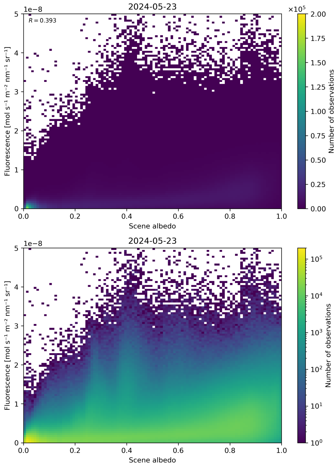
Figure 104: Scatter density plot of “Scene albedo” against “Fluorescence” for 2024-05-23 to 2024-05-24.
