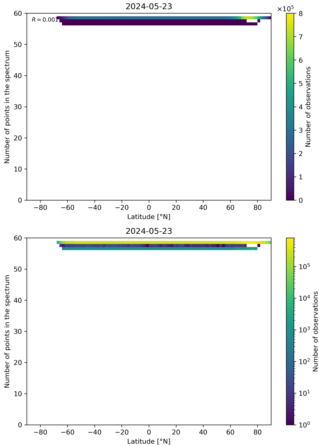
Figure 94: Scatter density plot of “Latitude” against “Number of points in the spectrum” for 2024-05-23 to 2024-05-24.
