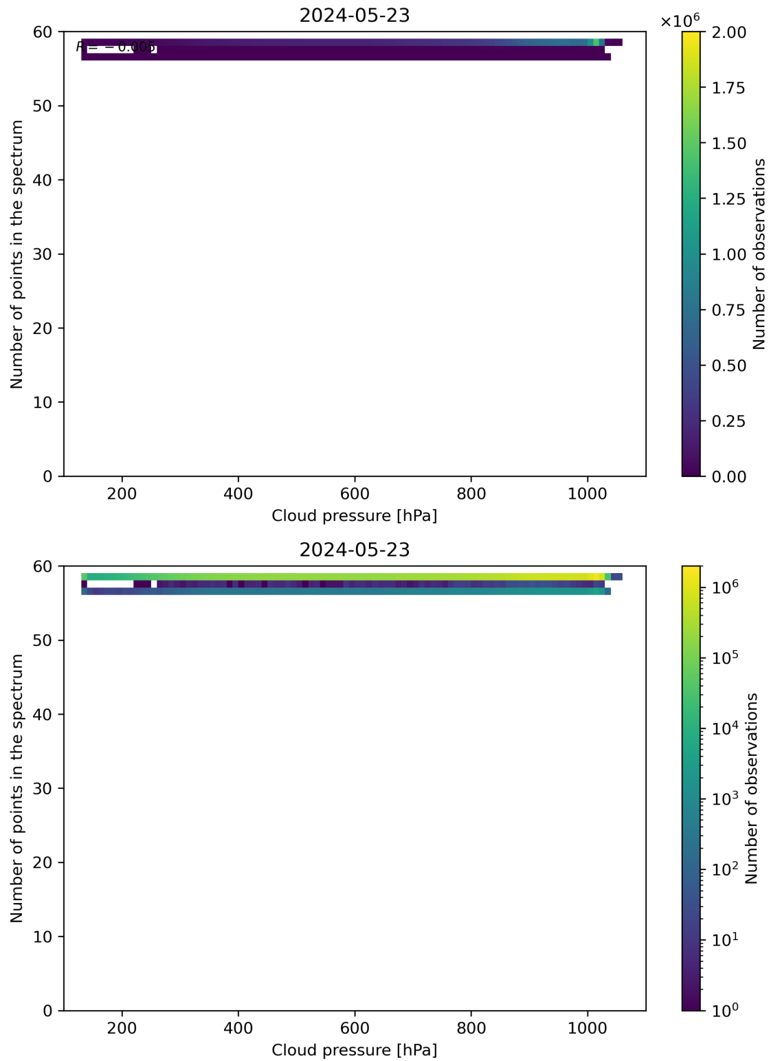
Figure 82: Scatter density plot of “Cloud pressure” against “Number of points in the spectrum” for 2024-05-23 to 2024-05-24.
