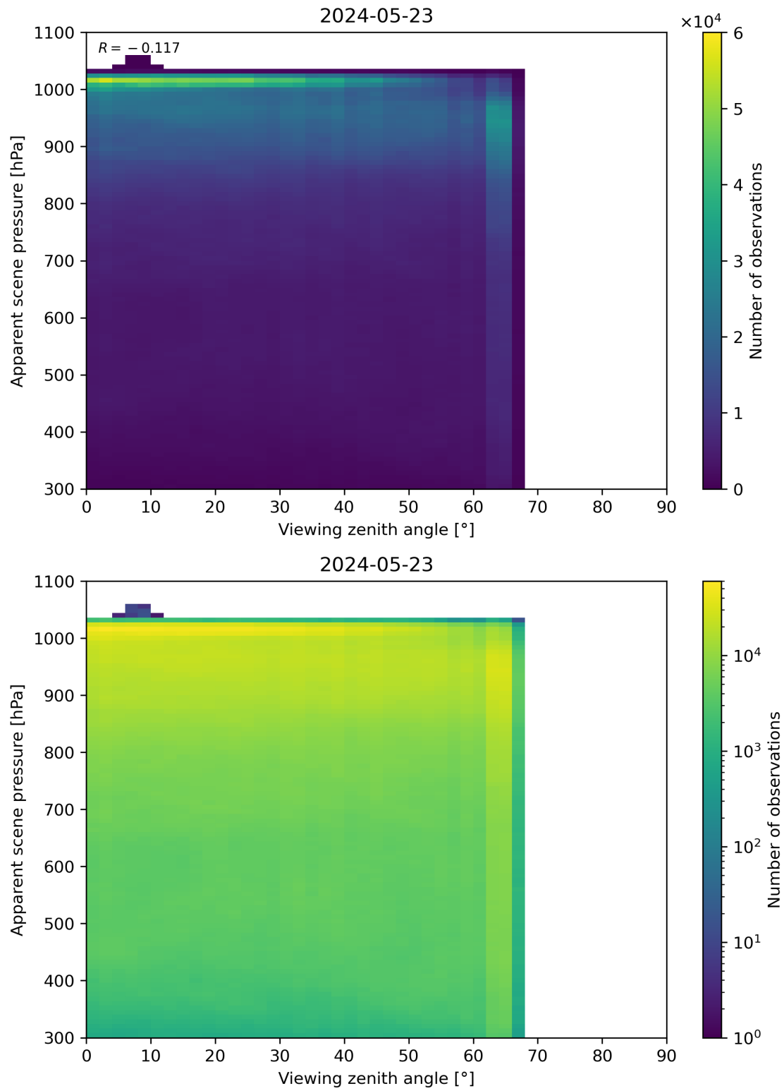
Figure 118: Scatter density plot of “Viewing zenith angle” against “Apparent scene pressure” for 2024-05-23 to 2024-05-24.
