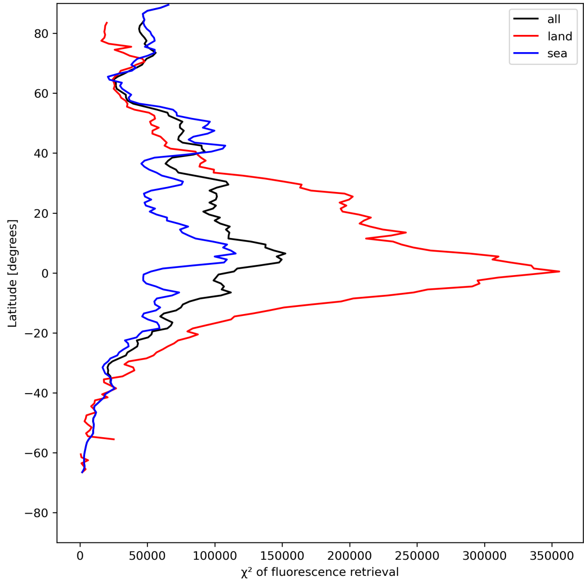
Figure 25: Zonal average of “ \chi^2 of fluorescence retrieval” for 2024-05-23 to 2024-05-24.
