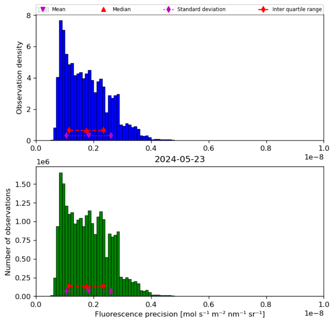
Figure 41: Histogram of “Fluorescence precision” for 2024-05-23 to 2024-05-24
