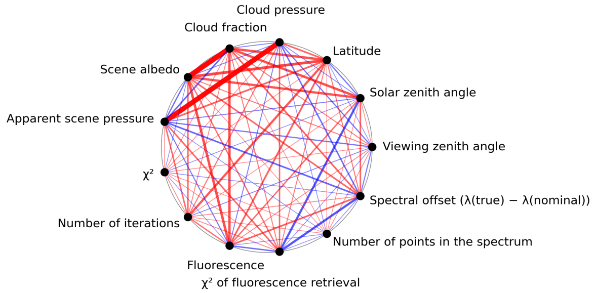
Figure 1: Map of correlation graph for 2024-05-23 to 2024-05-24.
