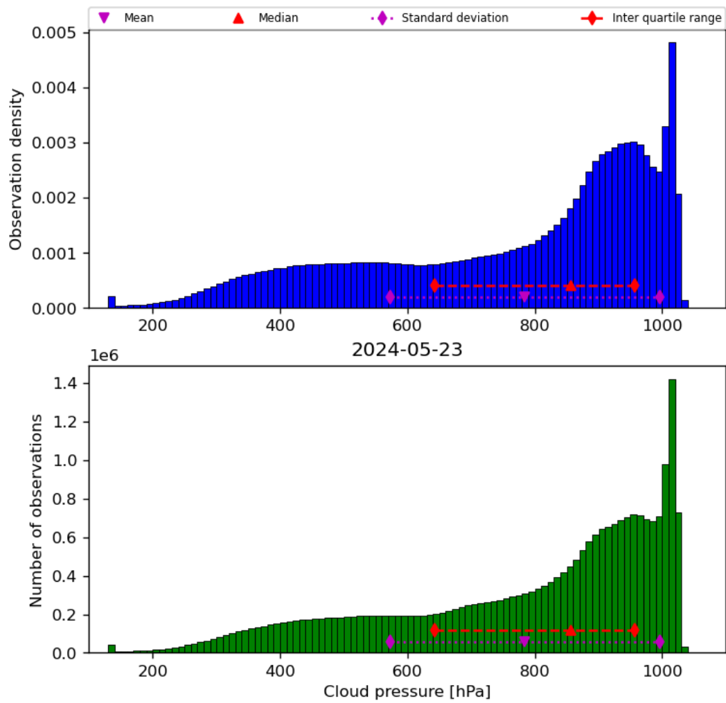
Figure 30: Histogram of “Cloud pressure” for 2024-05-23 to 2024-05-24
