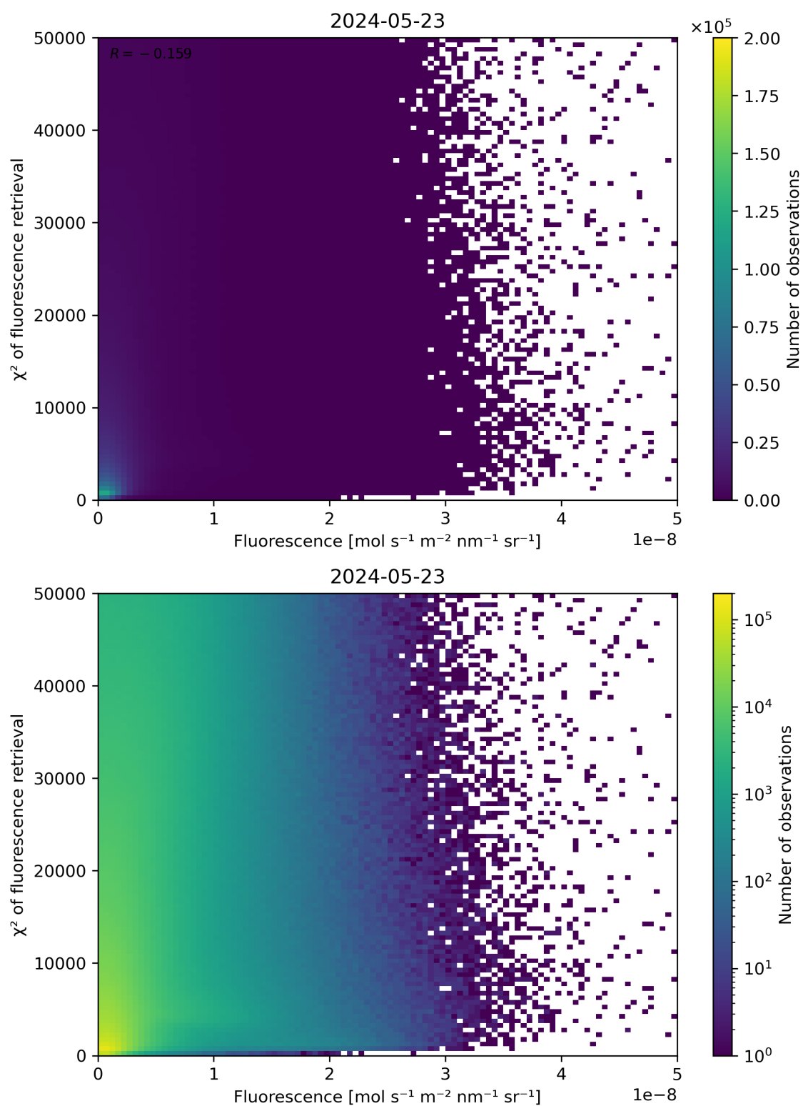
Figure 85: Scatter density plot of “Fluorescence” against “ \chi^2 of fluorescence retrieval” for 2024-05-23 to 2024-05-24.
