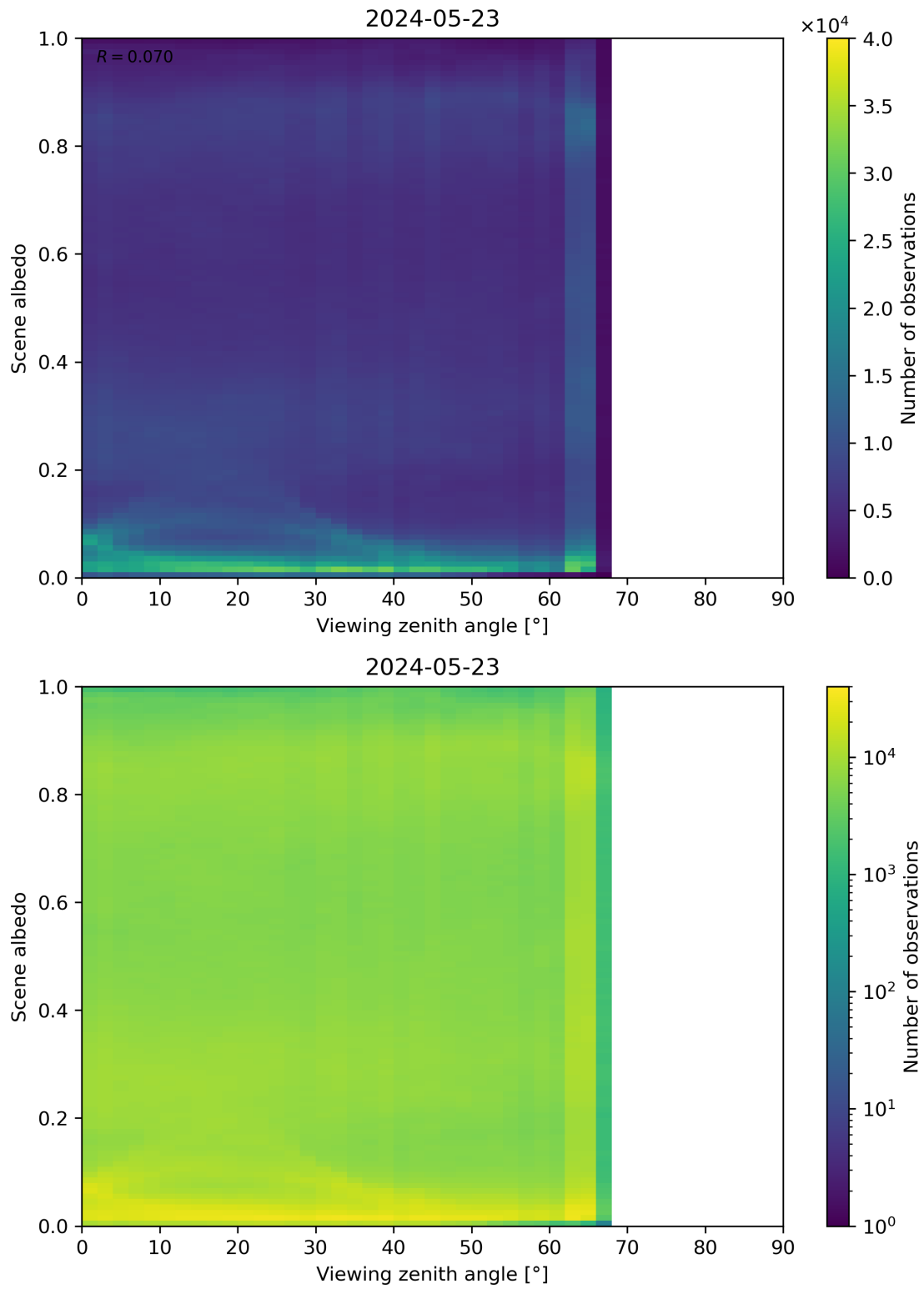
Figure 126: Scatter density plot of “Viewing zenith angle” against “Scene albedo” for 2024-05-23 to 2024-05-24.
