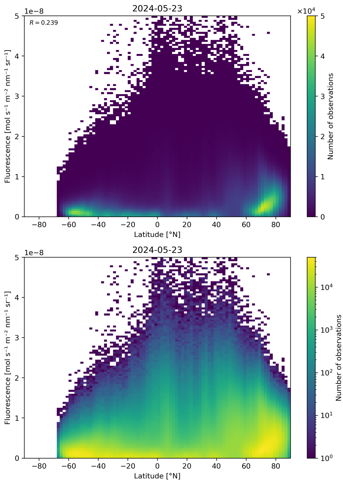
Figure 92: Scatter density plot of “Latitude” against “Fluorescence” for 2024-05-23 to 2024-05-24.
