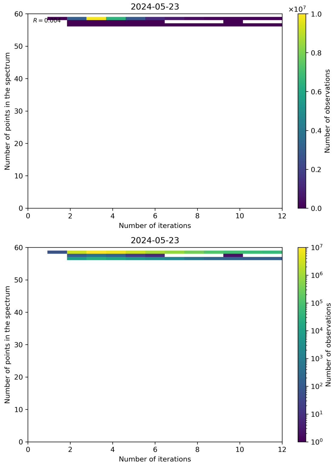
Figure 99: Scatter density plot of “Number of iterations” against “Number of points in the spectrum” for 2024-05-23 to 2024-05-24.
