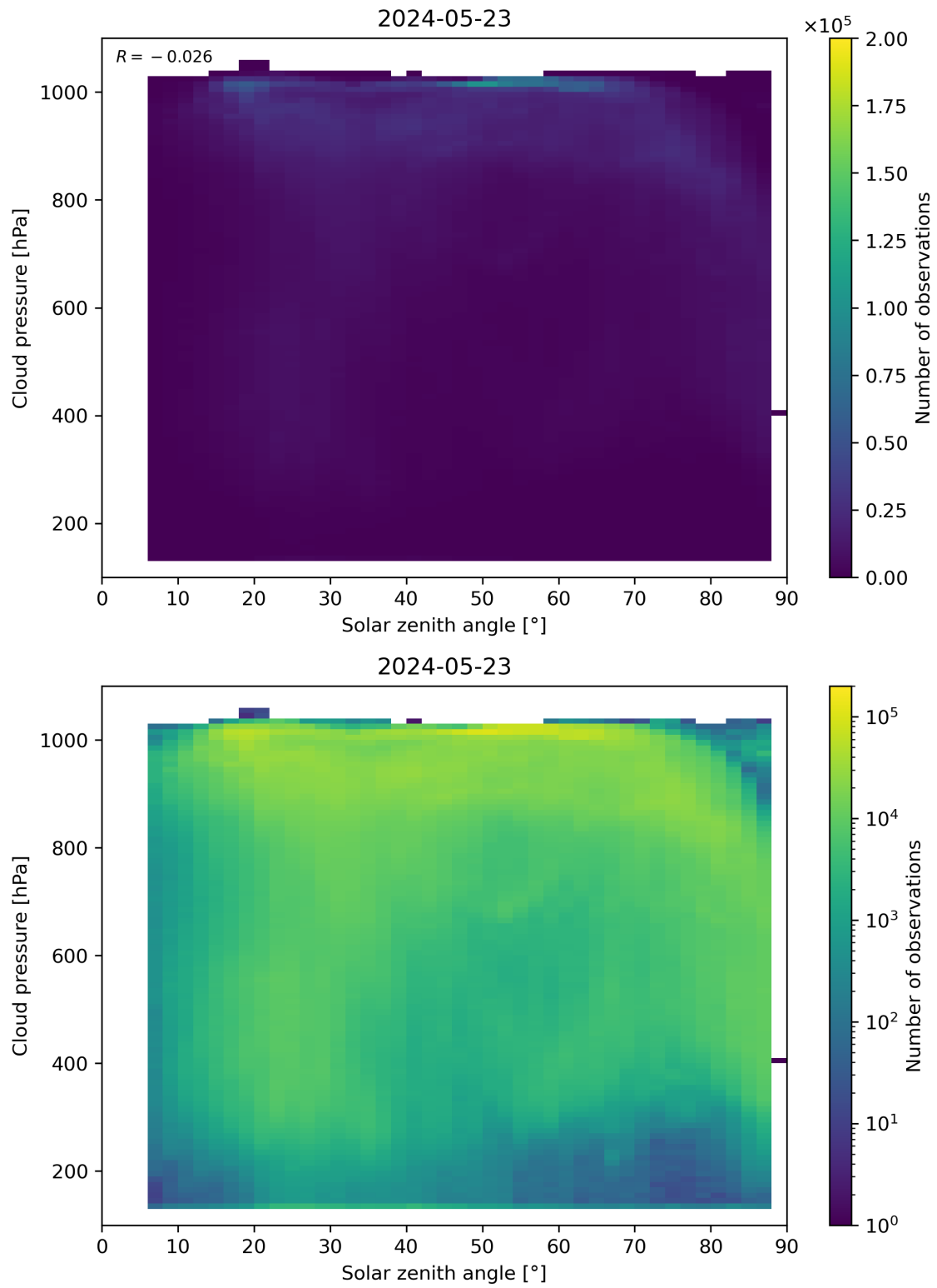
Figure 111: Scatter density plot of “Solar zenith angle” against “Cloud pressure” for 2024-05-23 to 2024-05-24.
