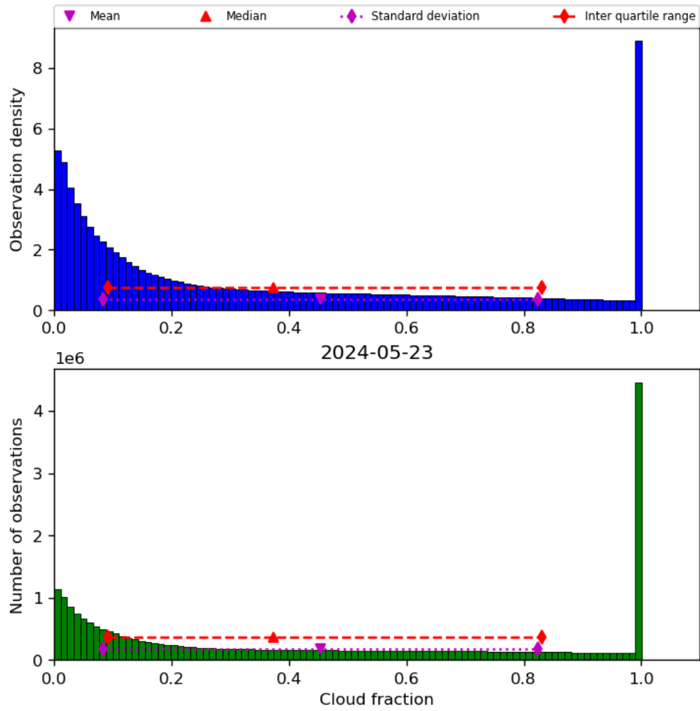
Figure 32: Histogram of “Cloud fraction” for 2024-05-23 to 2024-05-24
