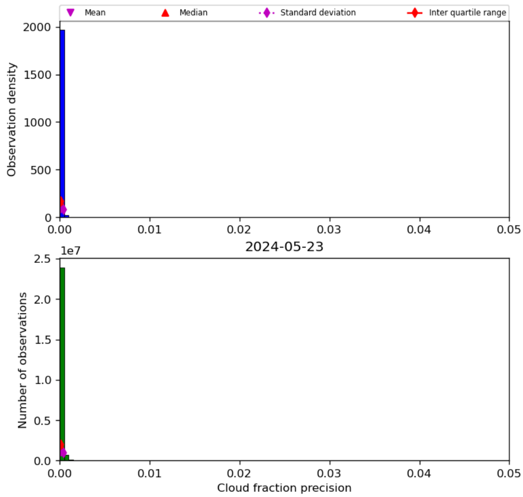
Figure 33: Histogram of “Cloud fraction precision” for 2024-05-23 to 2024-05-24
