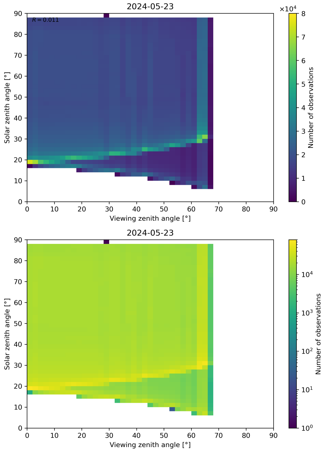
Figure 127: Scatter density plot of “Viewing zenith angle” against “Solar zenith angle” for 2024-05-23 to 2024-05-24.
