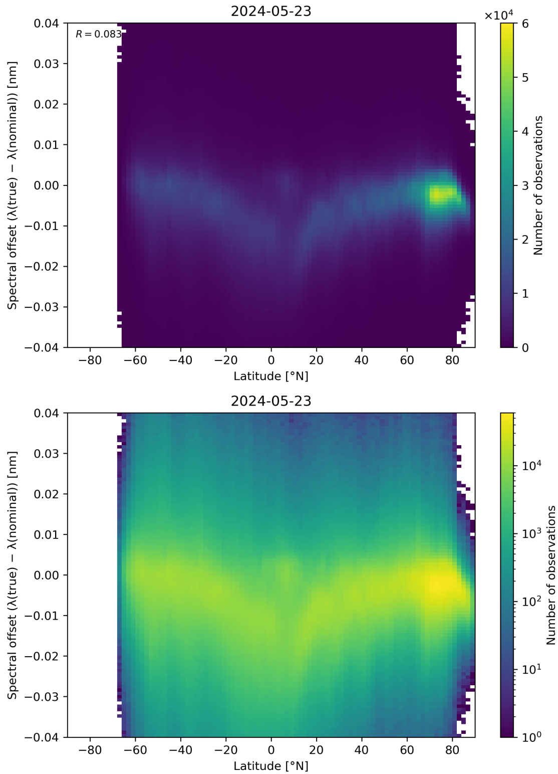
Figure 96: Scatter density plot of “Latitude” against “Spectral offset ( \lambda(\text{true}) - \lambda(\text{nominal}) )” for 2024-05-23 to 2024-05-24.
