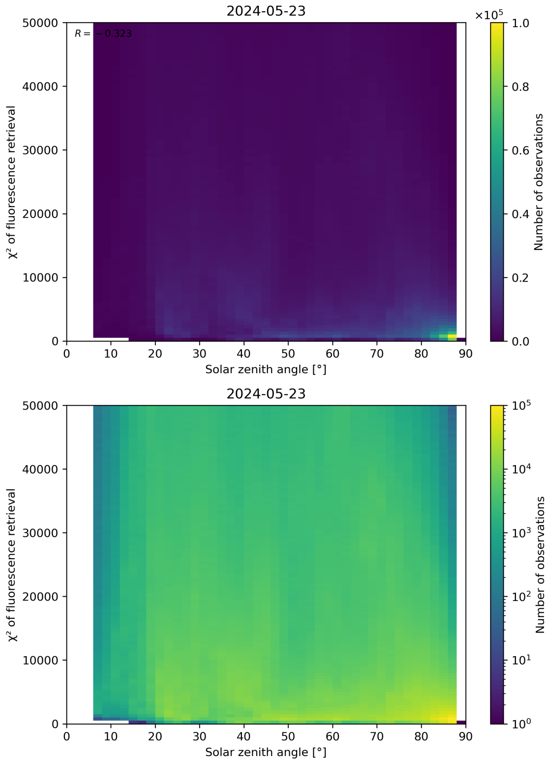
Figure 109: Scatter density plot of “Solar zenith angle” against “ \chi^2 of fluorescence retrieval” for 2024-05-23 to 2024-05-24.
