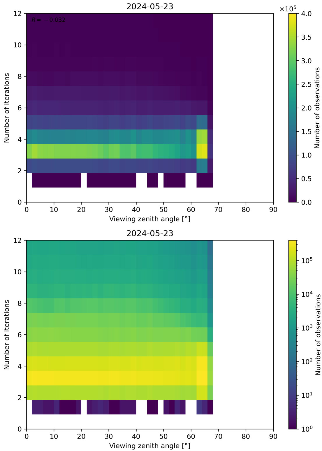
Figure 124: Scatter density plot of “Viewing zenith angle” against “Number of iterations” for 2024-05-23 to 2024-05-24.
