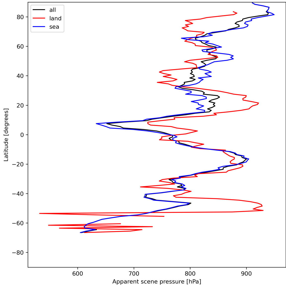
Figure 19: Zonal average of “Apparent scene pressure” for 2024-05-23 to 2024-05-24.
