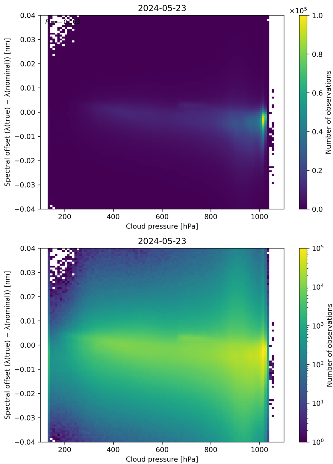
Figure 84: Scatter density plot of “Cloud pressure” against “Spectral offset ( \lambda(\text{true}) - \lambda(\text{nominal}) )” for 2024-05-23 to 2024-05-24.
