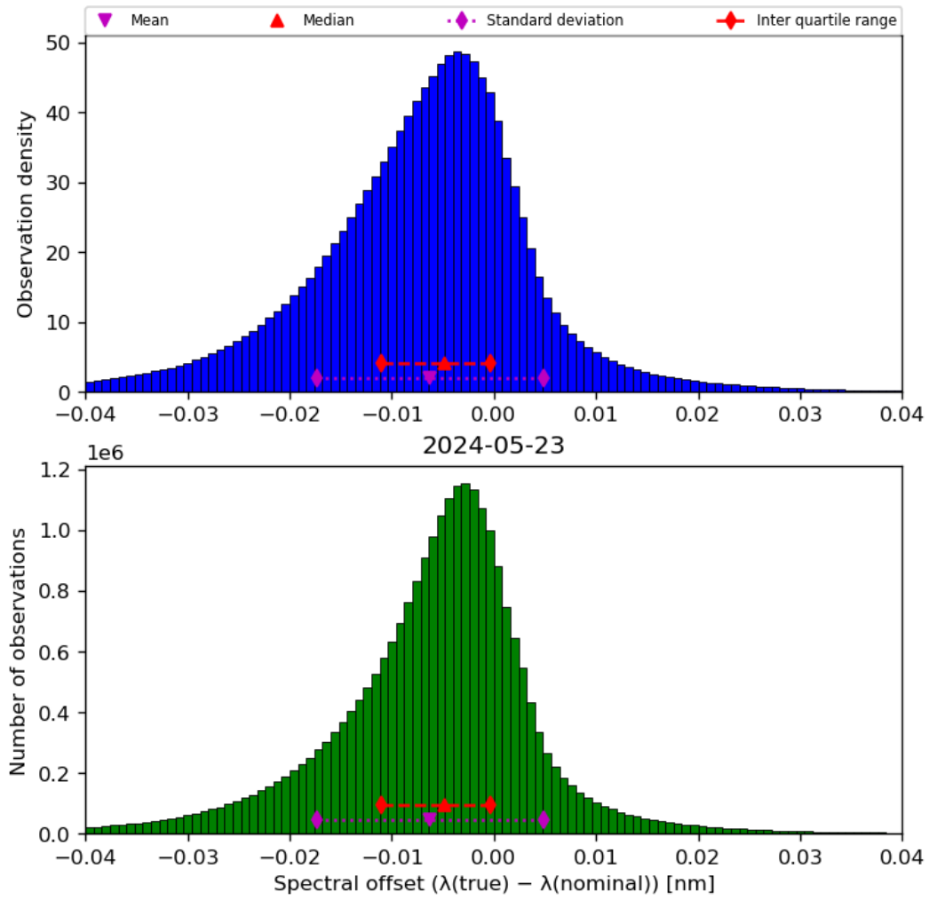
Figure 45: Histogram of “Spectral offset ( \lambda(\text{true}) - \lambda(\text{nominal}) )” for 2024-05-23 to 2024-05-24
