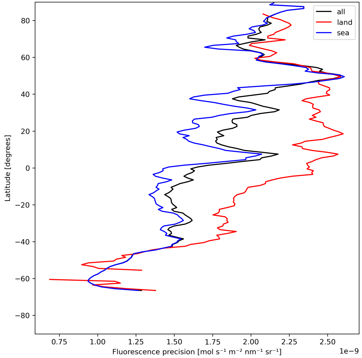
Figure 24: Zonal average of “Fluorescence precision” for 2024-05-23 to 2024-05-24.
