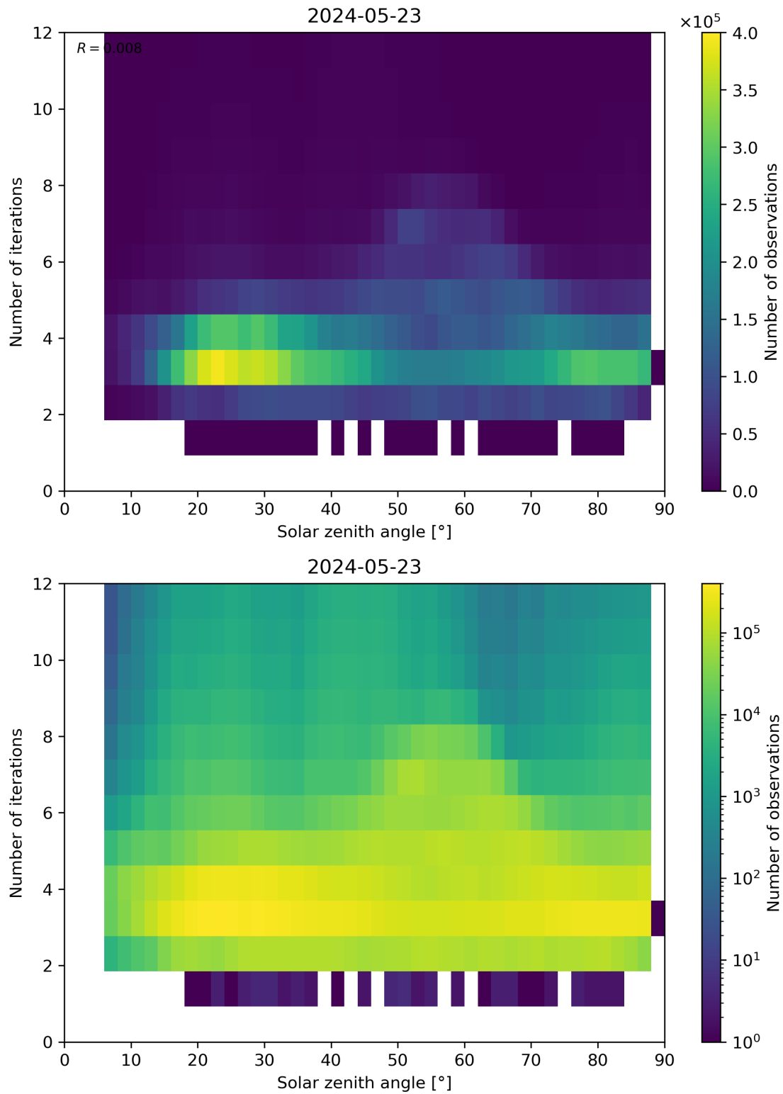
Figure 114: Scatter density plot of “Solar zenith angle” against “Number of iterations” for 2024-05-23 to 2024-05-24.
