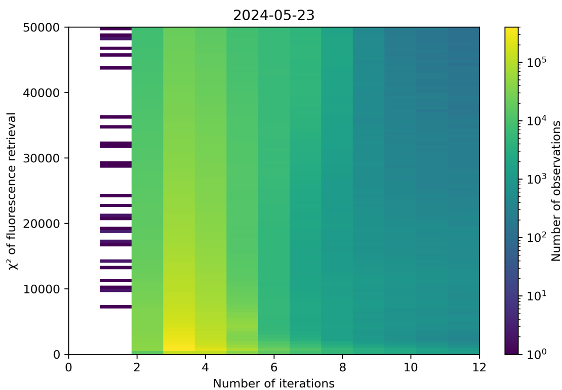
Figure 97: Scatter density plot of “Number of iterations” against “ \chi^2 of fluorescence retrieval” for 2024-05-23 to 2024-05-24.
