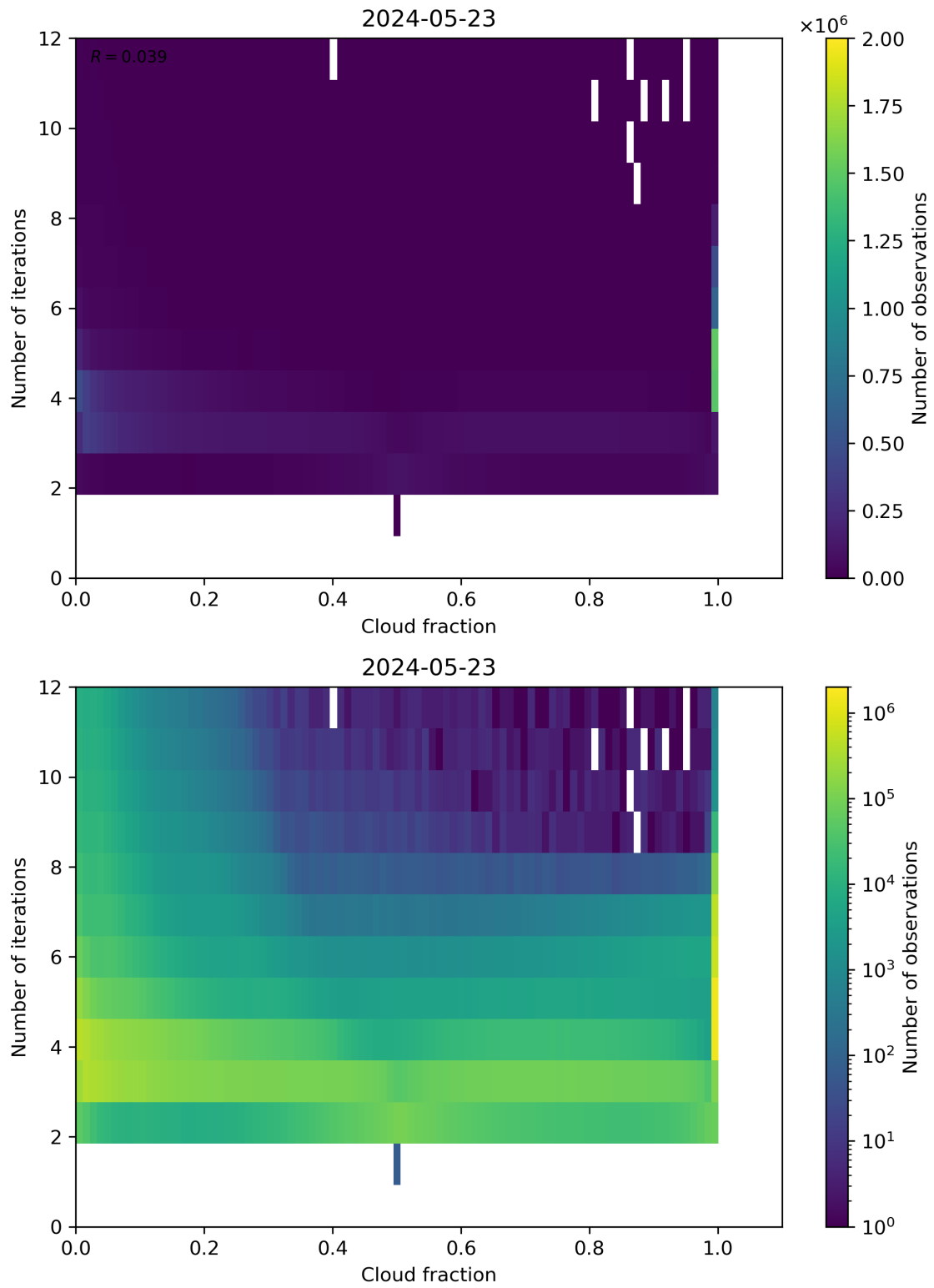
Figure 73: Scatter density plot of “Cloud fraction” against “Number of iterations” for 2024-05-23 to 2024-05-24.
