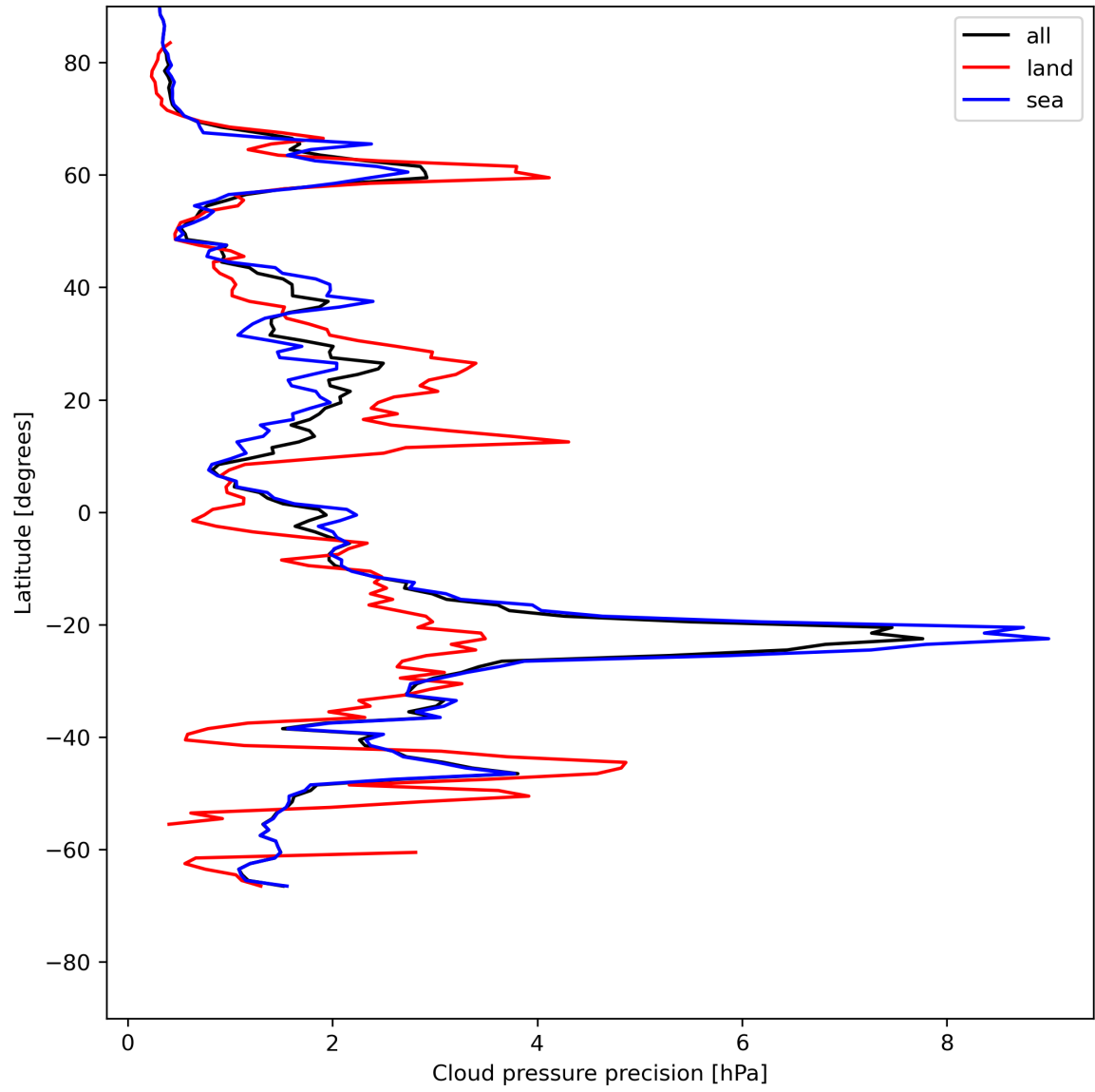
Figure 14: Zonal average of “Cloud pressure precision” for 2024-05-23 to 2024-05-24.
