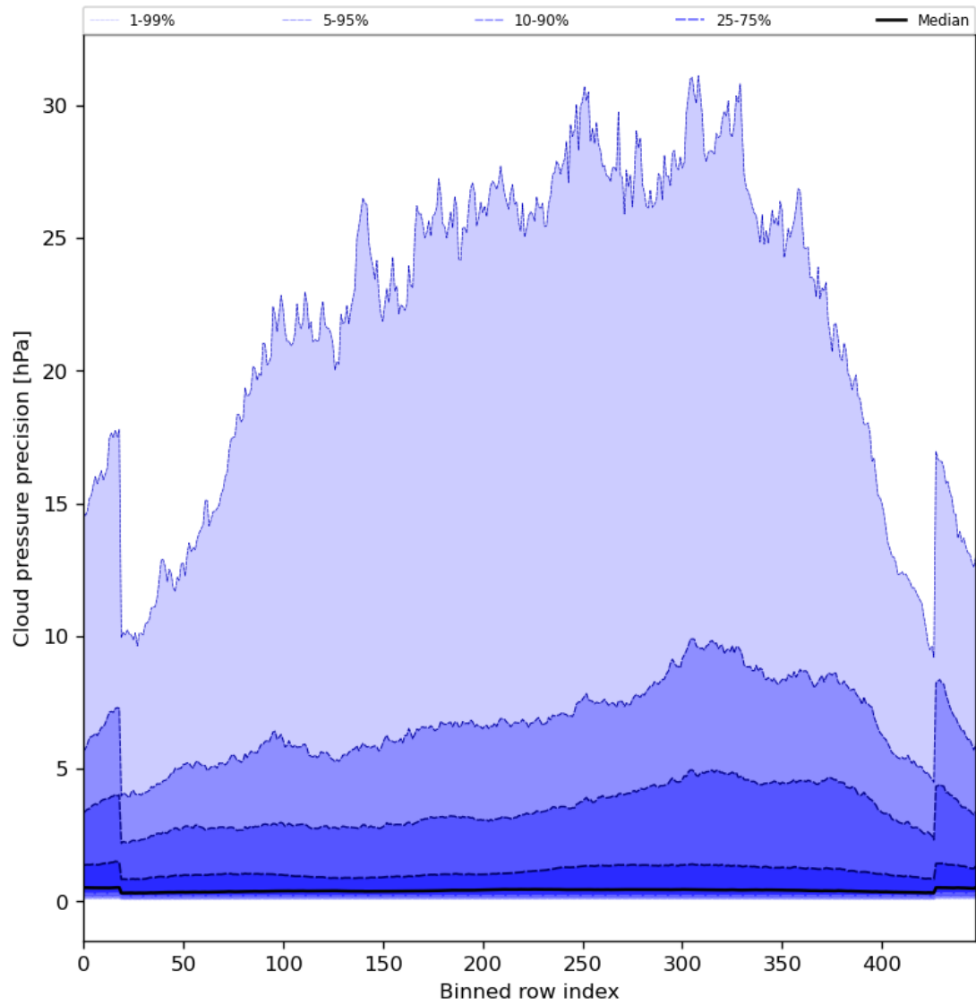
Figure 48: Along track statistics of “Cloud pressure precision” for 2024-05-23 to 2024-05-24
