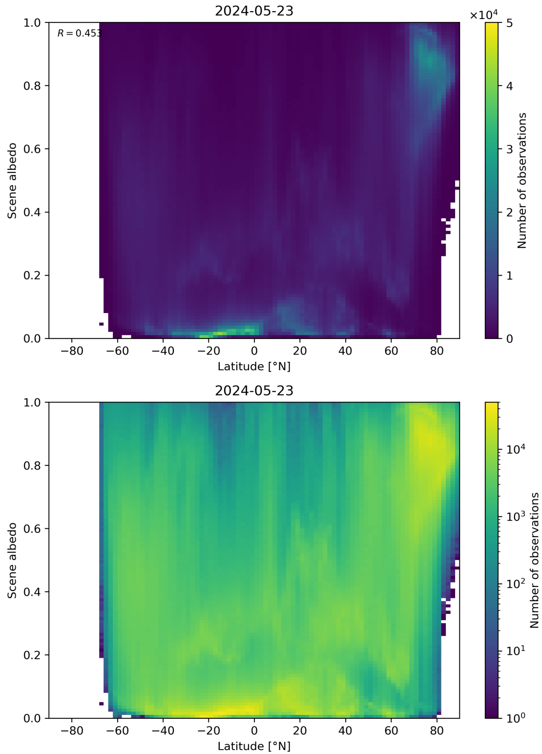
Figure 95: Scatter density plot of “Latitude” against “Scene albedo” for 2024-05-23 to 2024-05-24.
