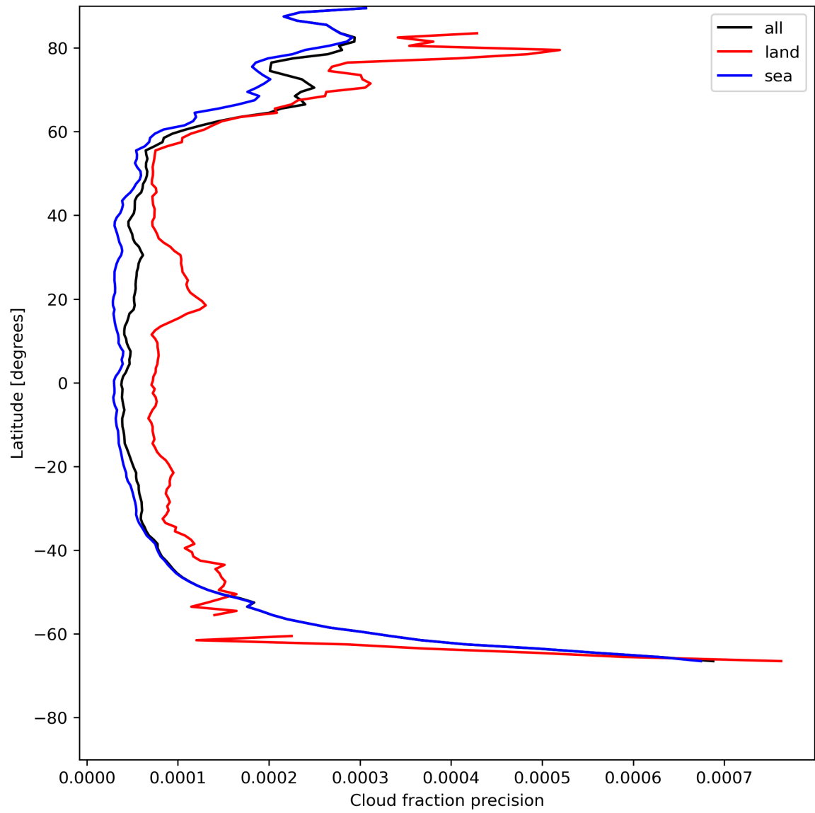
Figure 16: Zonal average of “Cloud fraction precision” for 2024-05-23 to 2024-05-24.
