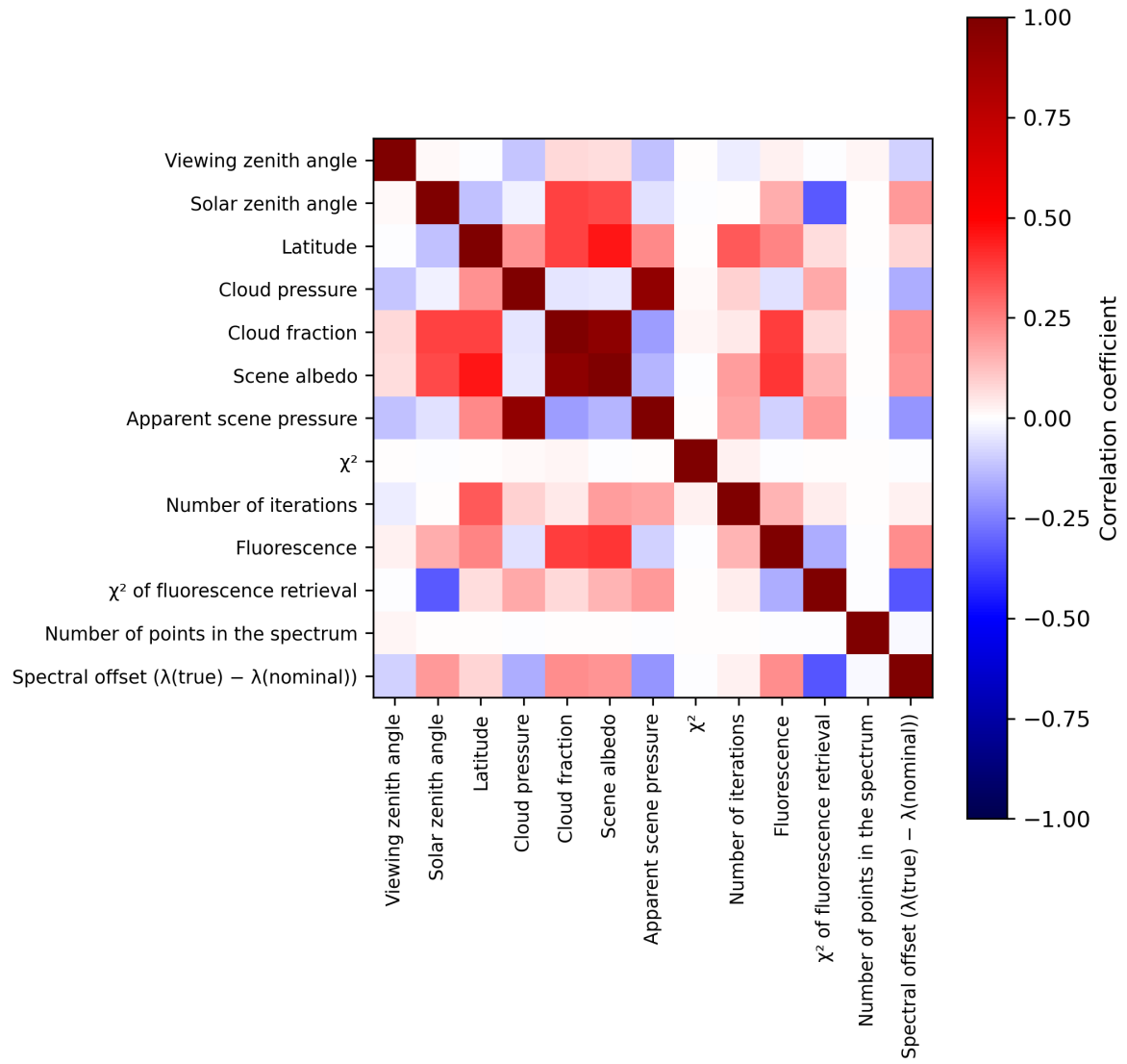
Figure 2: Map of correlation matrix for 2024-05-23 to 2024-05-24.
