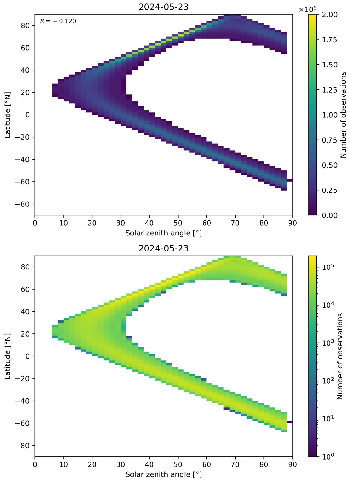
Figure 113: Scatter density plot of “Solar zenith angle” against “Latitude” for 2024-05-23 to 2024-05-24.
