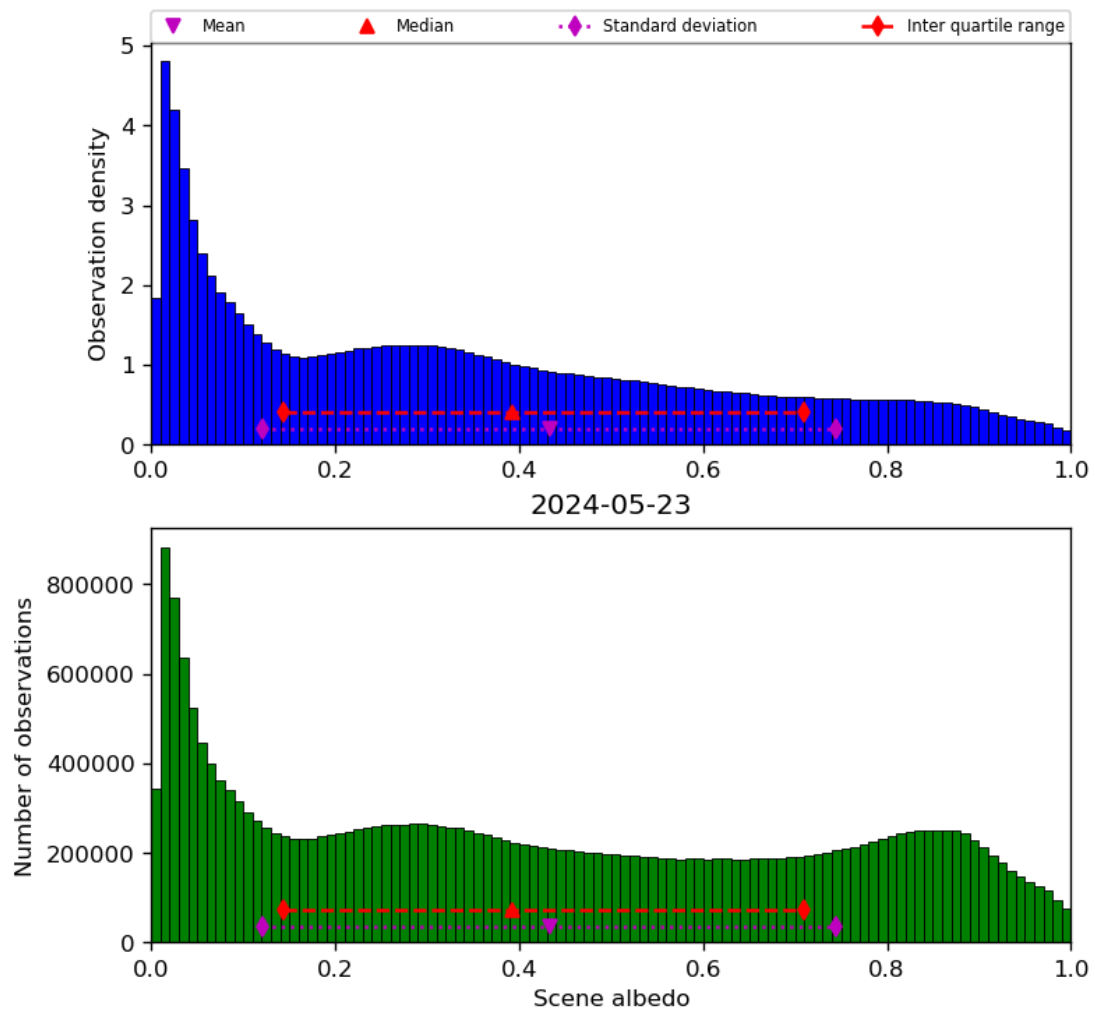
Figure 34: Histogram of “Scene albedo” for 2024-05-23 to 2024-05-24
