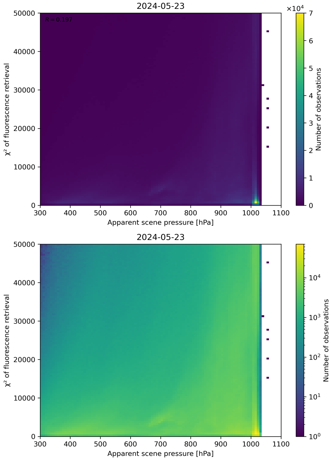
Figure 63: Scatter density plot of “Apparent scene pressure” against “ \chi^2 of fluorescence retrieval” for 2024-05-23 to 2024-05-24.
