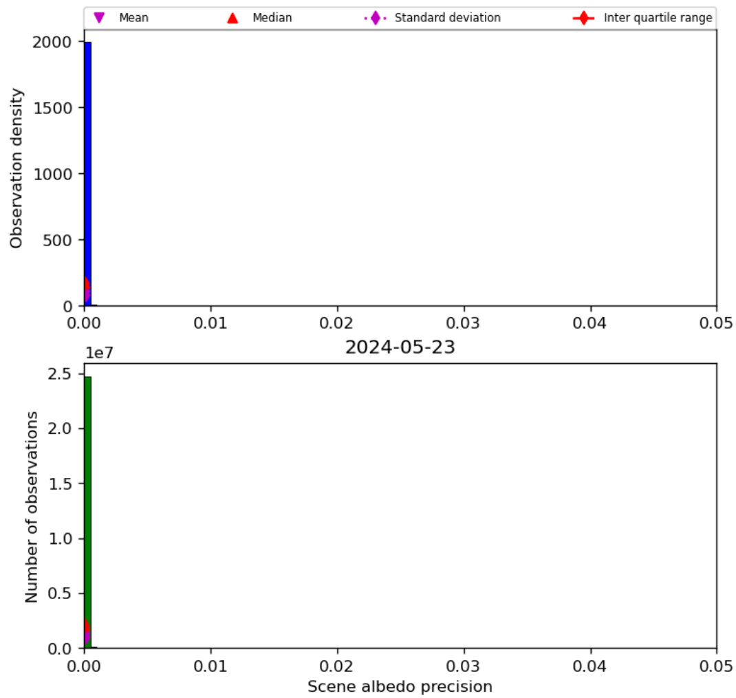
Figure 35: Histogram of “Scene albedo precision” for 2024-05-23 to 2024-05-24
