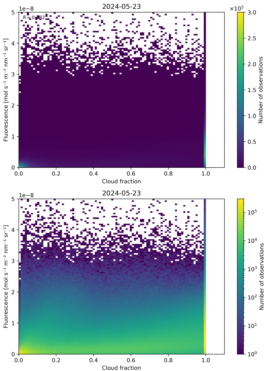
Figure 72: Scatter density plot of “Cloud fraction” against “Fluorescence” for 2024-05-23 to 2024-05-24.
