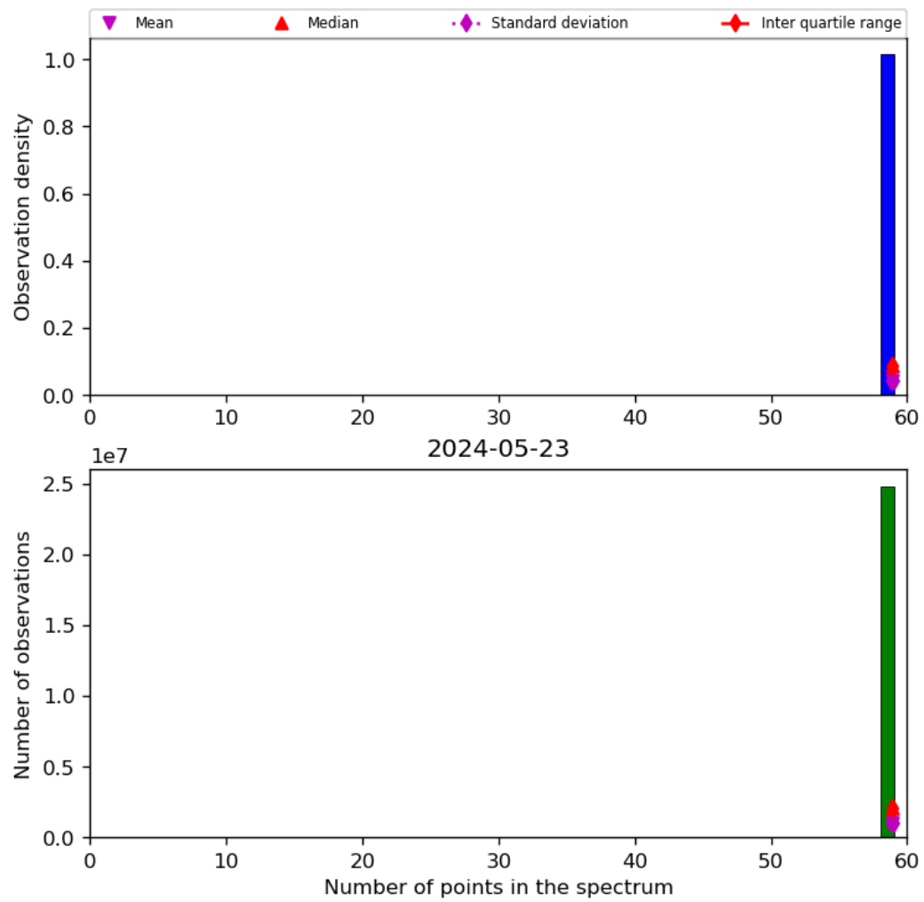
Figure 44: Histogram of “Number of points in the spectrum” for 2024-05-23 to 2024-05-24
