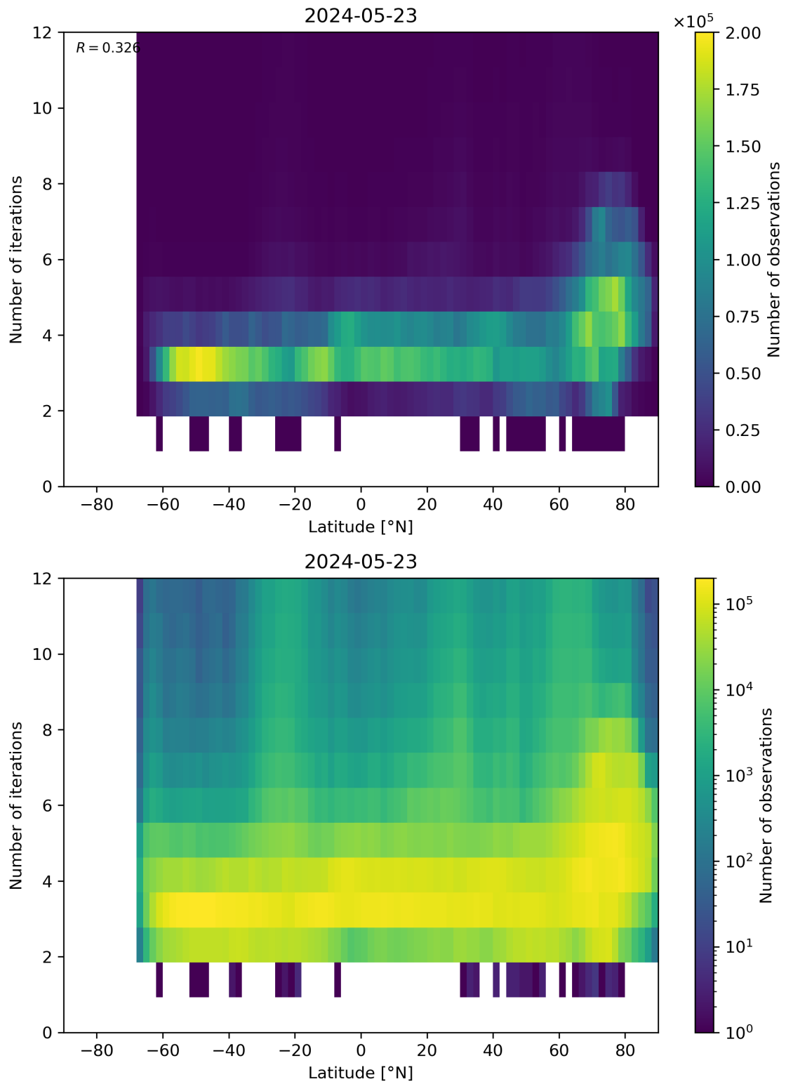
Figure 93: Scatter density plot of “Latitude” against “Number of iterations” for 2024-05-23 to 2024-05-24.
