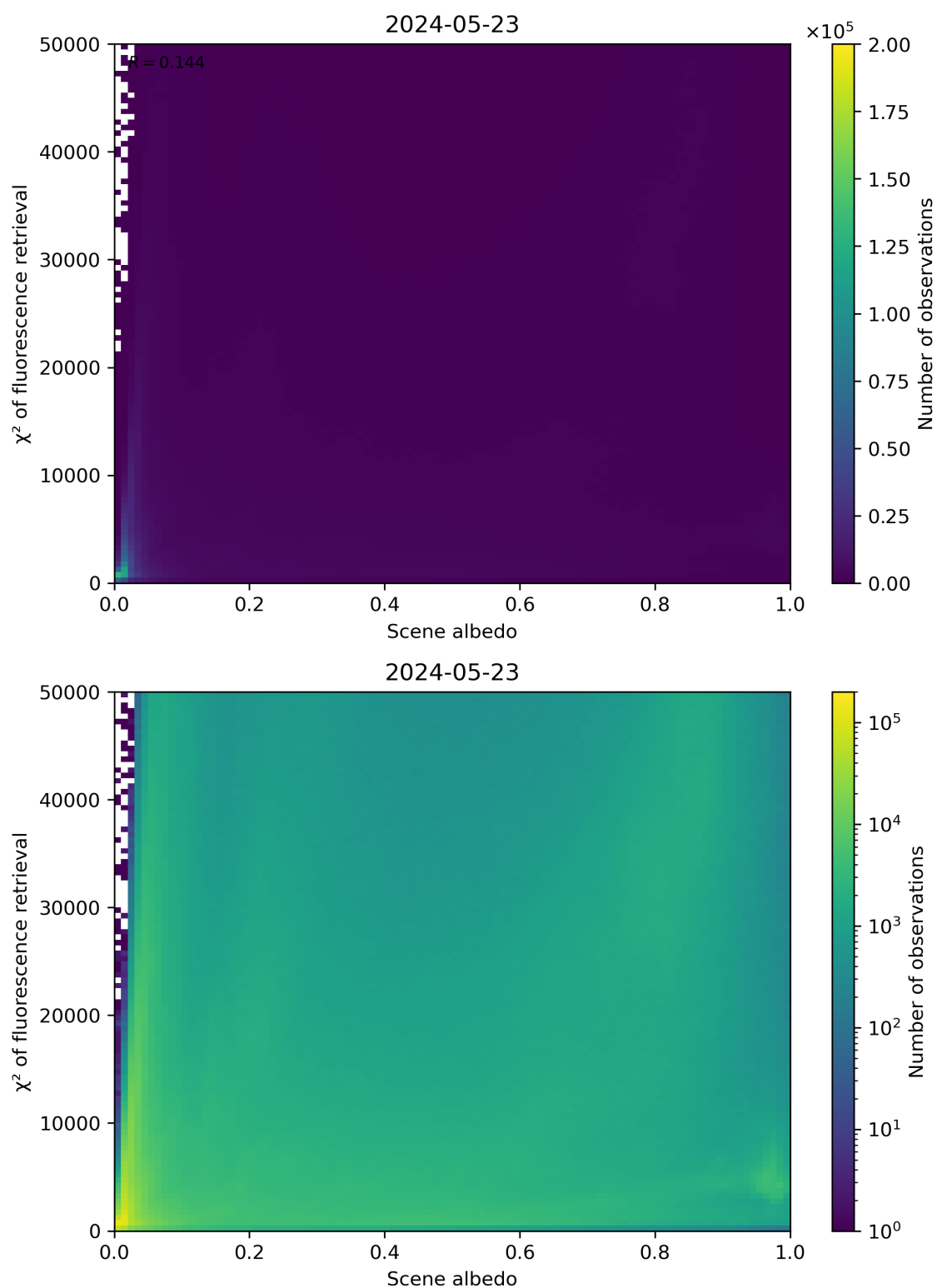
Figure 103: Scatter density plot of “Scene albedo” against “ \chi^2 of fluorescence retrieval” for 2024-05-23 to 2024-05-24.
