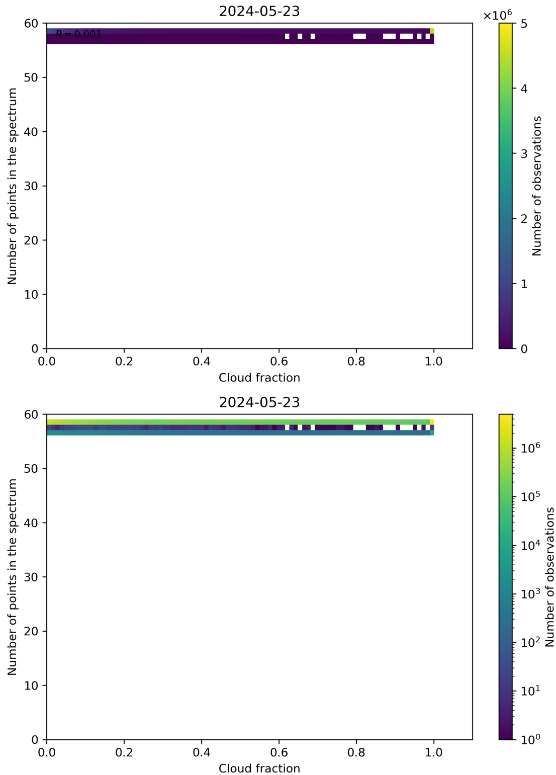
Figure 74: Scatter density plot of “Cloud fraction” against “Number of points in the spectrum” for 2024-05-23 to 2024-05-24.
