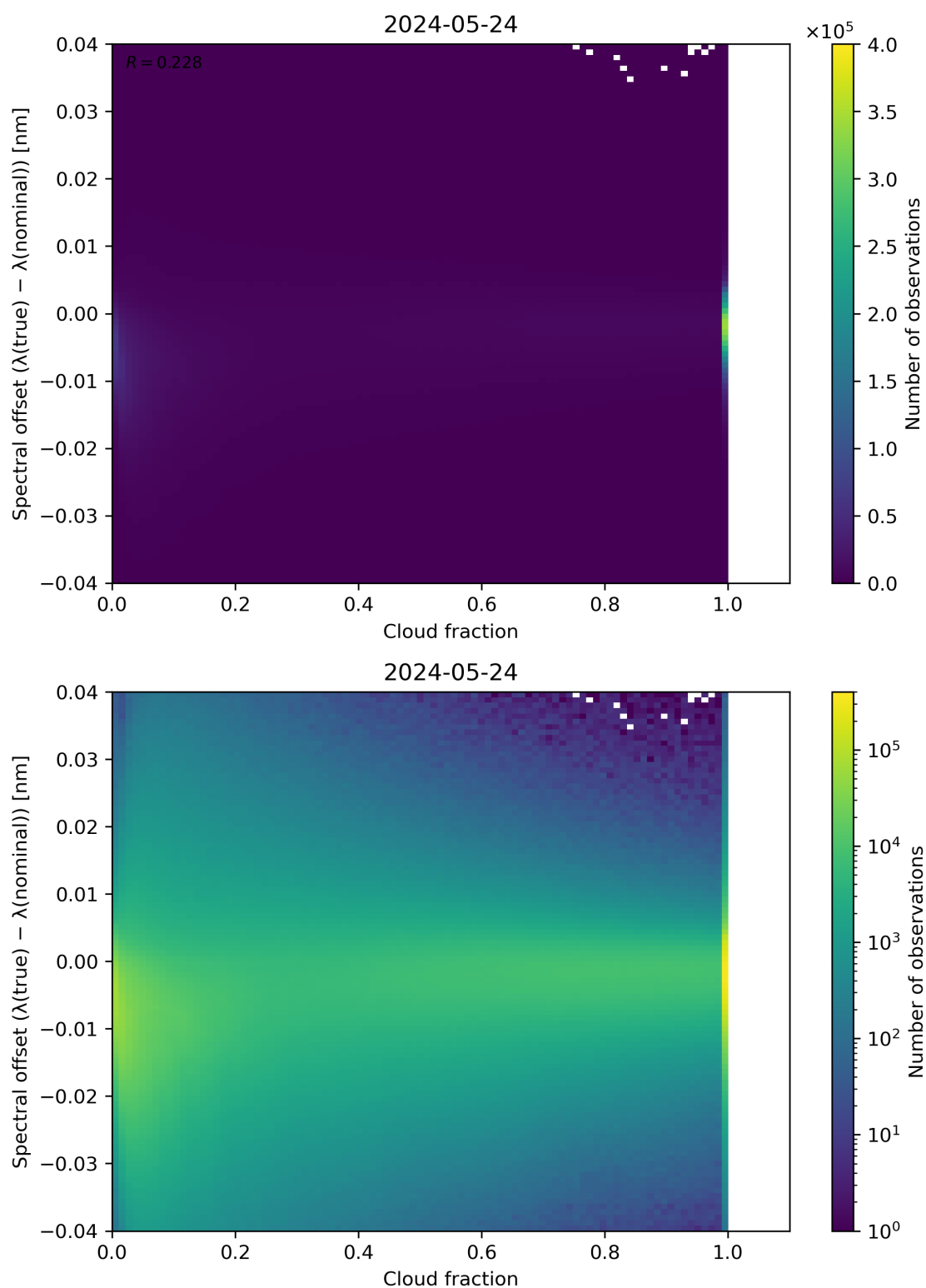
Figure 76: Scatter density plot of “Cloud fraction” against “Spectral offset ( \lambda(\text{true}) - \lambda(\text{nominal}) )” for 2024-05-23 to 2024-05-25.
