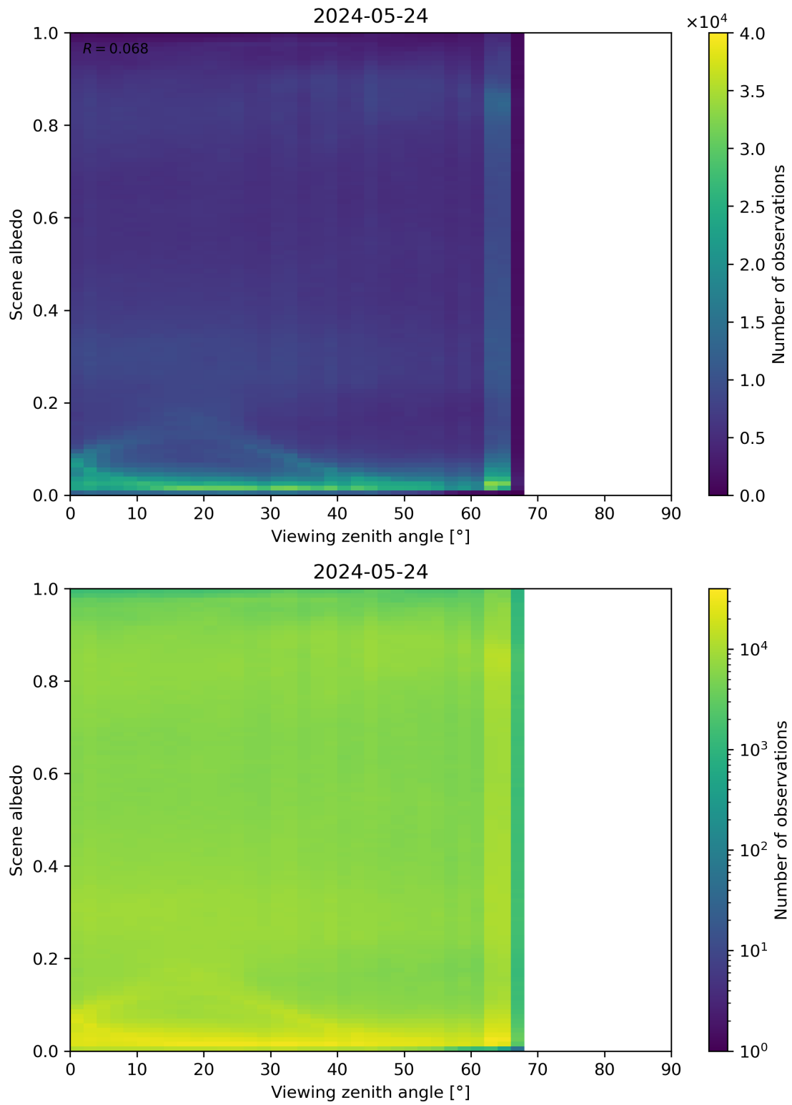
Figure 126: Scatter density plot of “Viewing zenith angle” against “Scene albedo” for 2024-05-23 to 2024-05-25.
