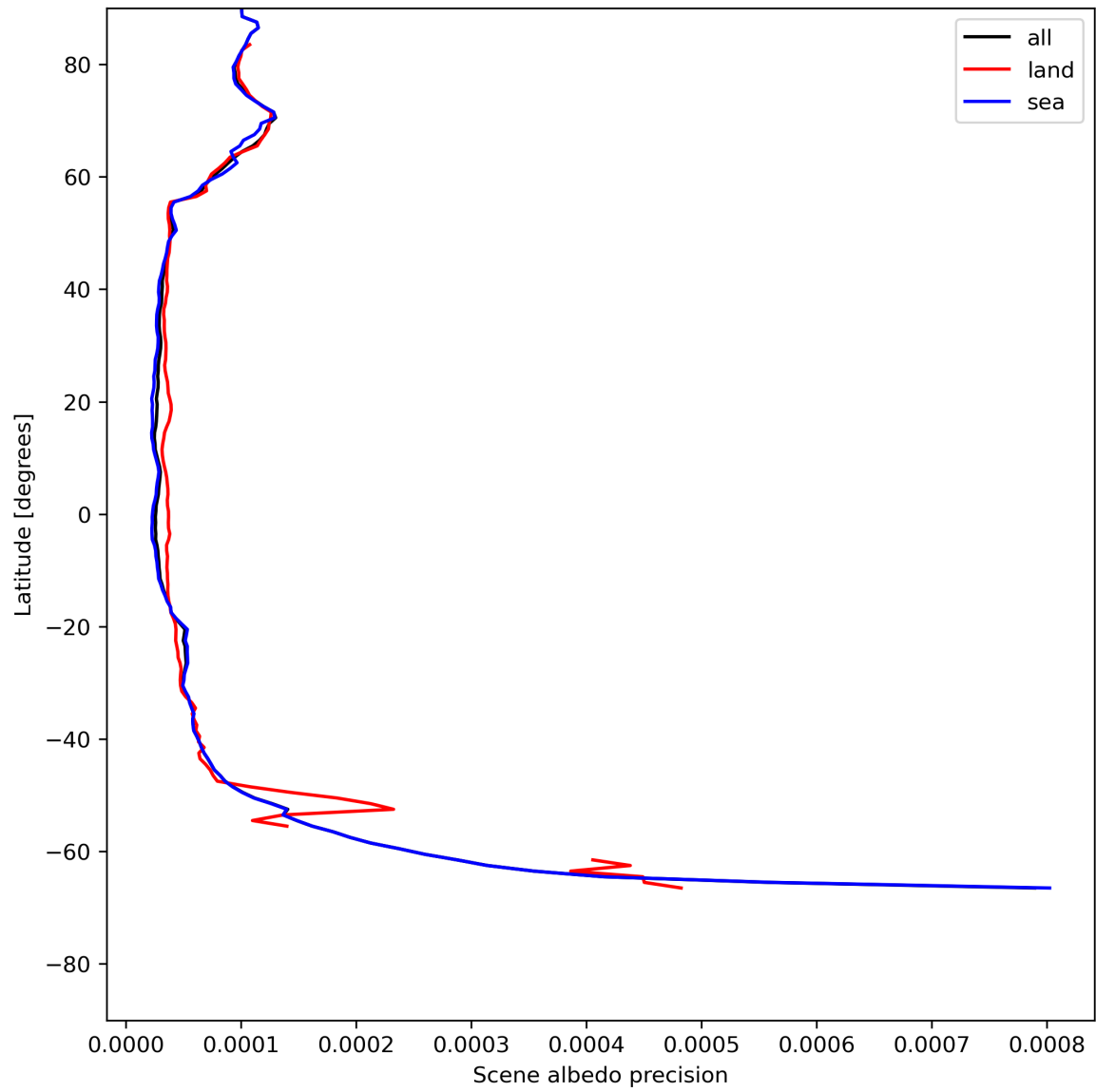
Figure 18: Zonal average of “Scene albedo precision” for 2024-05-23 to 2024-05-25.
