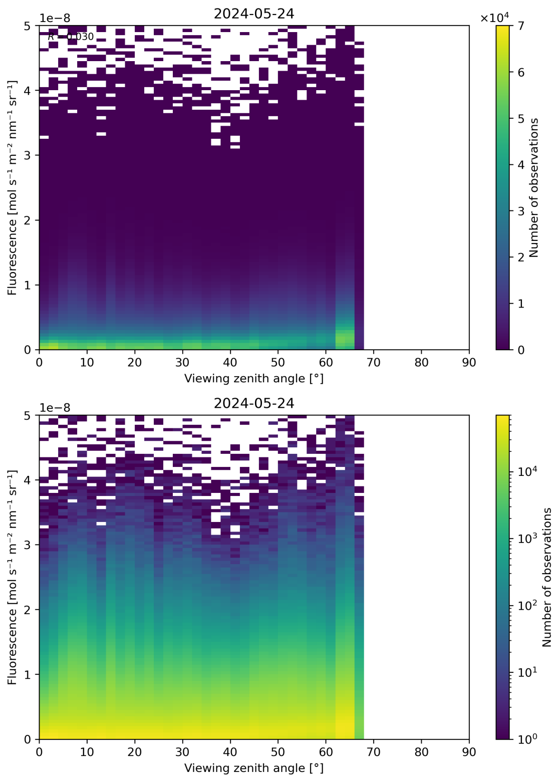
Figure 122: Scatter density plot of “Viewing zenith angle” against “Fluorescence” for 2024-05-23 to 2024-05-25.
