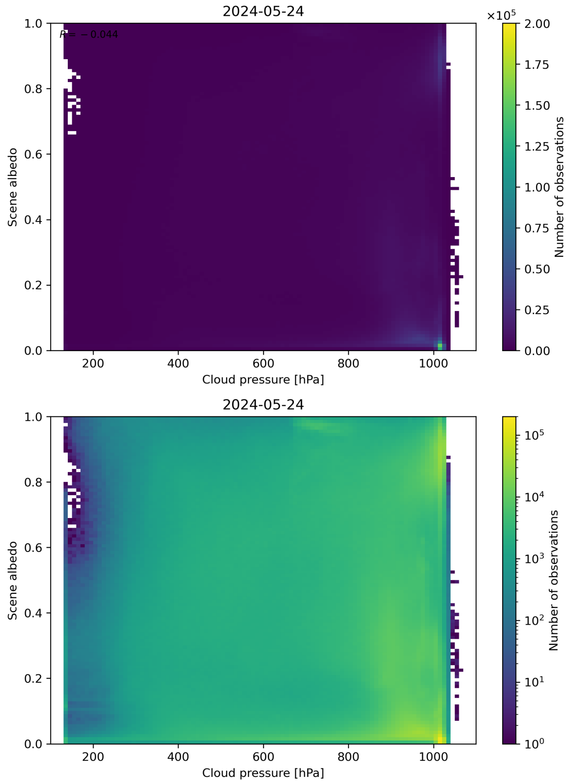
Figure 83: Scatter density plot of “Cloud pressure” against “Scene albedo” for 2024-05-23 to 2024-05-25.
