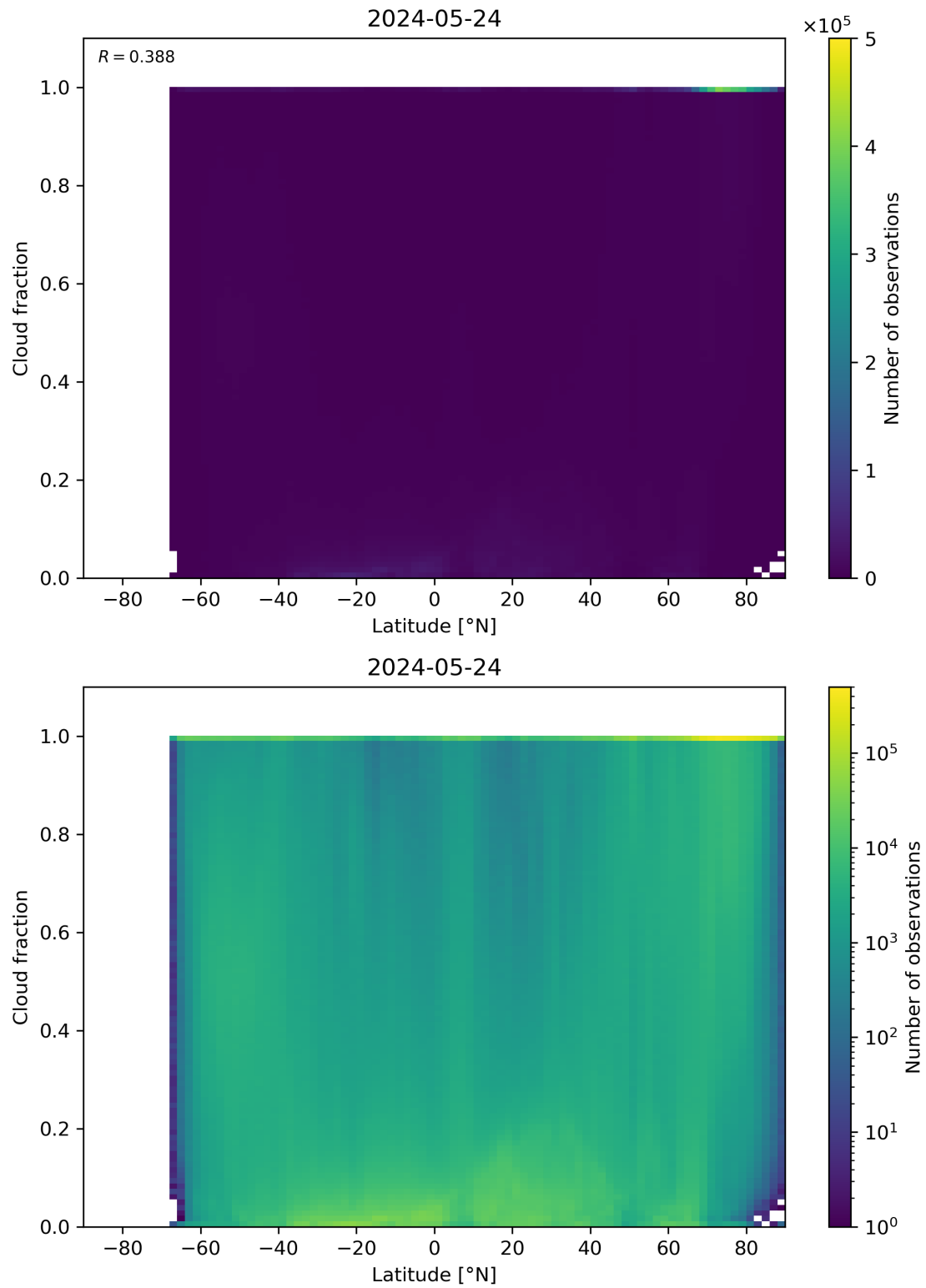
Figure 90: Scatter density plot of “Latitude” against “Cloud fraction” for 2024-05-23 to 2024-05-25.
