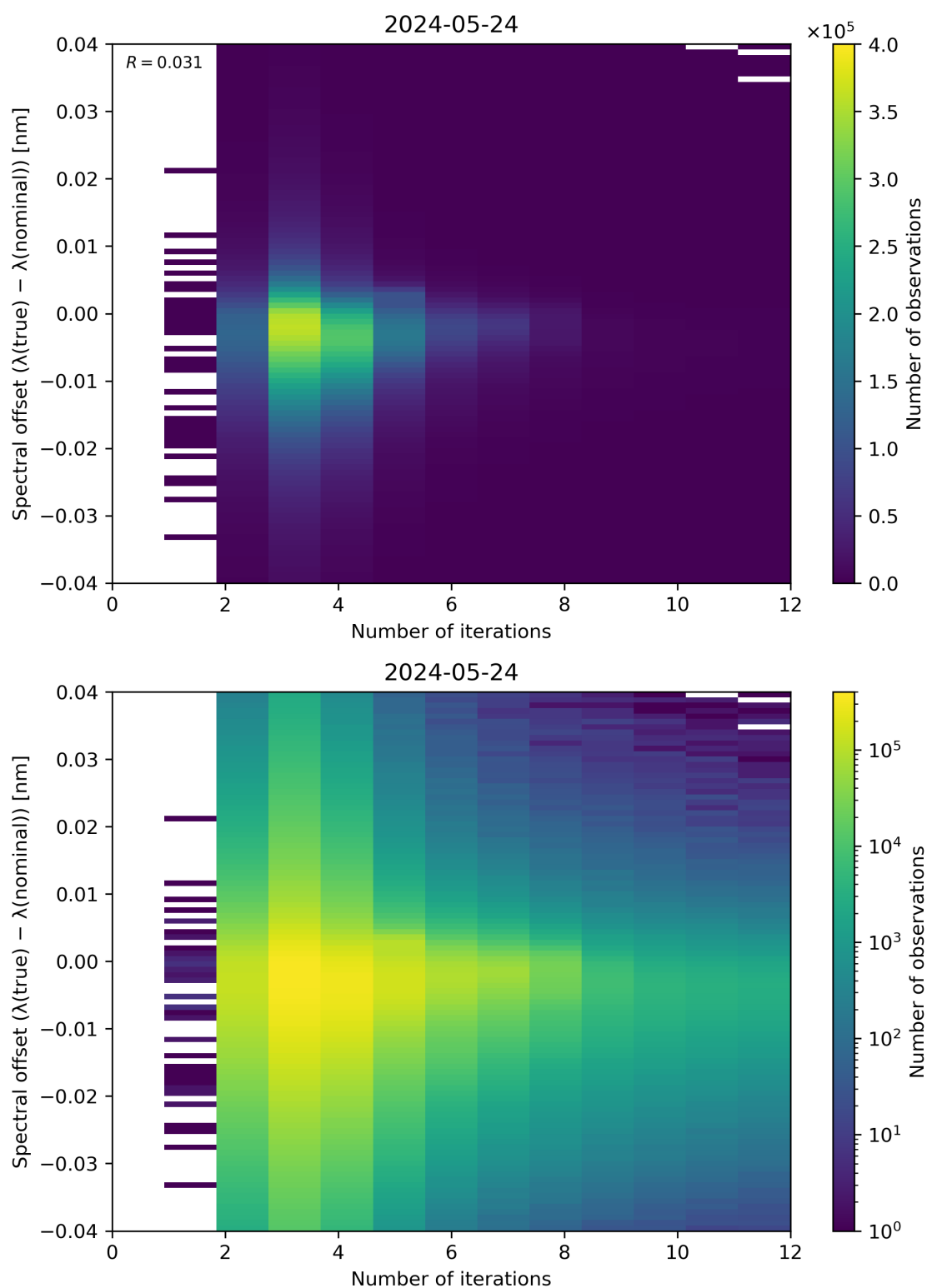
Figure 100: Scatter density plot of “Number of iterations” against “Spectral offset ( \lambda(\text{true}) - \lambda(\text{nominal}) )” for 2024-05-23 to 2024-05-25.
