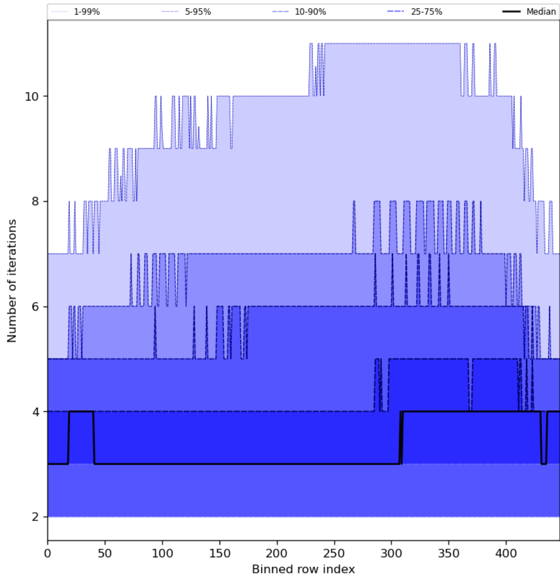
Figure 56: Along track statistics of “Number of iterations” for 2024-05-23 to 2024-05-25
