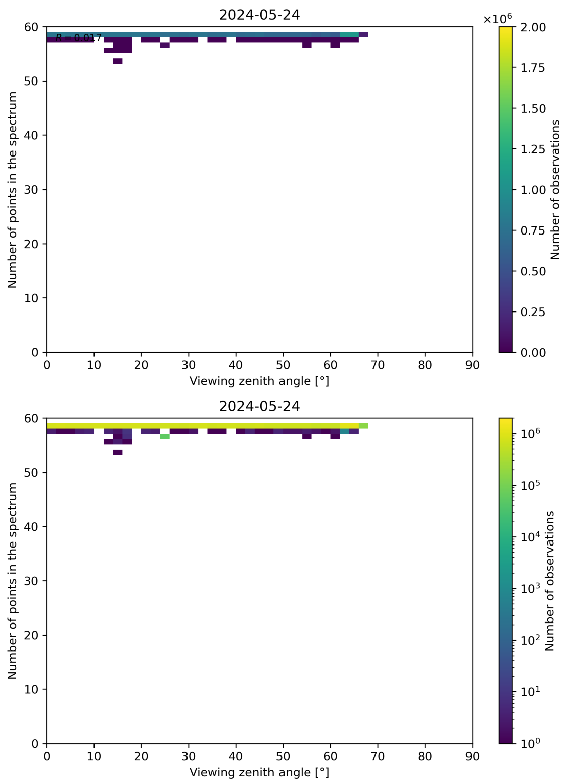
Figure 125: Scatter density plot of “Viewing zenith angle” against “Number of points in the spectrum” for 2024-05-23 to 2024-05-25.
