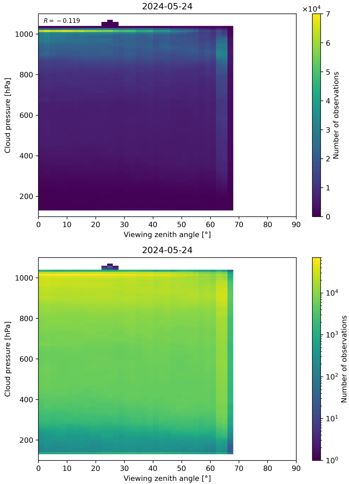
Figure 121: Scatter density plot of “Viewing zenith angle” against “Cloud pressure” for 2024-05-23 to 2024-05-25.
