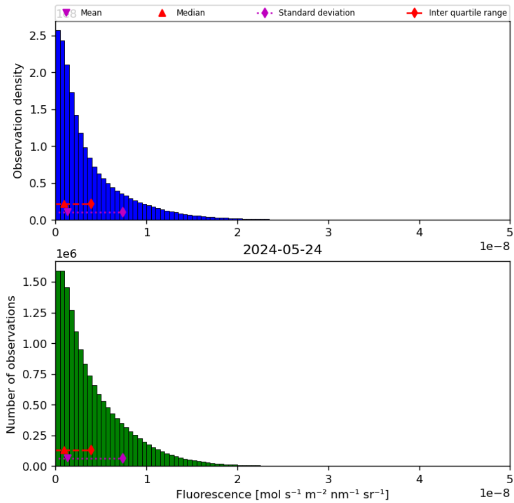
Figure 40: Histogram of “Fluorescence” for 2024-05-23 to 2024-05-25
