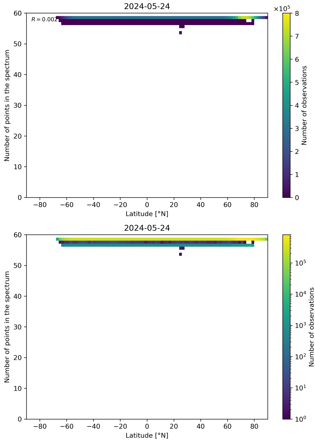
Figure 94: Scatter density plot of “Latitude” against “Number of points in the spectrum” for 2024-05-23 to 2024-05-25.
