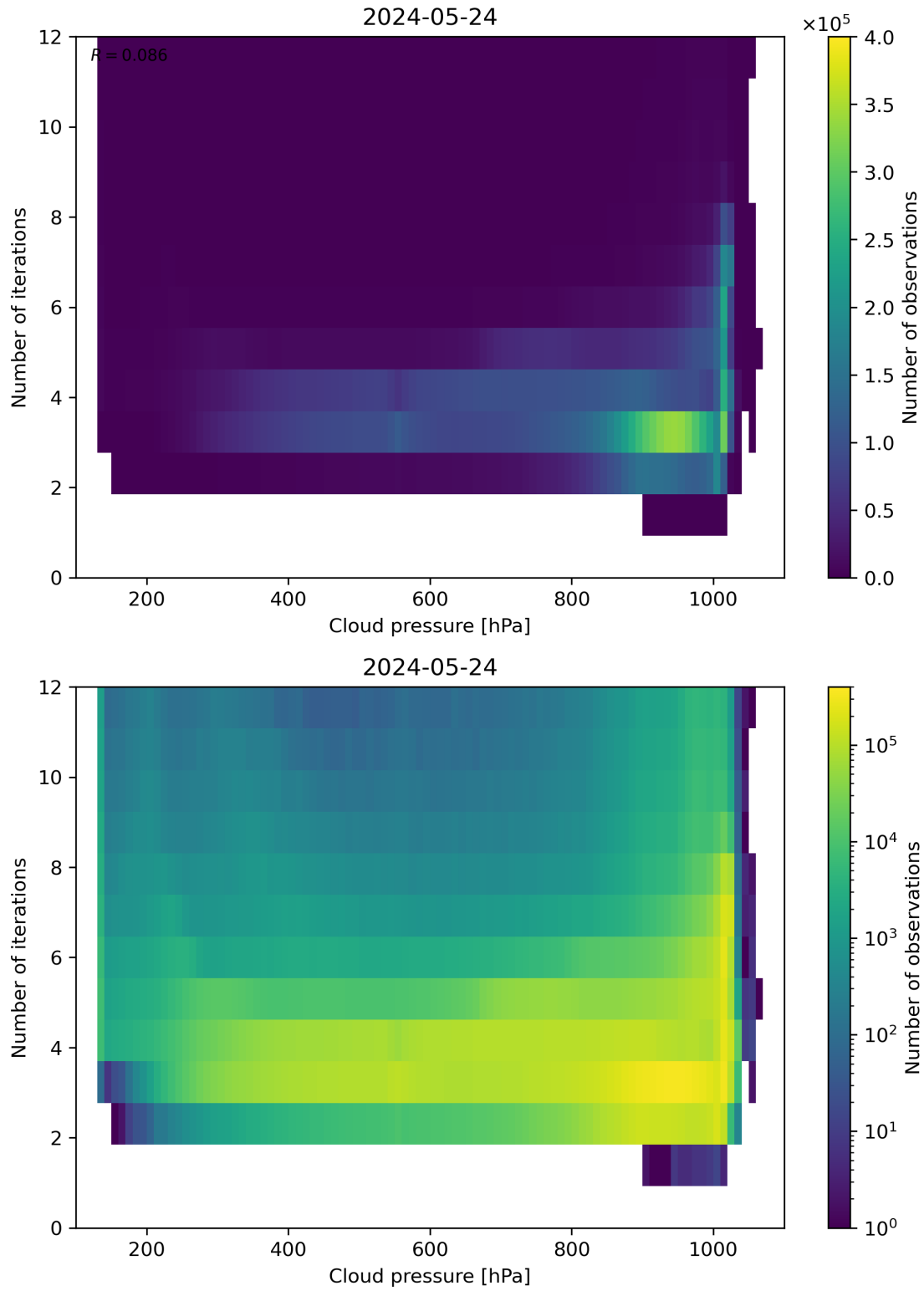
Figure 81: Scatter density plot of “Cloud pressure” against “Number of iterations” for 2024-05-23 to 2024-05-25.
