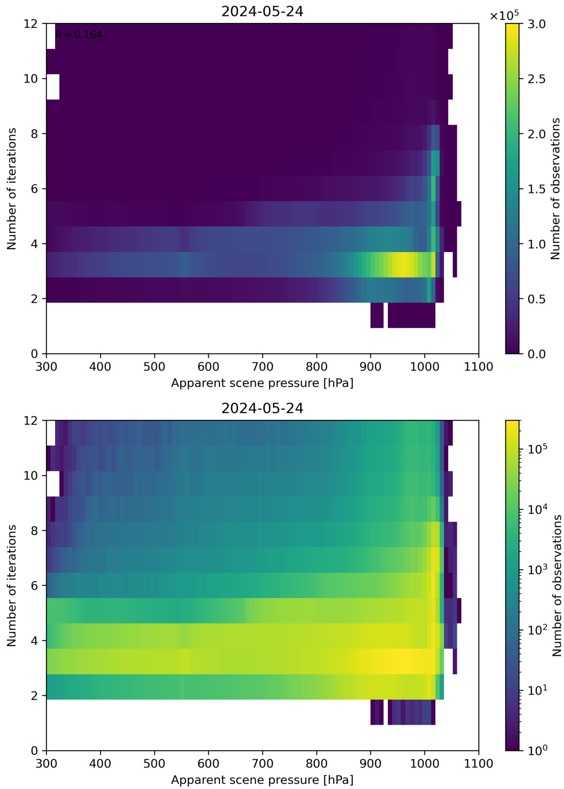
Figure 65: Scatter density plot of “Apparent scene pressure” against “Number of iterations” for 2024-05-23 to 2024-05-25.
