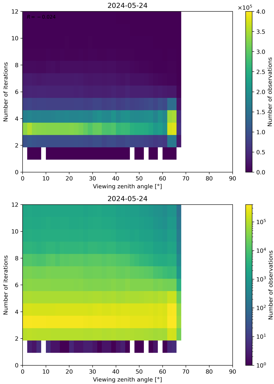
Figure 124: Scatter density plot of “Viewing zenith angle” against “Number of iterations” for 2024-05-23 to 2024-05-25.
