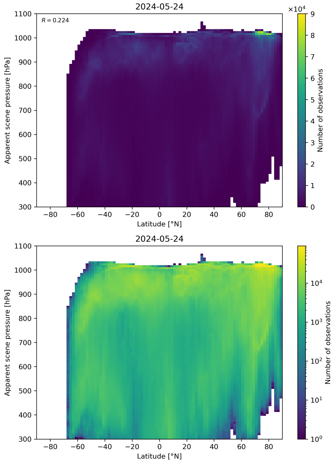
Figure 88: Scatter density plot of “Latitude” against “Apparent scene pressure” for 2024-05-23 to 2024-05-25.
