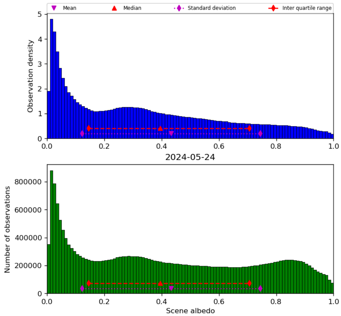
Figure 34: Histogram of “Scene albedo” for 2024-05-23 to 2024-05-25
