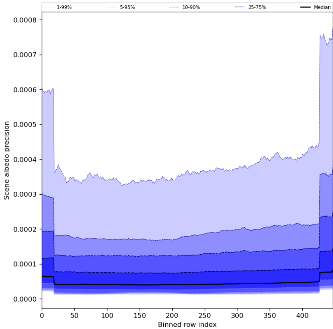
Figure 52: Along track statistics of “Scene albedo precision” for 2024-05-23 to 2024-05-25
