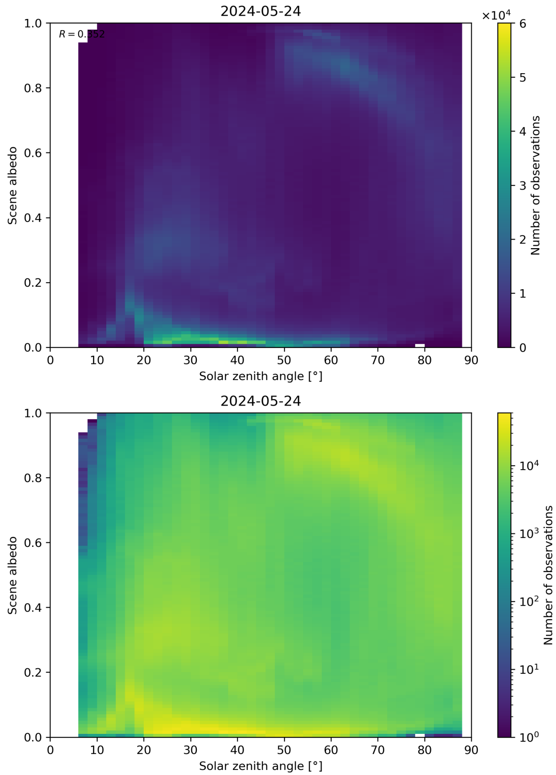
Figure 116: Scatter density plot of “Solar zenith angle” against “Scene albedo” for 2024-05-23 to 2024-05-25.
