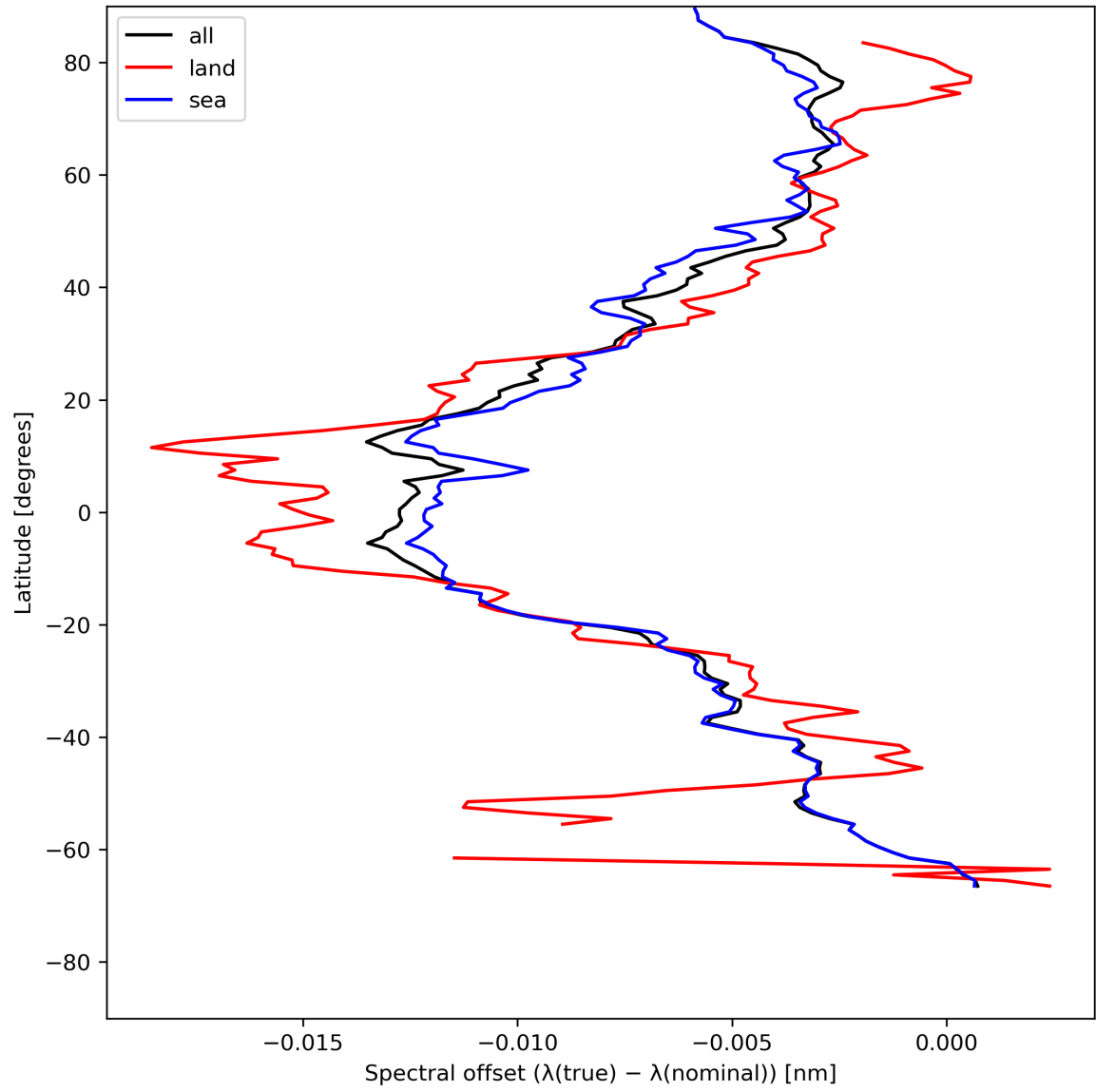
Figure 28: Zonal average of “Spectral offset ( \lambda(\text{true}) - \lambda(\text{nominal}) )” for 2024-05-23 to 2024-05-25.
