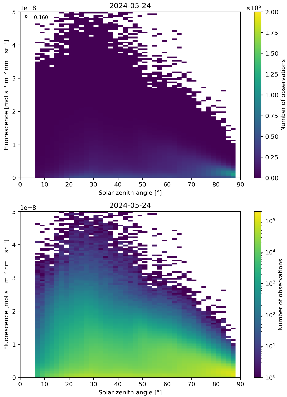
Figure 112: Scatter density plot of “Solar zenith angle” against “Fluorescence” for 2024-05-23 to 2024-05-25.
