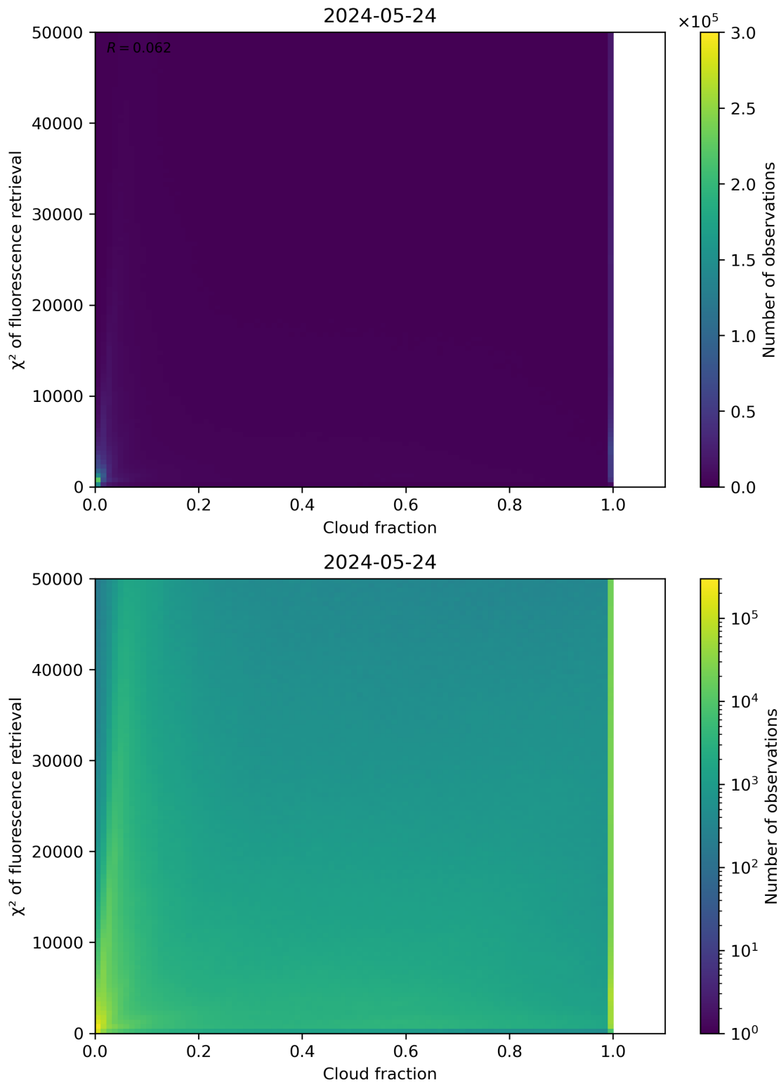
Figure 71: Scatter density plot of “Cloud fraction” against “ \chi^2 of fluorescence retrieval” for 2024-05-23 to 2024-05-25.
