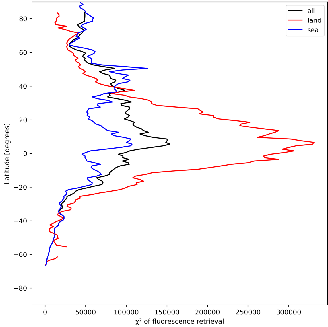
Figure 25: Zonal average of “ \chi^2 of fluorescence retrieval” for 2024-05-23 to 2024-05-25.
