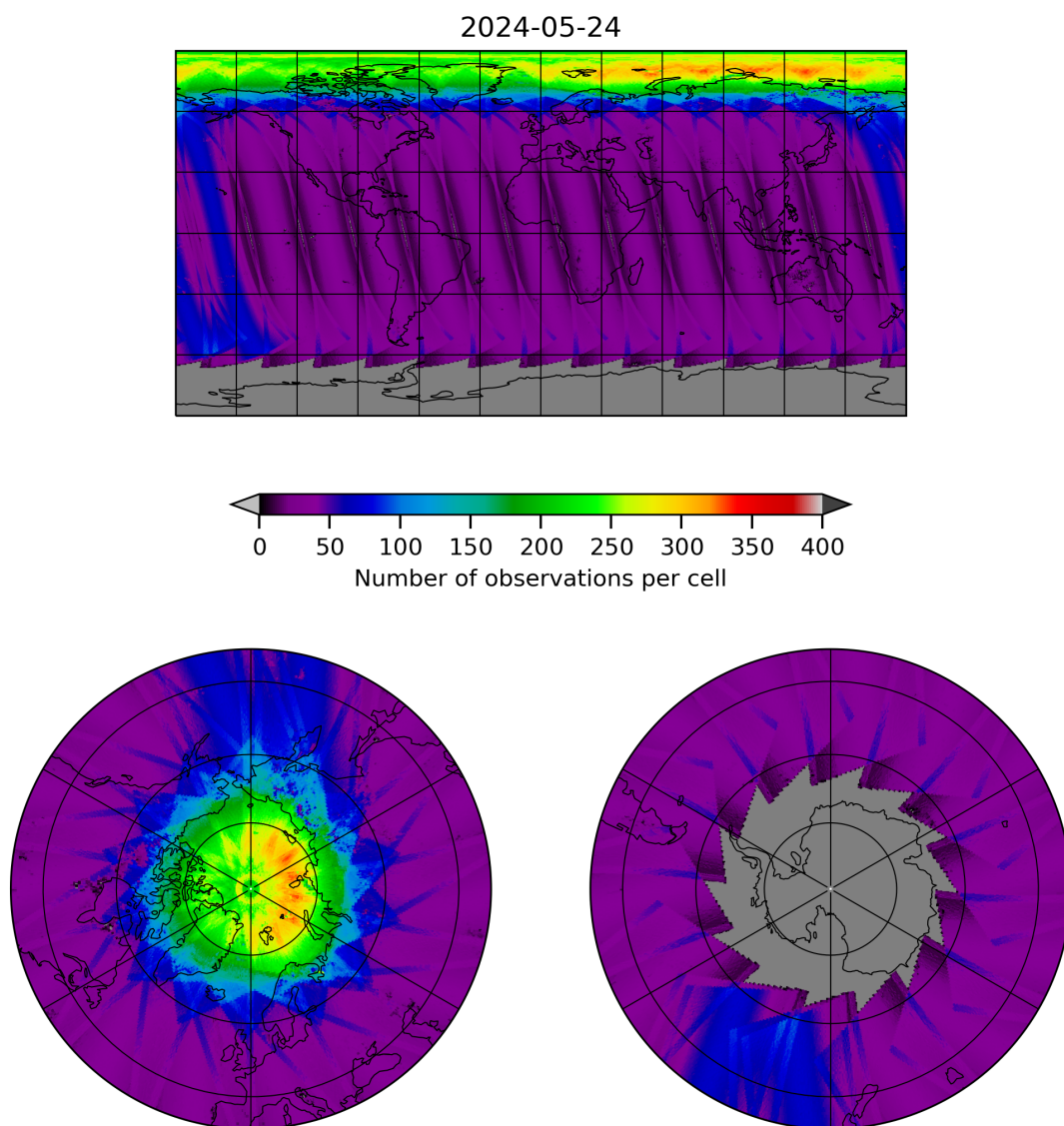
Figure 11: Map of the number of observations for 2024-05-23 to 2024-05-25
