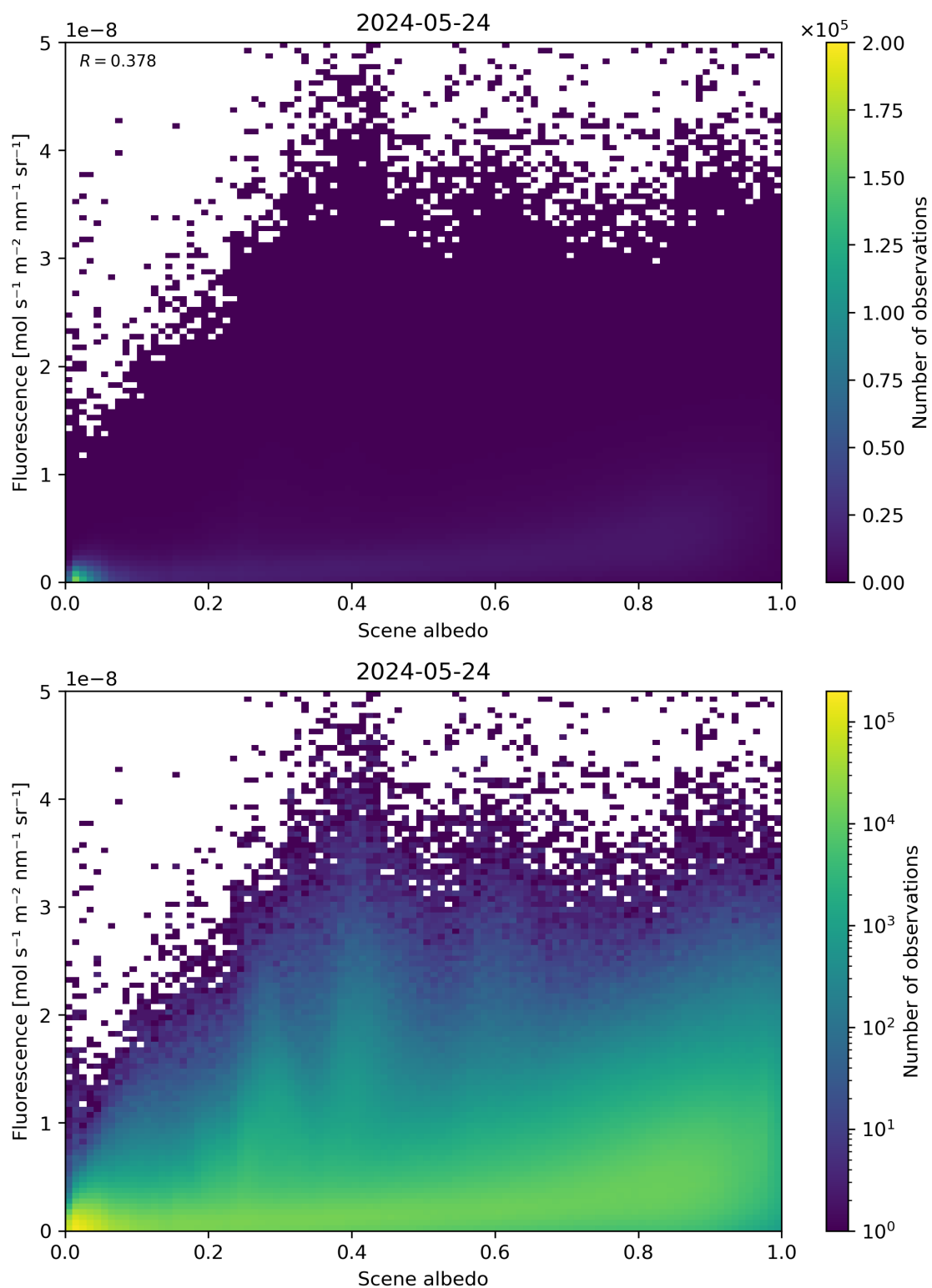
Figure 104: Scatter density plot of “Scene albedo” against “Fluorescence” for 2024-05-23 to 2024-05-25.
