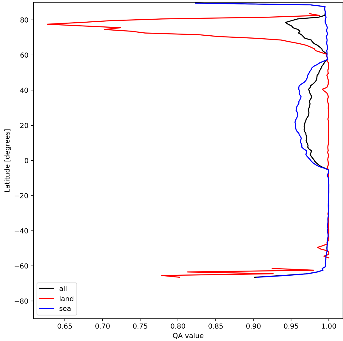
Figure 12: Zonal average of “QA value” for 2024-05-23 to 2024-05-25.
