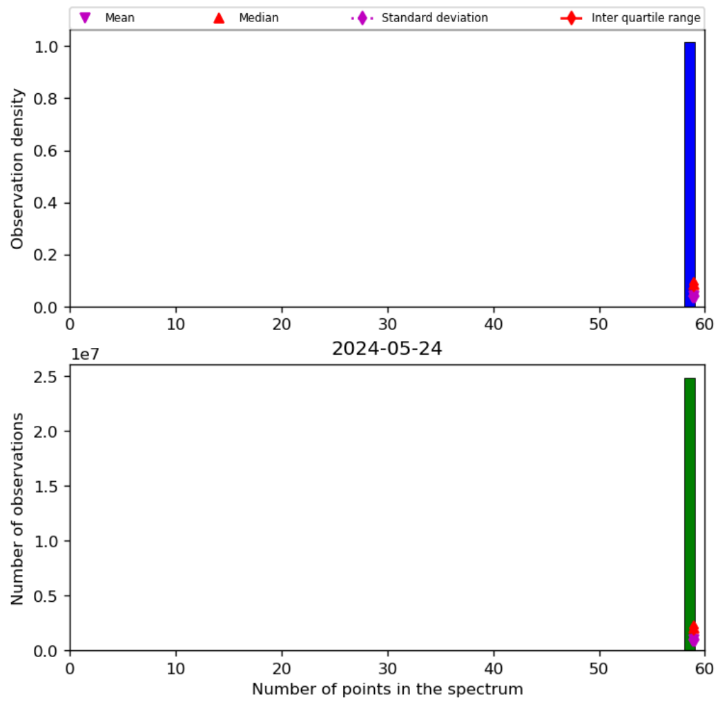
Figure 44: Histogram of “Number of points in the spectrum” for 2024-05-23 to 2024-05-25
