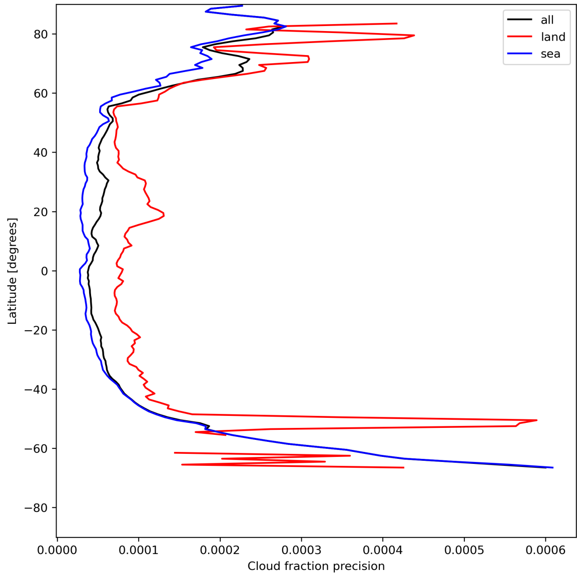
Figure 16: Zonal average of “Cloud fraction precision” for 2024-05-23 to 2024-05-25.
