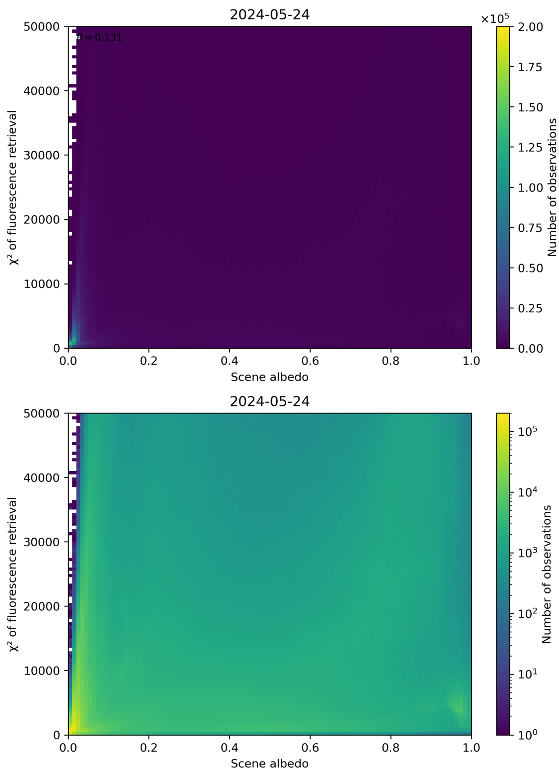
Figure 103: Scatter density plot of “Scene albedo” against “ \chi^2 of fluorescence retrieval” for 2024-05-23 to 2024-05-25.
