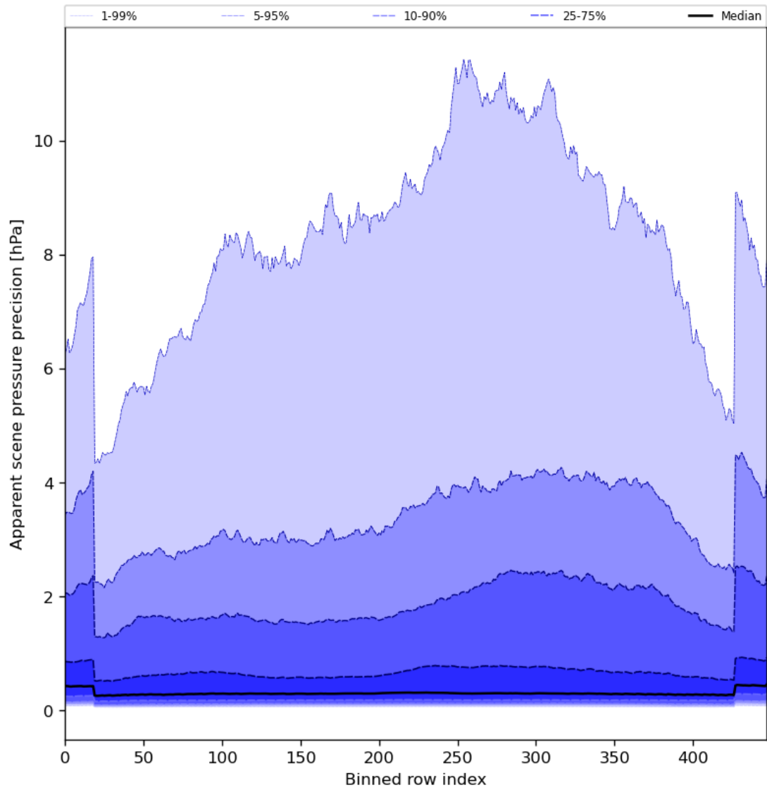
Figure 54: Along track statistics of “Apparent scene pressure precision” for 2024-05-23 to 2024-05-25
