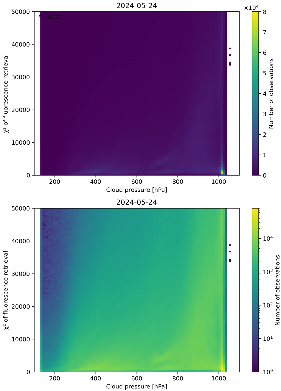
Figure 78: Scatter density plot of “Cloud pressure” against “ \chi^2 of fluorescence retrieval” for 2024-05-23 to 2024-05-25.
