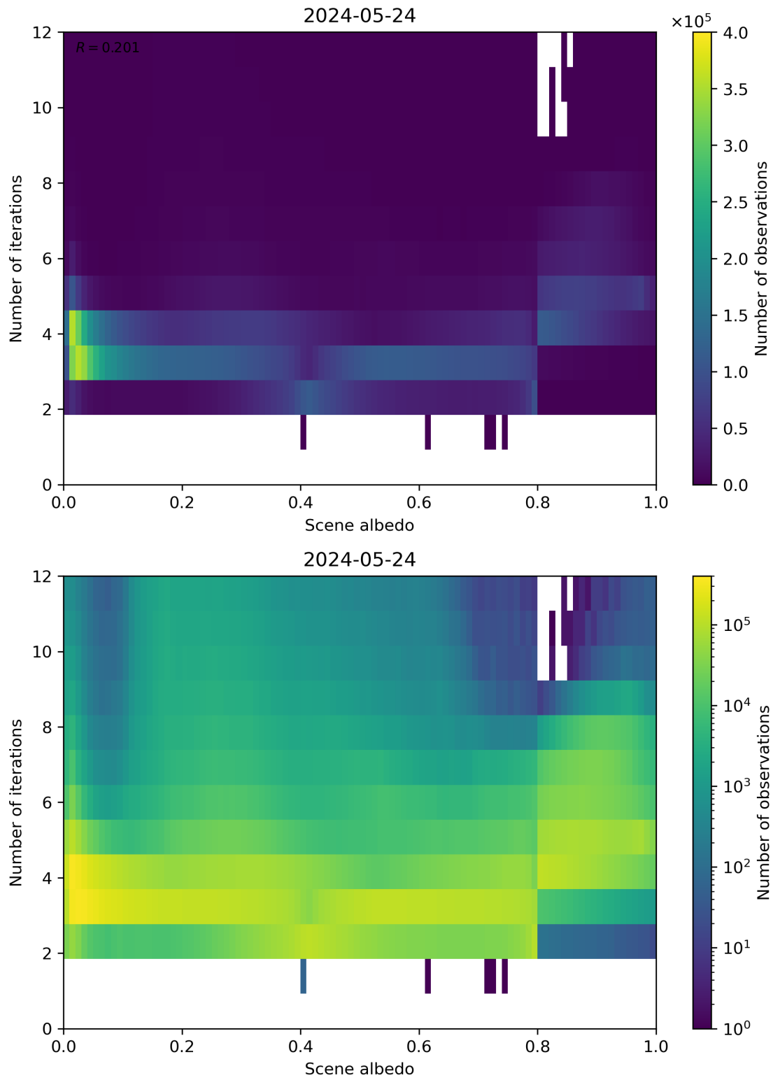
Figure 105: Scatter density plot of “Scene albedo” against “Number of iterations” for 2024-05-23 to 2024-05-25.
