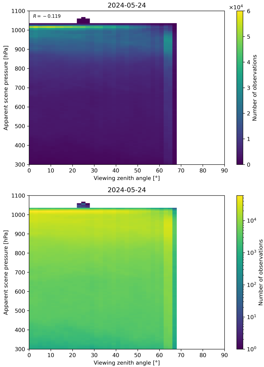
Figure 118: Scatter density plot of “Viewing zenith angle” against “Apparent scene pressure” for 2024-05-23 to 2024-05-25.
