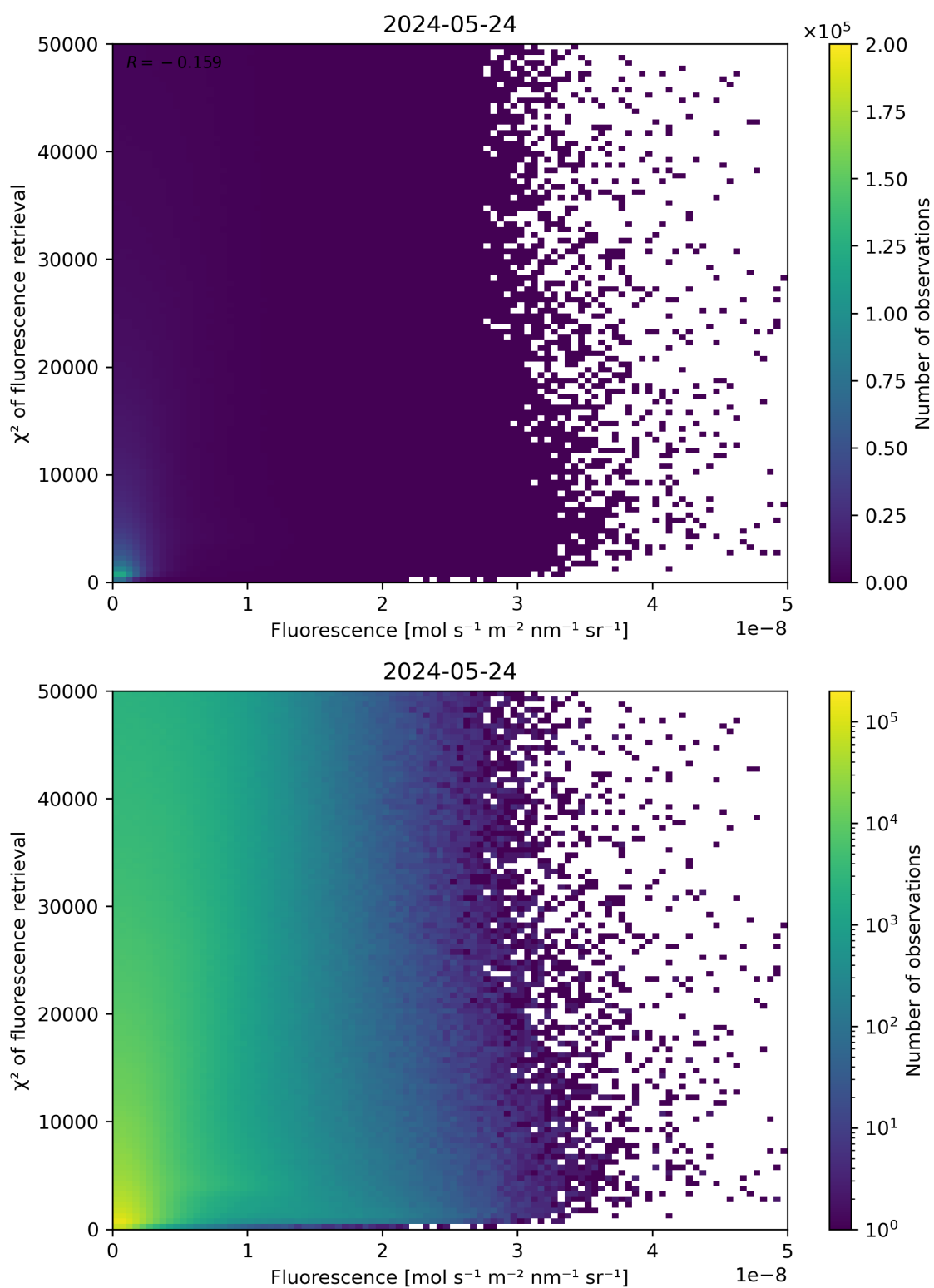
Figure 85: Scatter density plot of “Fluorescence” against “ \chi^2 of fluorescence retrieval” for 2024-05-23 to 2024-05-25.
