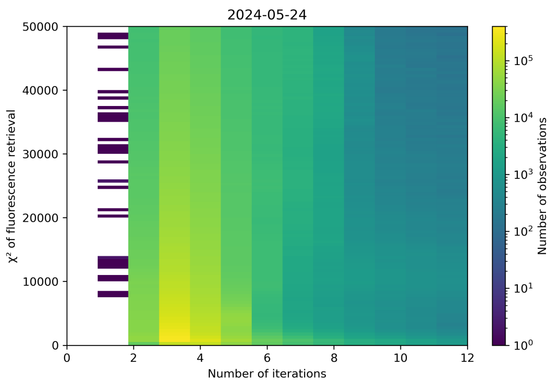
Figure 97: Scatter density plot of “Number of iterations” against “ \chi^2 of fluorescence retrieval” for 2024-05-23 to 2024-05-25.
