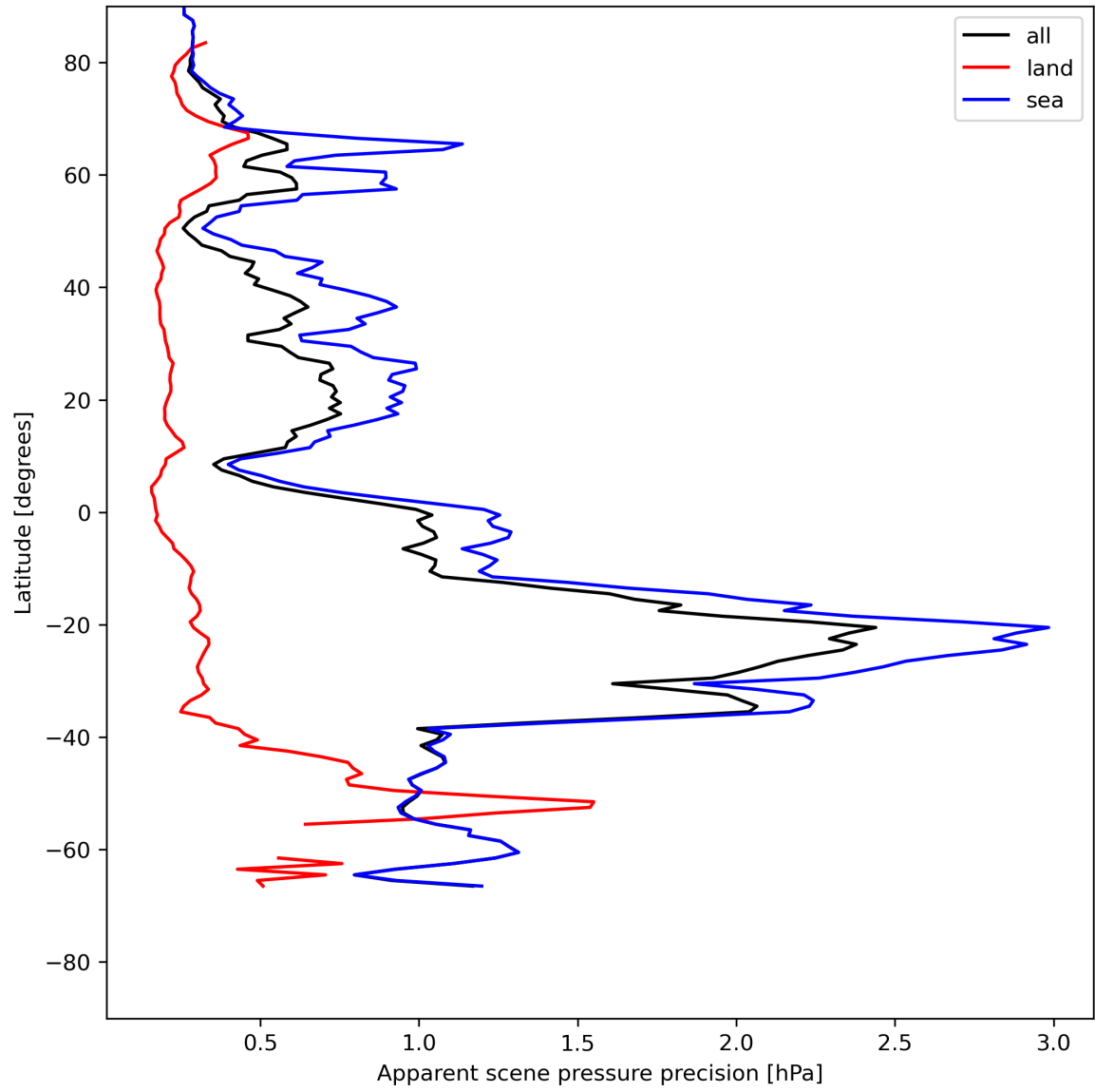
Figure 20: Zonal average of “Apparent scene pressure precision” for 2024-05-23 to 2024-05-25.
