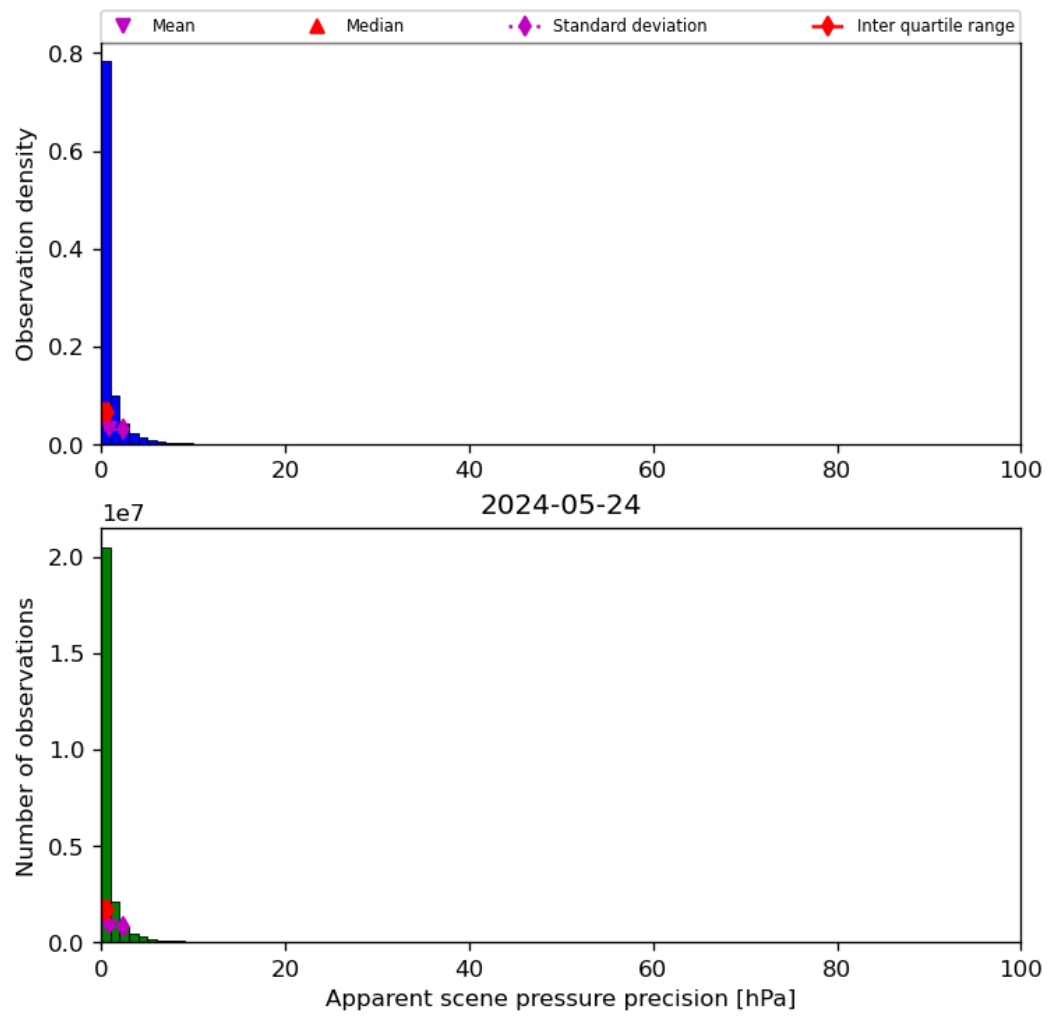
Figure 37: Histogram of “Apparent scene pressure precision” for 2024-05-23 to 2024-05-25
