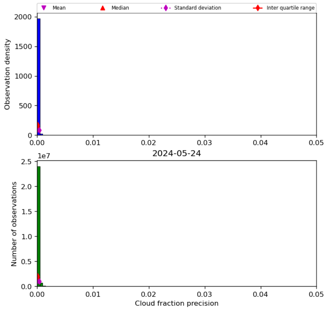
Figure 33: Histogram of “Cloud fraction precision” for 2024-05-23 to 2024-05-25
