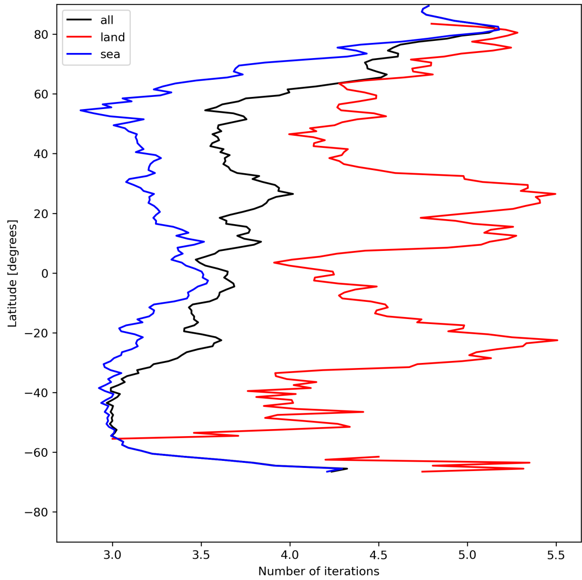
Figure 22: Zonal average of “Number of iterations” for 2024-05-23 to 2024-05-25.
