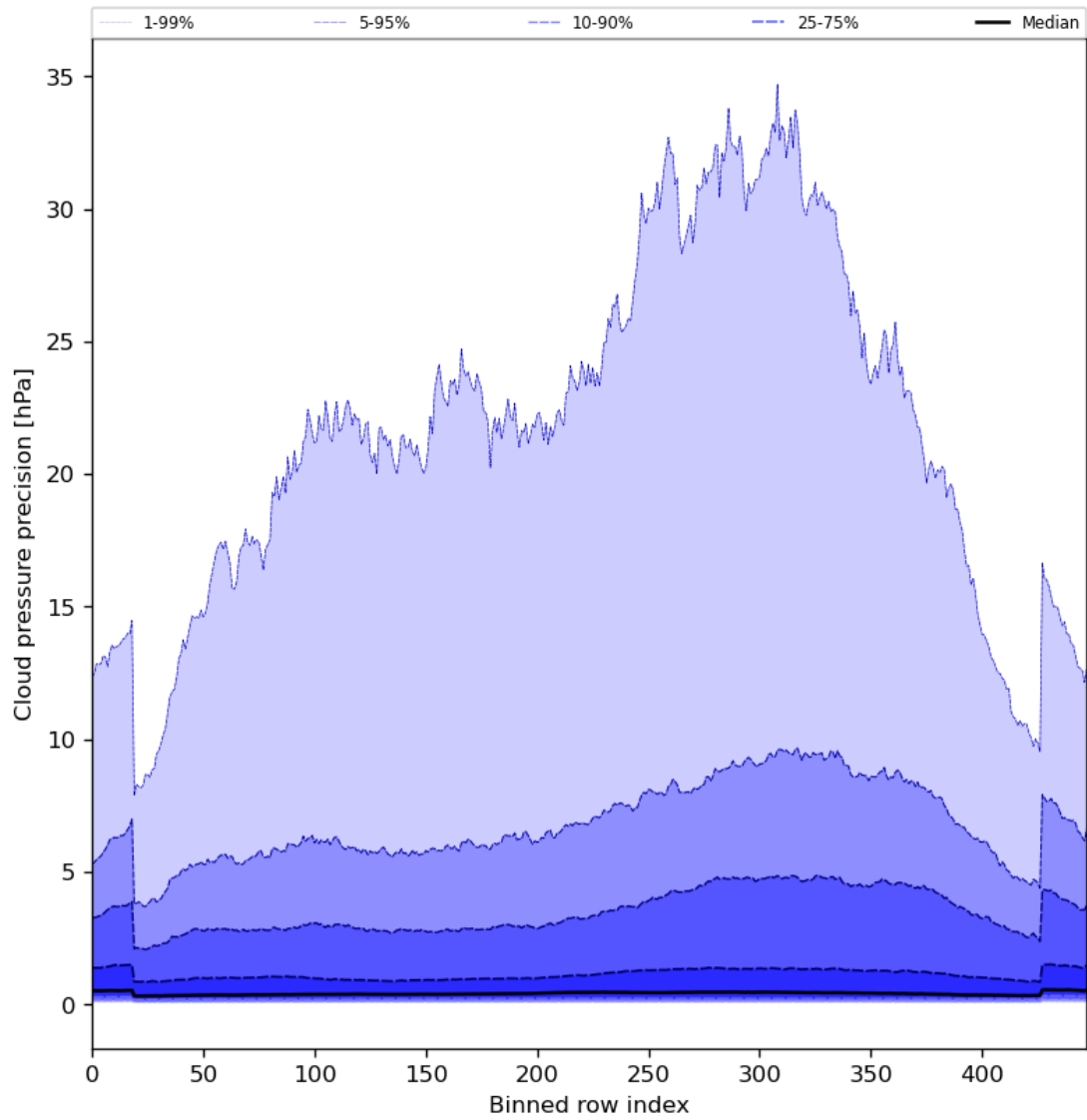
Figure 48: Along track statistics of “Cloud pressure precision” for 2024-05-23 to 2024-05-25
