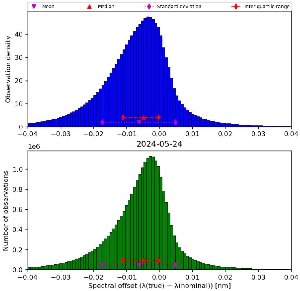
Figure 45: Histogram of “Spectral offset ( \lambda(\text{true}) - \lambda(\text{nominal}) )” for 2024-05-23 to 2024-05-25
