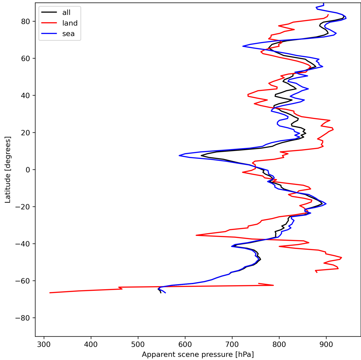
Figure 19: Zonal average of “Apparent scene pressure” for 2024-05-23 to 2024-05-25.
