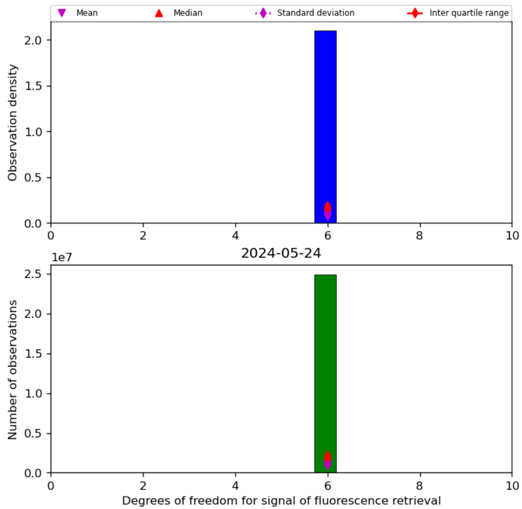
Figure 43: Histogram of “Degrees of freedom for signal of fluorescence retrieval” for 2024-05-23 to 2024-05-25
