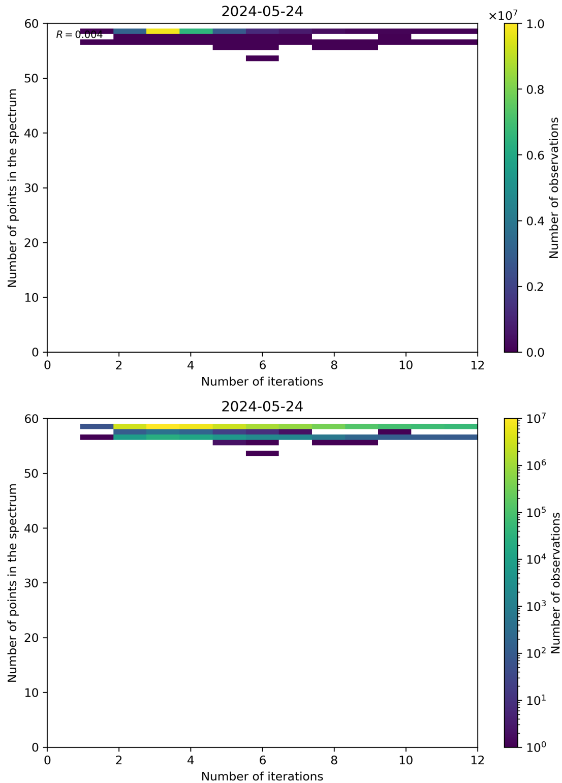
Figure 99: Scatter density plot of “Number of iterations” against “Number of points in the spectrum” for 2024-05-23 to 2024-05-25.
