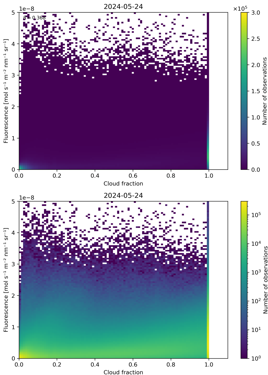
Figure 72: Scatter density plot of “Cloud fraction” against “Fluorescence” for 2024-05-23 to 2024-05-25.
