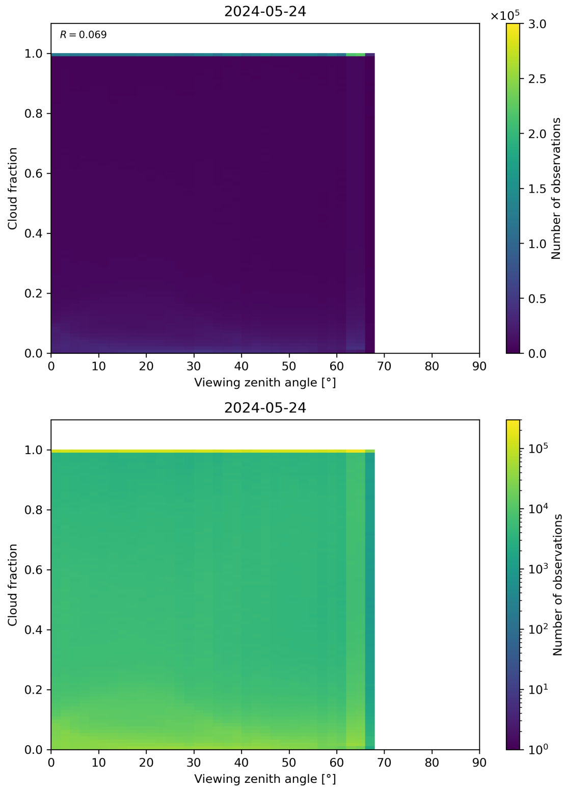
Figure 120: Scatter density plot of “Viewing zenith angle” against “Cloud fraction” for 2024-05-23 to 2024-05-25.
