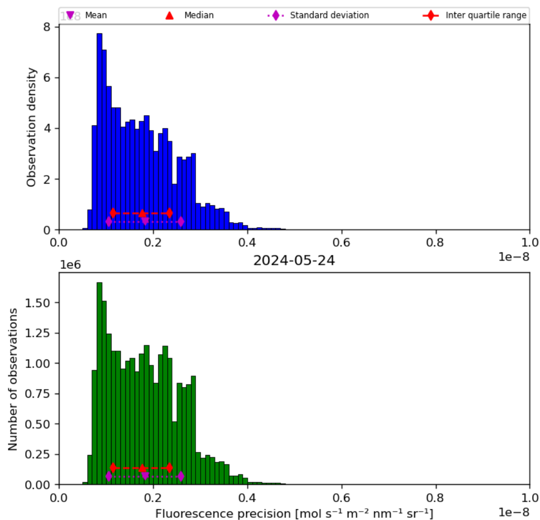
Figure 41: Histogram of “Fluorescence precision” for 2024-05-23 to 2024-05-25
