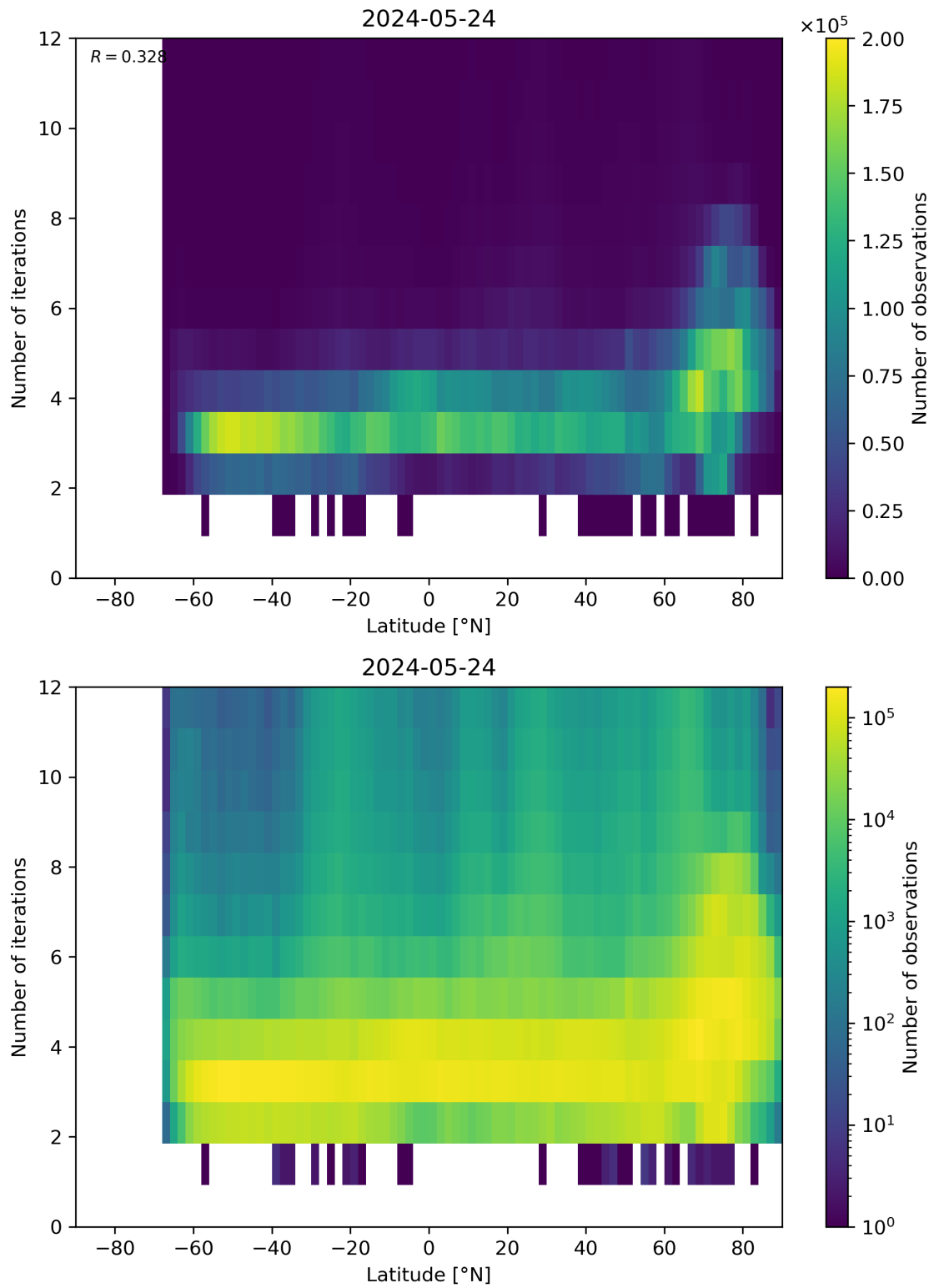
Figure 93: Scatter density plot of “Latitude” against “Number of iterations” for 2024-05-23 to 2024-05-25.
