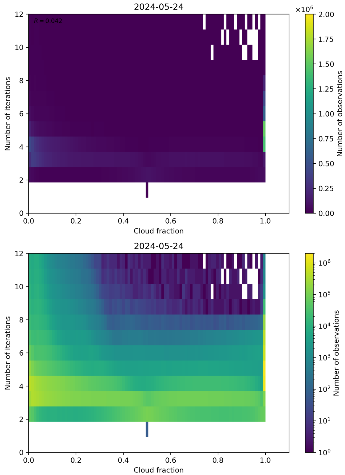
Figure 73: Scatter density plot of “Cloud fraction” against “Number of iterations” for 2024-05-23 to 2024-05-25.
