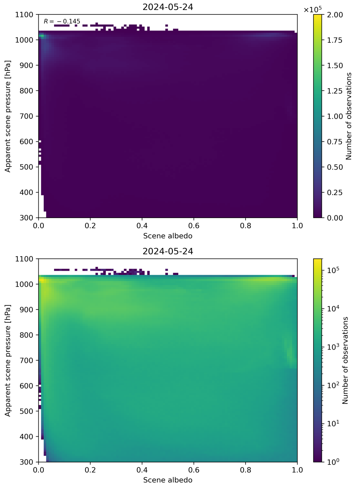
Figure 102: Scatter density plot of “Scene albedo” against “Apparent scene pressure” for 2024-05-23 to 2024-05-25.
