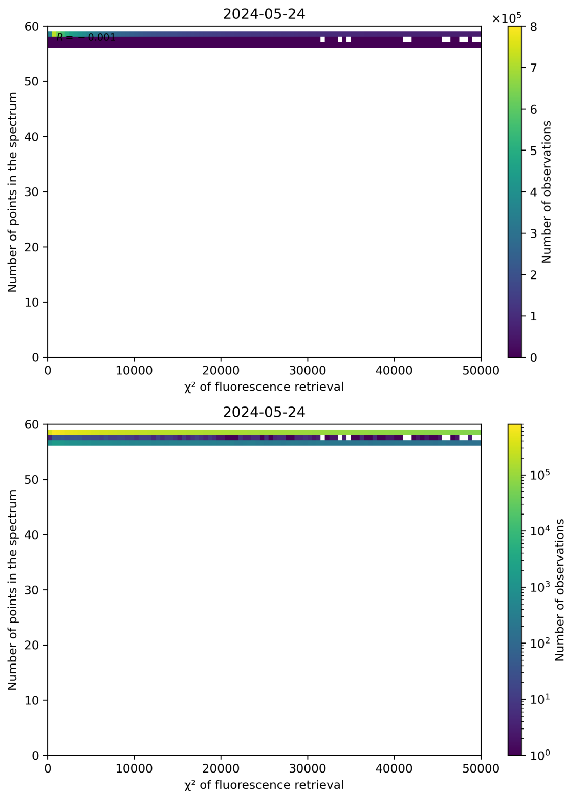
Figure 68: Scatter density plot of " \chi^2 of fluorescence retrieval" against "Number of points in the spectrum" for 2024-05-23 to 2024-05-25.
