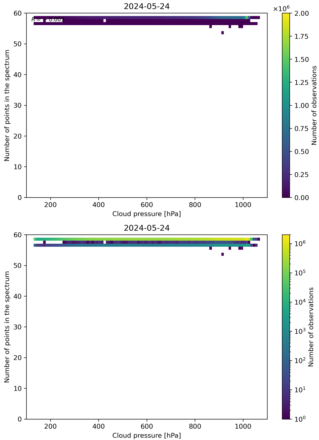
Figure 82: Scatter density plot of “Cloud pressure” against “Number of points in the spectrum” for 2024-05-23 to 2024-05-25.
