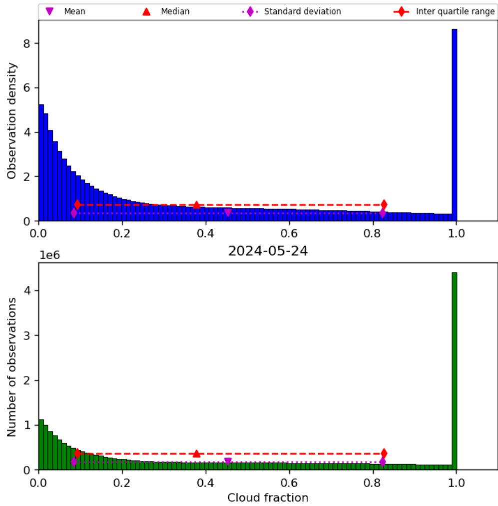
Figure 32: Histogram of “Cloud fraction” for 2024-05-23 to 2024-05-25
