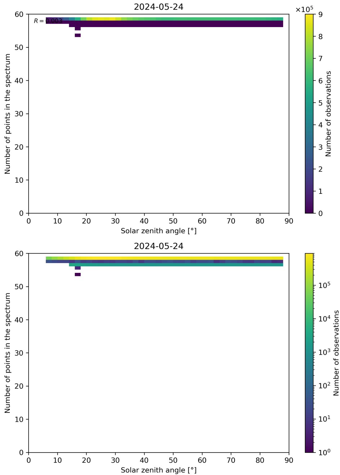
Figure 115: Scatter density plot of “Solar zenith angle” against “Number of points in the spectrum” for 2024-05-23 to 2024-05-25.
