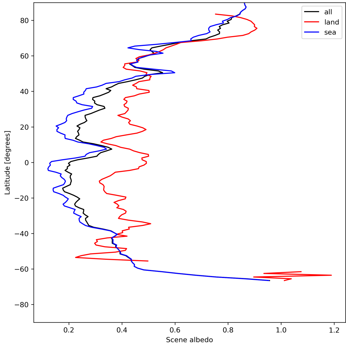
Figure 17: Zonal average of “Scene albedo” for 2024-05-23 to 2024-05-25.
