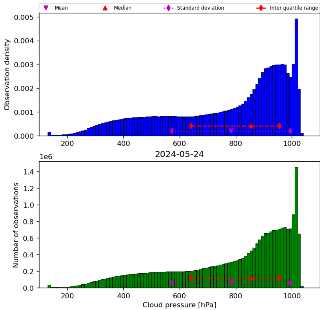
Figure 30: Histogram of “Cloud pressure” for 2024-05-23 to 2024-05-25
