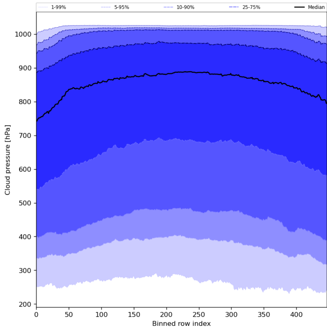
Figure 47: Along track statistics of "Cloud pressure" for 2024-05-23 to 2024-05-25
