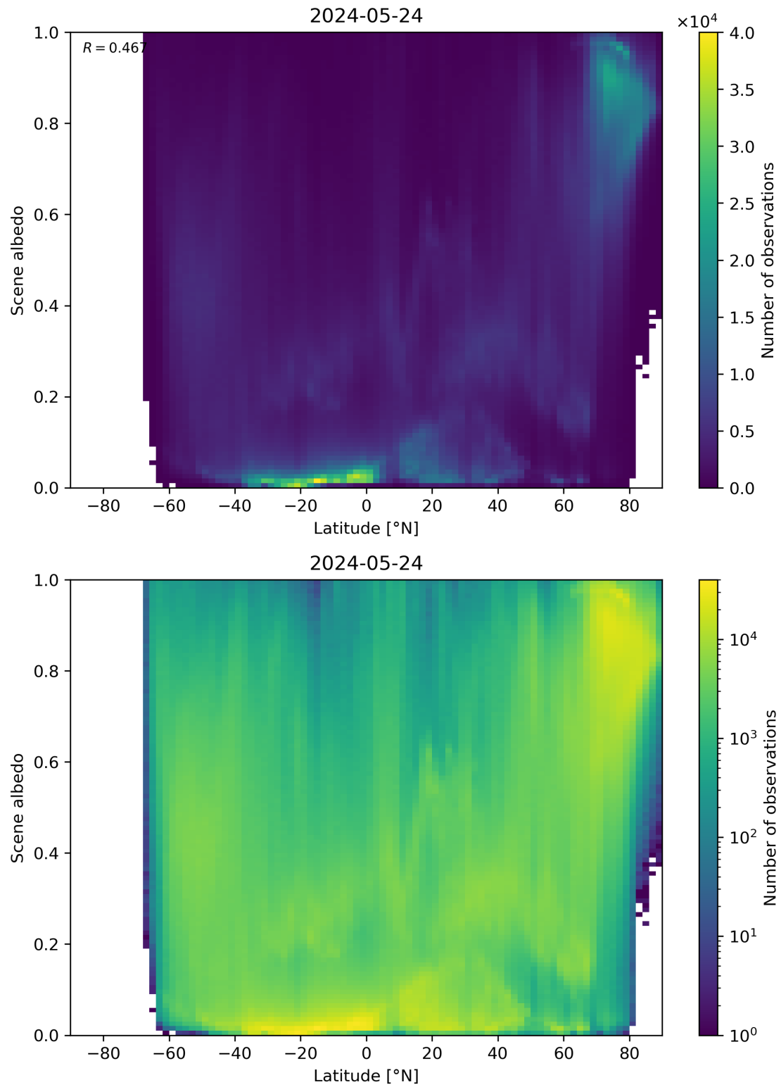
Figure 95: Scatter density plot of “Latitude” against “Scene albedo” for 2024-05-23 to 2024-05-25.
