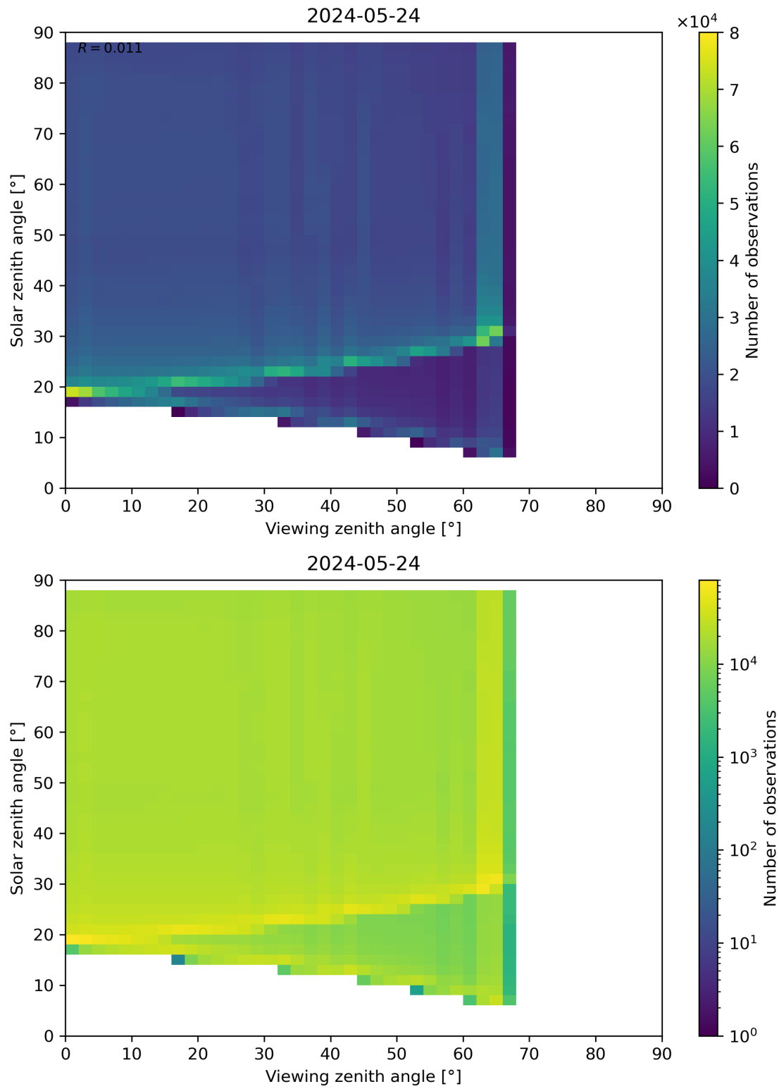
Figure 127: Scatter density plot of “Viewing zenith angle” against “Solar zenith angle” for 2024-05-23 to 2024-05-25.
