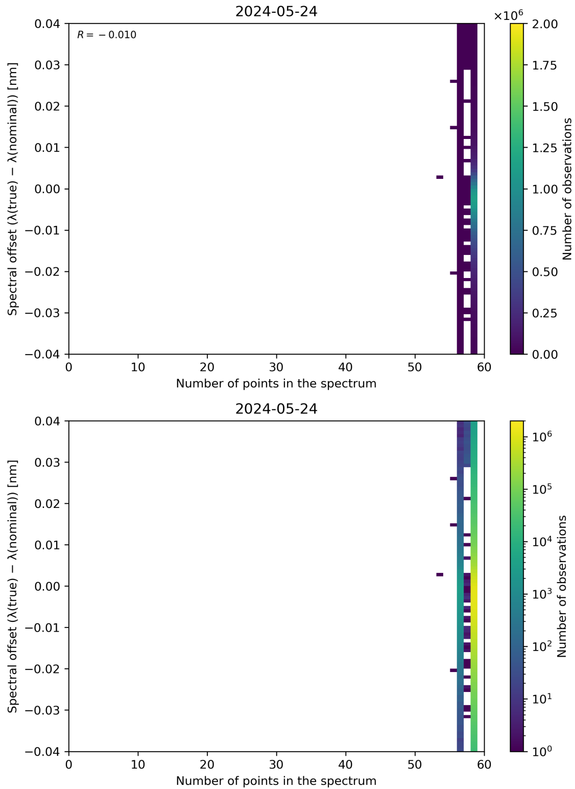
Figure 101: Scatter density plot of “Number of points in the spectrum” against “Spectral offset ( \lambda(\text{true}) - \lambda(\text{nominal}) )” for 2024-05-23 to 2024-05-25.
