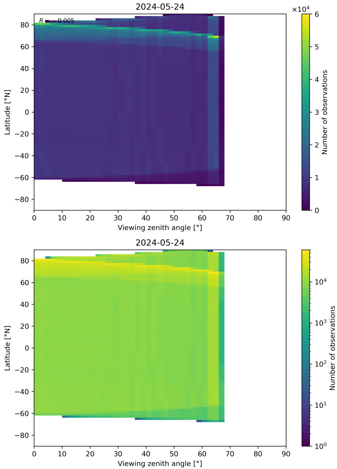
Figure 123: Scatter density plot of “Viewing zenith angle” against “Latitude” for 2024-05-23 to 2024-05-25.
