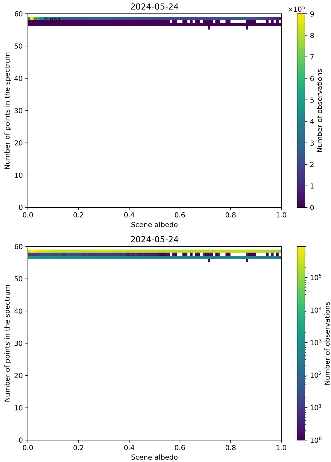
Figure 106: Scatter density plot of “Scene albedo” against “Number of points in the spectrum” for 2024-05-23 to 2024-05-25.
