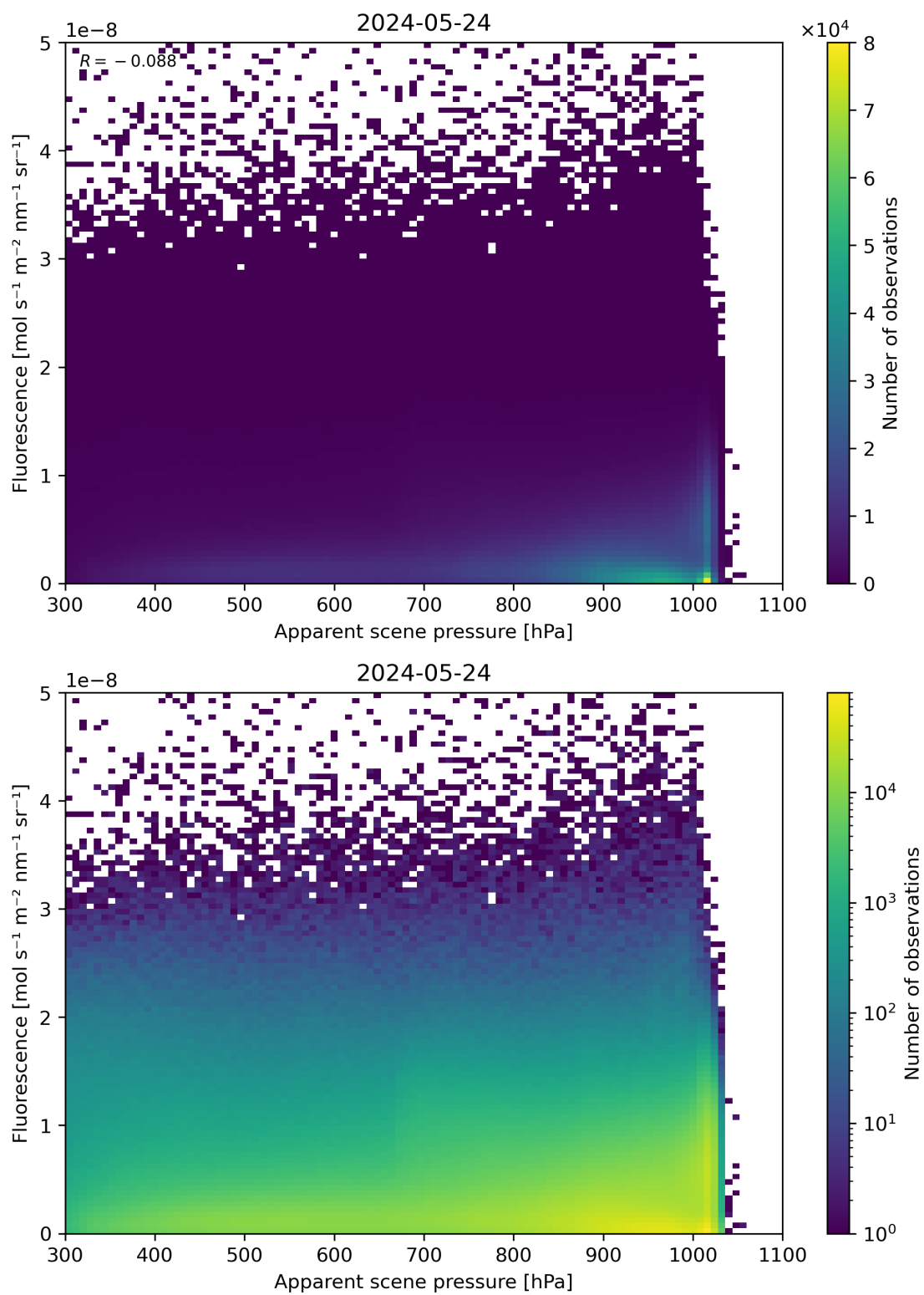
Figure 64: Scatter density plot of “Apparent scene pressure” against “Fluorescence” for 2024-05-23 to 2024-05-25.
