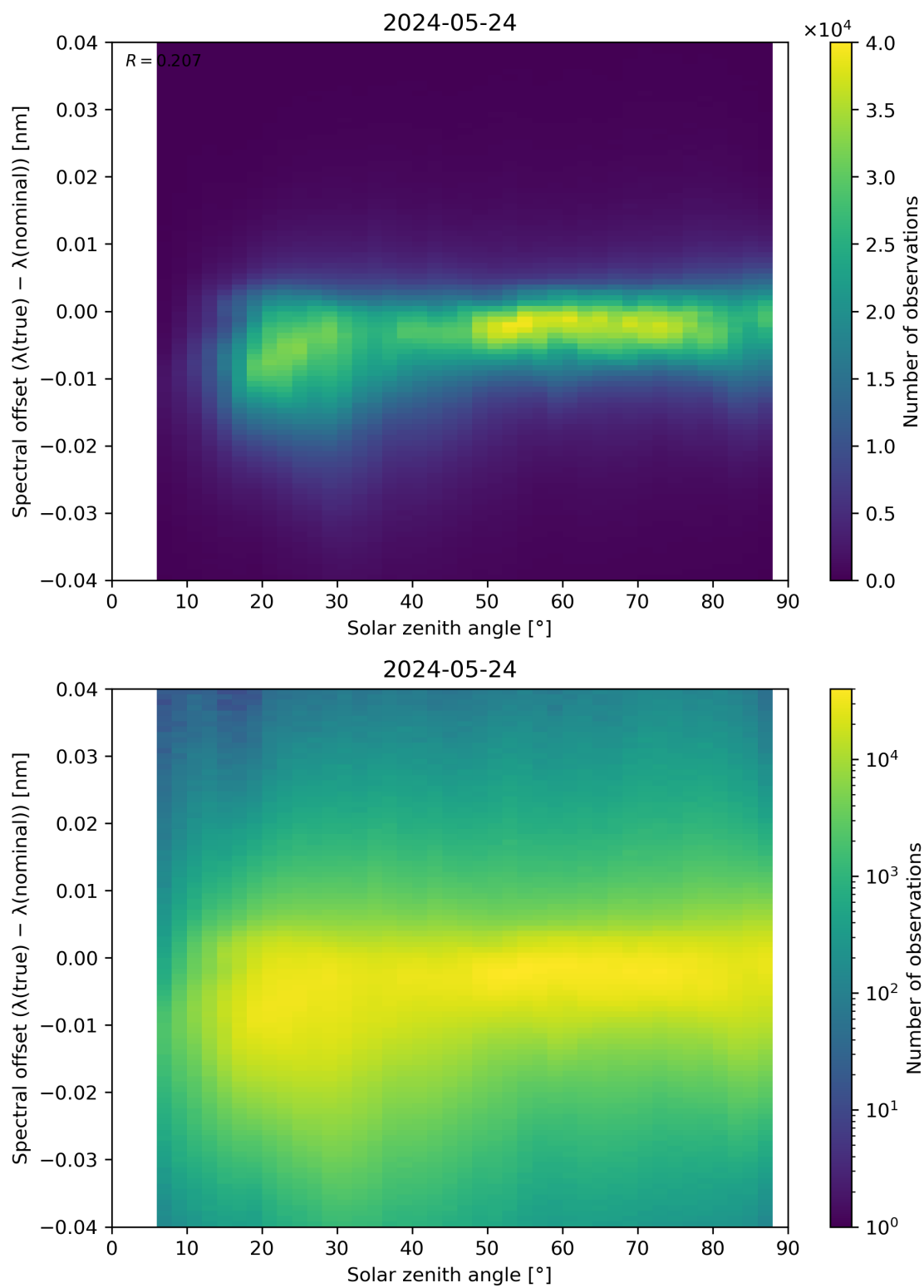
Figure 117: Scatter density plot of “Solar zenith angle” against “Spectral offset ( \lambda(\text{true}) - \lambda(\text{nominal}) )” for 2024-05-23 to 2024-05-25.
