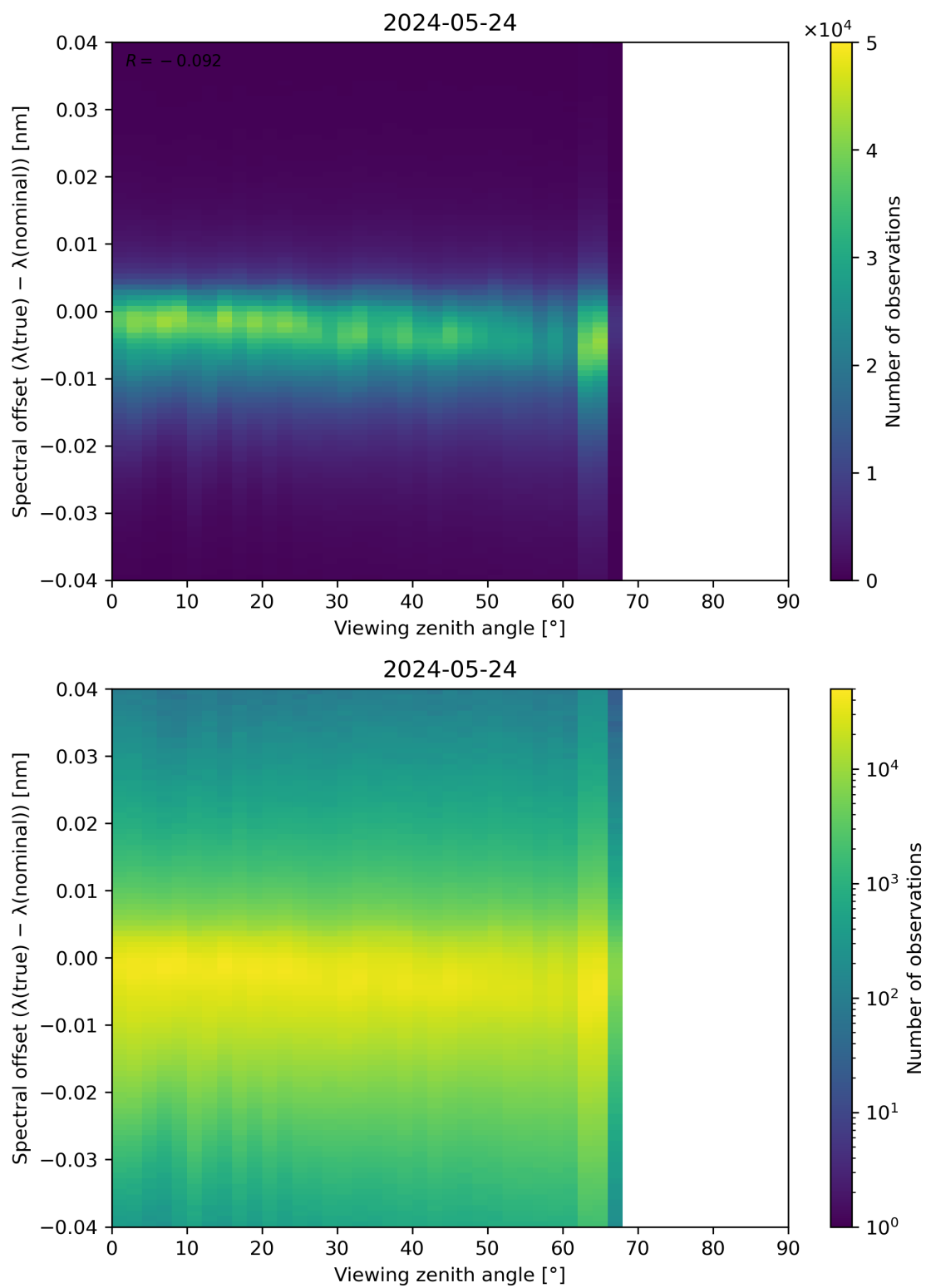
Figure 128: Scatter density plot of “Viewing zenith angle” against “Spectral offset ( \lambda(\text{true}) - \lambda(\text{nominal}) )” for 2024-05-23 to 2024-05-25.
