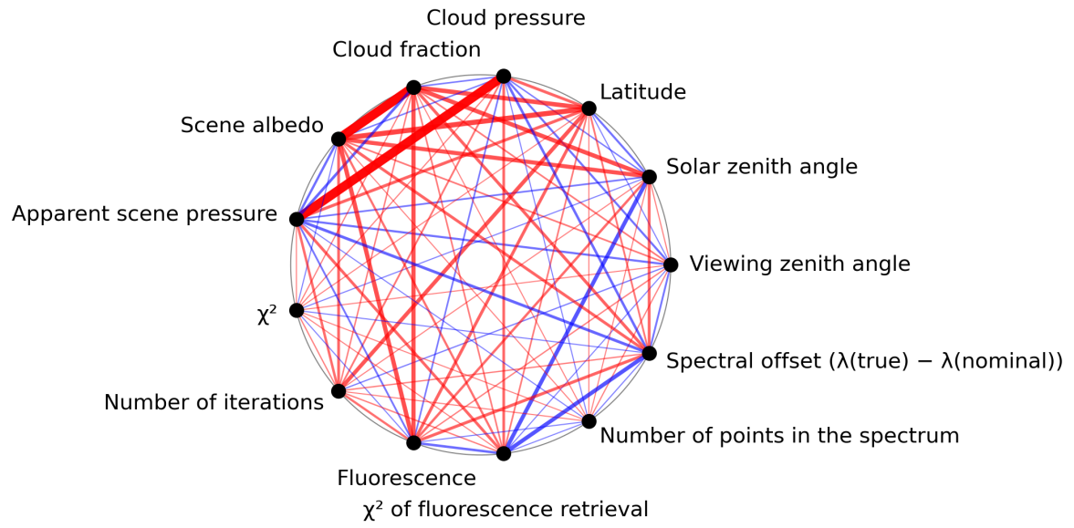
Figure 1: Map of correlation graph for 2024-05-23 to 2024-05-25.
