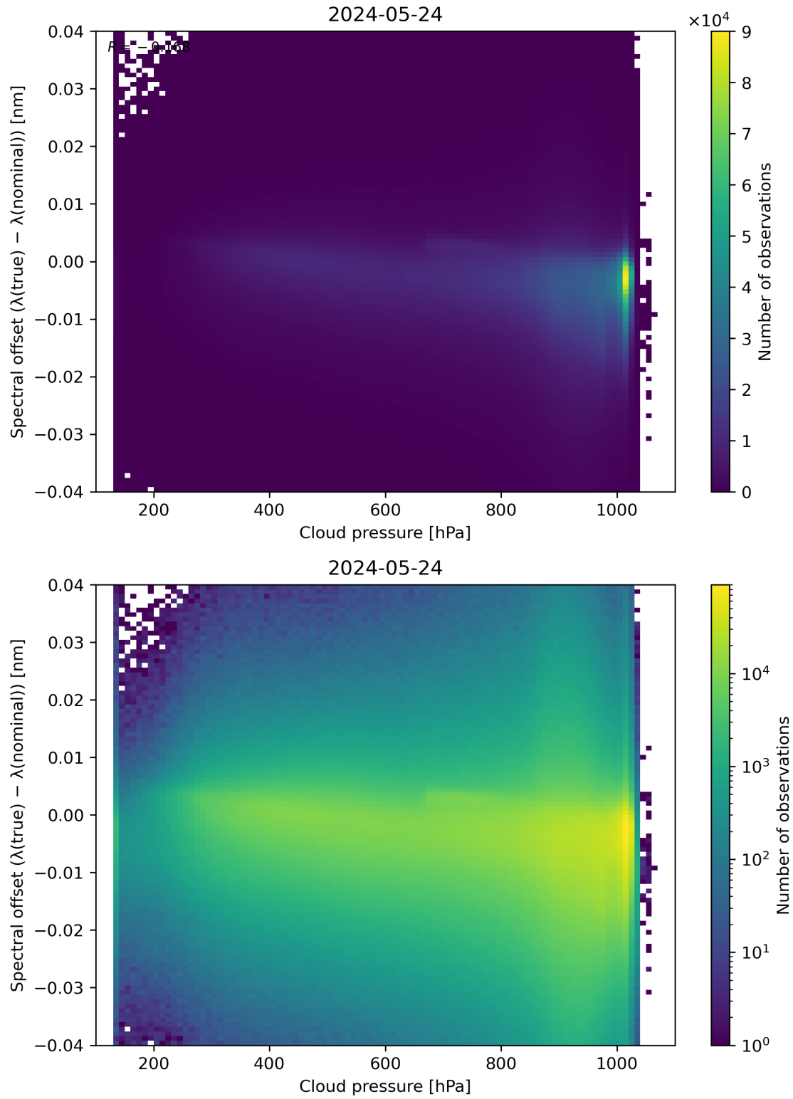
Figure 84: Scatter density plot of “Cloud pressure” against “Spectral offset ( \lambda(\text{true}) - \lambda(\text{nominal}) )” for 2024-05-23 to 2024-05-25.
