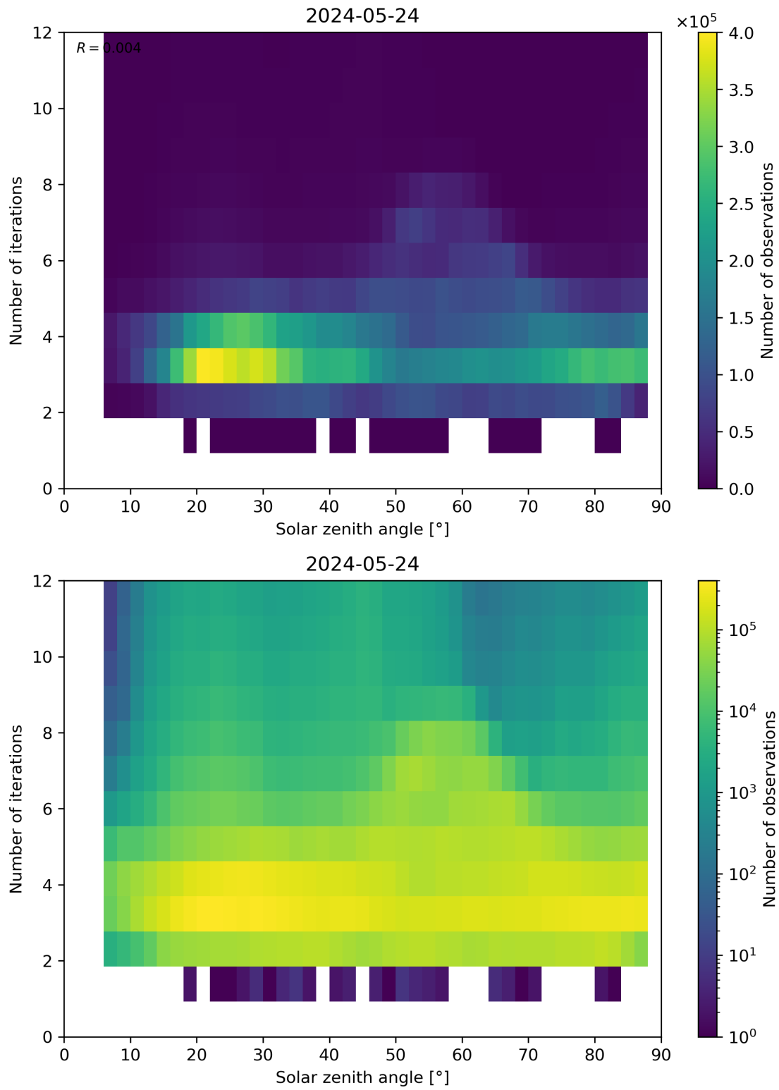
Figure 114: Scatter density plot of “Solar zenith angle” against “Number of iterations” for 2024-05-23 to 2024-05-25.
