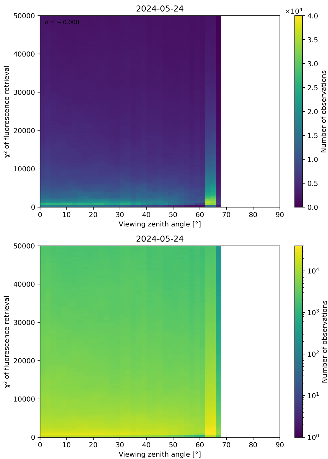
Figure 119: Scatter density plot of “Viewing zenith angle” against “ \chi^2 of fluorescence retrieval” for 2024-05-23 to 2024-05-25.
