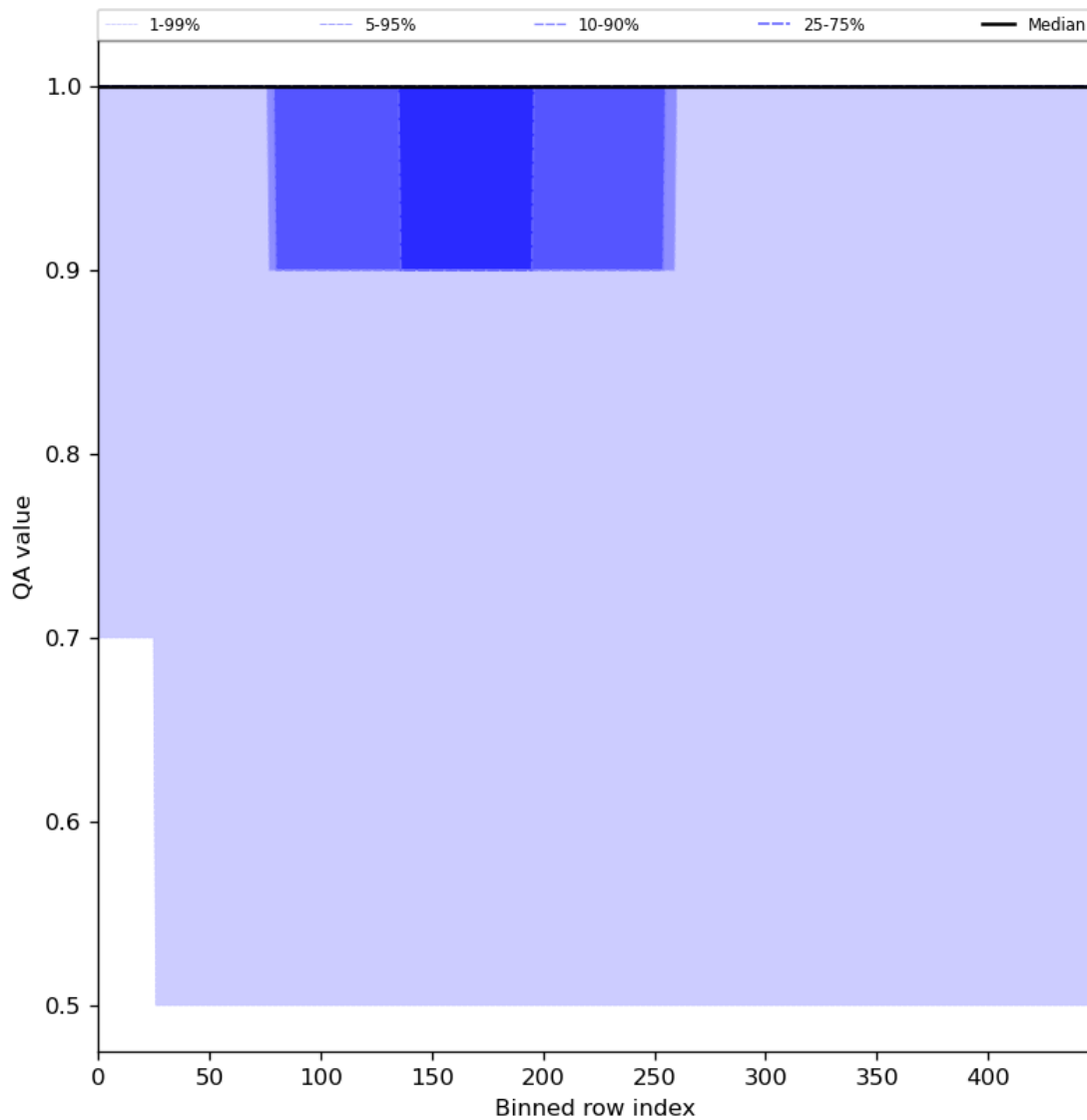
Figure 46: Along track statistics of “QA value” for 2024-05-23 to 2024-05-25
