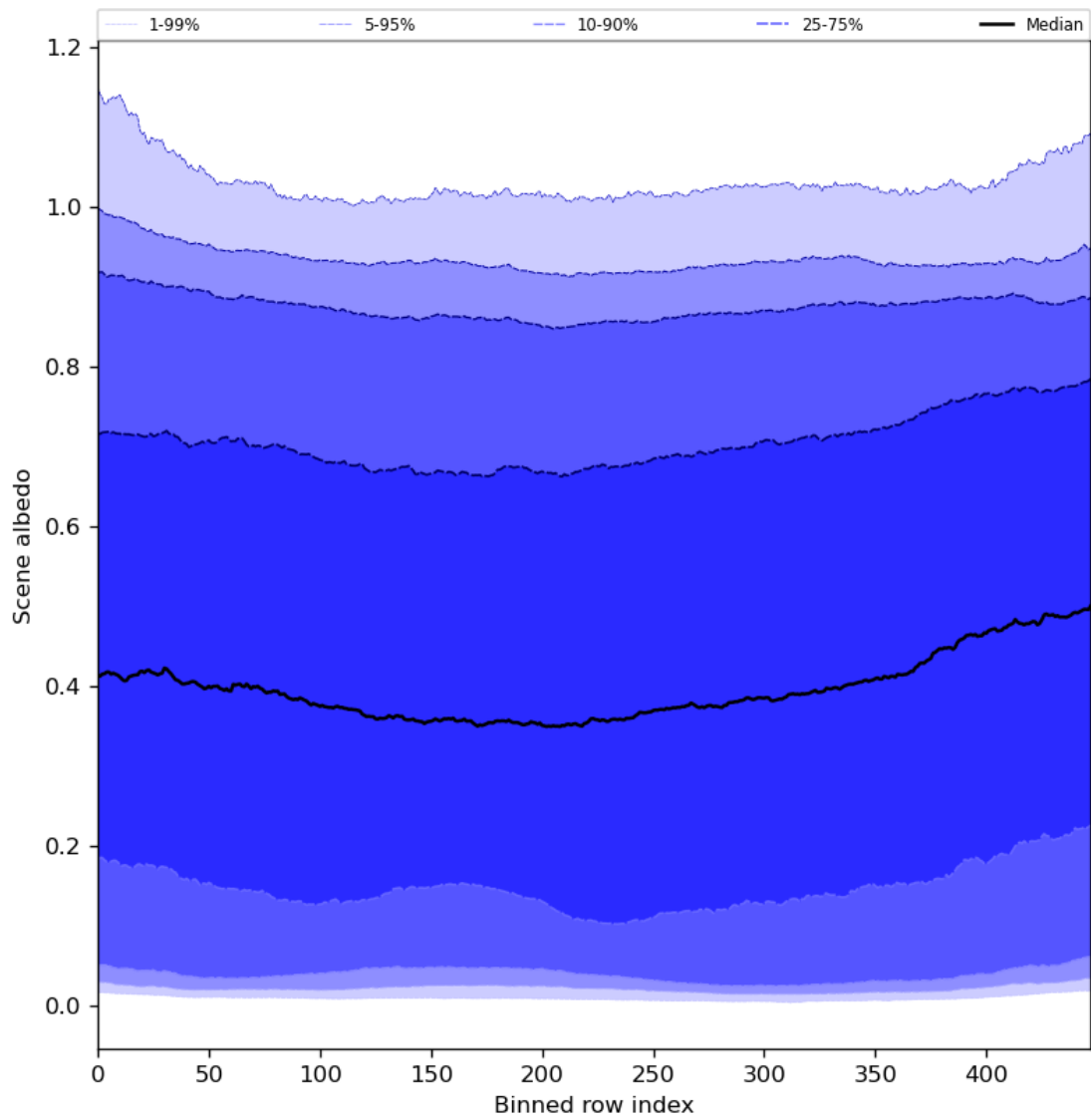
Figure 51: Along track statistics of “Scene albedo” for 2024-05-23 to 2024-05-25
