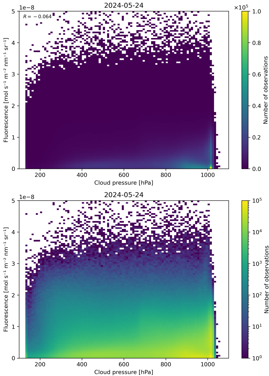
Figure 80: Scatter density plot of “Cloud pressure” against “Fluorescence” for 2024-05-23 to 2024-05-25.
