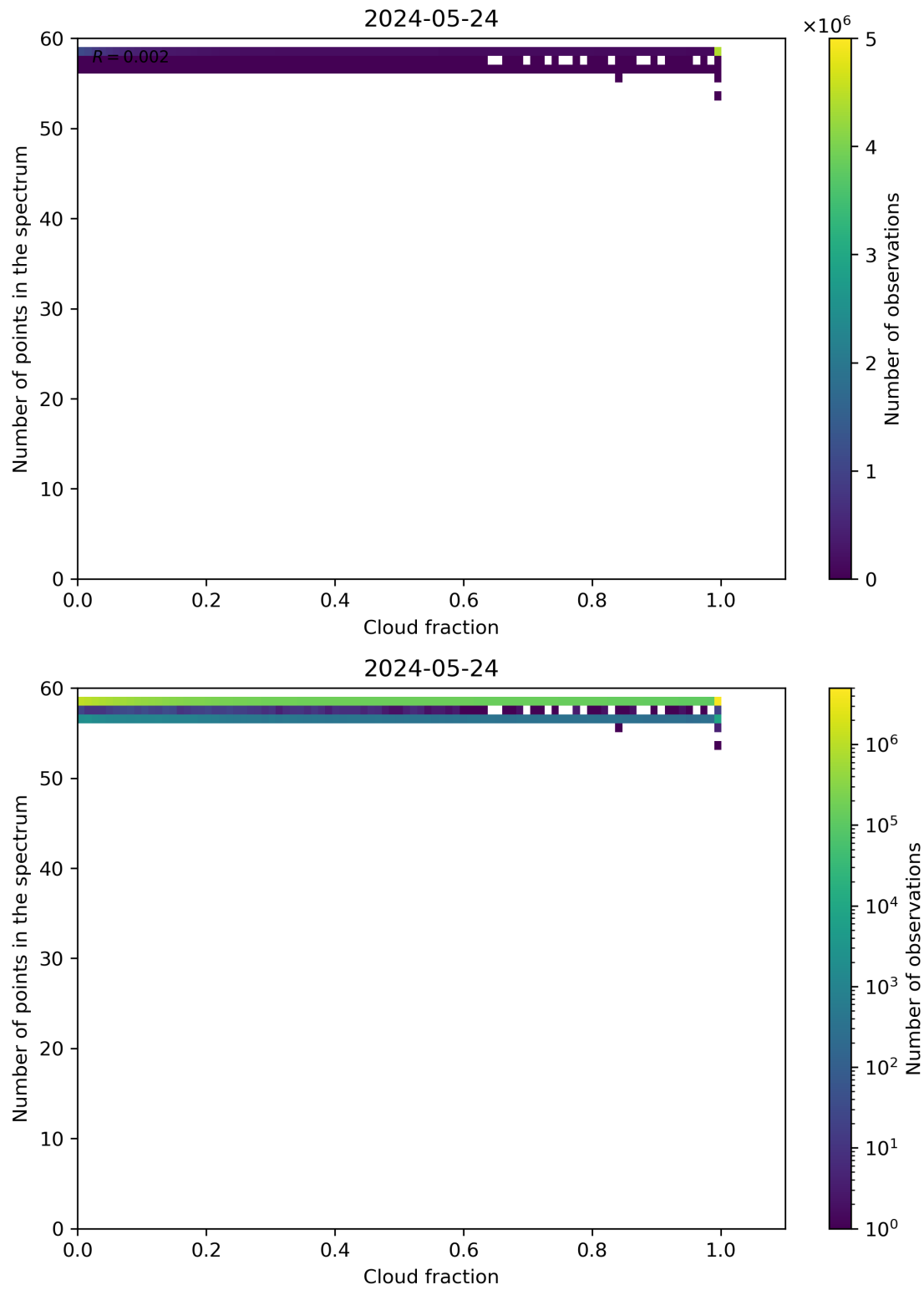
Figure 74: Scatter density plot of “Cloud fraction” against “Number of points in the spectrum” for 2024-05-23 to 2024-05-25.
