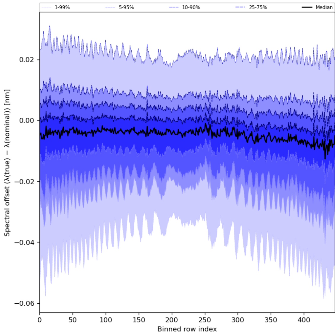
Figure 62: Along track statistics of “Spectral offset ( \lambda(\text{true}) - \lambda(\text{nominal}) )” for 2024-05-23 to 2024-05-25
