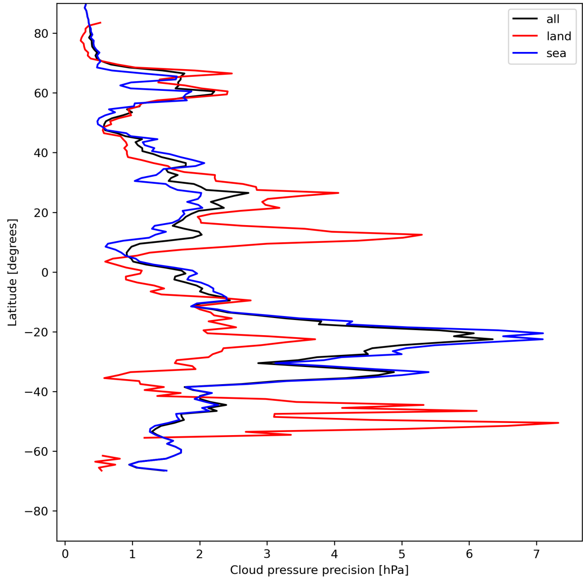
Figure 14: Zonal average of “Cloud pressure precision” for 2024-05-23 to 2024-05-25.
