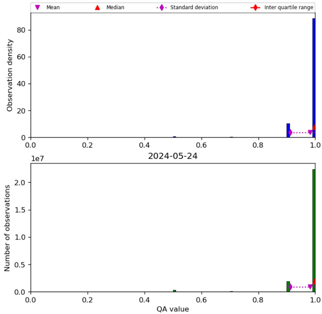
Figure 29: Histogram of “QA value” for 2024-05-23 to 2024-05-25
