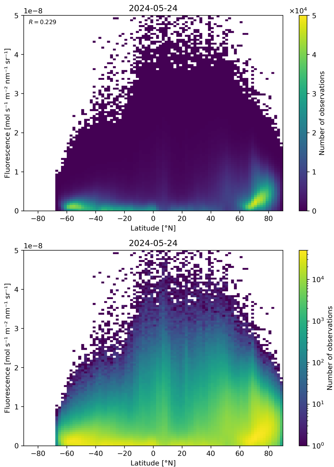
Figure 92: Scatter density plot of “Latitude” against “Fluorescence” for 2024-05-23 to 2024-05-25.
