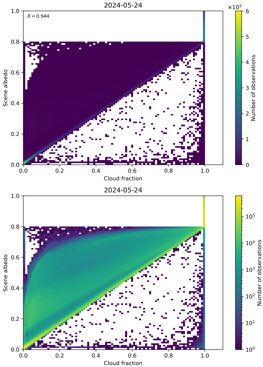
Figure 75: Scatter density plot of “Cloud fraction” against “Scene albedo” for 2024-05-23 to 2024-05-25.
