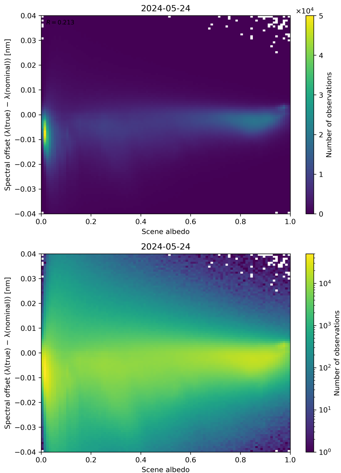
Figure 107: Scatter density plot of “Scene albedo” against “Spectral offset ( \lambda(\text{true}) - \lambda(\text{nominal}) )” for 2024-05-23 to 2024-05-25.
