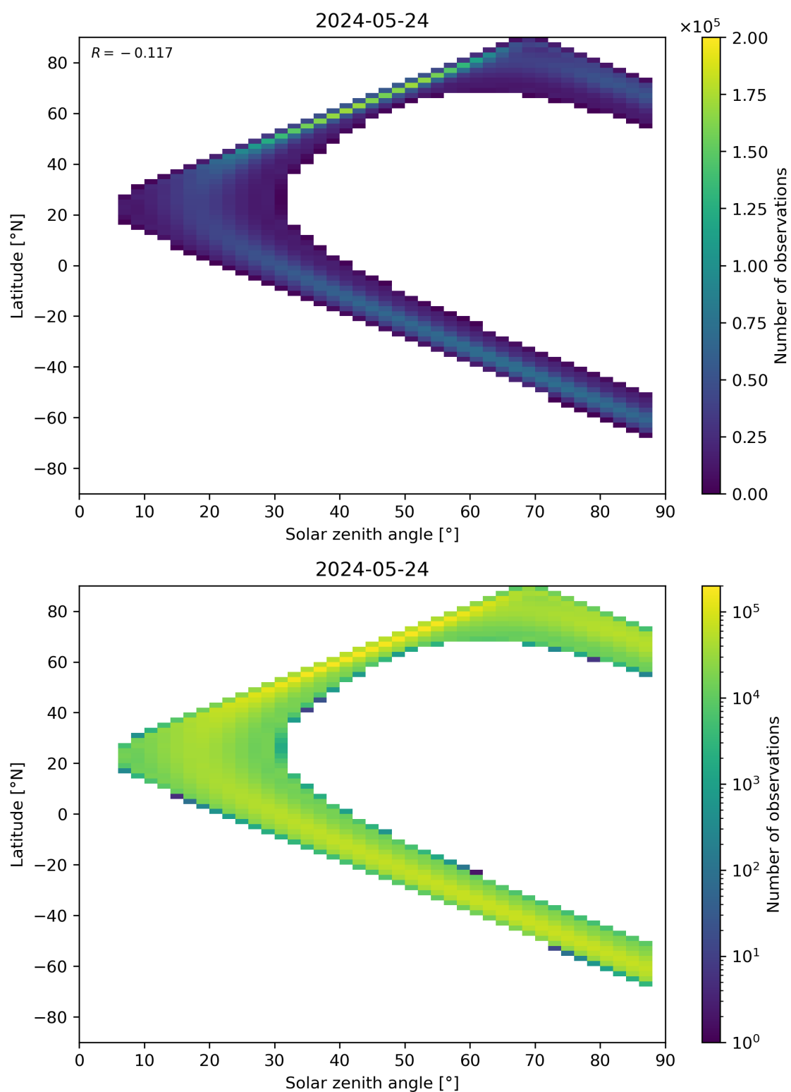
Figure 113: Scatter density plot of “Solar zenith angle” against “Latitude” for 2024-05-23 to 2024-05-25.
