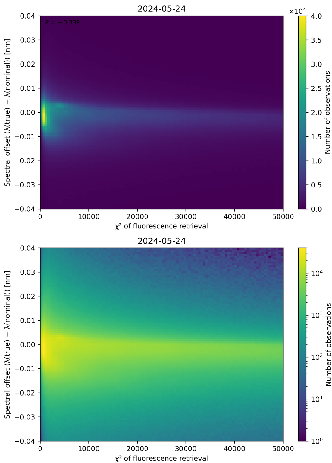
Figure 69: Scatter density plot of " \chi^2 of fluorescence retrieval" against "Spectral offset ( \lambda(\text{true}) - \lambda(\text{nominal})) " for 2024-05-23 to 2024-05-25.
