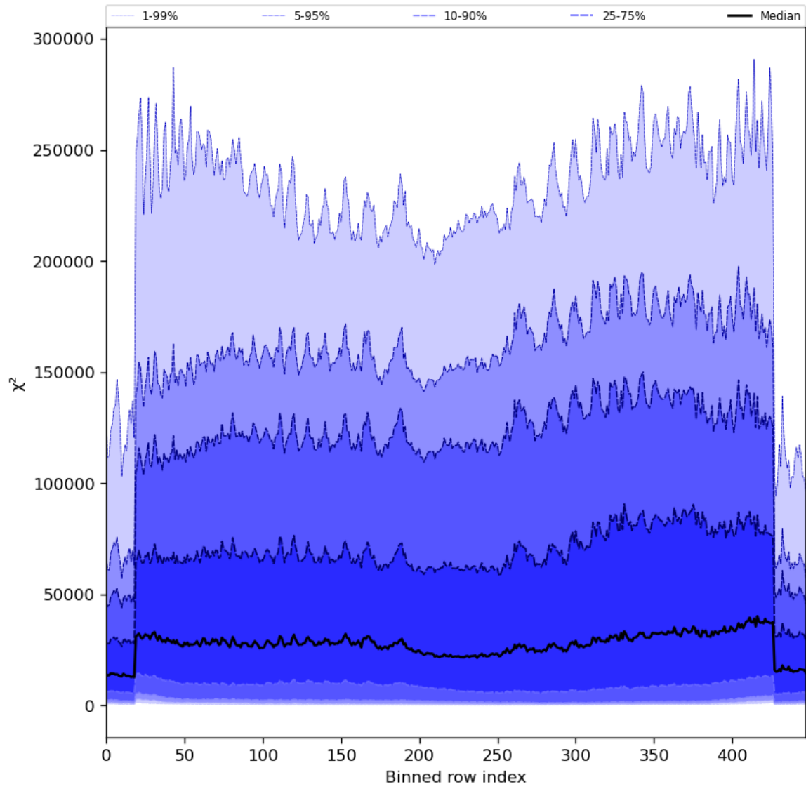
Figure 55: Along track statistics of “ \chi^2 ” for 2024-05-23 to 2024-05-25
