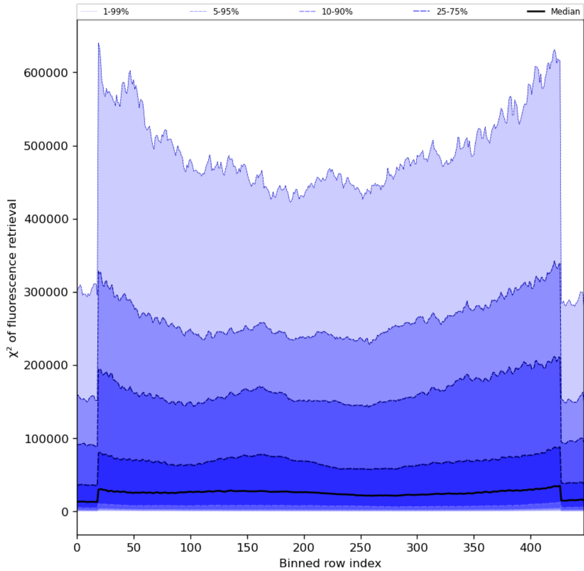
Figure 59: Along track statistics of " \chi^2 of fluorescence retrieval" for 2024-05-23 to 2024-05-25
