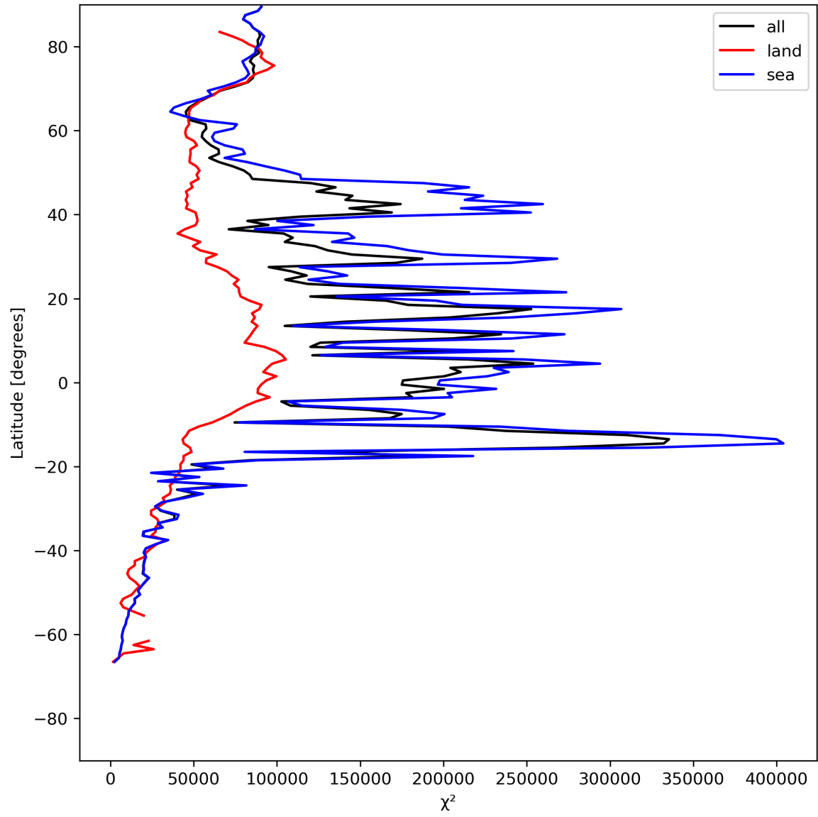
Figure 21: Zonal average of “ \chi^2 ” for 2024-05-23 to 2024-05-25.
