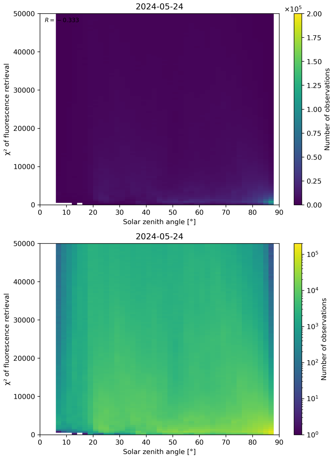
Figure 109: Scatter density plot of “Solar zenith angle” against “ \chi^2 of fluorescence retrieval” for 2024-05-23 to 2024-05-25.
