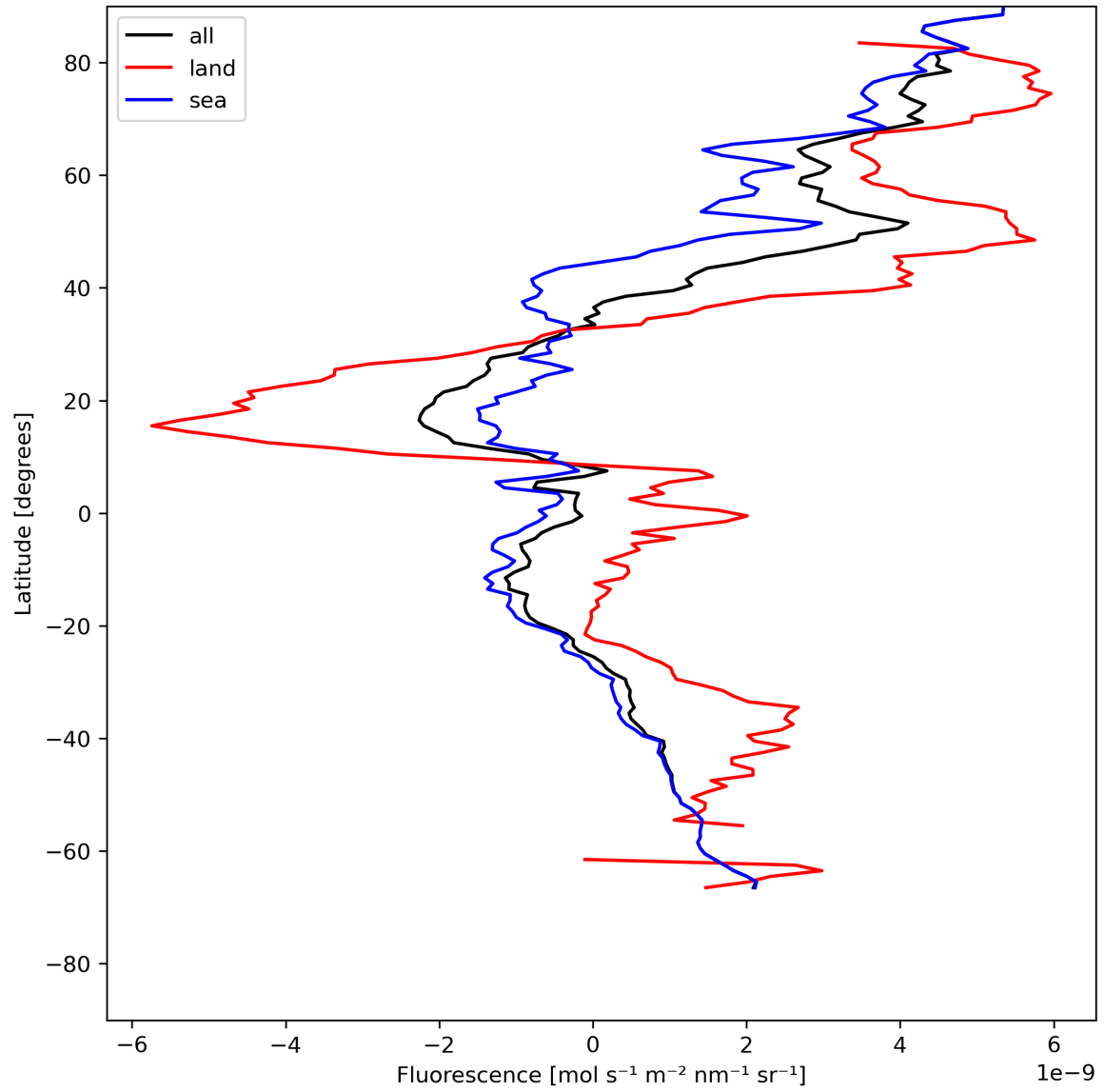
Figure 23: Zonal average of “Fluorescence” for 2024-05-23 to 2024-05-25.
