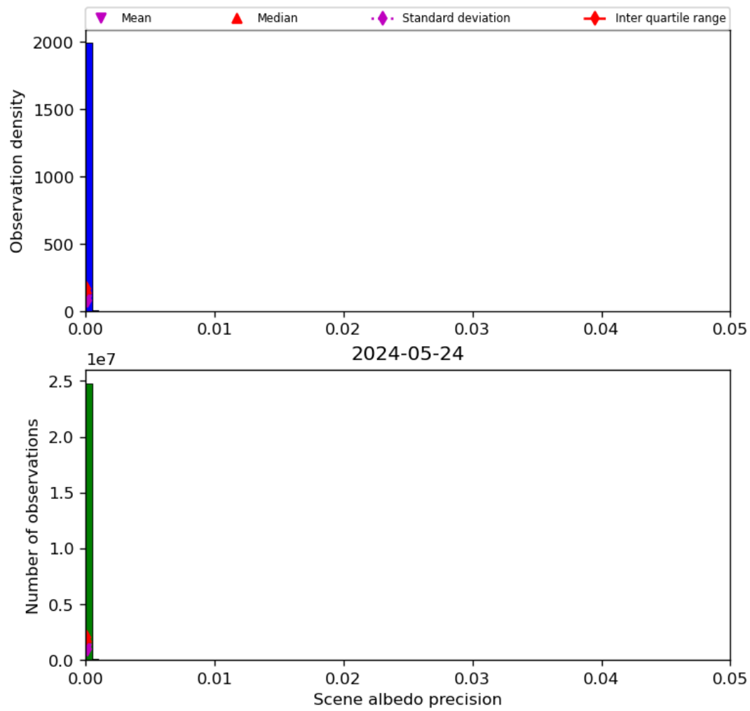
Figure 35: Histogram of “Scene albedo precision” for 2024-05-23 to 2024-05-25
