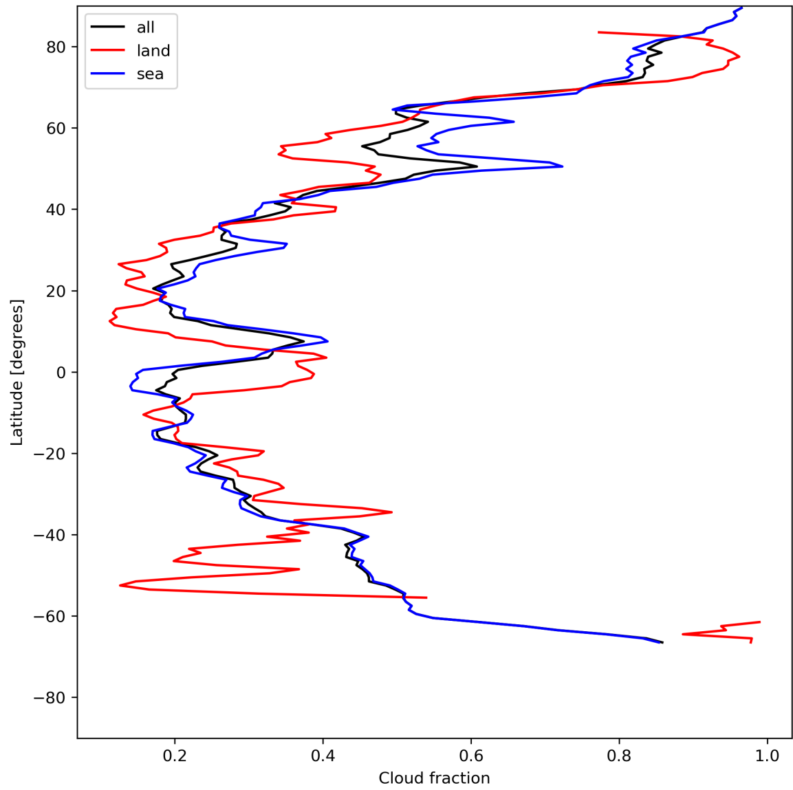
Figure 15: Zonal average of “Cloud fraction” for 2024-05-23 to 2024-05-25.
