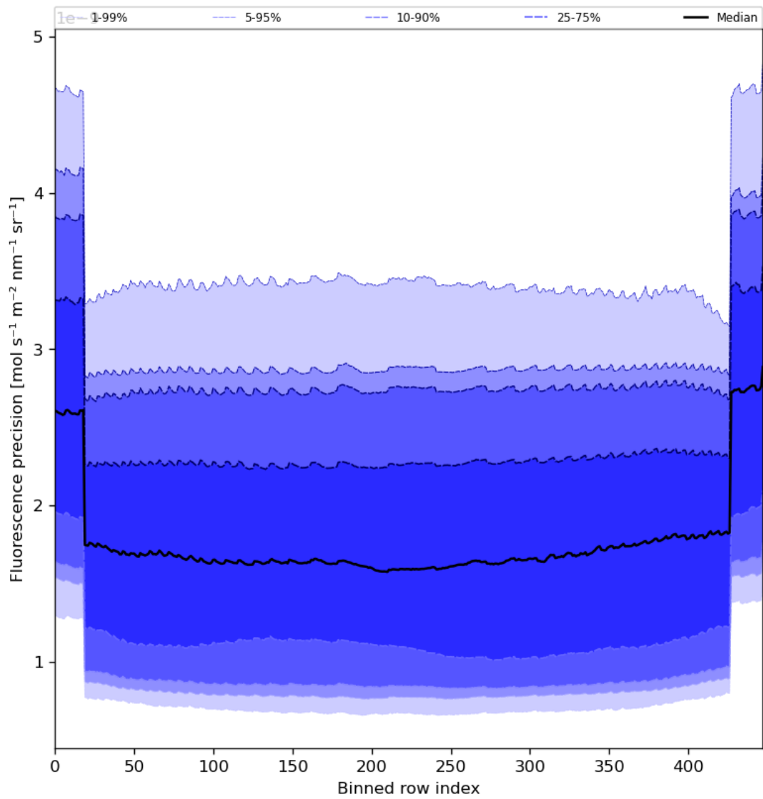
Figure 58: Along track statistics of “Fluorescence precision” for 2024-05-23 to 2024-05-25
