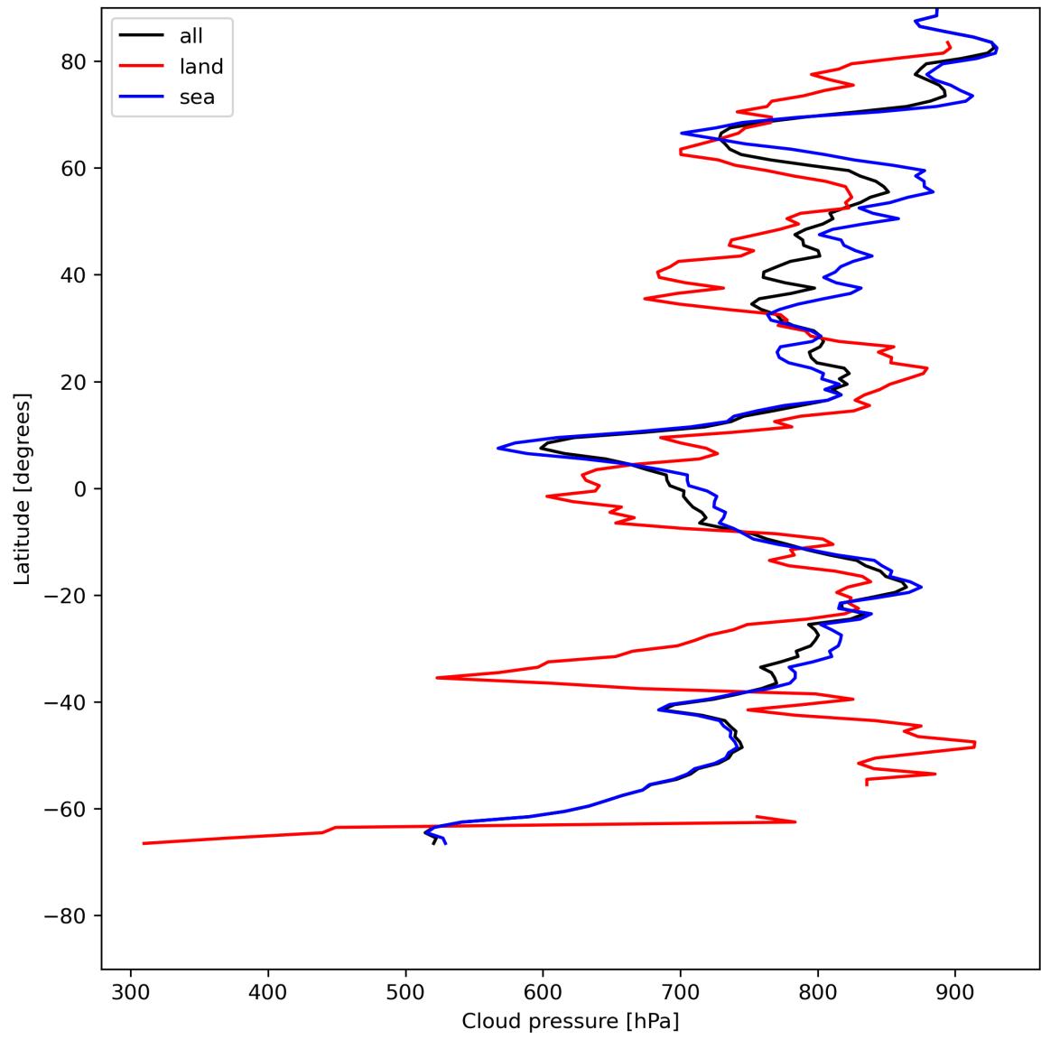
Figure 13: Zonal average of “Cloud pressure” for 2024-05-23 to 2024-05-25.
