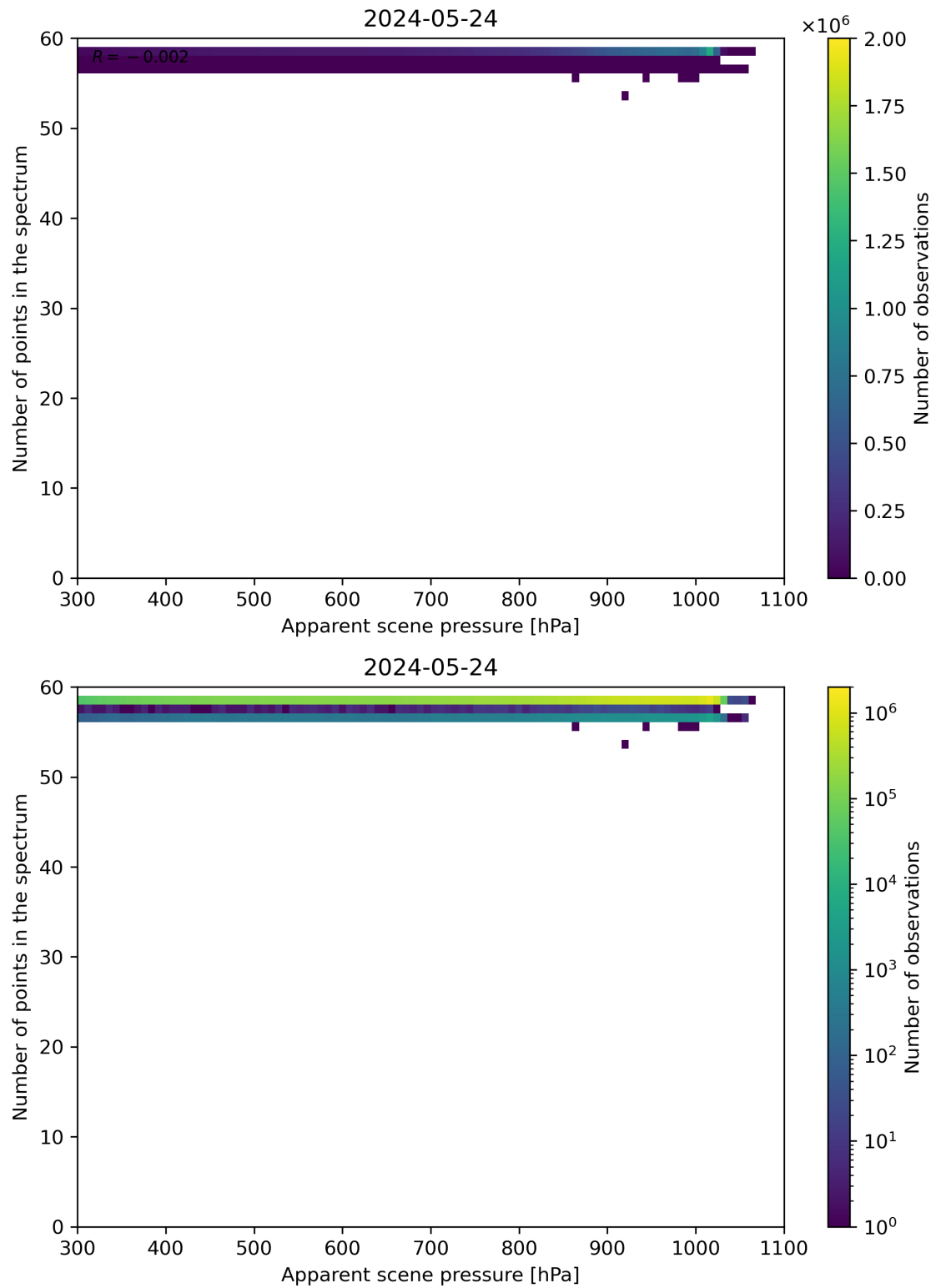
Figure 66: Scatter density plot of “Apparent scene pressure” against “Number of points in the spectrum” for 2024-05-23 to 2024-05-25.
