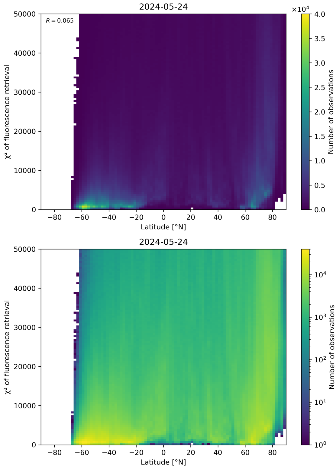
Figure 89: Scatter density plot of “Latitude” against “ \chi^2 of fluorescence retrieval” for 2024-05-23 to 2024-05-25.
