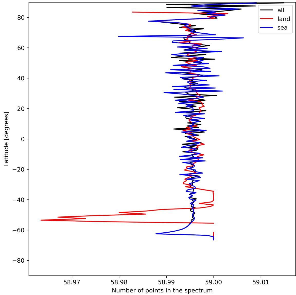
Figure 27: Zonal average of “Number of points in the spectrum” for 2024-05-23 to 2024-05-25.
