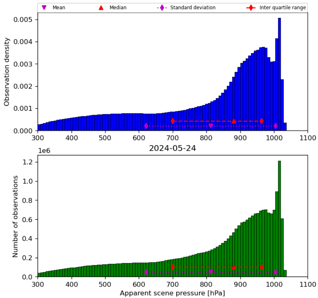
Figure 36: Histogram of “Apparent scene pressure” for 2024-05-23 to 2024-05-25
