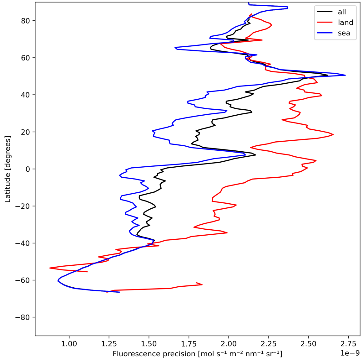
Figure 24: Zonal average of “Fluorescence precision” for 2024-05-23 to 2024-05-25.
