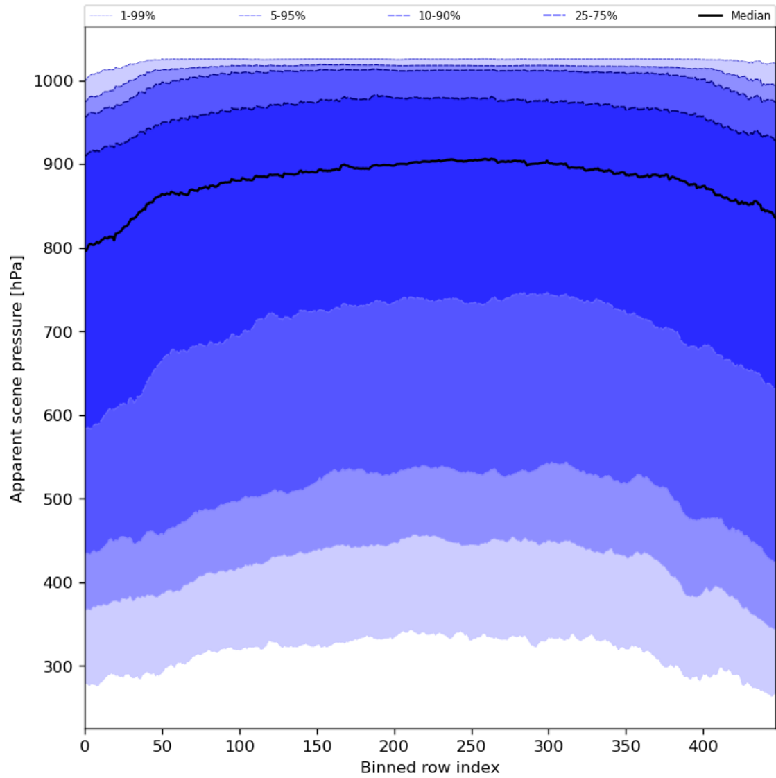
Figure 53: Along track statistics of “Apparent scene pressure” for 2024-05-23 to 2024-05-25
