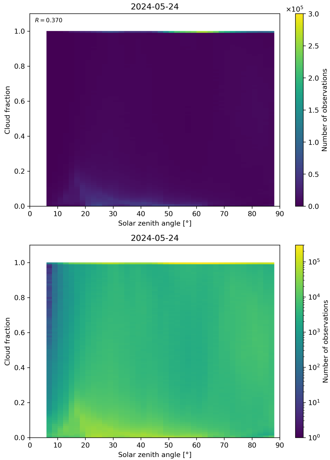
Figure 110: Scatter density plot of “Solar zenith angle” against “Cloud fraction” for 2024-05-23 to 2024-05-25.
