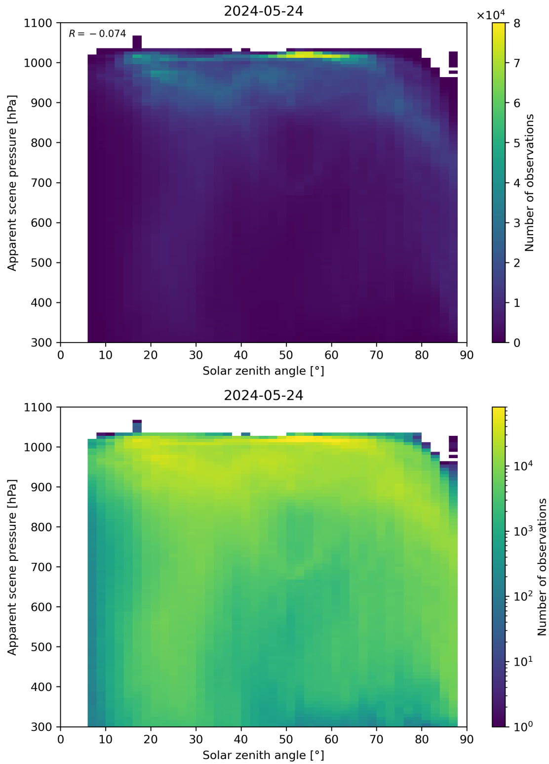
Figure 108: Scatter density plot of “Solar zenith angle” against “Apparent scene pressure” for 2024-05-23 to 2024-05-25.
