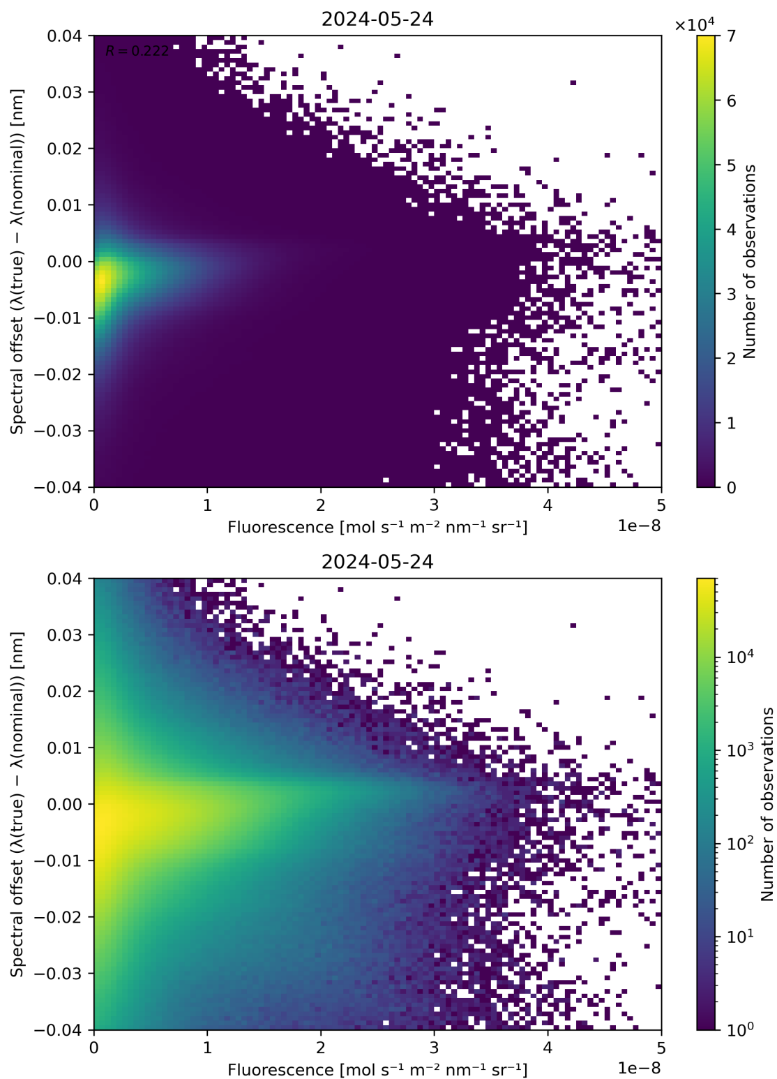
Figure 87: Scatter density plot of “Fluorescence” against “Spectral offset ( \lambda(\text{true}) - \lambda(\text{nominal}) )” for 2024-05-23 to 2024-05-25.
