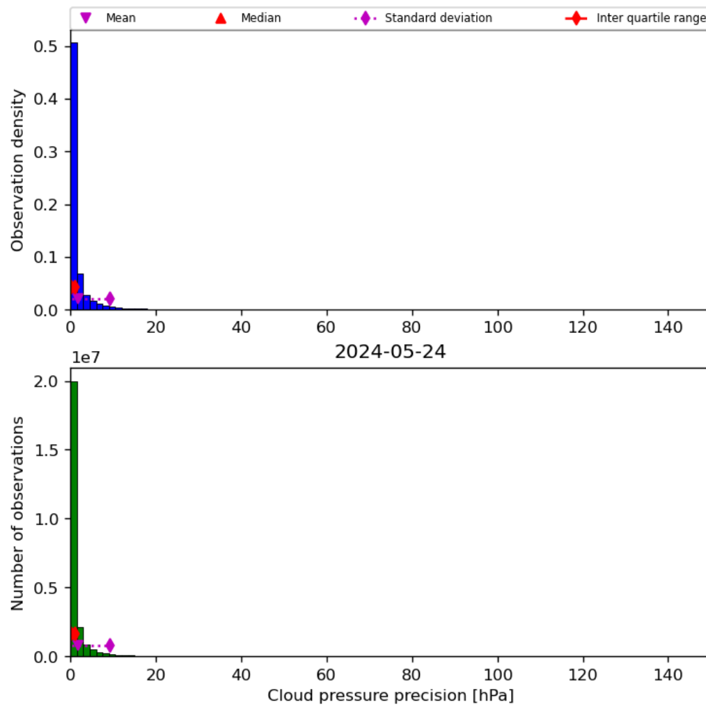
Figure 31: Histogram of “Cloud pressure precision” for 2024-05-23 to 2024-05-25
