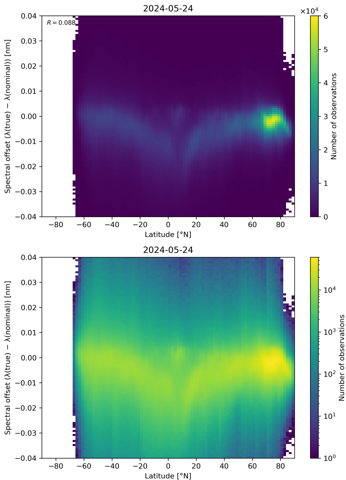
Figure 96: Scatter density plot of “Latitude” against “Spectral offset ( \lambda(\text{true}) - \lambda(\text{nominal}) )” for 2024-05-23 to 2024-05-25.
