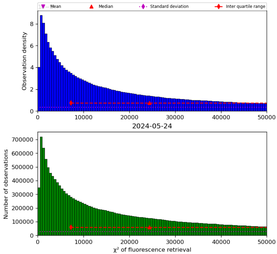
Figure 42: Histogram of “ \chi^2 of fluorescence retrieval” for 2024-05-23 to 2024-05-25
