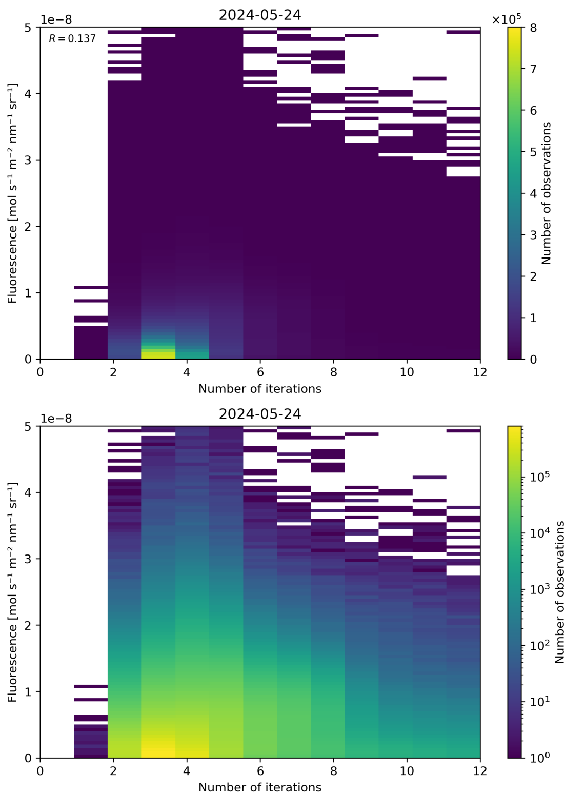
Figure 98: Scatter density plot of “Number of iterations” against “Fluorescence” for 2024-05-23 to 2024-05-25.
