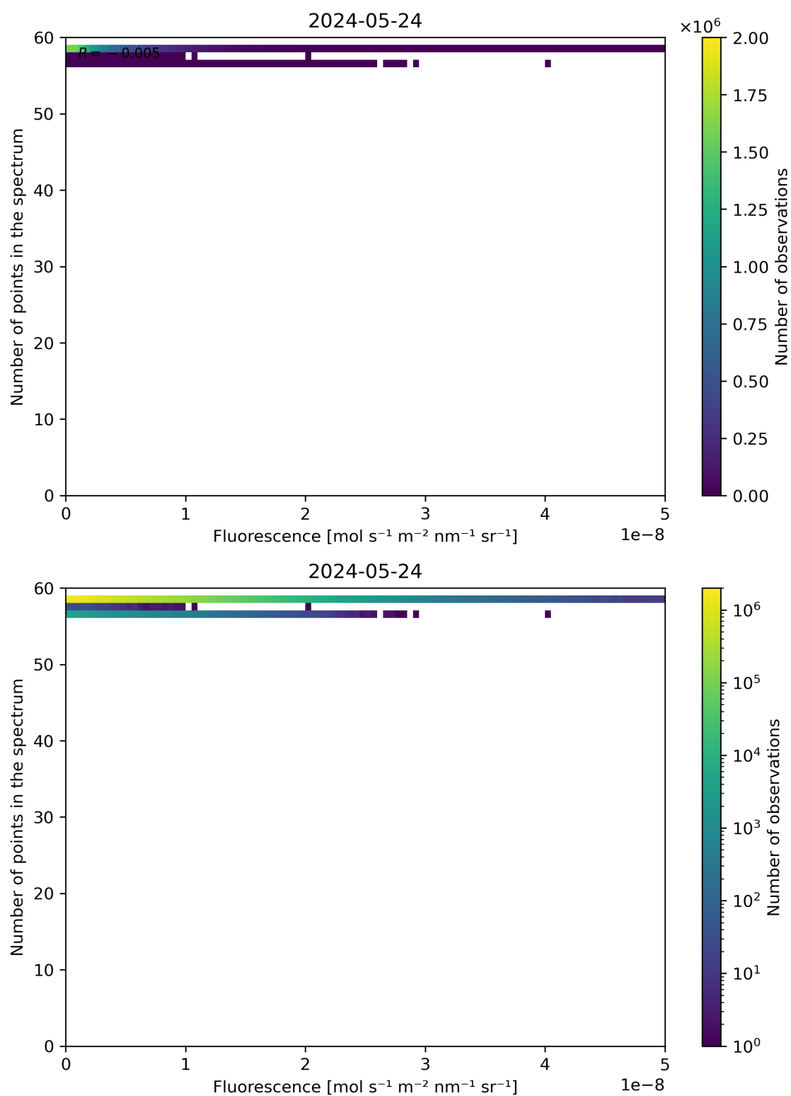
Figure 86: Scatter density plot of “Fluorescence” against “Number of points in the spectrum” for 2024-05-23 to 2024-05-25.
