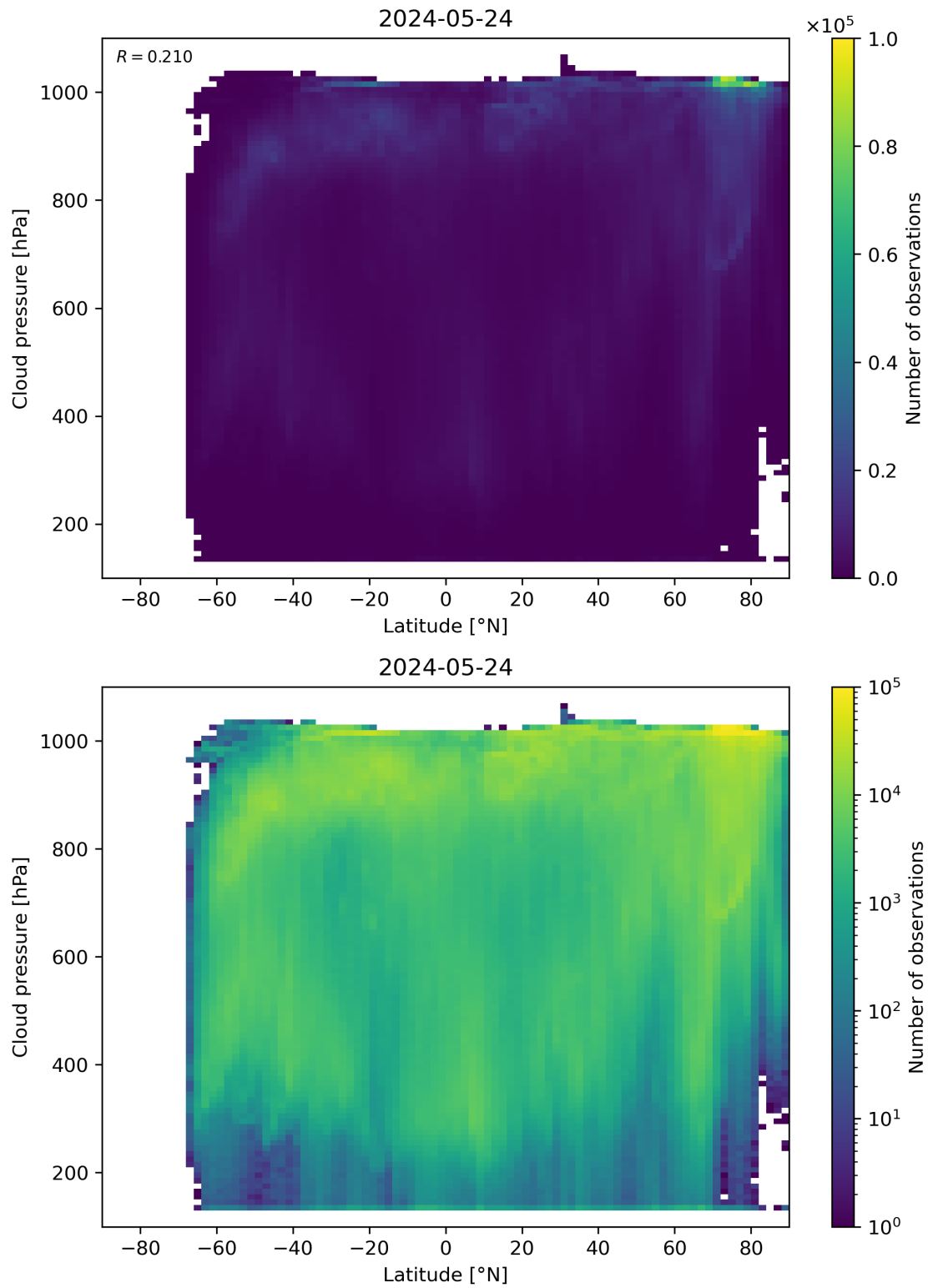
Figure 91: Scatter density plot of “Latitude” against “Cloud pressure” for 2024-05-23 to 2024-05-25.
