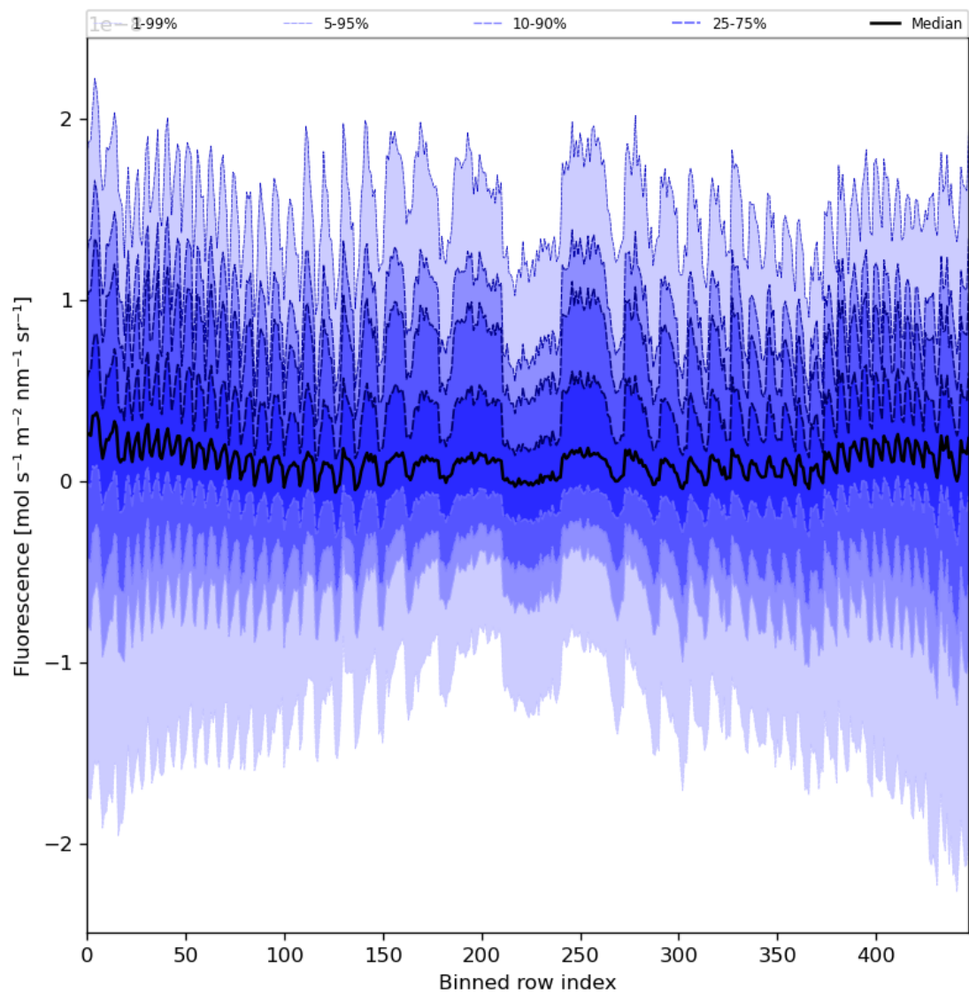
Figure 57: Along track statistics of “Fluorescence” for 2024-05-23 to 2024-05-25
