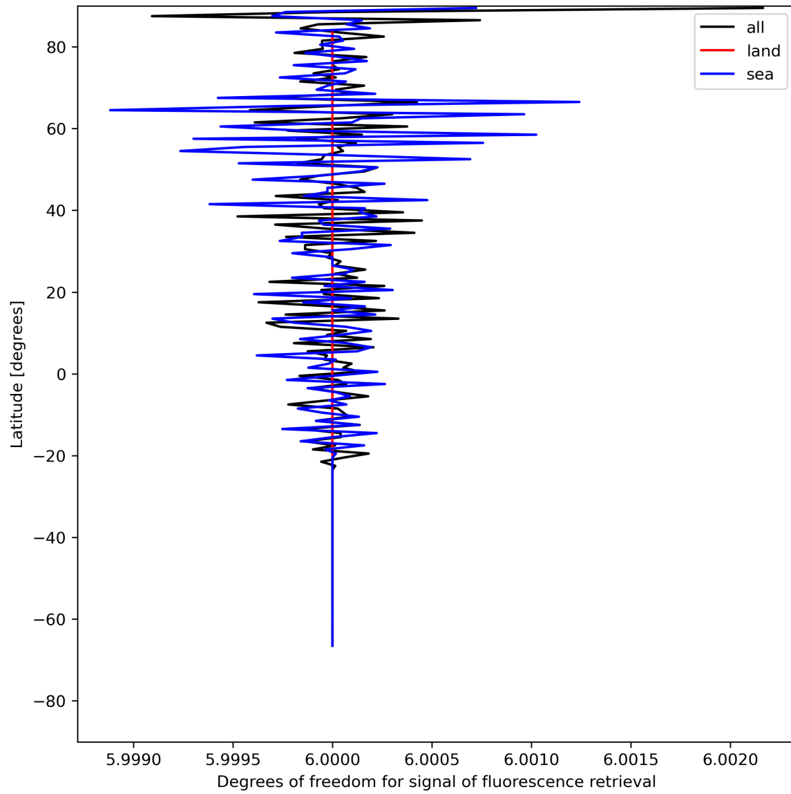
Figure 26: Zonal average of “Degrees of freedom for signal of fluorescence retrieval” for 2024-05-23 to 2024-05-25.
