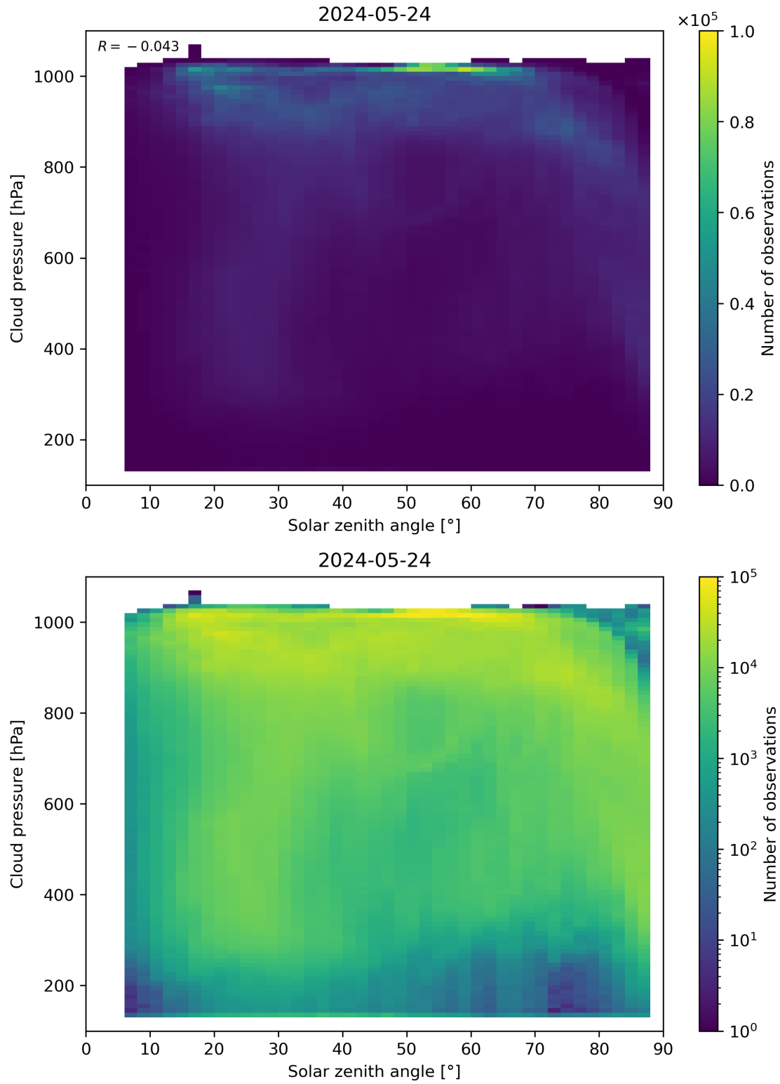
Figure 111: Scatter density plot of “Solar zenith angle” against “Cloud pressure” for 2024-05-23 to 2024-05-25.
