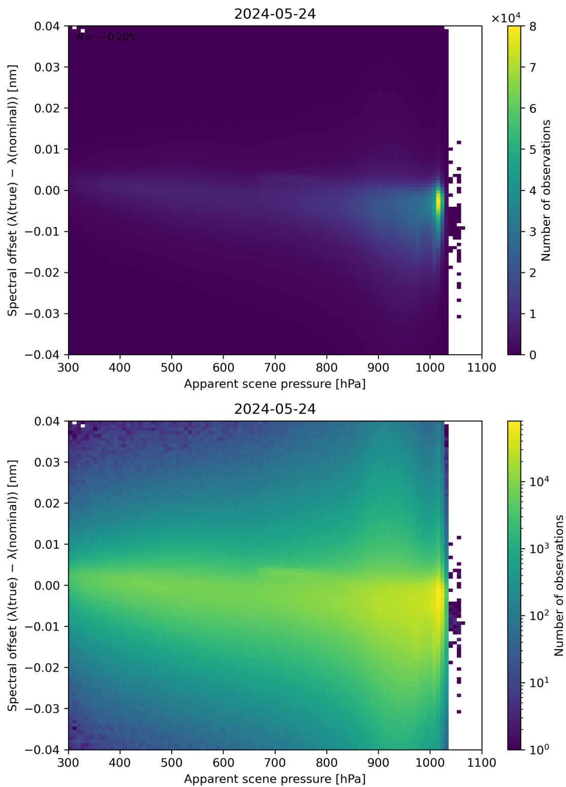
Figure 67: Scatter density plot of “Apparent scene pressure” against “Spectral offset ( \lambda(\text{true}) - \lambda(\text{nominal}) )” for 2024-05-23 to 2024-05-25.
