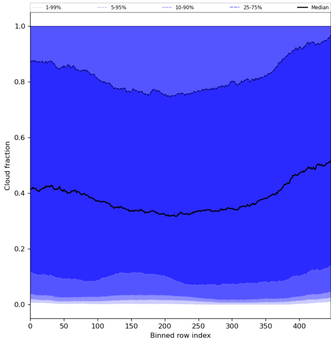
Figure 49: Along track statistics of “Cloud fraction” for 2024-05-23 to 2024-05-25
