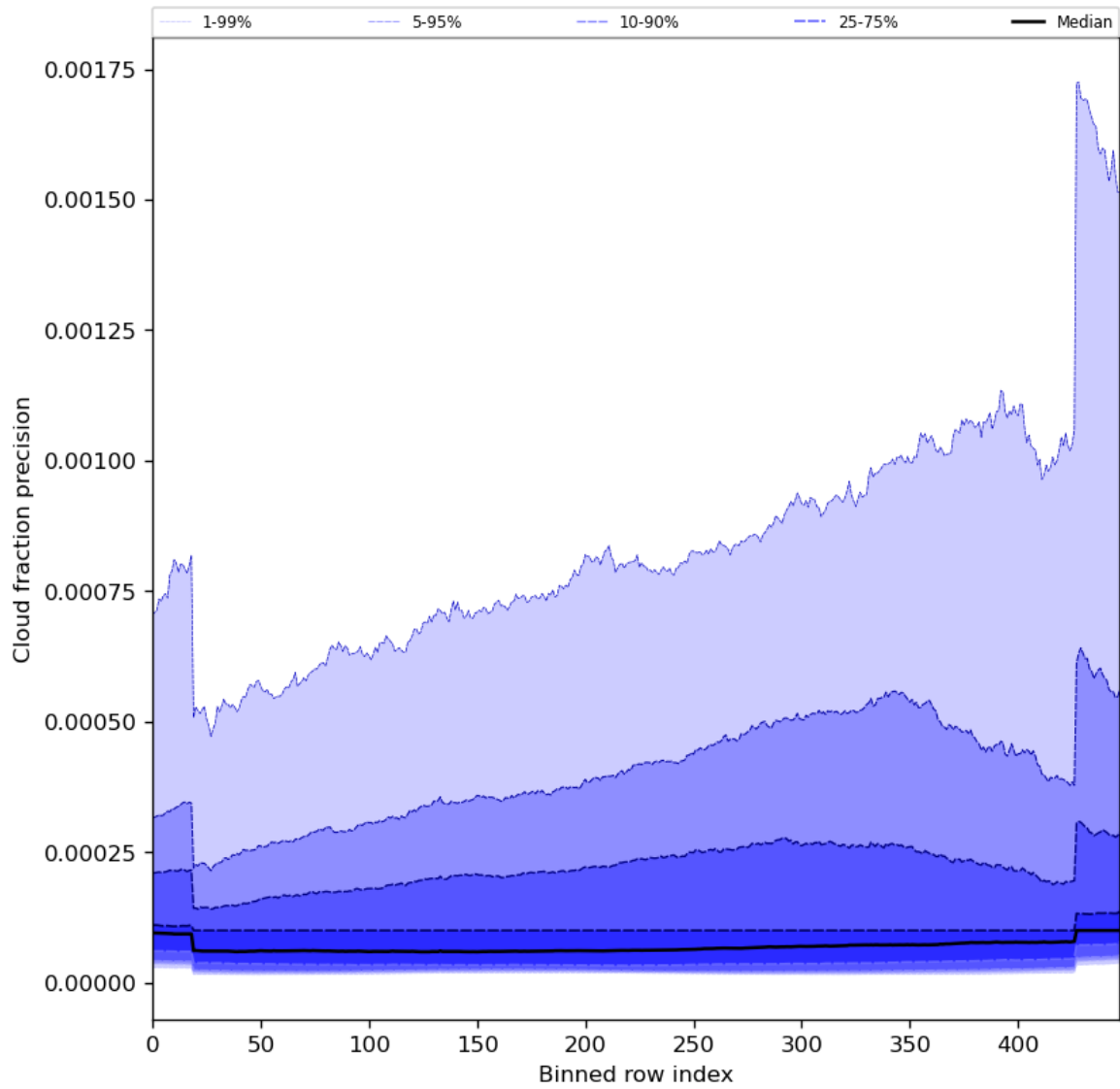
Figure 50: Along track statistics of “Cloud fraction precision” for 2024-05-23 to 2024-05-25
