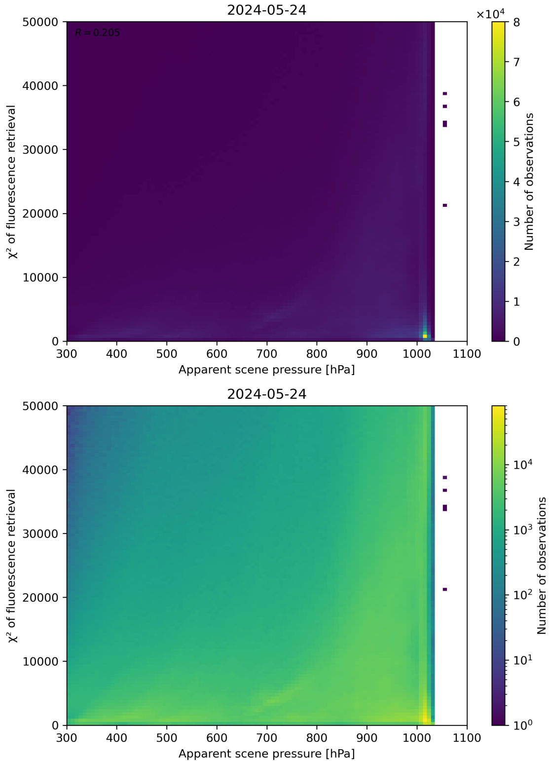
Figure 63: Scatter density plot of “Apparent scene pressure” against “ \chi^2 of fluorescence retrieval” for 2024-05-23 to 2024-05-25.
