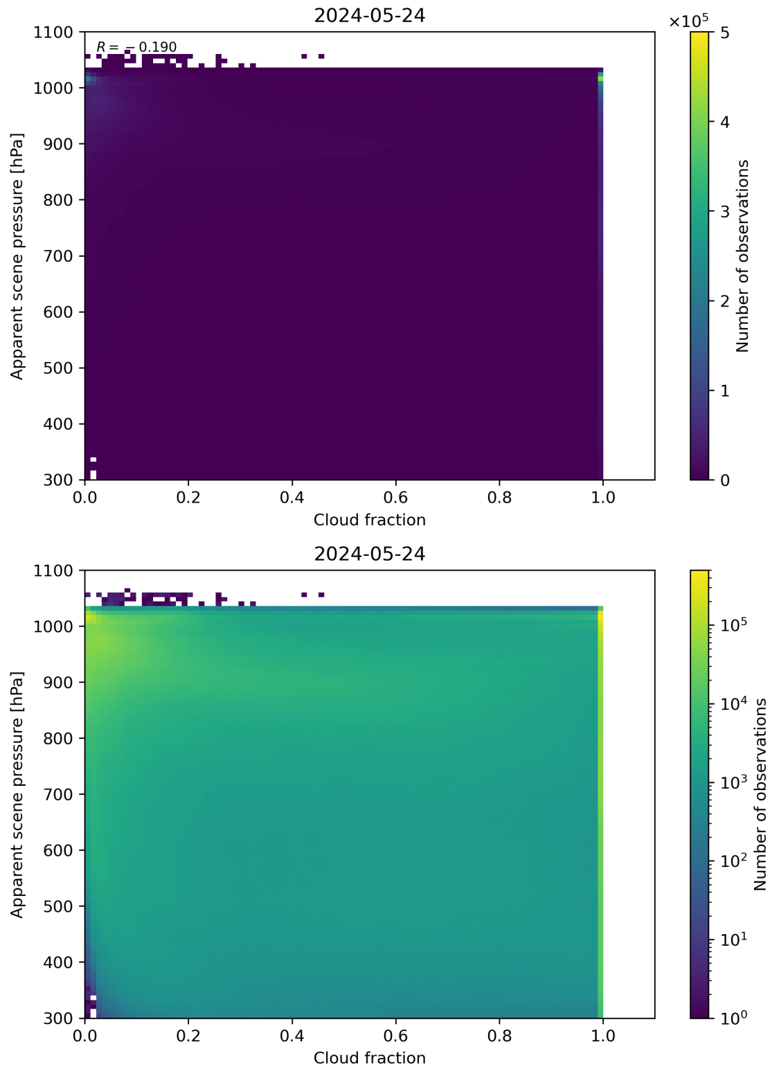
Figure 70: Scatter density plot of “Cloud fraction” against “Apparent scene pressure” for 2024-05-23 to 2024-05-25.
