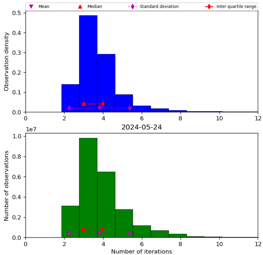
Figure 39: Histogram of “Number of iterations” for 2024-05-23 to 2024-05-25
