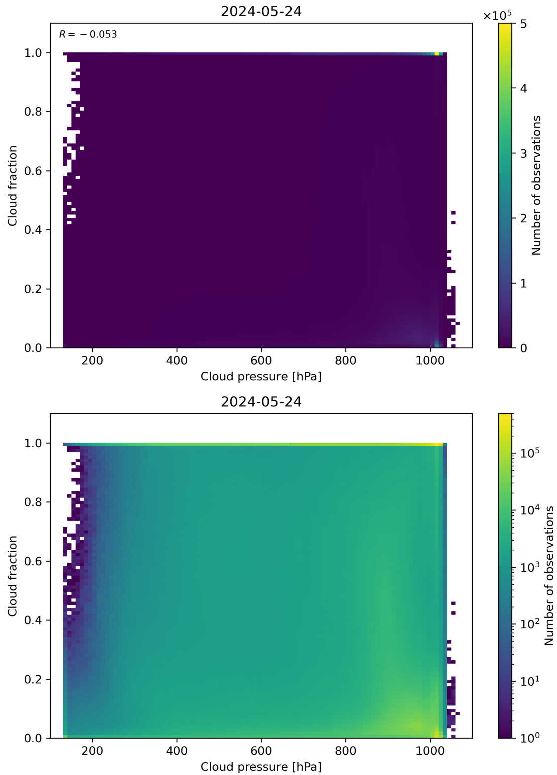
Figure 79: Scatter density plot of “Cloud pressure” against “Cloud fraction” for 2024-05-23 to 2024-05-25.
