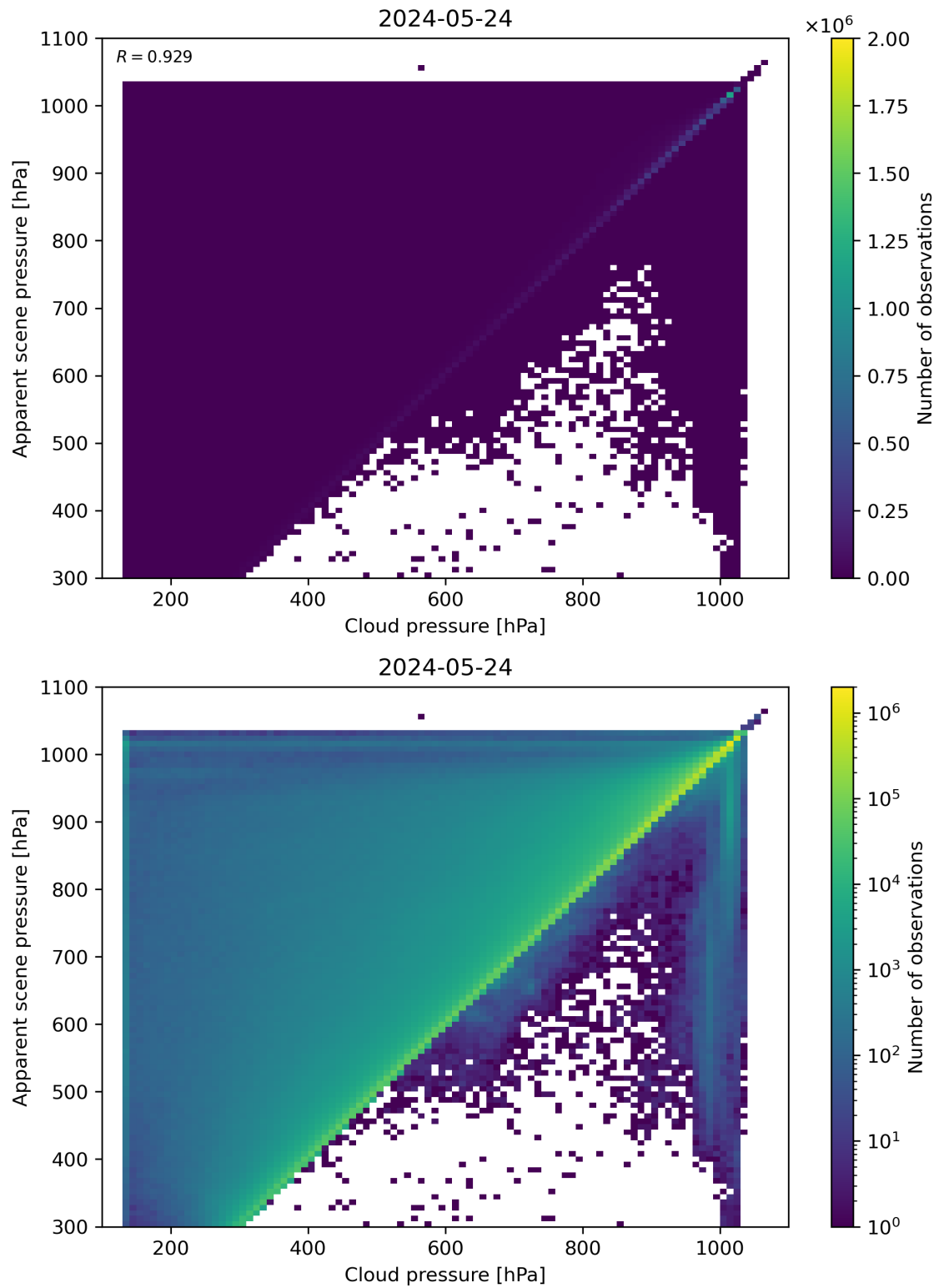
Figure 77: Scatter density plot of “Cloud pressure” against “Apparent scene pressure” for 2024-05-23 to 2024-05-25.
