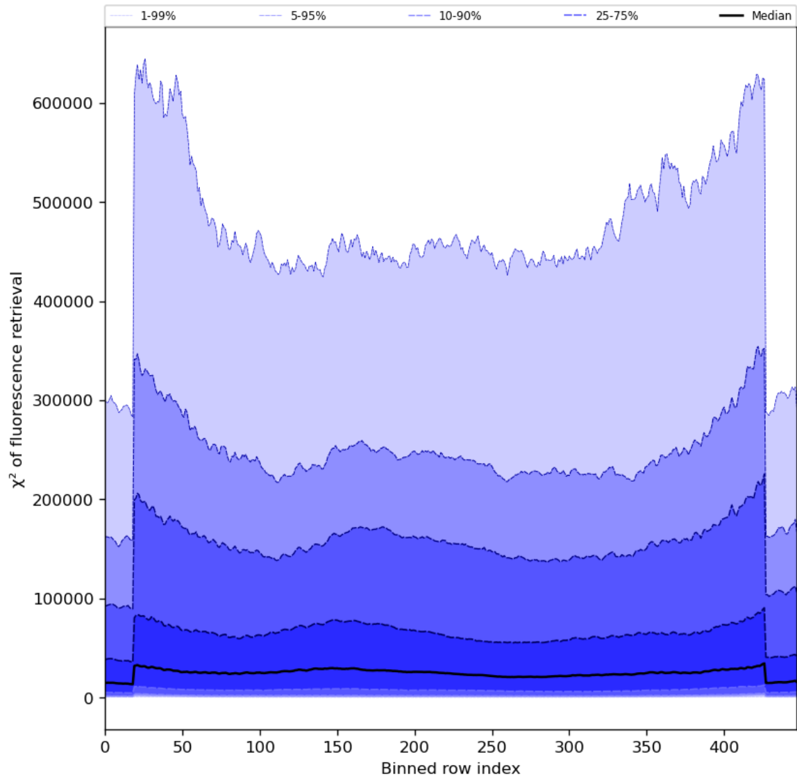
Figure 59: Along track statistics of “ \chi^2 of fluorescence retrieval” for 2024-05-24 to 2024-05-26
