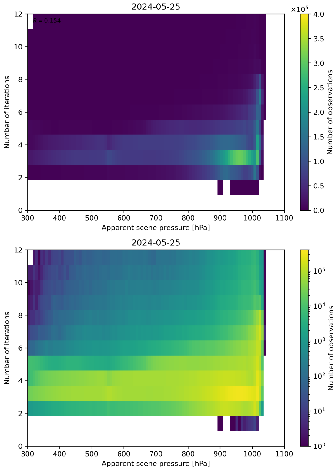
Figure 65: Scatter density plot of “Apparent scene pressure” against “Number of iterations” for 2024-05-24 to 2024-05-26.
