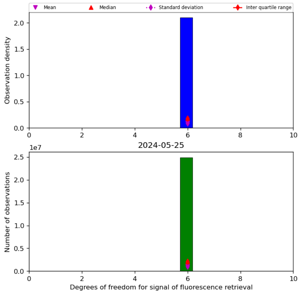
Figure 43: Histogram of "Degrees of freedom for signal of fluorescence retrieval" for 2024-05-24 to 2024-05-26
