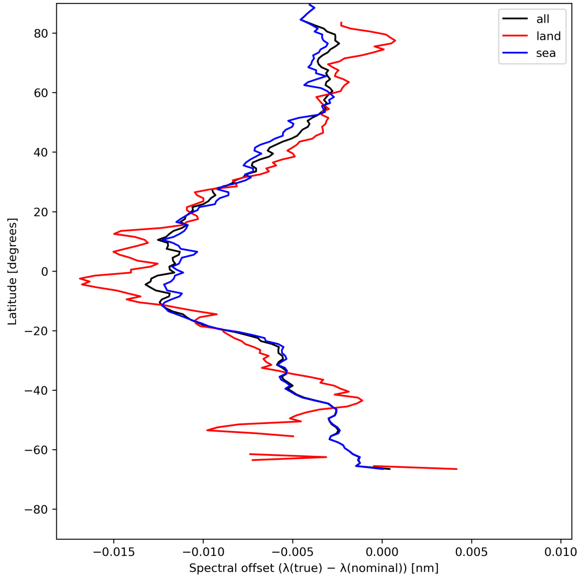
Figure 28: Zonal average of “Spectral offset ( \lambda(\text{true}) - \lambda(\text{nominal}) )” for 2024-05-24 to 2024-05-26.
