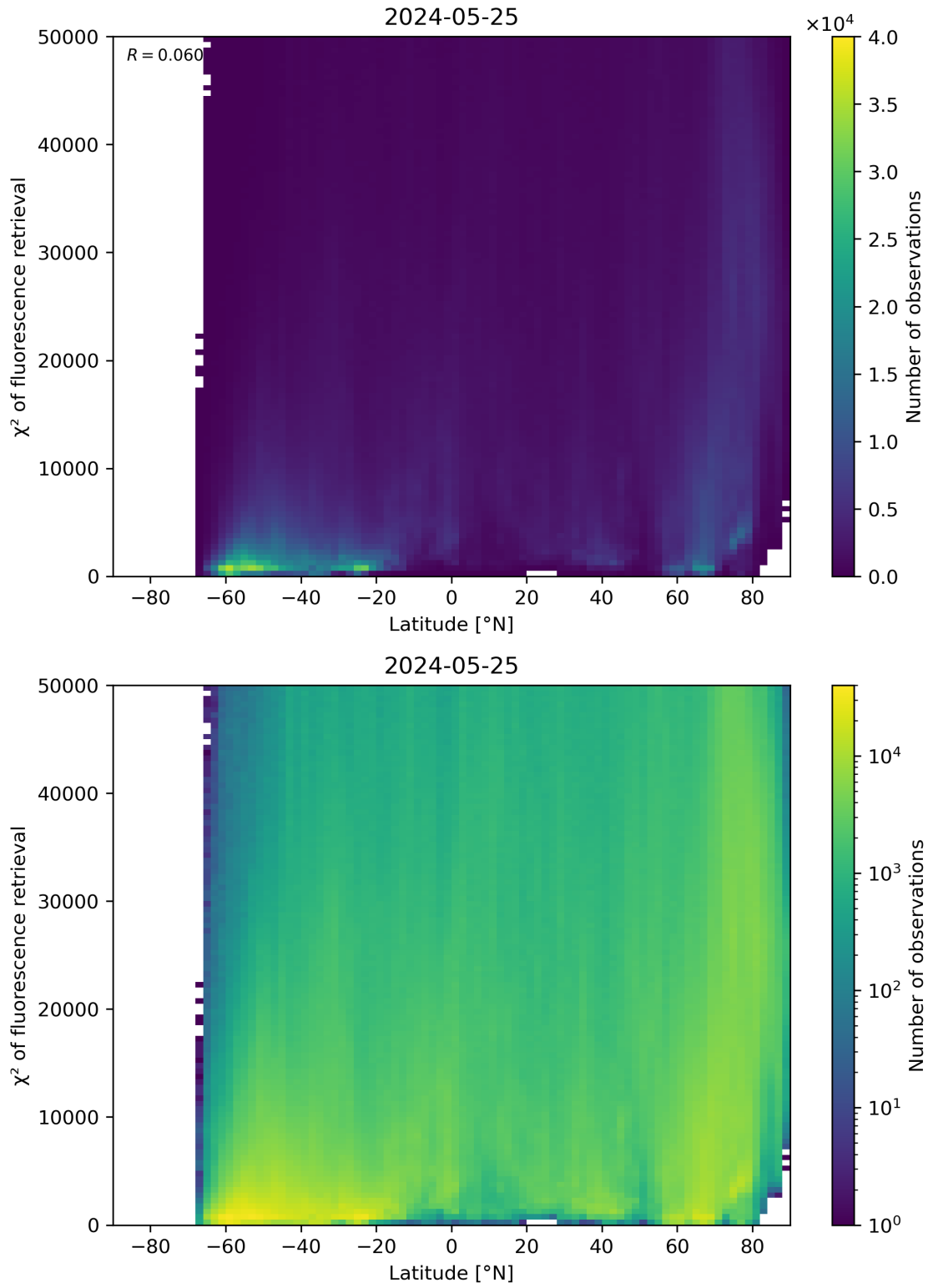
Figure 89: Scatter density plot of “Latitude” against “ \chi^2 of fluorescence retrieval” for 2024-05-24 to 2024-05-26.
