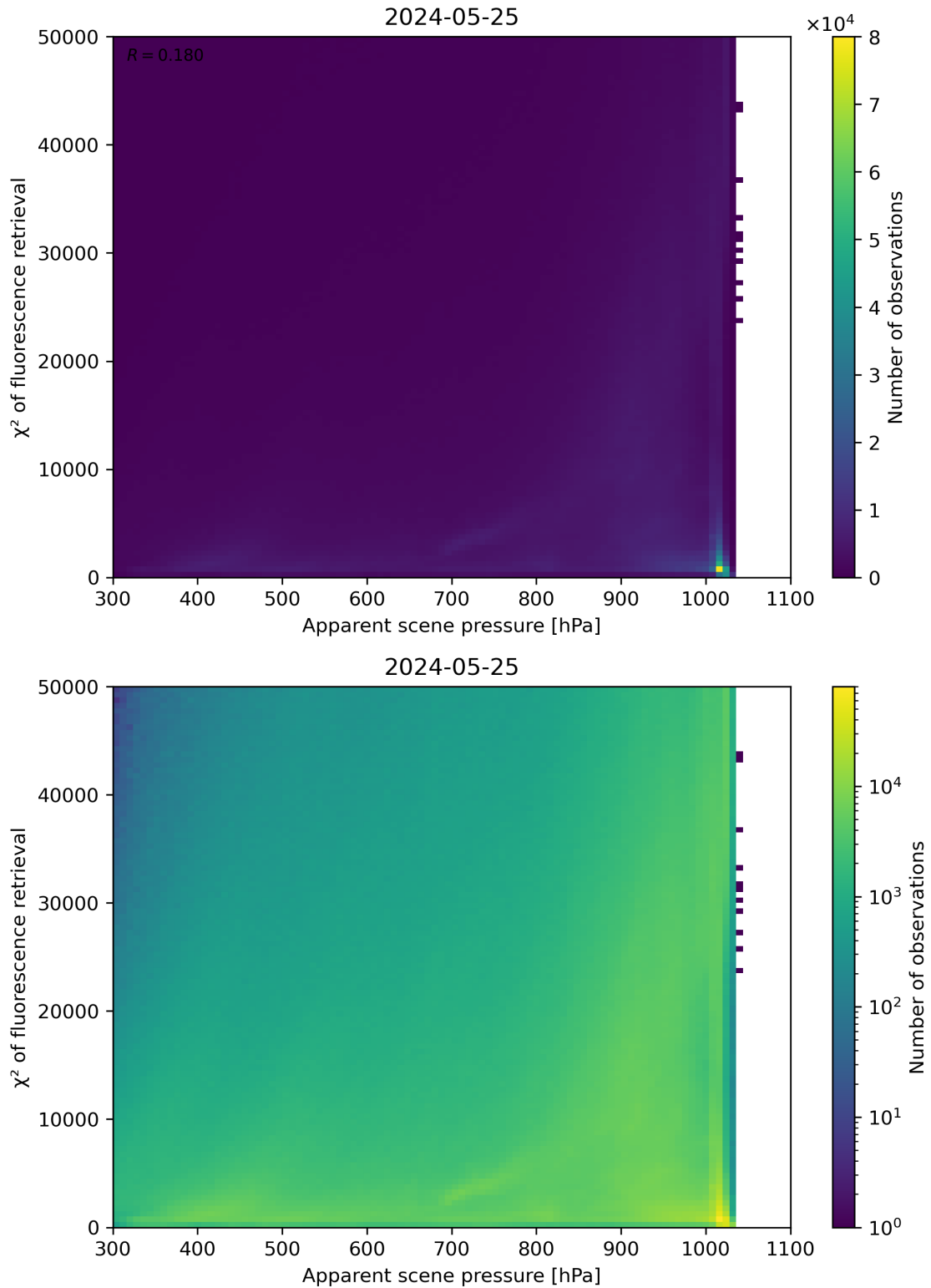
Figure 63: Scatter density plot of “Apparent scene pressure” against “ \chi^2 of fluorescence retrieval” for 2024-05-24 to 2024-05-26.
