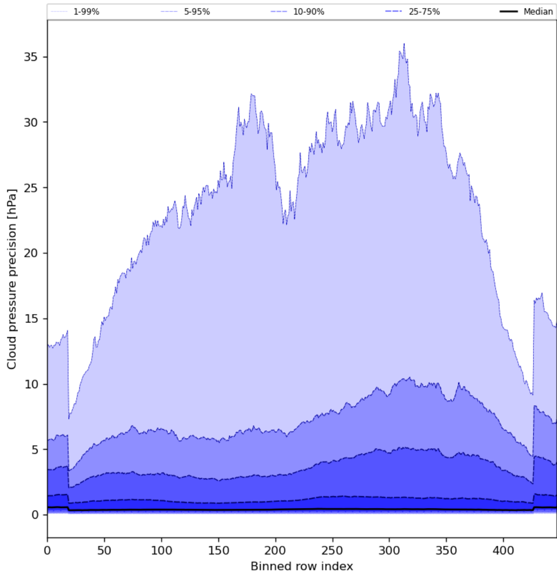
Figure 48: Along track statistics of “Cloud pressure precision” for 2024-05-24 to 2024-05-26
