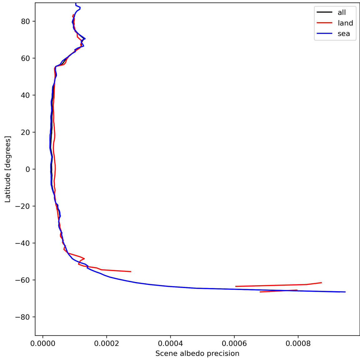
Figure 18: Zonal average of “Scene albedo precision” for 2024-05-24 to 2024-05-26.
