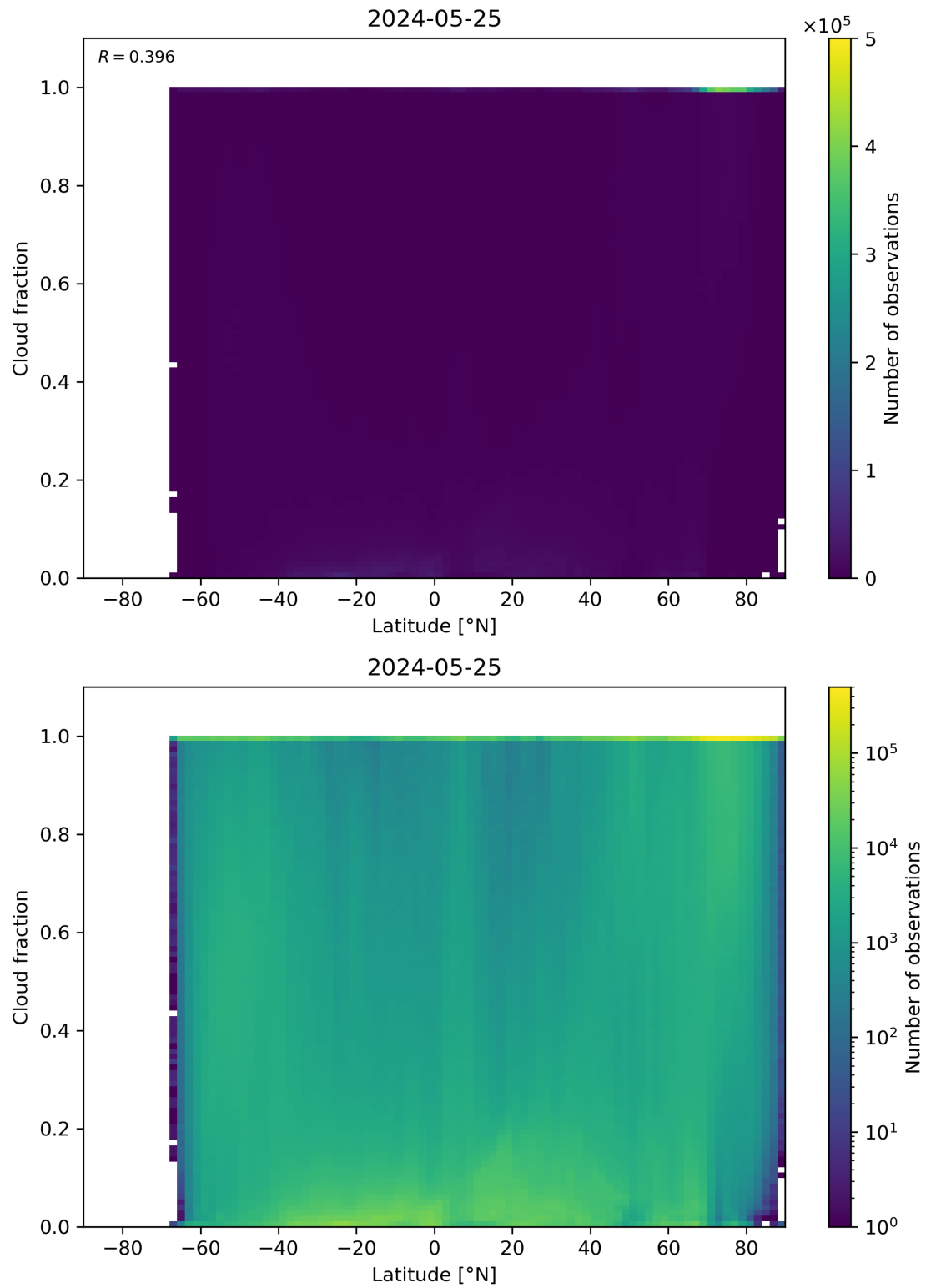
Figure 90: Scatter density plot of “Latitude” against “Cloud fraction” for 2024-05-24 to 2024-05-26.
