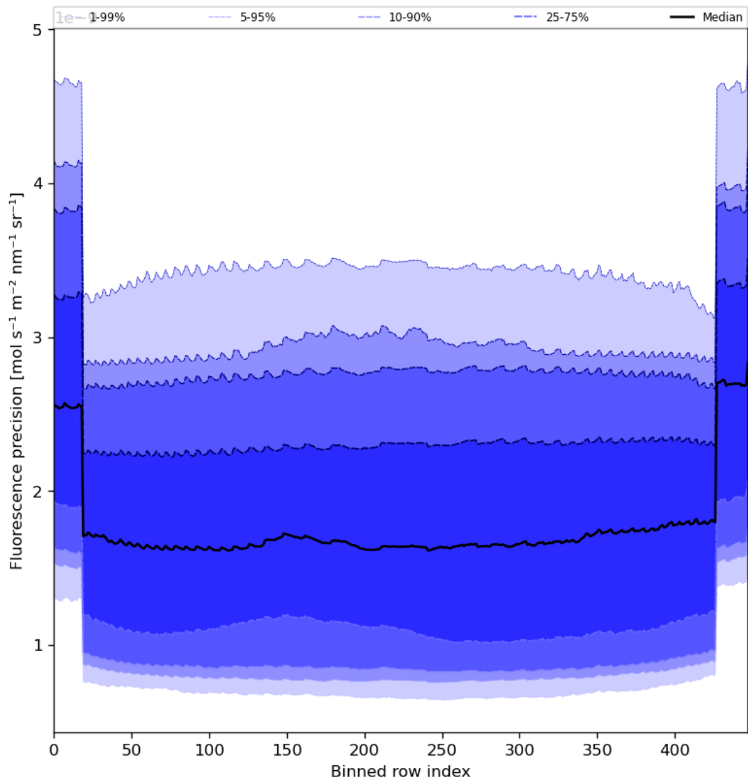
Figure 58: Along track statistics of “Fluorescence precision” for 2024-05-24 to 2024-05-26
