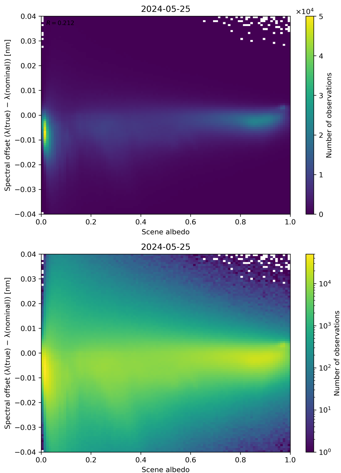
Figure 107: Scatter density plot of “Scene albedo” against “Spectral offset ( \lambda(\text{true}) - \lambda(\text{nominal}) )” for 2024-05-24 to 2024-05-26.
