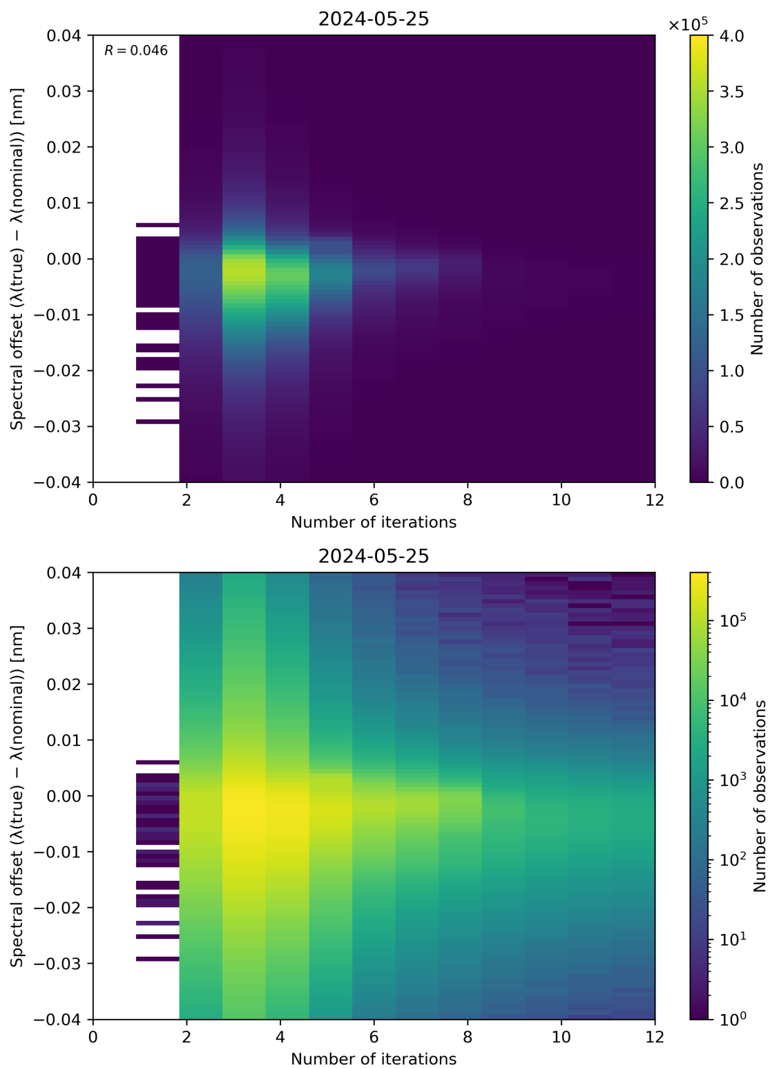
Figure 100: Scatter density plot of “Number of iterations” against “Spectral offset ( \lambda(\text{true}) - \lambda(\text{nominal}) )” for 2024-05-24 to 2024-05-26.
