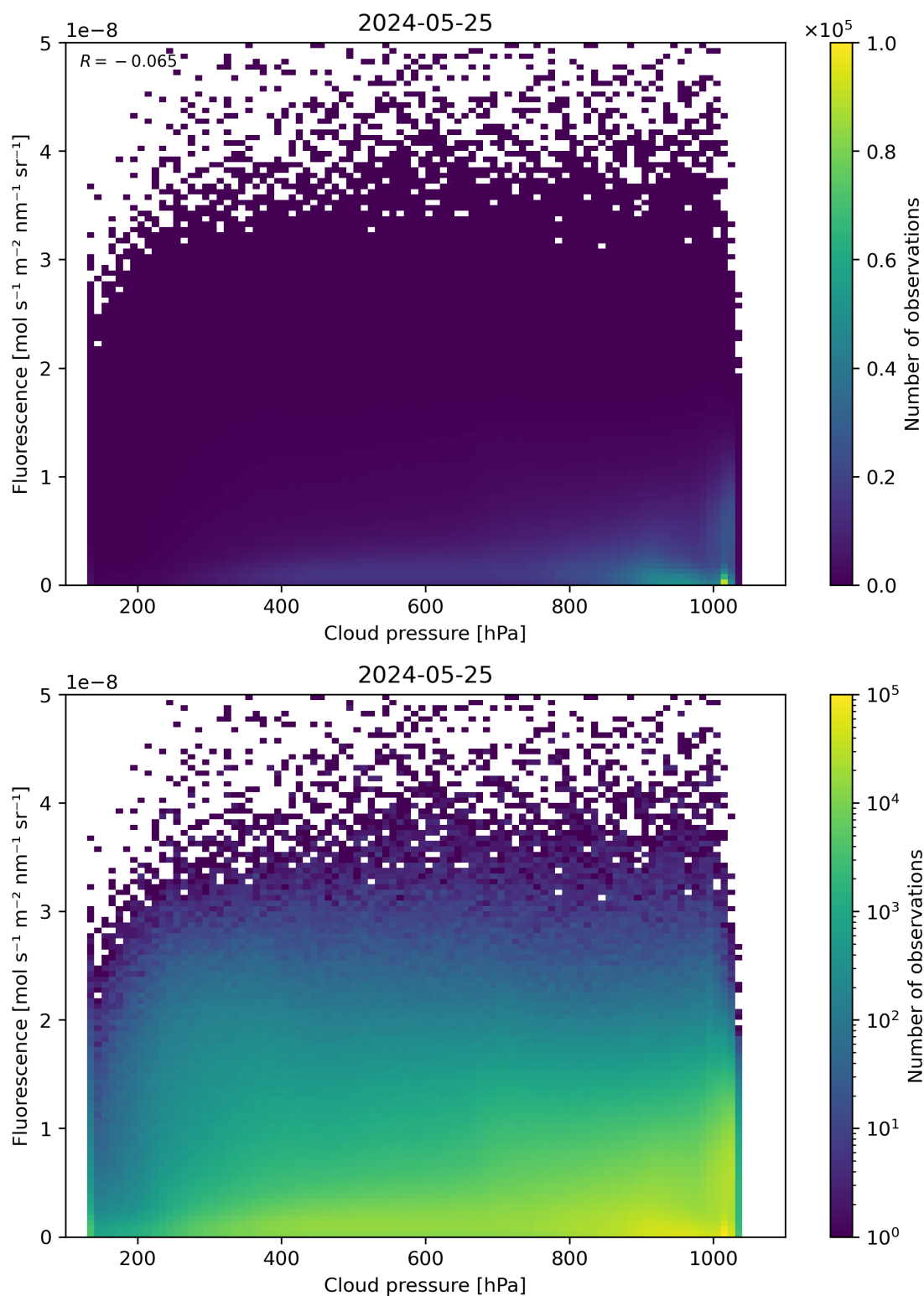
Figure 80: Scatter density plot of “Cloud pressure” against “Fluorescence” for 2024-05-24 to 2024-05-26.
