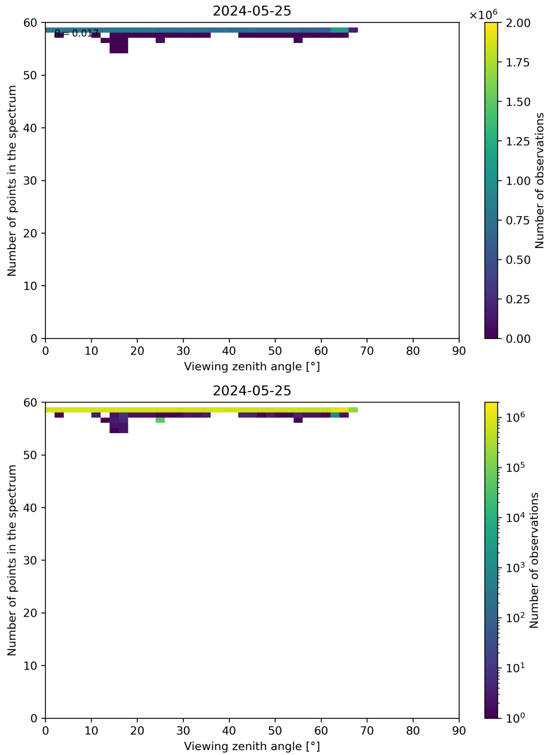
Figure 125: Scatter density plot of “Viewing zenith angle” against “Number of points in the spectrum” for 2024-05-24 to 2024-05-26.
