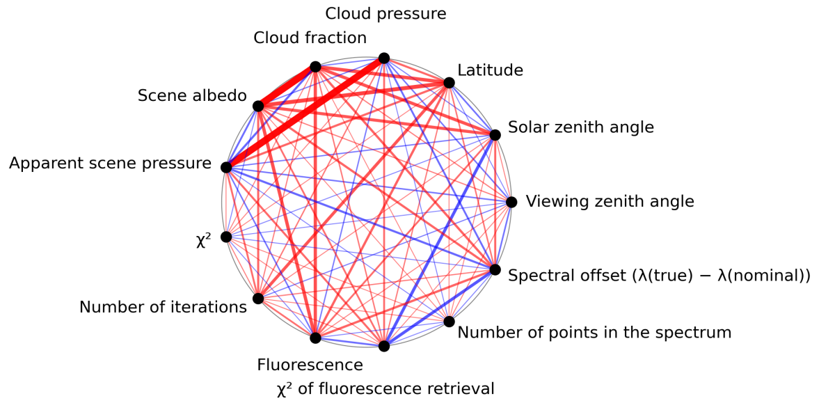
Figure 1: Map of correlation graph for 2024-05-24 to 2024-05-26.
