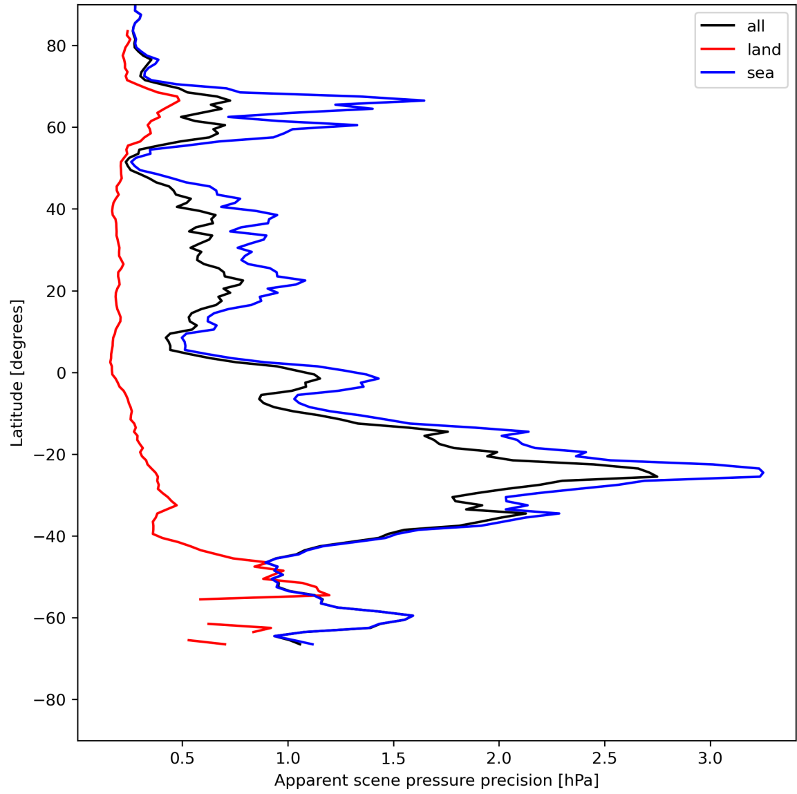
Figure 20: Zonal average of “Apparent scene pressure precision” for 2024-05-24 to 2024-05-26.
