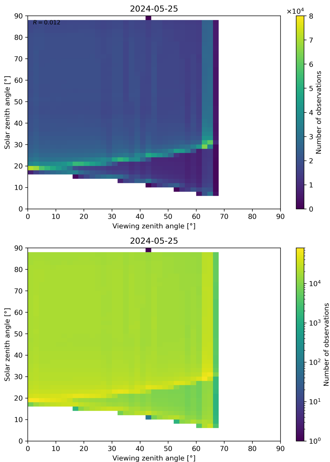
Figure 127: Scatter density plot of “Viewing zenith angle” against “Solar zenith angle” for 2024-05-24 to 2024-05-26.
