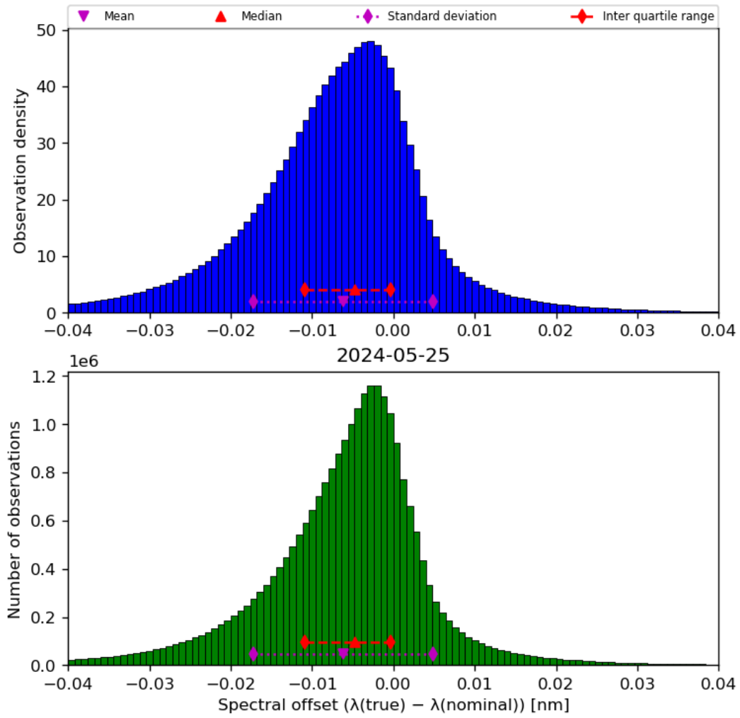
Figure 45: Histogram of “Spectral offset ( \lambda(\text{true}) - \lambda(\text{nominal}) )” for 2024-05-24 to 2024-05-26
