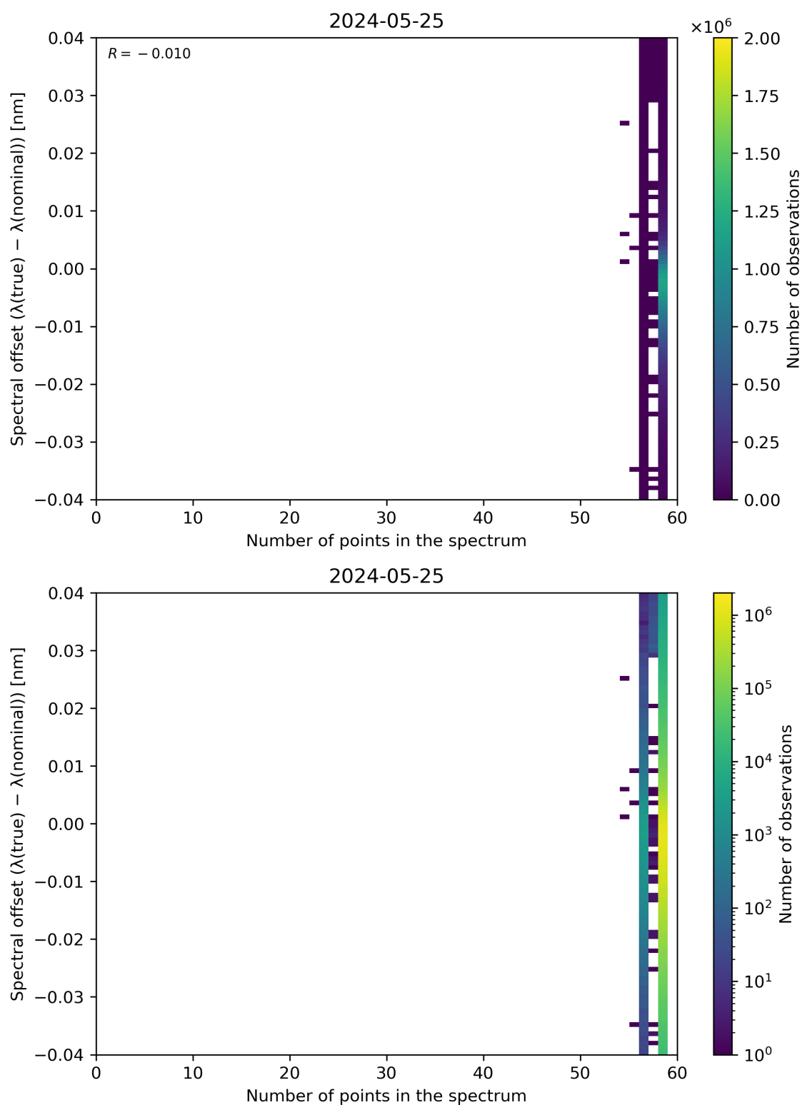
Figure 101: Scatter density plot of “Number of points in the spectrum” against “Spectral offset ( \lambda(\text{true}) - \lambda(\text{nominal}) )” for 2024-05-24 to 2024-05-26.
