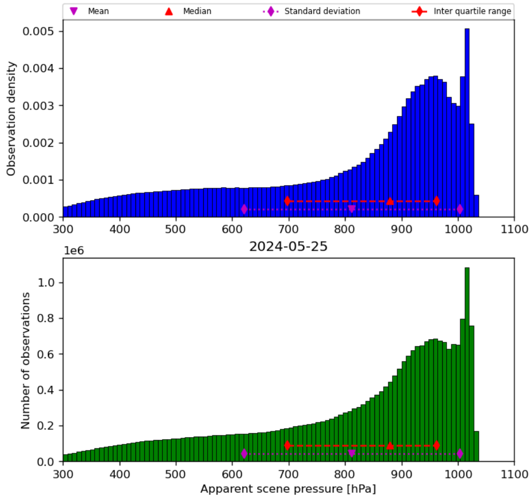
Figure 36: Histogram of “Apparent scene pressure” for 2024-05-24 to 2024-05-26
