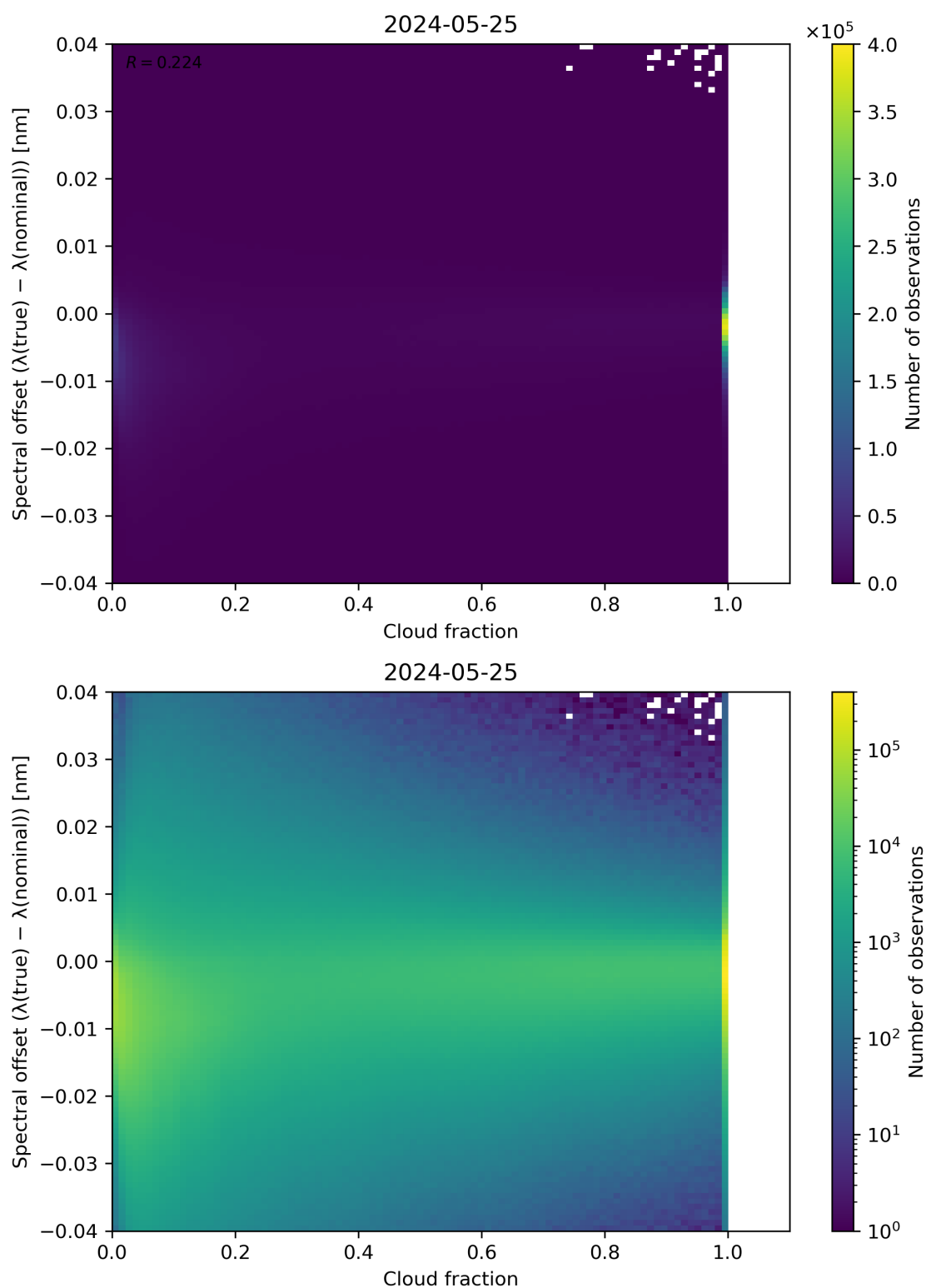
Figure 76: Scatter density plot of “Cloud fraction” against “Spectral offset ( \lambda(\text{true}) - \lambda(\text{nominal}) )” for 2024-05-24 to 2024-05-26.
