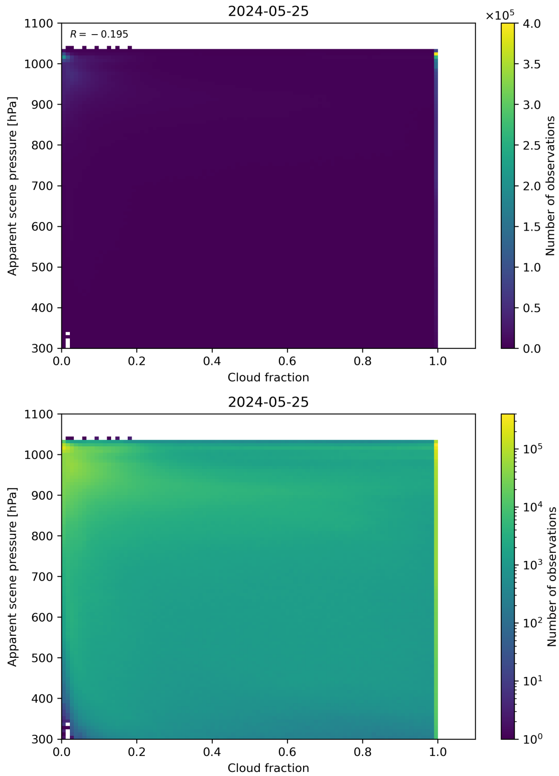
Figure 70: Scatter density plot of “Cloud fraction” against “Apparent scene pressure” for 2024-05-24 to 2024-05-26.
