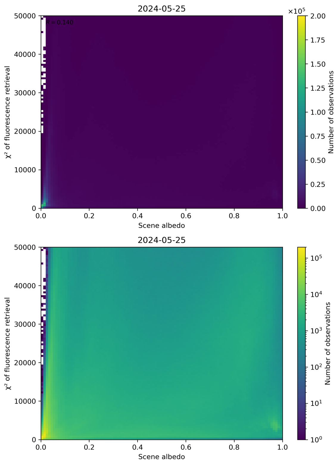
Figure 103: Scatter density plot of “Scene albedo” against “ \chi^2 of fluorescence retrieval” for 2024-05-24 to 2024-05-26.
