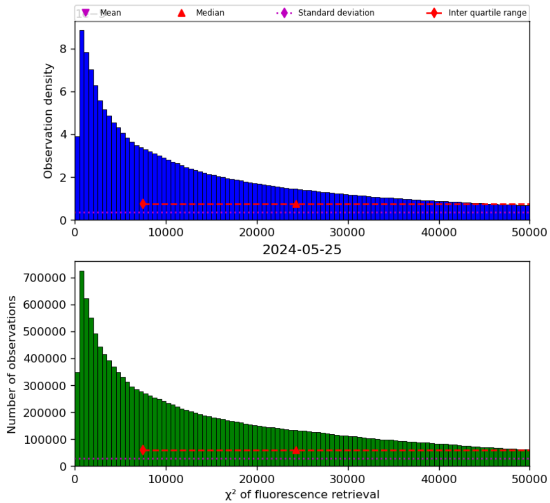
Figure 42: Histogram of “ \chi^2 of fluorescence retrieval” for 2024-05-24 to 2024-05-26
