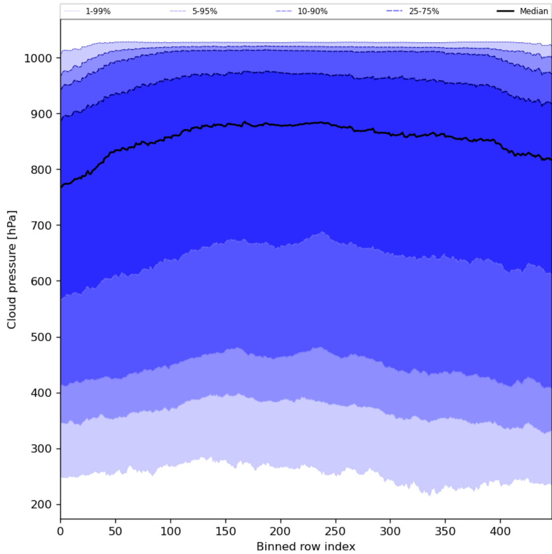
Figure 47: Along track statistics of “Cloud pressure” for 2024-05-24 to 2024-05-26
