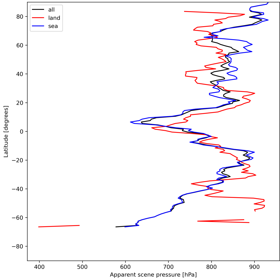
Figure 19: Zonal average of “Apparent scene pressure” for 2024-05-24 to 2024-05-26.
