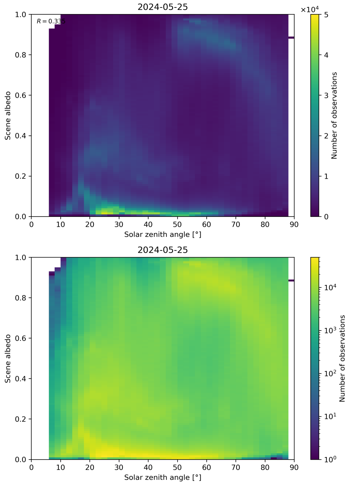
Figure 116: Scatter density plot of “Solar zenith angle” against “Scene albedo” for 2024-05-24 to 2024-05-26.
