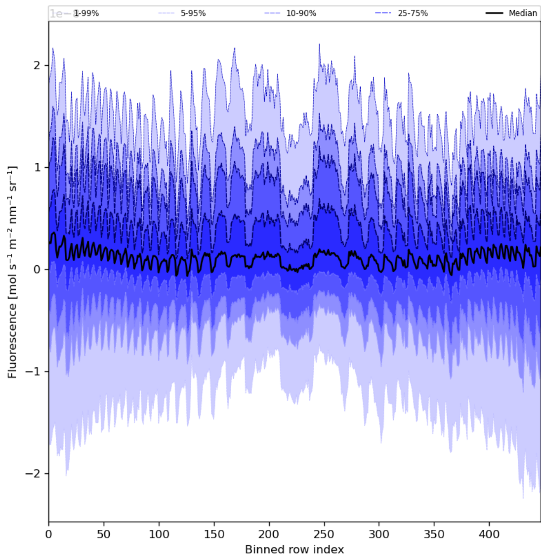
Figure 57: Along track statistics of “Fluorescence” for 2024-05-24 to 2024-05-26
