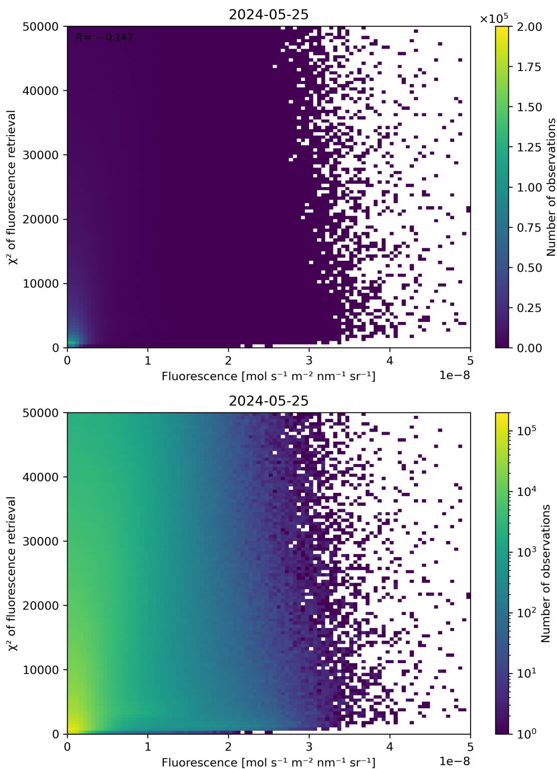
Figure 85: Scatter density plot of “Fluorescence” against “ \chi^2 of fluorescence retrieval” for 2024-05-24 to 2024-05-26.
