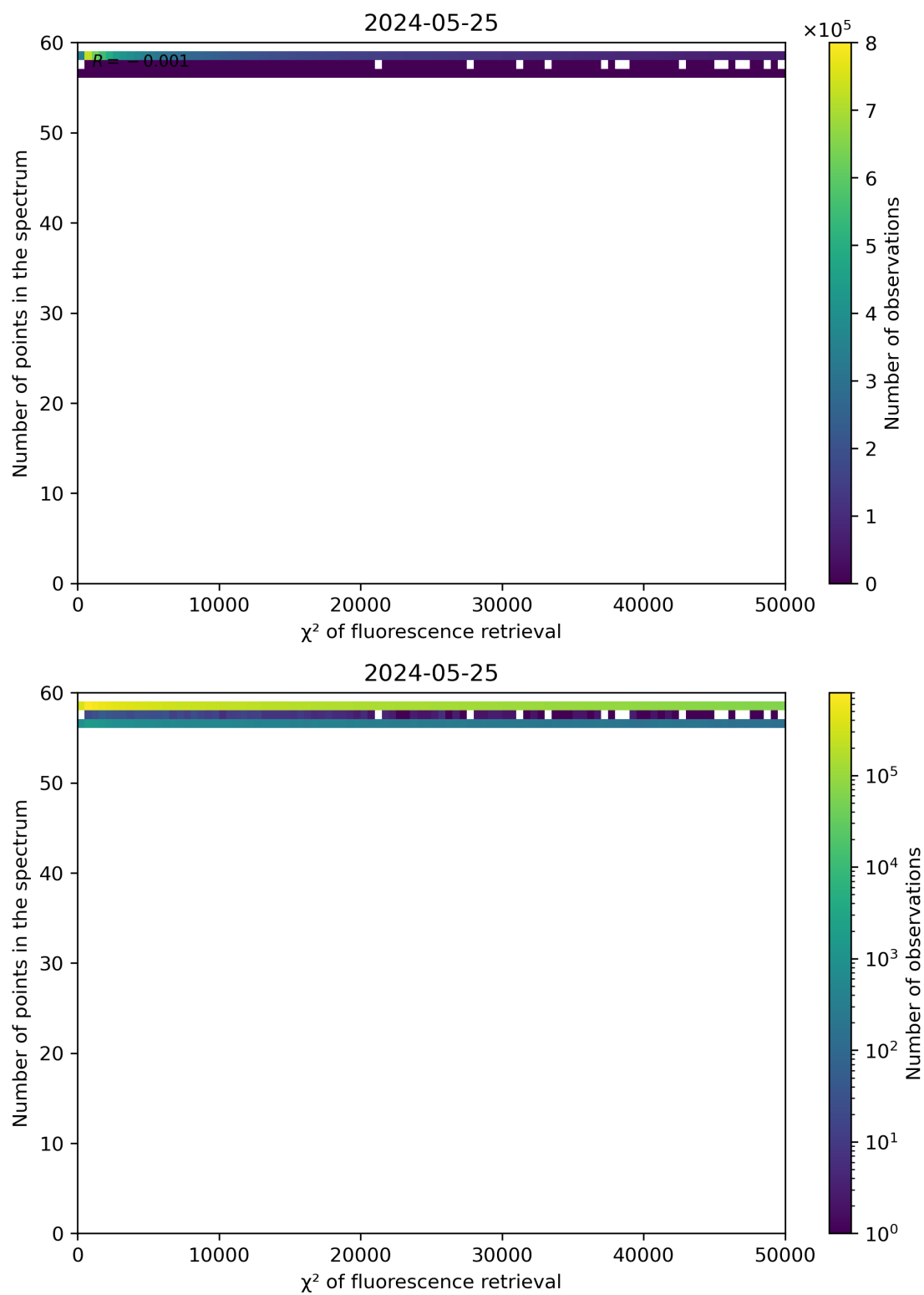
Figure 68: Scatter density plot of " \chi^2 of fluorescence retrieval" against "Number of points in the spectrum" for 2024-05-24 to 2024-05-26.
