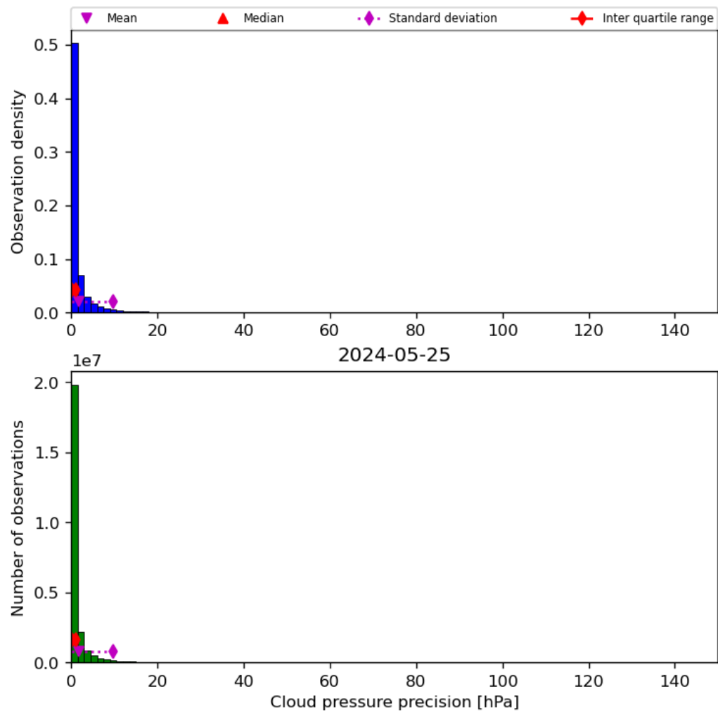
Figure 31: Histogram of “Cloud pressure precision” for 2024-05-24 to 2024-05-26
