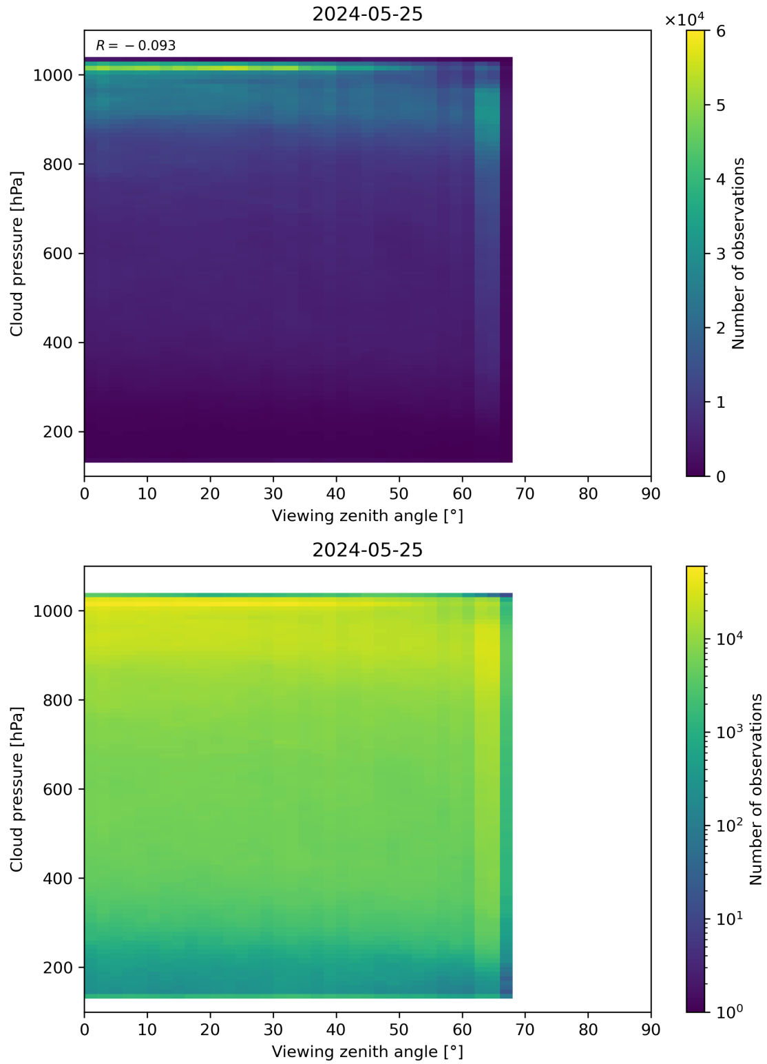
Figure 121: Scatter density plot of “Viewing zenith angle” against “Cloud pressure” for 2024-05-24 to 2024-05-26.
