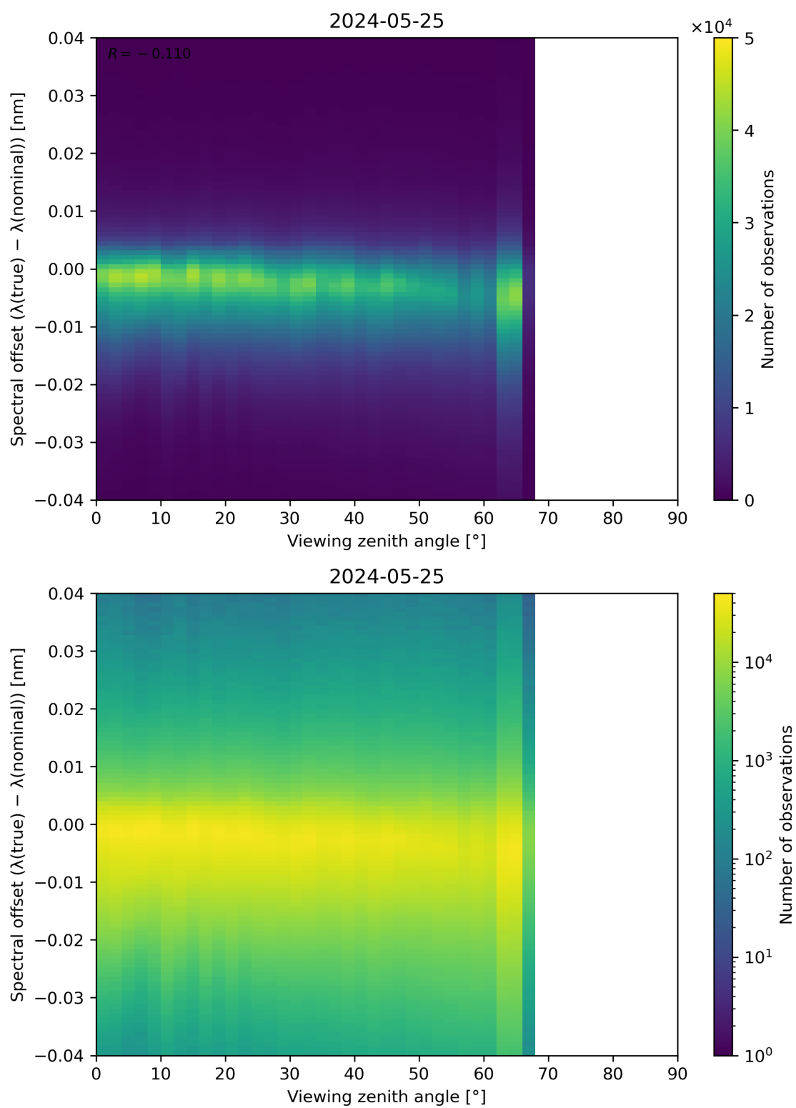
Figure 128: Scatter density plot of “Viewing zenith angle” against “Spectral offset ( \lambda(\text{true}) - \lambda(\text{nominal}) )” for 2024-05-24 to 2024-05-26.
