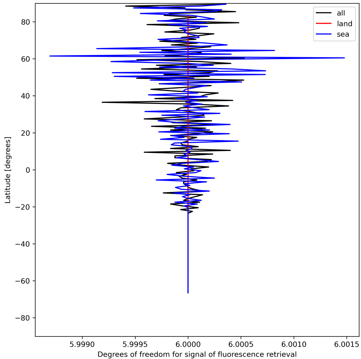
Figure 26: Zonal average of “Degrees of freedom for signal of fluorescence retrieval” for 2024-05-24 to 2024-05-26.
