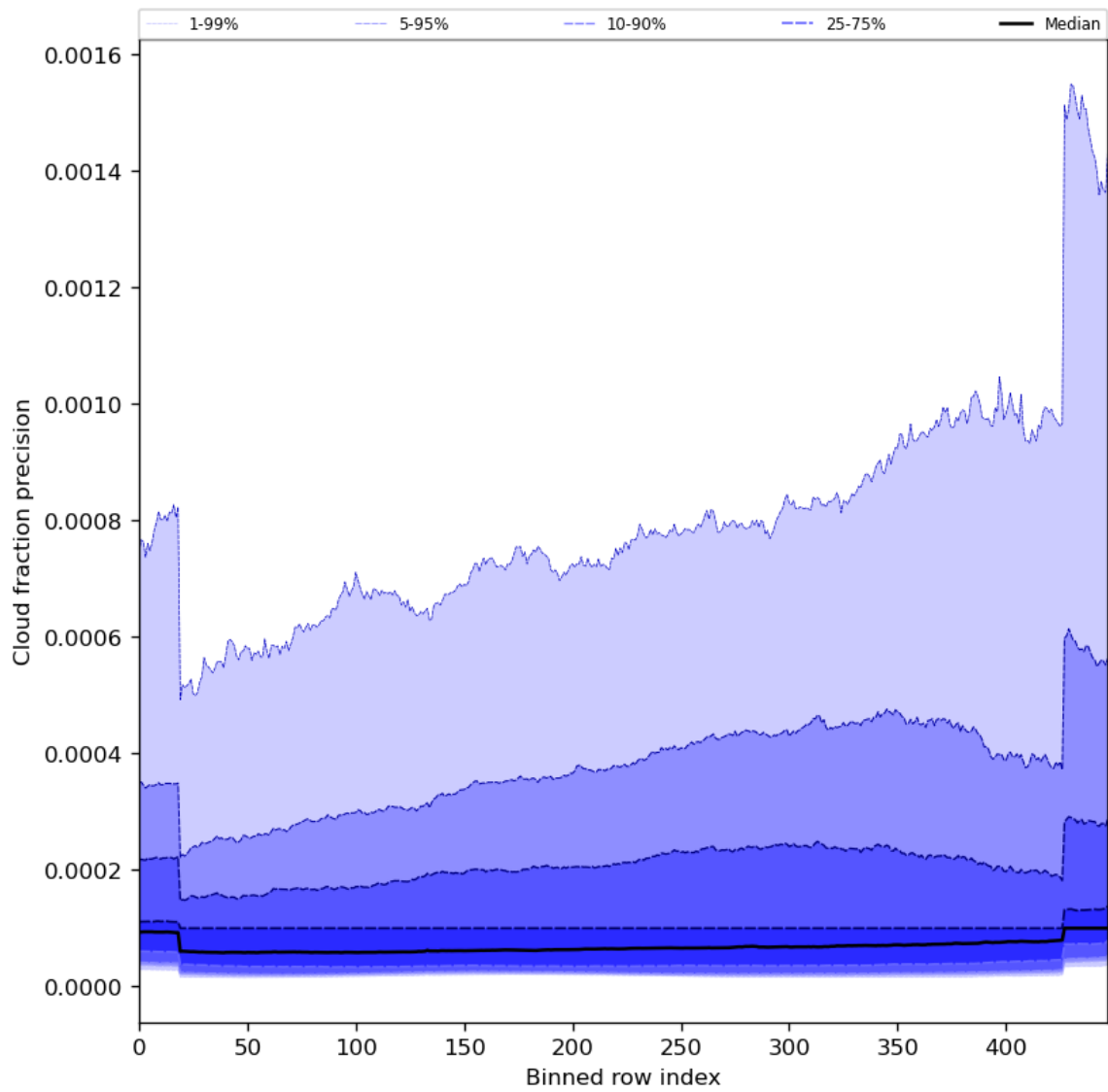
Figure 50: Along track statistics of “Cloud fraction precision” for 2024-05-24 to 2024-05-26
