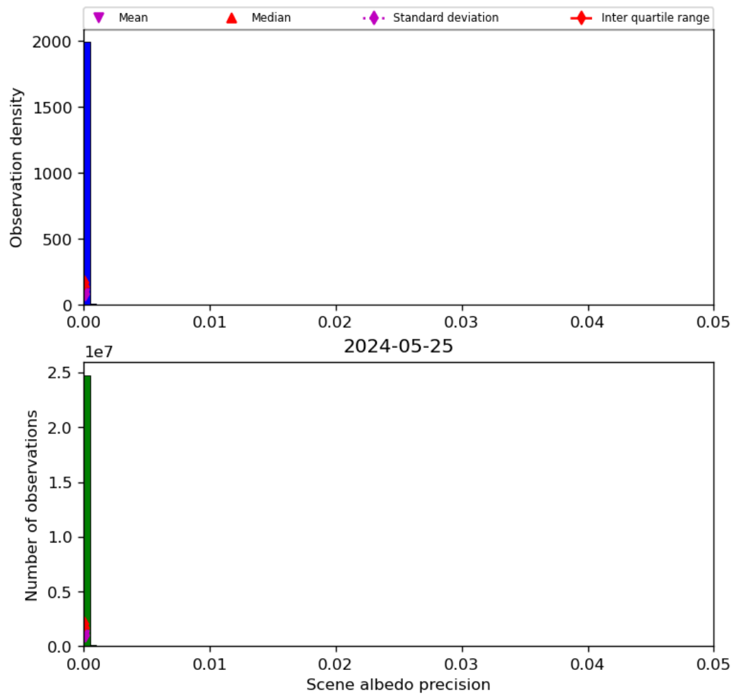
Figure 35: Histogram of “Scene albedo precision” for 2024-05-24 to 2024-05-26
