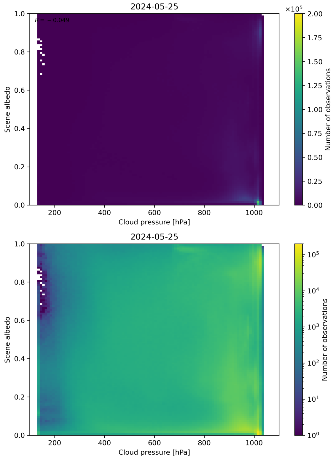
Figure 83: Scatter density plot of “Cloud pressure” against “Scene albedo” for 2024-05-24 to 2024-05-26.
