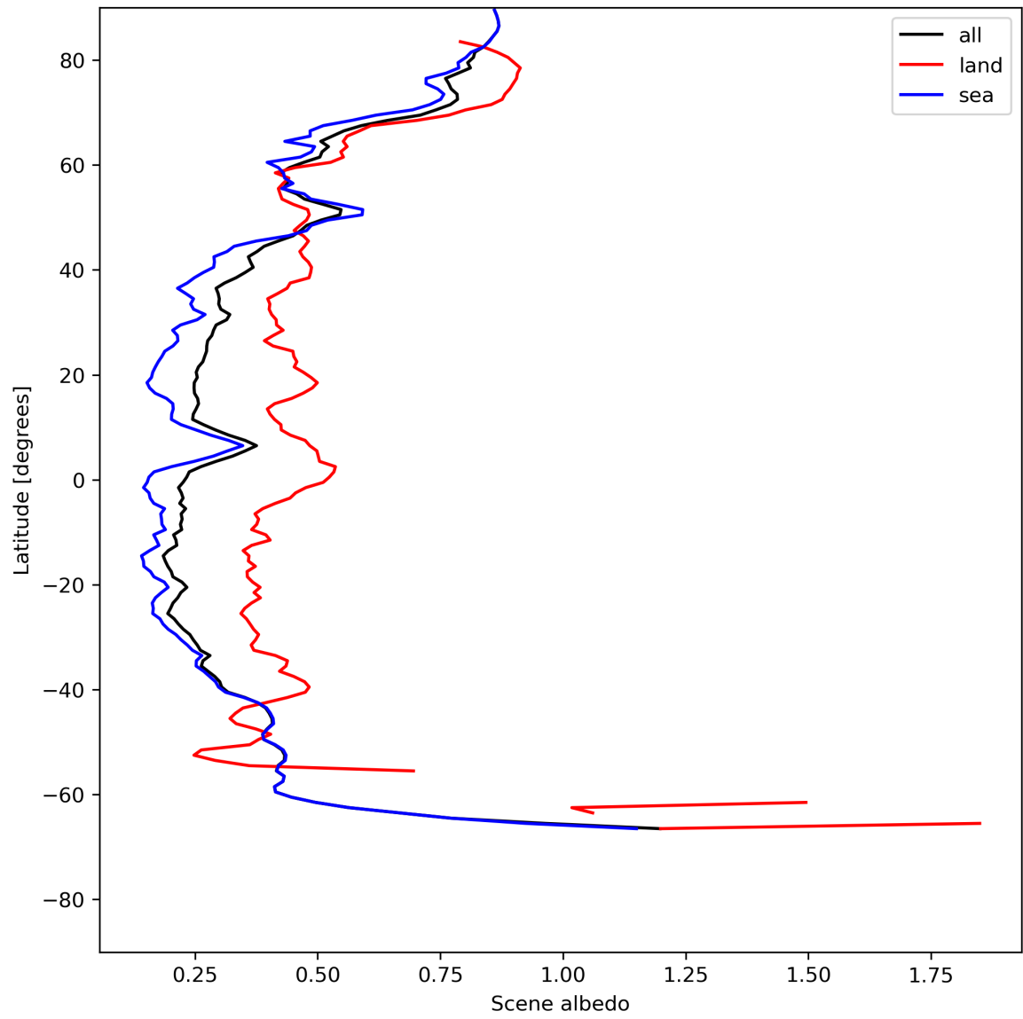
Figure 17: Zonal average of “Scene albedo” for 2024-05-24 to 2024-05-26.
