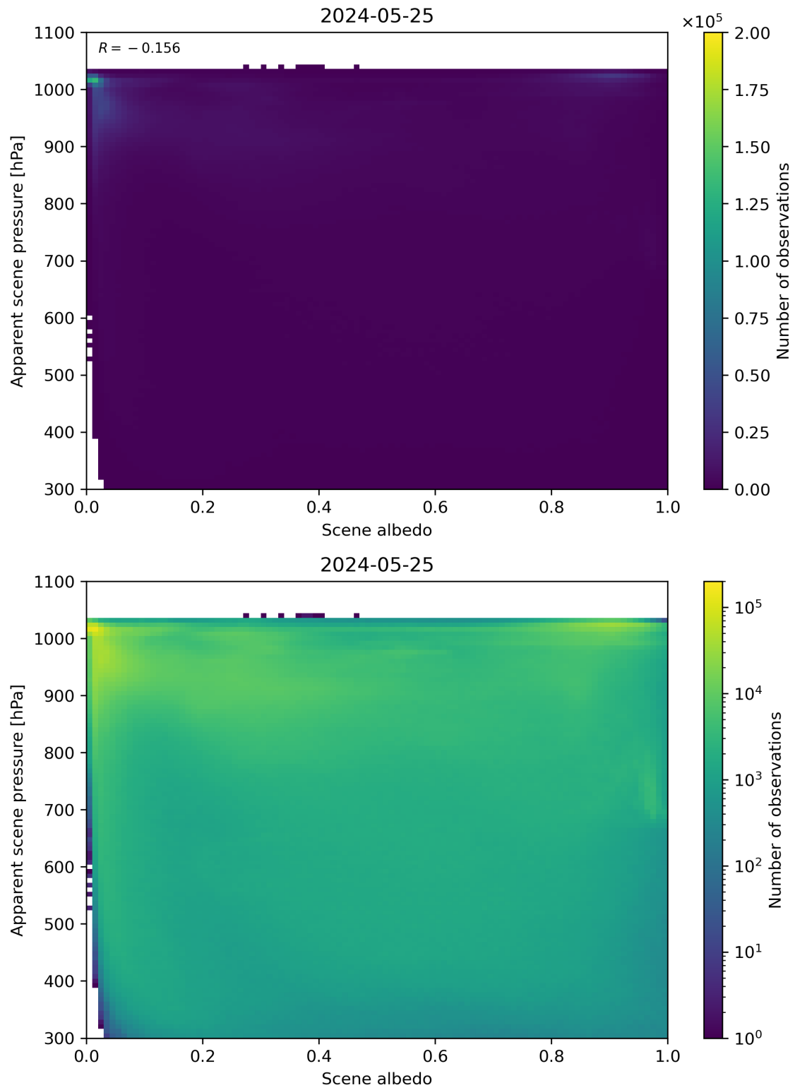
Figure 102: Scatter density plot of “Scene albedo” against “Apparent scene pressure” for 2024-05-24 to 2024-05-26.
