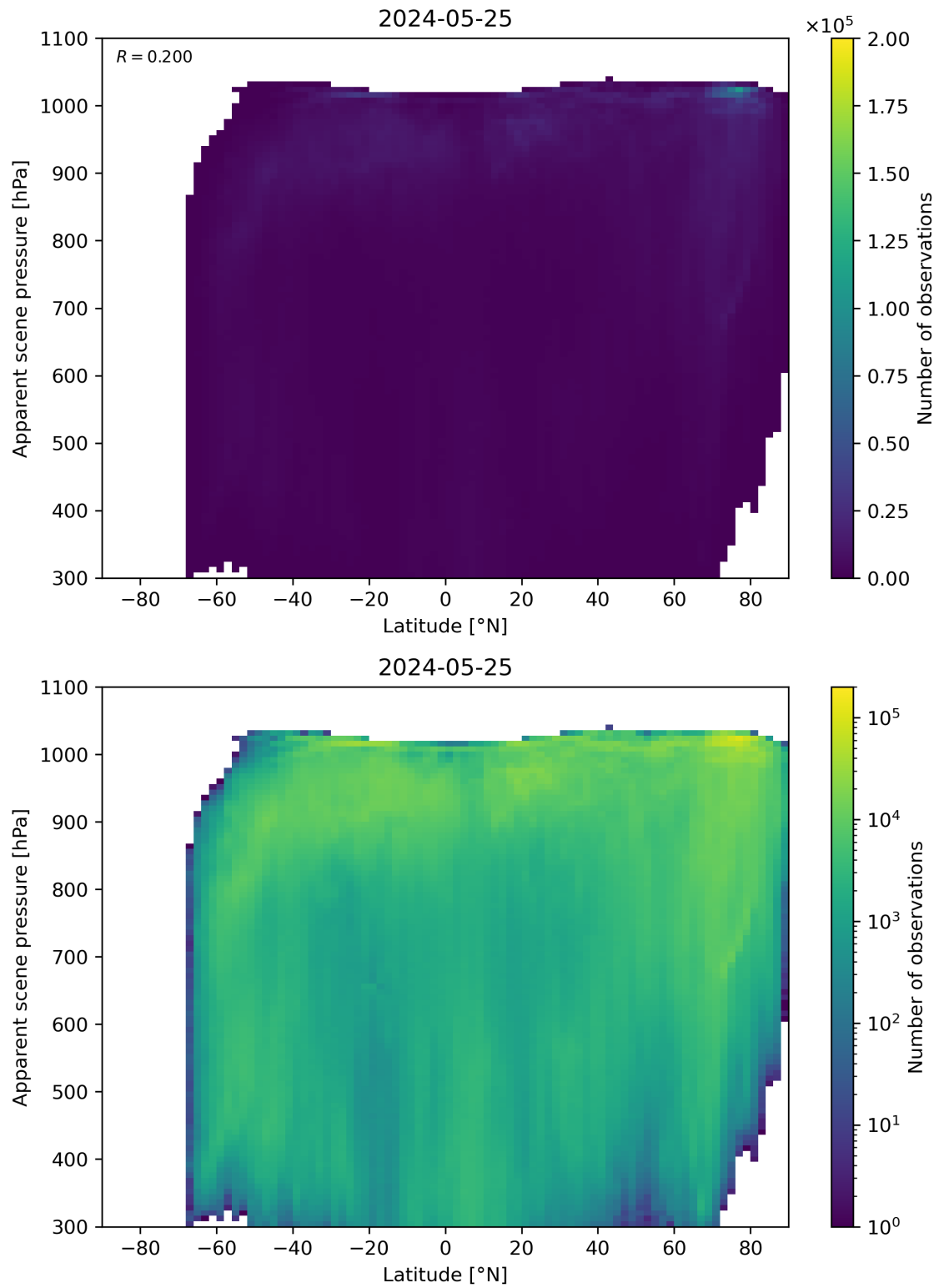
Figure 88: Scatter density plot of “Latitude” against “Apparent scene pressure” for 2024-05-24 to 2024-05-26.
