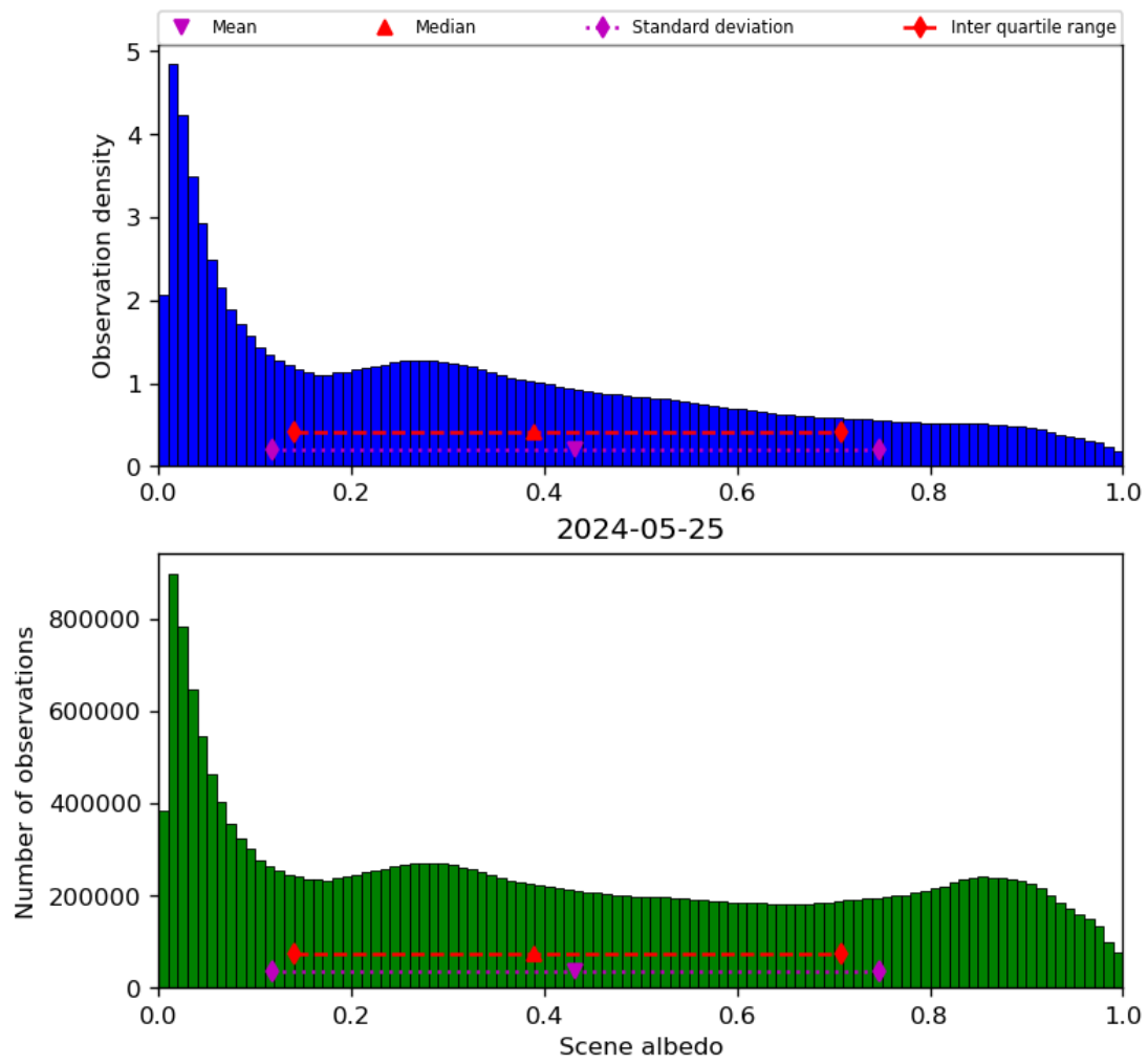
Figure 34: Histogram of “Scene albedo” for 2024-05-24 to 2024-05-26
