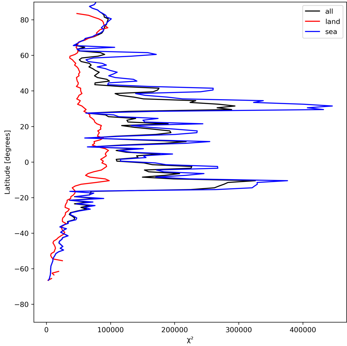
Figure 21: Zonal average of “ \chi^2 ” for 2024-05-24 to 2024-05-26.
