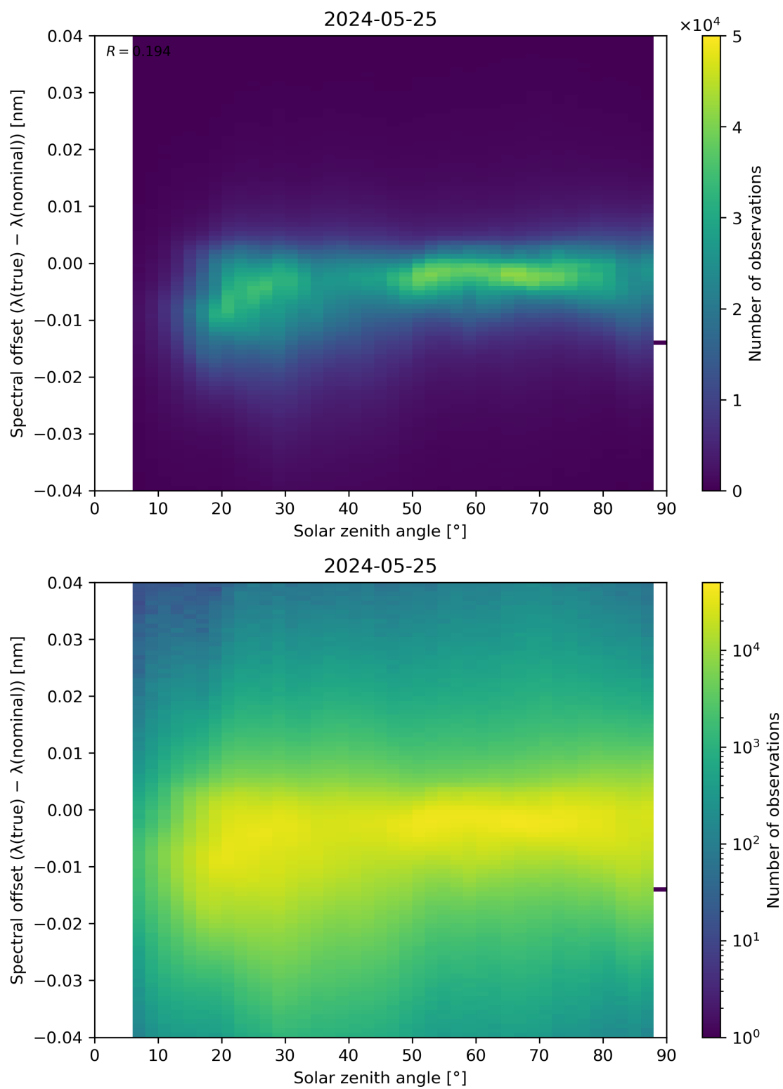
Figure 117: Scatter density plot of “Solar zenith angle” against “Spectral offset ( \lambda(\text{true}) - \lambda(\text{nominal}) )” for 2024-05-24 to 2024-05-26.
