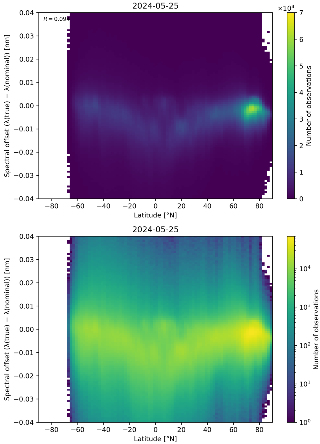
Figure 96: Scatter density plot of “Latitude” against “Spectral offset ( \lambda(\text{true}) - \lambda(\text{nominal}) )” for 2024-05-24 to 2024-05-26.
