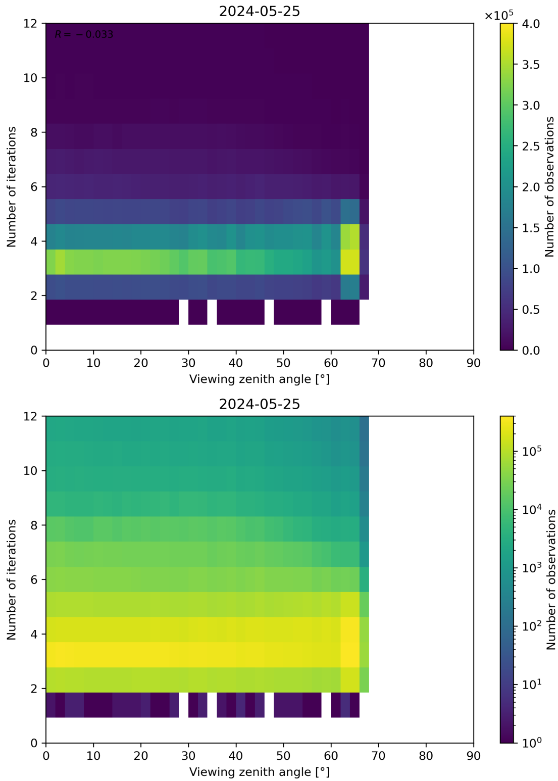
Figure 124: Scatter density plot of “Viewing zenith angle” against “Number of iterations” for 2024-05-24 to 2024-05-26.
