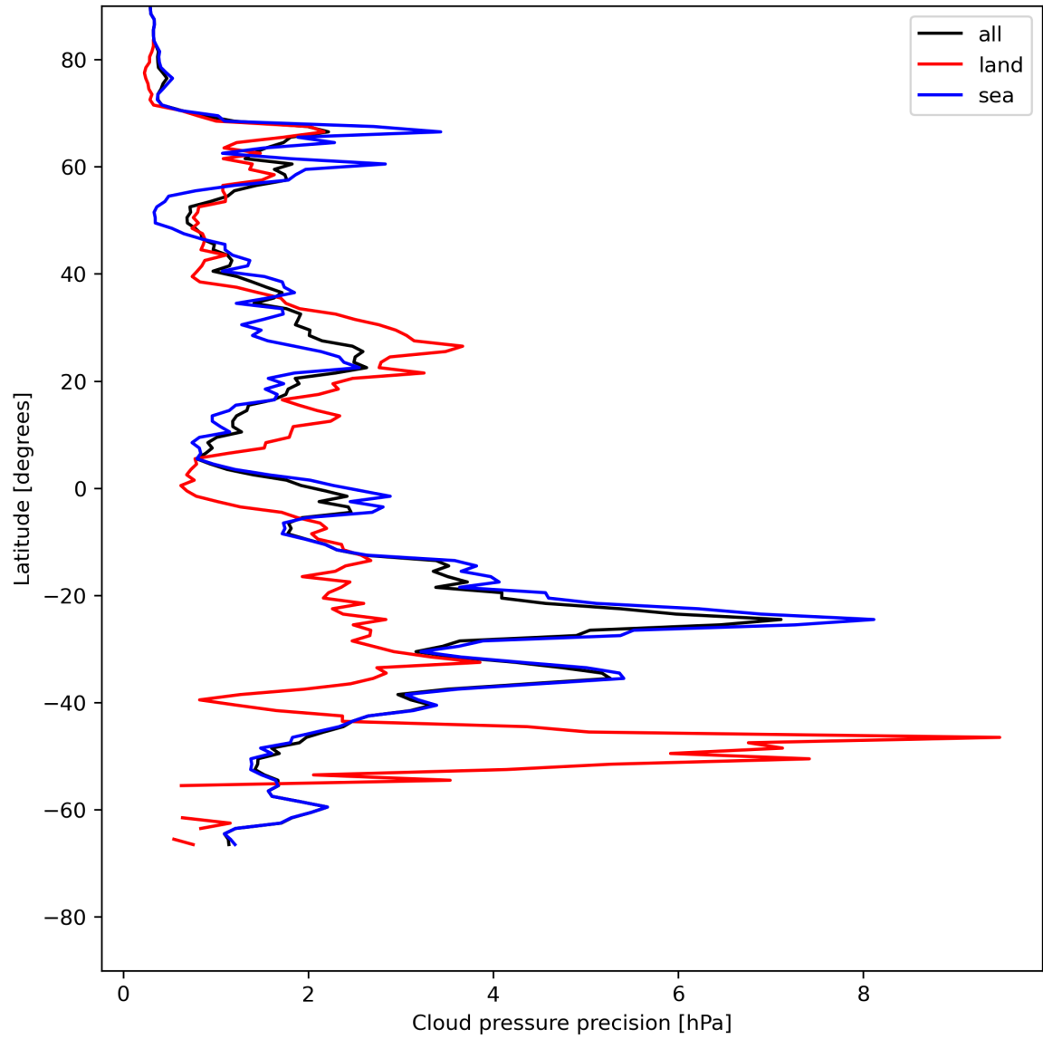
Figure 14: Zonal average of “Cloud pressure precision” for 2024-05-24 to 2024-05-26.
