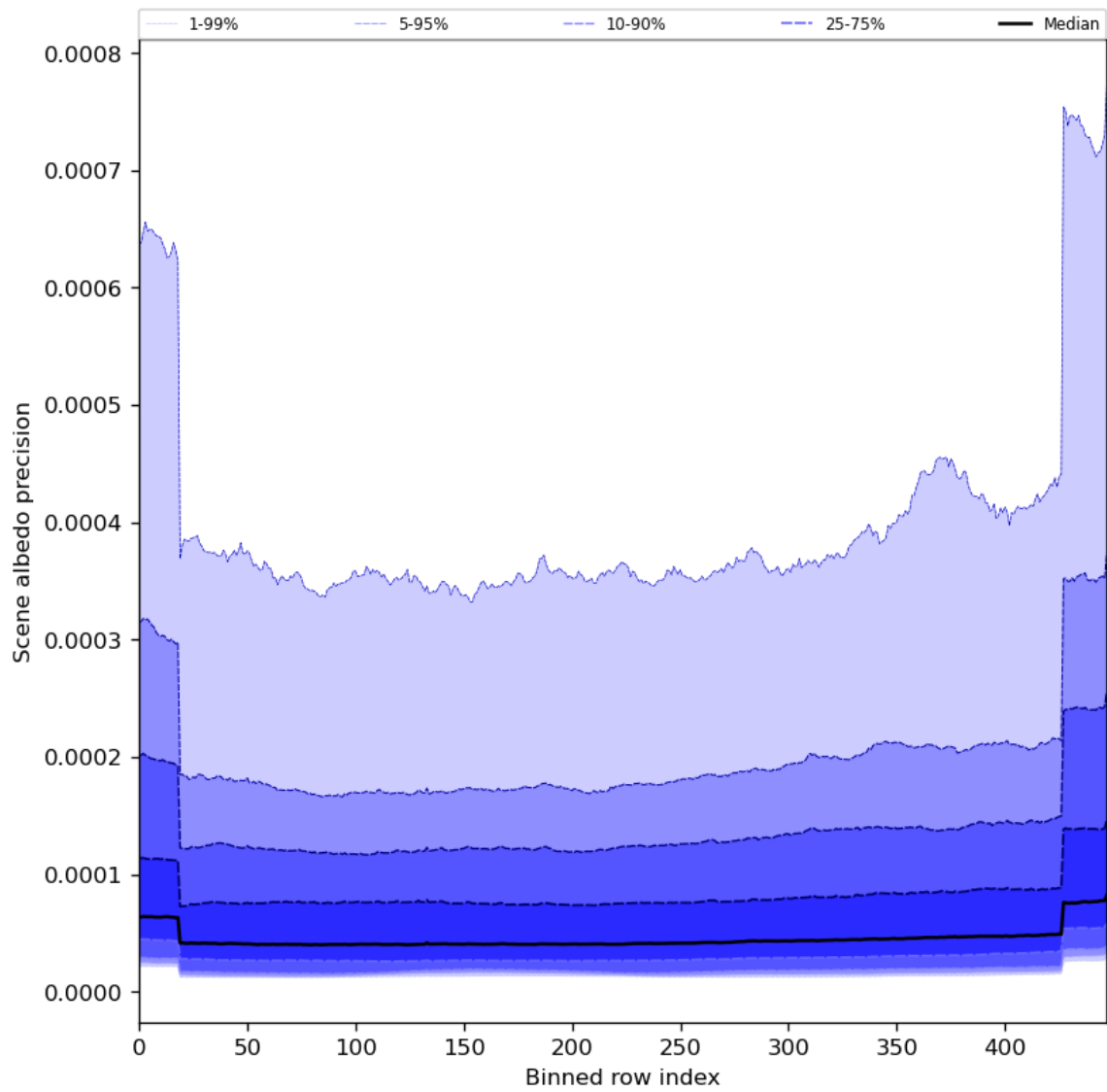
Figure 52: Along track statistics of “Scene albedo precision” for 2024-05-24 to 2024-05-26
