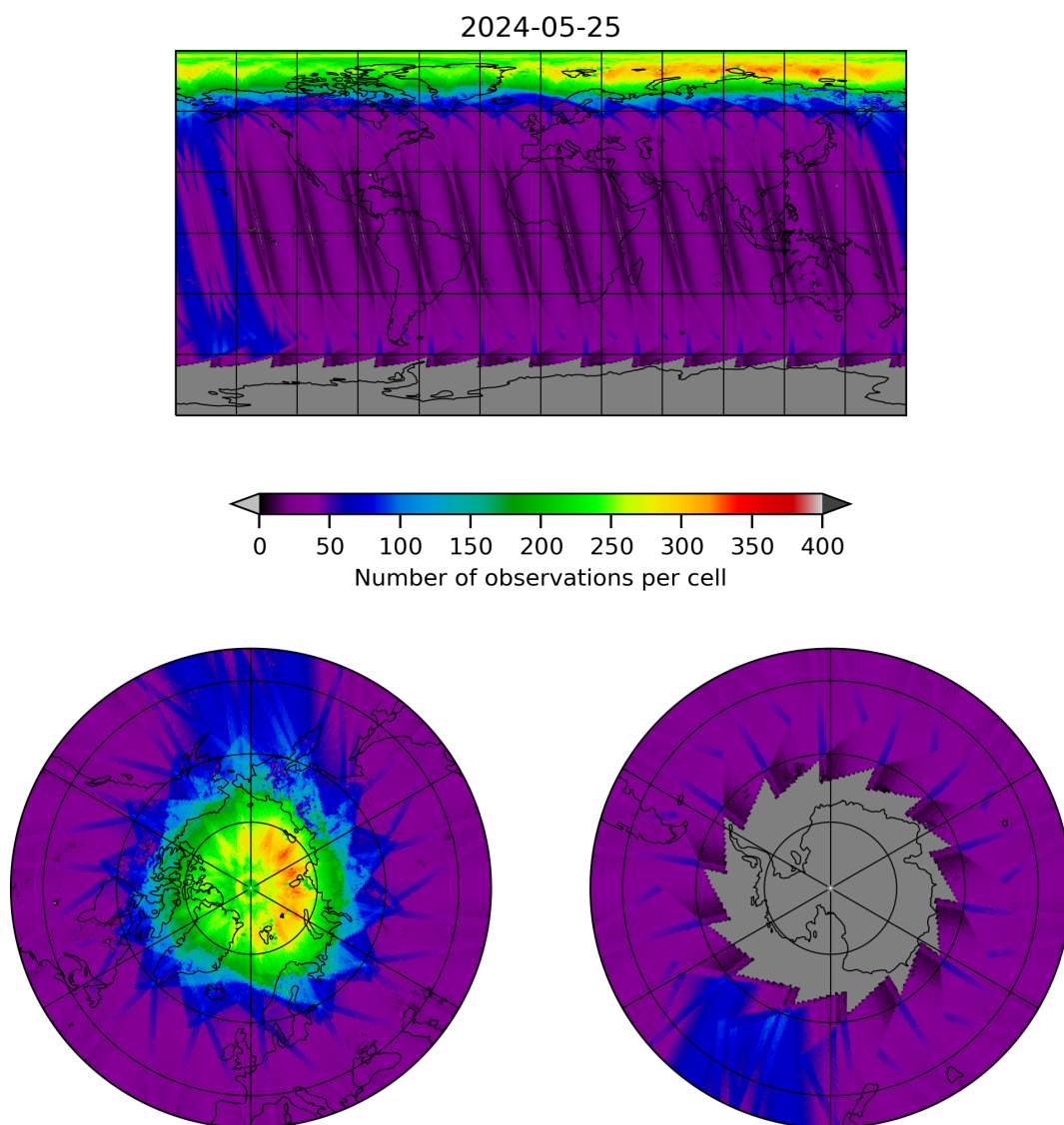
Figure 11: Map of the number of observations for 2024-05-24 to 2024-05-26
