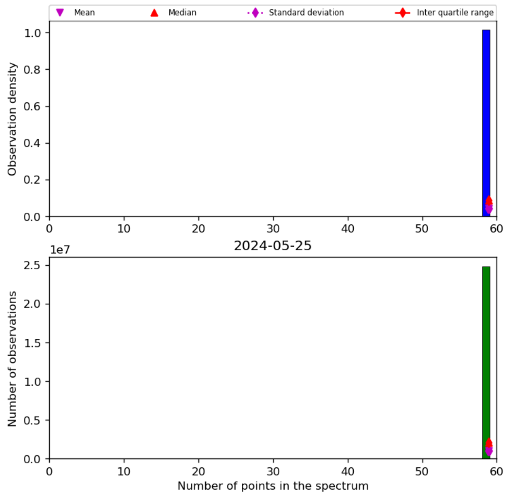
Figure 44: Histogram of “Number of points in the spectrum” for 2024-05-24 to 2024-05-26
