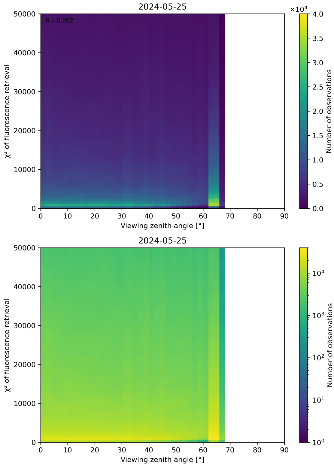
Figure 119: Scatter density plot of “Viewing zenith angle” against “ \chi^2 of fluorescence retrieval” for 2024-05-24 to 2024-05-26.
