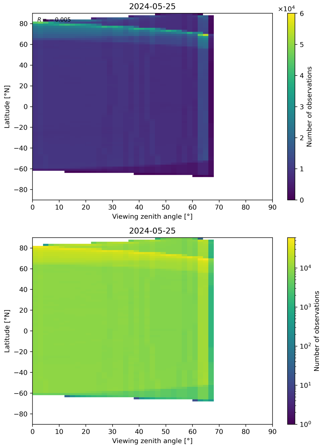
Figure 123: Scatter density plot of “Viewing zenith angle” against “Latitude” for 2024-05-24 to 2024-05-26.
