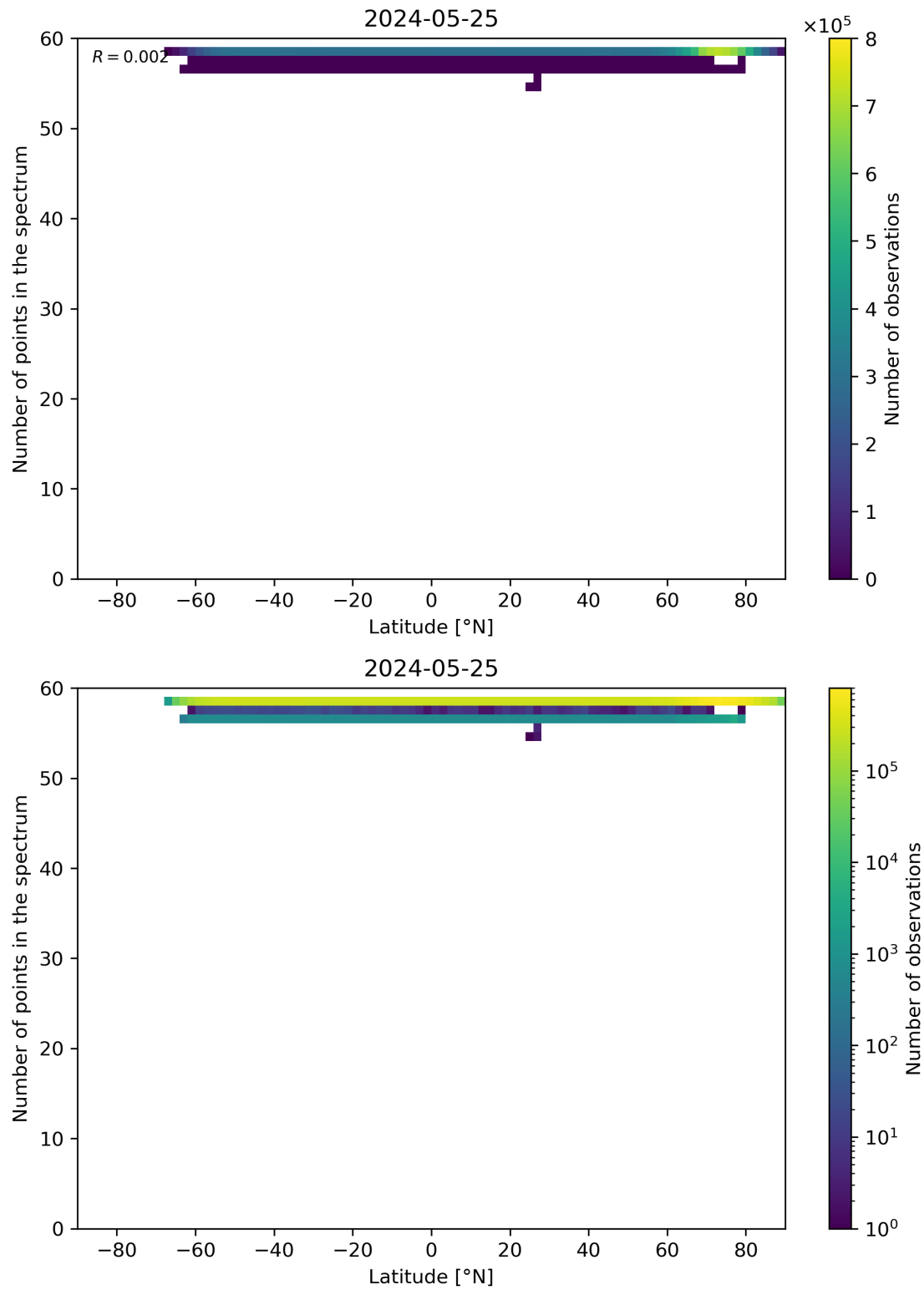
Figure 94: Scatter density plot of “Latitude” against “Number of points in the spectrum” for 2024-05-24 to 2024-05-26.
