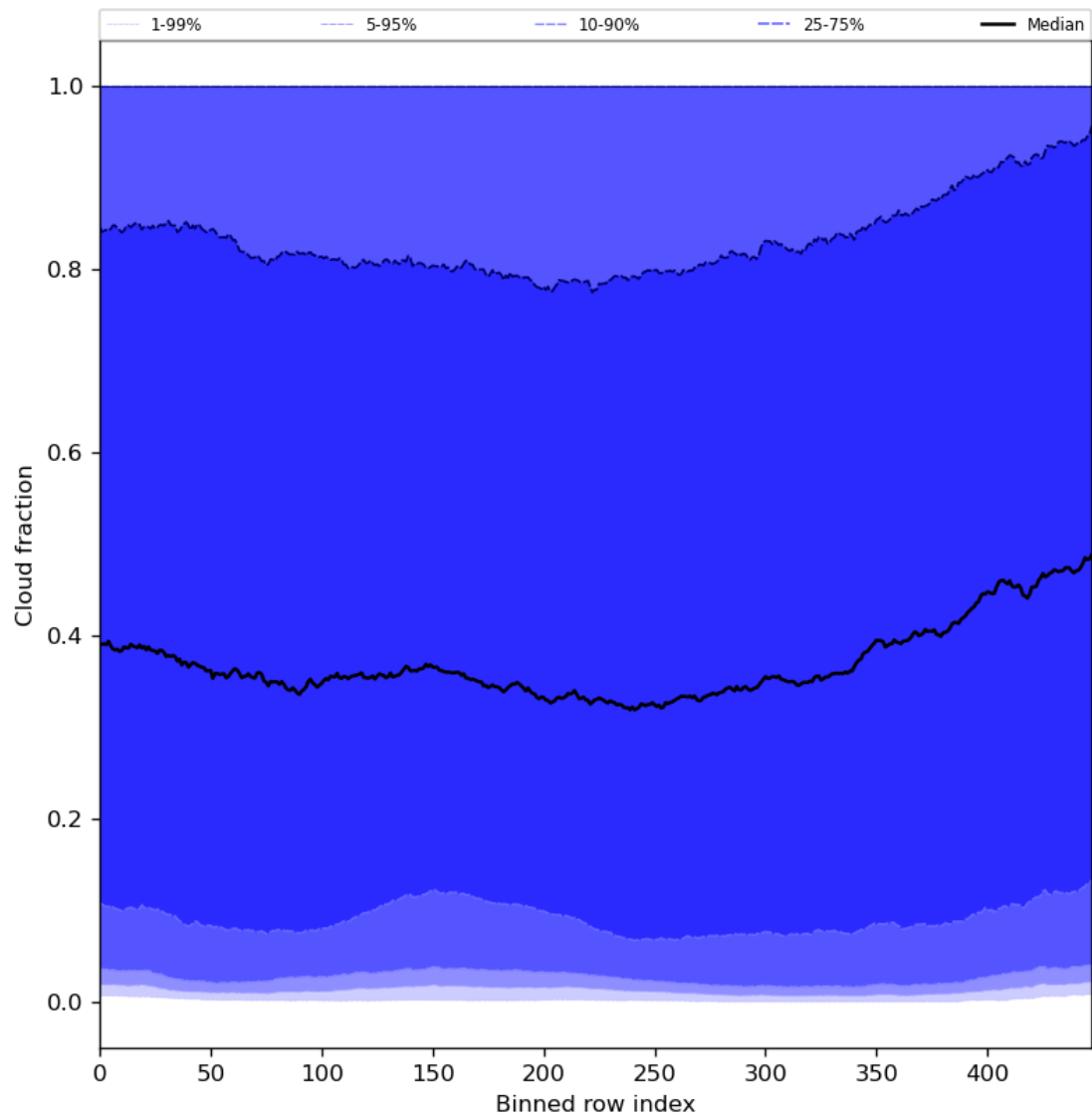
Figure 49: Along track statistics of “Cloud fraction” for 2024-05-24 to 2024-05-26
