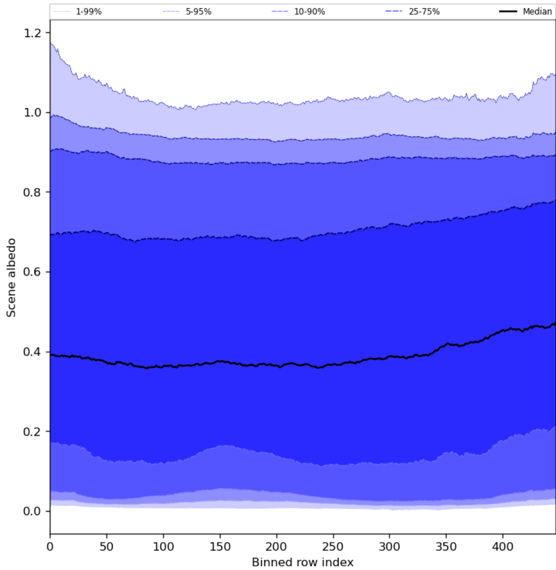
Figure 51: Along track statistics of “Scene albedo” for 2024-05-24 to 2024-05-26
