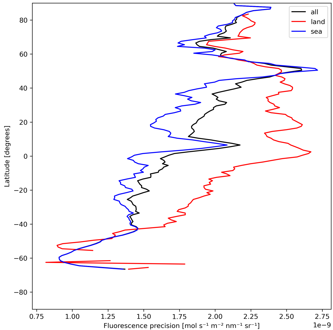
Figure 24: Zonal average of “Fluorescence precision” for 2024-05-24 to 2024-05-26.
