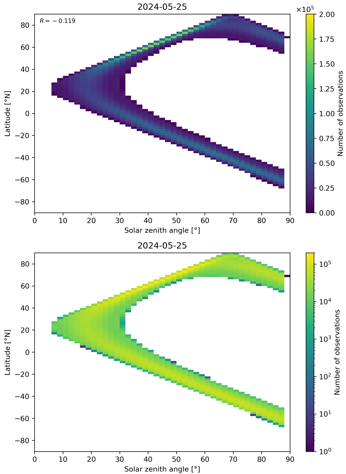
Figure 113: Scatter density plot of “Solar zenith angle” against “Latitude” for 2024-05-24 to 2024-05-26.
