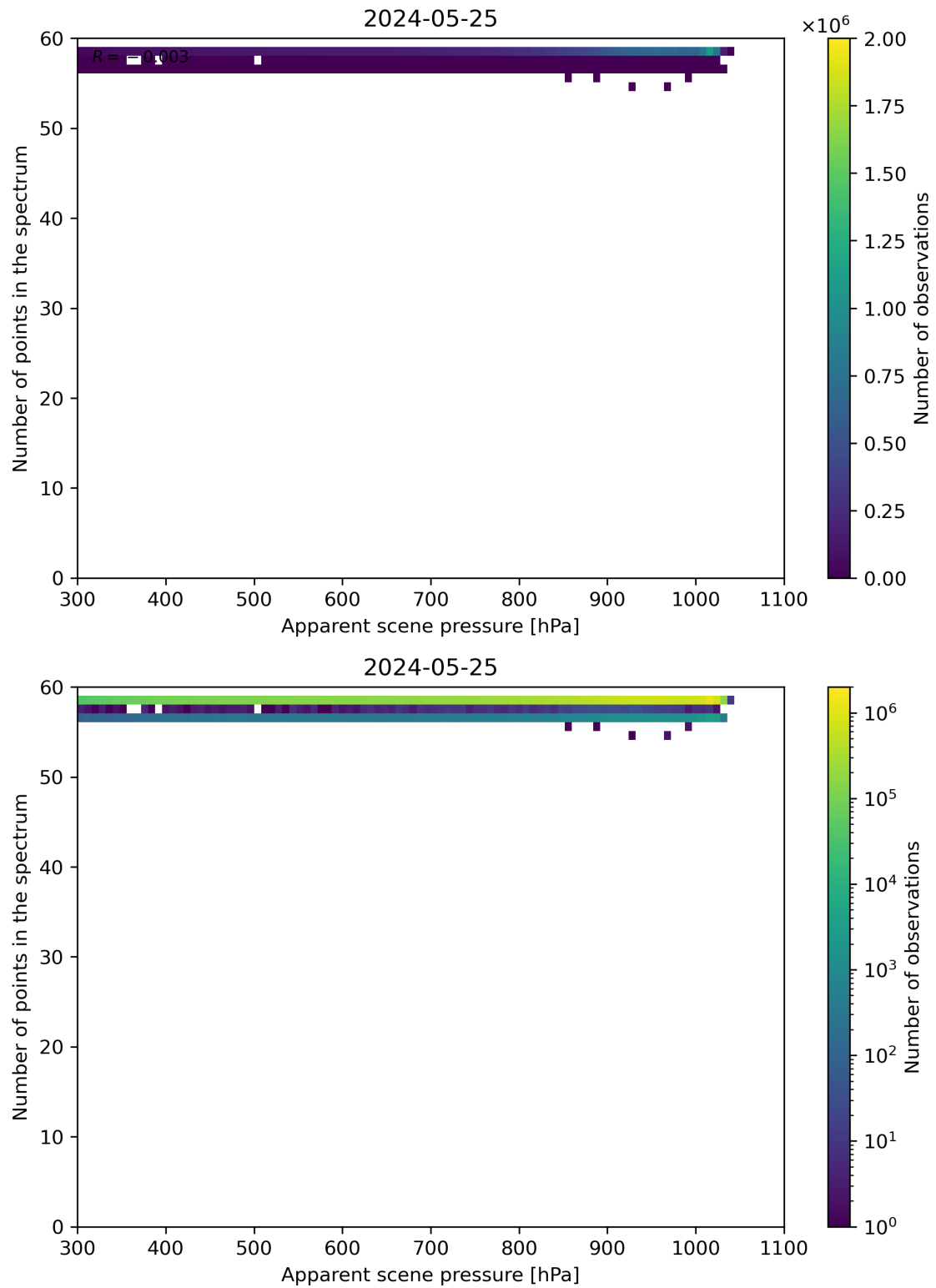
Figure 66: Scatter density plot of “Apparent scene pressure” against “Number of points in the spectrum” for 2024-05-24 to 2024-05-26.
