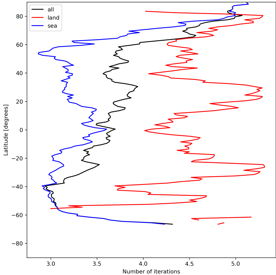
Figure 22: Zonal average of “Number of iterations” for 2024-05-24 to 2024-05-26.
