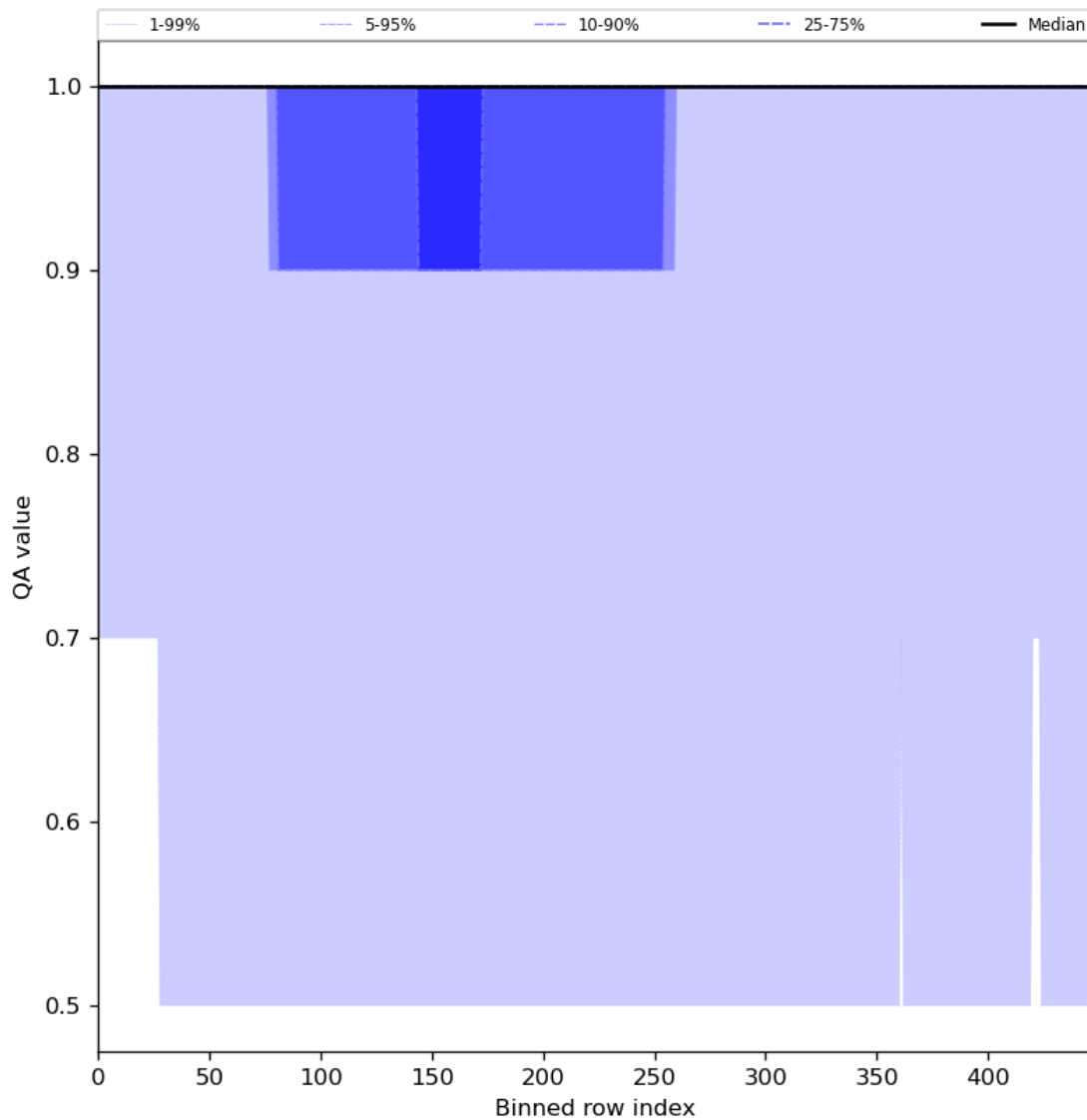
Figure 46: Along track statistics of “QA value” for 2024-05-24 to 2024-05-26
