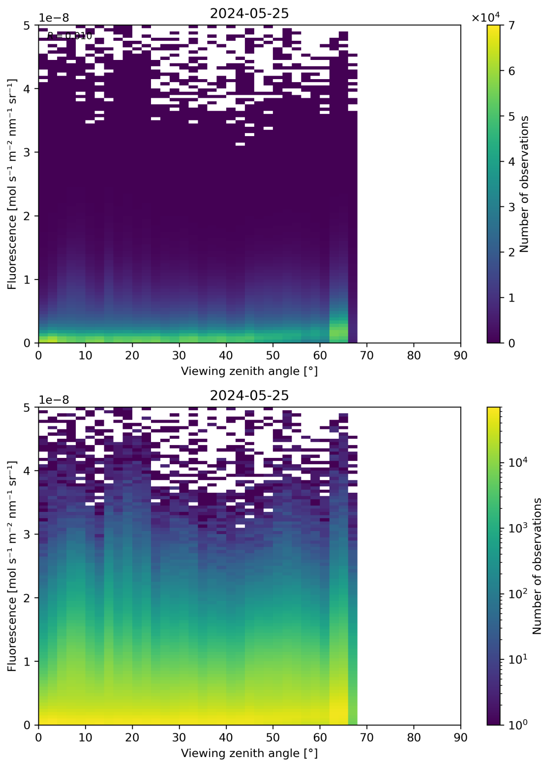
Figure 122: Scatter density plot of “Viewing zenith angle” against “Fluorescence” for 2024-05-24 to 2024-05-26.
