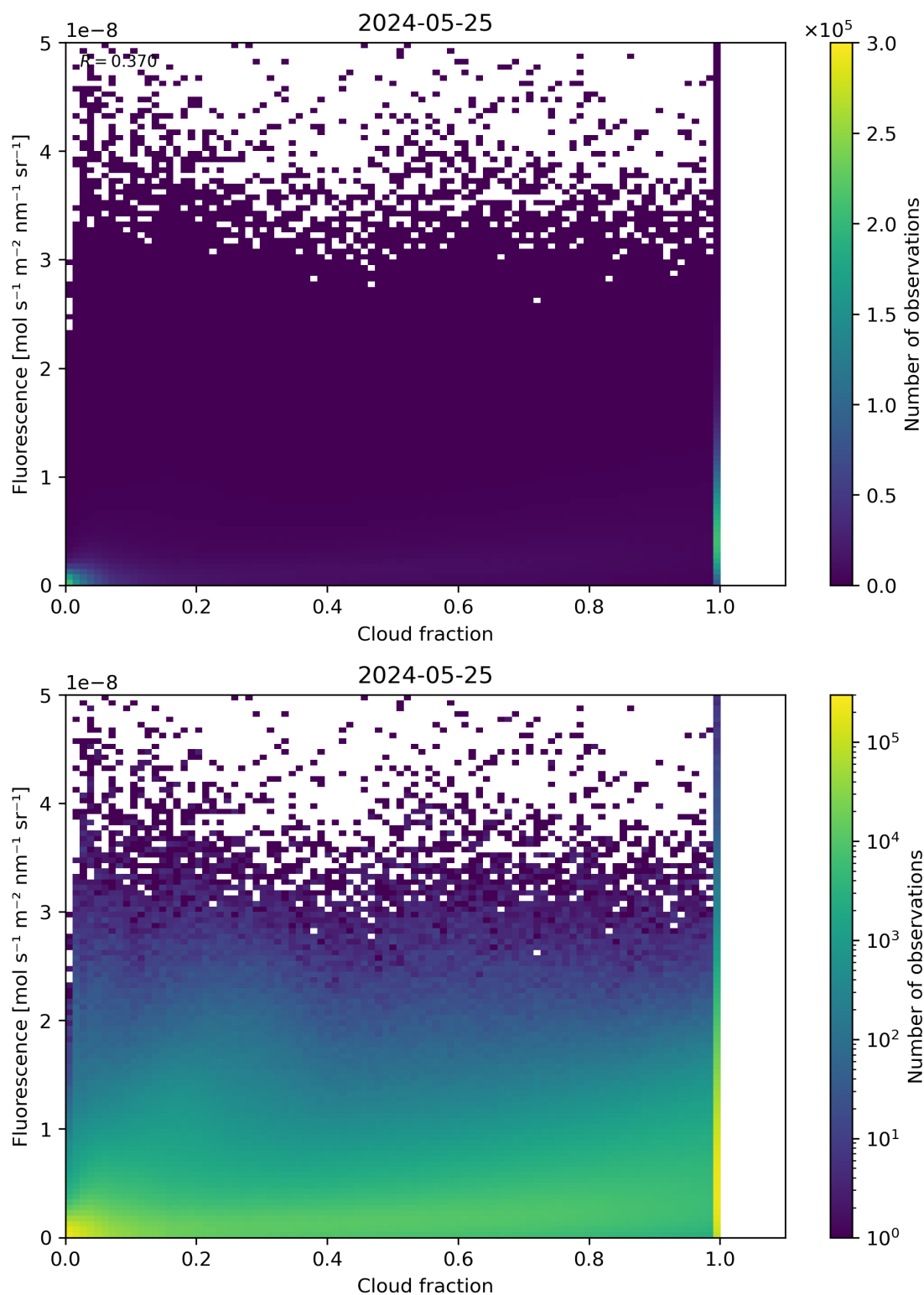
Figure 72: Scatter density plot of “Cloud fraction” against “Fluorescence” for 2024-05-24 to 2024-05-26.
