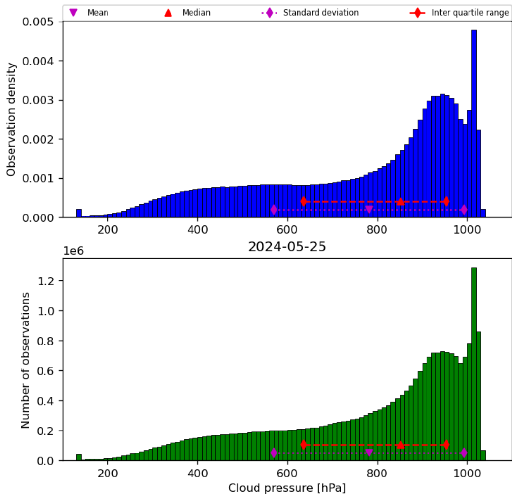
Figure 30: Histogram of “Cloud pressure” for 2024-05-24 to 2024-05-26
