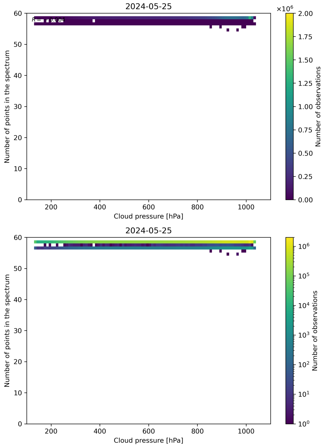
Figure 82: Scatter density plot of “Cloud pressure” against “Number of points in the spectrum” for 2024-05-24 to 2024-05-26.
