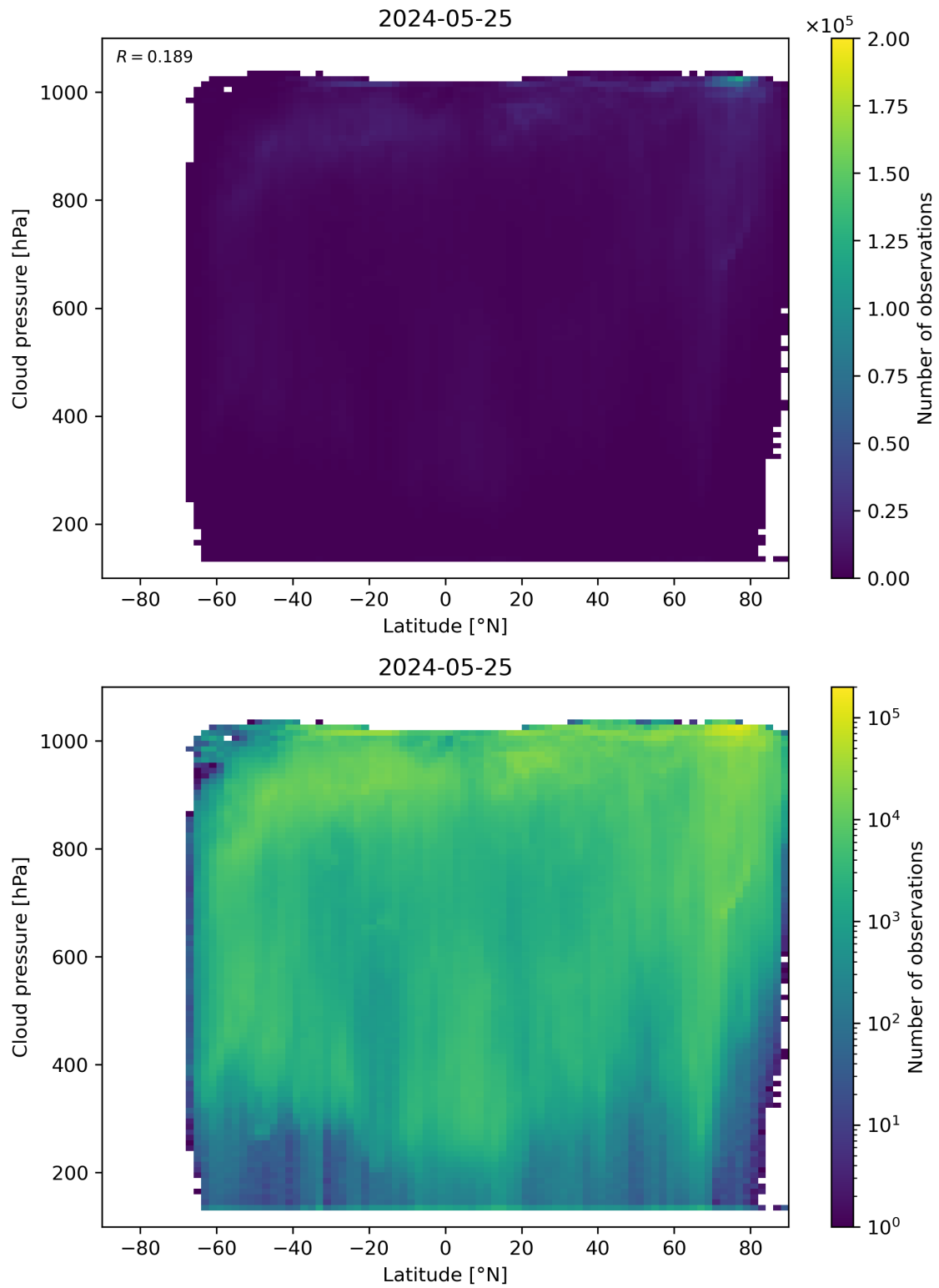
Figure 91: Scatter density plot of “Latitude” against “Cloud pressure” for 2024-05-24 to 2024-05-26.
