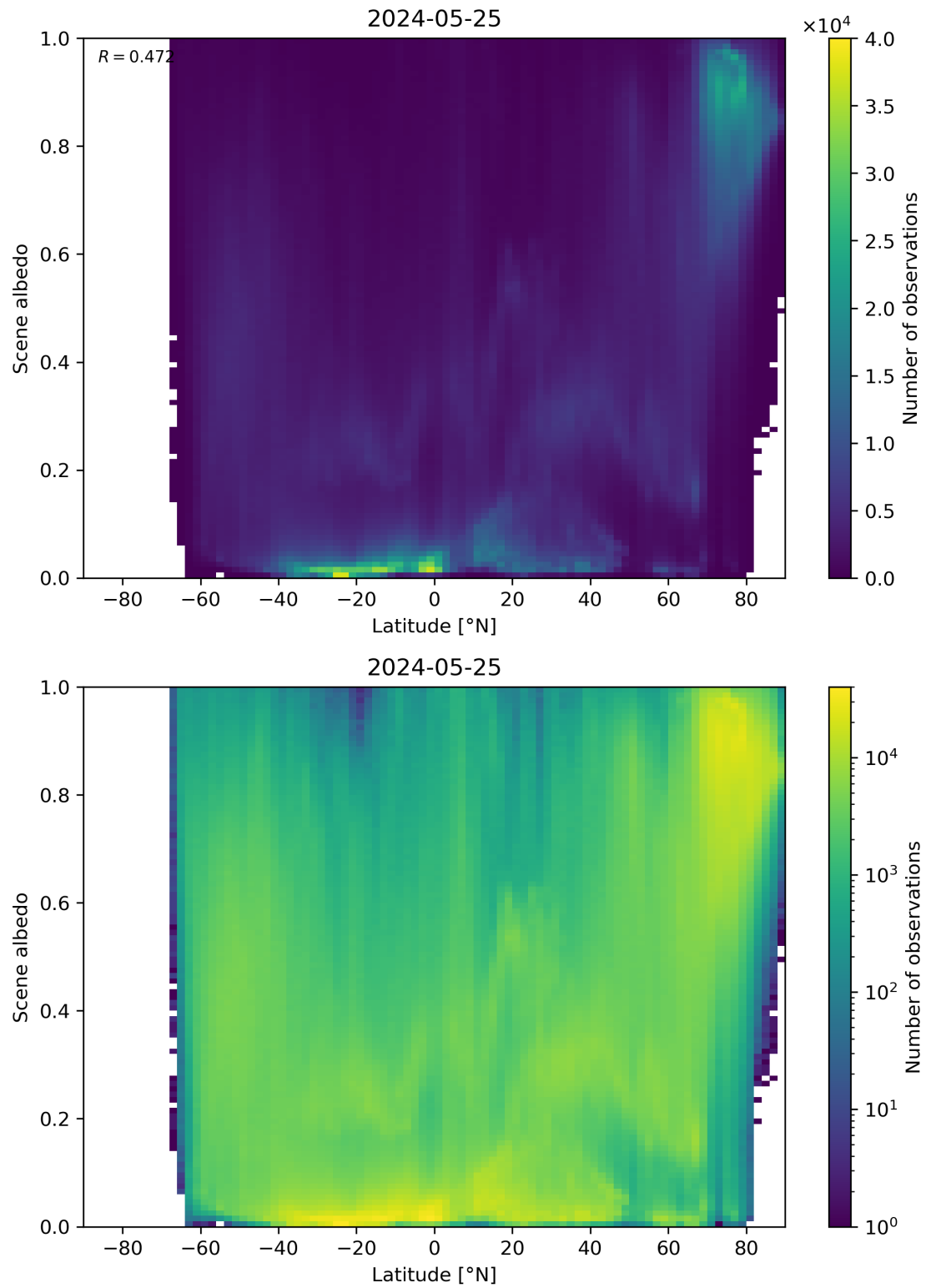
Figure 95: Scatter density plot of “Latitude” against “Scene albedo” for 2024-05-24 to 2024-05-26.
