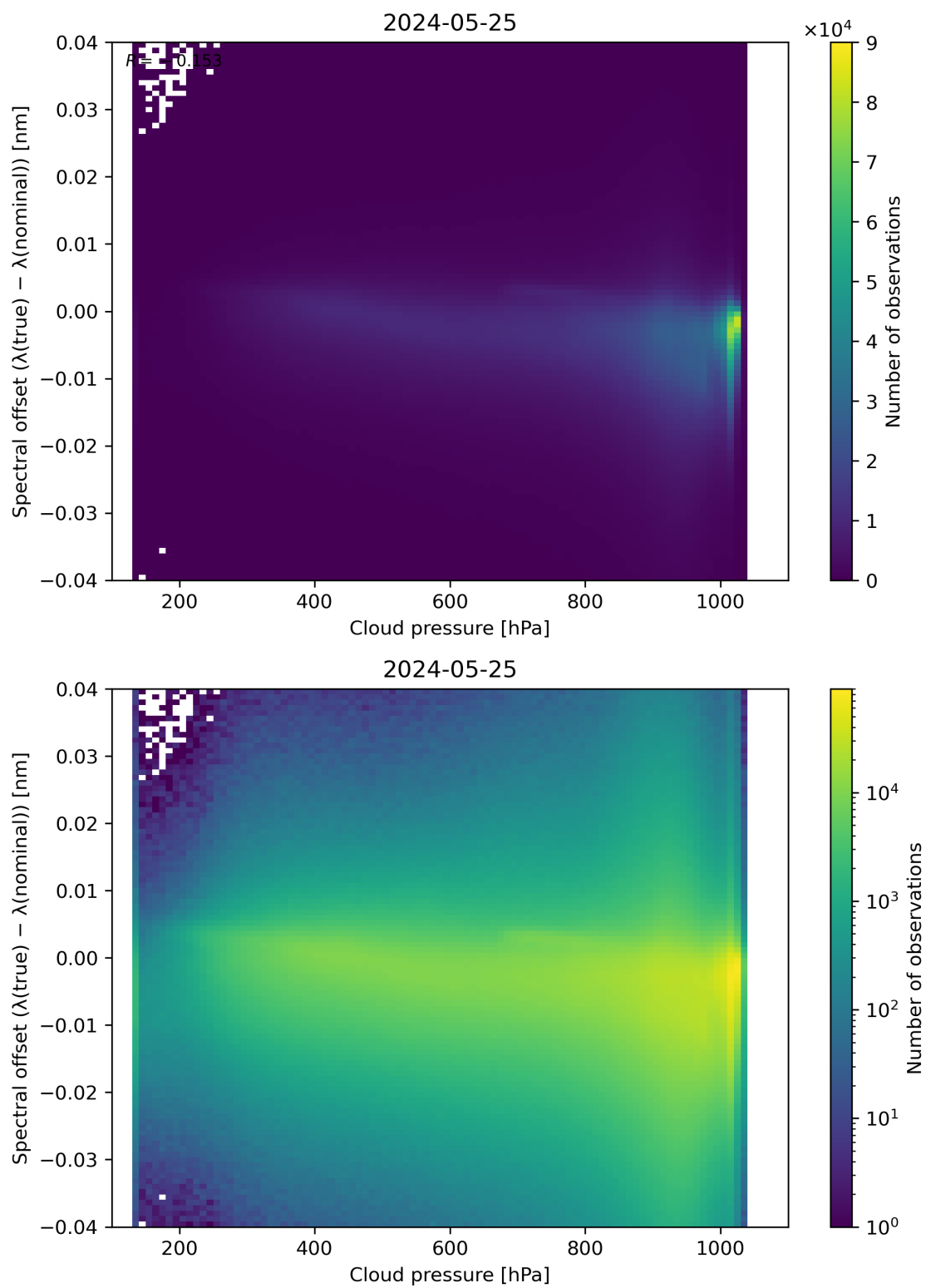
Figure 84: Scatter density plot of “Cloud pressure” against “Spectral offset ( \lambda(\text{true}) - \lambda(\text{nominal}) )” for 2024-05-24 to 2024-05-26.
