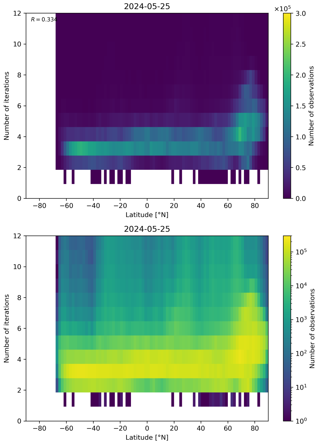
Figure 93: Scatter density plot of “Latitude” against “Number of iterations” for 2024-05-24 to 2024-05-26.
