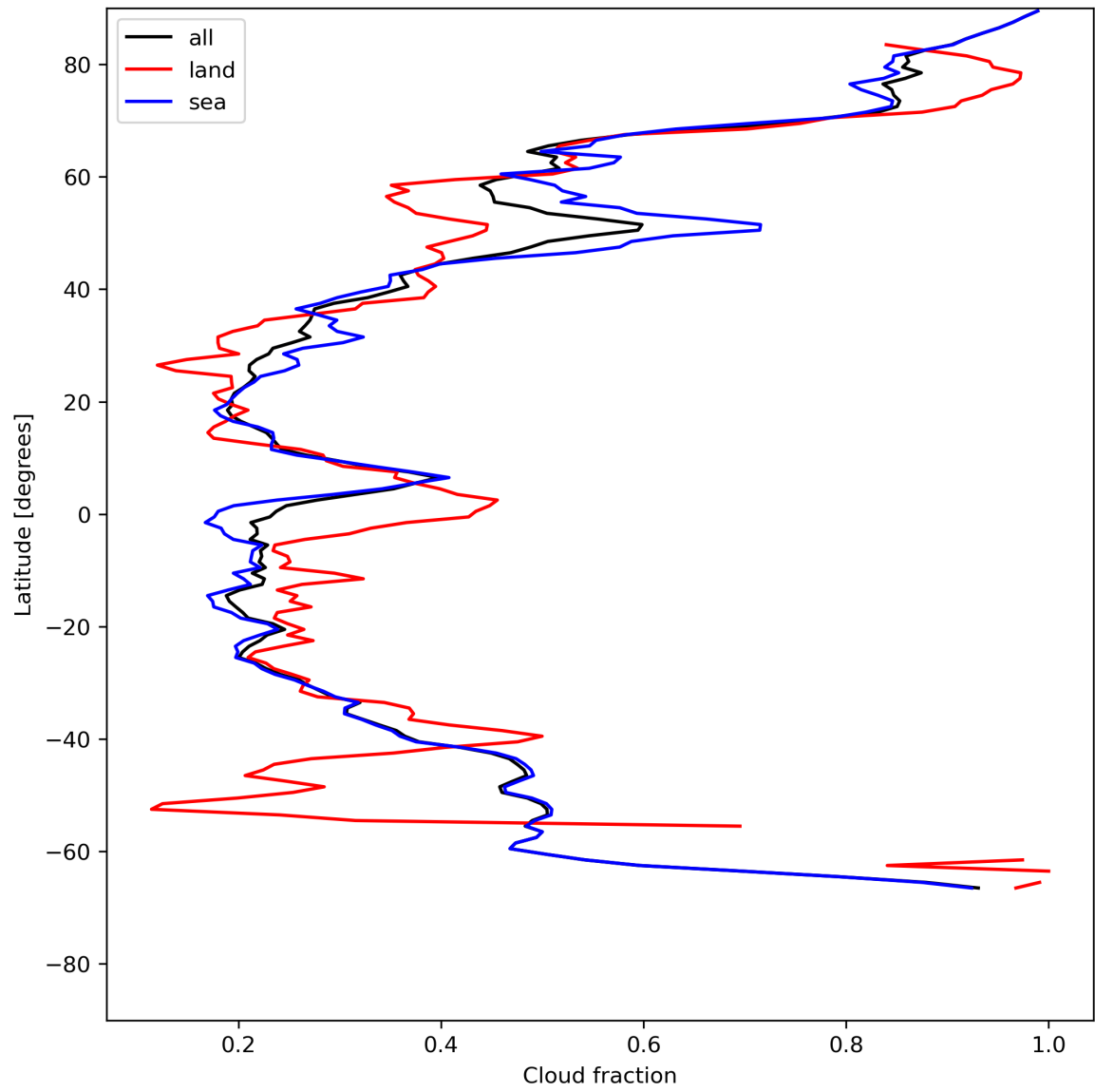
Figure 15: Zonal average of “Cloud fraction” for 2024-05-24 to 2024-05-26.
