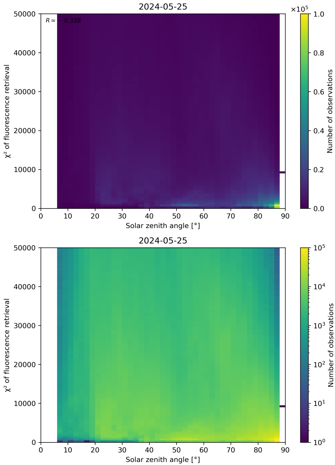
Figure 109: Scatter density plot of “Solar zenith angle” against “ \chi^2 of fluorescence retrieval” for 2024-05-24 to 2024-05-26.
