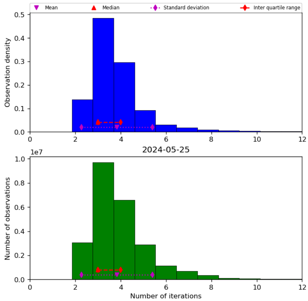
Figure 39: Histogram of “Number of iterations” for 2024-05-24 to 2024-05-26
