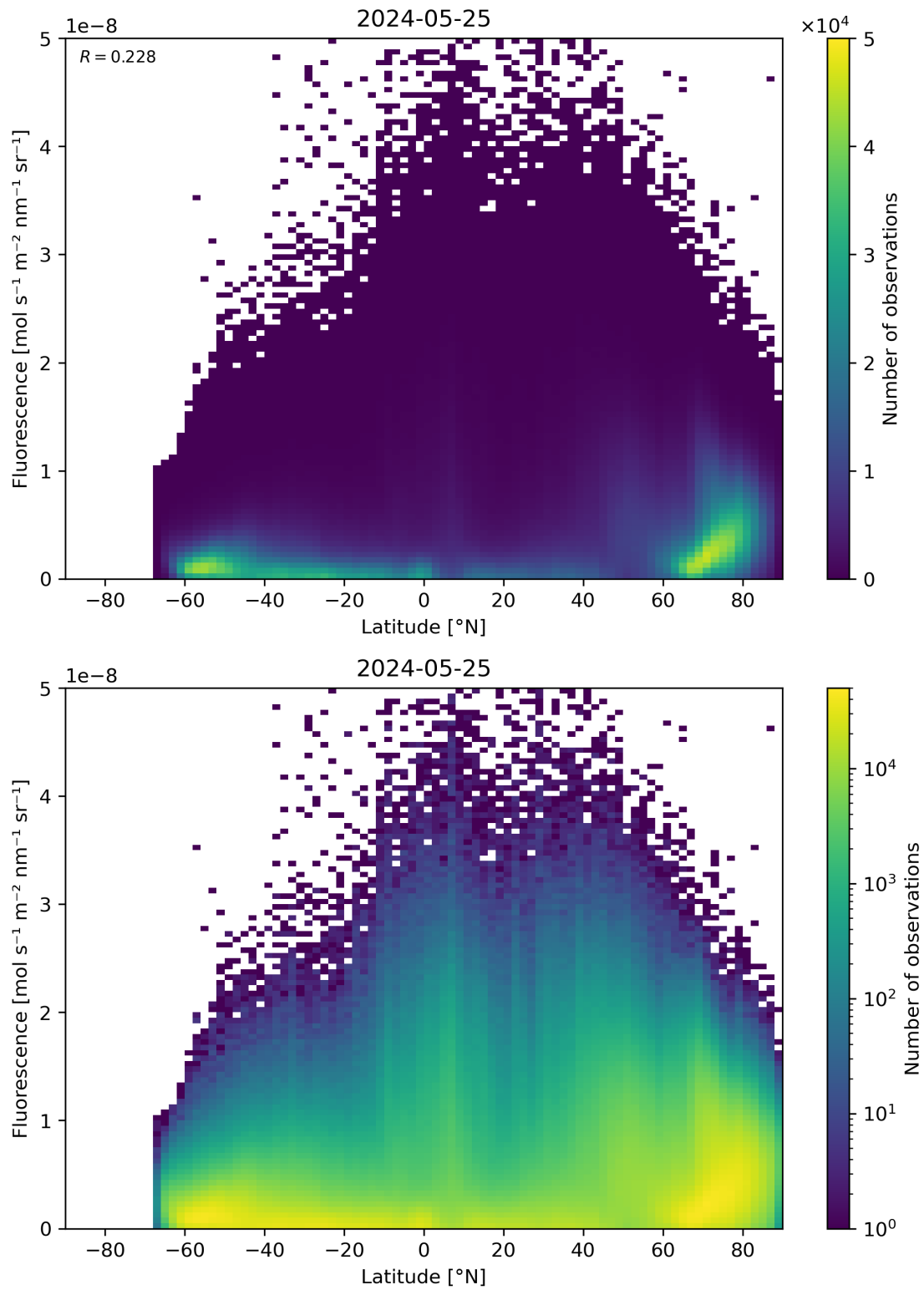
Figure 92: Scatter density plot of “Latitude” against “Fluorescence” for 2024-05-24 to 2024-05-26.
