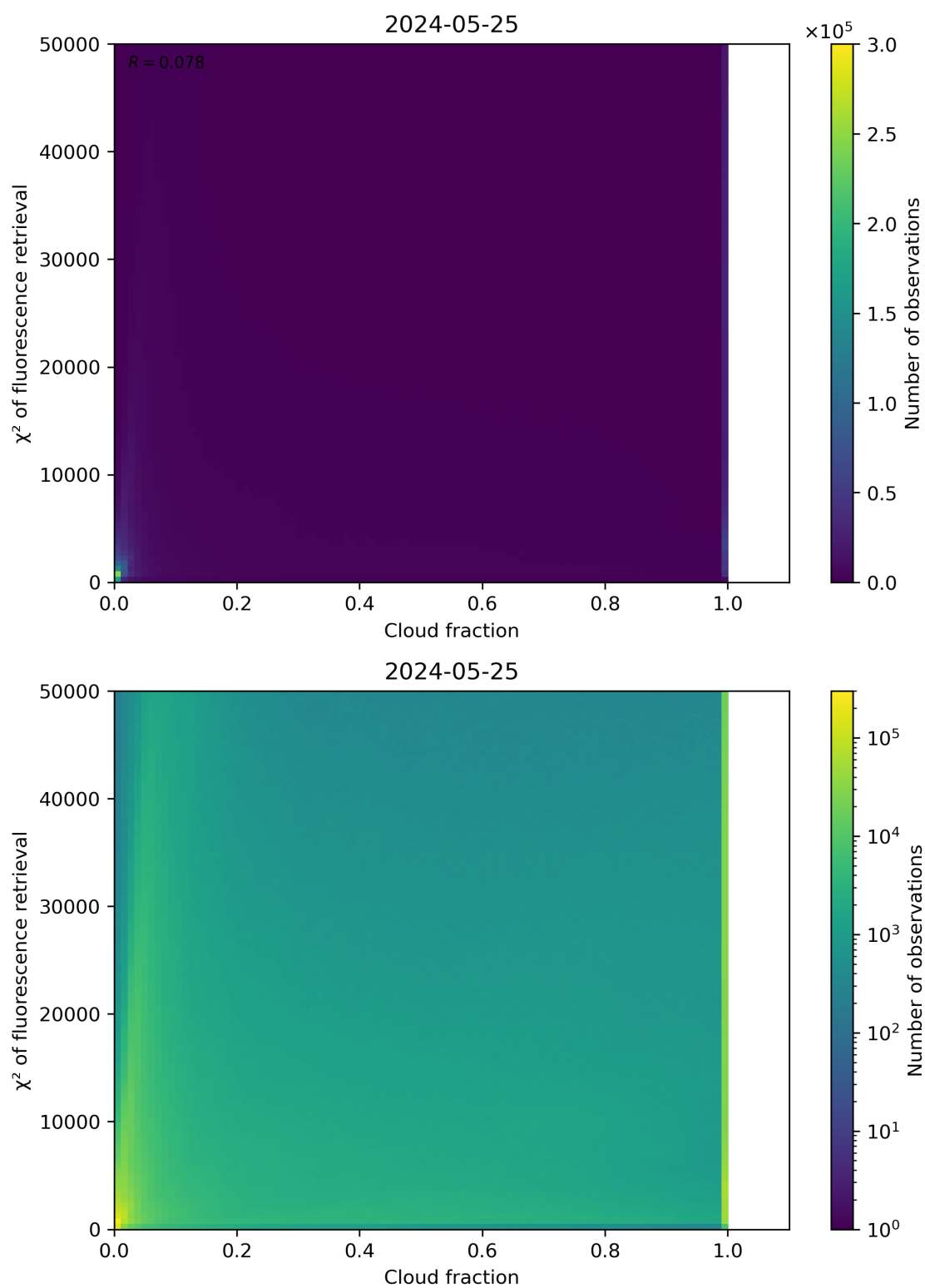
Figure 71: Scatter density plot of “Cloud fraction” against “ \chi^2 of fluorescence retrieval” for 2024-05-24 to 2024-05-26.
