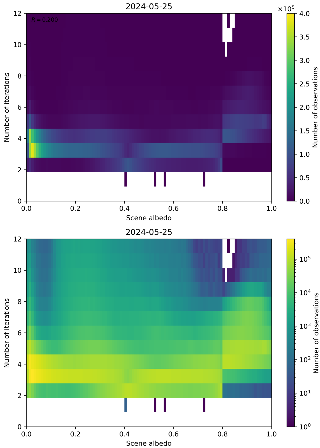
Figure 105: Scatter density plot of “Scene albedo” against “Number of iterations” for 2024-05-24 to 2024-05-26.
