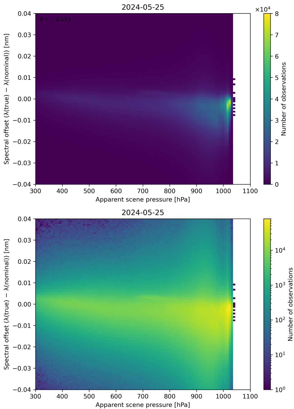
Figure 67: Scatter density plot of “Apparent scene pressure” against “Spectral offset ( \lambda(\text{true}) - \lambda(\text{nominal}) )” for 2024-05-24 to 2024-05-26.
