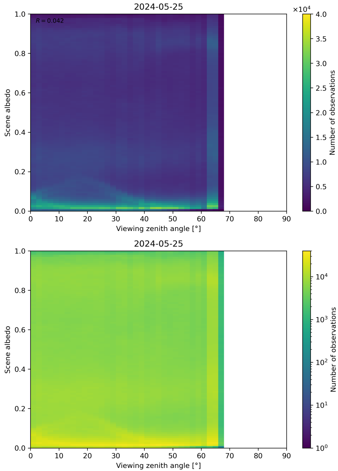
Figure 126: Scatter density plot of “Viewing zenith angle” against “Scene albedo” for 2024-05-24 to 2024-05-26.
