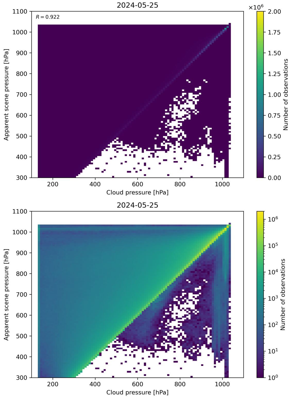
Figure 77: Scatter density plot of “Cloud pressure” against “Apparent scene pressure” for 2024-05-24 to 2024-05-26.
