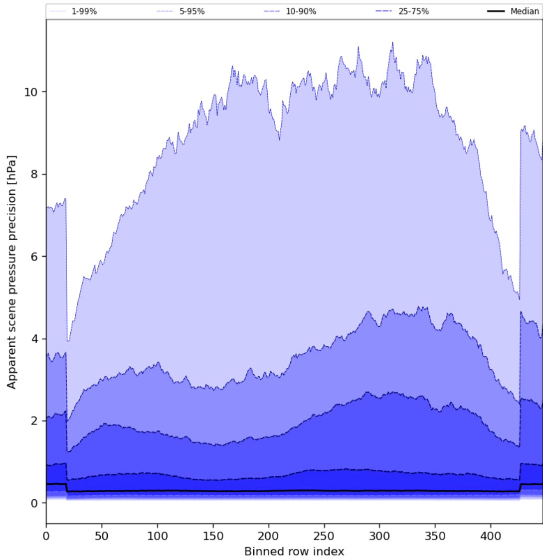
Figure 54: Along track statistics of “Apparent scene pressure precision” for 2024-05-24 to 2024-05-26
