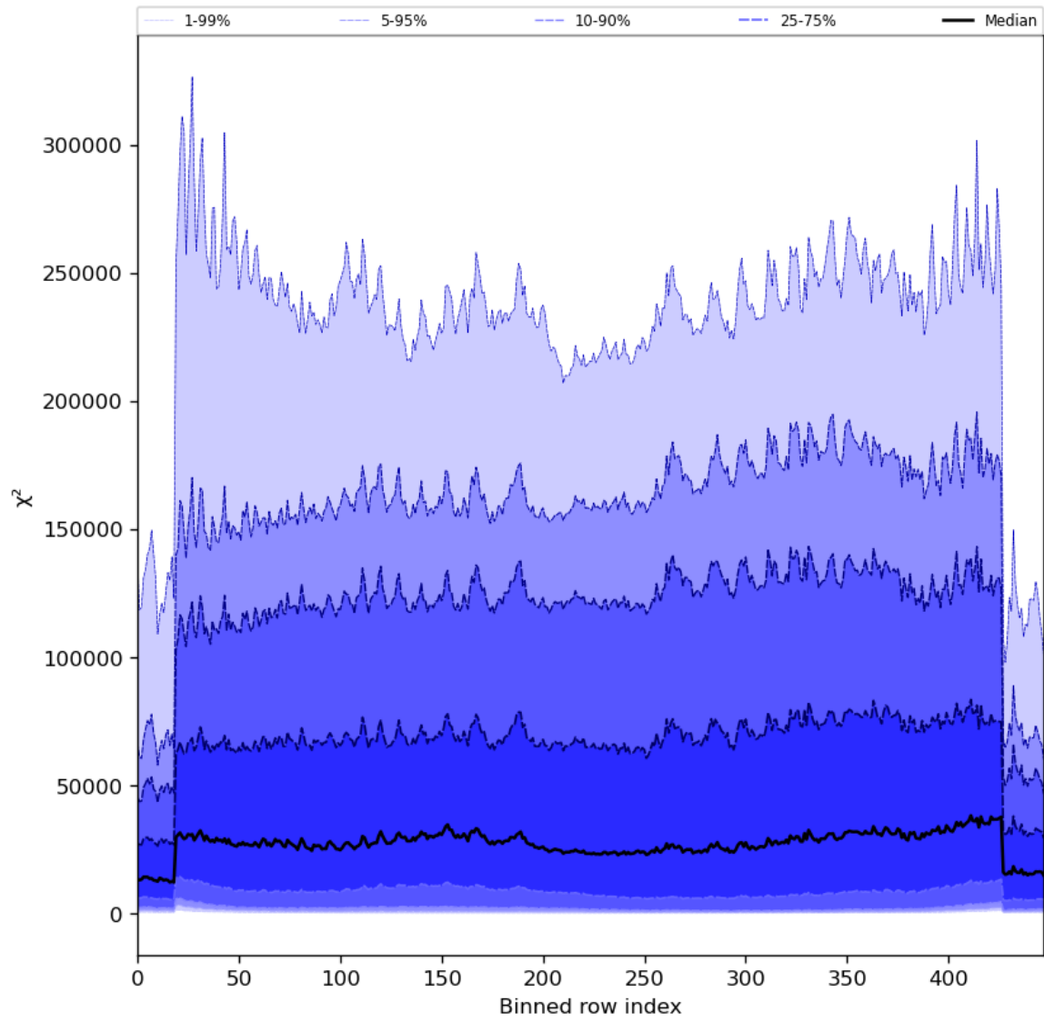
Figure 55: Along track statistics of “ \chi^2 ” for 2024-05-24 to 2024-05-26
