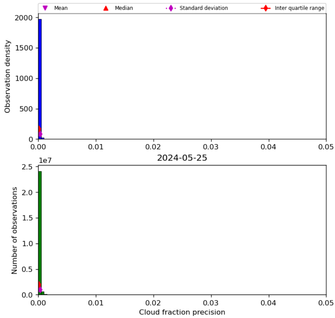
Figure 33: Histogram of “Cloud fraction precision” for 2024-05-24 to 2024-05-26
