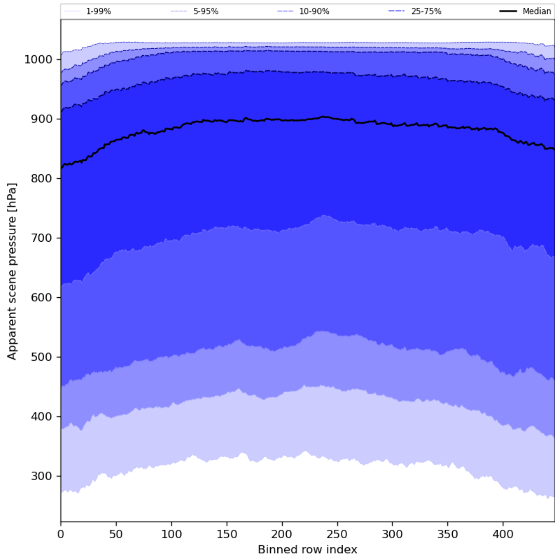
Figure 53: Along track statistics of “Apparent scene pressure” for 2024-05-24 to 2024-05-26
