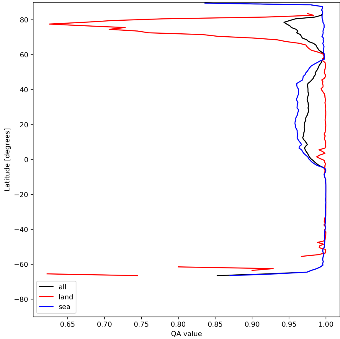
Figure 12: Zonal average of “QA value” for 2024-05-24 to 2024-05-26.
