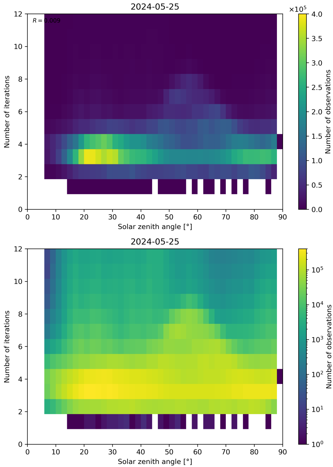
Figure 114: Scatter density plot of “Solar zenith angle” against “Number of iterations” for 2024-05-24 to 2024-05-26.
