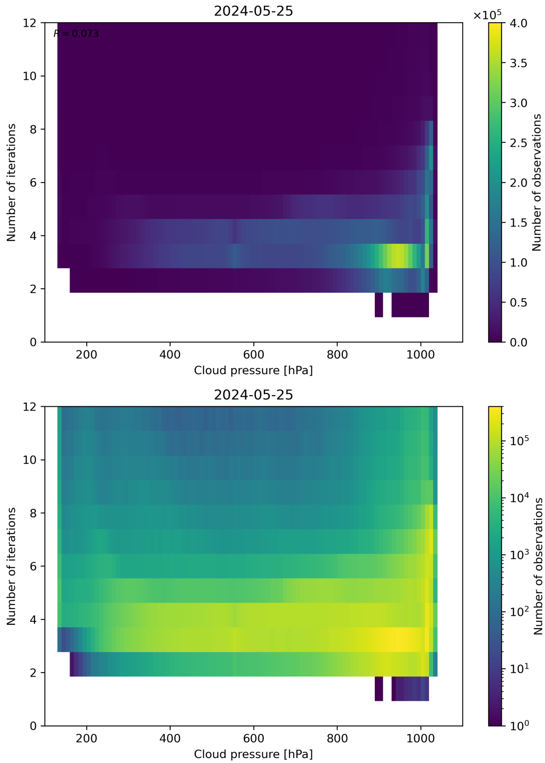
Figure 81: Scatter density plot of “Cloud pressure” against “Number of iterations” for 2024-05-24 to 2024-05-26.
