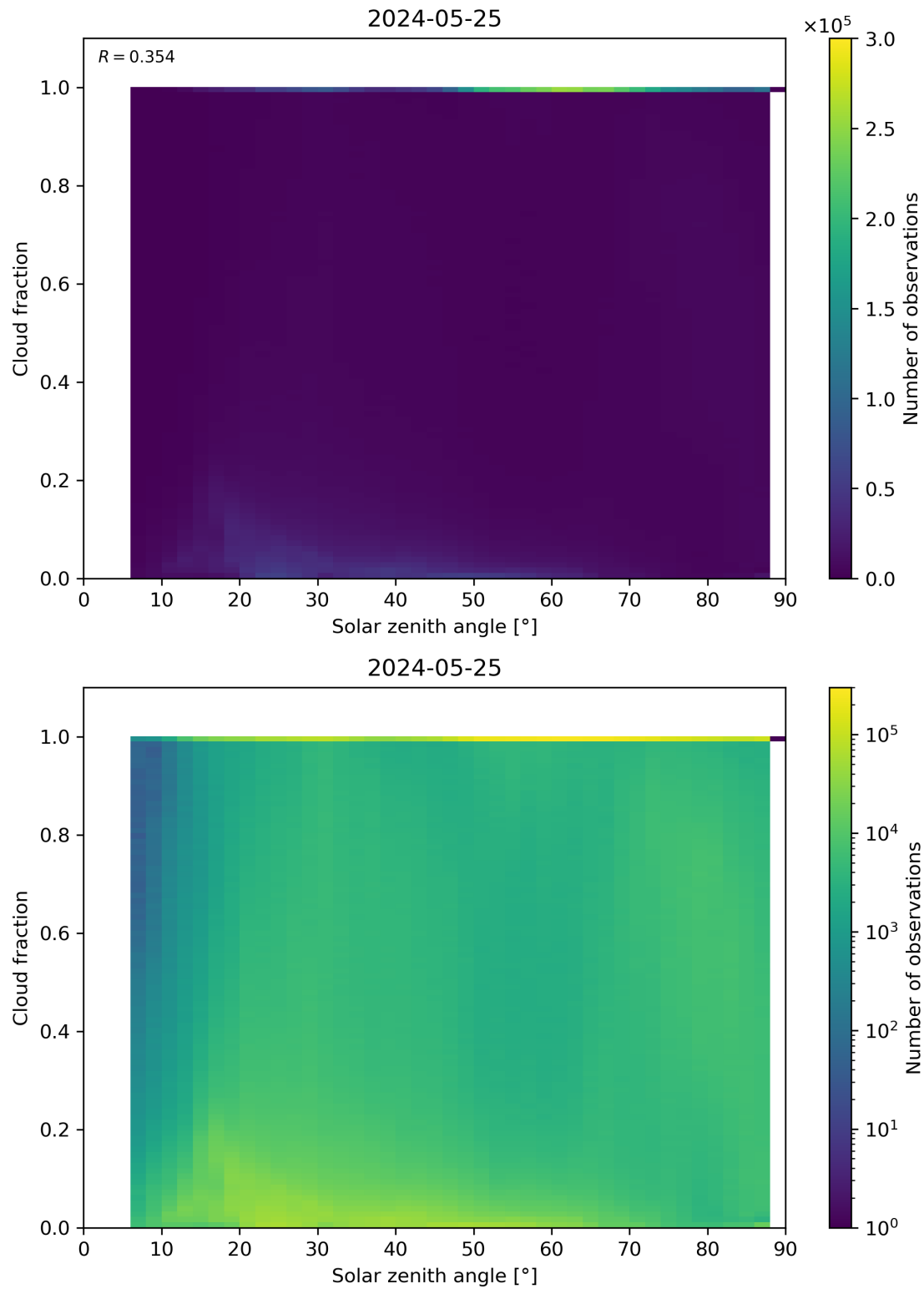
Figure 110: Scatter density plot of “Solar zenith angle” against “Cloud fraction” for 2024-05-24 to 2024-05-26.
