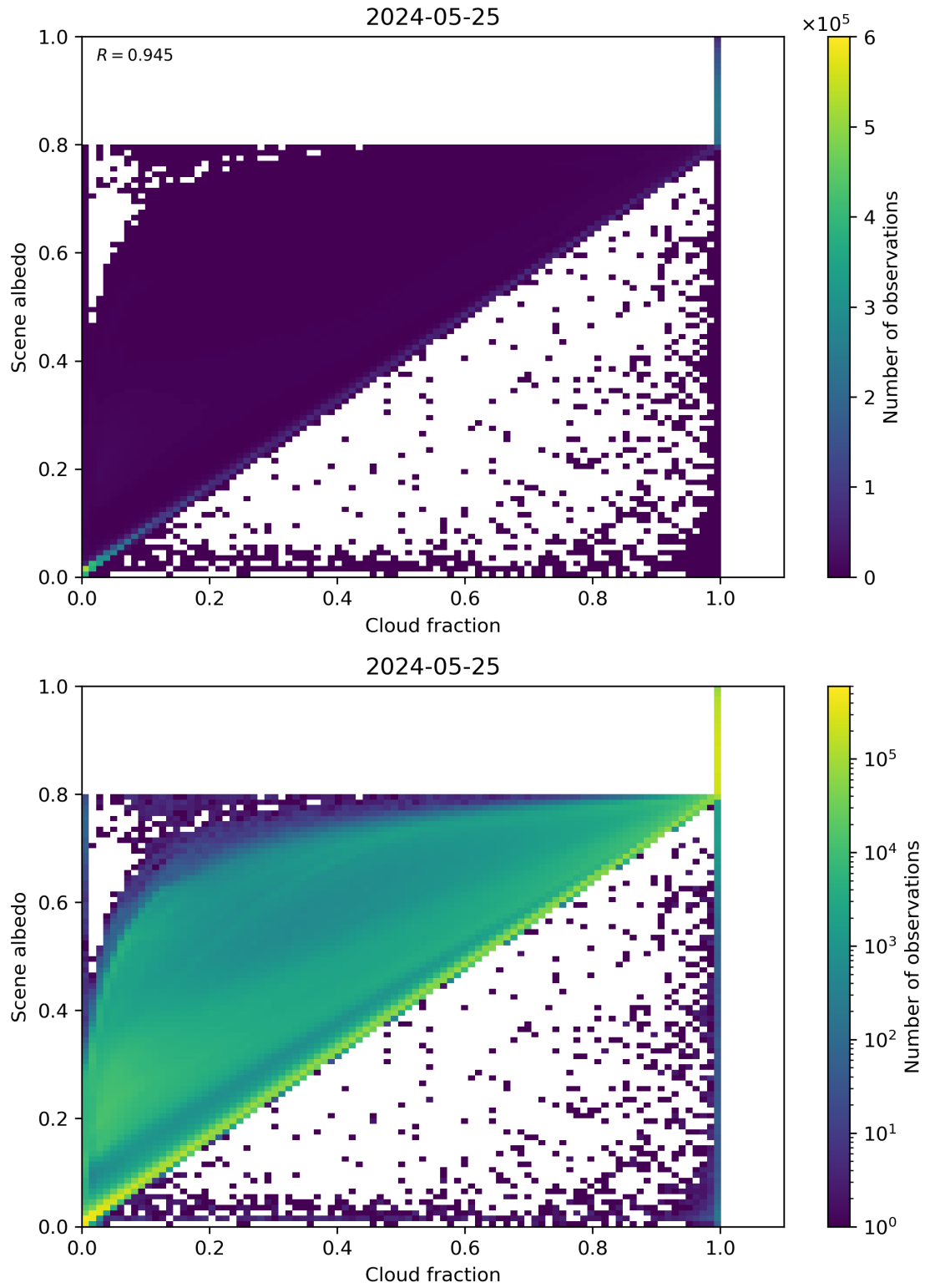
Figure 75: Scatter density plot of “Cloud fraction” against “Scene albedo” for 2024-05-24 to 2024-05-26.
