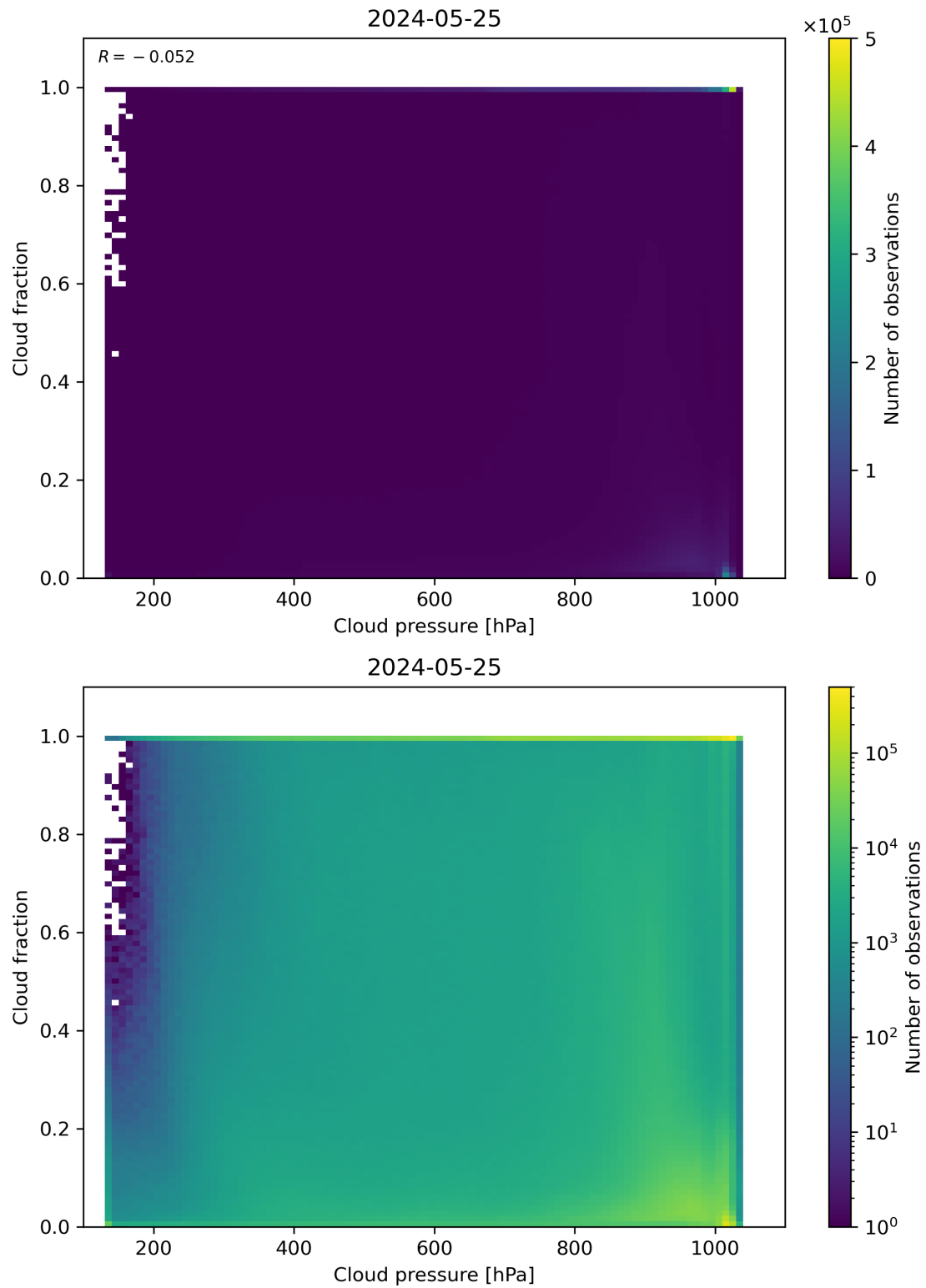
Figure 79: Scatter density plot of “Cloud pressure” against “Cloud fraction” for 2024-05-24 to 2024-05-26.
