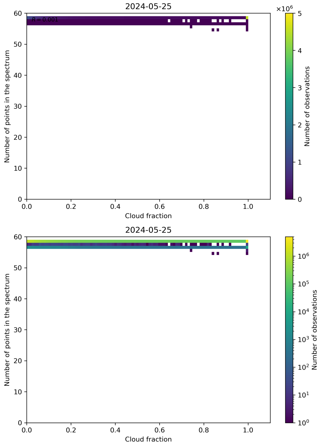
Figure 74: Scatter density plot of “Cloud fraction” against “Number of points in the spectrum” for 2024-05-24 to 2024-05-26.
