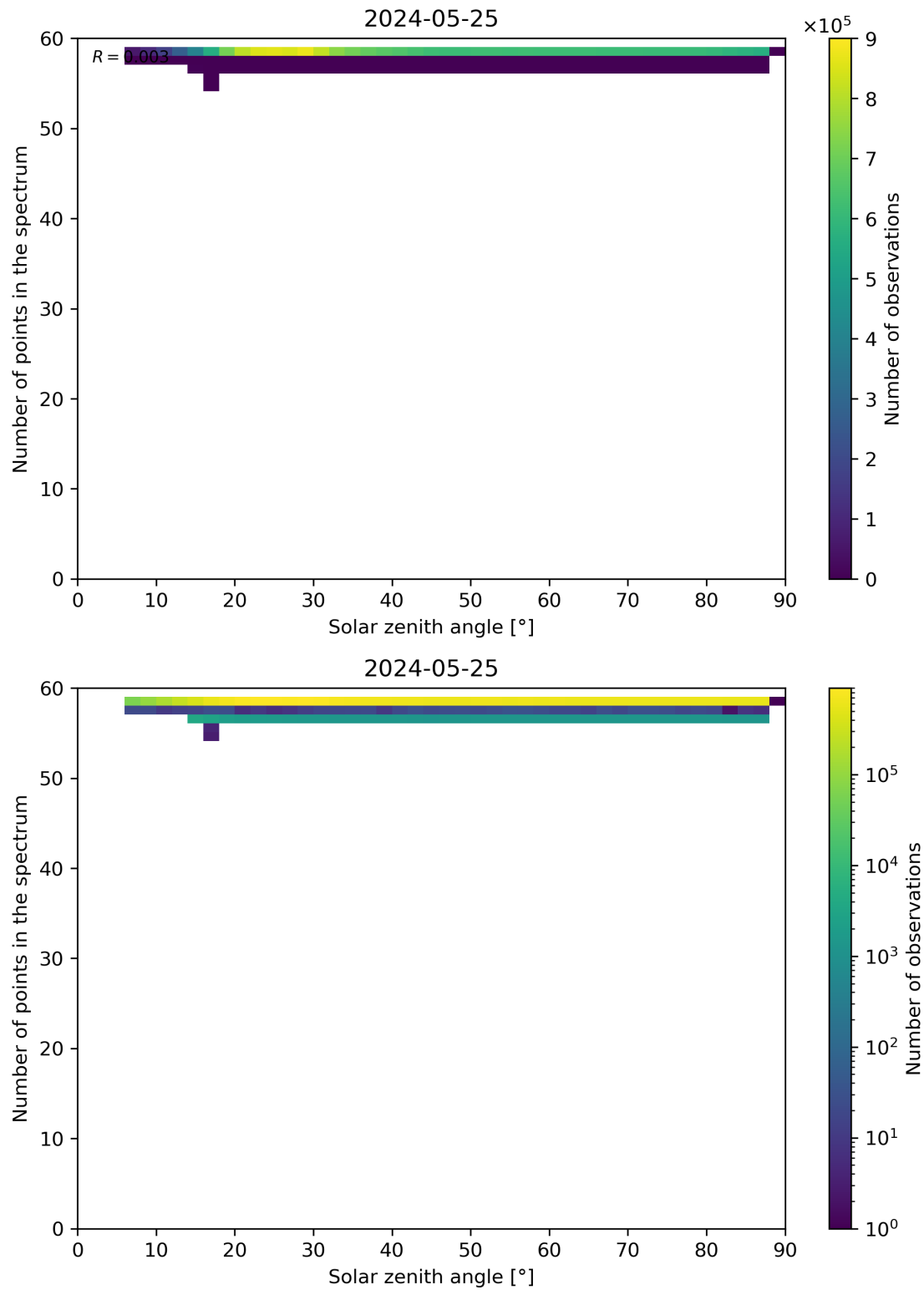
Figure 115: Scatter density plot of “Solar zenith angle” against “Number of points in the spectrum” for 2024-05-24 to 2024-05-26.
