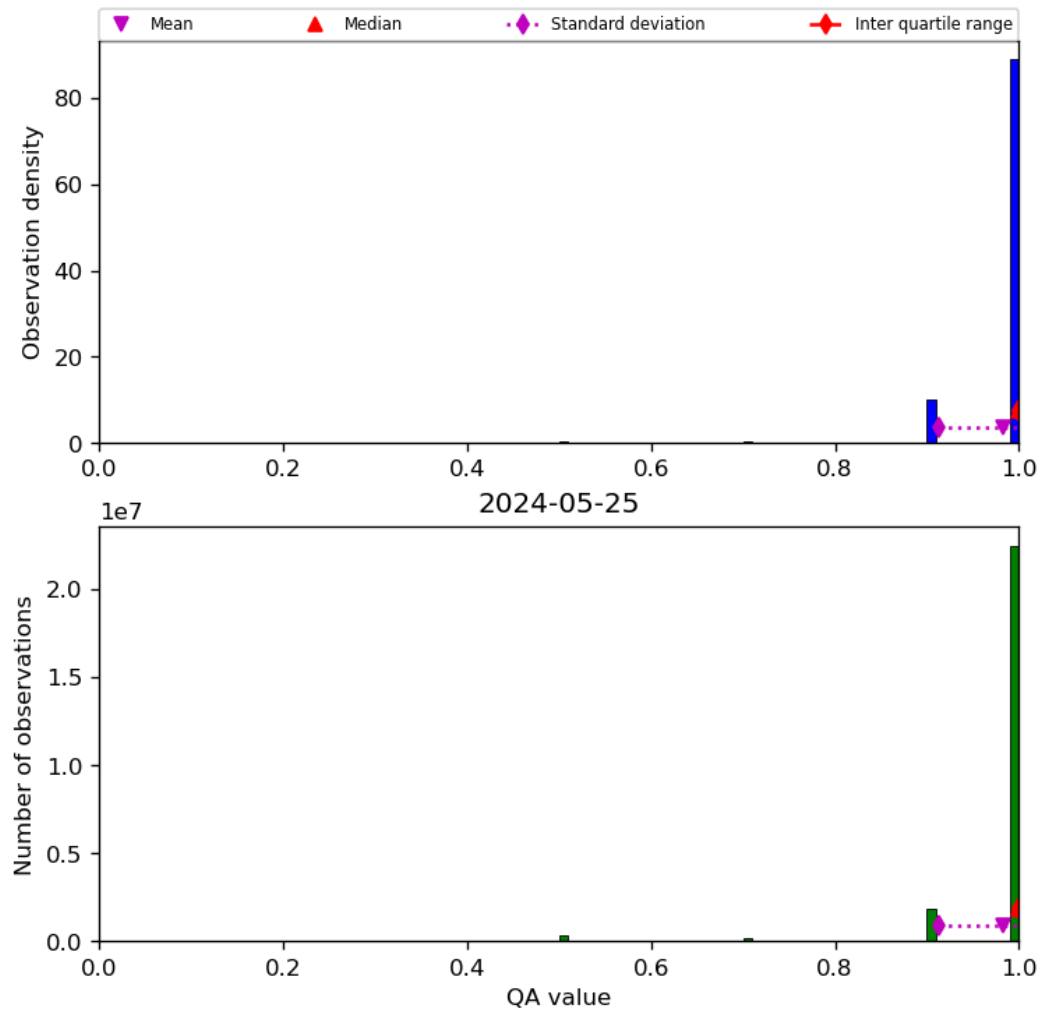
Figure 29: Histogram of “QA value” for 2024-05-24 to 2024-05-26
