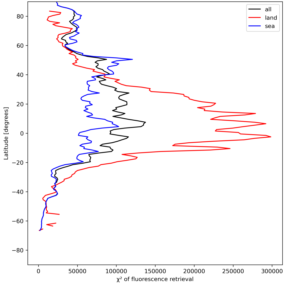
Figure 25: Zonal average of “ \chi^2 of fluorescence retrieval” for 2024-05-24 to 2024-05-26.
