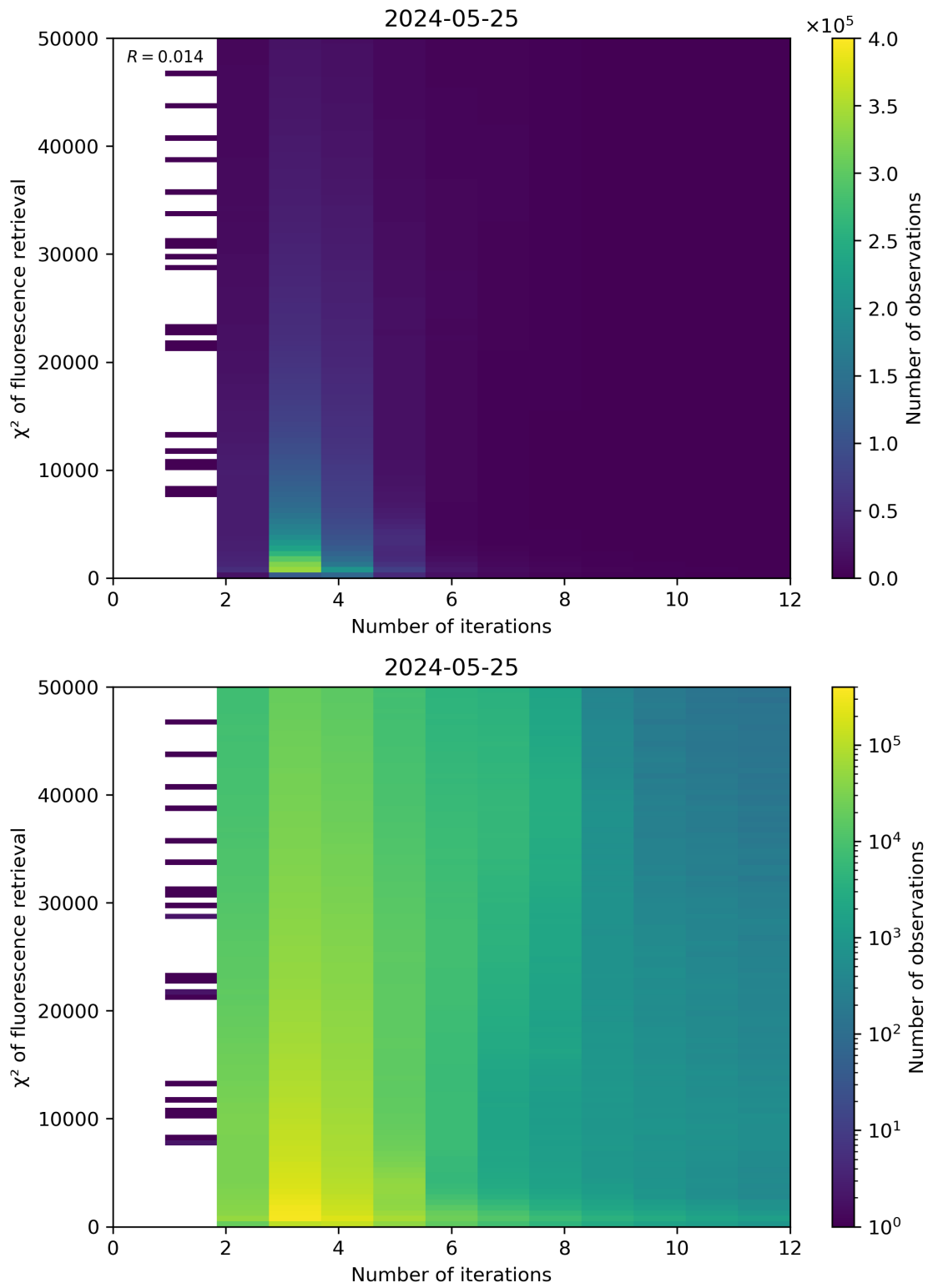
Figure 97: Scatter density plot of “Number of iterations” against “ \chi^2 of fluorescence retrieval” for 2024-05-24 to 2024-05-26.
