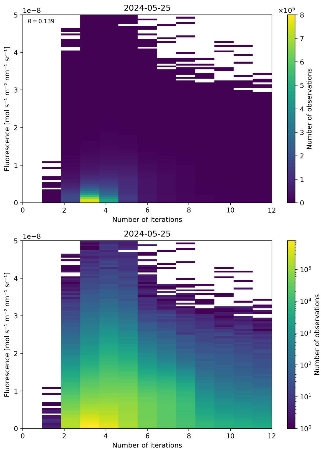
Figure 98: Scatter density plot of “Number of iterations” against “Fluorescence” for 2024-05-24 to 2024-05-26.
