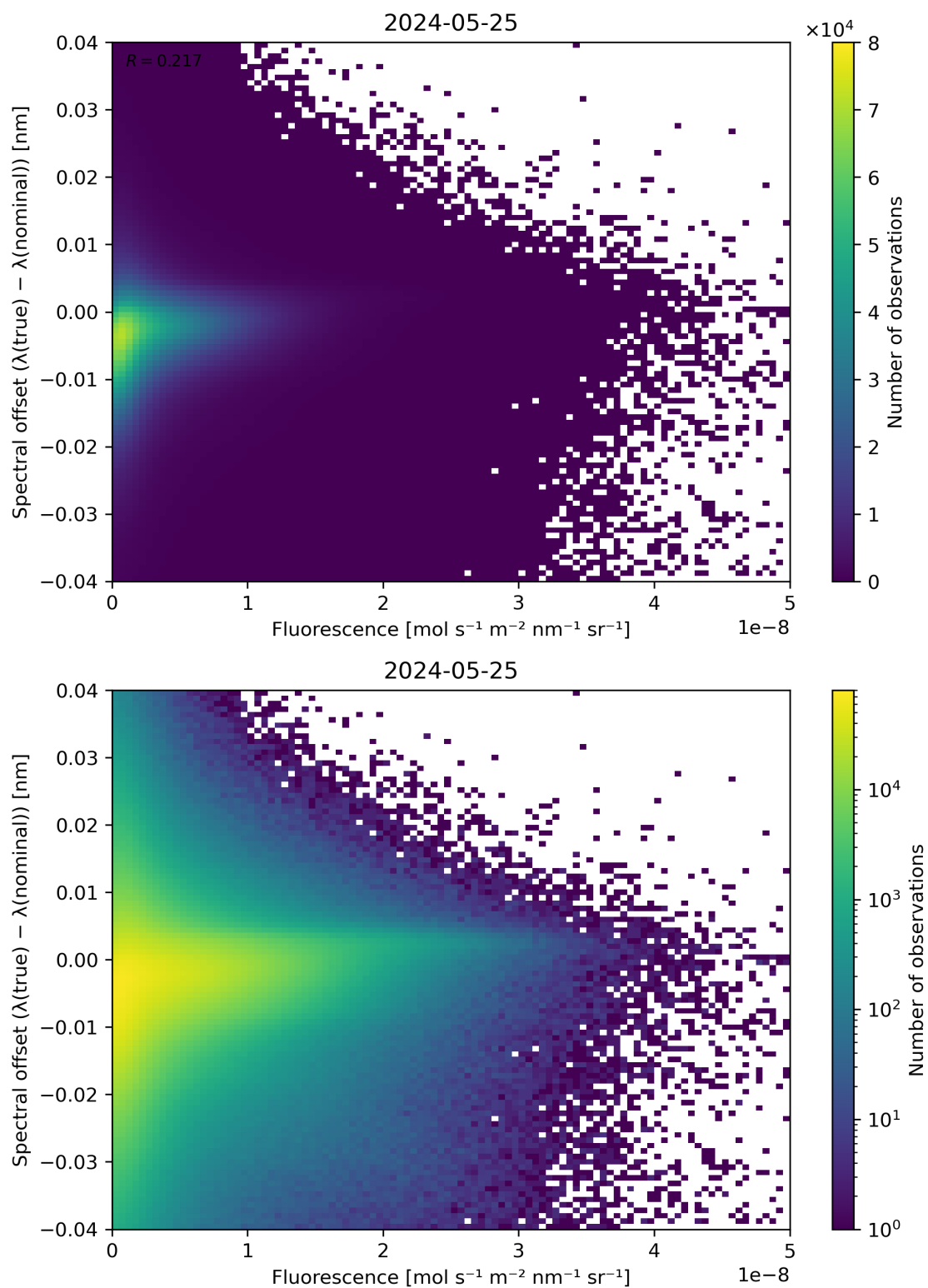
Figure 87: Scatter density plot of “Fluorescence” against “Spectral offset ( \lambda(\text{true}) - \lambda(\text{nominal}) )” for 2024-05-24 to 2024-05-26.
