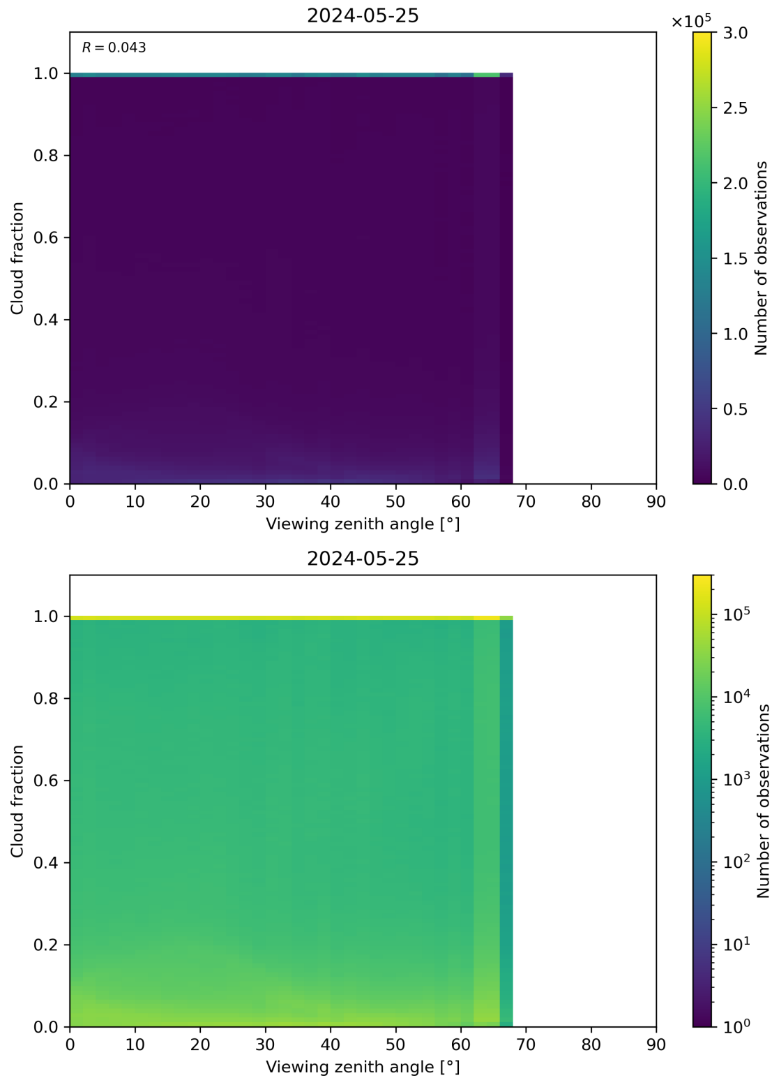
Figure 120: Scatter density plot of “Viewing zenith angle” against “Cloud fraction” for 2024-05-24 to 2024-05-26.
