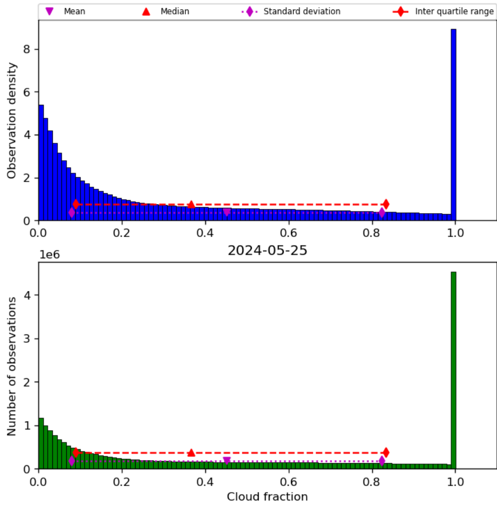
Figure 32: Histogram of “Cloud fraction” for 2024-05-24 to 2024-05-26
