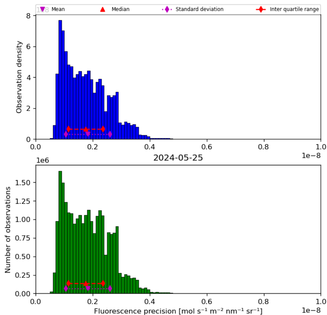
Figure 41: Histogram of “Fluorescence precision” for 2024-05-24 to 2024-05-26
