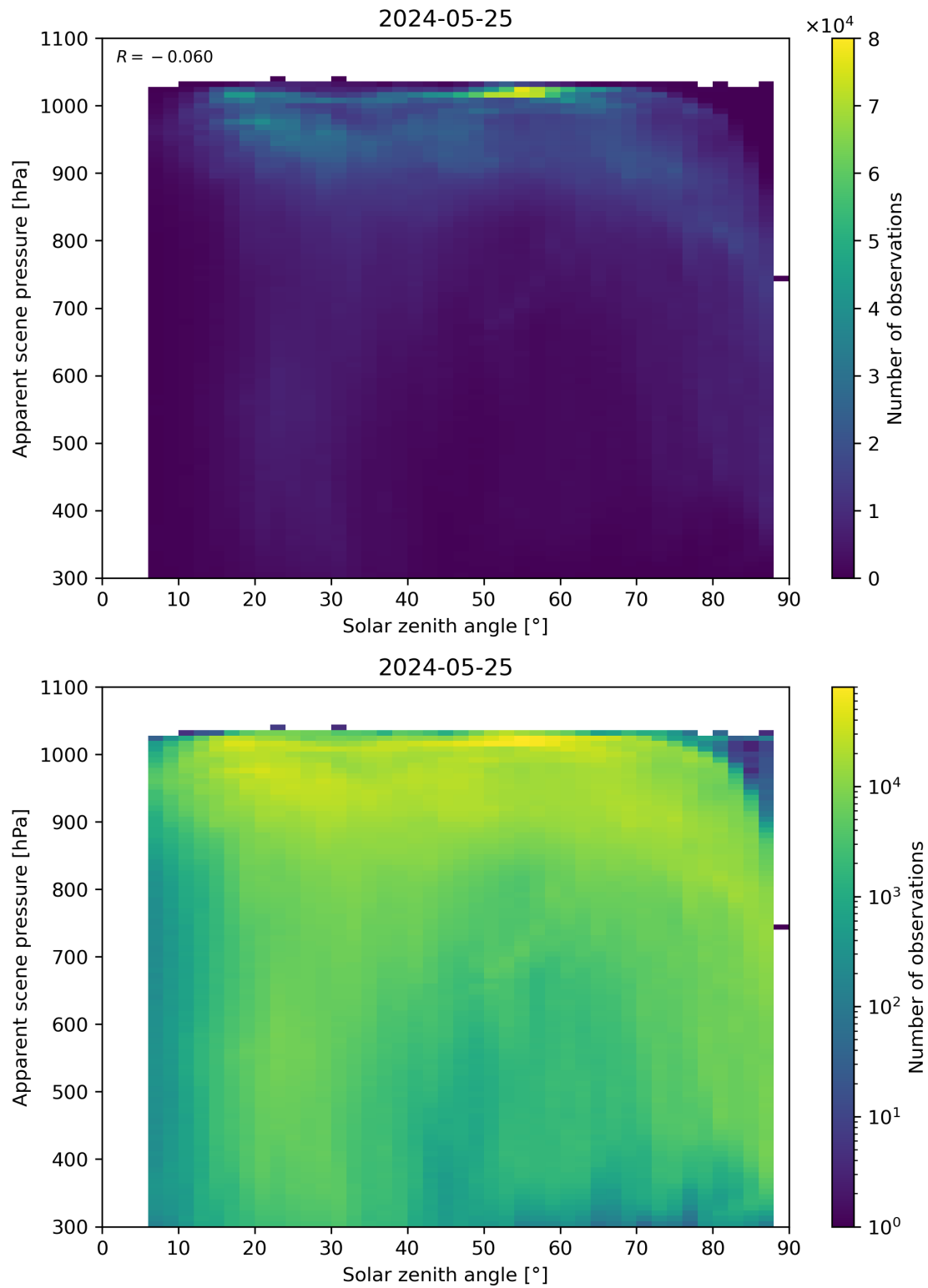
Figure 108: Scatter density plot of “Solar zenith angle” against “Apparent scene pressure” for 2024-05-24 to 2024-05-26.
