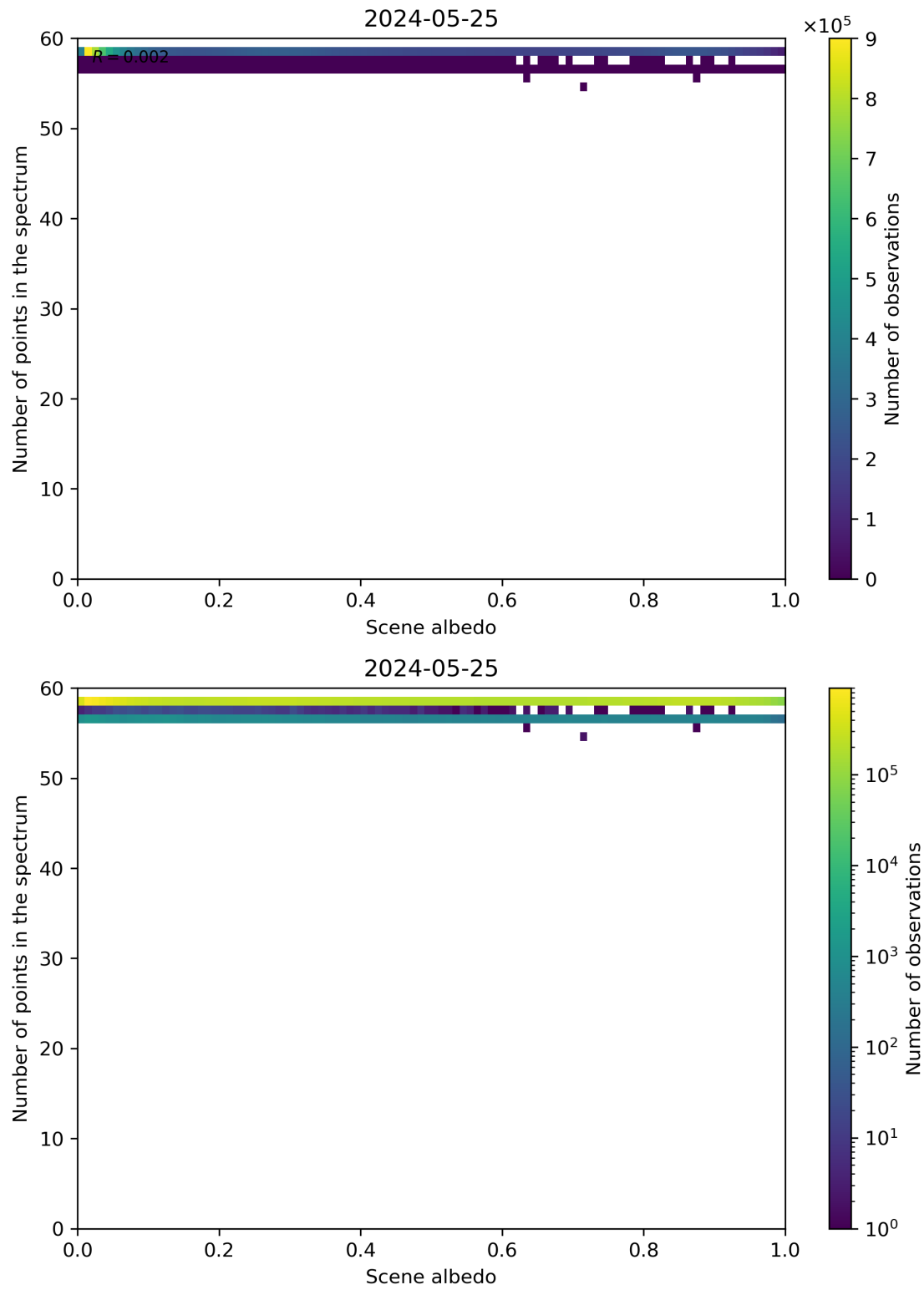
Figure 106: Scatter density plot of “Scene albedo” against “Number of points in the spectrum” for 2024-05-24 to 2024-05-26.
