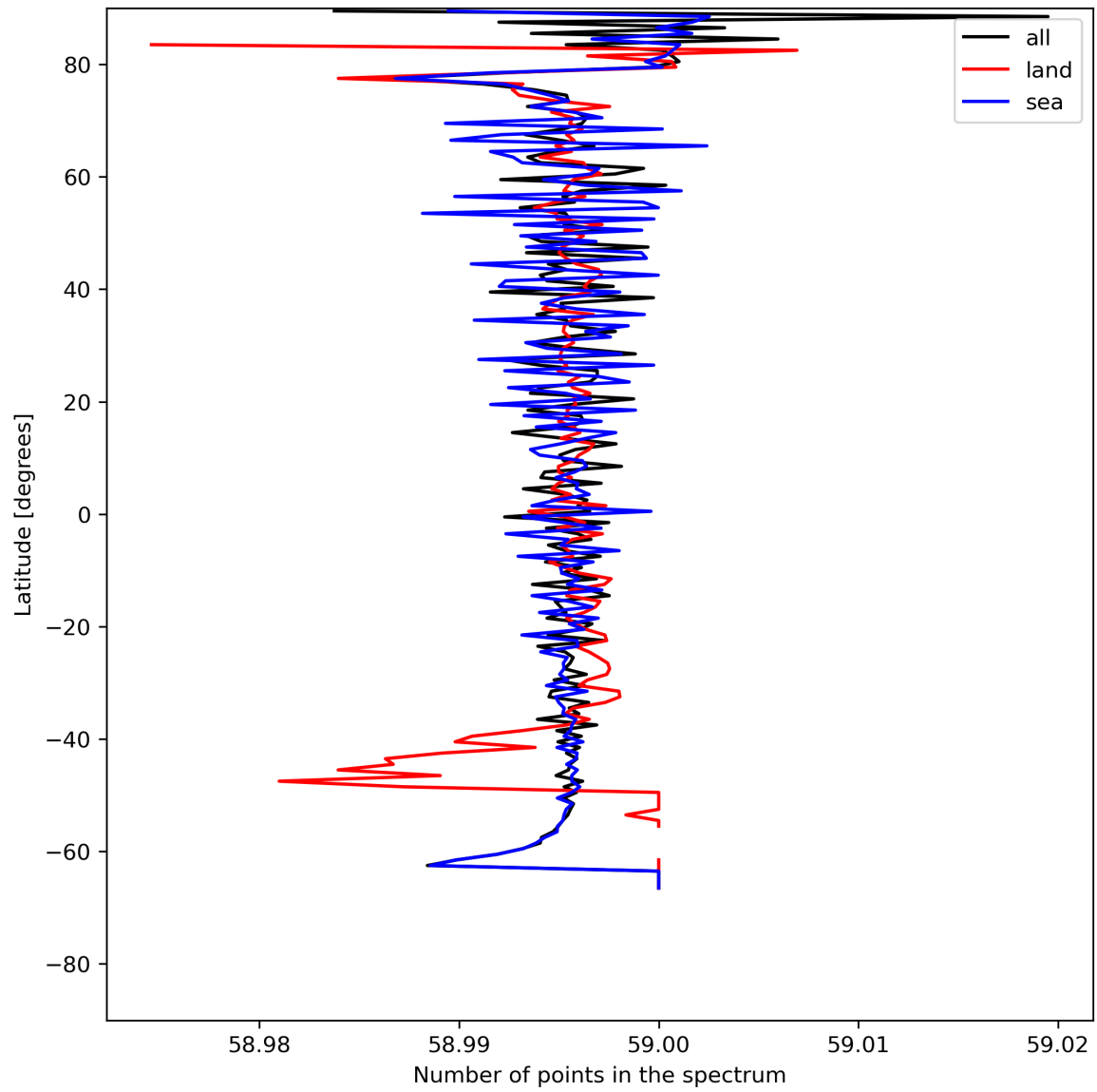
Figure 27: Zonal average of “Number of points in the spectrum” for 2024-05-24 to 2024-05-26.
