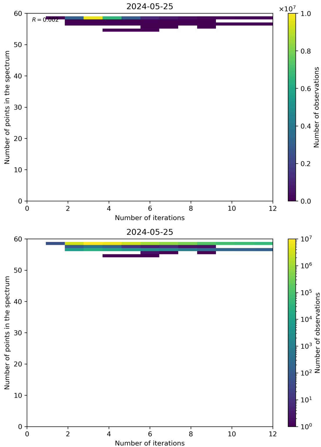
Figure 99: Scatter density plot of “Number of iterations” against “Number of points in the spectrum” for 2024-05-24 to 2024-05-26.
