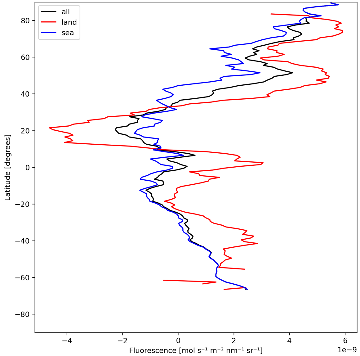
Figure 23: Zonal average of “Fluorescence” for 2024-05-24 to 2024-05-26.
