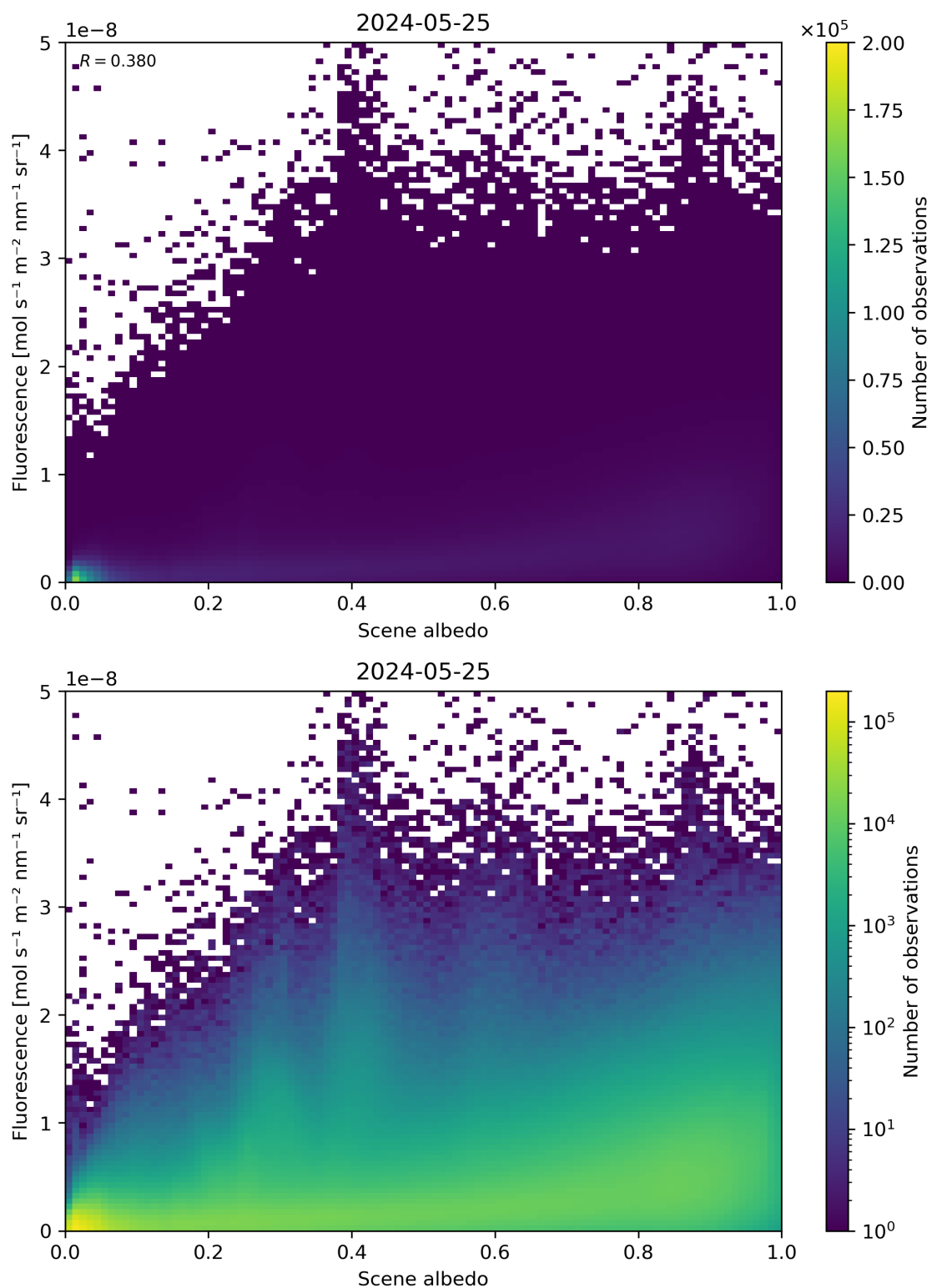
Figure 104: Scatter density plot of “Scene albedo” against “Fluorescence” for 2024-05-24 to 2024-05-26.
