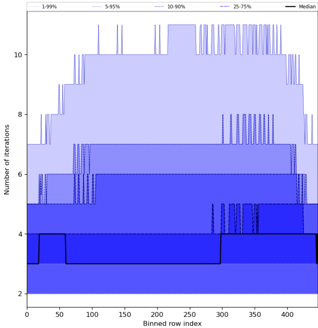
Figure 56: Along track statistics of “Number of iterations” for 2024-05-24 to 2024-05-26
