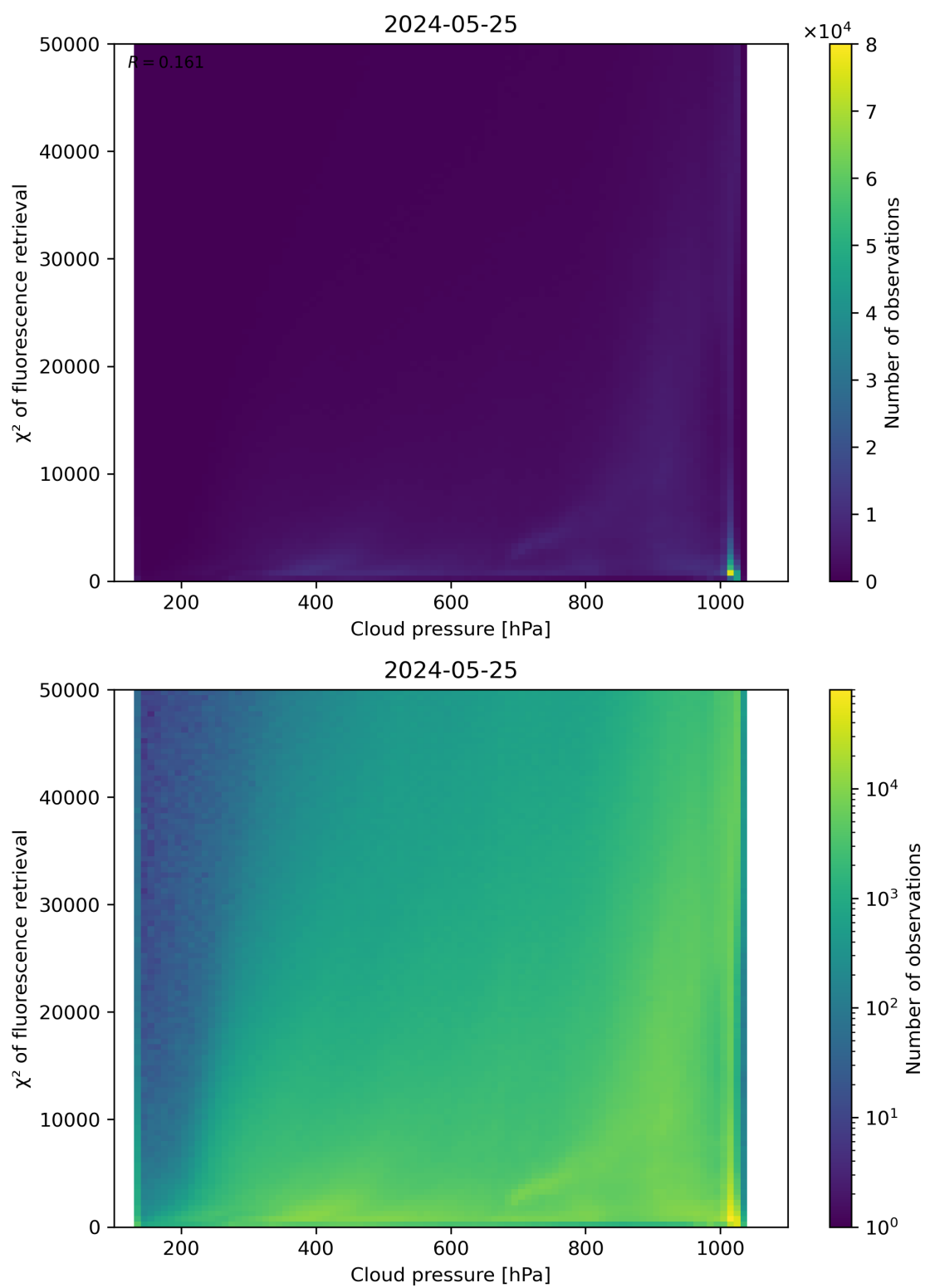
Figure 78: Scatter density plot of “Cloud pressure” against “ \chi^2 of fluorescence retrieval” for 2024-05-24 to 2024-05-26.
