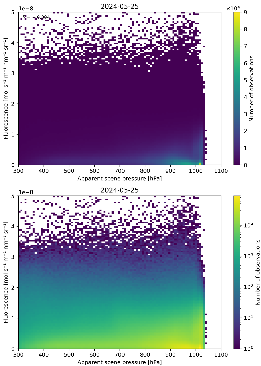
Figure 64: Scatter density plot of “Apparent scene pressure” against “Fluorescence” for 2024-05-24 to 2024-05-26.
