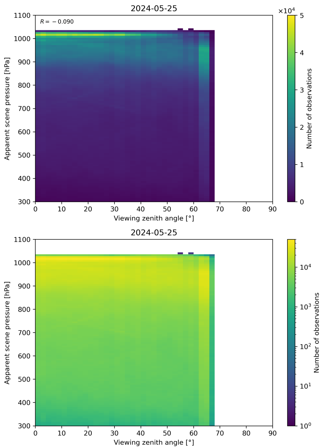
Figure 118: Scatter density plot of “Viewing zenith angle” against “Apparent scene pressure” for 2024-05-24 to 2024-05-26.
