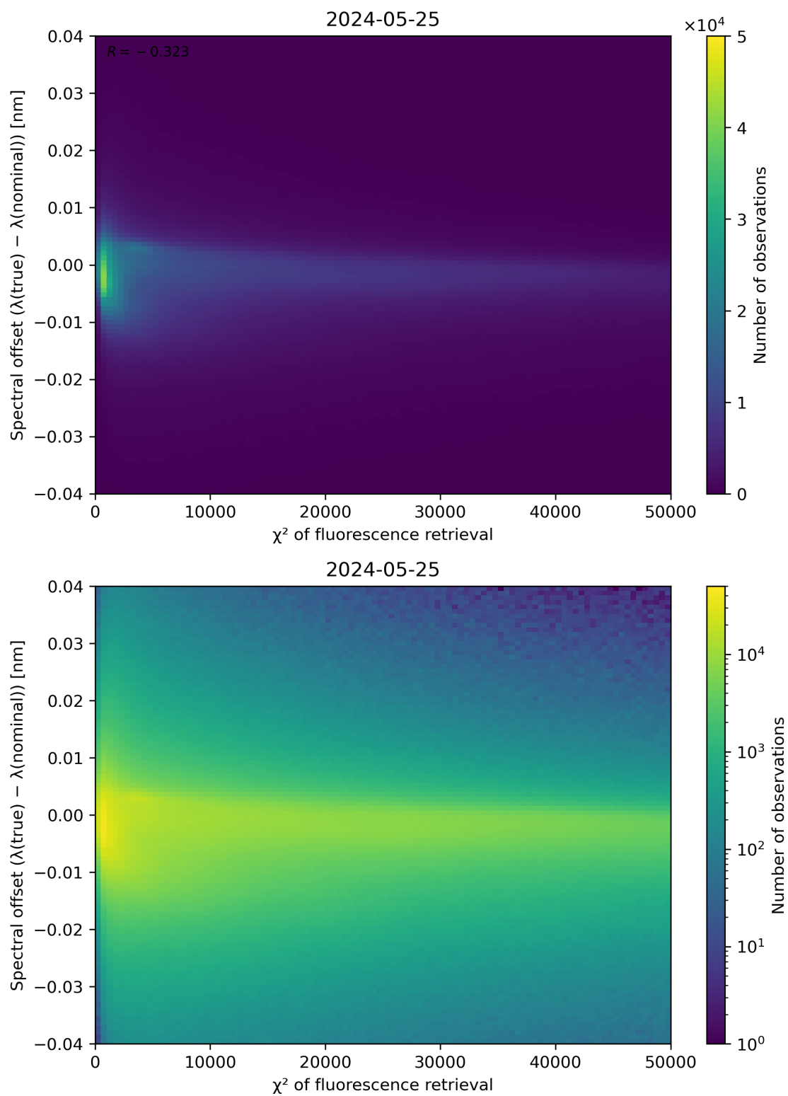
Figure 69: Scatter density plot of " \chi^2 of fluorescence retrieval" against "Spectral offset ( \lambda(\text{true}) - \lambda(\text{nominal})) " for 2024-05-24 to 2024-05-26.
