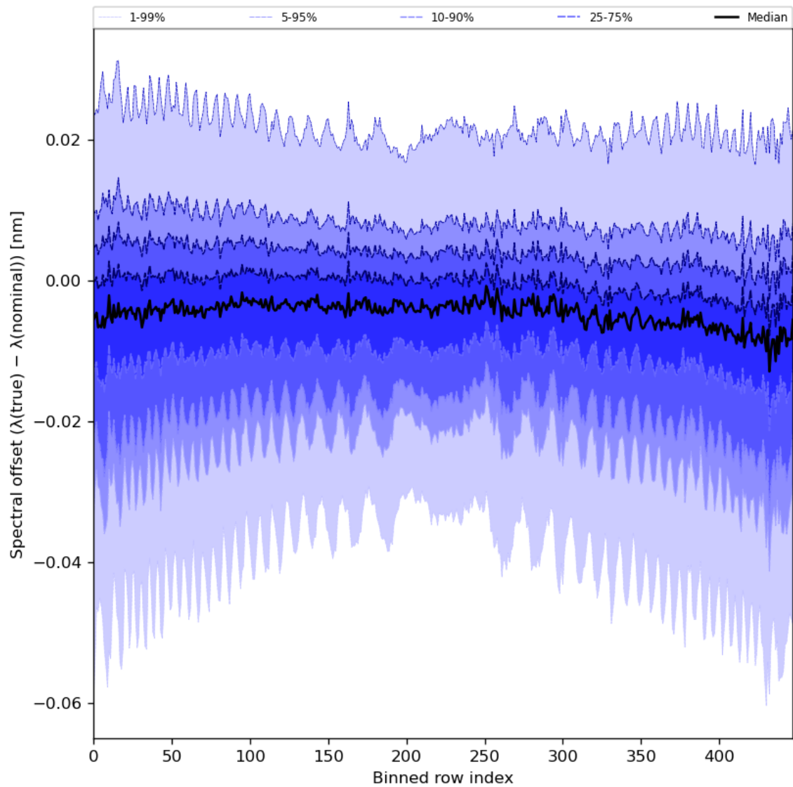
Figure 62: Along track statistics of “Spectral offset ( \lambda(\text{true}) - \lambda(\text{nominal}) )” for 2024-05-24 to 2024-05-26
