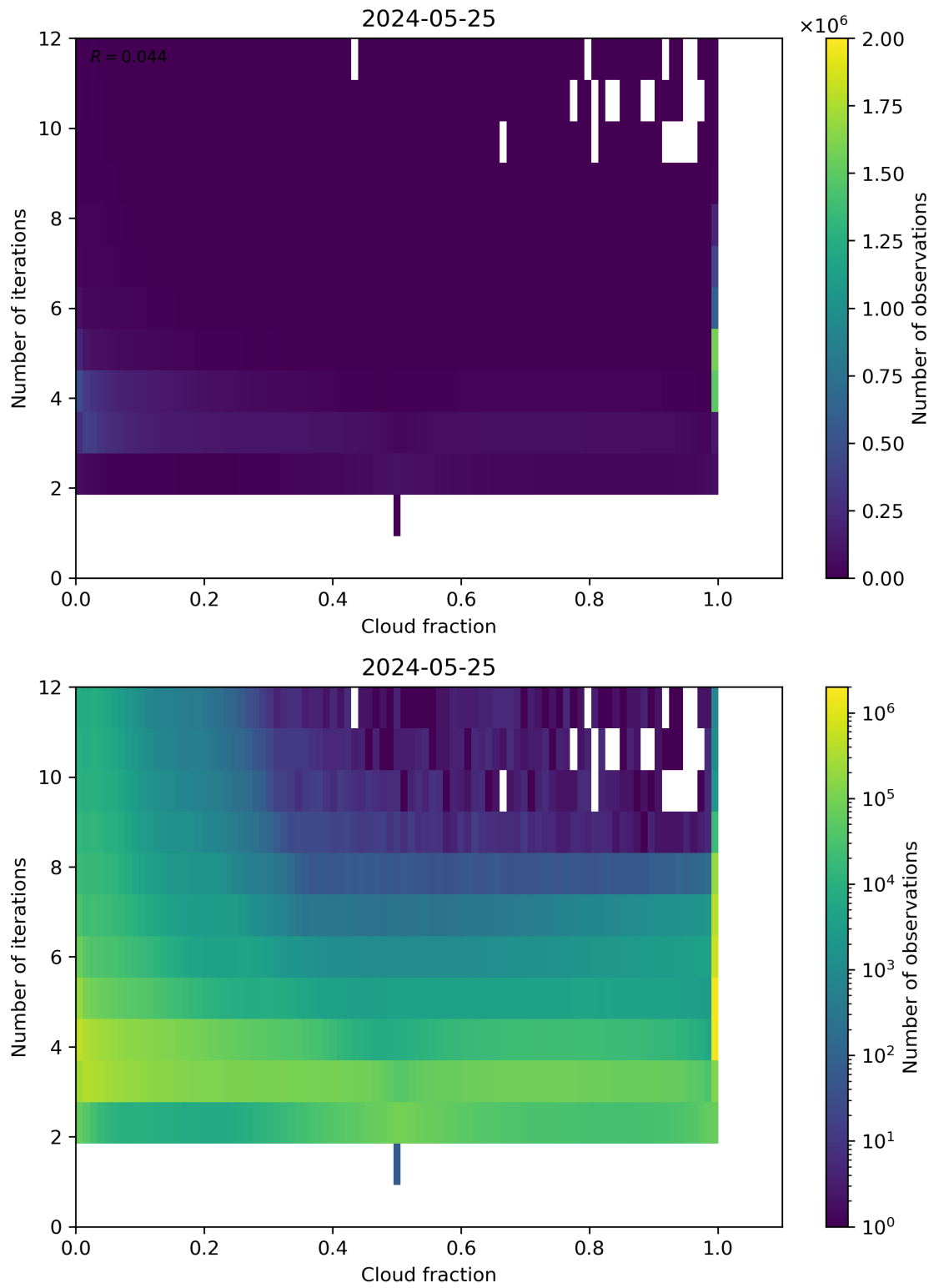
Figure 73: Scatter density plot of “Cloud fraction” against “Number of iterations” for 2024-05-24 to 2024-05-26.
