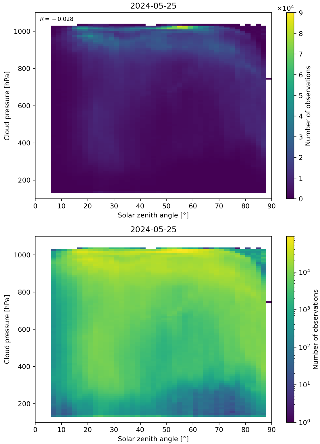
Figure 111: Scatter density plot of “Solar zenith angle” against “Cloud pressure” for 2024-05-24 to 2024-05-26.
