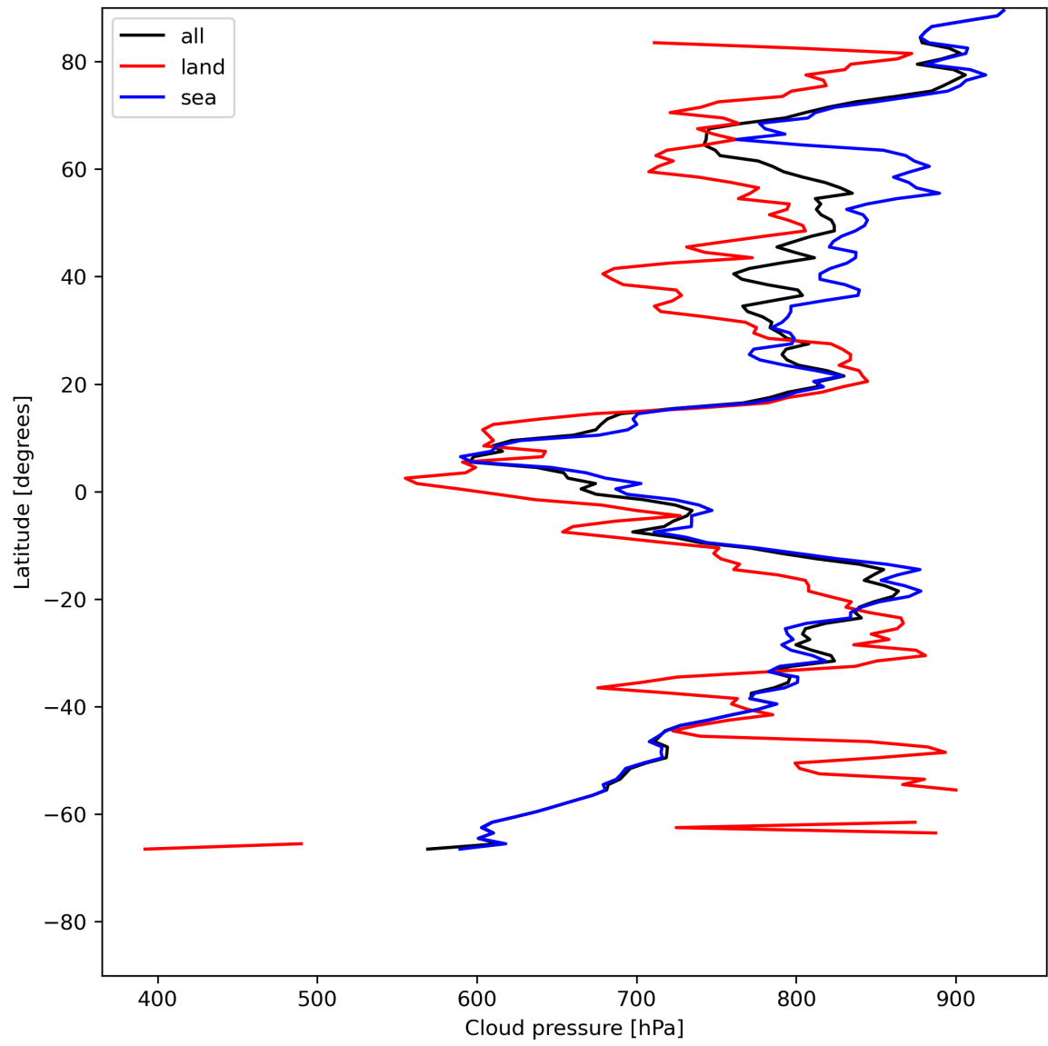
Figure 13: Zonal average of “Cloud pressure” for 2024-05-24 to 2024-05-26.
