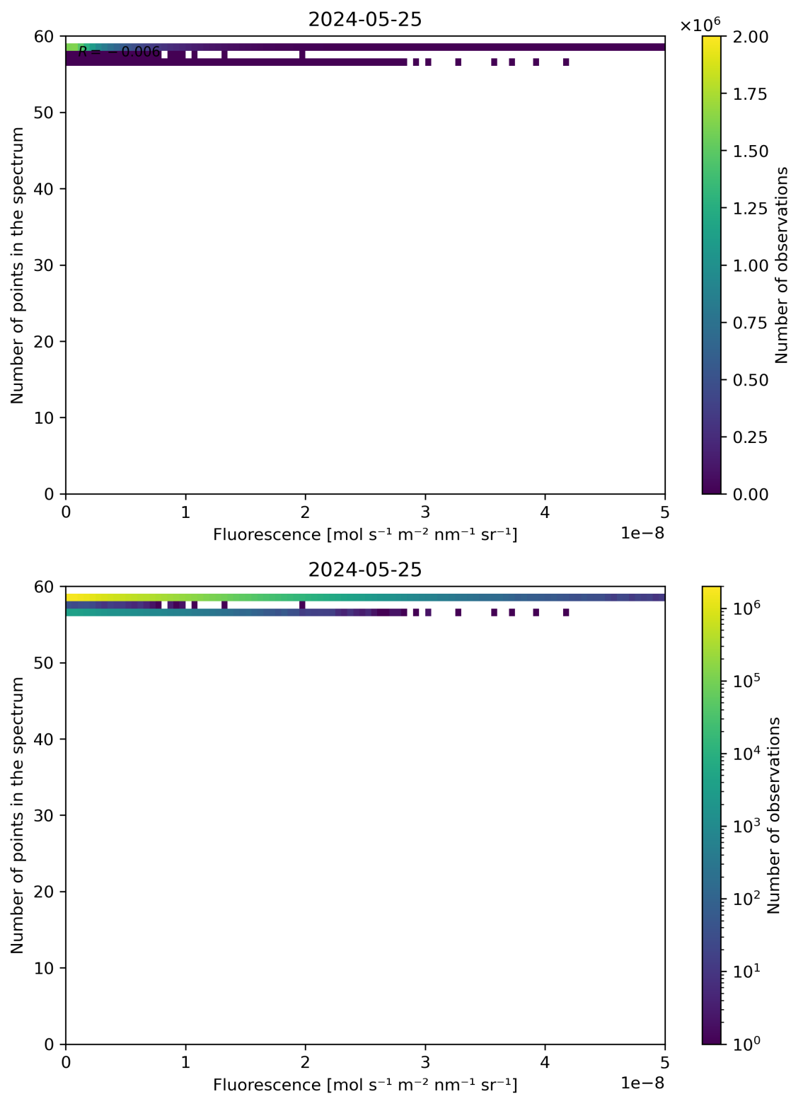
Figure 86: Scatter density plot of “Fluorescence” against “Number of points in the spectrum” for 2024-05-24 to 2024-05-26.
