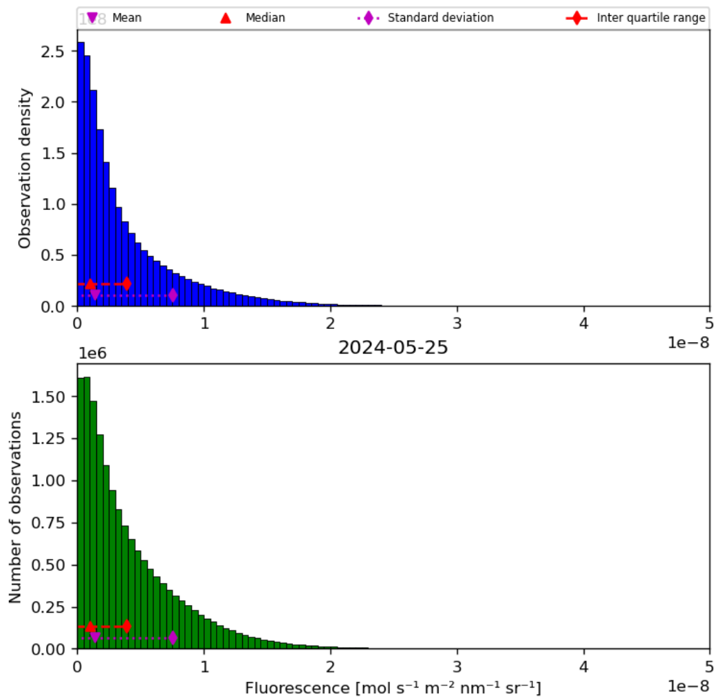
Figure 40: Histogram of “Fluorescence” for 2024-05-24 to 2024-05-26
