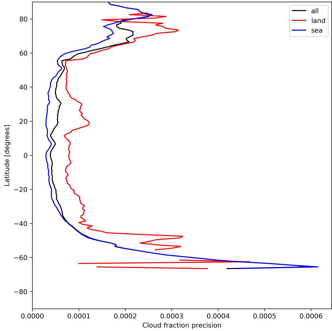
Figure 16: Zonal average of “Cloud fraction precision” for 2024-05-24 to 2024-05-26.
