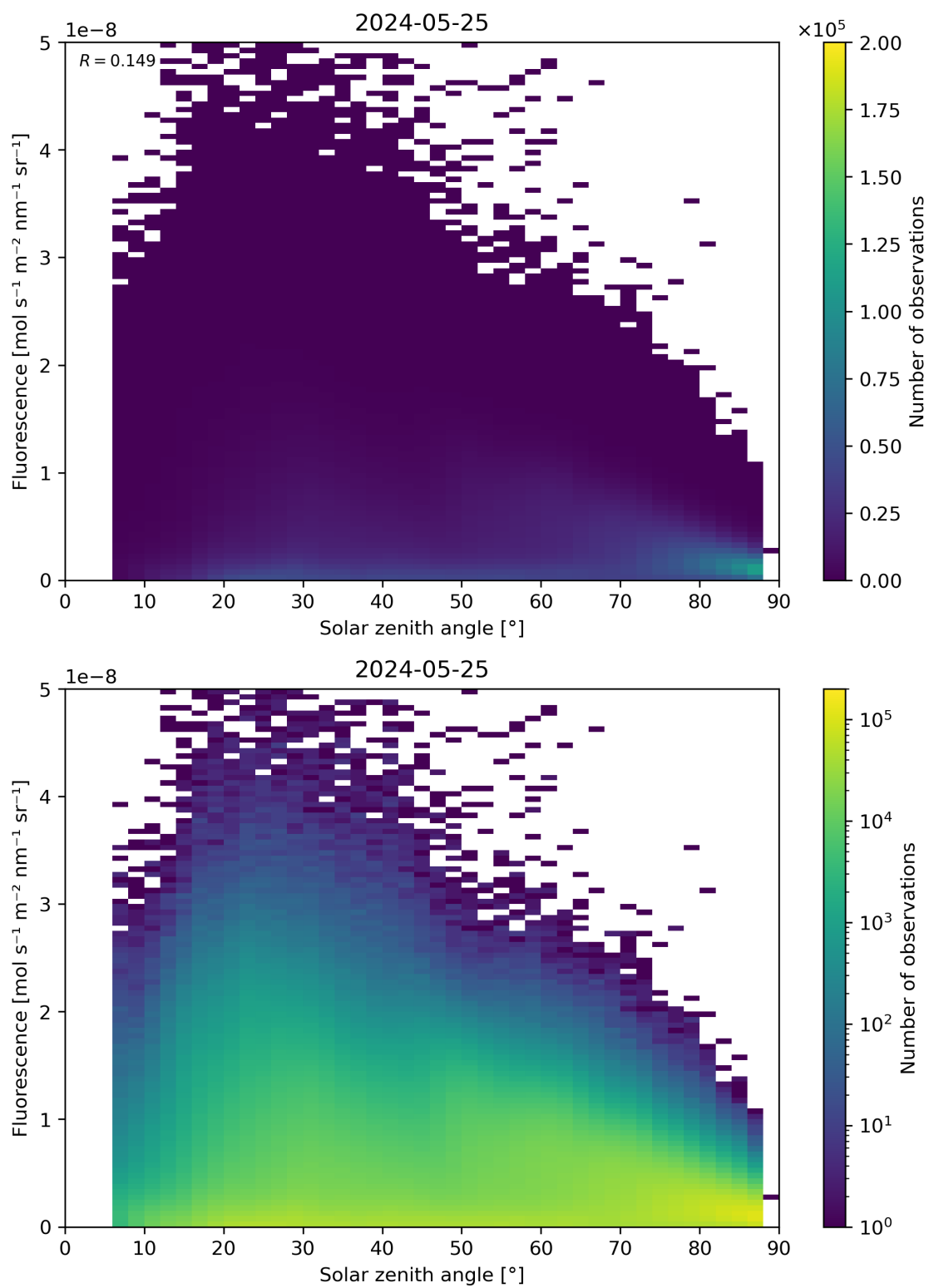
Figure 112: Scatter density plot of “Solar zenith angle” against “Fluorescence” for 2024-05-24 to 2024-05-26.
