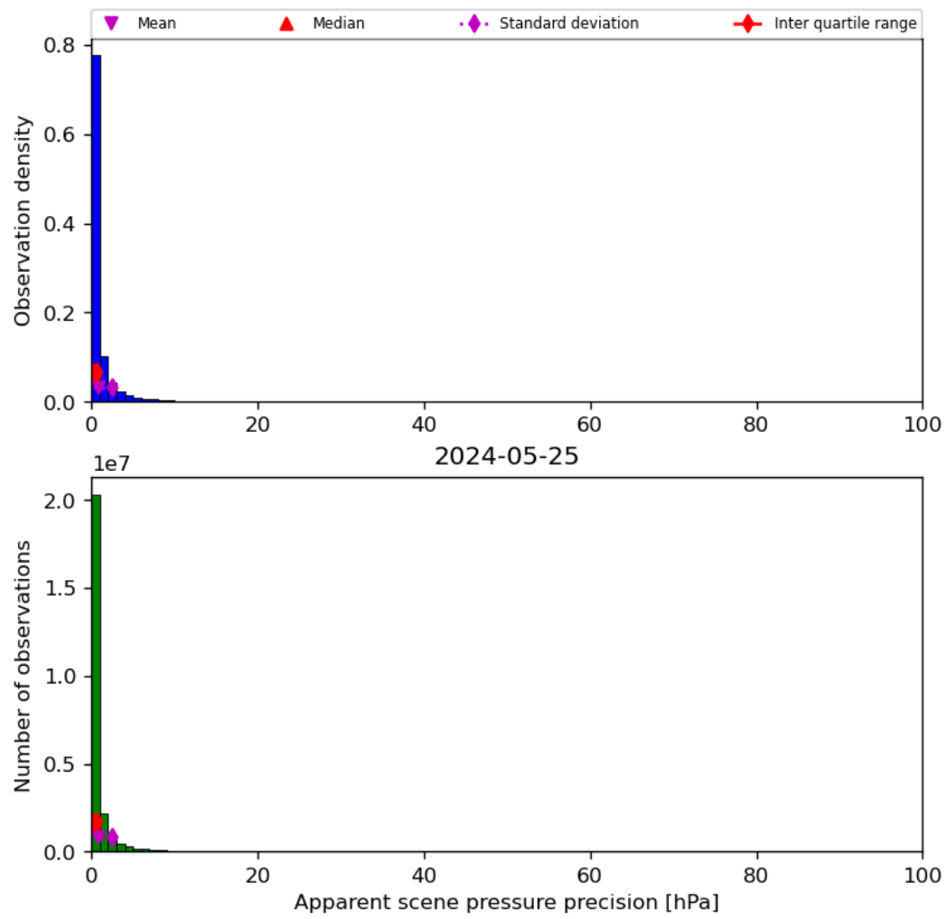
Figure 37: Histogram of “Apparent scene pressure precision” for 2024-05-24 to 2024-05-26
