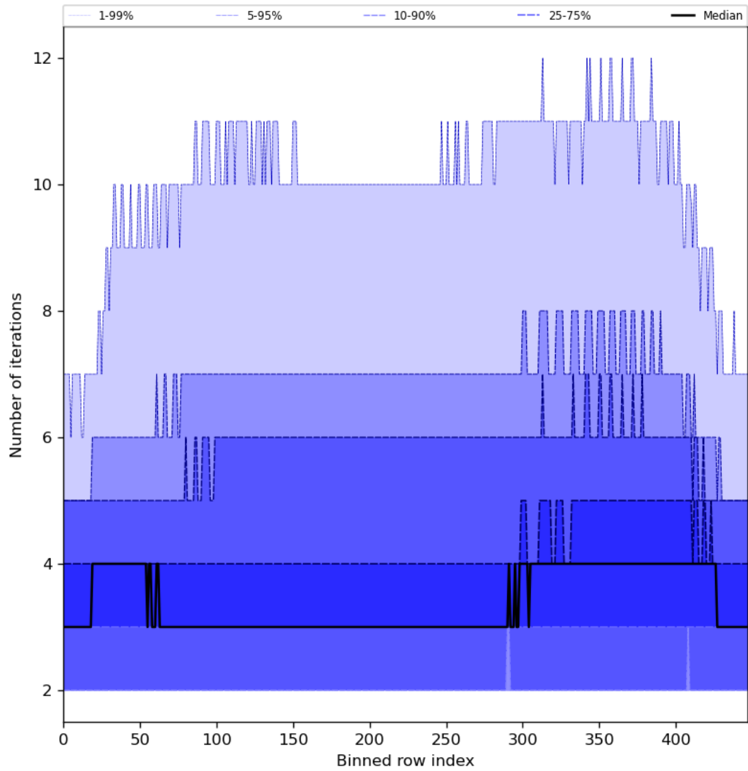
Figure 56: Along track statistics of “Number of iterations” for 2024-05-25 to 2024-05-27
