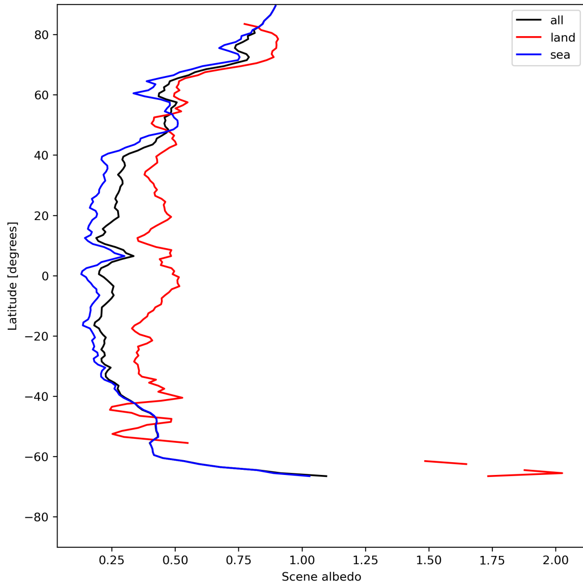
Figure 17: Zonal average of “Scene albedo” for 2024-05-25 to 2024-05-27.
