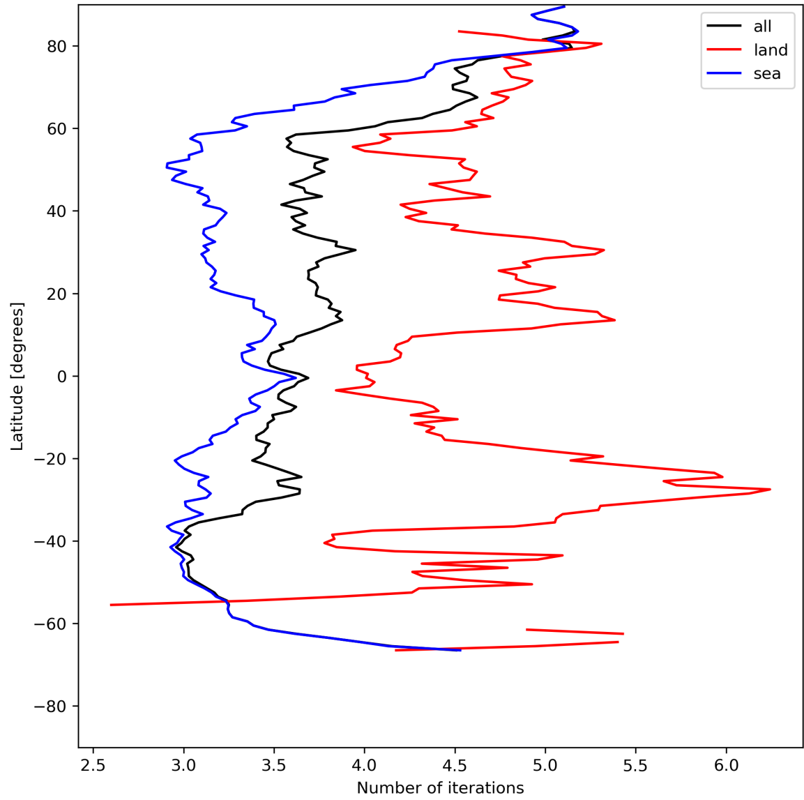
Figure 22: Zonal average of “Number of iterations” for 2024-05-25 to 2024-05-27.
