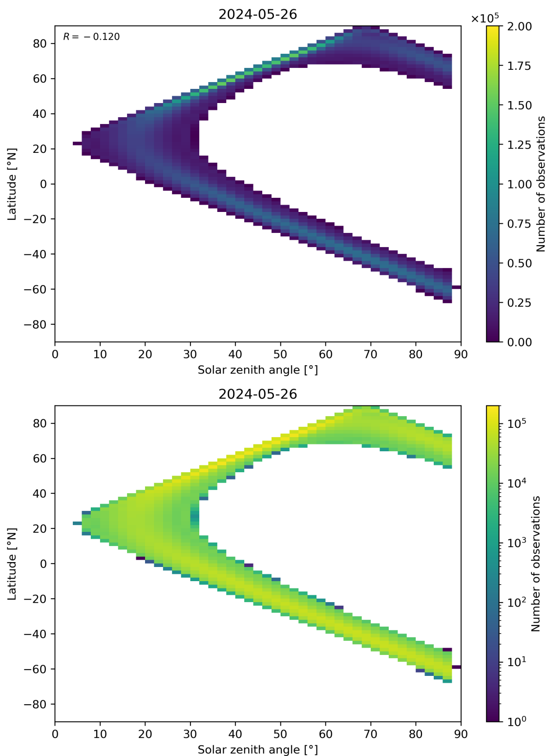
Figure 113: Scatter density plot of “Solar zenith angle” against “Latitude” for 2024-05-25 to 2024-05-27.
