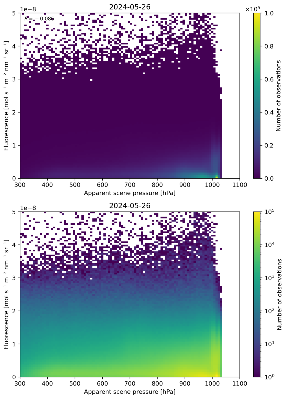
Figure 64: Scatter density plot of “Apparent scene pressure” against “Fluorescence” for 2024-05-25 to 2024-05-27.
