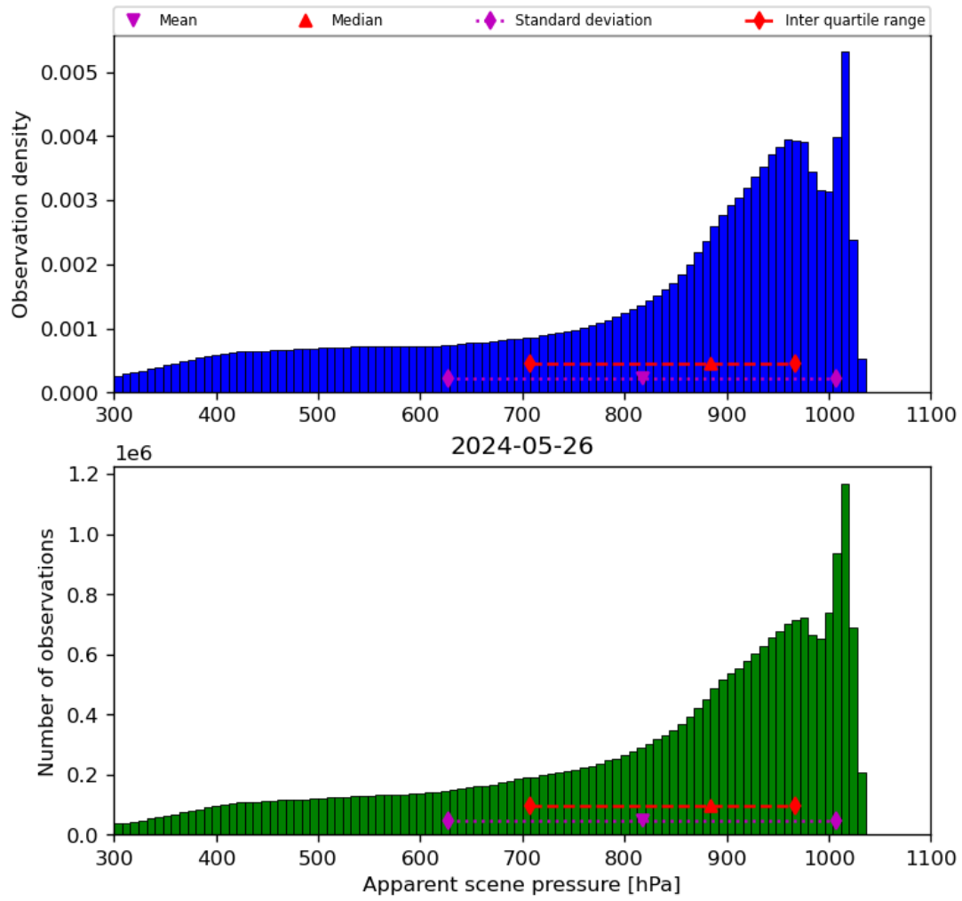
Figure 36: Histogram of “Apparent scene pressure” for 2024-05-25 to 2024-05-27
