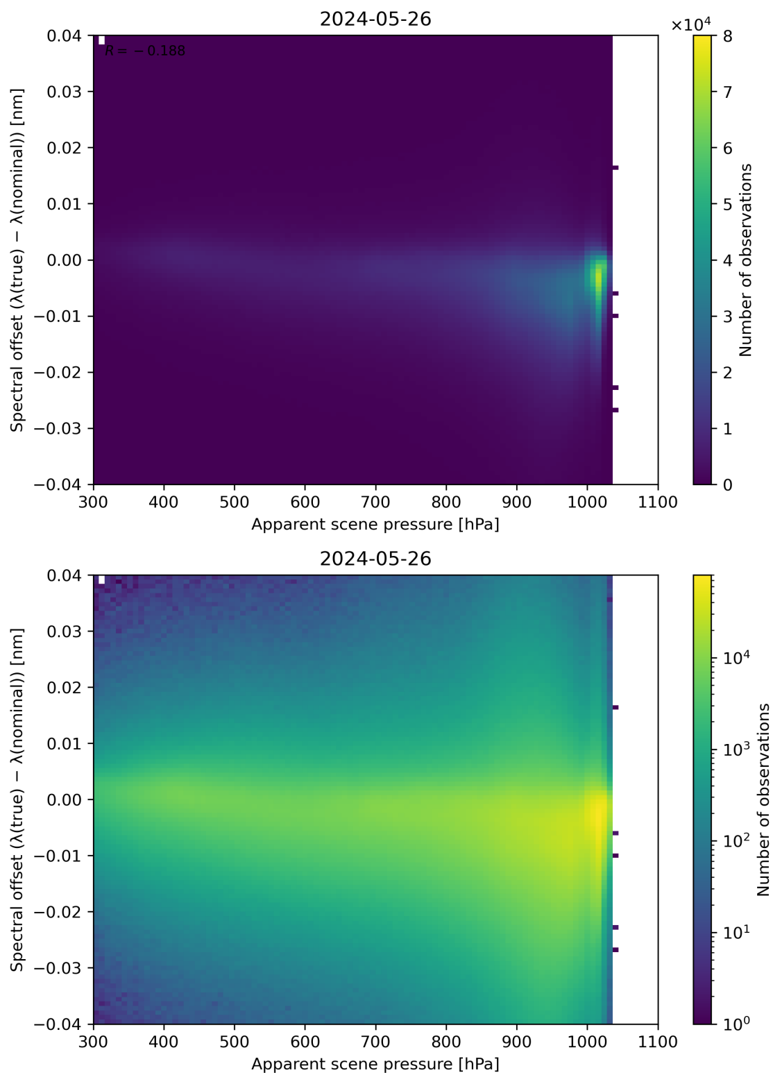
Figure 67: Scatter density plot of “Apparent scene pressure” against “Spectral offset ( \lambda(\text{true}) - \lambda(\text{nominal}) )” for 2024-05-25 to 2024-05-27.
