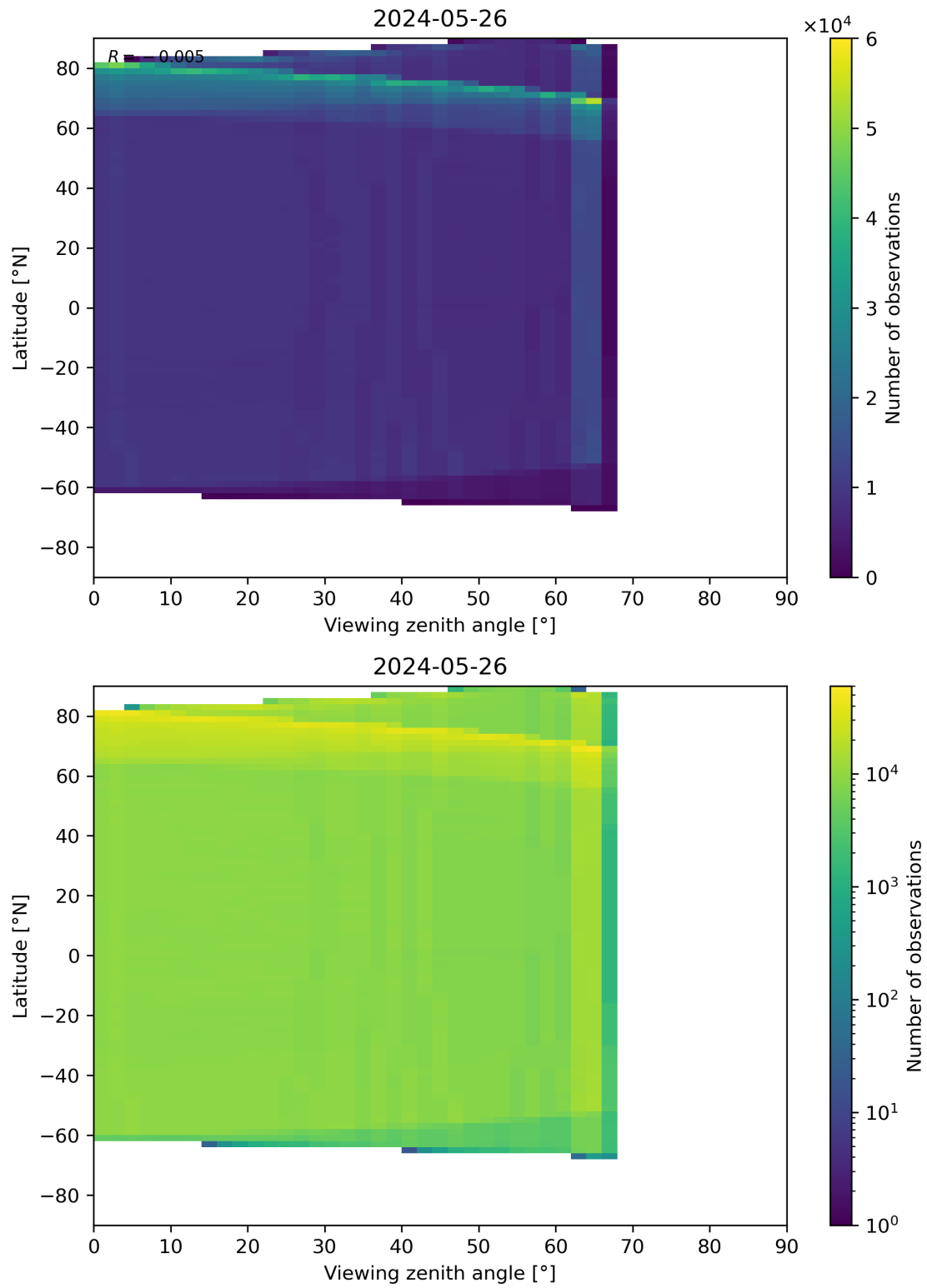
Figure 123: Scatter density plot of “Viewing zenith angle” against “Latitude” for 2024-05-25 to 2024-05-27.
