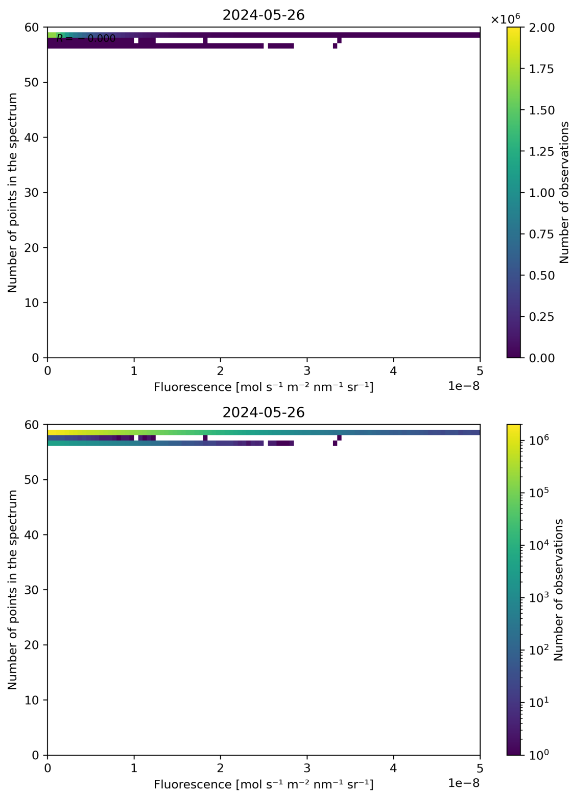
Figure 86: Scatter density plot of “Fluorescence” against “Number of points in the spectrum” for 2024-05-25 to 2024-05-27.
