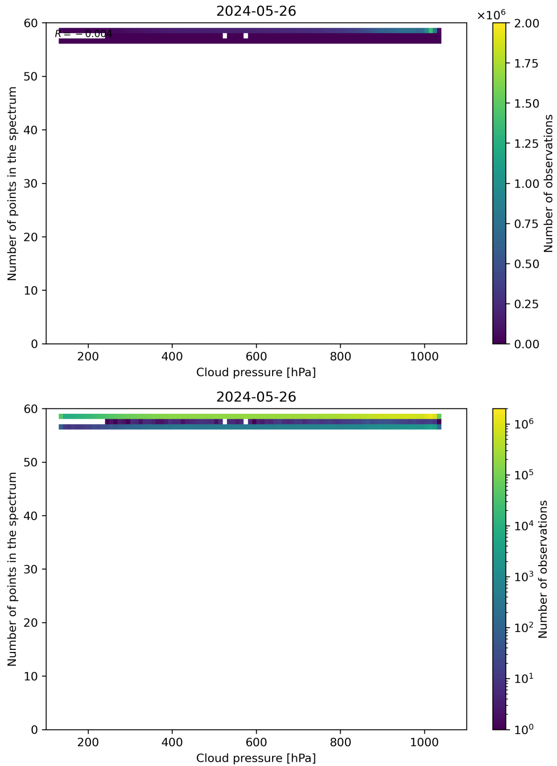
Figure 82: Scatter density plot of “Cloud pressure” against “Number of points in the spectrum” for 2024-05-25 to 2024-05-27.
