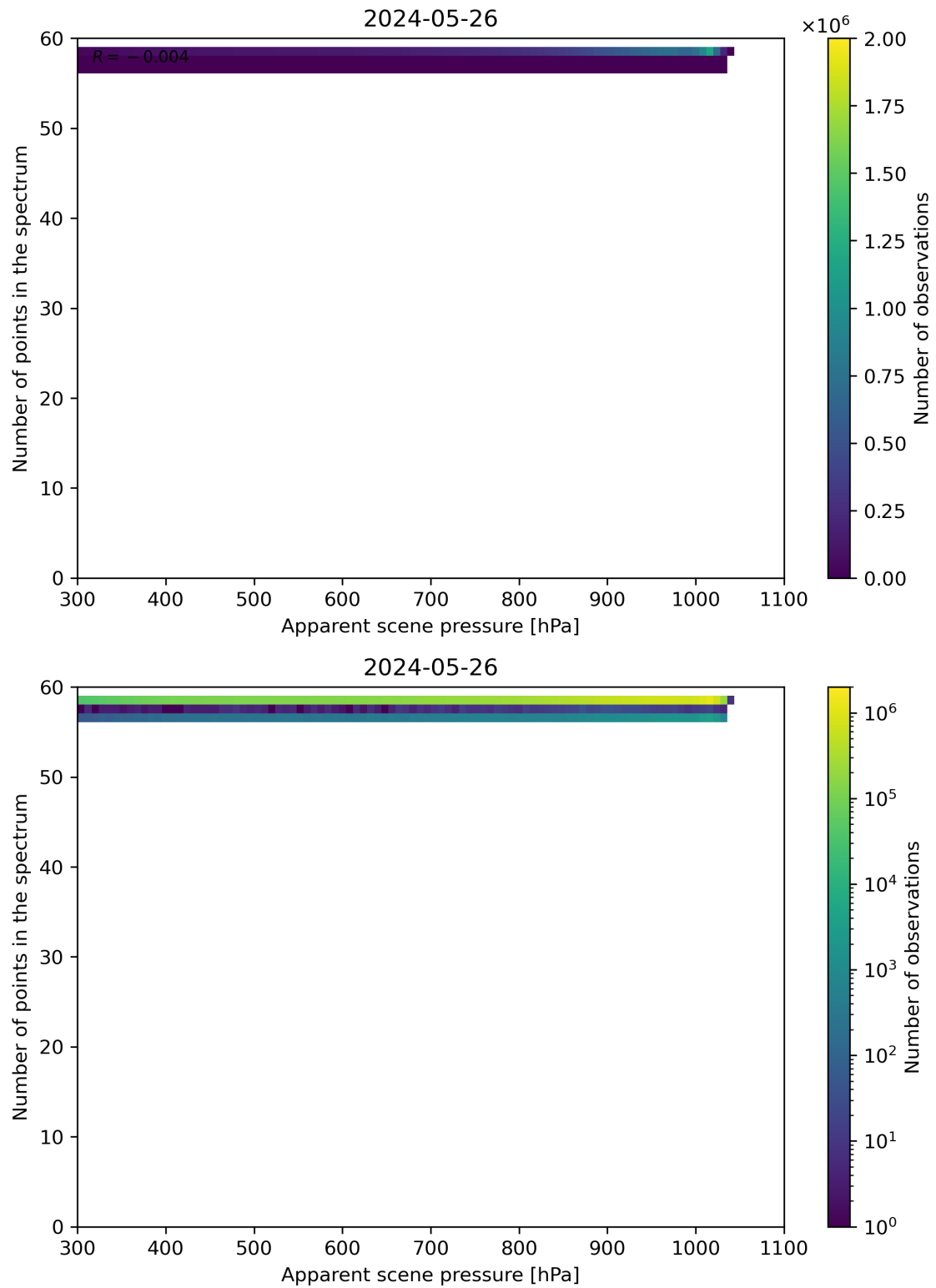
Figure 66: Scatter density plot of “Apparent scene pressure” against “Number of points in the spectrum” for 2024-05-25 to 2024-05-27.
