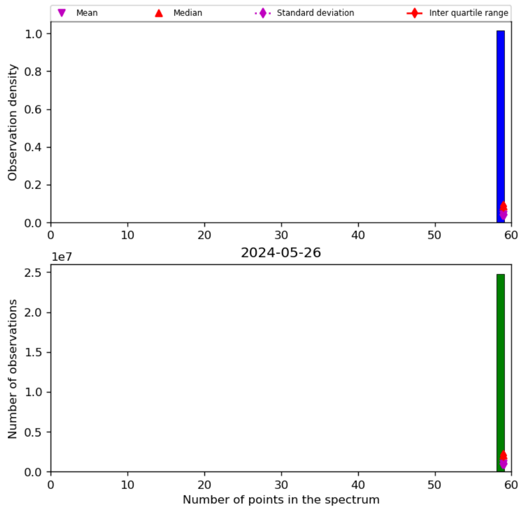
Figure 44: Histogram of “Number of points in the spectrum” for 2024-05-25 to 2024-05-27
