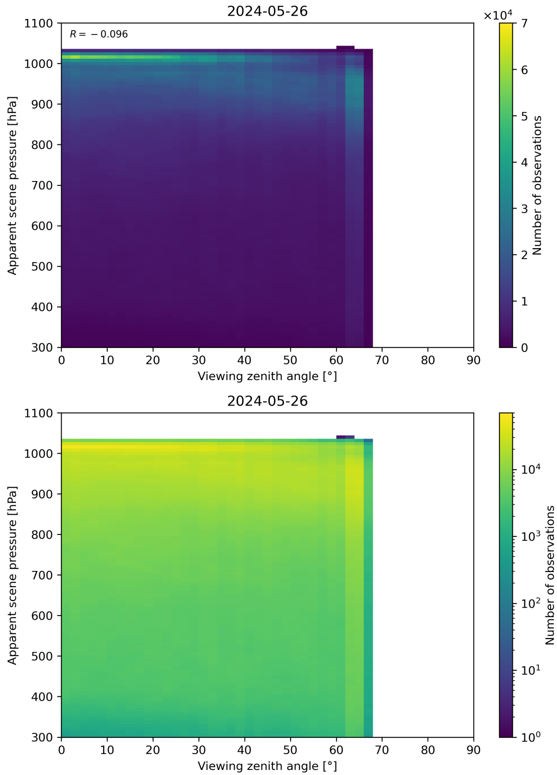
Figure 118: Scatter density plot of “Viewing zenith angle” against “Apparent scene pressure” for 2024-05-25 to 2024-05-27.
