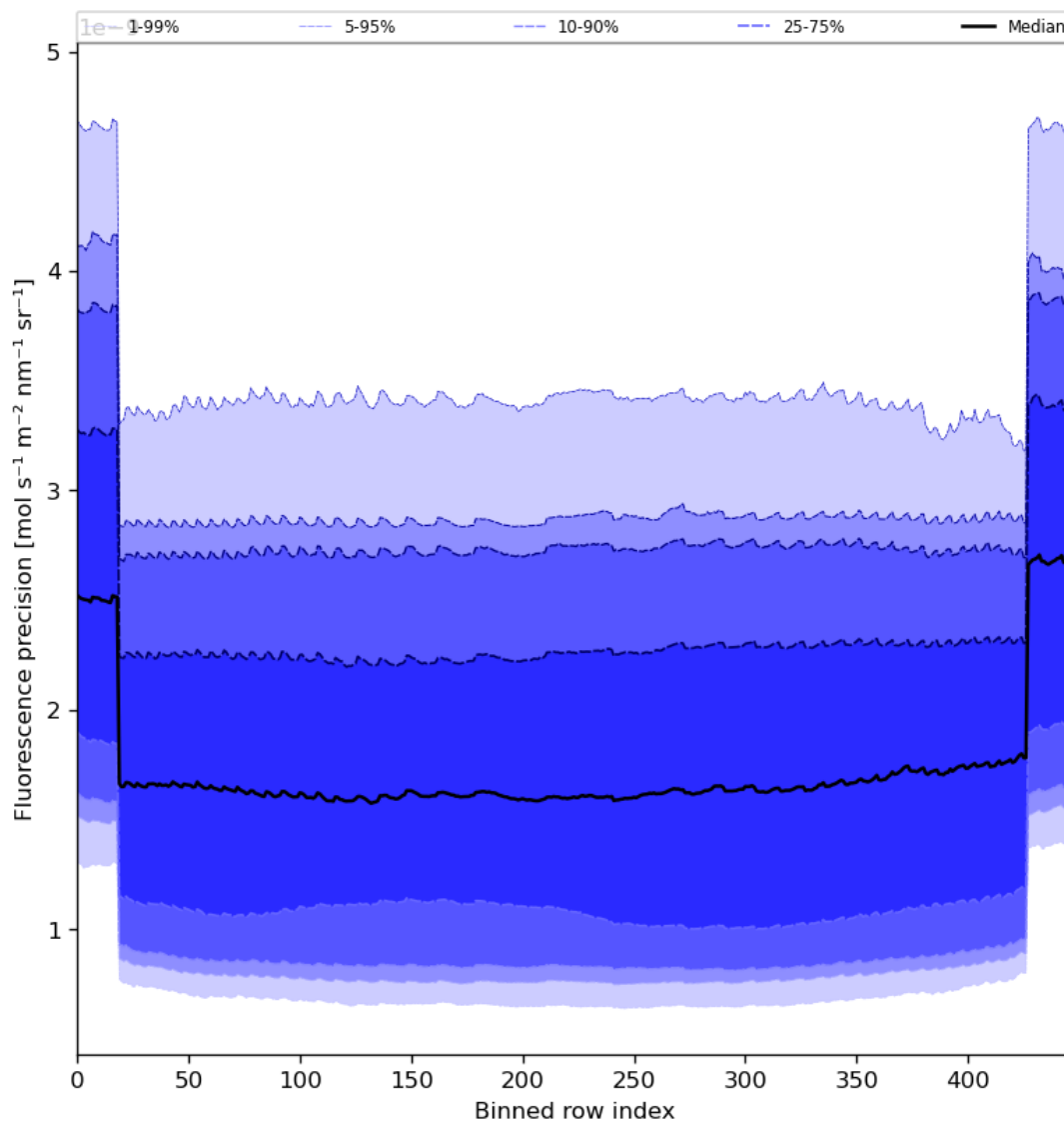
Figure 58: Along track statistics of “Fluorescence precision” for 2024-05-25 to 2024-05-27
