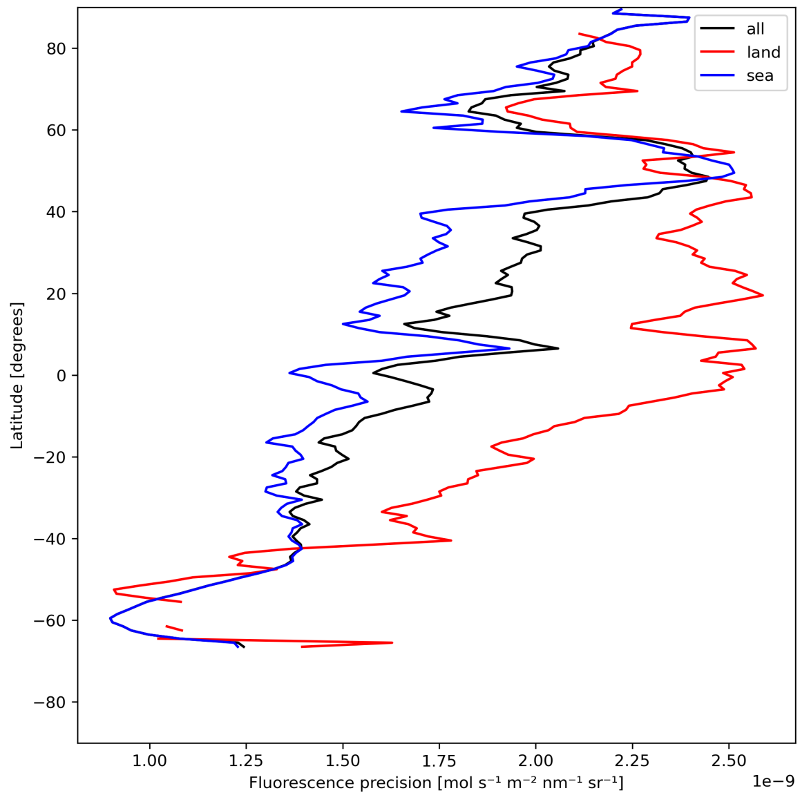
Figure 24: Zonal average of “Fluorescence precision” for 2024-05-25 to 2024-05-27.
