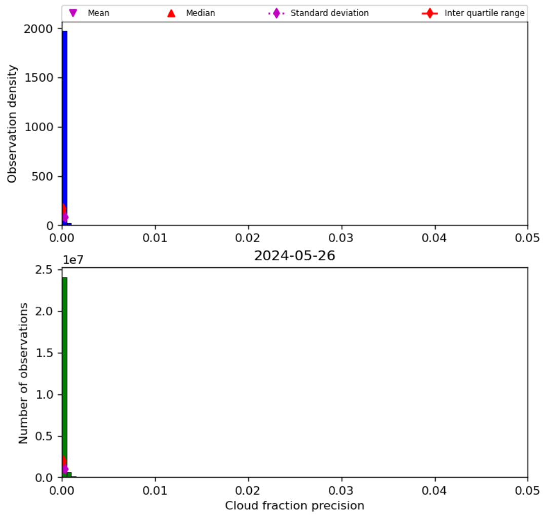
Figure 33: Histogram of “Cloud fraction precision” for 2024-05-25 to 2024-05-27
