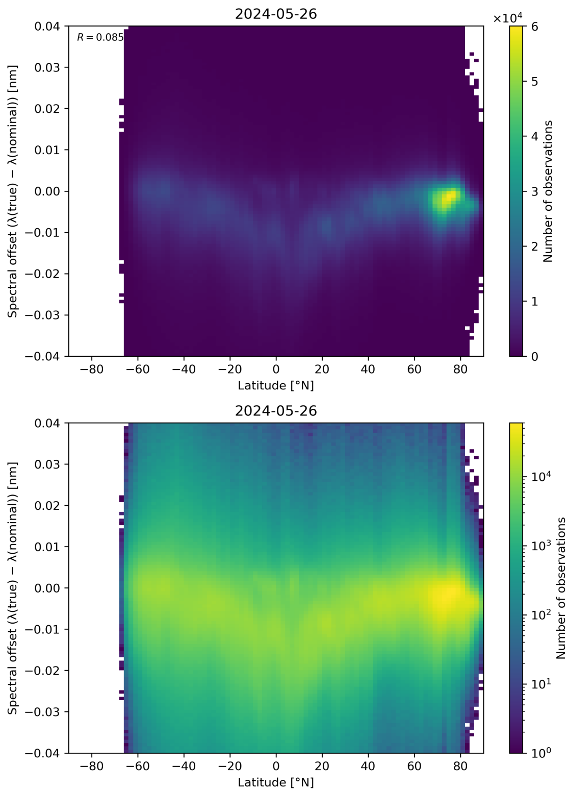
Figure 96: Scatter density plot of “Latitude” against “Spectral offset ( \lambda(\text{true}) - \lambda(\text{nominal}) )” for 2024-05-25 to 2024-05-27.
