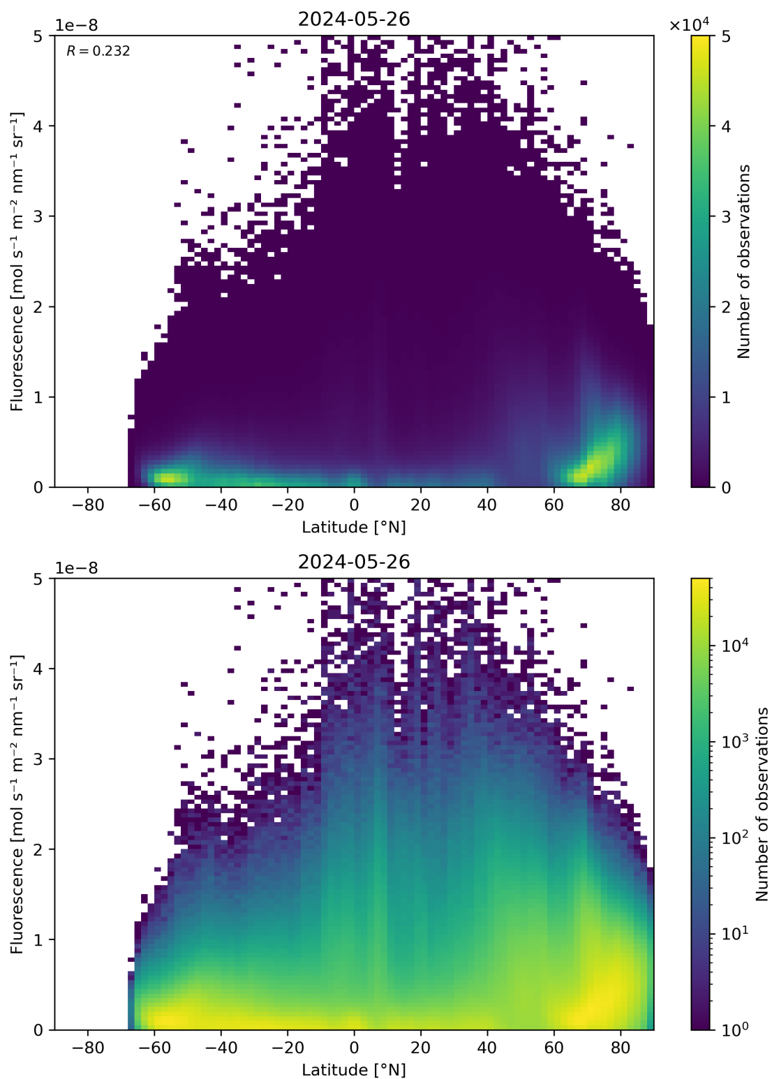
Figure 92: Scatter density plot of “Latitude” against “Fluorescence” for 2024-05-25 to 2024-05-27.
