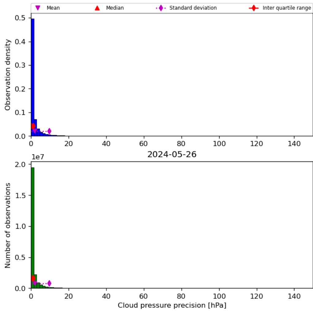
Figure 31: Histogram of “Cloud pressure precision” for 2024-05-25 to 2024-05-27
