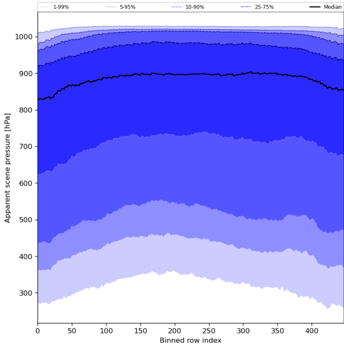
Figure 53: Along track statistics of “Apparent scene pressure” for 2024-05-25 to 2024-05-27
