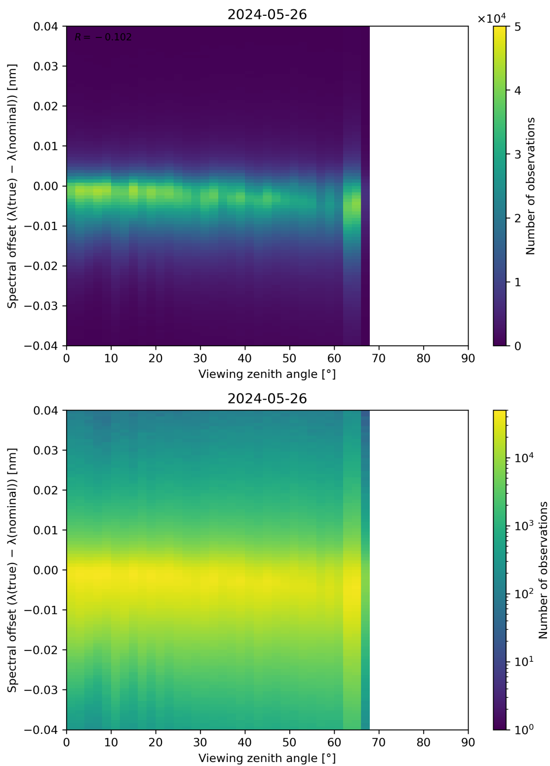
Figure 128: Scatter density plot of “Viewing zenith angle” against “Spectral offset ( \lambda(\text{true}) - \lambda(\text{nominal}) )” for 2024-05-25 to 2024-05-27.
