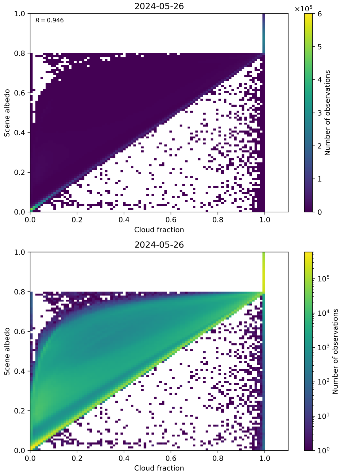
Figure 75: Scatter density plot of “Cloud fraction” against “Scene albedo” for 2024-05-25 to 2024-05-27.
