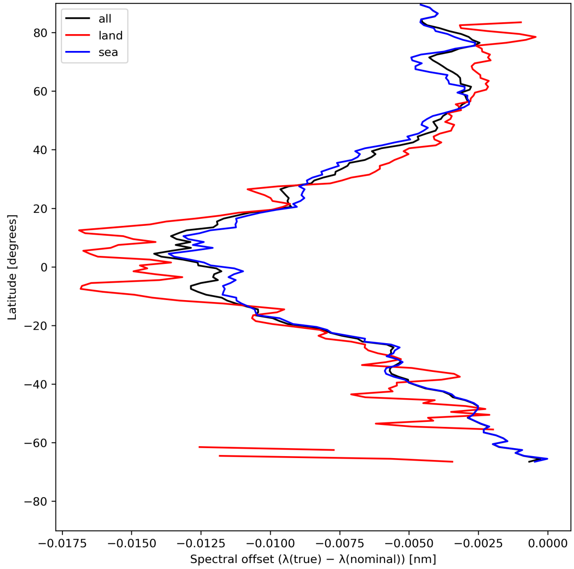
Figure 28: Zonal average of “Spectral offset ( \lambda(\text{true}) - \lambda(\text{nominal}) )” for 2024-05-25 to 2024-05-27.
