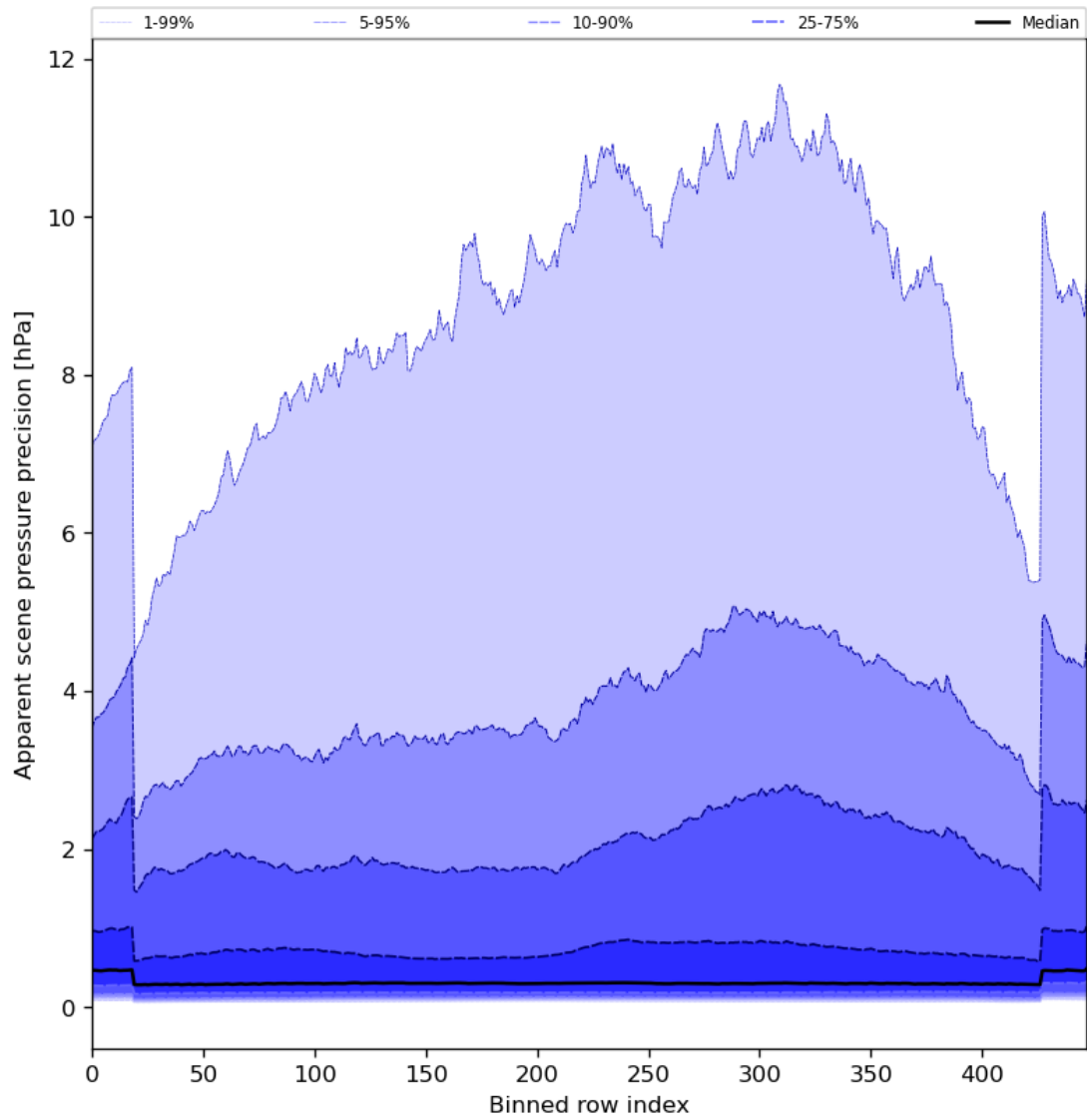
Figure 54: Along track statistics of “Apparent scene pressure precision” for 2024-05-25 to 2024-05-27
