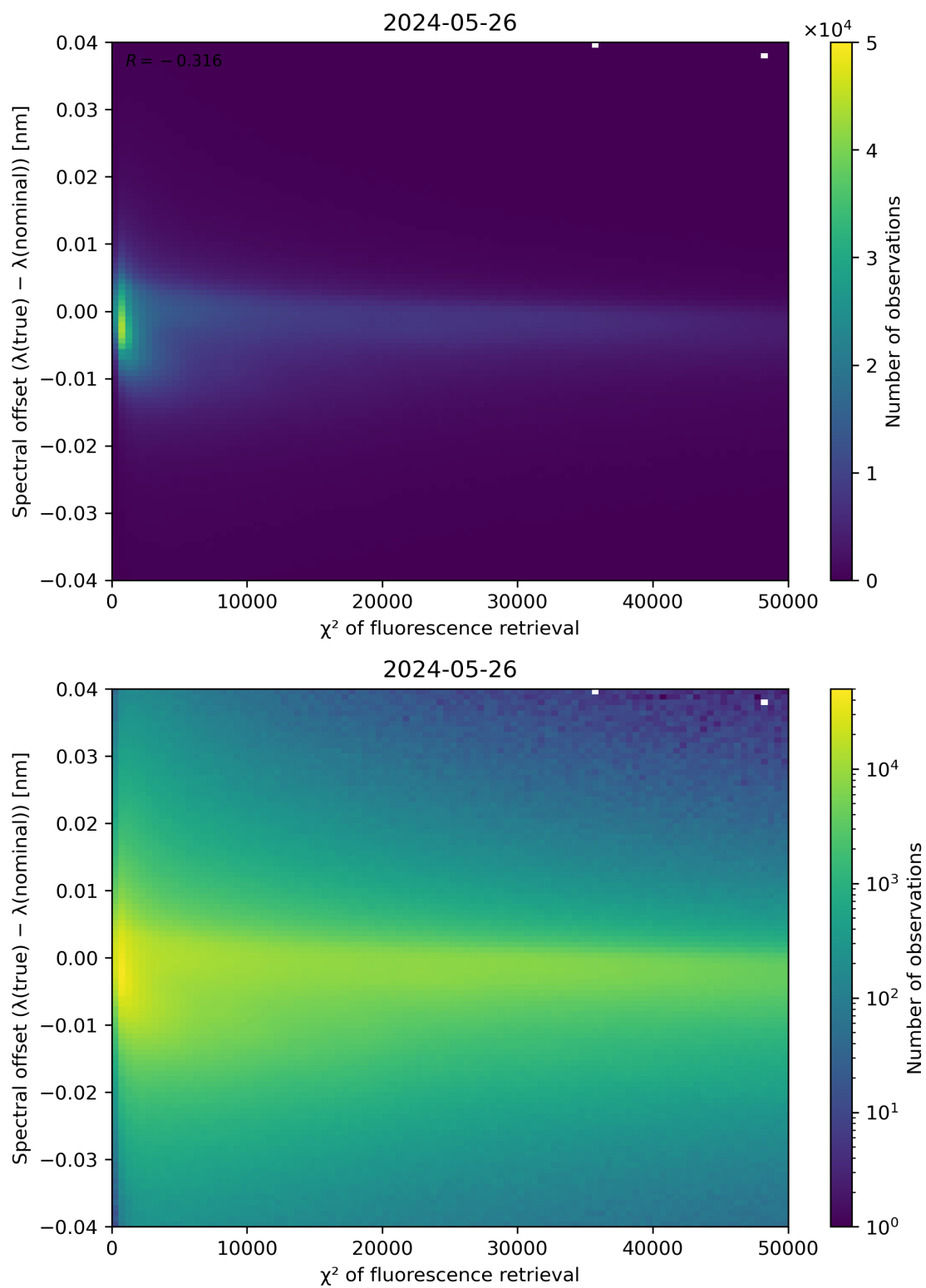
Figure 69: Scatter density plot of “ \chi^2 of fluorescence retrieval” against “Spectral offset ( \lambda(\text{true}) - \lambda(\text{nominal}) )” for 2024-05-25 to 2024-05-27.
