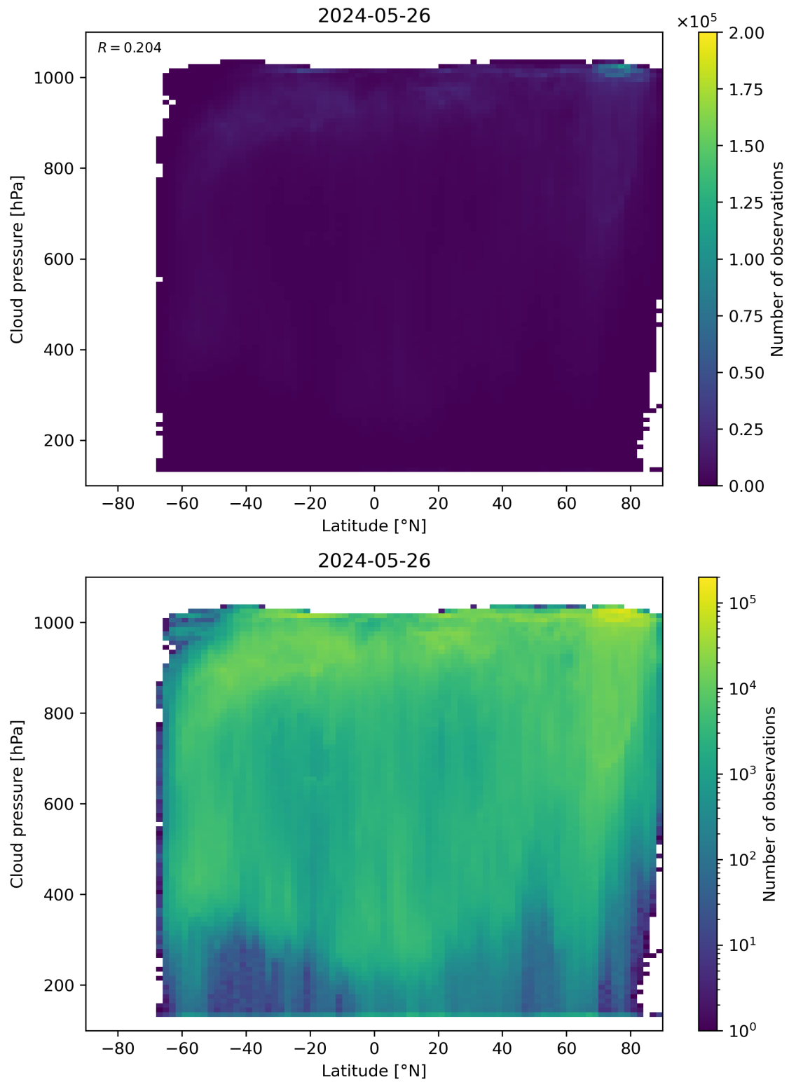
Figure 91: Scatter density plot of “Latitude” against “Cloud pressure” for 2024-05-25 to 2024-05-27.
