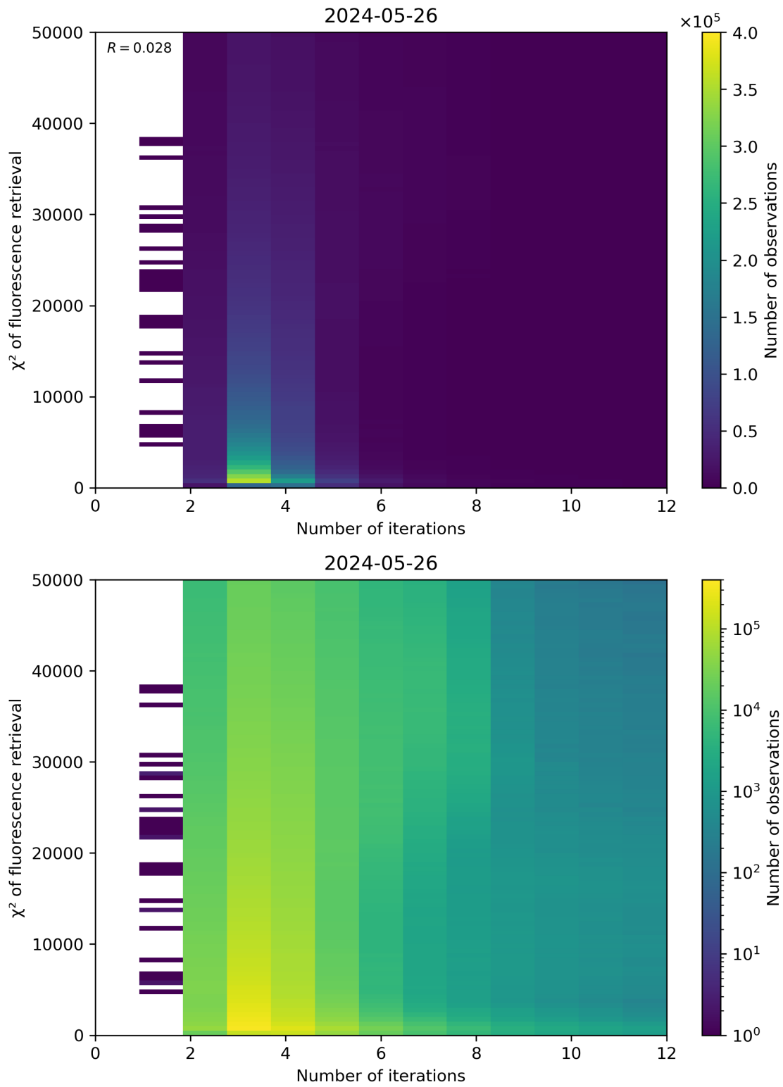
Figure 97: Scatter density plot of “Number of iterations” against “ \chi^2 of fluorescence retrieval” for 2024-05-25 to 2024-05-27.
