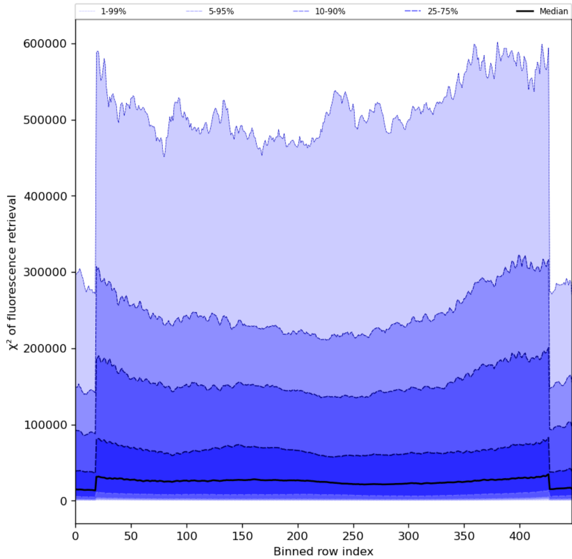
Figure 59: Along track statistics of “ \chi^2 of fluorescence retrieval” for 2024-05-25 to 2024-05-27
