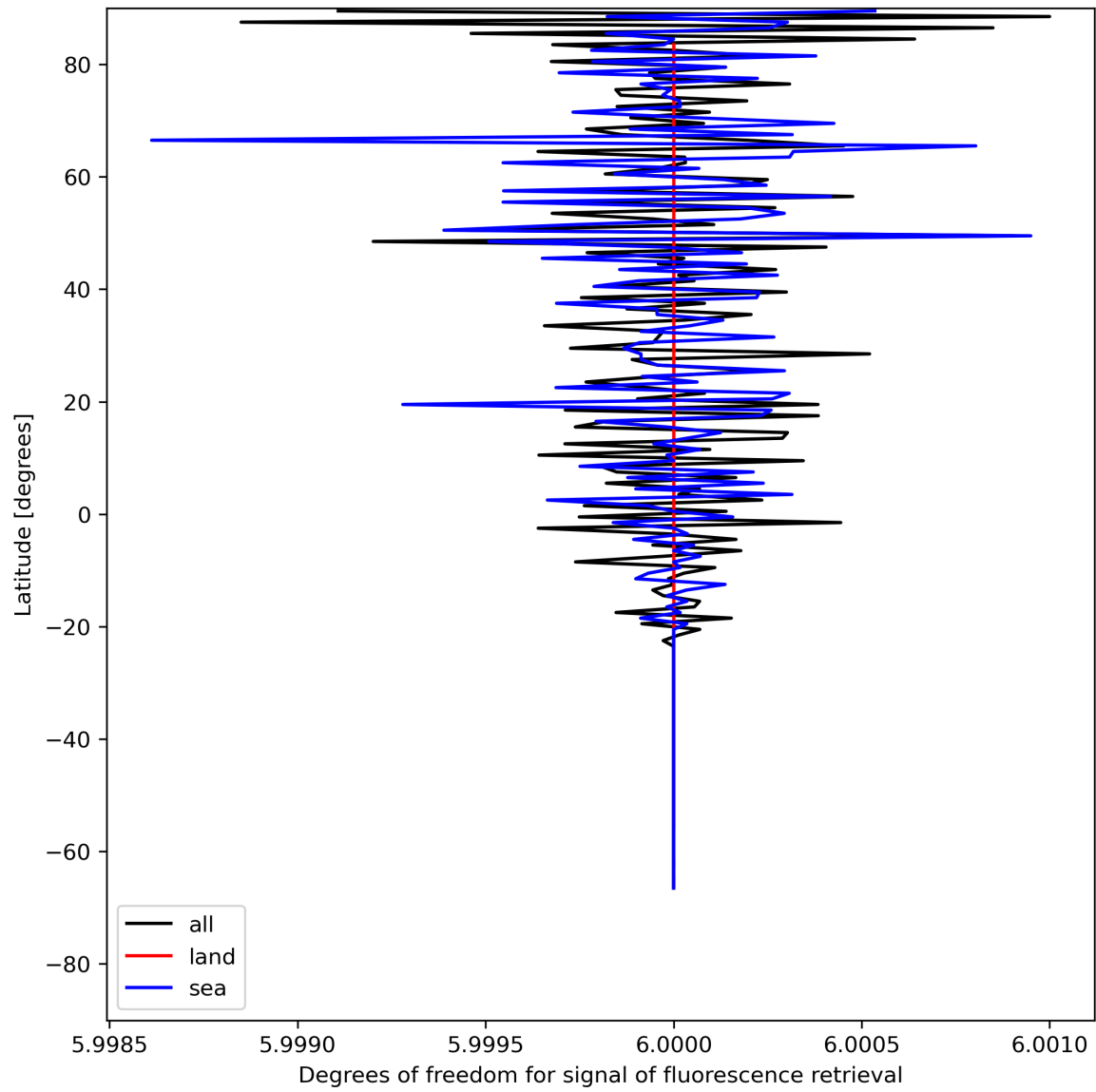
Figure 26: Zonal average of “Degrees of freedom for signal of fluorescence retrieval” for 2024-05-25 to 2024-05-27.
