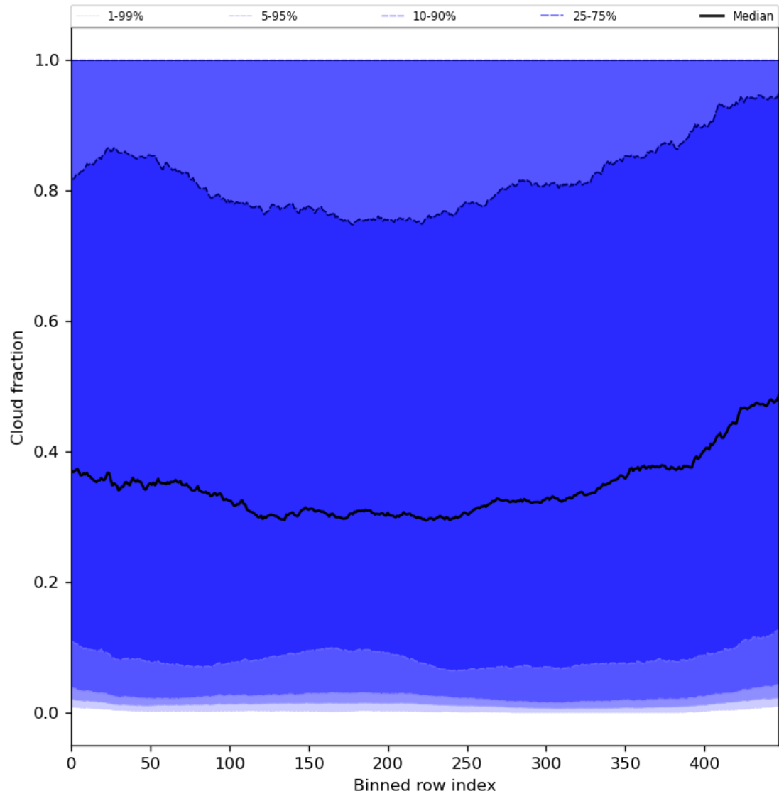
Figure 49: Along track statistics of “Cloud fraction” for 2024-05-25 to 2024-05-27
