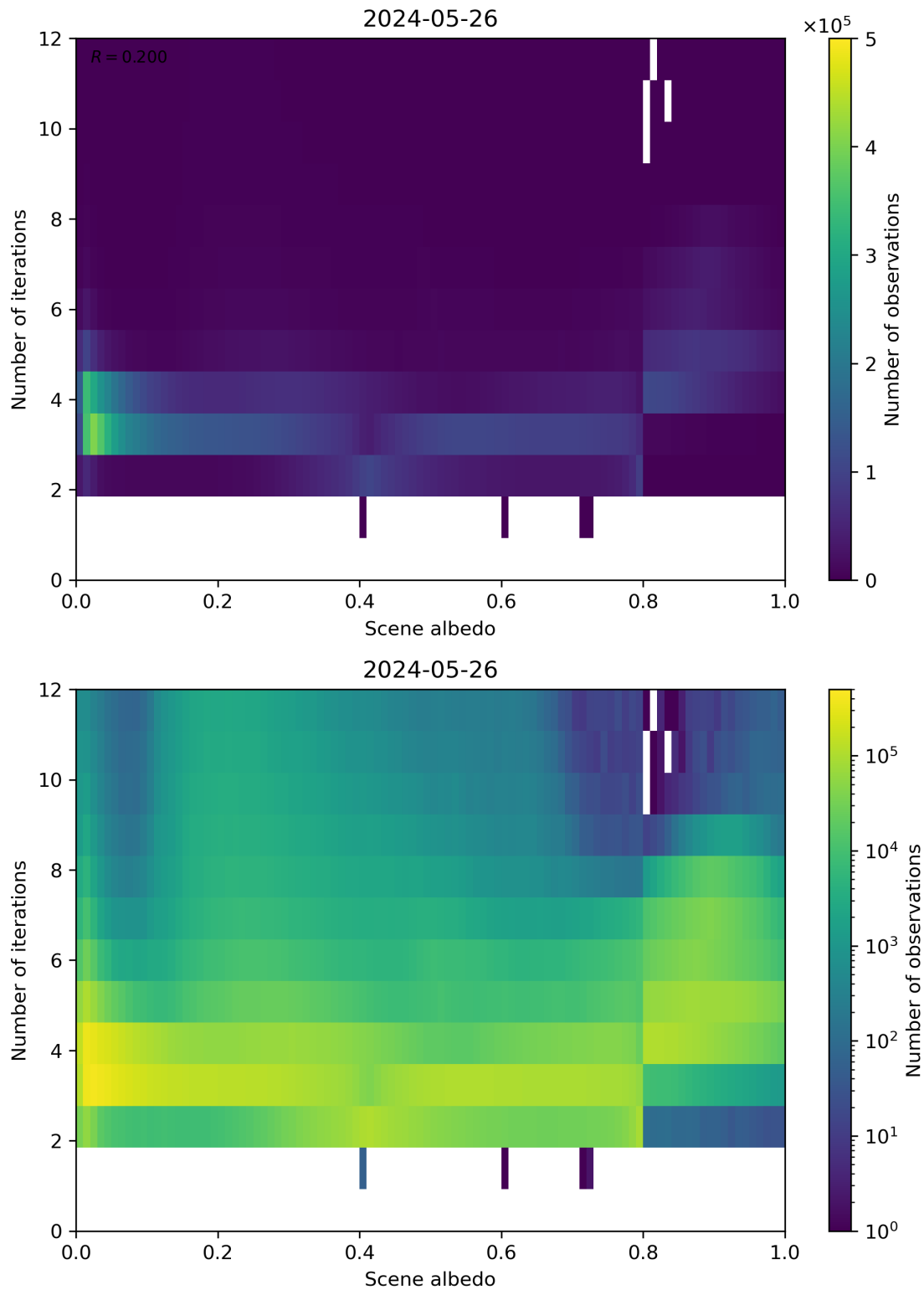
Figure 105: Scatter density plot of “Scene albedo” against “Number of iterations” for 2024-05-25 to 2024-05-27.
