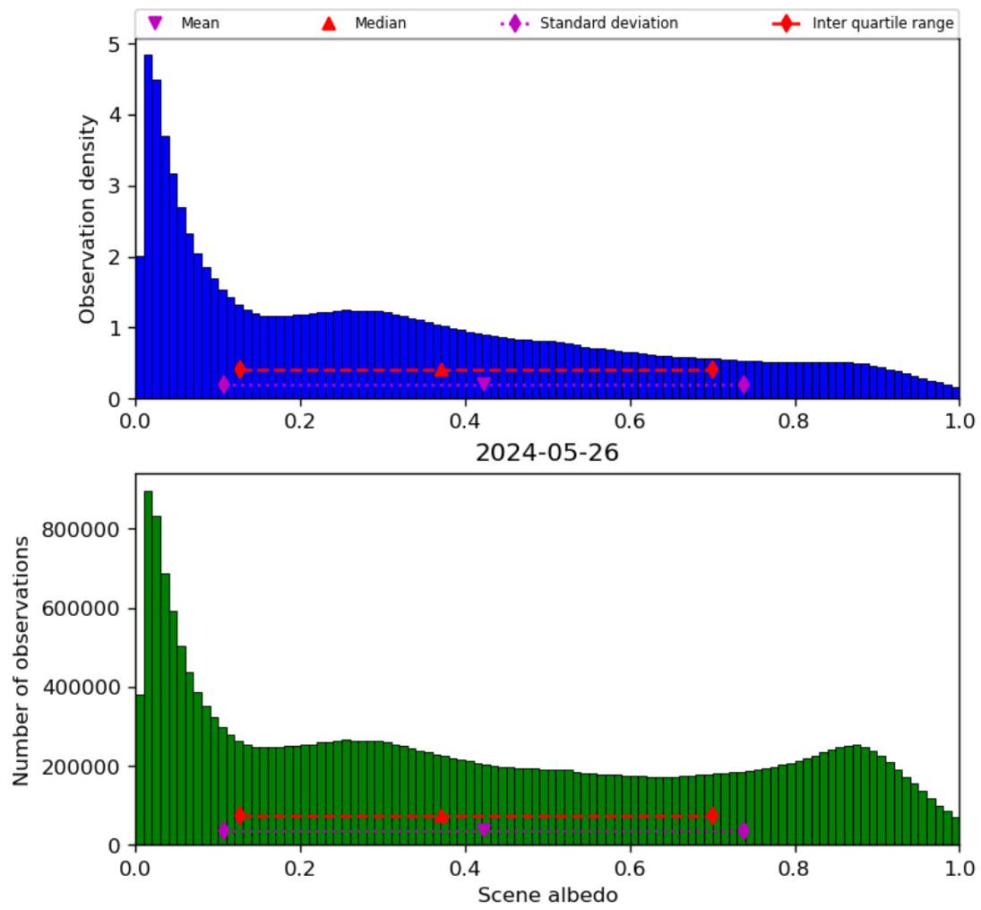
Figure 34: Histogram of “Scene albedo” for 2024-05-25 to 2024-05-27
