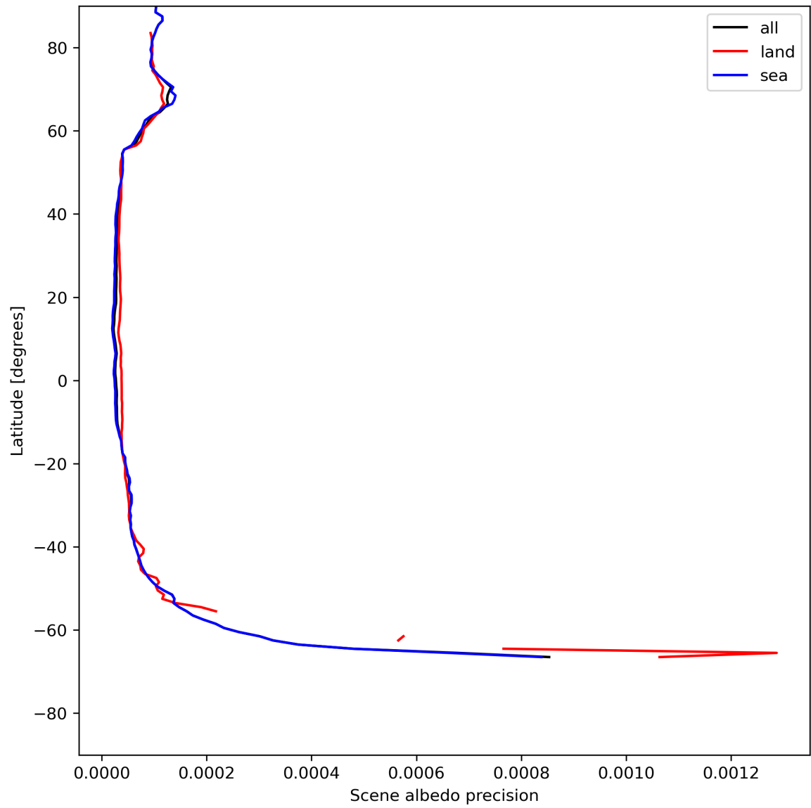
Figure 18: Zonal average of “Scene albedo precision” for 2024-05-25 to 2024-05-27.
