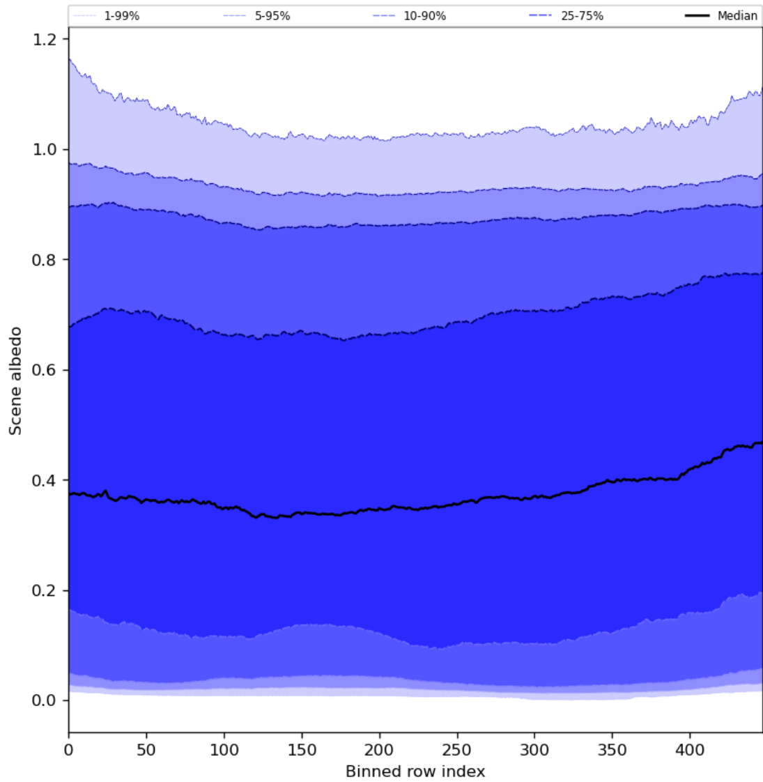
Figure 51: Along track statistics of “Scene albedo” for 2024-05-25 to 2024-05-27
