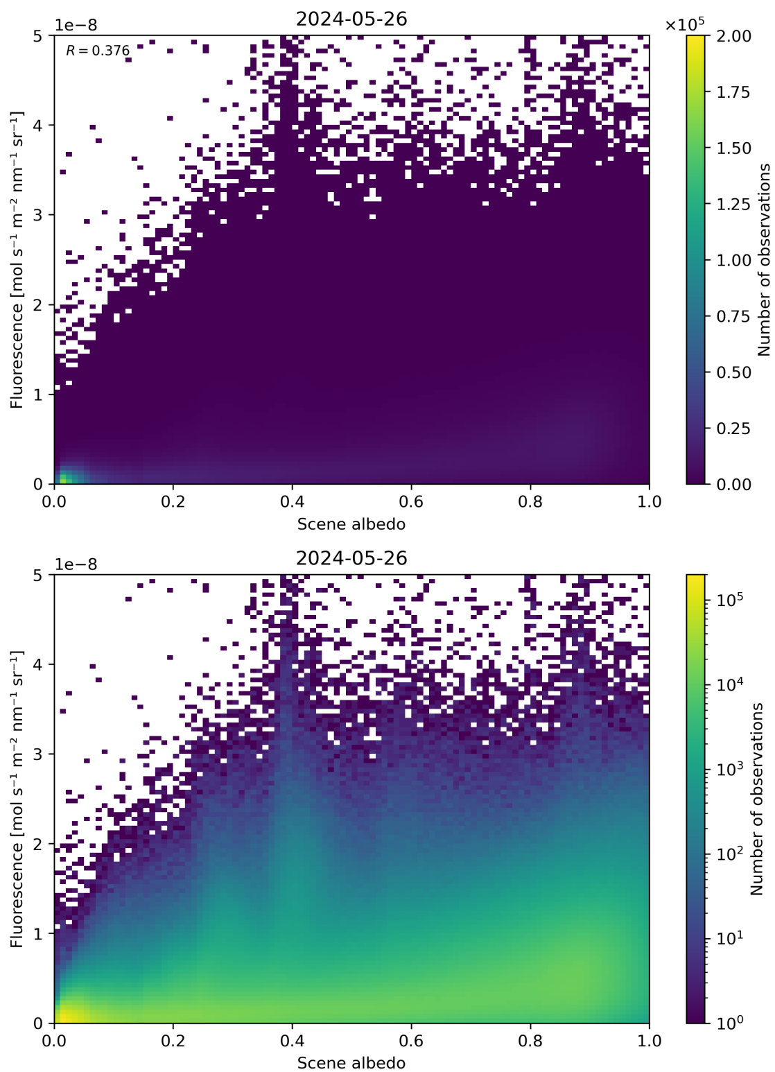
Figure 104: Scatter density plot of “Scene albedo” against “Fluorescence” for 2024-05-25 to 2024-05-27.
