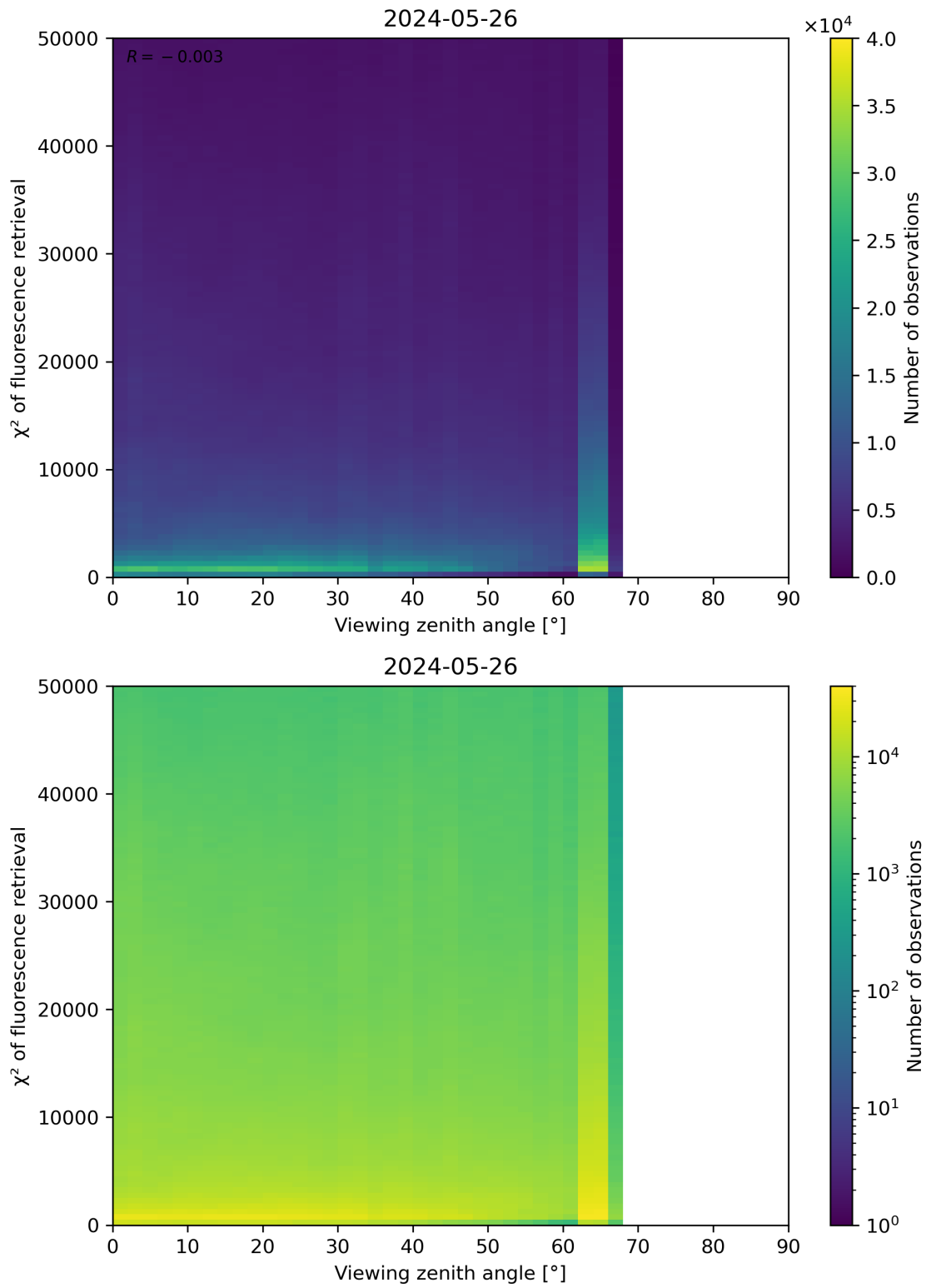
Figure 119: Scatter density plot of “Viewing zenith angle” against “ \chi^2 of fluorescence retrieval” for 2024-05-25 to 2024-05-27.
