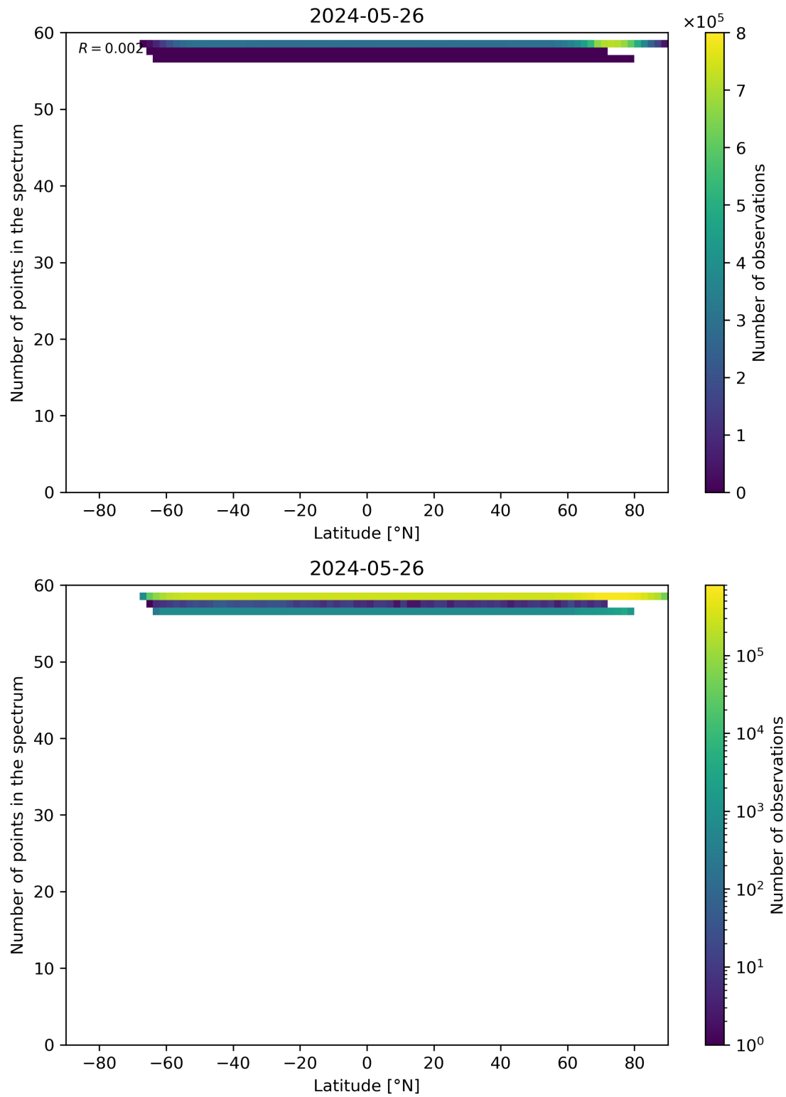
Figure 94: Scatter density plot of “Latitude” against “Number of points in the spectrum” for 2024-05-25 to 2024-05-27.
