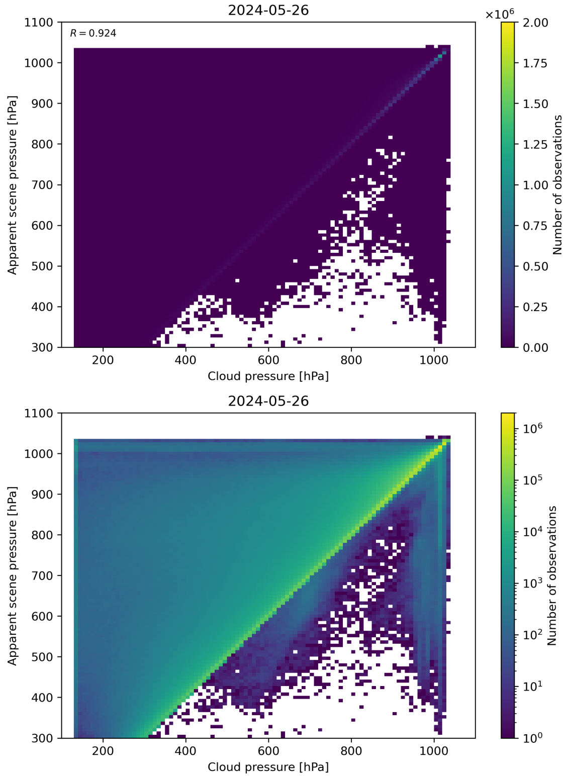
Figure 77: Scatter density plot of “Cloud pressure” against “Apparent scene pressure” for 2024-05-25 to 2024-05-27.
