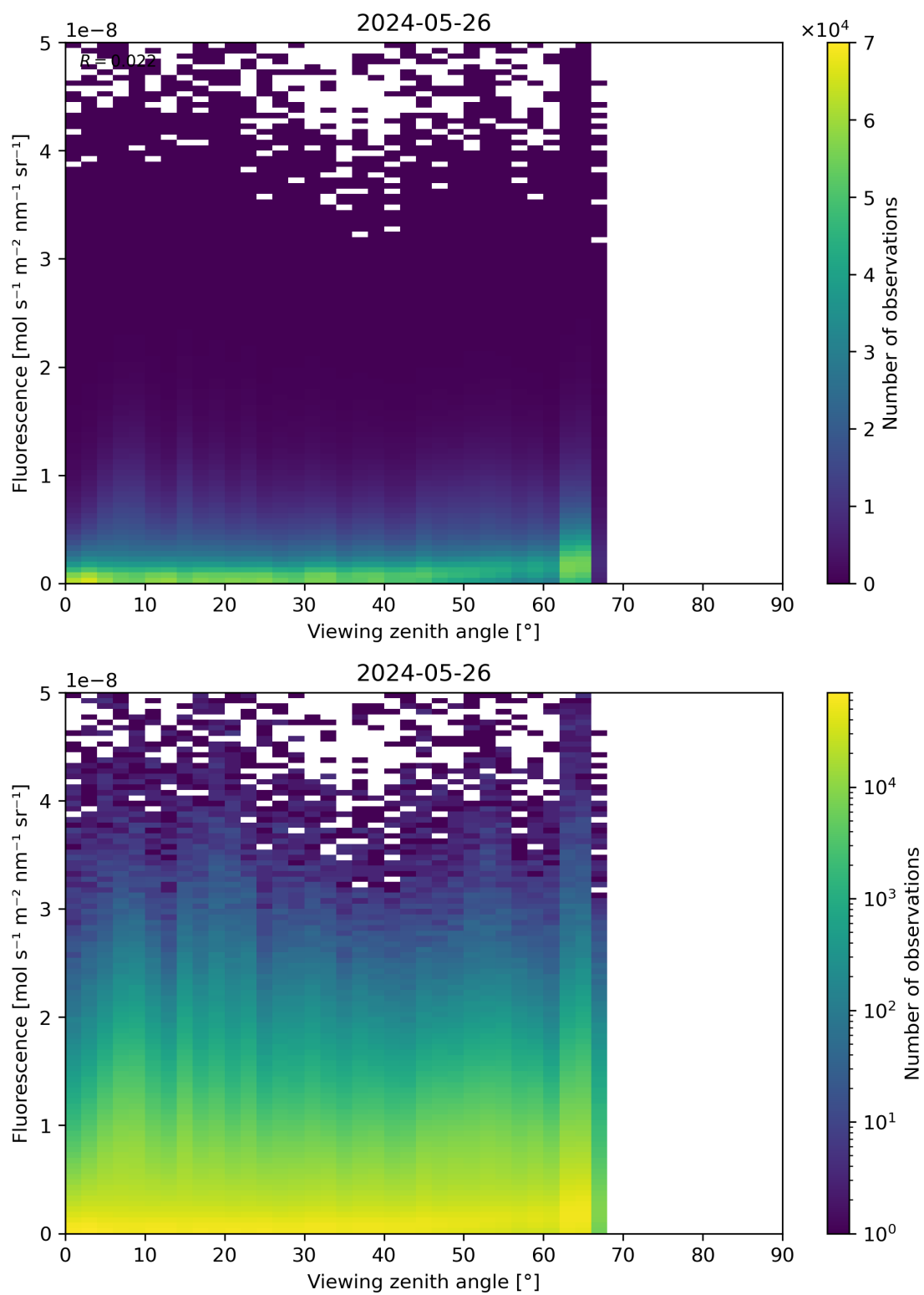
Figure 122: Scatter density plot of “Viewing zenith angle” against “Fluorescence” for 2024-05-25 to 2024-05-27.
