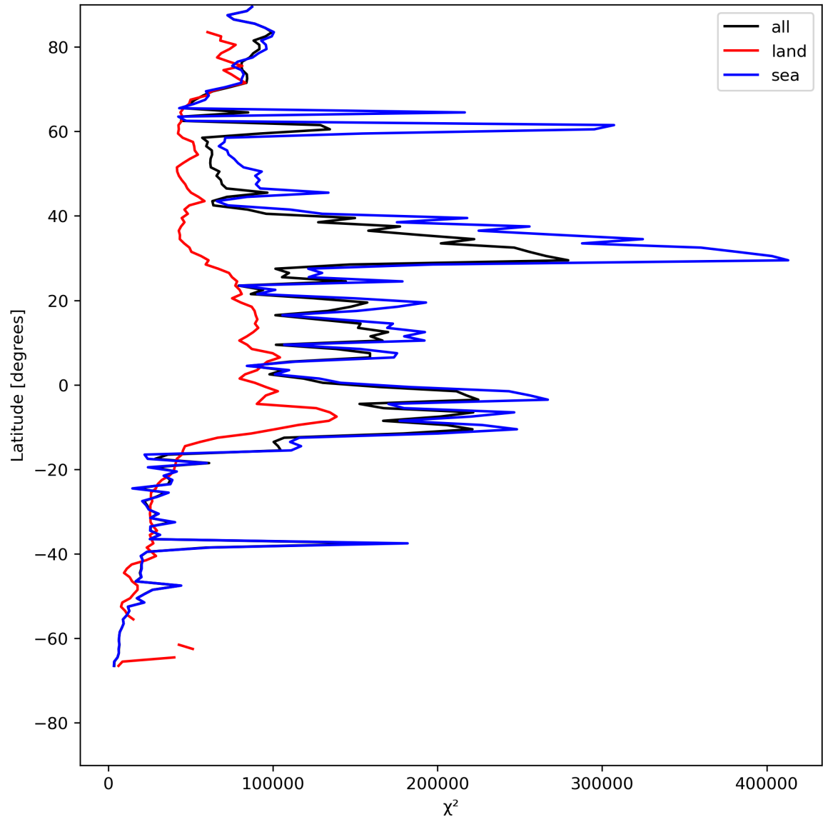
Figure 21: Zonal average of “ \chi^2 ” for 2024-05-25 to 2024-05-27.
