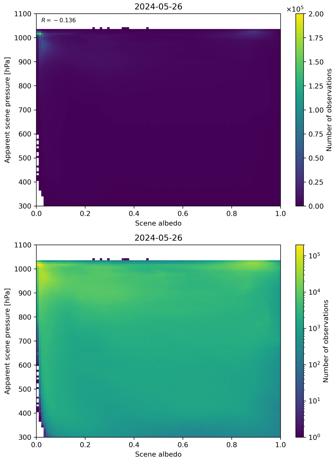
Figure 102: Scatter density plot of “Scene albedo” against “Apparent scene pressure” for 2024-05-25 to 2024-05-27.
