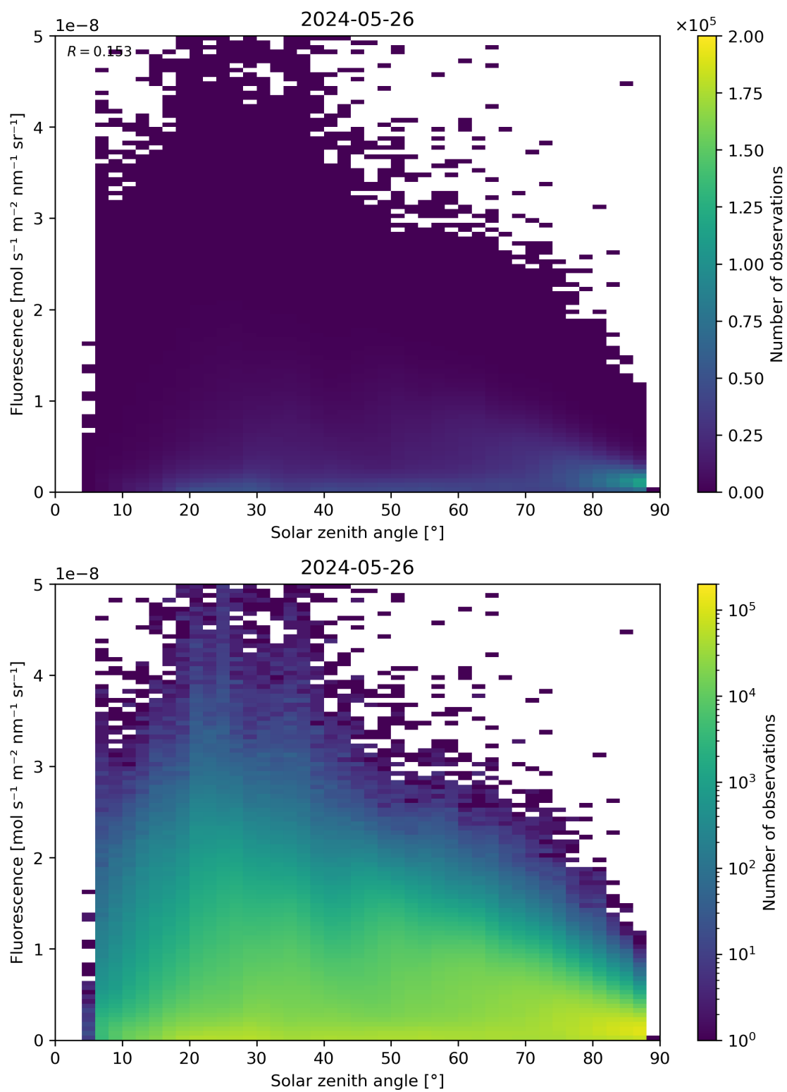
Figure 112: Scatter density plot of “Solar zenith angle” against “Fluorescence” for 2024-05-25 to 2024-05-27.
