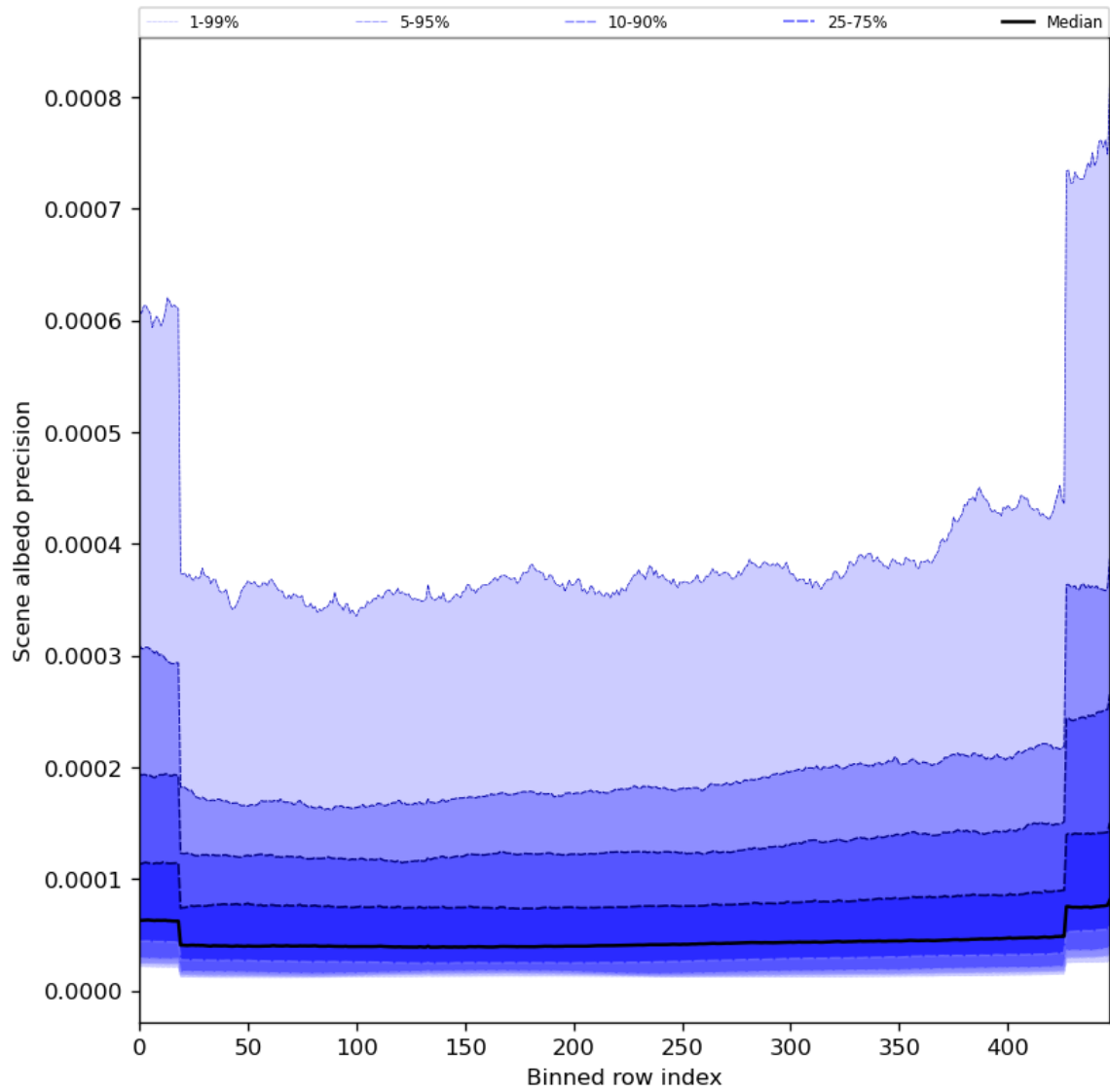
Figure 52: Along track statistics of “Scene albedo precision” for 2024-05-25 to 2024-05-27
