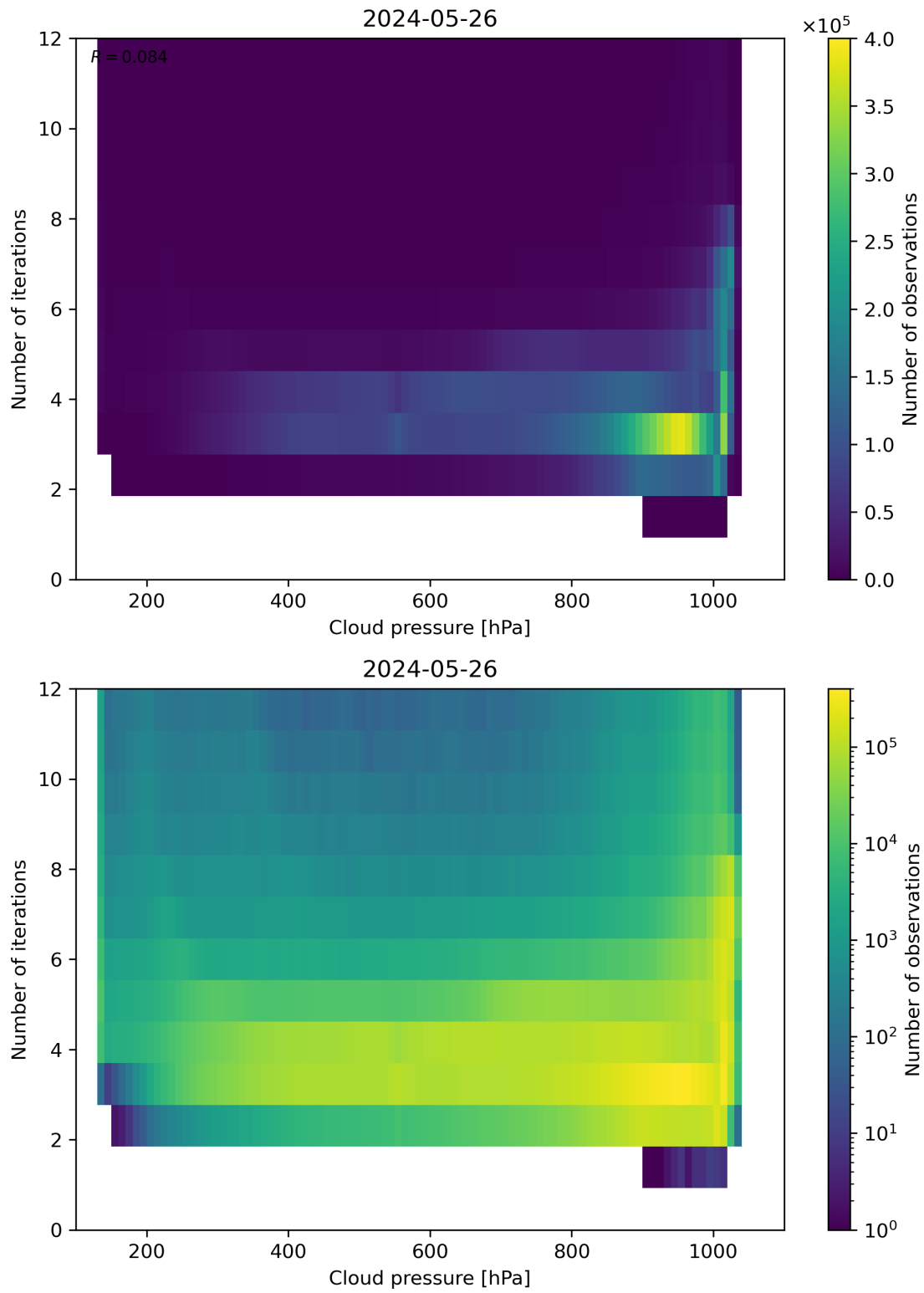
Figure 81: Scatter density plot of “Cloud pressure” against “Number of iterations” for 2024-05-25 to 2024-05-27.
