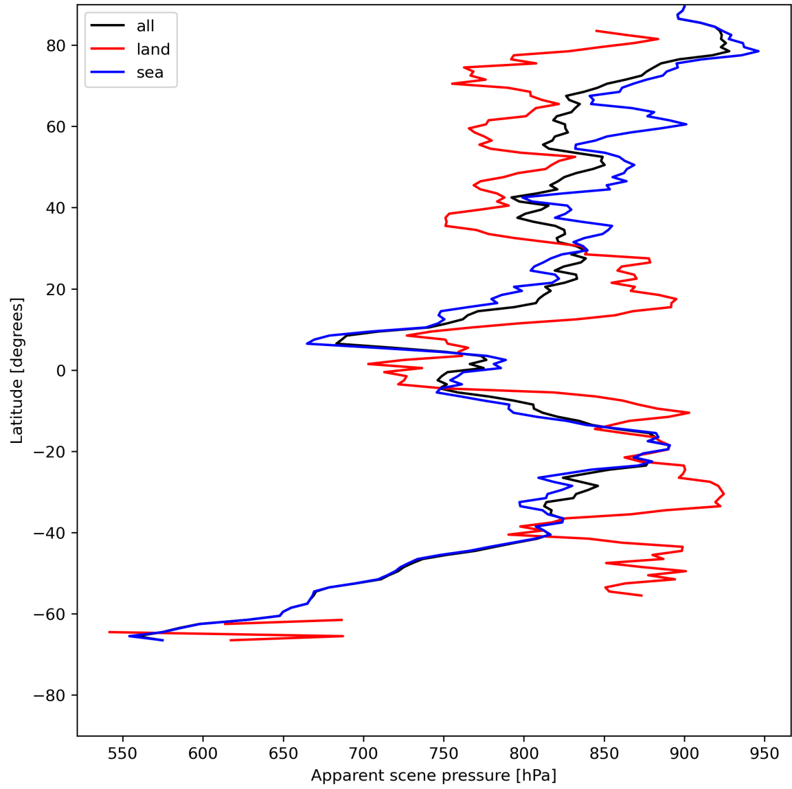
Figure 19: Zonal average of “Apparent scene pressure” for 2024-05-25 to 2024-05-27.
