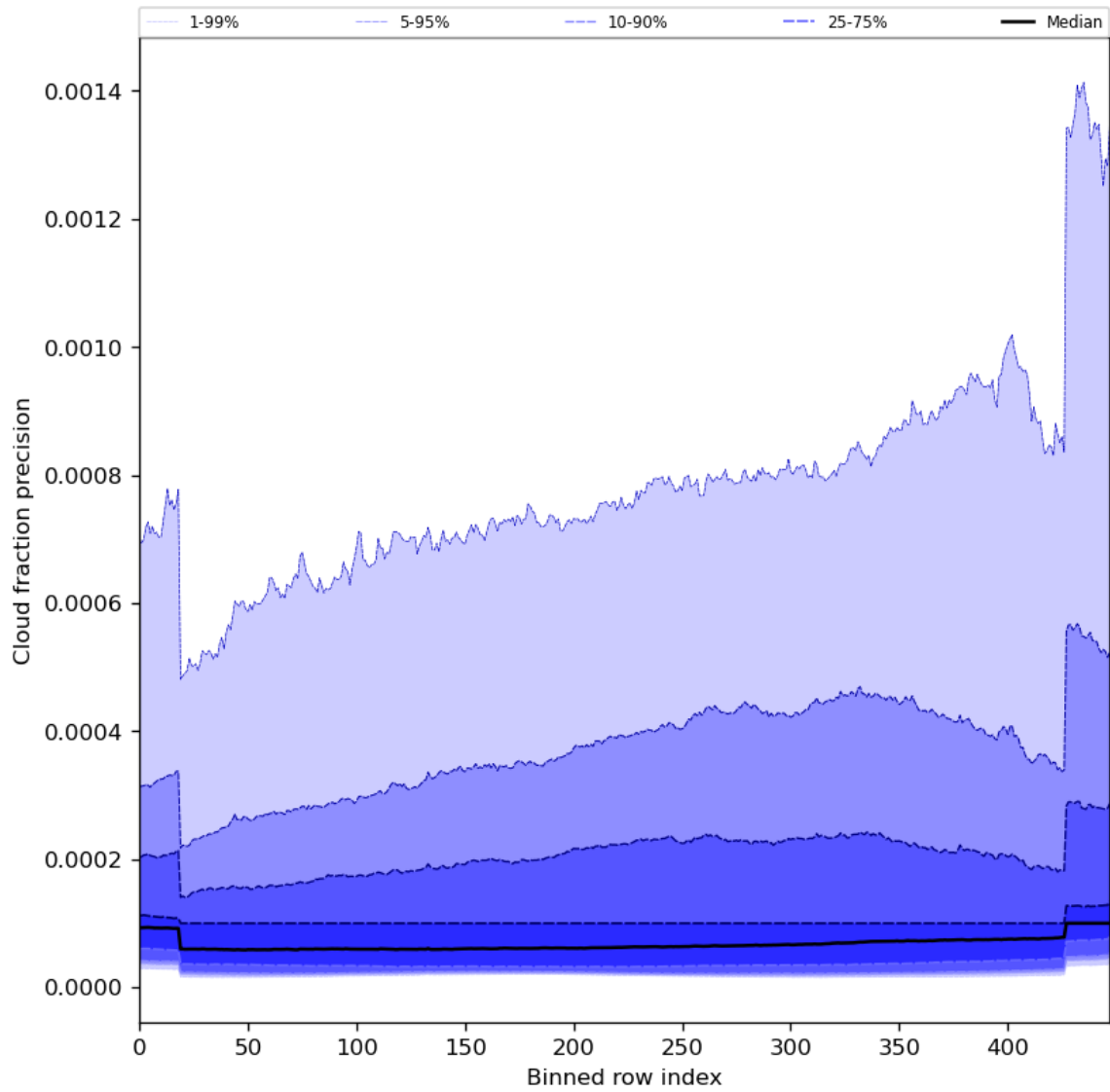
Figure 50: Along track statistics of “Cloud fraction precision” for 2024-05-25 to 2024-05-27
