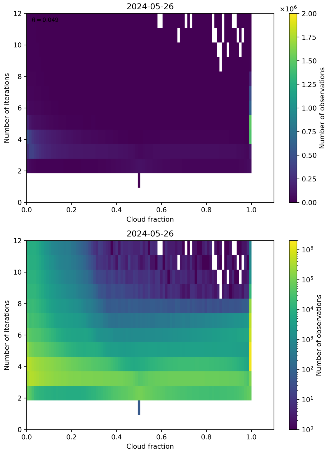
Figure 73: Scatter density plot of “Cloud fraction” against “Number of iterations” for 2024-05-25 to 2024-05-27.
