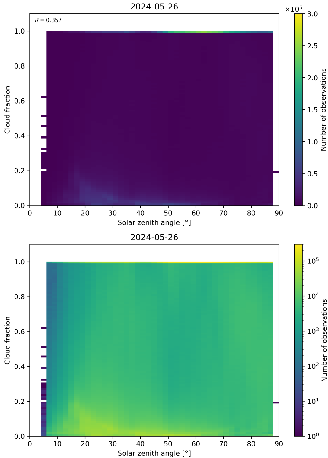
Figure 110: Scatter density plot of “Solar zenith angle” against “Cloud fraction” for 2024-05-25 to 2024-05-27.
