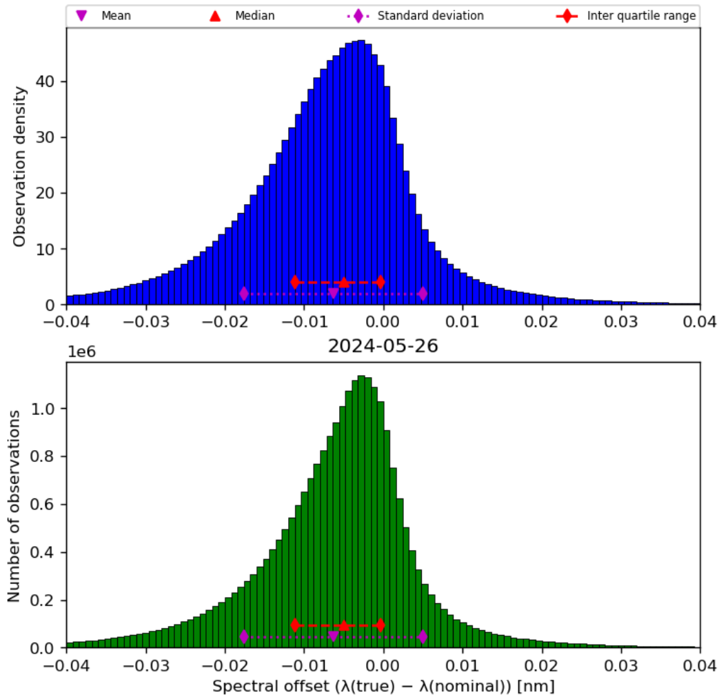
Figure 45: Histogram of “Spectral offset ( \lambda(\text{true}) - \lambda(\text{nominal}) )” for 2024-05-25 to 2024-05-27
