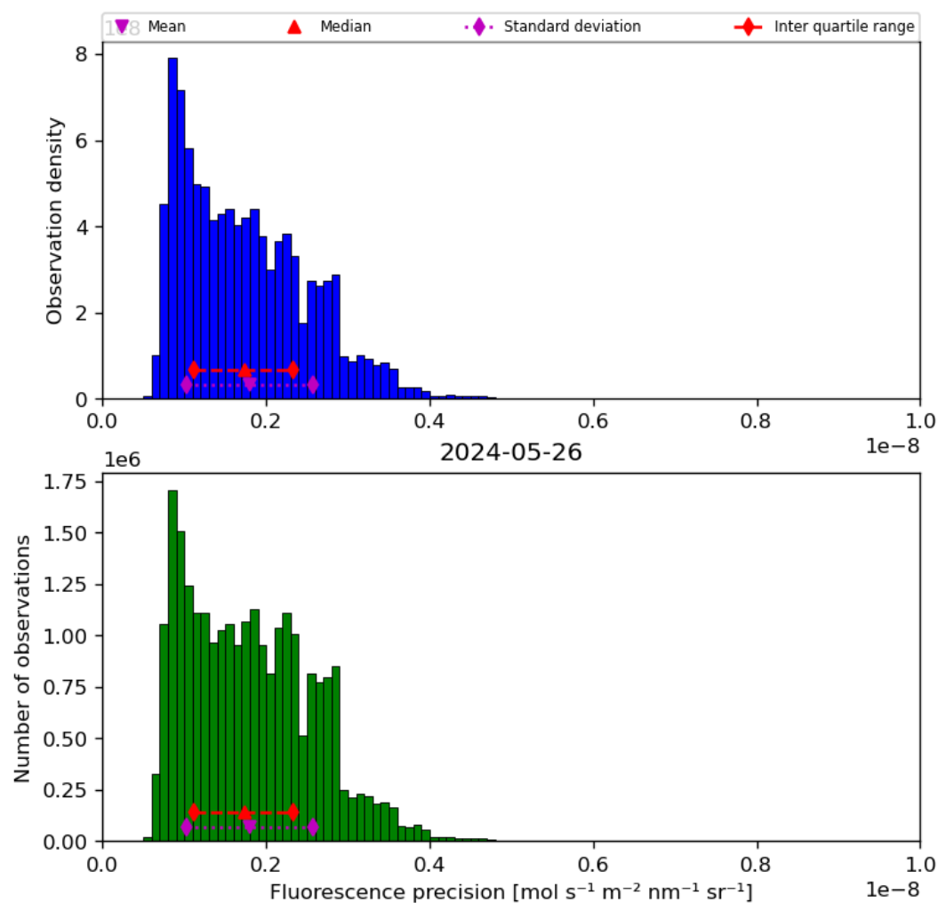
Figure 41: Histogram of “Fluorescence precision” for 2024-05-25 to 2024-05-27
