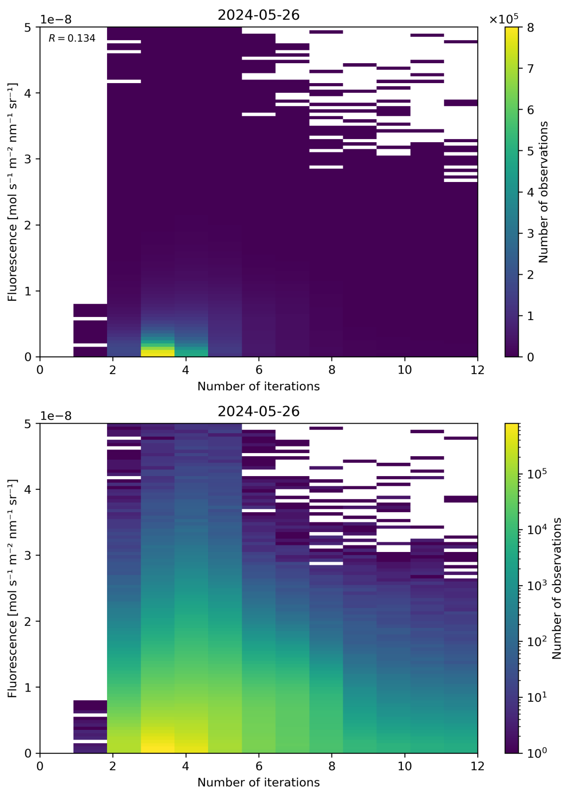
Figure 98: Scatter density plot of “Number of iterations” against “Fluorescence” for 2024-05-25 to 2024-05-27.
