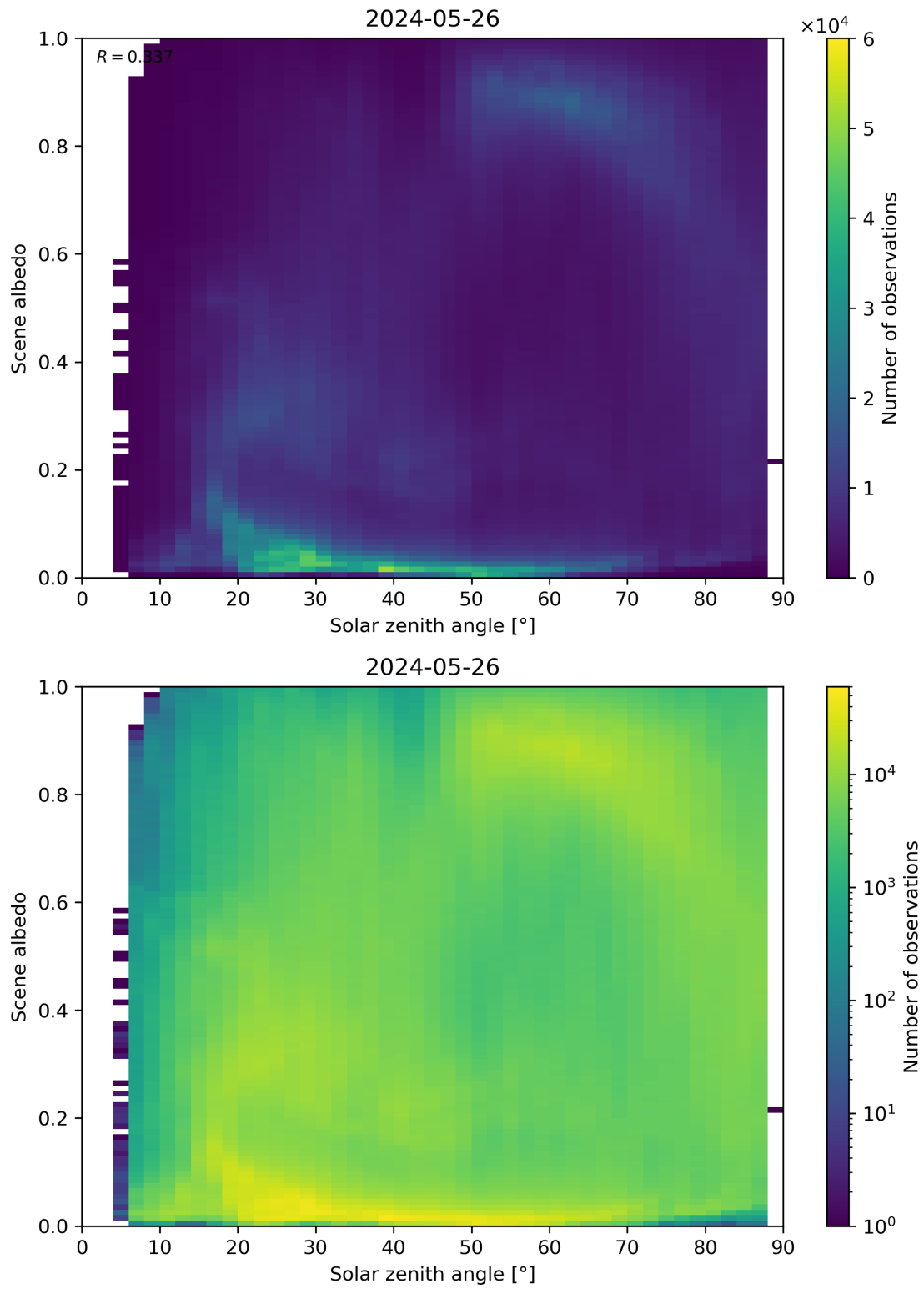
Figure 116: Scatter density plot of “Solar zenith angle” against “Scene albedo” for 2024-05-25 to 2024-05-27.
