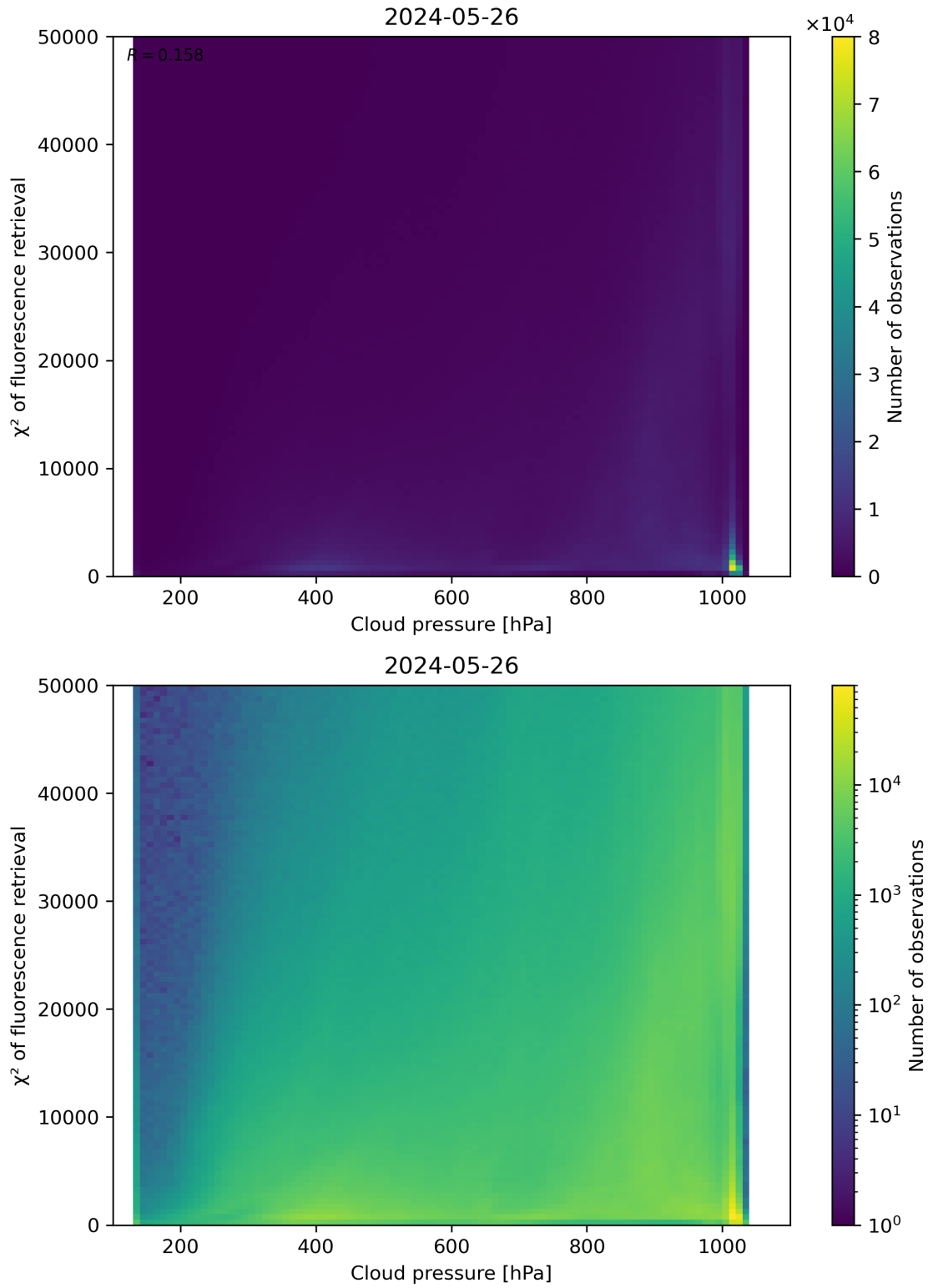
Figure 78: Scatter density plot of “Cloud pressure” against “ \chi^2 of fluorescence retrieval” for 2024-05-25 to 2024-05-27.
