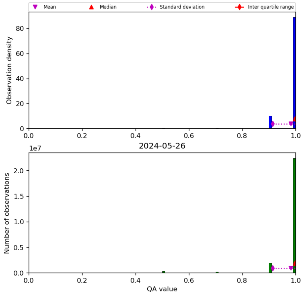
Figure 29: Histogram of “QA value” for 2024-05-25 to 2024-05-27
