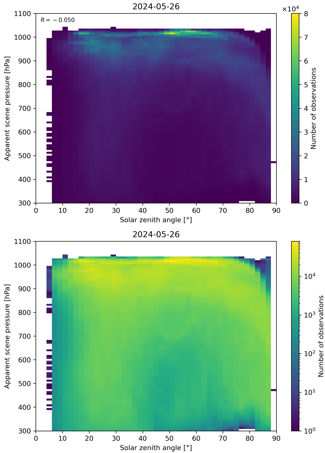
Figure 108: Scatter density plot of “Solar zenith angle” against “Apparent scene pressure” for 2024-05-25 to 2024-05-27.
