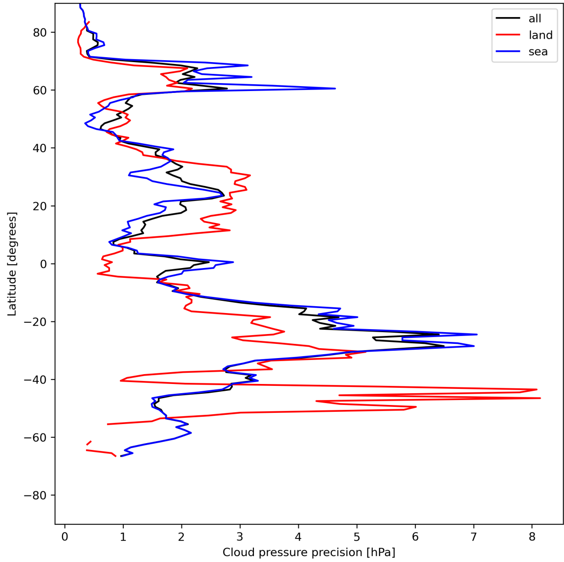
Figure 14: Zonal average of “Cloud pressure precision” for 2024-05-25 to 2024-05-27.
