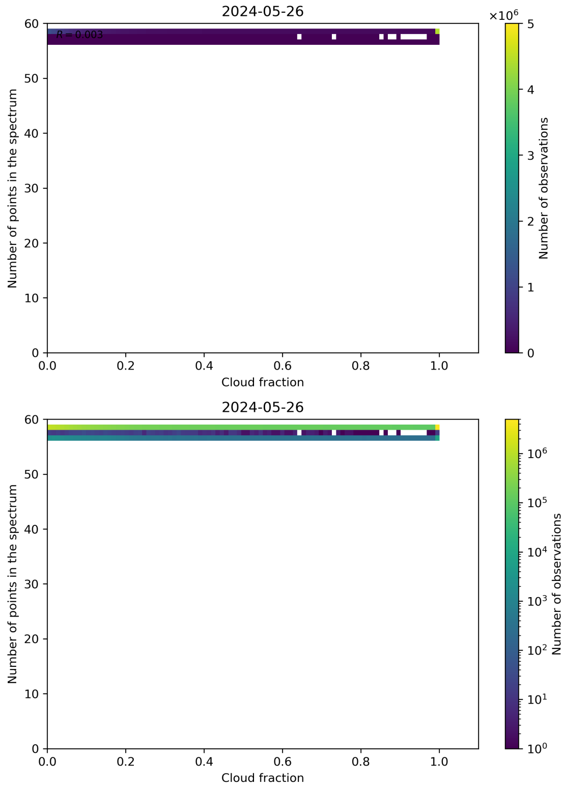
Figure 74: Scatter density plot of “Cloud fraction” against “Number of points in the spectrum” for 2024-05-25 to 2024-05-27.
