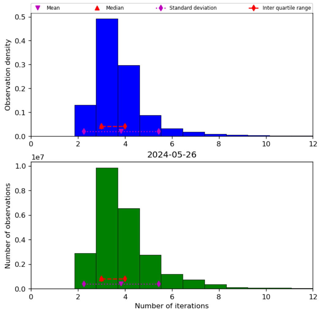
Figure 39: Histogram of “Number of iterations” for 2024-05-25 to 2024-05-27
