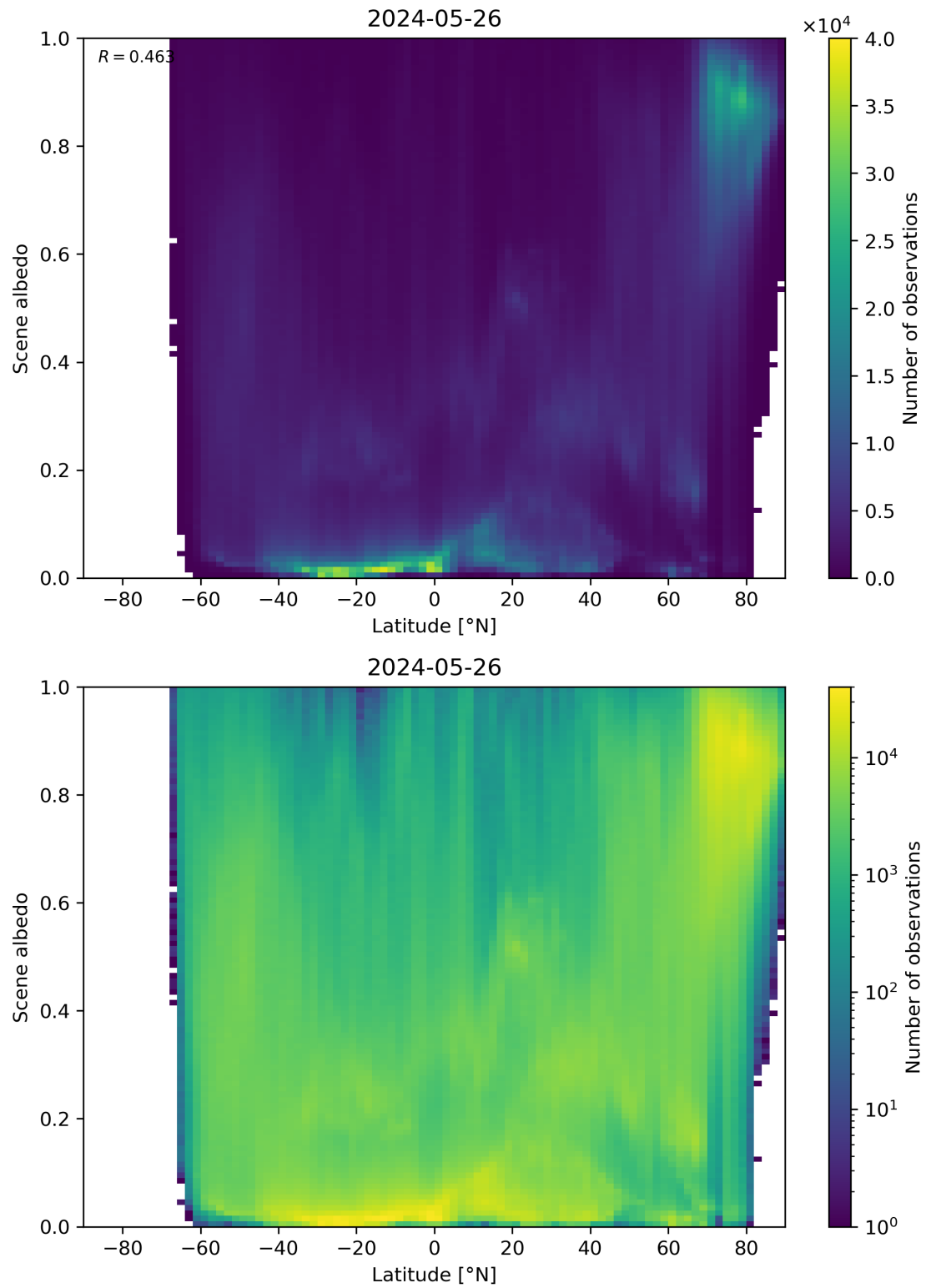
Figure 95: Scatter density plot of “Latitude” against “Scene albedo” for 2024-05-25 to 2024-05-27.
