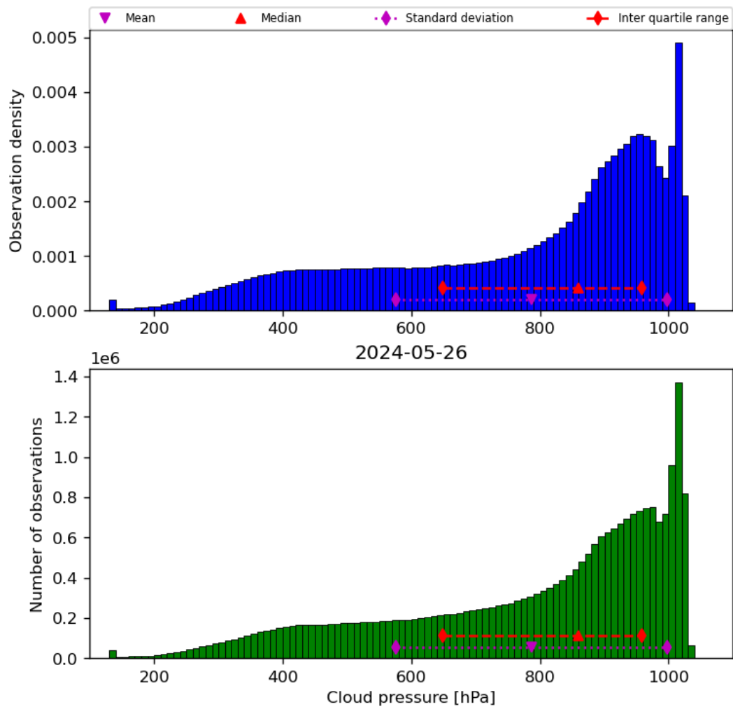
Figure 30: Histogram of “Cloud pressure” for 2024-05-25 to 2024-05-27
