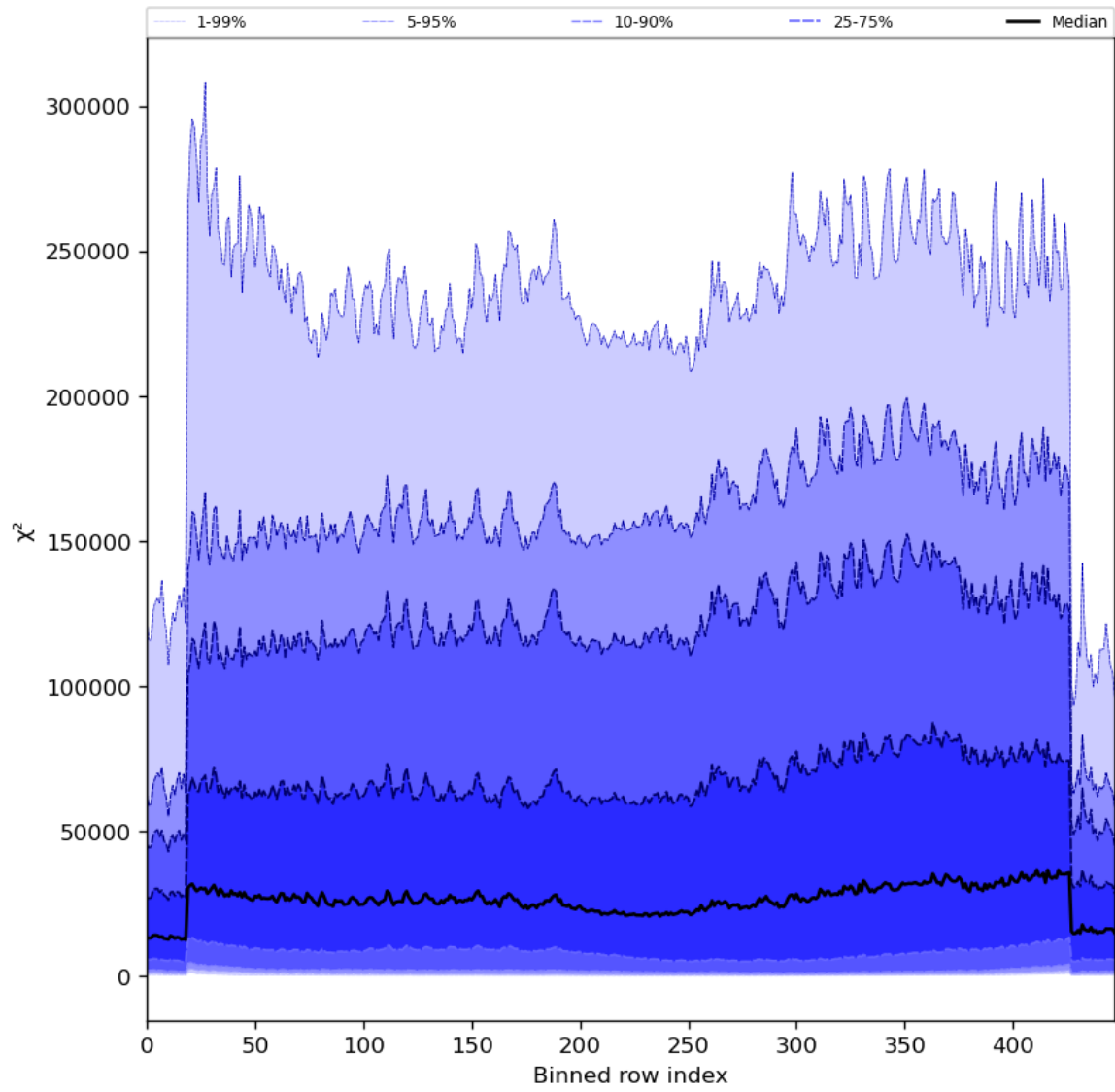
Figure 55: Along track statistics of “ \chi^2 ” for 2024-05-25 to 2024-05-27
