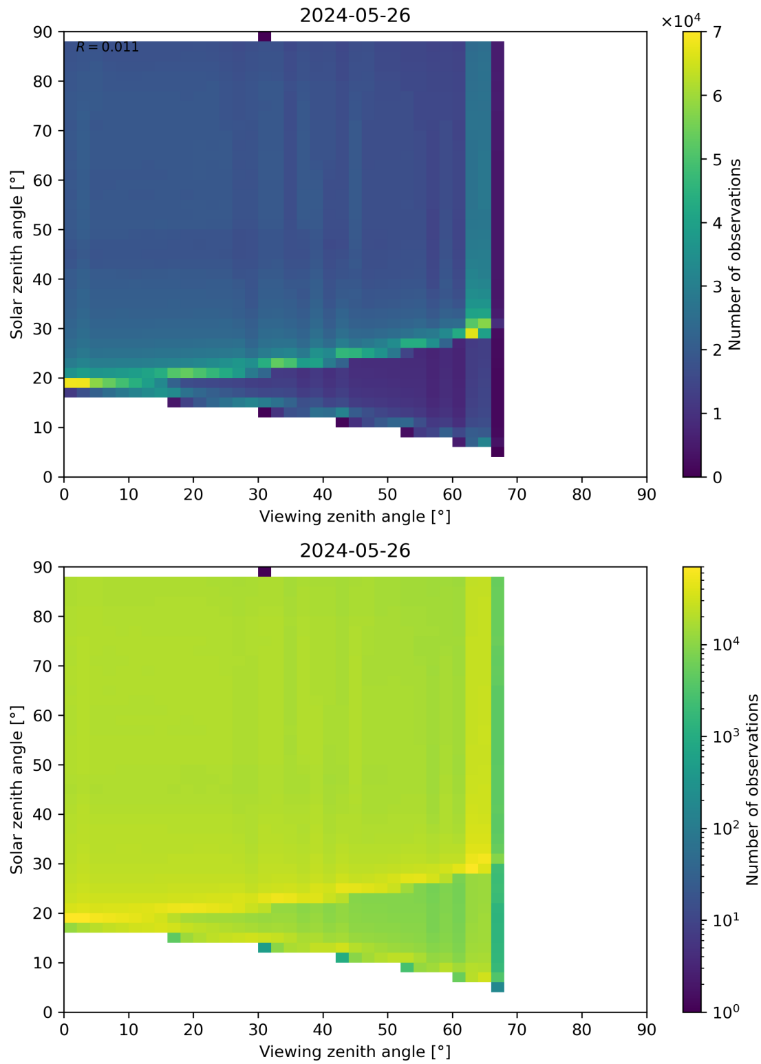
Figure 127: Scatter density plot of “Viewing zenith angle” against “Solar zenith angle” for 2024-05-25 to 2024-05-27.
