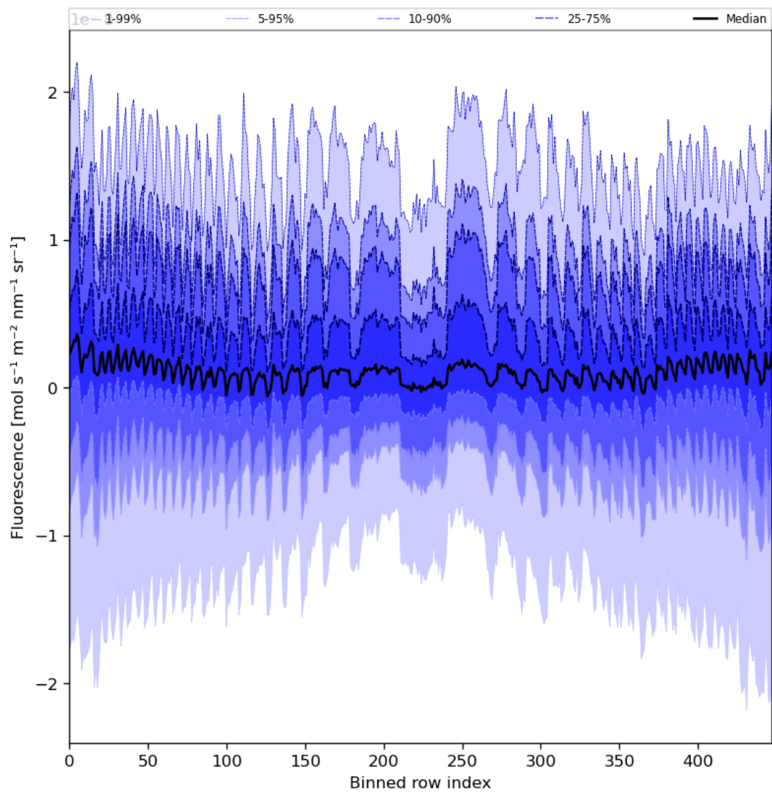
Figure 57: Along track statistics of “Fluorescence” for 2024-05-25 to 2024-05-27
