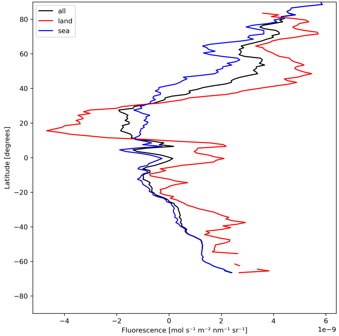
Figure 23: Zonal average of “Fluorescence” for 2024-05-25 to 2024-05-27.
