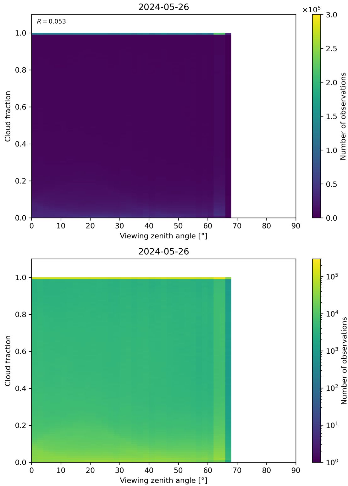
Figure 120: Scatter density plot of “Viewing zenith angle” against “Cloud fraction” for 2024-05-25 to 2024-05-27.
