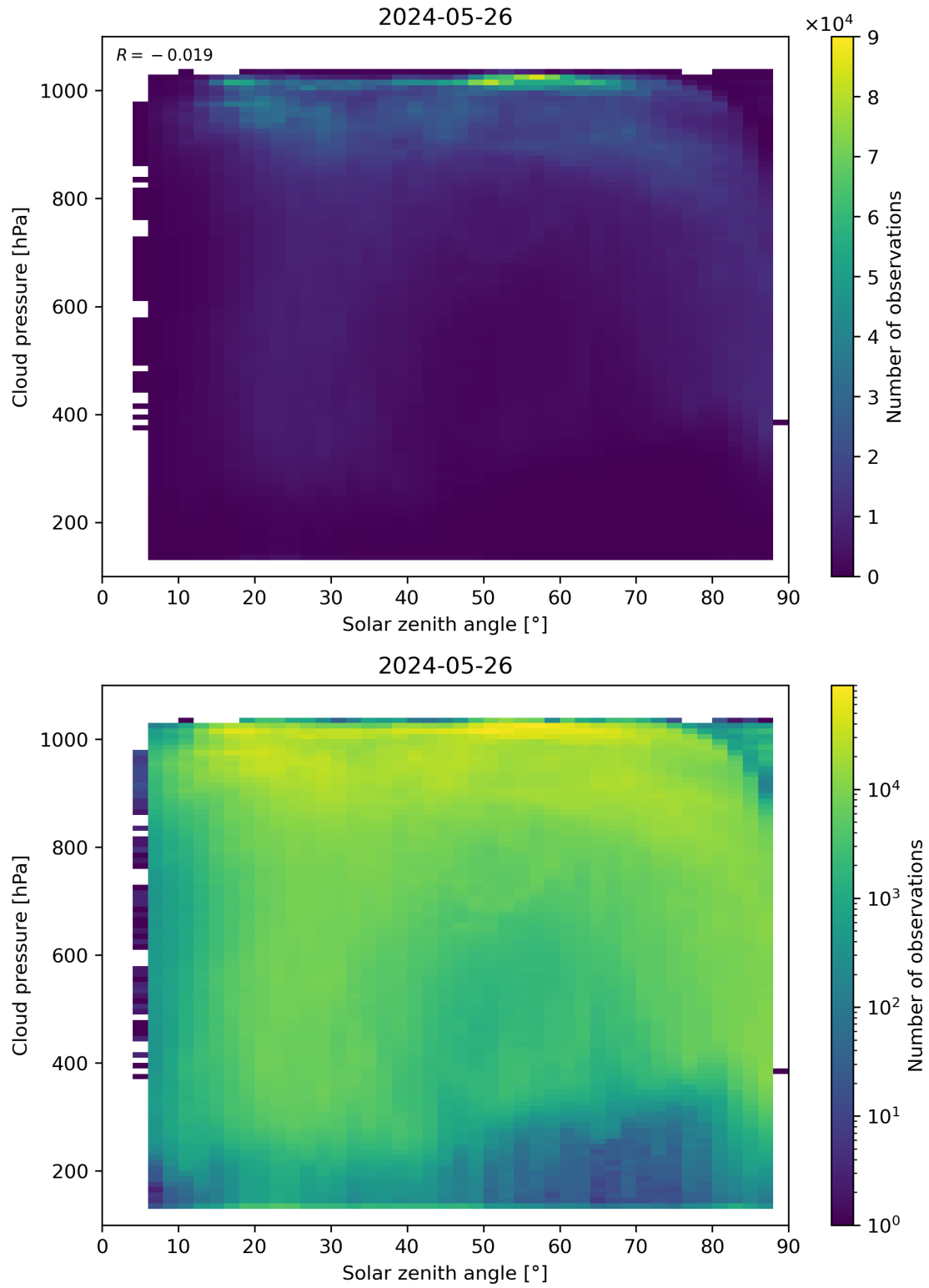
Figure 111: Scatter density plot of “Solar zenith angle” against “Cloud pressure” for 2024-05-25 to 2024-05-27.
