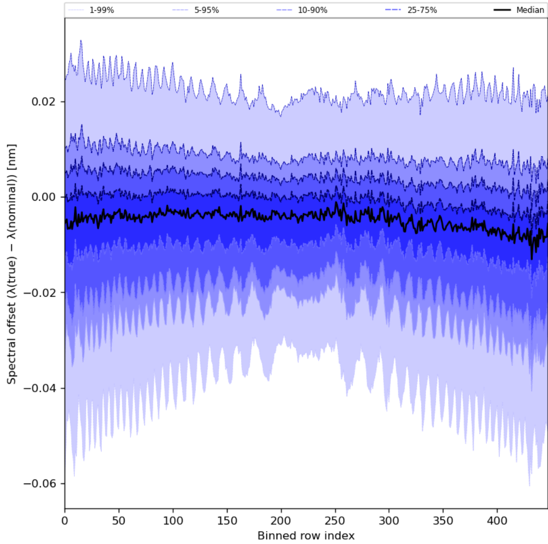
Figure 62: Along track statistics of “Spectral offset ( \lambda(\text{true}) - \lambda(\text{nominal}) )” for 2024-05-25 to 2024-05-27
