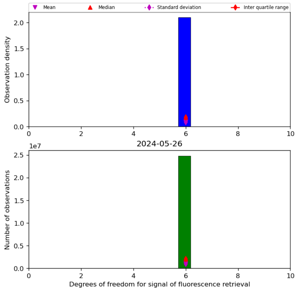
Figure 43: Histogram of “Degrees of freedom for signal of fluorescence retrieval” for 2024-05-25 to 2024-05-27
