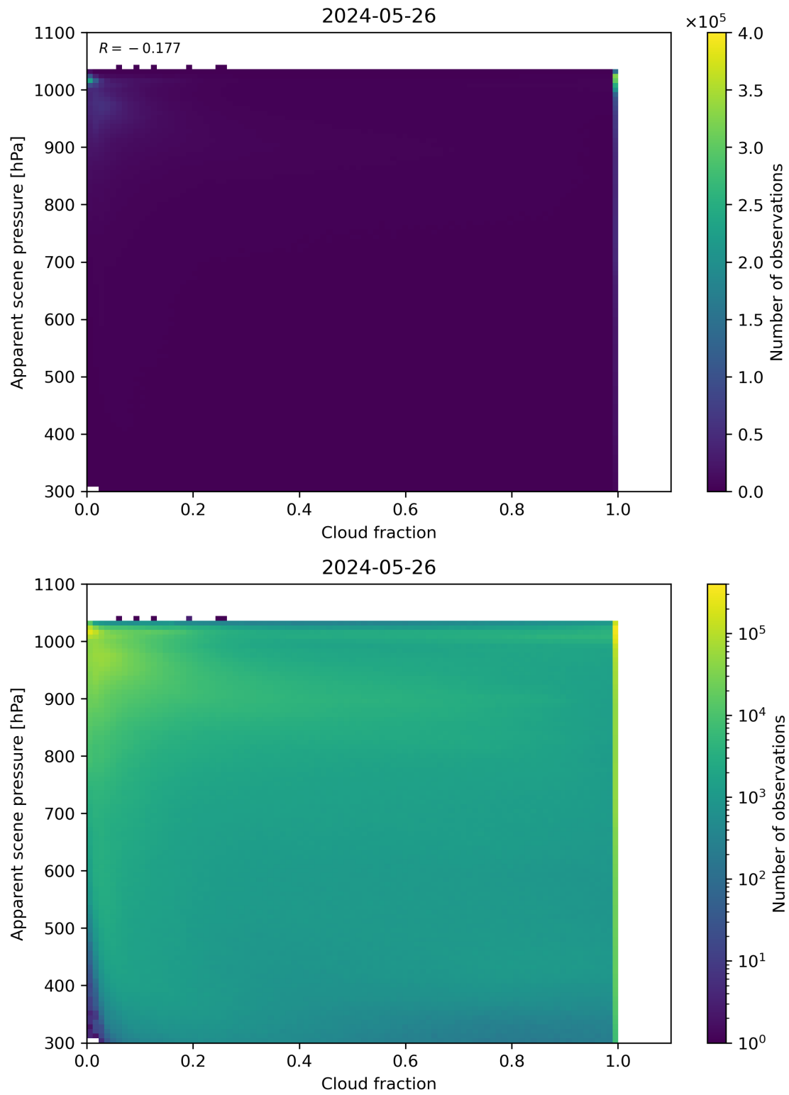
Figure 70: Scatter density plot of “Cloud fraction” against “Apparent scene pressure” for 2024-05-25 to 2024-05-27.
