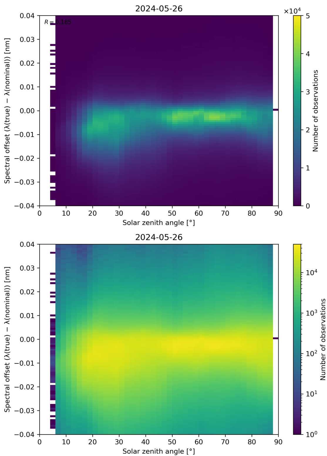
Figure 117: Scatter density plot of “Solar zenith angle” against “Spectral offset ( \lambda(\text{true}) - \lambda(\text{nominal}) )” for 2024-05-25 to 2024-05-27.
