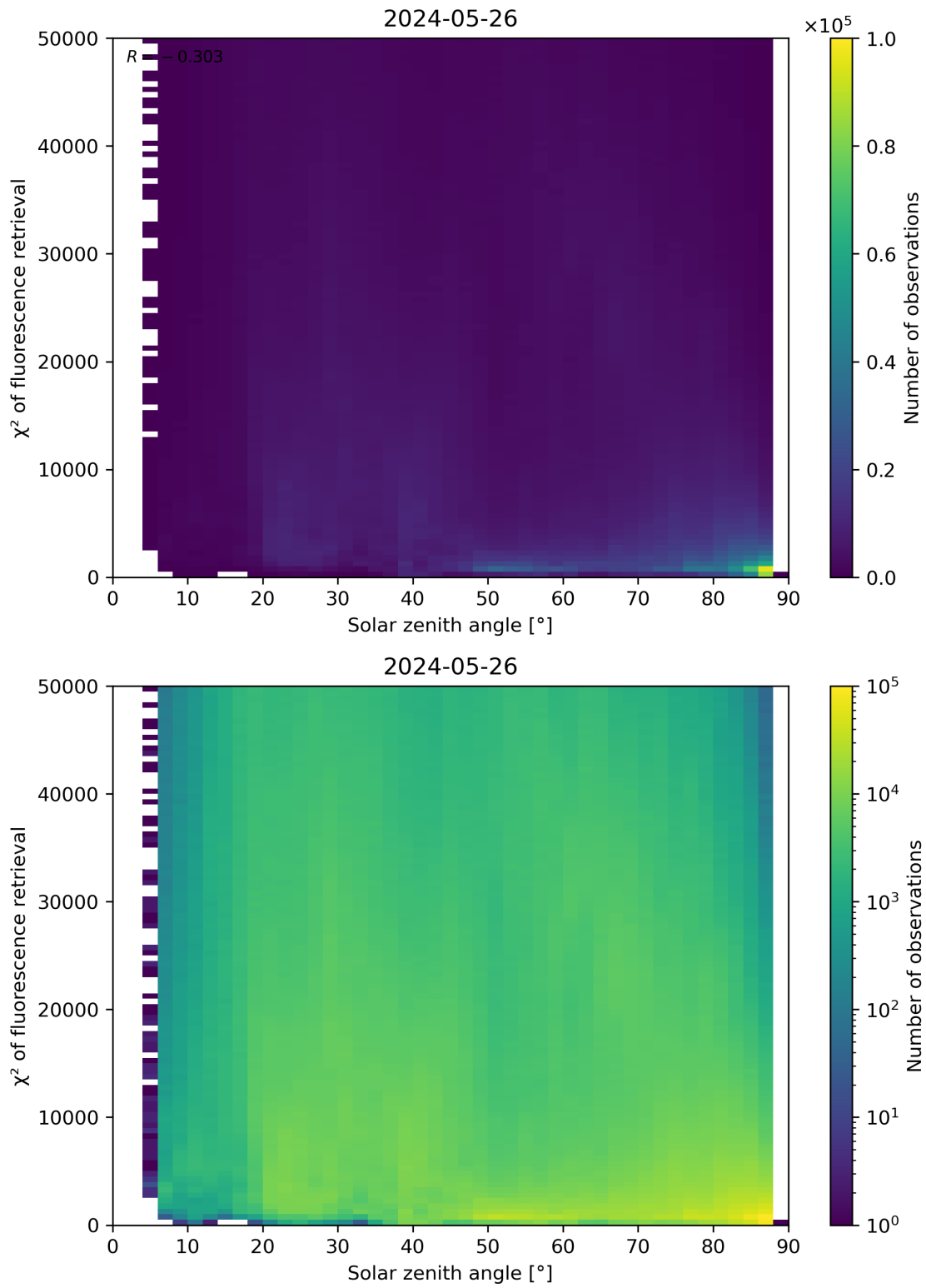
Figure 109: Scatter density plot of “Solar zenith angle” against “ \chi^2 of fluorescence retrieval” for 2024-05-25 to 2024-05-27.
