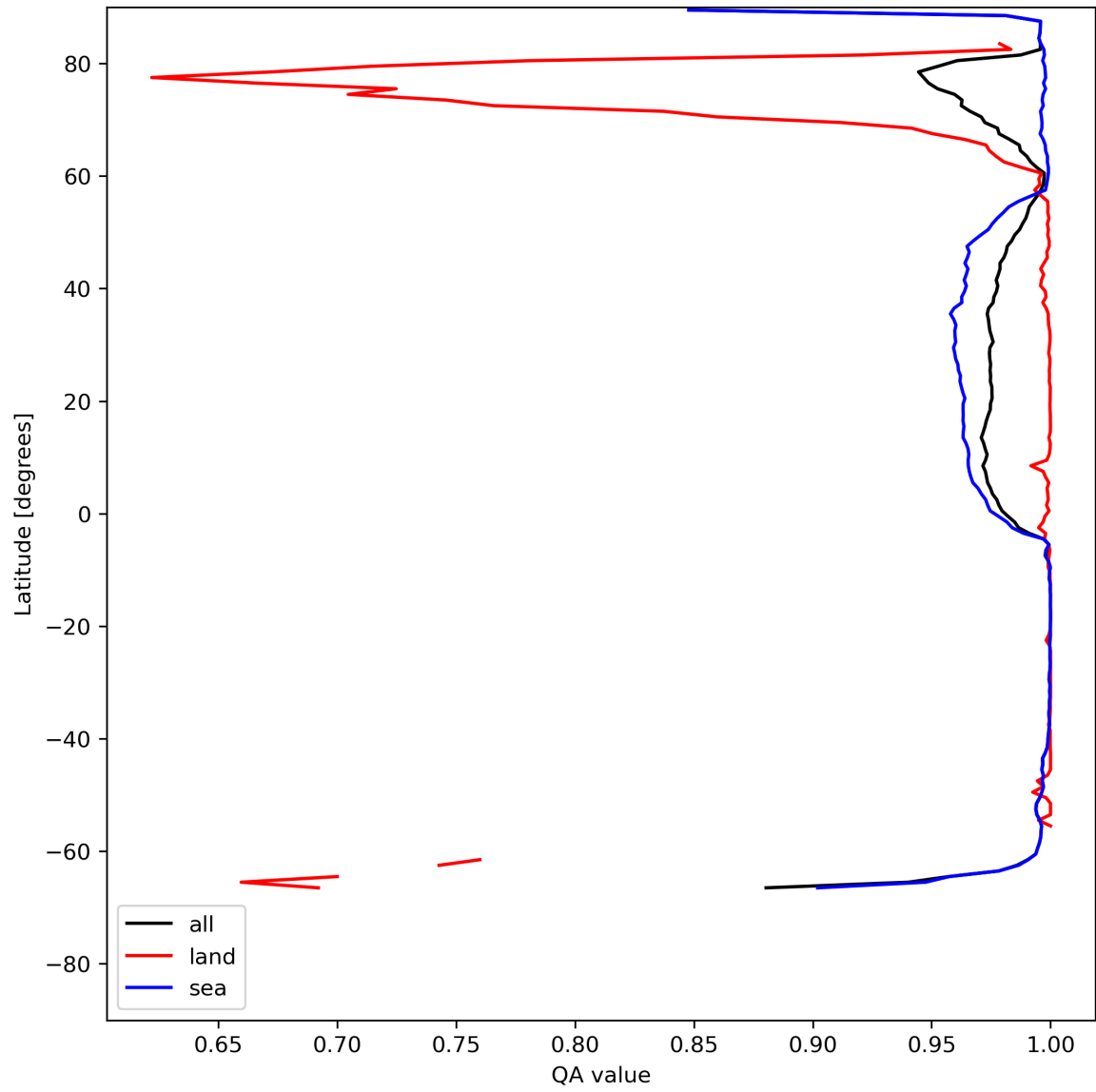
Figure 12: Zonal average of “QA value” for 2024-05-25 to 2024-05-27.
