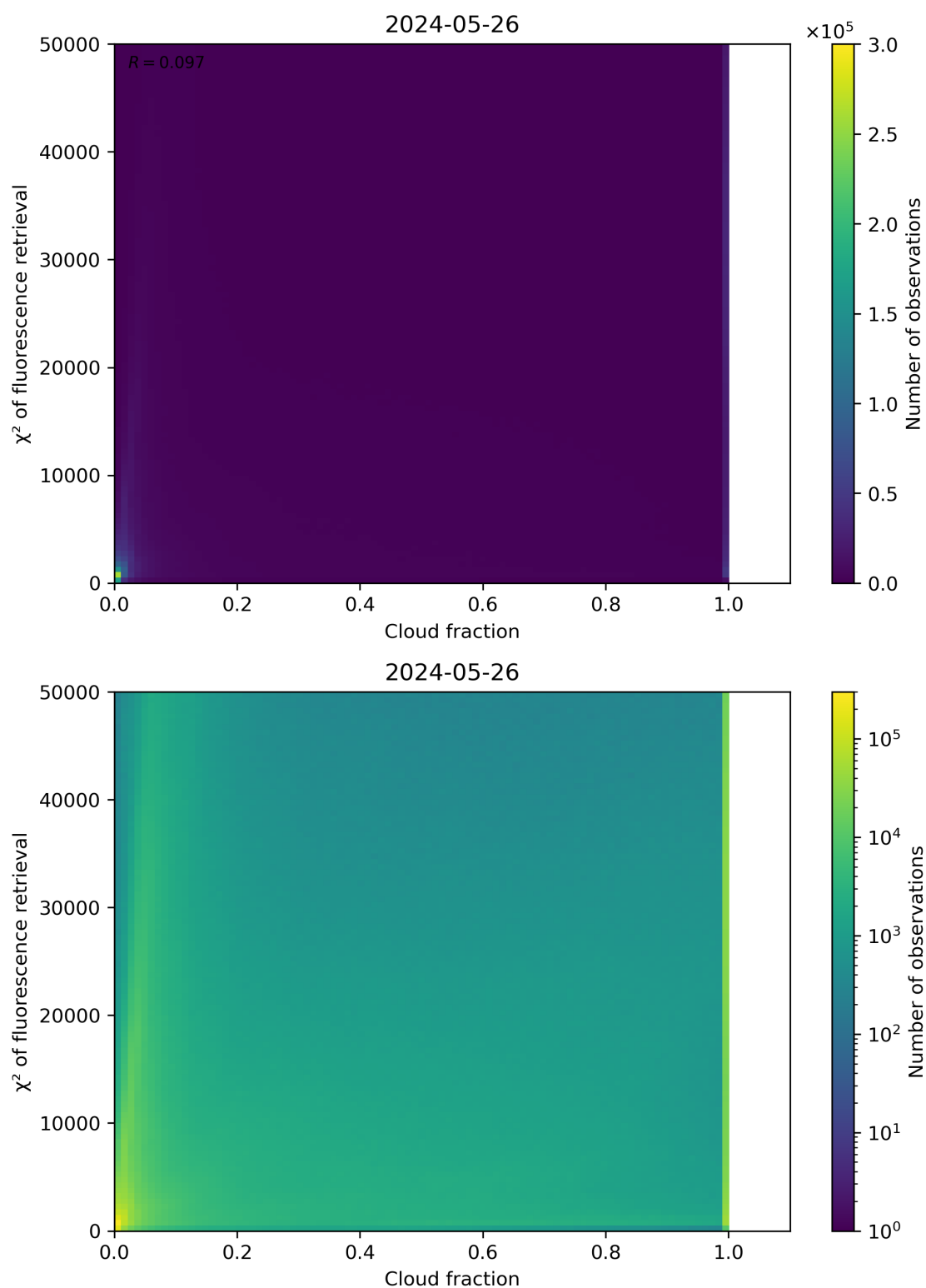
Figure 71: Scatter density plot of “Cloud fraction” against “ \chi^2 of fluorescence retrieval” for 2024-05-25 to 2024-05-27.
