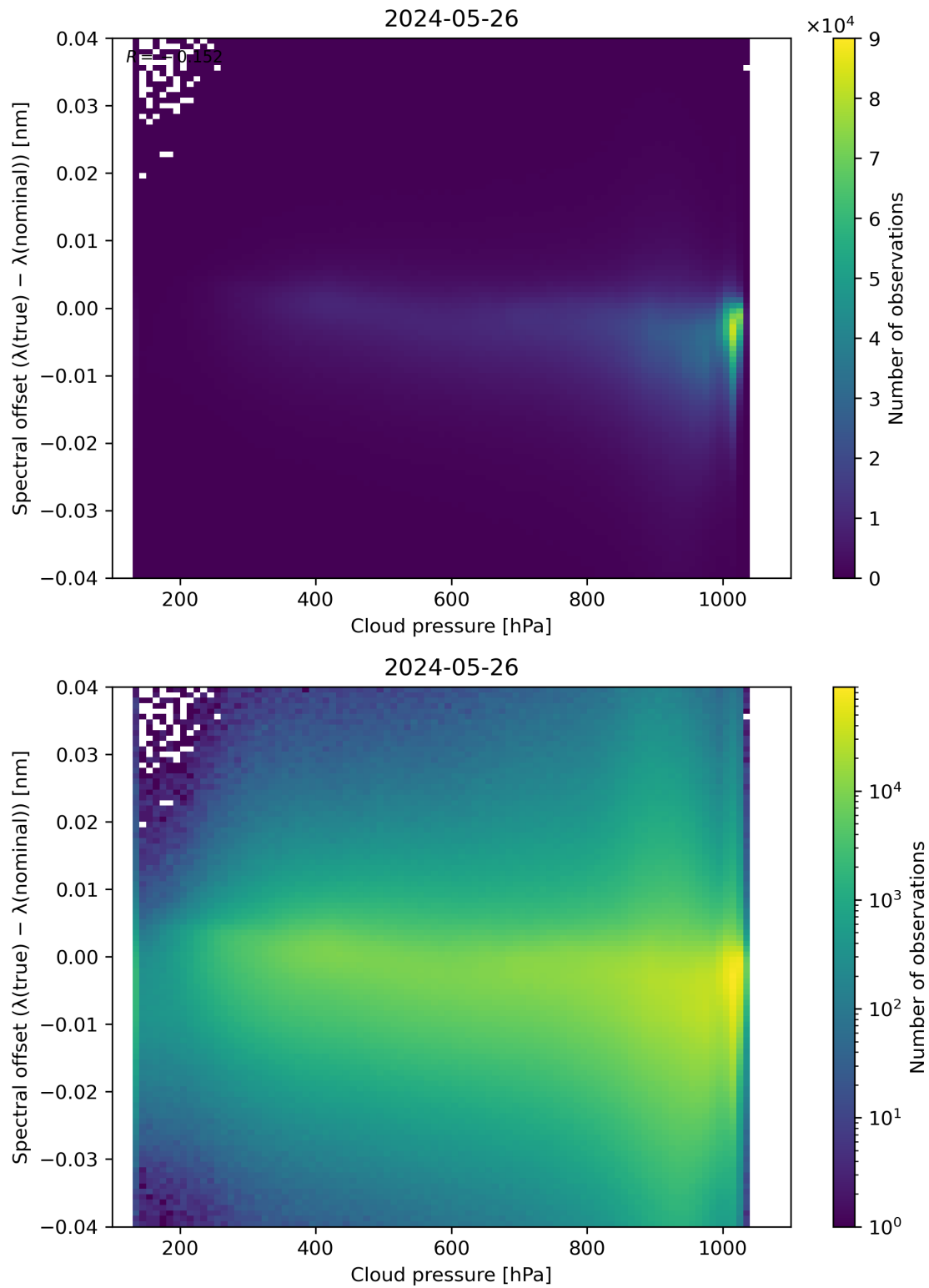
Figure 84: Scatter density plot of “Cloud pressure” against “Spectral offset ( \lambda(\text{true}) - \lambda(\text{nominal}) )” for 2024-05-25 to 2024-05-27.
