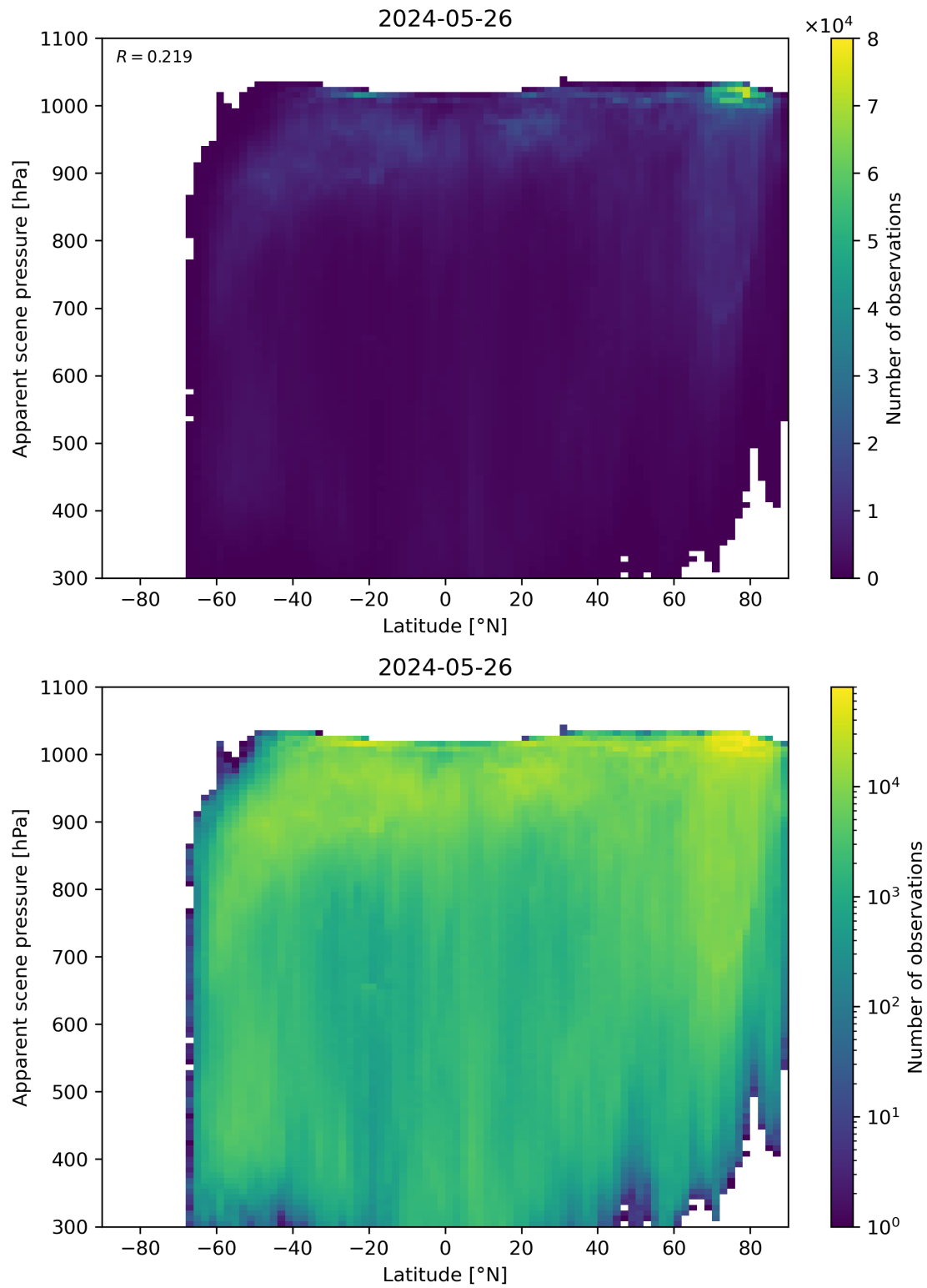
Figure 88: Scatter density plot of “Latitude” against “Apparent scene pressure” for 2024-05-25 to 2024-05-27.
