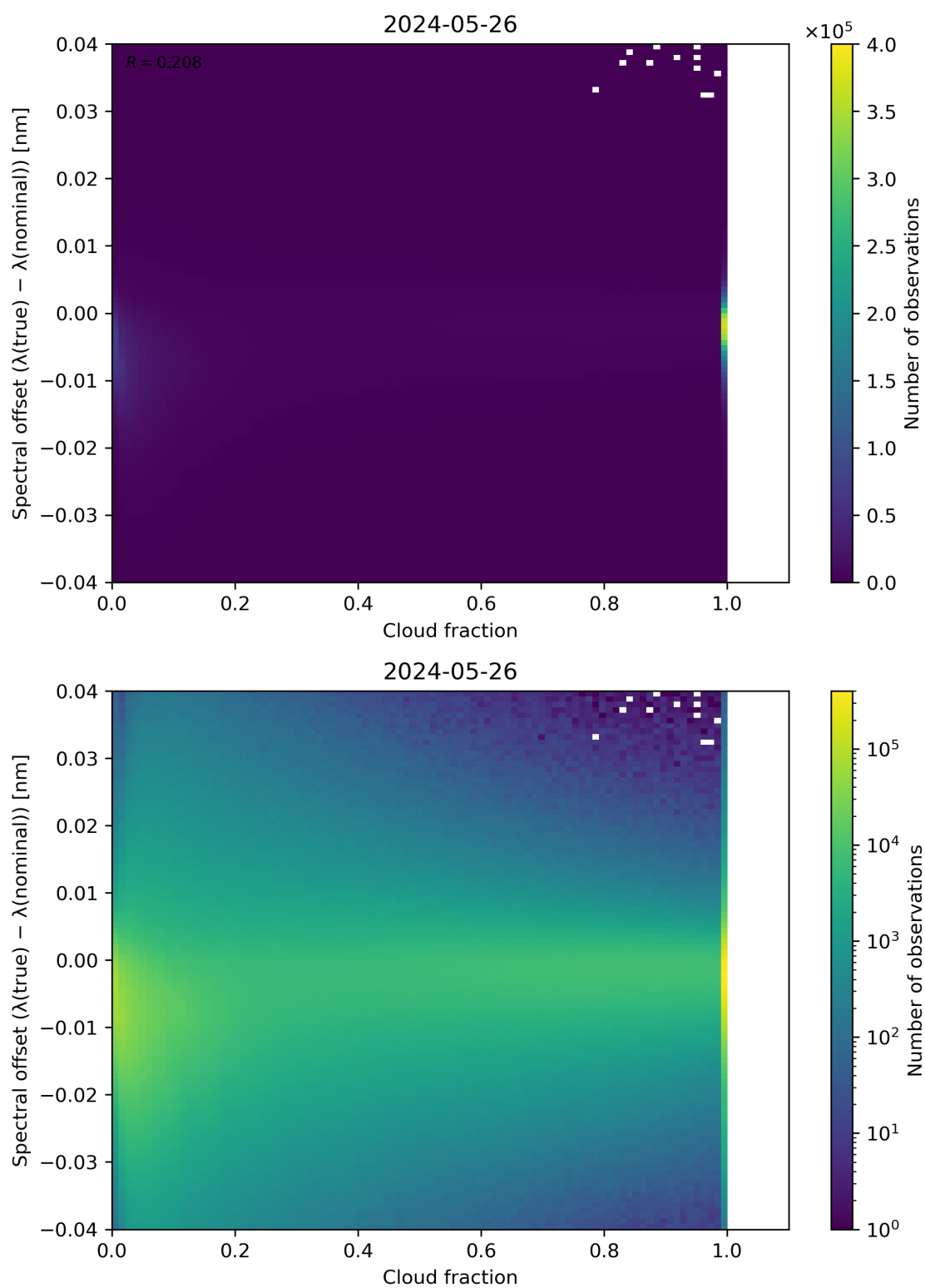
Figure 76: Scatter density plot of “Cloud fraction” against “Spectral offset ( \lambda(\text{true}) - \lambda(\text{nominal}) )” for 2024-05-25 to 2024-05-27.
