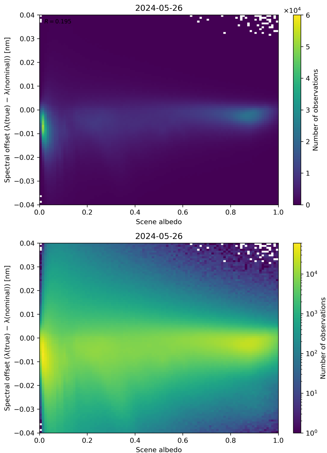
Figure 107: Scatter density plot of “Scene albedo” against “Spectral offset ( \lambda(\text{true}) - \lambda(\text{nominal}) )” for 2024-05-25 to 2024-05-27.
