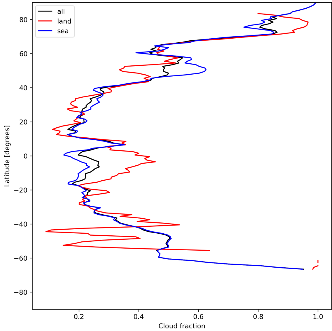
Figure 15: Zonal average of “Cloud fraction” for 2024-05-25 to 2024-05-27.
