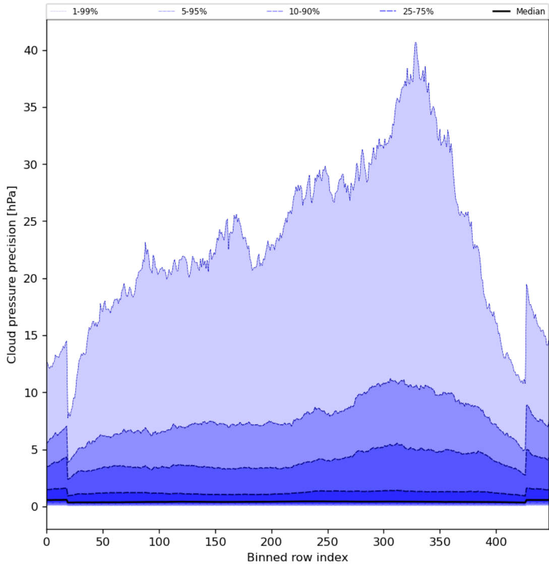
Figure 48: Along track statistics of “Cloud pressure precision” for 2024-05-25 to 2024-05-27
