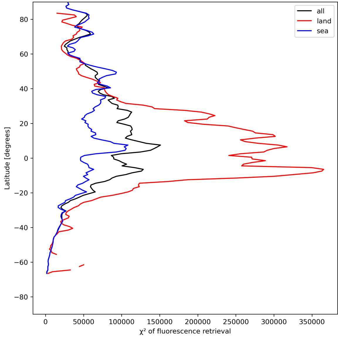
Figure 25: Zonal average of “ \chi^2 of fluorescence retrieval” for 2024-05-25 to 2024-05-27.
