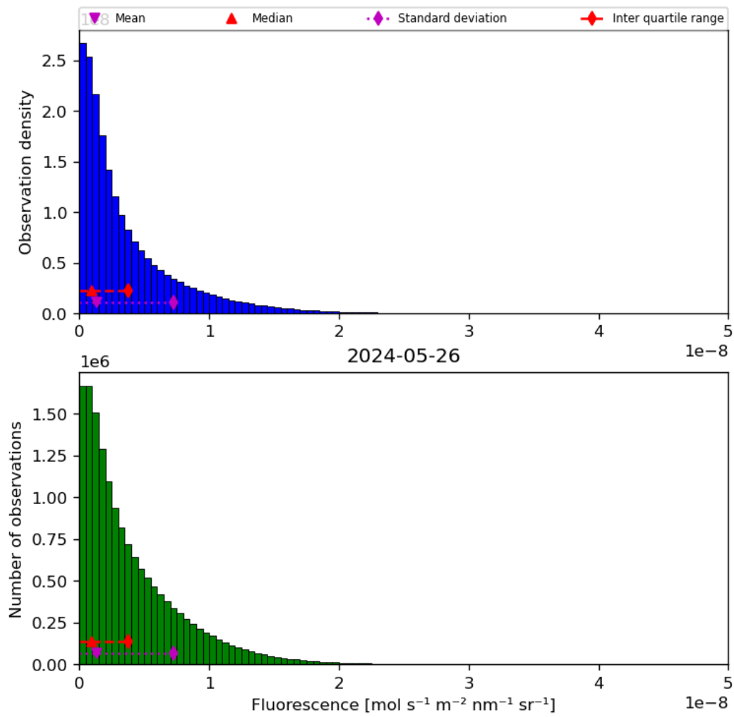
Figure 40: Histogram of “Fluorescence” for 2024-05-25 to 2024-05-27
