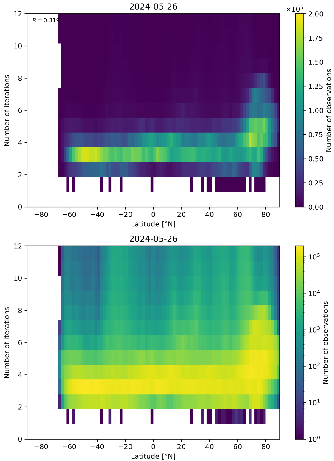
Figure 93: Scatter density plot of “Latitude” against “Number of iterations” for 2024-05-25 to 2024-05-27.
