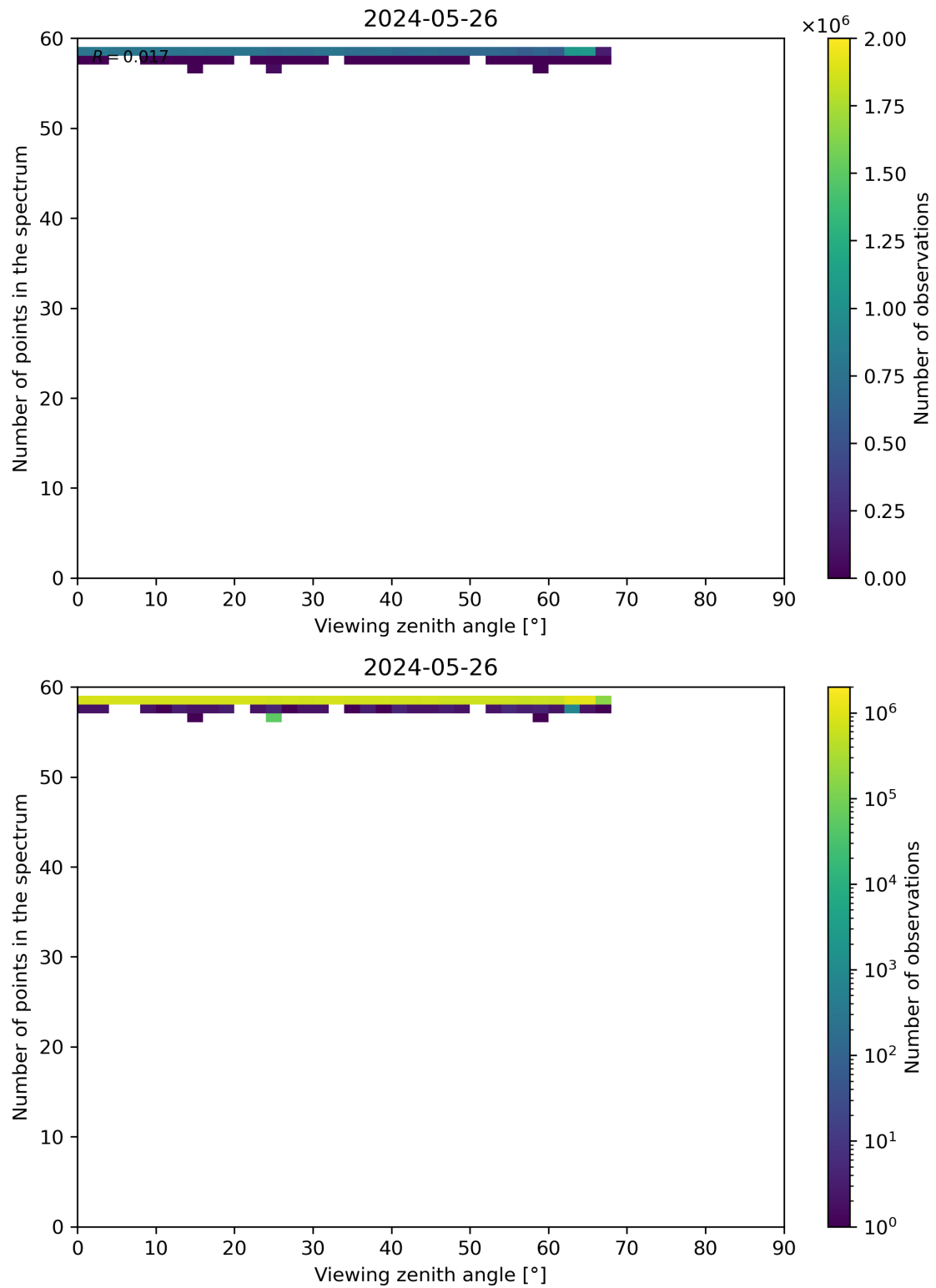
Figure 125: Scatter density plot of “Viewing zenith angle” against “Number of points in the spectrum” for 2024-05-25 to 2024-05-27.
