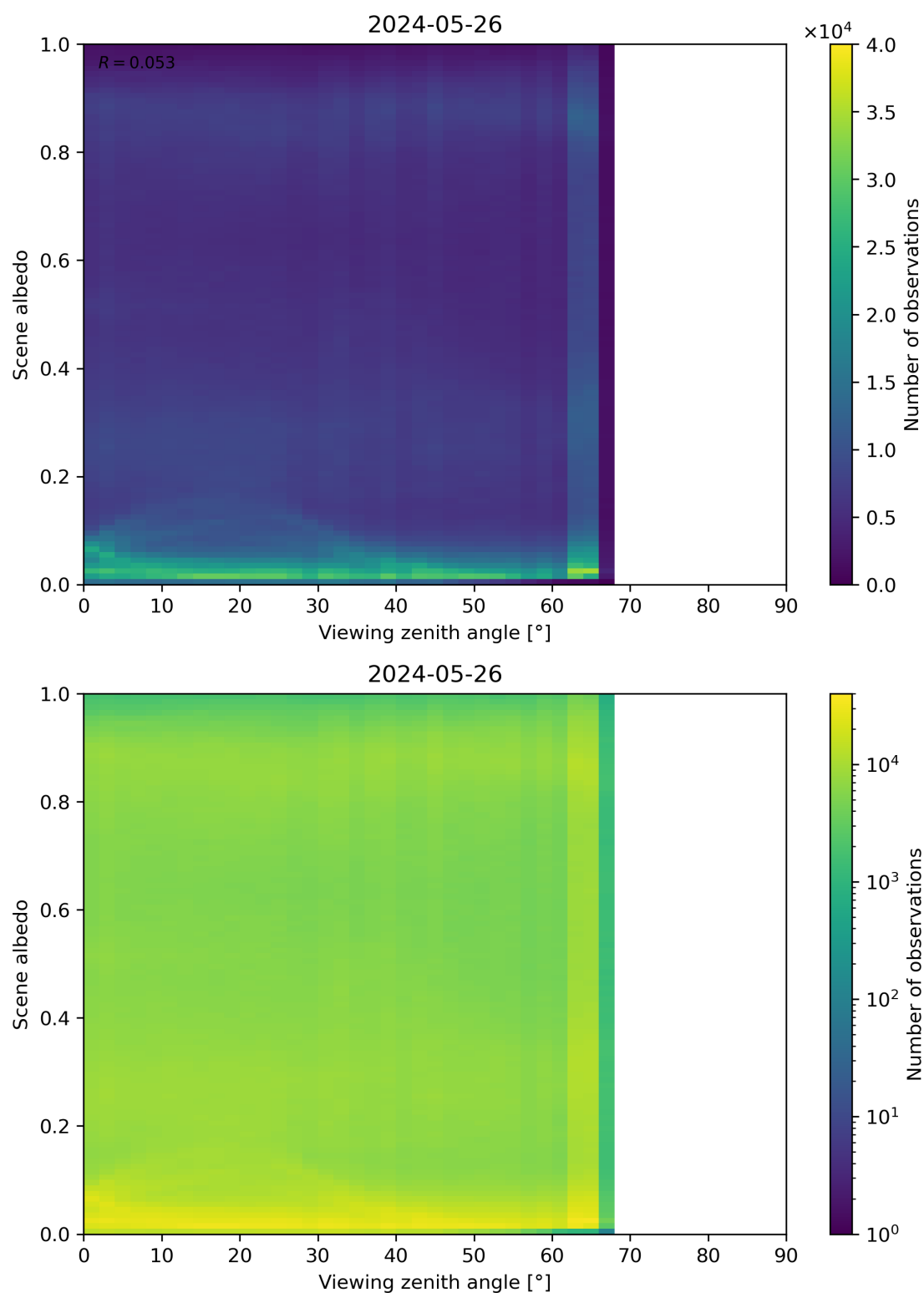
Figure 126: Scatter density plot of “Viewing zenith angle” against “Scene albedo” for 2024-05-25 to 2024-05-27.
