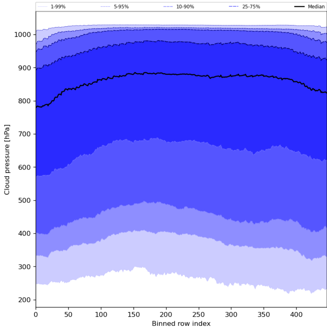
Figure 47: Along track statistics of “Cloud pressure” for 2024-05-25 to 2024-05-27
