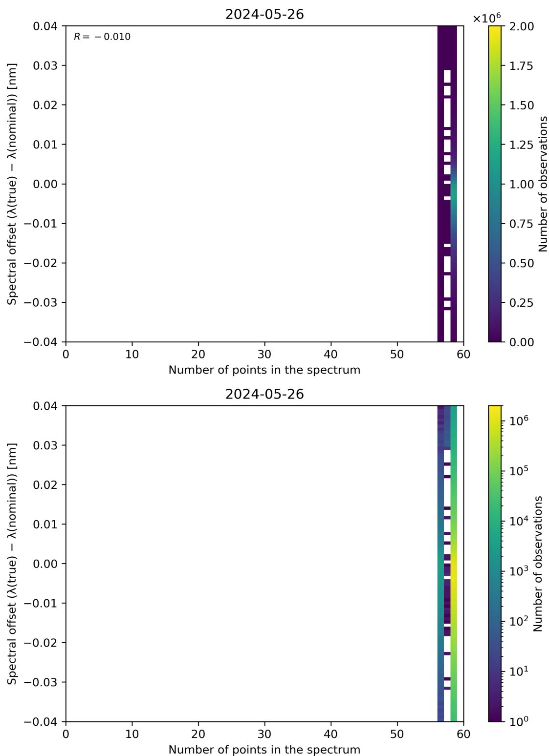
Figure 101: Scatter density plot of “Number of points in the spectrum” against “Spectral offset ( \lambda(\text{true}) - \lambda(\text{nominal}) )” for 2024-05-25 to 2024-05-27.
