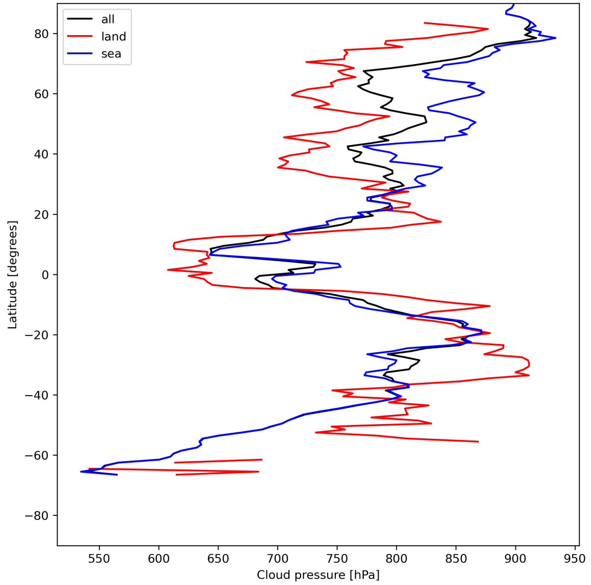
Figure 13: Zonal average of “Cloud pressure” for 2024-05-25 to 2024-05-27.
