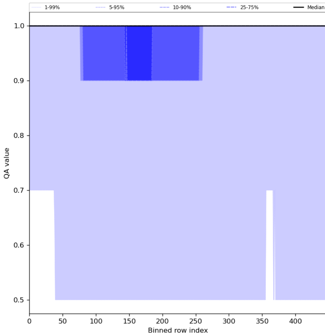
Figure 46: Along track statistics of “QA value” for 2024-05-25 to 2024-05-27
