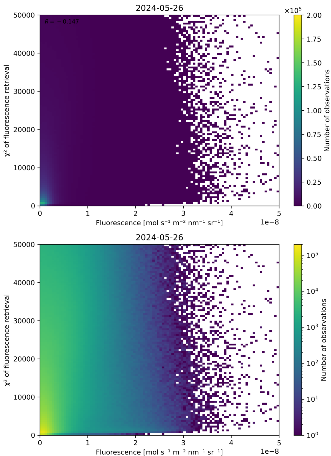
Figure 85: Scatter density plot of “Fluorescence” against “ \chi^2 of fluorescence retrieval” for 2024-05-25 to 2024-05-27.
