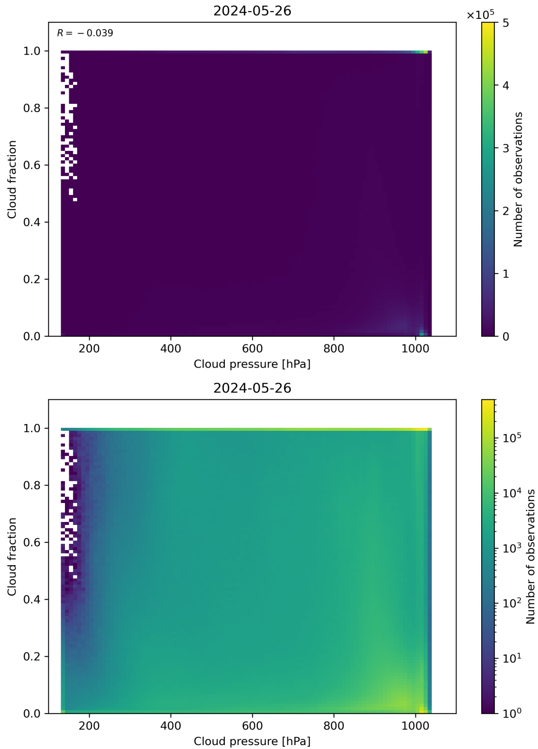
Figure 79: Scatter density plot of “Cloud pressure” against “Cloud fraction” for 2024-05-25 to 2024-05-27.
