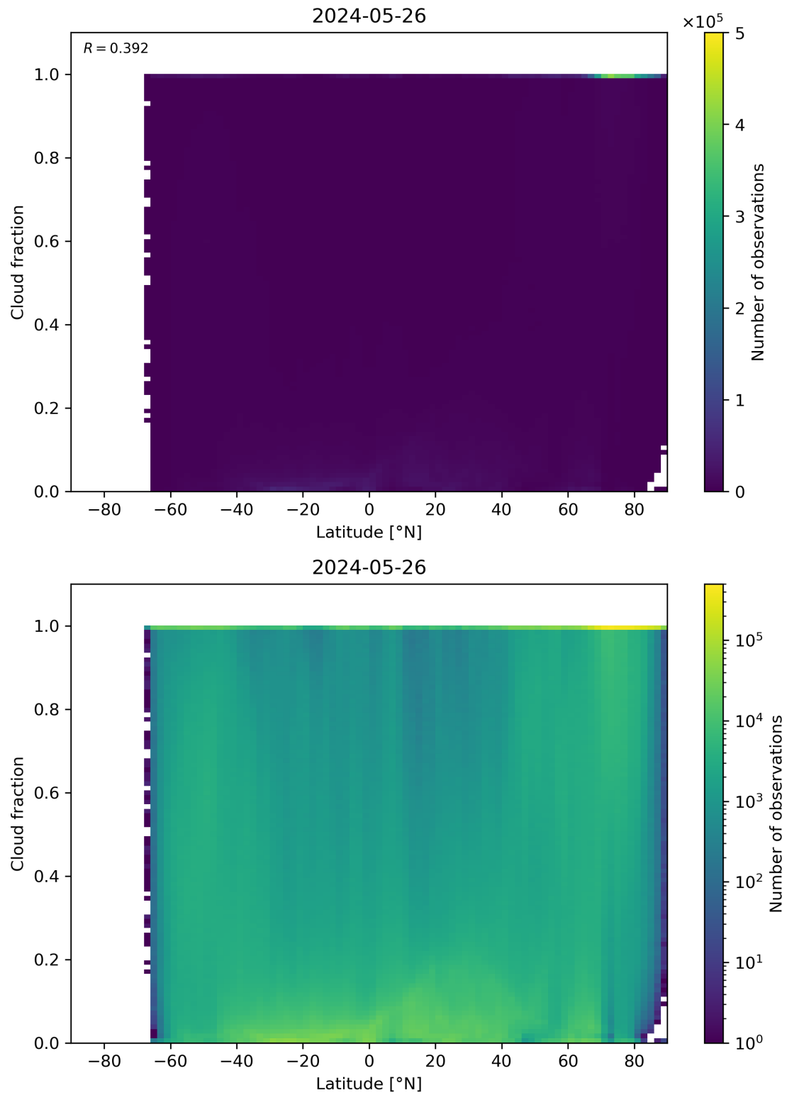
Figure 90: Scatter density plot of “Latitude” against “Cloud fraction” for 2024-05-25 to 2024-05-27.
