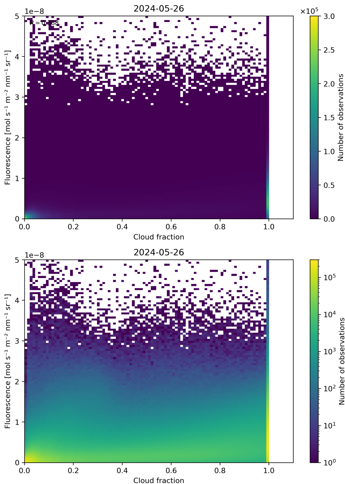
Figure 72: Scatter density plot of “Cloud fraction” against “Fluorescence” for 2024-05-25 to 2024-05-27.
