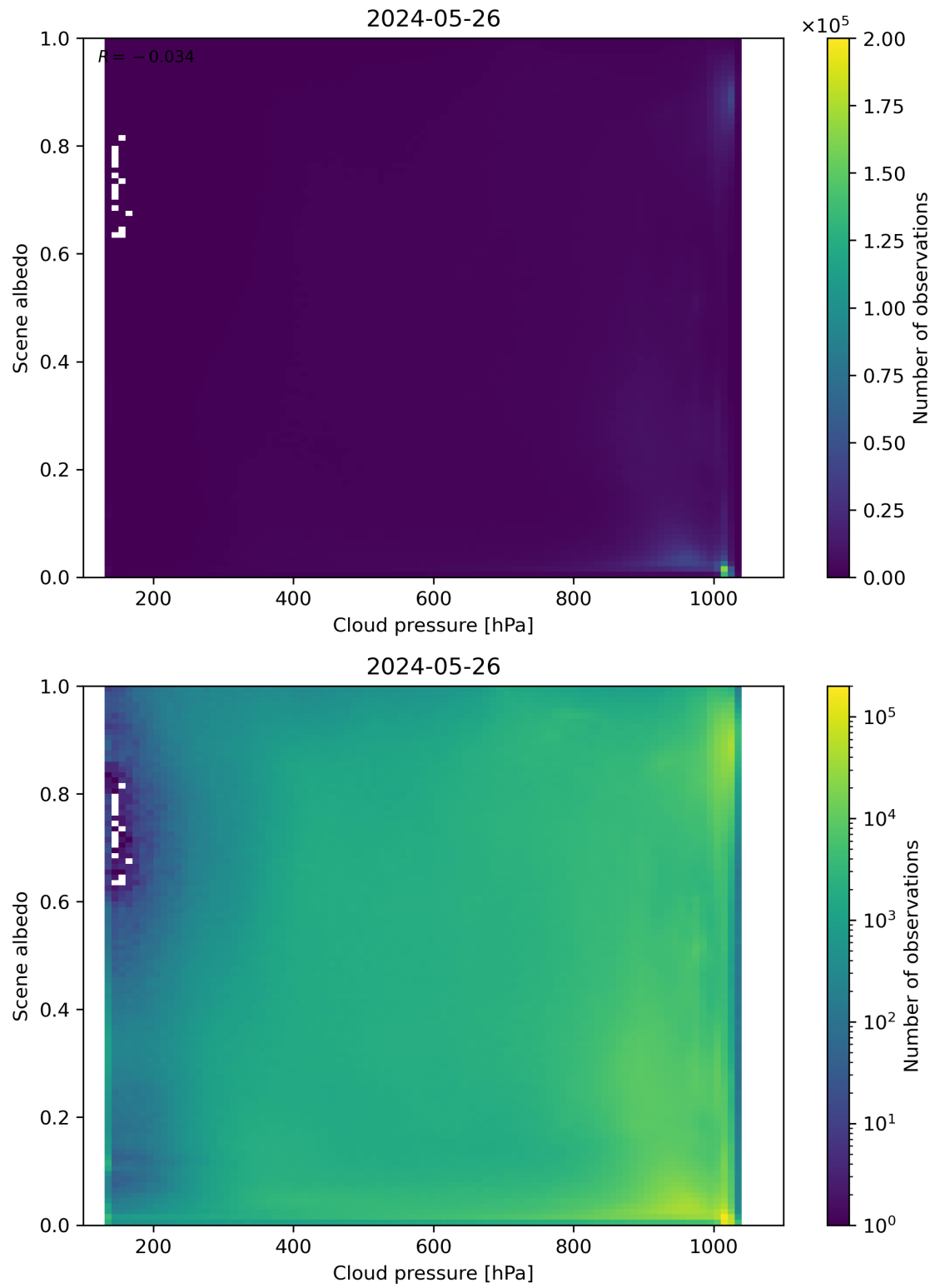
Figure 83: Scatter density plot of “Cloud pressure” against “Scene albedo” for 2024-05-25 to 2024-05-27.
