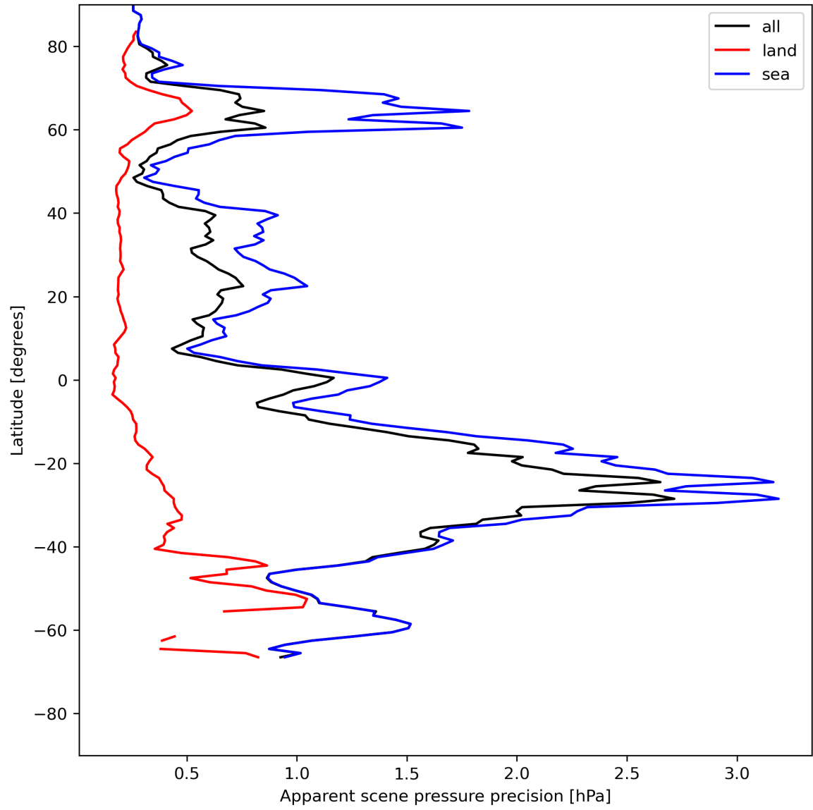
Figure 20: Zonal average of “Apparent scene pressure precision” for 2024-05-25 to 2024-05-27.
