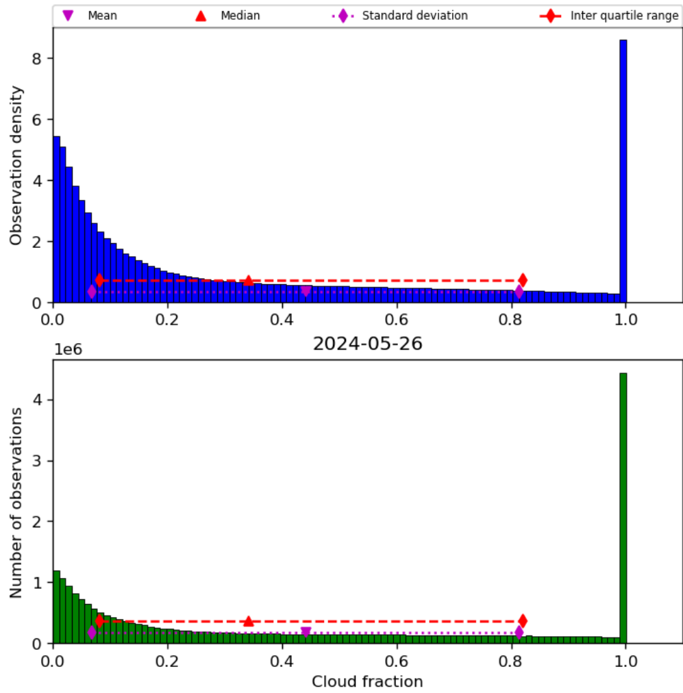
Figure 32: Histogram of “Cloud fraction” for 2024-05-25 to 2024-05-27
