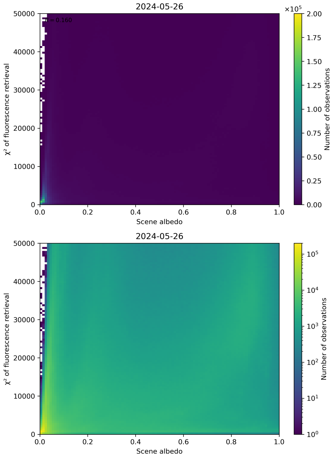
Figure 103: Scatter density plot of “Scene albedo” against “ \chi^2 of fluorescence retrieval” for 2024-05-25 to 2024-05-27.
