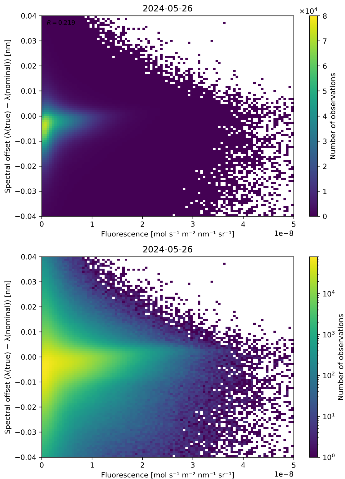
Figure 87: Scatter density plot of “Fluorescence” against “Spectral offset ( \lambda(\text{true}) - \lambda(\text{nominal}) )” for 2024-05-25 to 2024-05-27.
