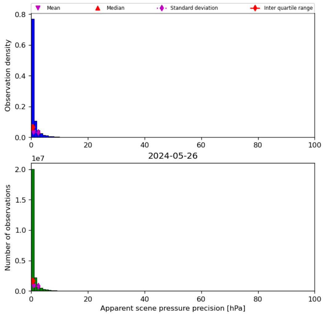
Figure 37: Histogram of “Apparent scene pressure precision” for 2024-05-25 to 2024-05-27
