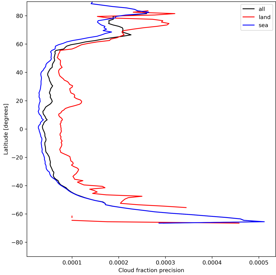
Figure 16: Zonal average of “Cloud fraction precision” for 2024-05-25 to 2024-05-27.
