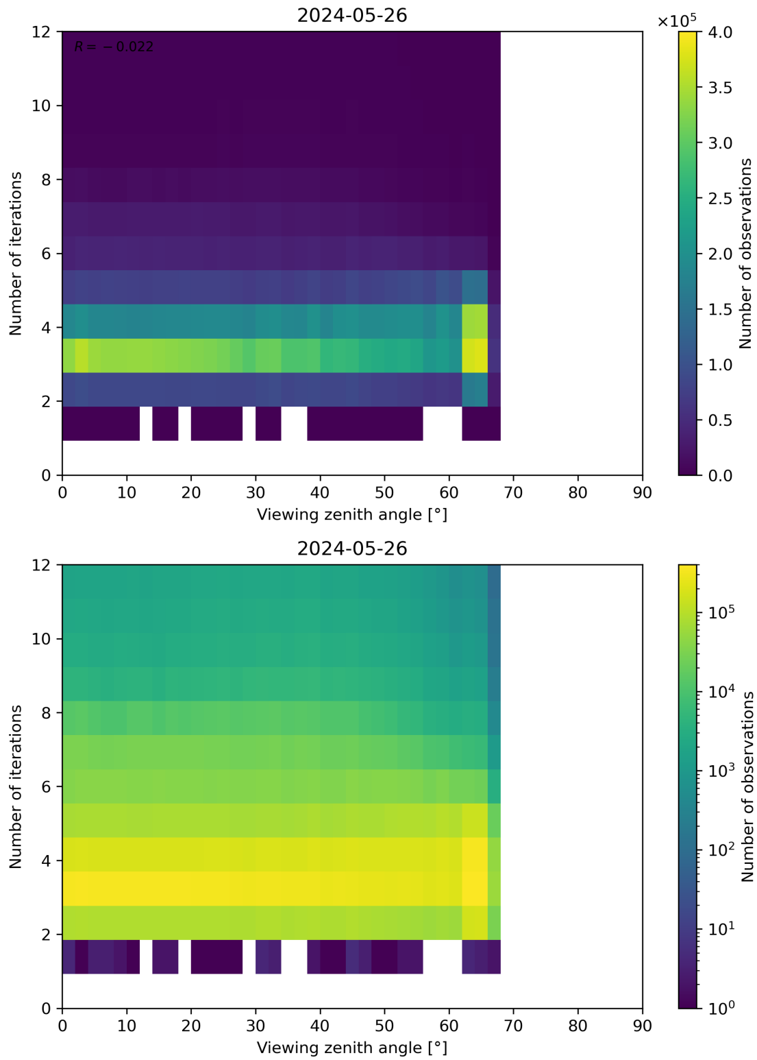
Figure 124: Scatter density plot of “Viewing zenith angle” against “Number of iterations” for 2024-05-25 to 2024-05-27.
