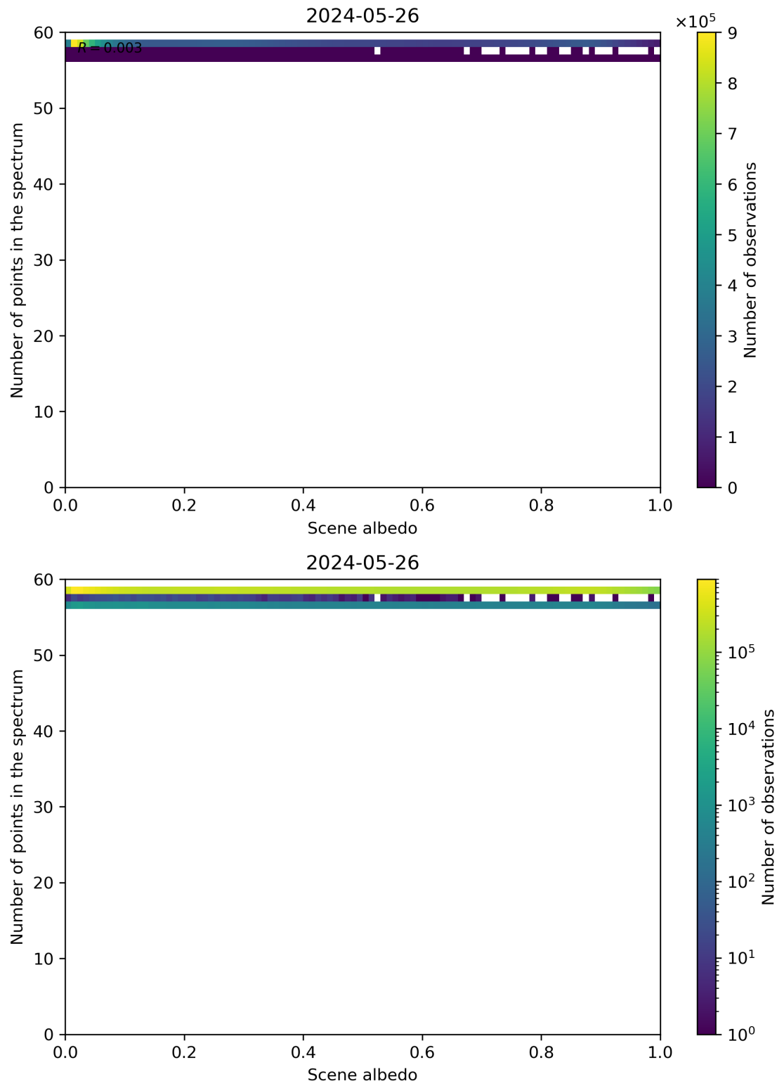
Figure 106: Scatter density plot of “Scene albedo” against “Number of points in the spectrum” for 2024-05-25 to 2024-05-27.
