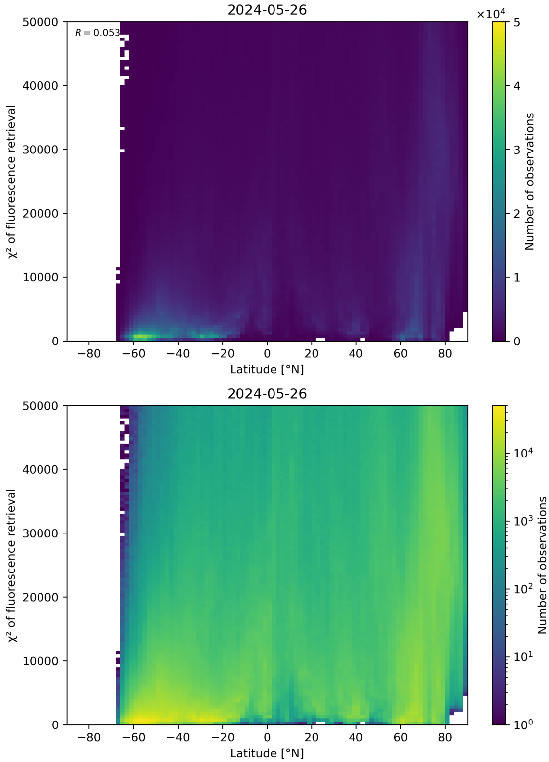
Figure 89: Scatter density plot of “Latitude” against “ \chi^2 of fluorescence retrieval” for 2024-05-25 to 2024-05-27.
