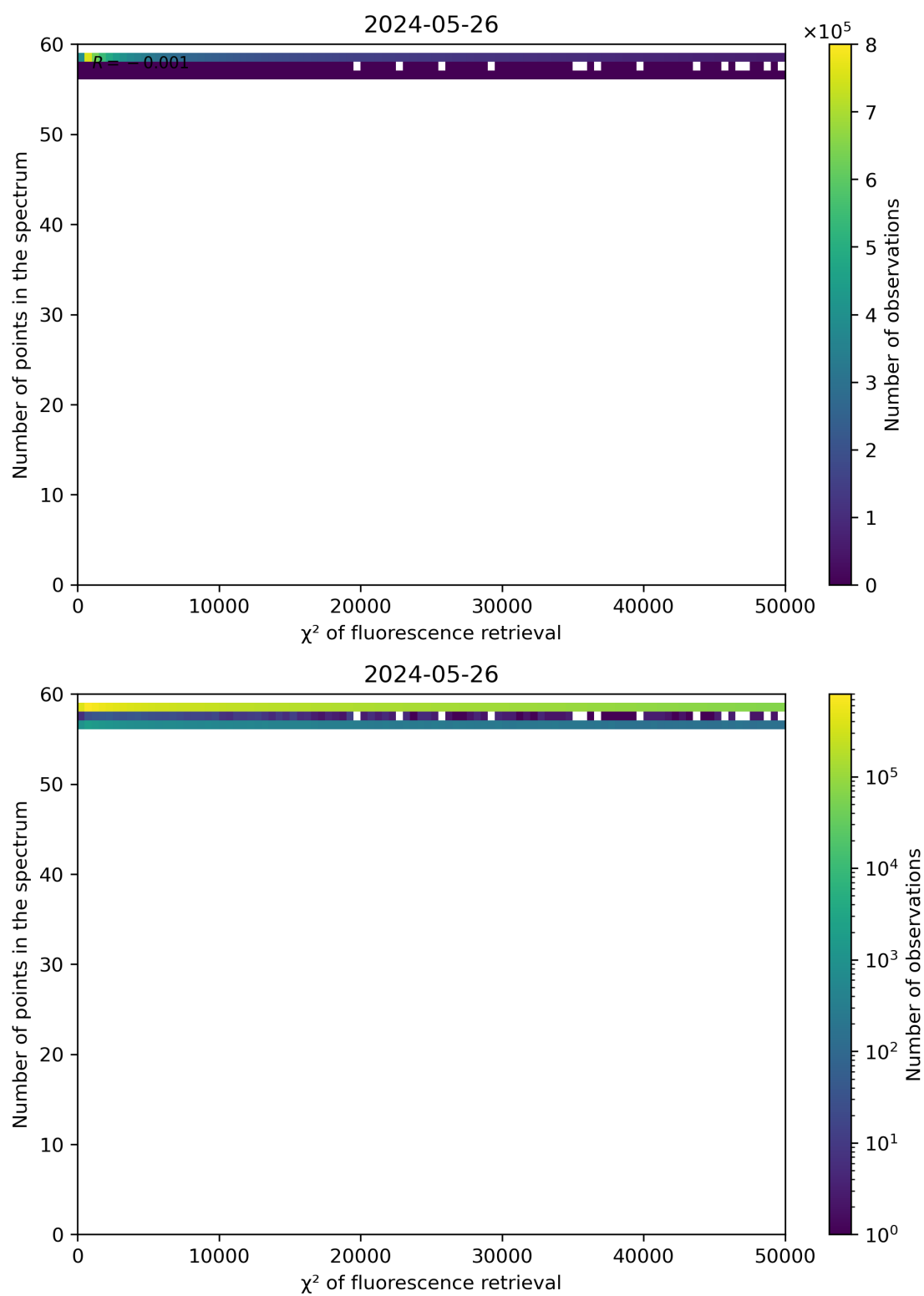
Figure 68: Scatter density plot of " \chi^2 of fluorescence retrieval" against "Number of points in the spectrum" for 2024-05-25 to 2024-05-27.
