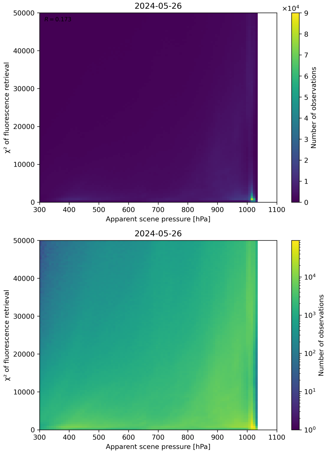
Figure 63: Scatter density plot of “Apparent scene pressure” against “ \chi^2 of fluorescence retrieval” for 2024-05-25 to 2024-05-27.
