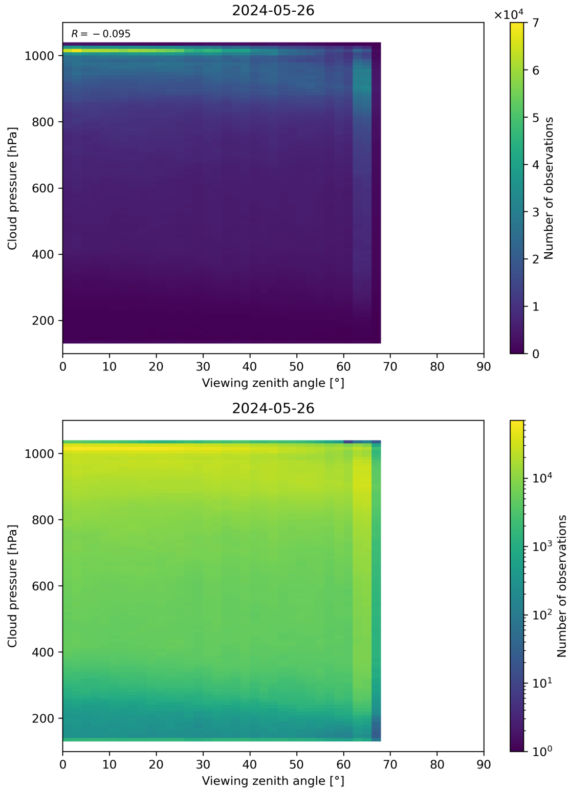
Figure 121: Scatter density plot of “Viewing zenith angle” against “Cloud pressure” for 2024-05-25 to 2024-05-27.
