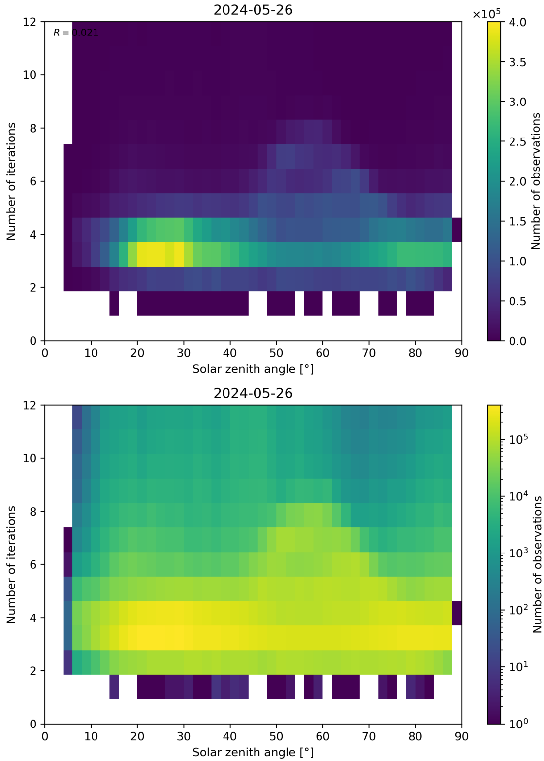
Figure 114: Scatter density plot of “Solar zenith angle” against “Number of iterations” for 2024-05-25 to 2024-05-27.
