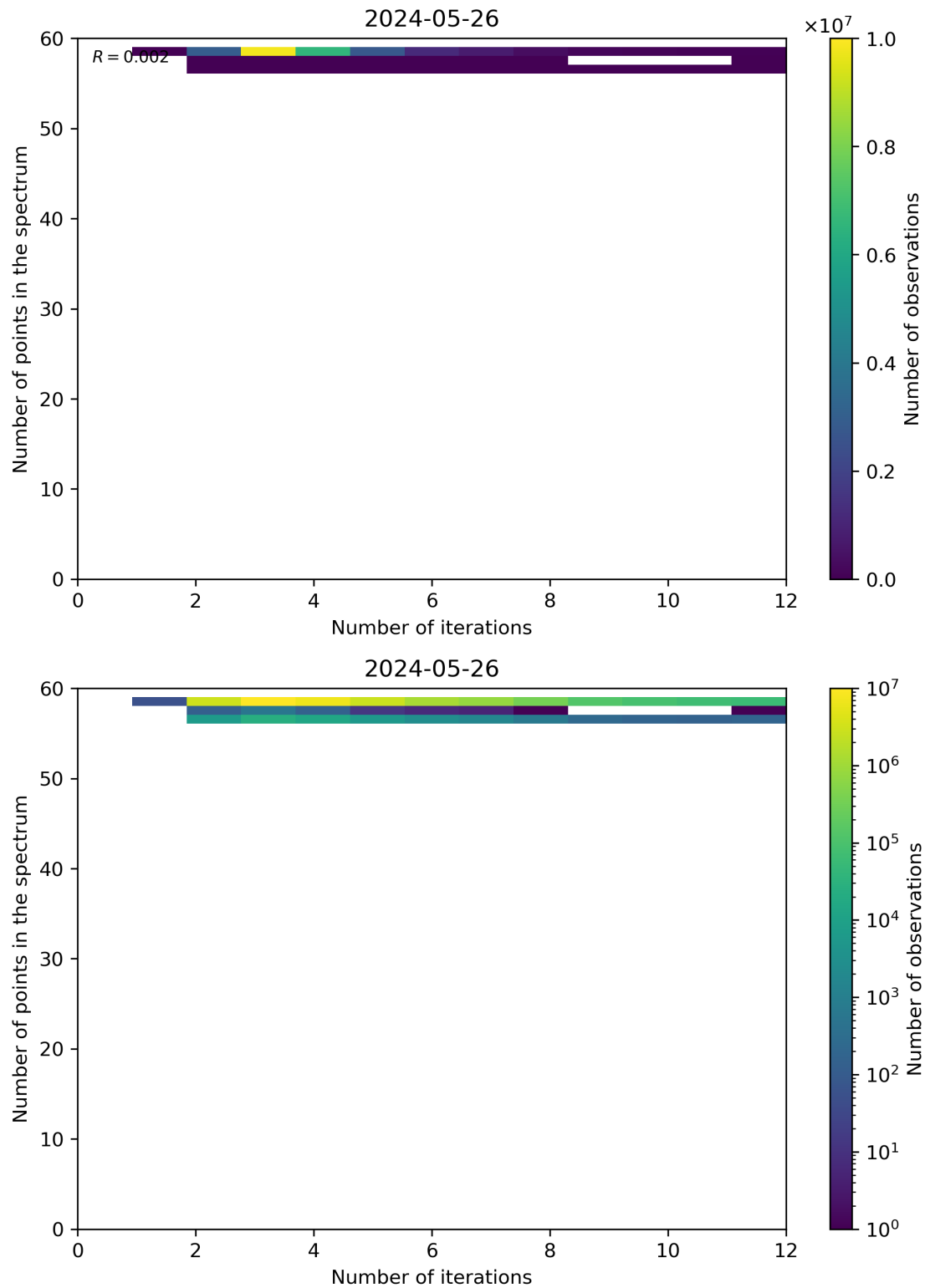
Figure 99: Scatter density plot of “Number of iterations” against “Number of points in the spectrum” for 2024-05-25 to 2024-05-27.
