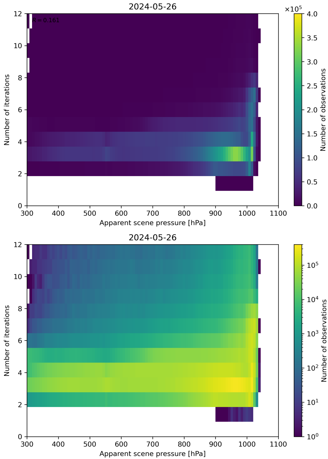
Figure 65: Scatter density plot of “Apparent scene pressure” against “Number of iterations” for 2024-05-25 to 2024-05-27.
