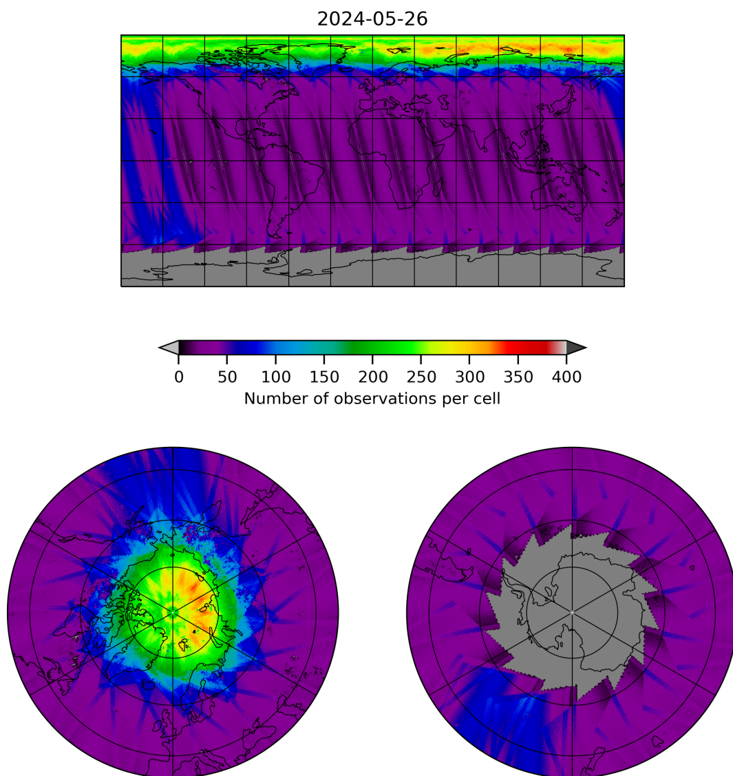
Figure 11: Map of the number of observations for 2024-05-25 to 2024-05-27
