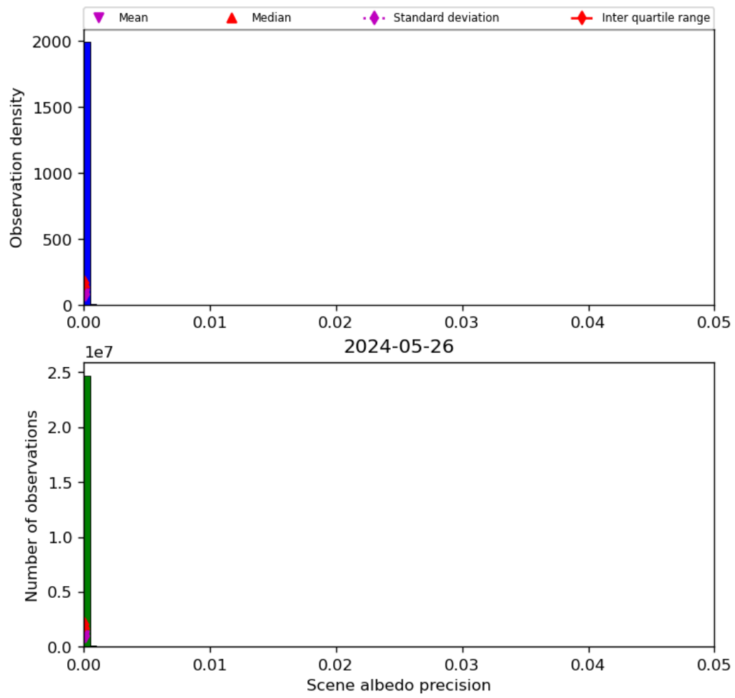
Figure 35: Histogram of “Scene albedo precision” for 2024-05-25 to 2024-05-27
