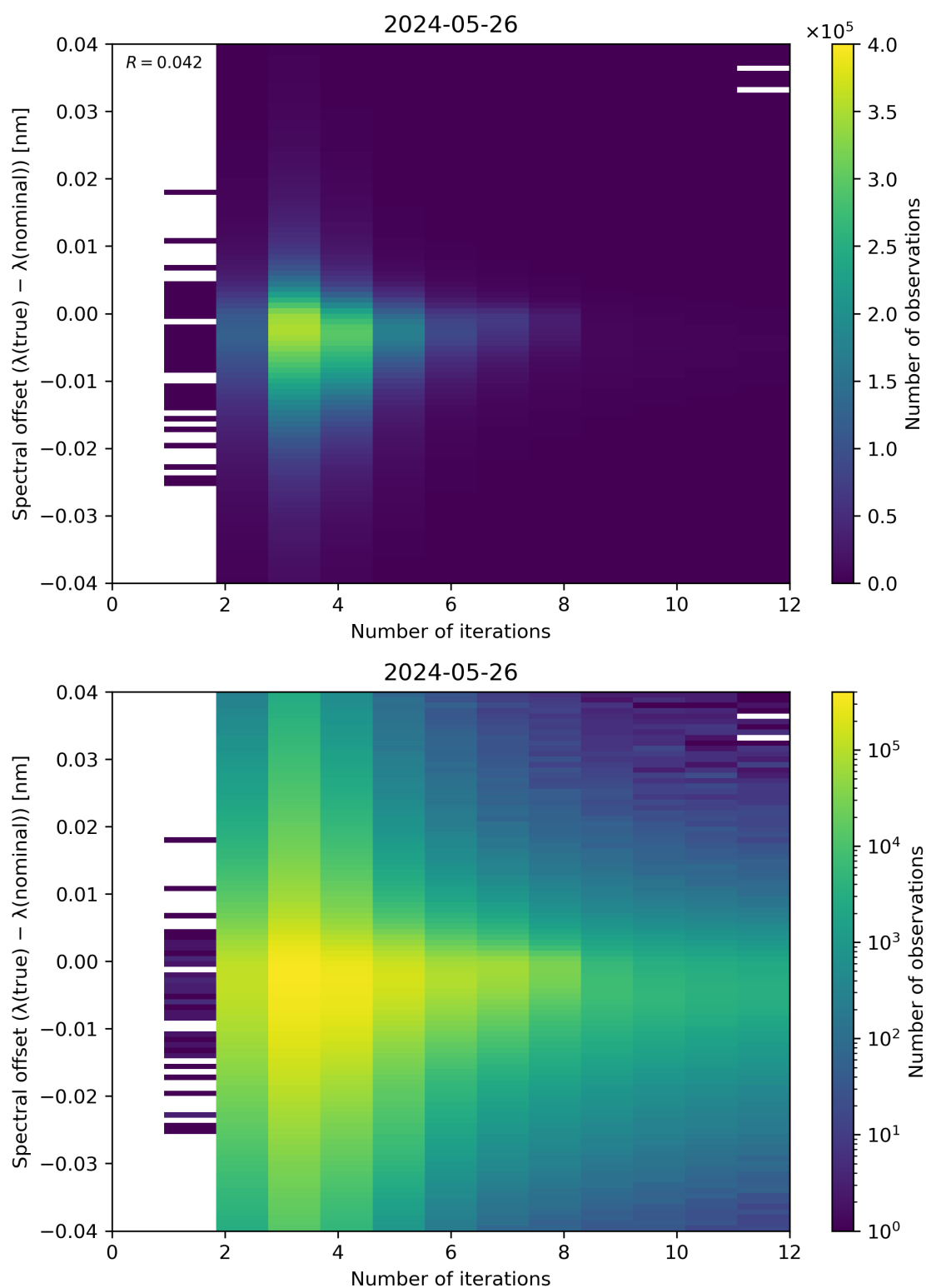
Figure 100: Scatter density plot of “Number of iterations” against “Spectral offset ( \lambda(\text{true}) - \lambda(\text{nominal}) )” for 2024-05-25 to 2024-05-27.
