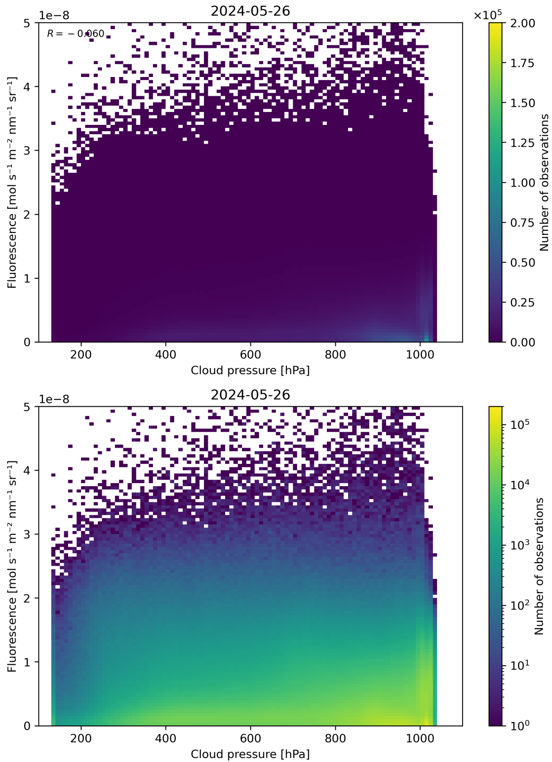
Figure 80: Scatter density plot of “Cloud pressure” against “Fluorescence” for 2024-05-25 to 2024-05-27.
