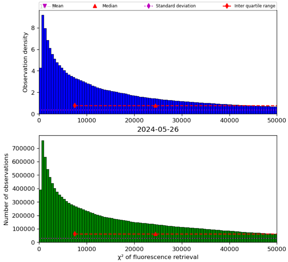
Figure 42: Histogram of “ \chi^2 of fluorescence retrieval” for 2024-05-25 to 2024-05-27
