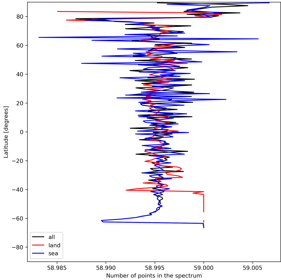
Figure 27: Zonal average of “Number of points in the spectrum” for 2024-05-25 to 2024-05-27.
