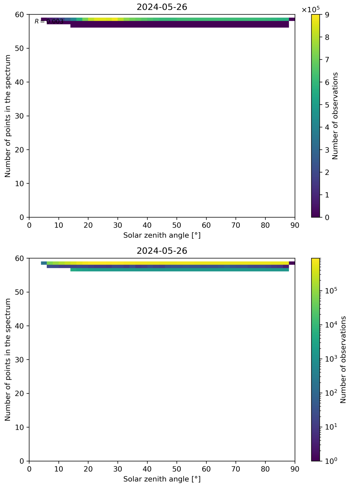
Figure 115: Scatter density plot of “Solar zenith angle” against “Number of points in the spectrum” for 2024-05-25 to 2024-05-27.
