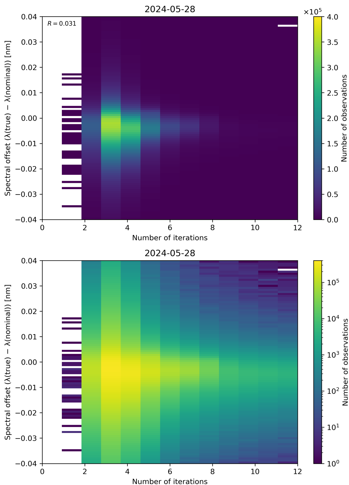
Figure 100: Scatter density plot of “Number of iterations” against “Spectral offset ( \lambda(\text{true}) - \lambda(\text{nominal}) )” for 2024-05-28 to 2024-05-29.
