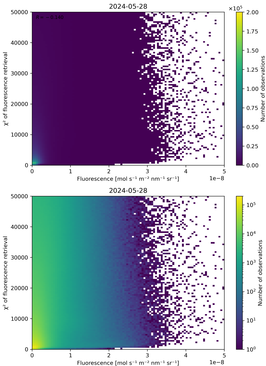
Figure 85: Scatter density plot of “Fluorescence” against “ \chi^2 of fluorescence retrieval” for 2024-05-28 to 2024-05-29.
