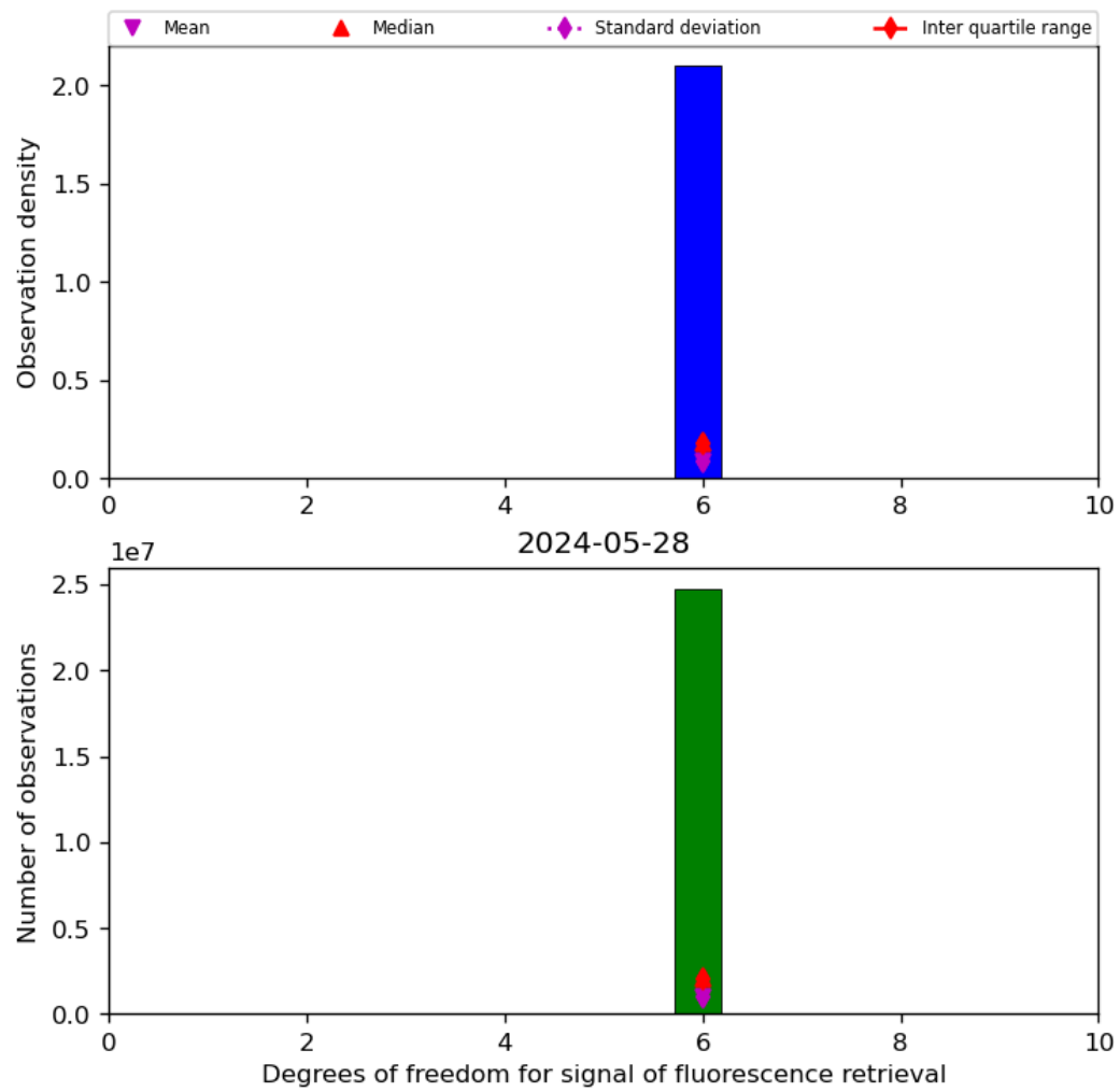
Figure 43: Histogram of “Degrees of freedom for signal of fluorescence retrieval” for 2024-05-28 to 2024-05-29
