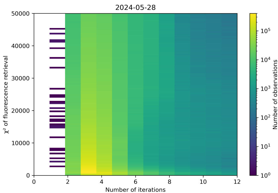
Figure 97: Scatter density plot of “Number of iterations” against “ \chi^2 of fluorescence retrieval” for 2024-05-28 to 2024-05-29.
