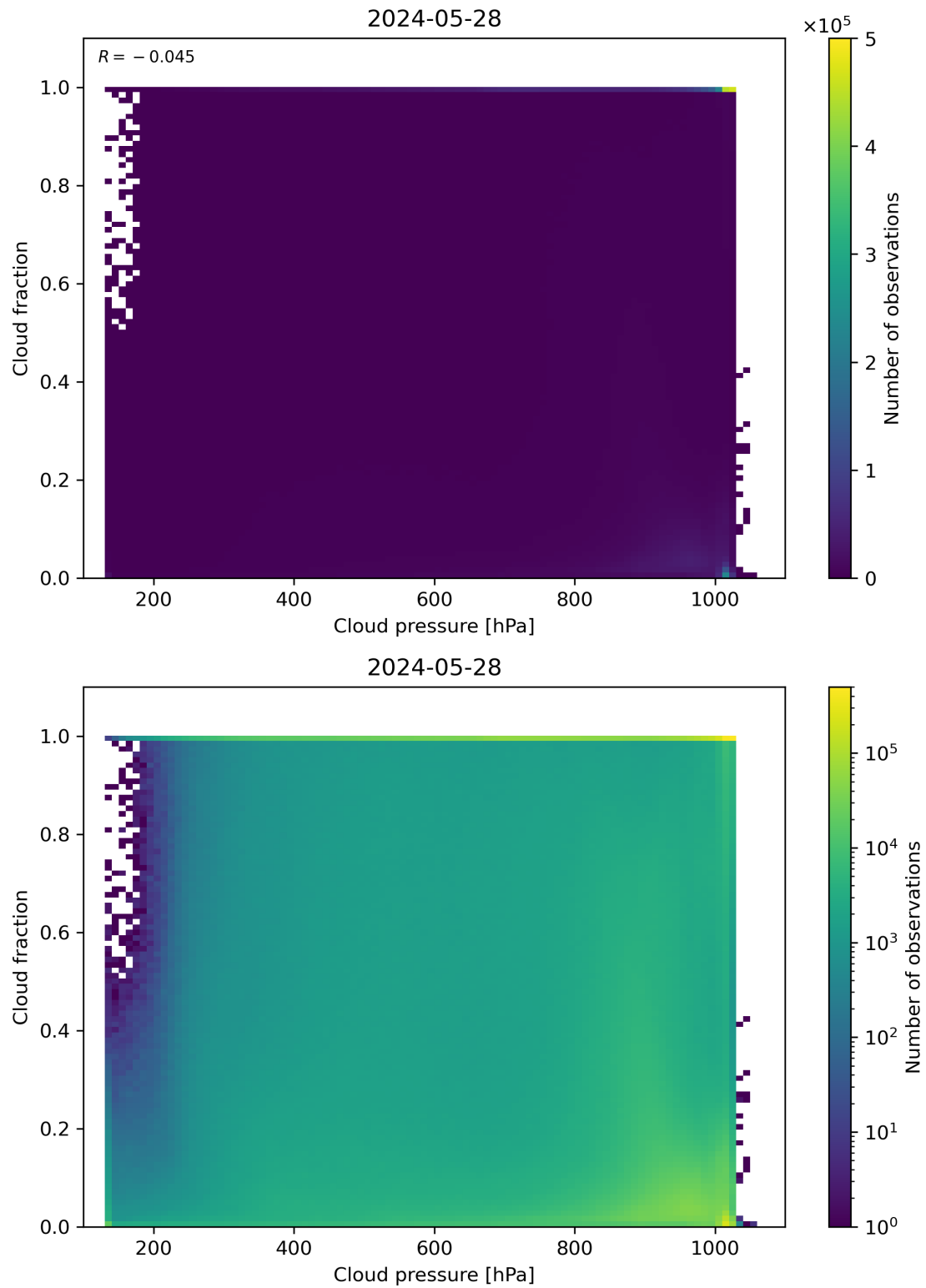
Figure 79: Scatter density plot of “Cloud pressure” against “Cloud fraction” for 2024-05-28 to 2024-05-29.
