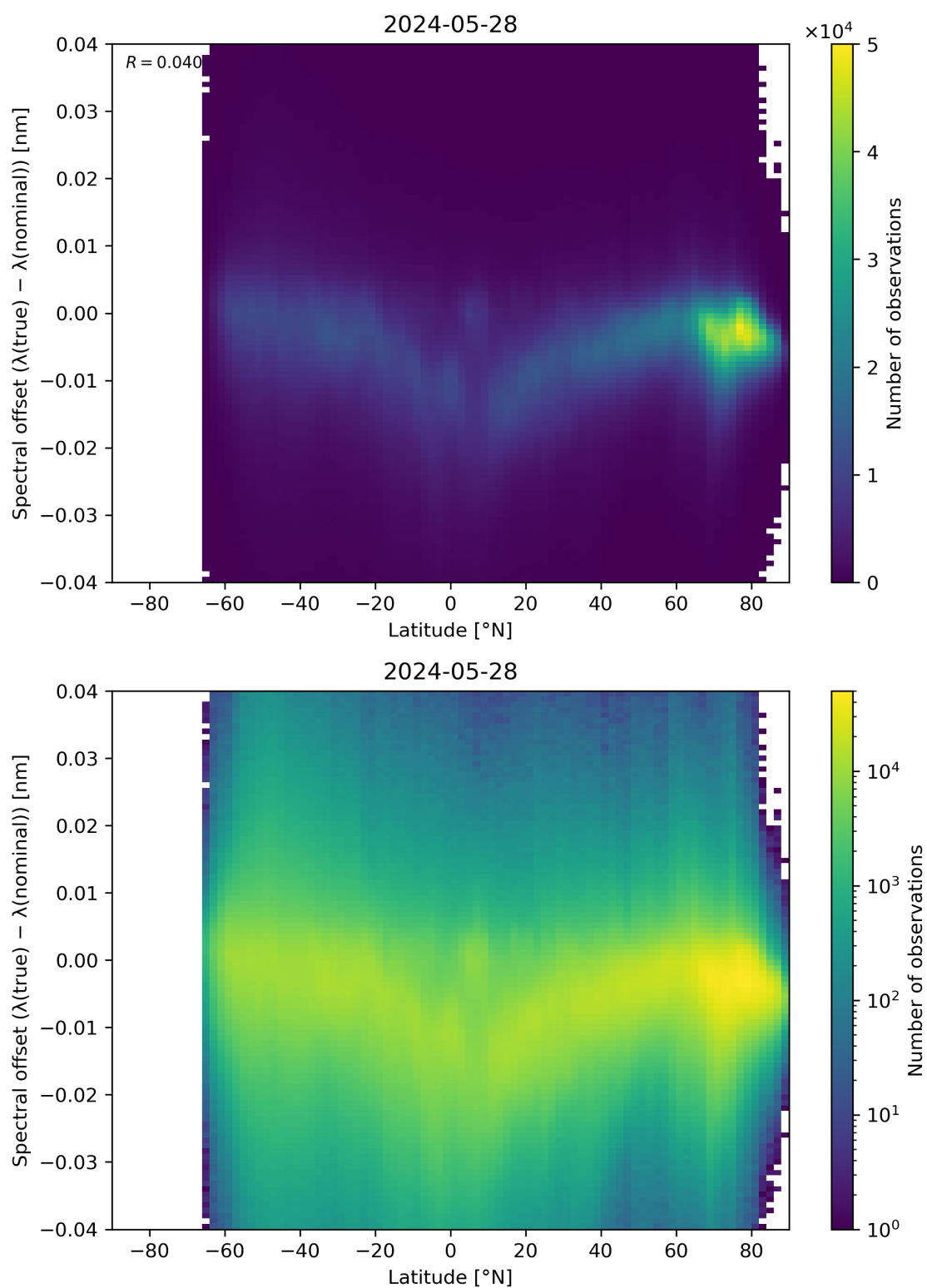
Figure 96: Scatter density plot of “Latitude” against “Spectral offset ( \lambda(\text{true}) - \lambda(\text{nominal}) )” for 2024-05-28 to 2024-05-29.
