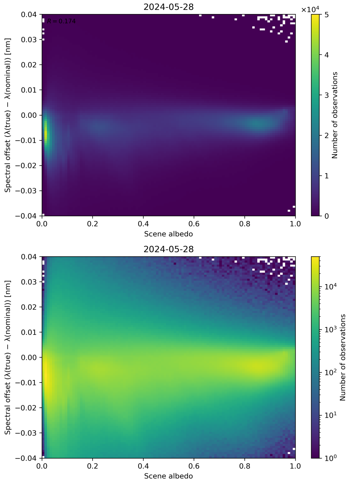
Figure 107: Scatter density plot of “Scene albedo” against “Spectral offset ( \lambda(\text{true}) - \lambda(\text{nominal}) )” for 2024-05-28 to 2024-05-29.
