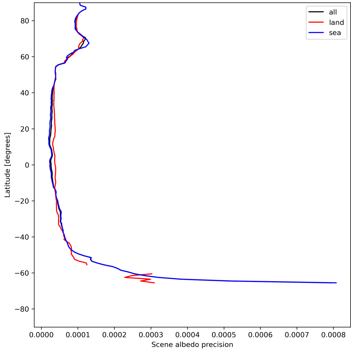
Figure 18: Zonal average of “Scene albedo precision” for 2024-05-28 to 2024-05-29.
