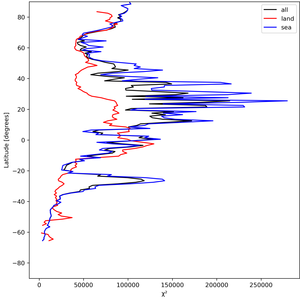
Figure 21: Zonal average of “ \chi^2 ” for 2024-05-28 to 2024-05-29.
