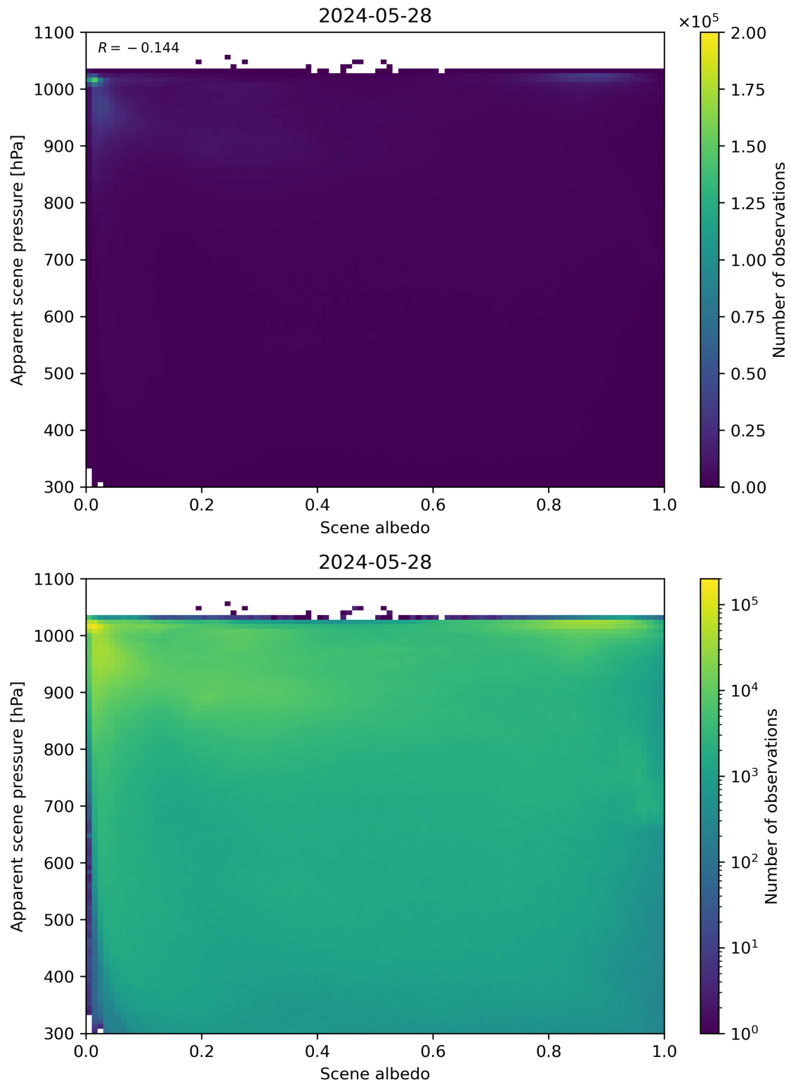
Figure 102: Scatter density plot of “Scene albedo” against “Apparent scene pressure” for 2024-05-28 to 2024-05-29.
