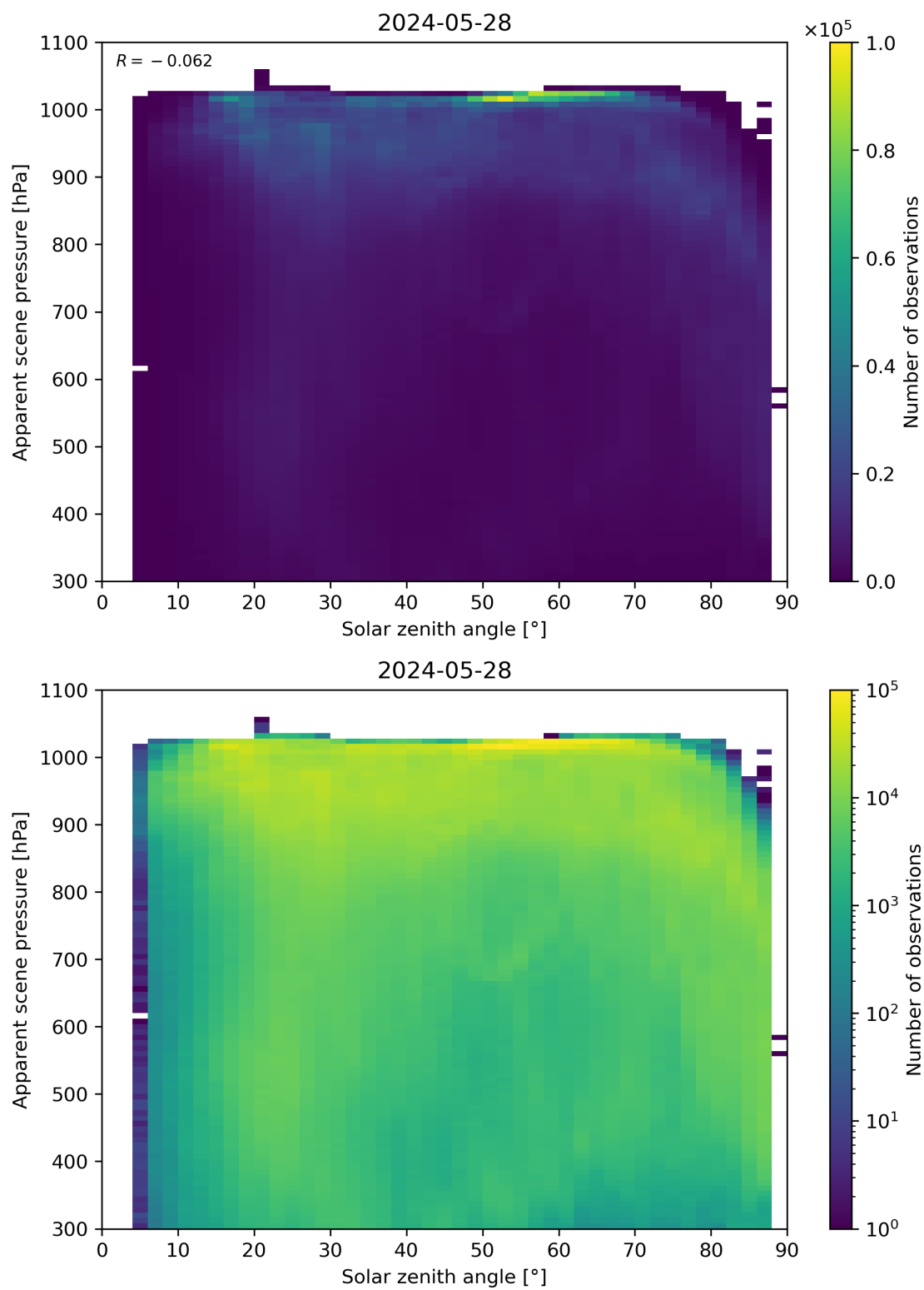
Figure 108: Scatter density plot of “Solar zenith angle” against “Apparent scene pressure” for 2024-05-28 to 2024-05-29.
