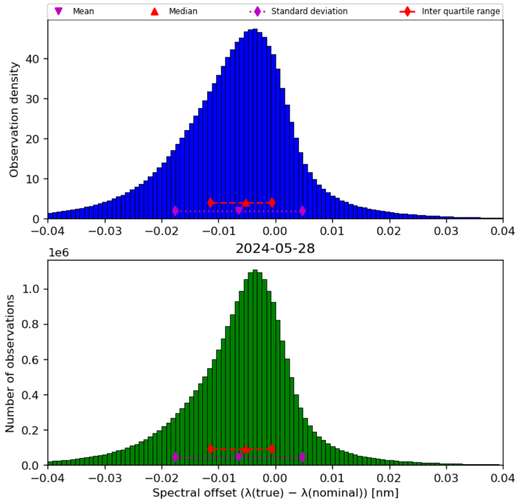
Figure 45: Histogram of “Spectral offset ( \lambda(\text{true}) - \lambda(\text{nominal}) )” for 2024-05-28 to 2024-05-29
