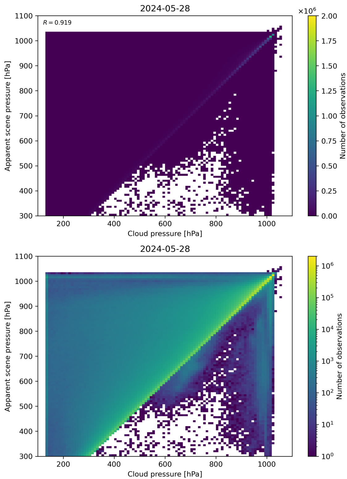
Figure 77: Scatter density plot of “Cloud pressure” against “Apparent scene pressure” for 2024-05-28 to 2024-05-29.
