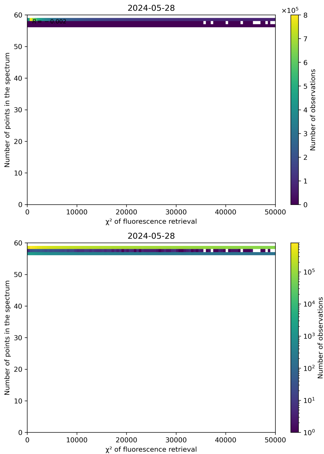
Figure 68: Scatter density plot of " \chi^2 of fluorescence retrieval" against "Number of points in the spectrum" for 2024-05-28 to 2024-05-29.
