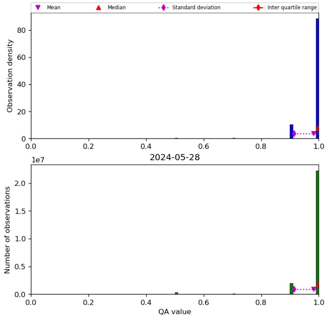
Figure 29: Histogram of “QA value” for 2024-05-28 to 2024-05-29
