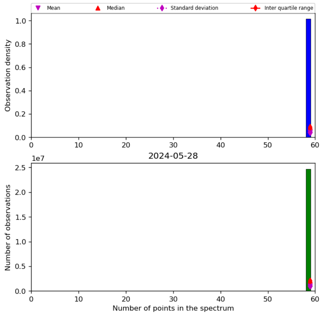
Figure 44: Histogram of “Number of points in the spectrum” for 2024-05-28 to 2024-05-29
