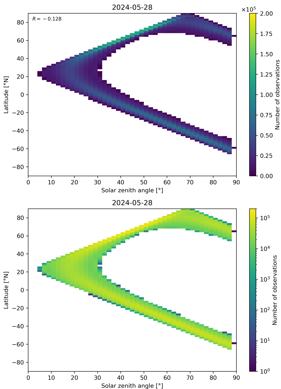
Figure 113: Scatter density plot of “Solar zenith angle” against “Latitude” for 2024-05-28 to 2024-05-29.
