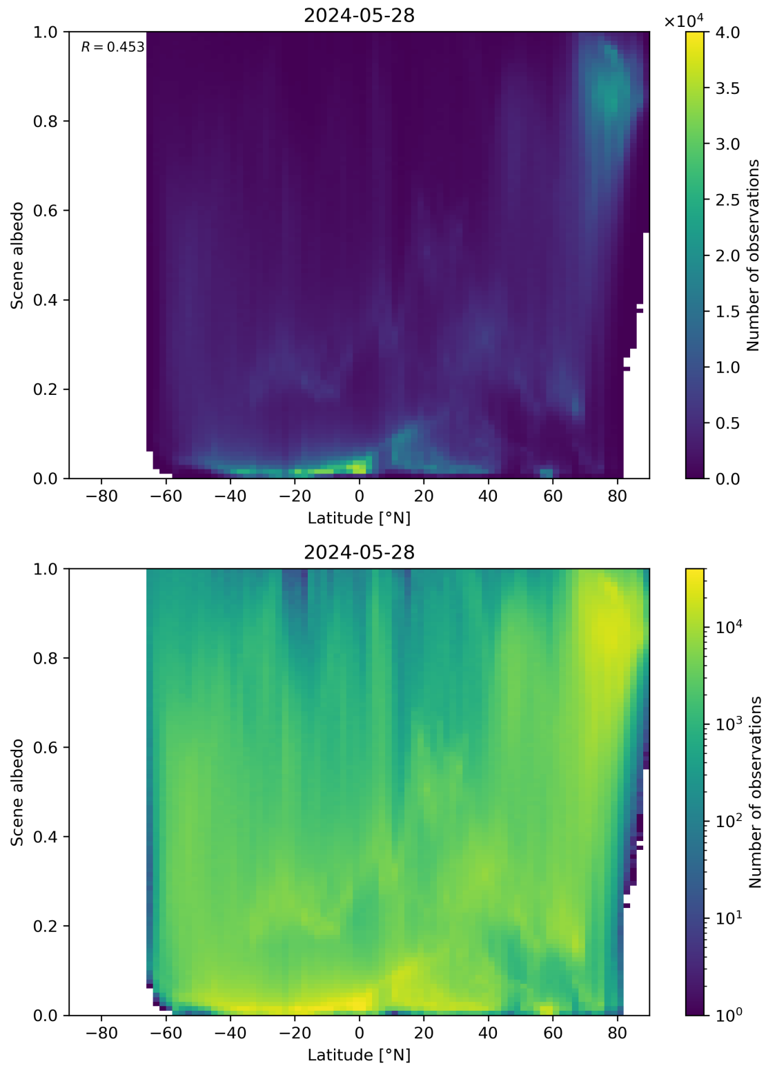
Figure 95: Scatter density plot of “Latitude” against “Scene albedo” for 2024-05-28 to 2024-05-29.
