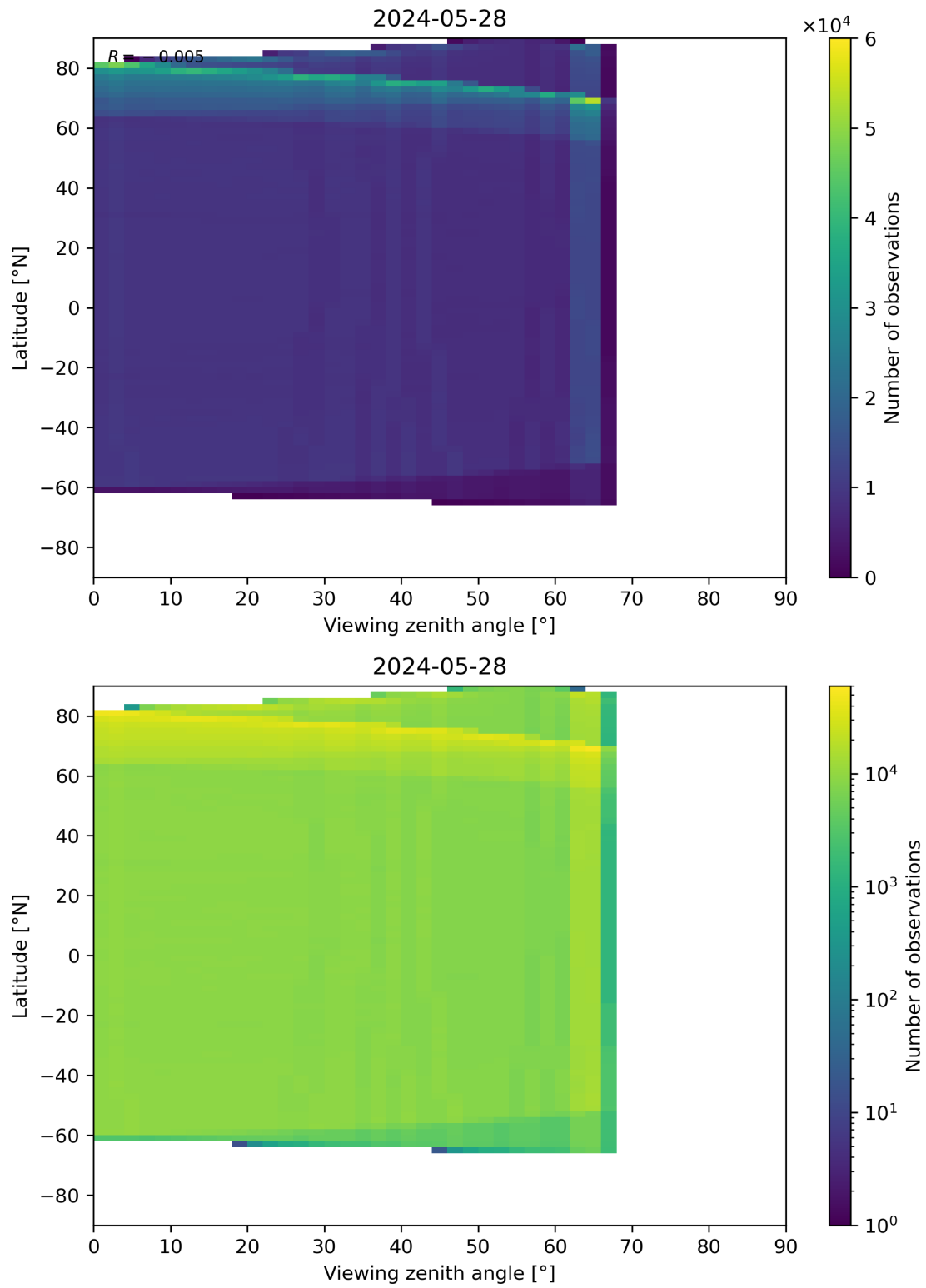
Figure 123: Scatter density plot of “Viewing zenith angle” against “Latitude” for 2024-05-28 to 2024-05-29.
