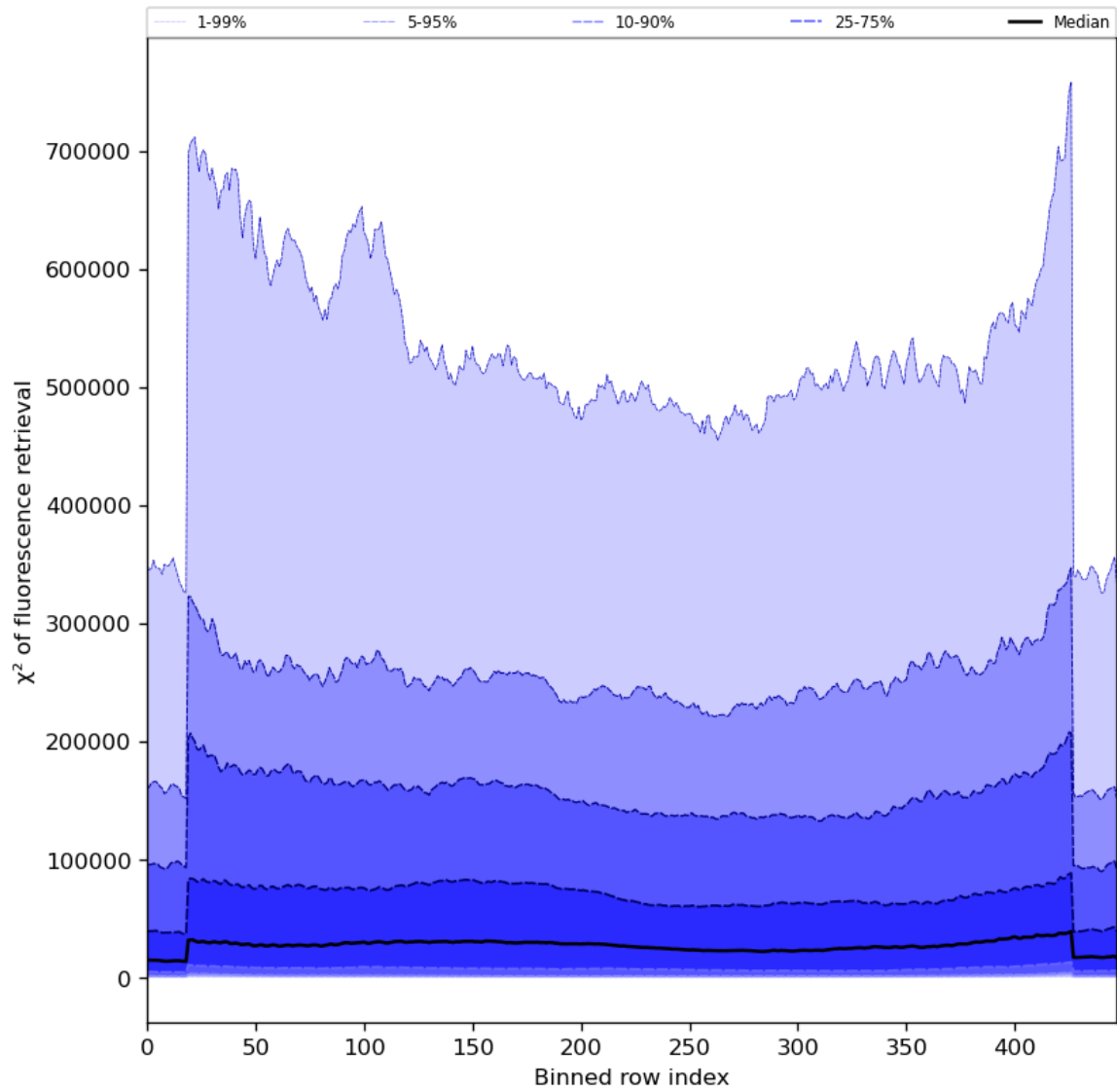
Figure 59: Along track statistics of " \chi^2 of fluorescence retrieval" for 2024-05-28 to 2024-05-29
