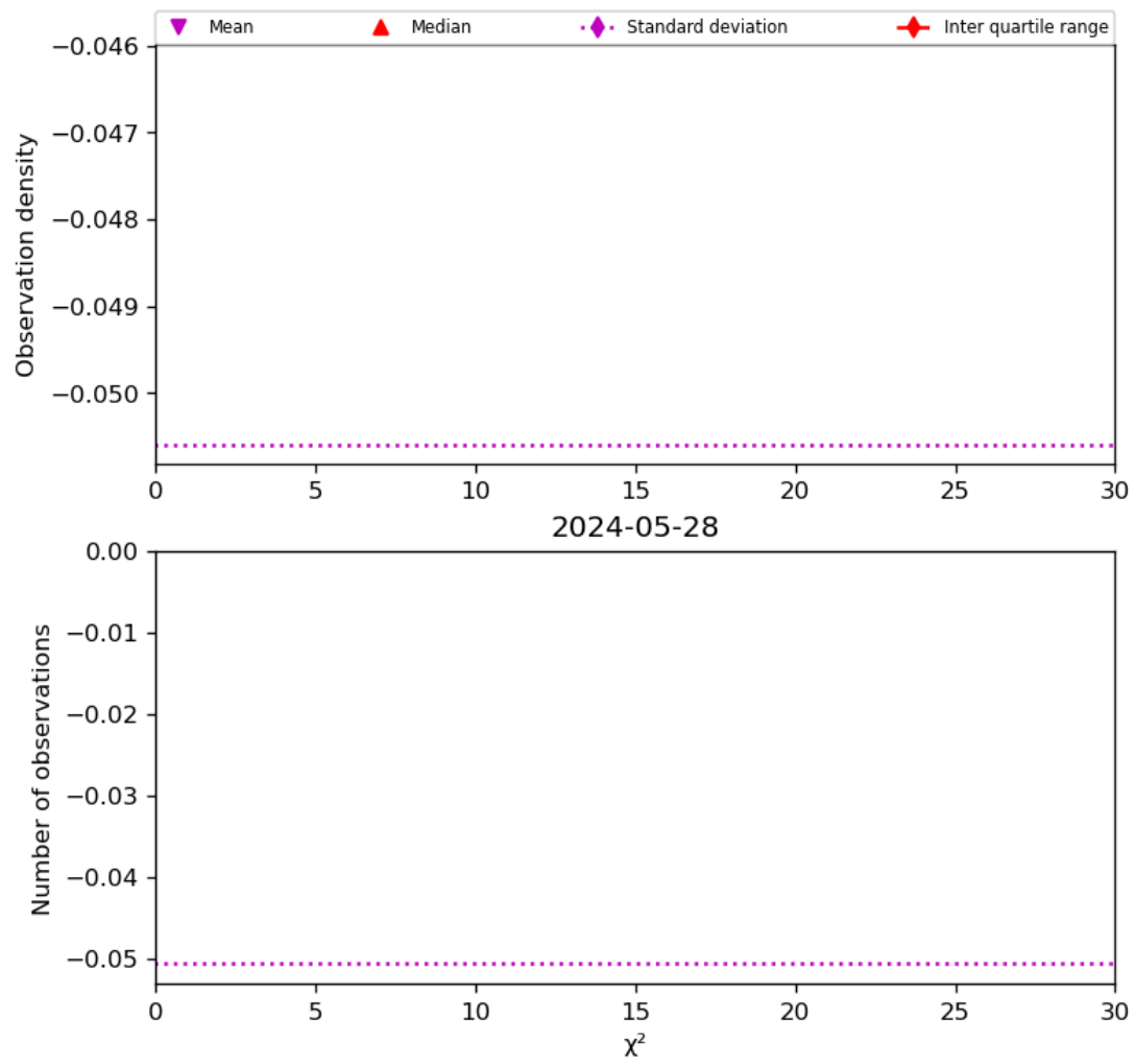
Figure 38: Histogram of “ \chi^2 ” for 2024-05-28 to 2024-05-29
