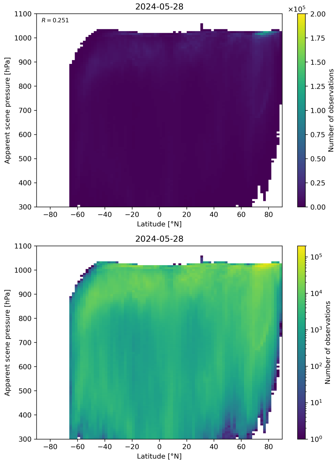
Figure 88: Scatter density plot of “Latitude” against “Apparent scene pressure” for 2024-05-28 to 2024-05-29.
