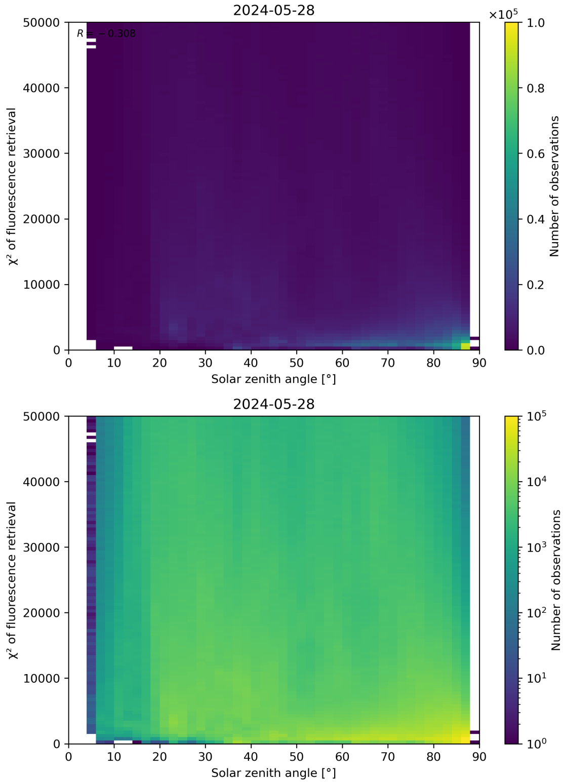
Figure 109: Scatter density plot of “Solar zenith angle” against “ \chi^2 of fluorescence retrieval” for 2024-05-28 to 2024-05-29.
