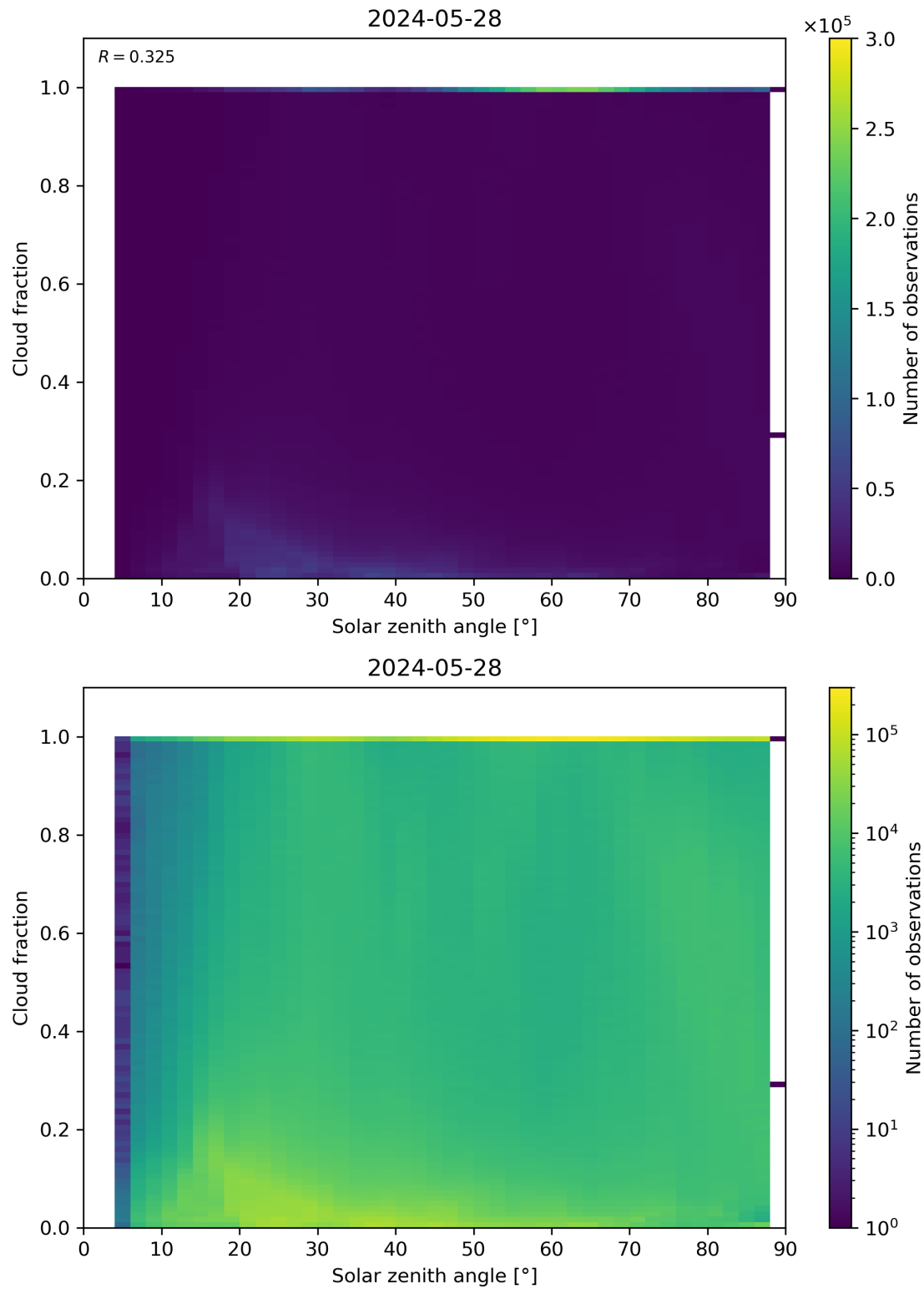
Figure 110: Scatter density plot of “Solar zenith angle” against “Cloud fraction” for 2024-05-28 to 2024-05-29.
