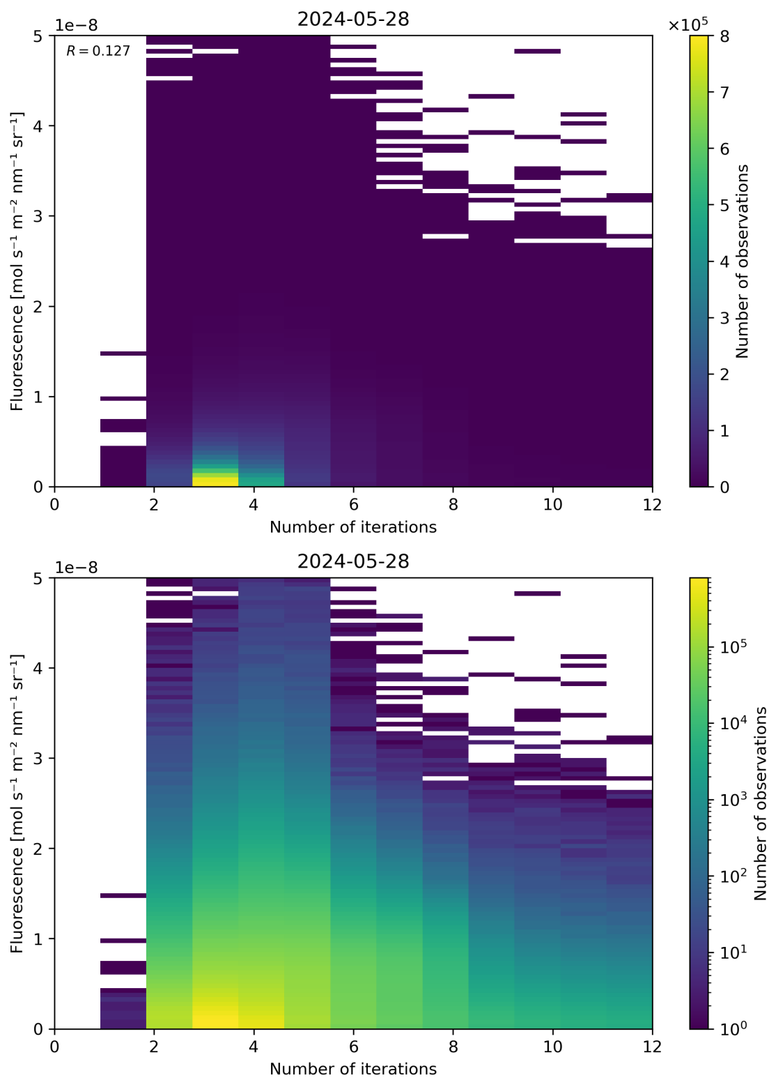
Figure 98: Scatter density plot of “Number of iterations” against “Fluorescence” for 2024-05-28 to 2024-05-29.
