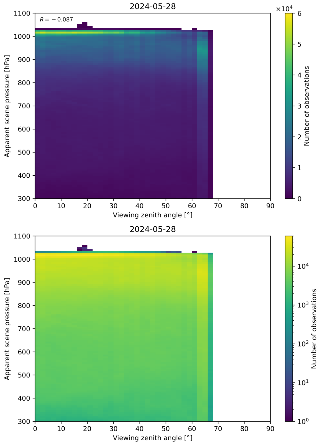
Figure 118: Scatter density plot of “Viewing zenith angle” against “Apparent scene pressure” for 2024-05-28 to 2024-05-29.
