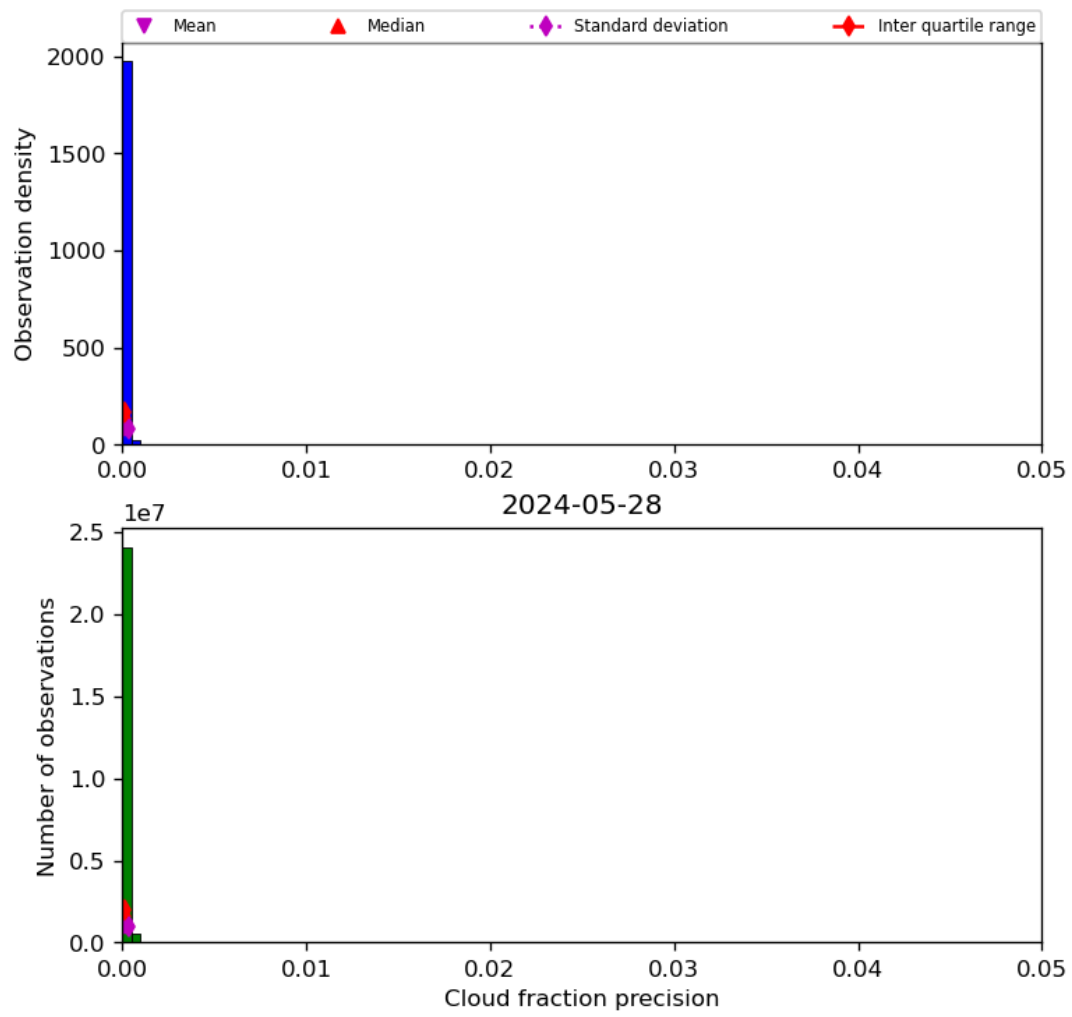
Figure 33: Histogram of “Cloud fraction precision” for 2024-05-28 to 2024-05-29
