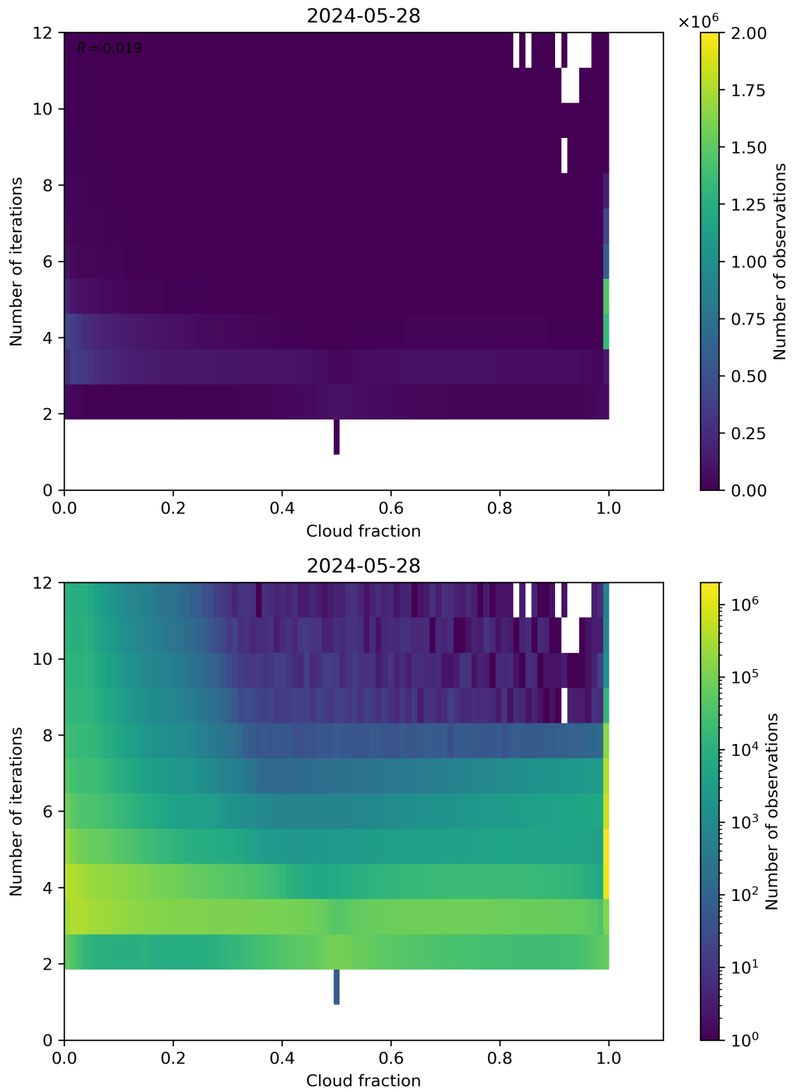
Figure 73: Scatter density plot of “Cloud fraction” against “Number of iterations” for 2024-05-28 to 2024-05-29.
