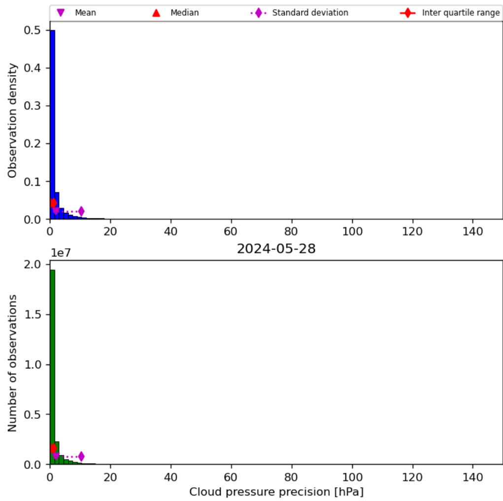
Figure 31: Histogram of “Cloud pressure precision” for 2024-05-28 to 2024-05-29
