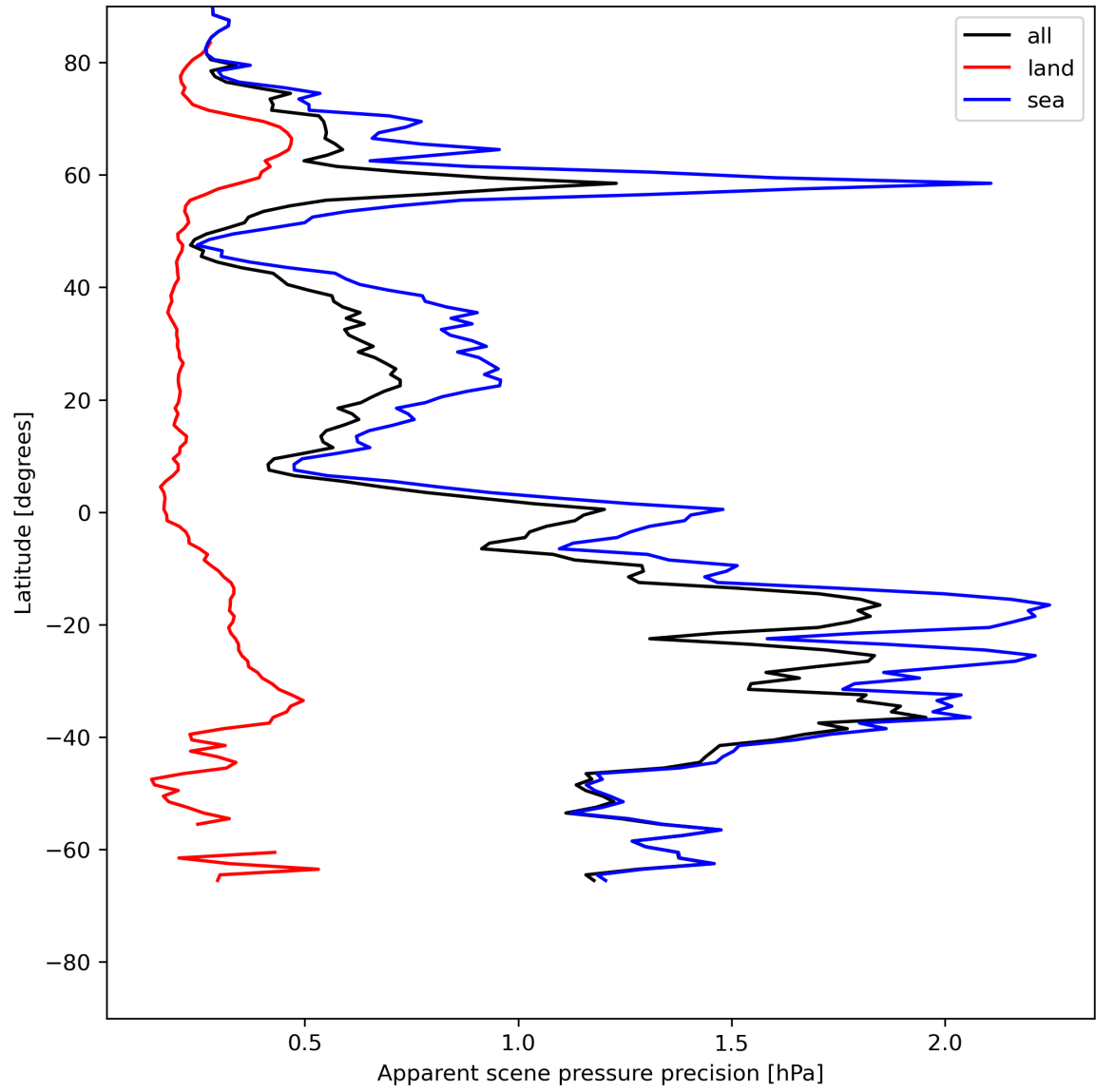
Figure 20: Zonal average of “Apparent scene pressure precision” for 2024-05-28 to 2024-05-29.
