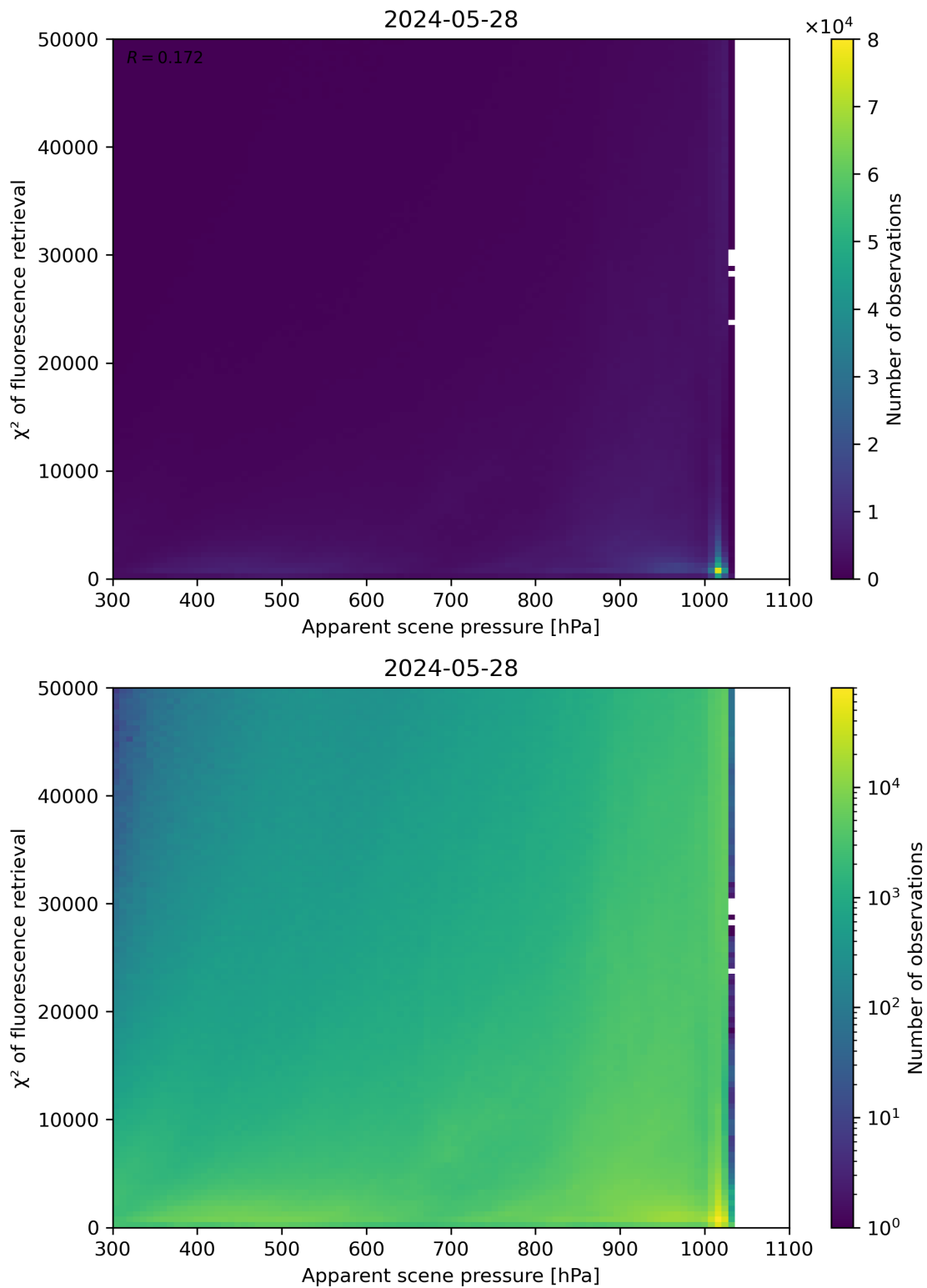
Figure 63: Scatter density plot of “Apparent scene pressure” against “ \chi^2 of fluorescence retrieval” for 2024-05-28 to 2024-05-29.
