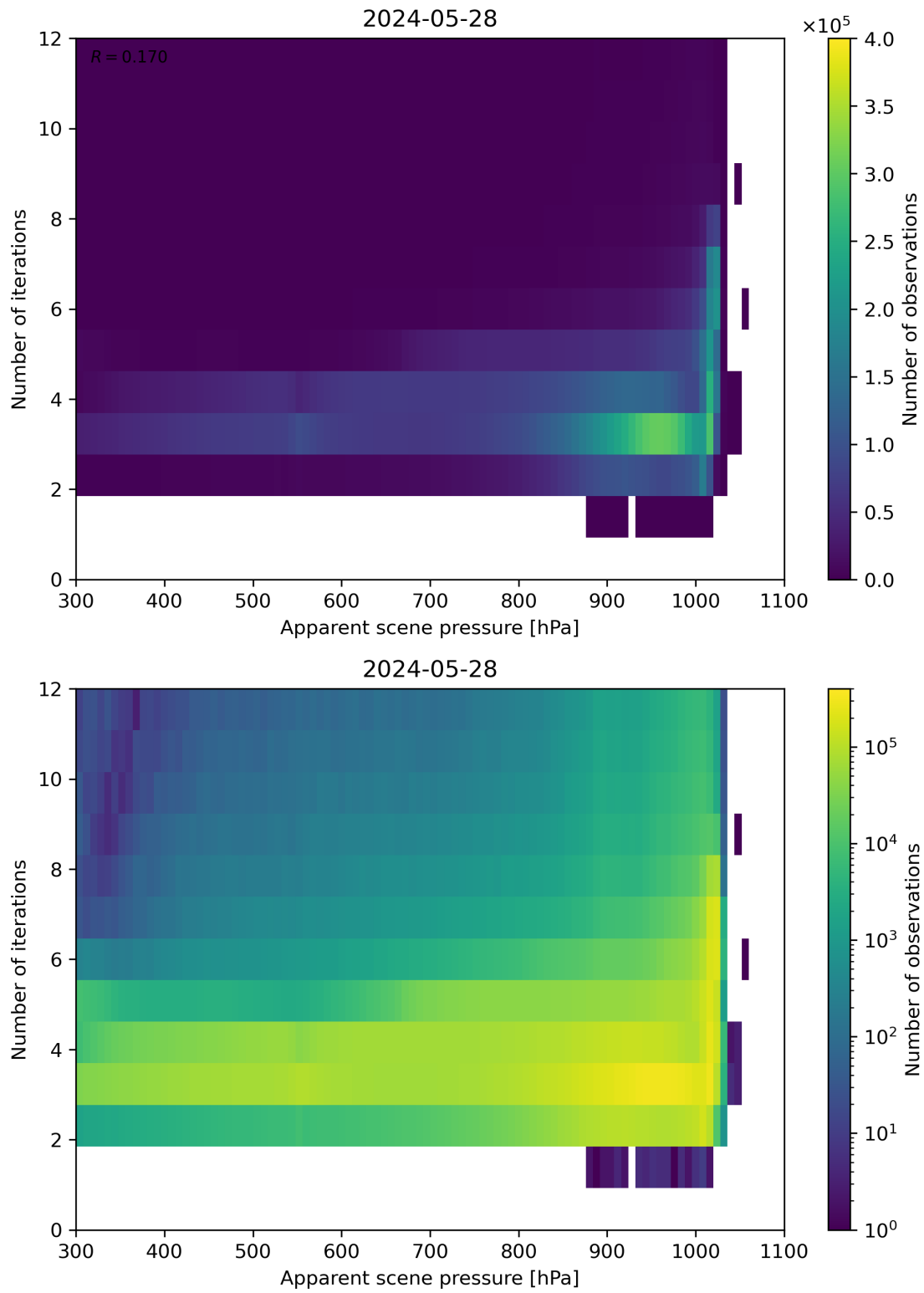
Figure 65: Scatter density plot of “Apparent scene pressure” against “Number of iterations” for 2024-05-28 to 2024-05-29.
