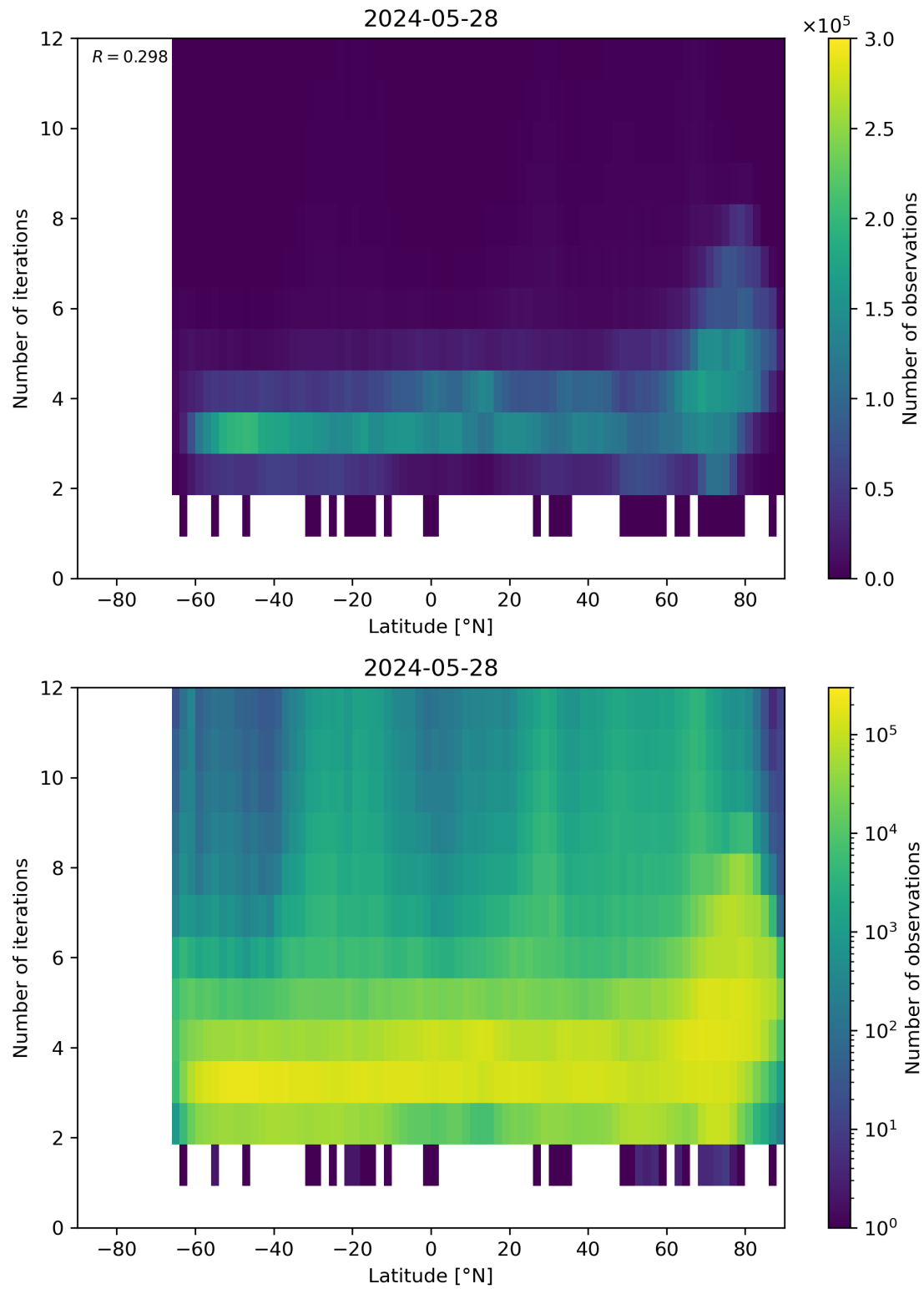
Figure 93: Scatter density plot of “Latitude” against “Number of iterations” for 2024-05-28 to 2024-05-29.
