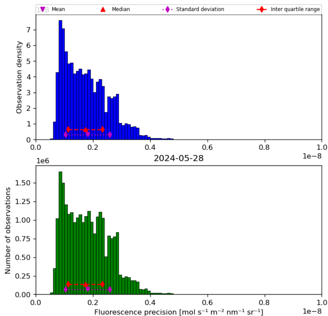
Figure 41: Histogram of “Fluorescence precision” for 2024-05-28 to 2024-05-29
