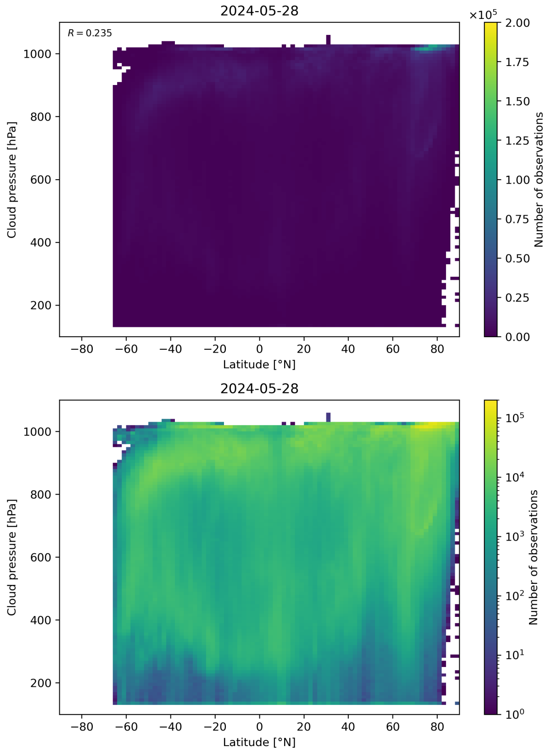
Figure 91: Scatter density plot of “Latitude” against “Cloud pressure” for 2024-05-28 to 2024-05-29.
