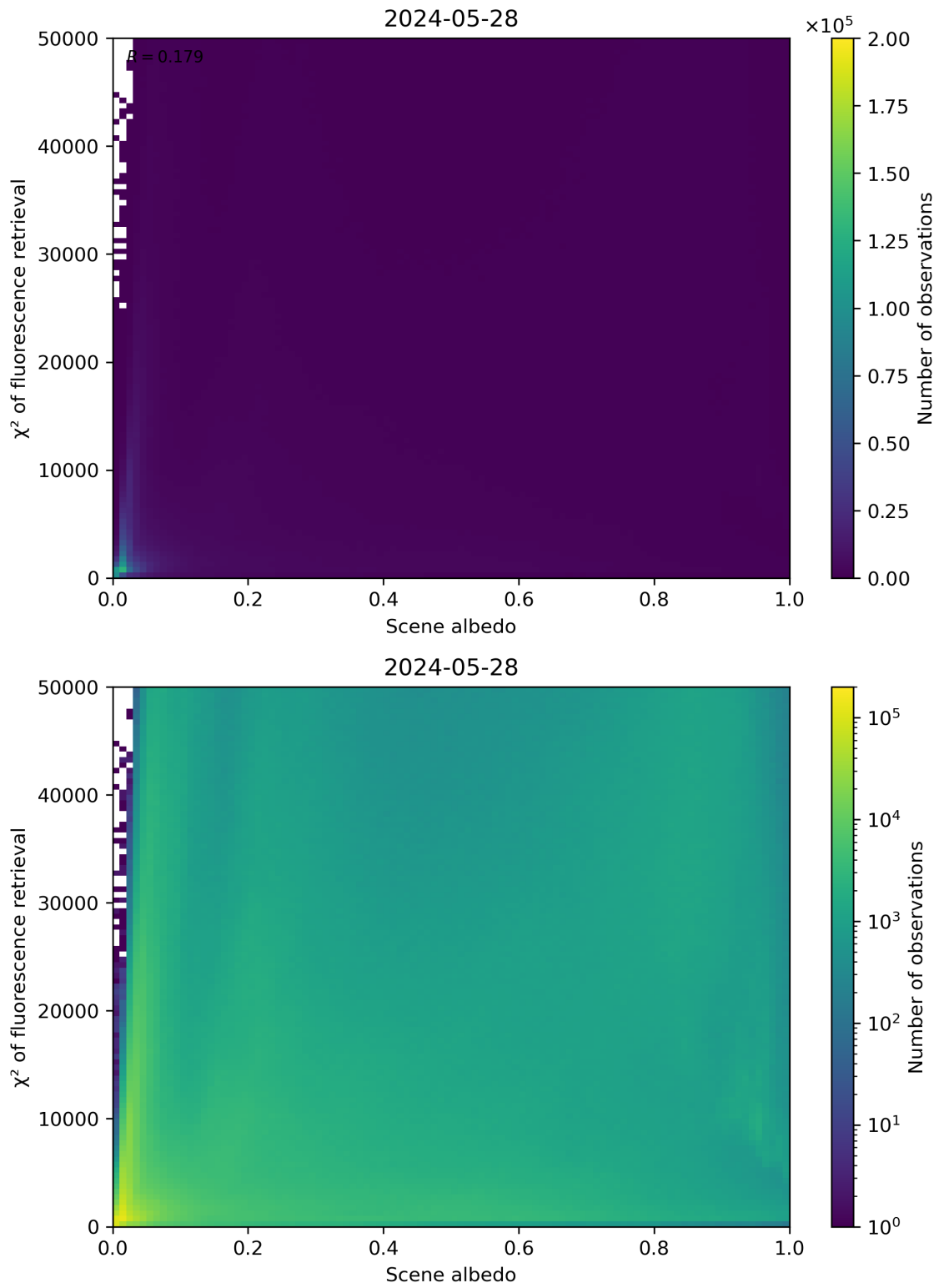
Figure 103: Scatter density plot of “Scene albedo” against “ \chi^2 of fluorescence retrieval” for 2024-05-28 to 2024-05-29.
