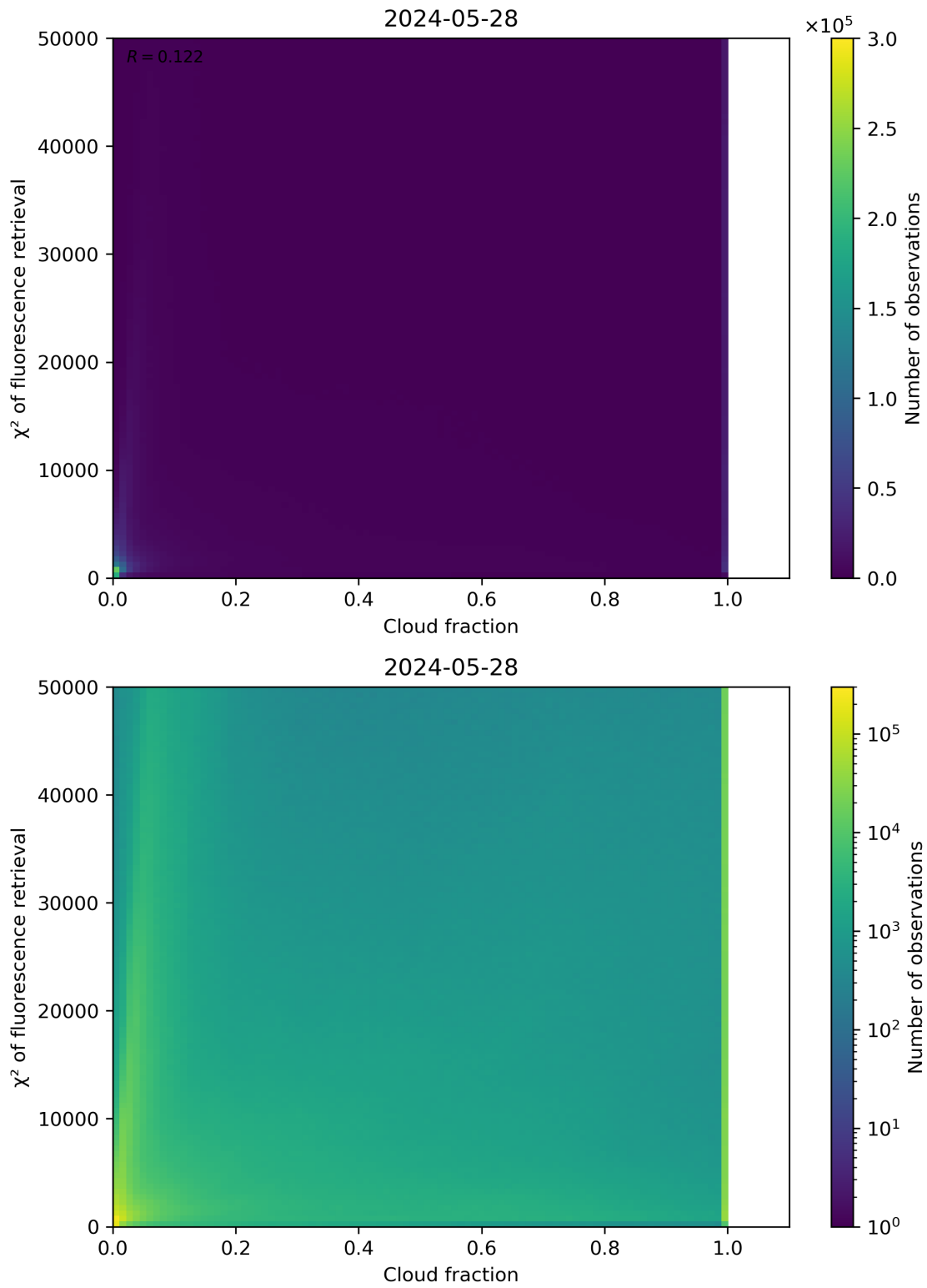
Figure 71: Scatter density plot of “Cloud fraction” against “ \chi^2 of fluorescence retrieval” for 2024-05-28 to 2024-05-29.
