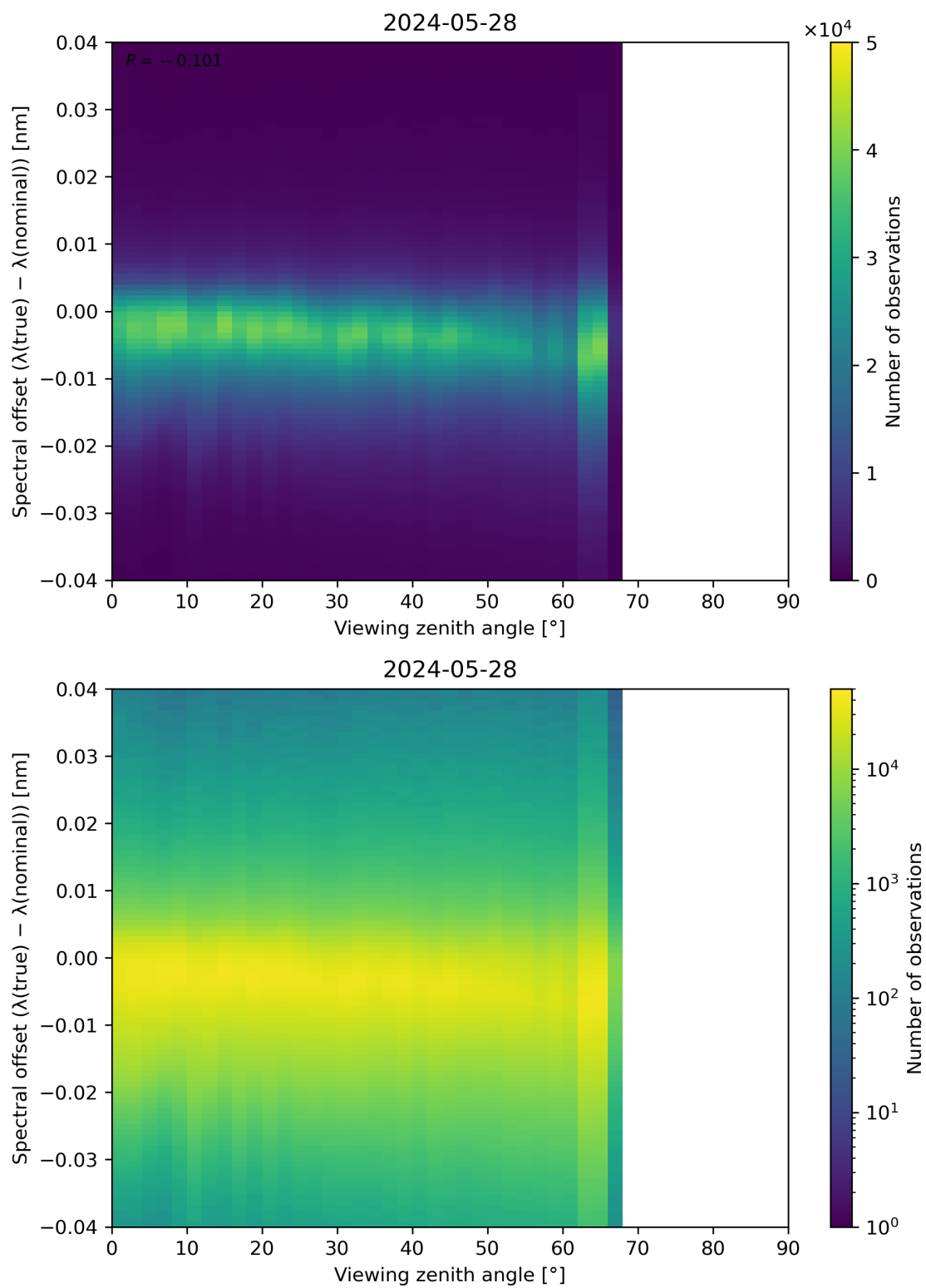
Figure 128: Scatter density plot of “Viewing zenith angle” against “Spectral offset ( \lambda(\text{true}) - \lambda(\text{nominal}) )” for 2024-05-28 to 2024-05-29.
