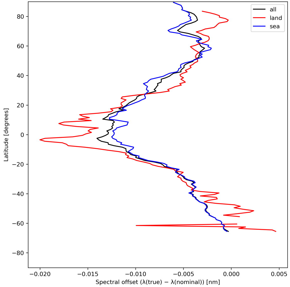
Figure 28: Zonal average of “Spectral offset ( \lambda(\text{true}) - \lambda(\text{nominal}) )” for 2024-05-28 to 2024-05-29.
