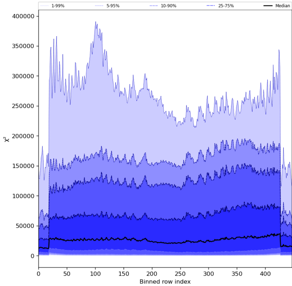
Figure 55: Along track statistics of “ \chi^2 ” for 2024-05-28 to 2024-05-29
