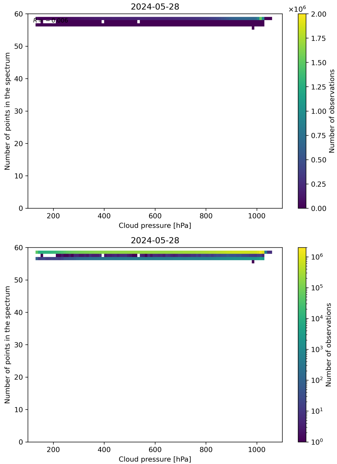
Figure 82: Scatter density plot of “Cloud pressure” against “Number of points in the spectrum” for 2024-05-28 to 2024-05-29.
