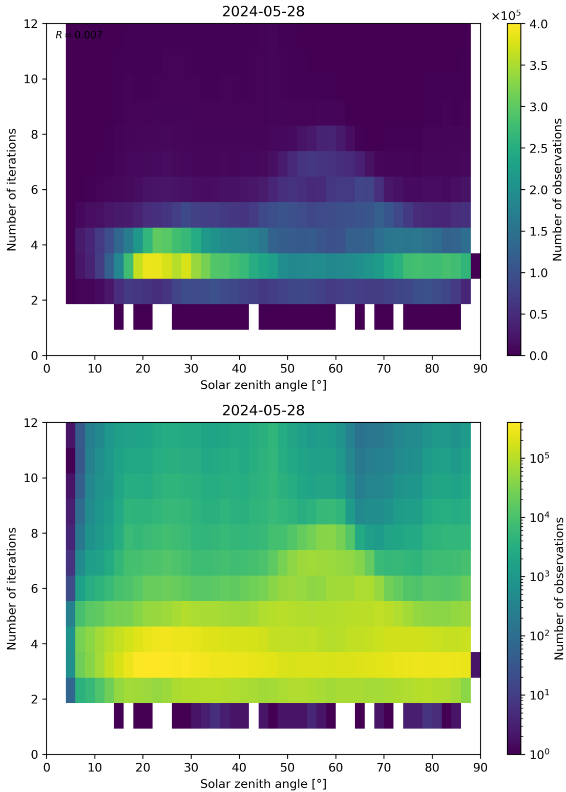
Figure 114: Scatter density plot of “Solar zenith angle” against “Number of iterations” for 2024-05-28 to 2024-05-29.
