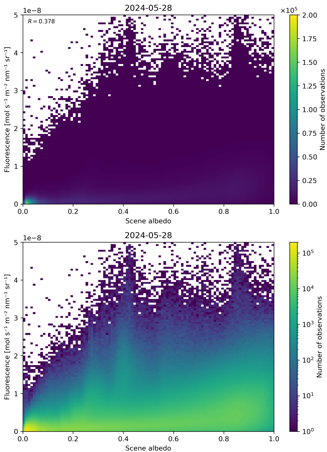
Figure 104: Scatter density plot of “Scene albedo” against “Fluorescence” for 2024-05-28 to 2024-05-29.
