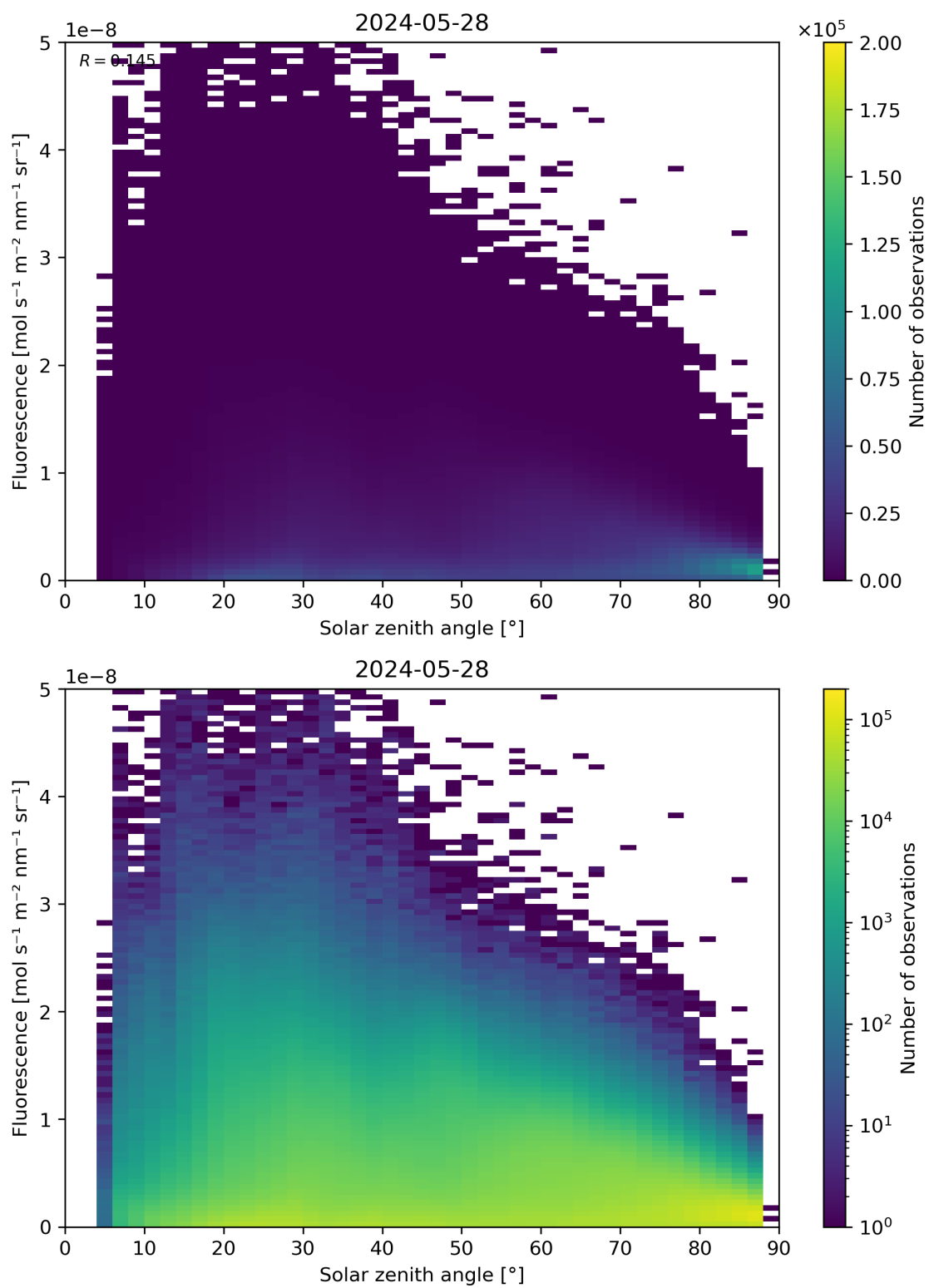
Figure 112: Scatter density plot of “Solar zenith angle” against “Fluorescence” for 2024-05-28 to 2024-05-29.
