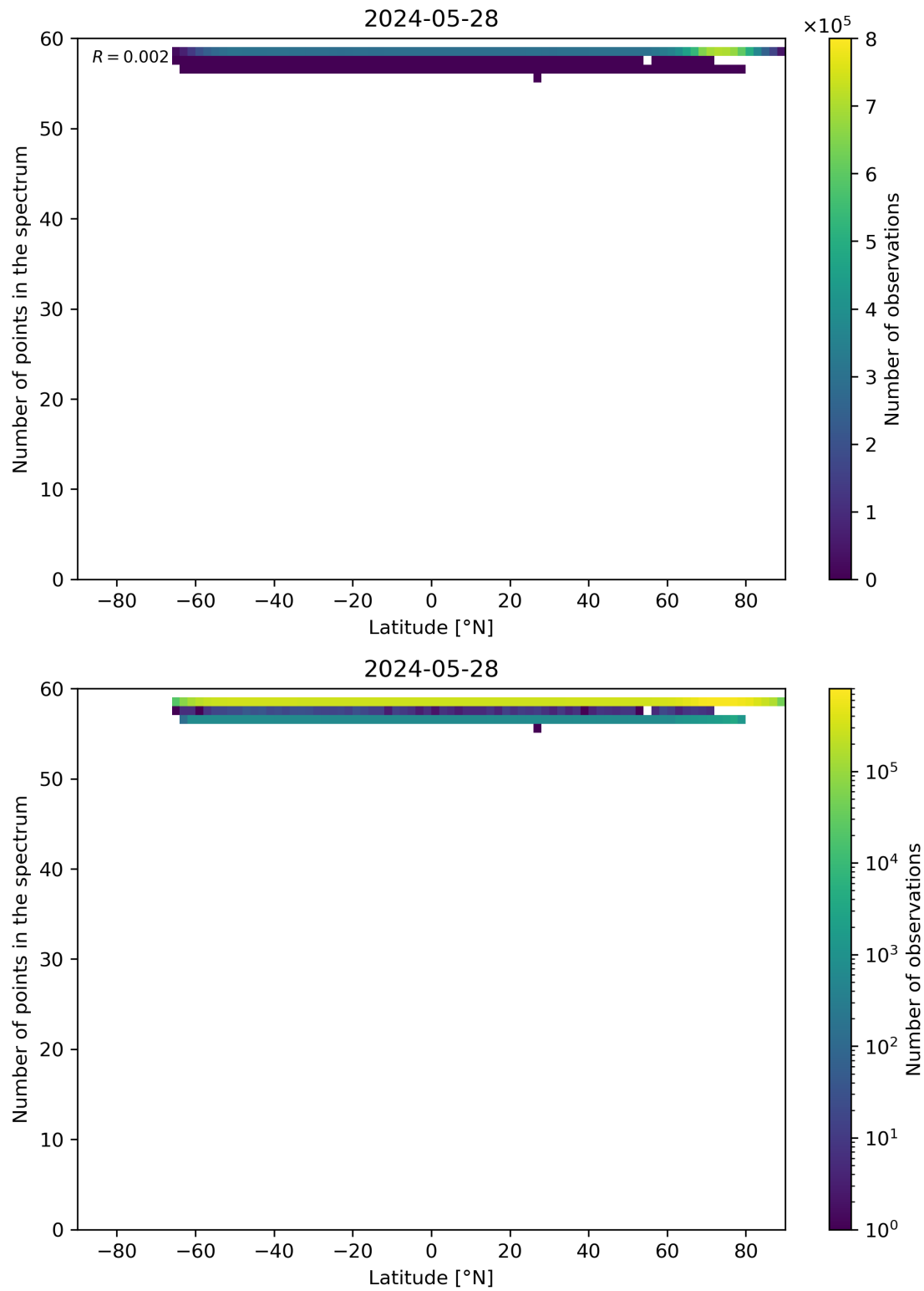
Figure 94: Scatter density plot of “Latitude” against “Number of points in the spectrum” for 2024-05-28 to 2024-05-29.
