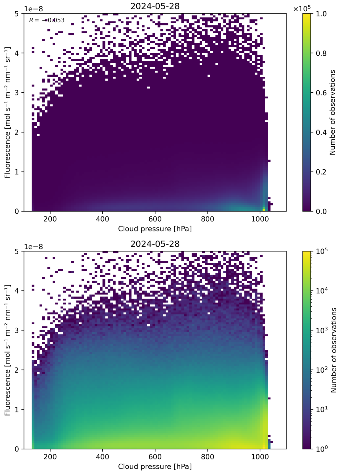
Figure 80: Scatter density plot of “Cloud pressure” against “Fluorescence” for 2024-05-28 to 2024-05-29.
