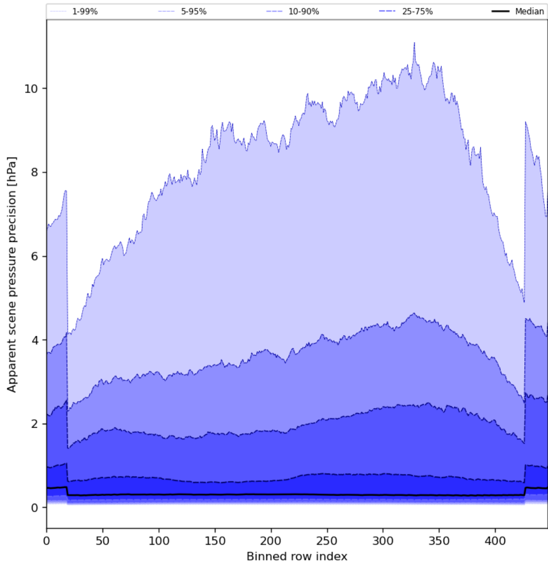
Figure 54: Along track statistics of “Apparent scene pressure precision” for 2024-05-28 to 2024-05-29
