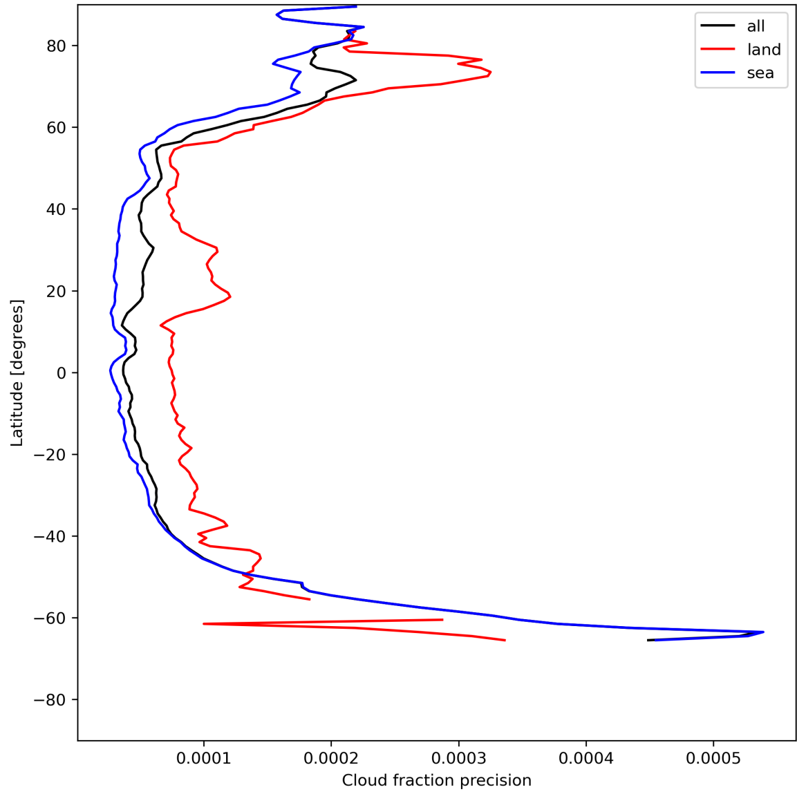
Figure 16: Zonal average of “Cloud fraction precision” for 2024-05-28 to 2024-05-29.
