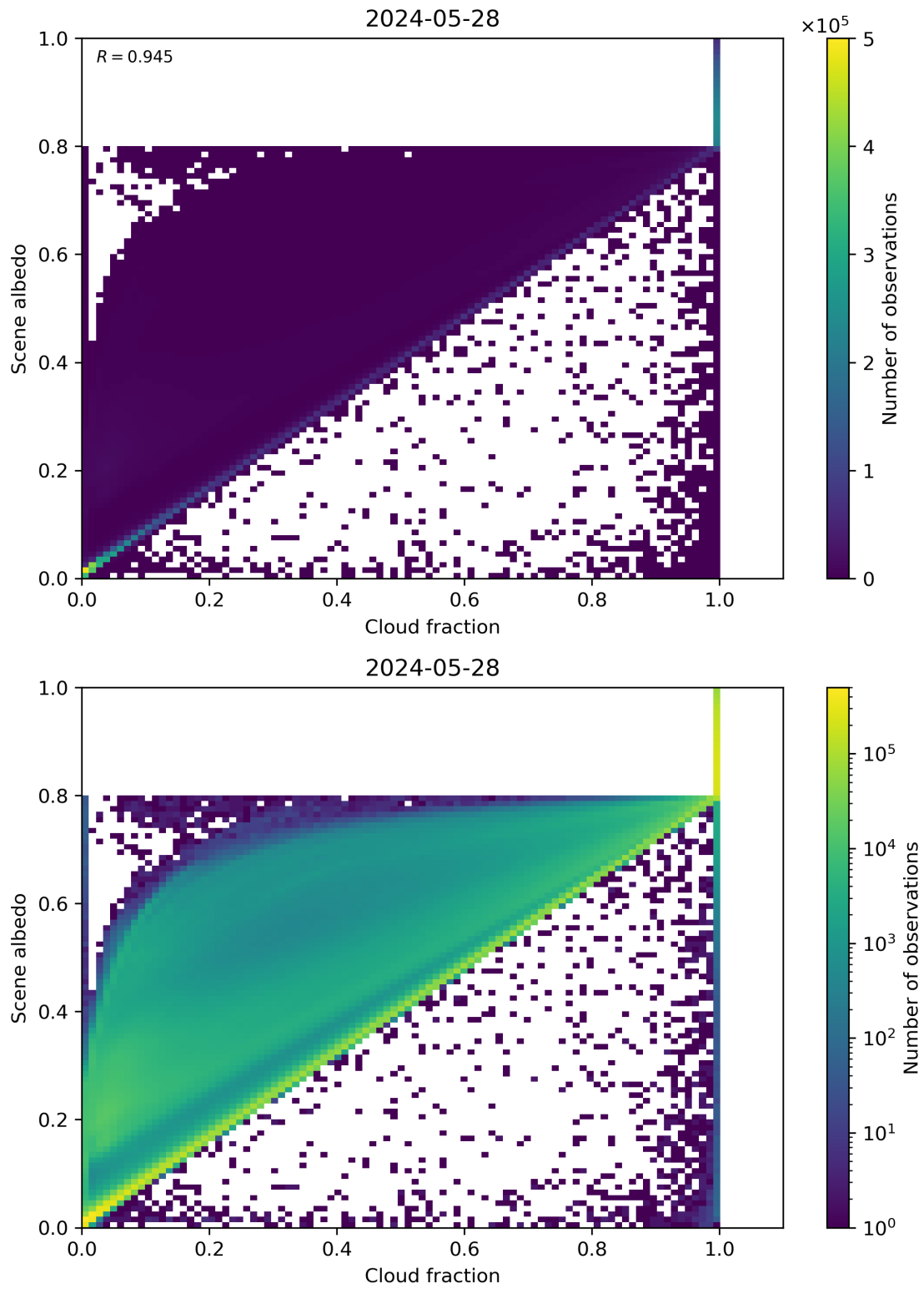
Figure 75: Scatter density plot of “Cloud fraction” against “Scene albedo” for 2024-05-28 to 2024-05-29.
