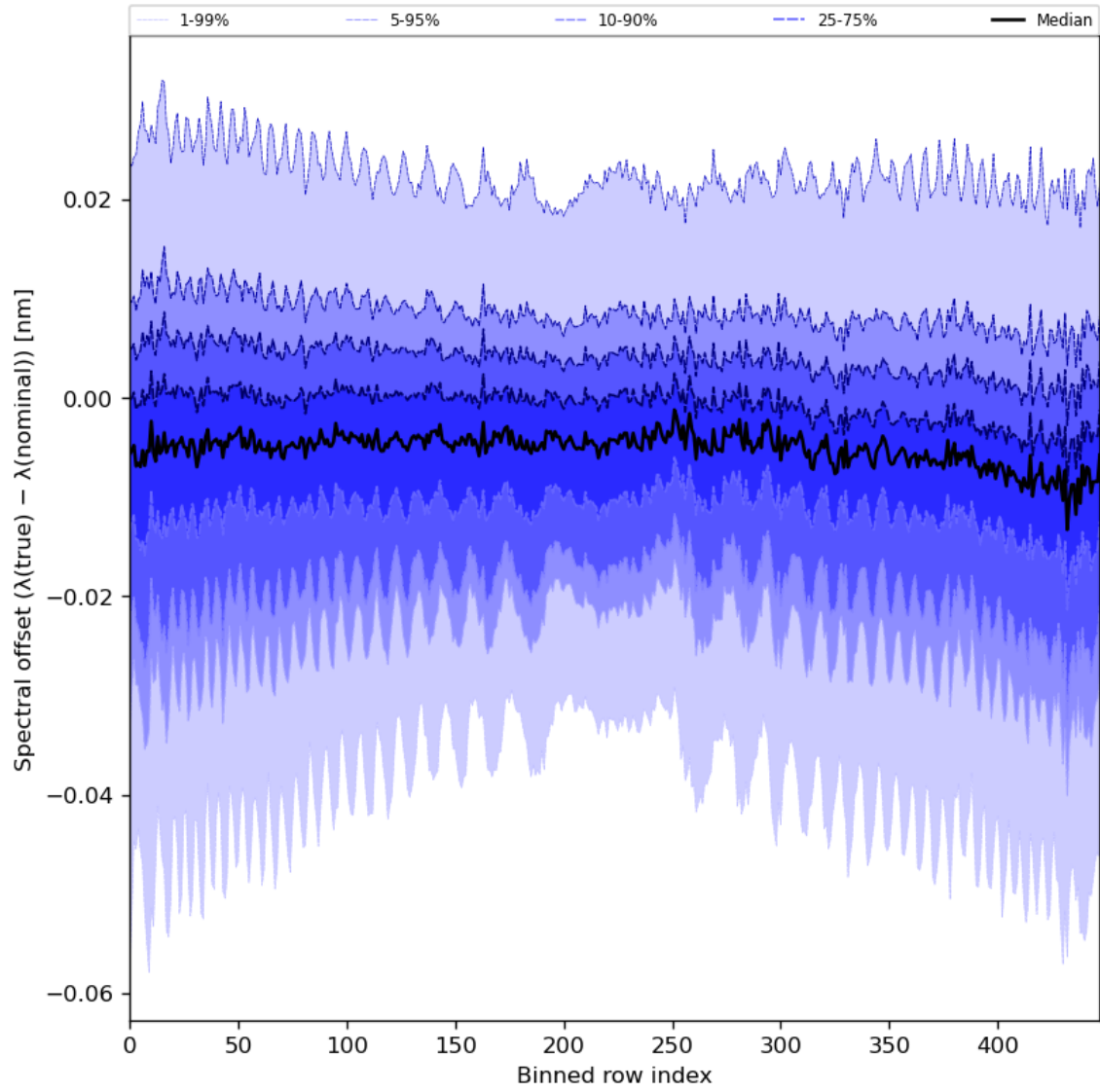
Figure 62: Along track statistics of “Spectral offset ( \lambda(\text{true}) - \lambda(\text{nominal}) )” for 2024-05-28 to 2024-05-29
