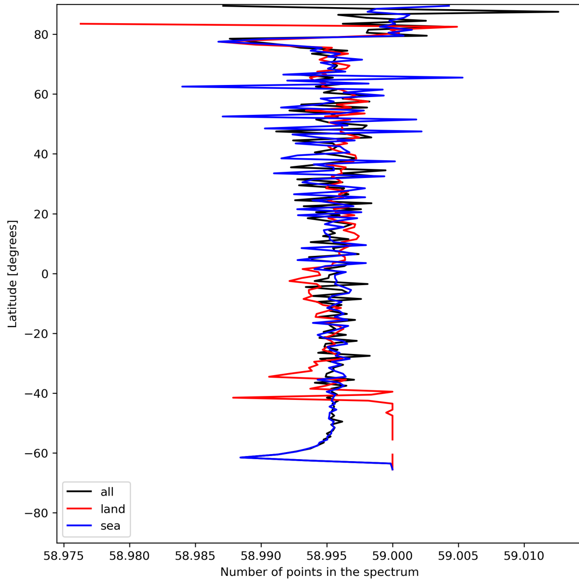
Figure 27: Zonal average of “Number of points in the spectrum” for 2024-05-28 to 2024-05-29.
