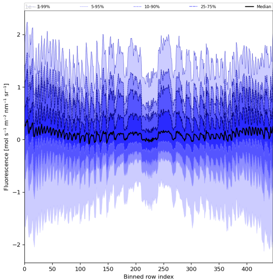
Figure 57: Along track statistics of “Fluorescence” for 2024-05-28 to 2024-05-29
