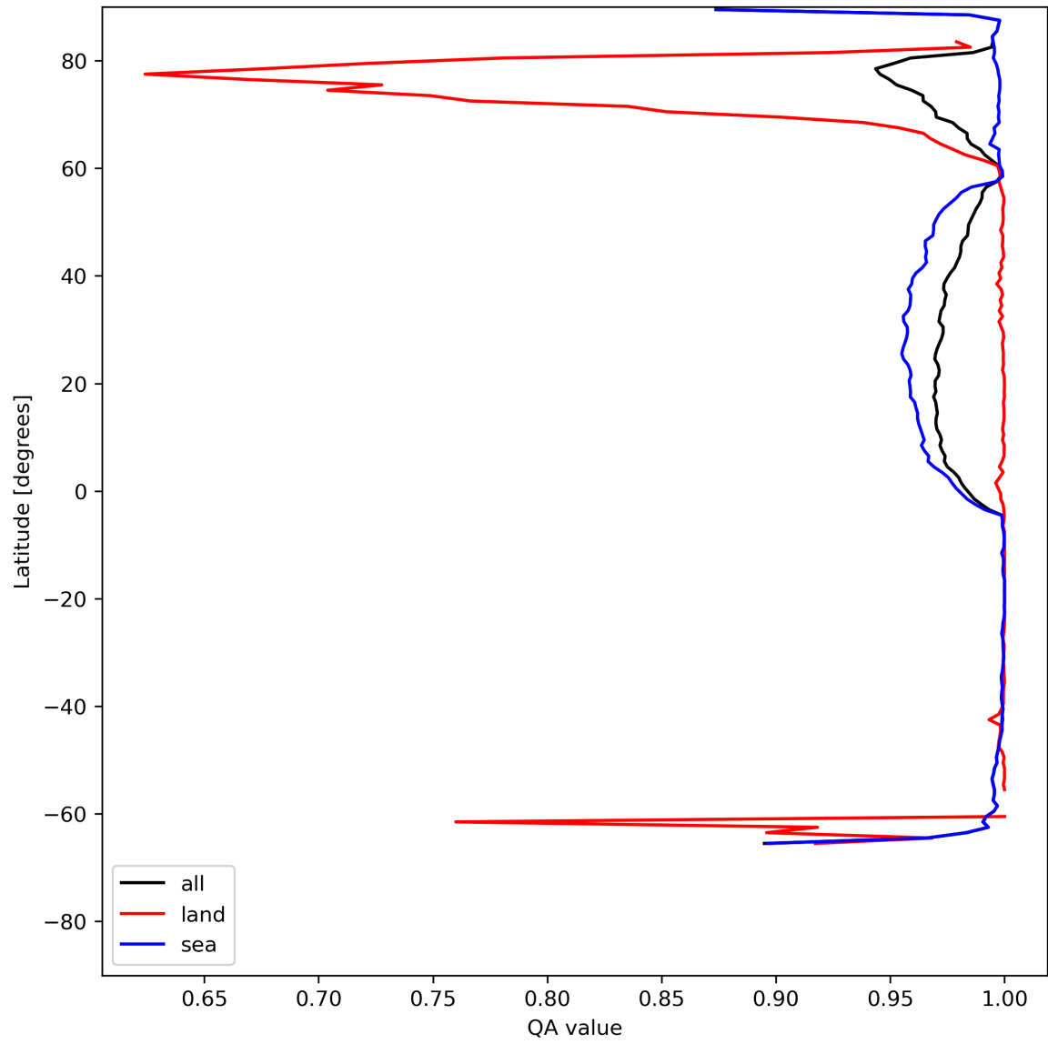
Figure 12: Zonal average of “QA value” for 2024-05-28 to 2024-05-29.
