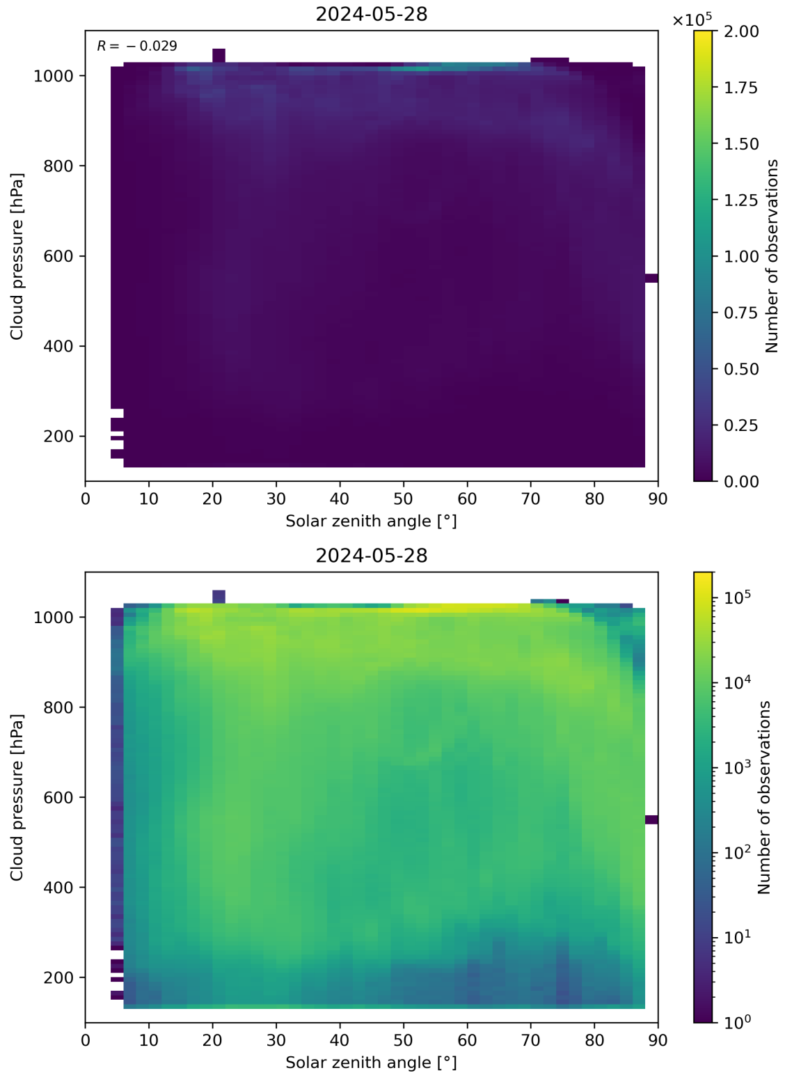
Figure 111: Scatter density plot of “Solar zenith angle” against “Cloud pressure” for 2024-05-28 to 2024-05-29.
