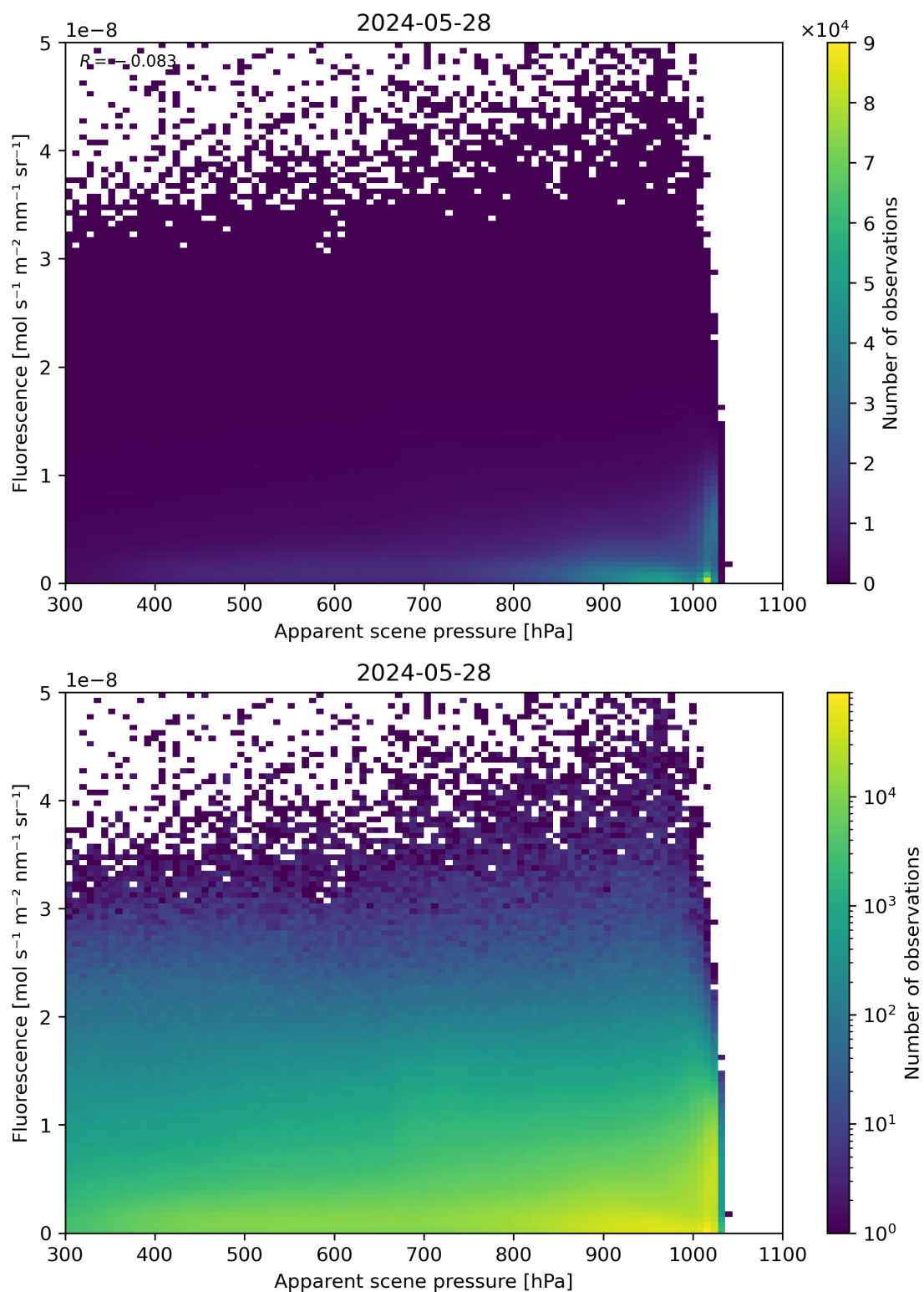
Figure 64: Scatter density plot of “Apparent scene pressure” against “Fluorescence” for 2024-05-28 to 2024-05-29.
