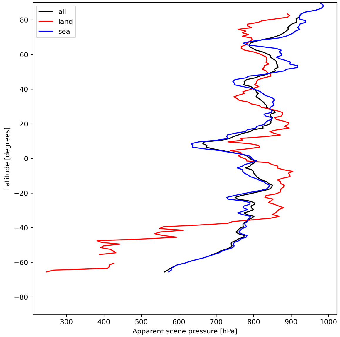
Figure 19: Zonal average of “Apparent scene pressure” for 2024-05-28 to 2024-05-29.
