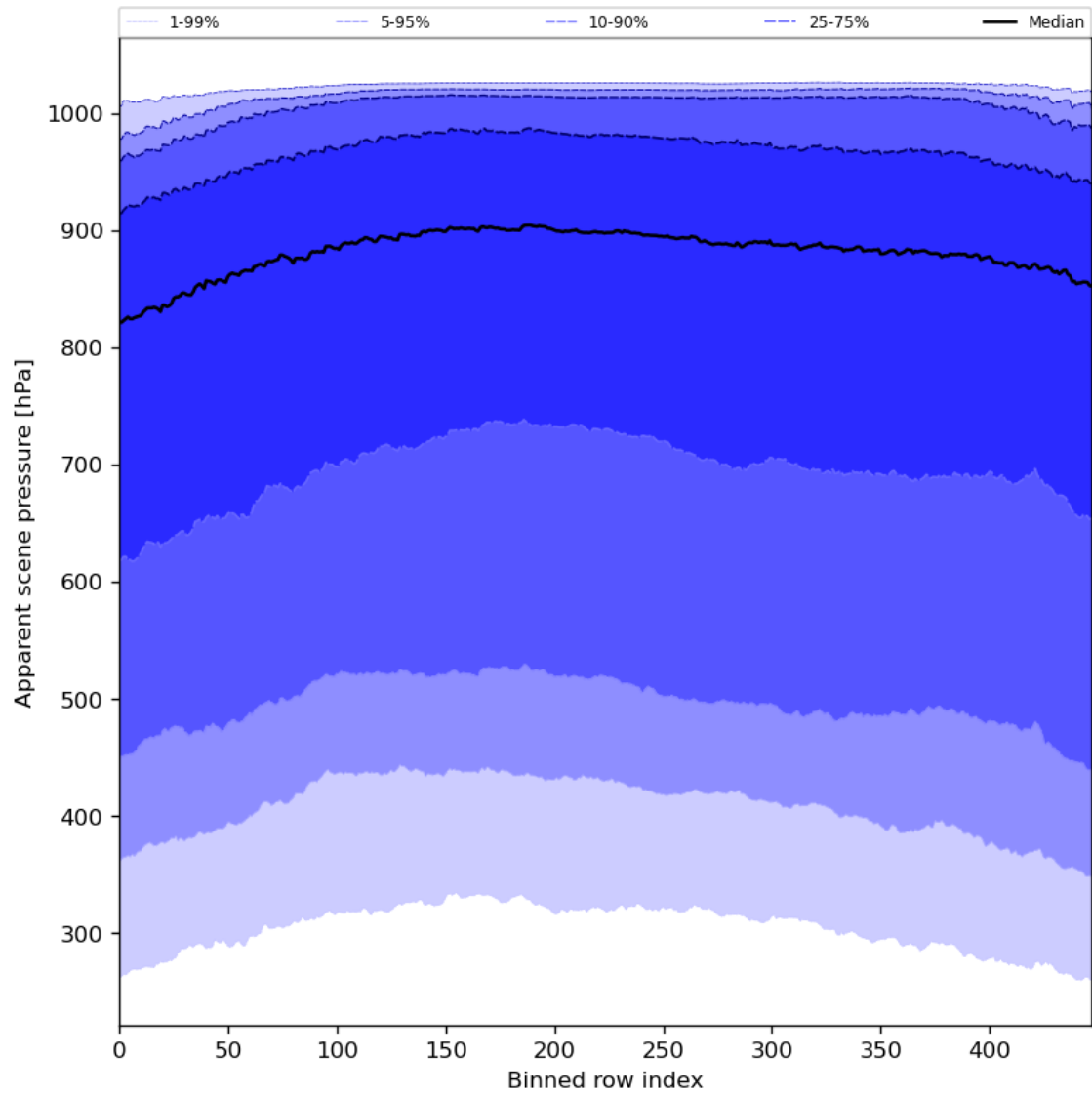
Figure 53: Along track statistics of “Apparent scene pressure” for 2024-05-28 to 2024-05-29
