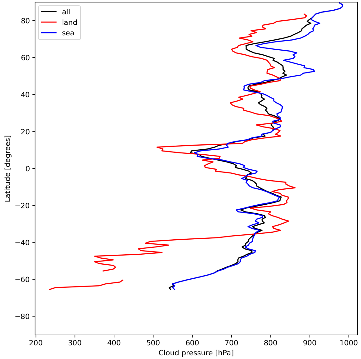
Figure 13: Zonal average of “Cloud pressure” for 2024-05-28 to 2024-05-29.
