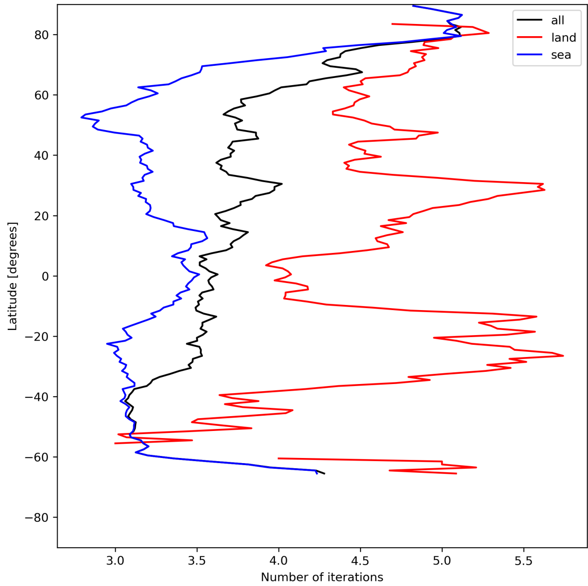
Figure 22: Zonal average of “Number of iterations” for 2024-05-28 to 2024-05-29.
