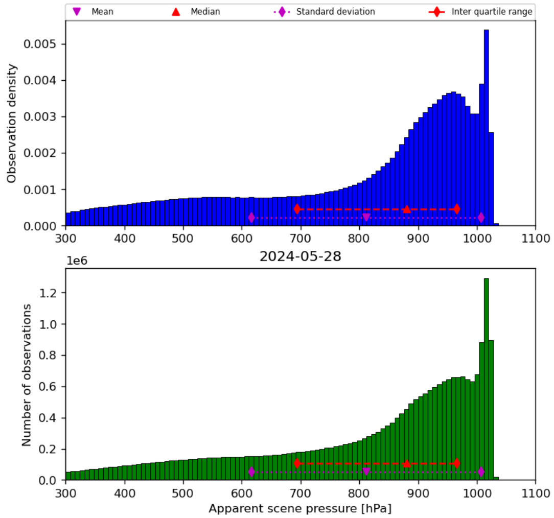
Figure 36: Histogram of “Apparent scene pressure” for 2024-05-28 to 2024-05-29
