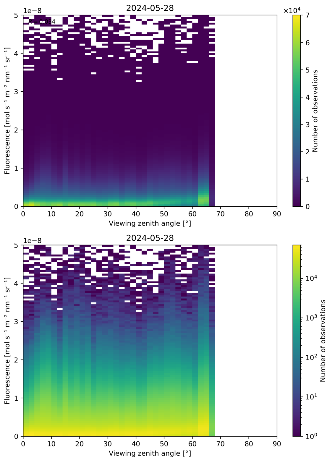
Figure 122: Scatter density plot of “Viewing zenith angle” against “Fluorescence” for 2024-05-28 to 2024-05-29.
