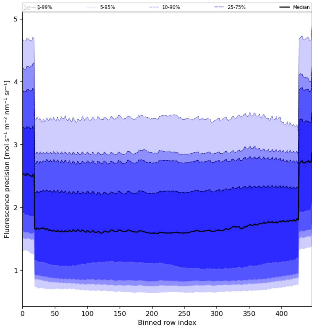
Figure 58: Along track statistics of “Fluorescence precision” for 2024-05-28 to 2024-05-29
