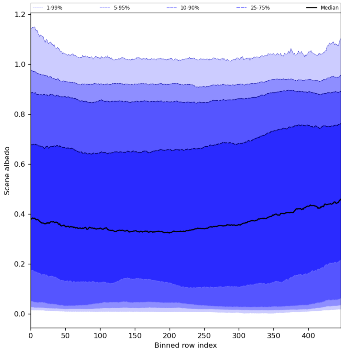
Figure 51: Along track statistics of “Scene albedo” for 2024-05-28 to 2024-05-29
