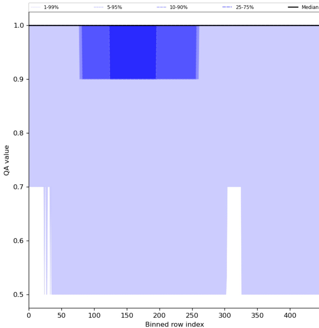
Figure 46: Along track statistics of “QA value” for 2024-05-28 to 2024-05-29
