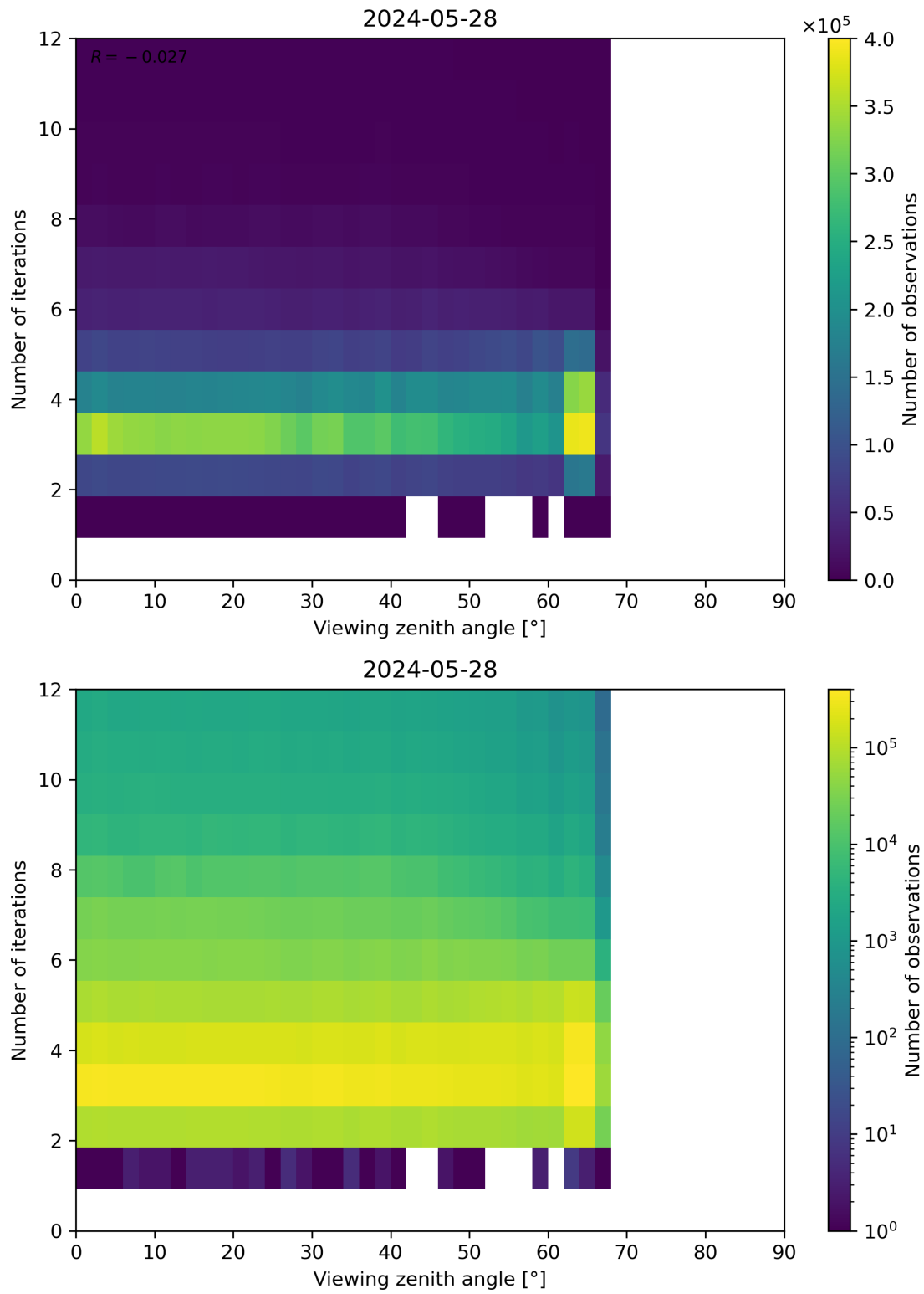
Figure 124: Scatter density plot of “Viewing zenith angle” against “Number of iterations” for 2024-05-28 to 2024-05-29.
