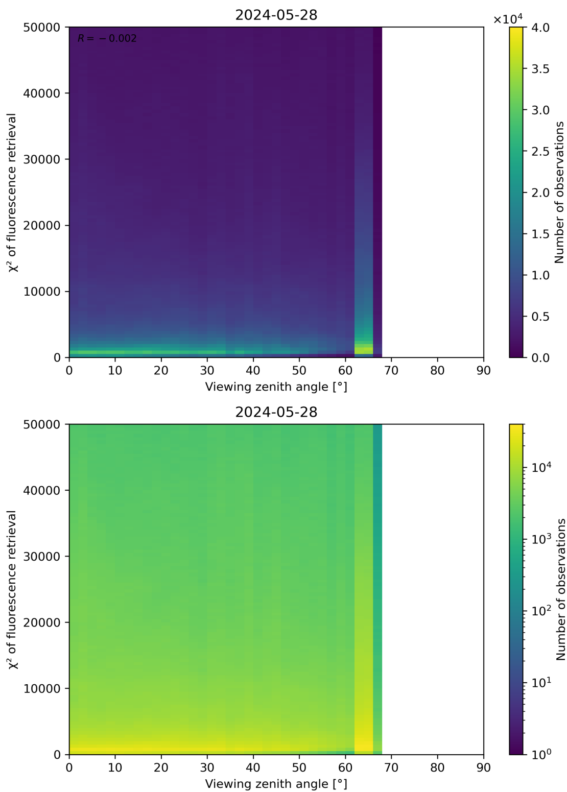
Figure 119: Scatter density plot of “Viewing zenith angle” against “ \chi^2 of fluorescence retrieval” for 2024-05-28 to 2024-05-29.
