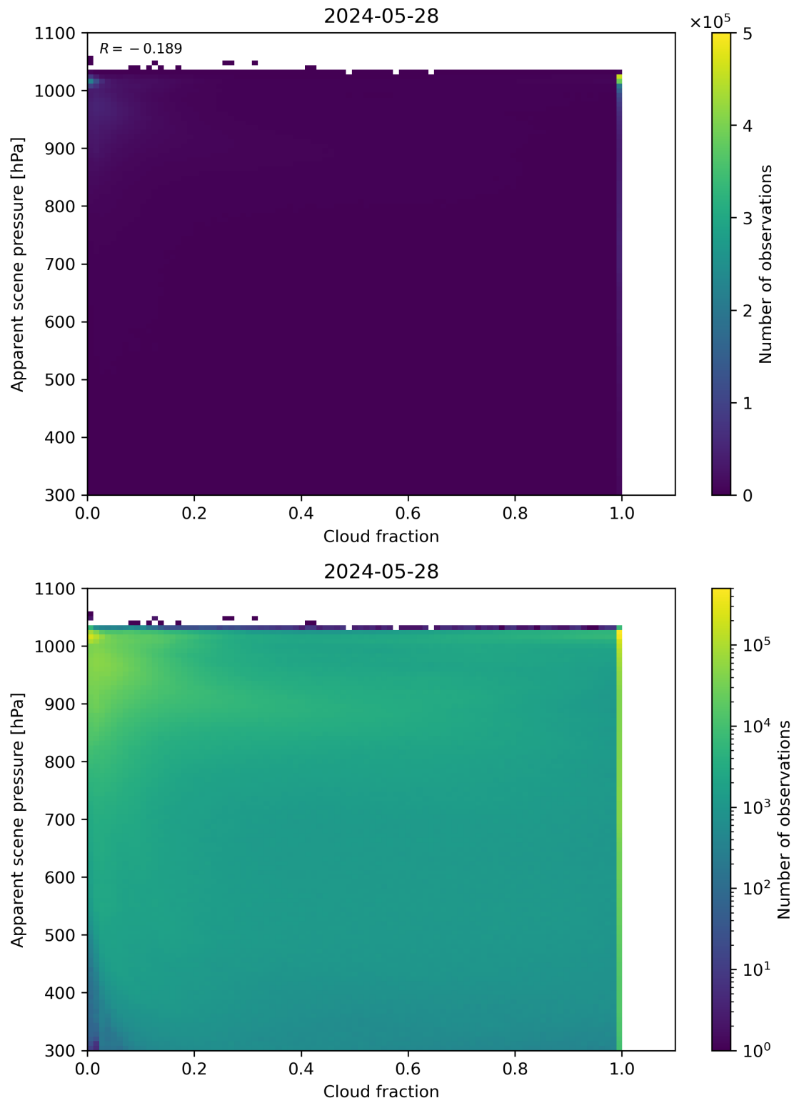
Figure 70: Scatter density plot of “Cloud fraction” against “Apparent scene pressure” for 2024-05-28 to 2024-05-29.
