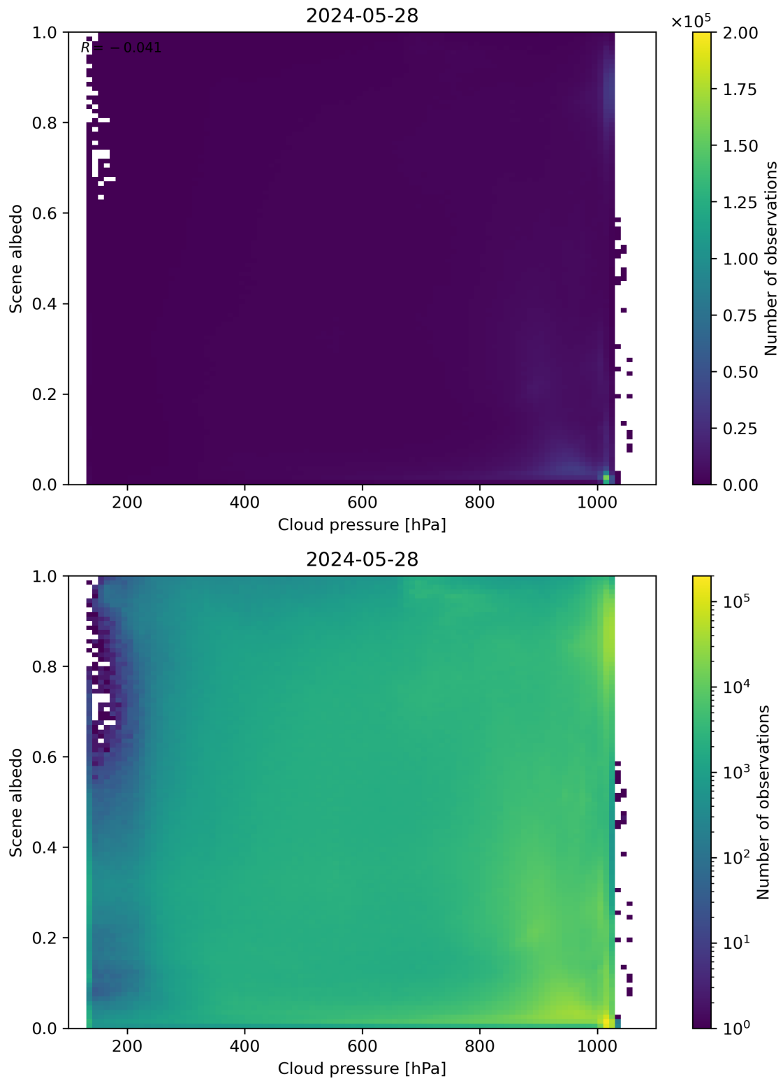
Figure 83: Scatter density plot of “Cloud pressure” against “Scene albedo” for 2024-05-28 to 2024-05-29.
