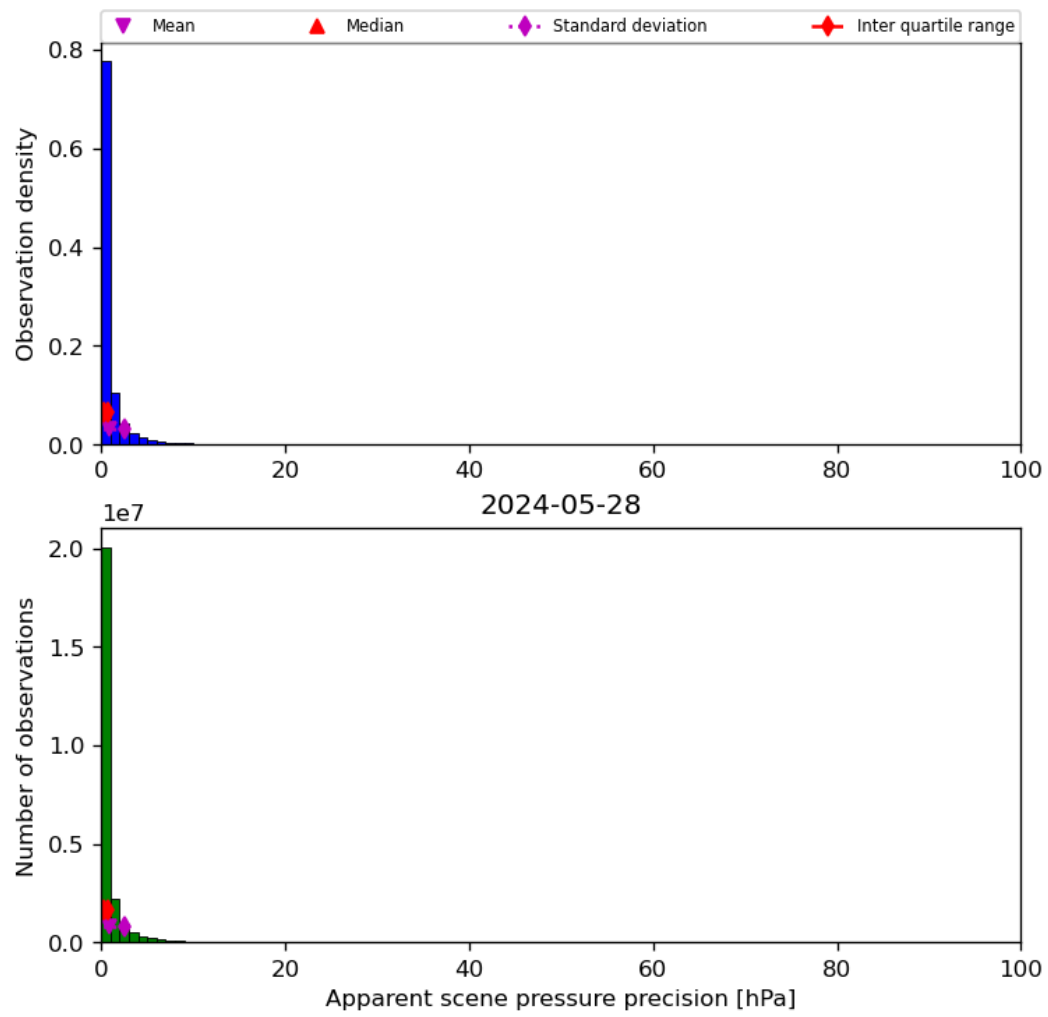
Figure 37: Histogram of “Apparent scene pressure precision” for 2024-05-28 to 2024-05-29
