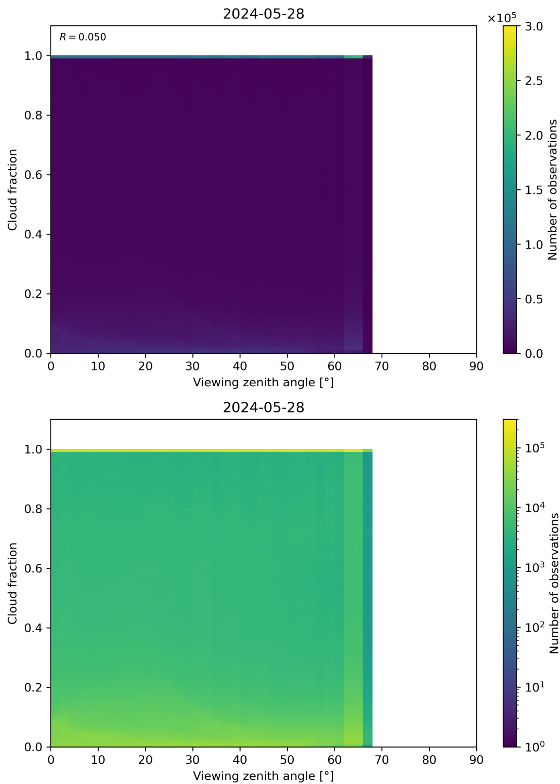
Figure 120: Scatter density plot of “Viewing zenith angle” against “Cloud fraction” for 2024-05-28 to 2024-05-29.
