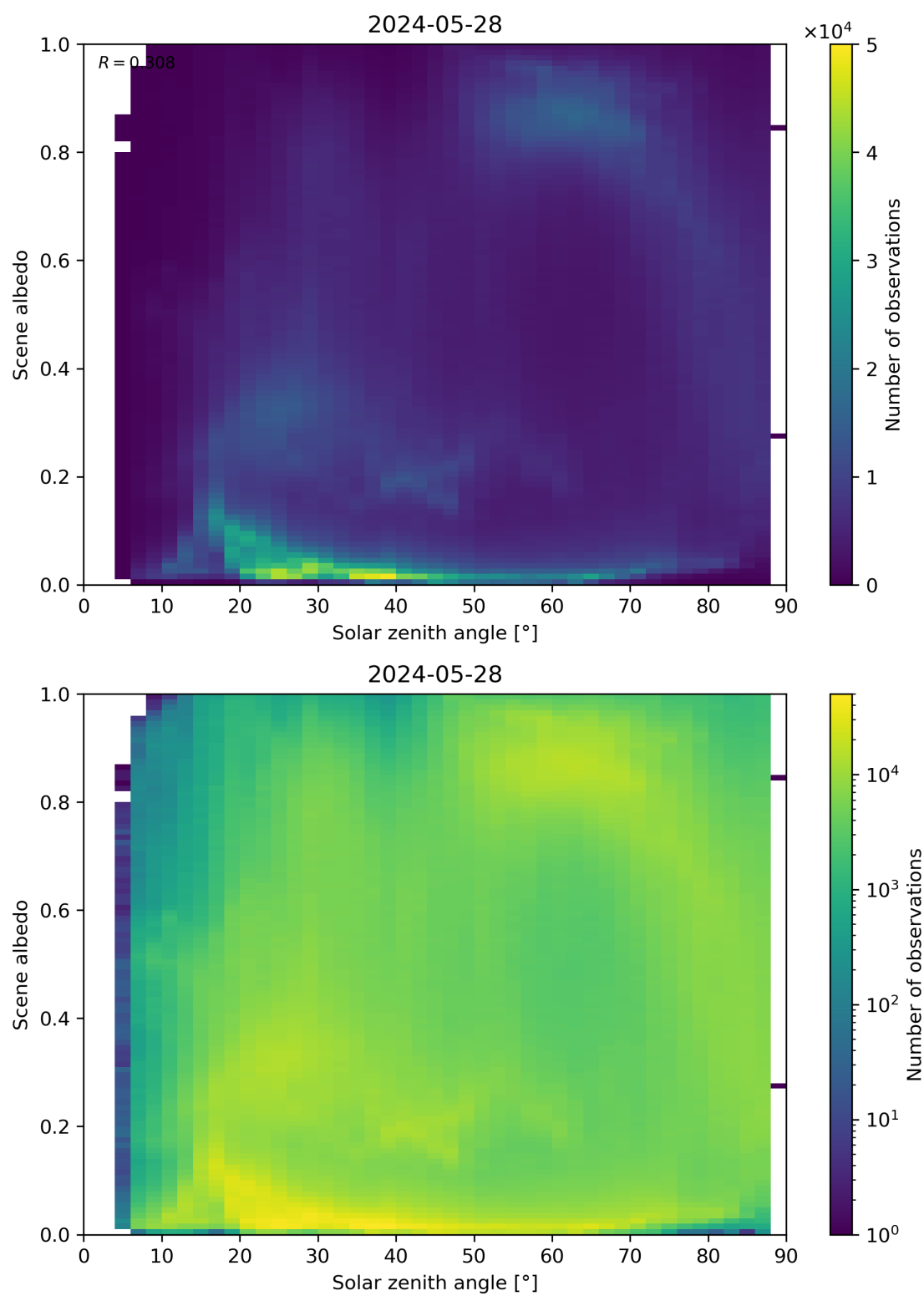
Figure 116: Scatter density plot of “Solar zenith angle” against “Scene albedo” for 2024-05-28 to 2024-05-29.
