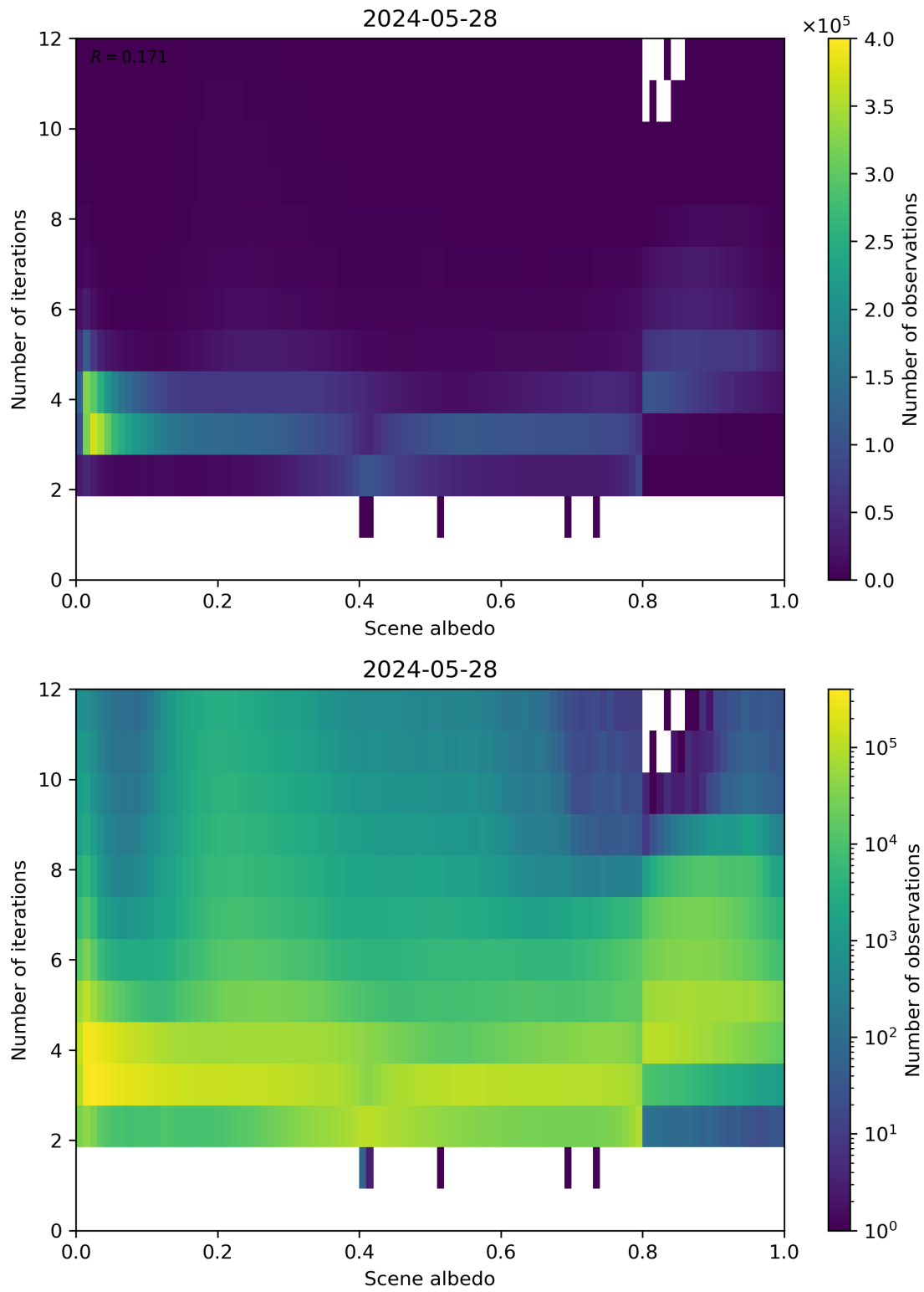
Figure 105: Scatter density plot of “Scene albedo” against “Number of iterations” for 2024-05-28 to 2024-05-29.
