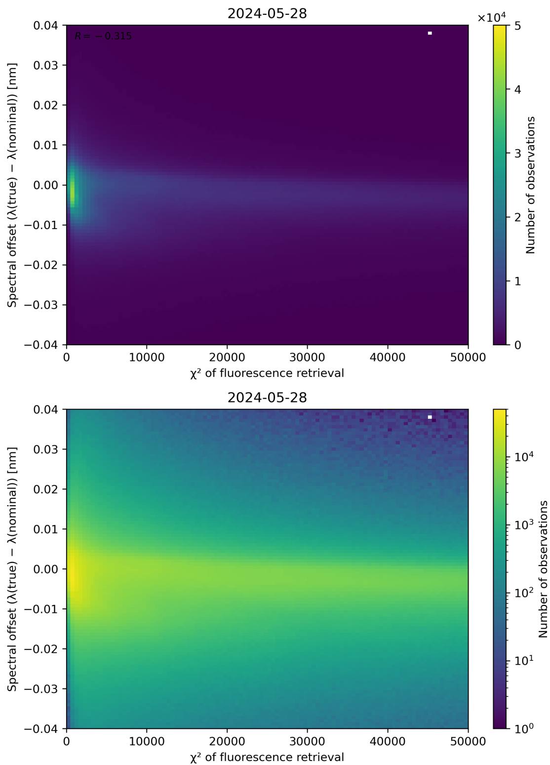
Figure 69: Scatter density plot of " \chi^2 of fluorescence retrieval" against "Spectral offset ( \lambda(\text{true}) - \lambda(\text{nominal}) )" for 2024-05-28 to 2024-05-29.
