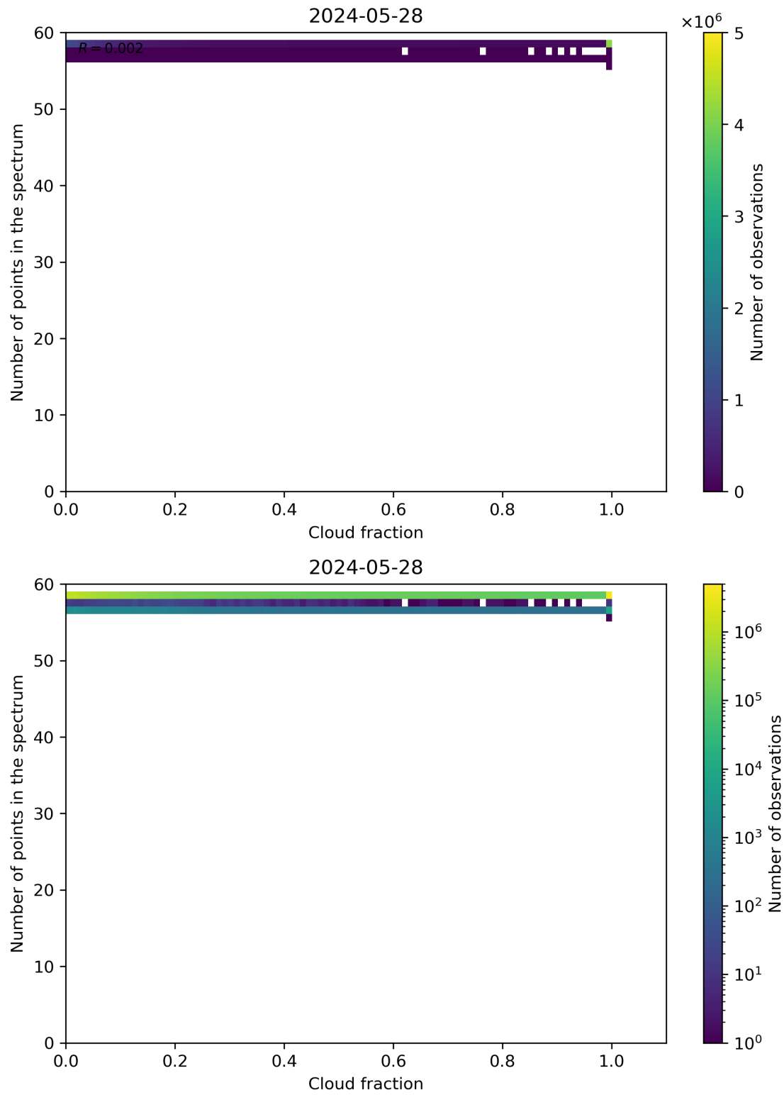
Figure 74: Scatter density plot of “Cloud fraction” against “Number of points in the spectrum” for 2024-05-28 to 2024-05-29.
