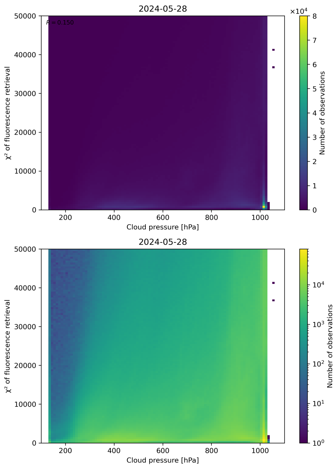
Figure 78: Scatter density plot of “Cloud pressure” against “ \chi^2 of fluorescence retrieval” for 2024-05-28 to 2024-05-29.
