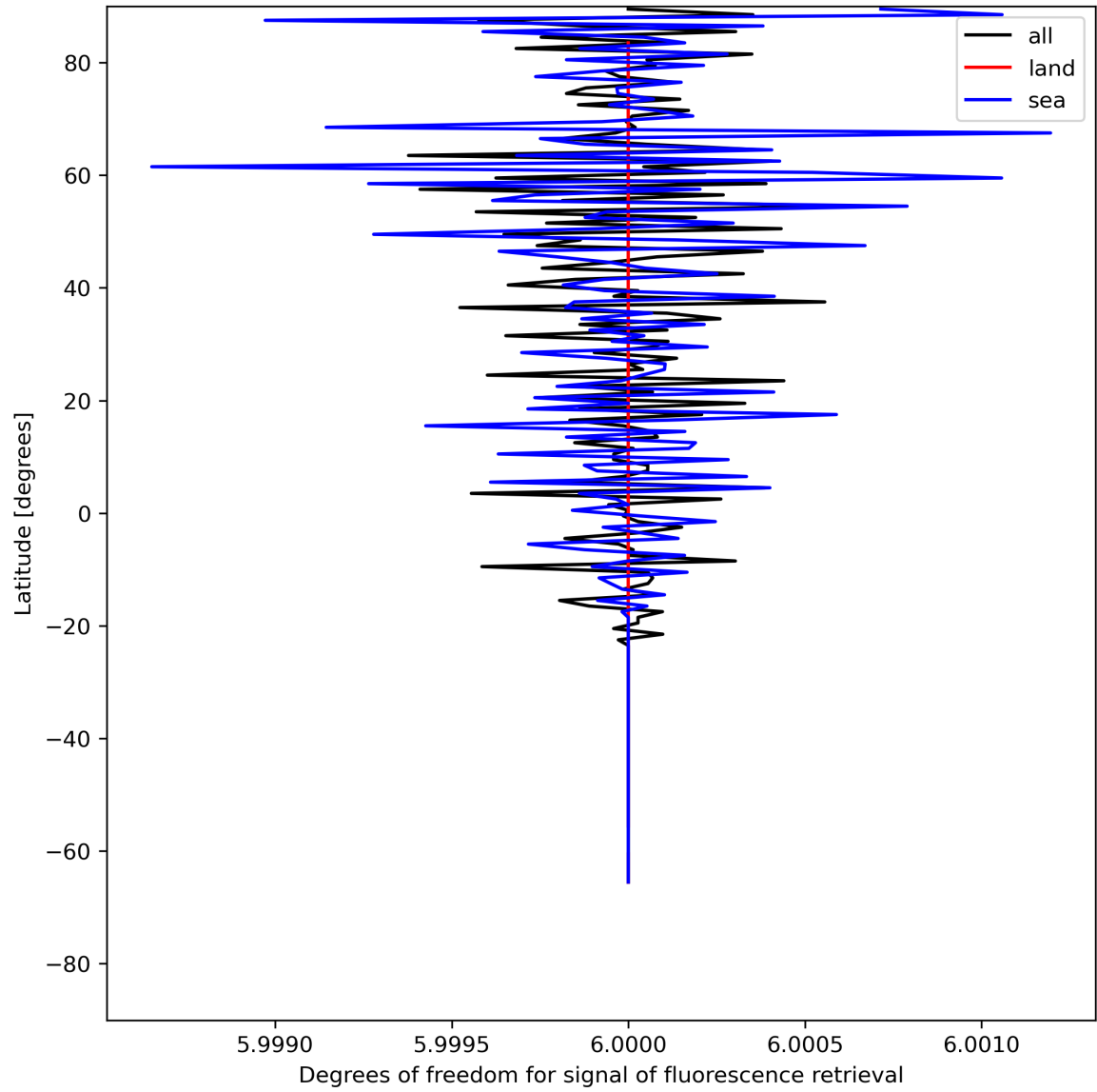
Figure 26: Zonal average of “Degrees of freedom for signal of fluorescence retrieval” for 2024-05-28 to 2024-05-29.
