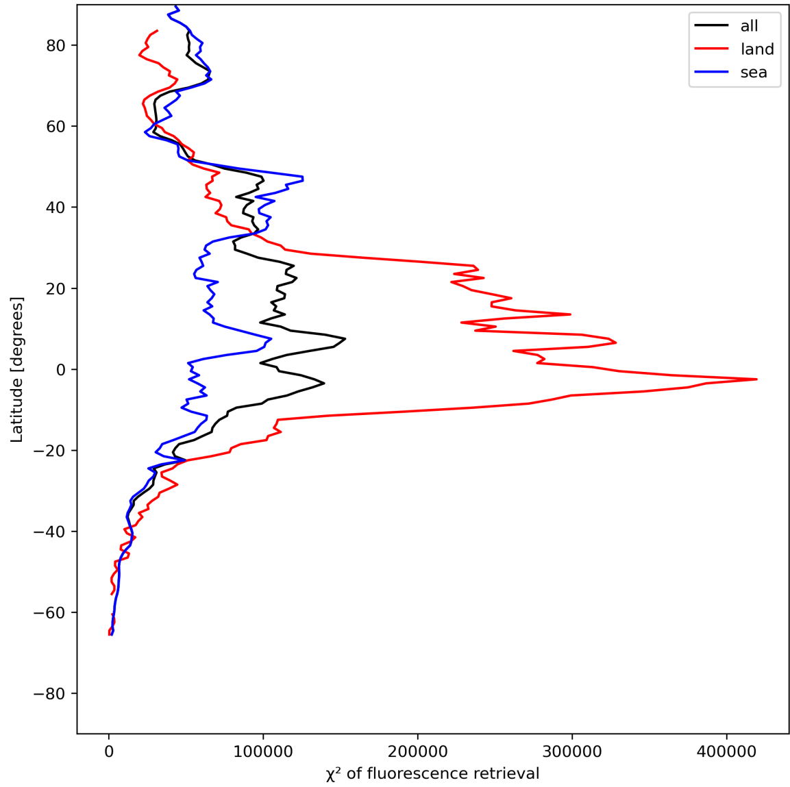
Figure 25: Zonal average of “ \chi^2 of fluorescence retrieval” for 2024-05-28 to 2024-05-29.
