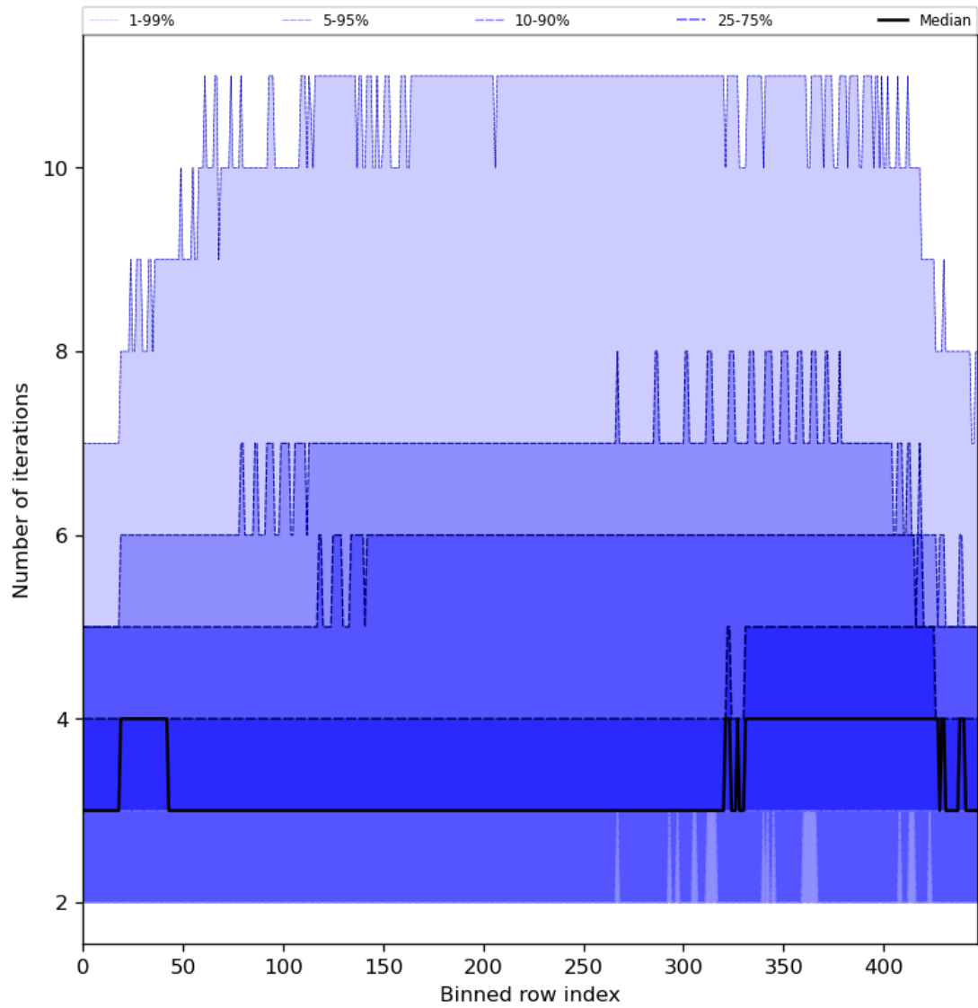
Figure 56: Along track statistics of “Number of iterations” for 2024-05-28 to 2024-05-29
