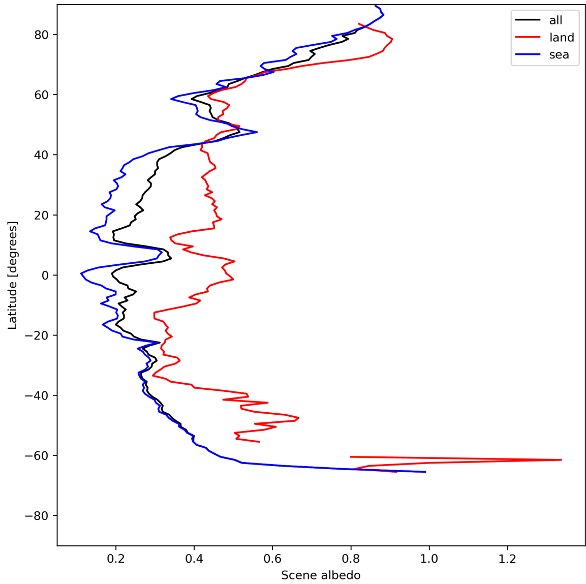
Figure 17: Zonal average of “Scene albedo” for 2024-05-28 to 2024-05-29.
