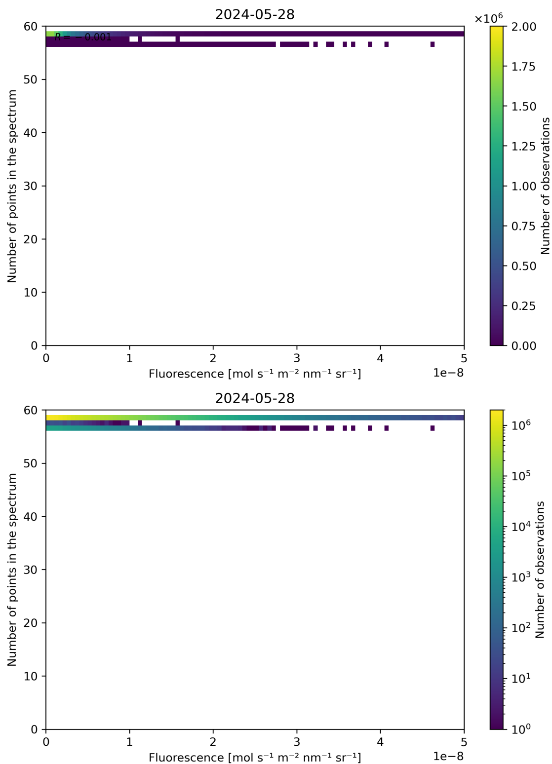
Figure 86: Scatter density plot of “Fluorescence” against “Number of points in the spectrum” for 2024-05-28 to 2024-05-29.
