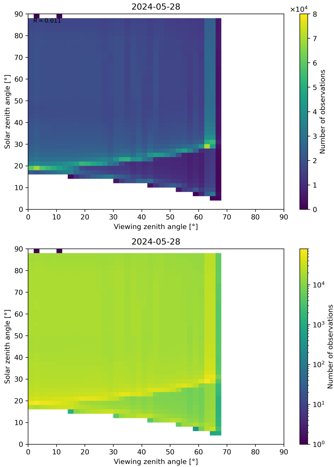
Figure 127: Scatter density plot of “Viewing zenith angle” against “Solar zenith angle” for 2024-05-28 to 2024-05-29.
