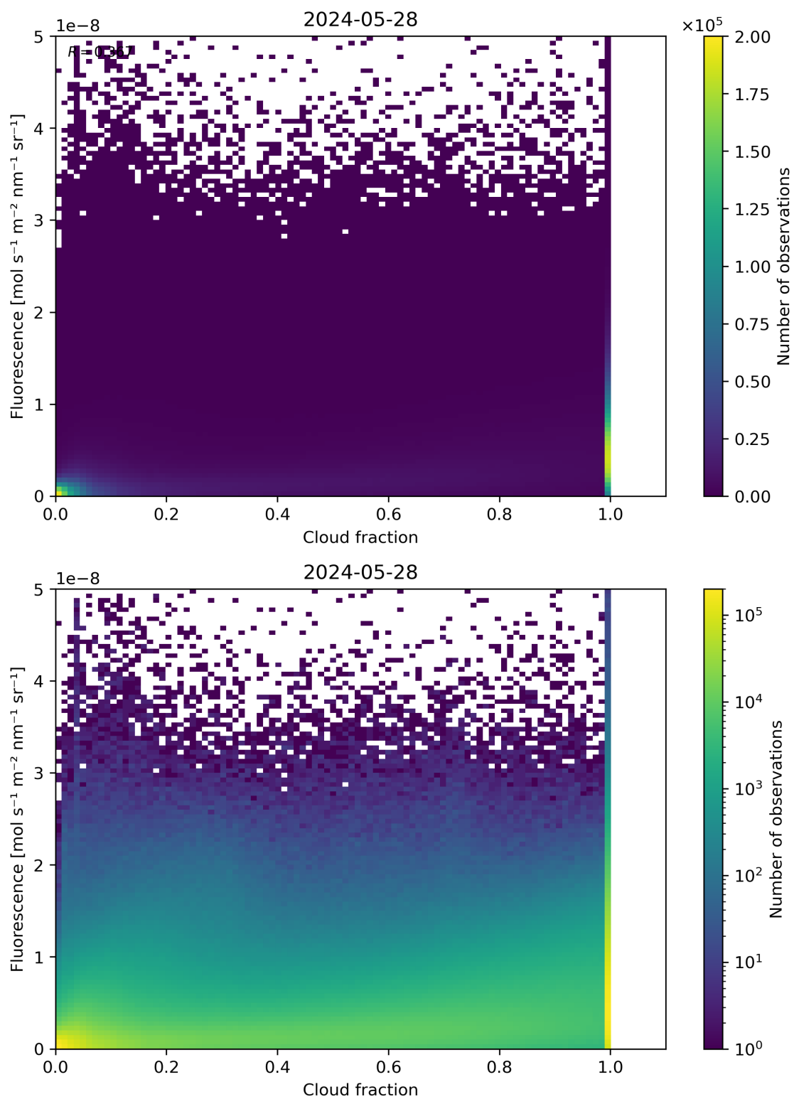
Figure 72: Scatter density plot of “Cloud fraction” against “Fluorescence” for 2024-05-28 to 2024-05-29.
