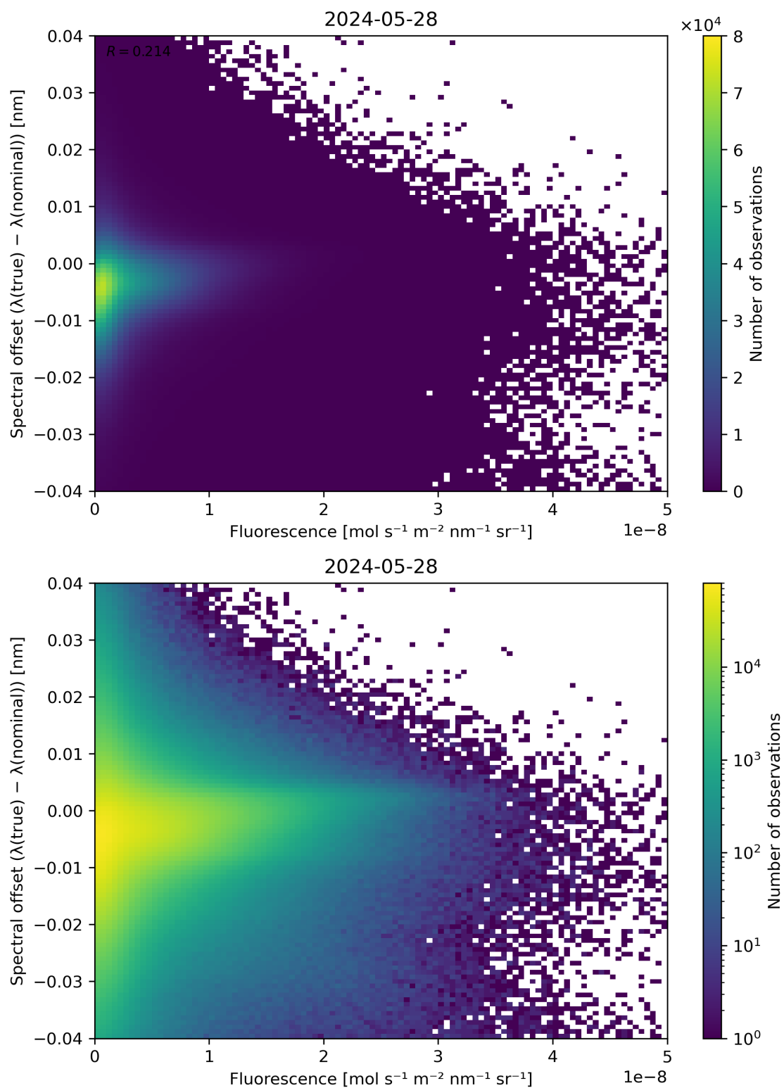
Figure 87: Scatter density plot of “Fluorescence” against “Spectral offset ( \lambda(\text{true}) - \lambda(\text{nominal}) )” for 2024-05-28 to 2024-05-29.
