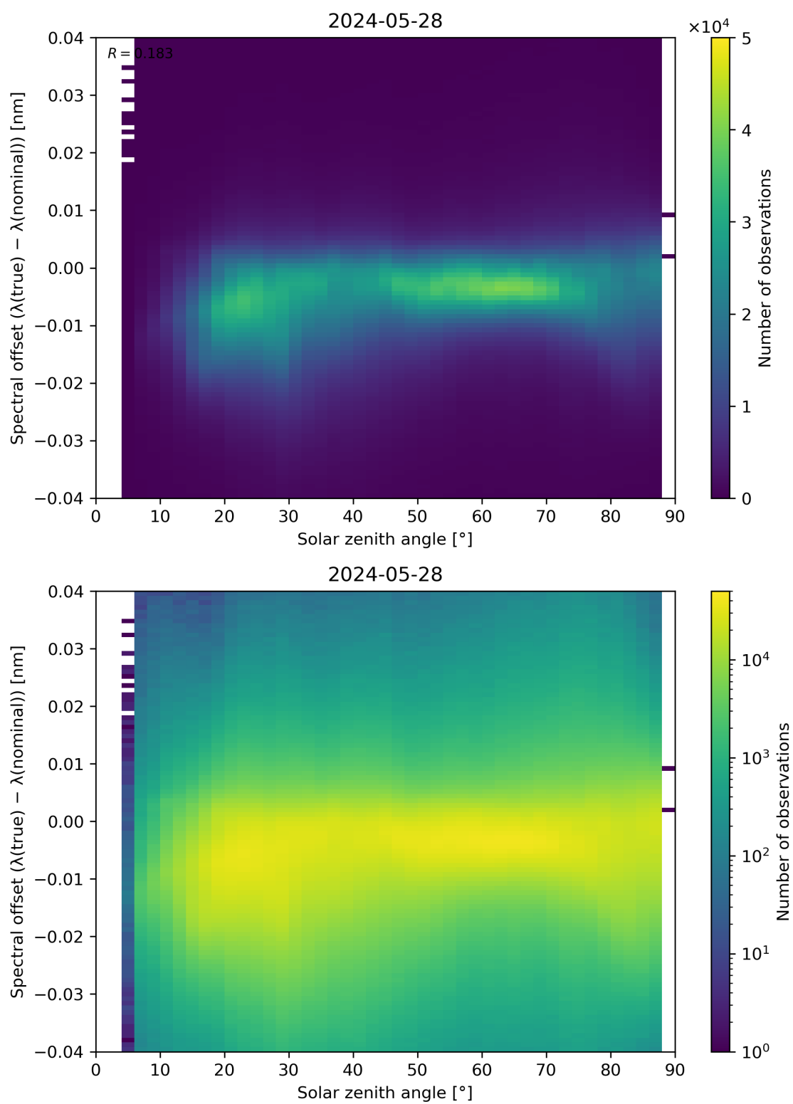
Figure 117: Scatter density plot of “Solar zenith angle” against “Spectral offset ( \lambda(\text{true}) - \lambda(\text{nominal}) )” for 2024-05-28 to 2024-05-29.
