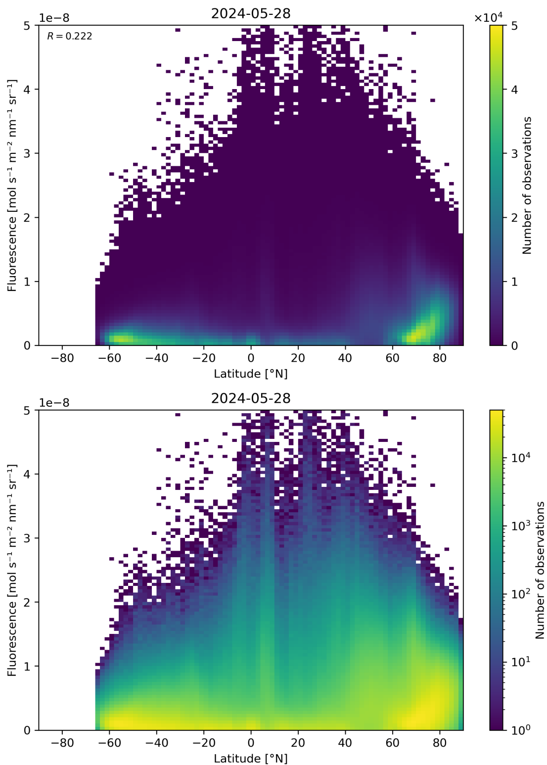
Figure 92: Scatter density plot of “Latitude” against “Fluorescence” for 2024-05-28 to 2024-05-29.
