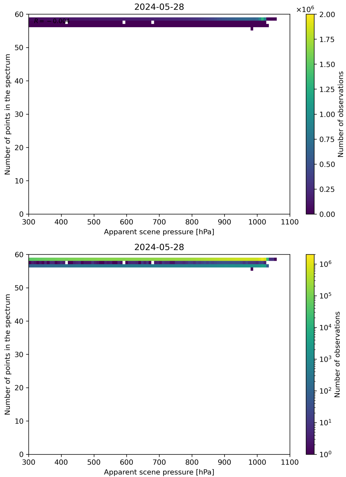
Figure 66: Scatter density plot of “Apparent scene pressure” against “Number of points in the spectrum” for 2024-05-28 to 2024-05-29.
