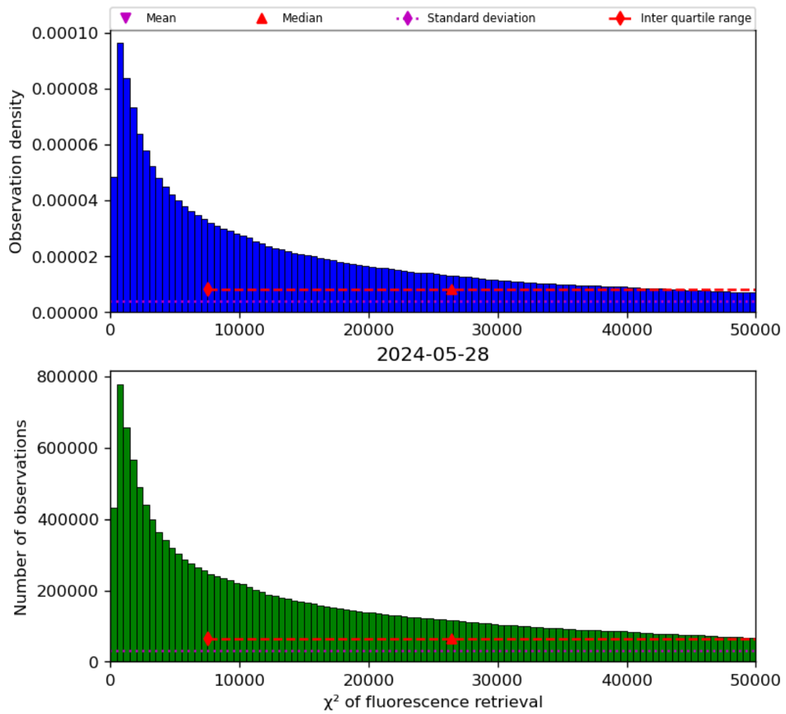
Figure 42: Histogram of “ \chi^2 of fluorescence retrieval” for 2024-05-28 to 2024-05-29
