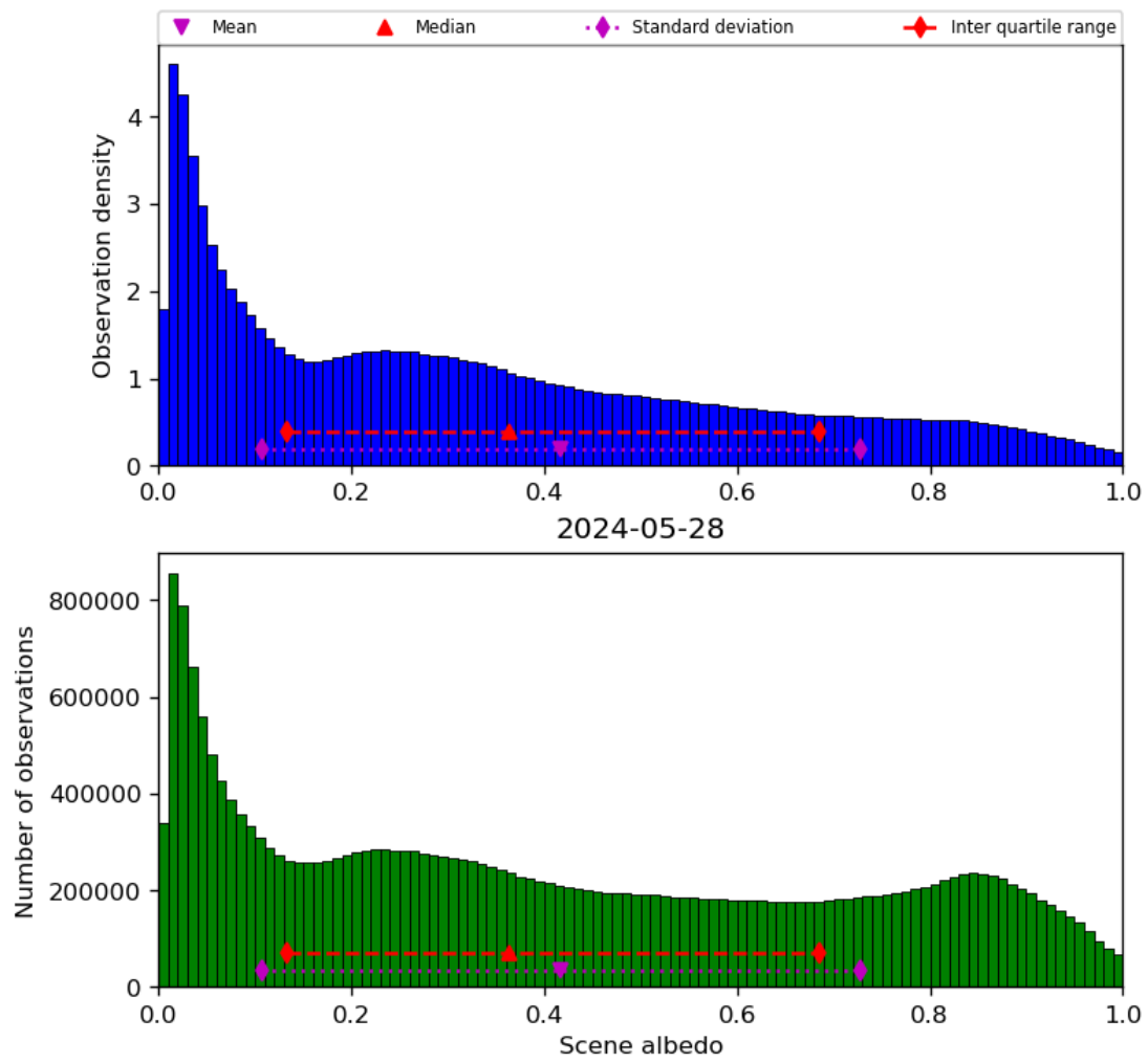
Figure 34: Histogram of “Scene albedo” for 2024-05-28 to 2024-05-29
