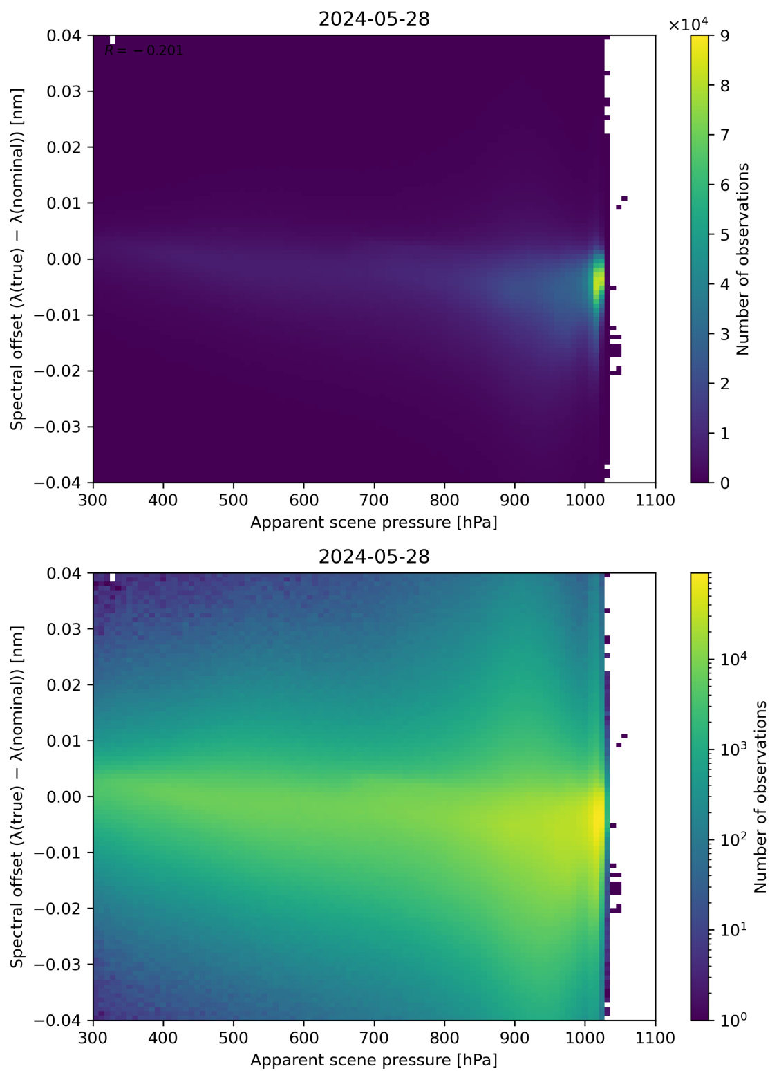
Figure 67: Scatter density plot of “Apparent scene pressure” against “Spectral offset ( \lambda(\text{true}) - \lambda(\text{nominal}) )” for 2024-05-28 to 2024-05-29.
