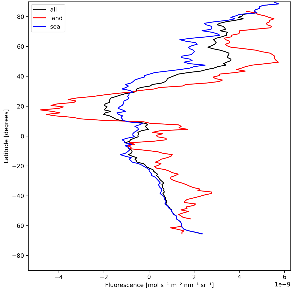
Figure 23: Zonal average of “Fluorescence” for 2024-05-28 to 2024-05-29.
