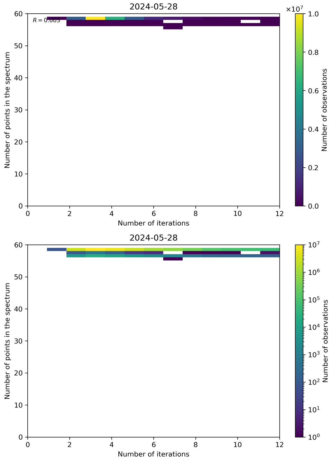
Figure 99: Scatter density plot of “Number of iterations” against “Number of points in the spectrum” for 2024-05-28 to 2024-05-29.
