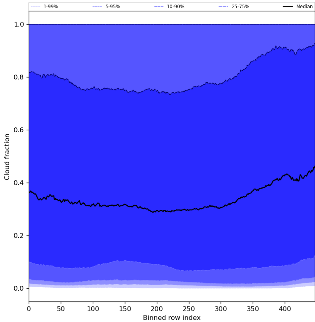
Figure 49: Along track statistics of “Cloud fraction” for 2024-05-28 to 2024-05-29
