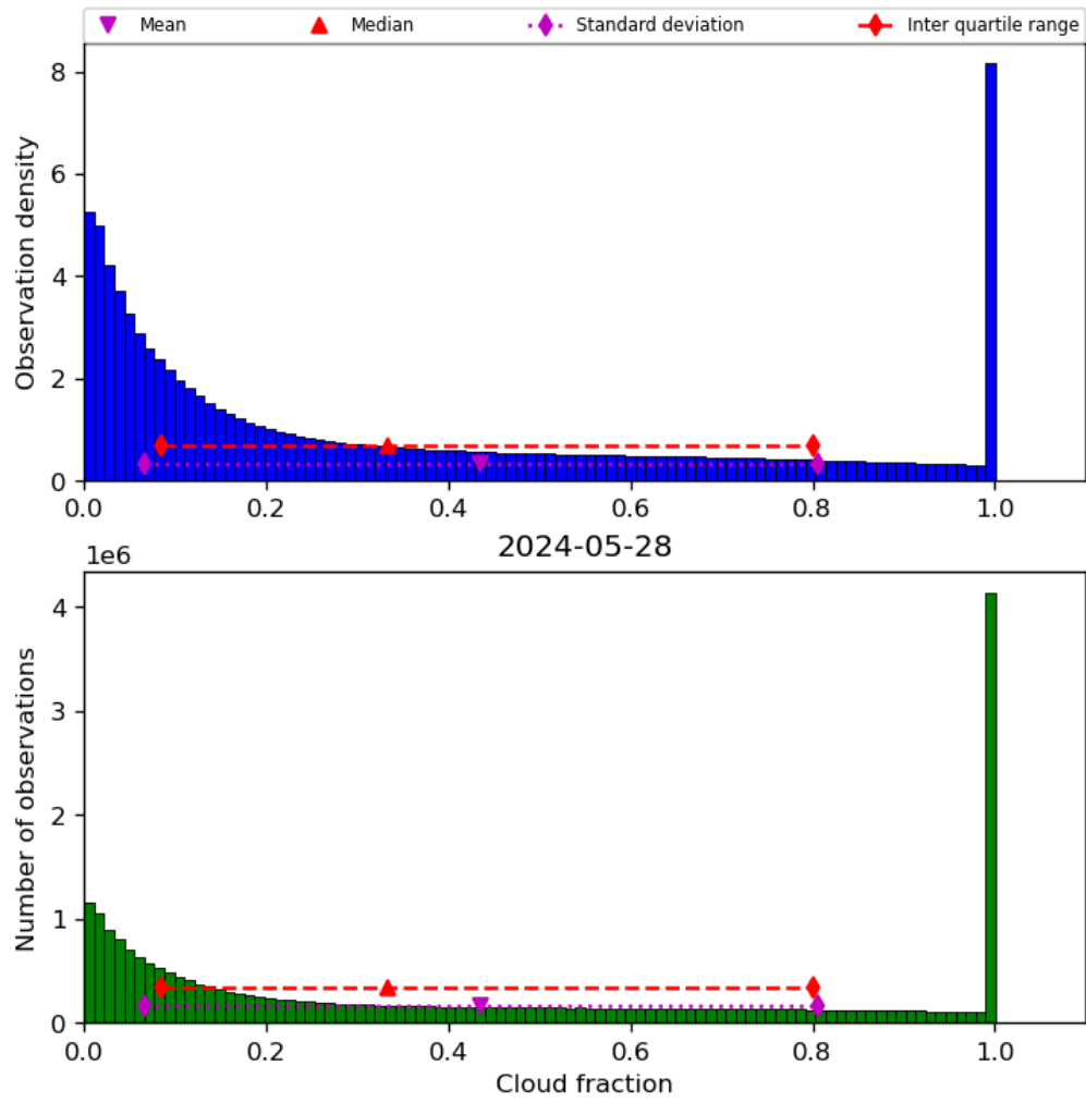
Figure 32: Histogram of “Cloud fraction” for 2024-05-28 to 2024-05-29
