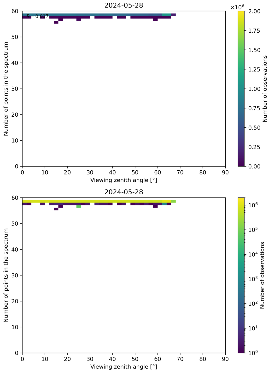
Figure 125: Scatter density plot of “Viewing zenith angle” against “Number of points in the spectrum” for 2024-05-28 to 2024-05-29.
