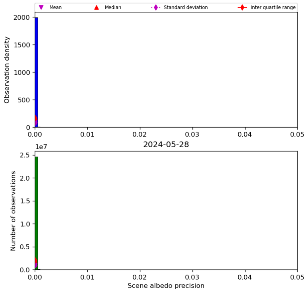
Figure 35: Histogram of “Scene albedo precision” for 2024-05-28 to 2024-05-29
