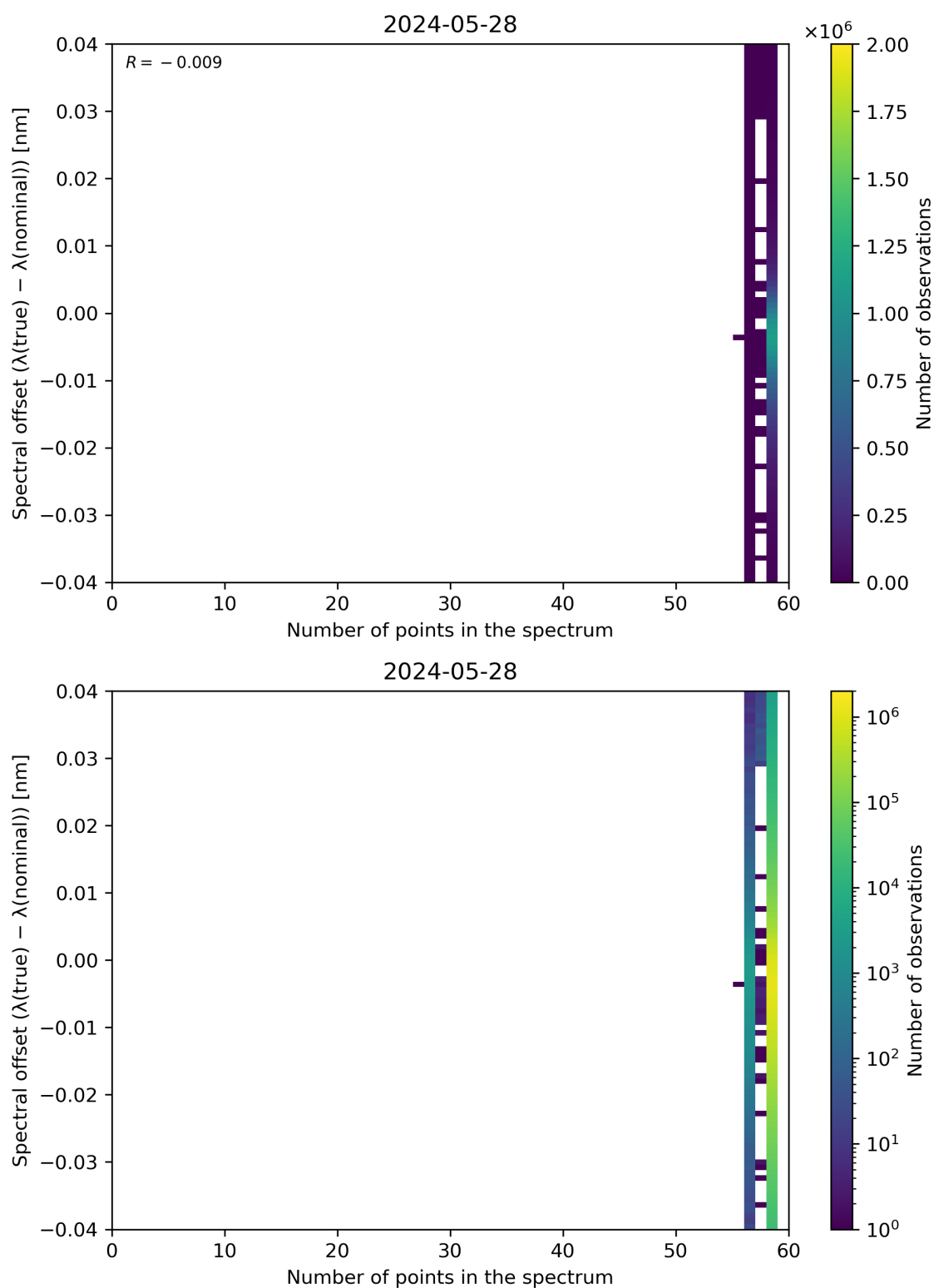
Figure 101: Scatter density plot of “Number of points in the spectrum” against “Spectral offset ( \lambda(\text{true}) - \lambda(\text{nominal}) )” for 2024-05-28 to 2024-05-29.
