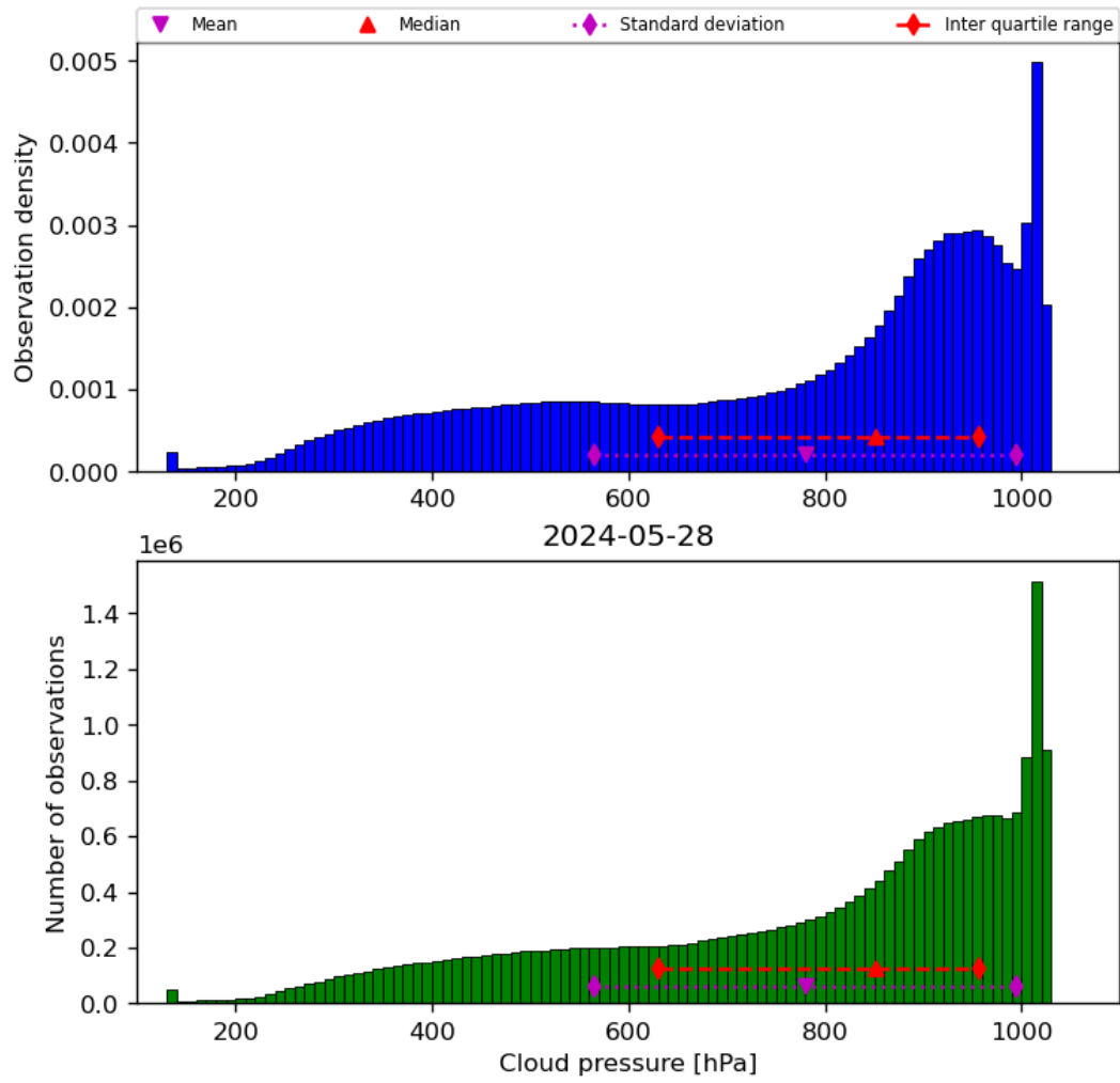
Figure 30: Histogram of “Cloud pressure” for 2024-05-28 to 2024-05-29
