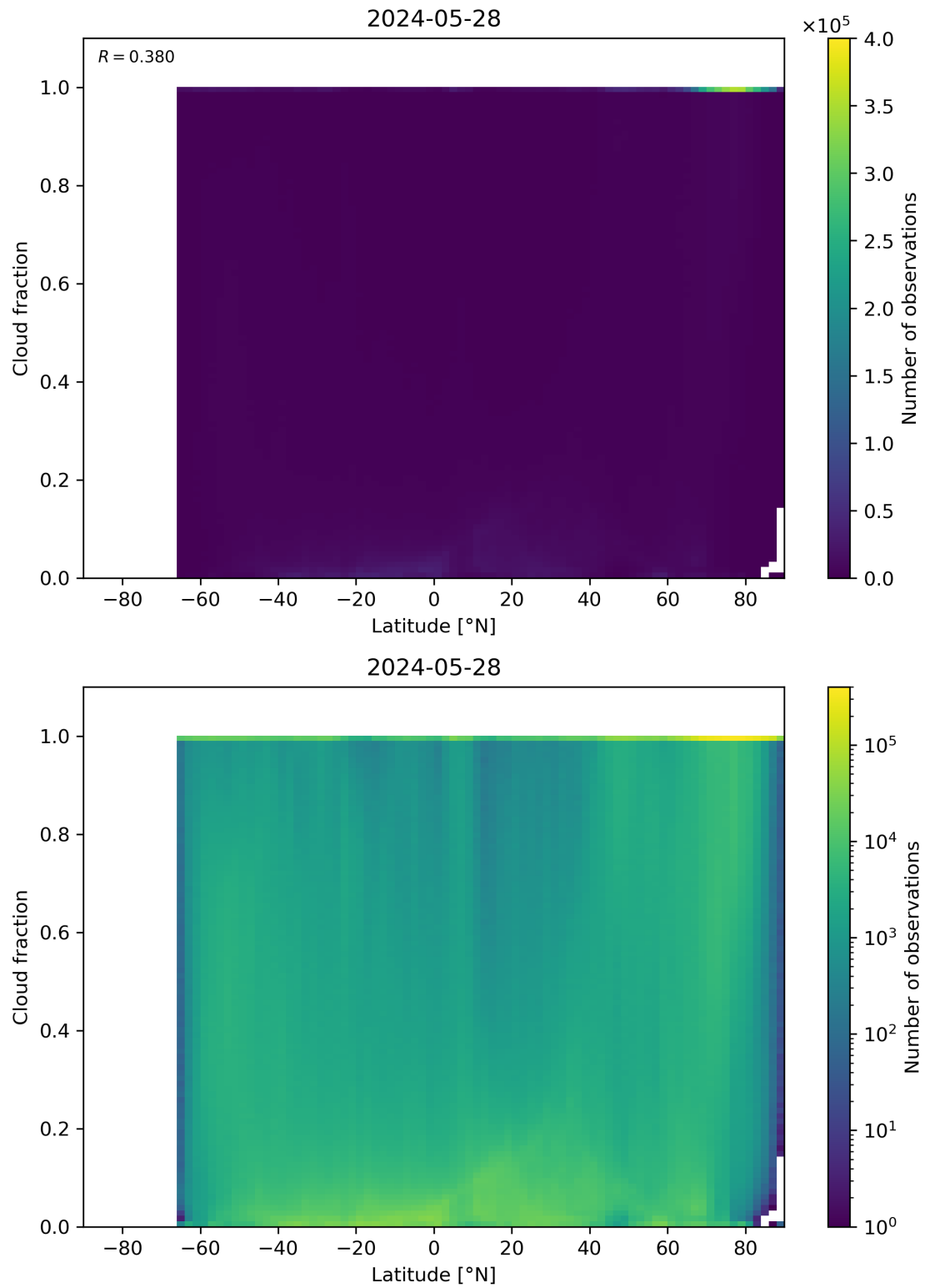
Figure 90: Scatter density plot of “Latitude” against “Cloud fraction” for 2024-05-28 to 2024-05-29.
