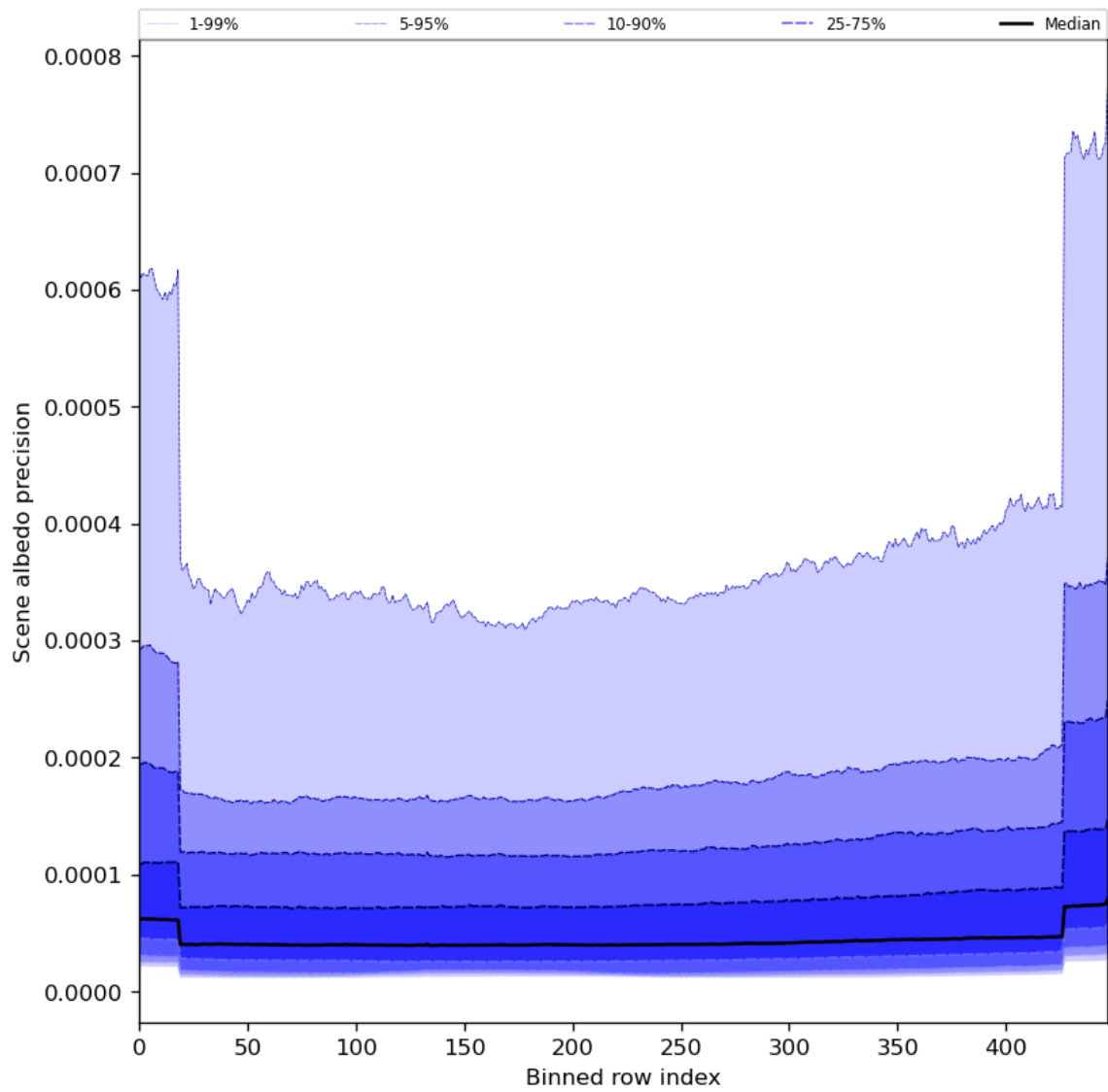
Figure 52: Along track statistics of “Scene albedo precision” for 2024-05-28 to 2024-05-29
