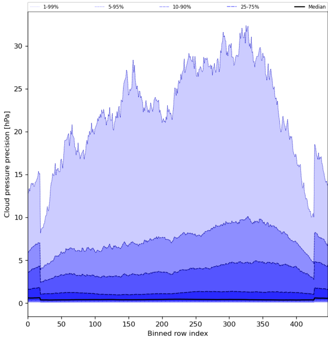
Figure 48: Along track statistics of “Cloud pressure precision” for 2024-05-28 to 2024-05-29
