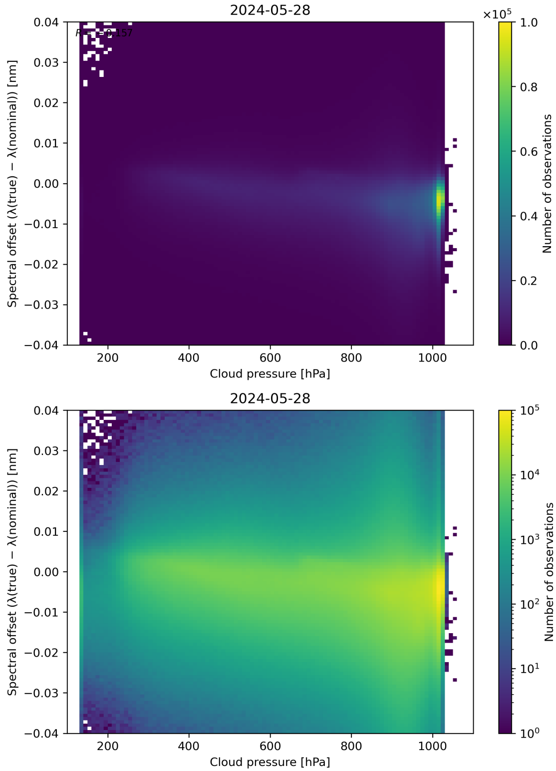
Figure 84: Scatter density plot of “Cloud pressure” against “Spectral offset ( \lambda(\text{true}) - \lambda(\text{nominal}) )” for 2024-05-28 to 2024-05-29.
