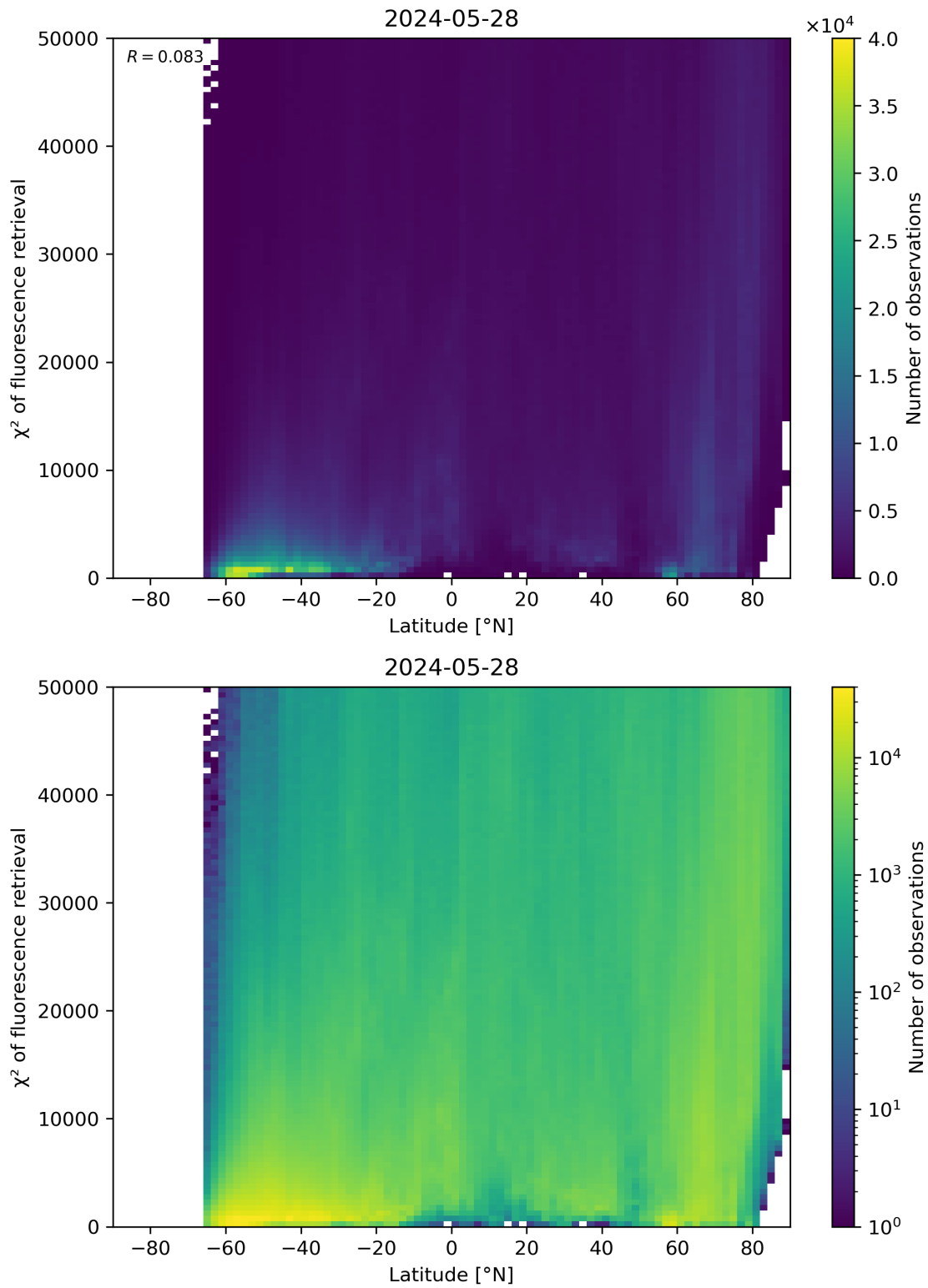
Figure 89: Scatter density plot of “Latitude” against “ \chi^2 of fluorescence retrieval” for 2024-05-28 to 2024-05-29.
