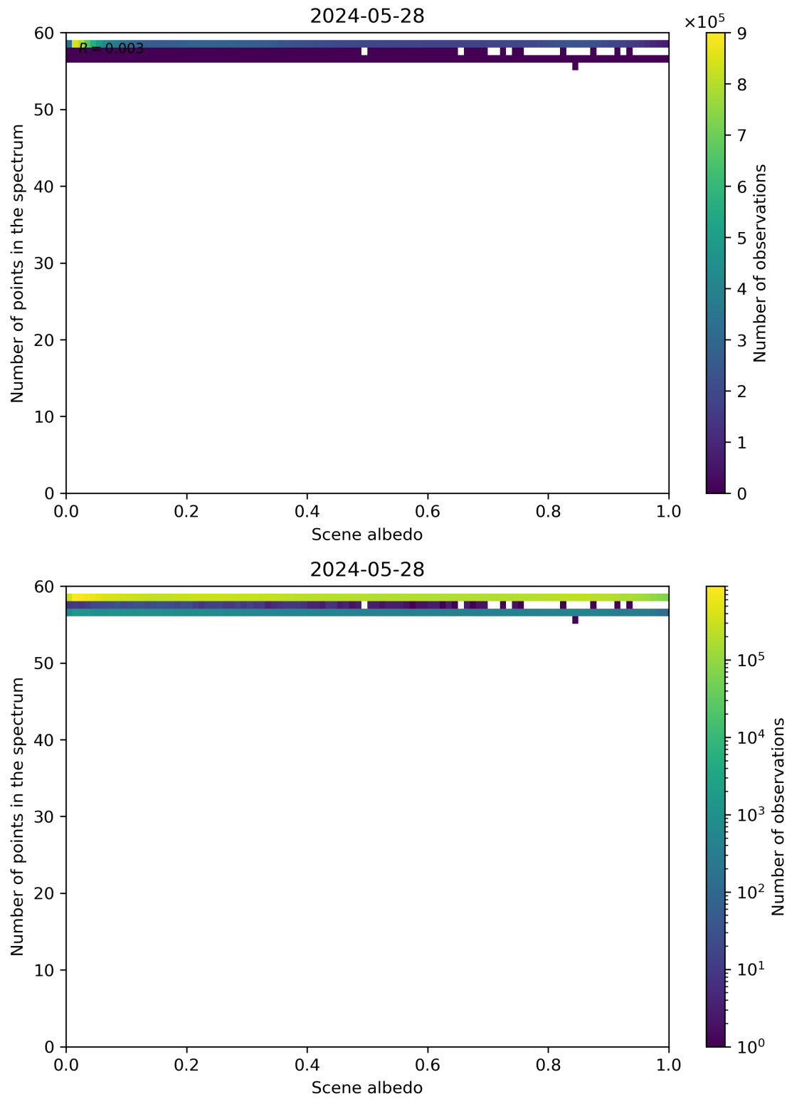
Figure 106: Scatter density plot of “Scene albedo” against “Number of points in the spectrum” for 2024-05-28 to 2024-05-29.
