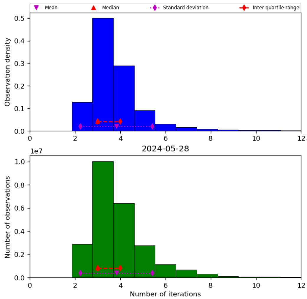
Figure 39: Histogram of “Number of iterations” for 2024-05-28 to 2024-05-29
