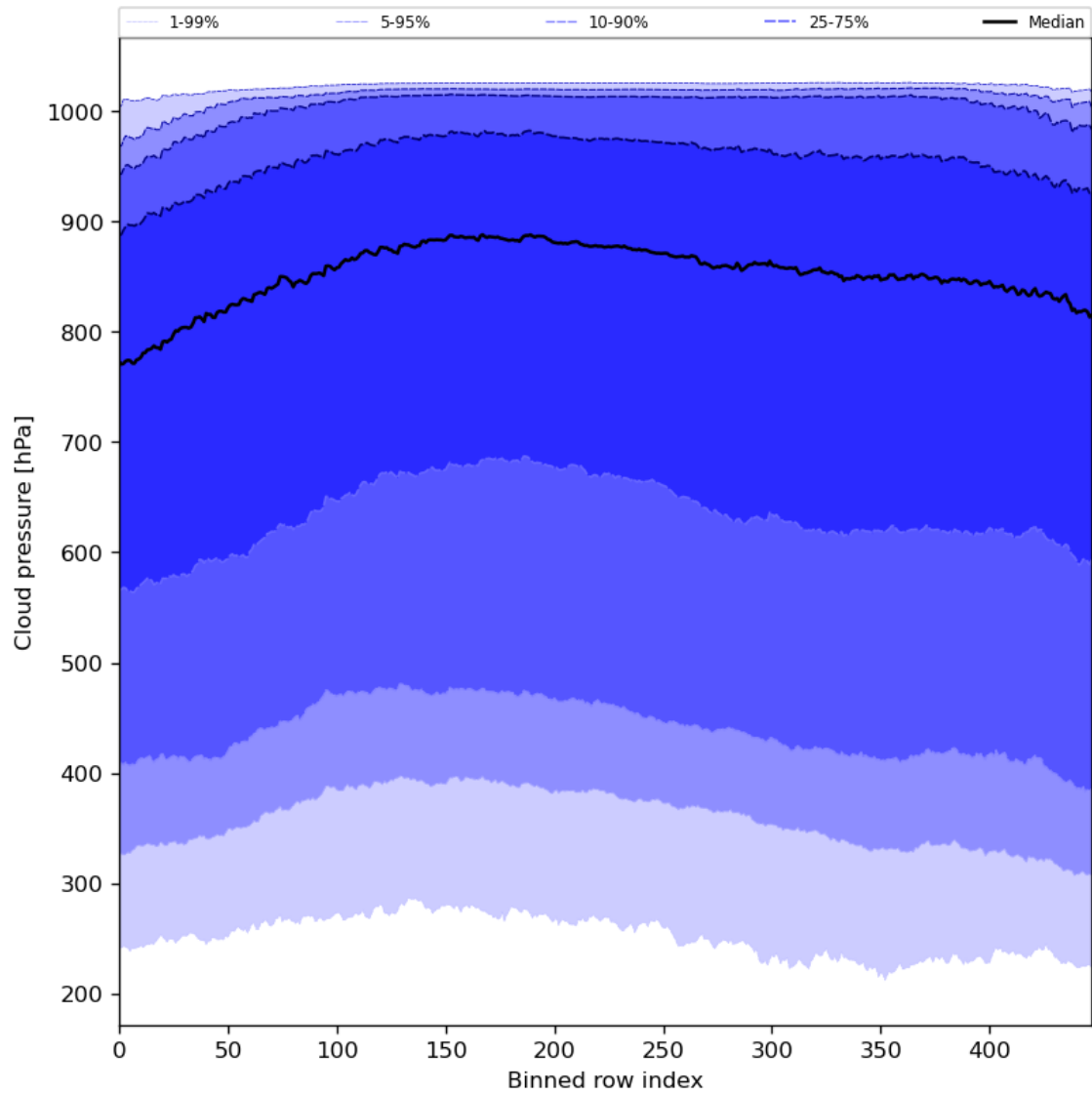
Figure 47: Along track statistics of “Cloud pressure” for 2024-05-28 to 2024-05-29
