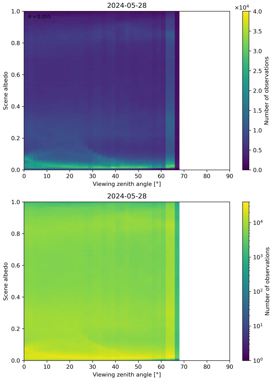
Figure 126: Scatter density plot of “Viewing zenith angle” against “Scene albedo” for 2024-05-28 to 2024-05-29.
