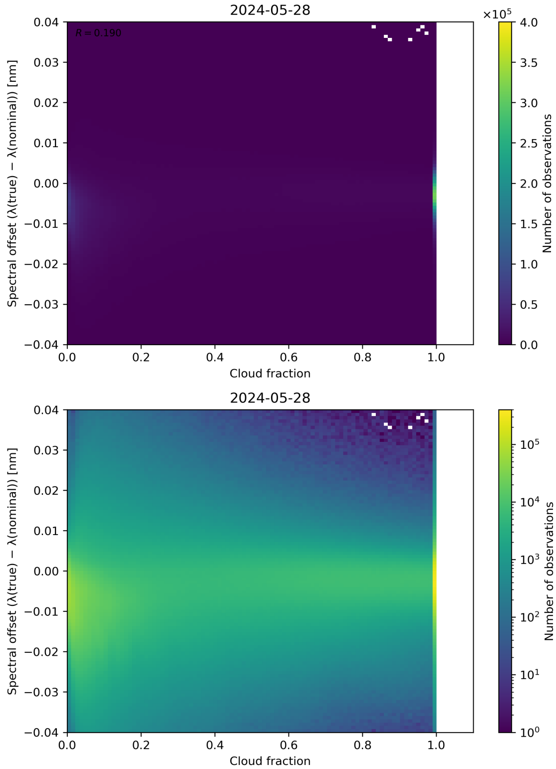
Figure 76: Scatter density plot of “Cloud fraction” against “Spectral offset ( \lambda(\text{true}) - \lambda(\text{nominal}) )” for 2024-05-28 to 2024-05-29.
