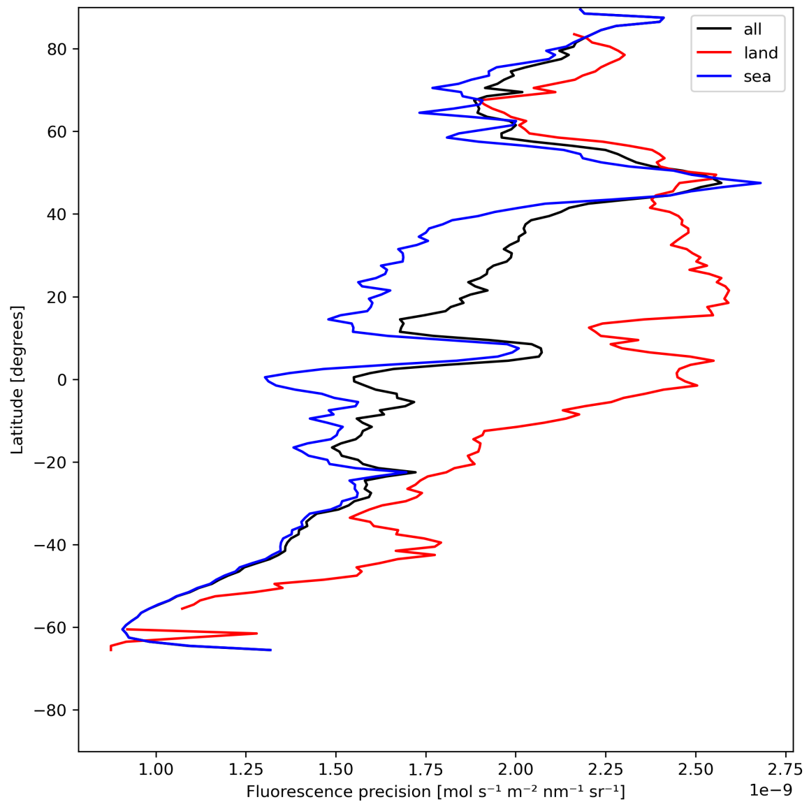
Figure 24: Zonal average of “Fluorescence precision” for 2024-05-28 to 2024-05-29.
