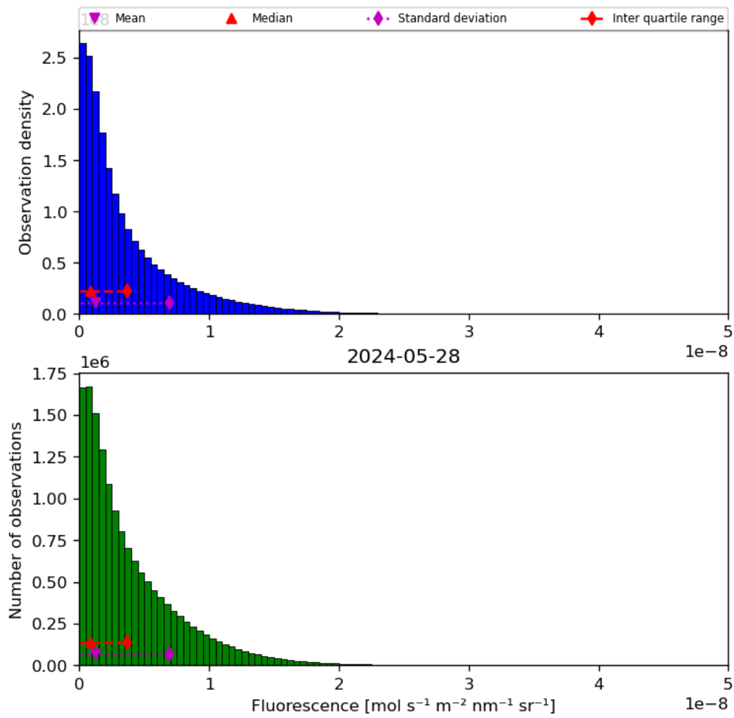
Figure 40: Histogram of “Fluorescence” for 2024-05-28 to 2024-05-29
