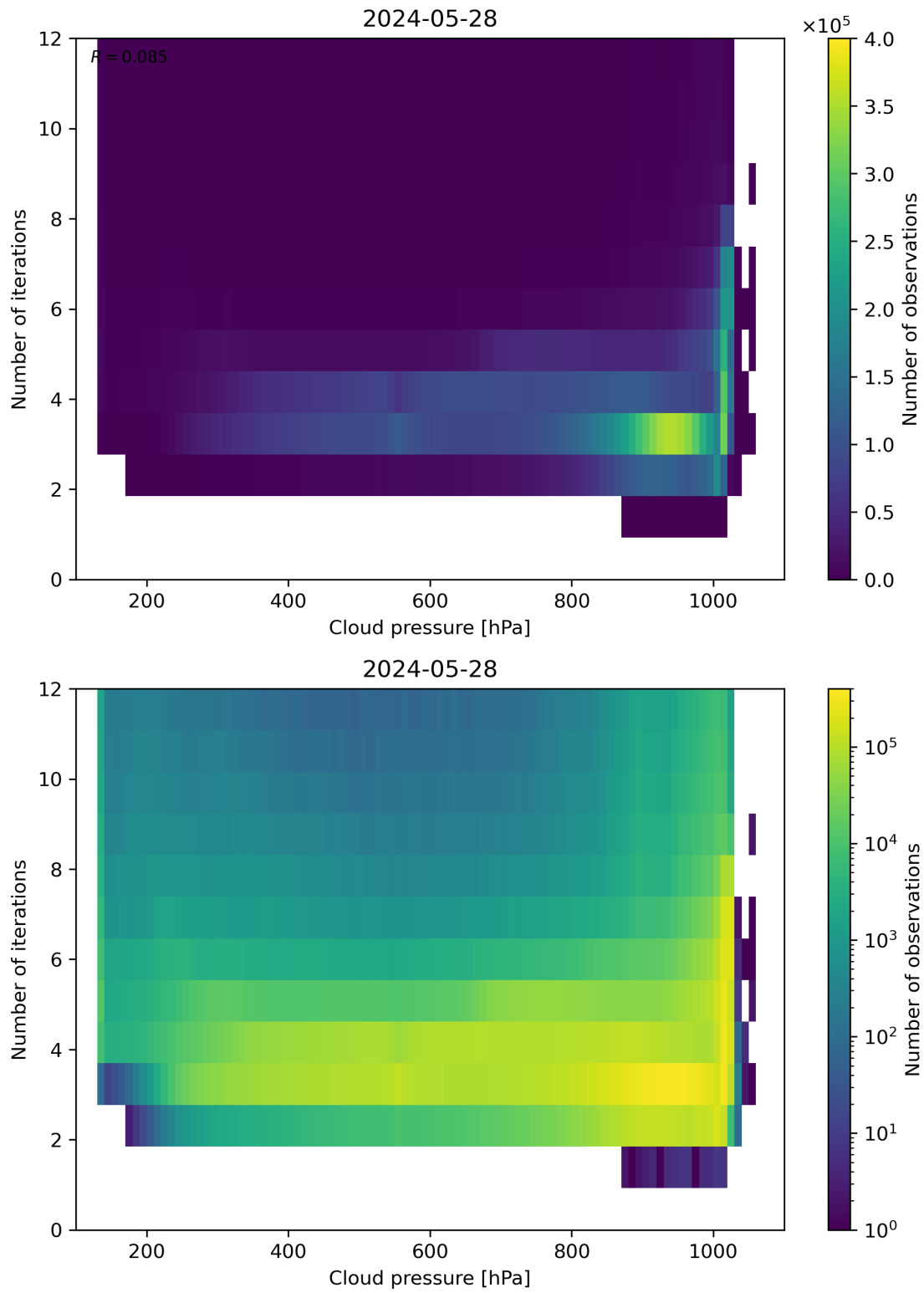
Figure 81: Scatter density plot of “Cloud pressure” against “Number of iterations” for 2024-05-28 to 2024-05-29.
