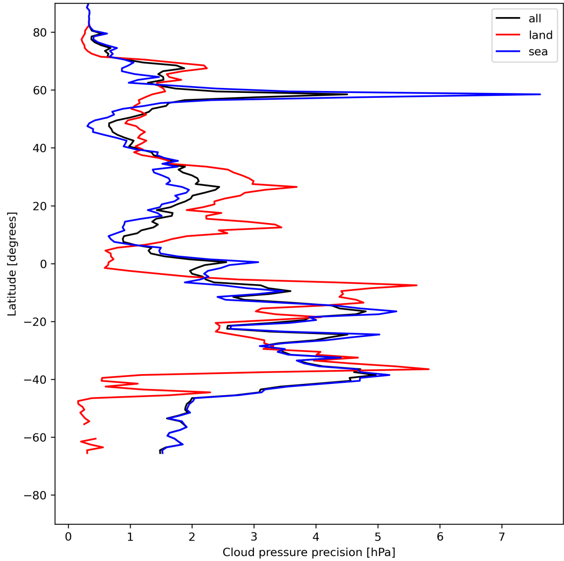
Figure 14: Zonal average of “Cloud pressure precision” for 2024-05-28 to 2024-05-29.
