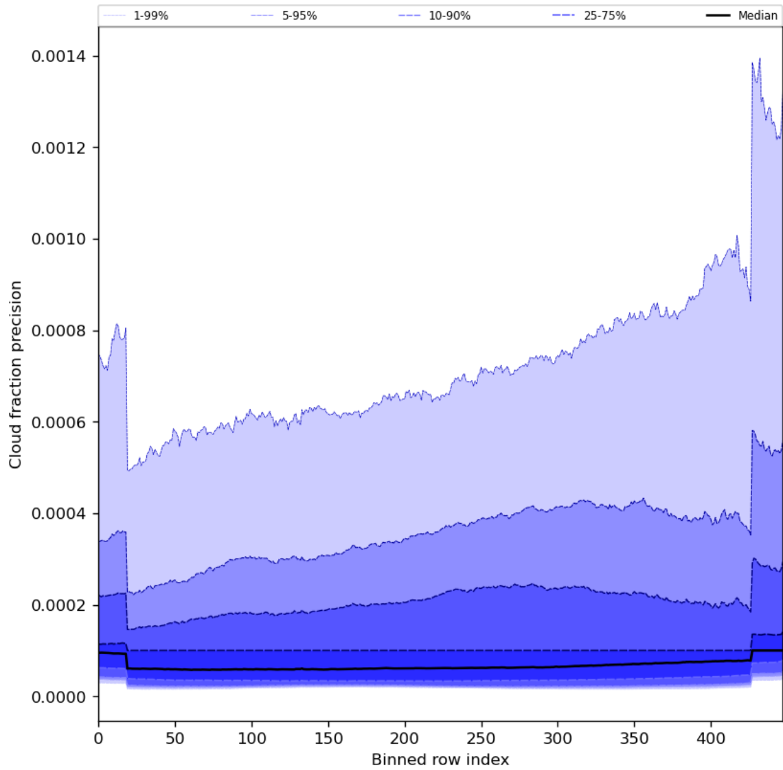
Figure 50: Along track statistics of “Cloud fraction precision” for 2024-05-28 to 2024-05-29
