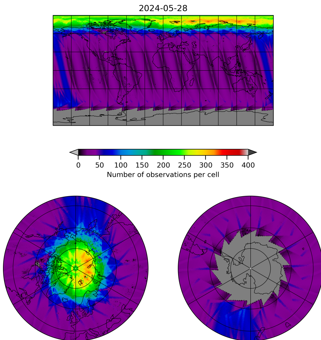
Figure 11: Map of the number of observations for 2024-05-28 to 2024-05-29
