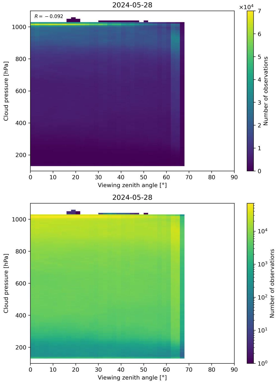
Figure 121: Scatter density plot of “Viewing zenith angle” against “Cloud pressure” for 2024-05-28 to 2024-05-29.
