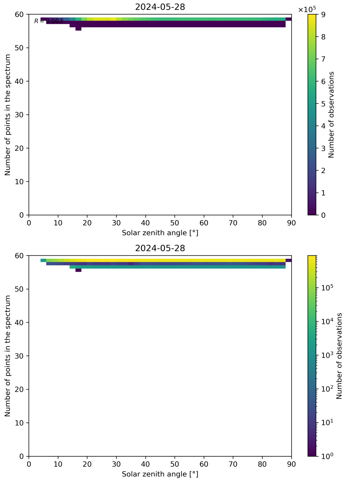
Figure 115: Scatter density plot of “Solar zenith angle” against “Number of points in the spectrum” for 2024-05-28 to 2024-05-29.
