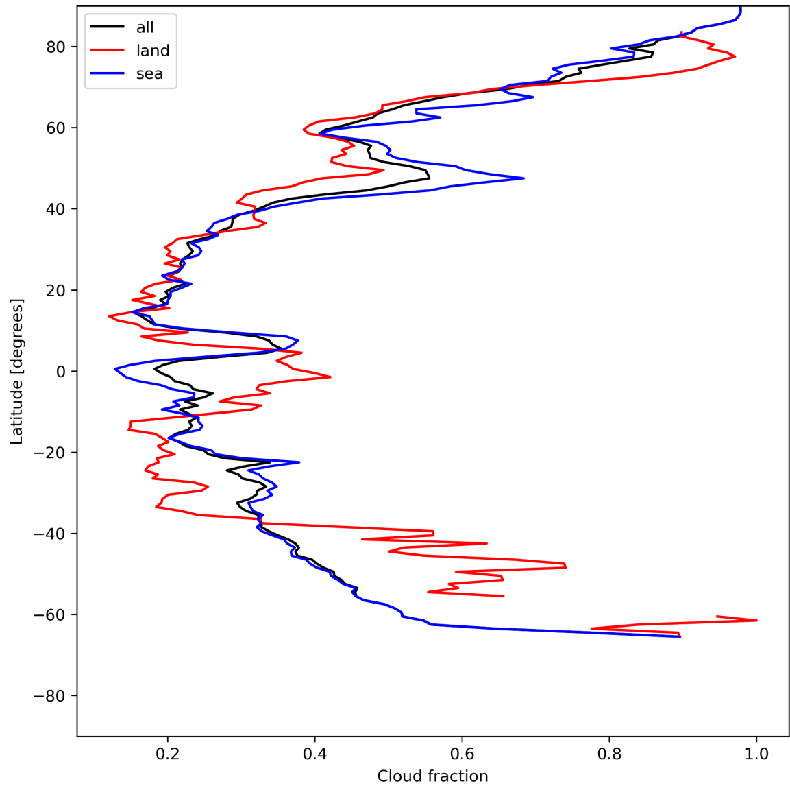
Figure 15: Zonal average of “Cloud fraction” for 2024-05-28 to 2024-05-29.
