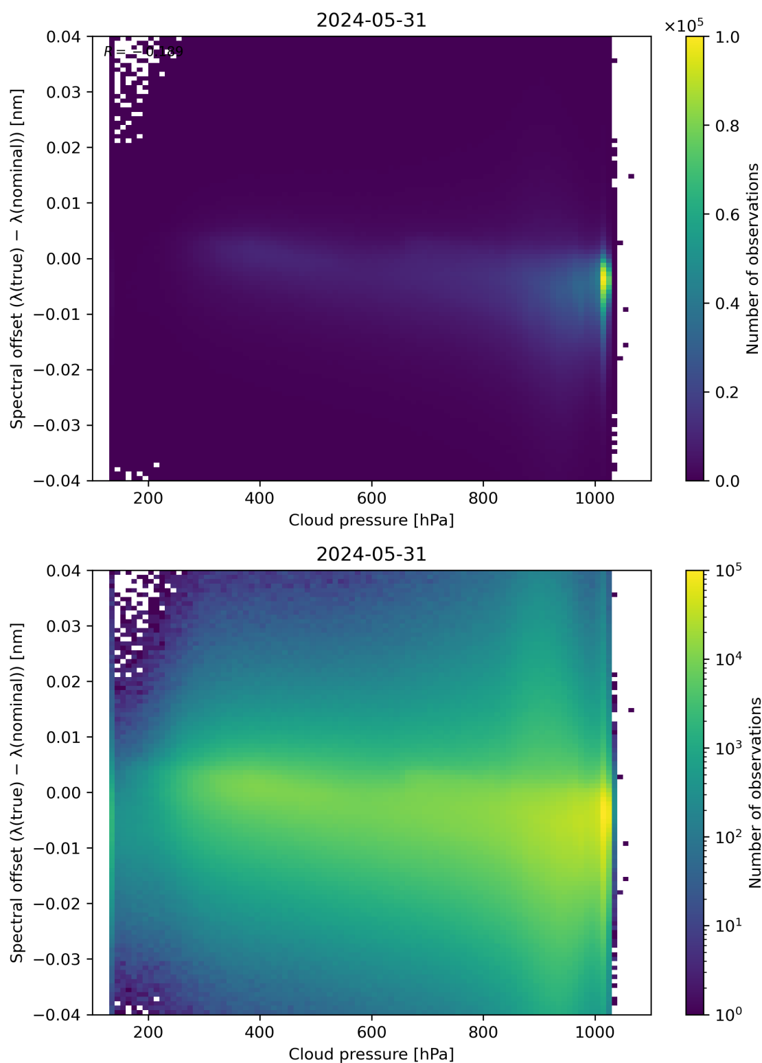
Figure 84: Scatter density plot of “Cloud pressure” against “Spectral offset ( \lambda(\text{true}) - \lambda(\text{nominal}) )” for 2024-05-30 to 2024-06-01.
