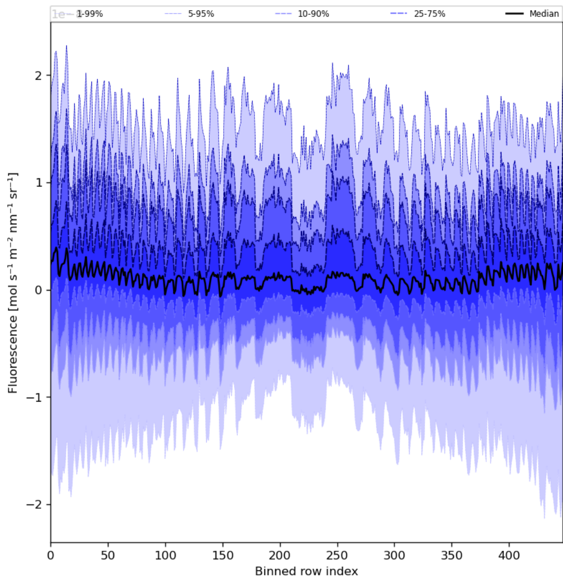
Figure 57: Along track statistics of “Fluorescence” for 2024-05-30 to 2024-06-01
