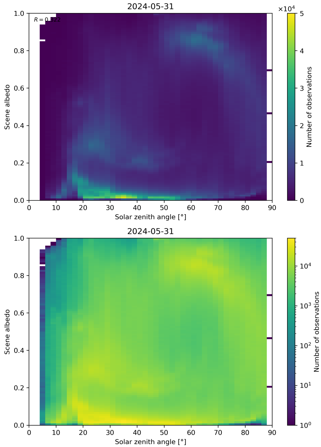
Figure 116: Scatter density plot of “Solar zenith angle” against “Scene albedo” for 2024-05-30 to 2024-06-01.
