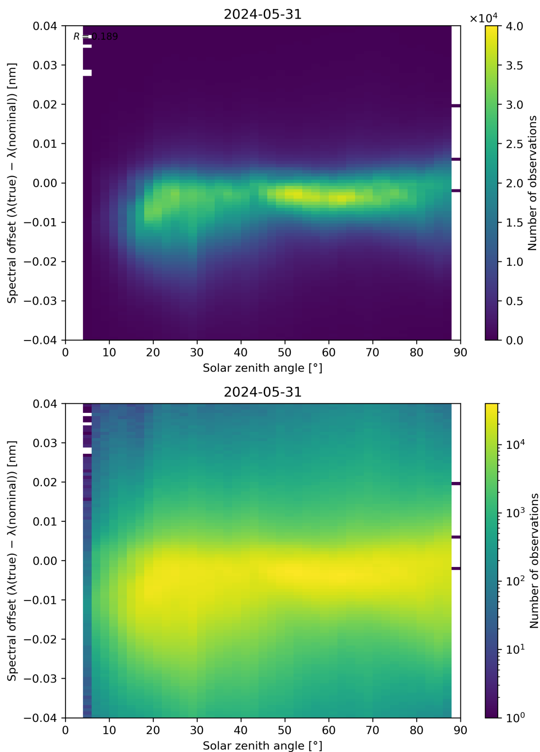
Figure 117: Scatter density plot of “Solar zenith angle” against “Spectral offset ( \lambda(\text{true}) - \lambda(\text{nominal}) )” for 2024-05-30 to 2024-06-01.
