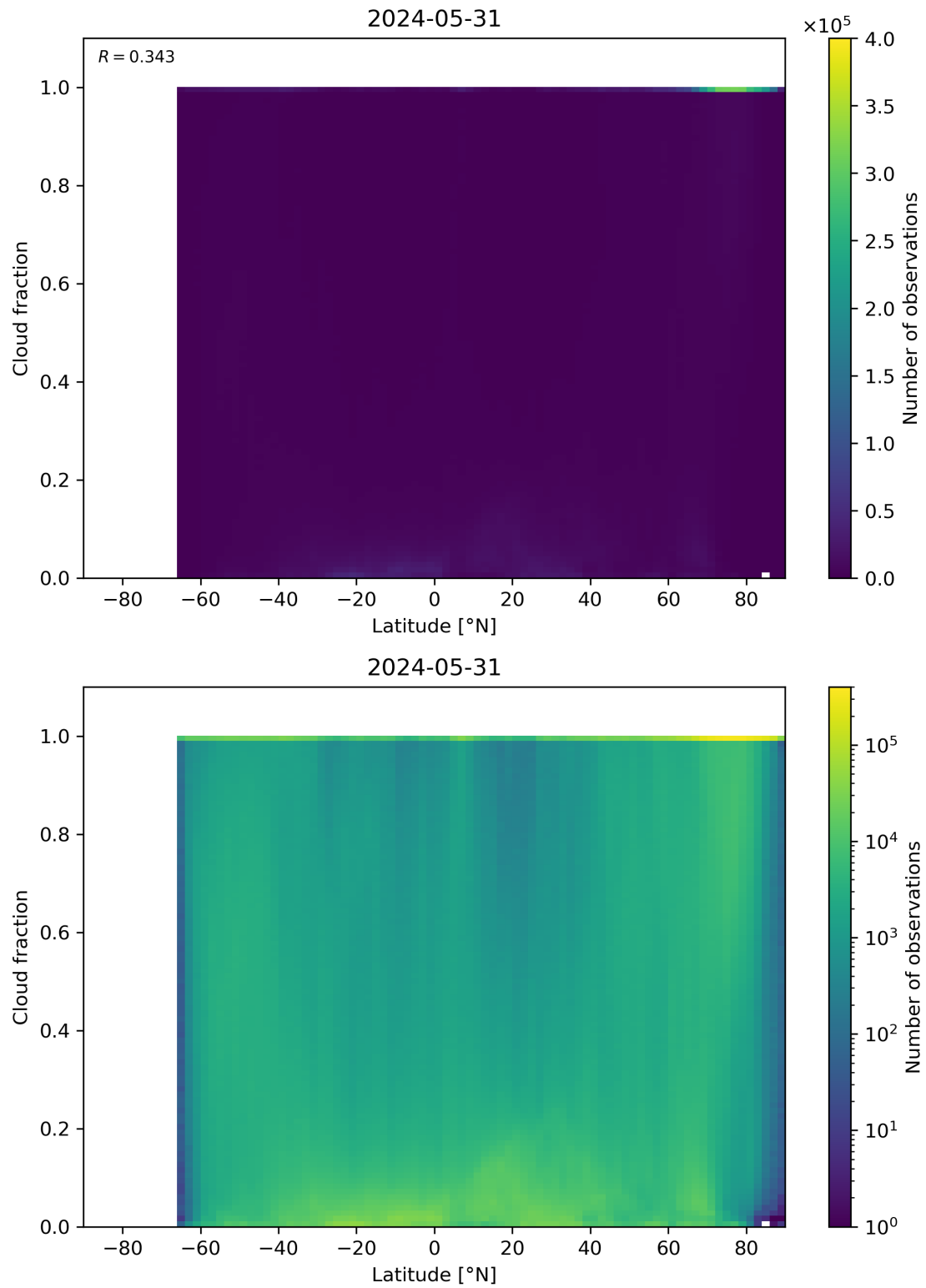
Figure 90: Scatter density plot of “Latitude” against “Cloud fraction” for 2024-05-30 to 2024-06-01.
