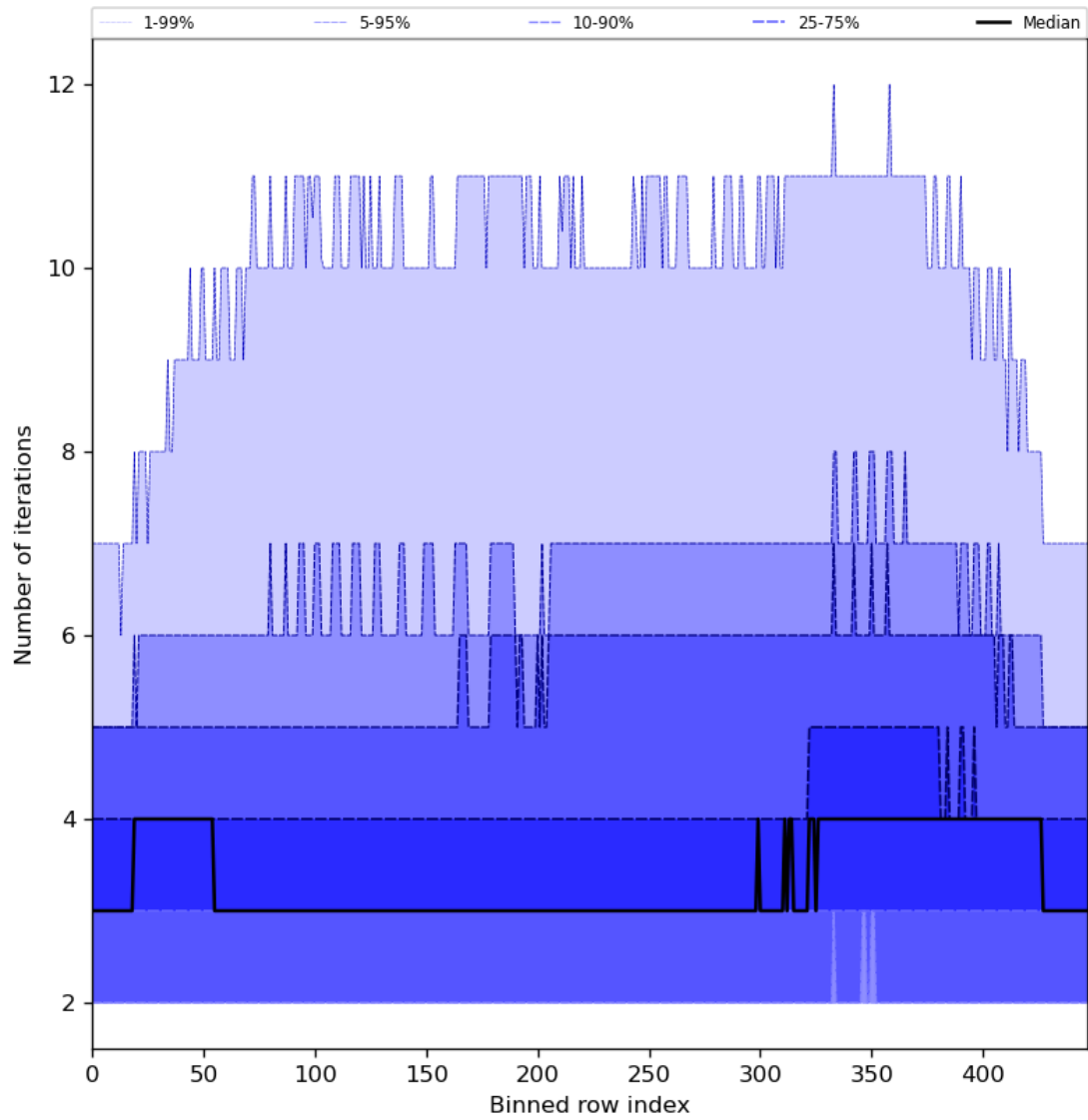
Figure 56: Along track statistics of “Number of iterations” for 2024-05-30 to 2024-06-01
