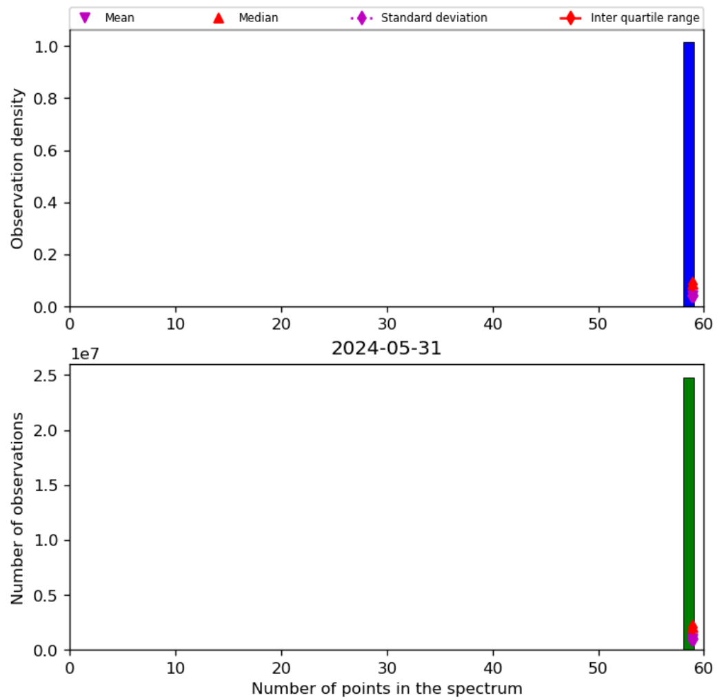
Figure 44: Histogram of “Number of points in the spectrum” for 2024-05-30 to 2024-06-01
