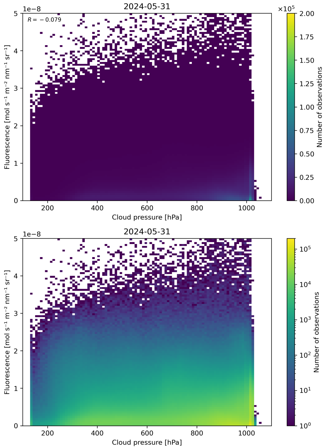
Figure 80: Scatter density plot of “Cloud pressure” against “Fluorescence” for 2024-05-30 to 2024-06-01.
