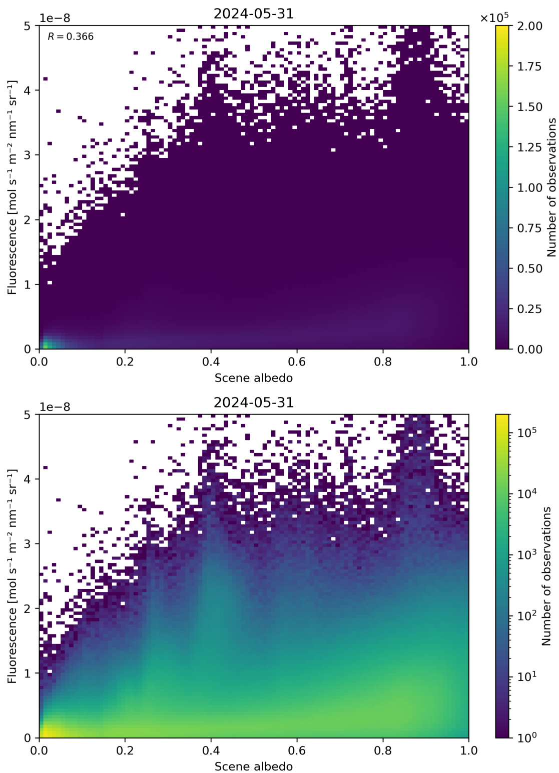
Figure 104: Scatter density plot of “Scene albedo” against “Fluorescence” for 2024-05-30 to 2024-06-01.
