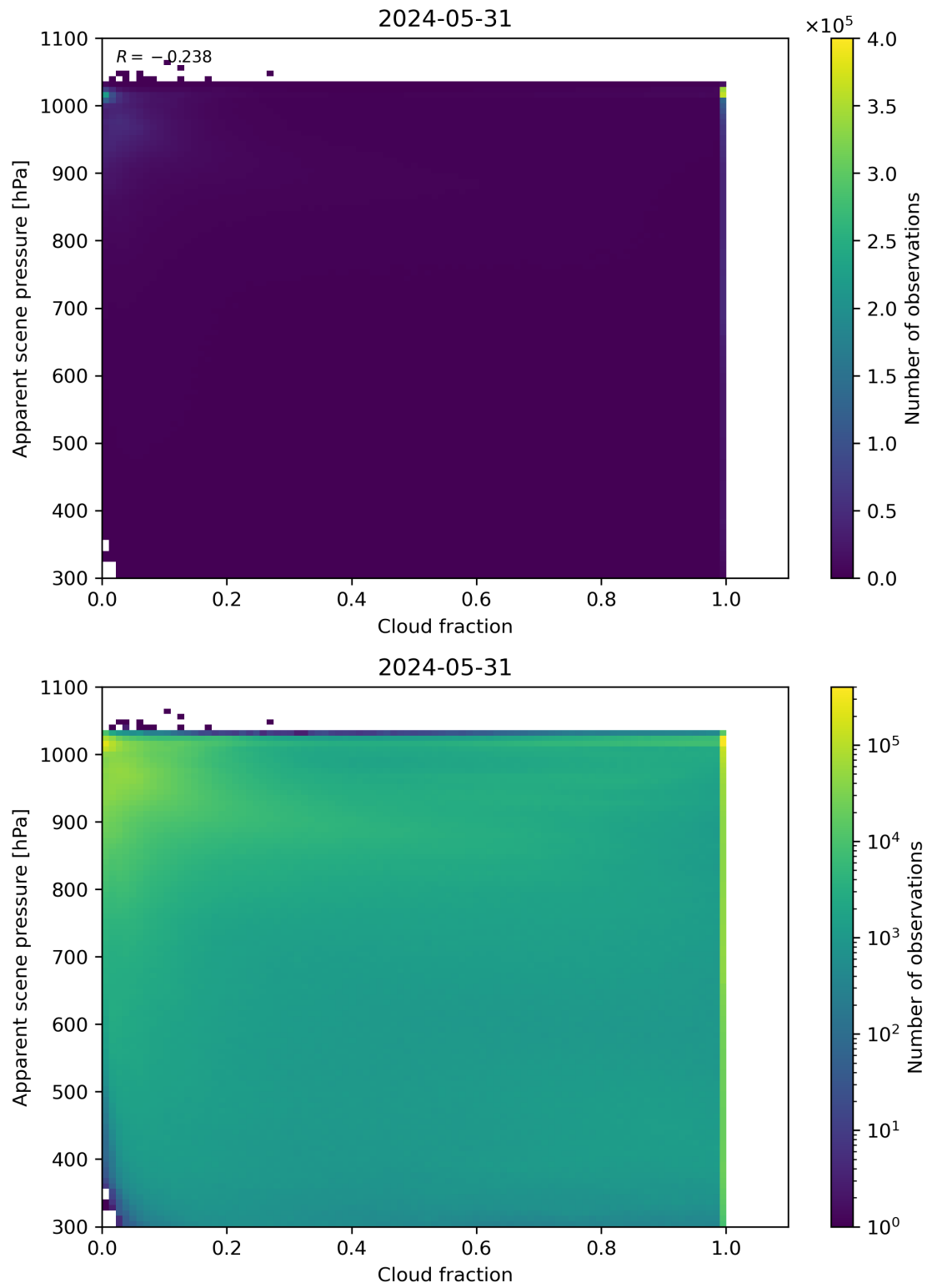
Figure 70: Scatter density plot of “Cloud fraction” against “Apparent scene pressure” for 2024-05-30 to 2024-06-01.
