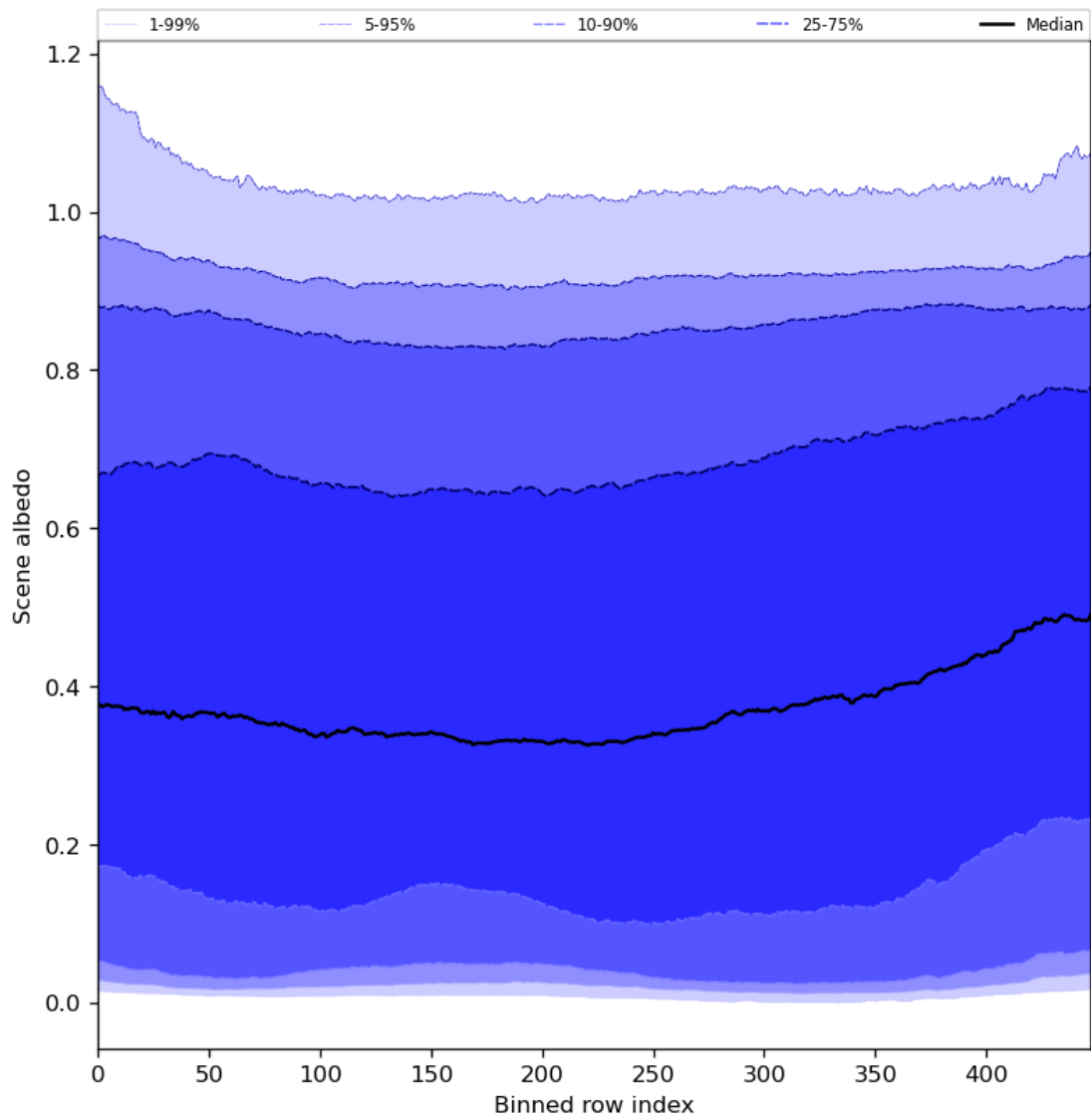
Figure 51: Along track statistics of “Scene albedo” for 2024-05-30 to 2024-06-01
