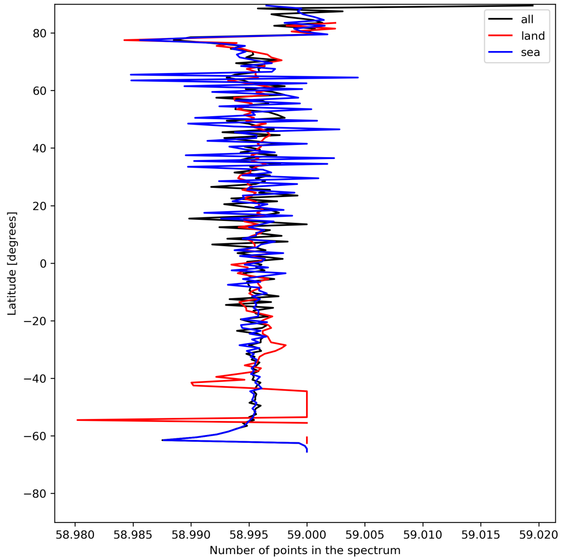
Figure 27: Zonal average of “Number of points in the spectrum” for 2024-05-30 to 2024-06-01.
