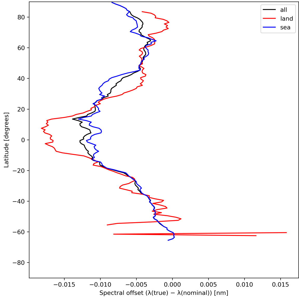
Figure 28: Zonal average of “Spectral offset ( \lambda(\text{true}) - \lambda(\text{nominal}) )” for 2024-05-30 to 2024-06-01.
