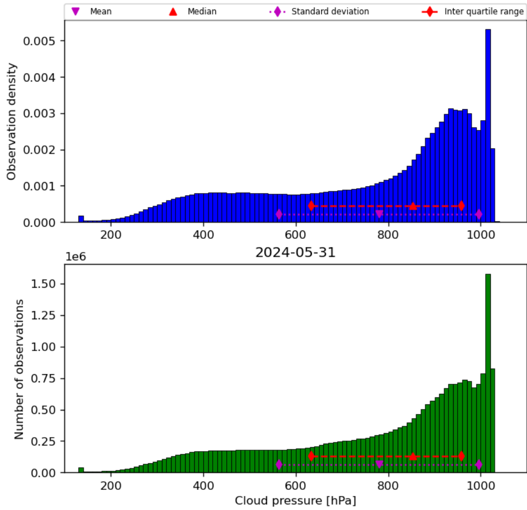
Figure 30: Histogram of “Cloud pressure” for 2024-05-30 to 2024-06-01
