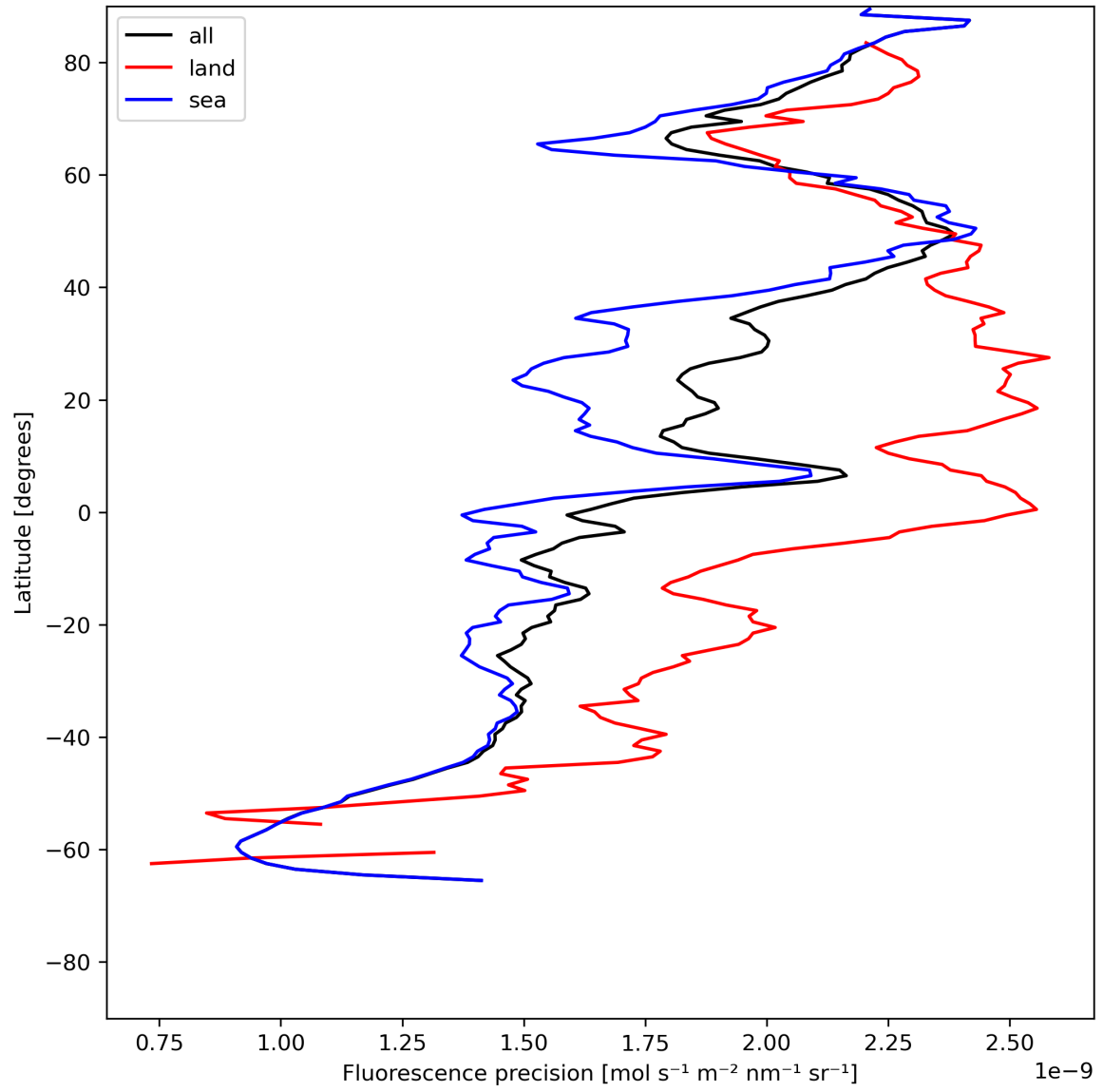
Figure 24: Zonal average of “Fluorescence precision” for 2024-05-30 to 2024-06-01.
