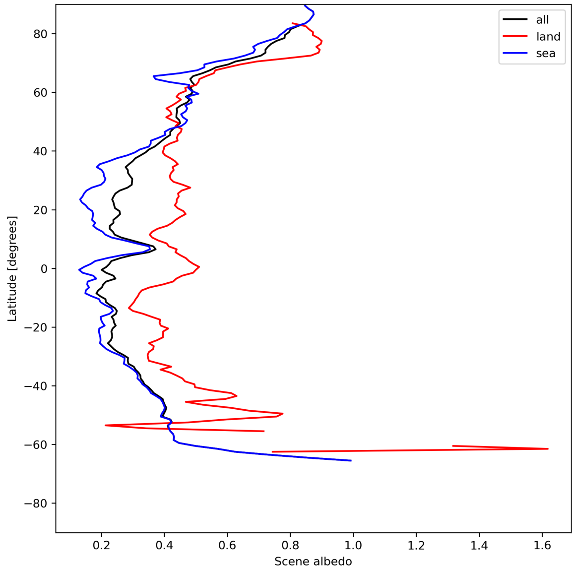
Figure 17: Zonal average of “Scene albedo” for 2024-05-30 to 2024-06-01.
