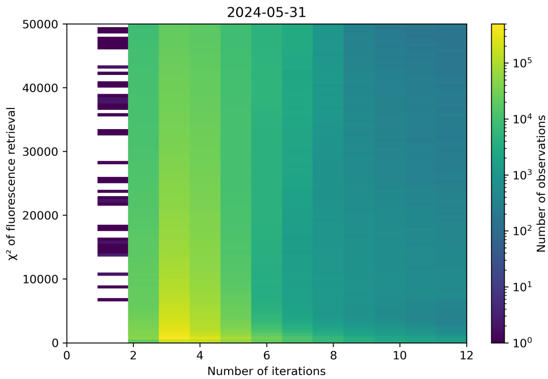
Figure 97: Scatter density plot of “Number of iterations” against “ \chi^2 of fluorescence retrieval” for 2024-05-30 to 2024-06-01.
