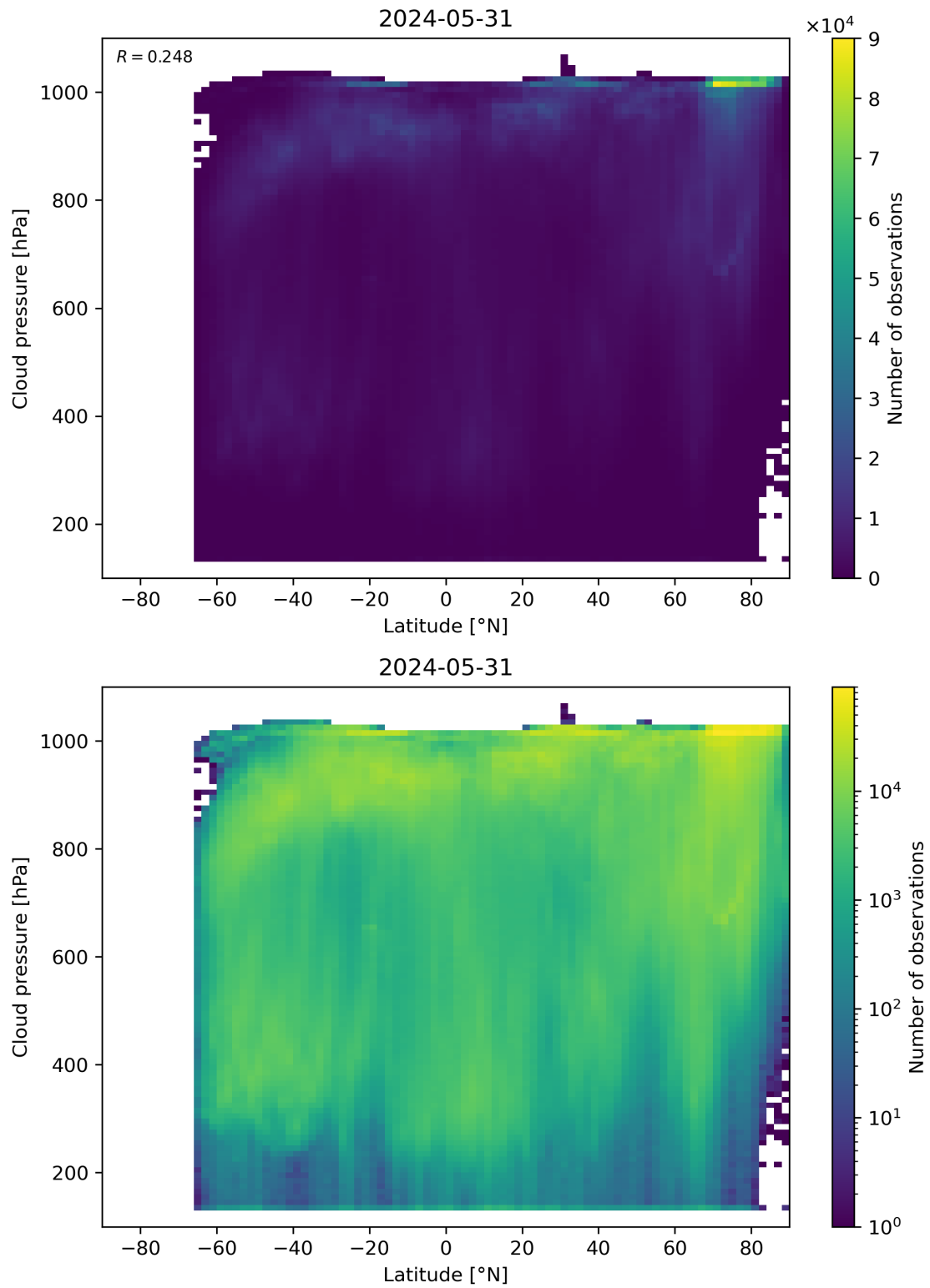
Figure 91: Scatter density plot of “Latitude” against “Cloud pressure” for 2024-05-30 to 2024-06-01.
