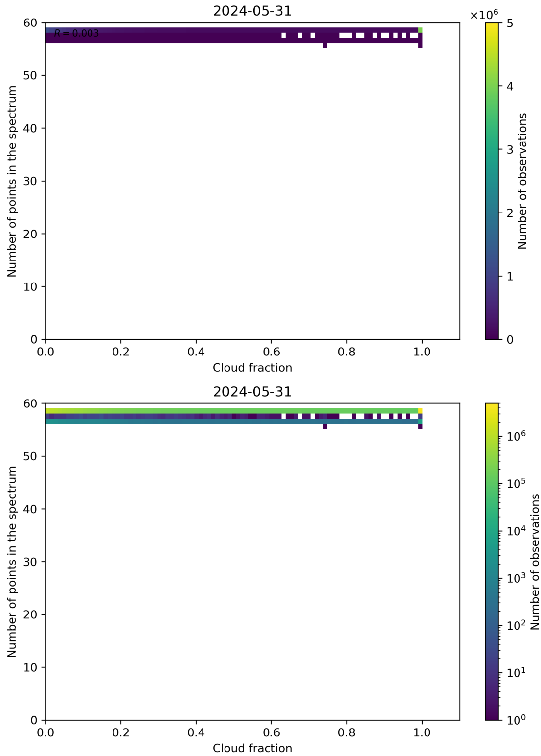
Figure 74: Scatter density plot of “Cloud fraction” against “Number of points in the spectrum” for 2024-05-30 to 2024-06-01.
