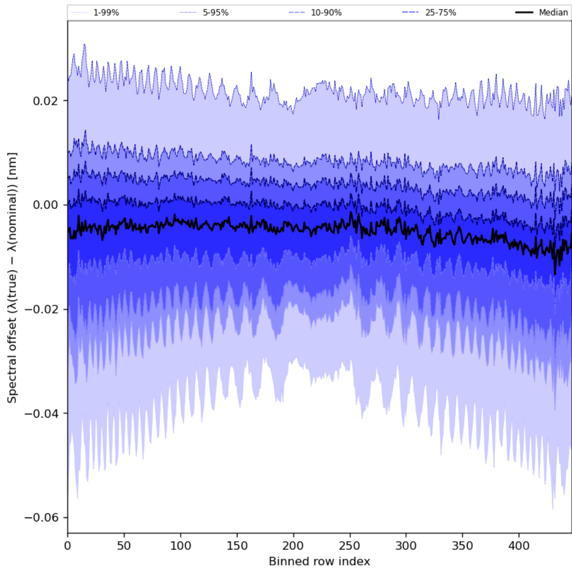
Figure 62: Along track statistics of “Spectral offset ( \lambda(\text{true}) - \lambda(\text{nominal}) )” for 2024-05-30 to 2024-06-01
