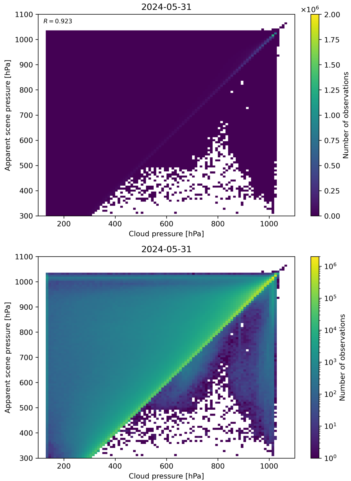
Figure 77: Scatter density plot of “Cloud pressure” against “Apparent scene pressure” for 2024-05-30 to 2024-06-01.
