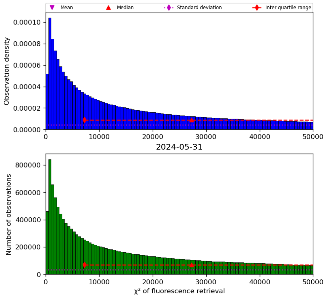
Figure 42: Histogram of “ \chi^2 of fluorescence retrieval” for 2024-05-30 to 2024-06-01
