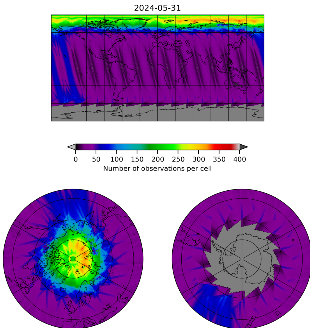
Figure 11: Map of the number of observations for 2024-05-30 to 2024-06-01
