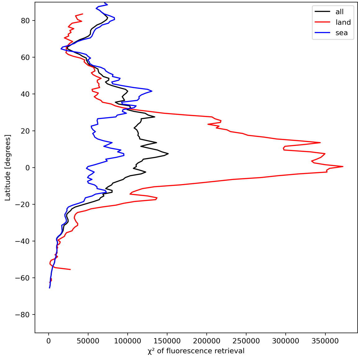
Figure 25: Zonal average of “ \chi^2 of fluorescence retrieval” for 2024-05-30 to 2024-06-01.
