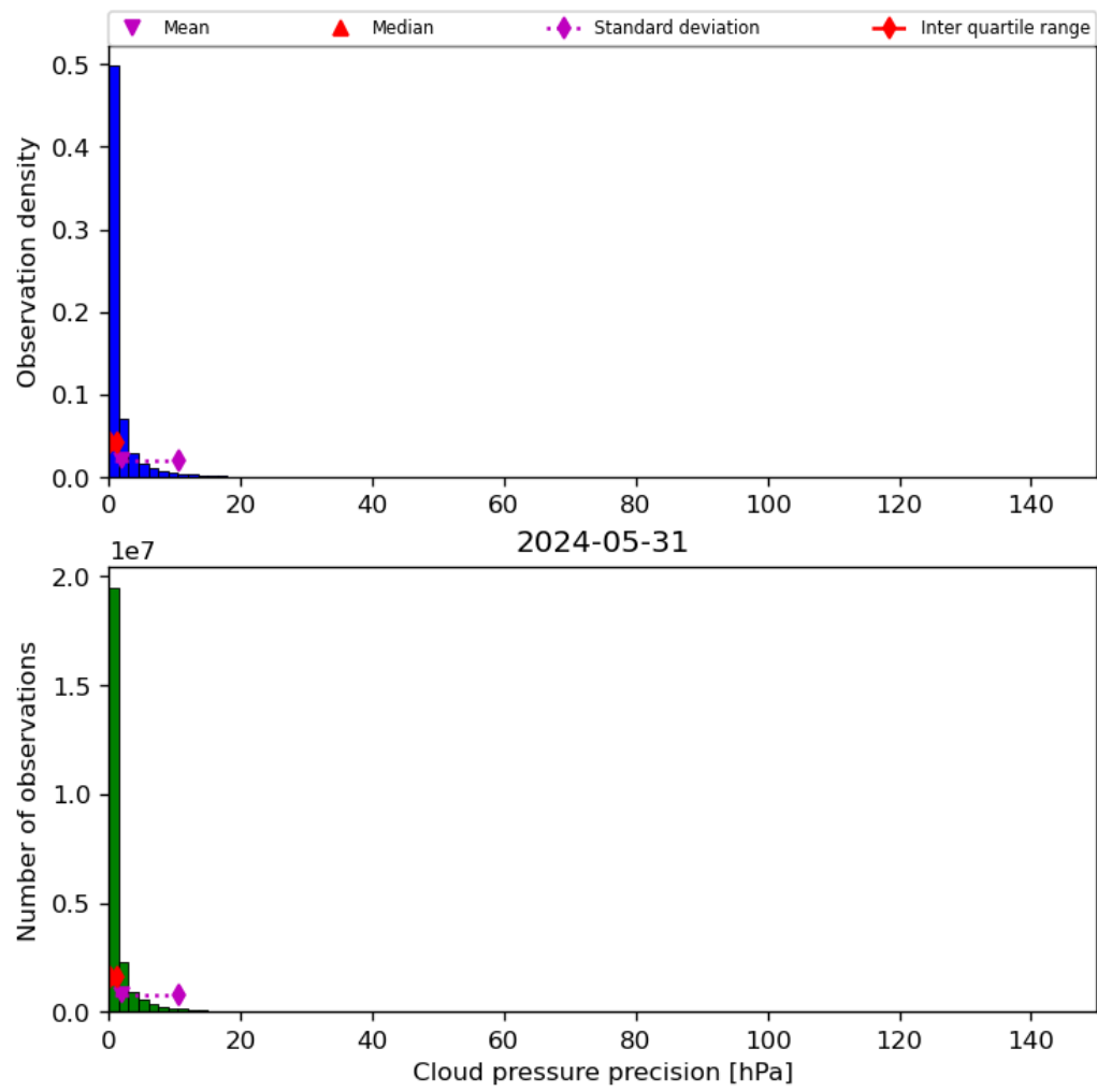
Figure 31: Histogram of “Cloud pressure precision” for 2024-05-30 to 2024-06-01
