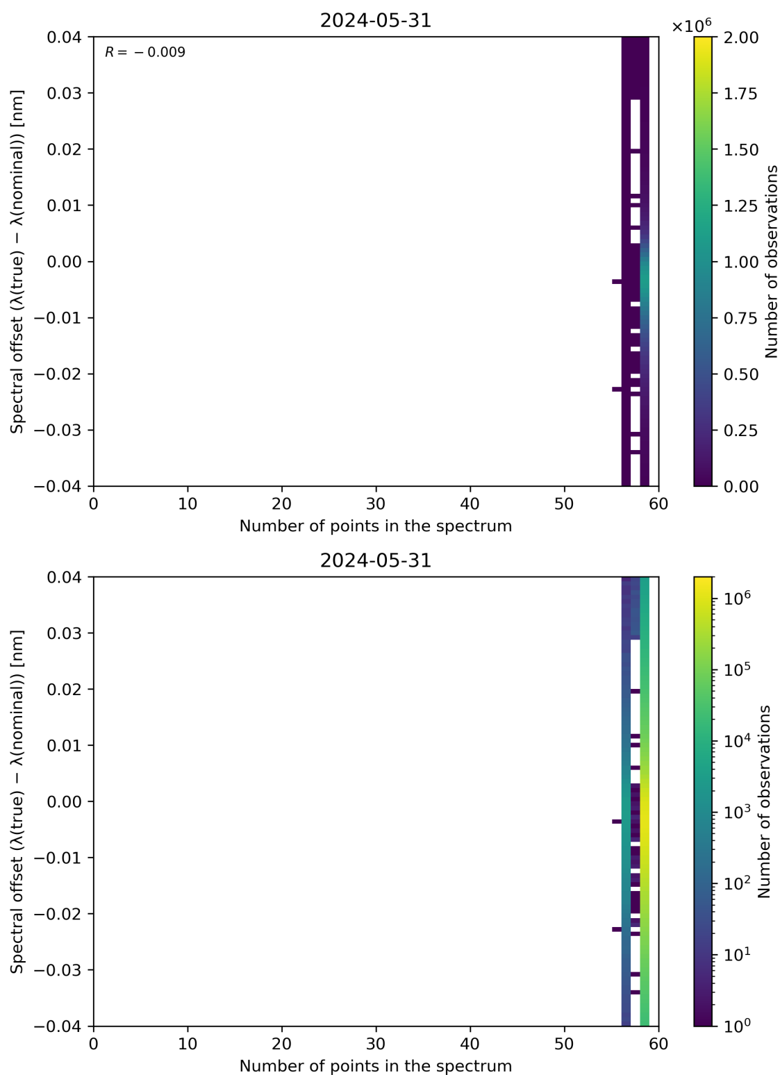
Figure 101: Scatter density plot of “Number of points in the spectrum” against “Spectral offset ( \lambda(\text{true}) - \lambda(\text{nominal}) )” for 2024-05-30 to 2024-06-01.
