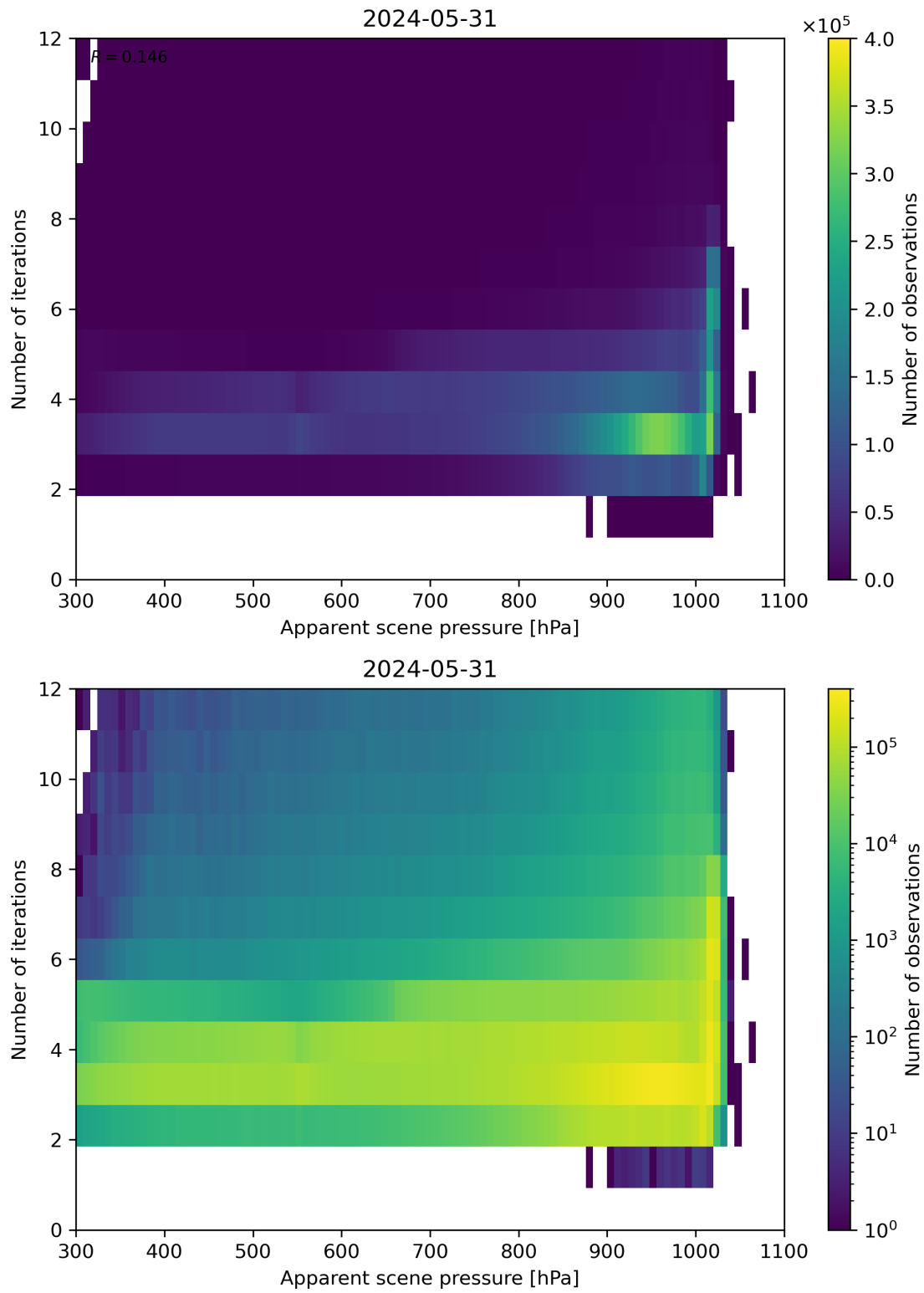
Figure 65: Scatter density plot of “Apparent scene pressure” against “Number of iterations” for 2024-05-30 to 2024-06-01.
