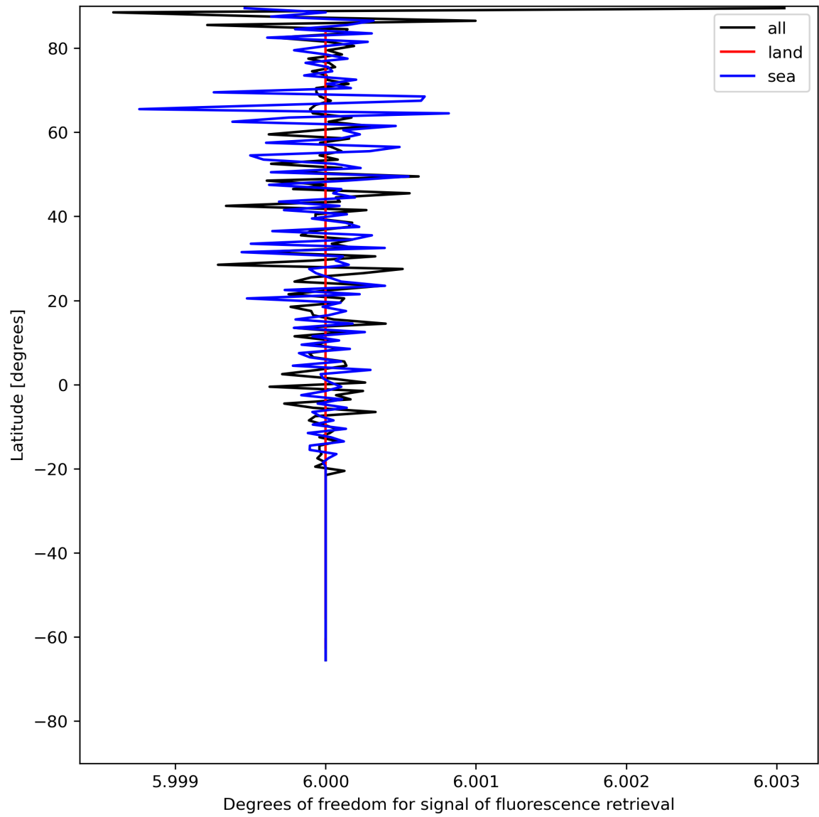
Figure 26: Zonal average of “Degrees of freedom for signal of fluorescence retrieval” for 2024-05-30 to 2024-06-01.
