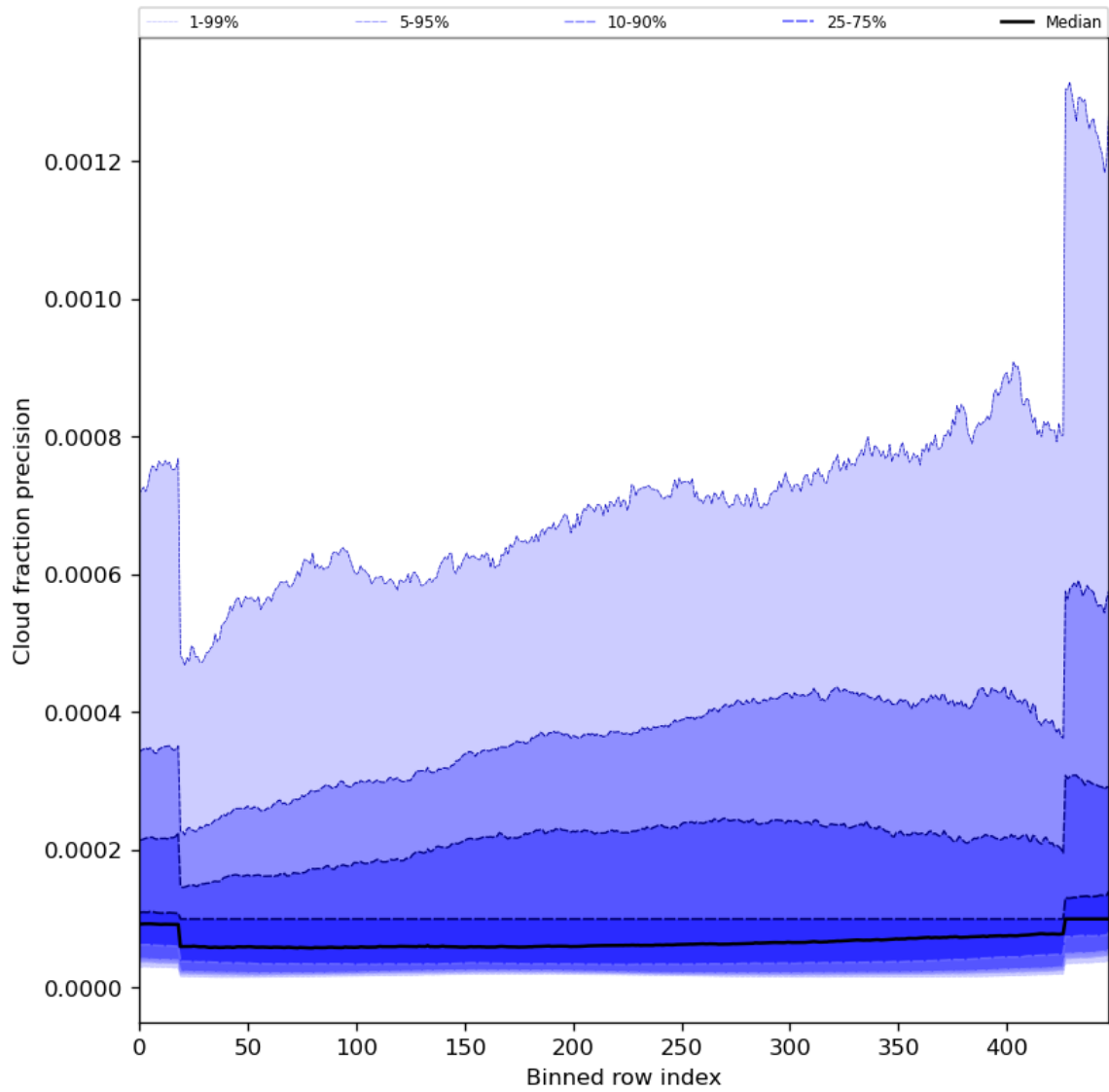
Figure 50: Along track statistics of “Cloud fraction precision” for 2024-05-30 to 2024-06-01
