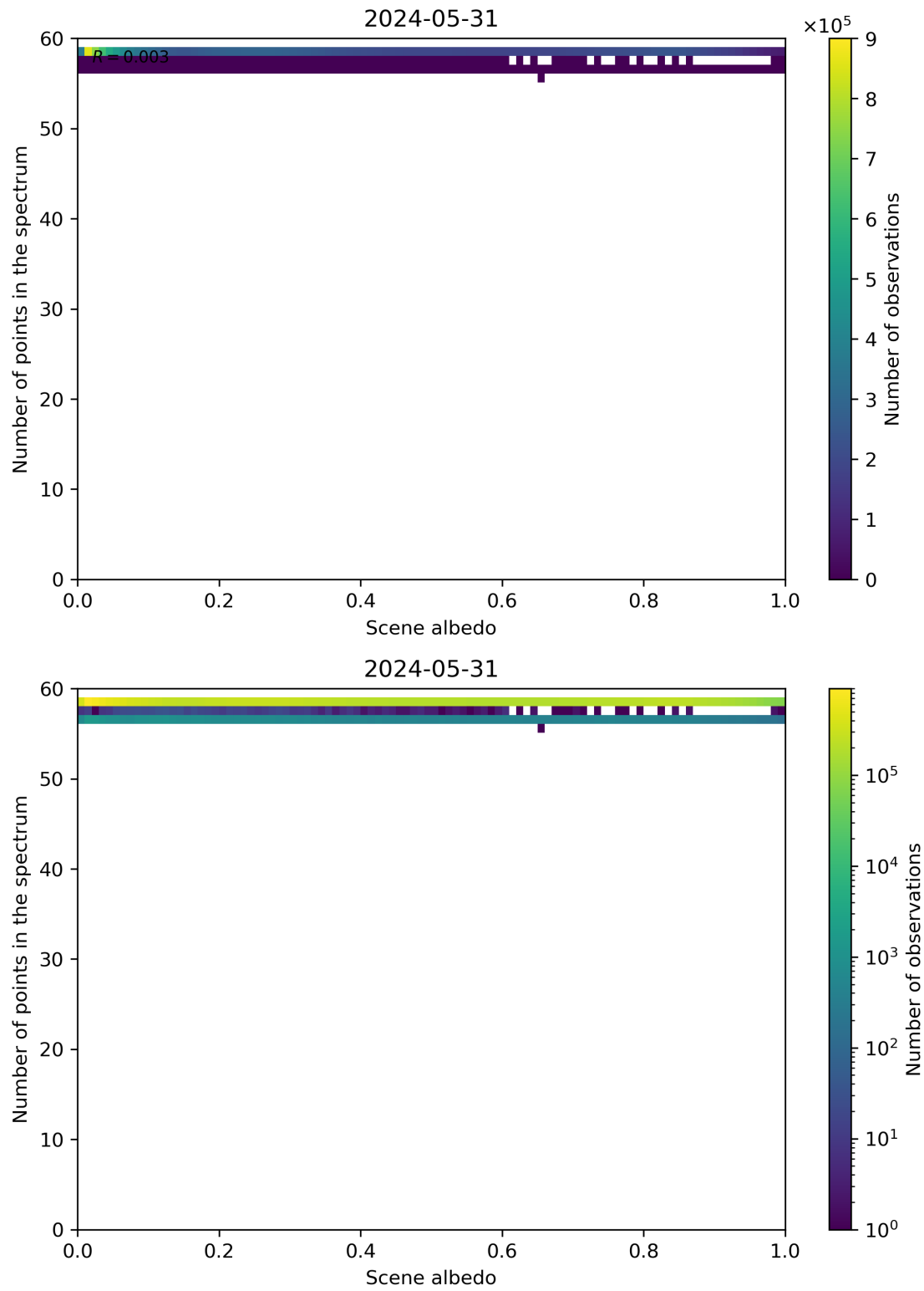
Figure 106: Scatter density plot of “Scene albedo” against “Number of points in the spectrum” for 2024-05-30 to 2024-06-01.
