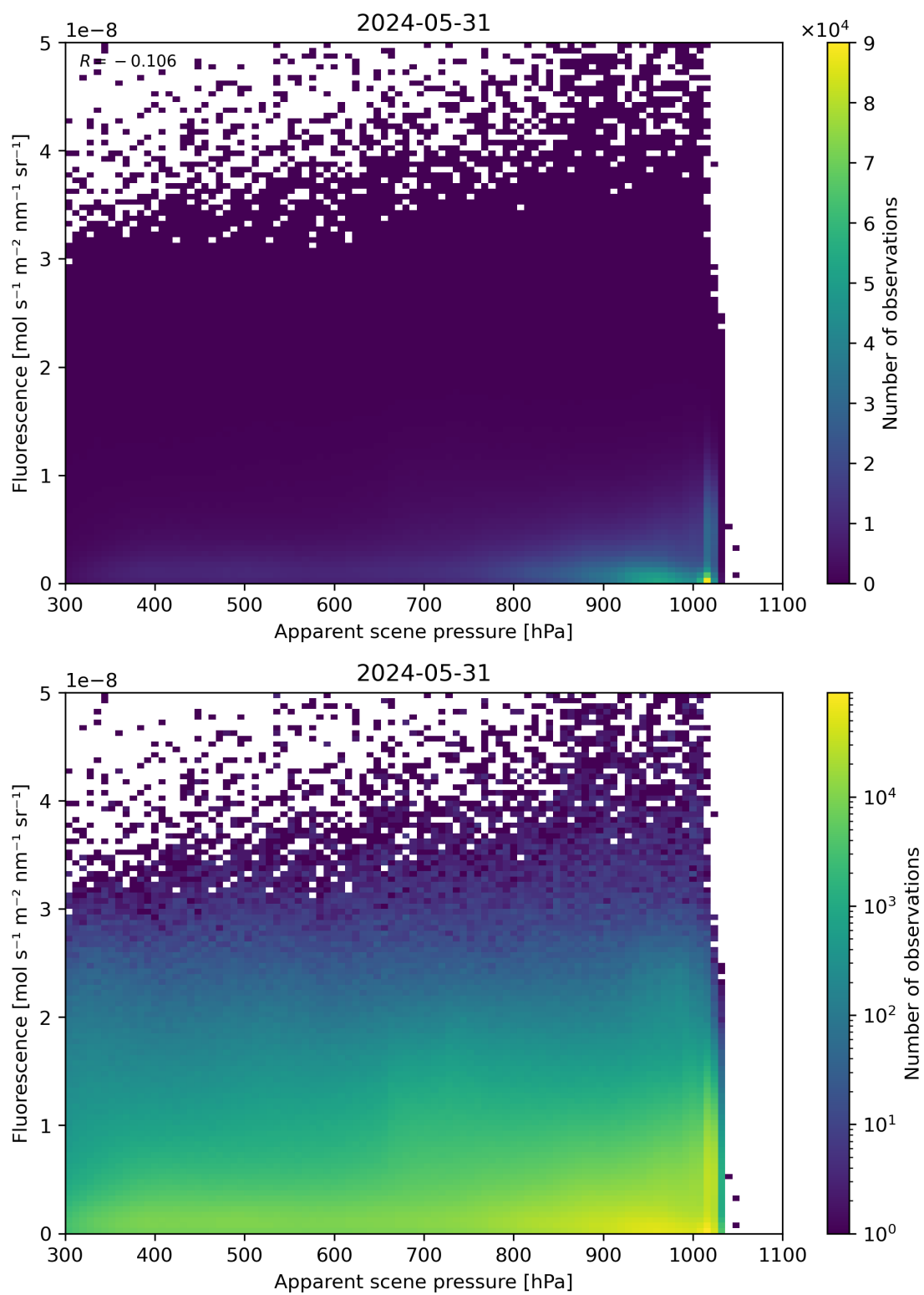
Figure 64: Scatter density plot of “Apparent scene pressure” against “Fluorescence” for 2024-05-30 to 2024-06-01.
