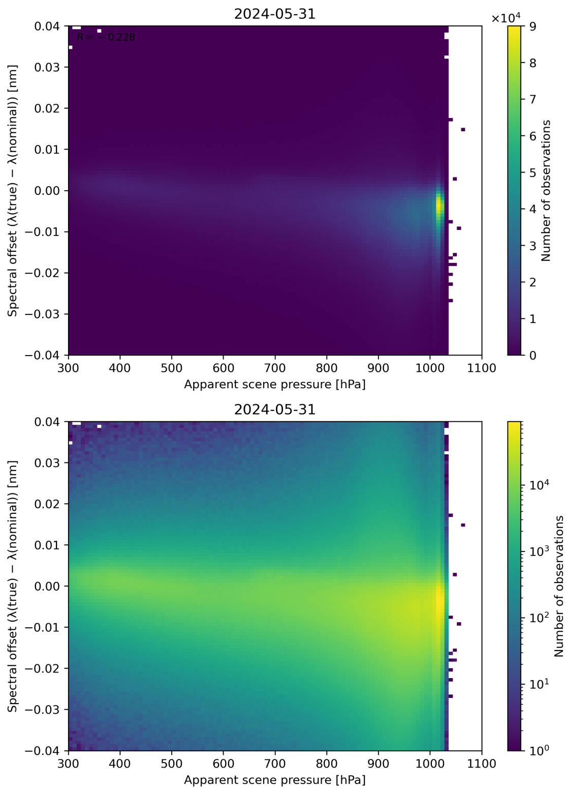
Figure 67: Scatter density plot of “Apparent scene pressure” against “Spectral offset ( \lambda(\text{true}) - \lambda(\text{nominal}) )” for 2024-05-30 to 2024-06-01.
