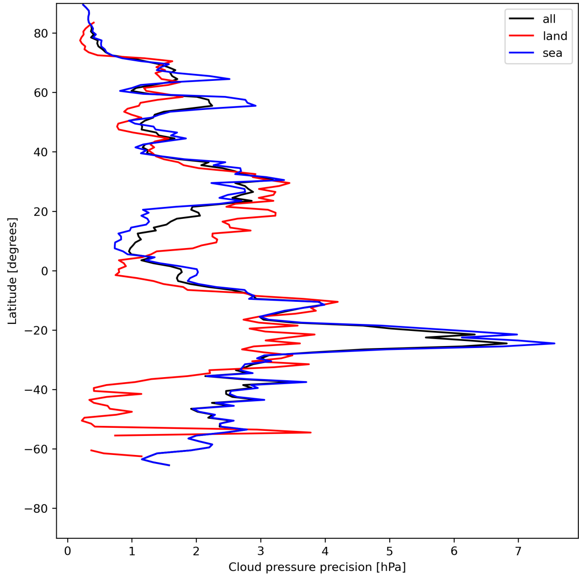
Figure 14: Zonal average of “Cloud pressure precision” for 2024-05-30 to 2024-06-01.
