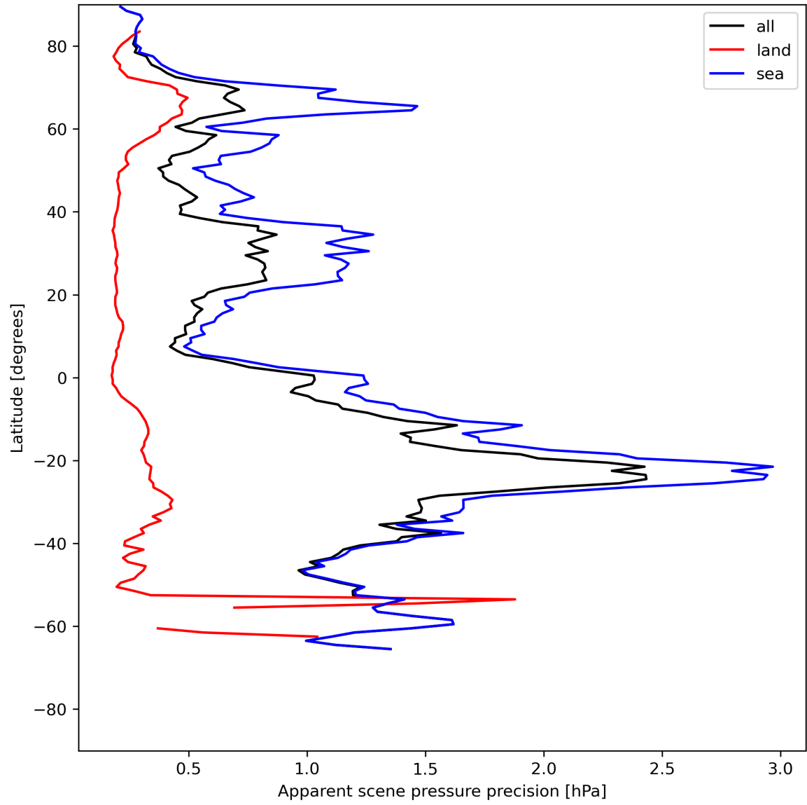
Figure 20: Zonal average of “Apparent scene pressure precision” for 2024-05-30 to 2024-06-01.
