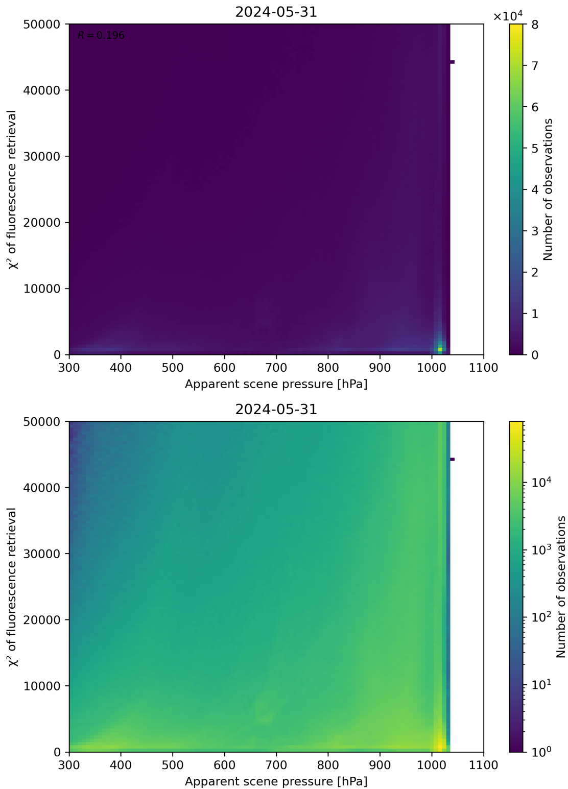
Figure 63: Scatter density plot of “Apparent scene pressure” against “ \chi^2 of fluorescence retrieval” for 2024-05-30 to 2024-06-01.
