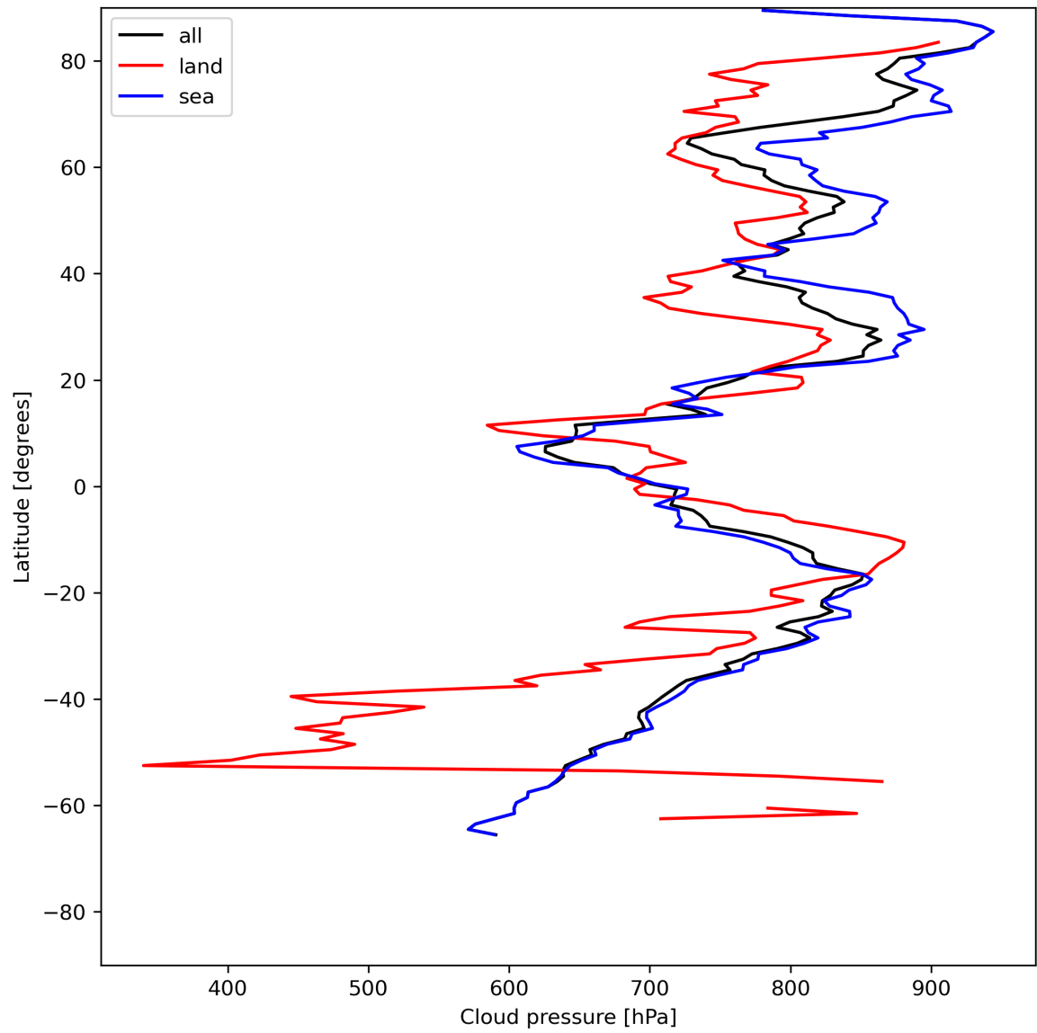
Figure 13: Zonal average of “Cloud pressure” for 2024-05-30 to 2024-06-01.
