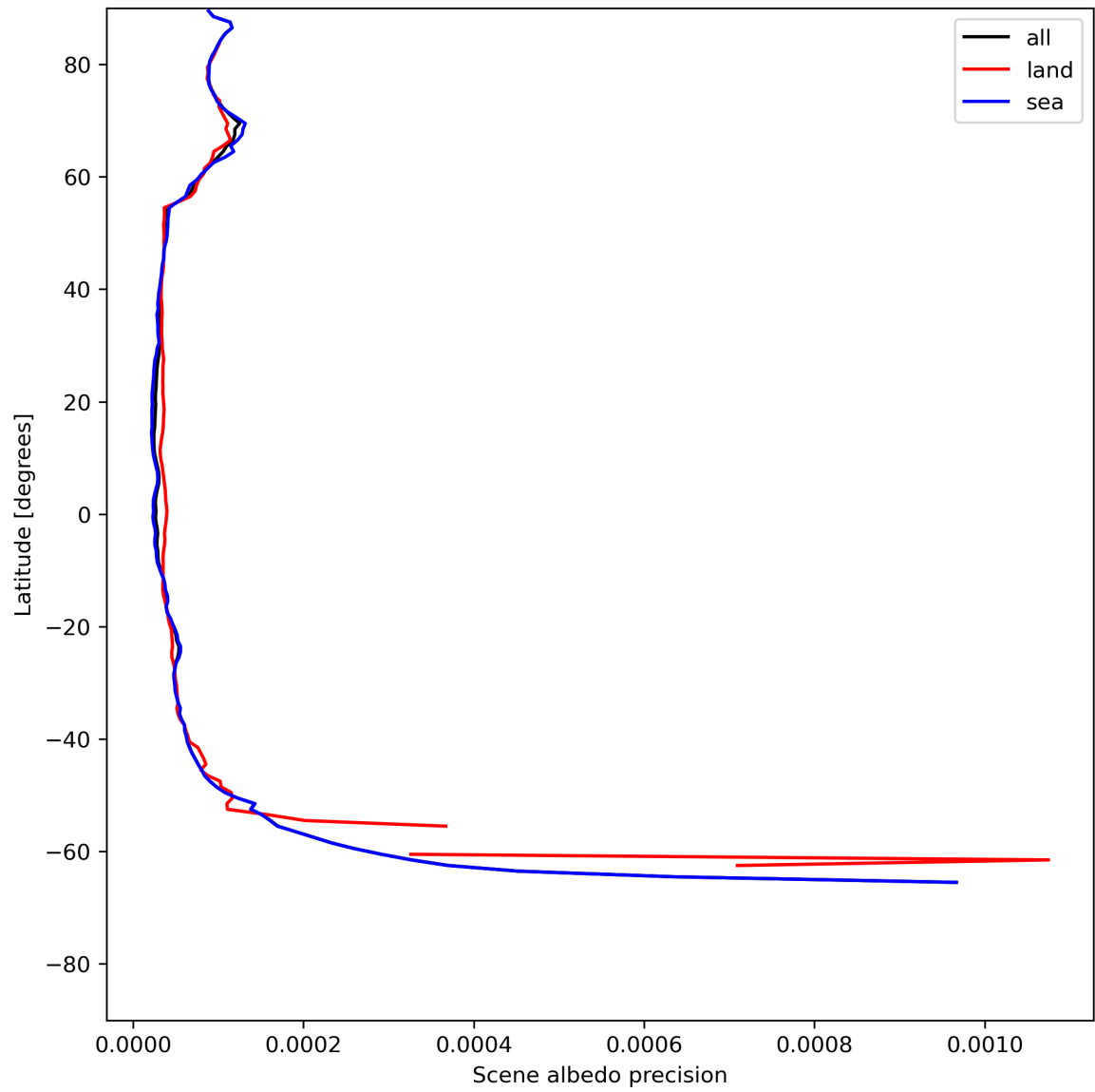
Figure 18: Zonal average of "Scene albedo precision" for 2024-05-30 to 2024-06-01.
