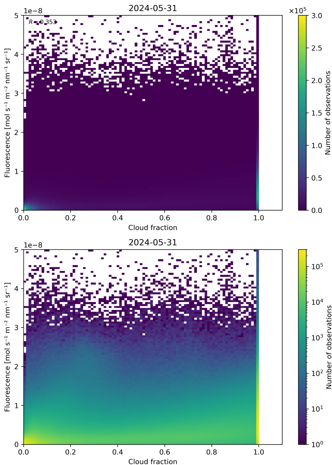
Figure 72: Scatter density plot of “Cloud fraction” against “Fluorescence” for 2024-05-30 to 2024-06-01.
