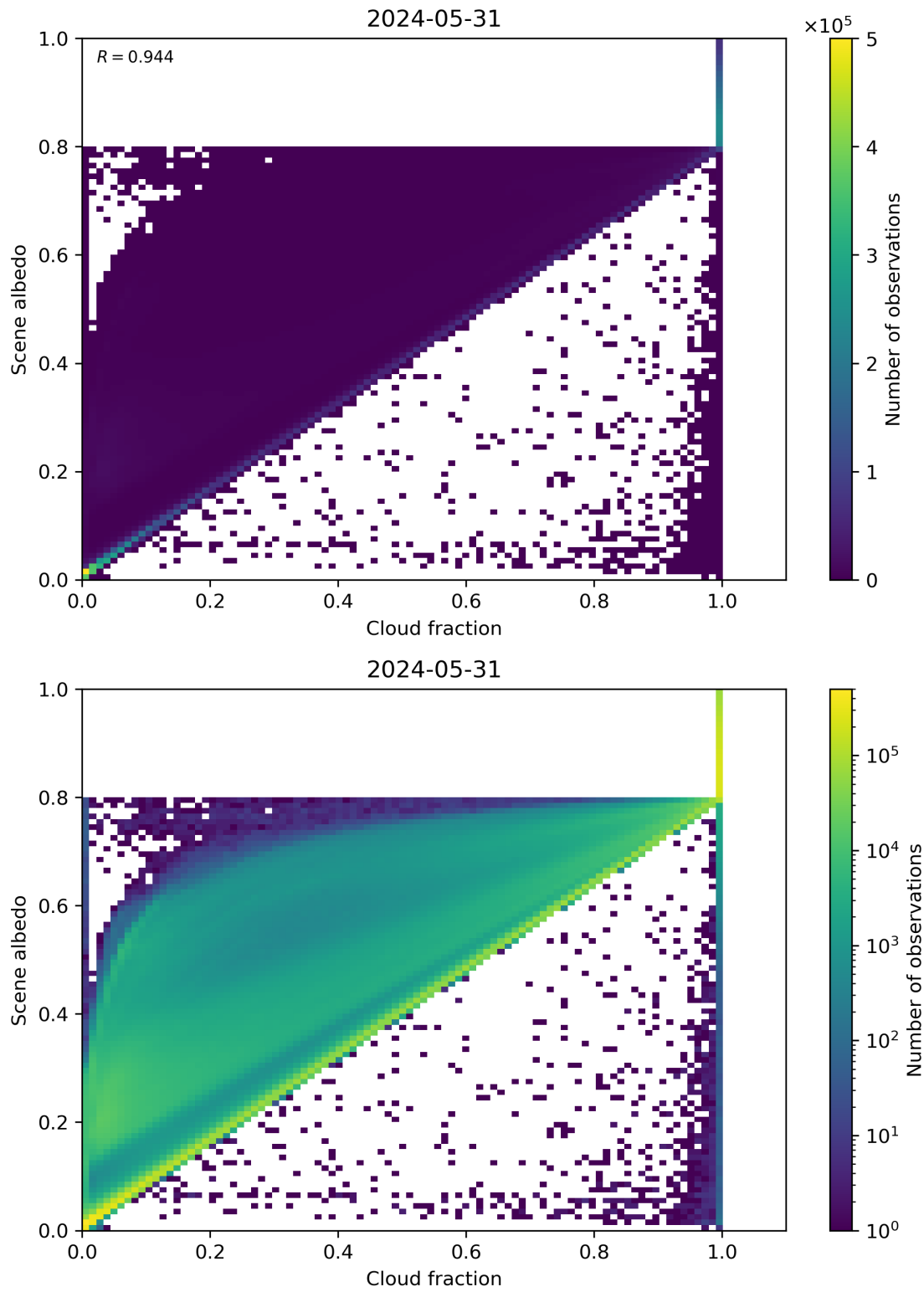
Figure 75: Scatter density plot of “Cloud fraction” against “Scene albedo” for 2024-05-30 to 2024-06-01.
