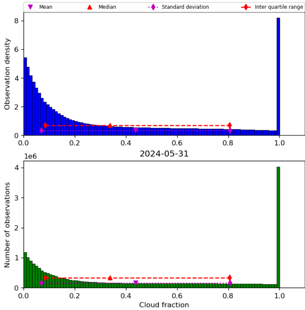
Figure 32: Histogram of “Cloud fraction” for 2024-05-30 to 2024-06-01
