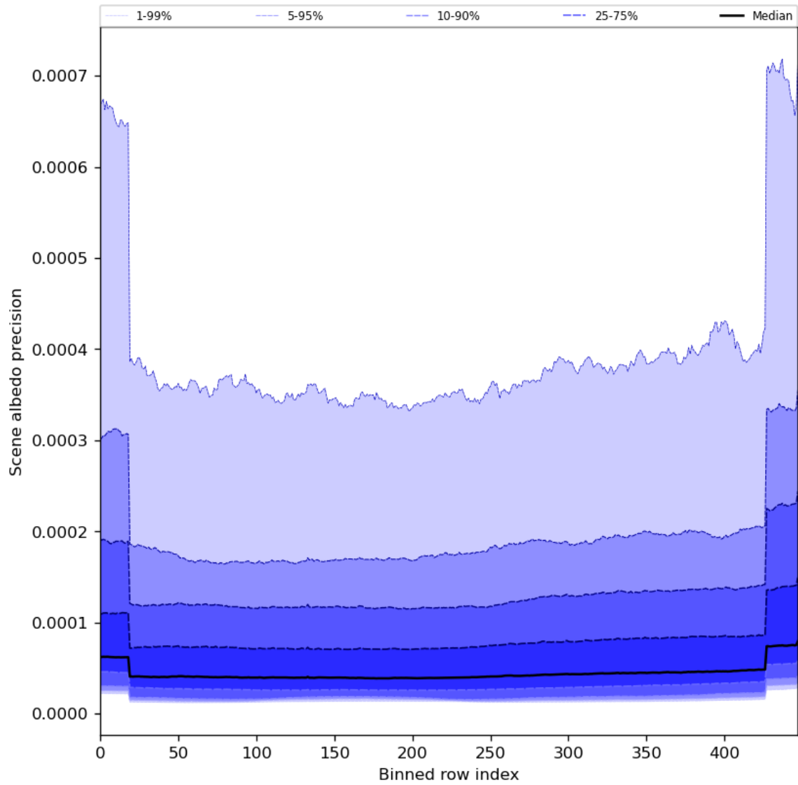
Figure 52: Along track statistics of “Scene albedo precision” for 2024-05-30 to 2024-06-01
