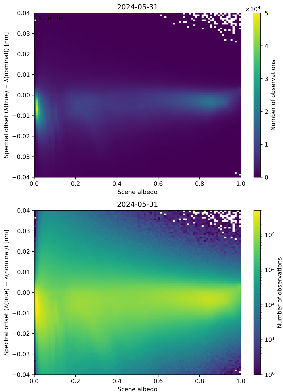
Figure 107: Scatter density plot of “Scene albedo” against “Spectral offset ( \lambda(\text{true}) - \lambda(\text{nominal}) )” for 2024-05-30 to 2024-06-01.
