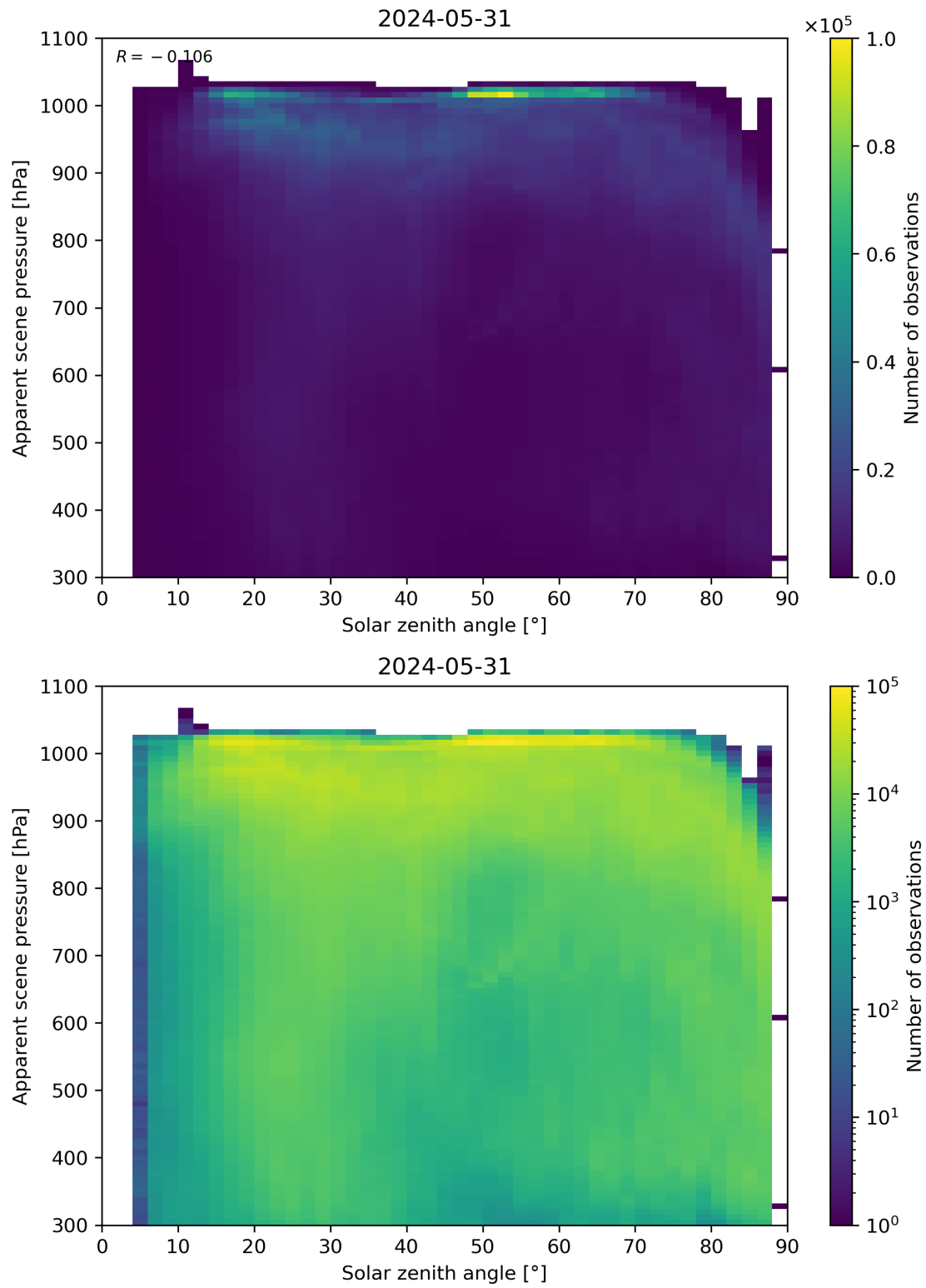
Figure 108: Scatter density plot of “Solar zenith angle” against “Apparent scene pressure” for 2024-05-30 to 2024-06-01.
