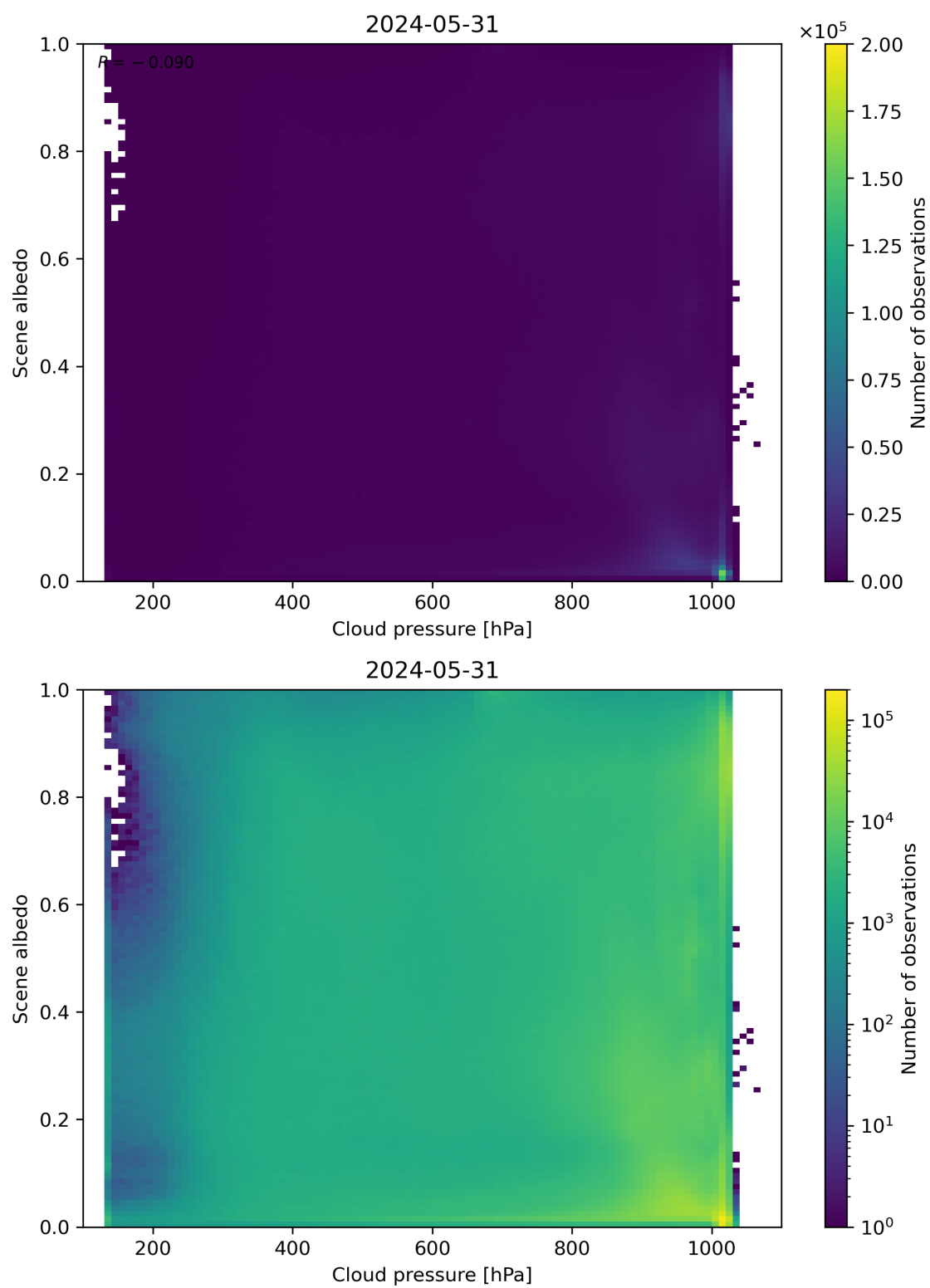
Figure 83: Scatter density plot of “Cloud pressure” against “Scene albedo” for 2024-05-30 to 2024-06-01.
