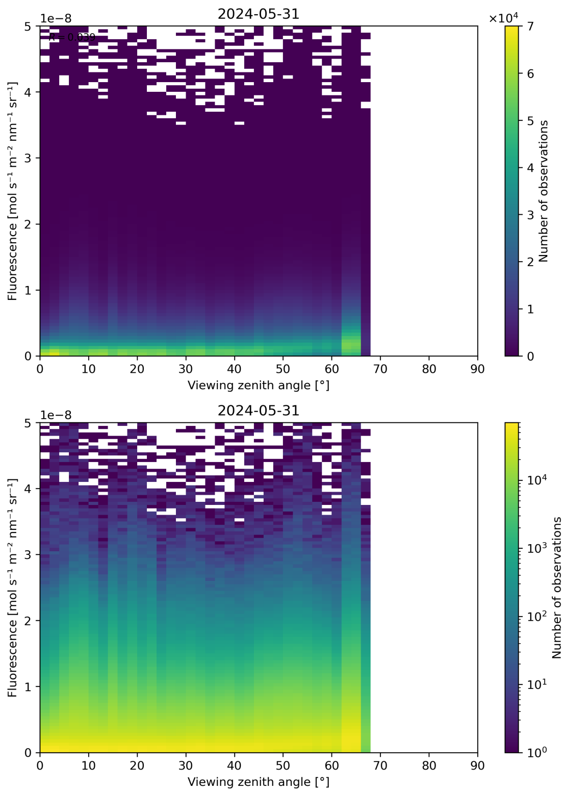
Figure 122: Scatter density plot of “Viewing zenith angle” against “Fluorescence” for 2024-05-30 to 2024-06-01.
