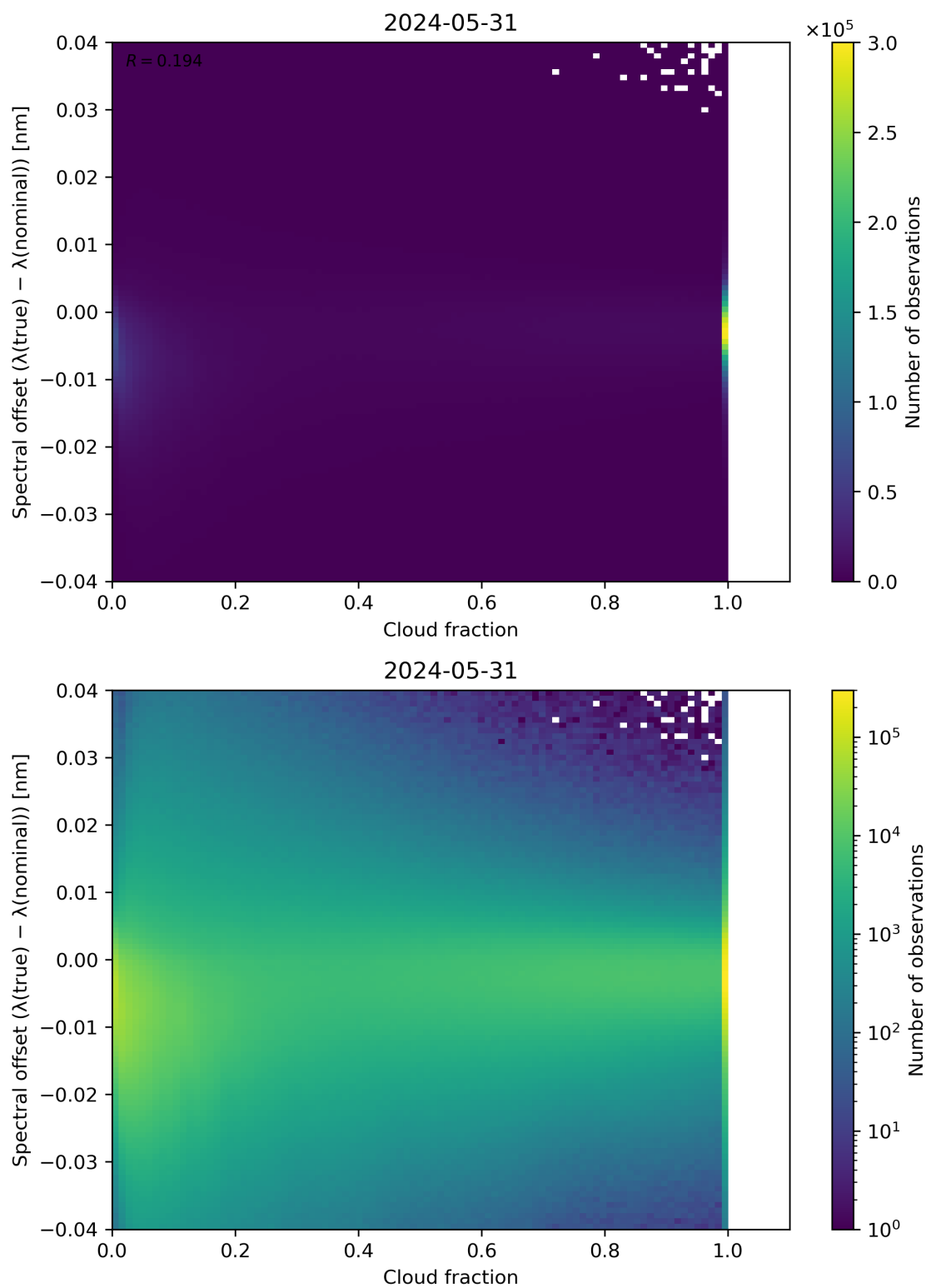
Figure 76: Scatter density plot of “Cloud fraction” against “Spectral offset ( \lambda(\text{true}) - \lambda(\text{nominal}) )” for 2024-05-30 to 2024-06-01.
