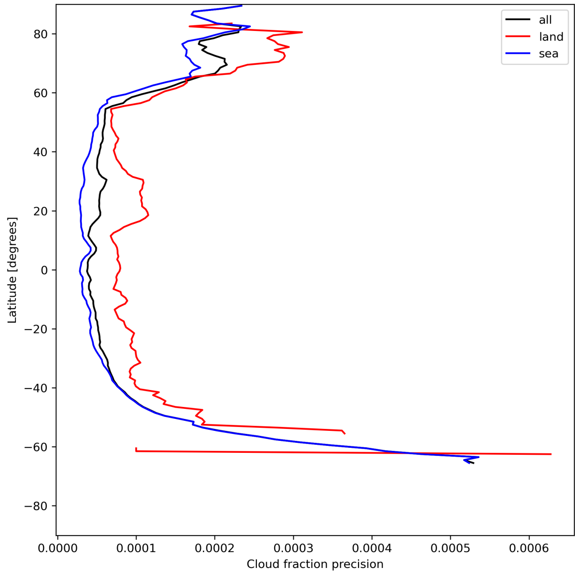
Figure 16: Zonal average of “Cloud fraction precision” for 2024-05-30 to 2024-06-01.
