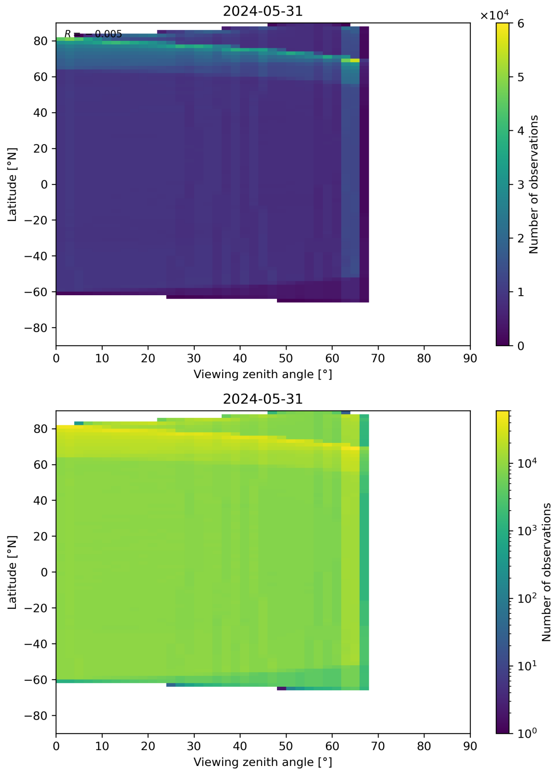
Figure 123: Scatter density plot of “Viewing zenith angle” against “Latitude” for 2024-05-30 to 2024-06-01.
