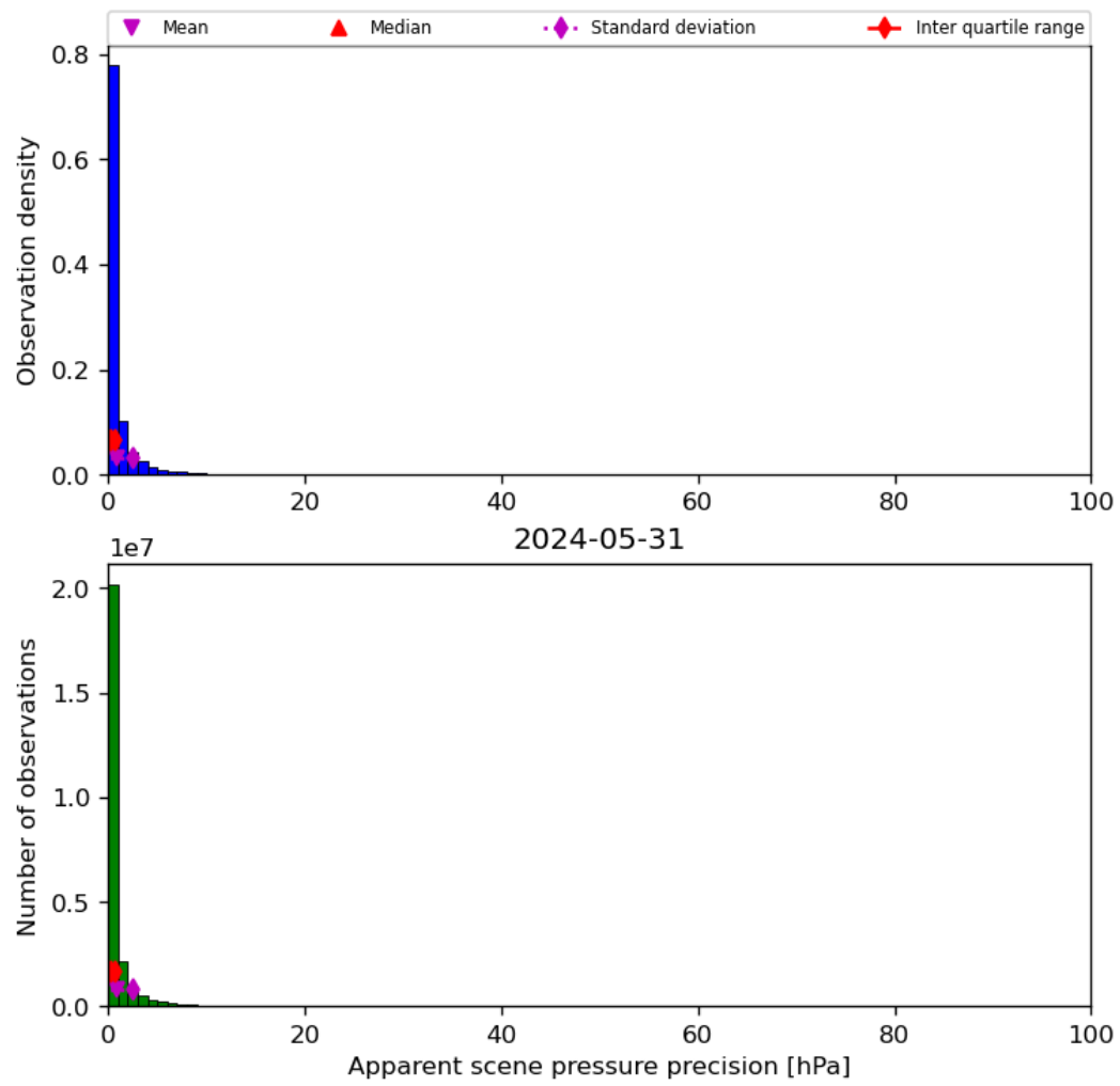
Figure 37: Histogram of “Apparent scene pressure precision” for 2024-05-30 to 2024-06-01
