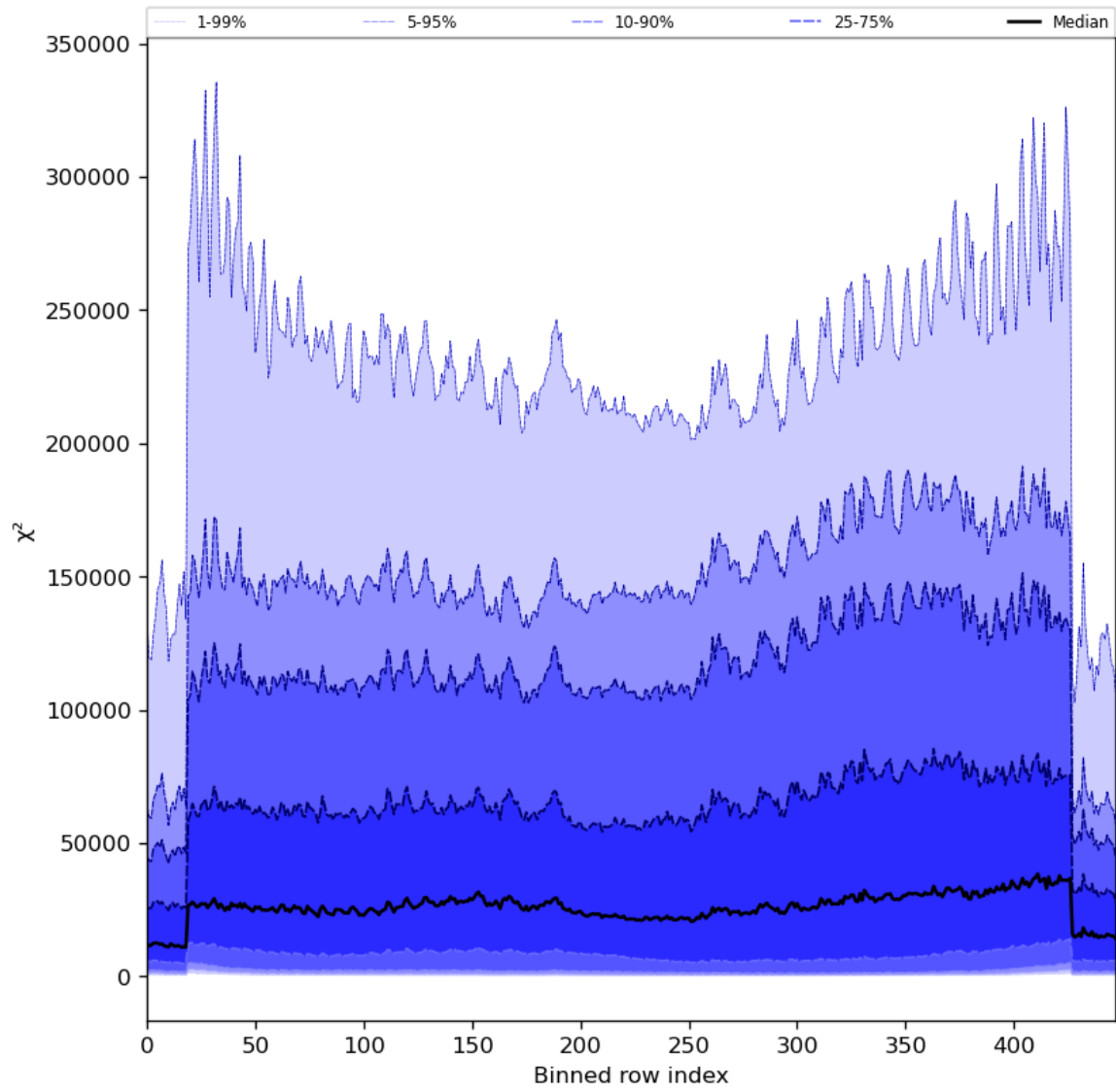
Figure 55: Along track statistics of “ \chi^2 ” for 2024-05-30 to 2024-06-01
