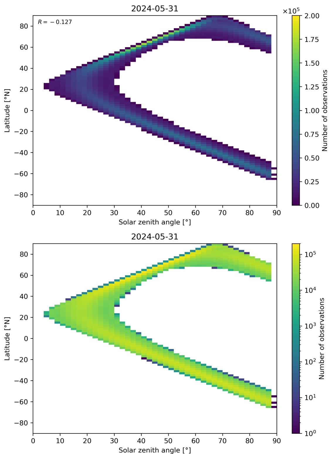
Figure 113: Scatter density plot of “Solar zenith angle” against “Latitude” for 2024-05-30 to 2024-06-01.
