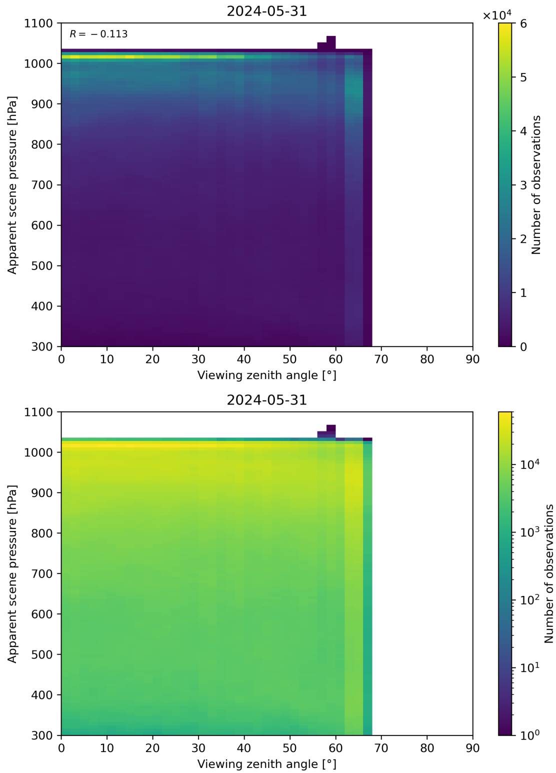
Figure 118: Scatter density plot of “Viewing zenith angle” against “Apparent scene pressure” for 2024-05-30 to 2024-06-01.
