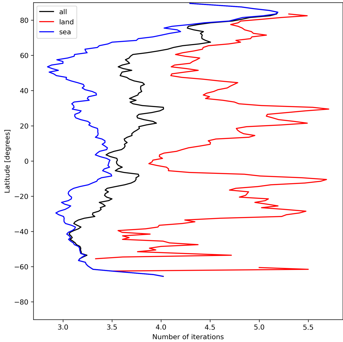
Figure 22: Zonal average of “Number of iterations” for 2024-05-30 to 2024-06-01.
