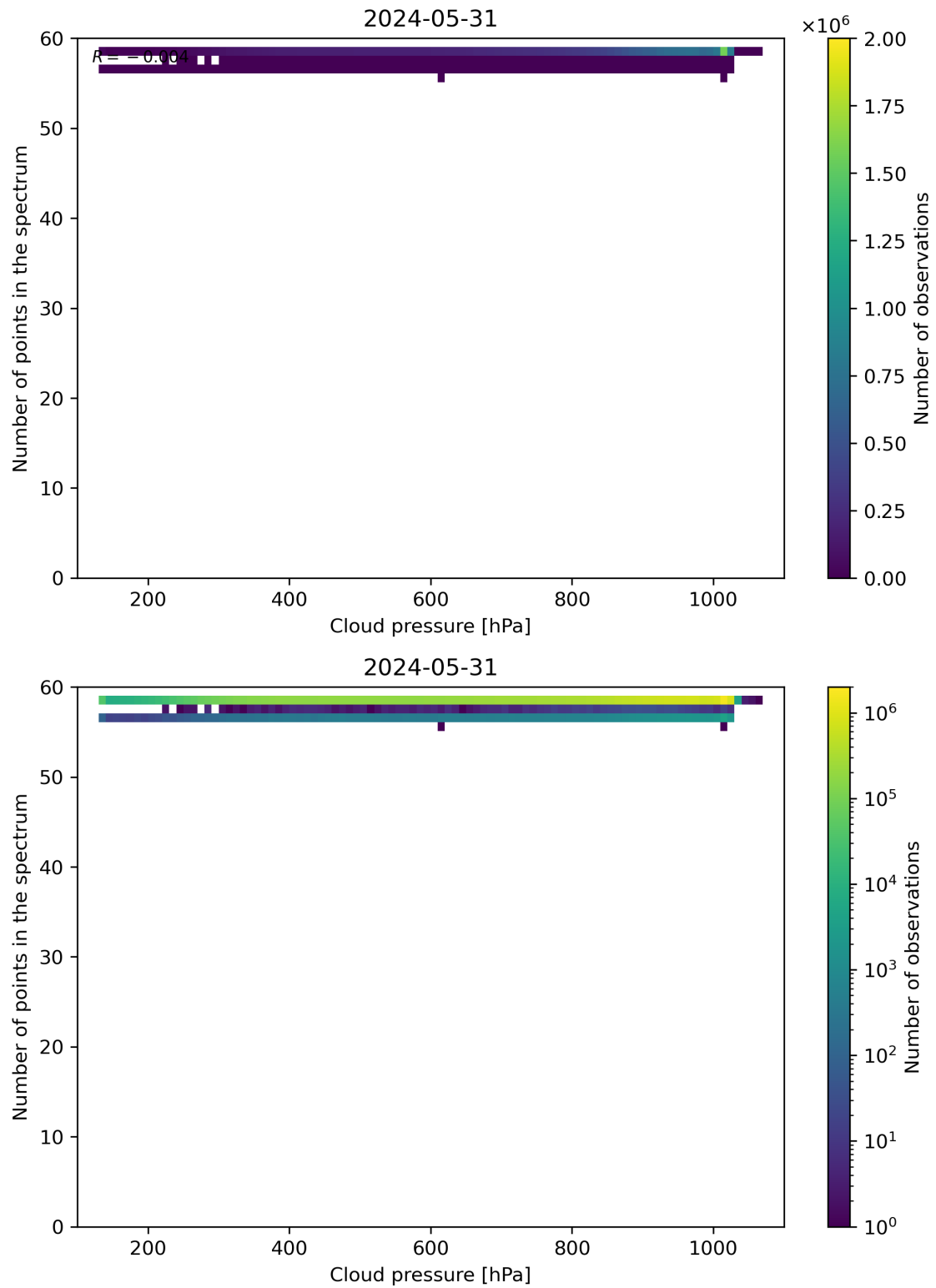
Figure 82: Scatter density plot of “Cloud pressure” against “Number of points in the spectrum” for 2024-05-30 to 2024-06-01.
