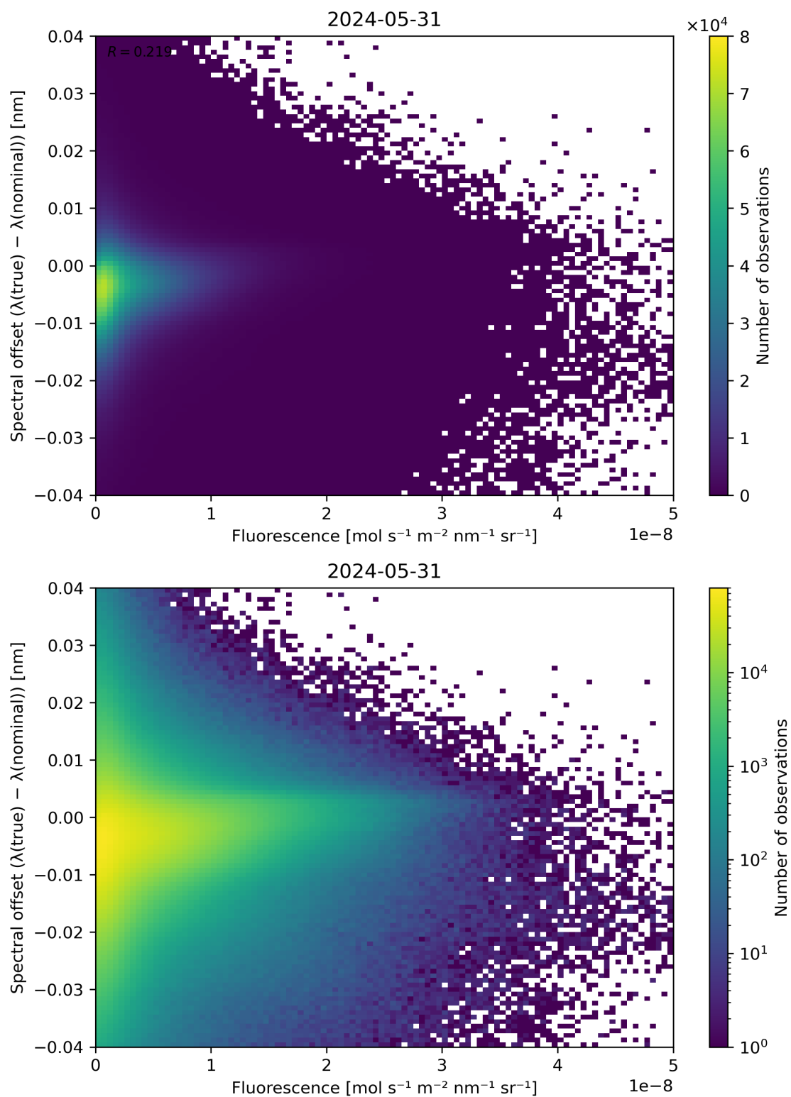
Figure 87: Scatter density plot of “Fluorescence” against “Spectral offset ( \lambda(\text{true}) - \lambda(\text{nominal}) )” for 2024-05-30 to 2024-06-01.
