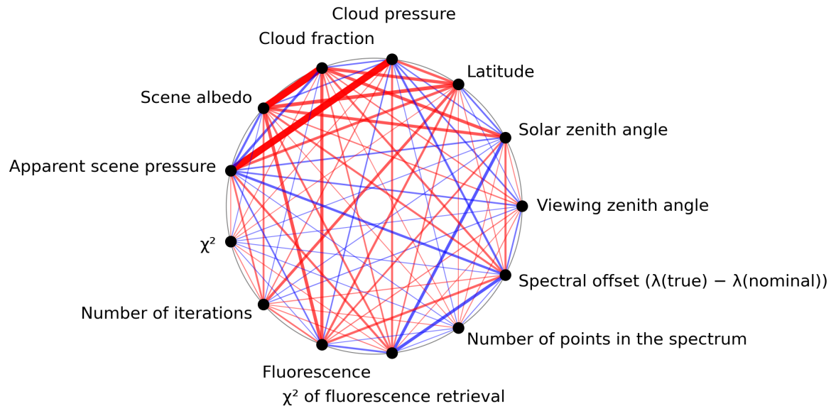
Figure 1: Map of correlation graph for 2024-05-30 to 2024-06-01.
