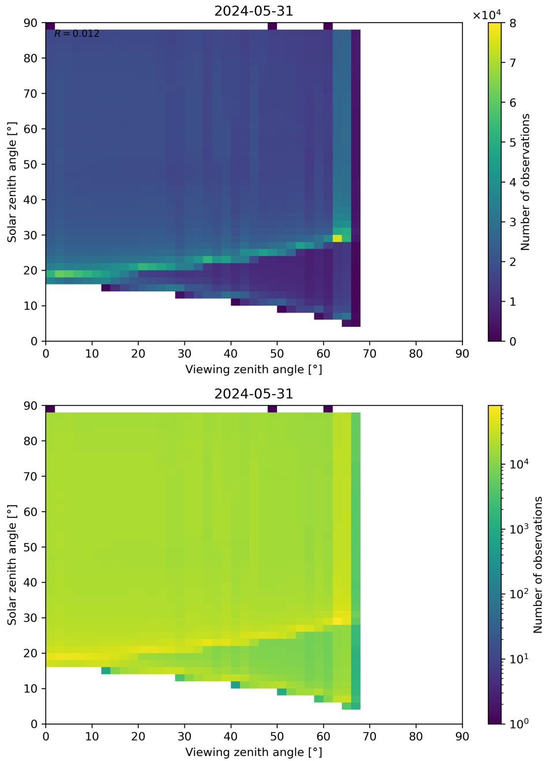
Figure 127: Scatter density plot of “Viewing zenith angle” against “Solar zenith angle” for 2024-05-30 to 2024-06-01.
