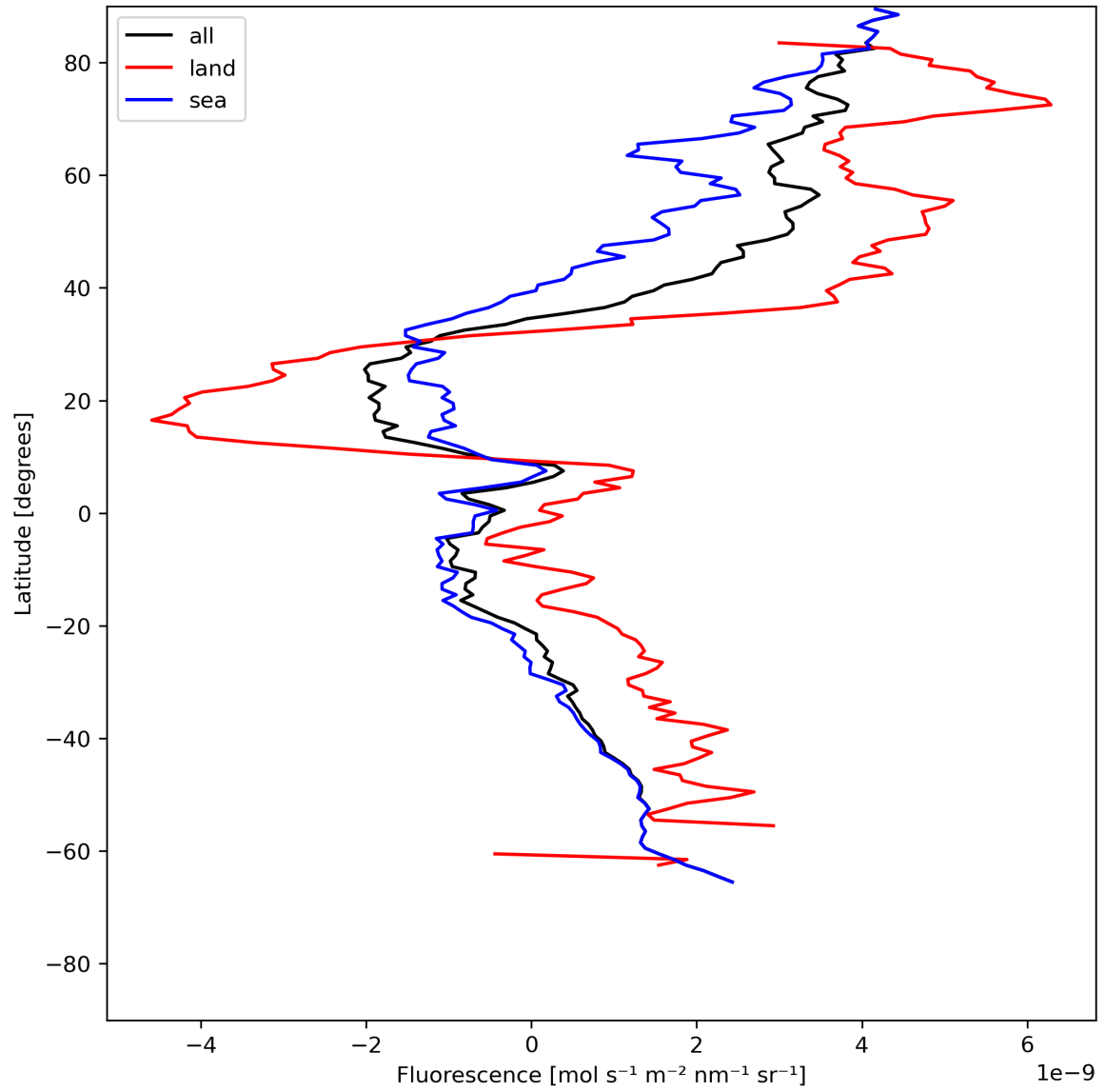
Figure 23: Zonal average of “Fluorescence” for 2024-05-30 to 2024-06-01.
