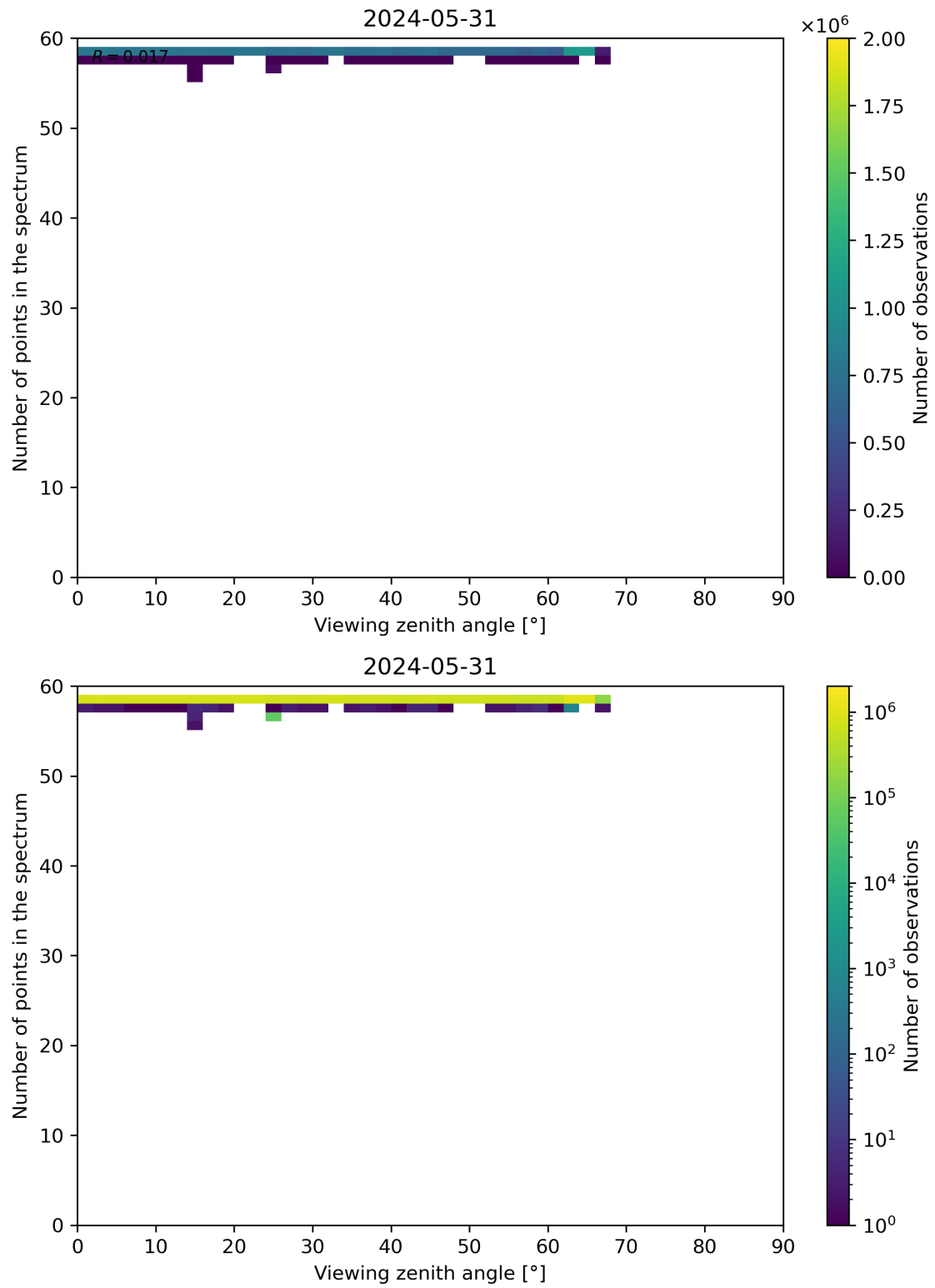
Figure 125: Scatter density plot of “Viewing zenith angle” against “Number of points in the spectrum” for 2024-05-30 to 2024-06-01.
