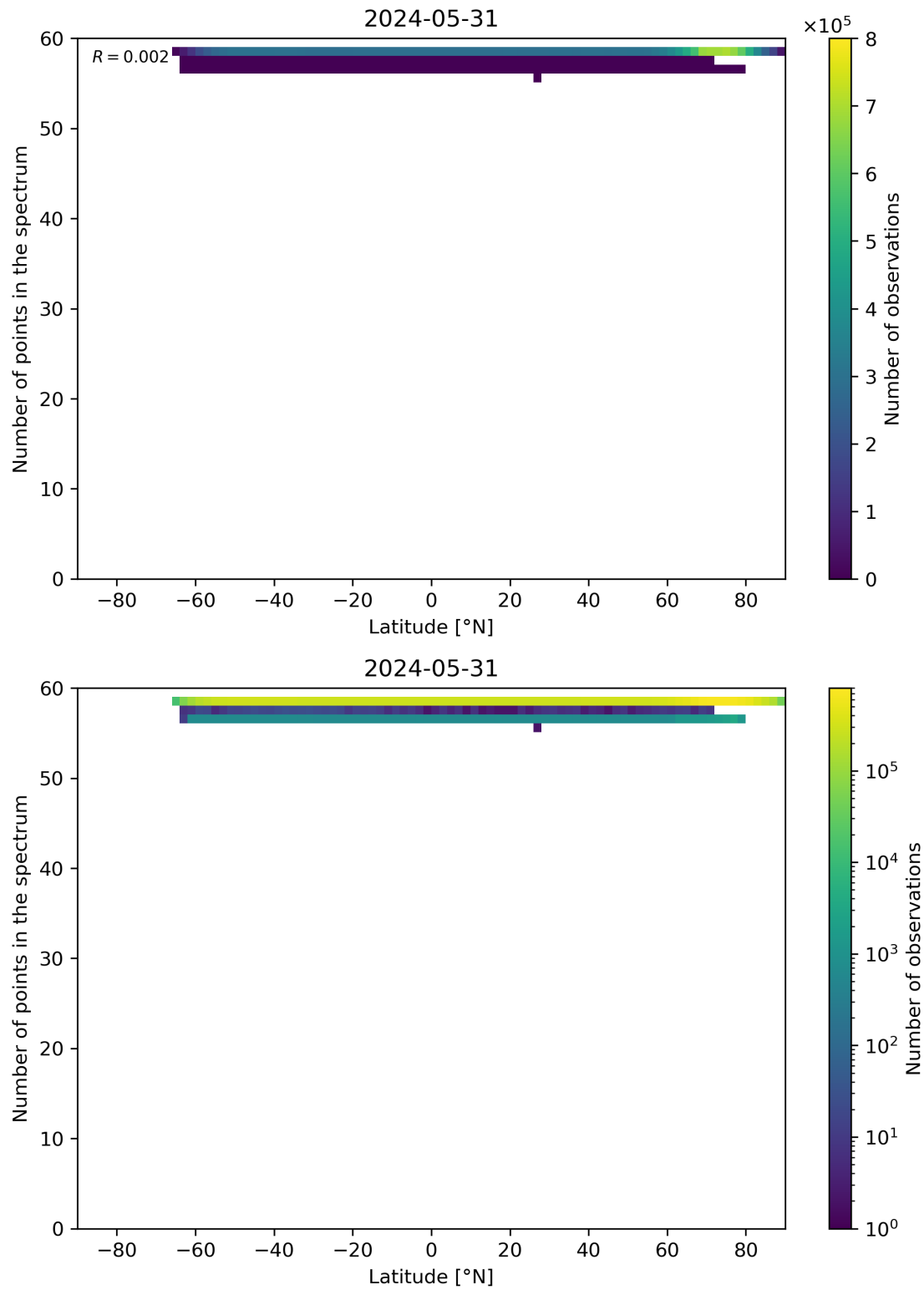
Figure 94: Scatter density plot of “Latitude” against “Number of points in the spectrum” for 2024-05-30 to 2024-06-01.
