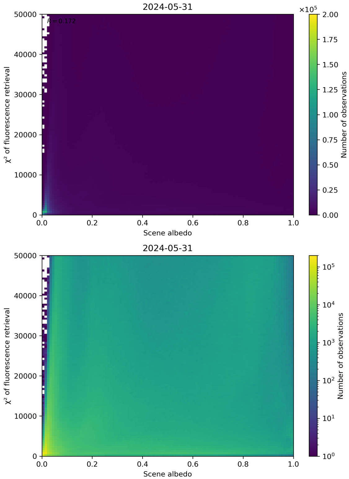
Figure 103: Scatter density plot of “Scene albedo” against “ \chi^2 of fluorescence retrieval” for 2024-05-30 to 2024-06-01.
