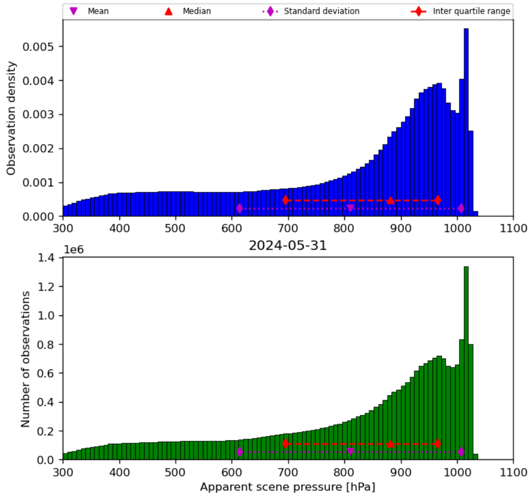
Figure 36: Histogram of “Apparent scene pressure” for 2024-05-30 to 2024-06-01
