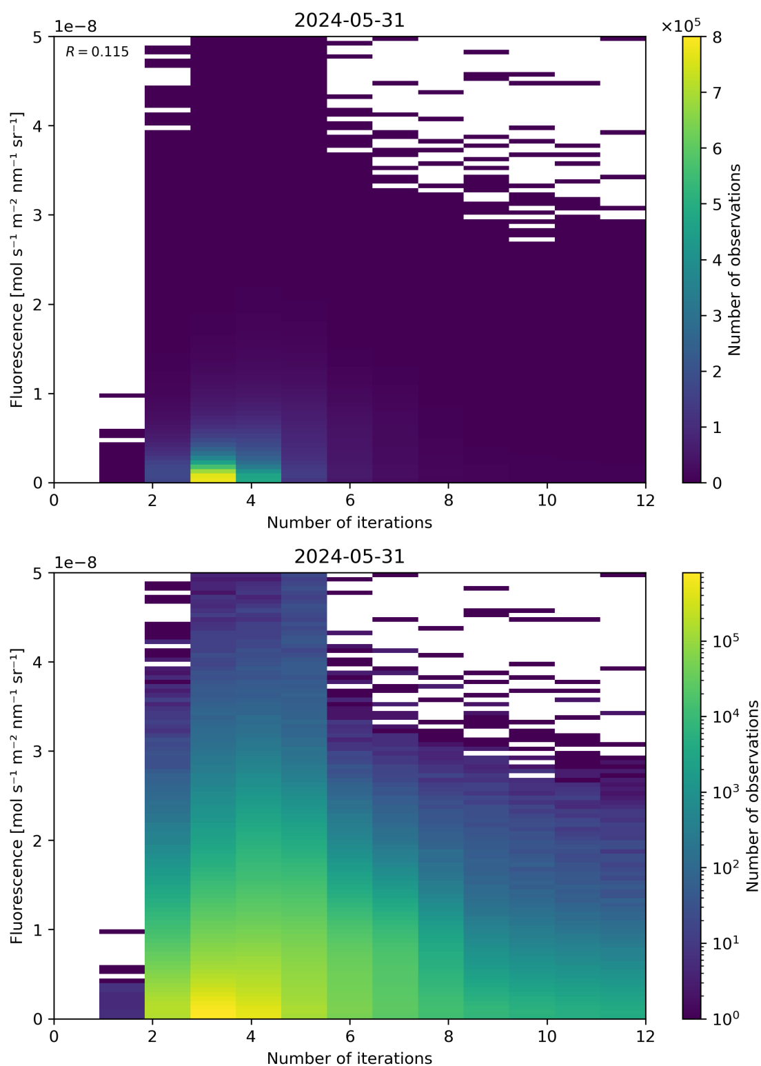
Figure 98: Scatter density plot of “Number of iterations” against “Fluorescence” for 2024-05-30 to 2024-06-01.
