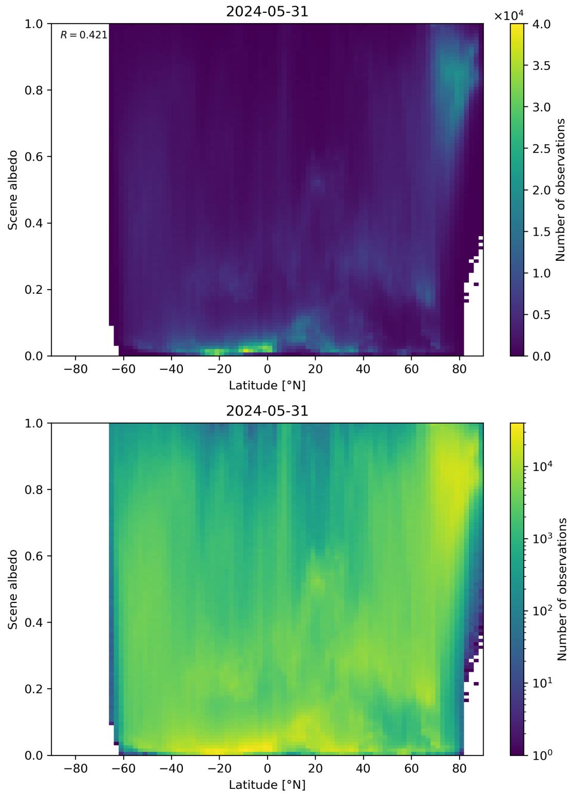
Figure 95: Scatter density plot of “Latitude” against “Scene albedo” for 2024-05-30 to 2024-06-01.
