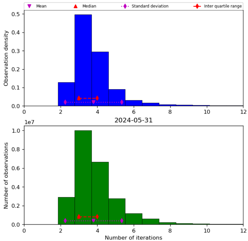
Figure 39: Histogram of “Number of iterations” for 2024-05-30 to 2024-06-01
