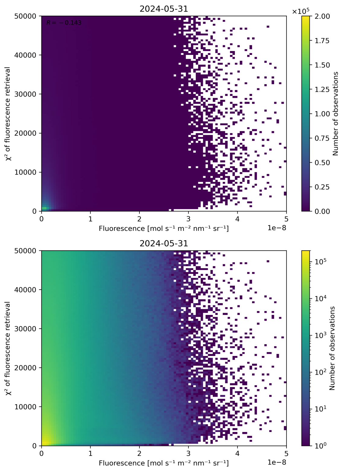
Figure 85: Scatter density plot of “Fluorescence” against “ \chi^2 of fluorescence retrieval” for 2024-05-30 to 2024-06-01.
