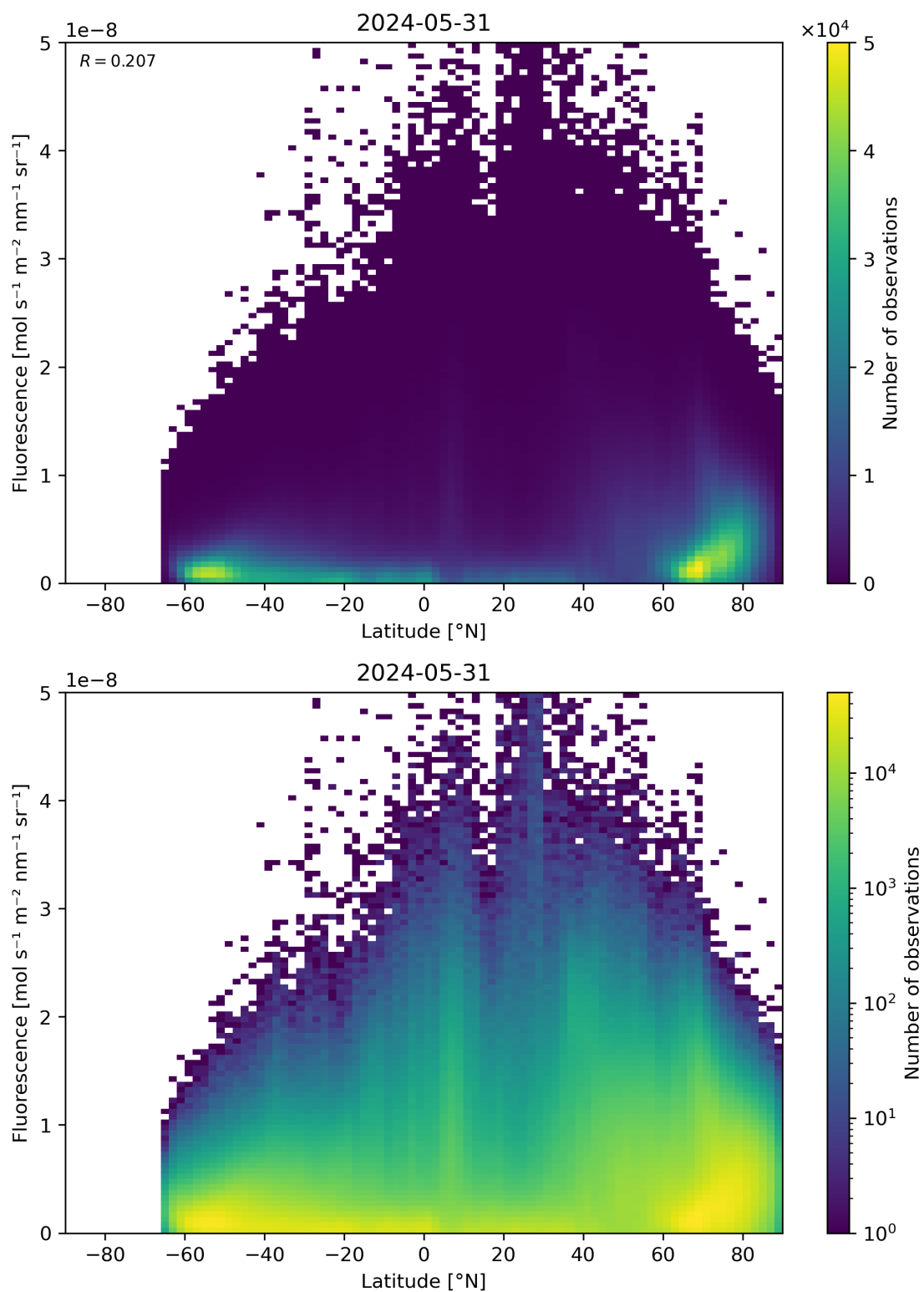
Figure 92: Scatter density plot of “Latitude” against “Fluorescence” for 2024-05-30 to 2024-06-01.
