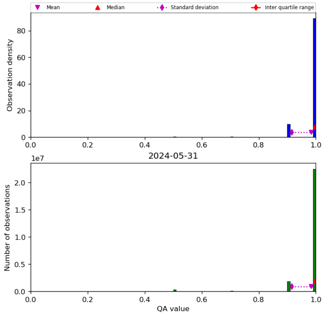
Figure 29: Histogram of “QA value” for 2024-05-30 to 2024-06-01
