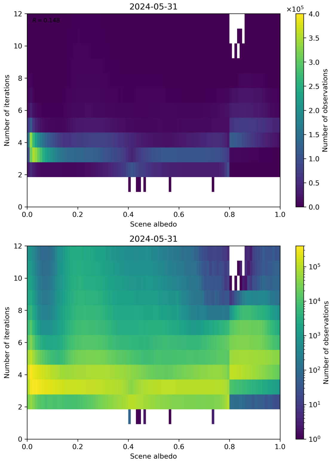
Figure 105: Scatter density plot of “Scene albedo” against “Number of iterations” for 2024-05-30 to 2024-06-01.
