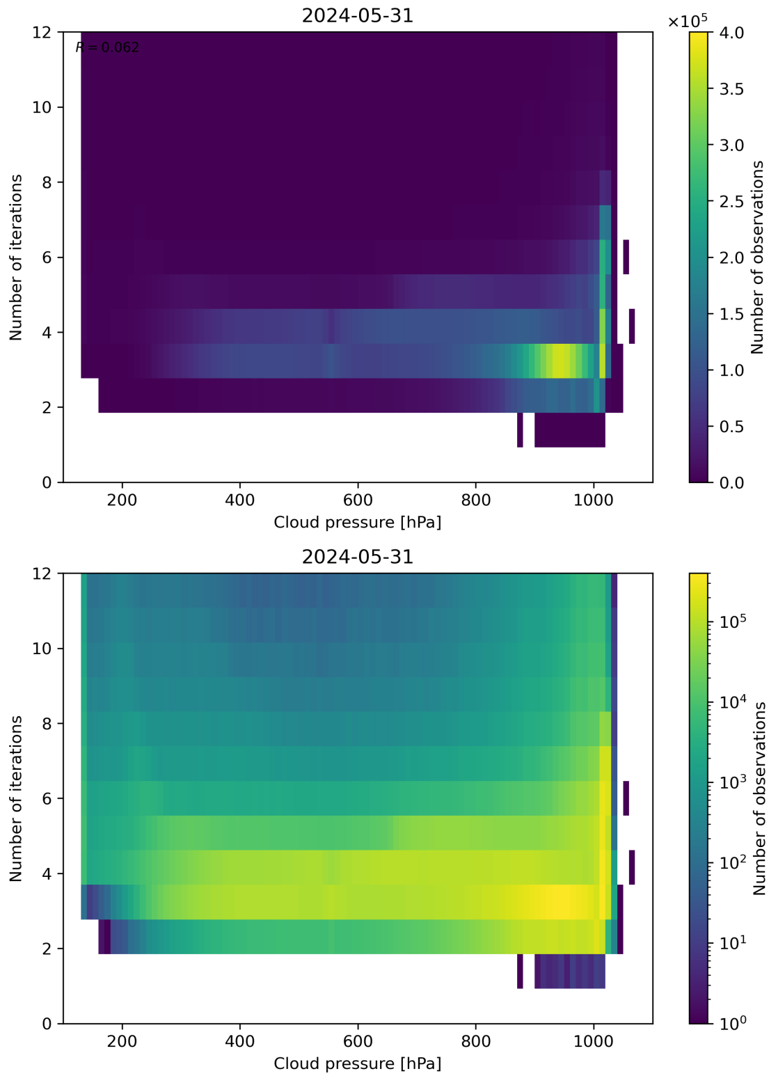
Figure 81: Scatter density plot of “Cloud pressure” against “Number of iterations” for 2024-05-30 to 2024-06-01.
