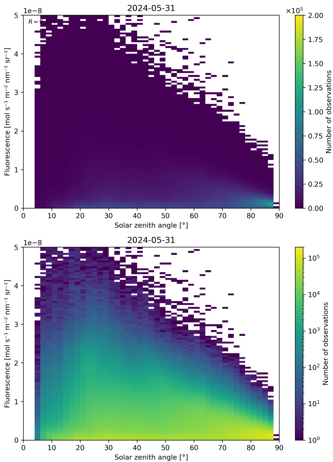
Figure 112: Scatter density plot of “Solar zenith angle” against “Fluorescence” for 2024-05-30 to 2024-06-01.
