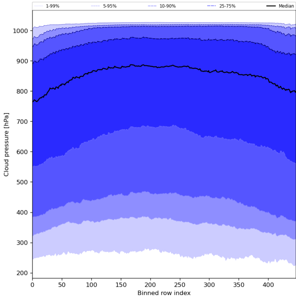
Figure 47: Along track statistics of “Cloud pressure” for 2024-05-30 to 2024-06-01
