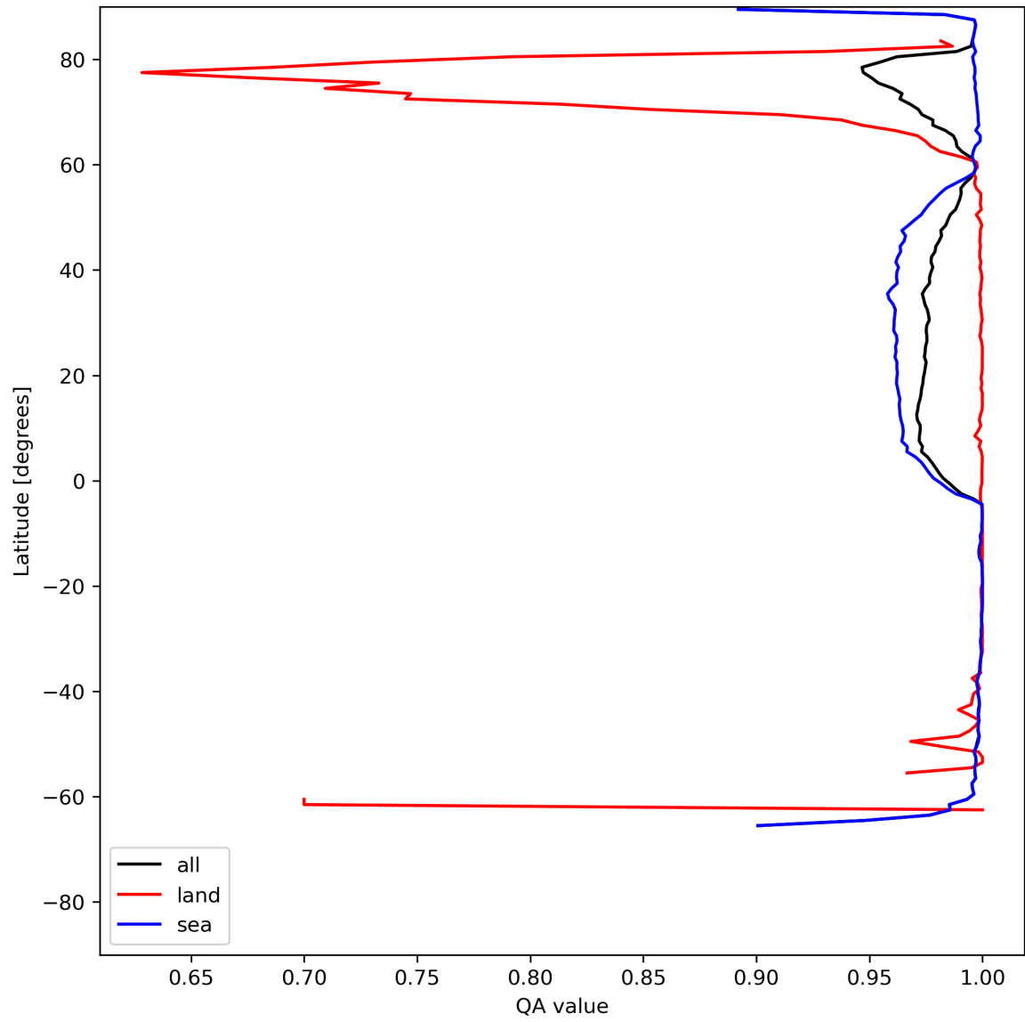
Figure 12: Zonal average of “QA value” for 2024-05-30 to 2024-06-01.
