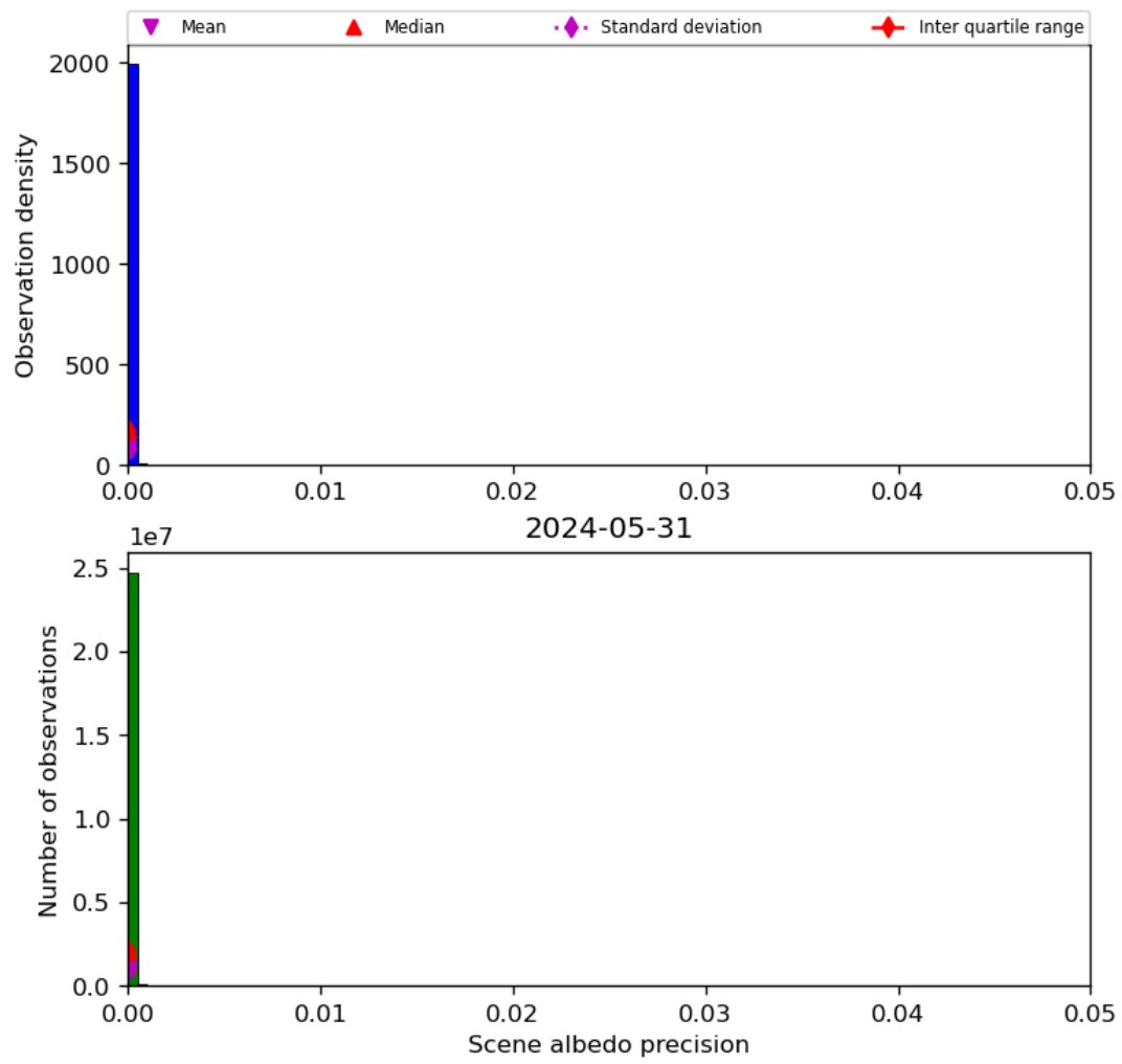
Figure 35: Histogram of “Scene albedo precision” for 2024-05-30 to 2024-06-01
