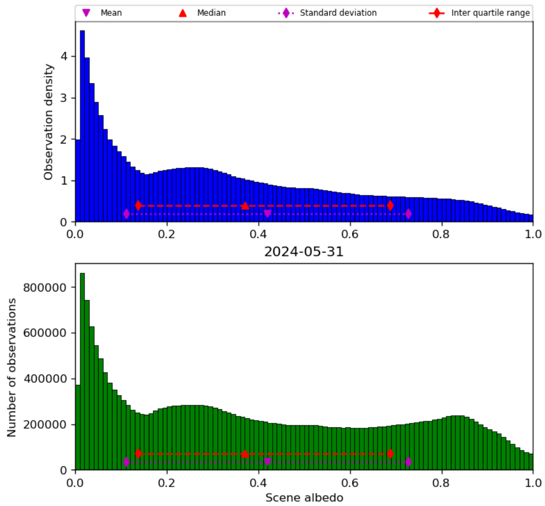
Figure 34: Histogram of “Scene albedo” for 2024-05-30 to 2024-06-01
