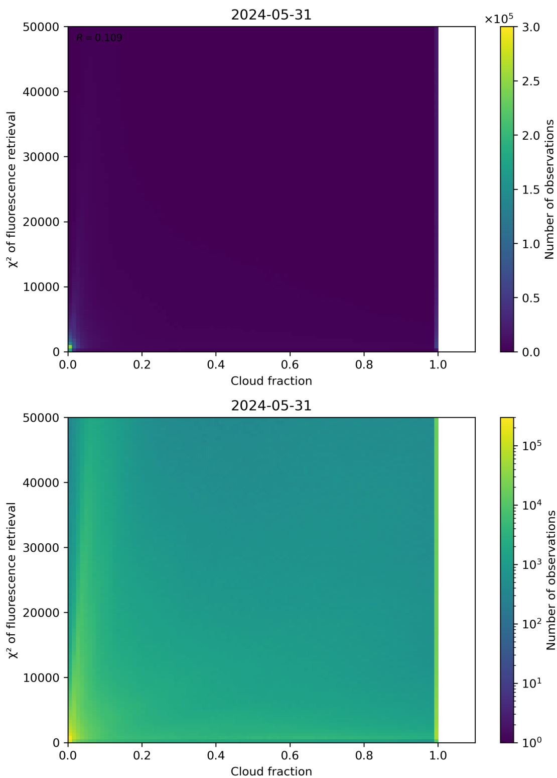
Figure 71: Scatter density plot of “Cloud fraction” against “ \chi^2 of fluorescence retrieval” for 2024-05-30 to 2024-06-01.
