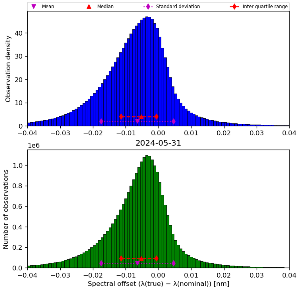
Figure 45: Histogram of “Spectral offset ( \lambda(\text{true}) - \lambda(\text{nominal}) )” for 2024-05-30 to 2024-06-01
