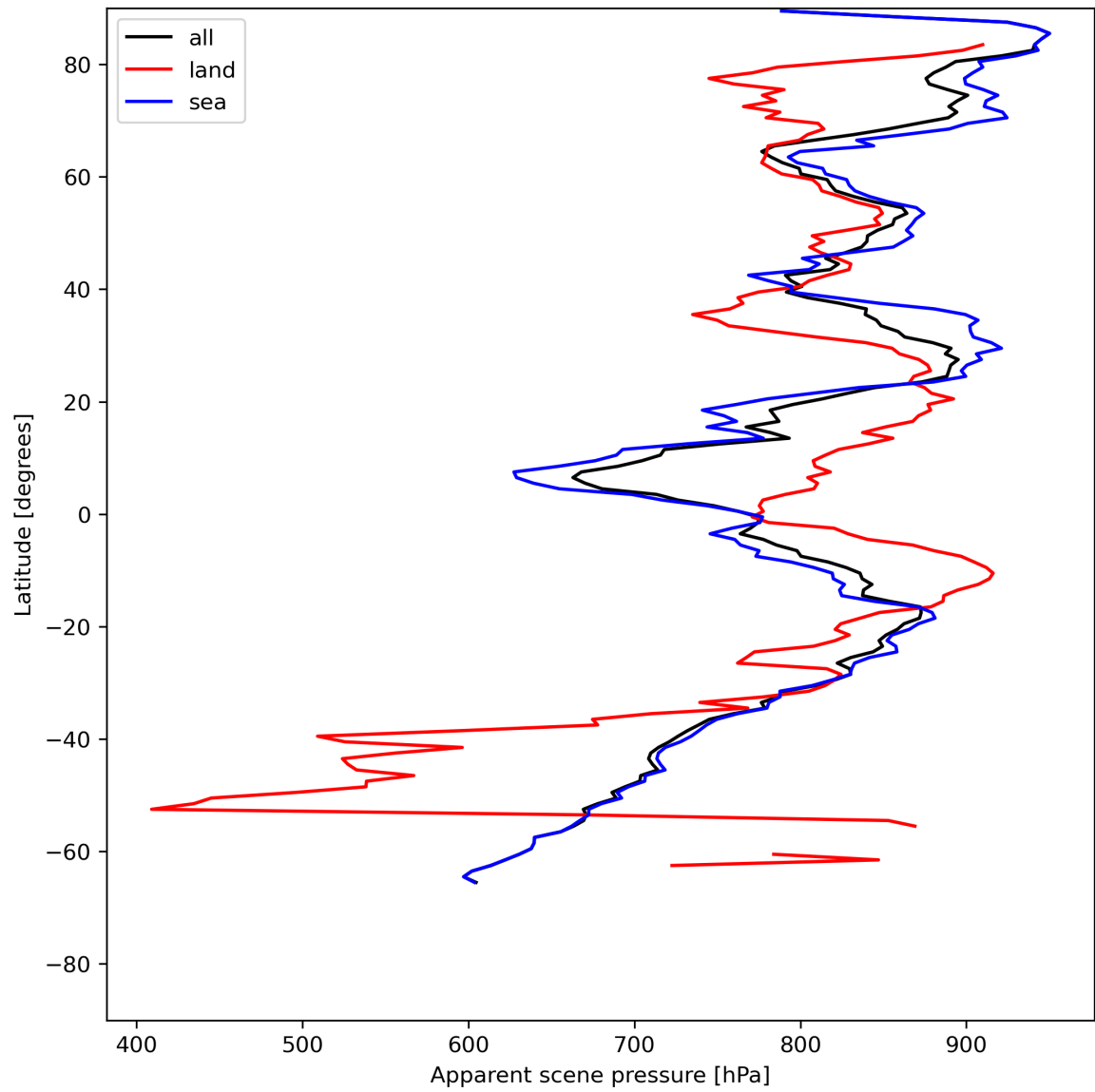
Figure 19: Zonal average of “Apparent scene pressure” for 2024-05-30 to 2024-06-01.
