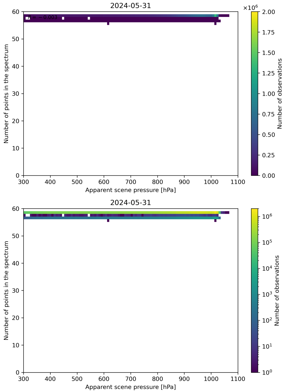
Figure 66: Scatter density plot of “Apparent scene pressure” against “Number of points in the spectrum” for 2024-05-30 to 2024-06-01.
