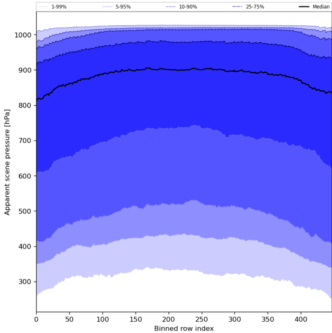
Figure 53: Along track statistics of “Apparent scene pressure” for 2024-05-30 to 2024-06-01
