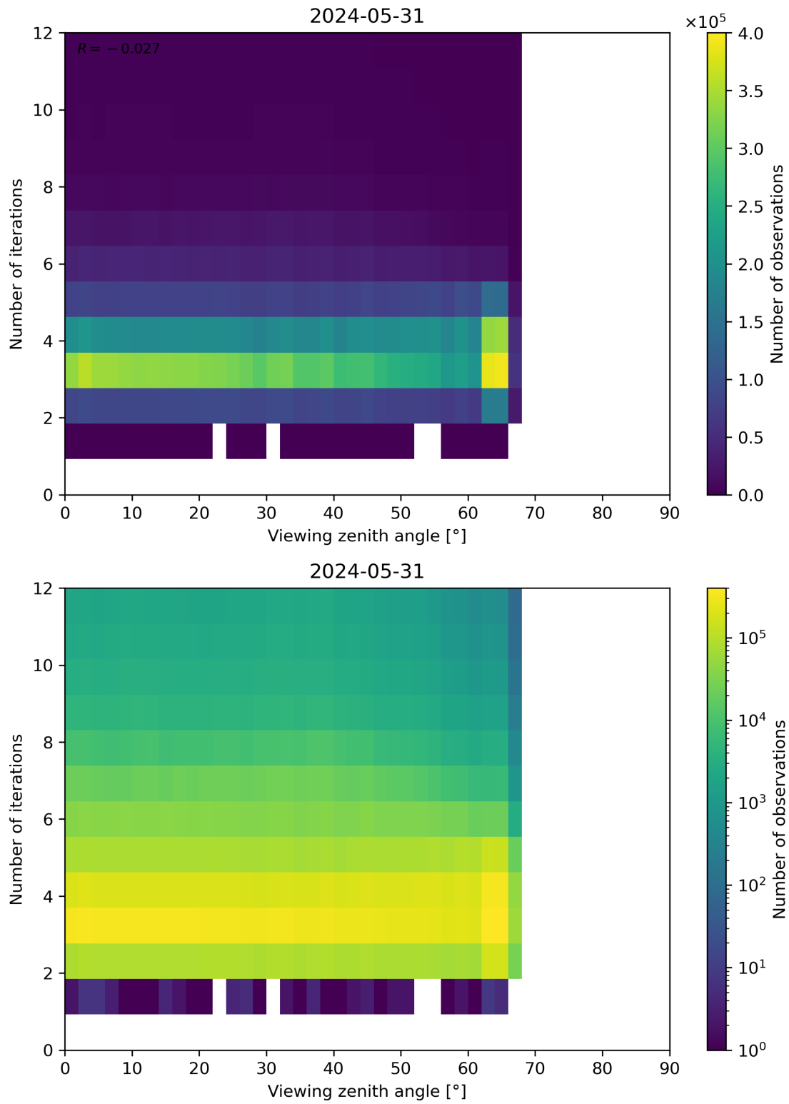
Figure 124: Scatter density plot of “Viewing zenith angle” against “Number of iterations” for 2024-05-30 to 2024-06-01.
