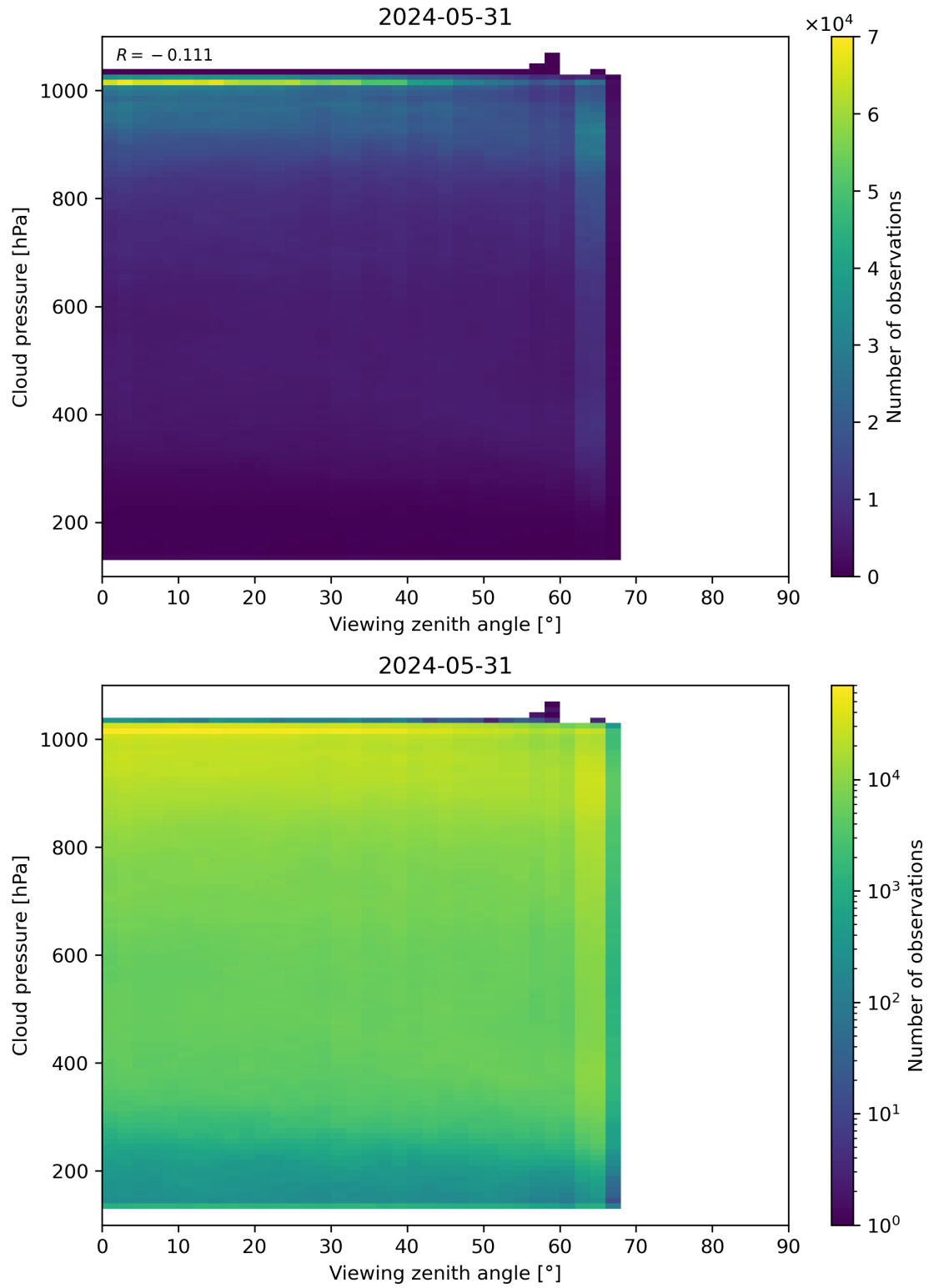
Figure 121: Scatter density plot of “Viewing zenith angle” against “Cloud pressure” for 2024-05-30 to 2024-06-01.
