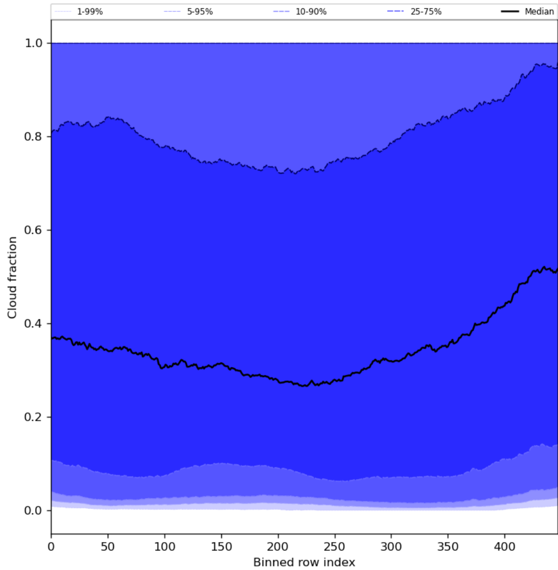
Figure 49: Along track statistics of “Cloud fraction” for 2024-05-30 to 2024-06-01
