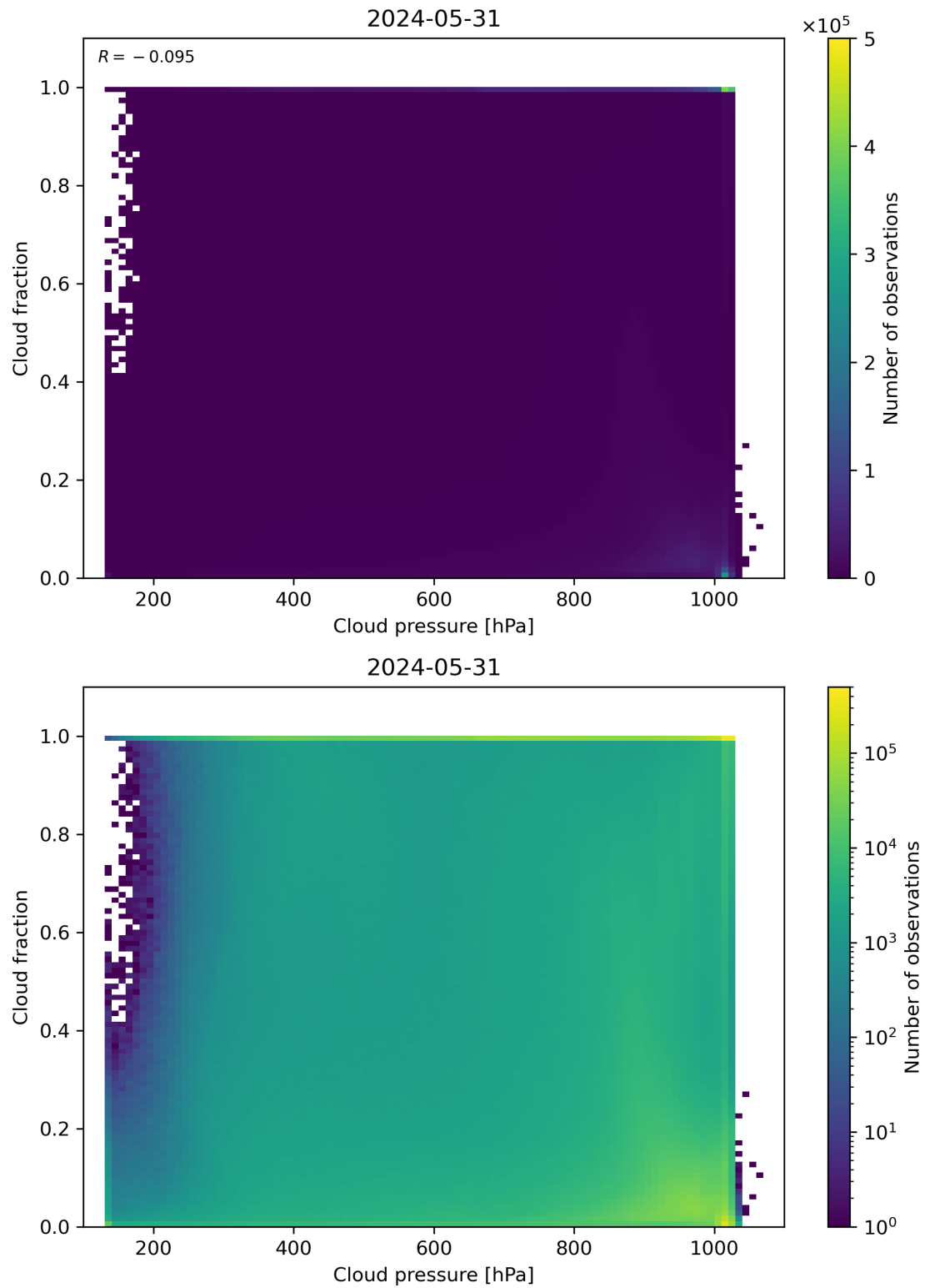
Figure 79: Scatter density plot of “Cloud pressure” against “Cloud fraction” for 2024-05-30 to 2024-06-01.
