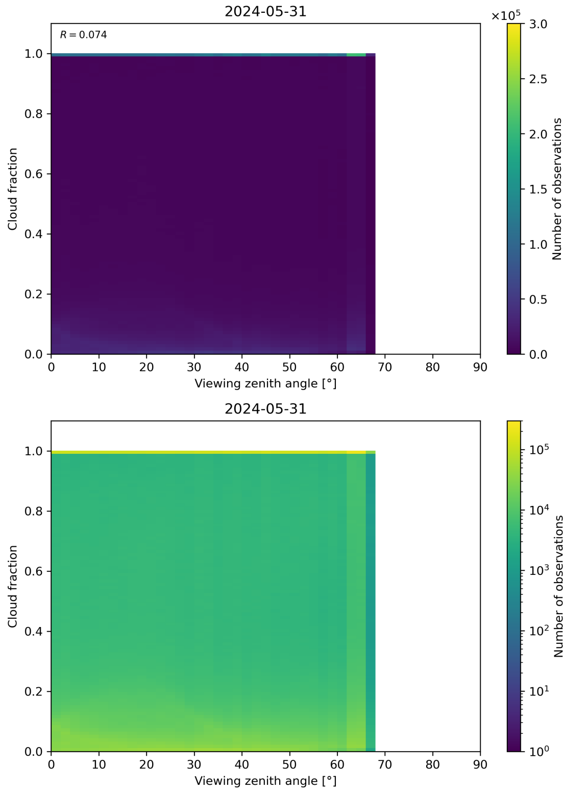
Figure 120: Scatter density plot of “Viewing zenith angle” against “Cloud fraction” for 2024-05-30 to 2024-06-01.
