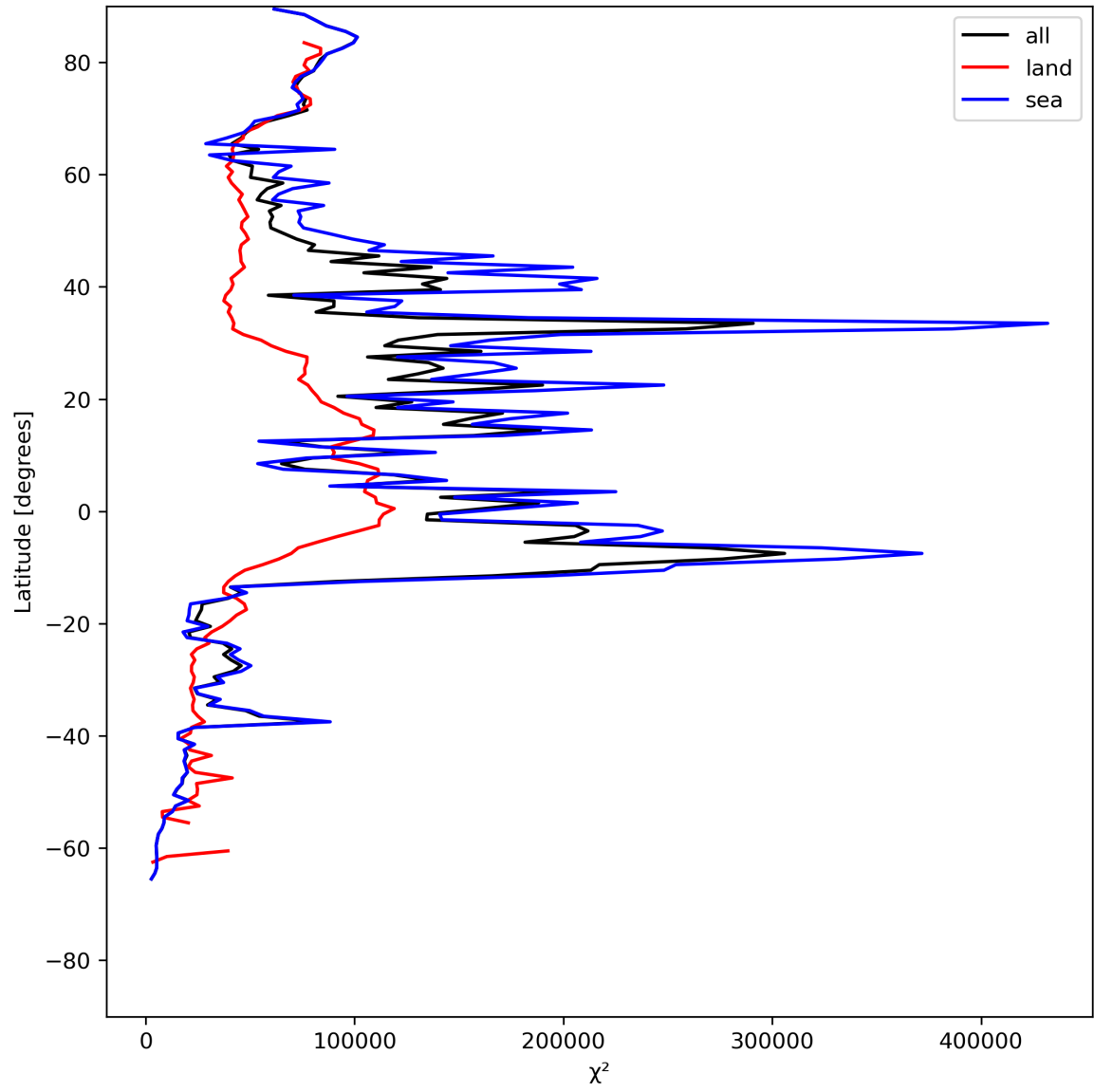
Figure 21: Zonal average of “ \chi^2 ” for 2024-05-30 to 2024-06-01.
