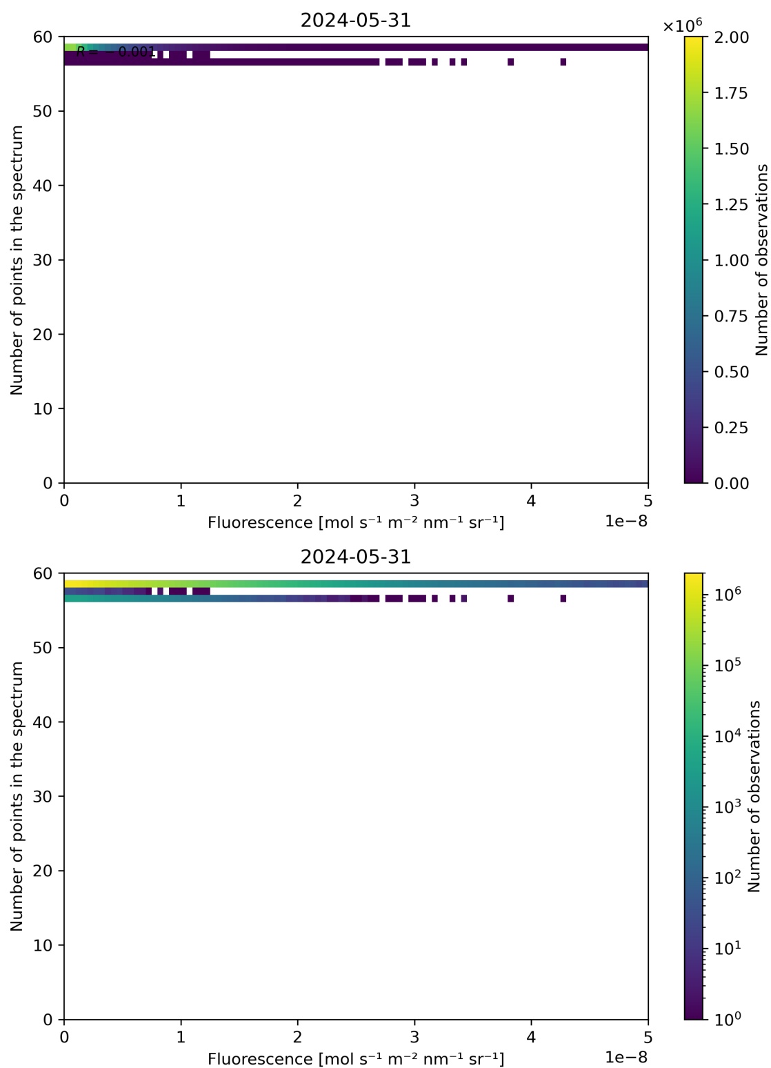
Figure 86: Scatter density plot of “Fluorescence” against “Number of points in the spectrum” for 2024-05-30 to 2024-06-01.
