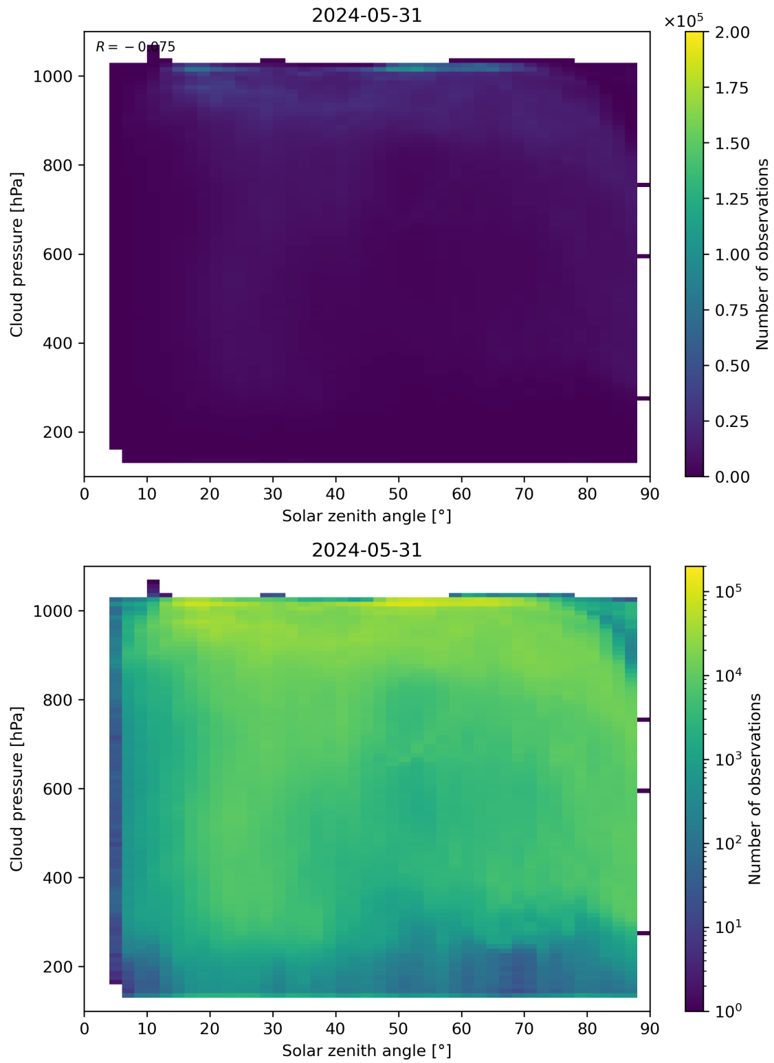
Figure 111: Scatter density plot of “Solar zenith angle” against “Cloud pressure” for 2024-05-30 to 2024-06-01.
