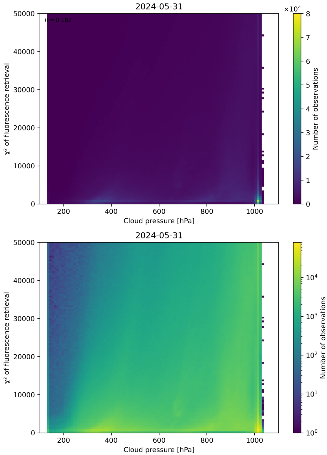
Figure 78: Scatter density plot of “Cloud pressure” against “ \chi^2 of fluorescence retrieval” for 2024-05-30 to 2024-06-01.
