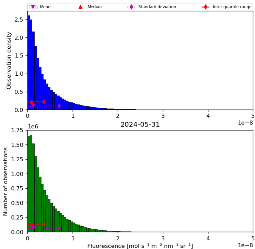
Figure 40: Histogram of “Fluorescence” for 2024-05-30 to 2024-06-01
