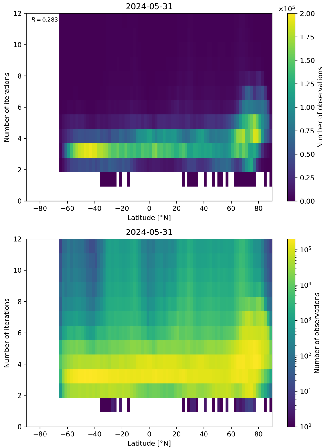
Figure 93: Scatter density plot of “Latitude” against “Number of iterations” for 2024-05-30 to 2024-06-01.
