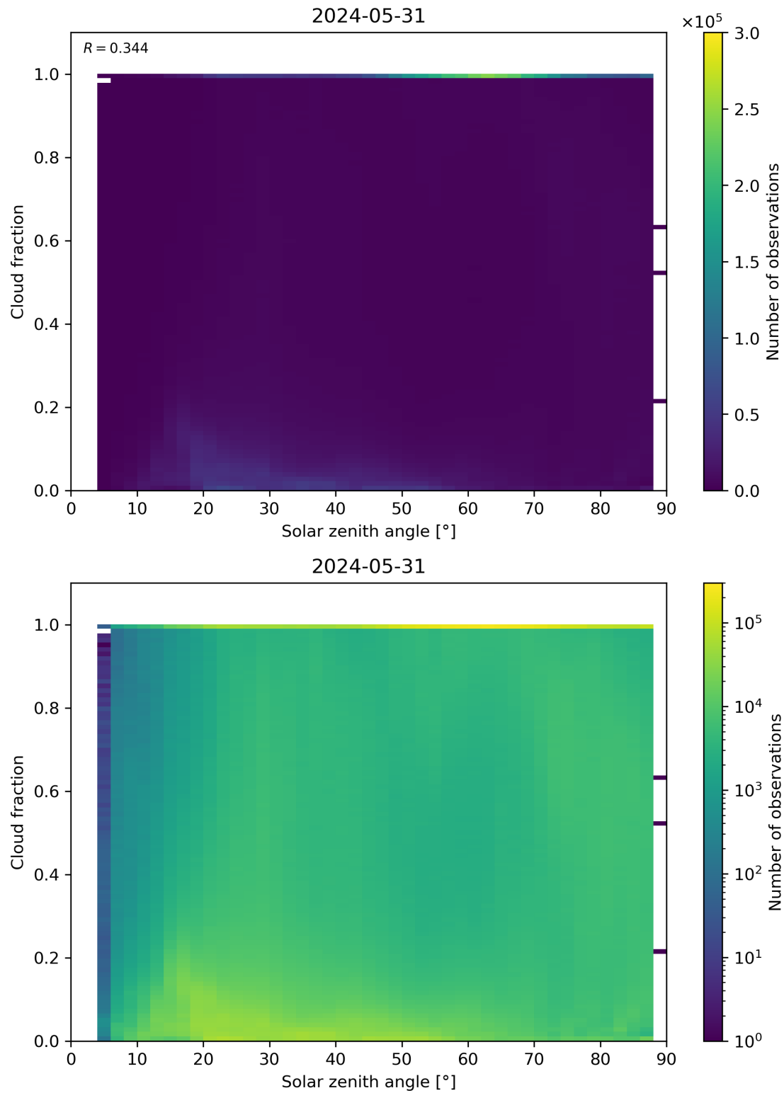
Figure 110: Scatter density plot of “Solar zenith angle” against “Cloud fraction” for 2024-05-30 to 2024-06-01.
