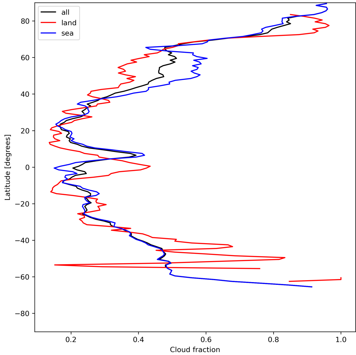
Figure 15: Zonal average of “Cloud fraction” for 2024-05-30 to 2024-06-01.
