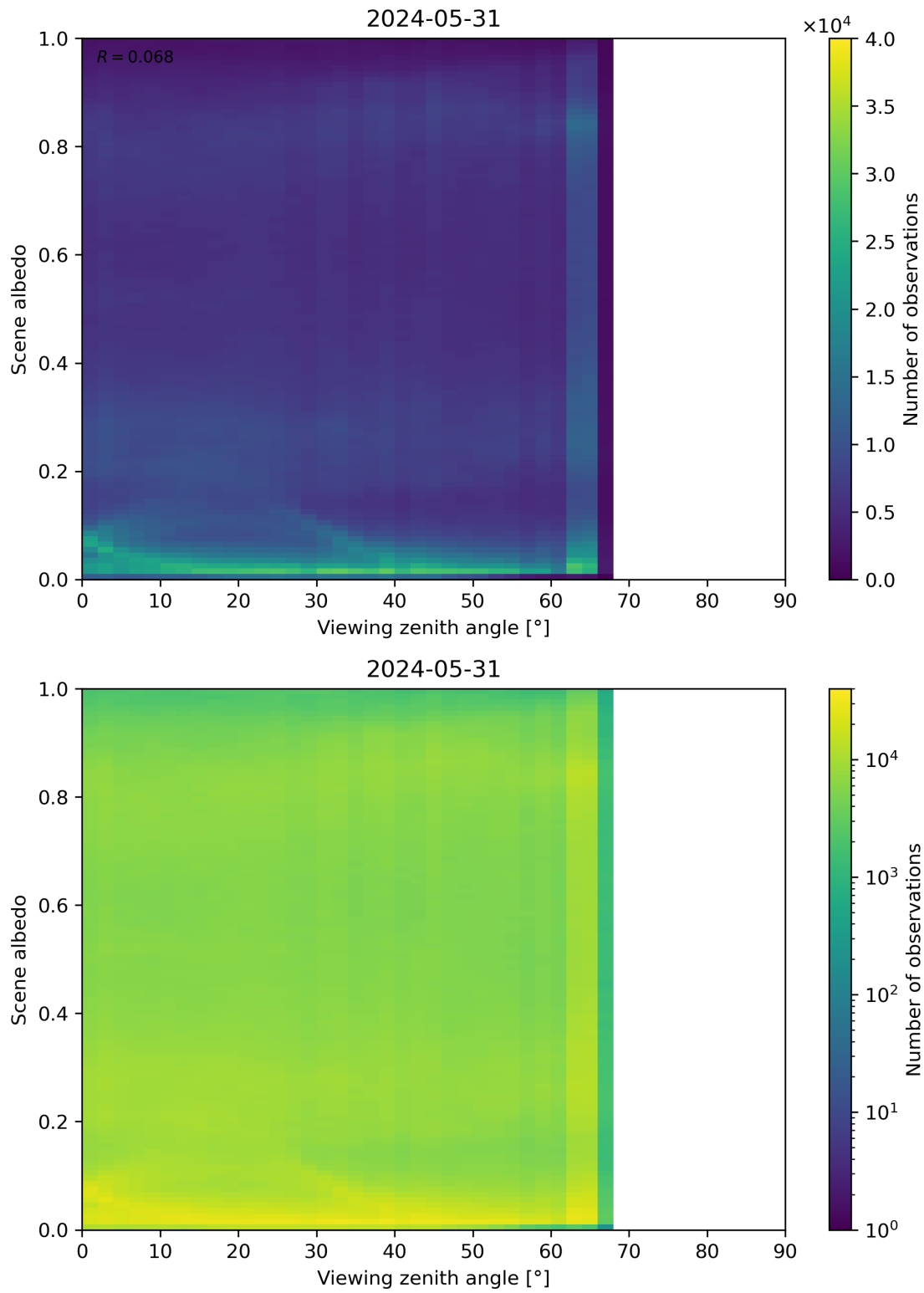
Figure 126: Scatter density plot of “Viewing zenith angle” against “Scene albedo” for 2024-05-30 to 2024-06-01.
