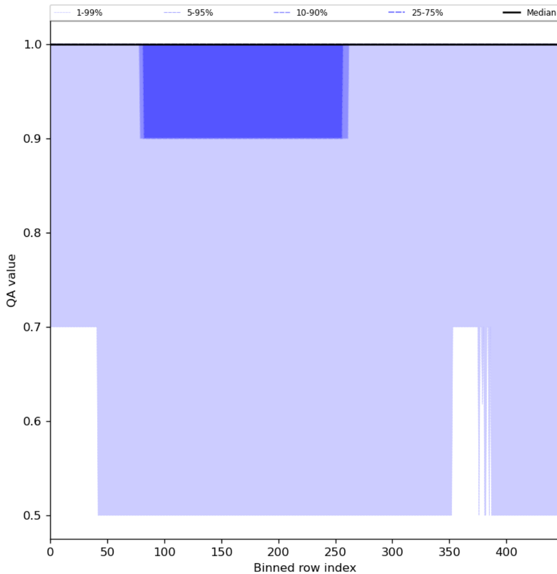
Figure 46: Along track statistics of “QA value” for 2024-05-30 to 2024-06-01
