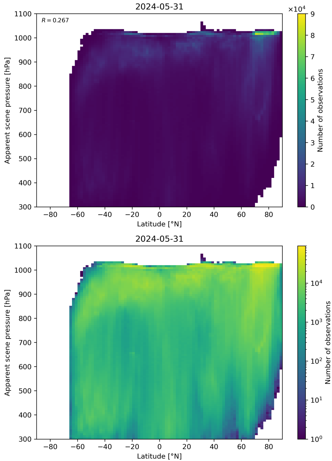
Figure 88: Scatter density plot of “Latitude” against “Apparent scene pressure” for 2024-05-30 to 2024-06-01.
