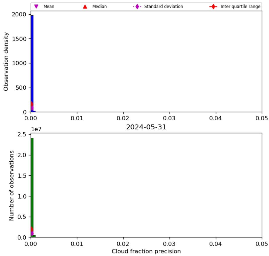
Figure 33: Histogram of “Cloud fraction precision” for 2024-05-30 to 2024-06-01
