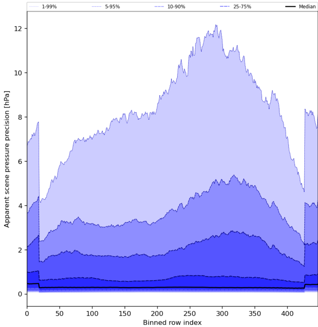
Figure 54: Along track statistics of “Apparent scene pressure precision” for 2024-05-30 to 2024-06-01
