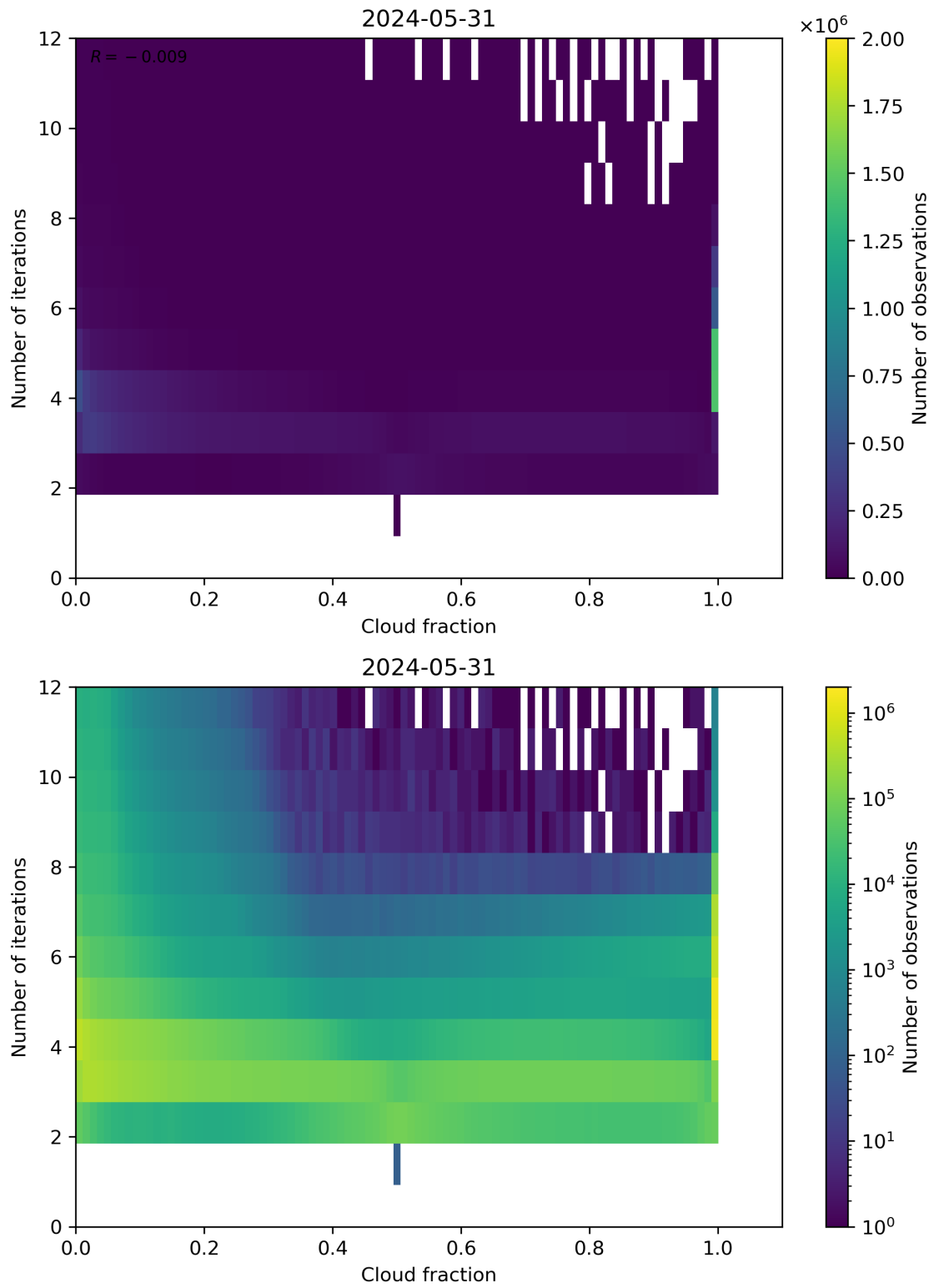
Figure 73: Scatter density plot of “Cloud fraction” against “Number of iterations” for 2024-05-30 to 2024-06-01.
