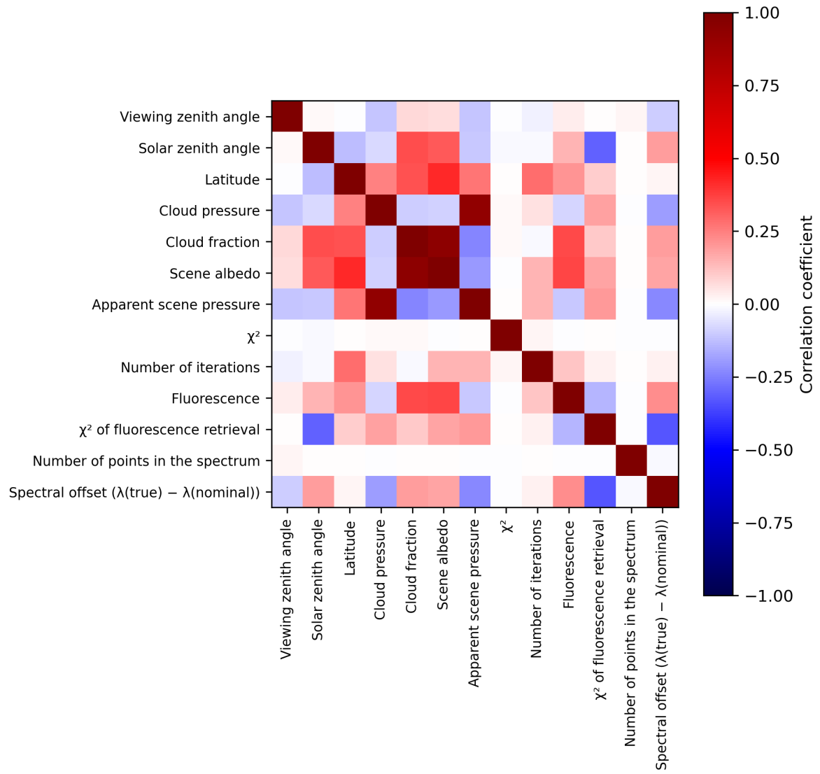
Figure 2: Map of correlation matrix for 2024-05-30 to 2024-06-01.
