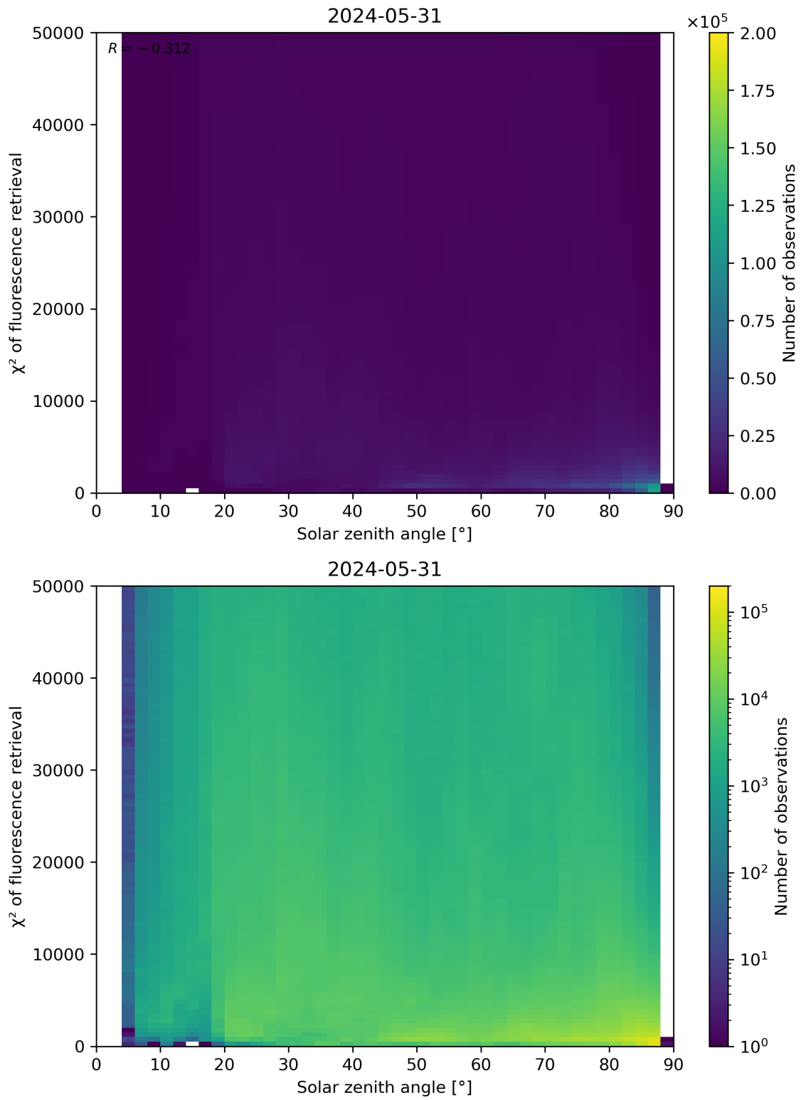
Figure 109: Scatter density plot of “Solar zenith angle” against “ \chi^2 of fluorescence retrieval” for 2024-05-30 to 2024-06-01.
