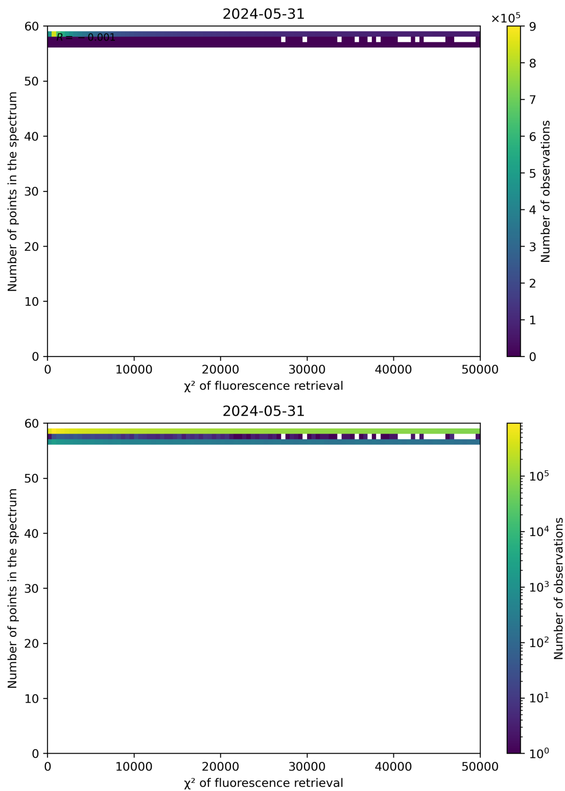
Figure 68: Scatter density plot of “ \chi^2 of fluorescence retrieval” against “Number of points in the spectrum” for 2024-05-30 to 2024-06-01.
