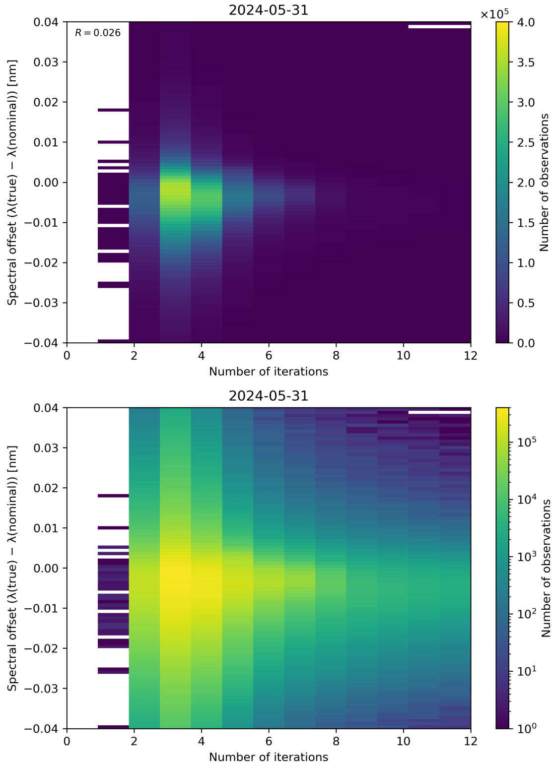
Figure 100: Scatter density plot of “Number of iterations” against “Spectral offset ( \lambda(\text{true}) - \lambda(\text{nominal}) )” for 2024-05-30 to 2024-06-01.
