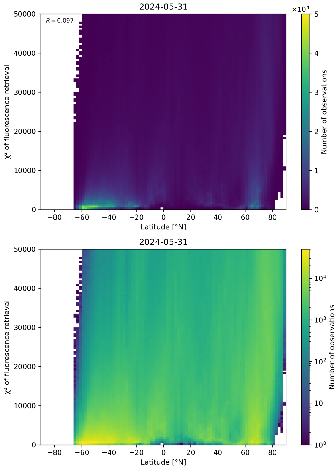
Figure 89: Scatter density plot of “Latitude” against “ \chi^2 of fluorescence retrieval” for 2024-05-30 to 2024-06-01.
