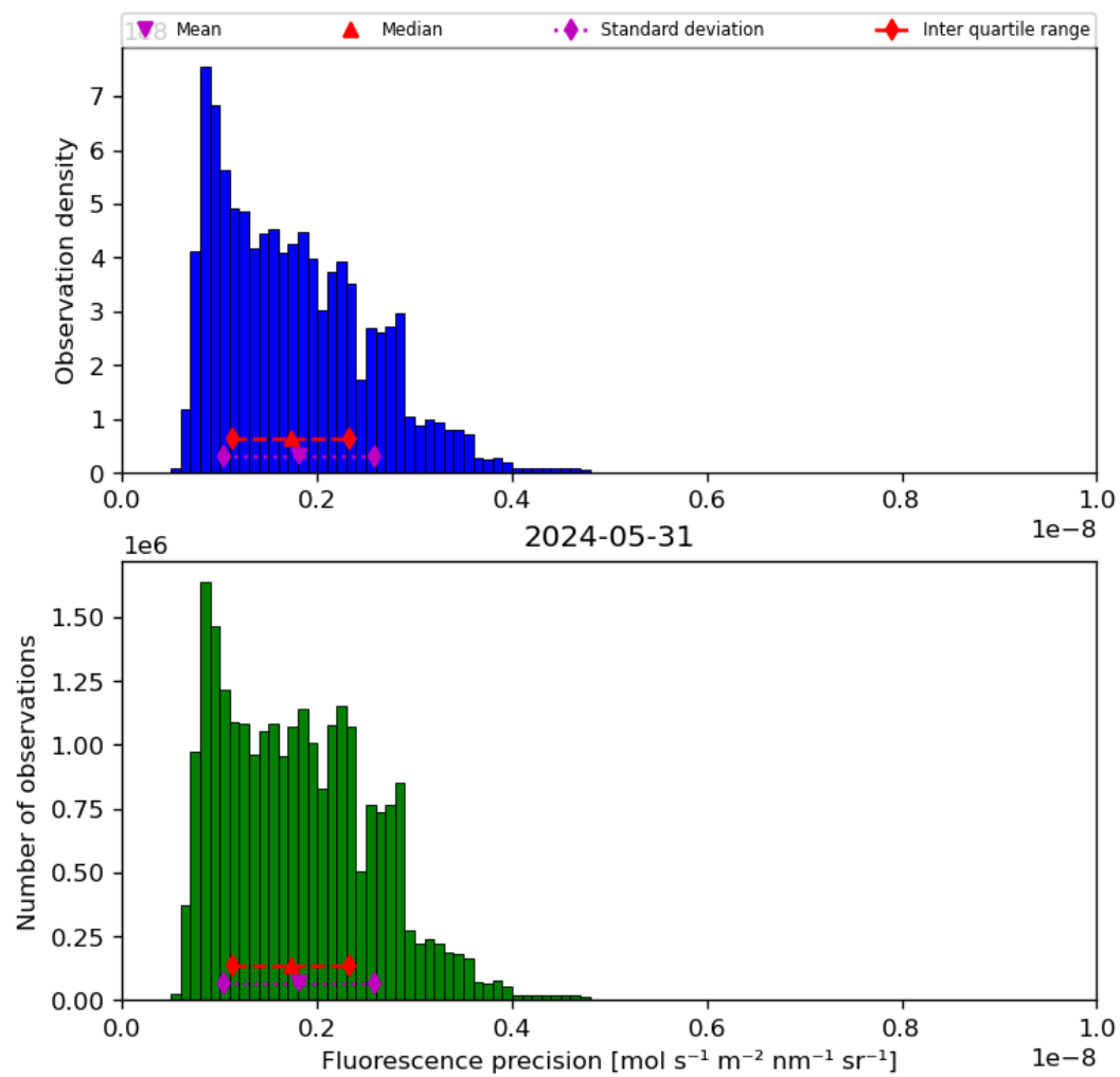
Figure 41: Histogram of “Fluorescence precision” for 2024-05-30 to 2024-06-01
