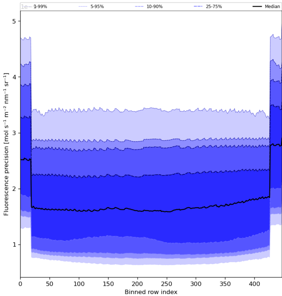
Figure 58: Along track statistics of “Fluorescence precision” for 2024-05-30 to 2024-06-01
