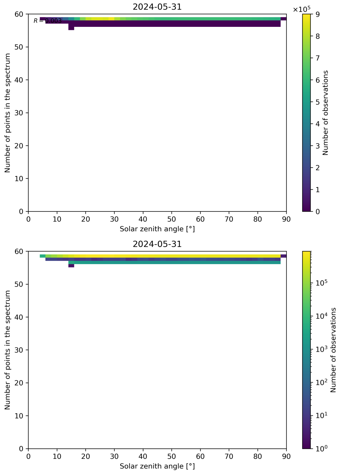
Figure 115: Scatter density plot of “Solar zenith angle” against “Number of points in the spectrum” for 2024-05-30 to 2024-06-01.
