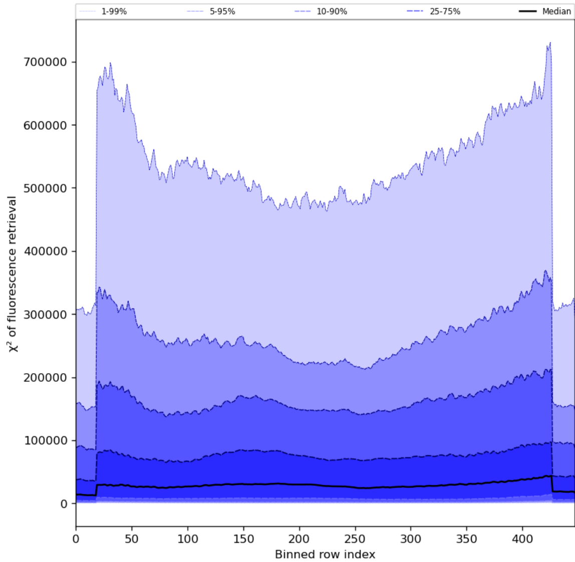
Figure 59: Along track statistics of “ \chi^2 of fluorescence retrieval” for 2024-05-30 to 2024-06-01
