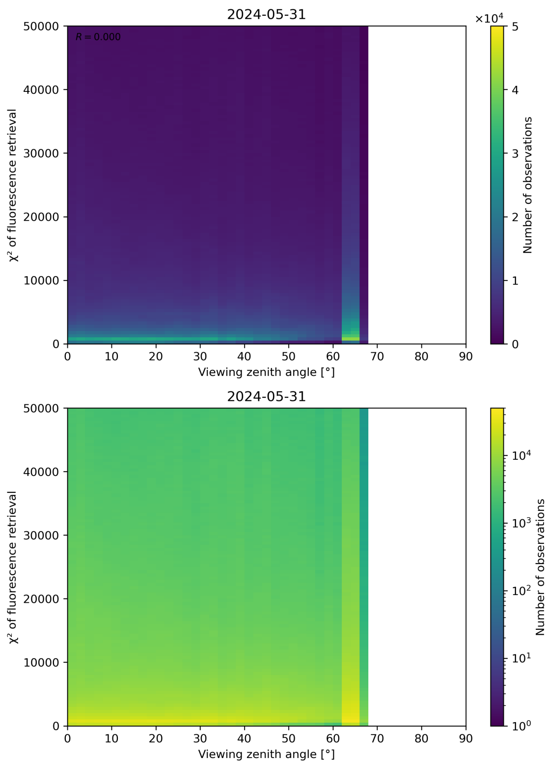
Figure 119: Scatter density plot of “Viewing zenith angle” against “ \chi^2 of fluorescence retrieval” for 2024-05-30 to 2024-06-01.
