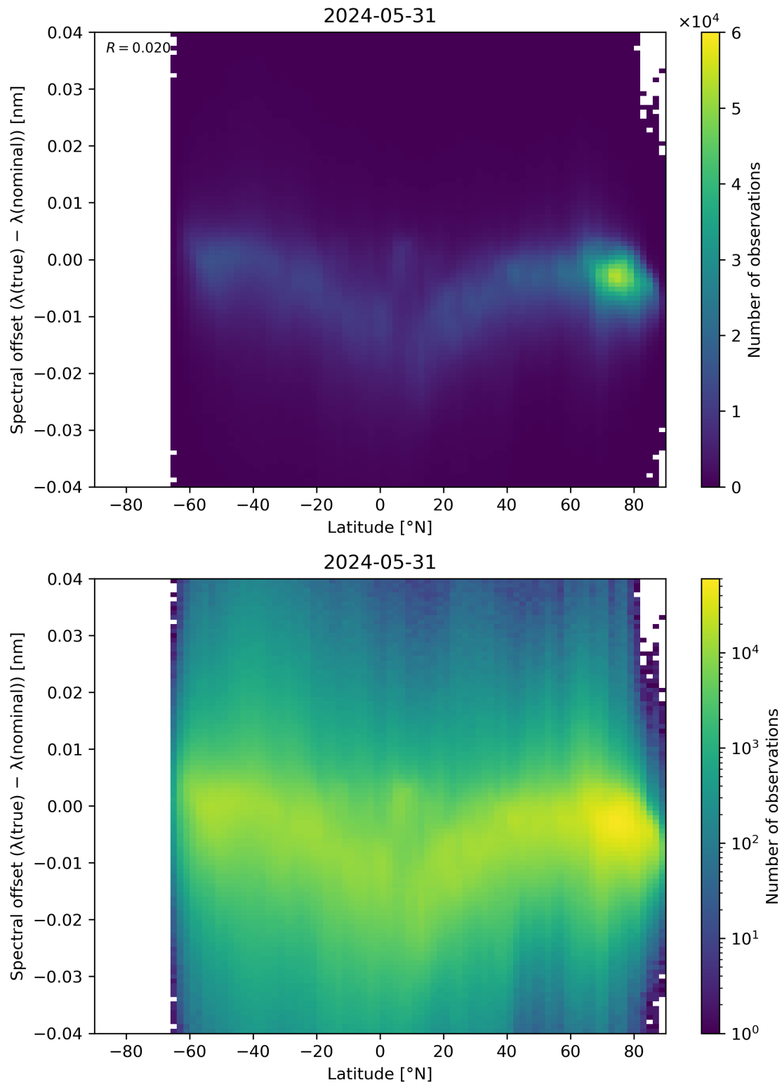
Figure 96: Scatter density plot of “Latitude” against “Spectral offset ( \lambda(\text{true}) - \lambda(\text{nominal}) )” for 2024-05-30 to 2024-06-01.
