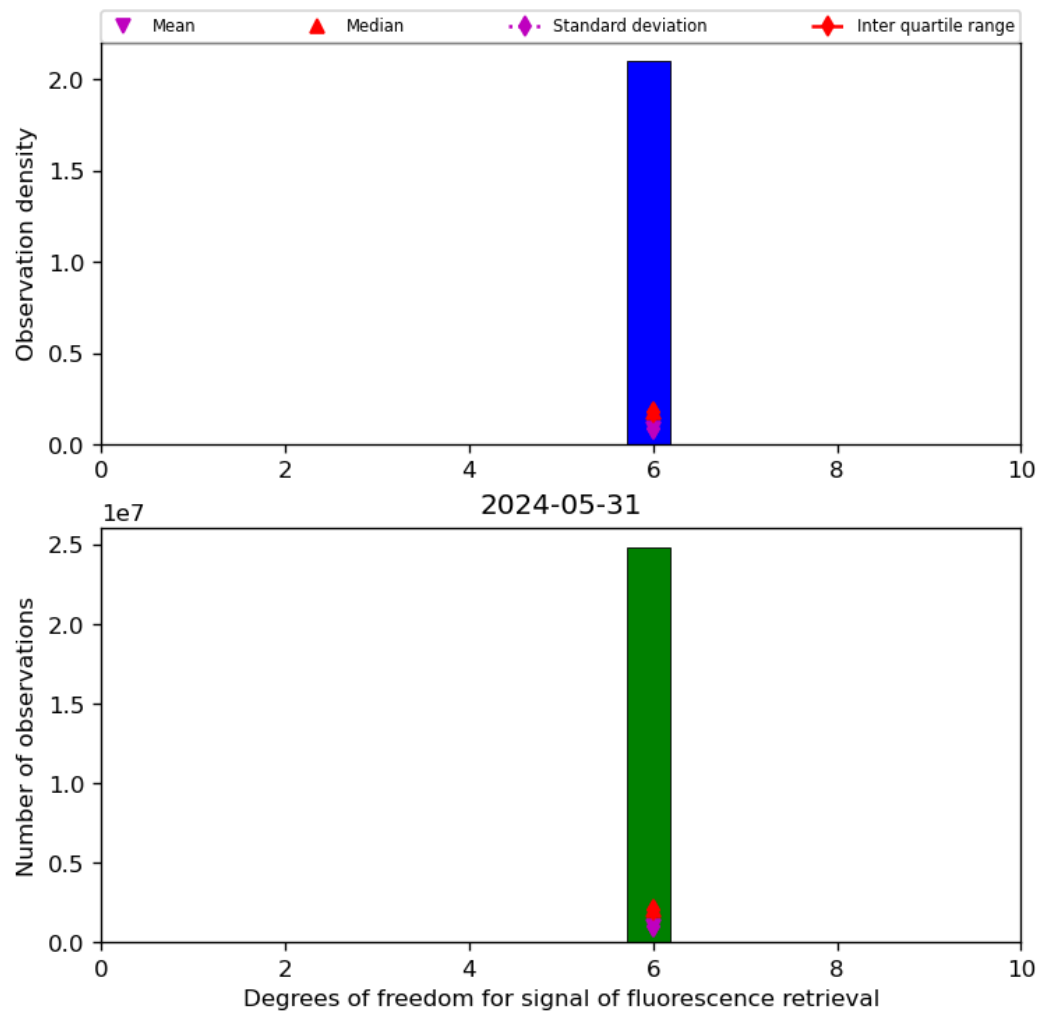
Figure 43: Histogram of “Degrees of freedom for signal of fluorescence retrieval” for 2024-05-30 to 2024-06-01
