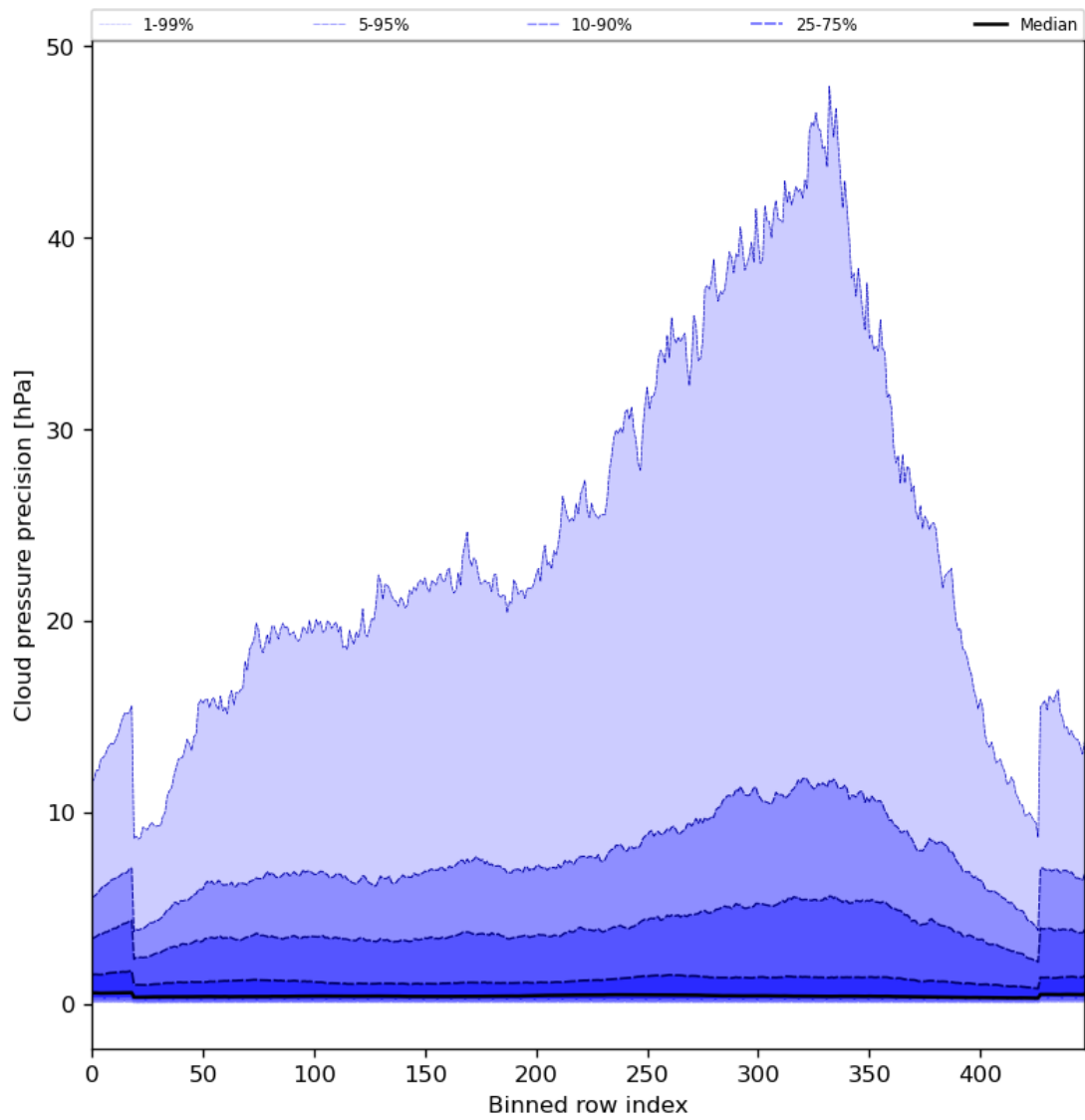
Figure 48: Along track statistics of “Cloud pressure precision” for 2024-05-30 to 2024-06-01
