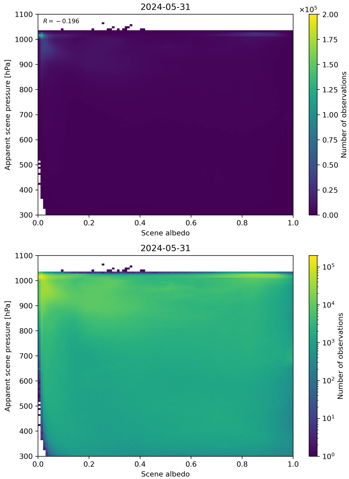
Figure 102: Scatter density plot of “Scene albedo” against “Apparent scene pressure” for 2024-05-30 to 2024-06-01.
