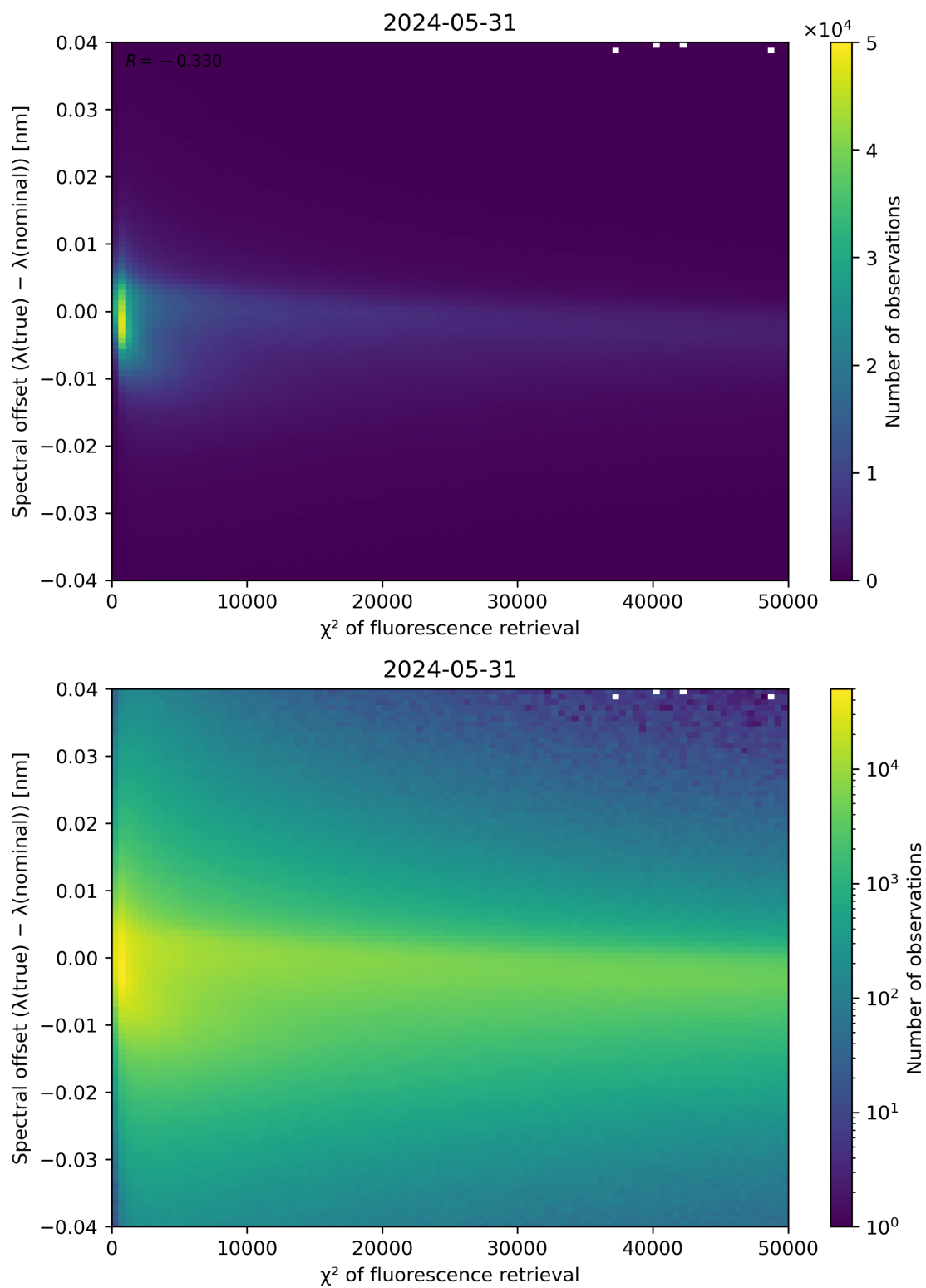
Figure 69: Scatter density plot of " \chi^2 of fluorescence retrieval" against "Spectral offset ( \lambda(\text{true}) - \lambda(\text{nominal}) )" for 2024-05-30 to 2024-06-01.
