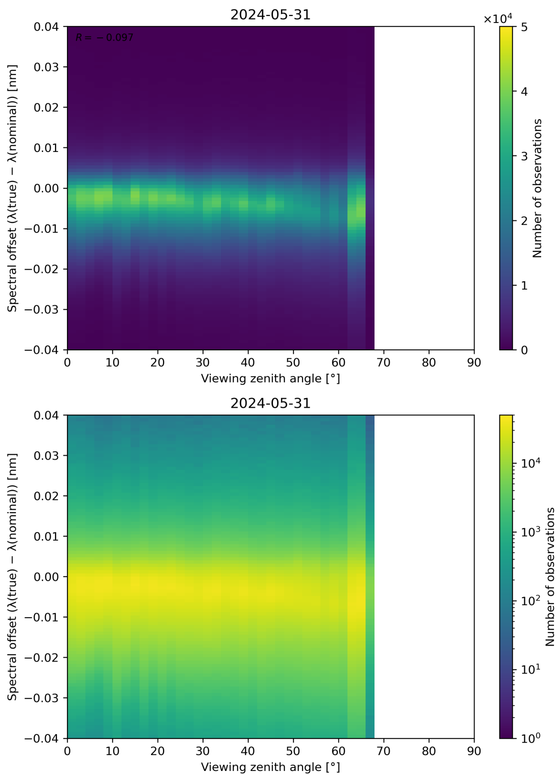
Figure 128: Scatter density plot of “Viewing zenith angle” against “Spectral offset ( \lambda(\text{true}) - \lambda(\text{nominal}) )” for 2024-05-30 to 2024-06-01.
