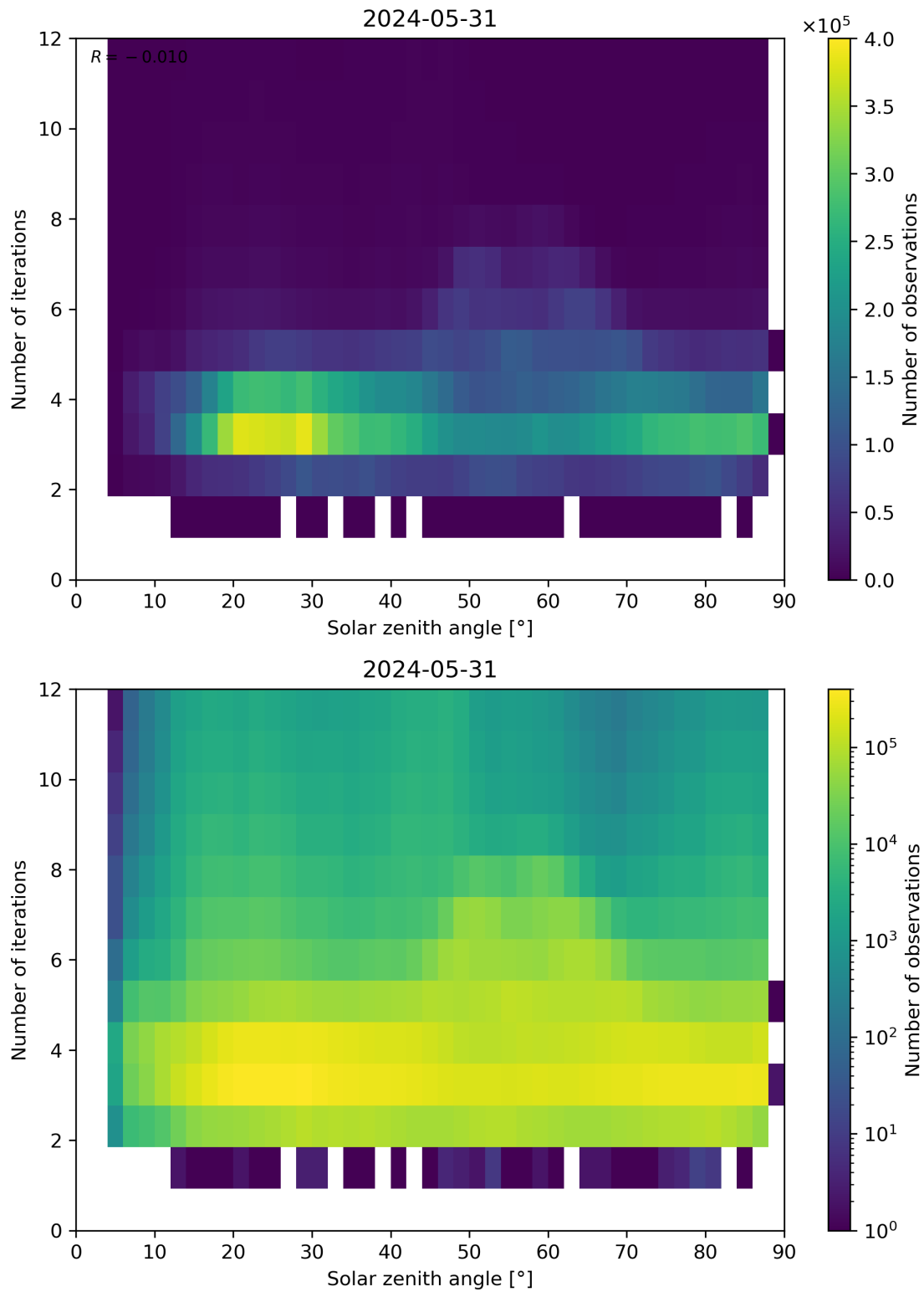
Figure 114: Scatter density plot of “Solar zenith angle” against “Number of iterations” for 2024-05-30 to 2024-06-01.
