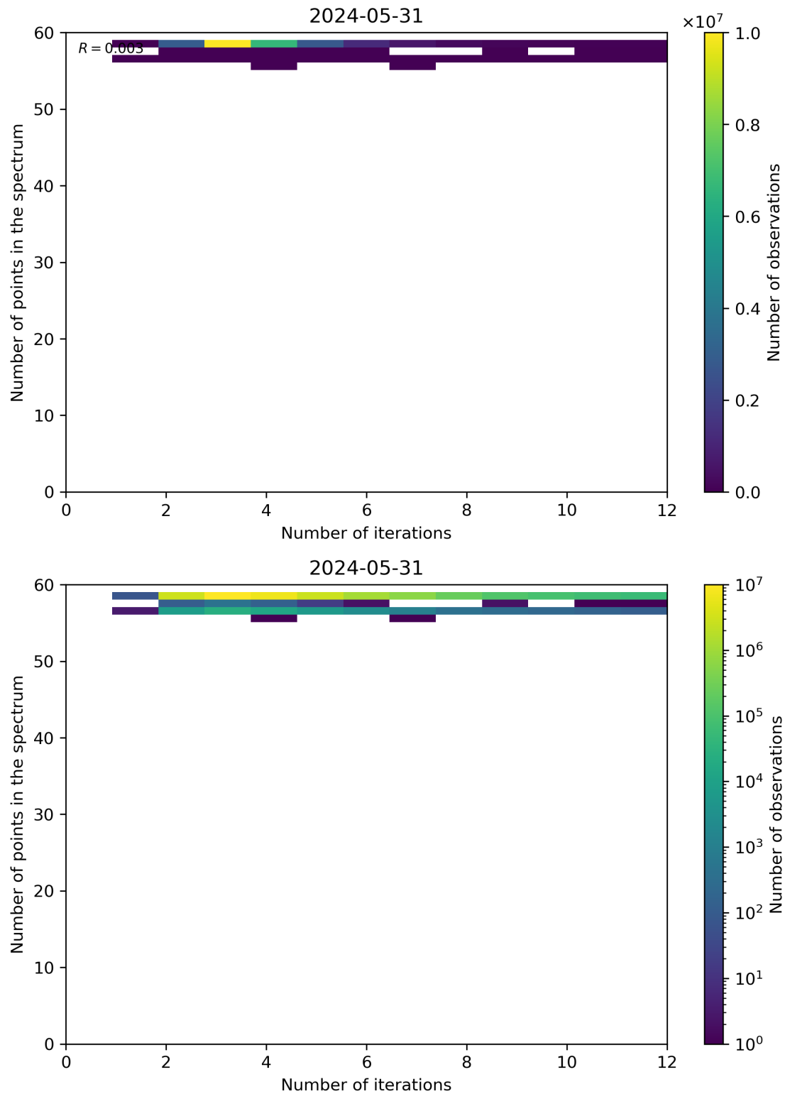
Figure 99: Scatter density plot of “Number of iterations” against “Number of points in the spectrum” for 2024-05-30 to 2024-06-01.
