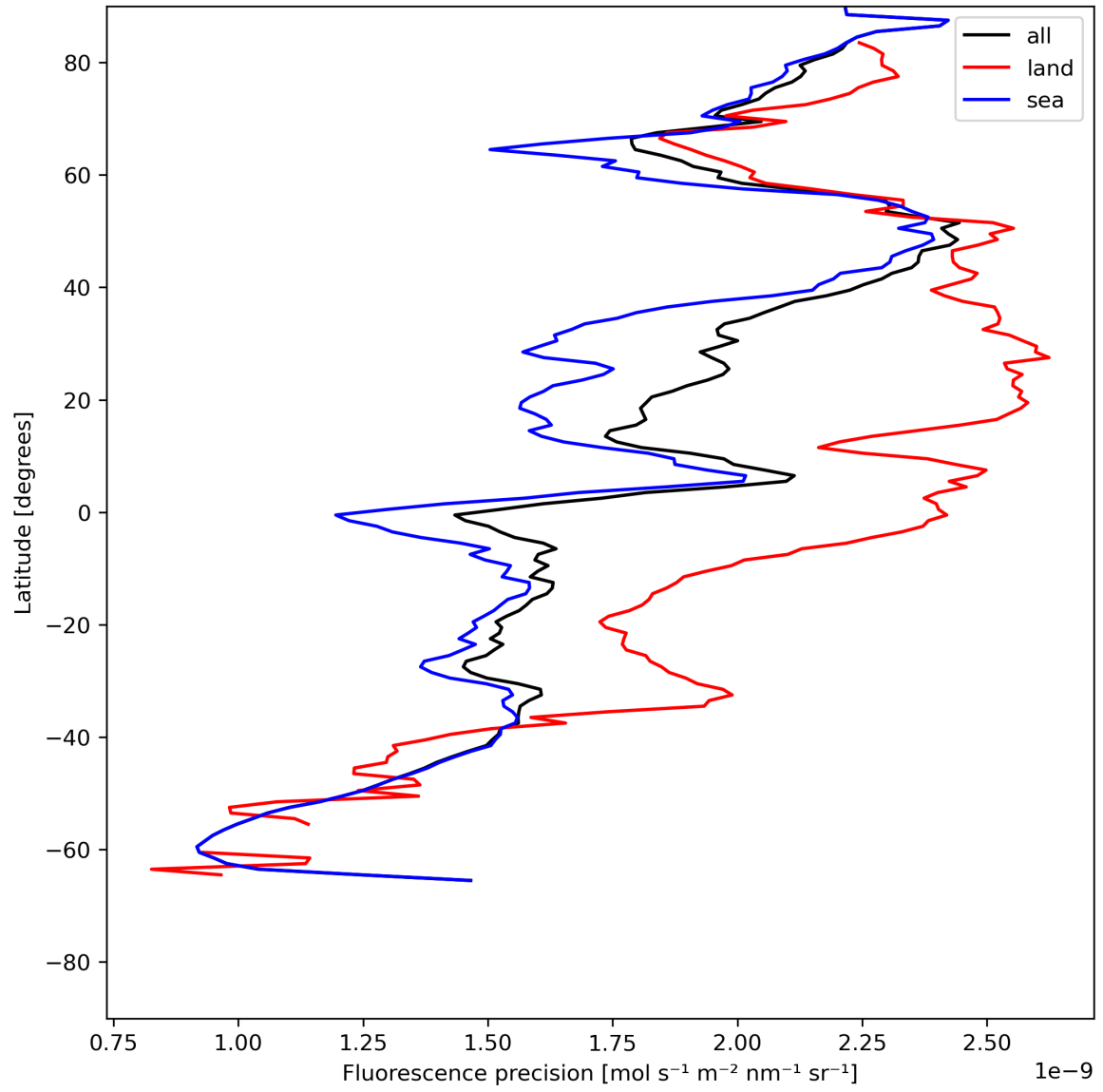
Figure 24: Zonal average of “Fluorescence precision” for 2024-06-01 to 2024-06-03.
