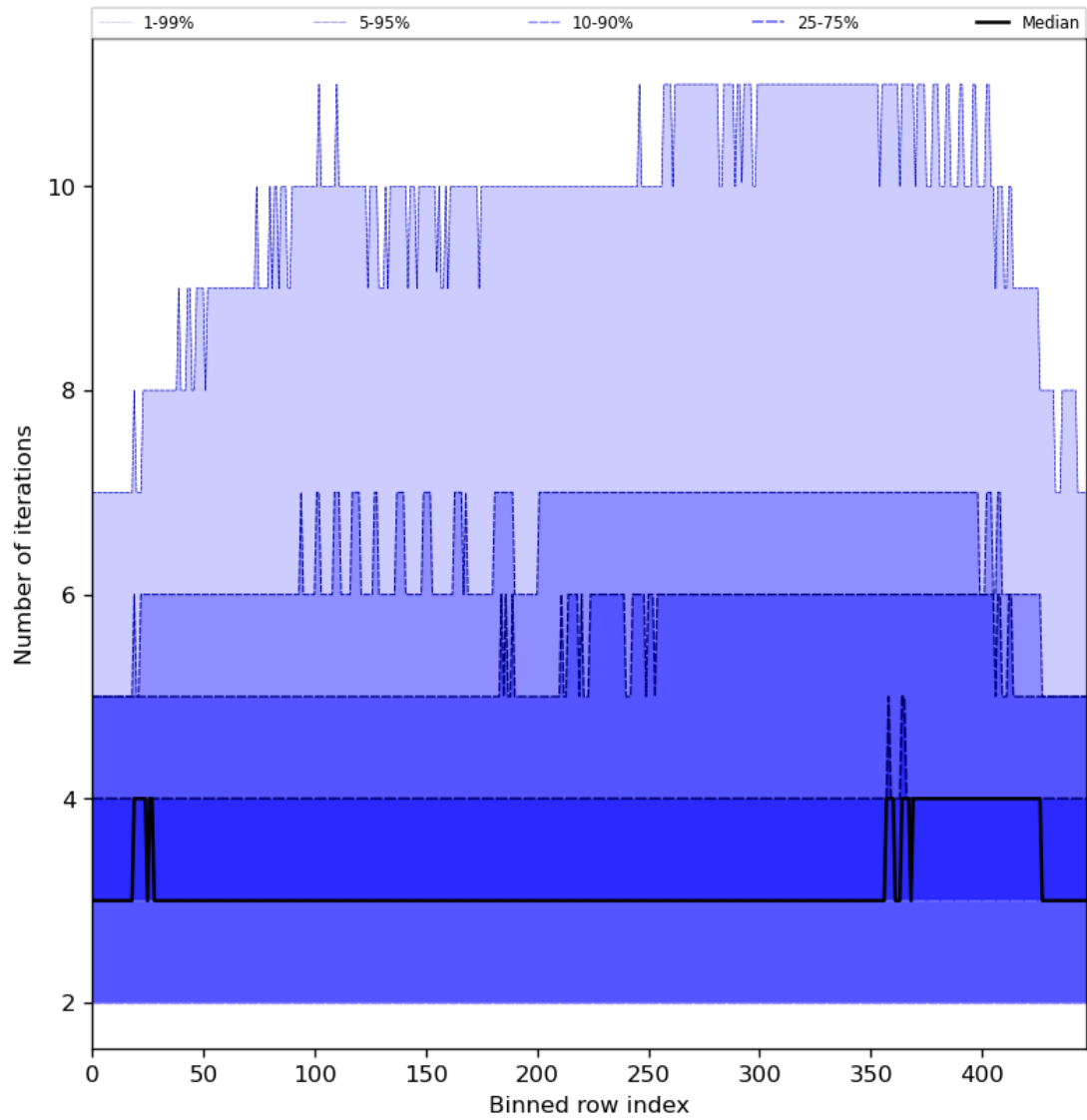
Figure 56: Along track statistics of “Number of iterations” for 2024-06-01 to 2024-06-03
