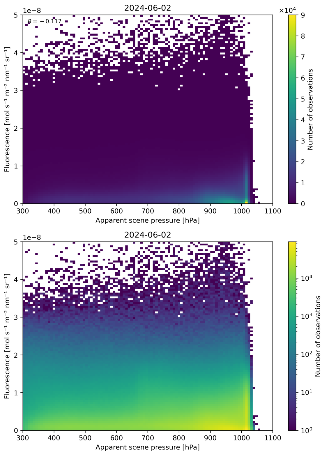
Figure 64: Scatter density plot of “Apparent scene pressure” against “Fluorescence” for 2024-06-01 to 2024-06-03.
