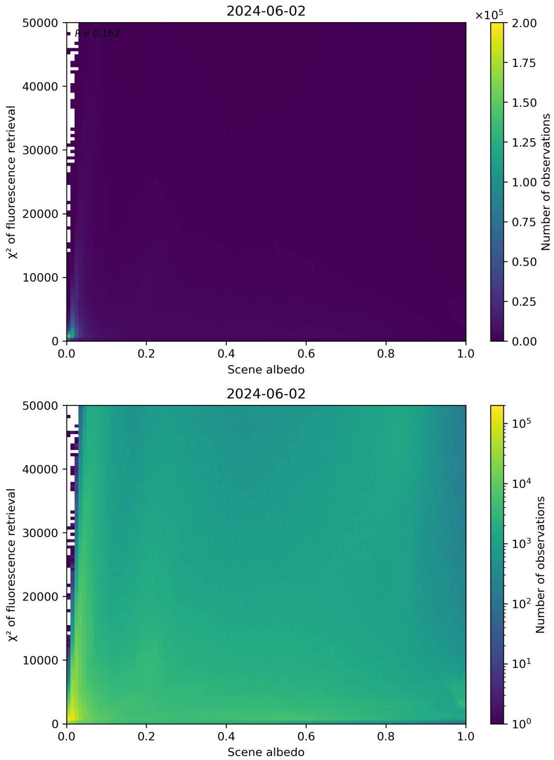
Figure 103: Scatter density plot of “Scene albedo” against “ \chi^2 of fluorescence retrieval” for 2024-06-01 to 2024-06-03.
