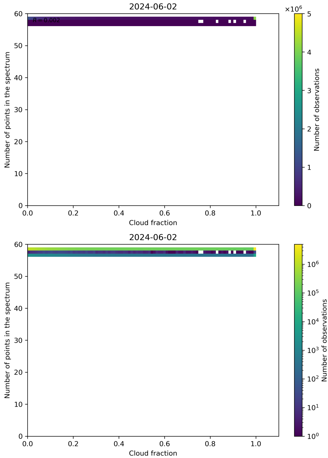
Figure 74: Scatter density plot of “Cloud fraction” against “Number of points in the spectrum” for 2024-06-01 to 2024-06-03.
