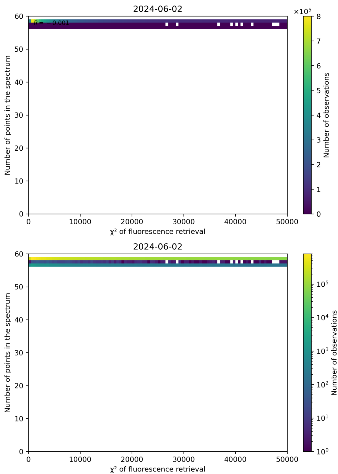
Figure 68: Scatter density plot of " \chi^2 of fluorescence retrieval" against "Number of points in the spectrum" for 2024-06-01 to 2024-06-03.
