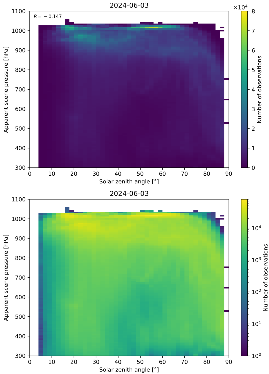
Figure 108: Scatter density plot of “Solar zenith angle” against “Apparent scene pressure” for 2024-06-03 to 2024-06-04.
