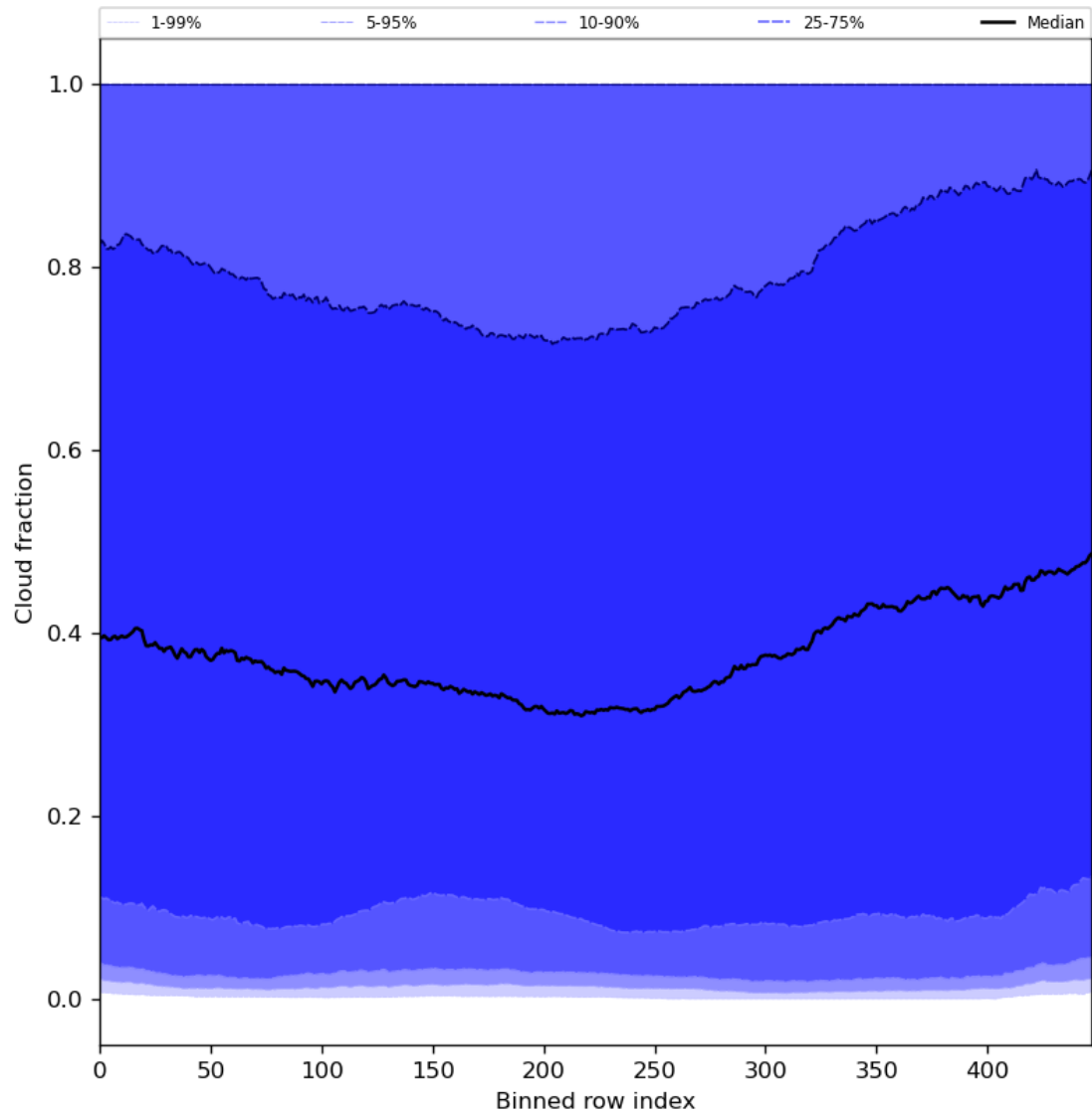
Figure 49: Along track statistics of “Cloud fraction” for 2024-06-03 to 2024-06-04
