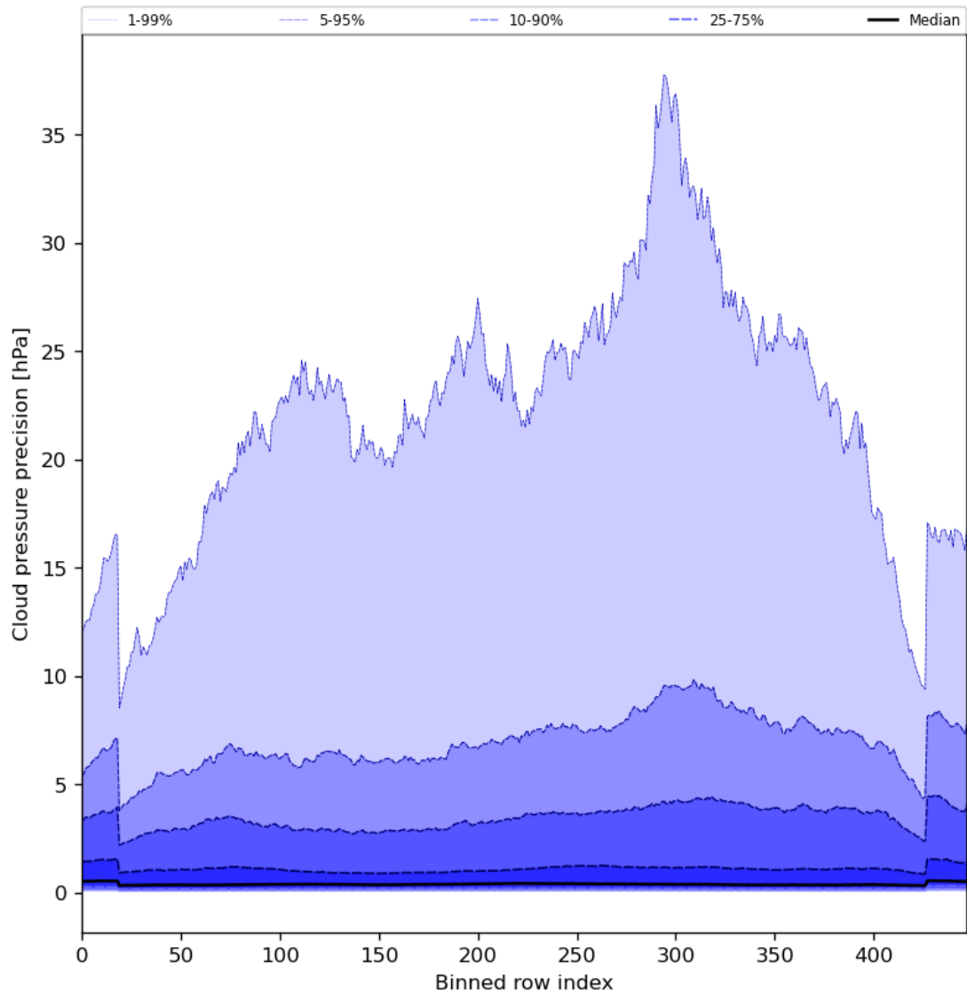
Figure 48: Along track statistics of “Cloud pressure precision” for 2024-06-03 to 2024-06-04
