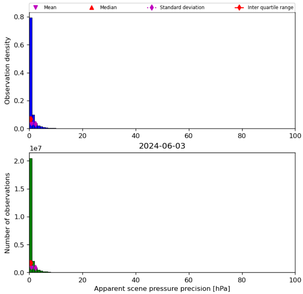
Figure 37: Histogram of “Apparent scene pressure precision” for 2024-06-03 to 2024-06-04
