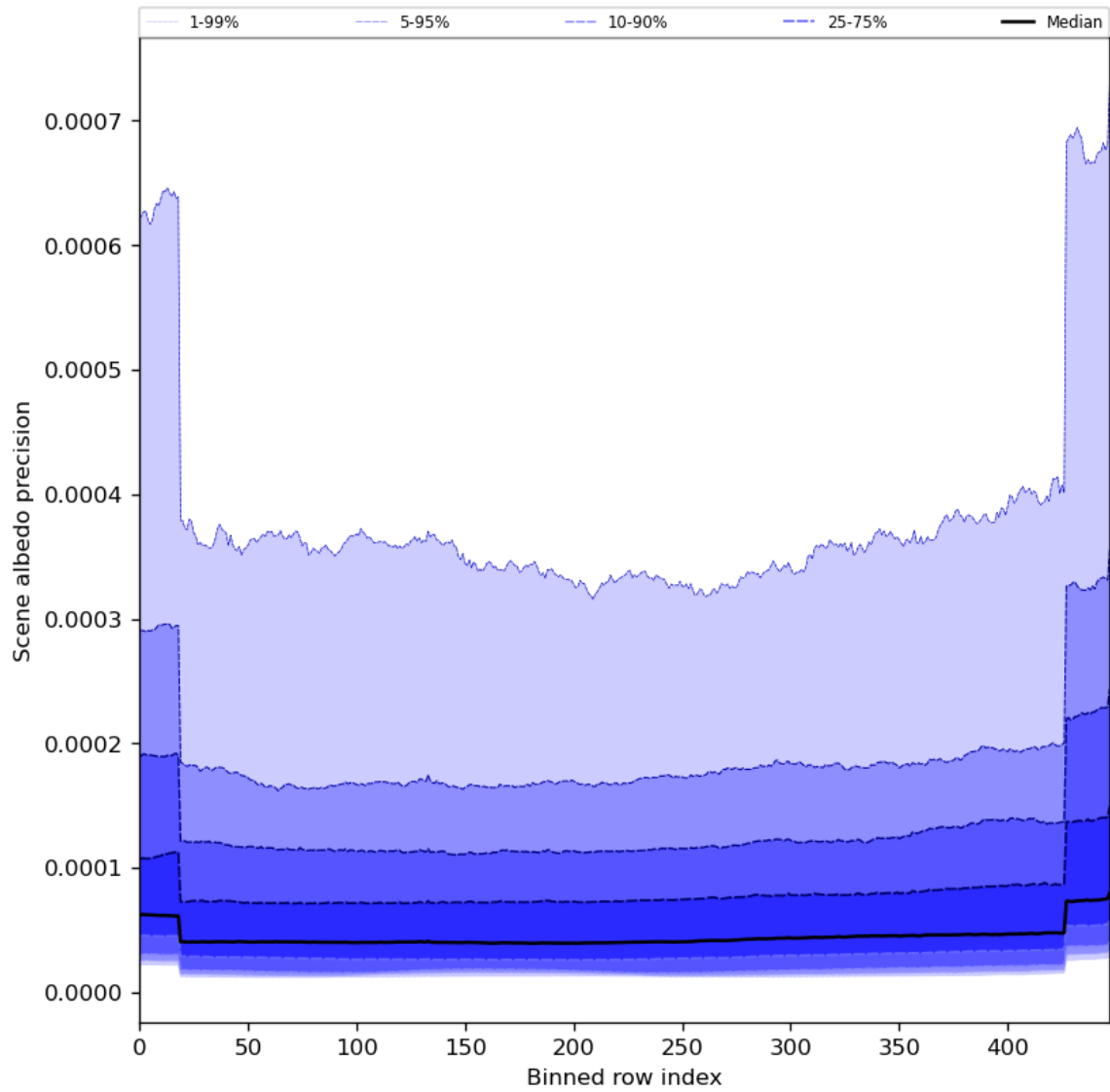
Figure 52: Along track statistics of “Scene albedo precision” for 2024-06-03 to 2024-06-04
