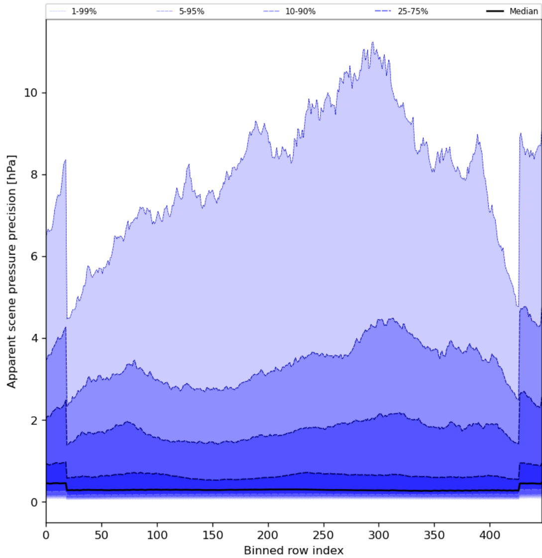
Figure 54: Along track statistics of “Apparent scene pressure precision” for 2024-06-03 to 2024-06-04
