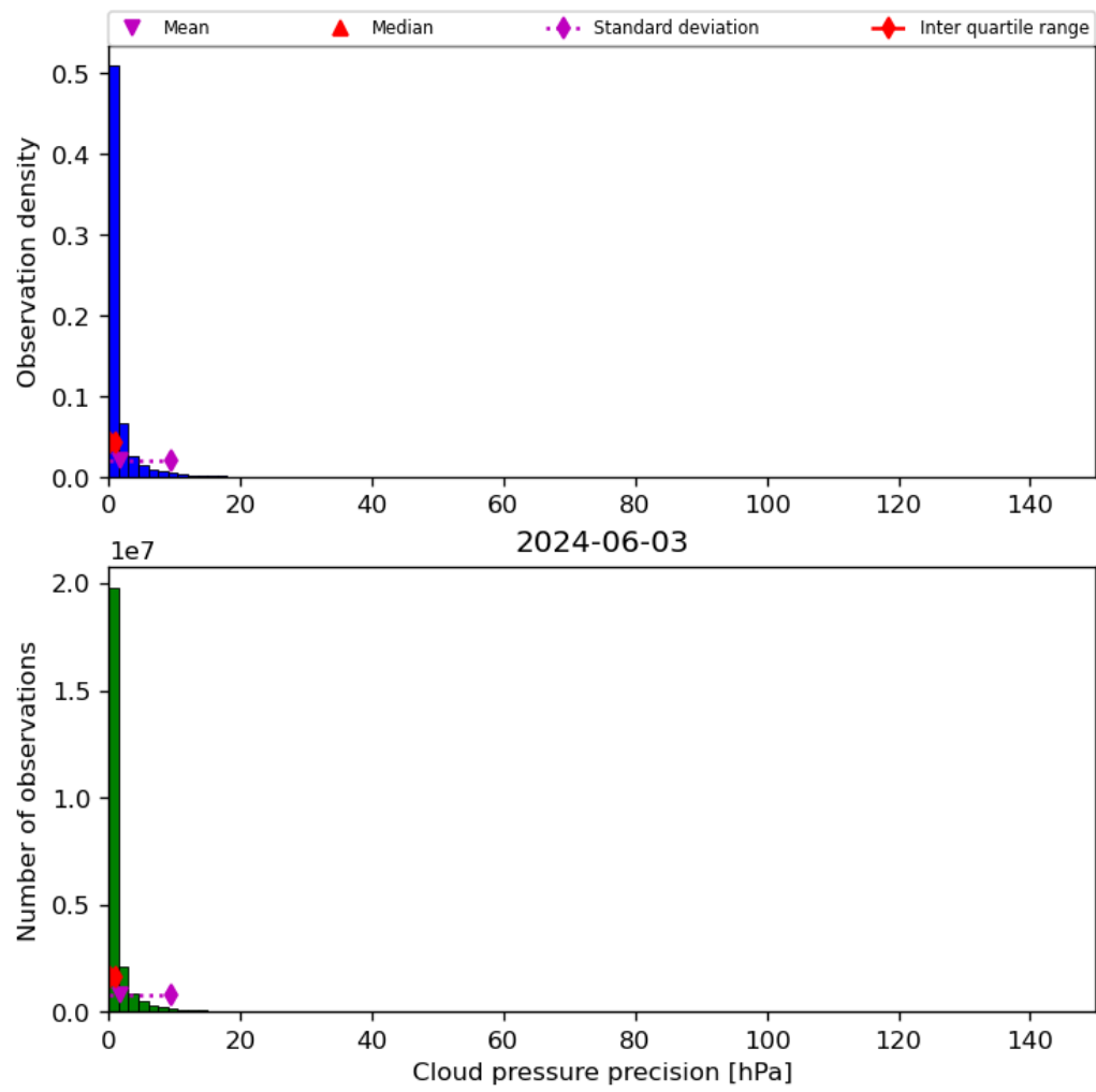
Figure 31: Histogram of “Cloud pressure precision” for 2024-06-03 to 2024-06-04
