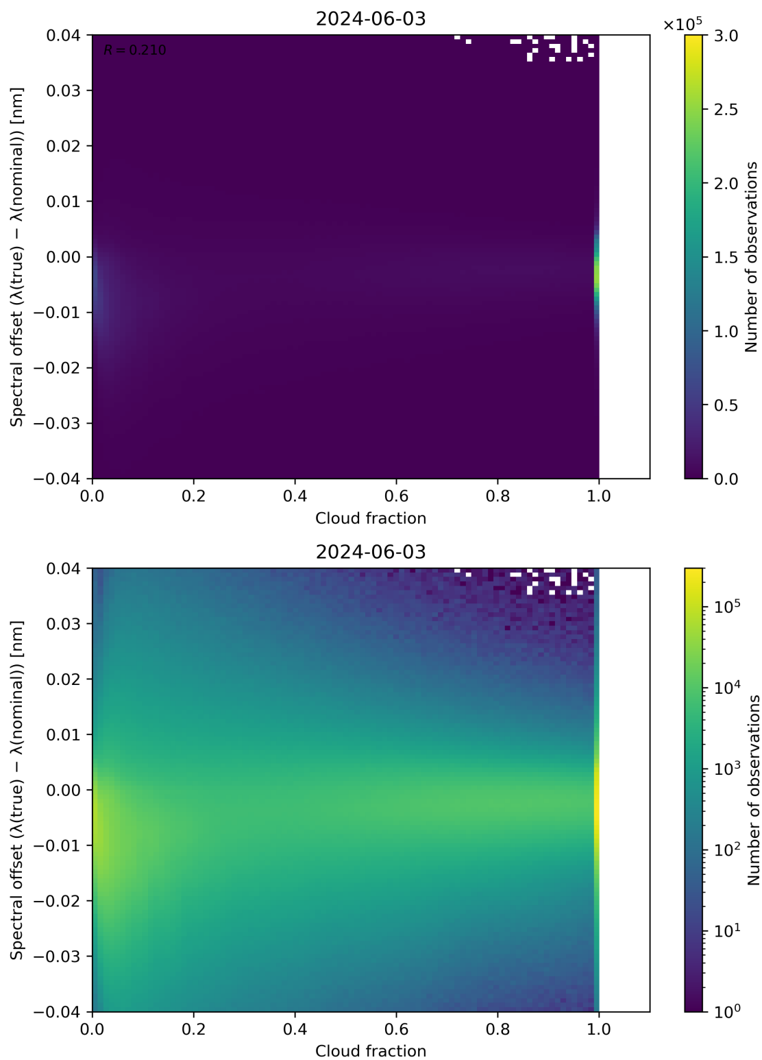
Figure 76: Scatter density plot of “Cloud fraction” against “Spectral offset ( \lambda(\text{true}) - \lambda(\text{nominal}) )” for 2024-06-03 to 2024-06-04.
