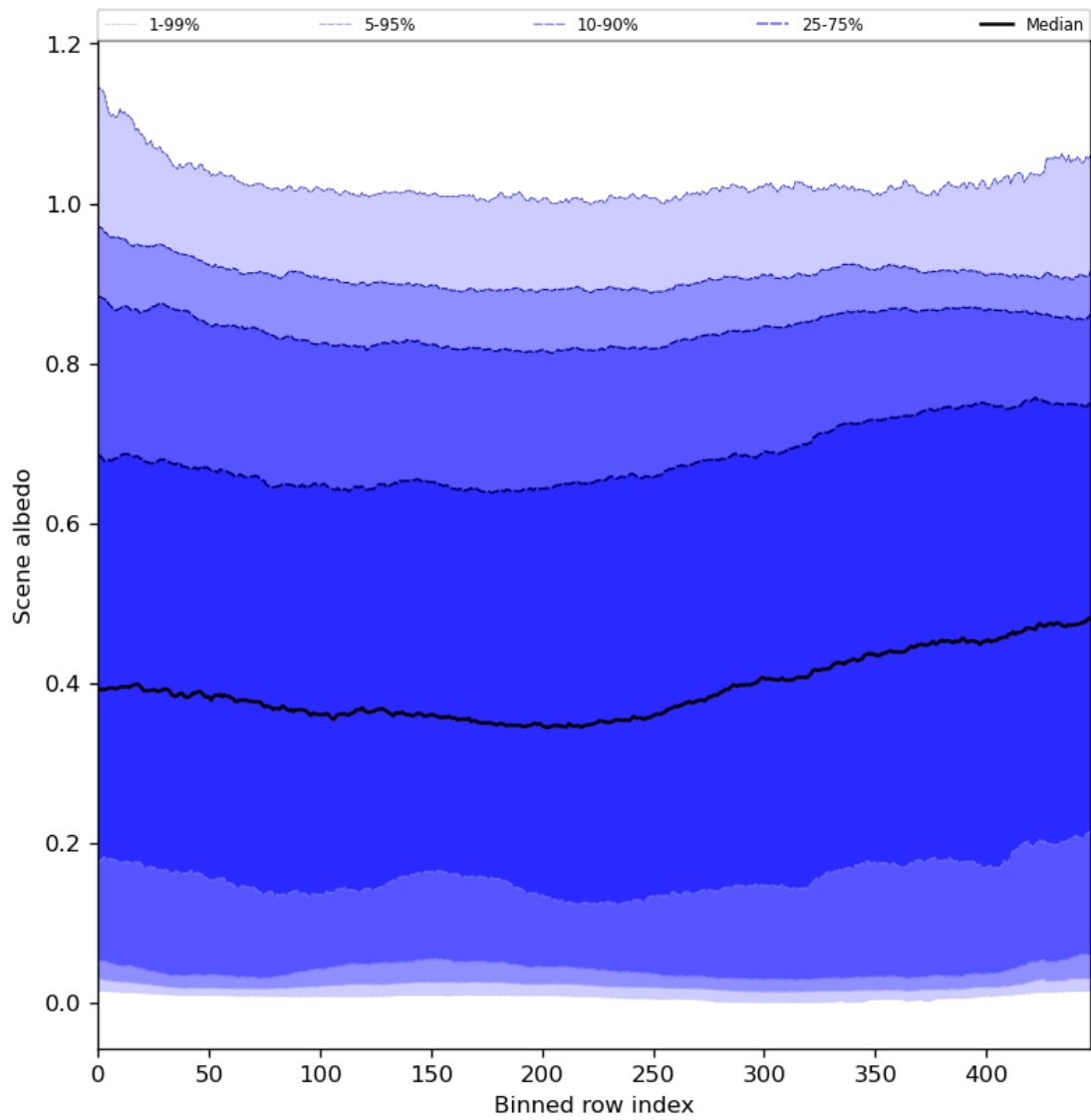
Figure 51: Along track statistics of “Scene albedo” for 2024-06-03 to 2024-06-04
