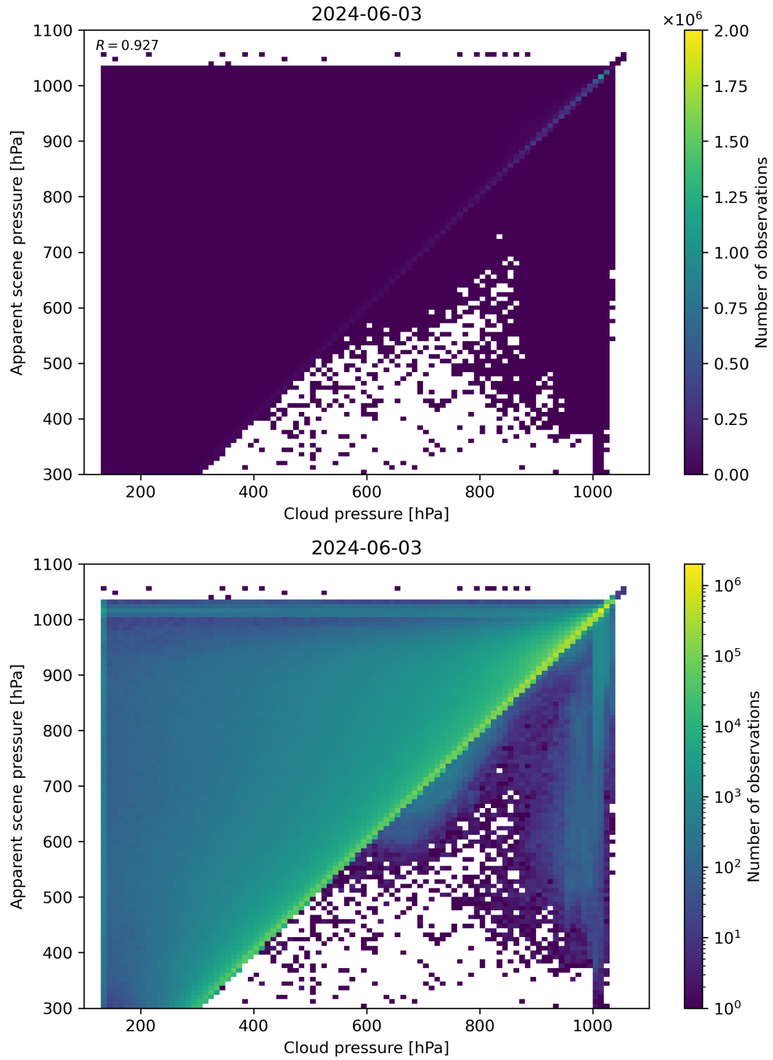
Figure 77: Scatter density plot of “Cloud pressure” against “Apparent scene pressure” for 2024-06-03 to 2024-06-04.
