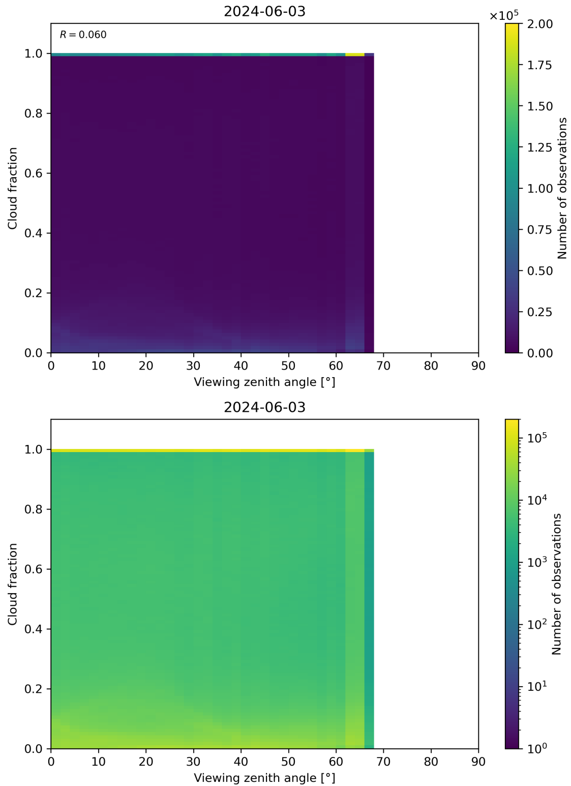
Figure 120: Scatter density plot of “Viewing zenith angle” against “Cloud fraction” for 2024-06-03 to 2024-06-04.
