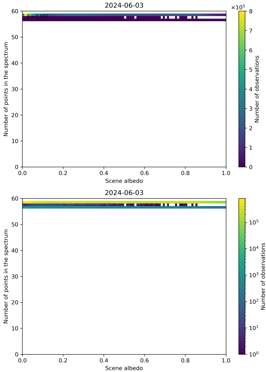
Figure 106: Scatter density plot of “Scene albedo” against “Number of points in the spectrum” for 2024-06-03 to 2024-06-04.
