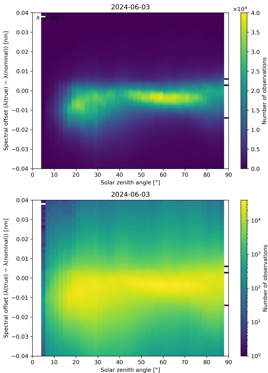
Figure 117: Scatter density plot of “Solar zenith angle” against “Spectral offset ( \lambda(\text{true}) - \lambda(\text{nominal}) )” for 2024-06-03 to 2024-06-04.
