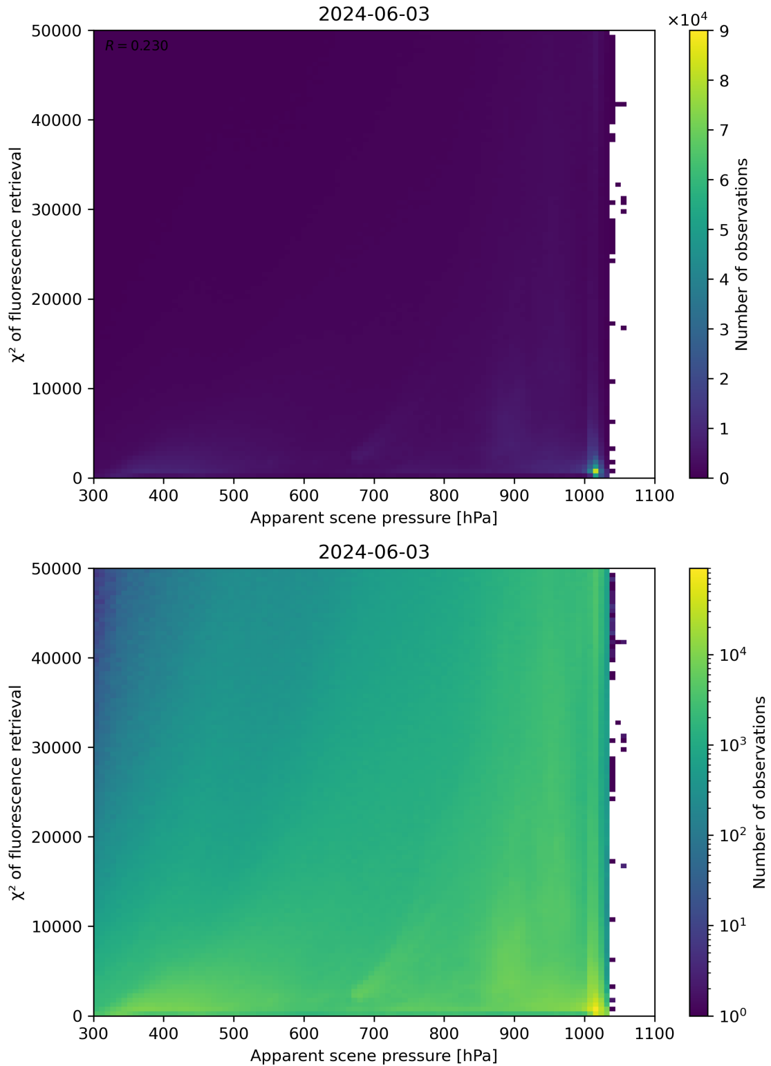
Figure 63: Scatter density plot of “Apparent scene pressure” against “ \chi^2 of fluorescence retrieval” for 2024-06-03 to 2024-06-04.
