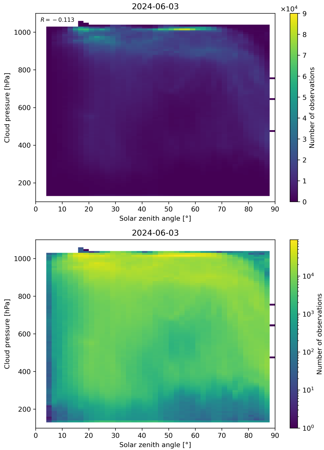
Figure 111: Scatter density plot of “Solar zenith angle” against “Cloud pressure” for 2024-06-03 to 2024-06-04.
