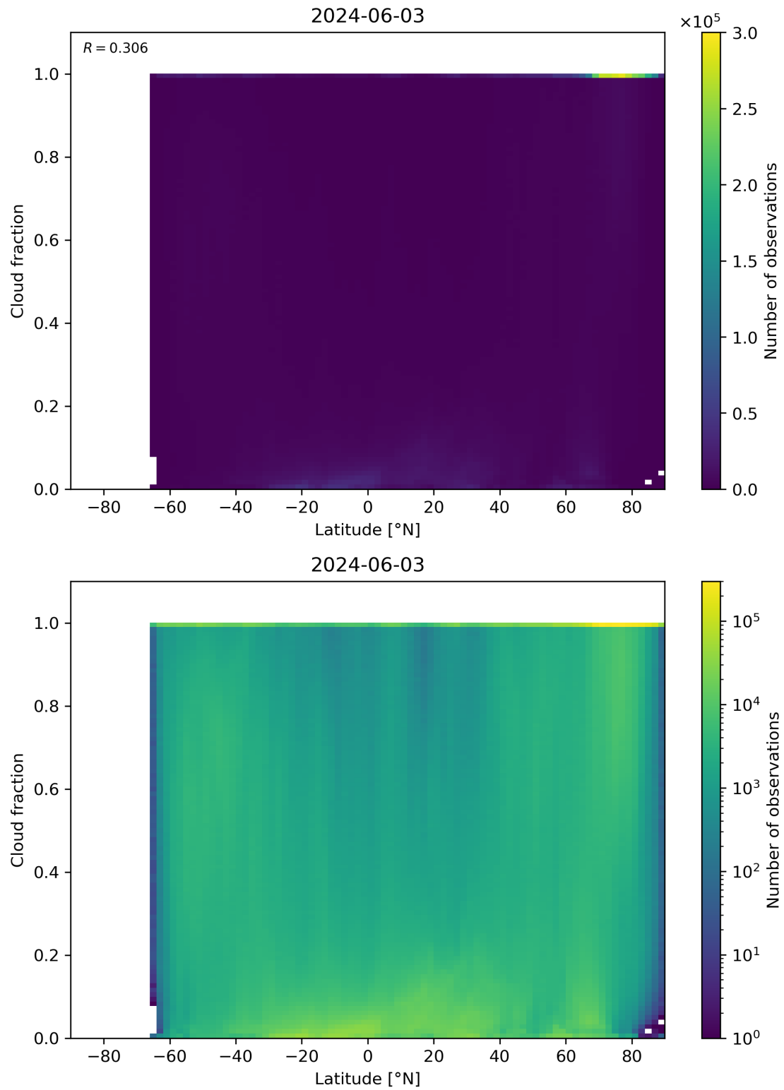
Figure 90: Scatter density plot of “Latitude” against “Cloud fraction” for 2024-06-03 to 2024-06-04.
