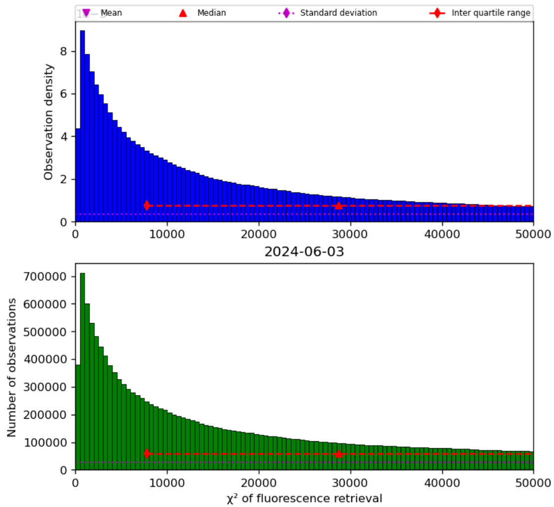
Figure 42: Histogram of “ \chi^2 of fluorescence retrieval” for 2024-06-03 to 2024-06-04
