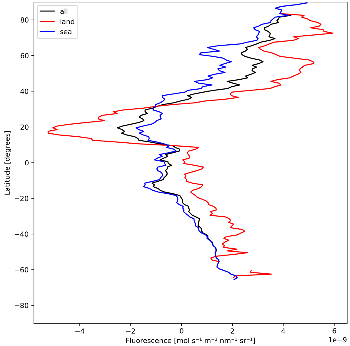
Figure 23: Zonal average of “Fluorescence” for 2024-06-03 to 2024-06-04.
