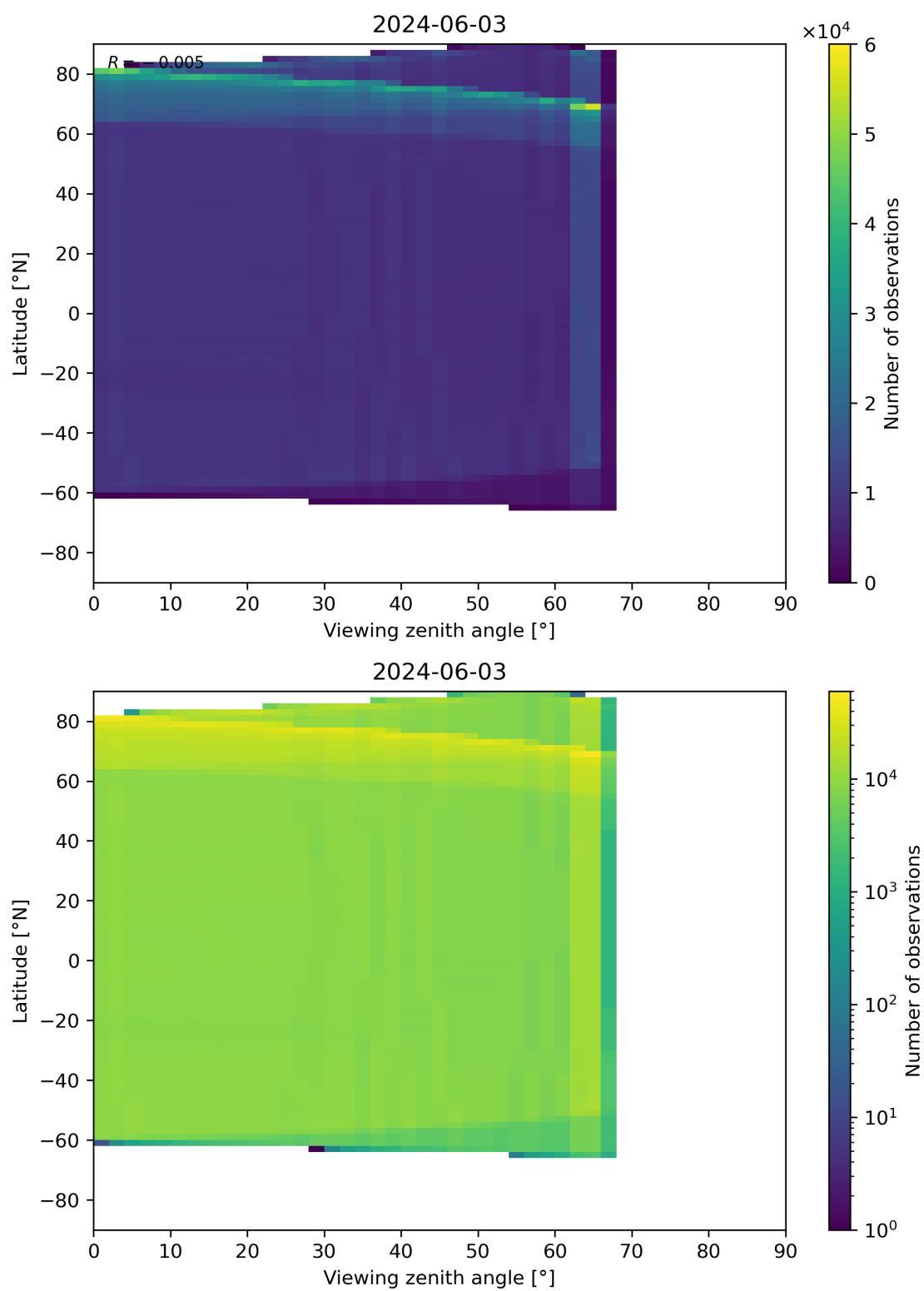
Figure 123: Scatter density plot of “Viewing zenith angle” against “Latitude” for 2024-06-03 to 2024-06-04.
