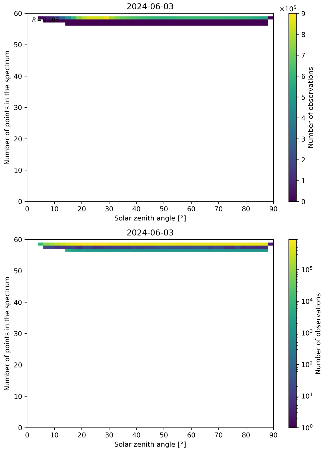
Figure 115: Scatter density plot of “Solar zenith angle” against “Number of points in the spectrum” for 2024-06-03 to 2024-06-04.
