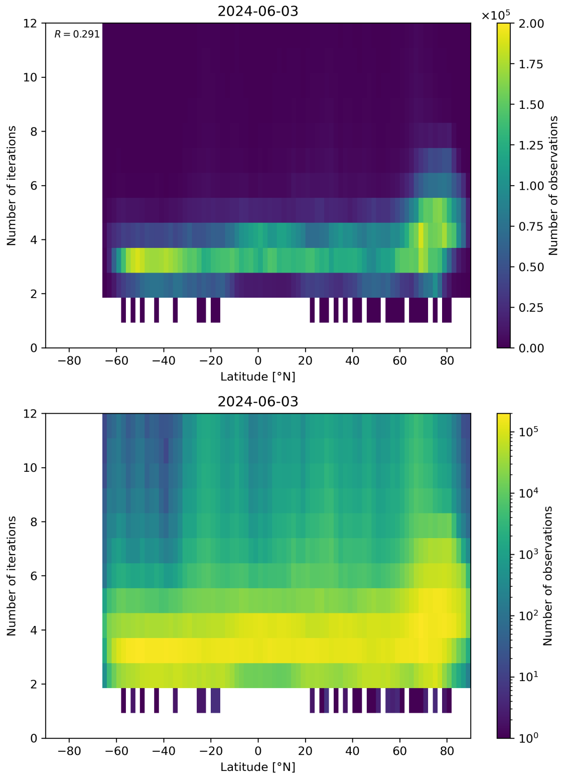
Figure 93: Scatter density plot of “Latitude” against “Number of iterations” for 2024-06-03 to 2024-06-04.
