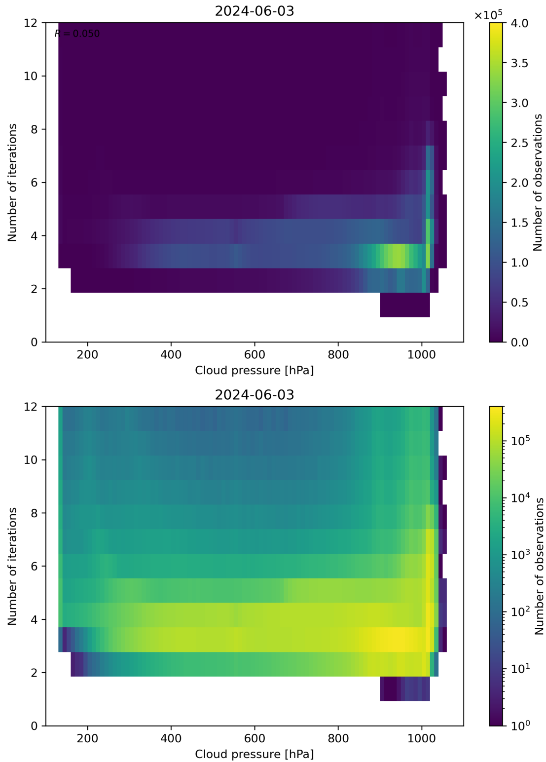
Figure 81: Scatter density plot of “Cloud pressure” against “Number of iterations” for 2024-06-03 to 2024-06-04.
