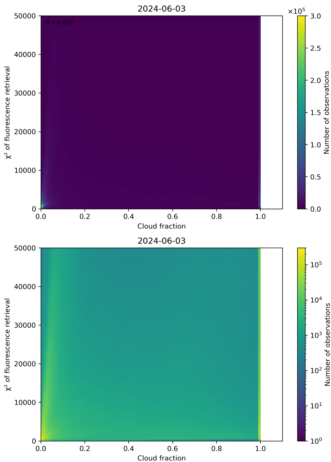
Figure 71: Scatter density plot of “Cloud fraction” against “ \chi^2 of fluorescence retrieval” for 2024-06-03 to 2024-06-04.
