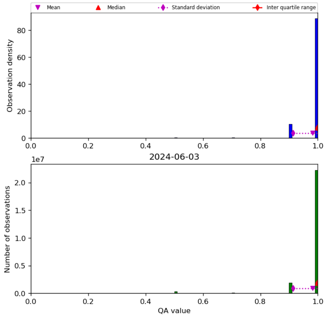
Figure 29: Histogram of “QA value” for 2024-06-03 to 2024-06-04
