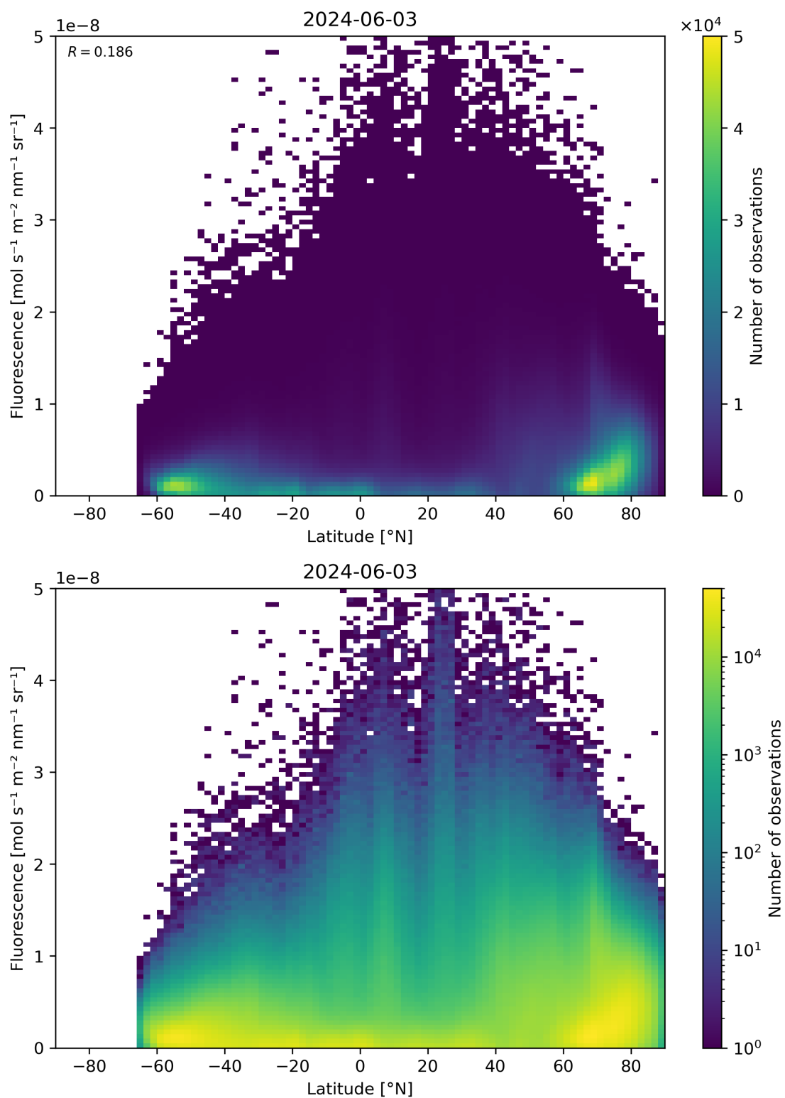
Figure 92: Scatter density plot of “Latitude” against “Fluorescence” for 2024-06-03 to 2024-06-04.
