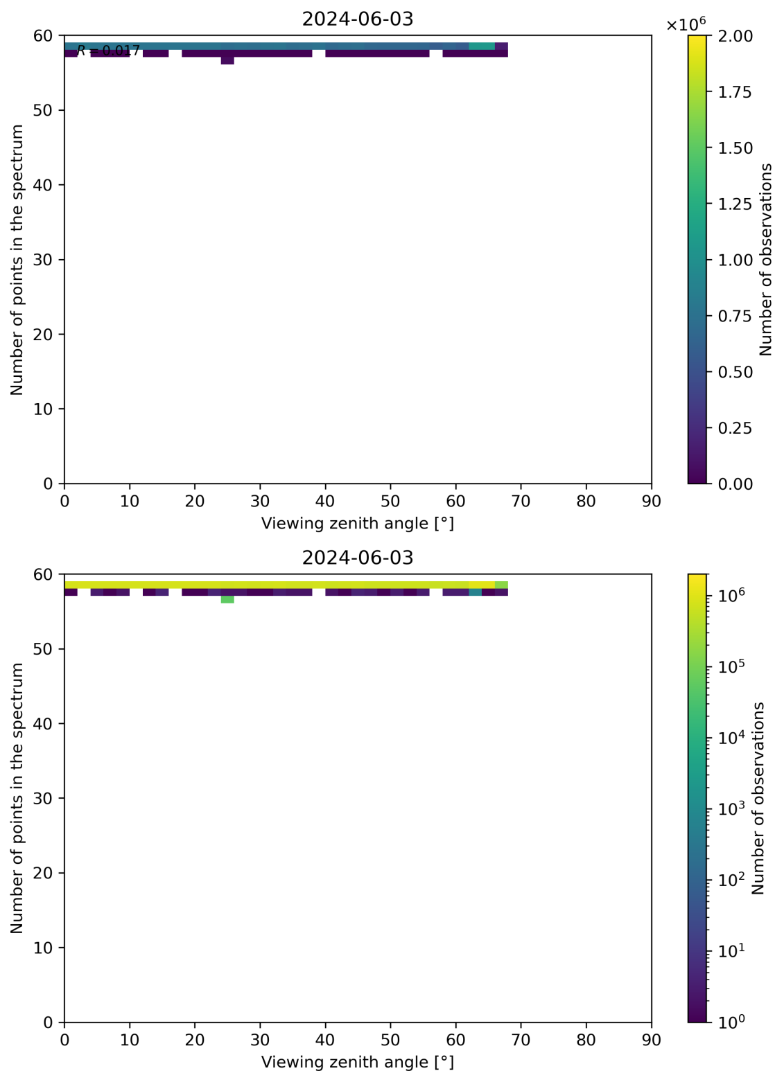
Figure 125: Scatter density plot of “Viewing zenith angle” against “Number of points in the spectrum” for 2024-06-03 to 2024-06-04.
