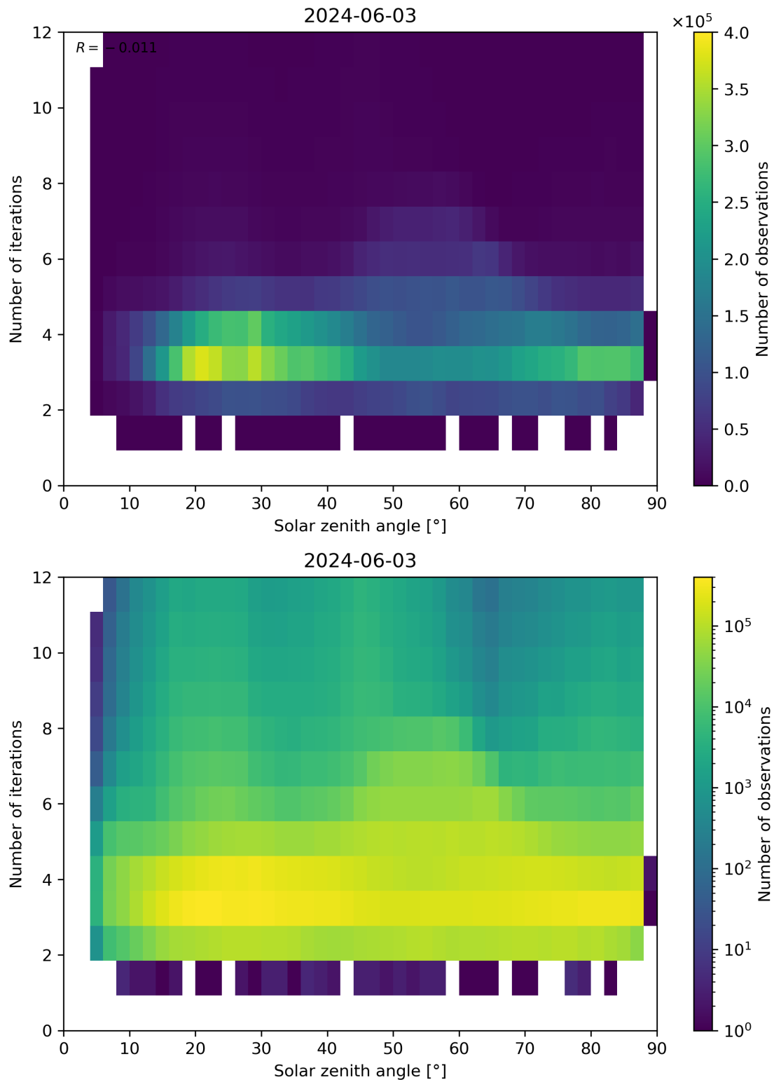
Figure 114: Scatter density plot of “Solar zenith angle” against “Number of iterations” for 2024-06-03 to 2024-06-04.
