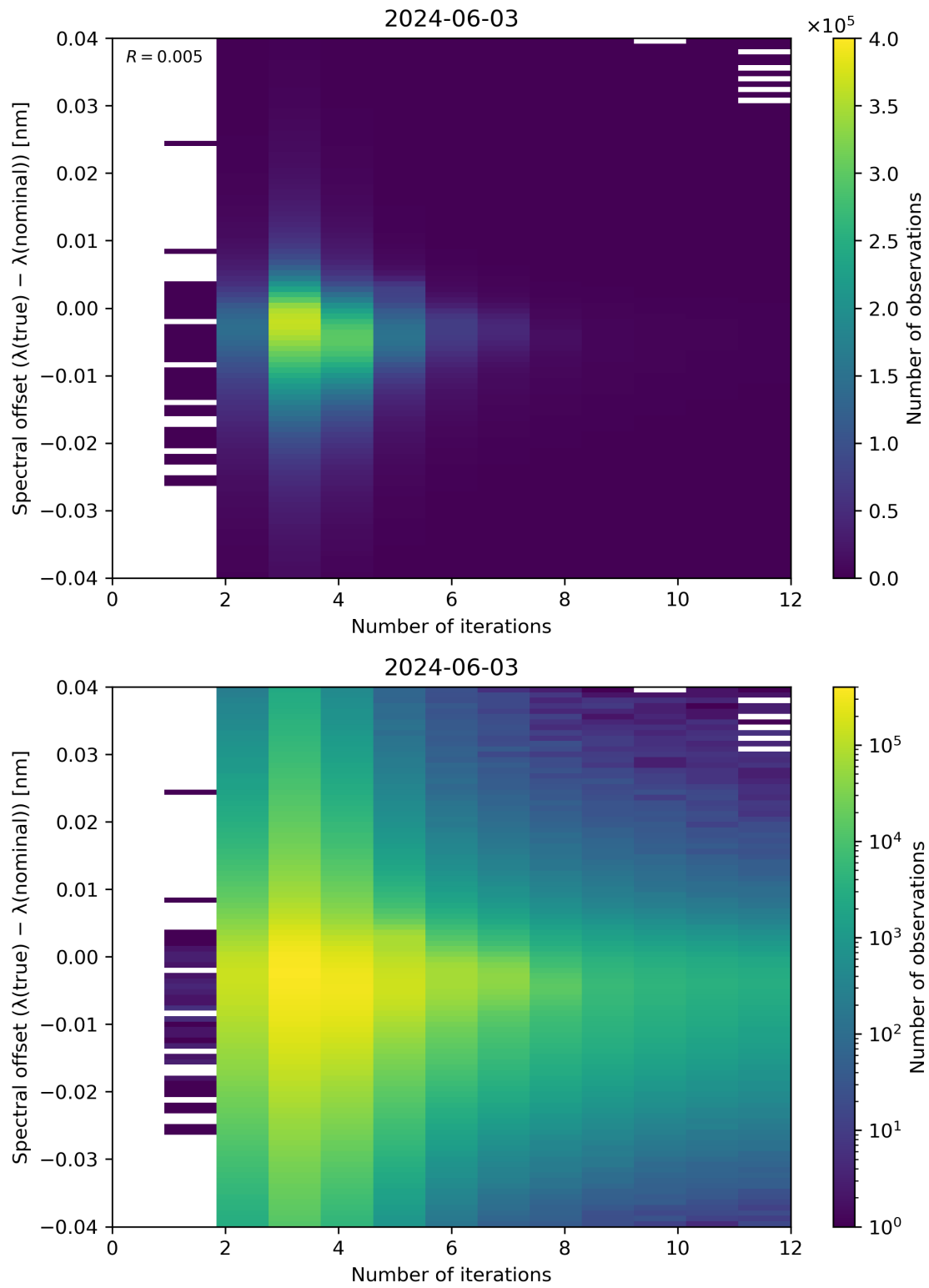
Figure 100: Scatter density plot of “Number of iterations” against “Spectral offset ( \lambda(\text{true}) - \lambda(\text{nominal}) )” for 2024-06-03 to 2024-06-04.
