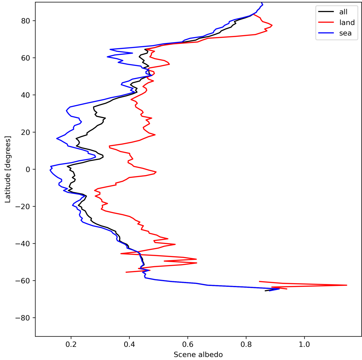
Figure 17: Zonal average of “Scene albedo” for 2024-06-03 to 2024-06-04.
