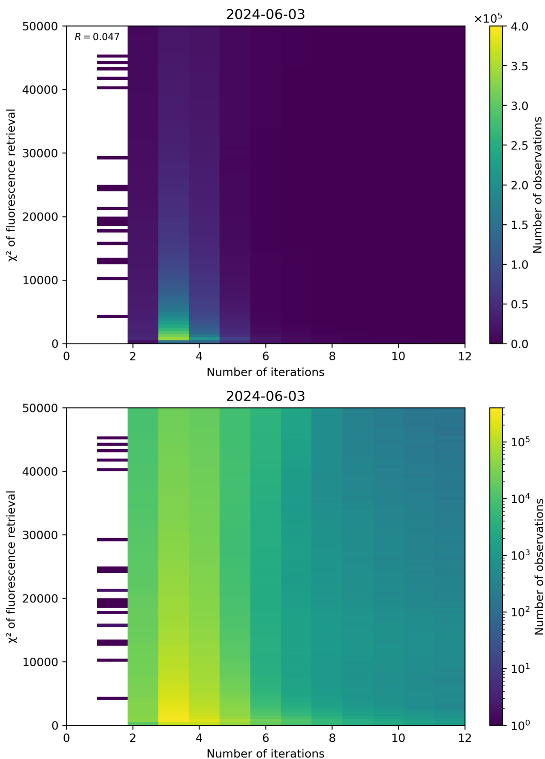
Figure 97: Scatter density plot of “Number of iterations” against “ \chi^2 of fluorescence retrieval” for 2024-06-03 to 2024-06-04.
