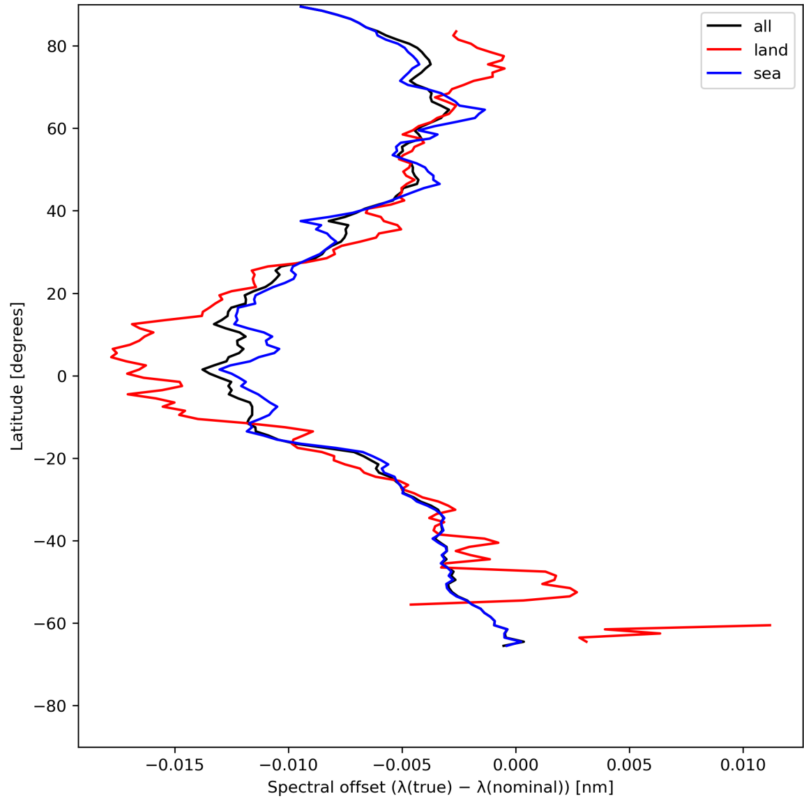
Figure 28: Zonal average of “Spectral offset ( \lambda(\text{true}) - \lambda(\text{nominal}) )” for 2024-06-03 to 2024-06-04.
