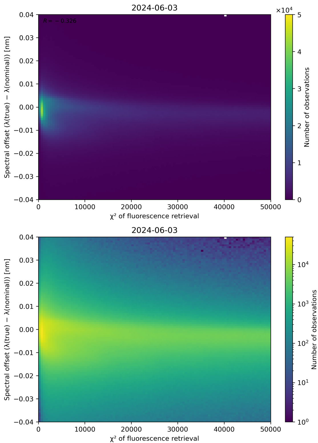
Figure 69: Scatter density plot of " \chi^2 of fluorescence retrieval" against "Spectral offset ( \lambda(\text{true}) - \lambda(\text{nominal}) )" for 2024-06-03 to 2024-06-04.
