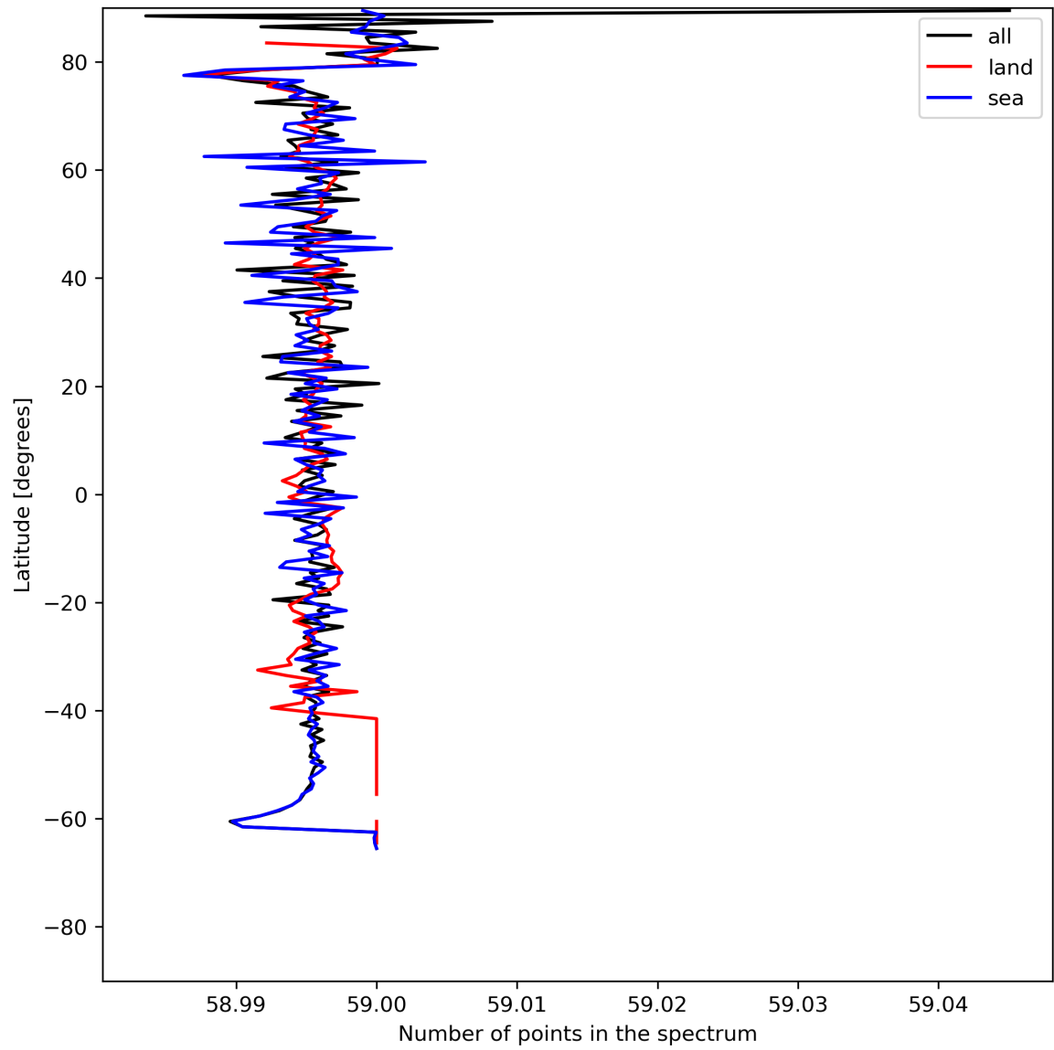
Figure 27: Zonal average of “Number of points in the spectrum” for 2024-06-03 to 2024-06-04.
