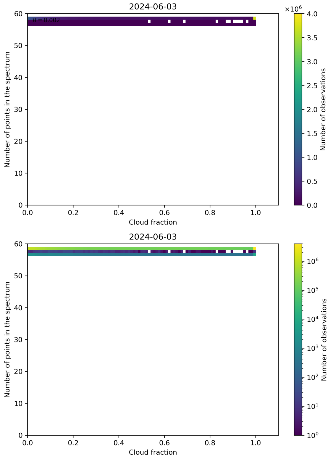
Figure 74: Scatter density plot of “Cloud fraction” against “Number of points in the spectrum” for 2024-06-03 to 2024-06-04.
