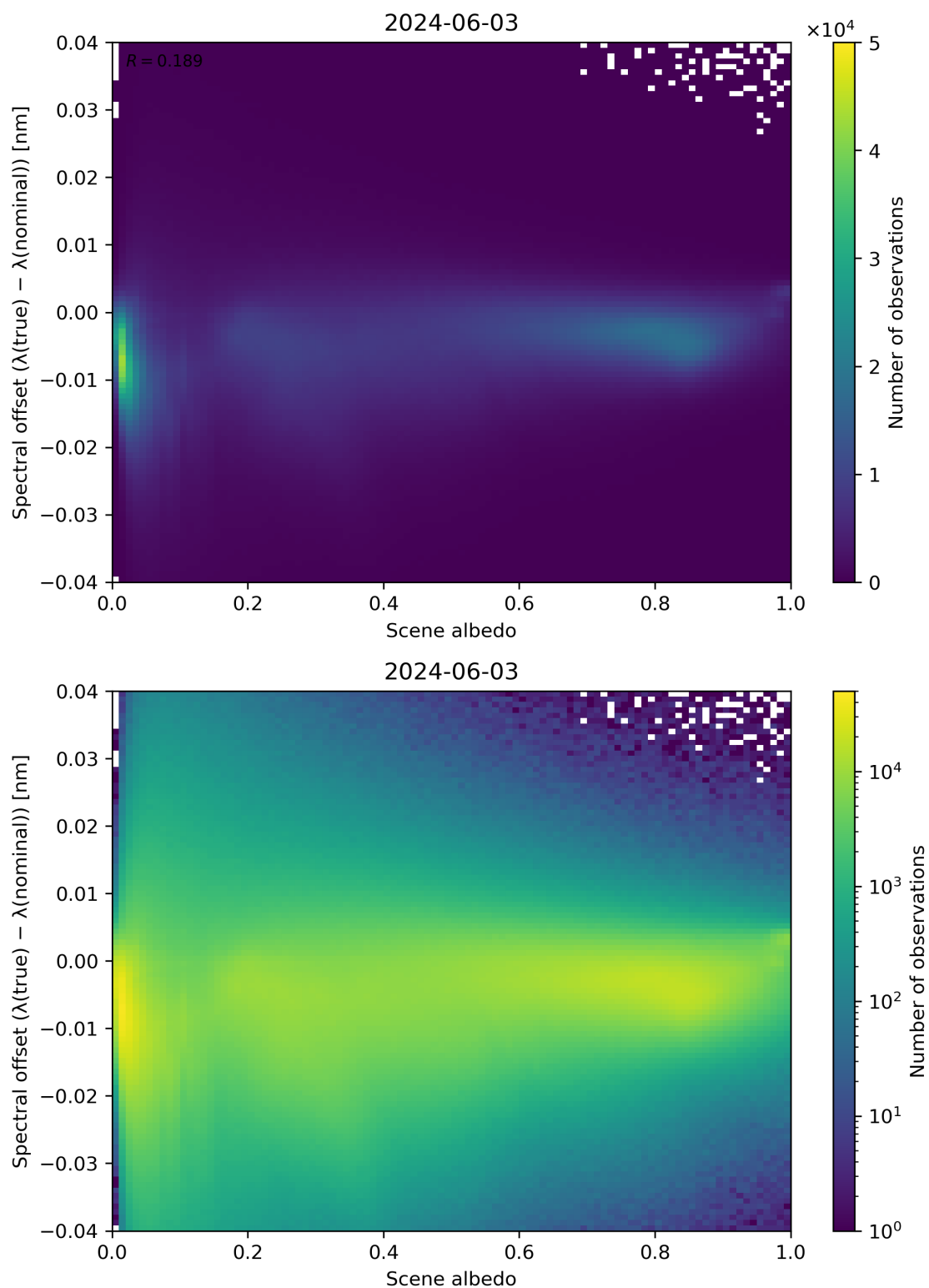
Figure 107: Scatter density plot of “Scene albedo” against “Spectral offset ( \lambda(\text{true}) - \lambda(\text{nominal}) )” for 2024-06-03 to 2024-06-04.
