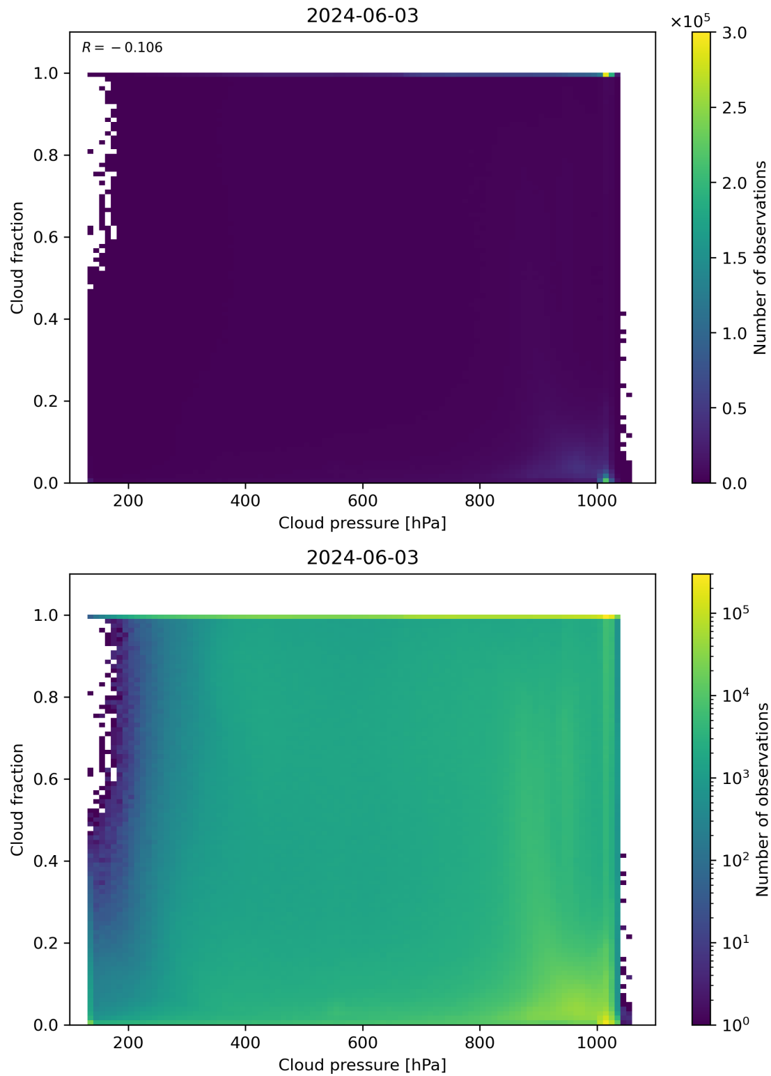
Figure 79: Scatter density plot of “Cloud pressure” against “Cloud fraction” for 2024-06-03 to 2024-06-04.
