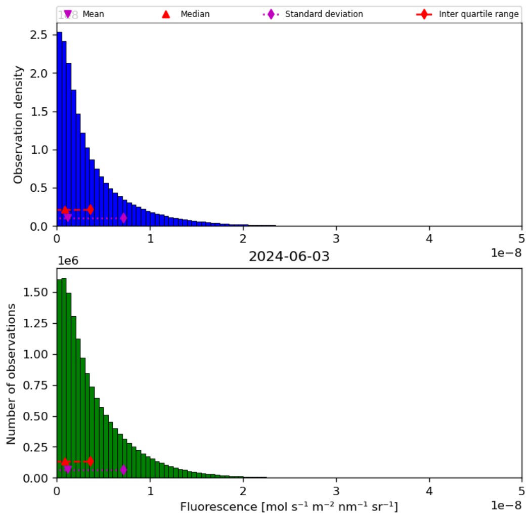
Figure 40: Histogram of “Fluorescence” for 2024-06-03 to 2024-06-04
