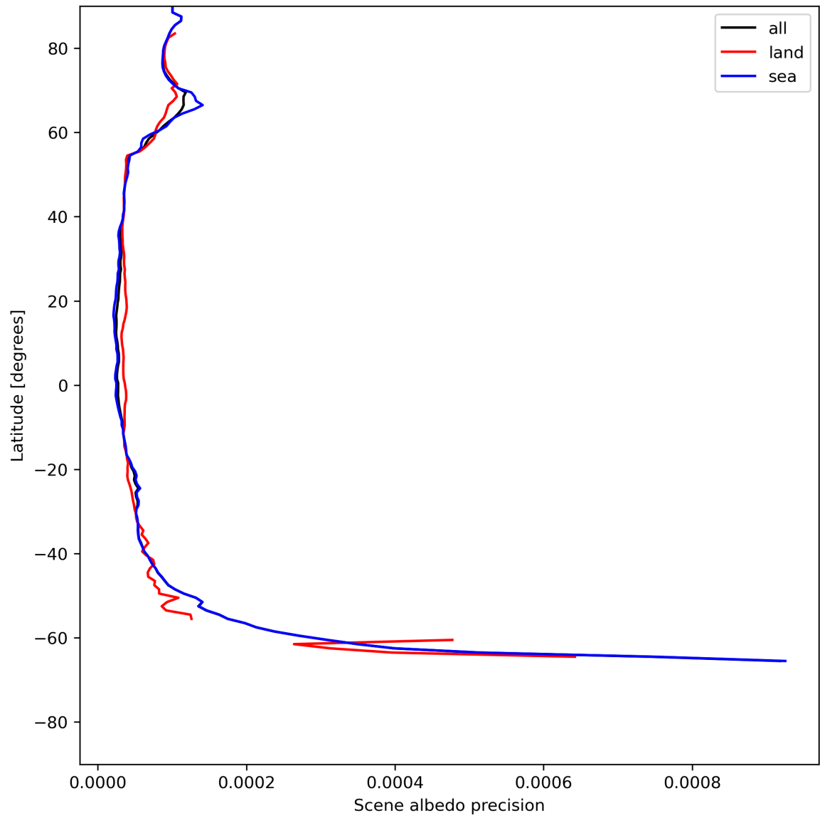
Figure 18: Zonal average of “Scene albedo precision” for 2024-06-03 to 2024-06-04.
