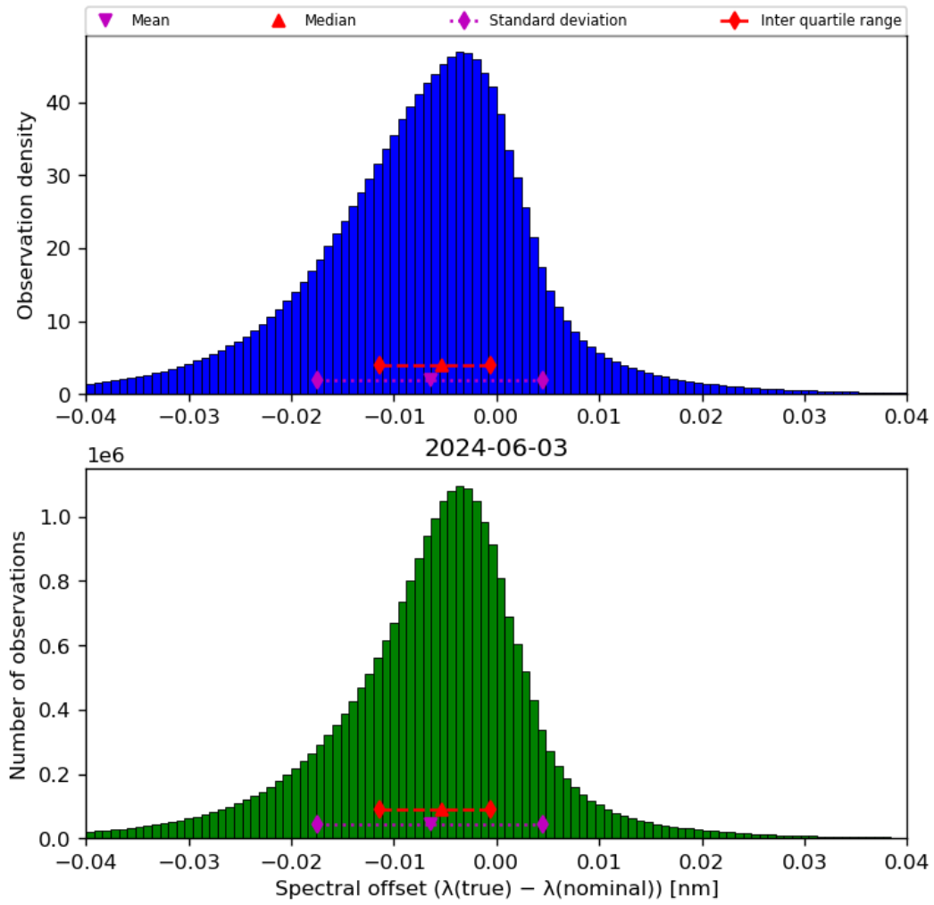
Figure 45: Histogram of “Spectral offset ( \lambda(\text{true}) - \lambda(\text{nominal}) )” for 2024-06-03 to 2024-06-04
