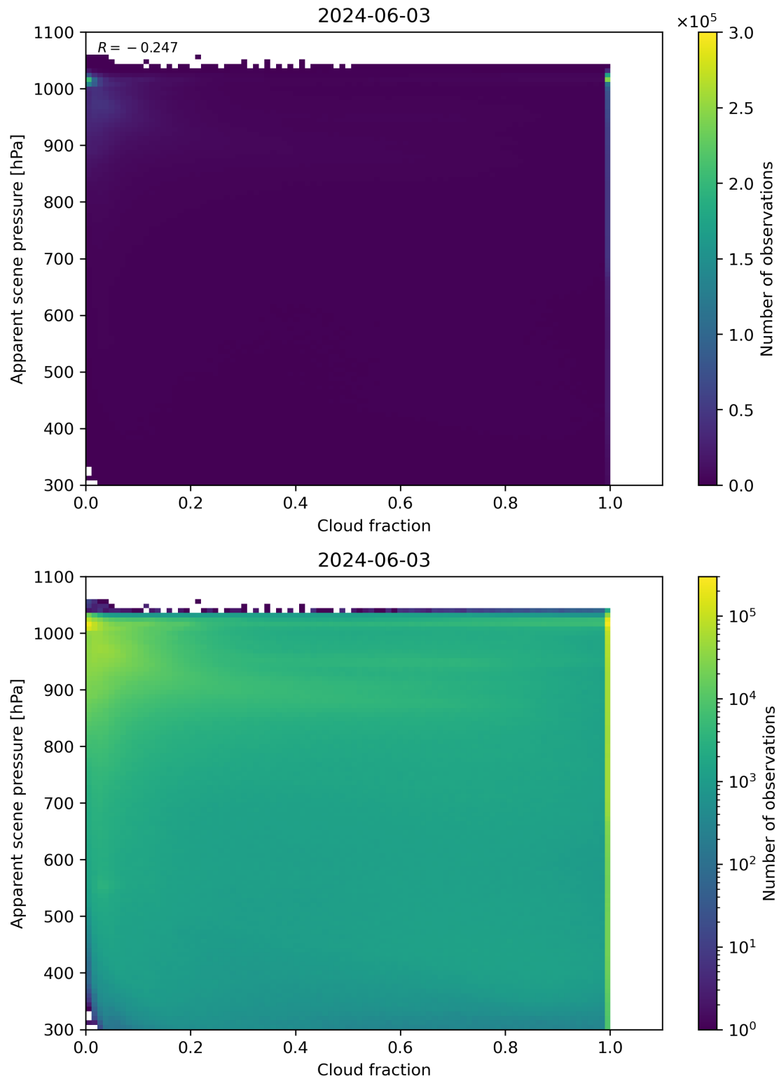
Figure 70: Scatter density plot of “Cloud fraction” against “Apparent scene pressure” for 2024-06-03 to 2024-06-04.
