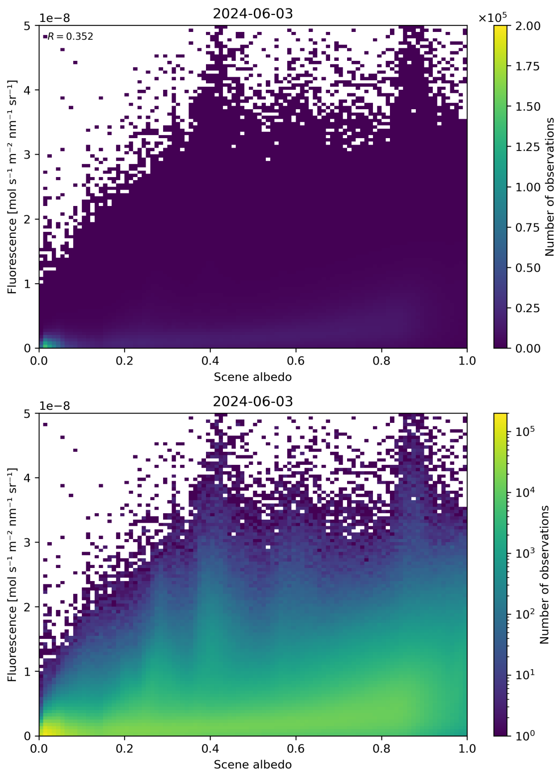
Figure 104: Scatter density plot of “Scene albedo” against “Fluorescence” for 2024-06-03 to 2024-06-04.
