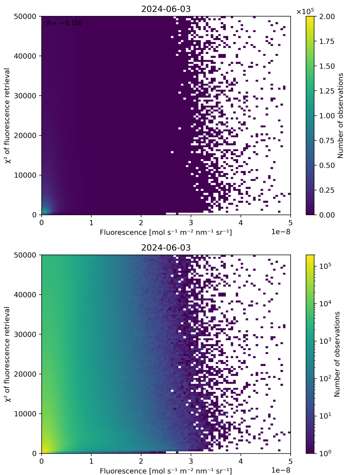
Figure 85: Scatter density plot of “Fluorescence” against “ \chi^2 of fluorescence retrieval” for 2024-06-03 to 2024-06-04.
