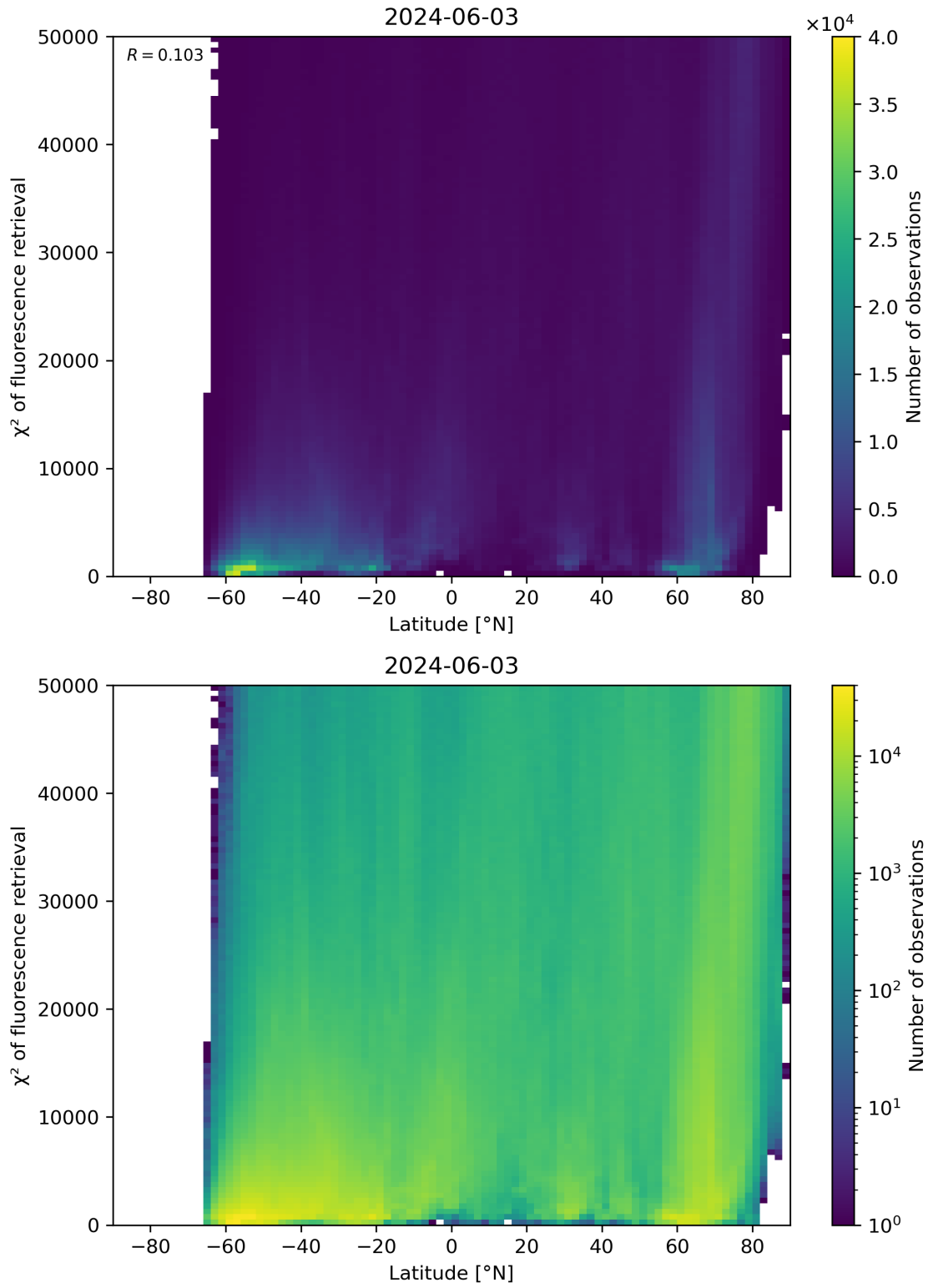
Figure 89: Scatter density plot of “Latitude” against “ \chi^2 of fluorescence retrieval” for 2024-06-03 to 2024-06-04.
