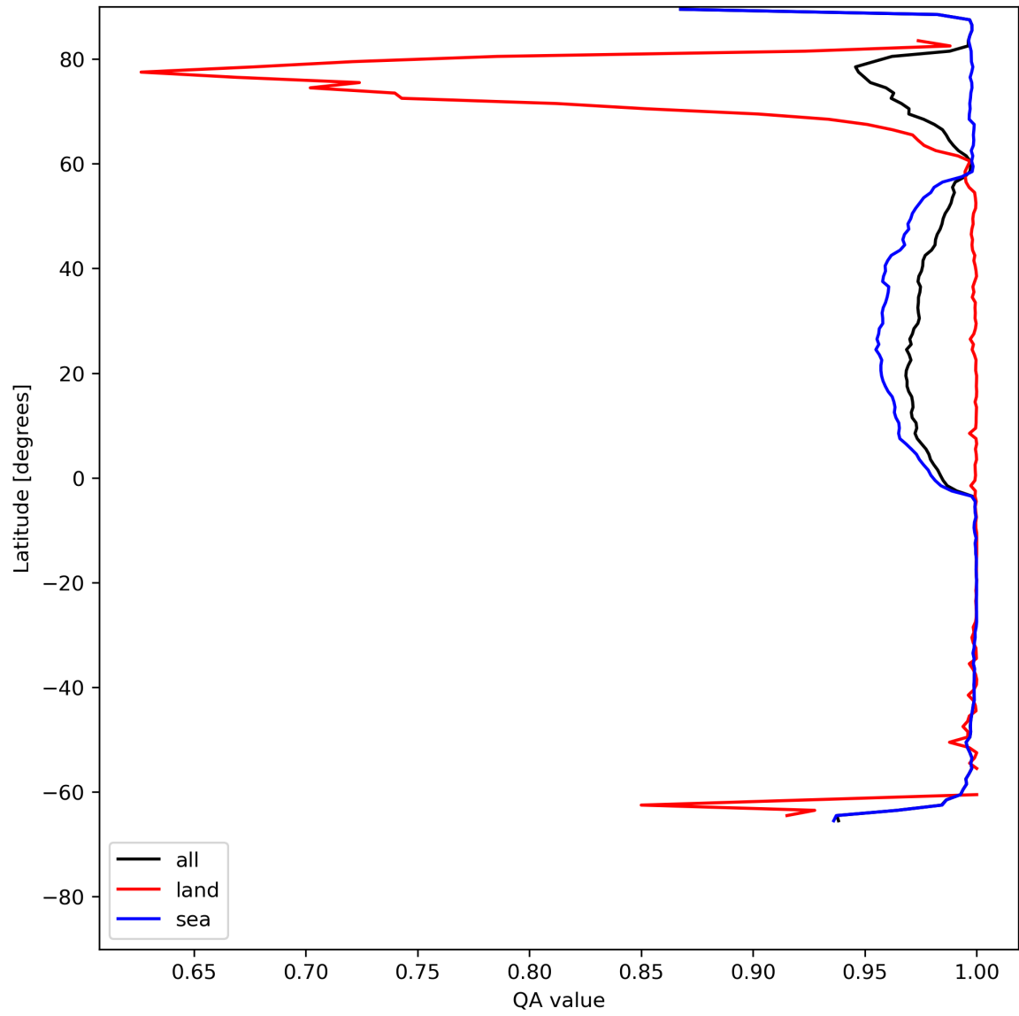
Figure 12: Zonal average of “QA value” for 2024-06-03 to 2024-06-04.
