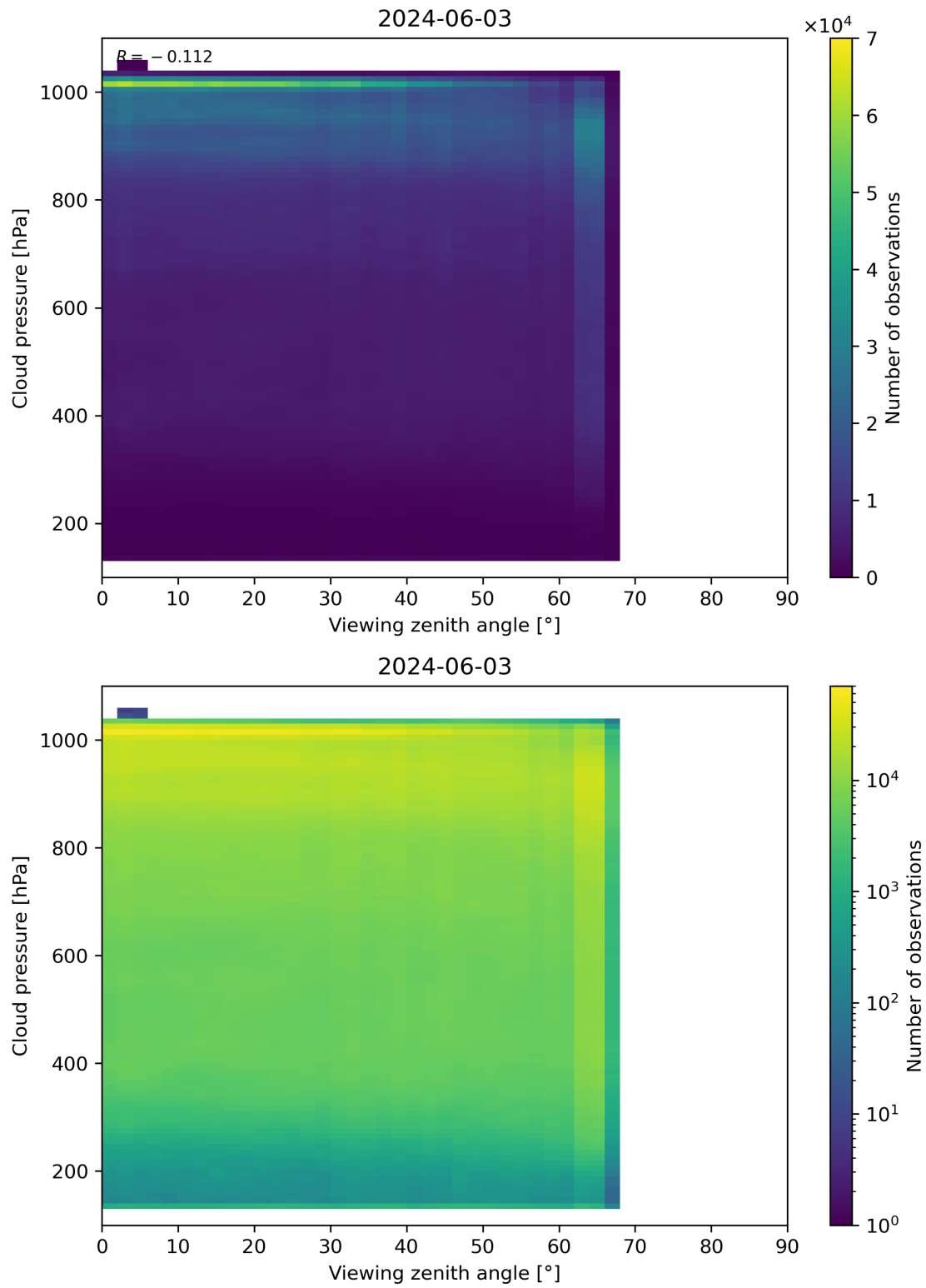
Figure 121: Scatter density plot of “Viewing zenith angle” against “Cloud pressure” for 2024-06-03 to 2024-06-04.
