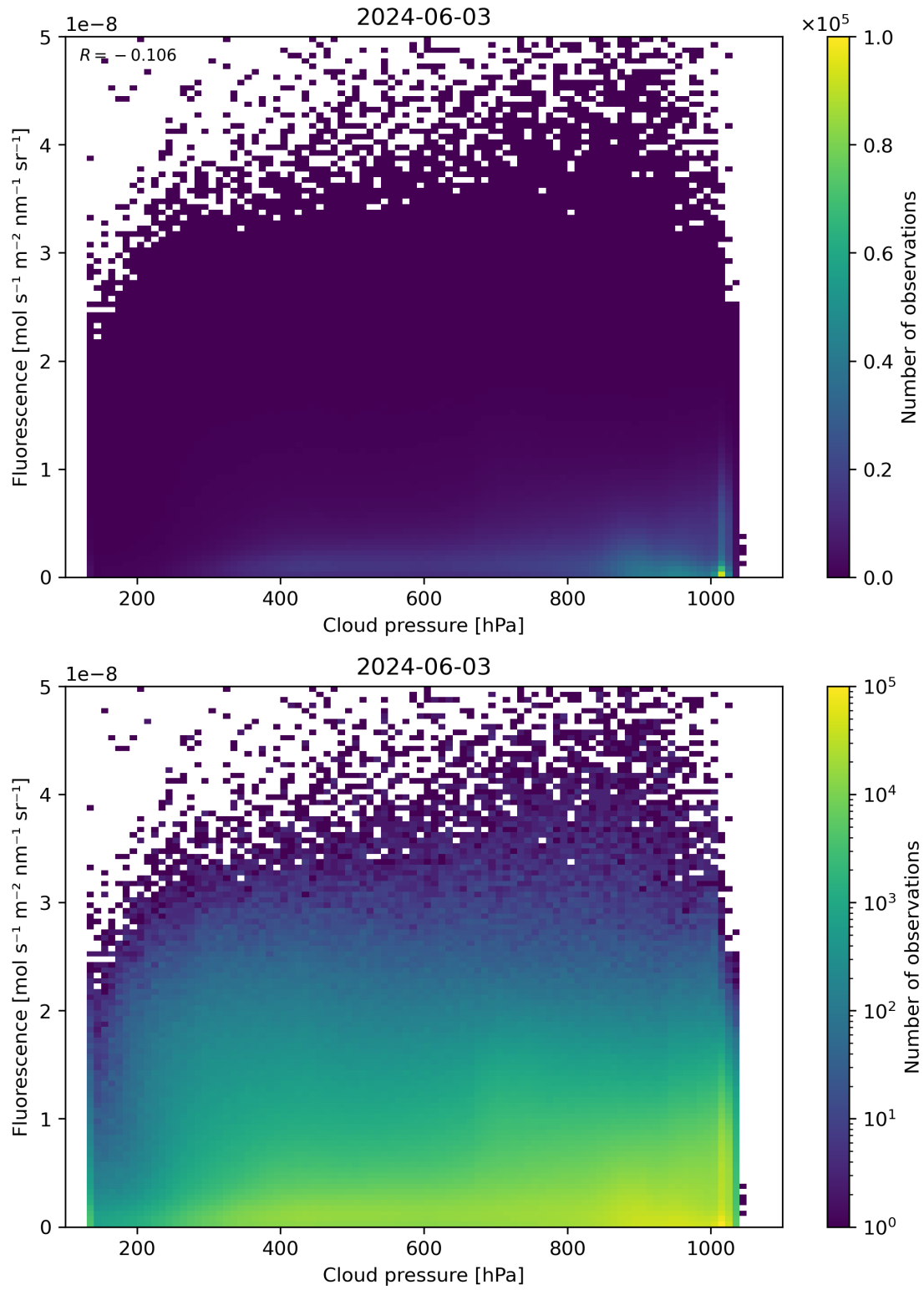
Figure 80: Scatter density plot of “Cloud pressure” against “Fluorescence” for 2024-06-03 to 2024-06-04.
