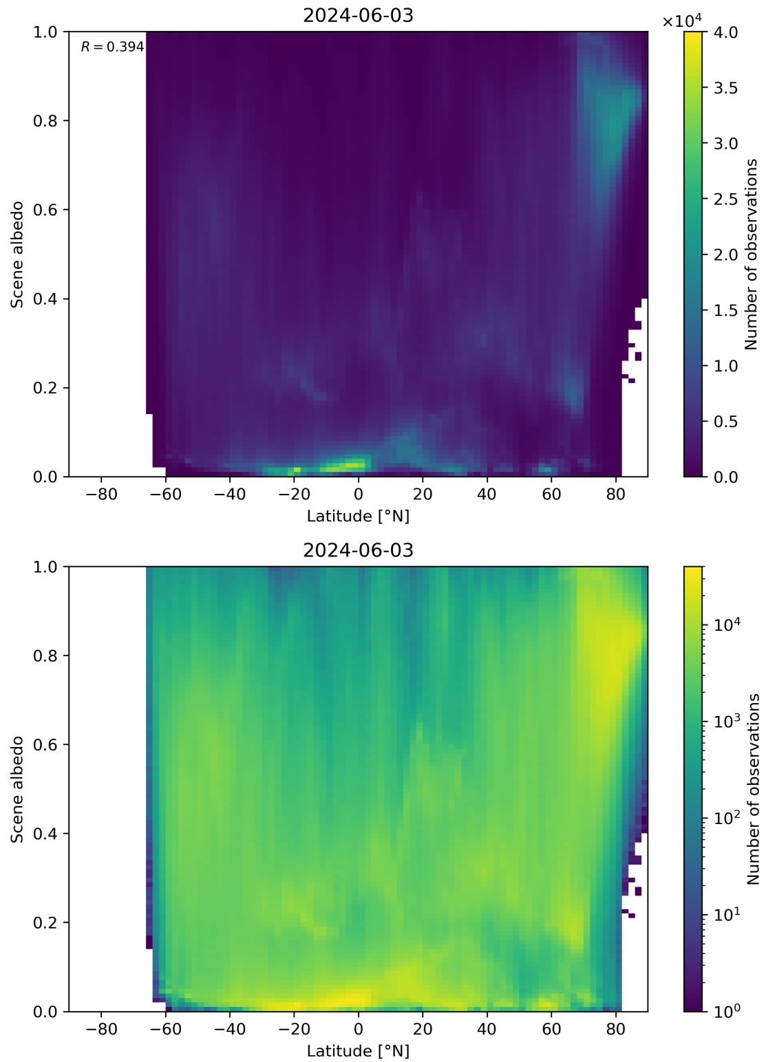
Figure 95: Scatter density plot of “Latitude” against “Scene albedo” for 2024-06-03 to 2024-06-04.
