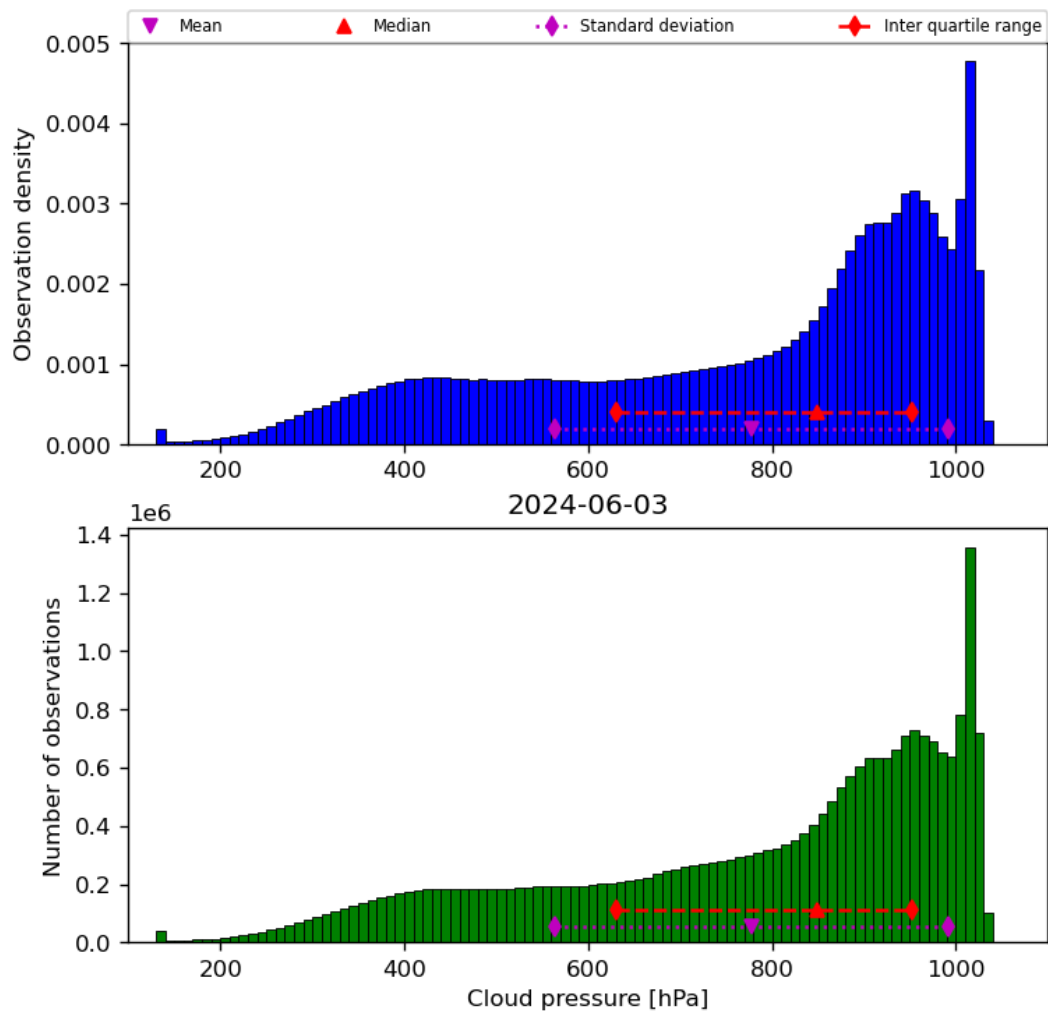
Figure 30: Histogram of “Cloud pressure” for 2024-06-03 to 2024-06-04
