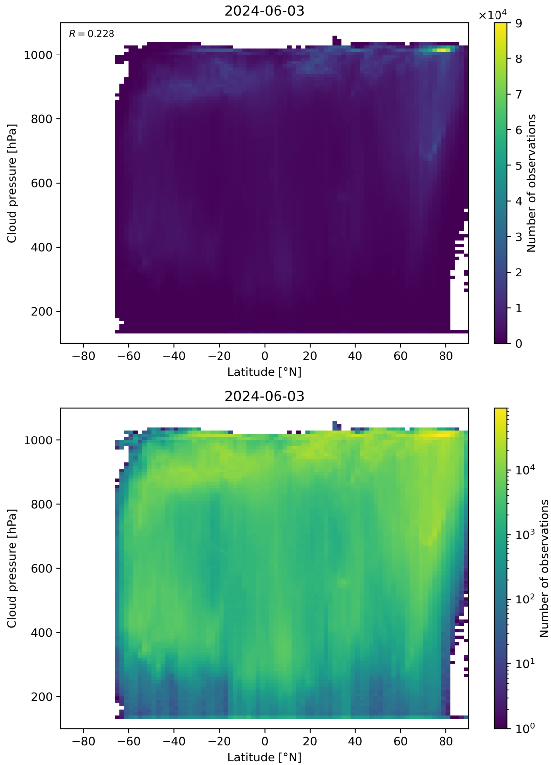
Figure 91: Scatter density plot of “Latitude” against “Cloud pressure” for 2024-06-03 to 2024-06-04.
