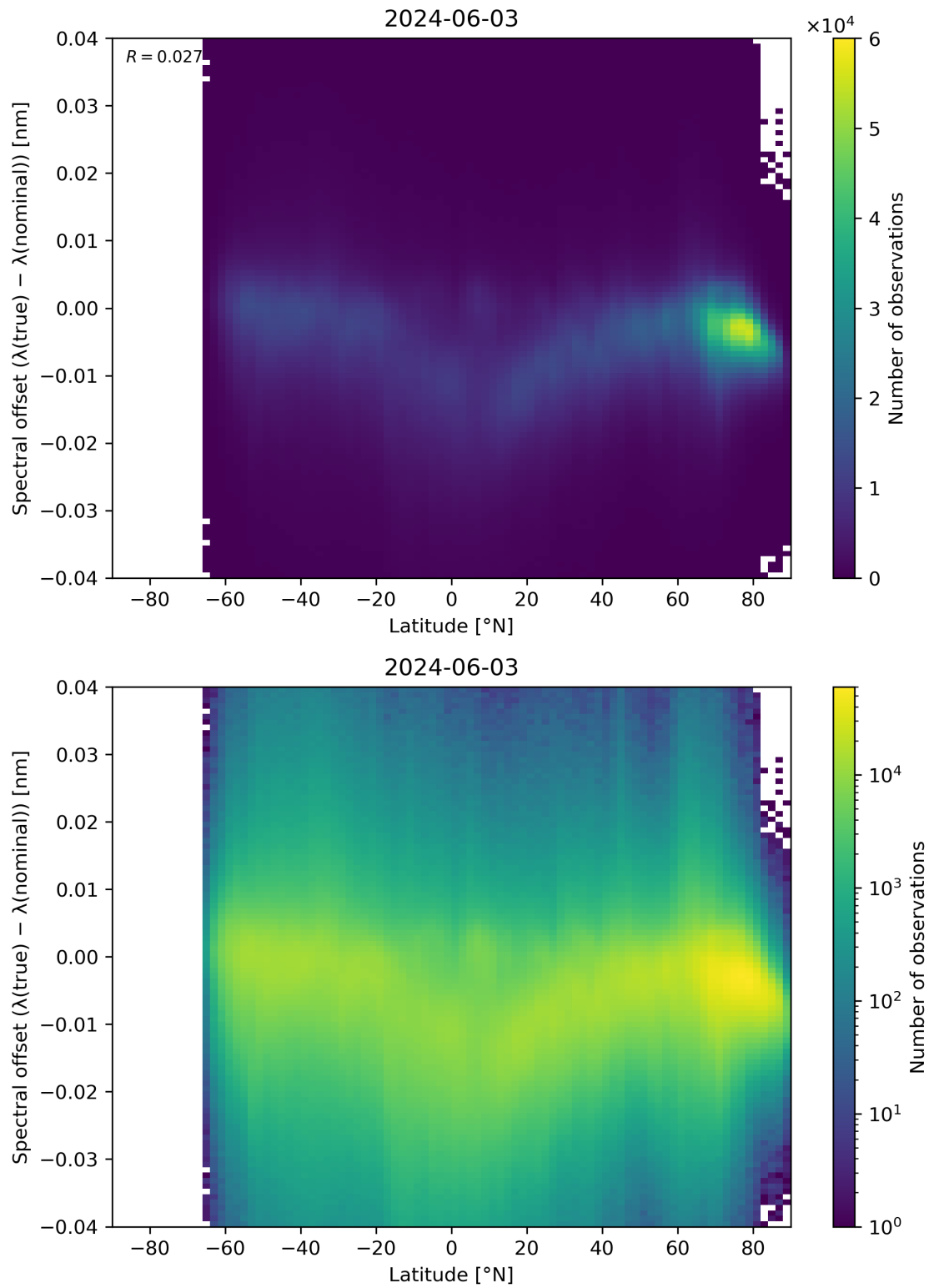
Figure 96: Scatter density plot of “Latitude” against “Spectral offset ( \lambda(\text{true}) - \lambda(\text{nominal}) )” for 2024-06-03 to 2024-06-04.
