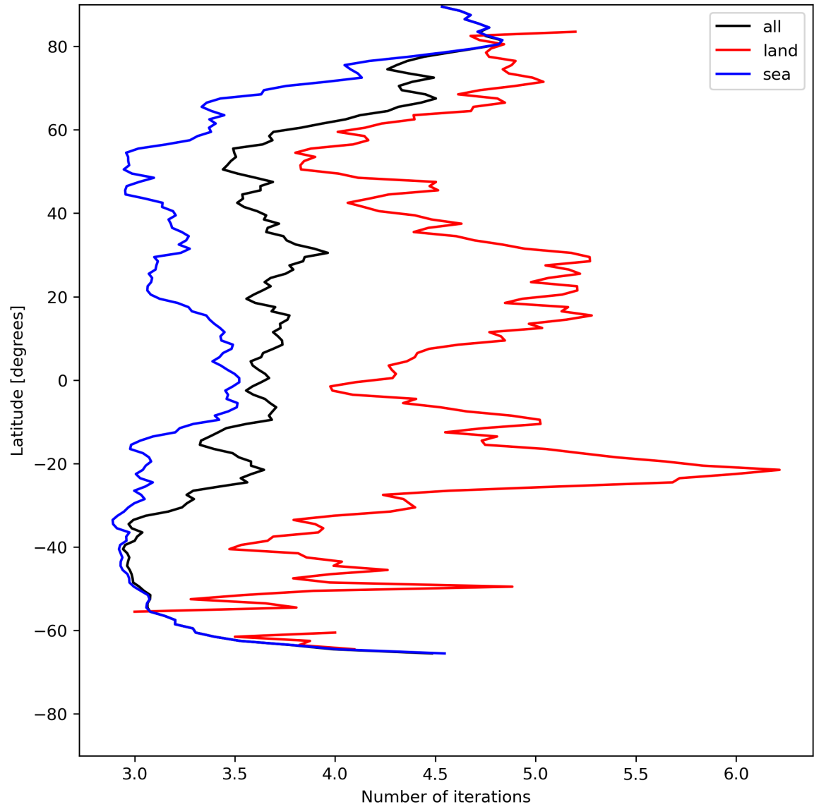
Figure 22: Zonal average of “Number of iterations” for 2024-06-03 to 2024-06-04.
