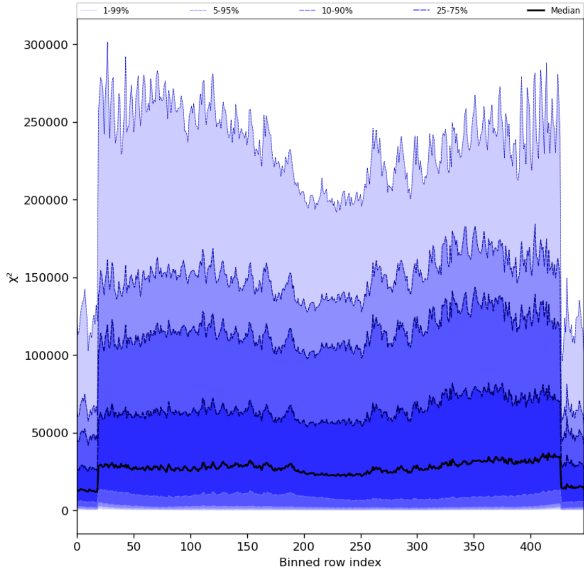
Figure 55: Along track statistics of “ \chi^2 ” for 2024-06-03 to 2024-06-04
