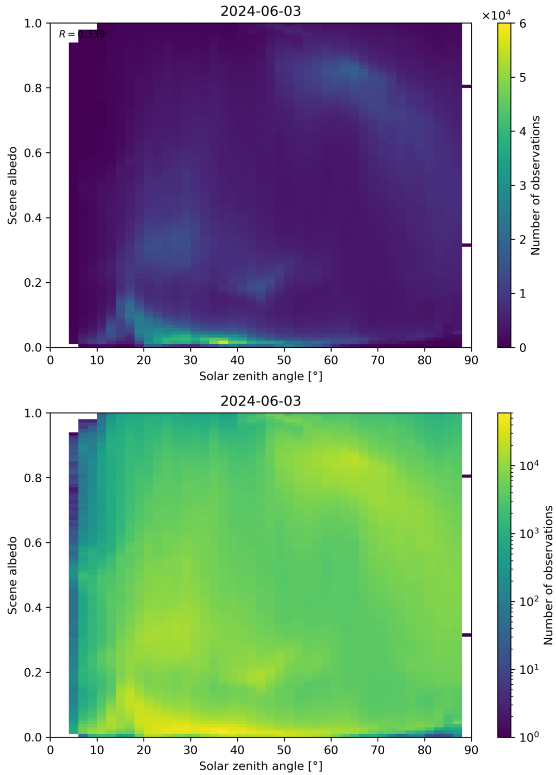
Figure 116: Scatter density plot of “Solar zenith angle” against “Scene albedo” for 2024-06-03 to 2024-06-04.
