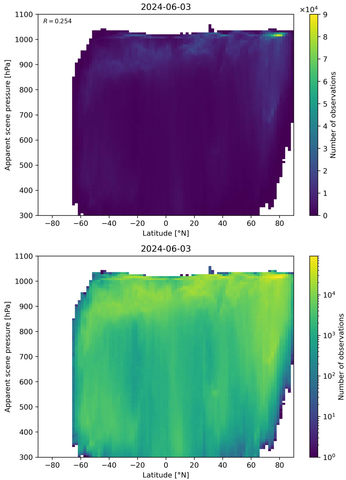
Figure 88: Scatter density plot of “Latitude” against “Apparent scene pressure” for 2024-06-03 to 2024-06-04.
