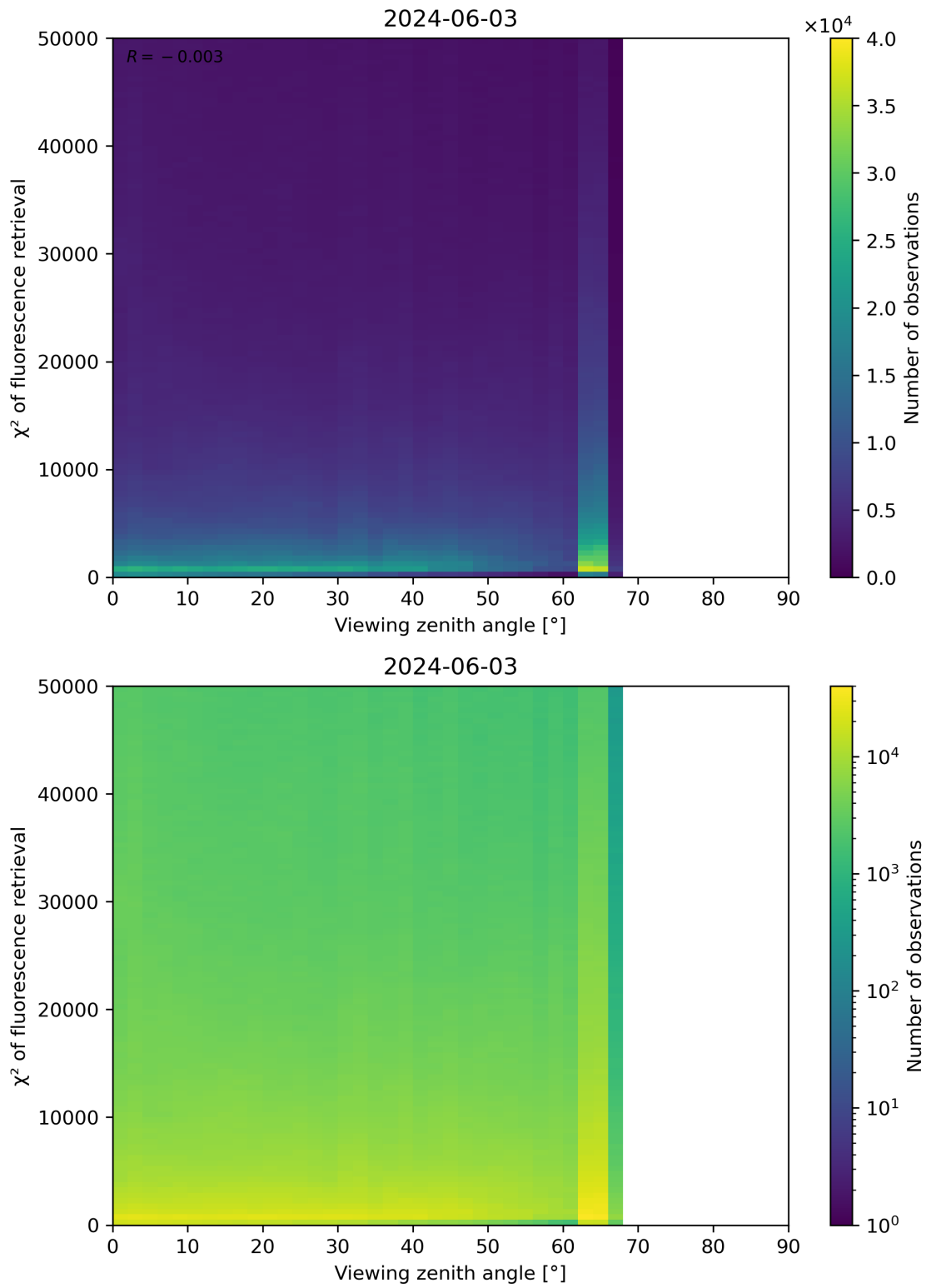
Figure 119: Scatter density plot of “Viewing zenith angle” against “ \chi^2 of fluorescence retrieval” for 2024-06-03 to 2024-06-04.
