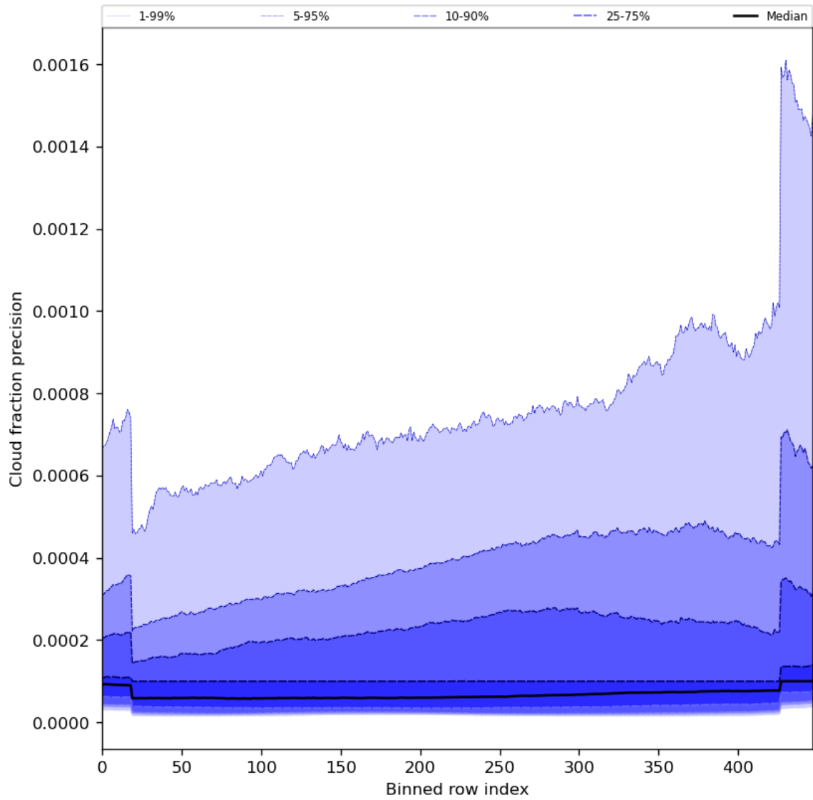
Figure 50: Along track statistics of “Cloud fraction precision” for 2024-06-03 to 2024-06-04
