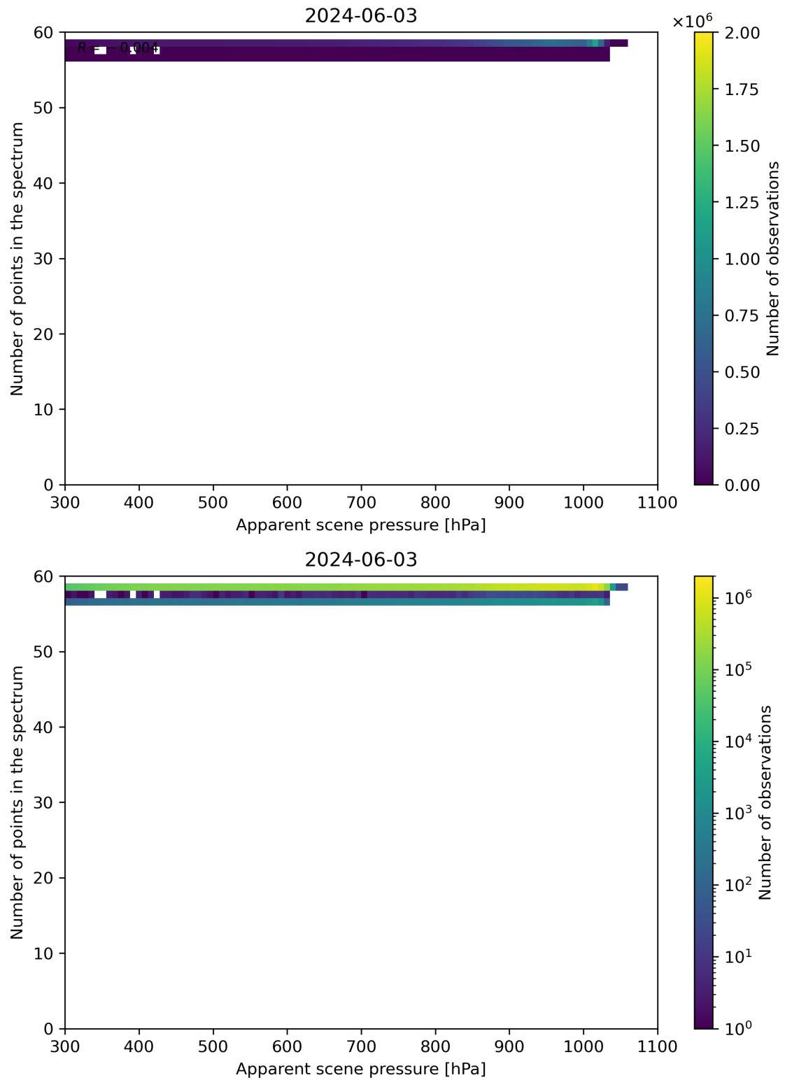
Figure 66: Scatter density plot of “Apparent scene pressure” against “Number of points in the spectrum” for 2024-06-03 to 2024-06-04.
