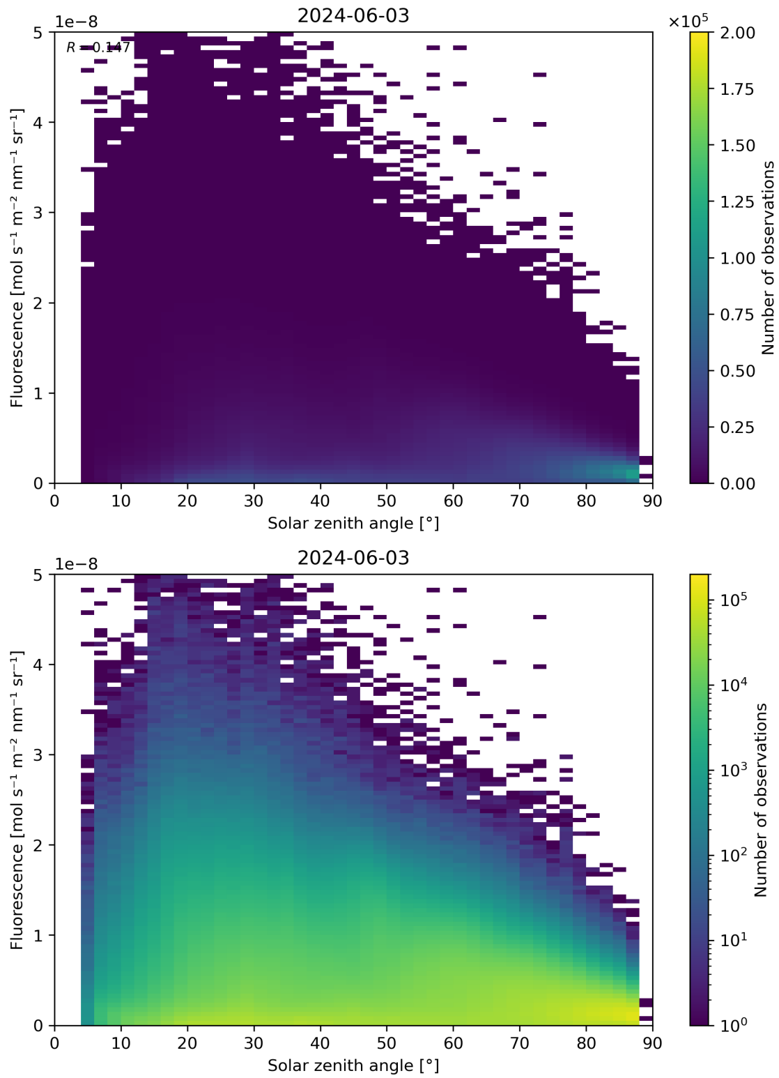
Figure 112: Scatter density plot of “Solar zenith angle” against “Fluorescence” for 2024-06-03 to 2024-06-04.
