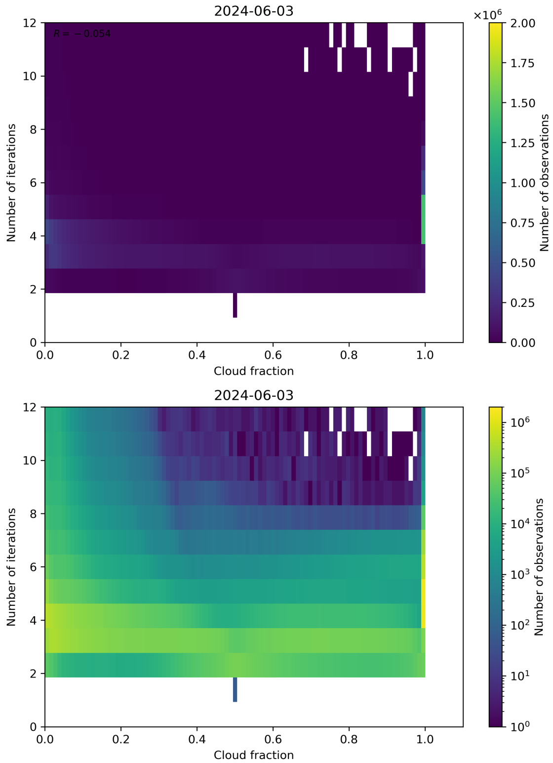
Figure 73: Scatter density plot of “Cloud fraction” against “Number of iterations” for 2024-06-03 to 2024-06-04.
