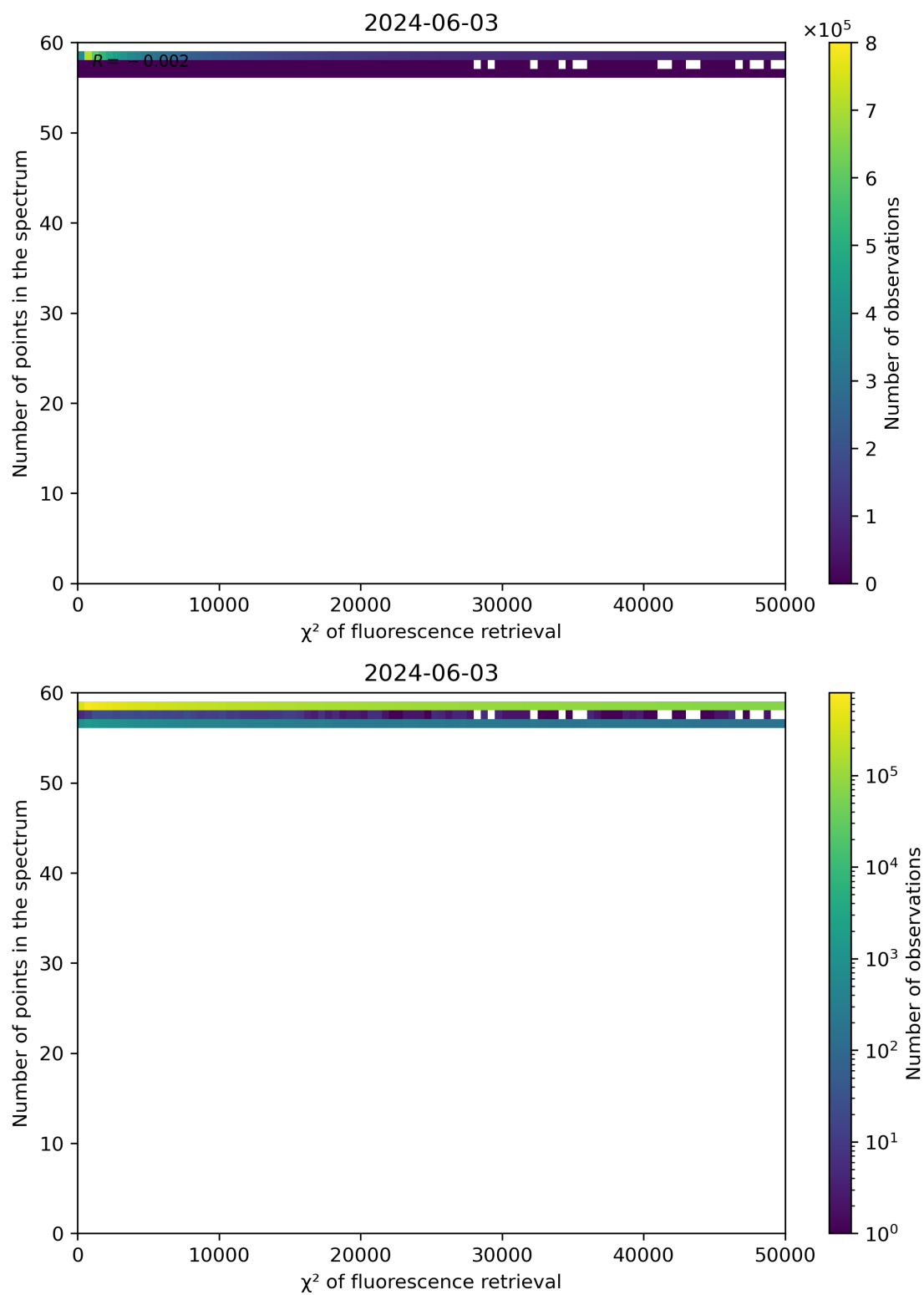
Figure 68: Scatter density plot of " \chi^2 of fluorescence retrieval" against "Number of points in the spectrum" for 2024-06-03 to 2024-06-04.
