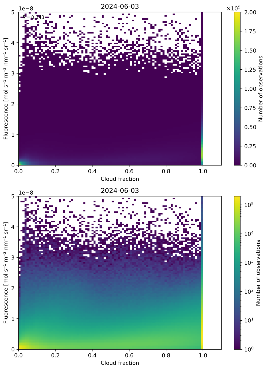
Figure 72: Scatter density plot of “Cloud fraction” against “Fluorescence” for 2024-06-03 to 2024-06-04.
