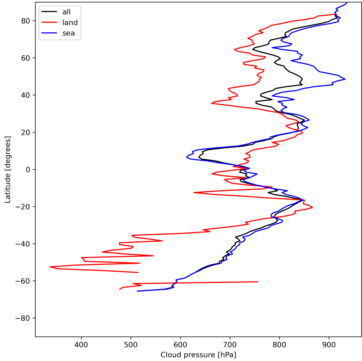
Figure 13: Zonal average of “Cloud pressure” for 2024-06-03 to 2024-06-04.
