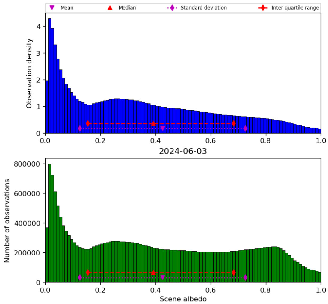
Figure 34: Histogram of “Scene albedo” for 2024-06-03 to 2024-06-04
