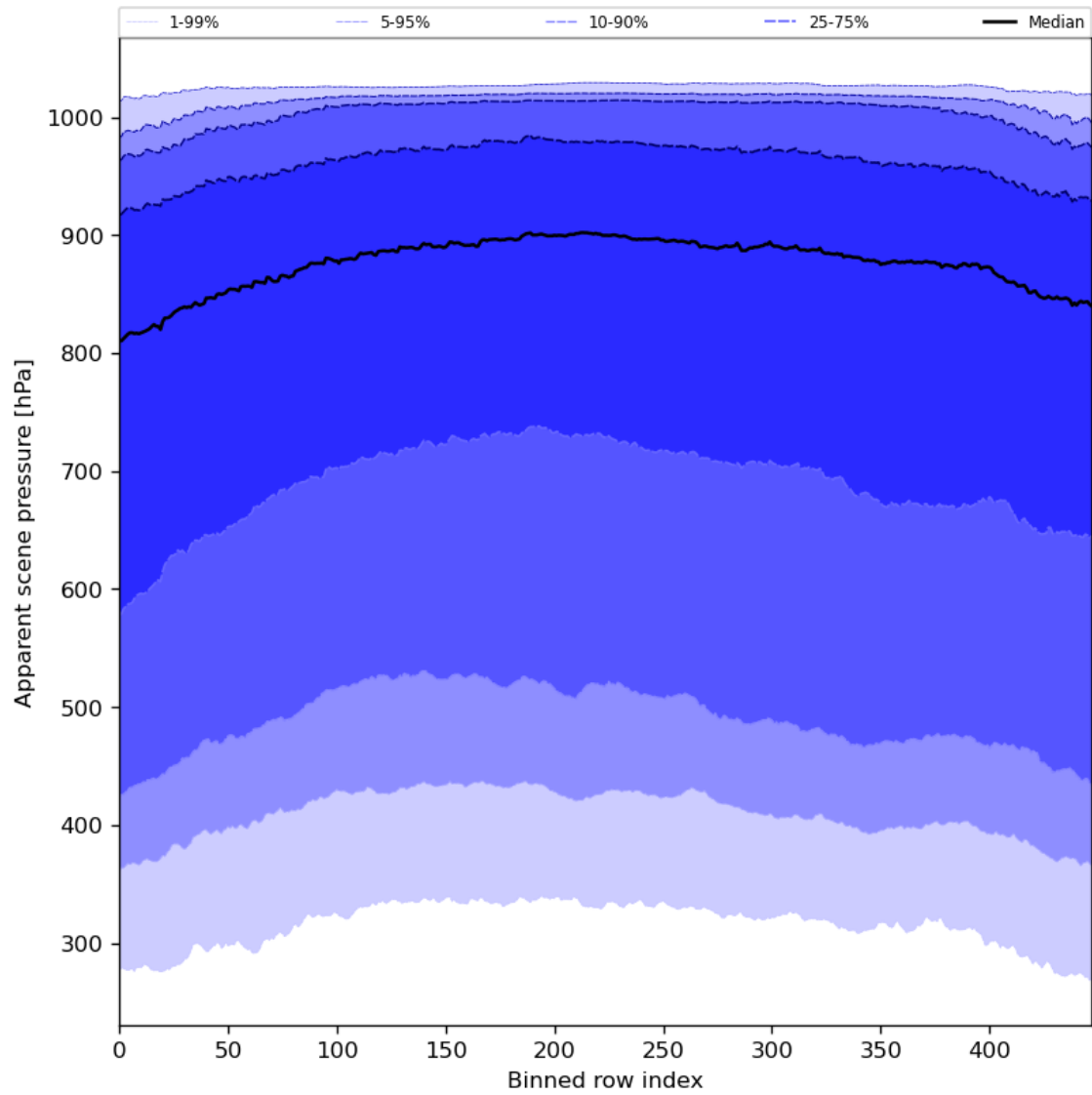
Figure 53: Along track statistics of “Apparent scene pressure” for 2024-06-03 to 2024-06-04
