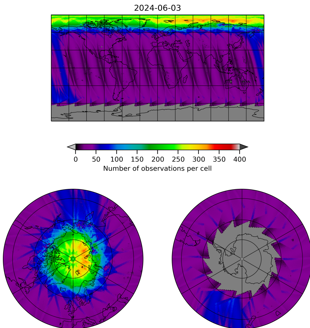
Figure 11: Map of the number of observations for 2024-06-03 to 2024-06-04
