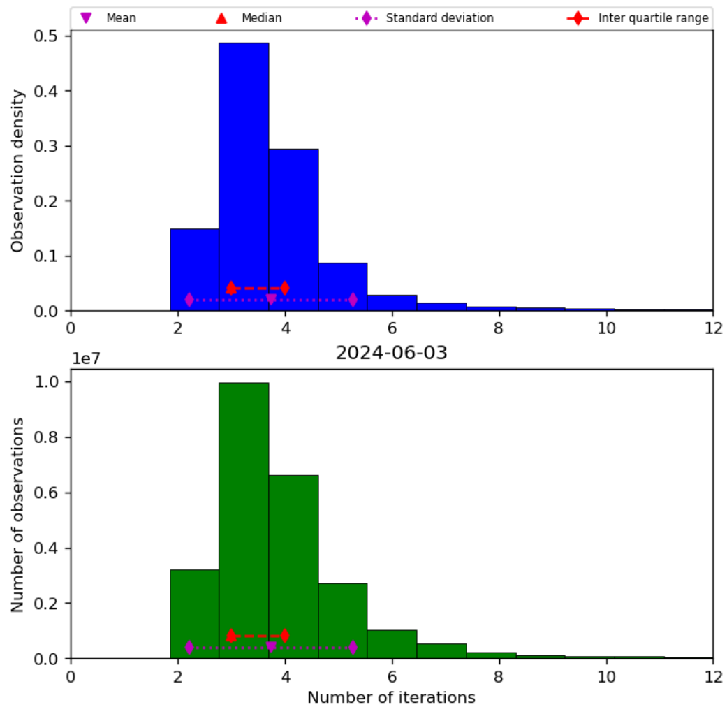
Figure 39: Histogram of “Number of iterations” for 2024-06-03 to 2024-06-04
