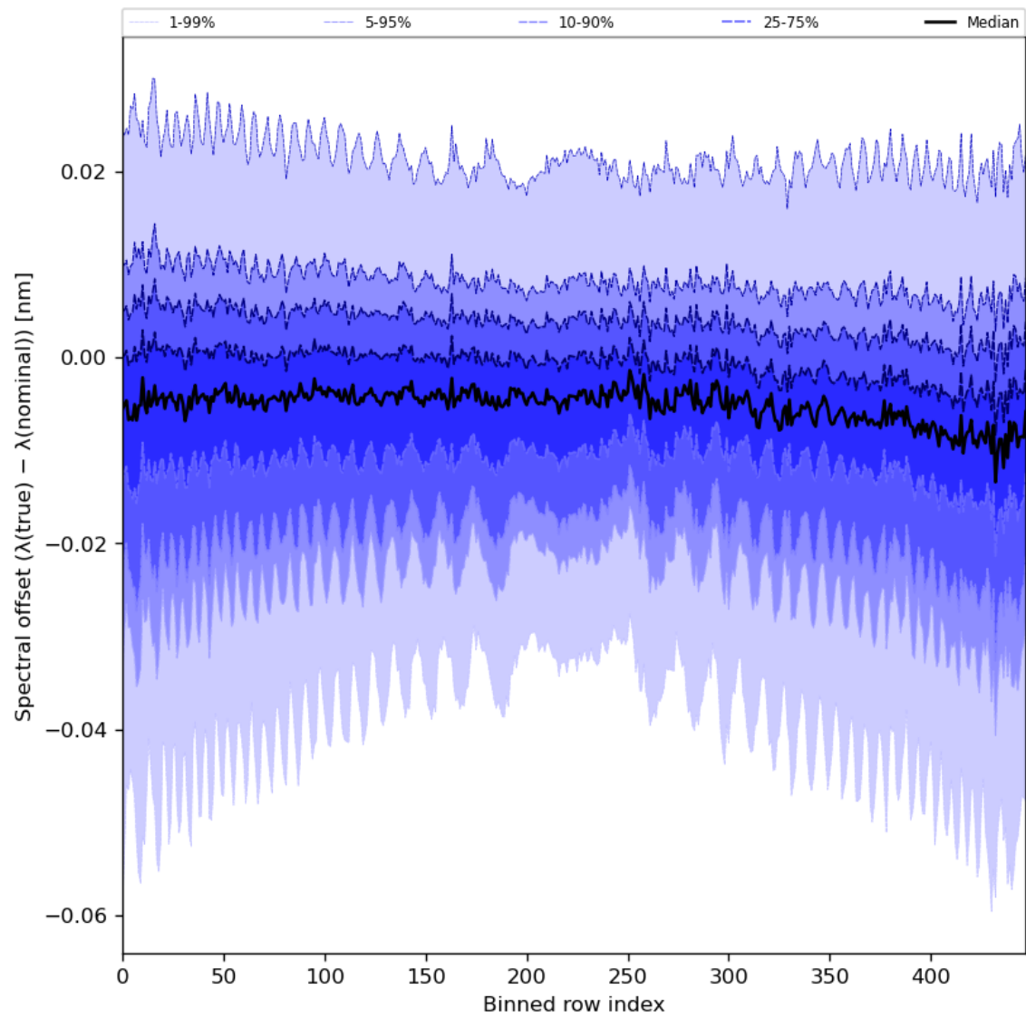
Figure 62: Along track statistics of “Spectral offset ( \lambda(\text{true}) - \lambda(\text{nominal}) )” for 2024-06-03 to 2024-06-04
