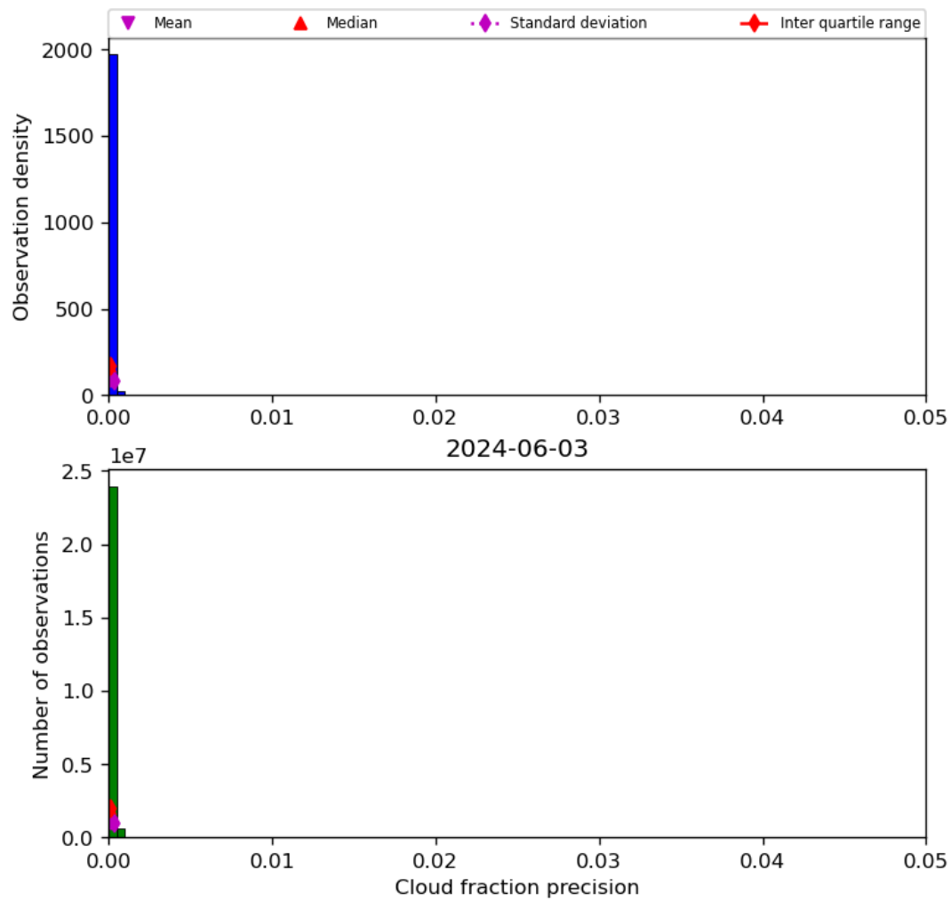
Figure 33: Histogram of “Cloud fraction precision” for 2024-06-03 to 2024-06-04
