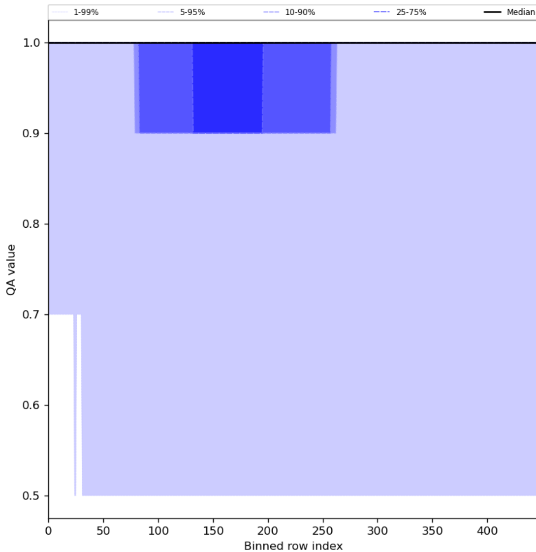
Figure 46: Along track statistics of “QA value” for 2024-06-03 to 2024-06-04
