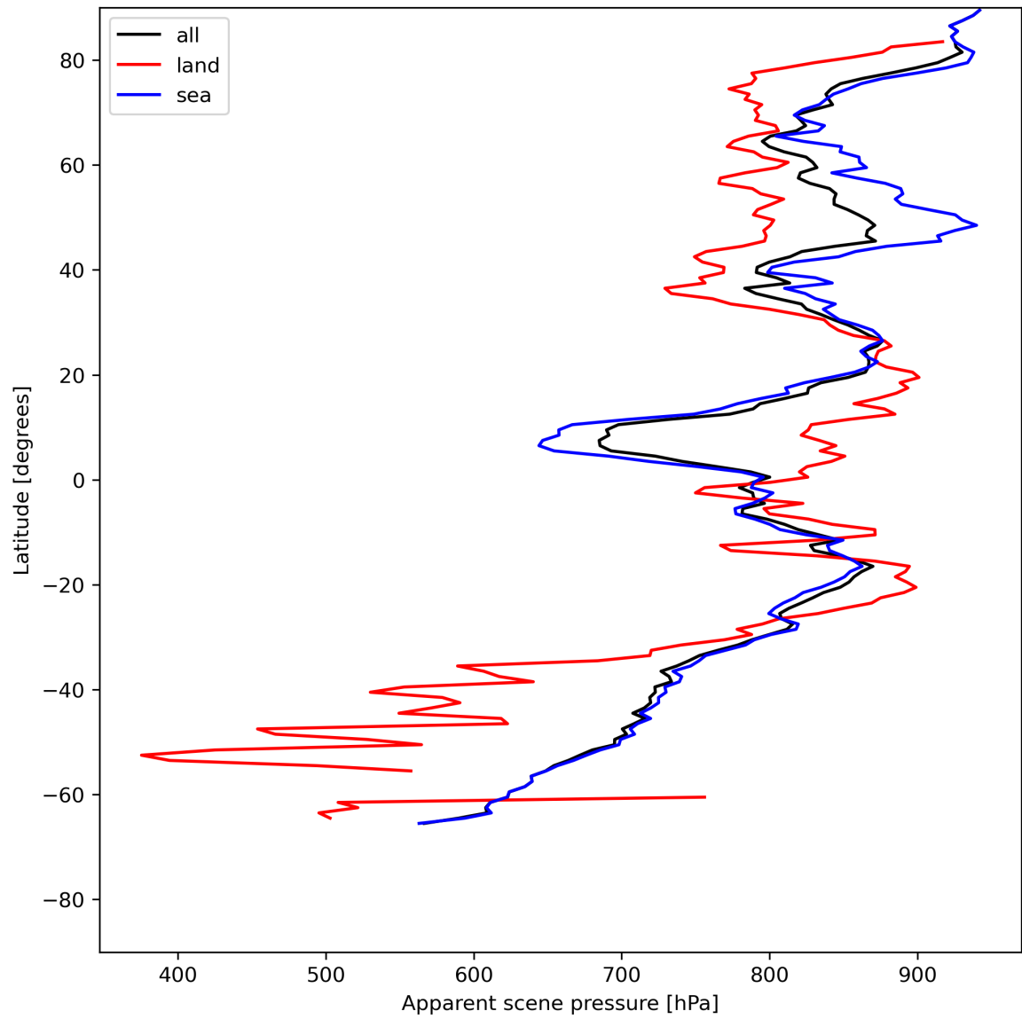
Figure 19: Zonal average of “Apparent scene pressure” for 2024-06-03 to 2024-06-04.
