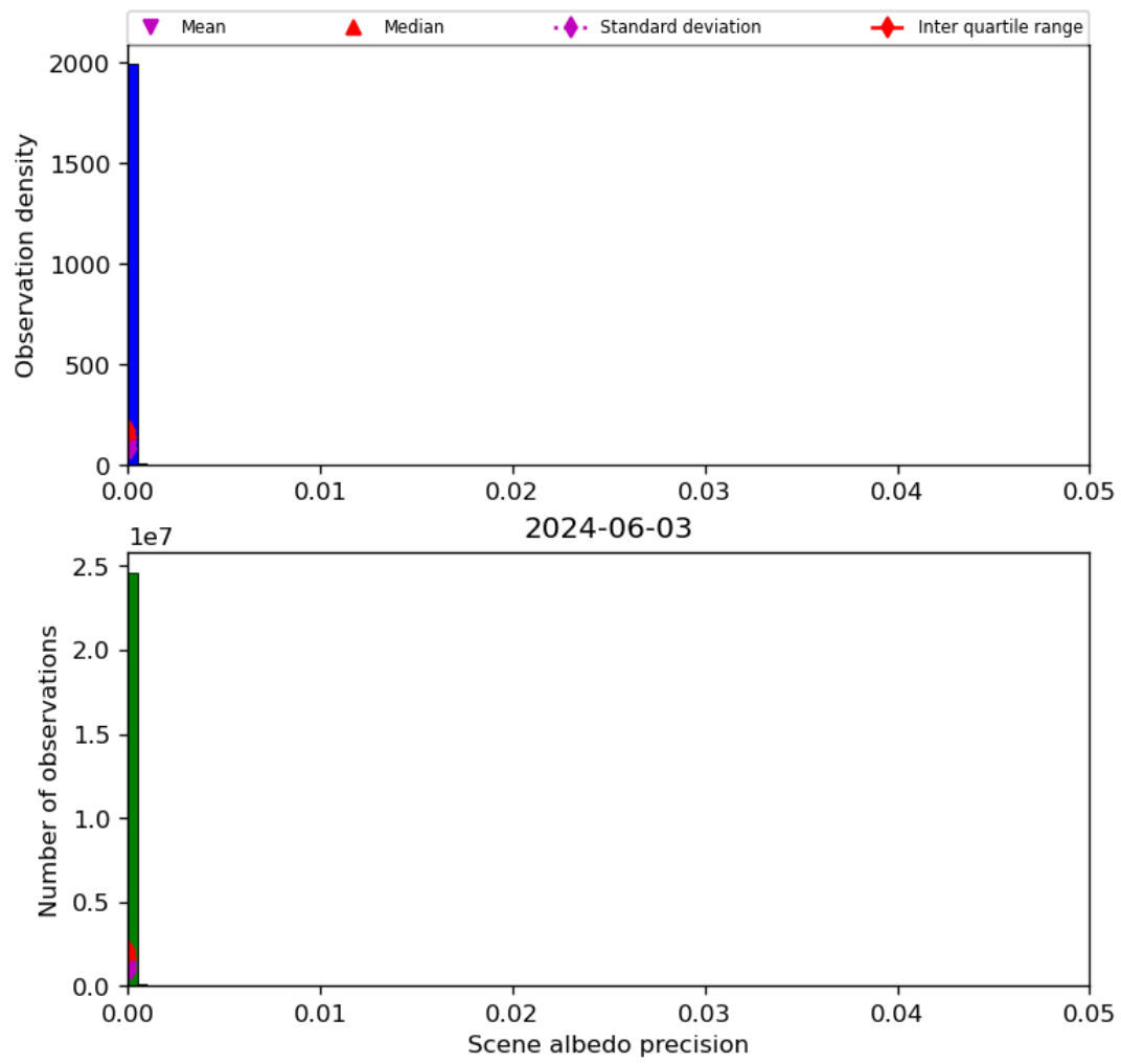
Figure 35: Histogram of “Scene albedo precision” for 2024-06-03 to 2024-06-04
