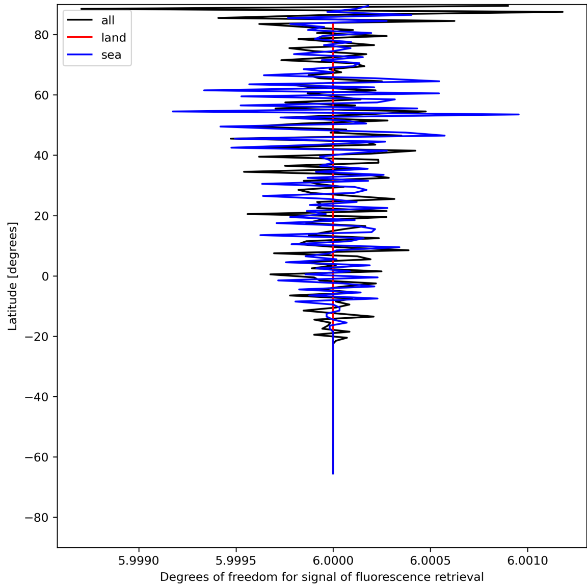
Figure 26: Zonal average of “Degrees of freedom for signal of fluorescence retrieval” for 2024-06-03 to 2024-06-04.
