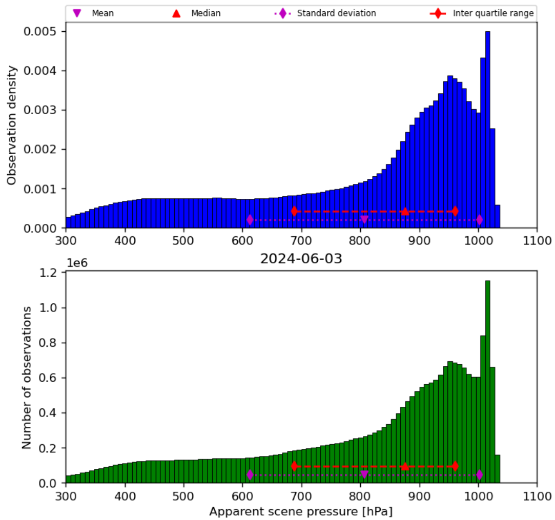
Figure 36: Histogram of “Apparent scene pressure” for 2024-06-03 to 2024-06-04
