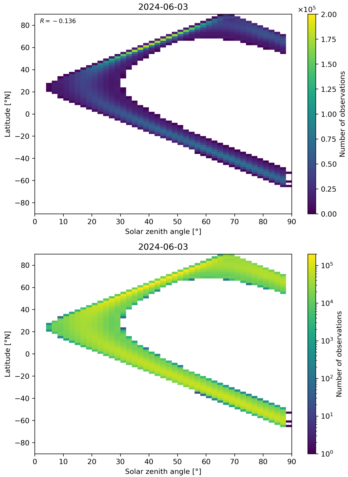
Figure 113: Scatter density plot of “Solar zenith angle” against “Latitude” for 2024-06-03 to 2024-06-04.
