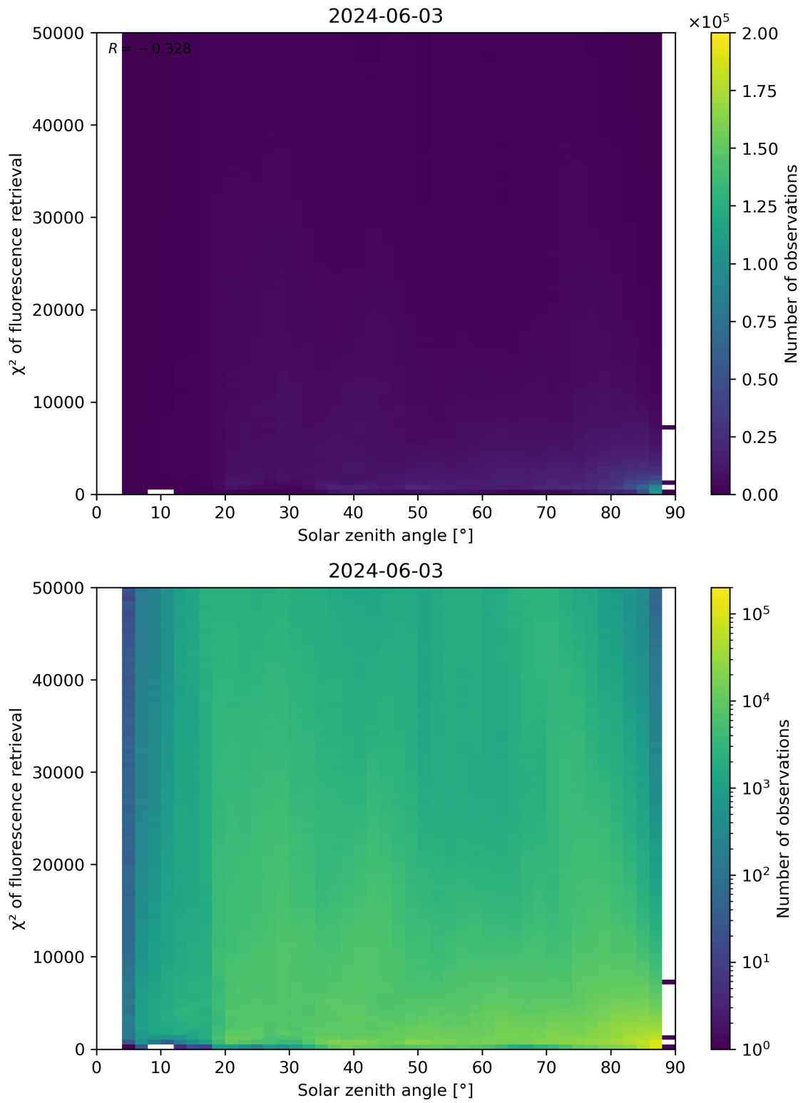
Figure 109: Scatter density plot of “Solar zenith angle” against “ \chi^2 of fluorescence retrieval” for 2024-06-03 to 2024-06-04.
