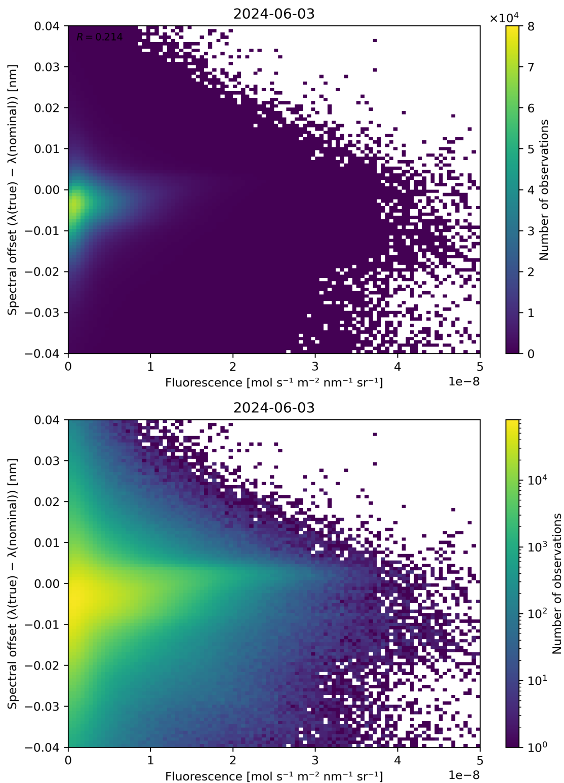
Figure 87: Scatter density plot of “Fluorescence” against “Spectral offset ( \lambda(\text{true}) - \lambda(\text{nominal}) )” for 2024-06-03 to 2024-06-04.
