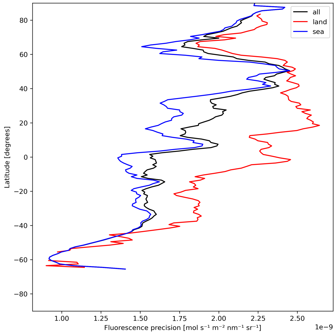
Figure 24: Zonal average of “Fluorescence precision” for 2024-06-03 to 2024-06-04.
