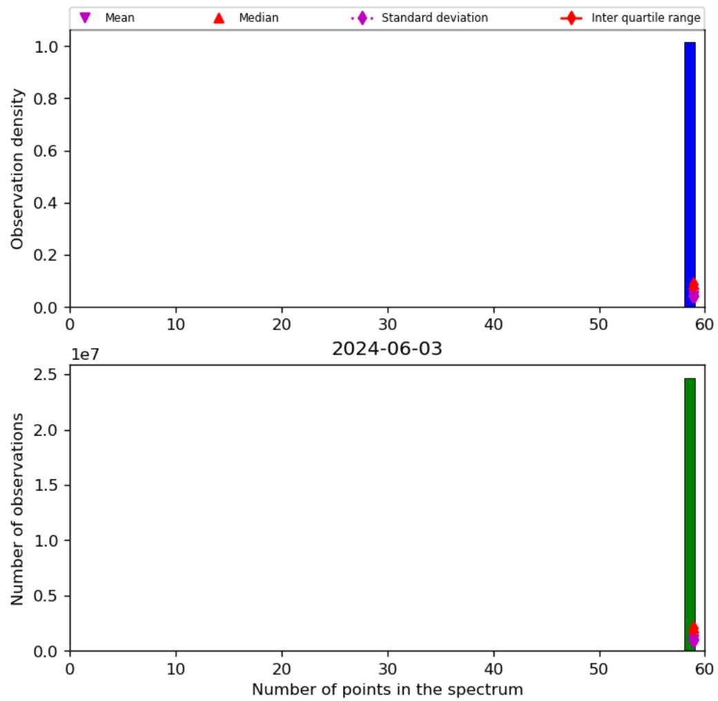
Figure 44: Histogram of “Number of points in the spectrum” for 2024-06-03 to 2024-06-04
