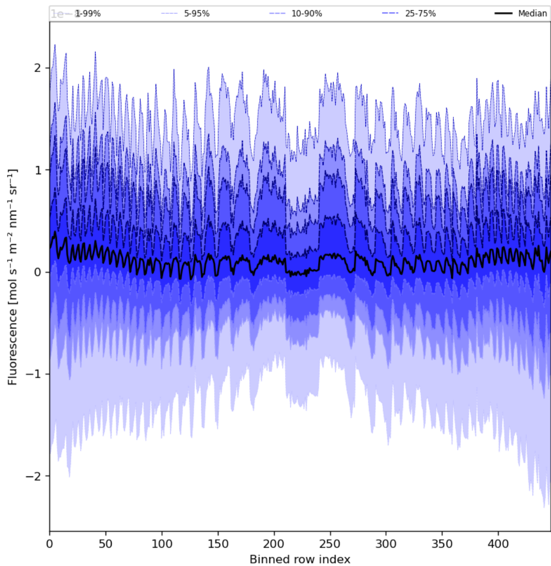
Figure 57: Along track statistics of “Fluorescence” for 2024-06-03 to 2024-06-04
