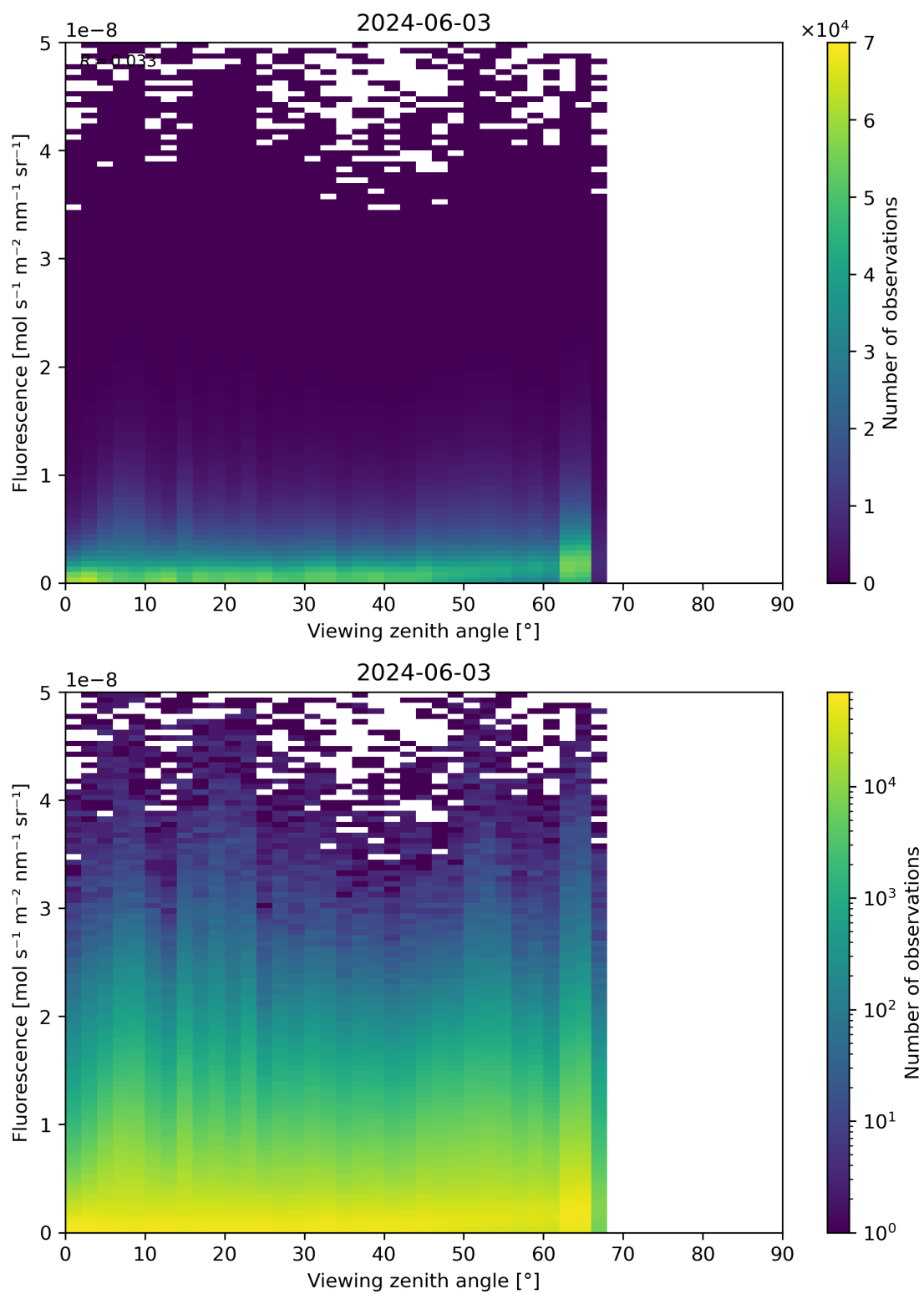
Figure 122: Scatter density plot of "Viewing zenith angle" against "Fluorescence" for 2024-06-03 to 2024-06-04.
