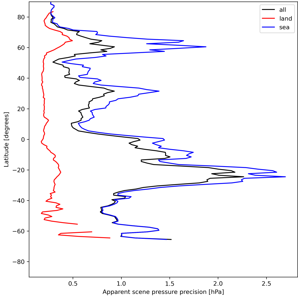
Figure 20: Zonal average of “Apparent scene pressure precision” for 2024-06-03 to 2024-06-04.
