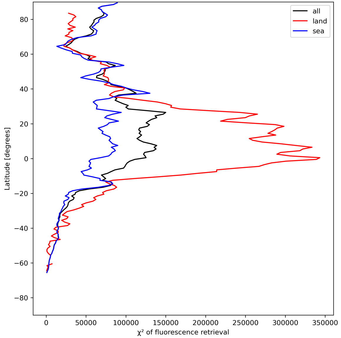
Figure 25: Zonal average of “ \chi^2 of fluorescence retrieval” for 2024-06-03 to 2024-06-04.
