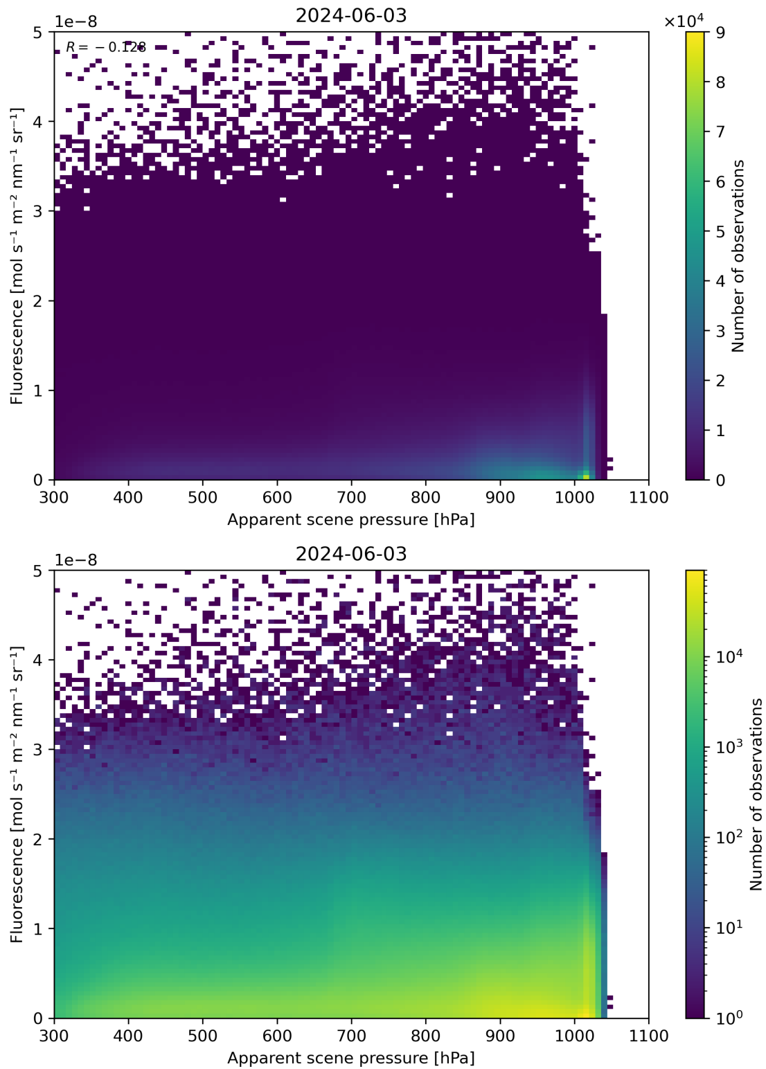
Figure 64: Scatter density plot of “Apparent scene pressure” against “Fluorescence” for 2024-06-03 to 2024-06-04.
