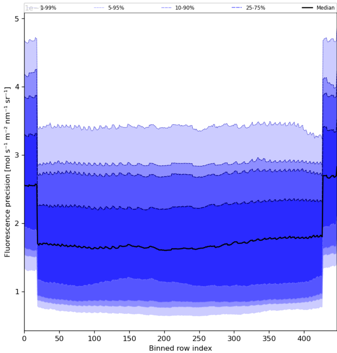
Figure 58: Along track statistics of “Fluorescence precision” for 2024-06-03 to 2024-06-04
