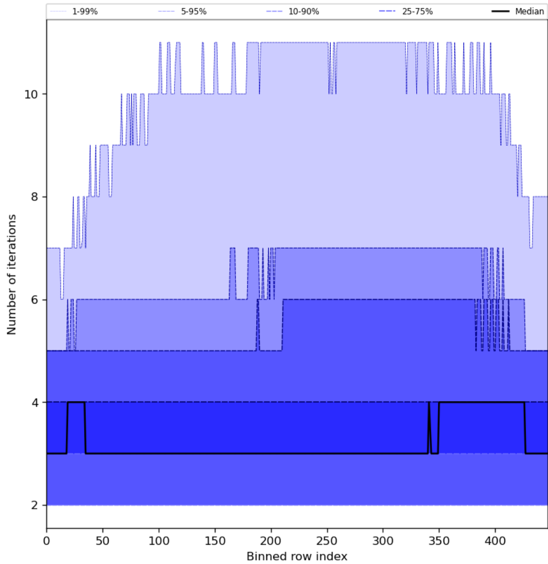
Figure 56: Along track statistics of “Number of iterations” for 2024-06-03 to 2024-06-04
