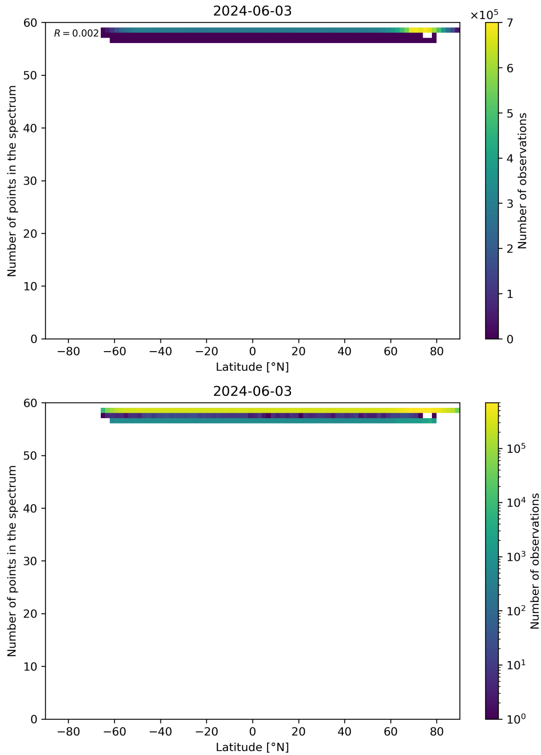
Figure 94: Scatter density plot of “Latitude” against “Number of points in the spectrum” for 2024-06-03 to 2024-06-04.
