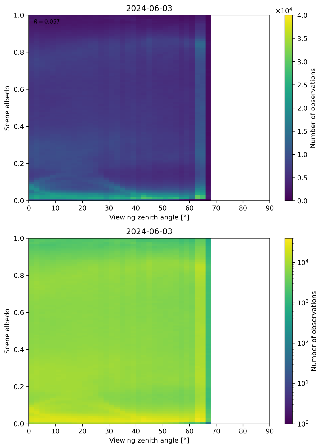
Figure 126: Scatter density plot of “Viewing zenith angle” against “Scene albedo” for 2024-06-03 to 2024-06-04.
