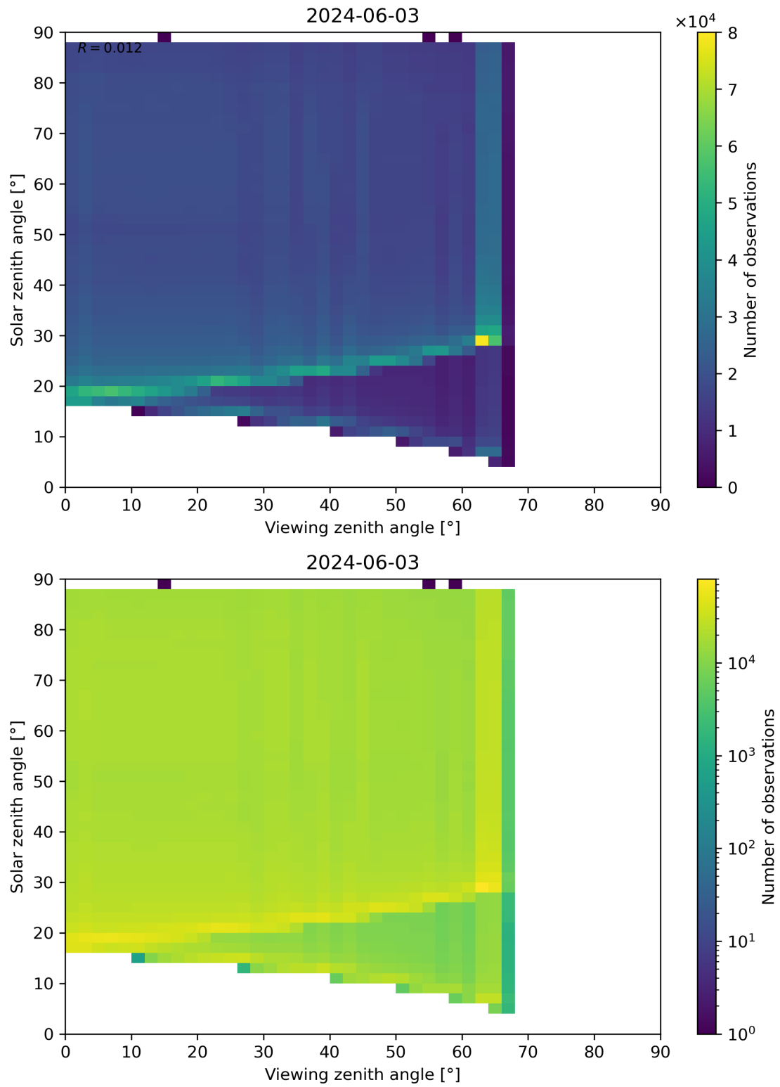
Figure 127: Scatter density plot of “Viewing zenith angle” against “Solar zenith angle” for 2024-06-03 to 2024-06-04.
