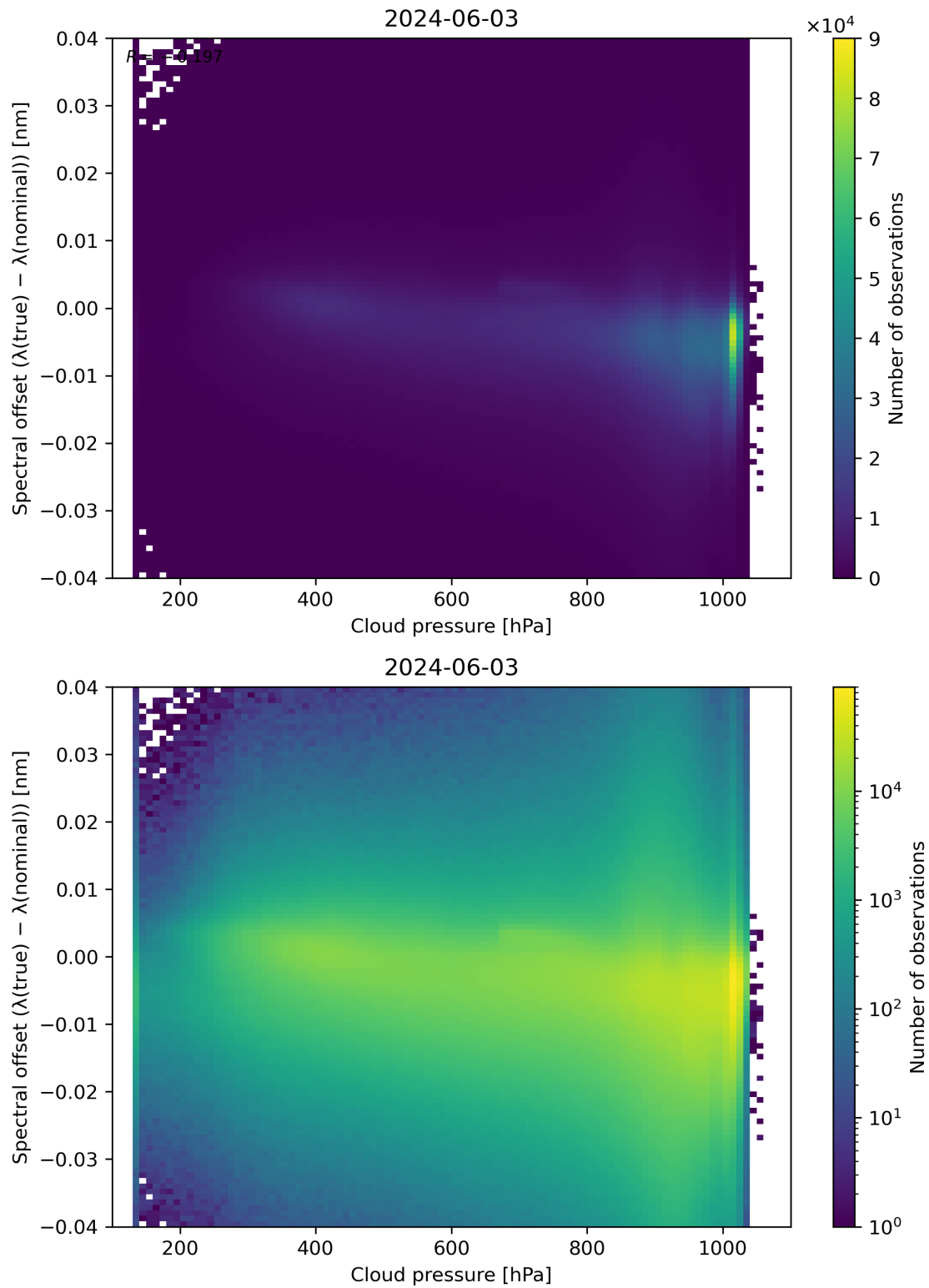
Figure 84: Scatter density plot of “Cloud pressure” against “Spectral offset ( \lambda(\text{true}) - \lambda(\text{nominal}) )” for 2024-06-03 to 2024-06-04.
