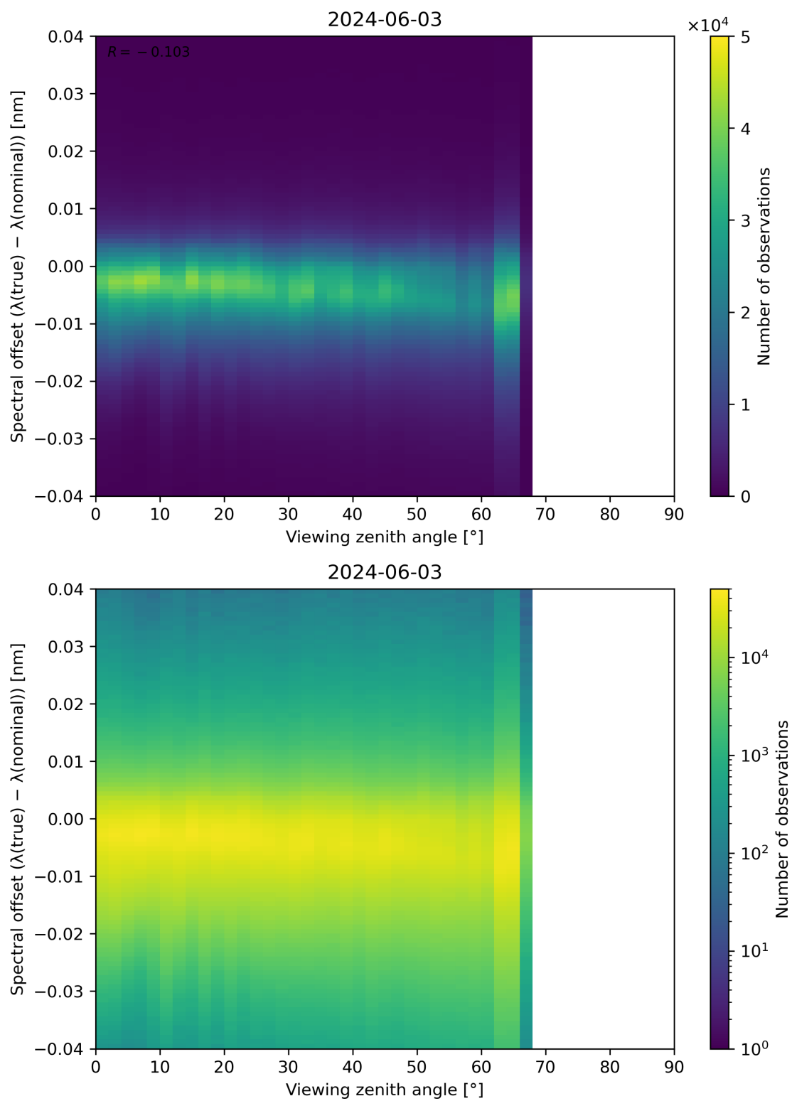
Figure 128: Scatter density plot of “Viewing zenith angle” against “Spectral offset ( \lambda(\text{true}) - \lambda(\text{nominal}) )” for 2024-06-03 to 2024-06-04.
