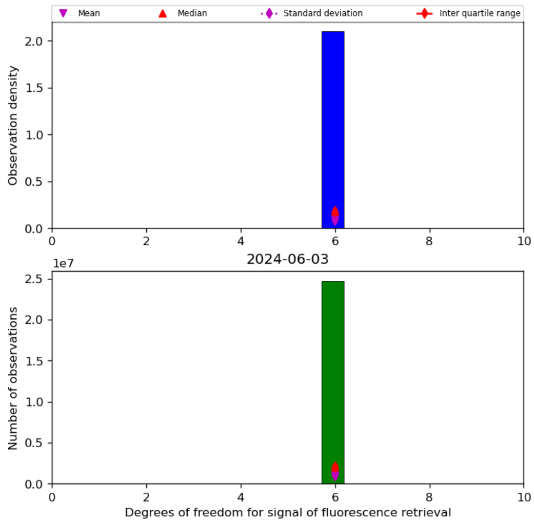
Figure 43: Histogram of “Degrees of freedom for signal of fluorescence retrieval” for 2024-06-03 to 2024-06-04
