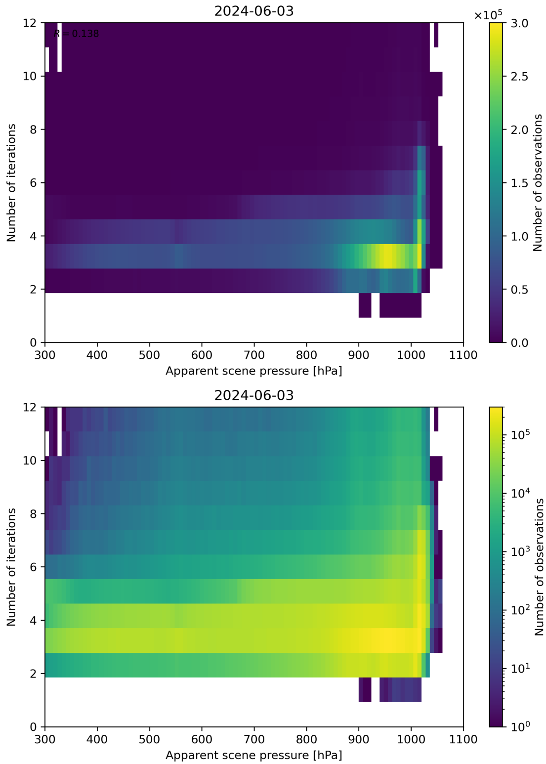
Figure 65: Scatter density plot of “Apparent scene pressure” against “Number of iterations” for 2024-06-03 to 2024-06-04.
