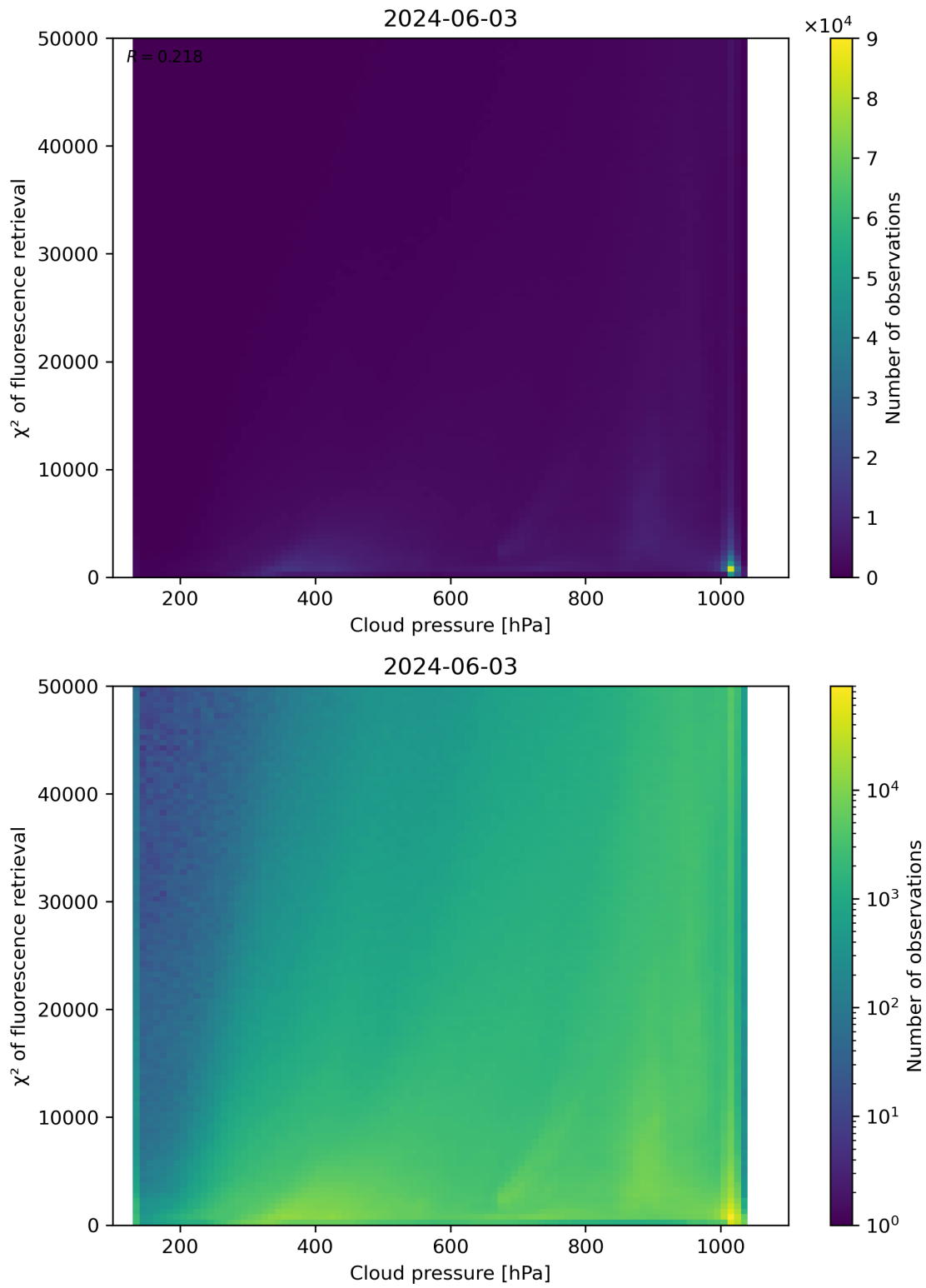
Figure 78: Scatter density plot of “Cloud pressure” against “ \chi^2 of fluorescence retrieval” for 2024-06-03 to 2024-06-04.
