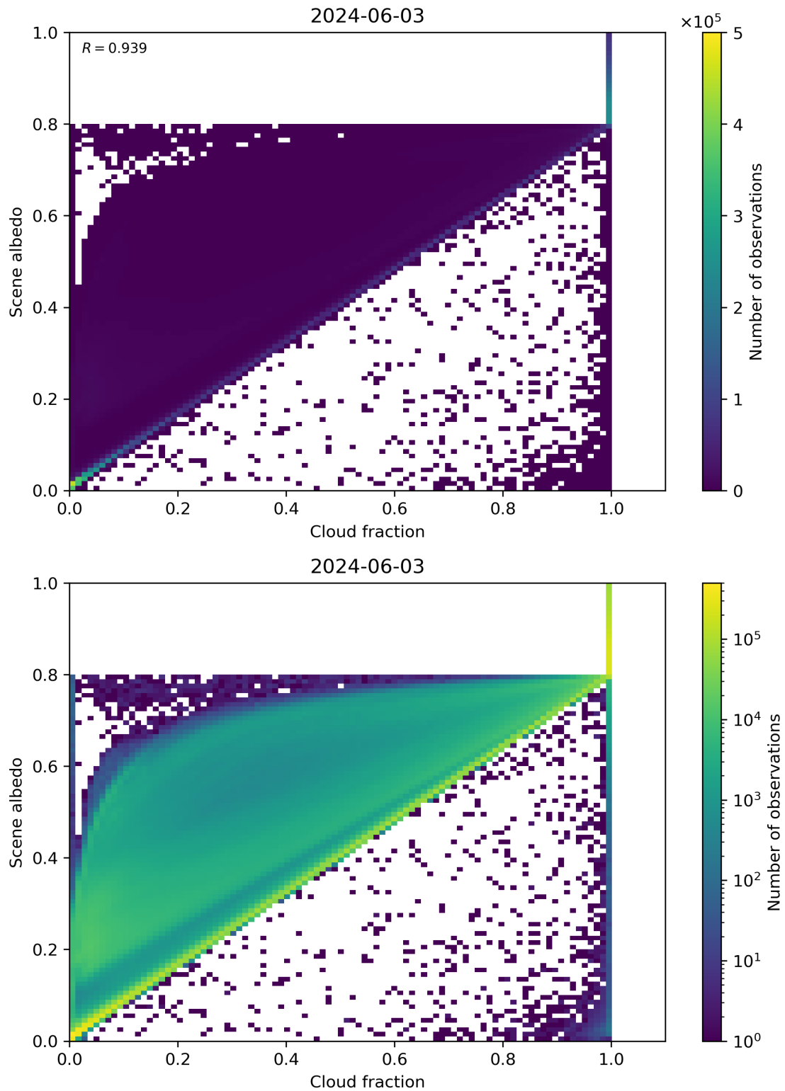
Figure 75: Scatter density plot of “Cloud fraction” against “Scene albedo” for 2024-06-03 to 2024-06-04.
