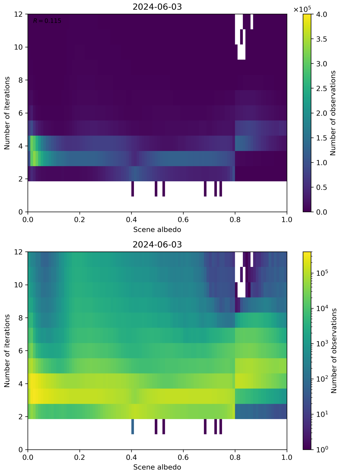
Figure 105: Scatter density plot of “Scene albedo” against “Number of iterations” for 2024-06-03 to 2024-06-04.
