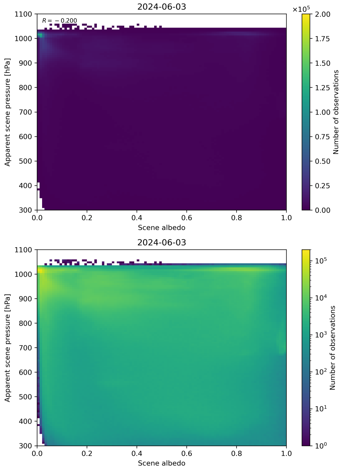
Figure 102: Scatter density plot of “Scene albedo” against “Apparent scene pressure” for 2024-06-03 to 2024-06-04.
