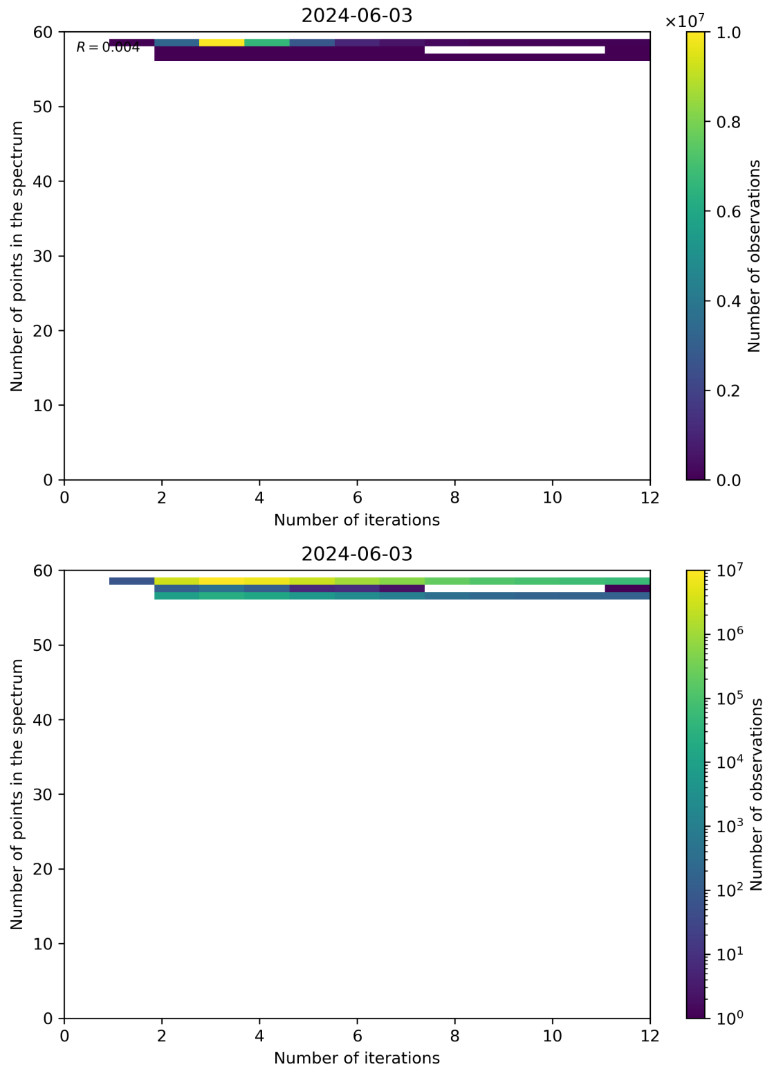
Figure 99: Scatter density plot of “Number of iterations” against “Number of points in the spectrum” for 2024-06-03 to 2024-06-04.
