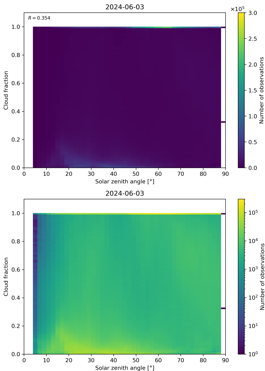
Figure 110: Scatter density plot of “Solar zenith angle” against “Cloud fraction” for 2024-06-03 to 2024-06-04.
