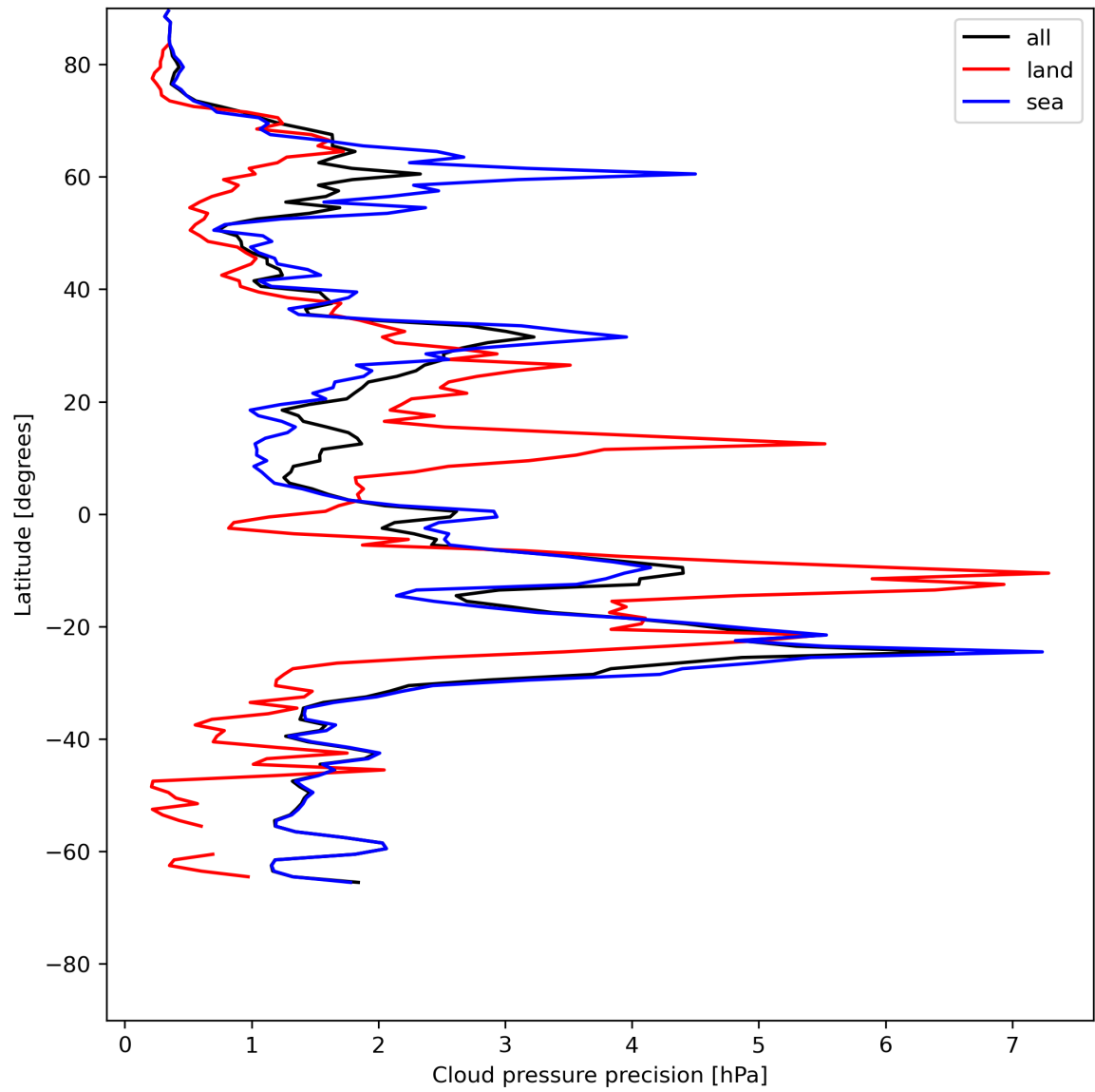
Figure 14: Zonal average of “Cloud pressure precision” for 2024-06-03 to 2024-06-04.
