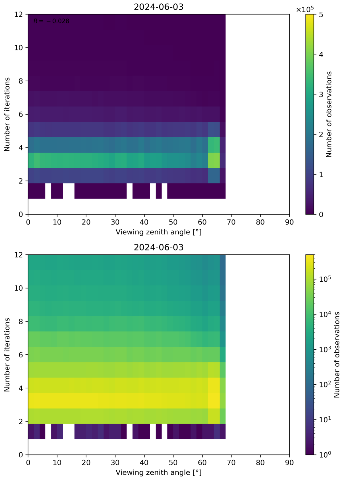
Figure 124: Scatter density plot of “Viewing zenith angle” against “Number of iterations” for 2024-06-03 to 2024-06-04.
