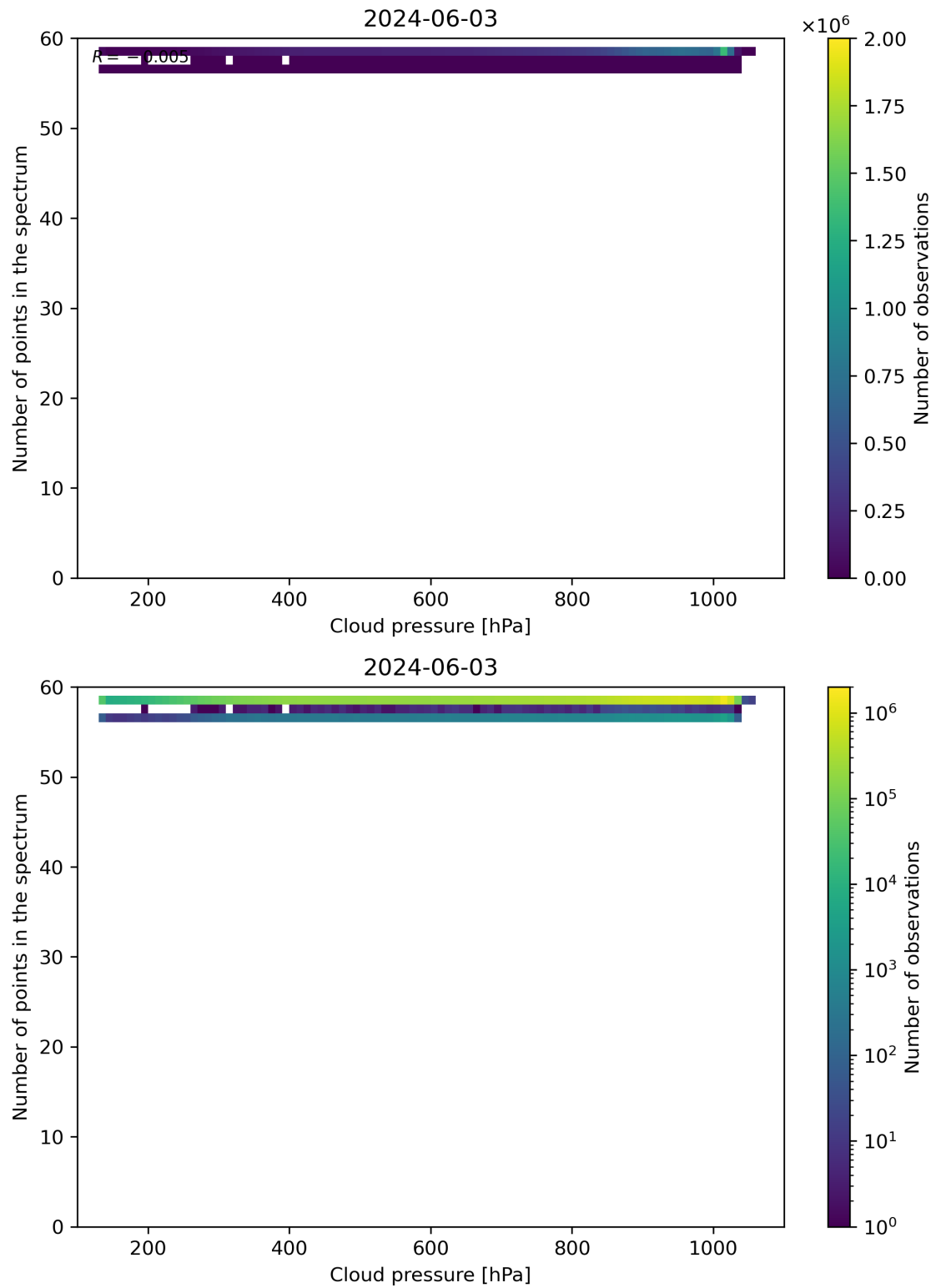
Figure 82: Scatter density plot of “Cloud pressure” against “Number of points in the spectrum” for 2024-06-03 to 2024-06-04.
