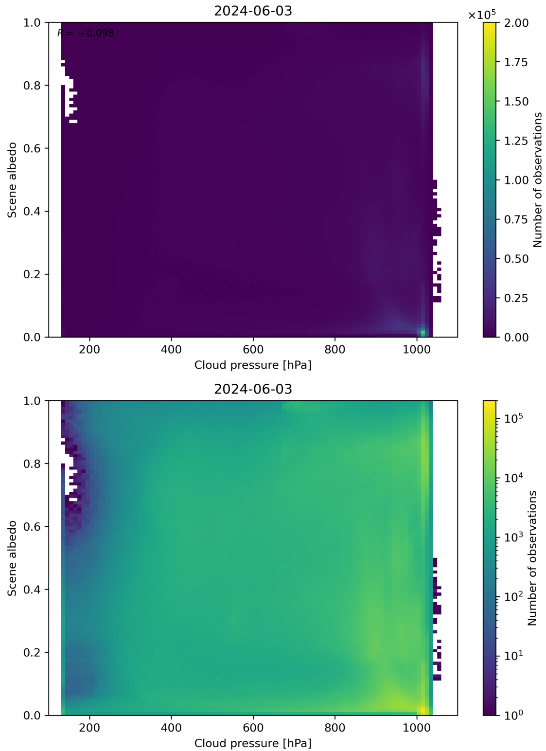
Figure 83: Scatter density plot of “Cloud pressure” against “Scene albedo” for 2024-06-03 to 2024-06-04.
