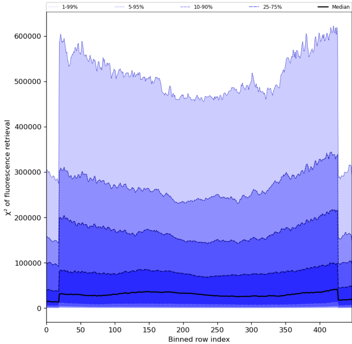
Figure 59: Along track statistics of " \chi^2 of fluorescence retrieval" for 2024-06-03 to 2024-06-04
