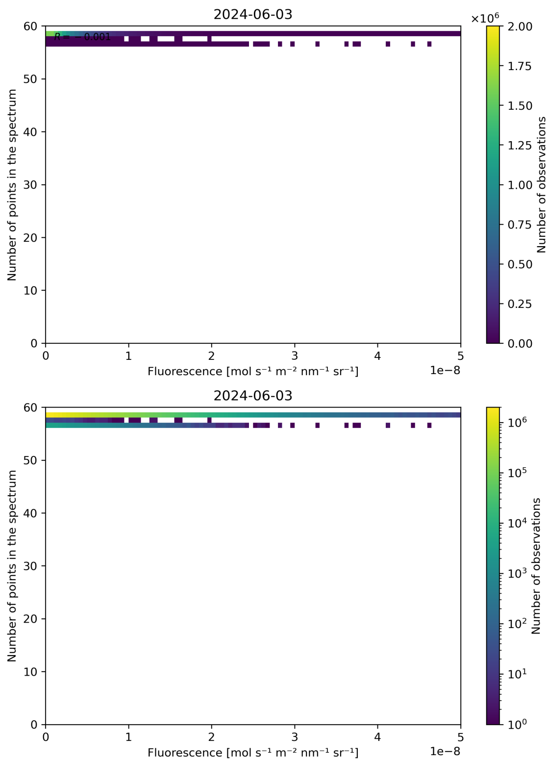
Figure 86: Scatter density plot of “Fluorescence” against “Number of points in the spectrum” for 2024-06-03 to 2024-06-04.
