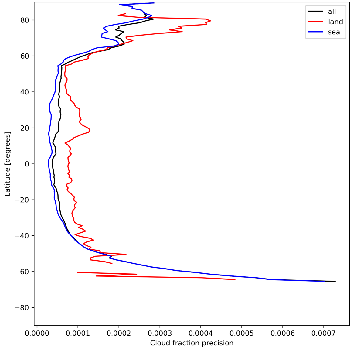
Figure 16: Zonal average of “Cloud fraction precision” for 2024-06-03 to 2024-06-04.
