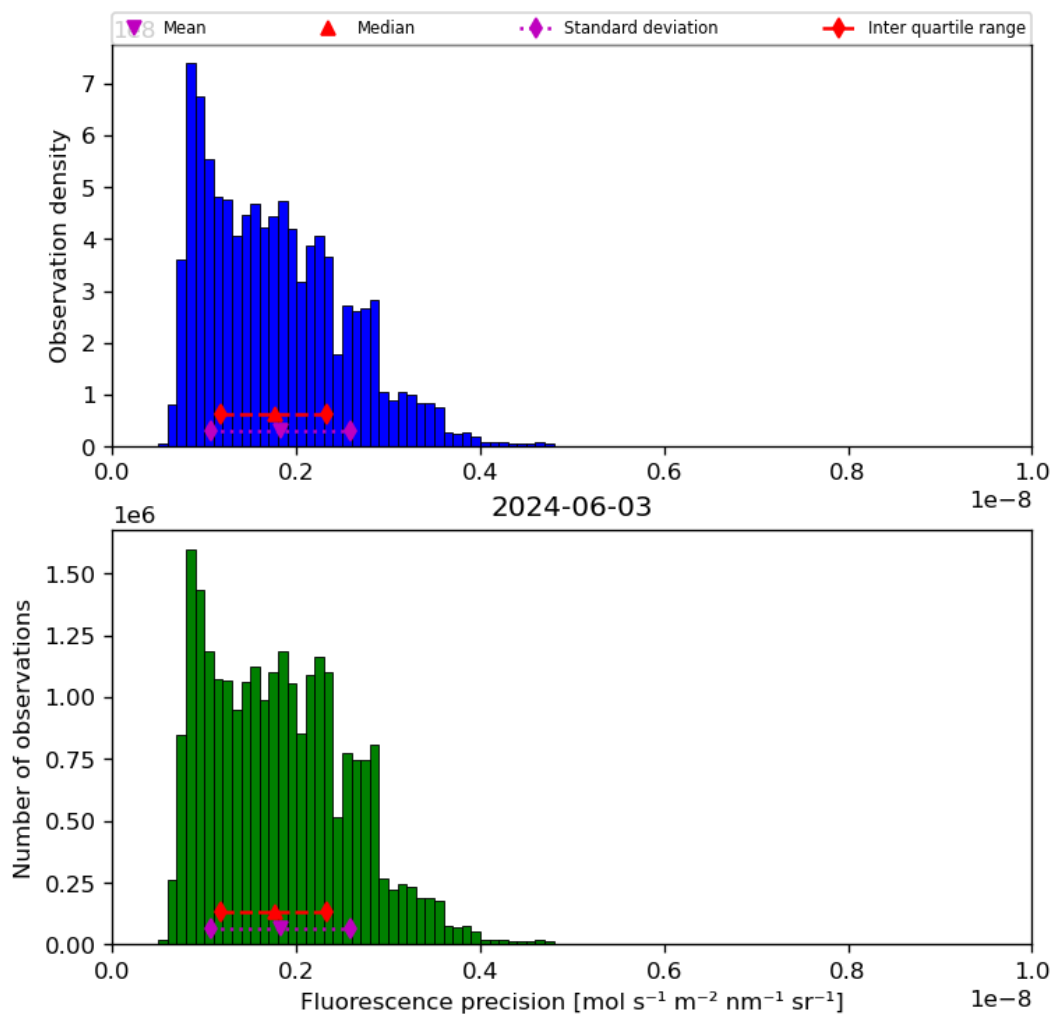
Figure 41: Histogram of “Fluorescence precision” for 2024-06-03 to 2024-06-04
