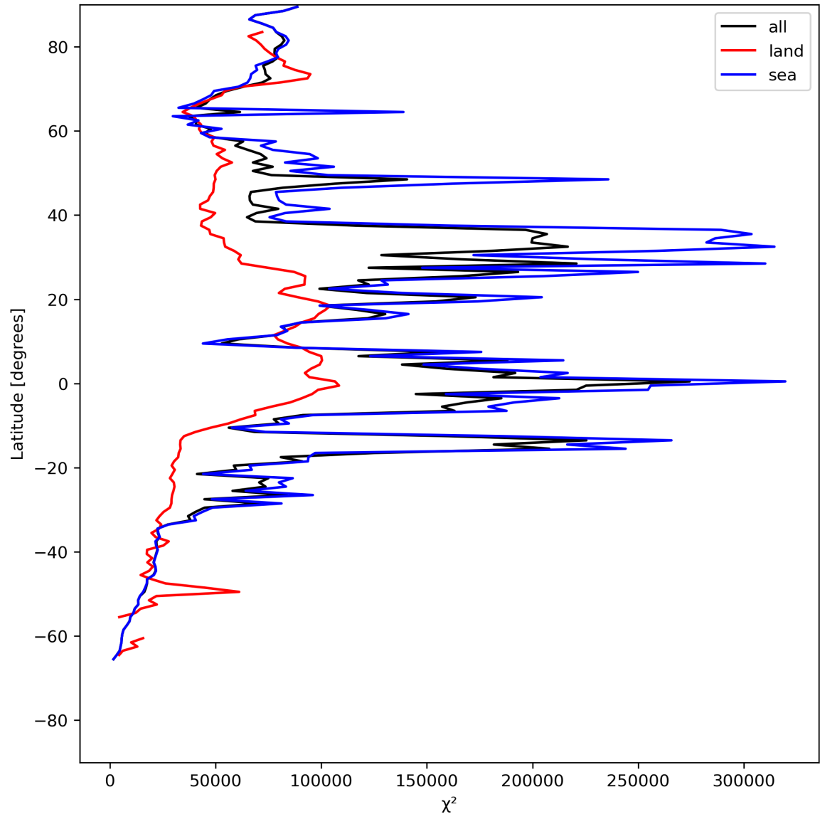
Figure 21: Zonal average of “ \chi^2 ” for 2024-06-03 to 2024-06-04.
