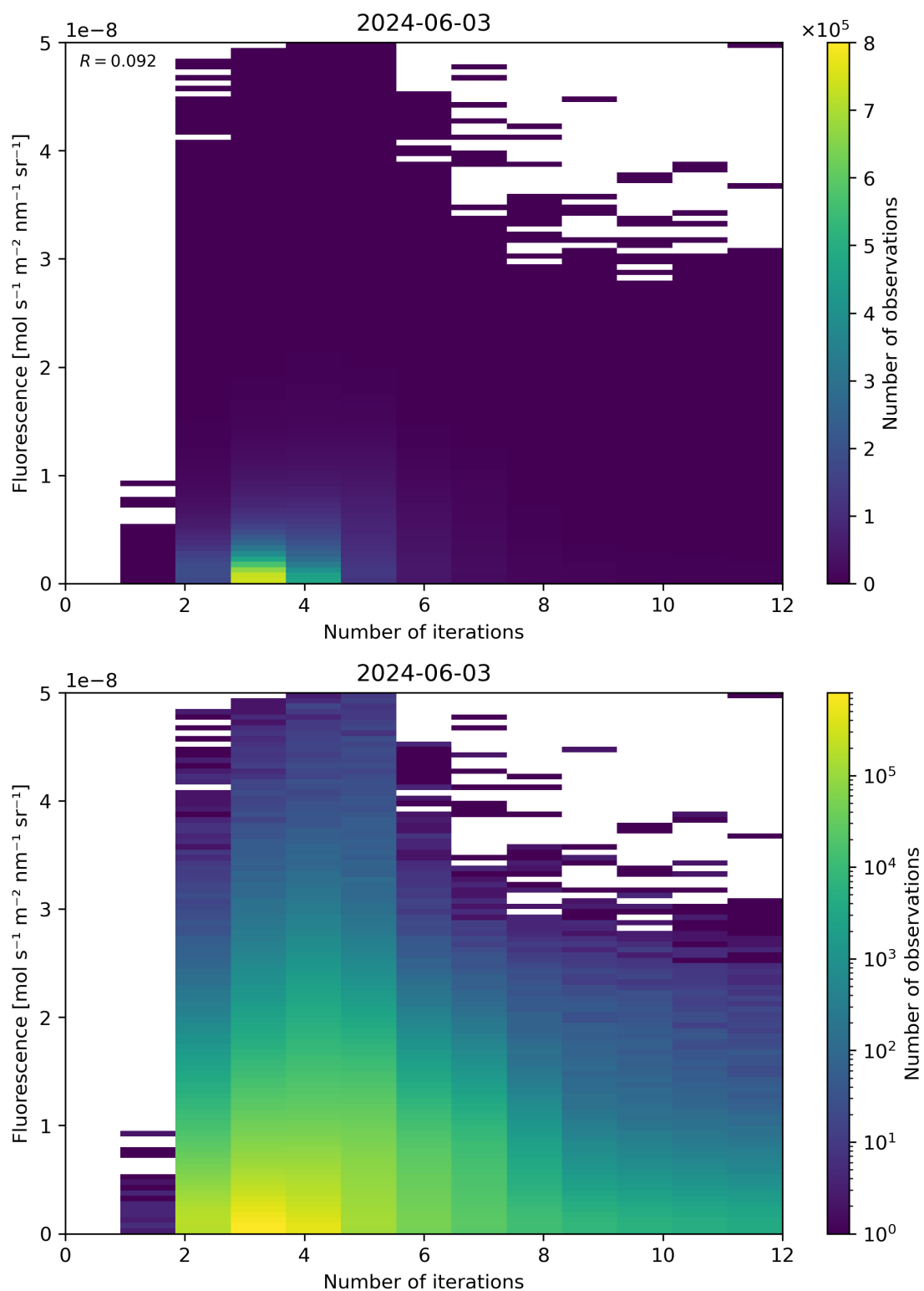
Figure 98: Scatter density plot of “Number of iterations” against “Fluorescence” for 2024-06-03 to 2024-06-04.
