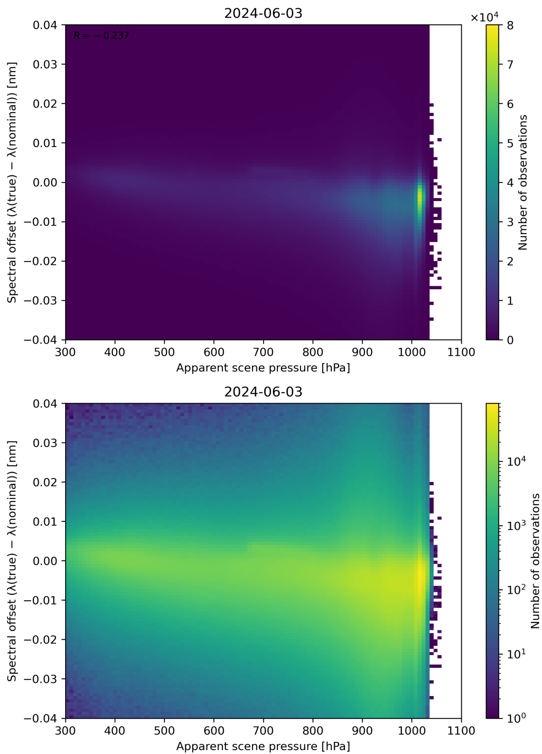
Figure 67: Scatter density plot of “Apparent scene pressure” against “Spectral offset ( \lambda(\text{true}) - \lambda(\text{nominal}) )” for 2024-06-03 to 2024-06-04.
