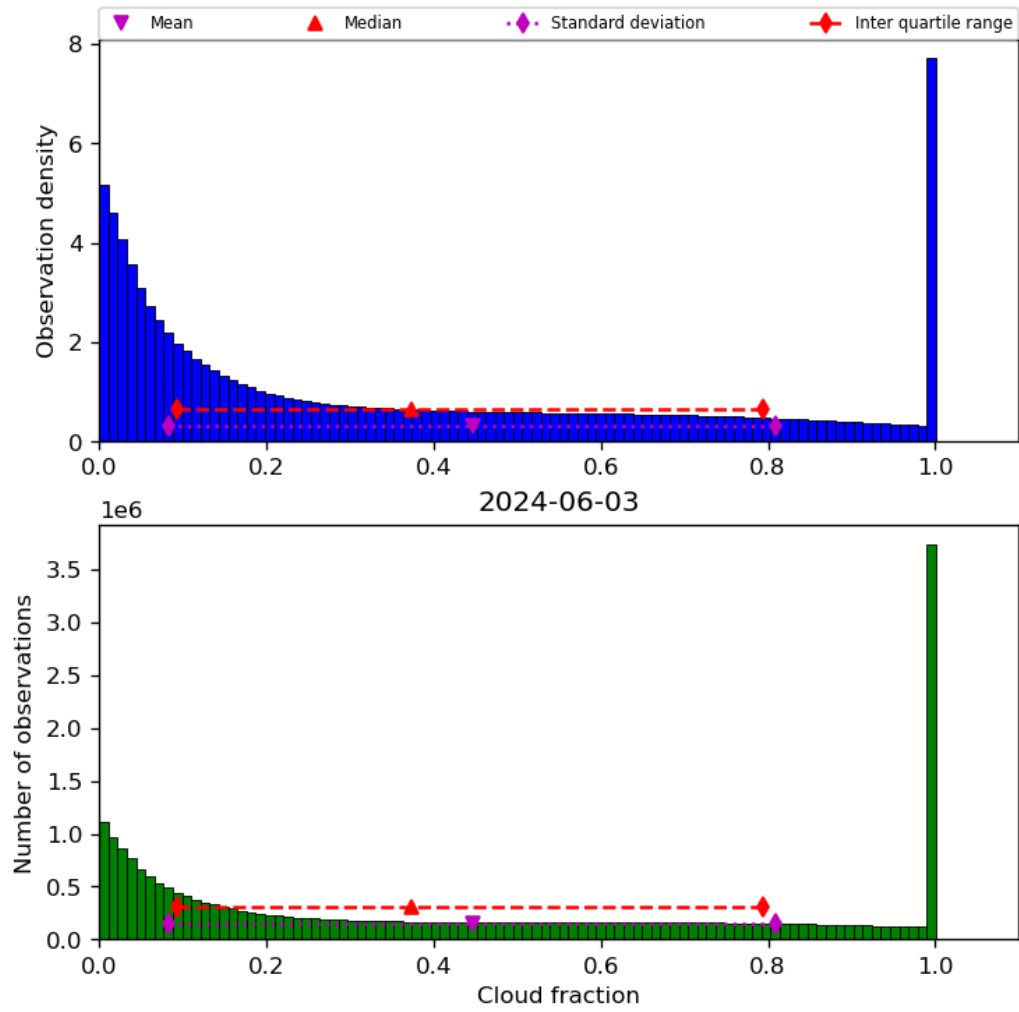
Figure 32: Histogram of “Cloud fraction” for 2024-06-03 to 2024-06-04
