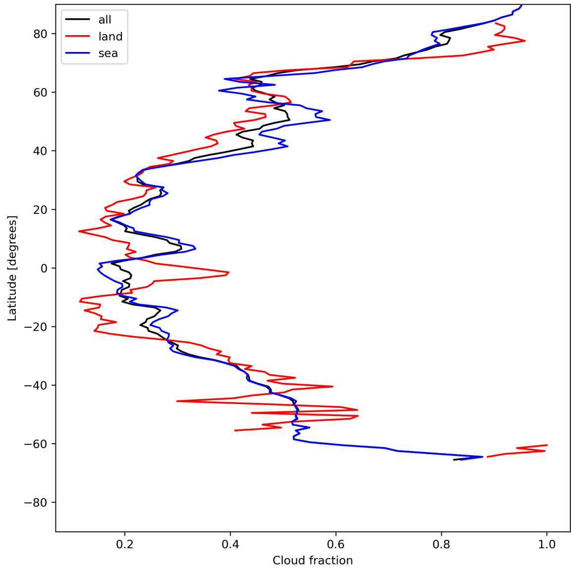
Figure 15: Zonal average of “Cloud fraction” for 2024-06-03 to 2024-06-04.
