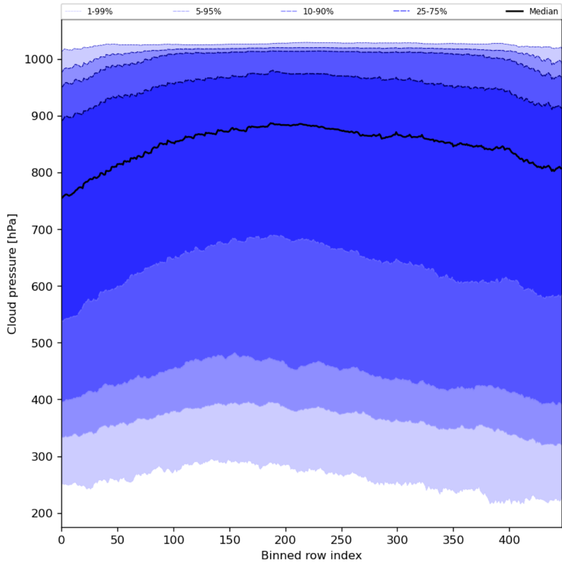
Figure 47: Along track statistics of “Cloud pressure” for 2024-06-03 to 2024-06-04
