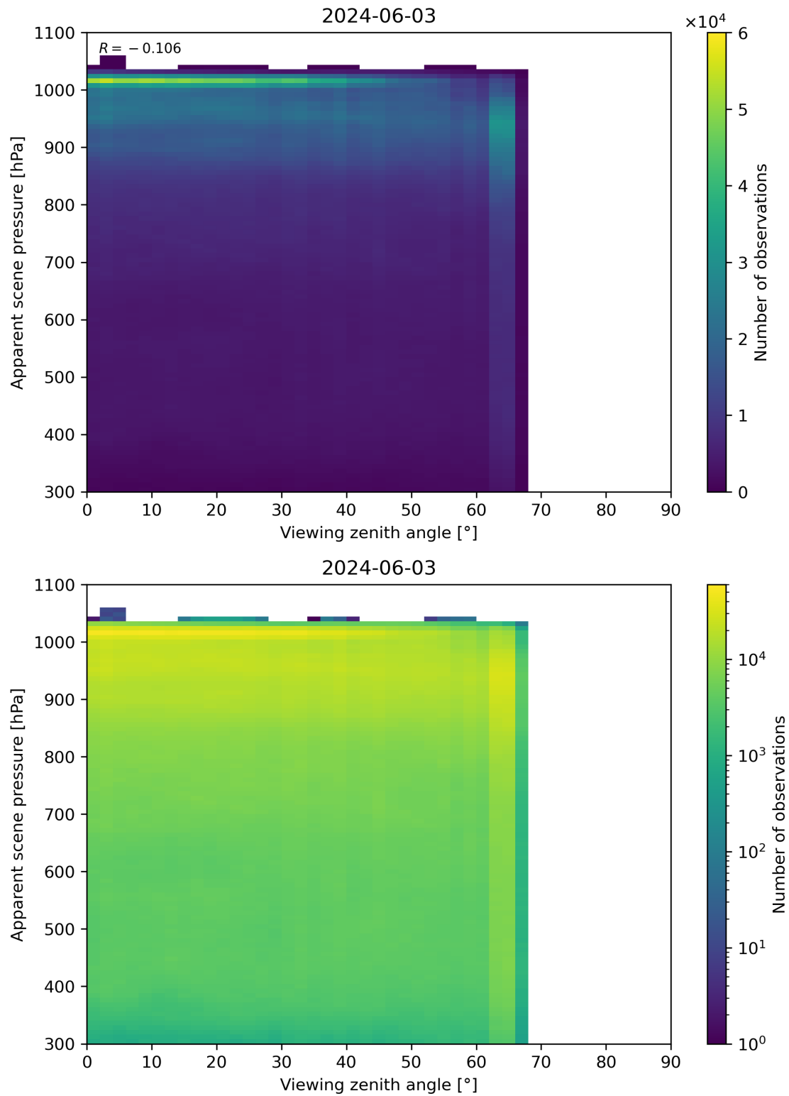
Figure 118: Scatter density plot of “Viewing zenith angle” against “Apparent scene pressure” for 2024-06-03 to 2024-06-04.
