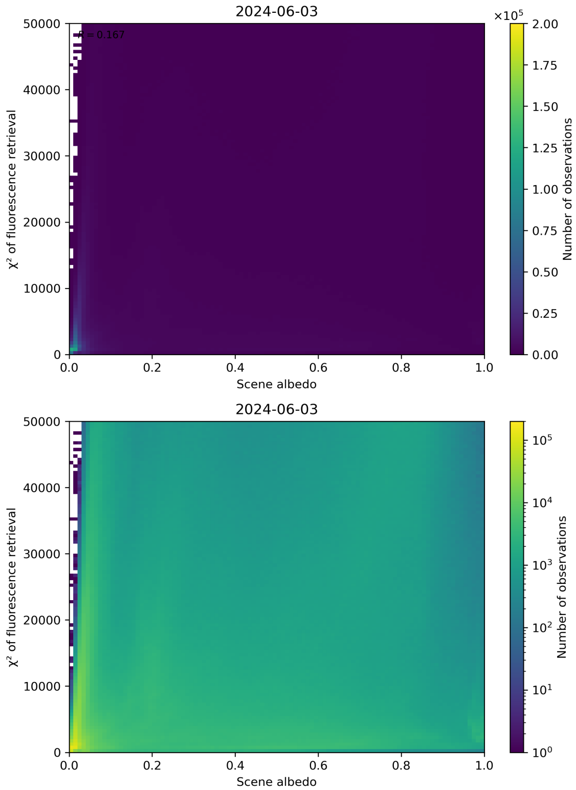
Figure 103: Scatter density plot of “Scene albedo” against “ \chi^2 of fluorescence retrieval” for 2024-06-03 to 2024-06-04.
