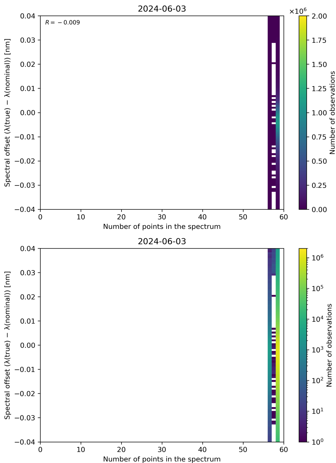
Figure 101: Scatter density plot of “Number of points in the spectrum” against “Spectral offset ( \lambda(\text{true}) - \lambda(\text{nominal}) )” for 2024-06-03 to 2024-06-04.
