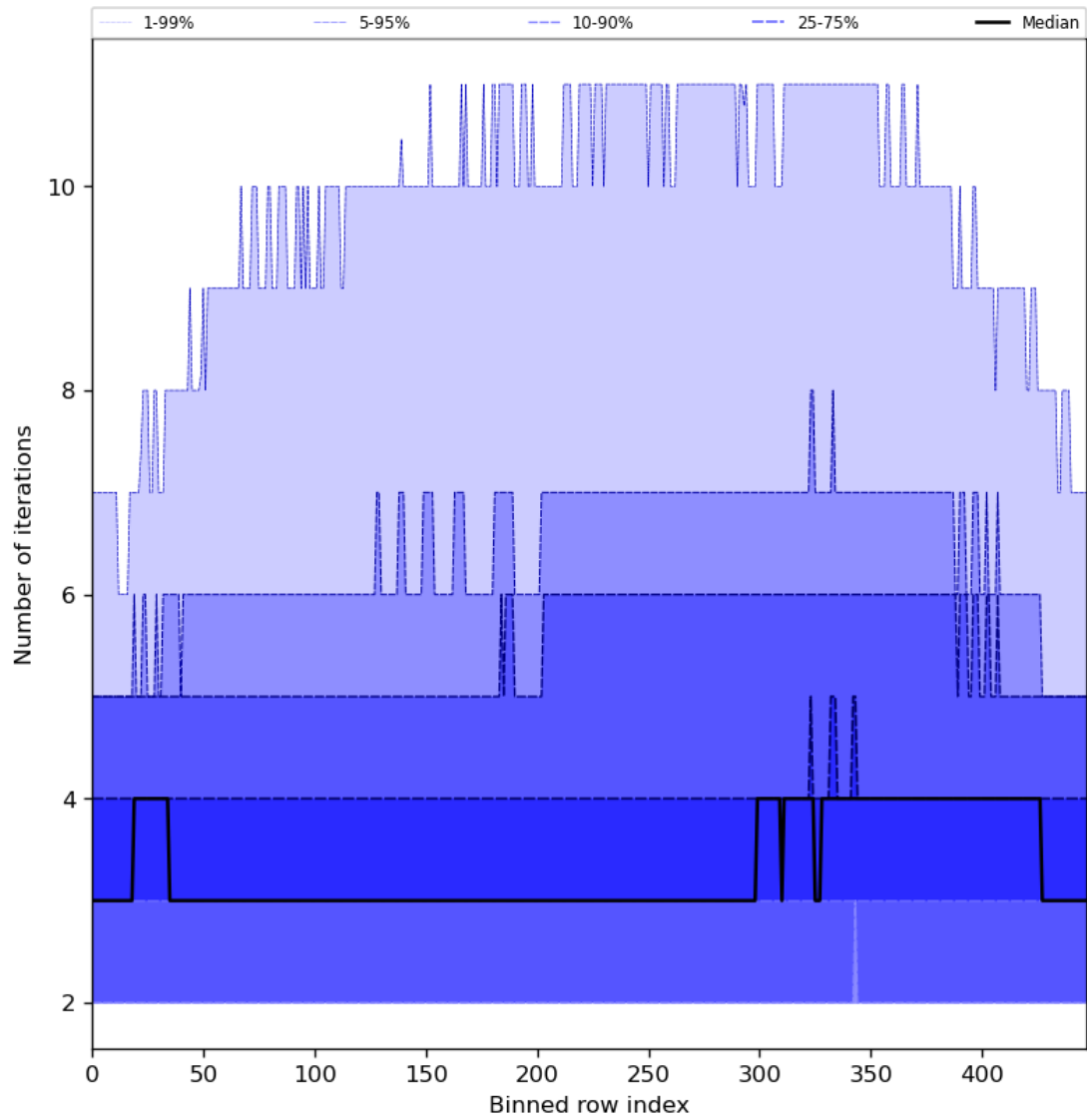
Figure 56: Along track statistics of “Number of iterations” for 2024-06-03 to 2024-06-05
