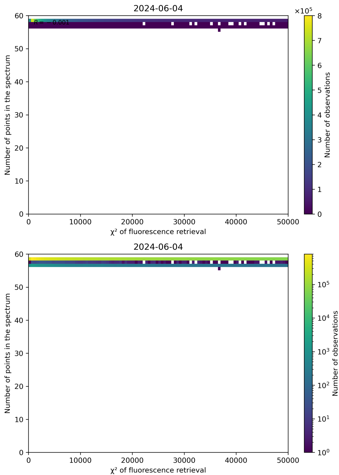
Figure 68: Scatter density plot of " \chi^2 of fluorescence retrieval" against "Number of points in the spectrum" for 2024-06-03 to 2024-06-05.
