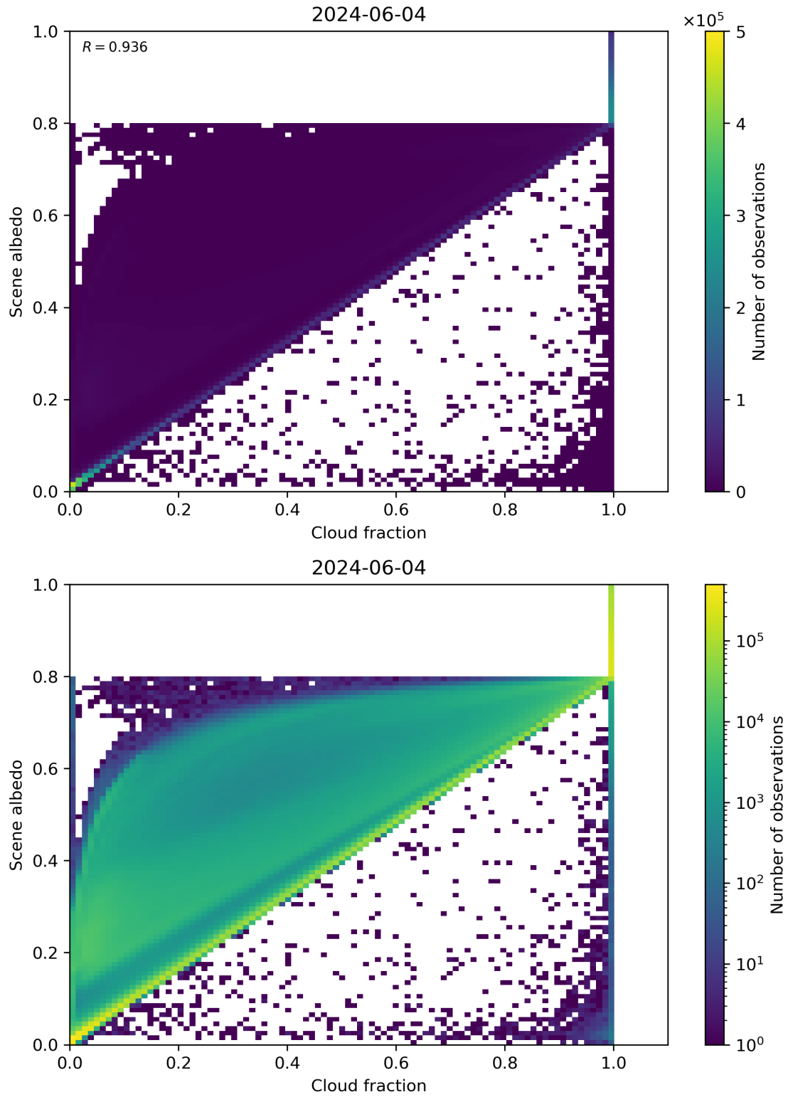
Figure 75: Scatter density plot of “Cloud fraction” against “Scene albedo” for 2024-06-03 to 2024-06-05.
