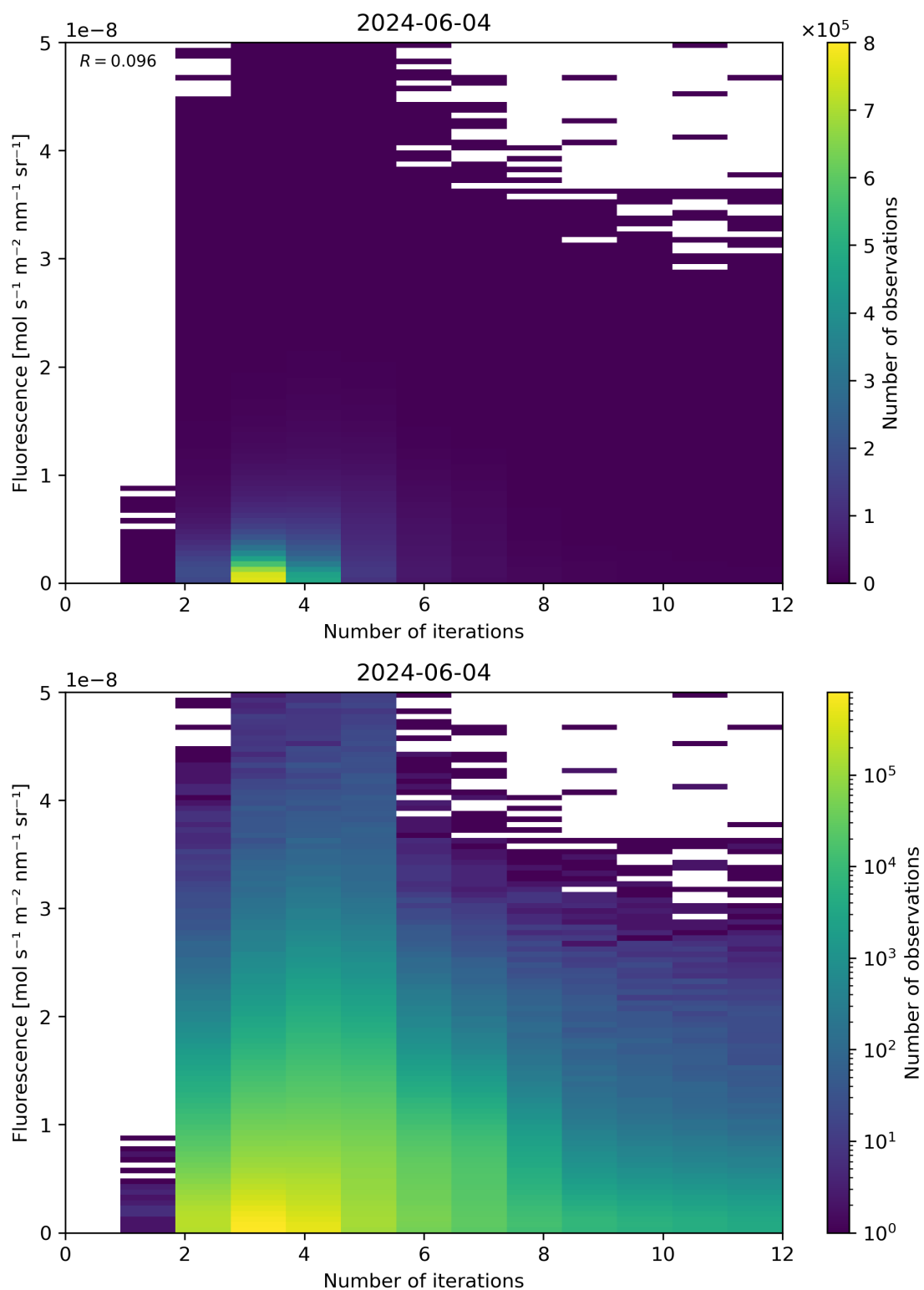
Figure 98: Scatter density plot of “Number of iterations” against “Fluorescence” for 2024-06-03 to 2024-06-05.
