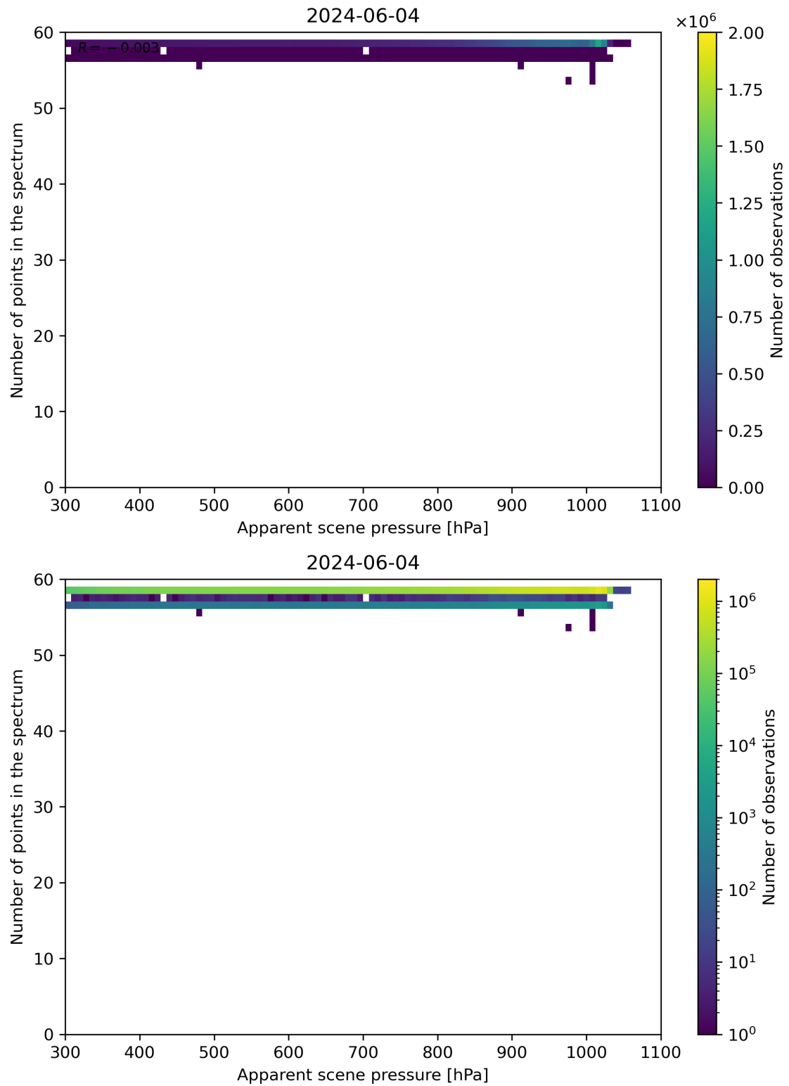
Figure 66: Scatter density plot of “Apparent scene pressure” against “Number of points in the spectrum” for 2024-06-03 to 2024-06-05.
