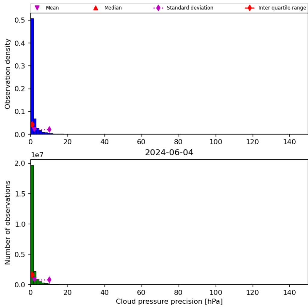
Figure 31: Histogram of “Cloud pressure precision” for 2024-06-03 to 2024-06-05
