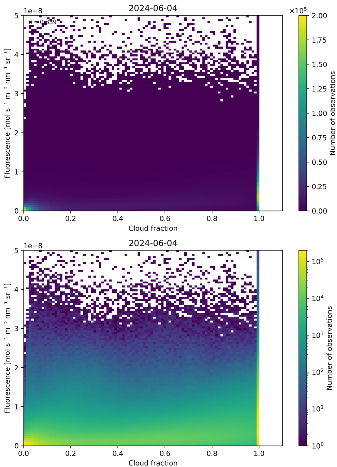
Figure 72: Scatter density plot of “Cloud fraction” against “Fluorescence” for 2024-06-03 to 2024-06-05.
