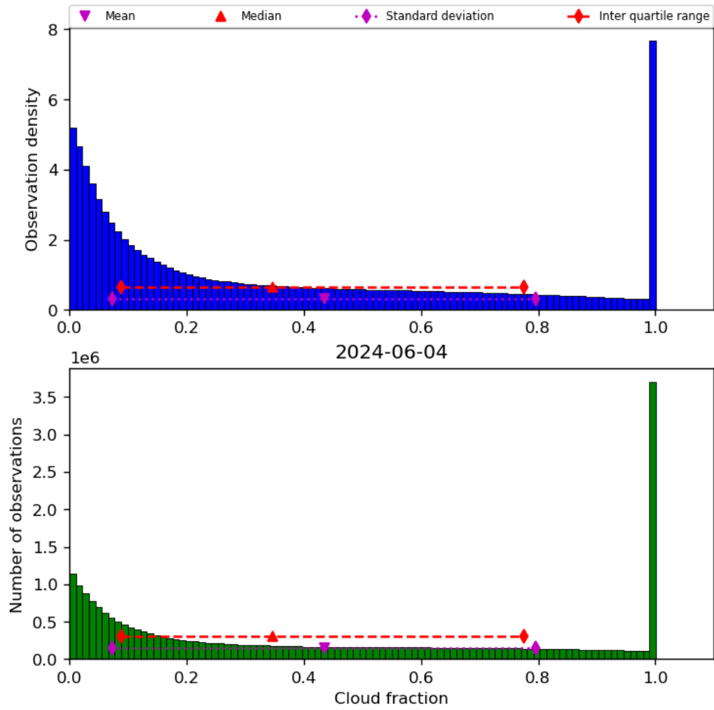
Figure 32: Histogram of “Cloud fraction” for 2024-06-03 to 2024-06-05
