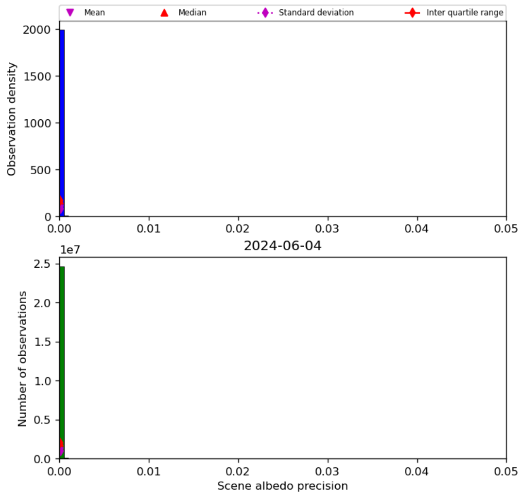
Figure 35: Histogram of “Scene albedo precision” for 2024-06-03 to 2024-06-05
