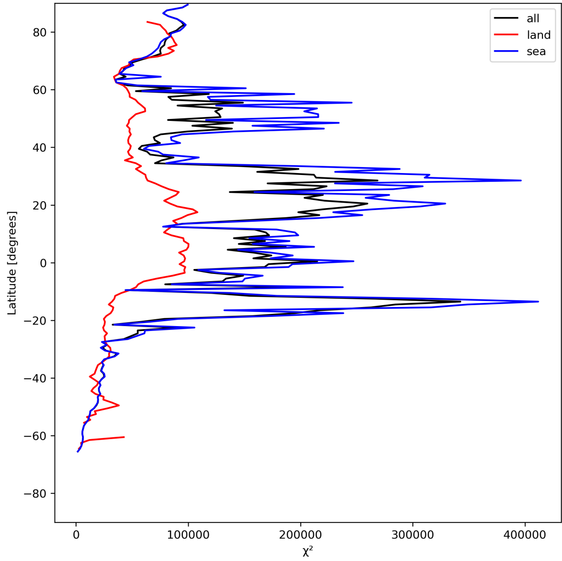
Figure 21: Zonal average of “ \chi^2 ” for 2024-06-03 to 2024-06-05.
