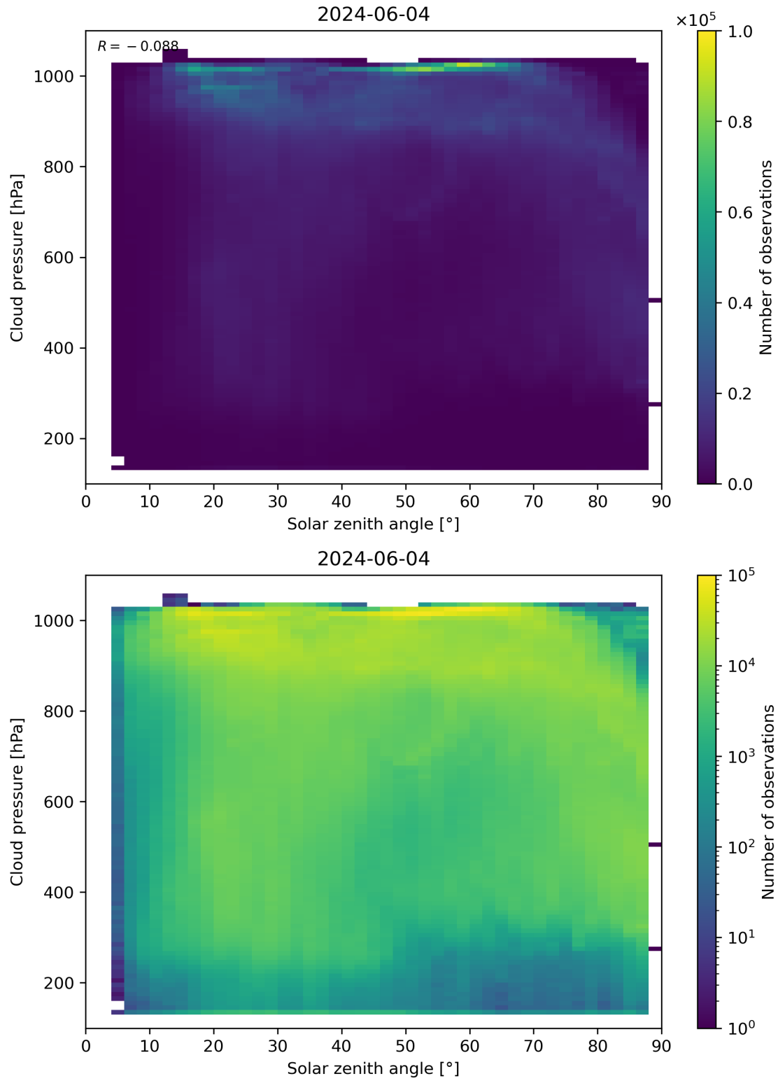
Figure 111: Scatter density plot of “Solar zenith angle” against “Cloud pressure” for 2024-06-03 to 2024-06-05.
