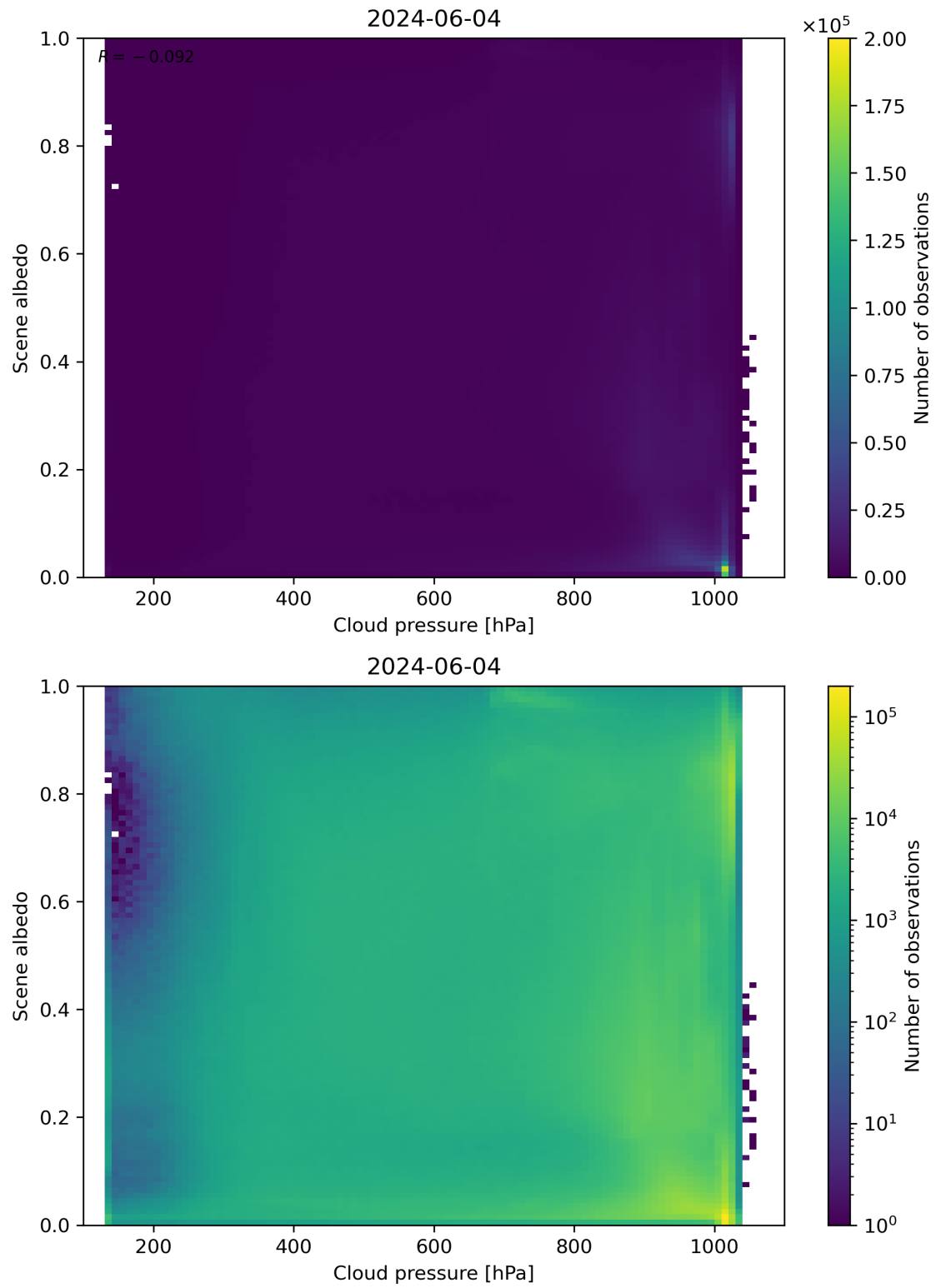
Figure 83: Scatter density plot of “Cloud pressure” against “Scene albedo” for 2024-06-03 to 2024-06-05.
