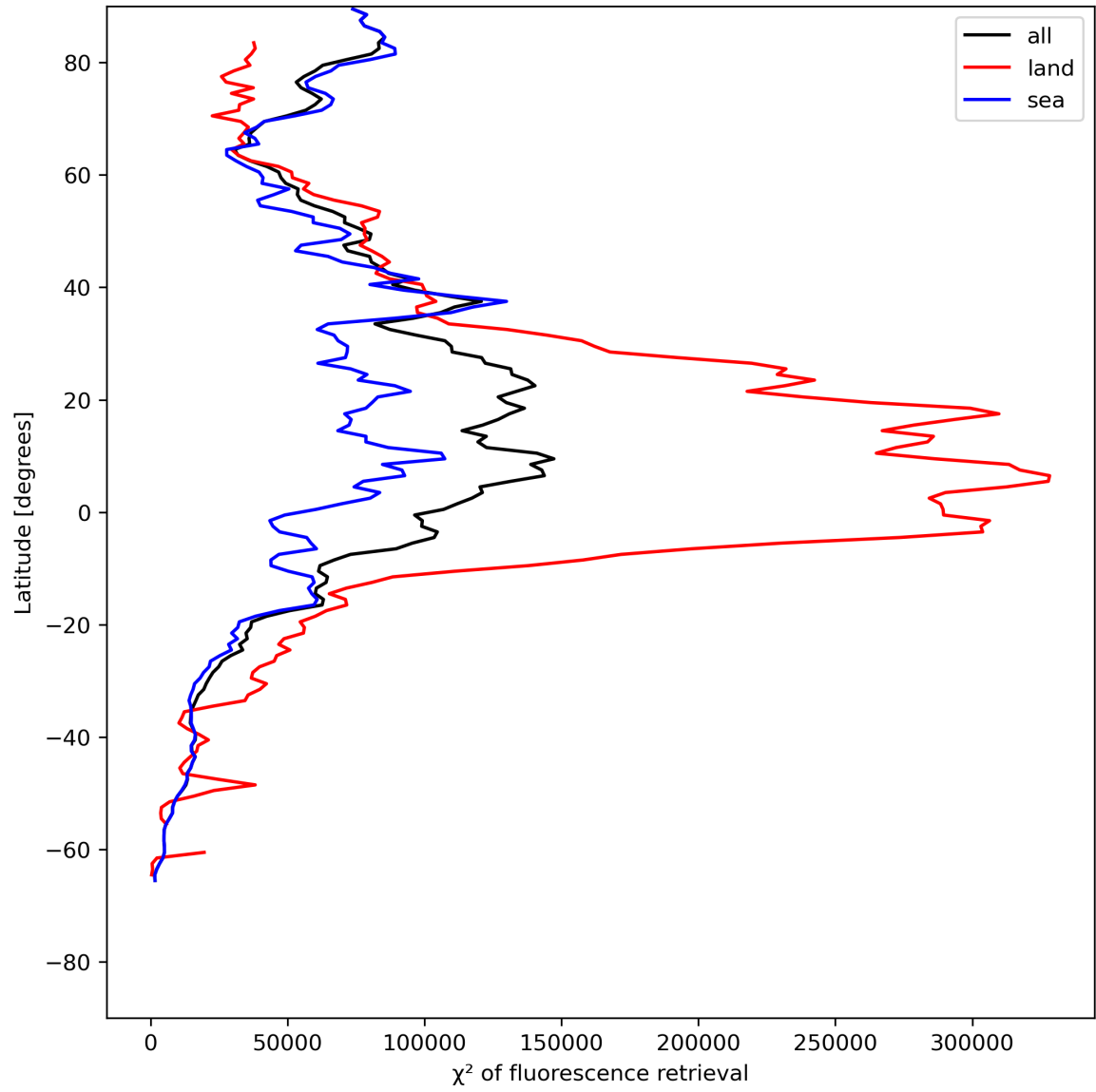
Figure 25: Zonal average of “ \chi^2 of fluorescence retrieval” for 2024-06-03 to 2024-06-05.
