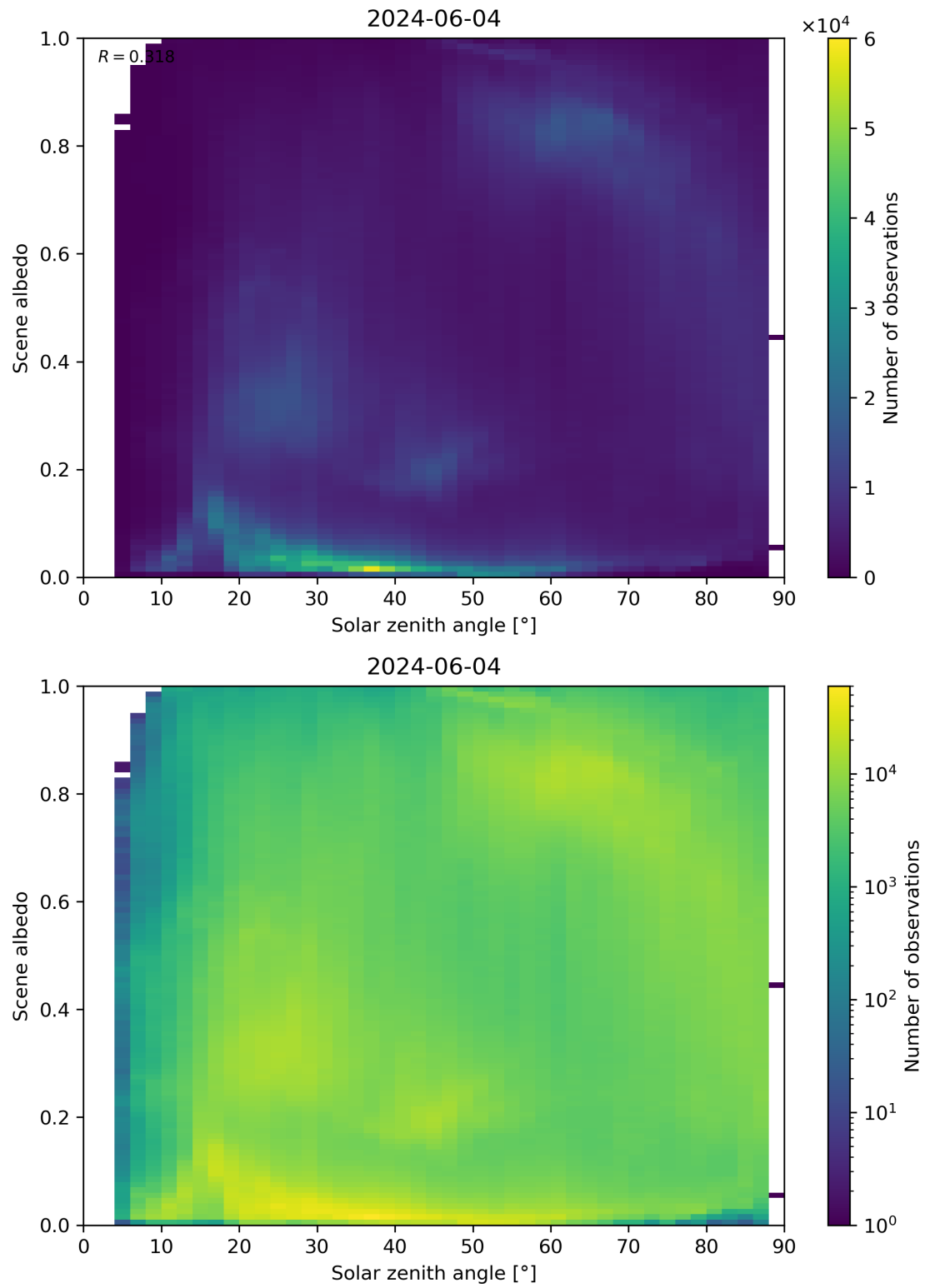
Figure 116: Scatter density plot of “Solar zenith angle” against “Scene albedo” for 2024-06-03 to 2024-06-05.
