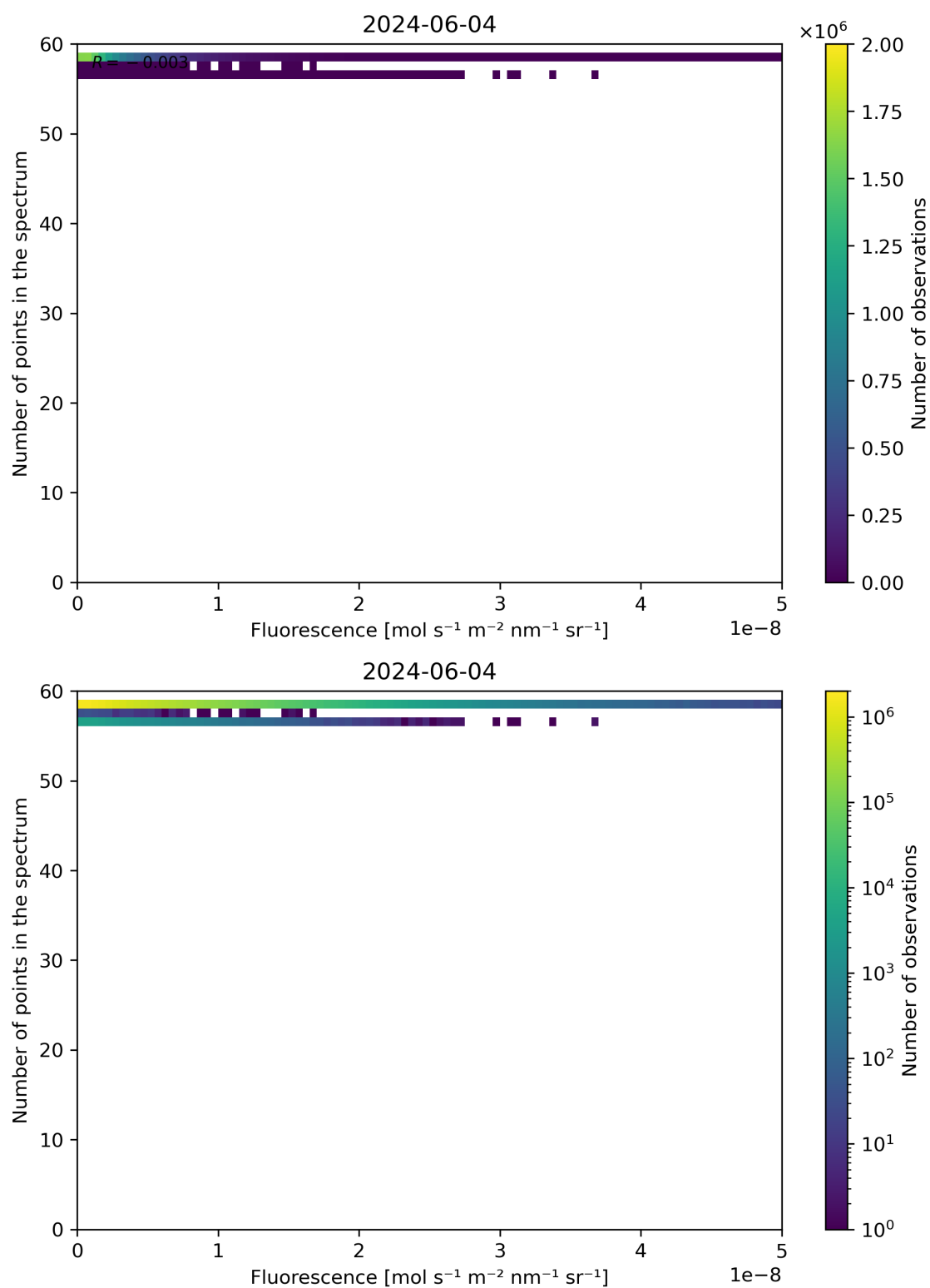
Figure 86: Scatter density plot of “Fluorescence” against “Number of points in the spectrum” for 2024-06-03 to 2024-06-05.
