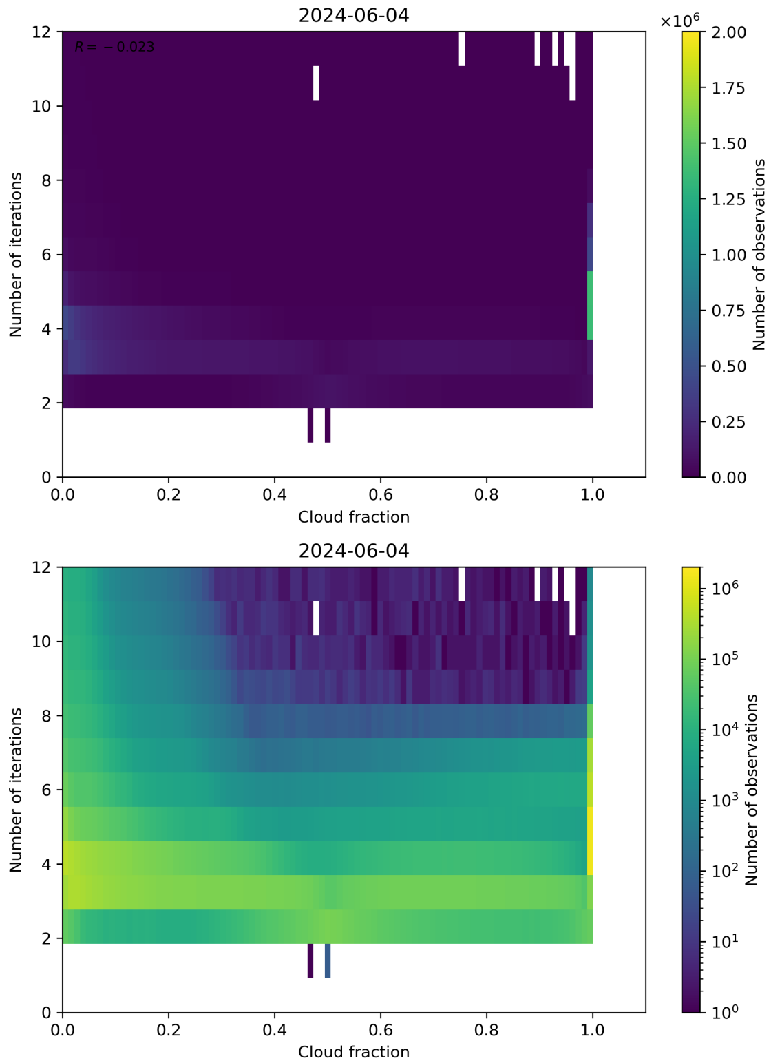
Figure 73: Scatter density plot of “Cloud fraction” against “Number of iterations” for 2024-06-03 to 2024-06-05.
