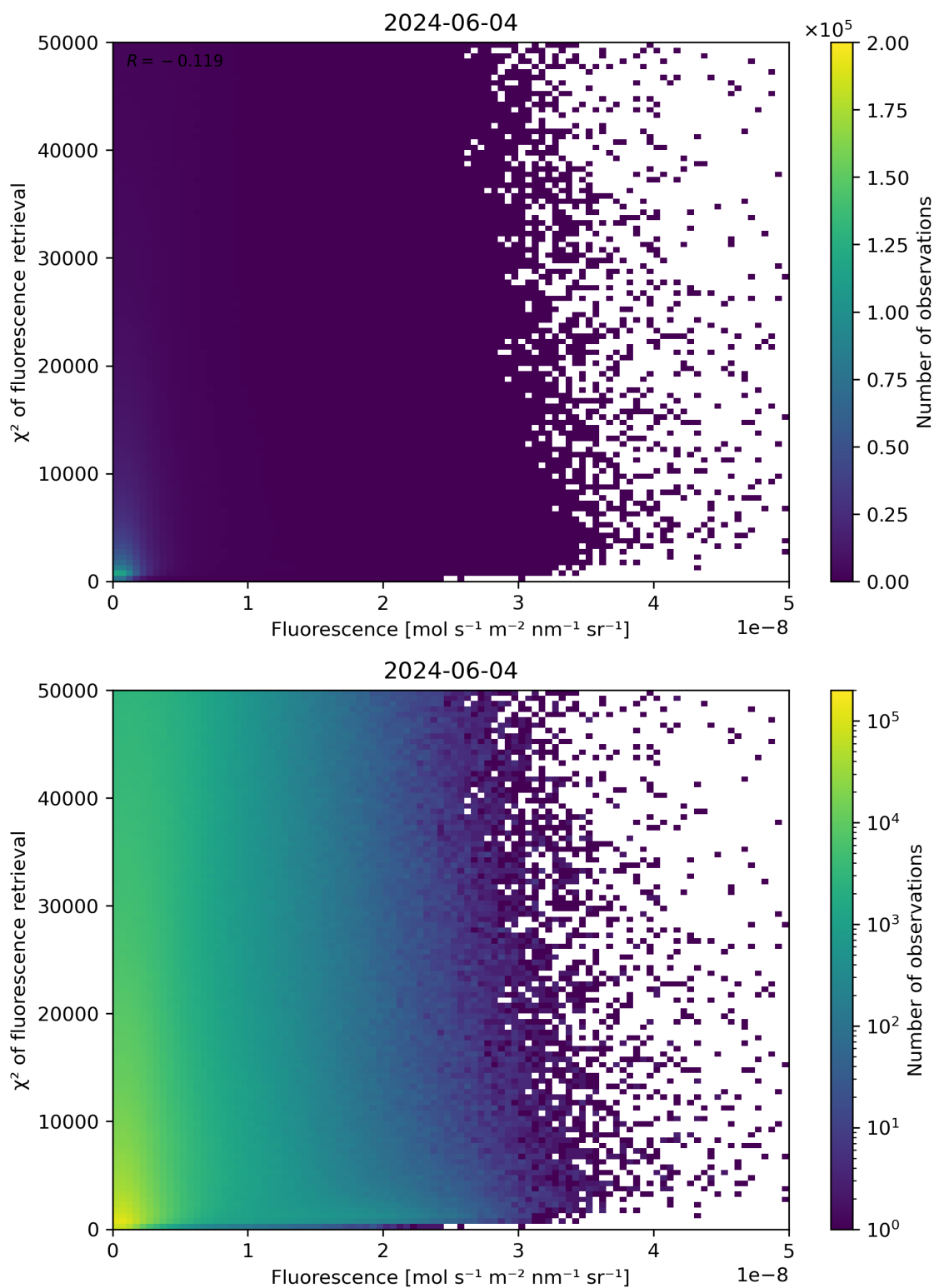
Figure 85: Scatter density plot of “Fluorescence” against “ \chi^2 of fluorescence retrieval” for 2024-06-03 to 2024-06-05.
