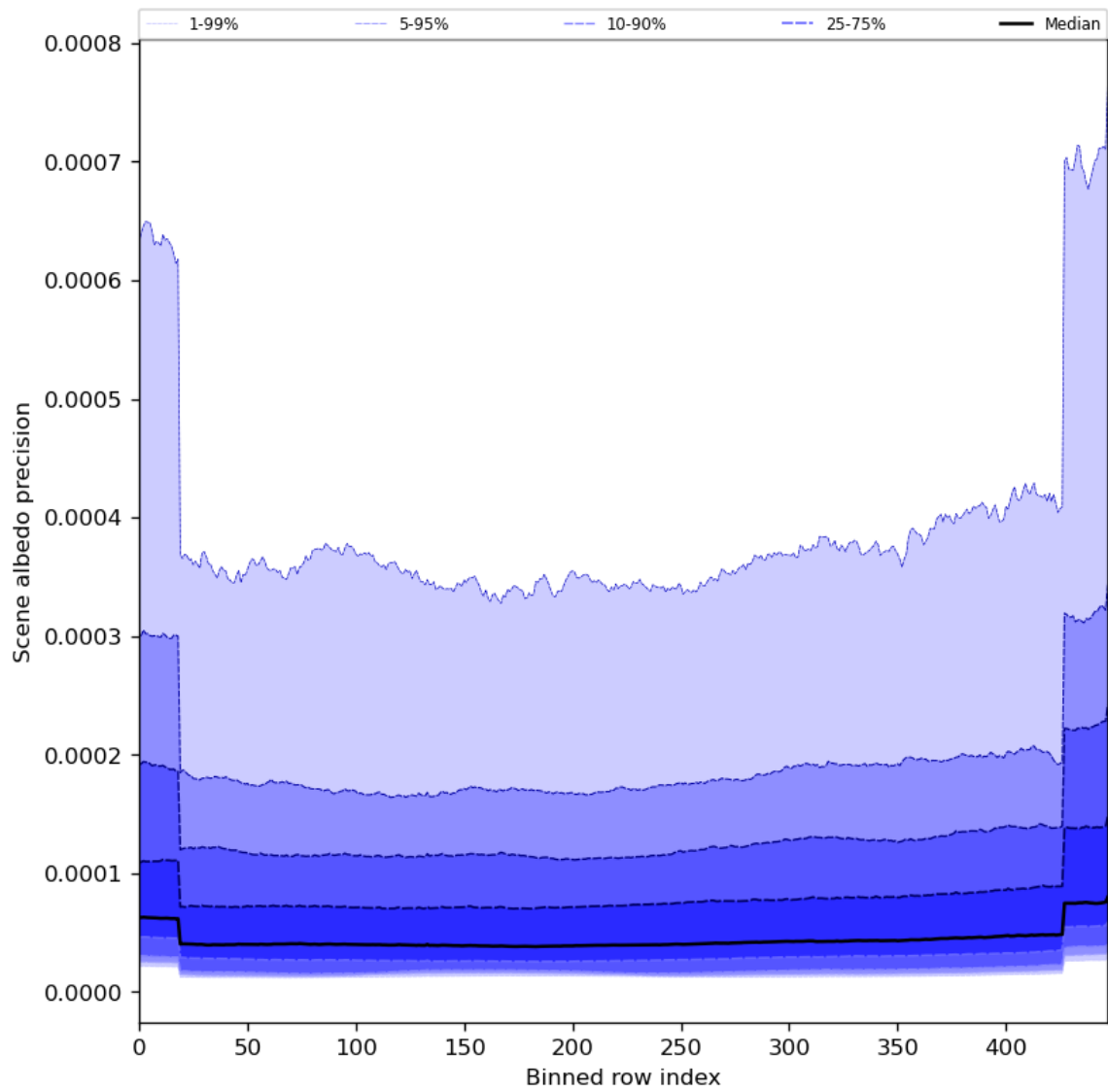
Figure 52: Along track statistics of “Scene albedo precision” for 2024-06-03 to 2024-06-05
