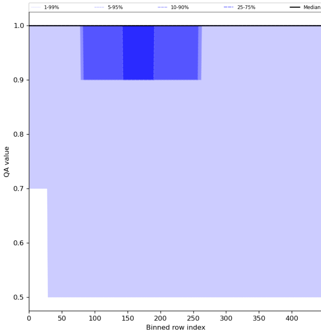
Figure 46: Along track statistics of “QA value” for 2024-06-03 to 2024-06-05
