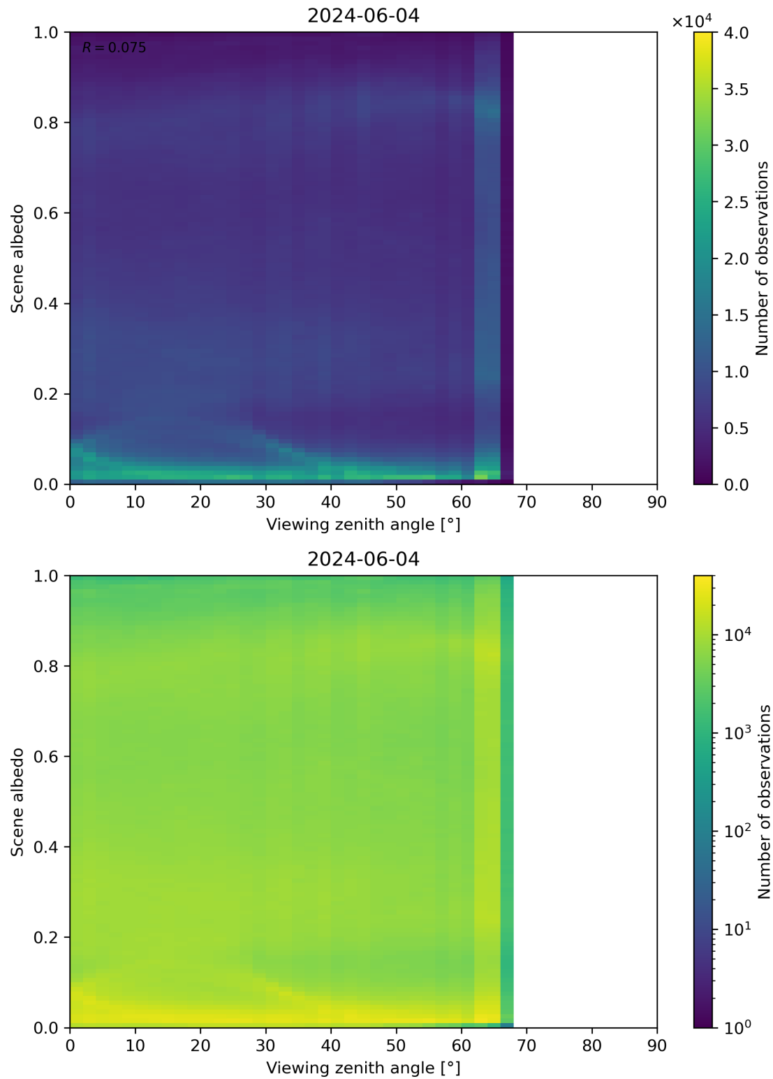
Figure 126: Scatter density plot of “Viewing zenith angle” against “Scene albedo” for 2024-06-03 to 2024-06-05.
