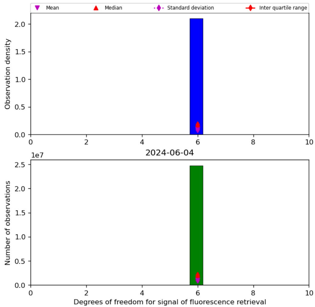
Figure 43: Histogram of “Degrees of freedom for signal of fluorescence retrieval” for 2024-06-03 to 2024-06-05
