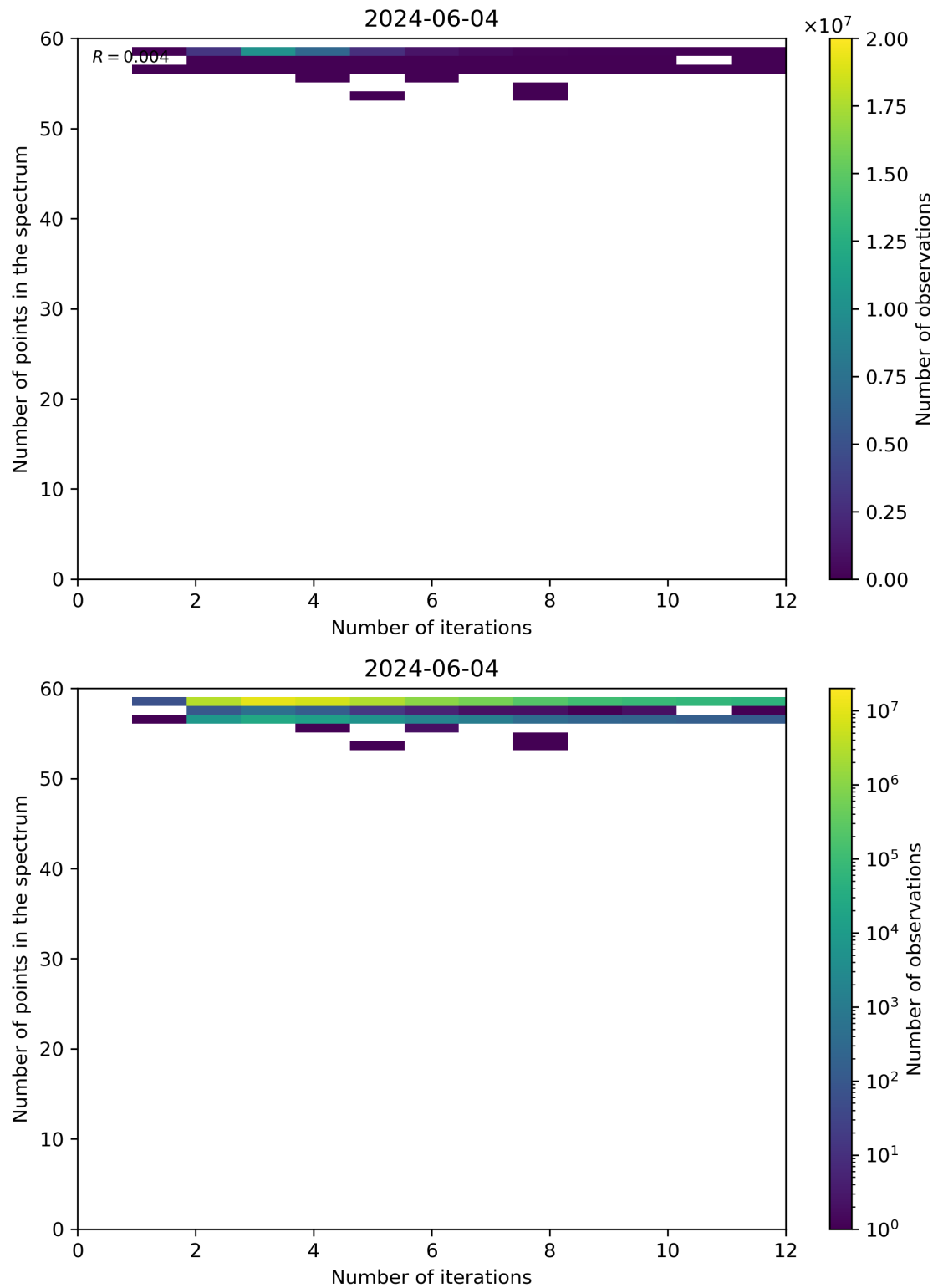
Figure 99: Scatter density plot of “Number of iterations” against “Number of points in the spectrum” for 2024-06-03 to 2024-06-05.
