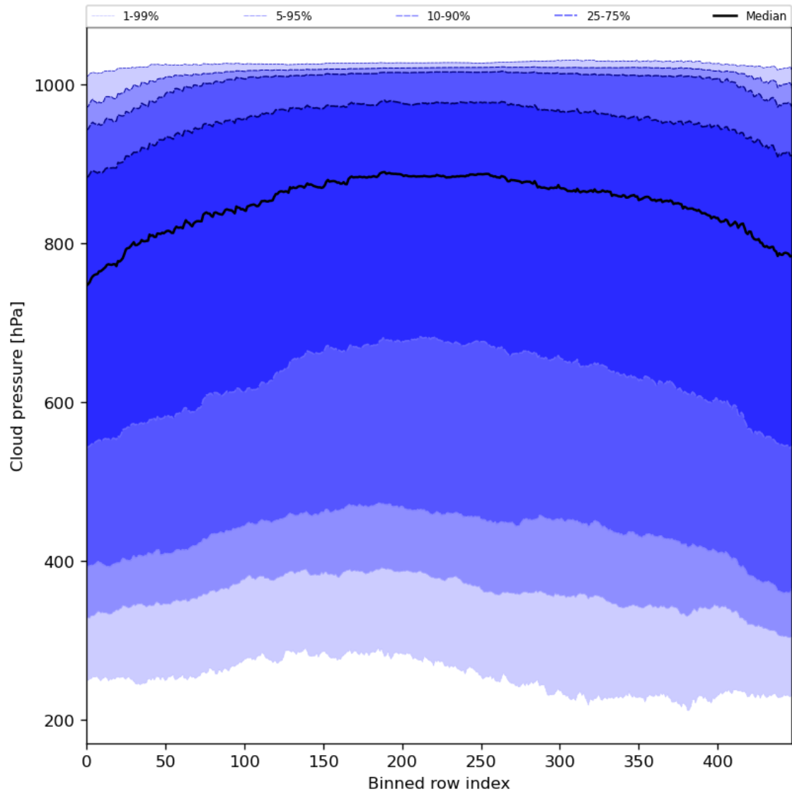
Figure 47: Along track statistics of “Cloud pressure” for 2024-06-03 to 2024-06-05
