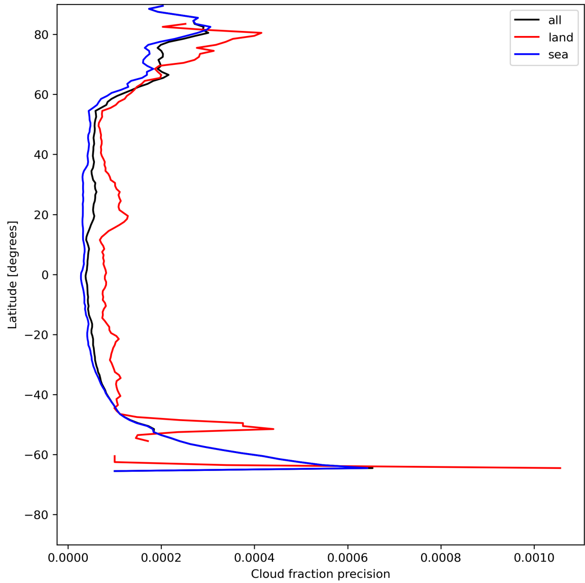
Figure 16: Zonal average of “Cloud fraction precision” for 2024-06-03 to 2024-06-05.
