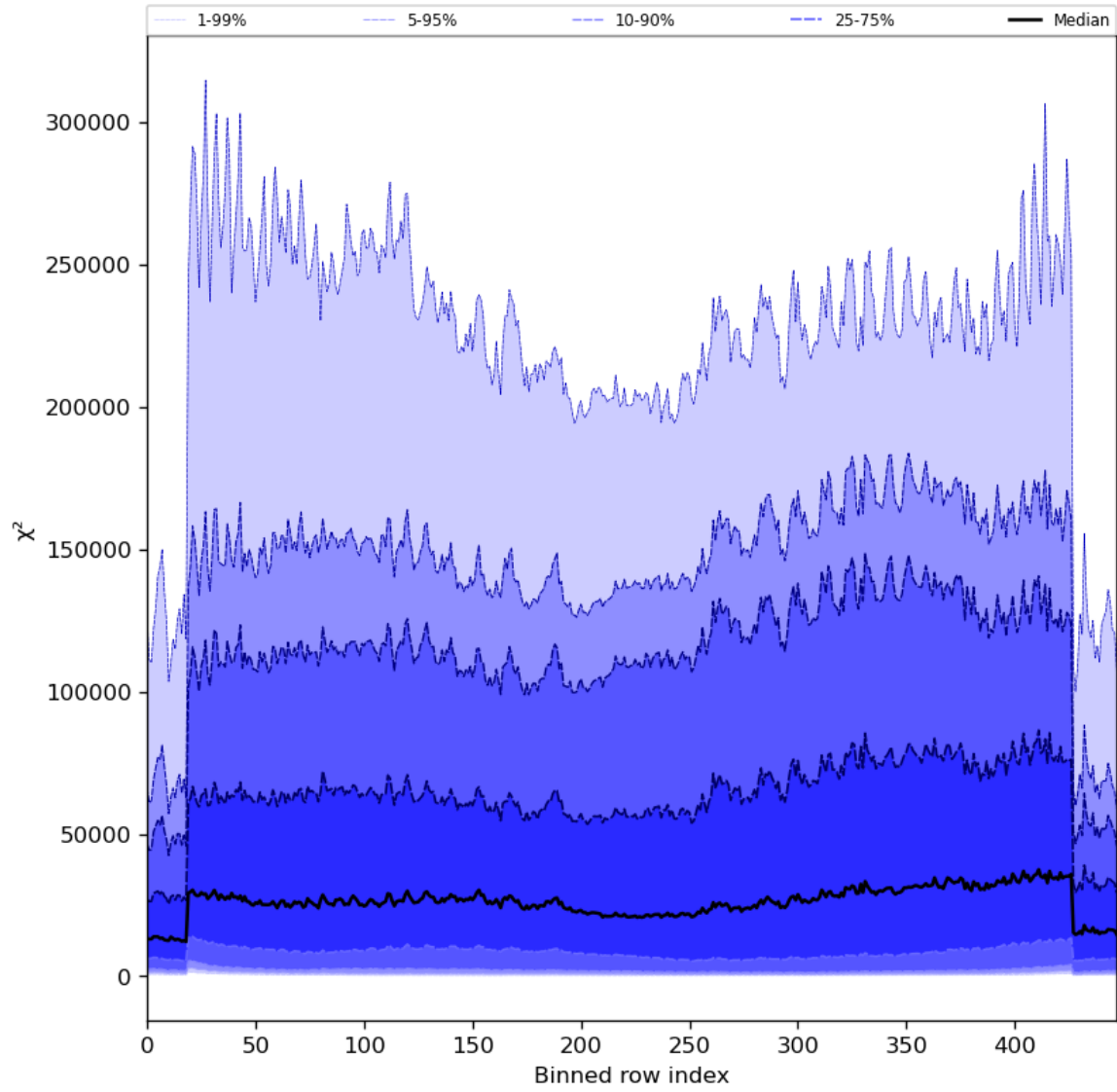
Figure 55: Along track statistics of “ \chi^2 ” for 2024-06-03 to 2024-06-05
