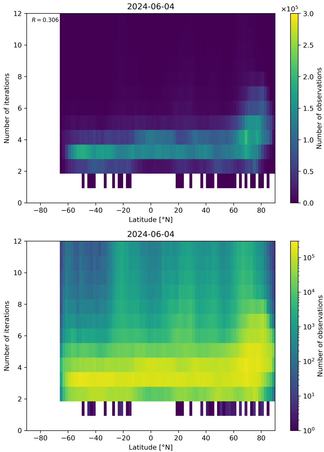
Figure 93: Scatter density plot of “Latitude” against “Number of iterations” for 2024-06-03 to 2024-06-05.
