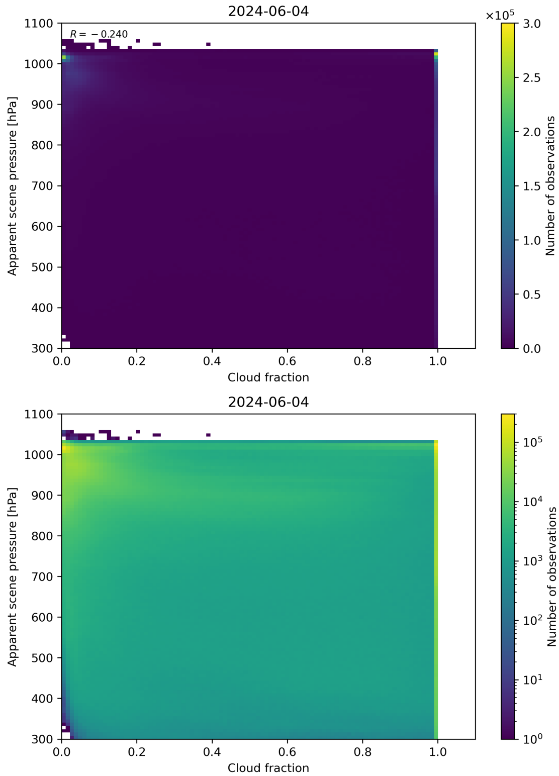
Figure 70: Scatter density plot of “Cloud fraction” against “Apparent scene pressure” for 2024-06-03 to 2024-06-05.
