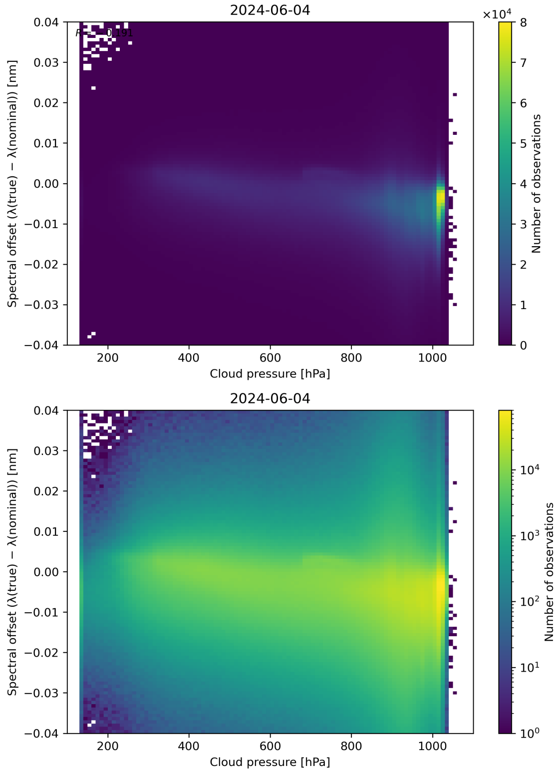
Figure 84: Scatter density plot of “Cloud pressure” against “Spectral offset ( \lambda(\text{true}) - \lambda(\text{nominal}) )” for 2024-06-03 to 2024-06-05.
