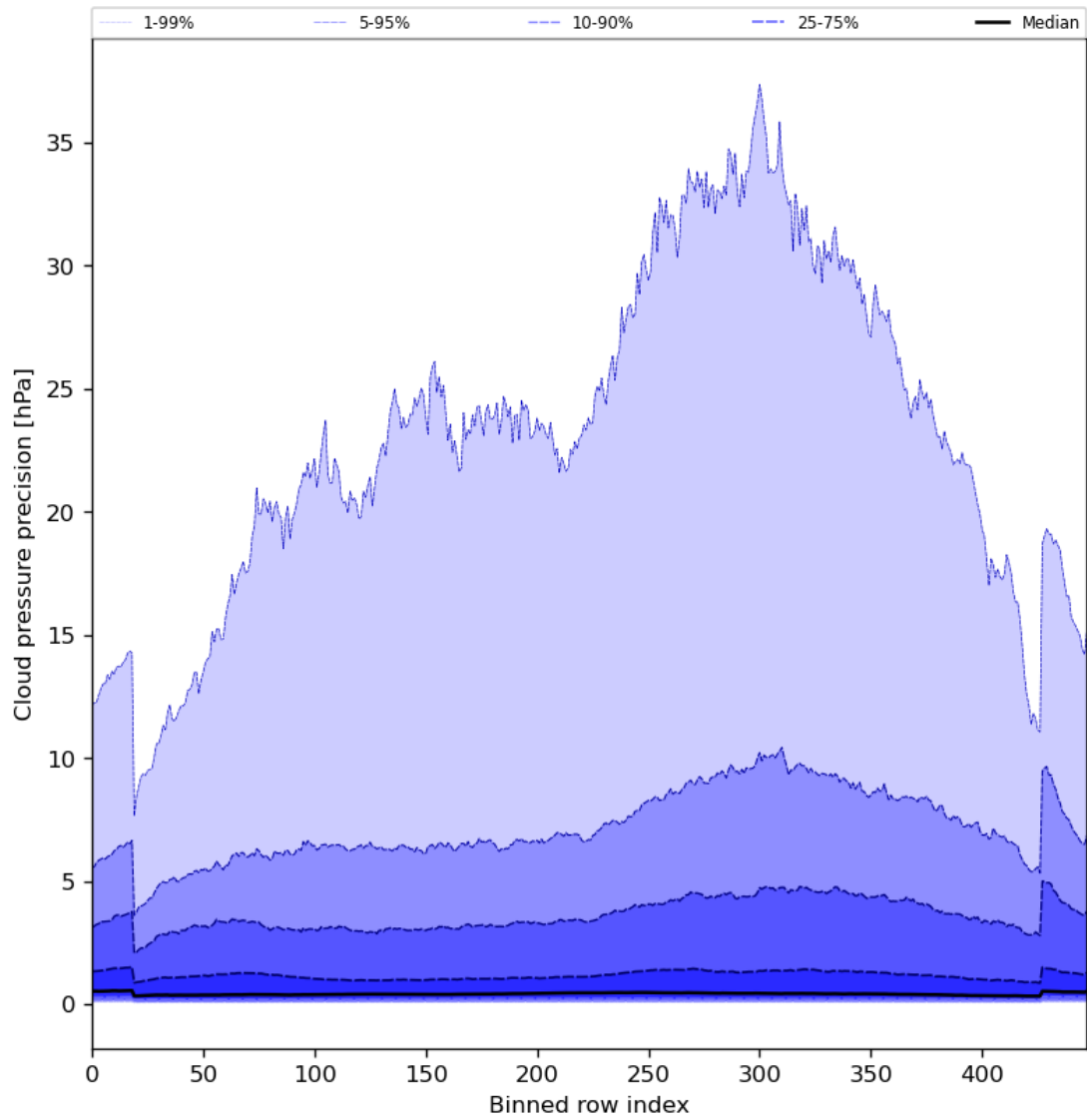
Figure 48: Along track statistics of “Cloud pressure precision” for 2024-06-03 to 2024-06-05
