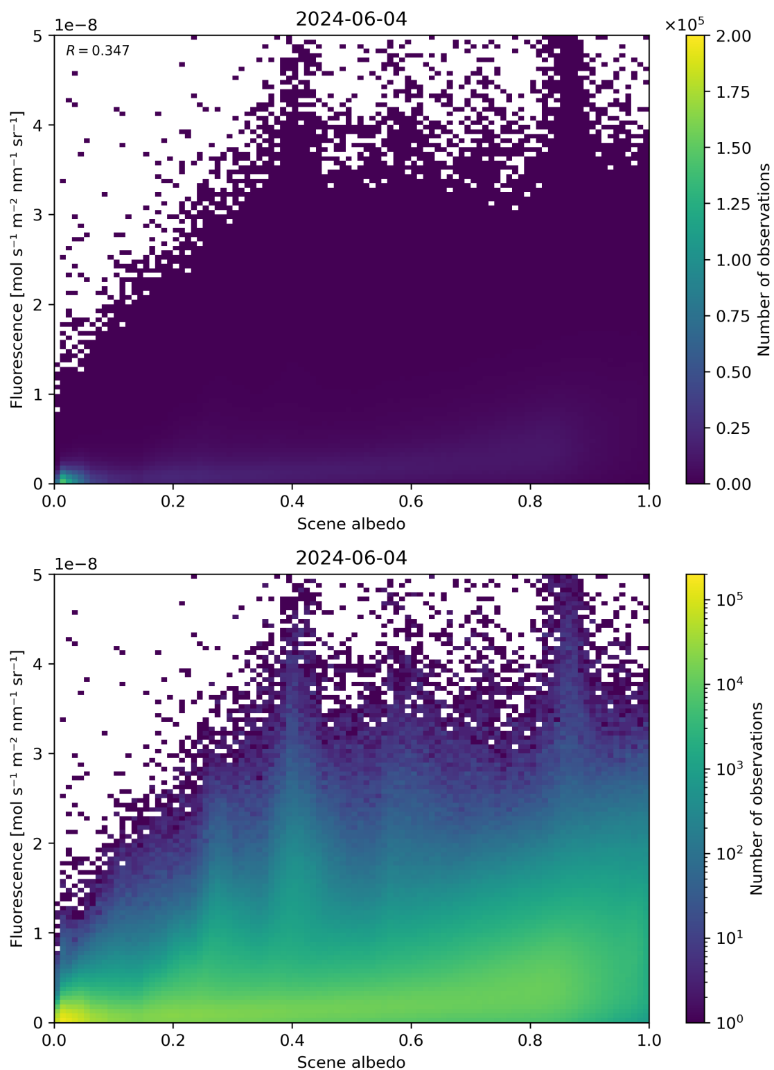
Figure 104: Scatter density plot of “Scene albedo” against “Fluorescence” for 2024-06-03 to 2024-06-05.
