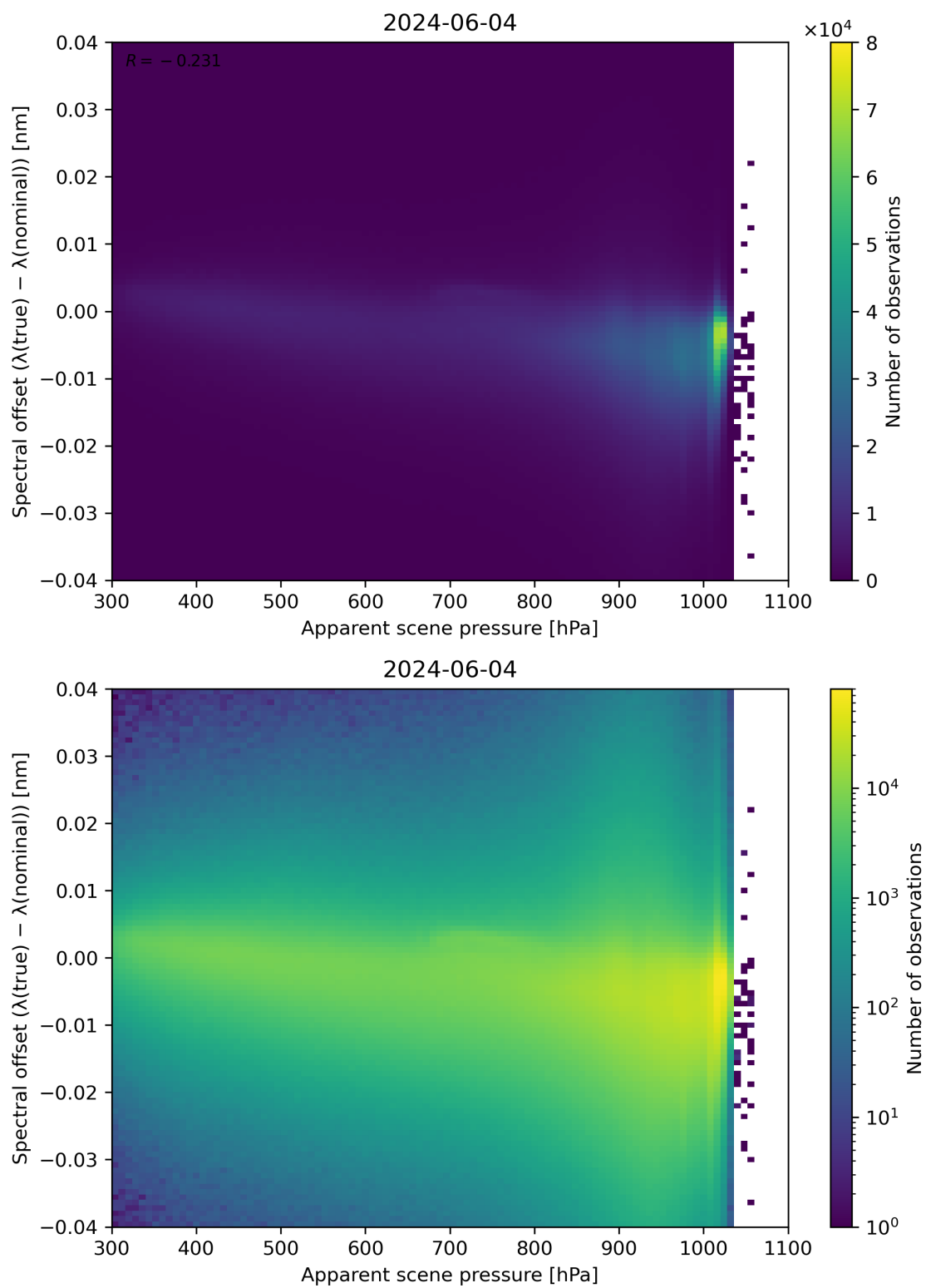
Figure 67: Scatter density plot of “Apparent scene pressure” against “Spectral offset ( \lambda(\text{true}) - \lambda(\text{nominal}) )” for 2024-06-03 to 2024-06-05.
