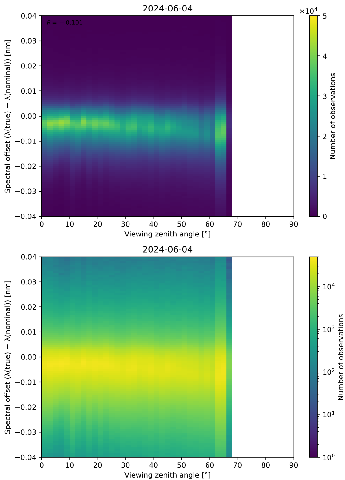
Figure 128: Scatter density plot of “Viewing zenith angle” against “Spectral offset ( \lambda(\text{true}) - \lambda(\text{nominal}) )” for 2024-06-03 to 2024-06-05.
