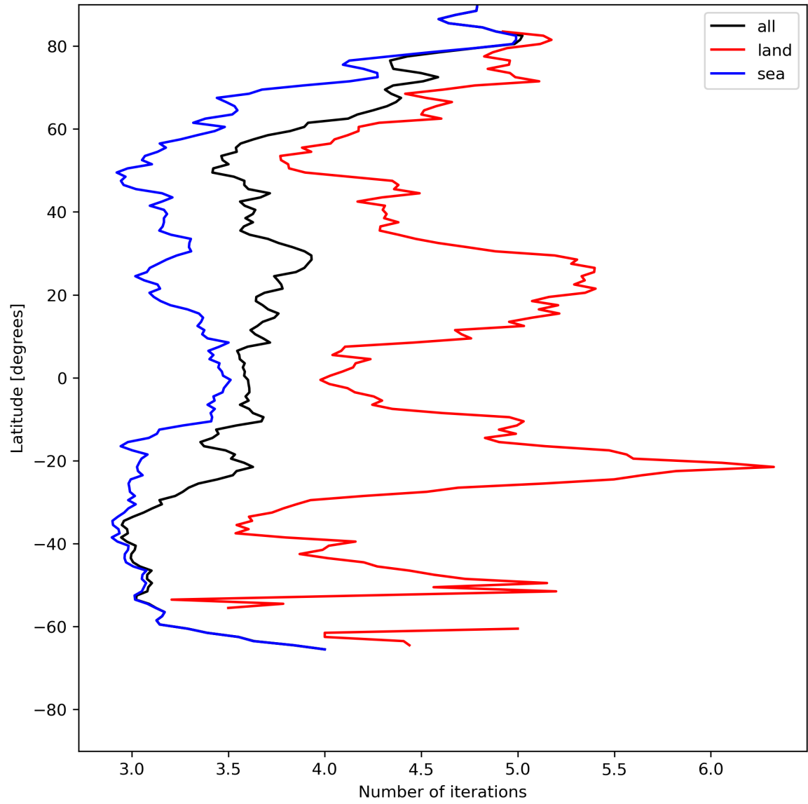
Figure 22: Zonal average of “Number of iterations” for 2024-06-03 to 2024-06-05.
