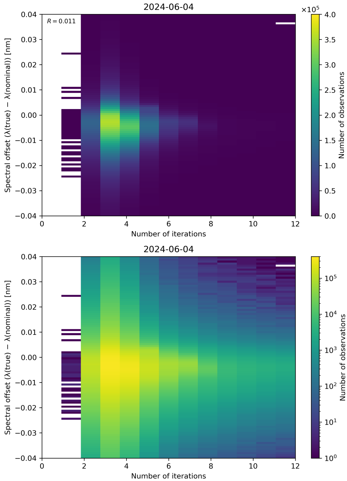
Figure 100: Scatter density plot of “Number of iterations” against “Spectral offset ( \lambda(\text{true}) - \lambda(\text{nominal}) )” for 2024-06-03 to 2024-06-05.
