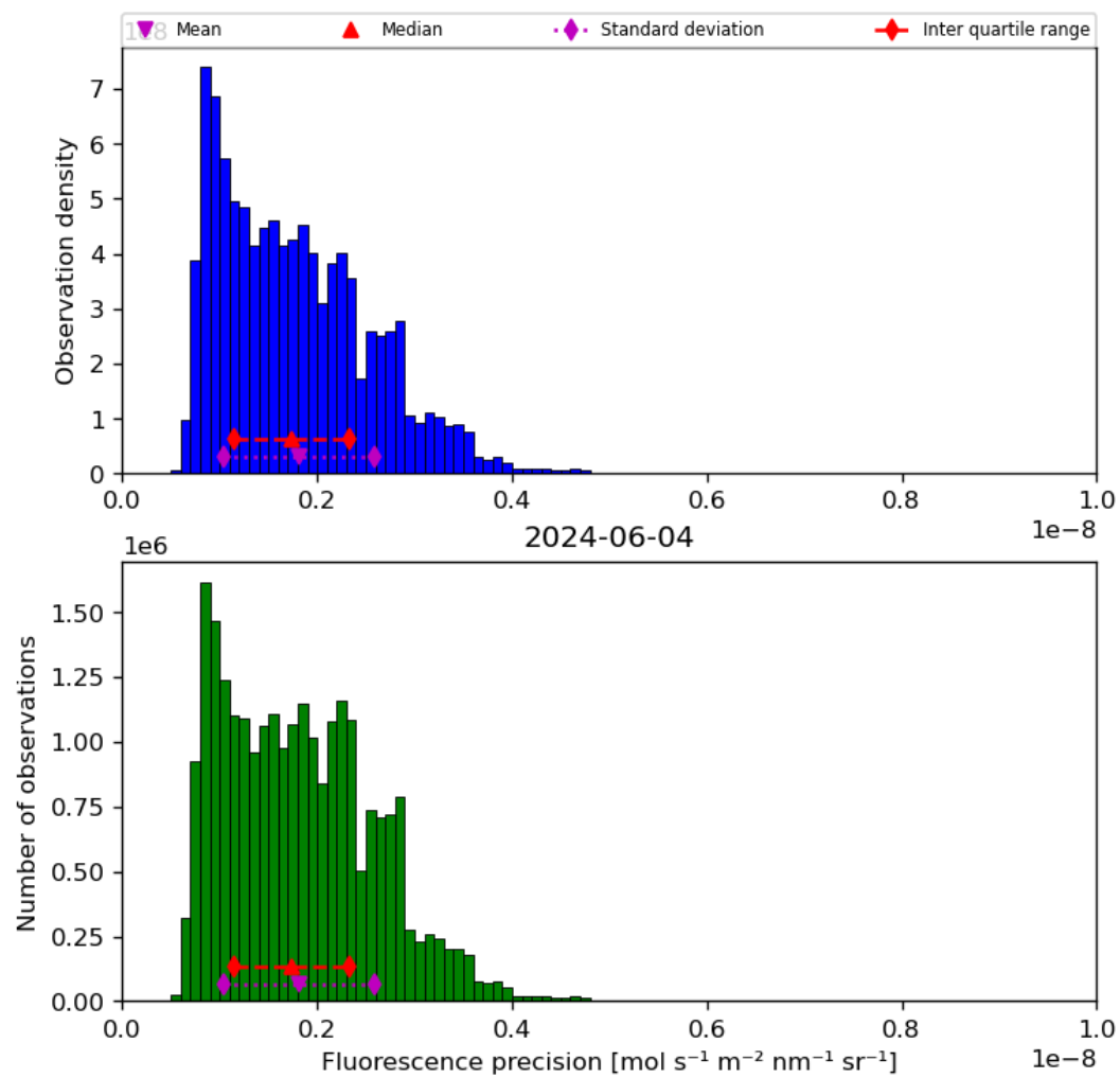
Figure 41: Histogram of “Fluorescence precision” for 2024-06-03 to 2024-06-05
