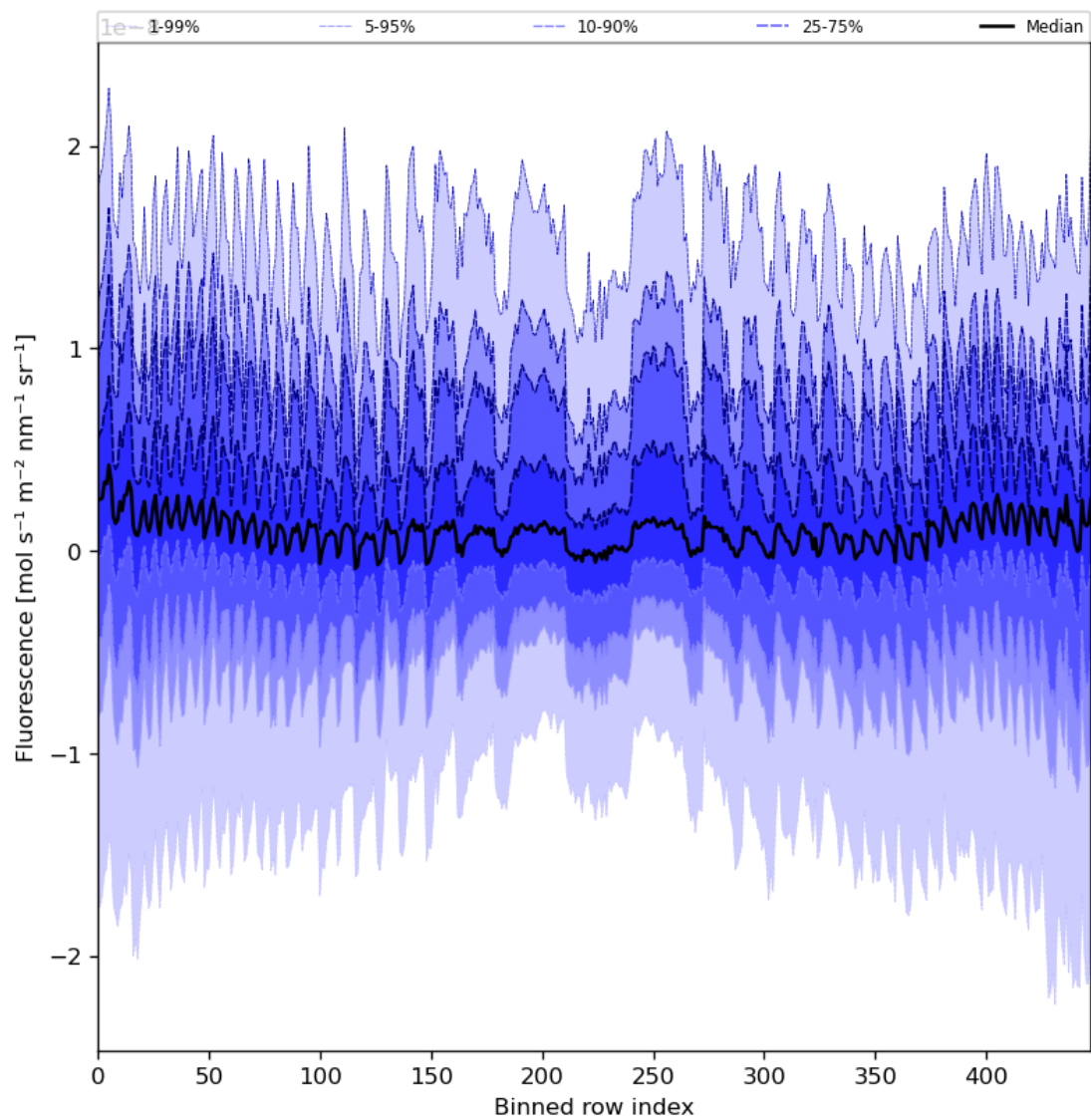
Figure 57: Along track statistics of “Fluorescence” for 2024-06-03 to 2024-06-05
