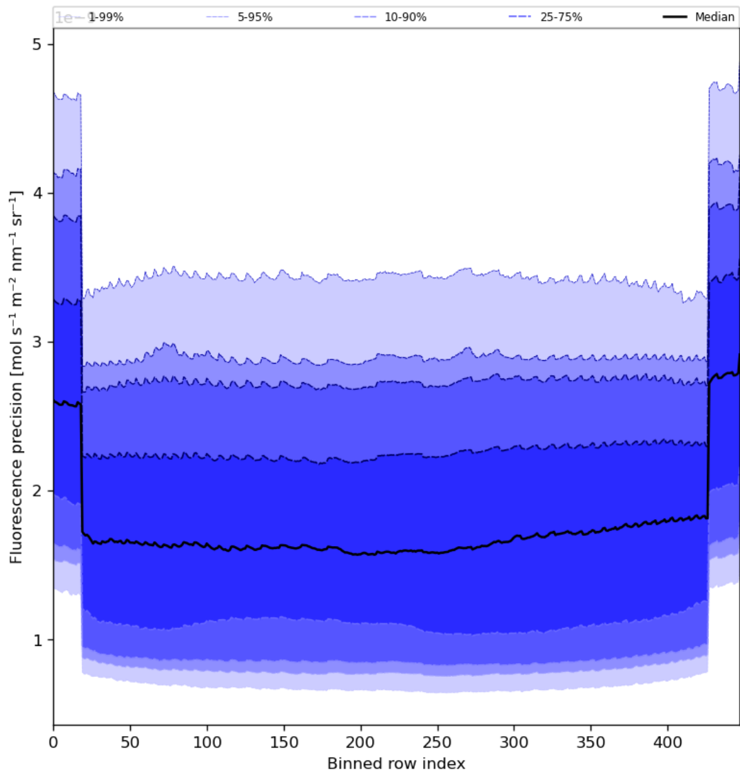
Figure 58: Along track statistics of “Fluorescence precision” for 2024-06-03 to 2024-06-05
