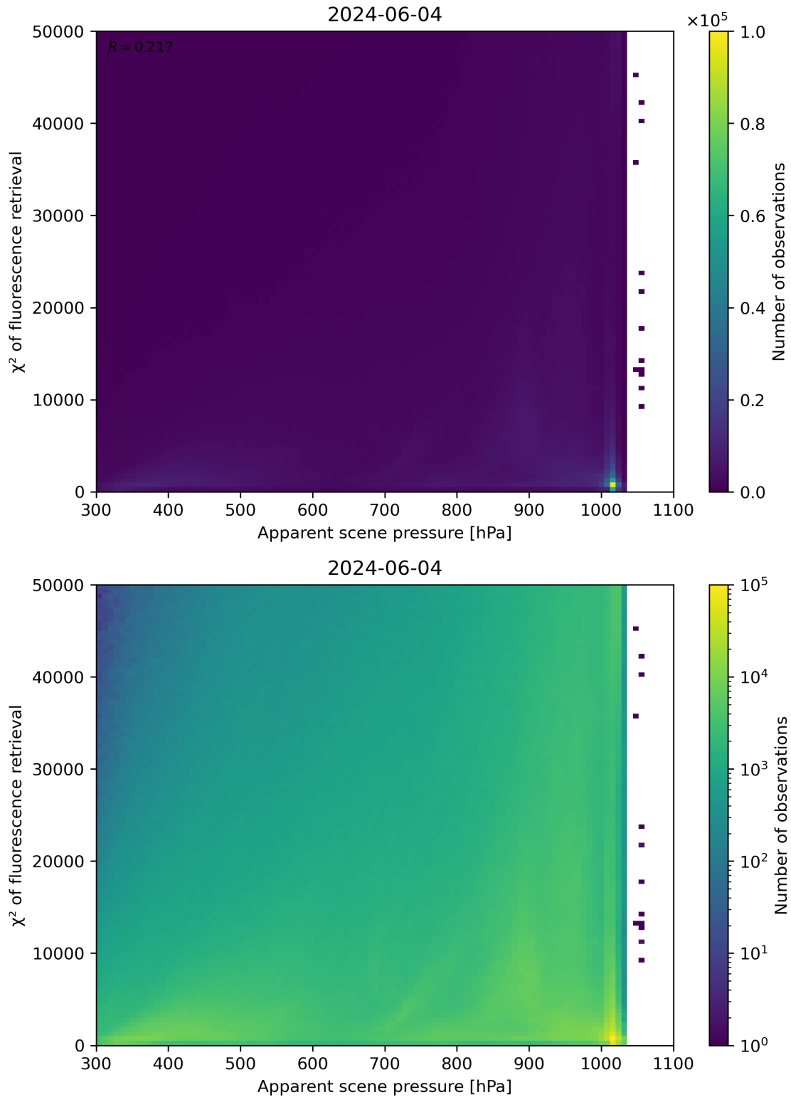
Figure 63: Scatter density plot of “Apparent scene pressure” against “ \chi^2 of fluorescence retrieval” for 2024-06-03 to 2024-06-05.
