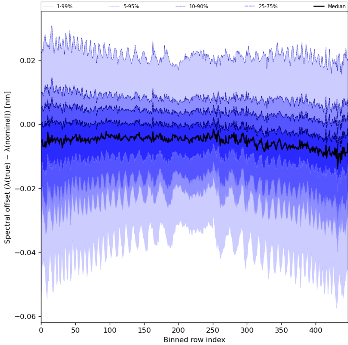
Figure 62: Along track statistics of “Spectral offset ( \lambda(\text{true}) - \lambda(\text{nominal}) )” for 2024-06-03 to 2024-06-05
