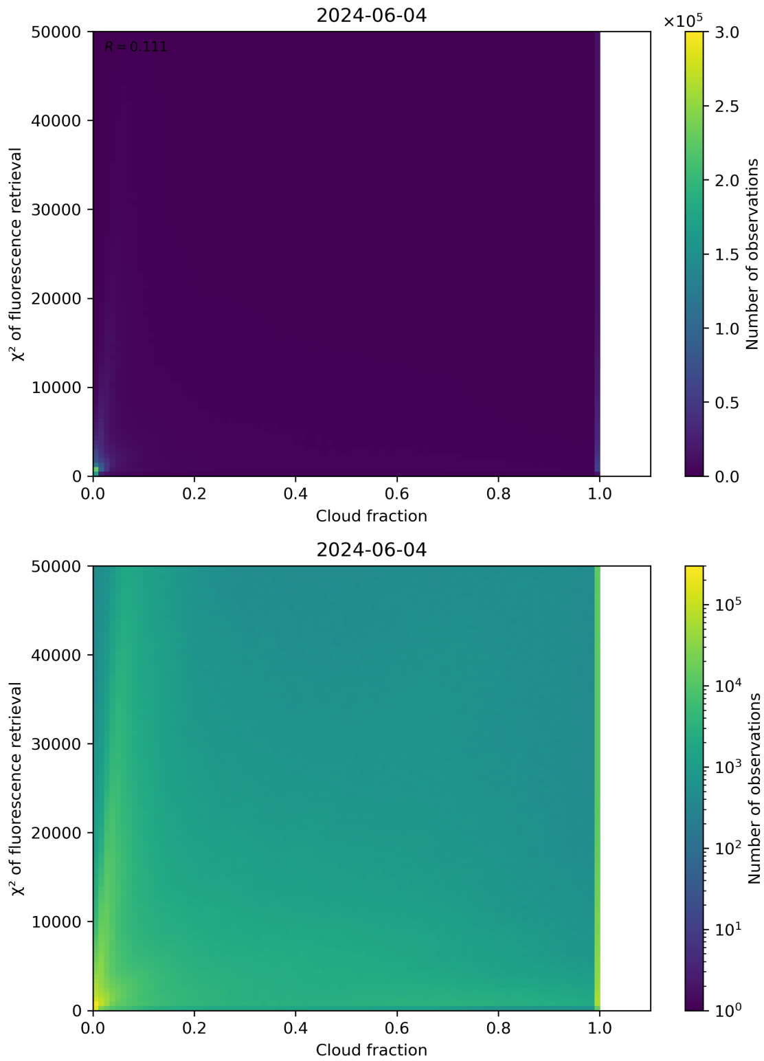
Figure 71: Scatter density plot of “Cloud fraction” against “ \chi^2 of fluorescence retrieval” for 2024-06-03 to 2024-06-05.
