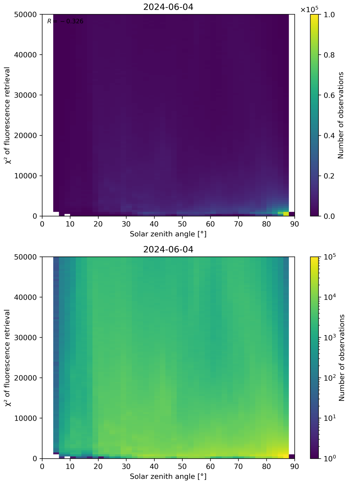
Figure 109: Scatter density plot of “Solar zenith angle” against “ \chi^2 of fluorescence retrieval” for 2024-06-03 to 2024-06-05.
