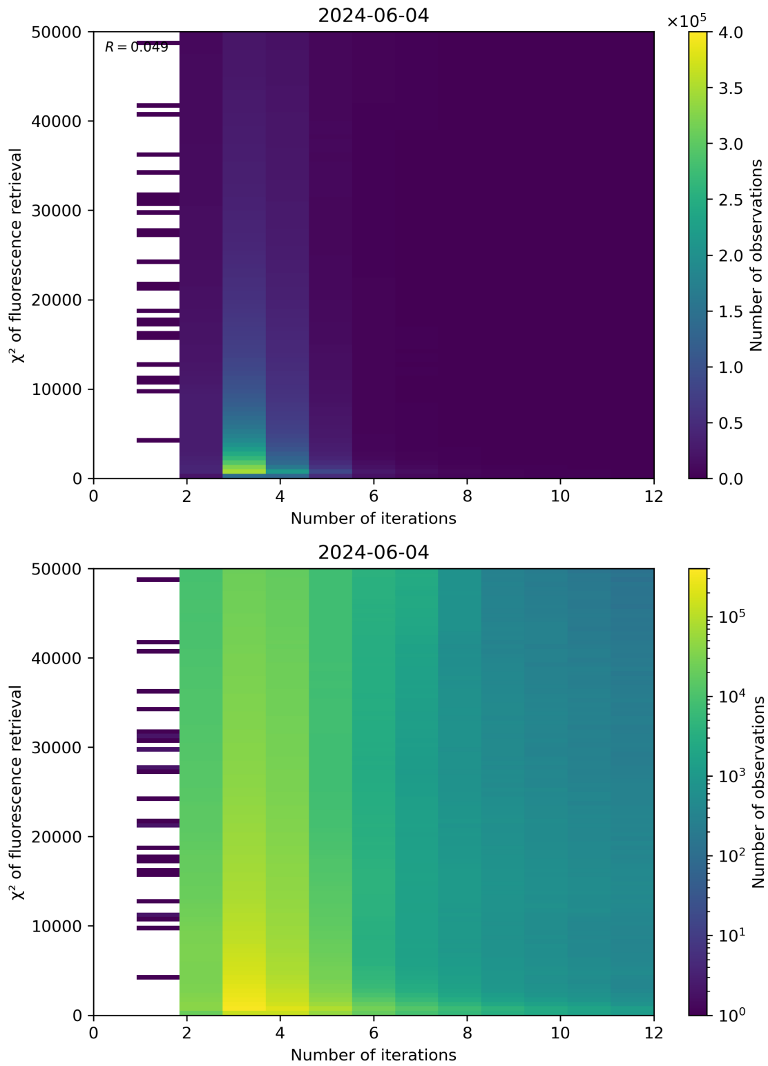
Figure 97: Scatter density plot of “Number of iterations” against “ \chi^2 of fluorescence retrieval” for 2024-06-03 to 2024-06-05.
