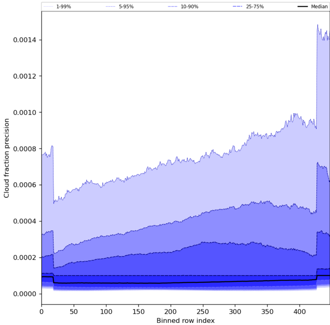
Figure 50: Along track statistics of “Cloud fraction precision” for 2024-06-03 to 2024-06-05
