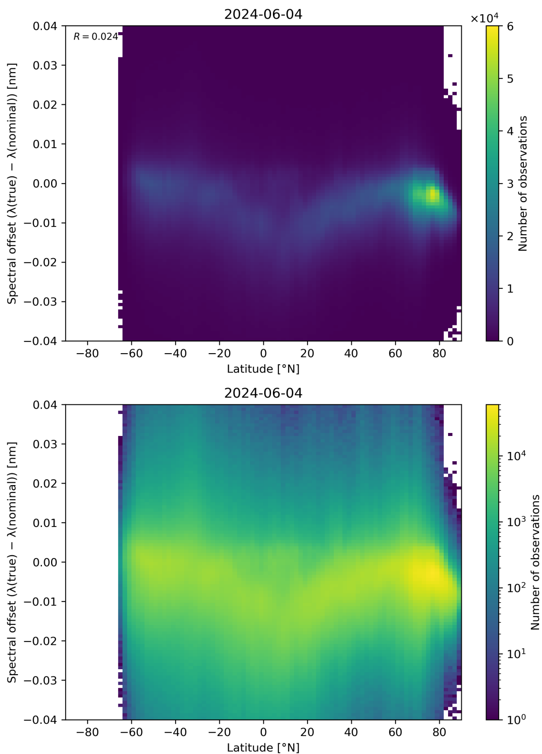
Figure 96: Scatter density plot of “Latitude” against “Spectral offset ( \lambda(\text{true}) - \lambda(\text{nominal}) )” for 2024-06-03 to 2024-06-05.
