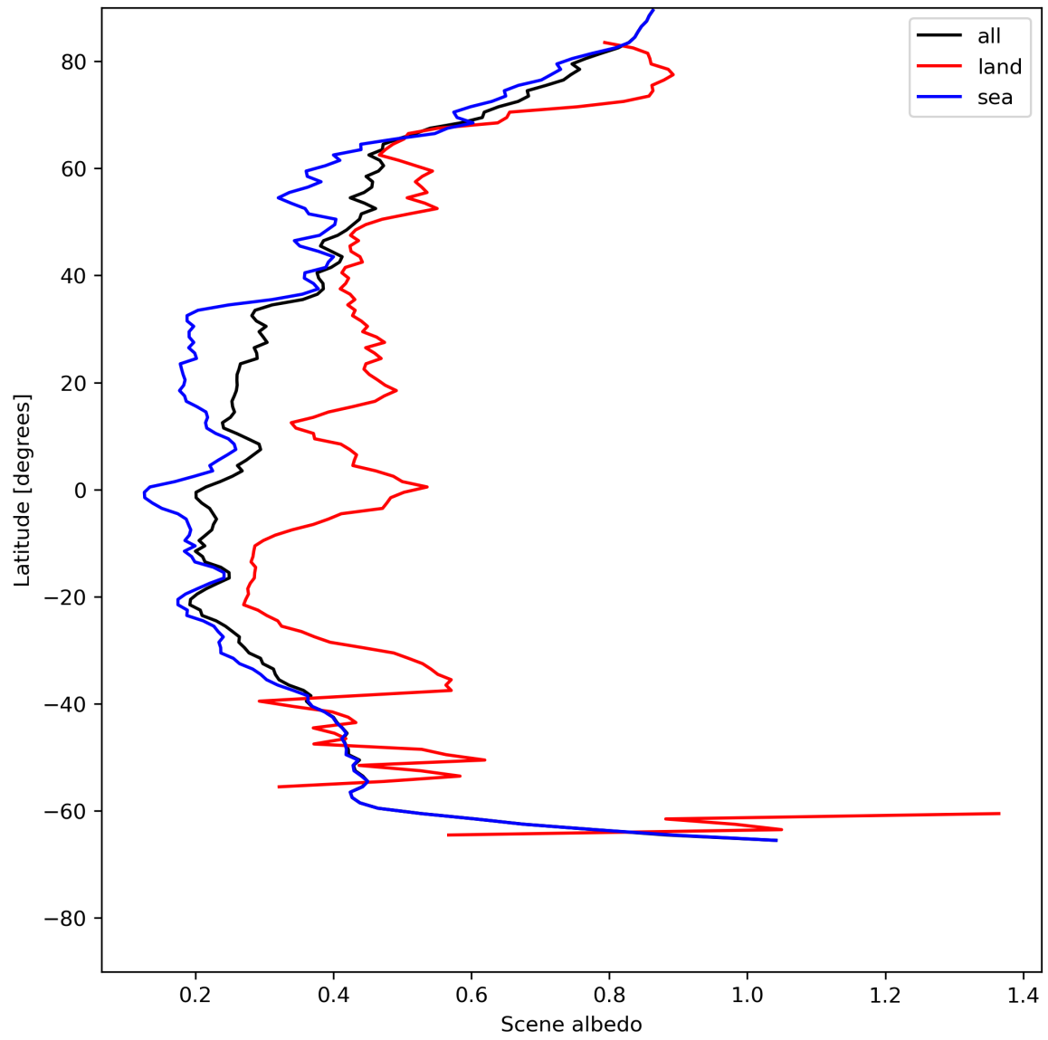
Figure 17: Zonal average of “Scene albedo” for 2024-06-03 to 2024-06-05.
