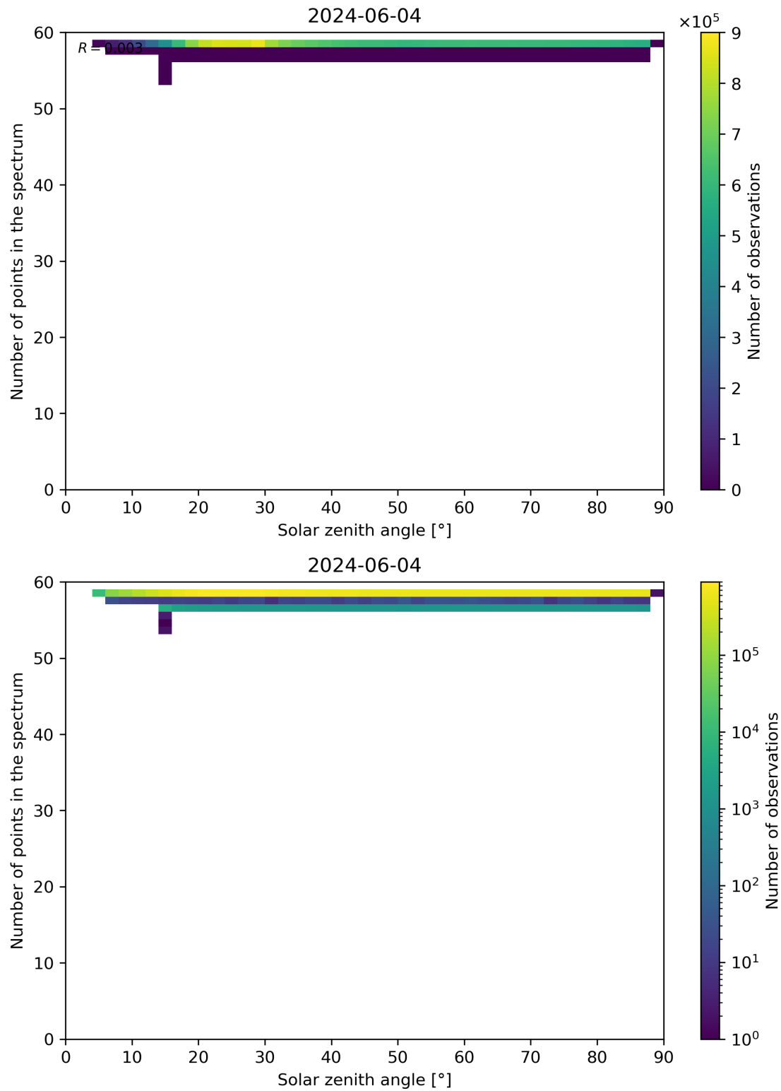
Figure 115: Scatter density plot of “Solar zenith angle” against “Number of points in the spectrum” for 2024-06-03 to 2024-06-05.
