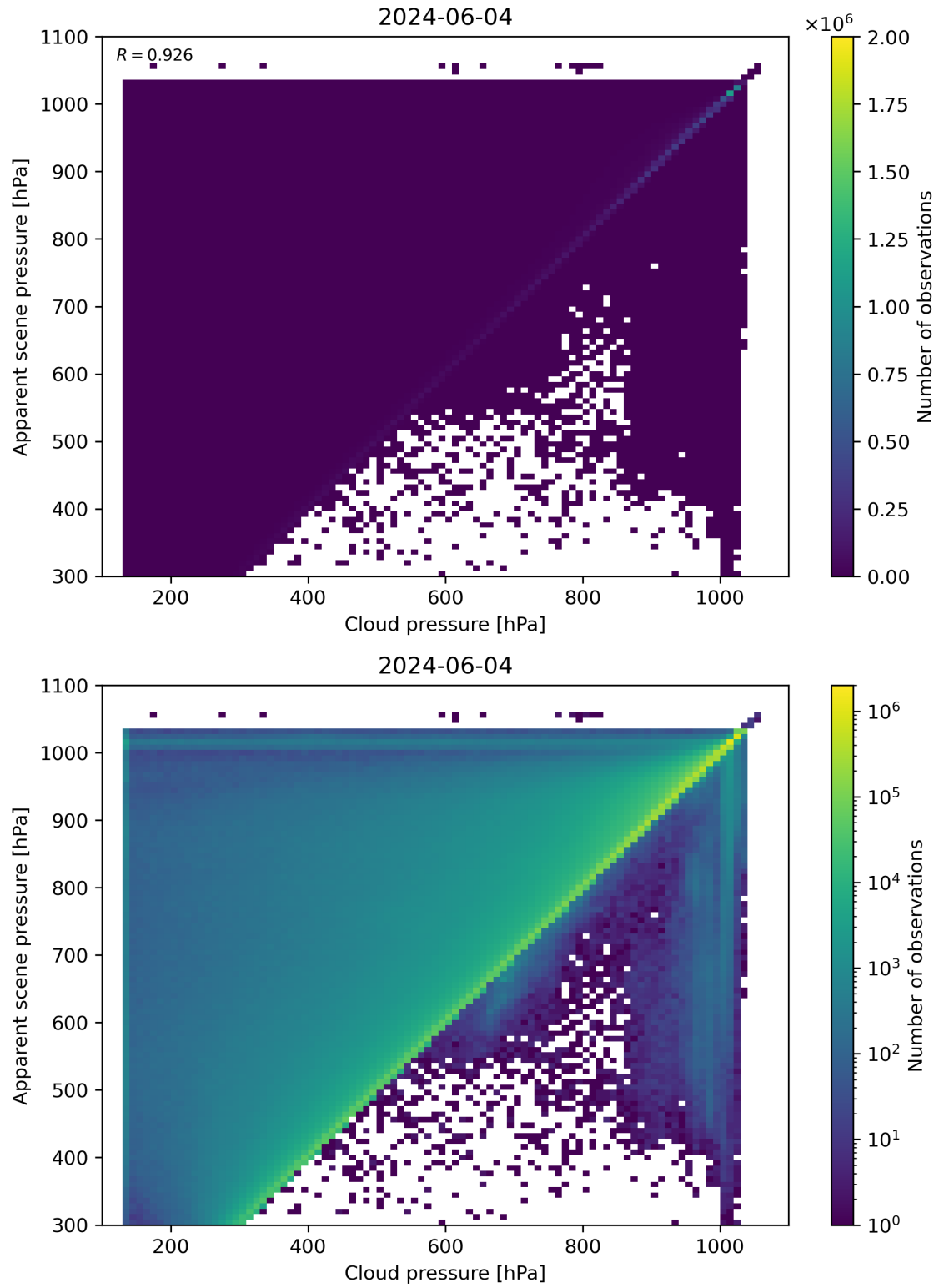
Figure 77: Scatter density plot of “Cloud pressure” against “Apparent scene pressure” for 2024-06-03 to 2024-06-05.
