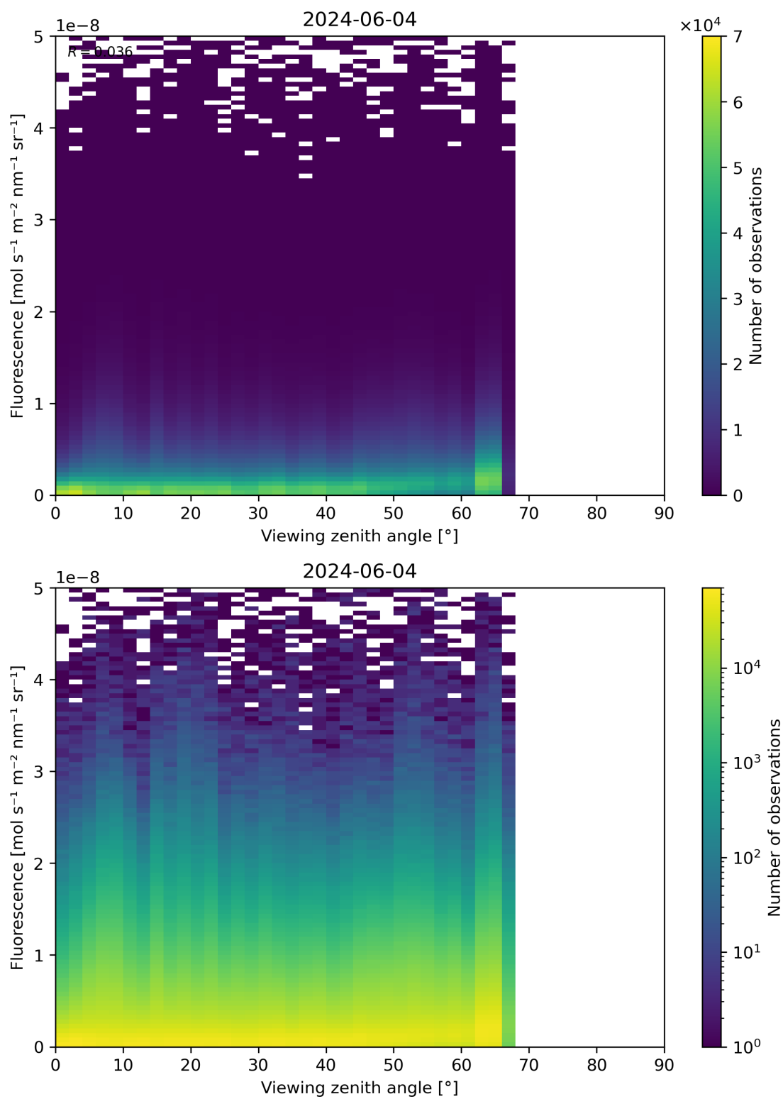
Figure 122: Scatter density plot of “Viewing zenith angle” against “Fluorescence” for 2024-06-03 to 2024-06-05.
