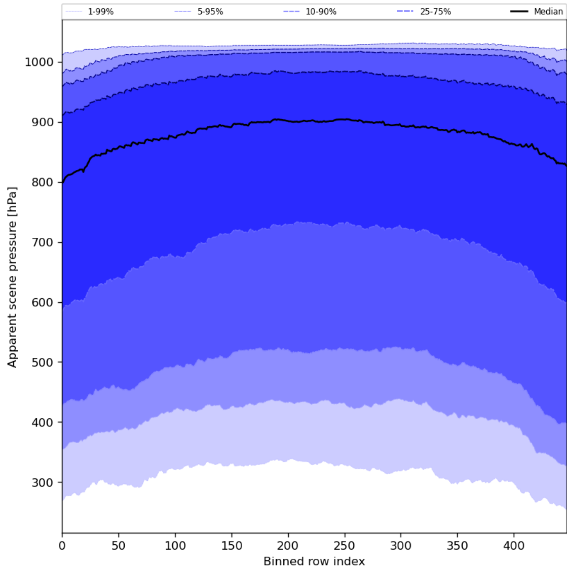
Figure 53: Along track statistics of “Apparent scene pressure” for 2024-06-03 to 2024-06-05
