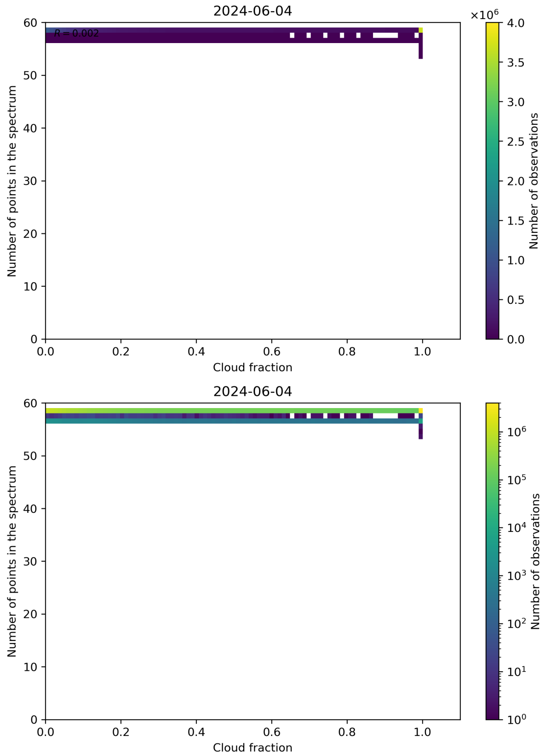
Figure 74: Scatter density plot of “Cloud fraction” against “Number of points in the spectrum” for 2024-06-03 to 2024-06-05.
