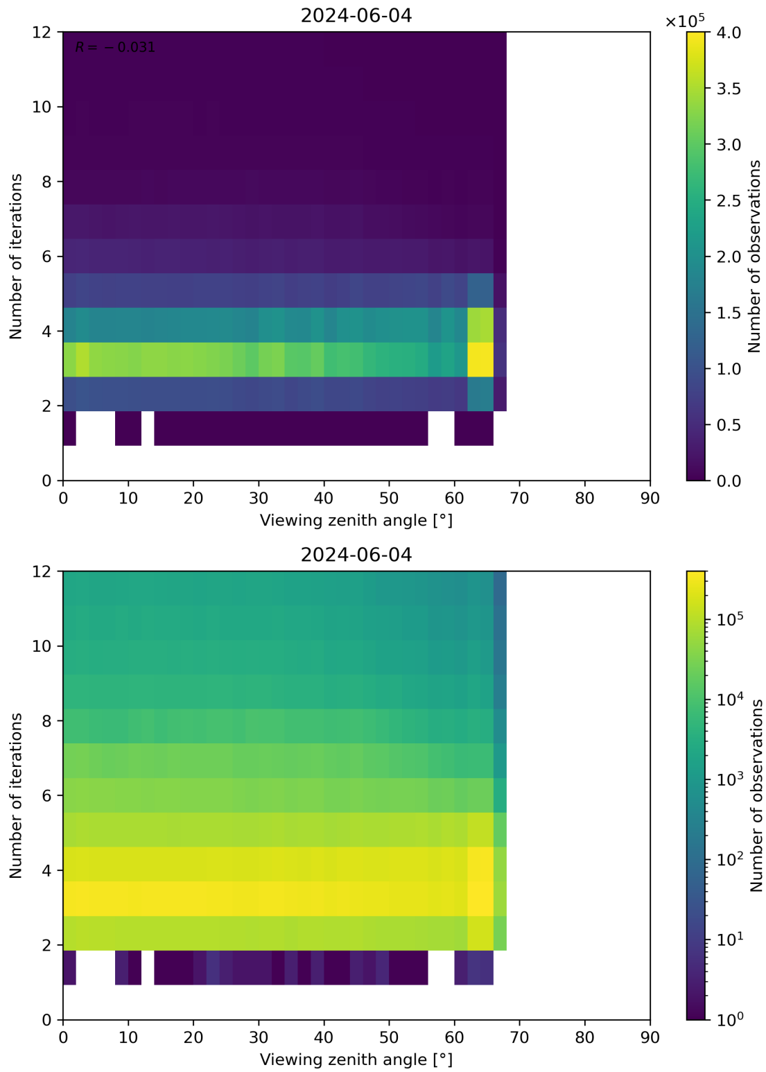
Figure 124: Scatter density plot of “Viewing zenith angle” against “Number of iterations” for 2024-06-03 to 2024-06-05.
