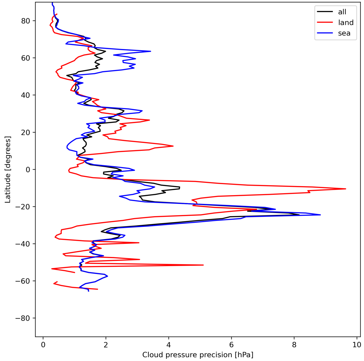
Figure 14: Zonal average of "Cloud pressure precision" for 2024-06-03 to 2024-06-05.
