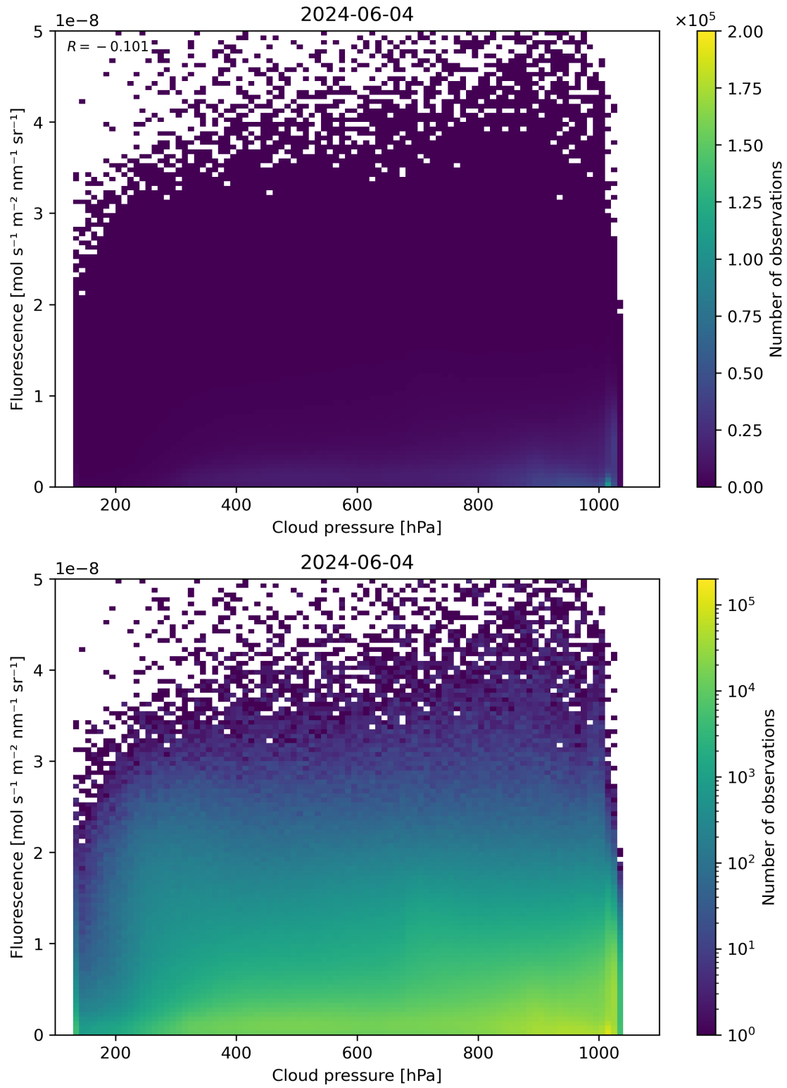
Figure 80: Scatter density plot of “Cloud pressure” against “Fluorescence” for 2024-06-03 to 2024-06-05.
