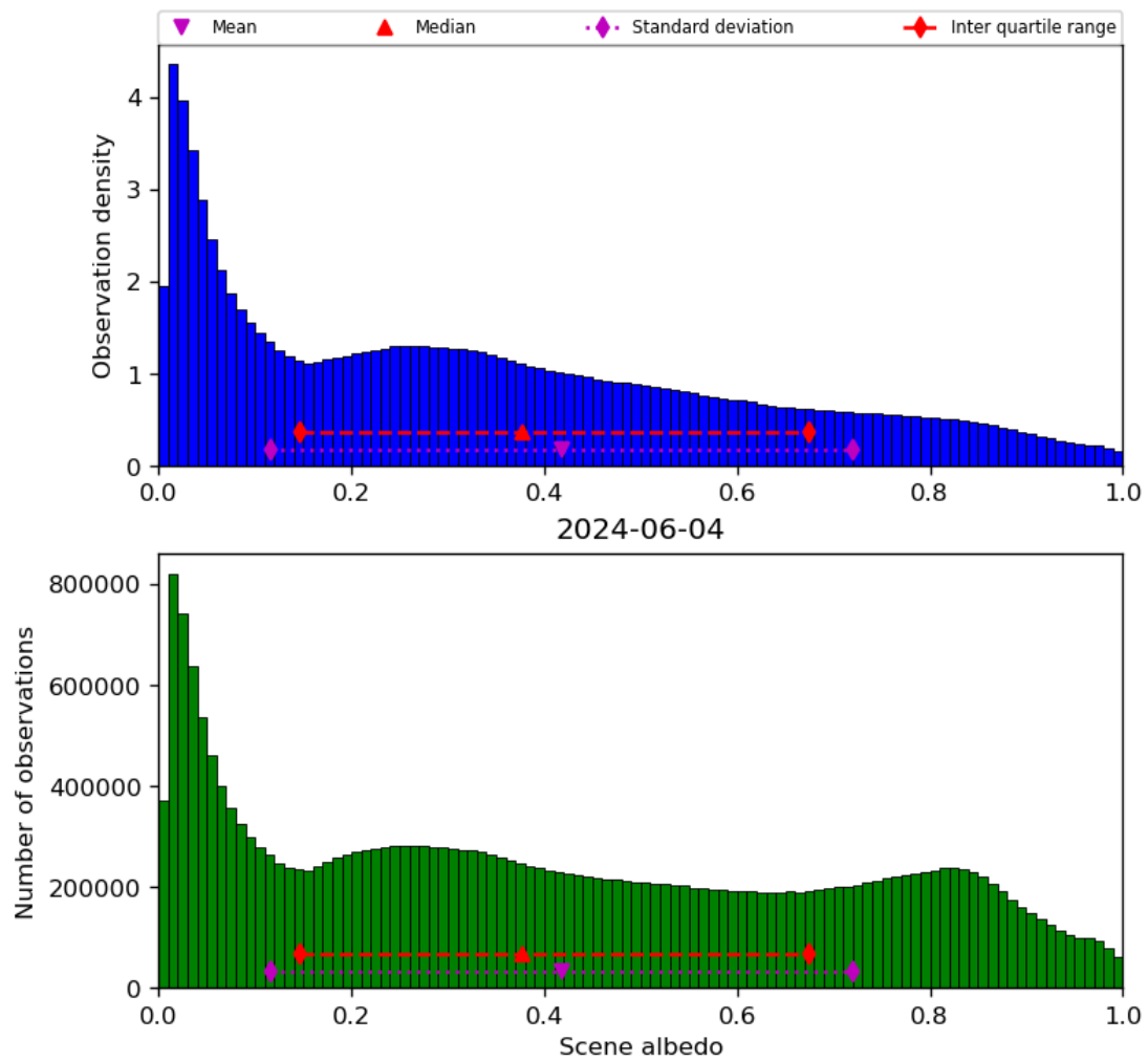
Figure 34: Histogram of “Scene albedo” for 2024-06-03 to 2024-06-05
