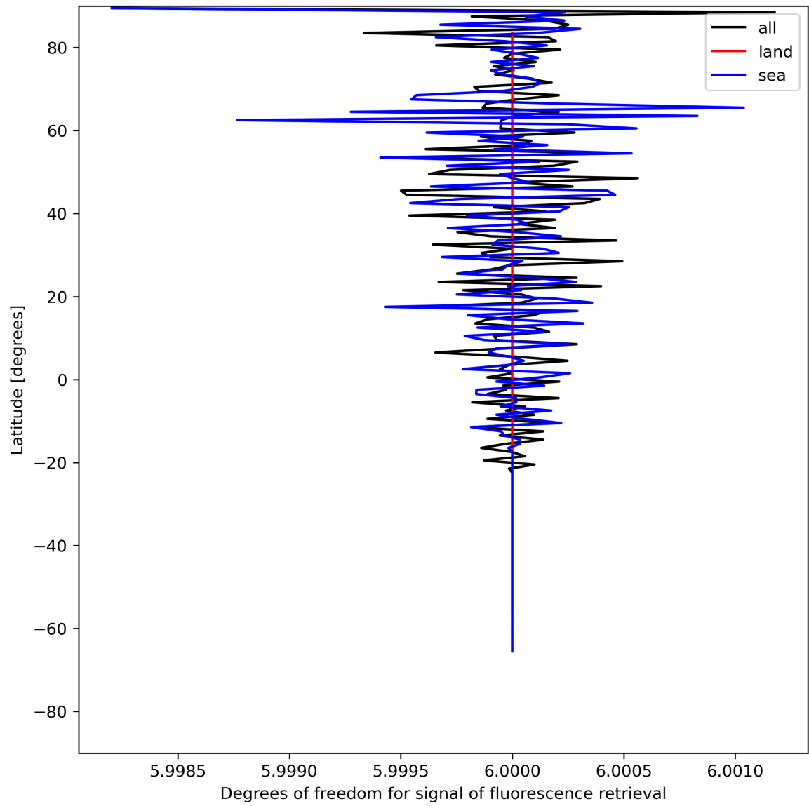
Figure 26: Zonal average of “Degrees of freedom for signal of fluorescence retrieval” for 2024-06-03 to 2024-06-05.
