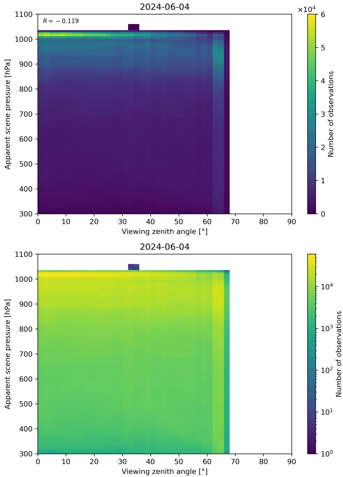
Figure 118: Scatter density plot of “Viewing zenith angle” against “Apparent scene pressure” for 2024-06-03 to 2024-06-05.
