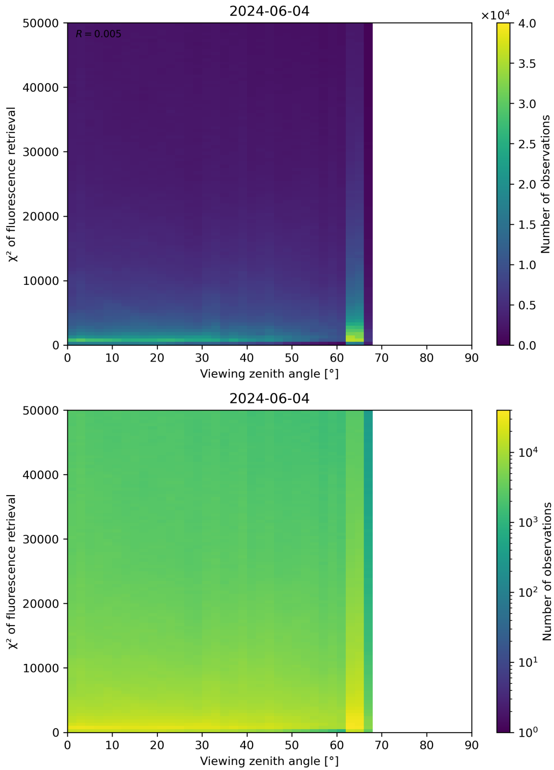
Figure 119: Scatter density plot of “Viewing zenith angle” against “ \chi^2 of fluorescence retrieval” for 2024-06-03 to 2024-06-05.
