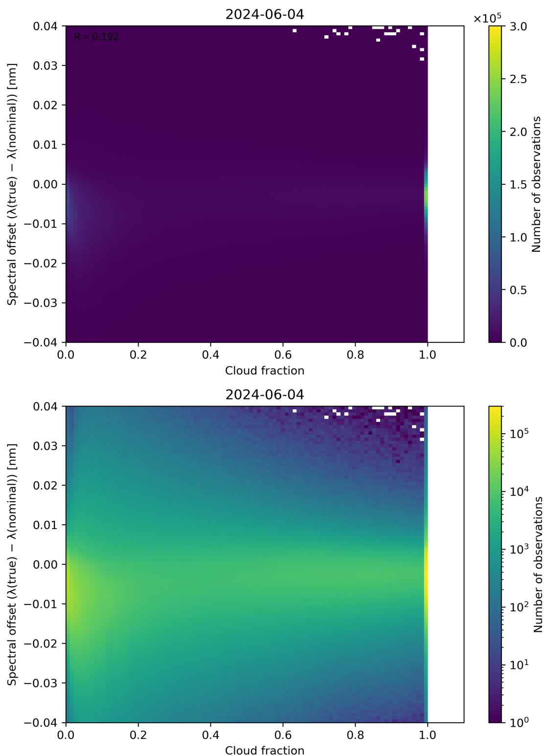
Figure 76: Scatter density plot of “Cloud fraction” against “Spectral offset ( \lambda(\text{true}) - \lambda(\text{nominal}) )” for 2024-06-03 to 2024-06-05.
