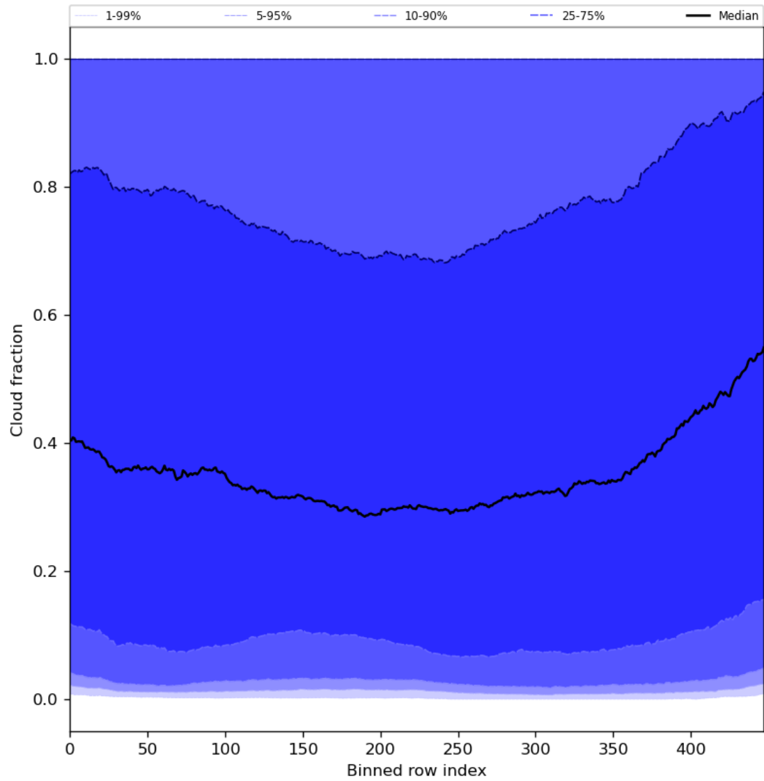
Figure 49: Along track statistics of “Cloud fraction” for 2024-06-03 to 2024-06-05
