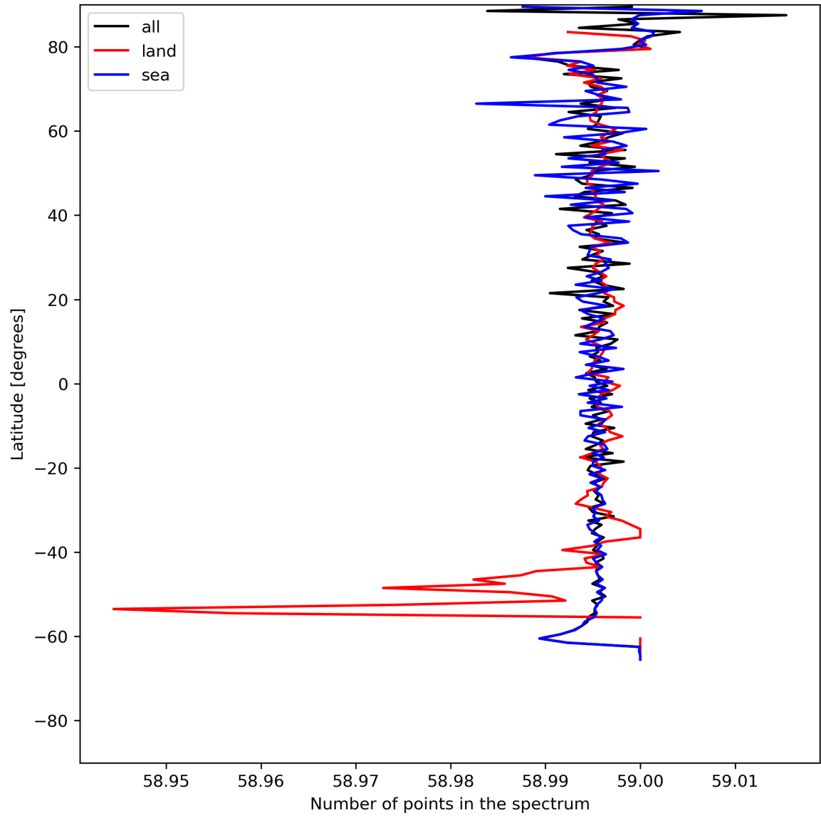
Figure 27: Zonal average of “Number of points in the spectrum” for 2024-06-03 to 2024-06-05.
