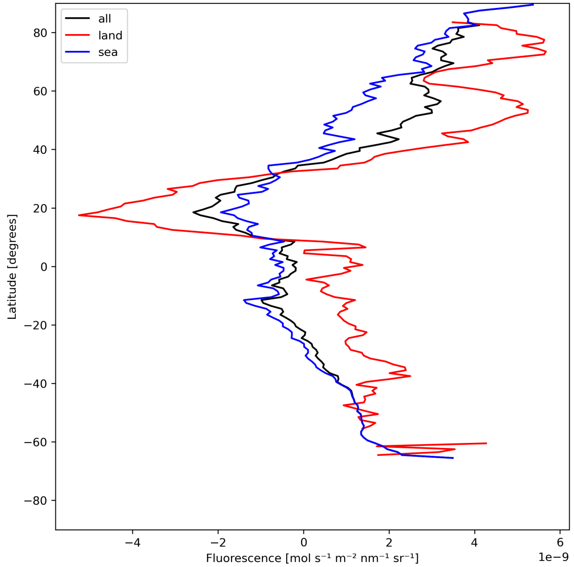
Figure 23: Zonal average of “Fluorescence” for 2024-06-03 to 2024-06-05.
