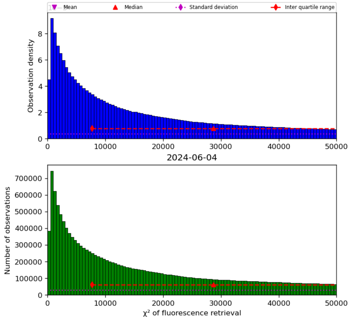
Figure 42: Histogram of “ \chi^2 of fluorescence retrieval” for 2024-06-03 to 2024-06-05
