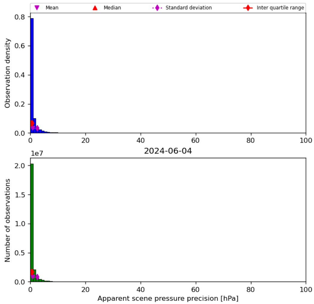
Figure 37: Histogram of “Apparent scene pressure precision” for 2024-06-03 to 2024-06-05
