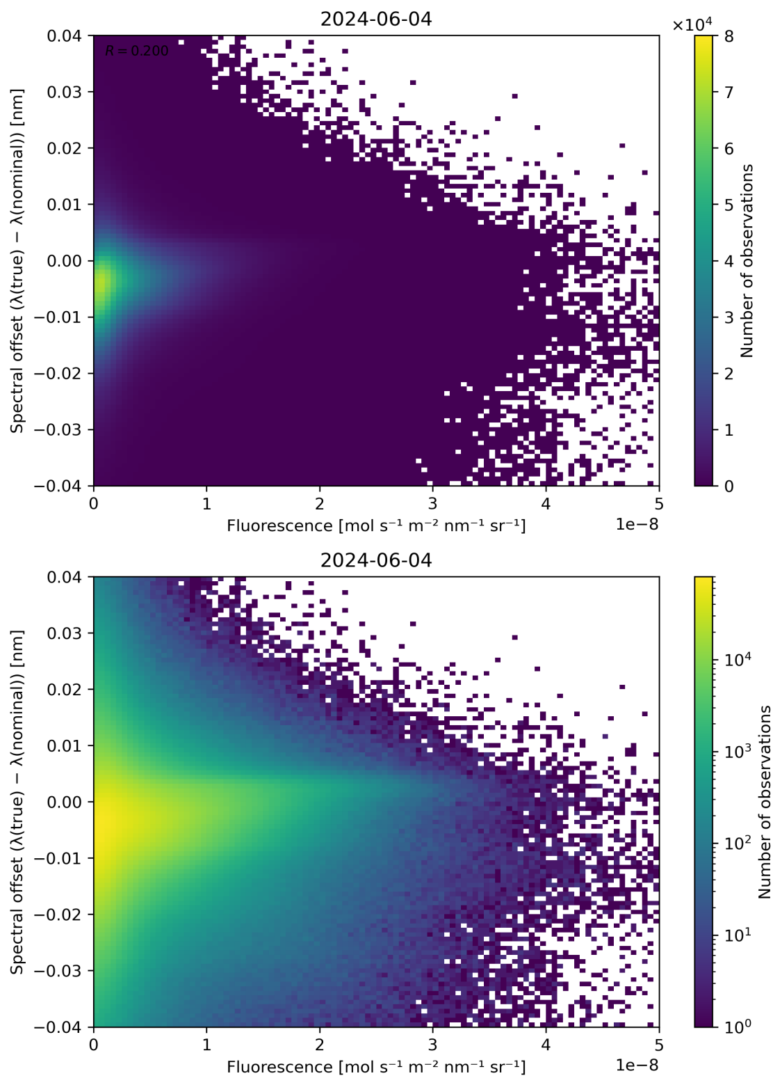
Figure 87: Scatter density plot of “Fluorescence” against “Spectral offset ( \lambda(\text{true}) - \lambda(\text{nominal}) )” for 2024-06-03 to 2024-06-05.
