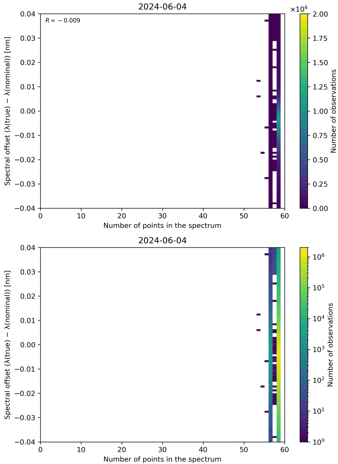
Figure 101: Scatter density plot of “Number of points in the spectrum” against “Spectral offset ( \lambda(\text{true}) - \lambda(\text{nominal}) )” for 2024-06-03 to 2024-06-05.
