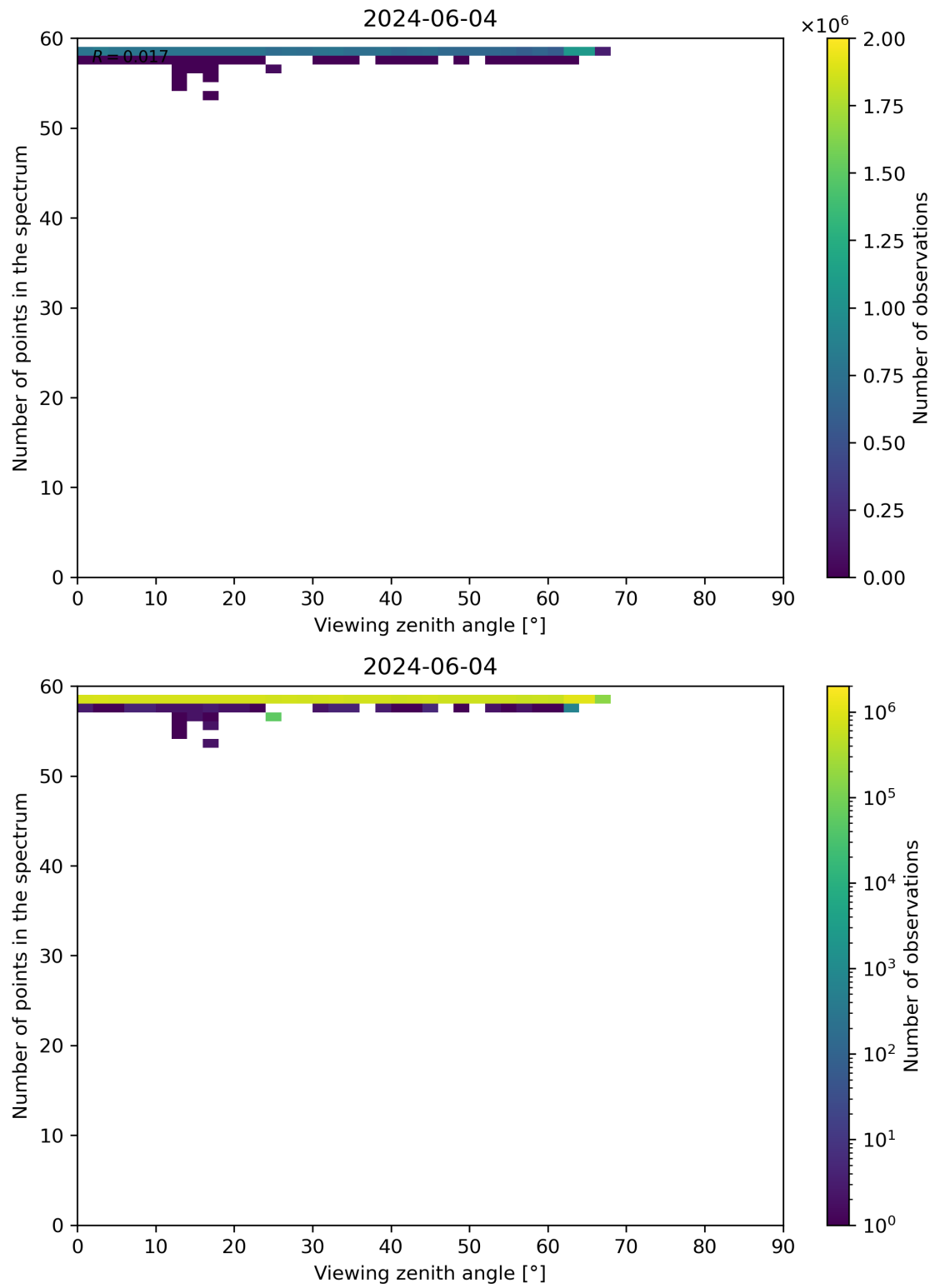
Figure 125: Scatter density plot of “Viewing zenith angle” against “Number of points in the spectrum” for 2024-06-03 to 2024-06-05.
