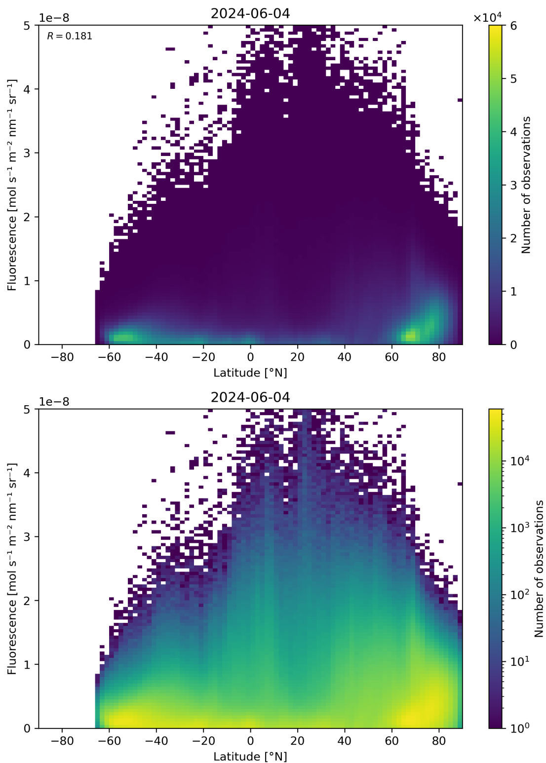
Figure 92: Scatter density plot of “Latitude” against “Fluorescence” for 2024-06-03 to 2024-06-05.
