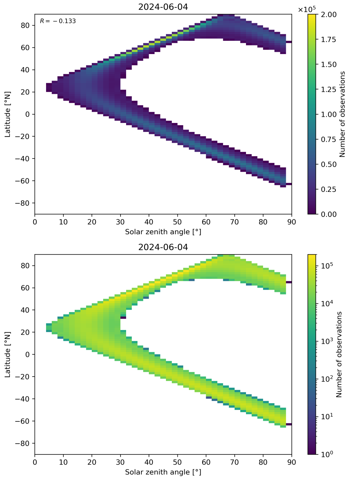
Figure 113: Scatter density plot of “Solar zenith angle” against “Latitude” for 2024-06-03 to 2024-06-05.
