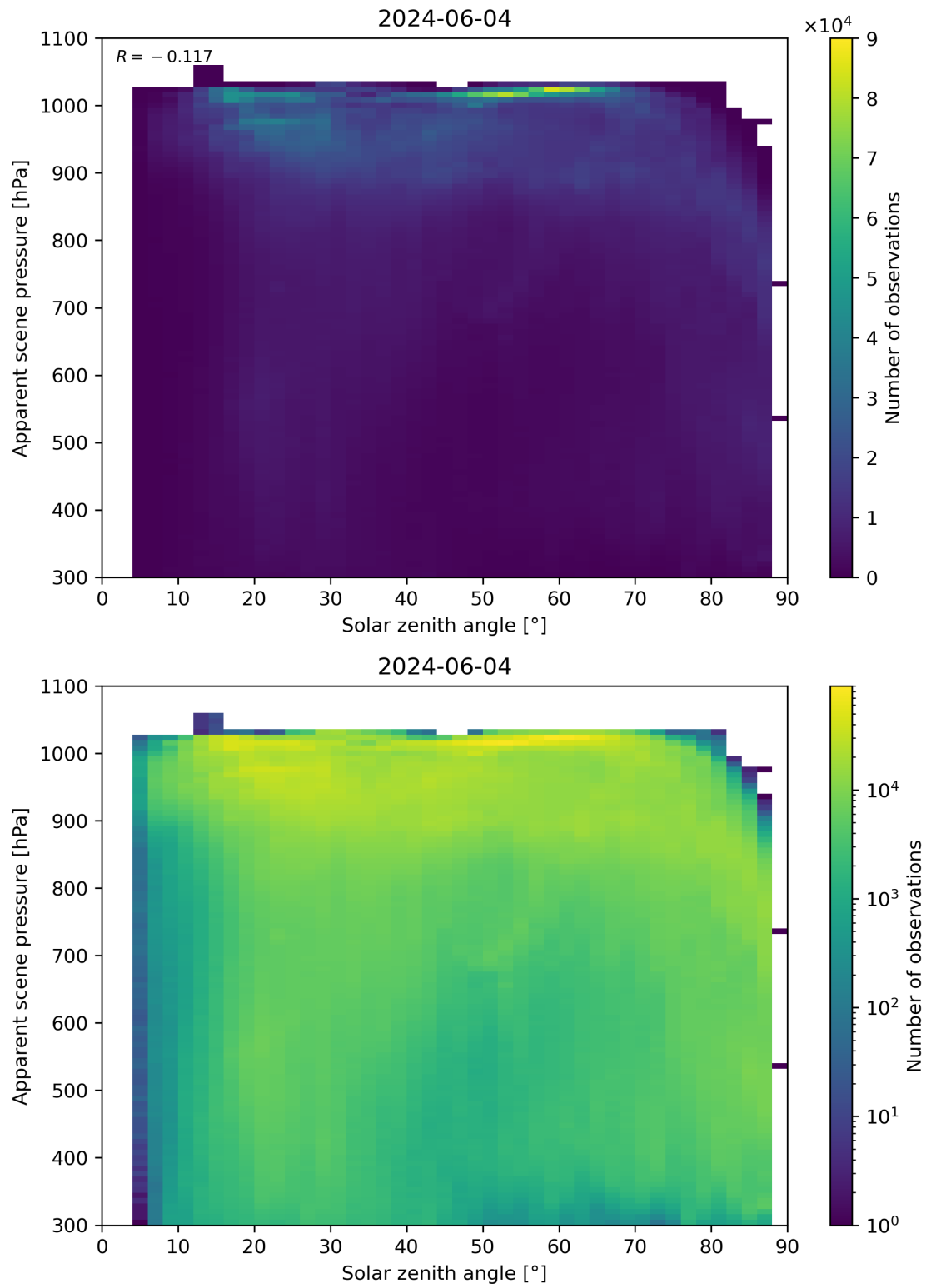
Figure 108: Scatter density plot of “Solar zenith angle” against “Apparent scene pressure” for 2024-06-03 to 2024-06-05.
