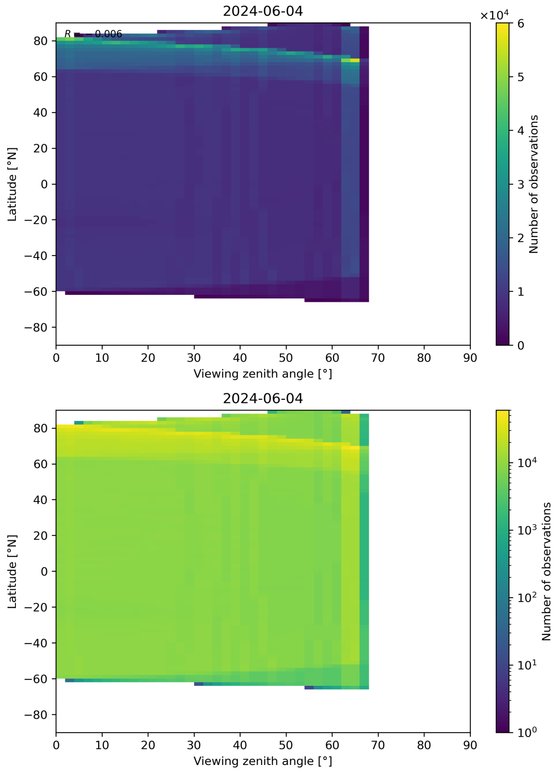
Figure 123: Scatter density plot of “Viewing zenith angle” against “Latitude” for 2024-06-03 to 2024-06-05.
