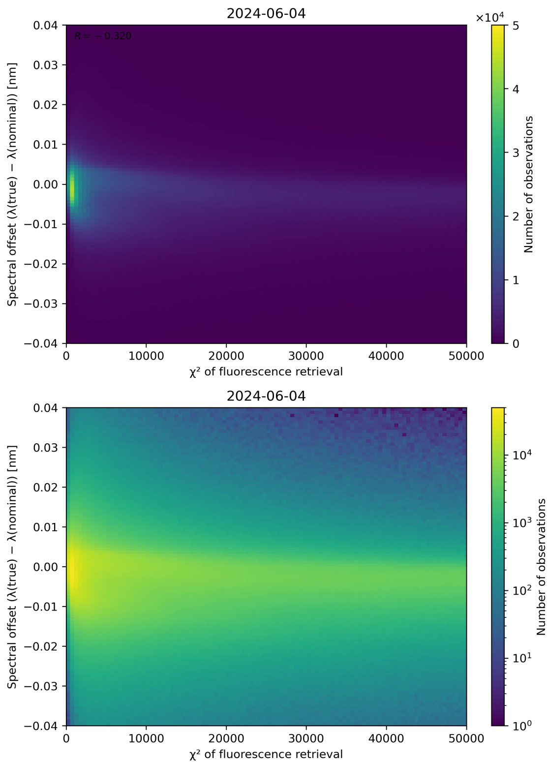
Figure 69: Scatter density plot of " \chi^2 of fluorescence retrieval" against "Spectral offset ( \lambda(\text{true}) - \lambda(\text{nominal})) " for 2024-06-03 to 2024-06-05.
