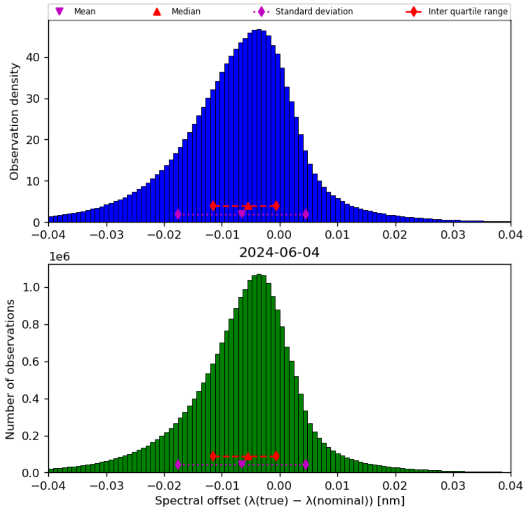
Figure 45: Histogram of “Spectral offset ( \lambda(\text{true}) - \lambda(\text{nominal}) )” for 2024-06-03 to 2024-06-05
