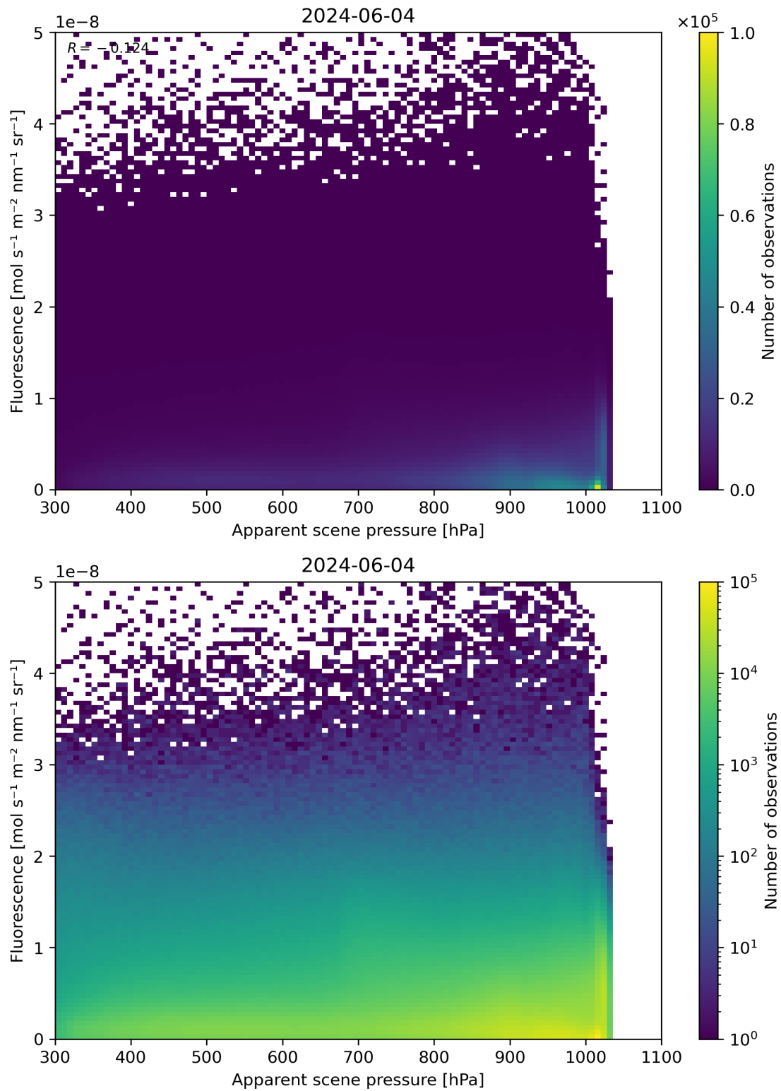
Figure 64: Scatter density plot of “Apparent scene pressure” against “Fluorescence” for 2024-06-03 to 2024-06-05.
