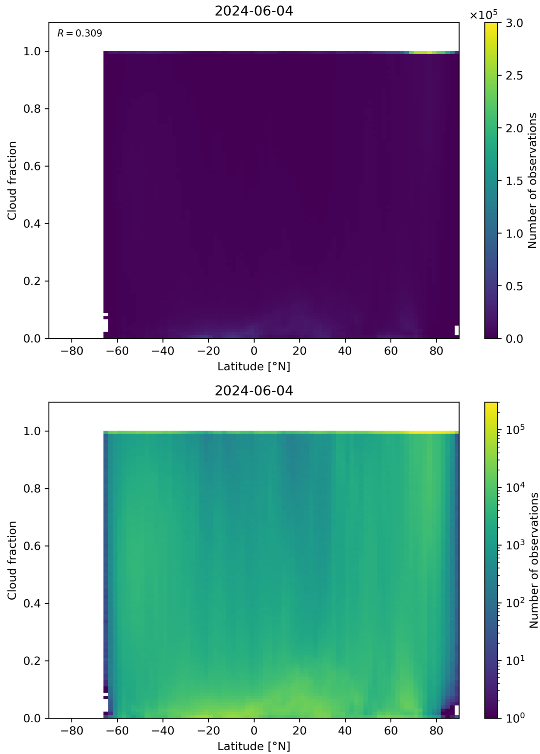
Figure 90: Scatter density plot of “Latitude” against “Cloud fraction” for 2024-06-03 to 2024-06-05.
