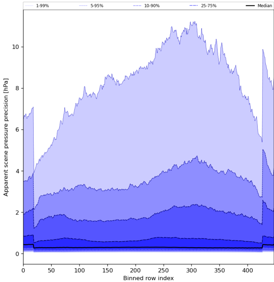
Figure 54: Along track statistics of “Apparent scene pressure precision” for 2024-06-03 to 2024-06-05
