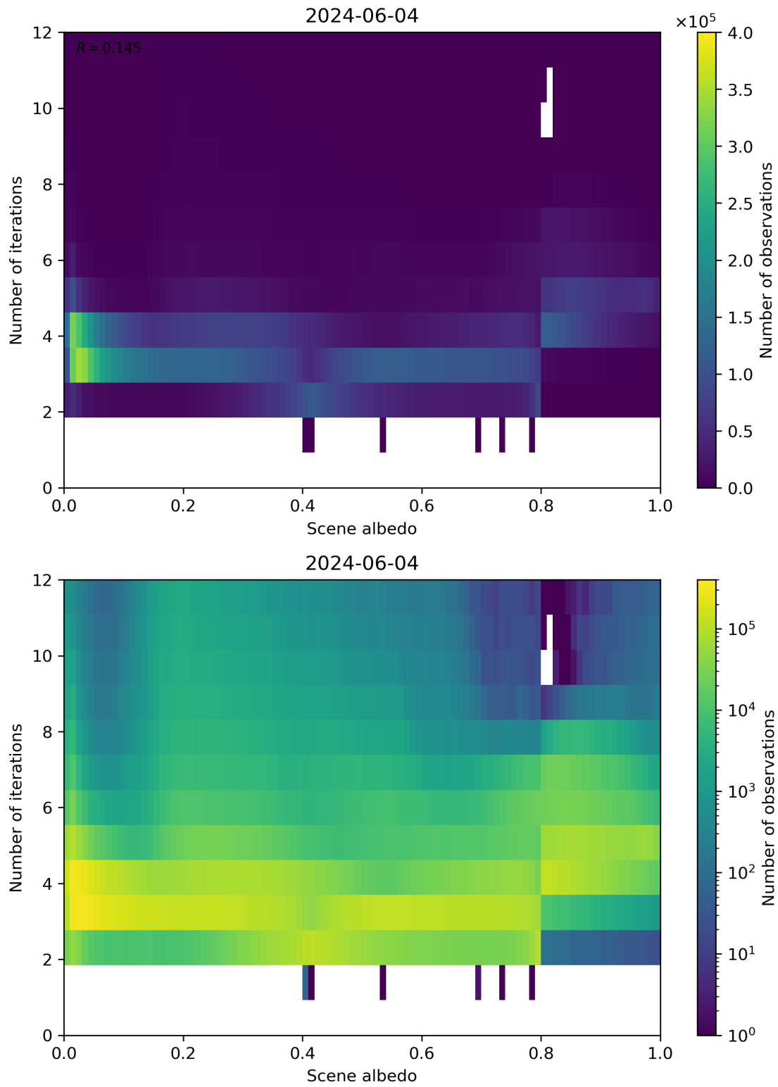
Figure 105: Scatter density plot of “Scene albedo” against “Number of iterations” for 2024-06-03 to 2024-06-05.
