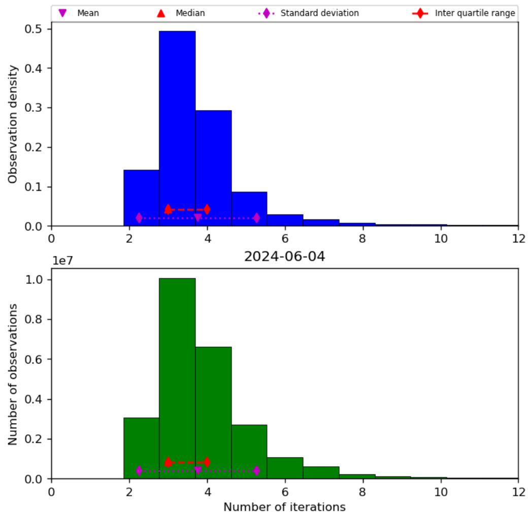
Figure 39: Histogram of “Number of iterations” for 2024-06-03 to 2024-06-05
