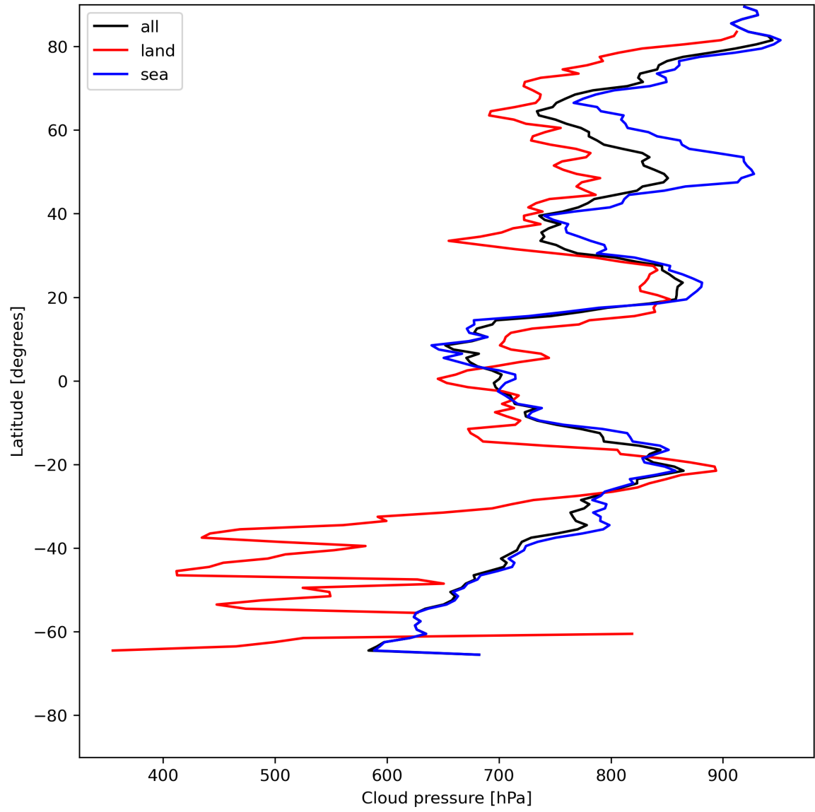
Figure 13: Zonal average of “Cloud pressure” for 2024-06-03 to 2024-06-05.
