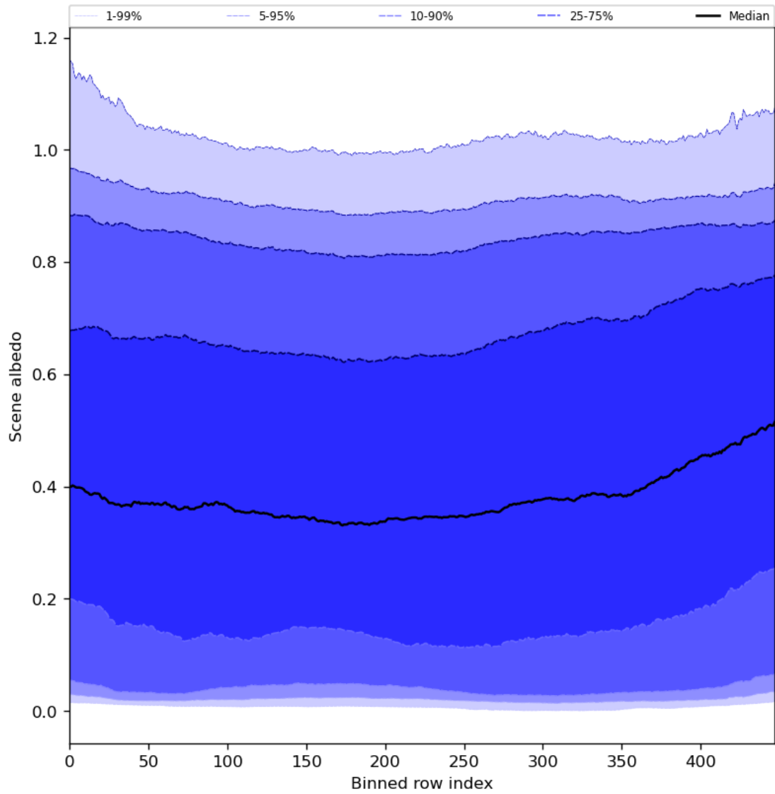
Figure 51: Along track statistics of “Scene albedo” for 2024-06-03 to 2024-06-05
