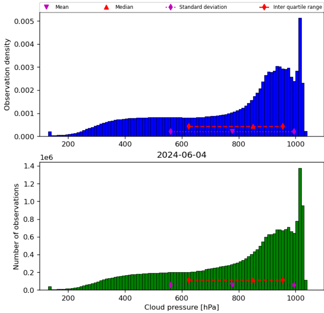
Figure 30: Histogram of “Cloud pressure” for 2024-06-03 to 2024-06-05
