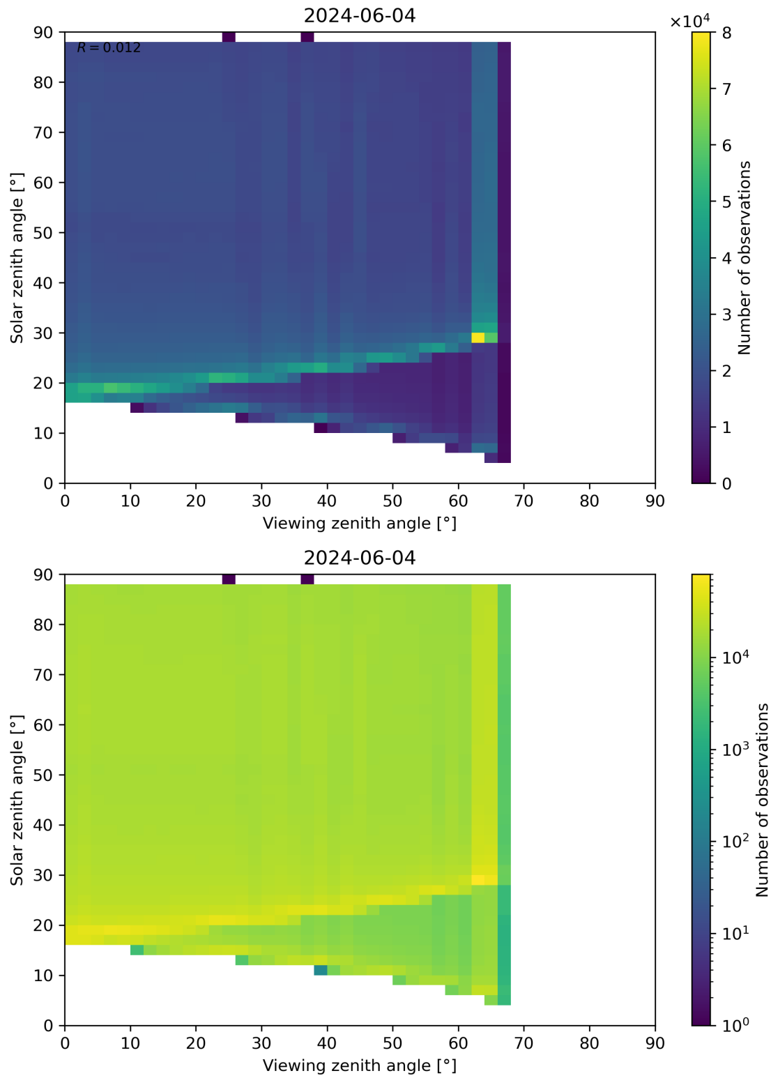
Figure 127: Scatter density plot of “Viewing zenith angle” against “Solar zenith angle” for 2024-06-03 to 2024-06-05.
