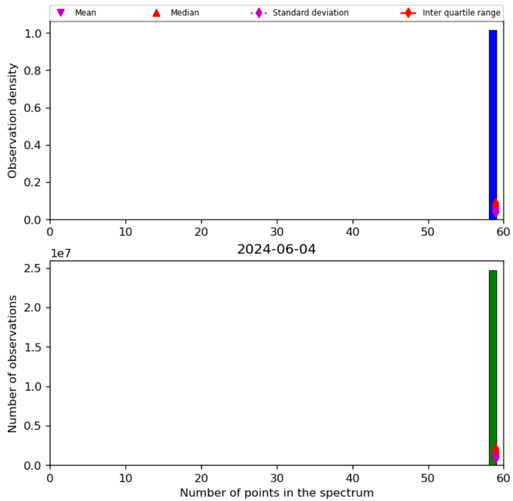
Figure 44: Histogram of “Number of points in the spectrum” for 2024-06-03 to 2024-06-05
