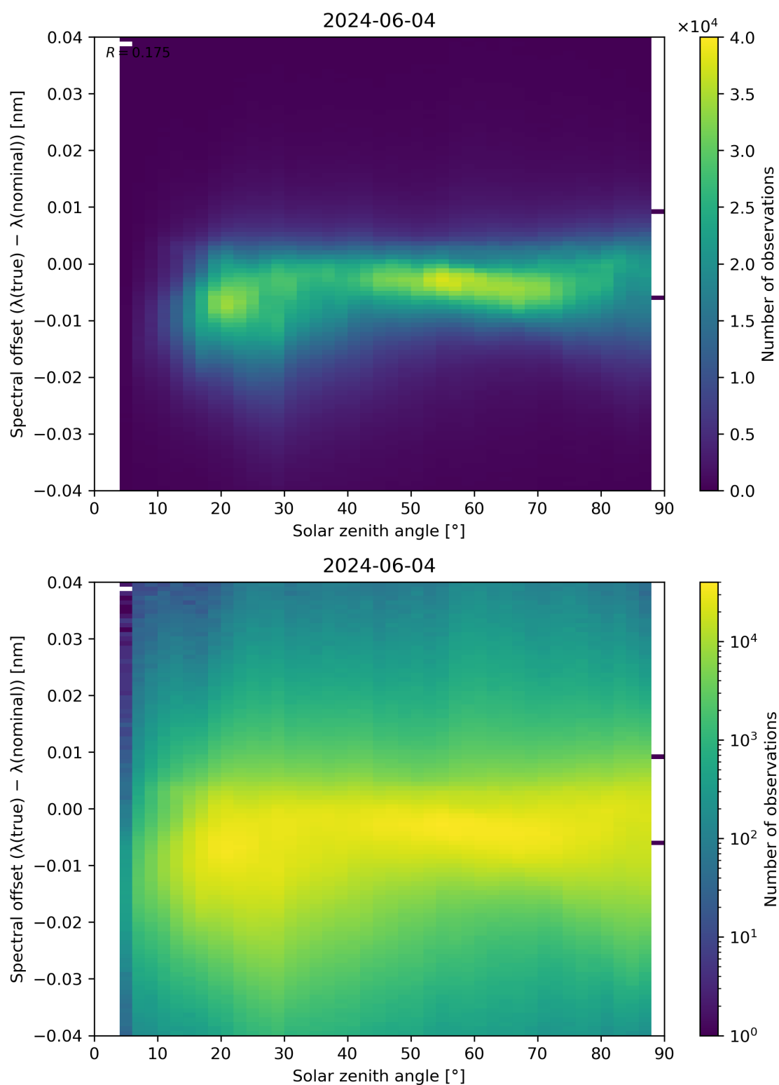
Figure 117: Scatter density plot of “Solar zenith angle” against “Spectral offset ( \lambda(\text{true}) - \lambda(\text{nominal}) )” for 2024-06-03 to 2024-06-05.
