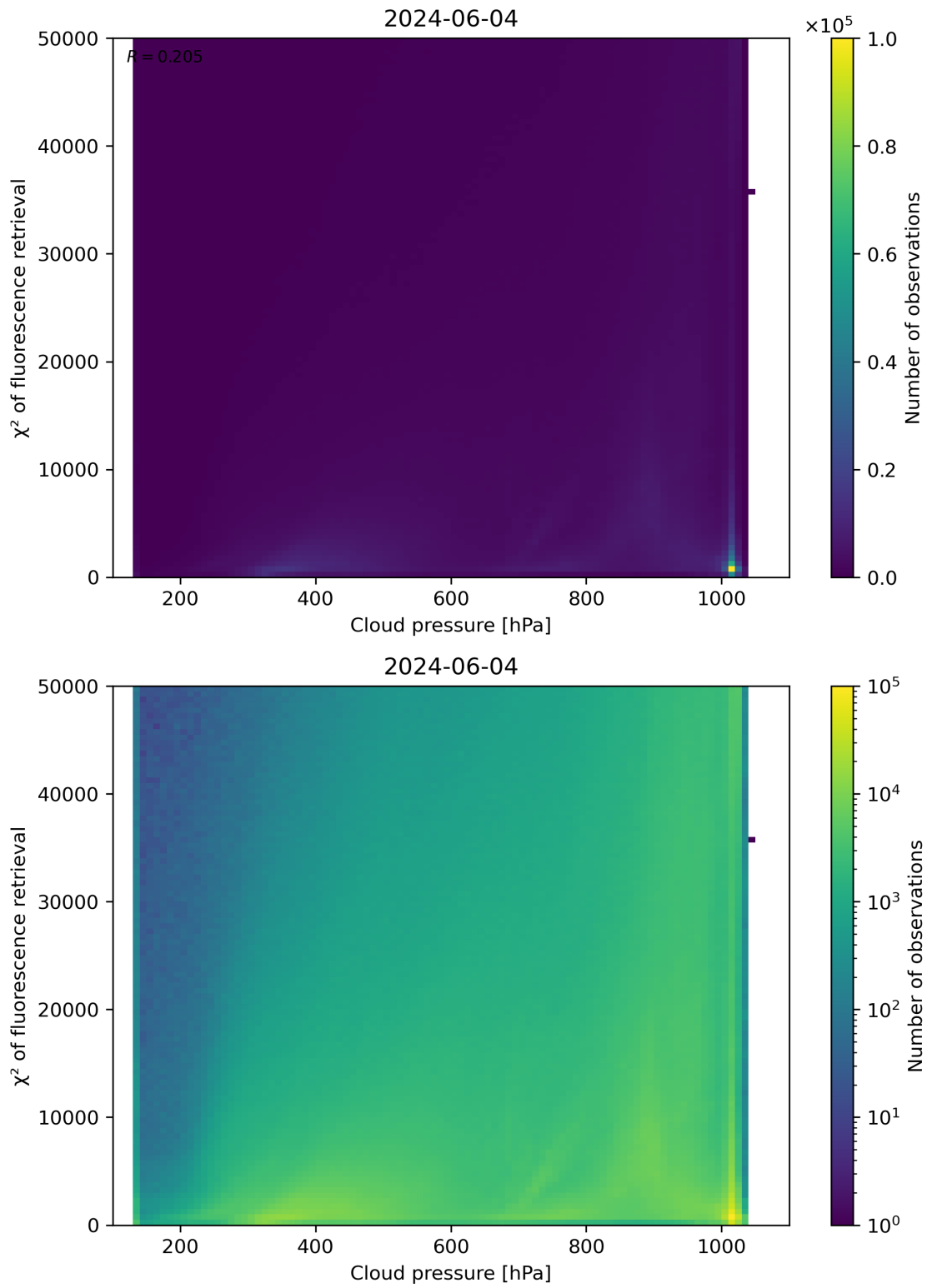
Figure 78: Scatter density plot of “Cloud pressure” against “ \chi^2 of fluorescence retrieval” for 2024-06-03 to 2024-06-05.
