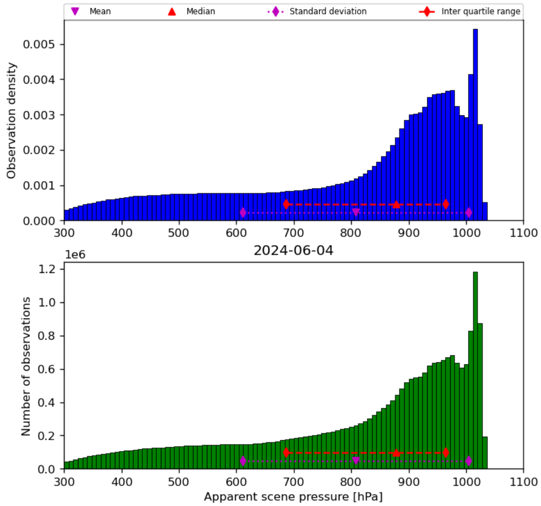
Figure 36: Histogram of “Apparent scene pressure” for 2024-06-03 to 2024-06-05
