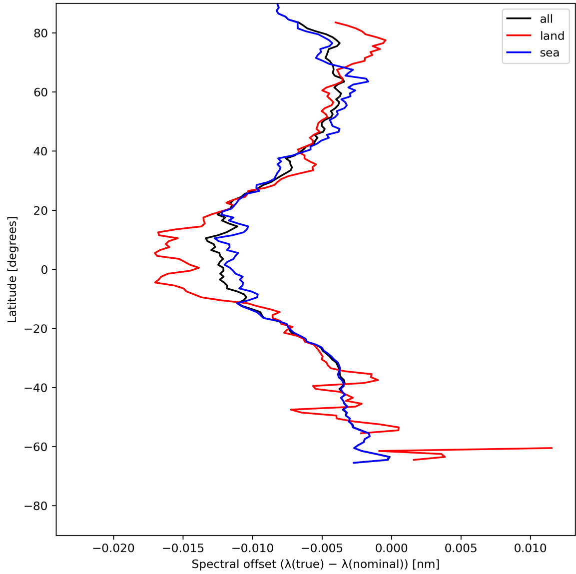
Figure 28: Zonal average of “Spectral offset ( \lambda(\text{true}) - \lambda(\text{nominal}) )” for 2024-06-03 to 2024-06-05.
