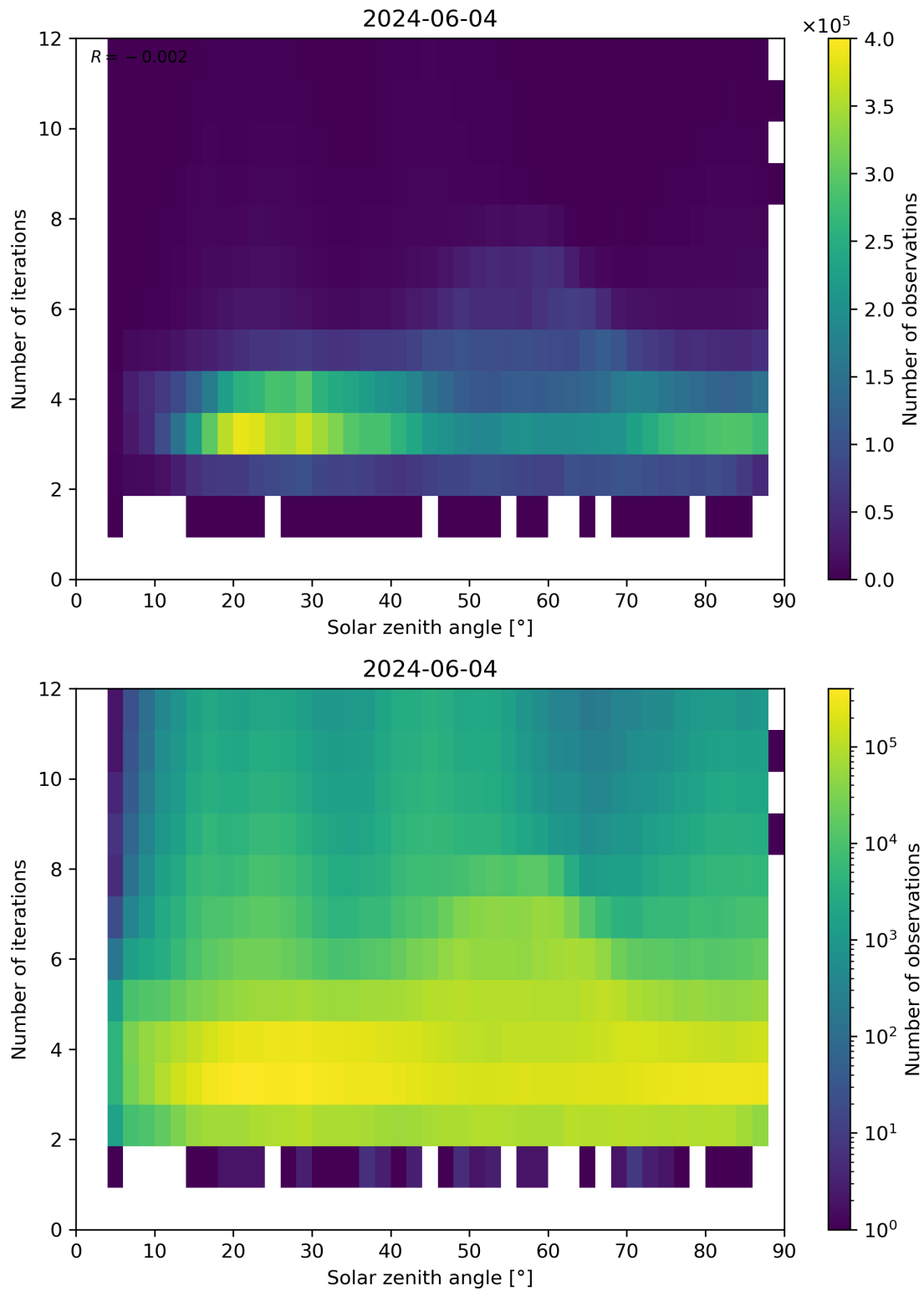
Figure 114: Scatter density plot of “Solar zenith angle” against “Number of iterations” for 2024-06-03 to 2024-06-05.
