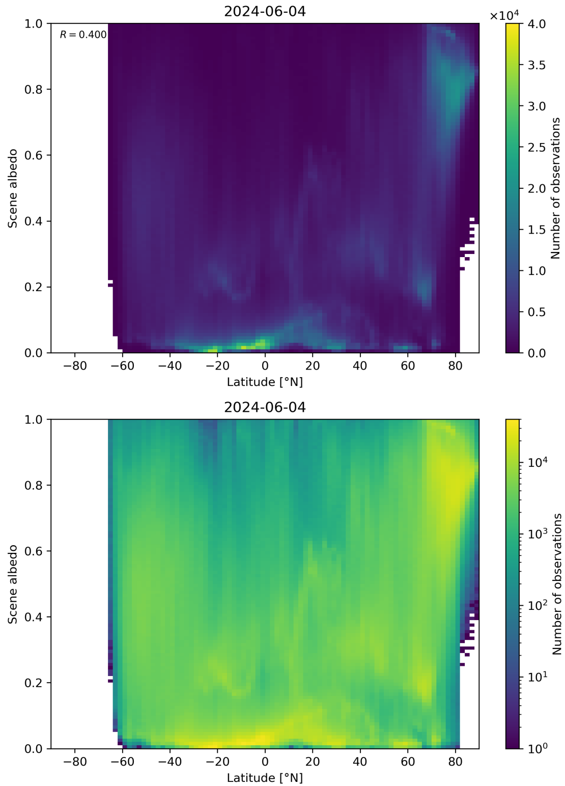
Figure 95: Scatter density plot of “Latitude” against “Scene albedo” for 2024-06-03 to 2024-06-05.
