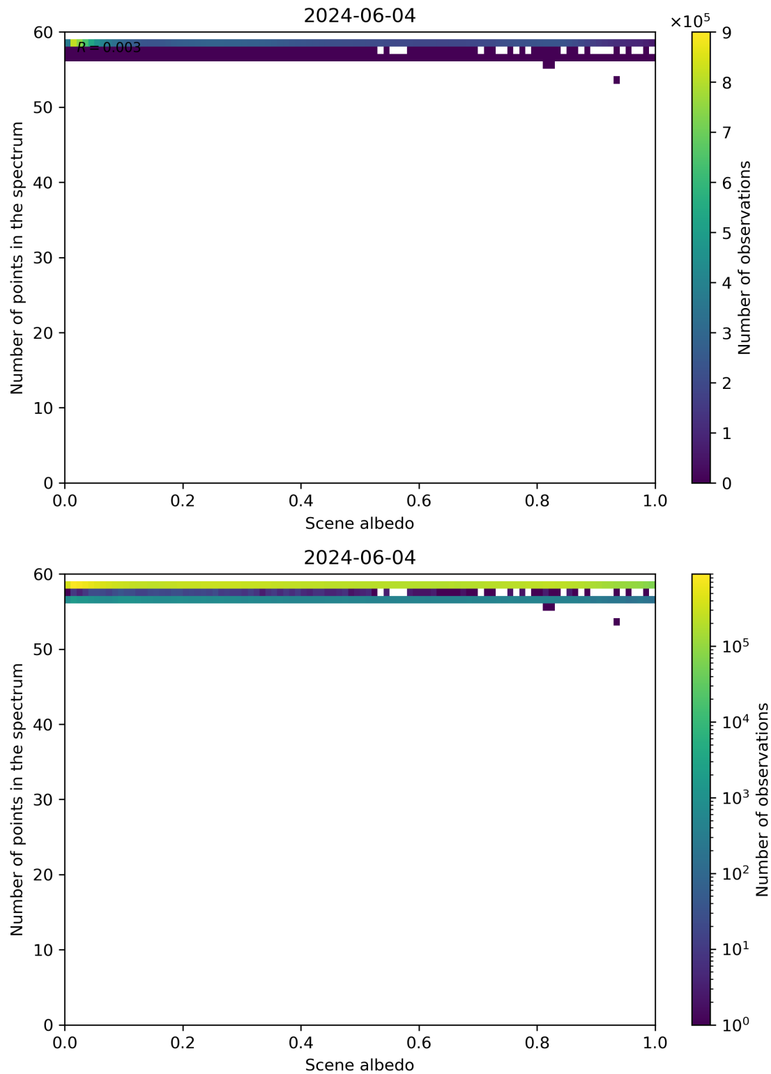
Figure 106: Scatter density plot of “Scene albedo” against “Number of points in the spectrum” for 2024-06-03 to 2024-06-05.
