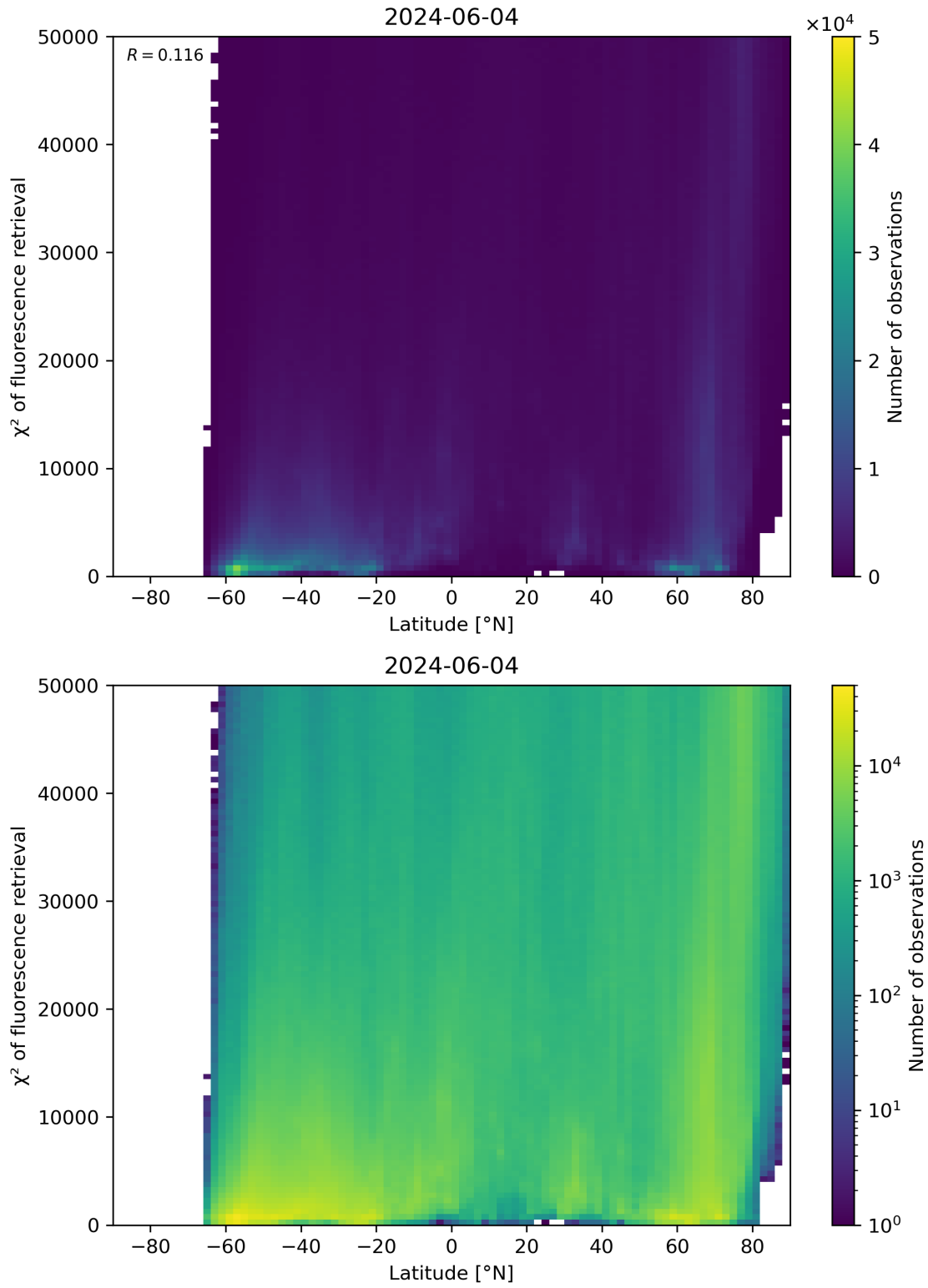
Figure 89: Scatter density plot of “Latitude” against “ \chi^2 of fluorescence retrieval” for 2024-06-03 to 2024-06-05.
