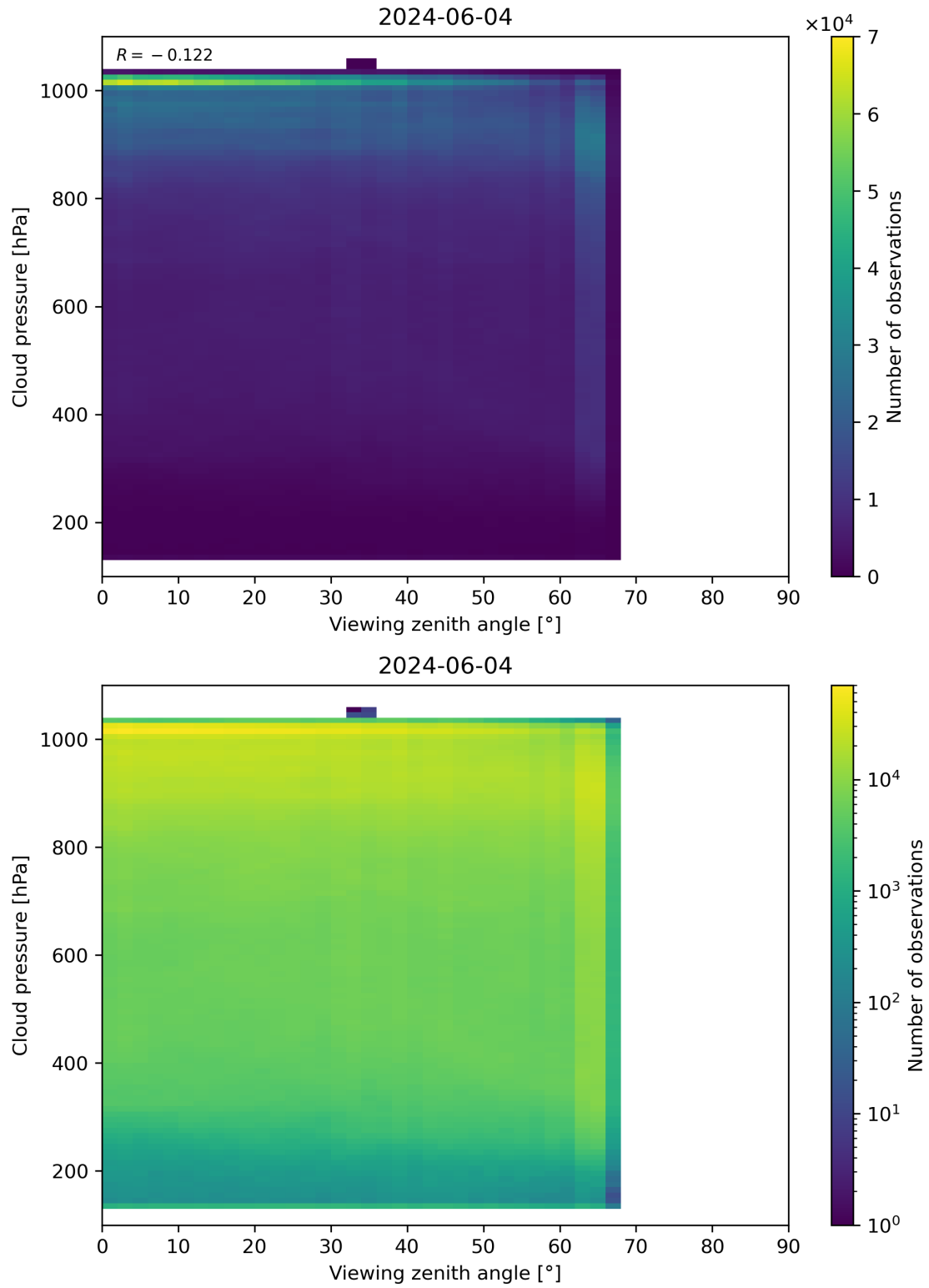
Figure 121: Scatter density plot of “Viewing zenith angle” against “Cloud pressure” for 2024-06-03 to 2024-06-05.
