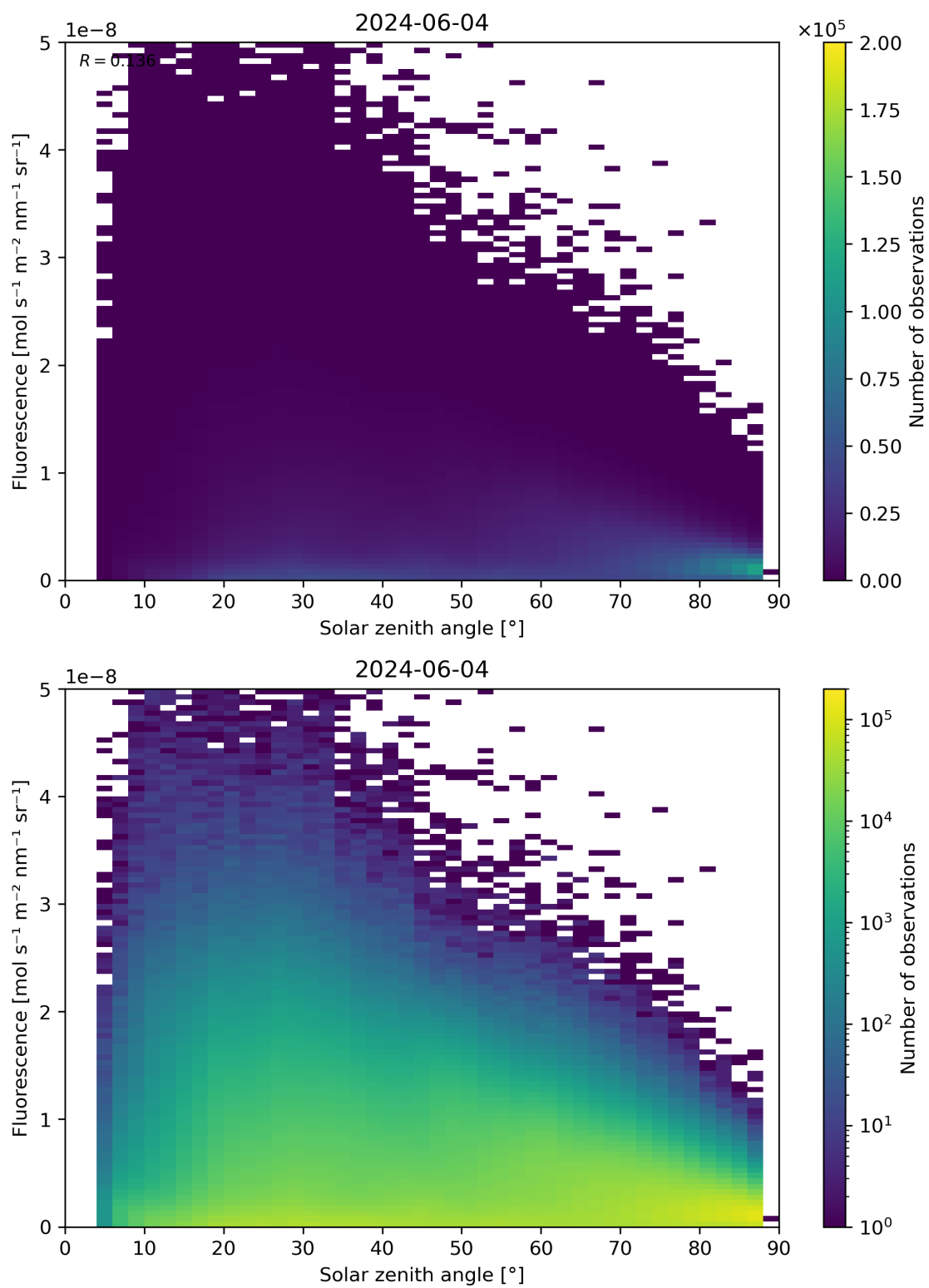
Figure 112: Scatter density plot of “Solar zenith angle” against “Fluorescence” for 2024-06-03 to 2024-06-05.
