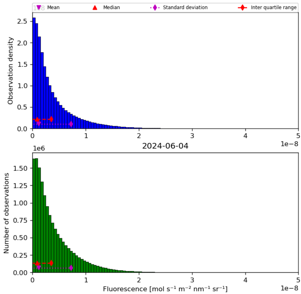
Figure 40: Histogram of “Fluorescence” for 2024-06-03 to 2024-06-05
