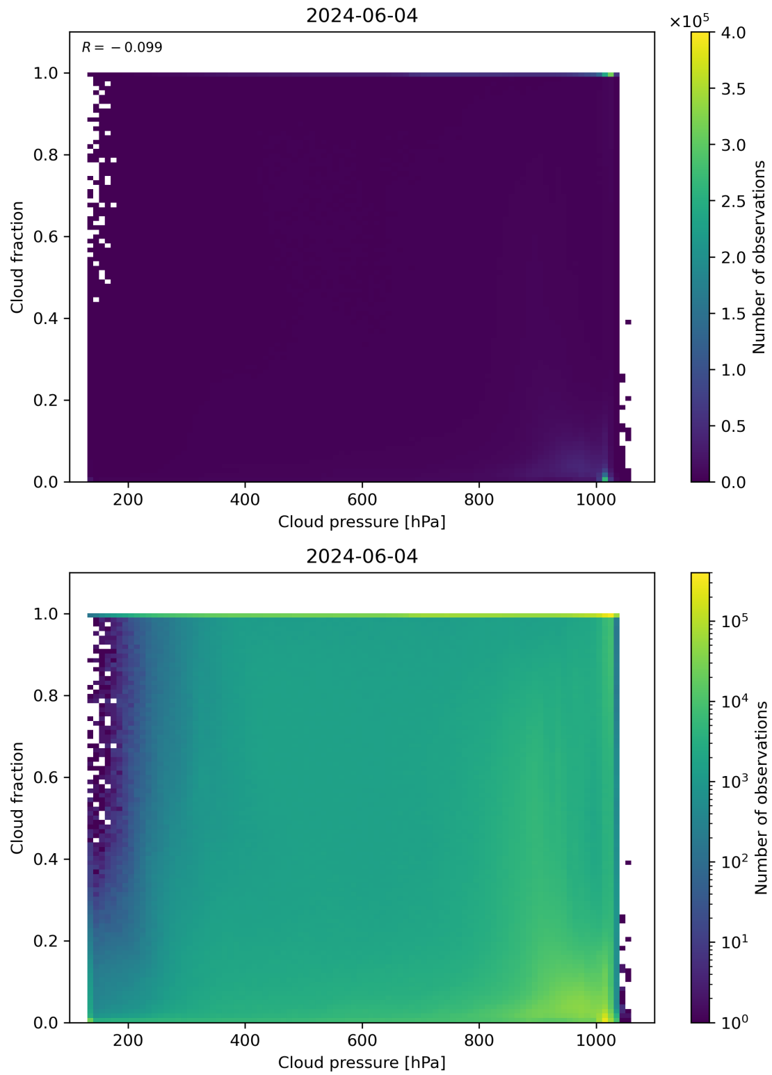
Figure 79: Scatter density plot of “Cloud pressure” against “Cloud fraction” for 2024-06-03 to 2024-06-05.
