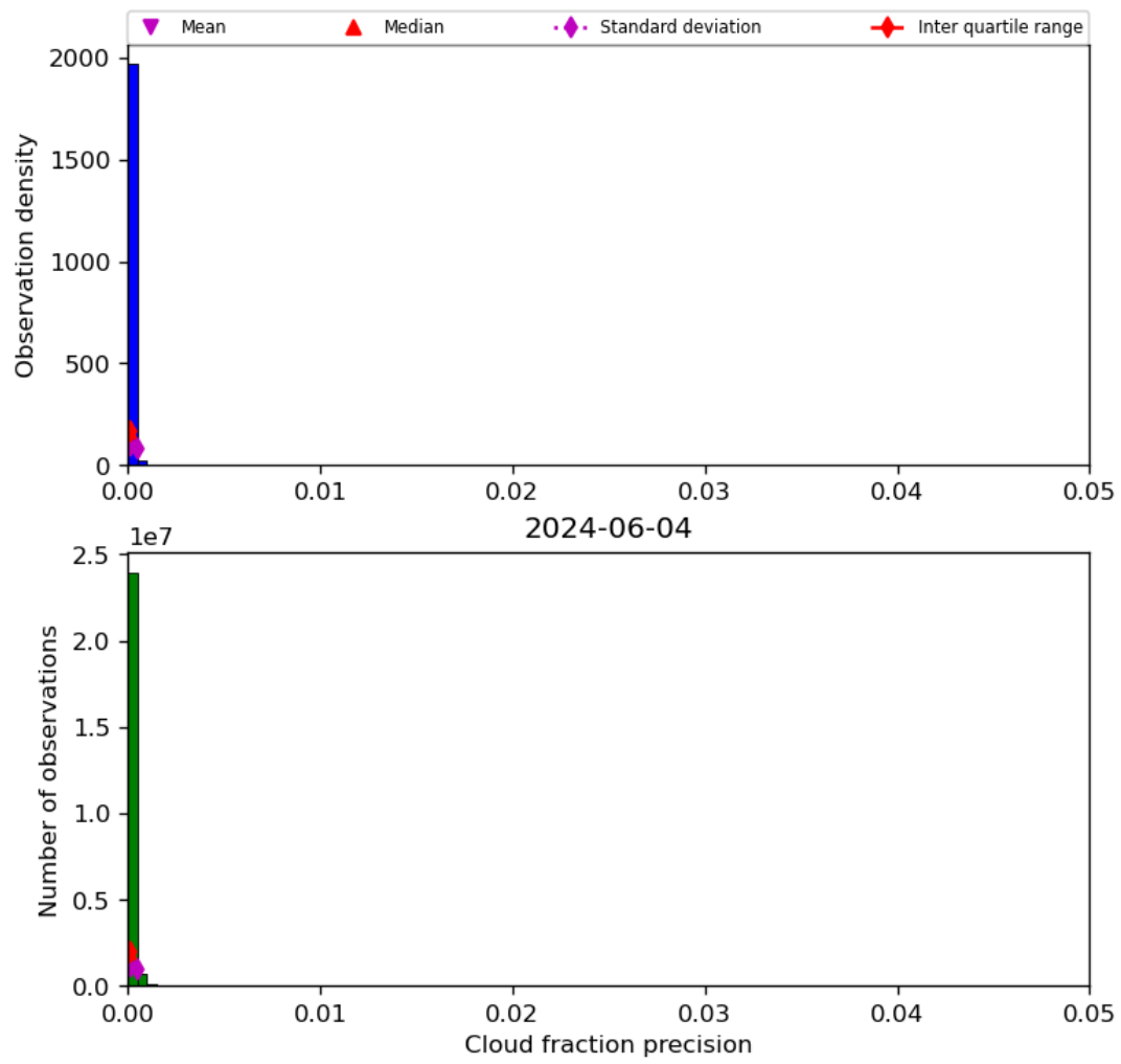
Figure 33: Histogram of “Cloud fraction precision” for 2024-06-03 to 2024-06-05
