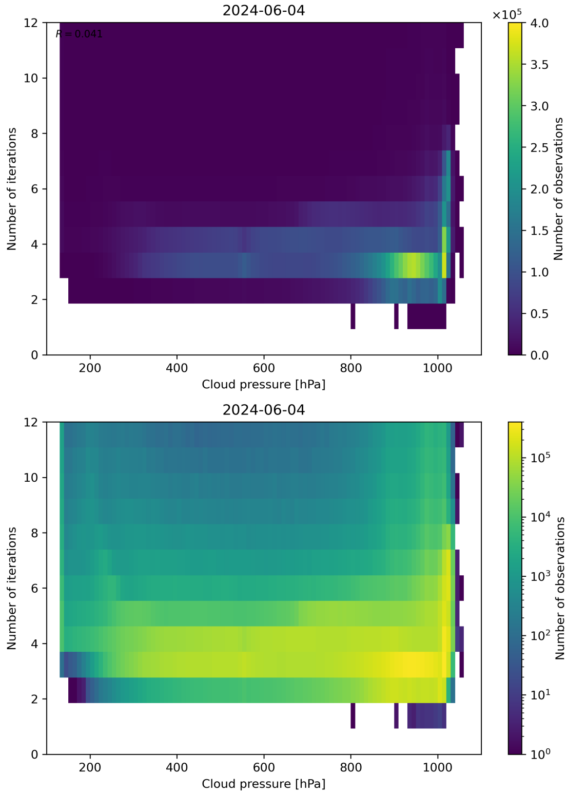
Figure 81: Scatter density plot of “Cloud pressure” against “Number of iterations” for 2024-06-03 to 2024-06-05.
