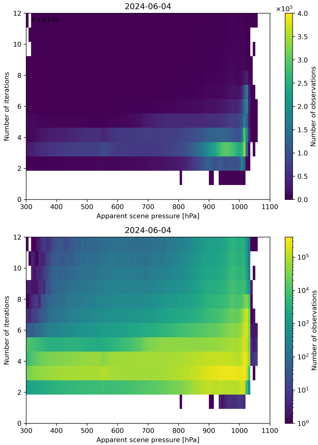
Figure 65: Scatter density plot of “Apparent scene pressure” against “Number of iterations” for 2024-06-03 to 2024-06-05.
