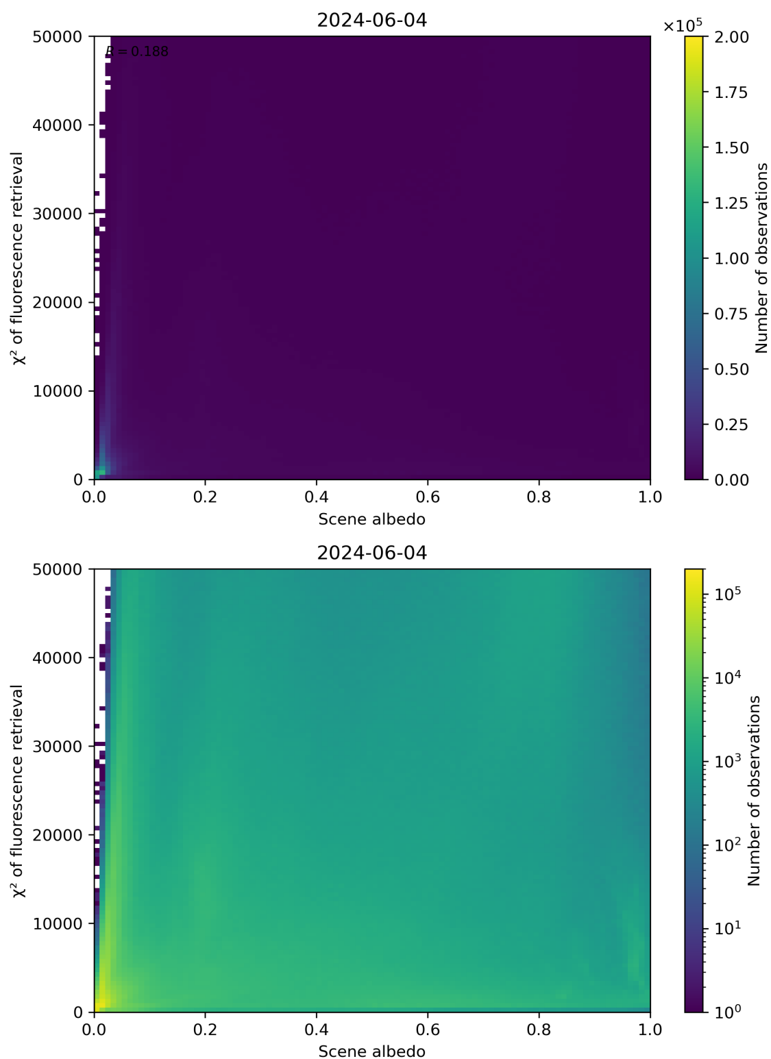
Figure 103: Scatter density plot of “Scene albedo” against “ \chi^2 of fluorescence retrieval” for 2024-06-03 to 2024-06-05.
