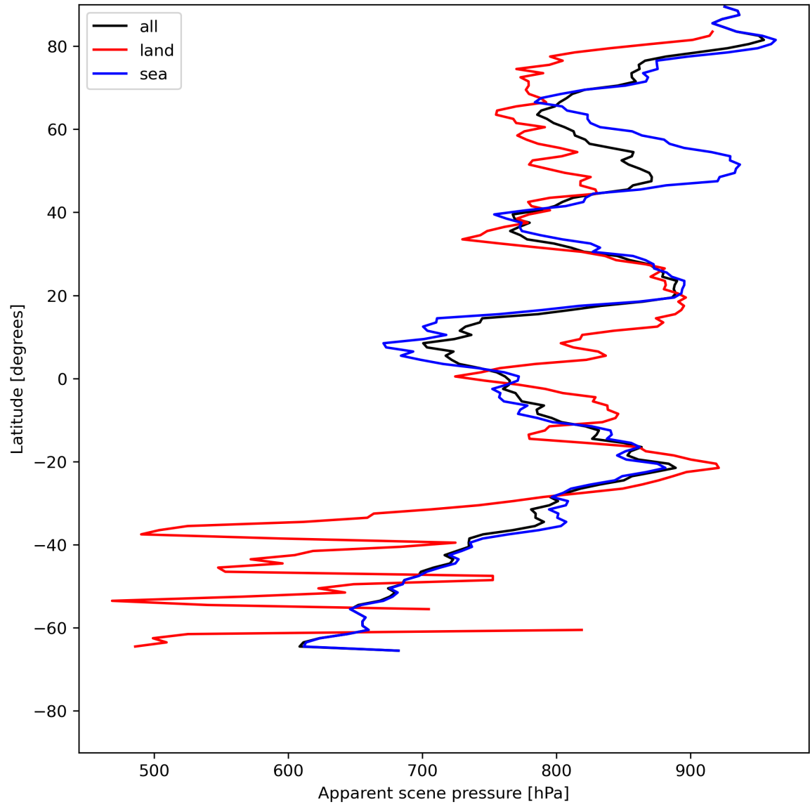
Figure 19: Zonal average of “Apparent scene pressure” for 2024-06-03 to 2024-06-05.
