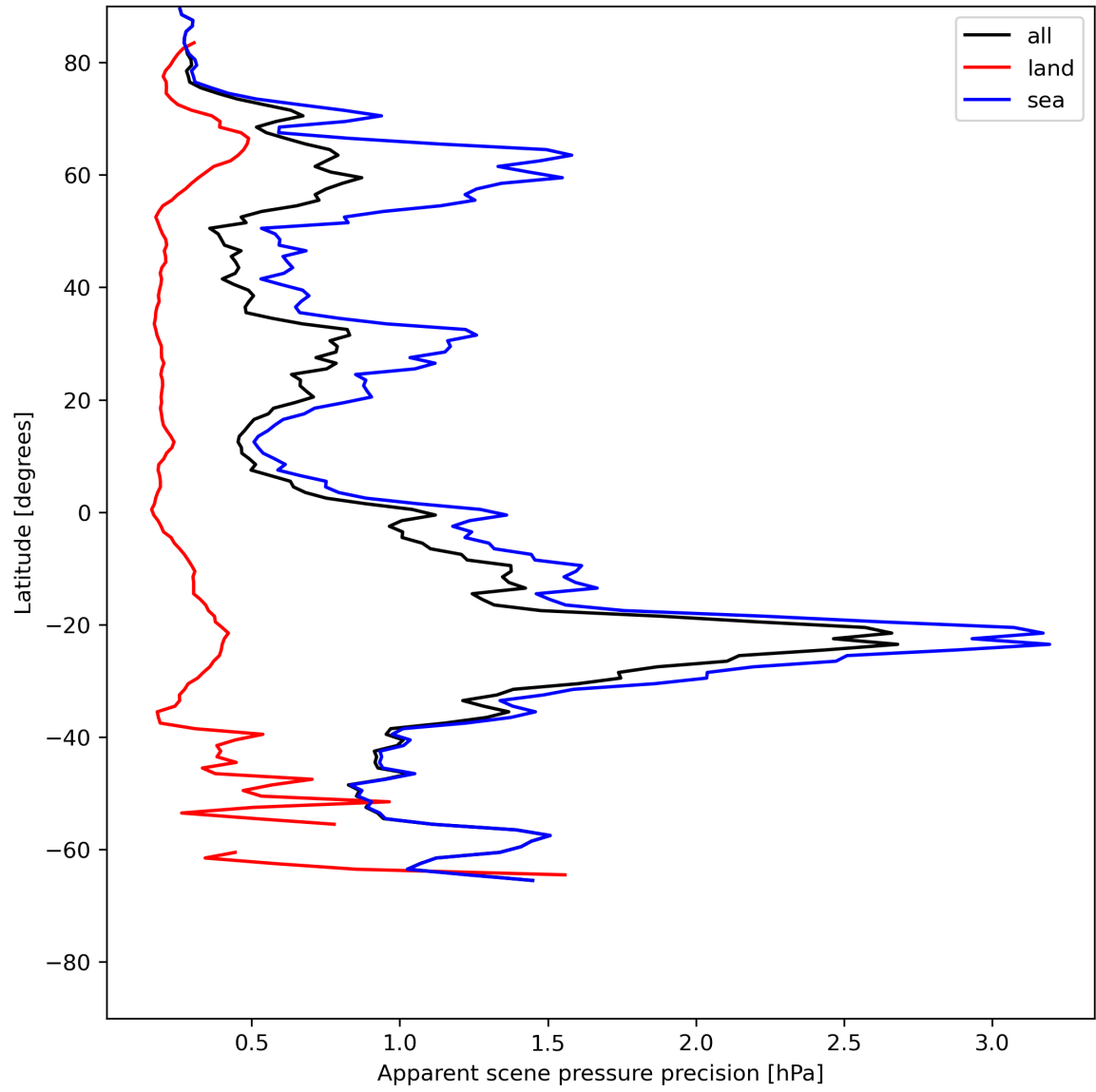
Figure 20: Zonal average of “Apparent scene pressure precision” for 2024-06-03 to 2024-06-05.
