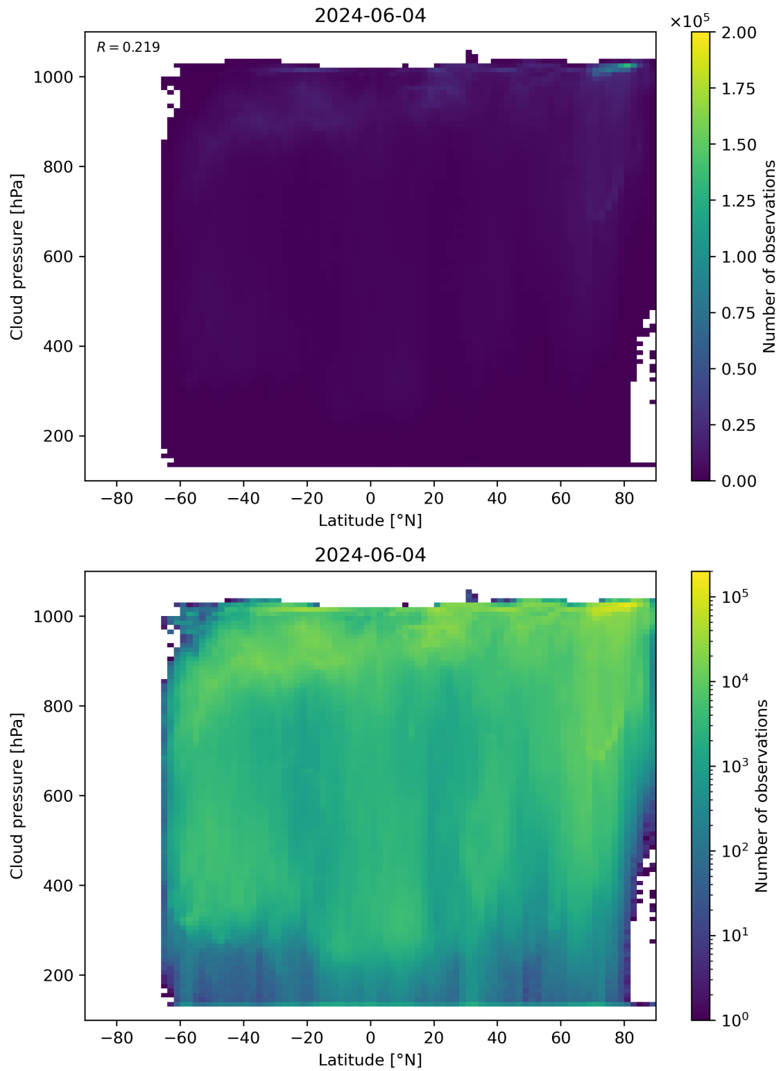
Figure 91: Scatter density plot of “Latitude” against “Cloud pressure” for 2024-06-03 to 2024-06-05.
