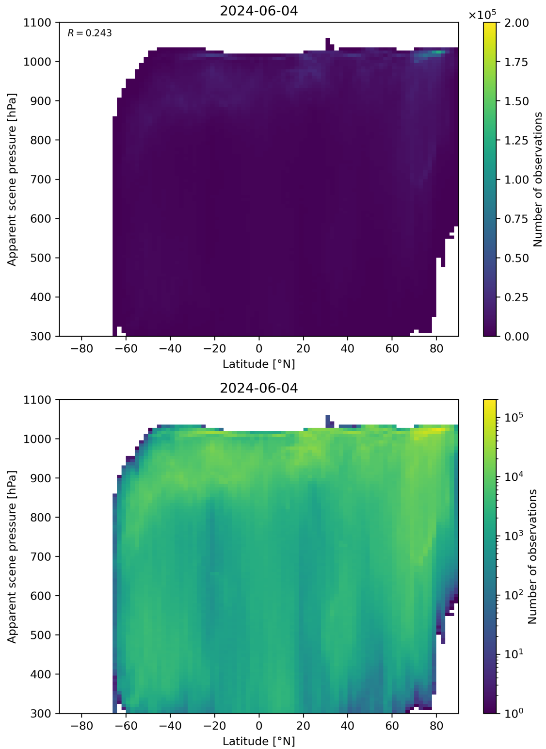
Figure 88: Scatter density plot of “Latitude” against “Apparent scene pressure” for 2024-06-03 to 2024-06-05.
