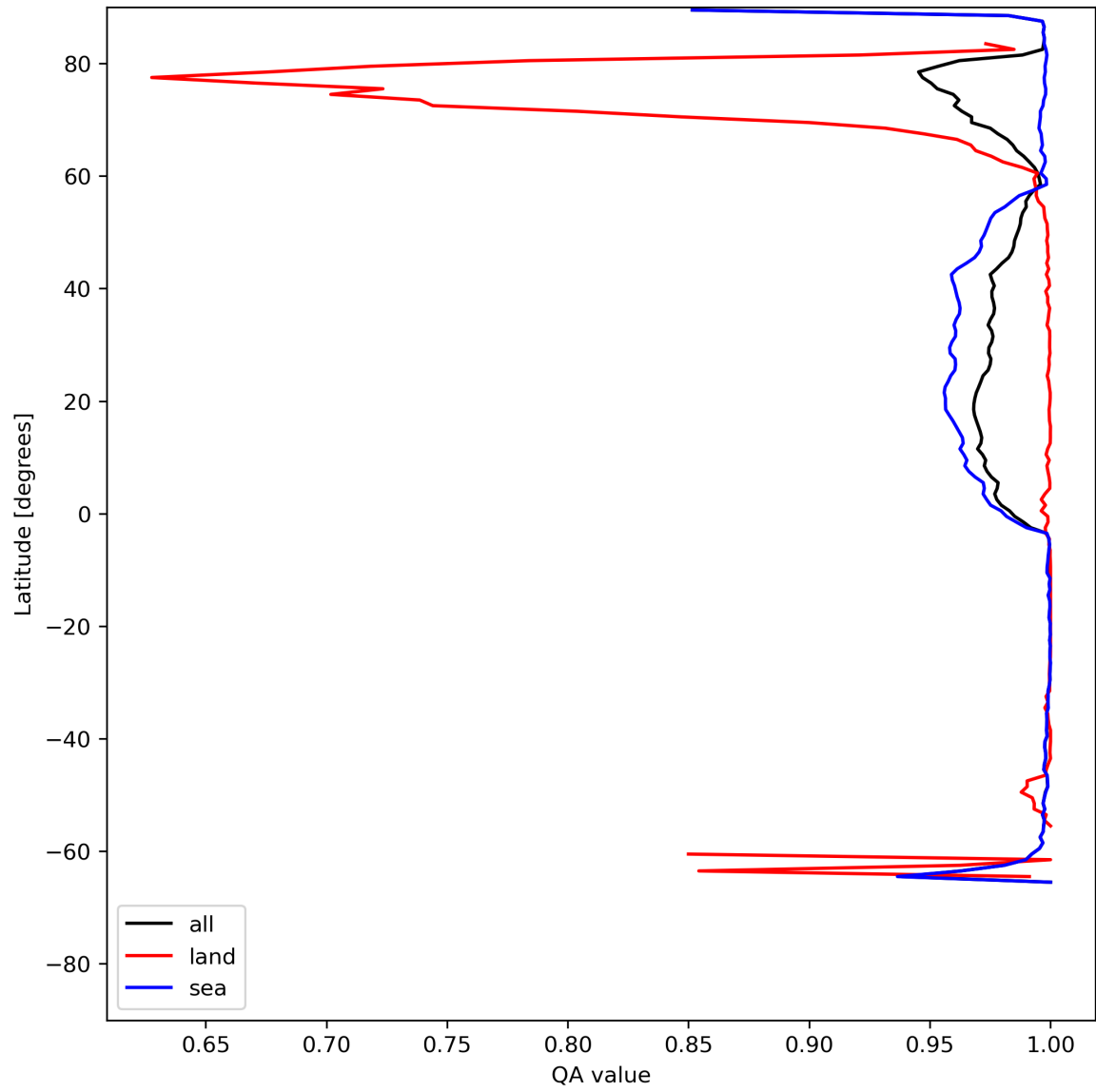
Figure 12: Zonal average of “QA value” for 2024-06-03 to 2024-06-05.
