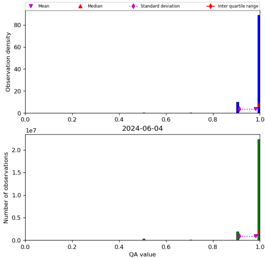
Figure 29: Histogram of “QA value” for 2024-06-03 to 2024-06-05
