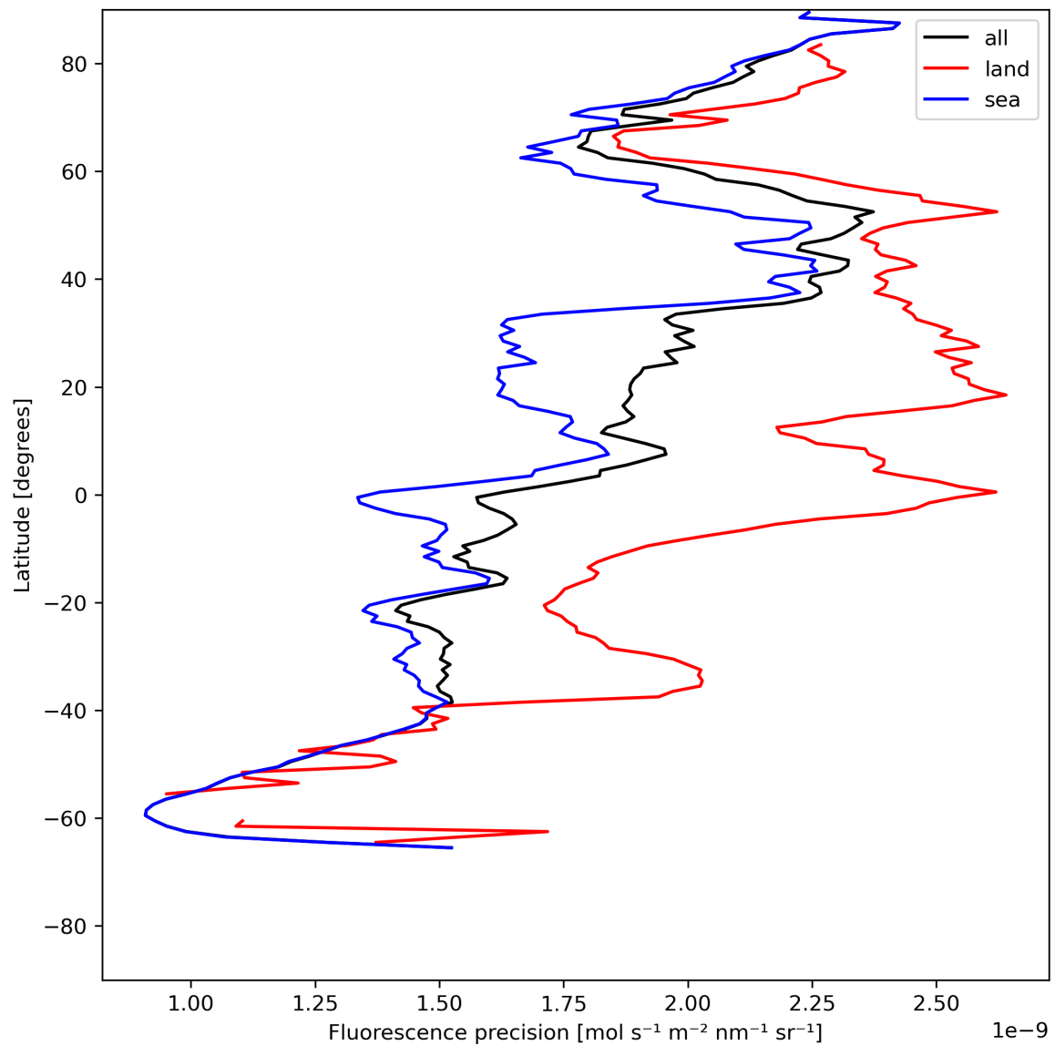
Figure 24: Zonal average of “Fluorescence precision” for 2024-06-03 to 2024-06-05.
