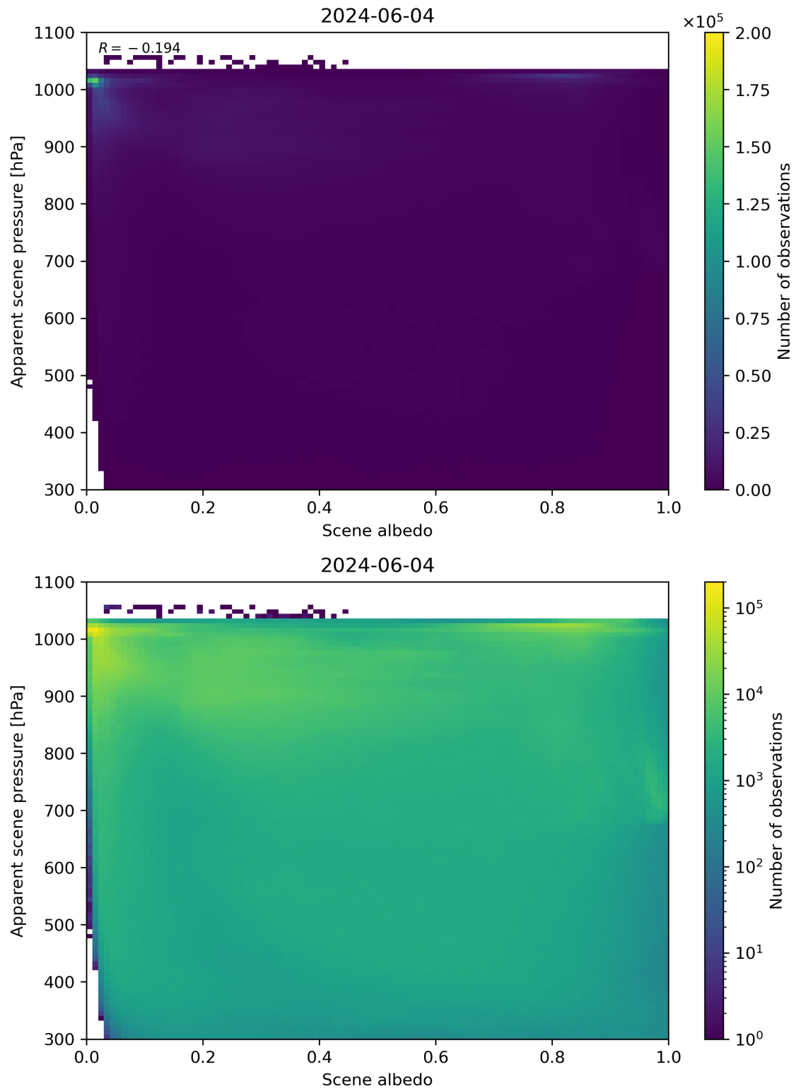
Figure 102: Scatter density plot of “Scene albedo” against “Apparent scene pressure” for 2024-06-03 to 2024-06-05.
