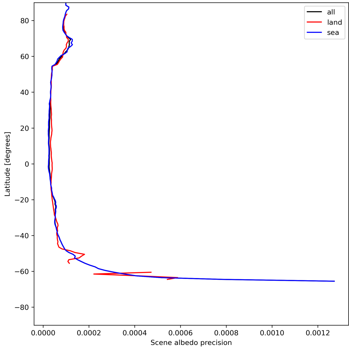
Figure 18: Zonal average of “Scene albedo precision” for 2024-06-03 to 2024-06-05.
