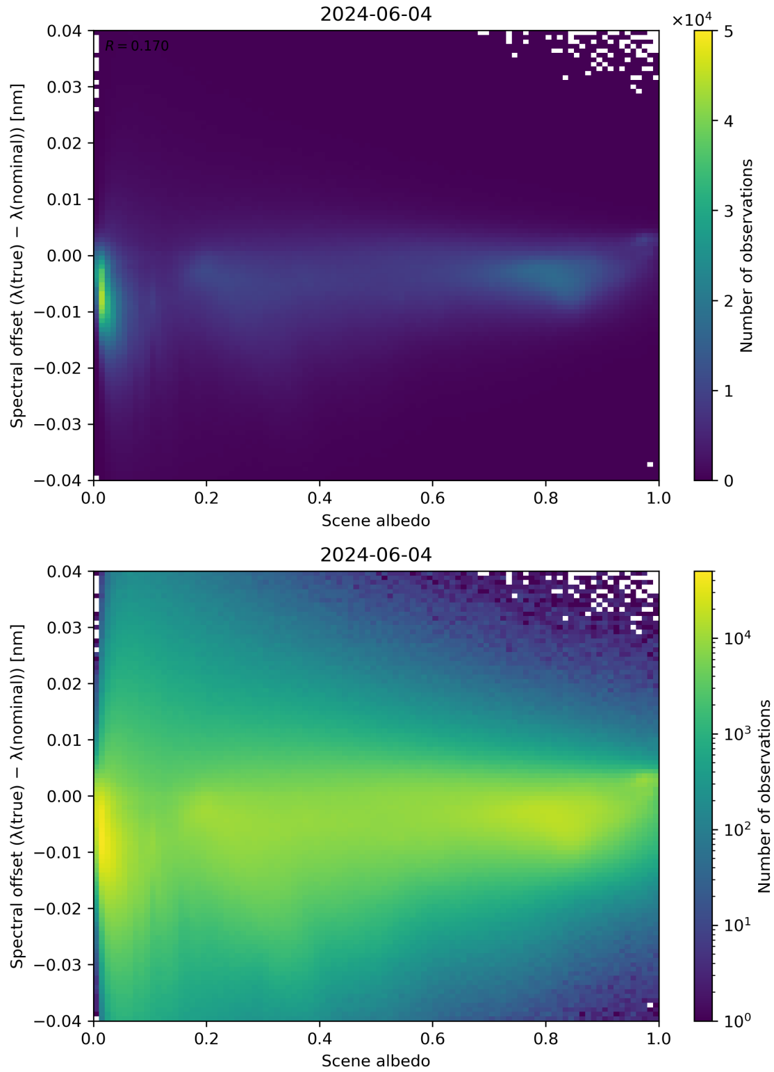
Figure 107: Scatter density plot of “Scene albedo” against “Spectral offset ( \lambda(\text{true}) - \lambda(\text{nominal}) )” for 2024-06-03 to 2024-06-05.
