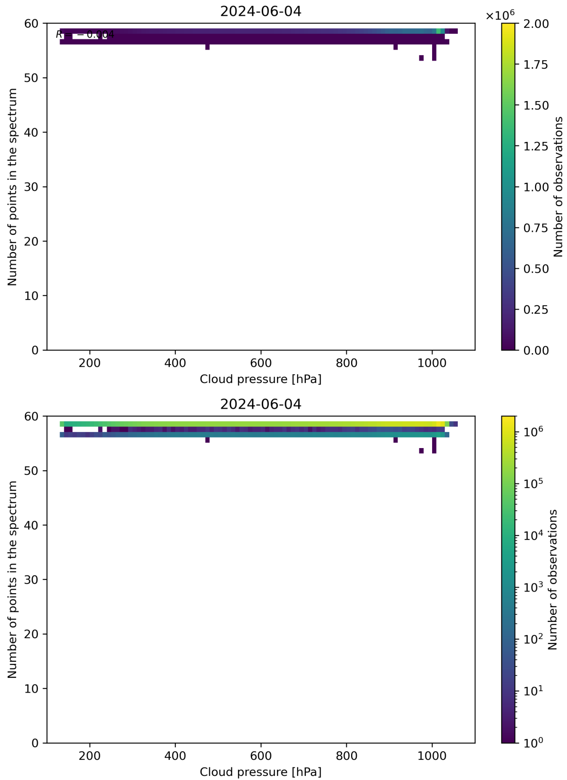
Figure 82: Scatter density plot of “Cloud pressure” against “Number of points in the spectrum” for 2024-06-03 to 2024-06-05.
