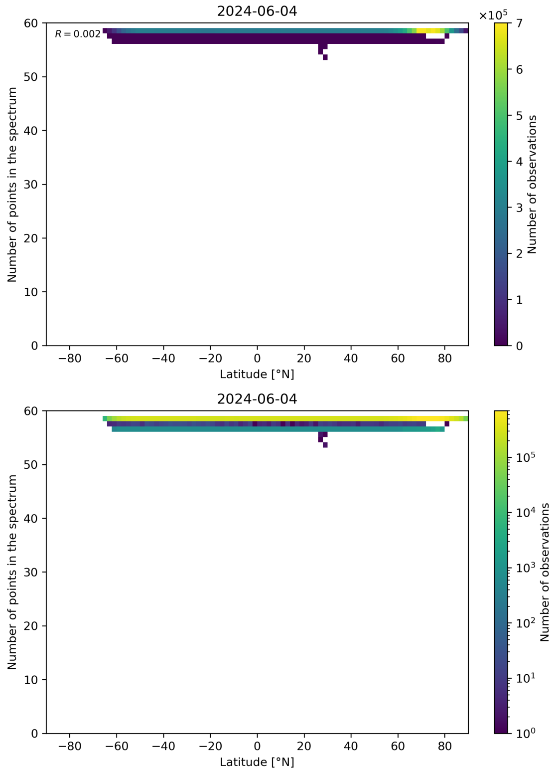
Figure 94: Scatter density plot of “Latitude” against “Number of points in the spectrum” for 2024-06-03 to 2024-06-05.
