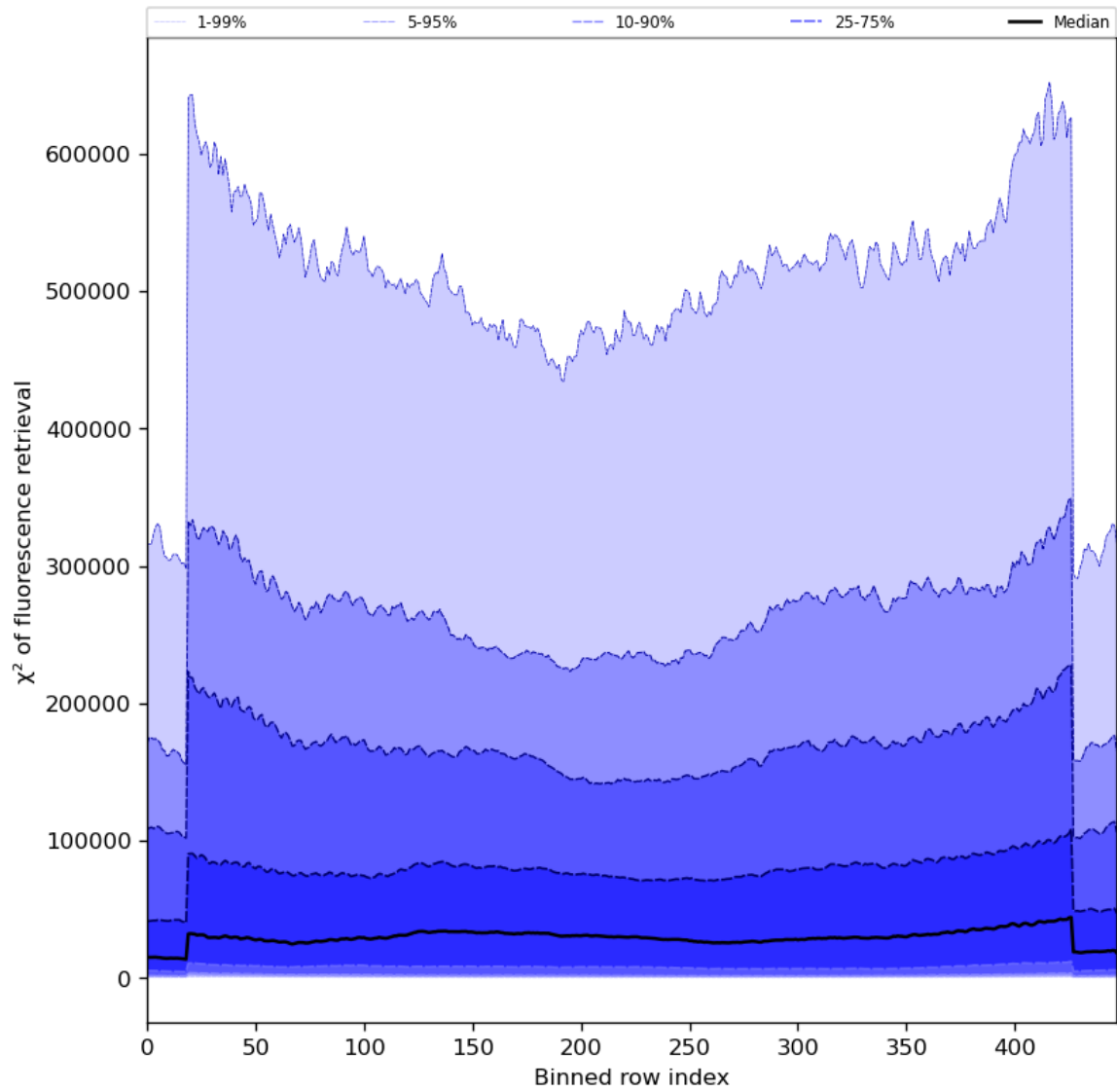
Figure 59: Along track statistics of “ \chi^2 of fluorescence retrieval” for 2024-06-03 to 2024-06-05
