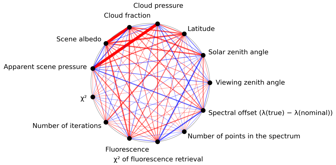
Figure 1: Map of correlation graph for 2024-06-03 to 2024-06-05.
