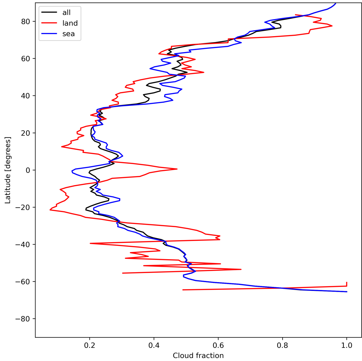
Figure 15: Zonal average of “Cloud fraction” for 2024-06-03 to 2024-06-05.
