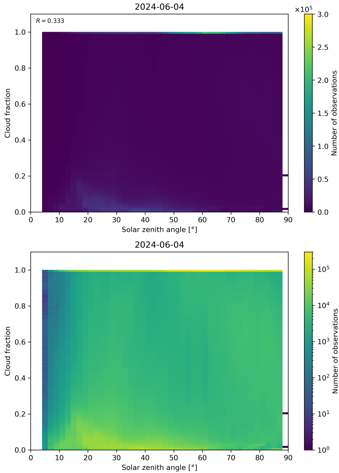
Figure 110: Scatter density plot of “Solar zenith angle” against “Cloud fraction” for 2024-06-03 to 2024-06-05.
