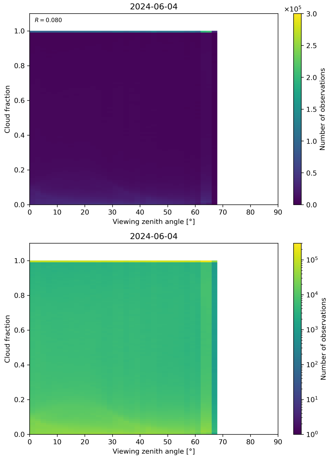
Figure 120: Scatter density plot of “Viewing zenith angle” against “Cloud fraction” for 2024-06-03 to 2024-06-05.
