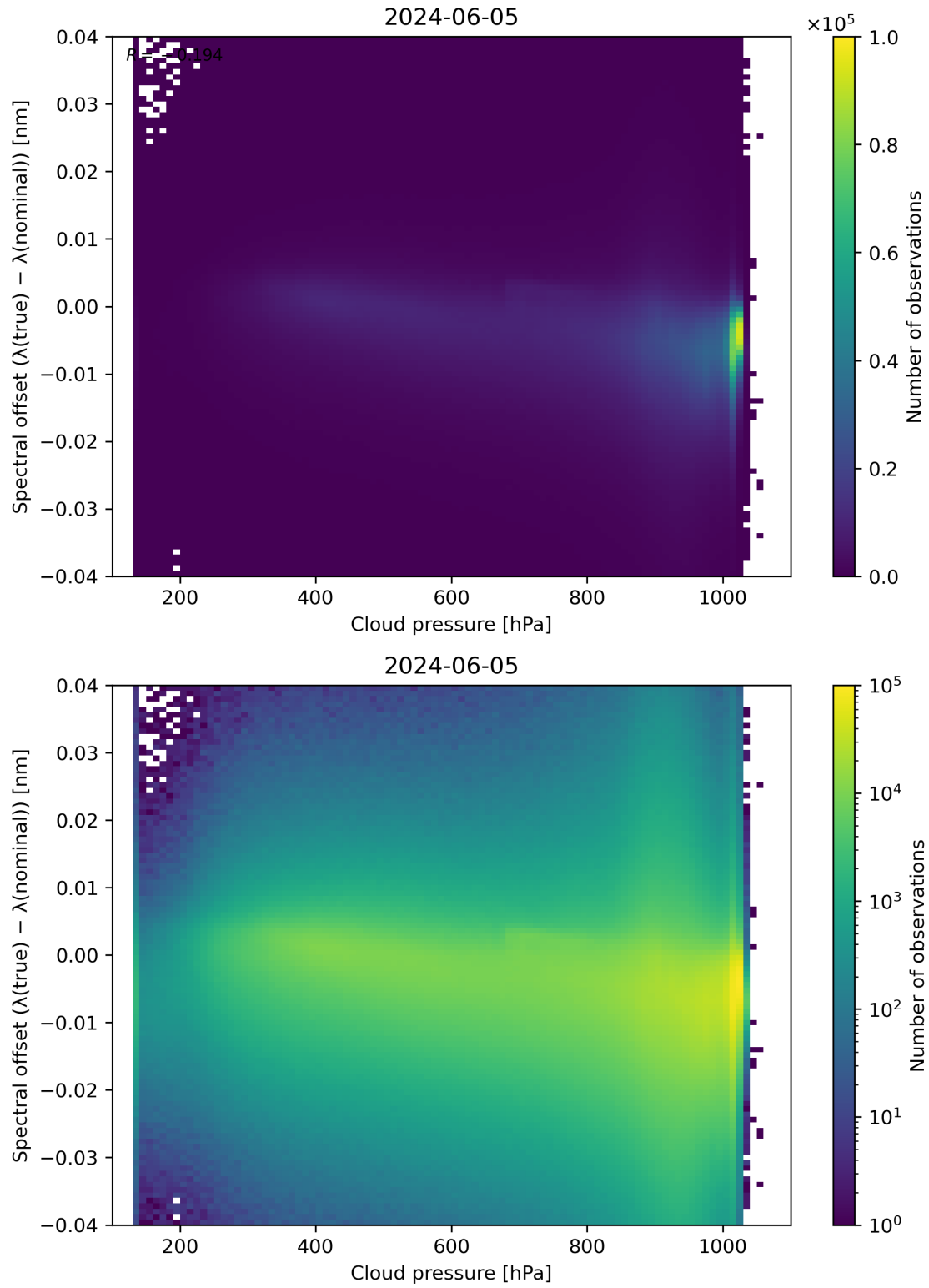
Figure 84: Scatter density plot of “Cloud pressure” against “Spectral offset ( \lambda(\text{true}) - \lambda(\text{nominal}) )” for 2024-06-04 to 2024-06-06.
