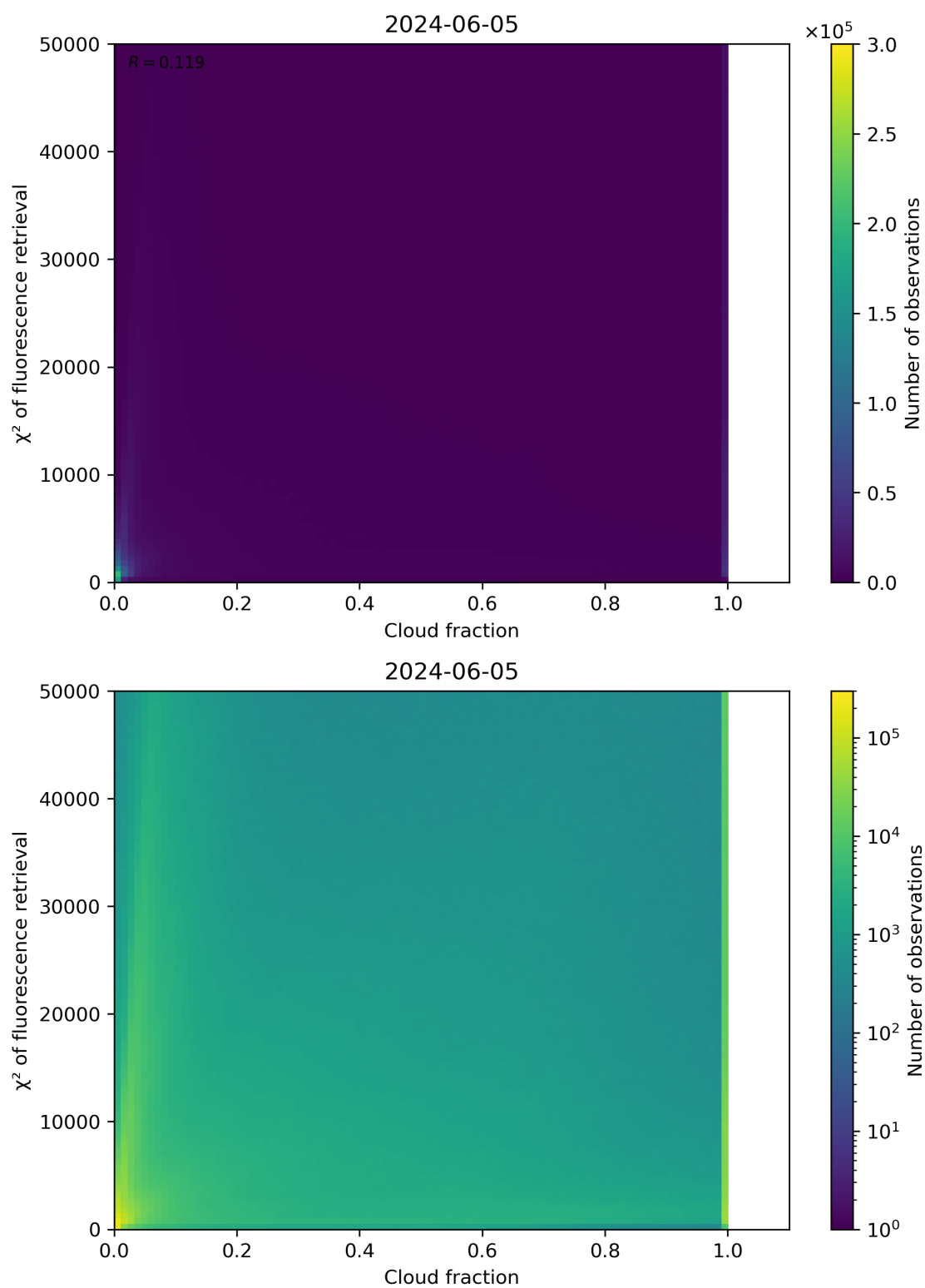
Figure 71: Scatter density plot of “Cloud fraction” against “ \chi^2 of fluorescence retrieval” for 2024-06-04 to 2024-06-06.
