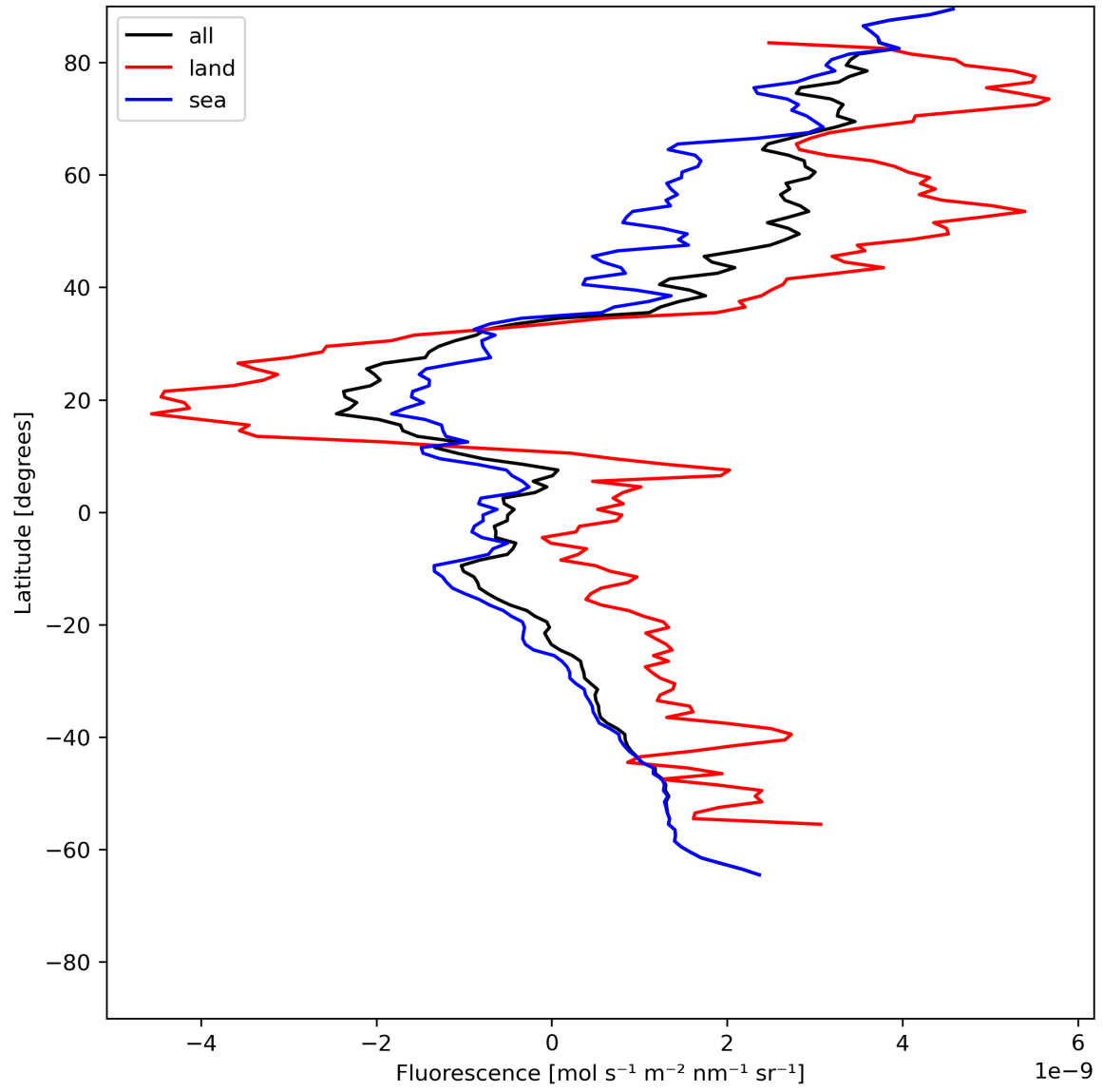
Figure 23: Zonal average of “Fluorescence” for 2024-06-04 to 2024-06-06.
