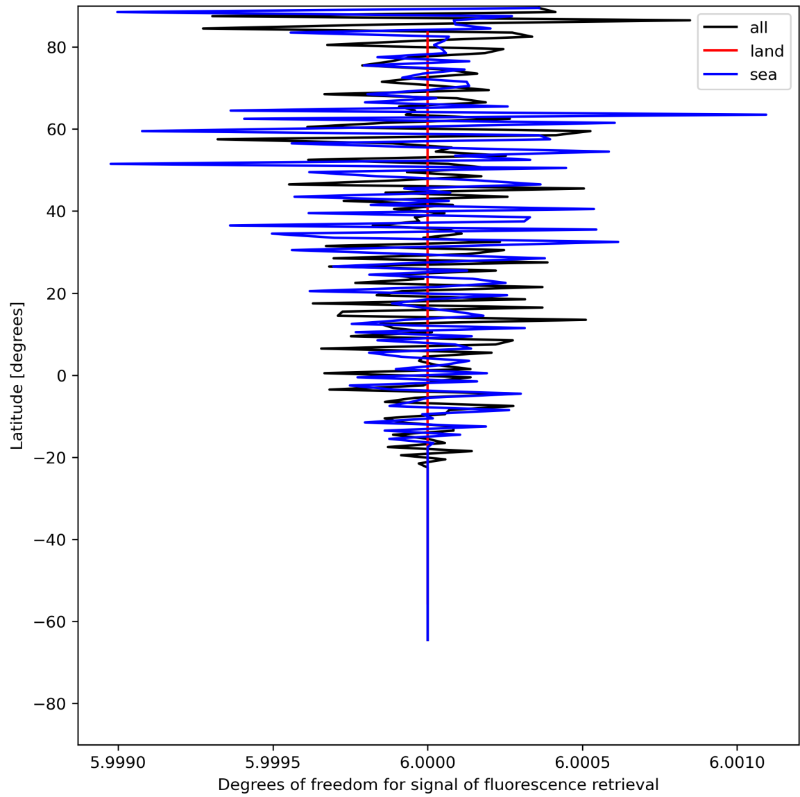
Figure 26: Zonal average of “Degrees of freedom for signal of fluorescence retrieval” for 2024-06-04 to 2024-06-06.
