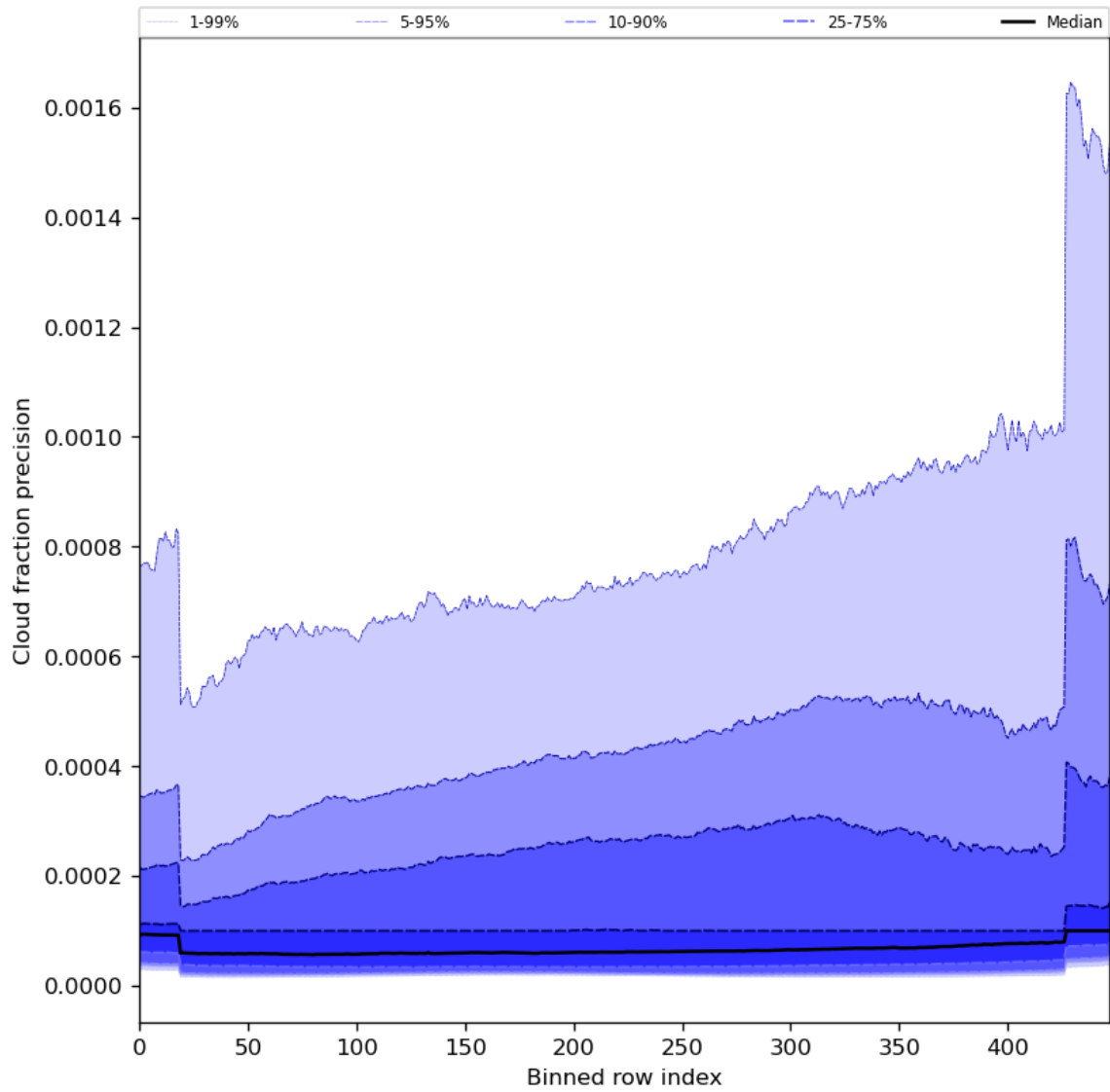
Figure 50: Along track statistics of “Cloud fraction precision” for 2024-06-04 to 2024-06-06
