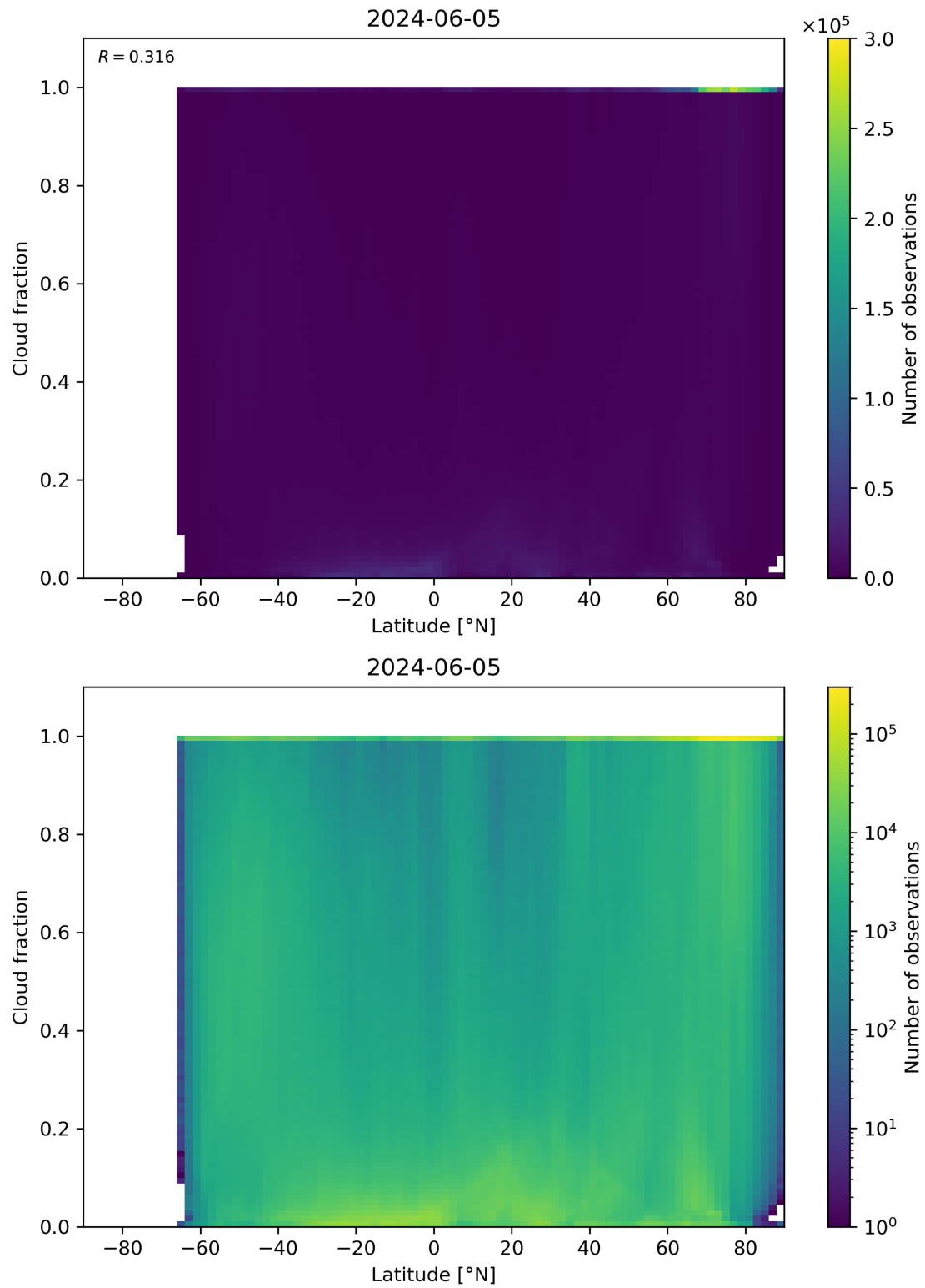
Figure 90: Scatter density plot of “Latitude” against “Cloud fraction” for 2024-06-04 to 2024-06-06.
