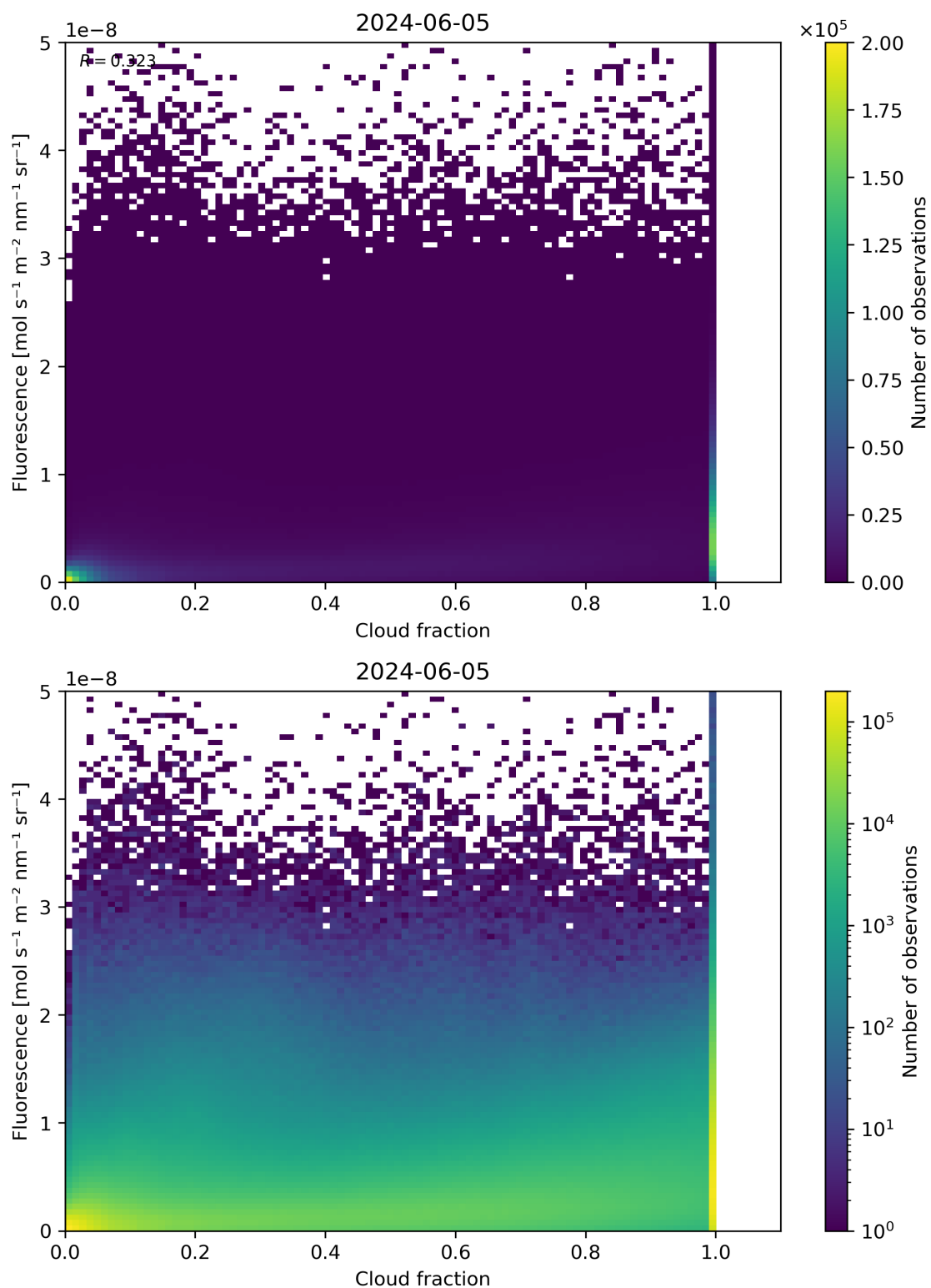
Figure 72: Scatter density plot of “Cloud fraction” against “Fluorescence” for 2024-06-04 to 2024-06-06.
