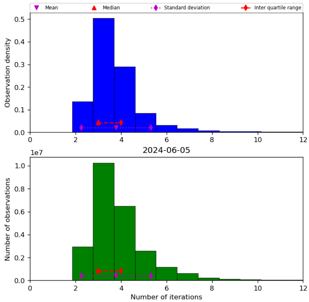
Figure 39: Histogram of “Number of iterations” for 2024-06-04 to 2024-06-06
