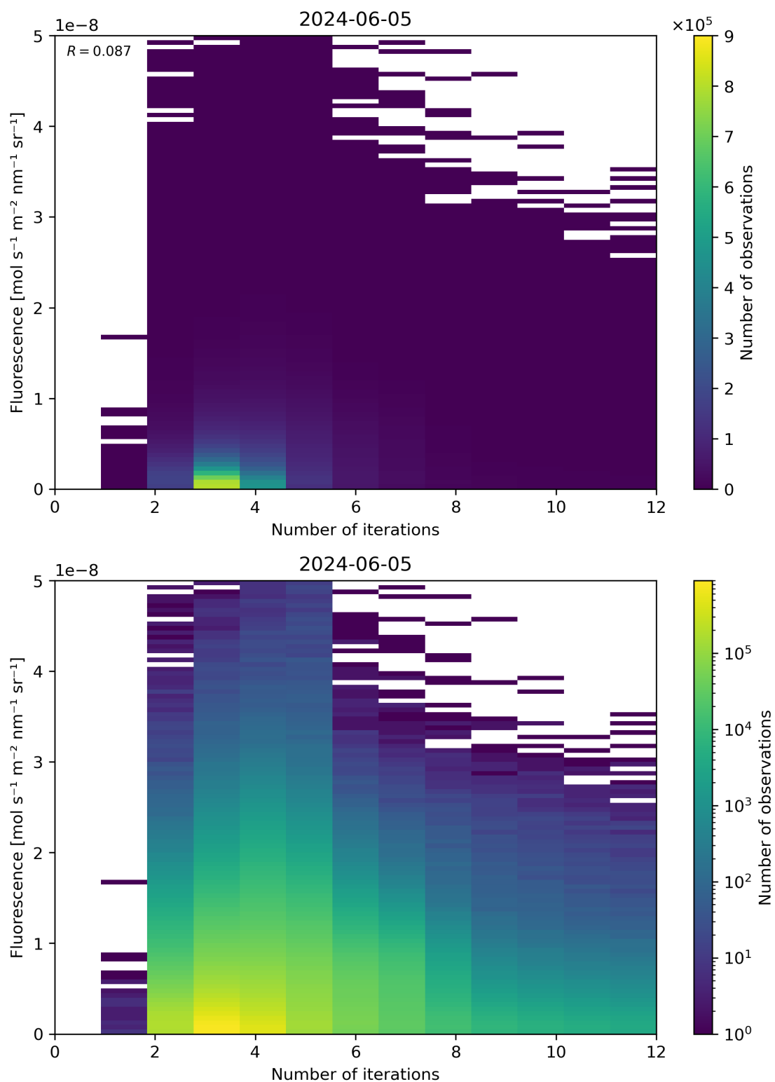
Figure 98: Scatter density plot of “Number of iterations” against “Fluorescence” for 2024-06-04 to 2024-06-06.
