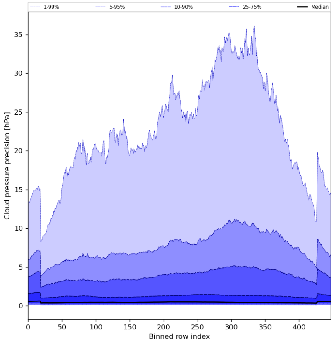
Figure 48: Along track statistics of “Cloud pressure precision” for 2024-06-04 to 2024-06-06
