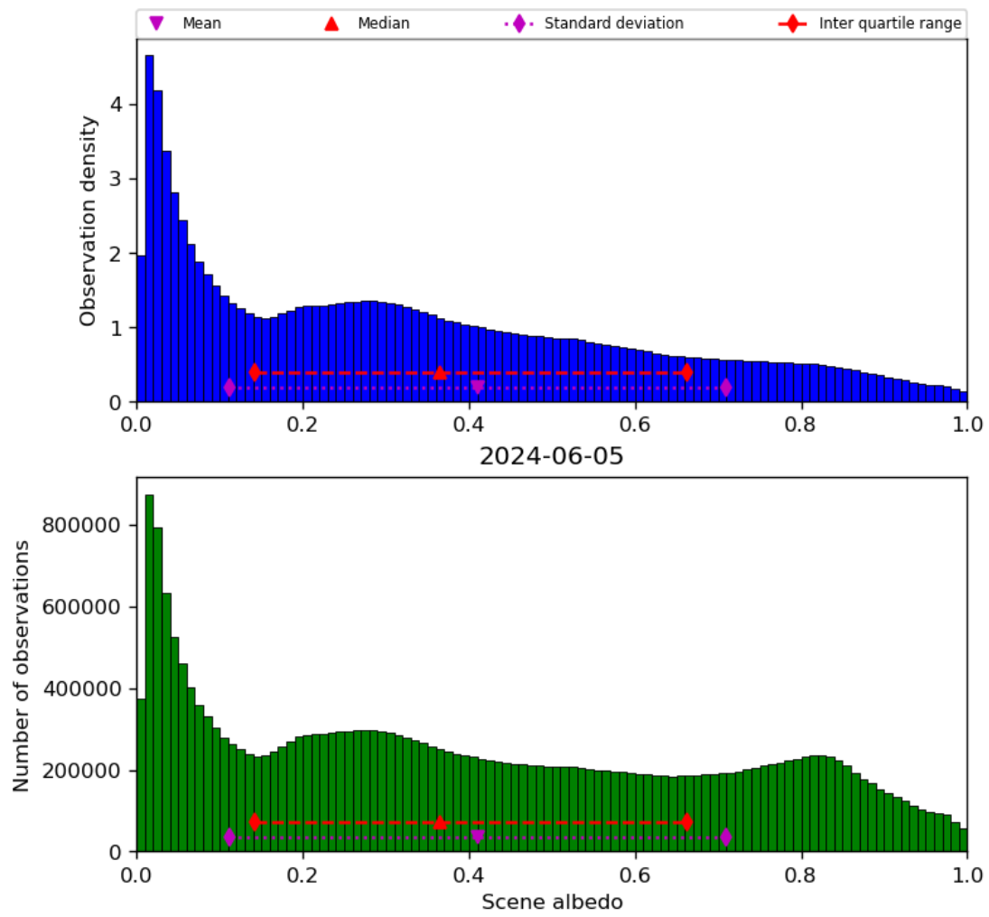
Figure 34: Histogram of “Scene albedo” for 2024-06-04 to 2024-06-06
