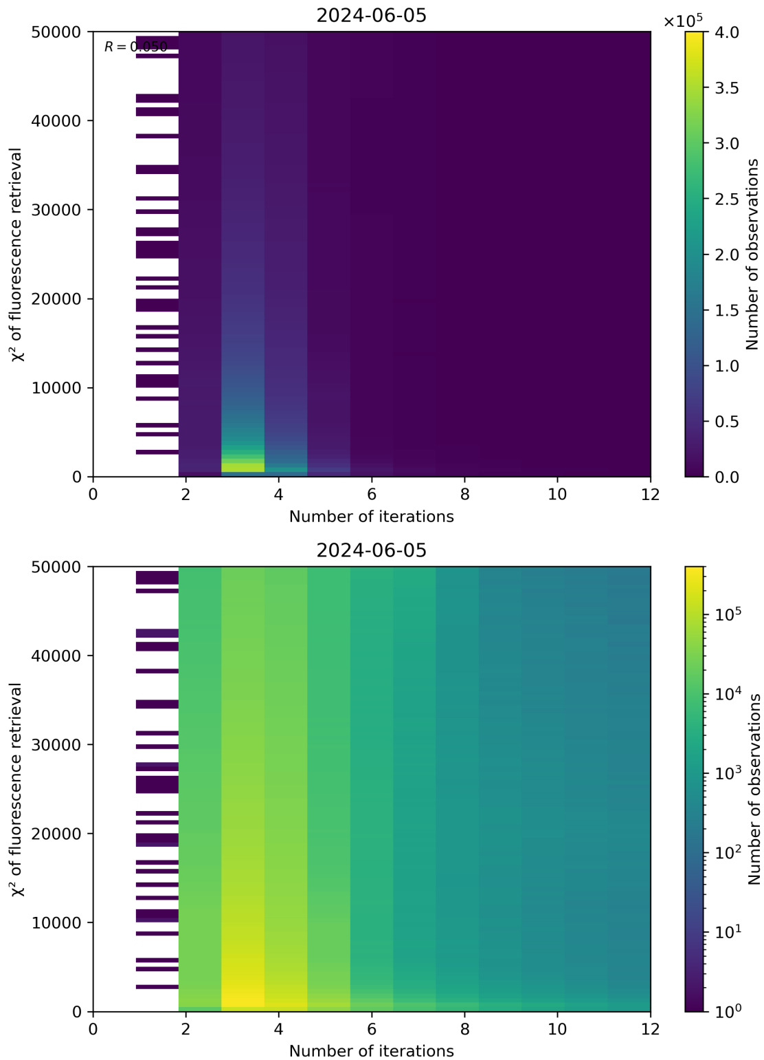
Figure 97: Scatter density plot of “Number of iterations” against “ \chi^2 of fluorescence retrieval” for 2024-06-04 to 2024-06-06.
