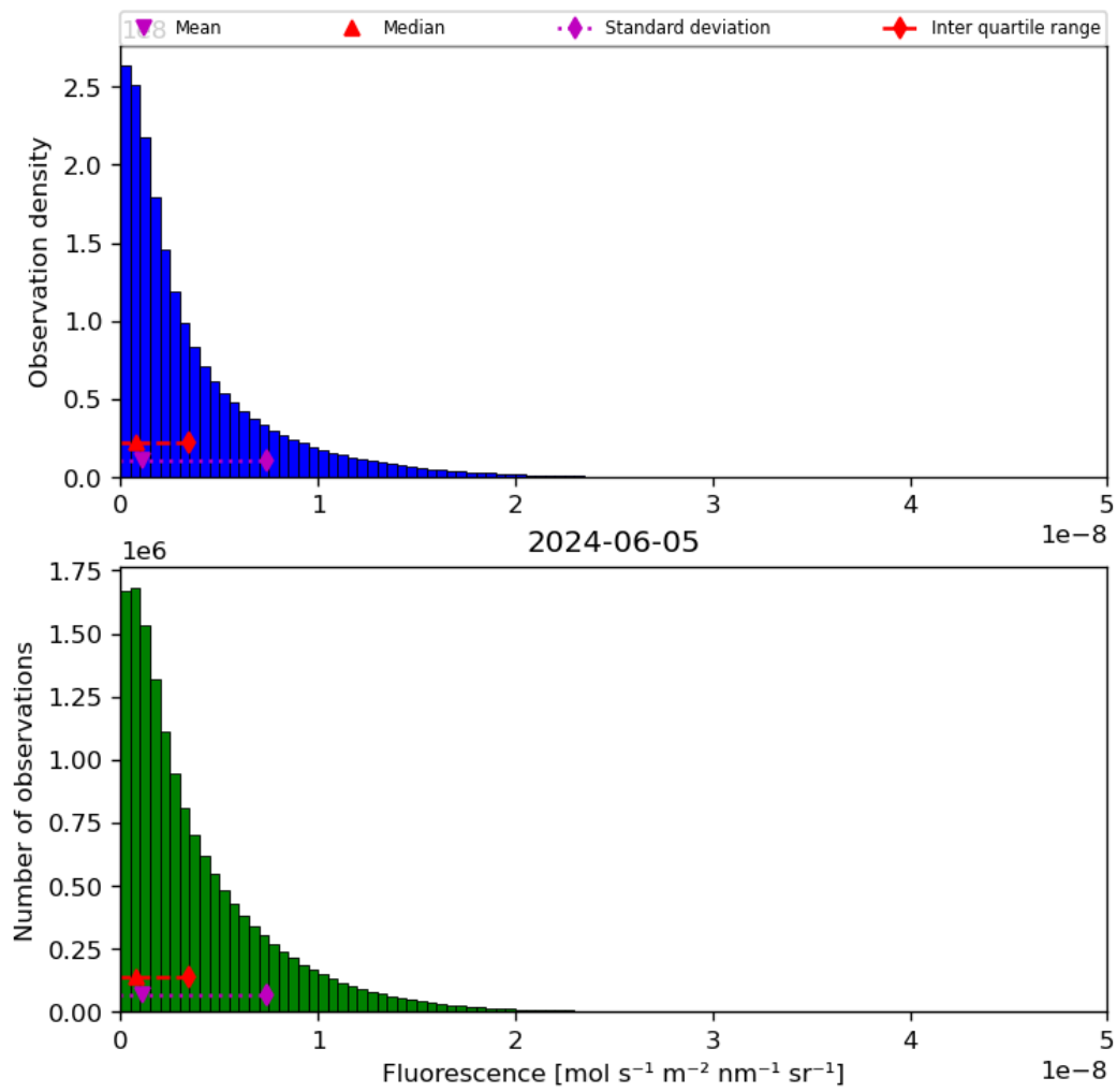
Figure 40: Histogram of “Fluorescence” for 2024-06-04 to 2024-06-06
