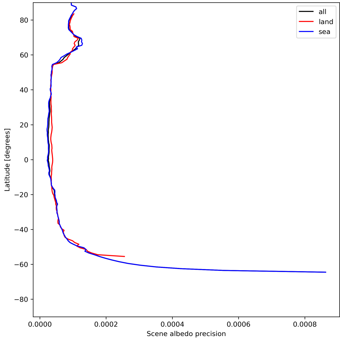
Figure 18: Zonal average of “Scene albedo precision” for 2024-06-04 to 2024-06-06.
