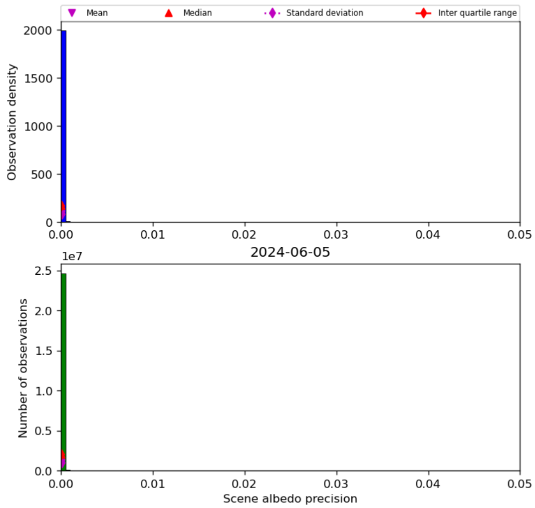
Figure 35: Histogram of “Scene albedo precision” for 2024-06-04 to 2024-06-06
