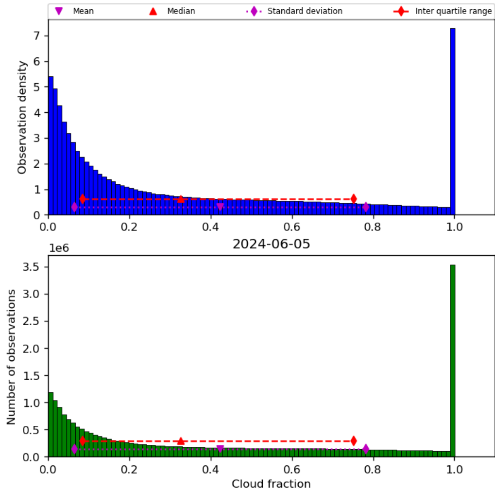
Figure 32: Histogram of “Cloud fraction” for 2024-06-04 to 2024-06-06
