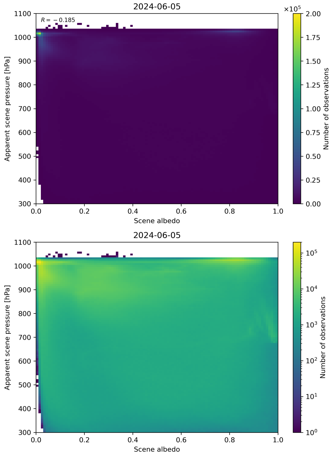
Figure 102: Scatter density plot of “Scene albedo” against “Apparent scene pressure” for 2024-06-04 to 2024-06-06.
