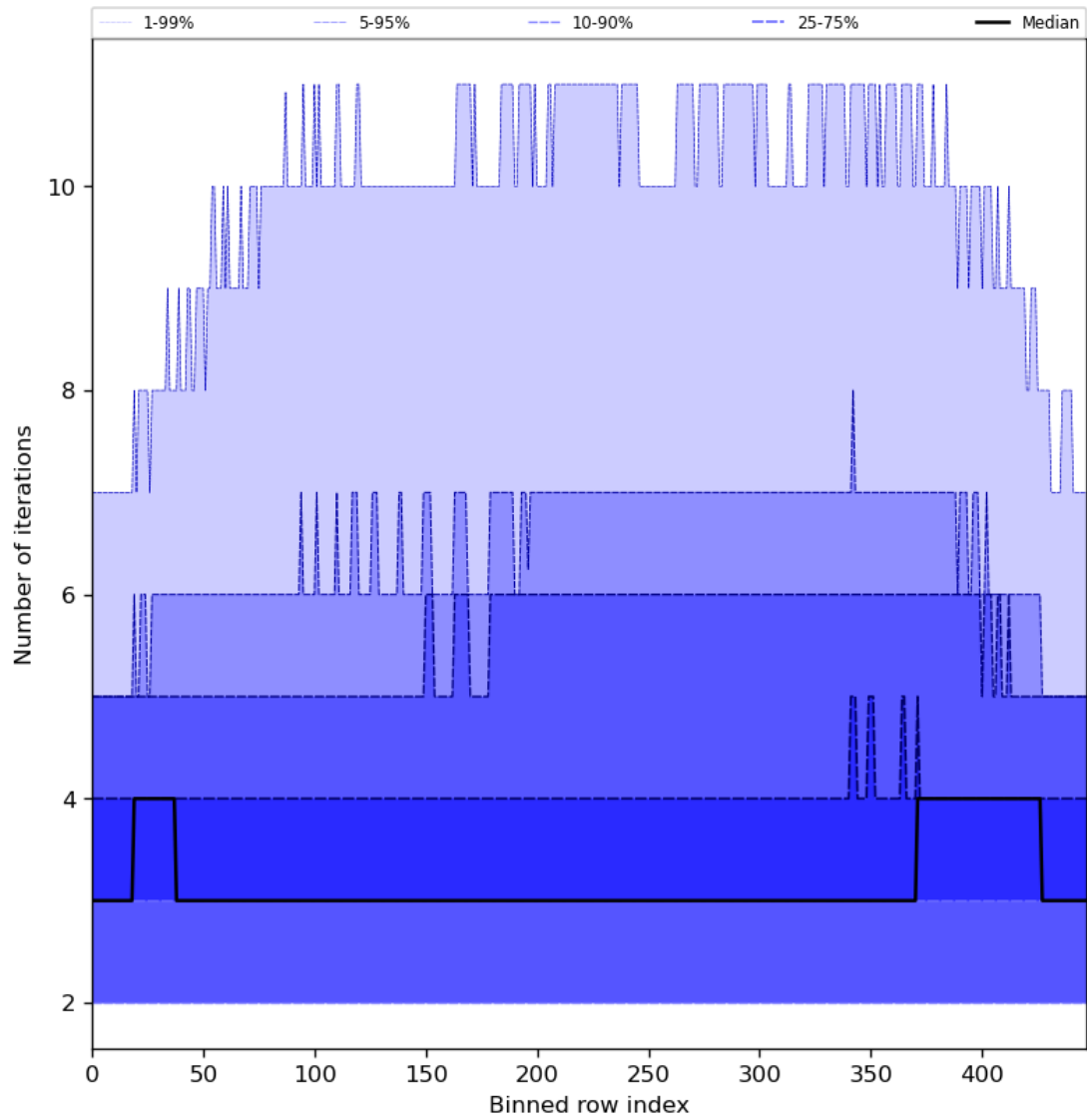
Figure 56: Along track statistics of “Number of iterations” for 2024-06-04 to 2024-06-06
