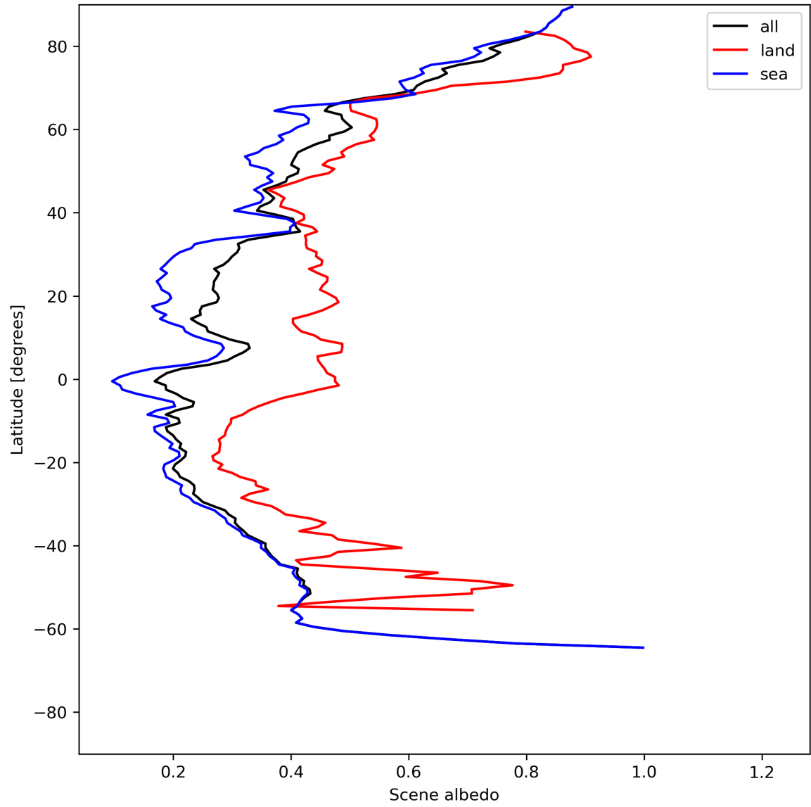
Figure 17: Zonal average of “Scene albedo” for 2024-06-04 to 2024-06-06.
