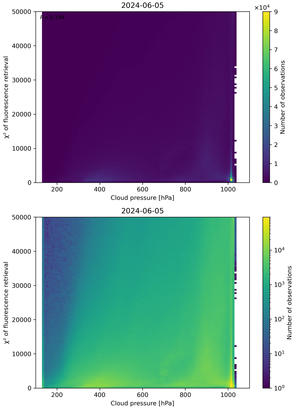
Figure 78: Scatter density plot of “Cloud pressure” against “ \chi^2 of fluorescence retrieval” for 2024-06-04 to 2024-06-06.
