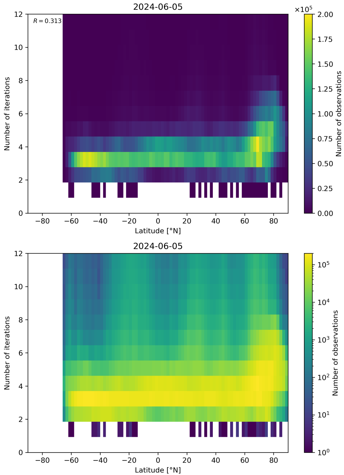
Figure 93: Scatter density plot of “Latitude” against “Number of iterations” for 2024-06-04 to 2024-06-06.
