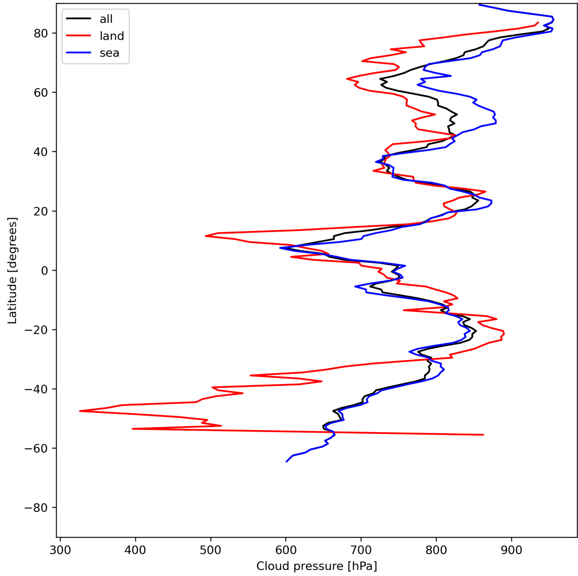
Figure 13: Zonal average of “Cloud pressure” for 2024-06-04 to 2024-06-06.
