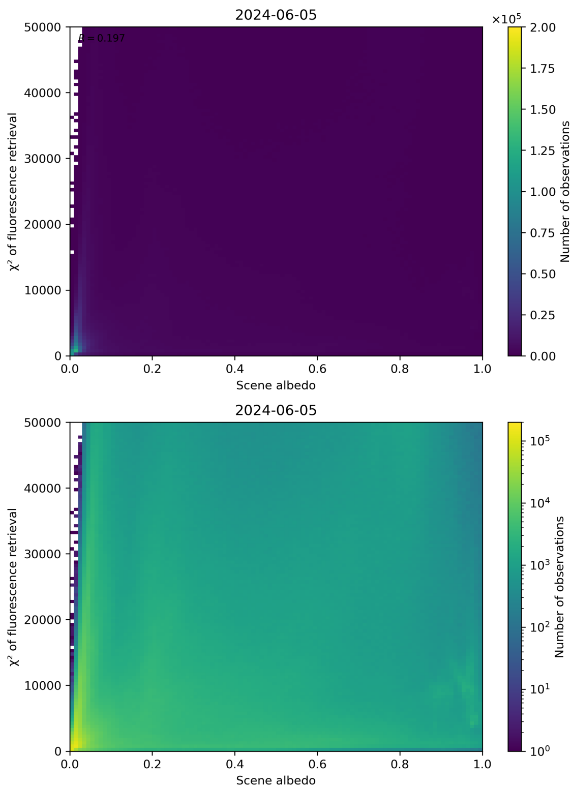
Figure 103: Scatter density plot of “Scene albedo” against “ \chi^2 of fluorescence retrieval” for 2024-06-04 to 2024-06-06.
