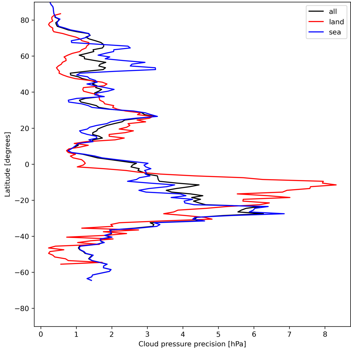
Figure 14: Zonal average of “Cloud pressure precision” for 2024-06-04 to 2024-06-06.
