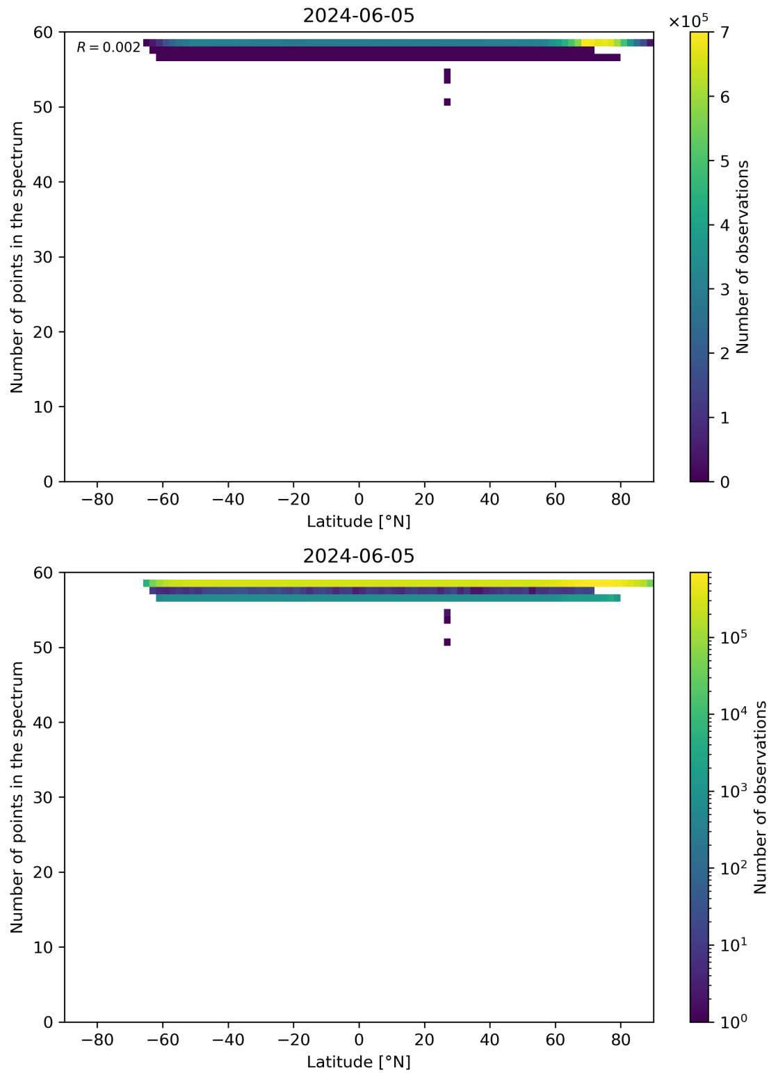
Figure 94: Scatter density plot of “Latitude” against “Number of points in the spectrum” for 2024-06-04 to 2024-06-06.
