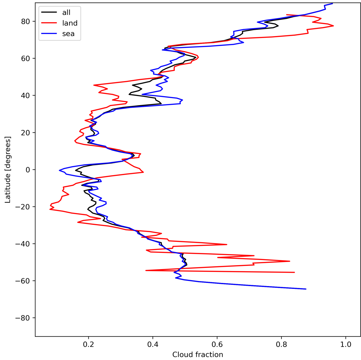
Figure 15: Zonal average of “Cloud fraction” for 2024-06-04 to 2024-06-06.
