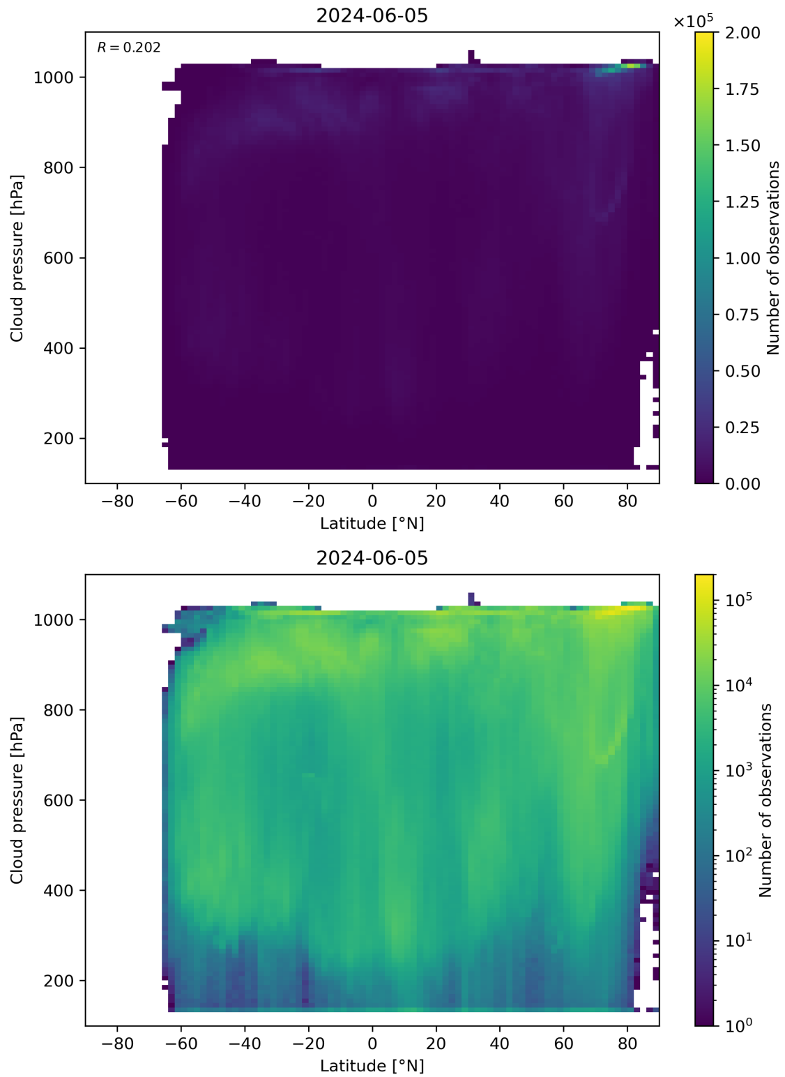
Figure 91: Scatter density plot of “Latitude” against “Cloud pressure” for 2024-06-04 to 2024-06-06.
