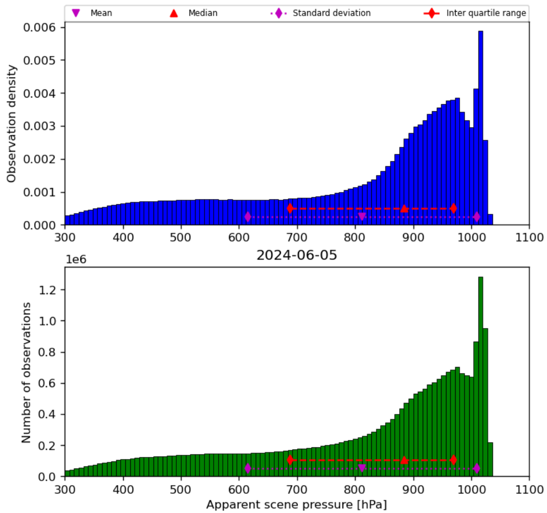
Figure 36: Histogram of “Apparent scene pressure” for 2024-06-04 to 2024-06-06
