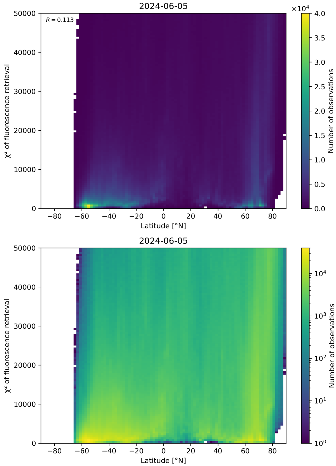
Figure 89: Scatter density plot of “Latitude” against “ \chi^2 of fluorescence retrieval” for 2024-06-04 to 2024-06-06.
