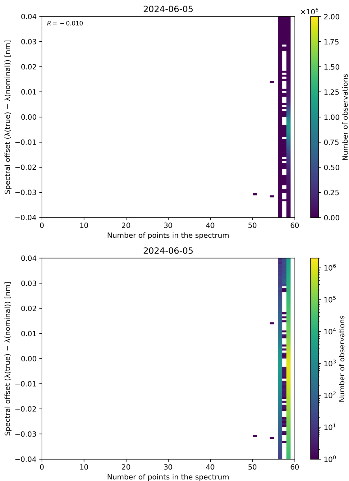
Figure 101: Scatter density plot of “Number of points in the spectrum” against “Spectral offset ( \lambda(\text{true}) - \lambda(\text{nominal}) )” for 2024-06-04 to 2024-06-06.
