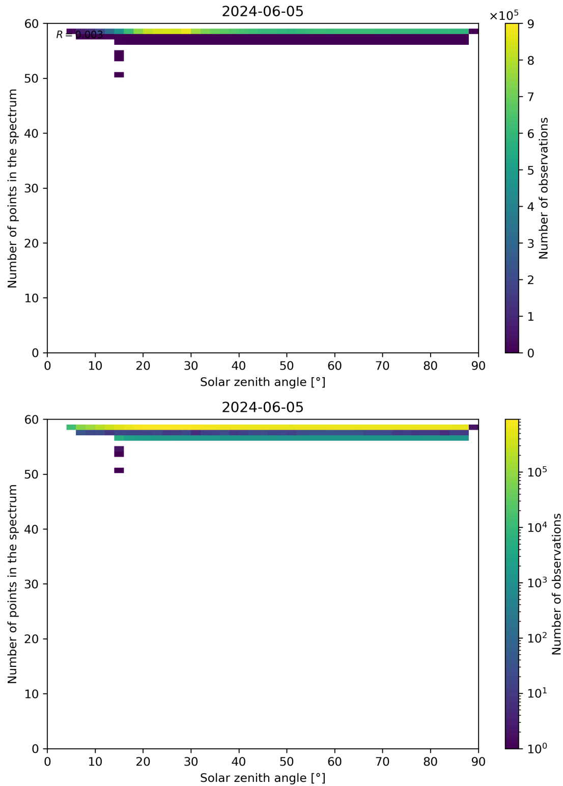
Figure 115: Scatter density plot of “Solar zenith angle” against “Number of points in the spectrum” for 2024-06-04 to 2024-06-06.
