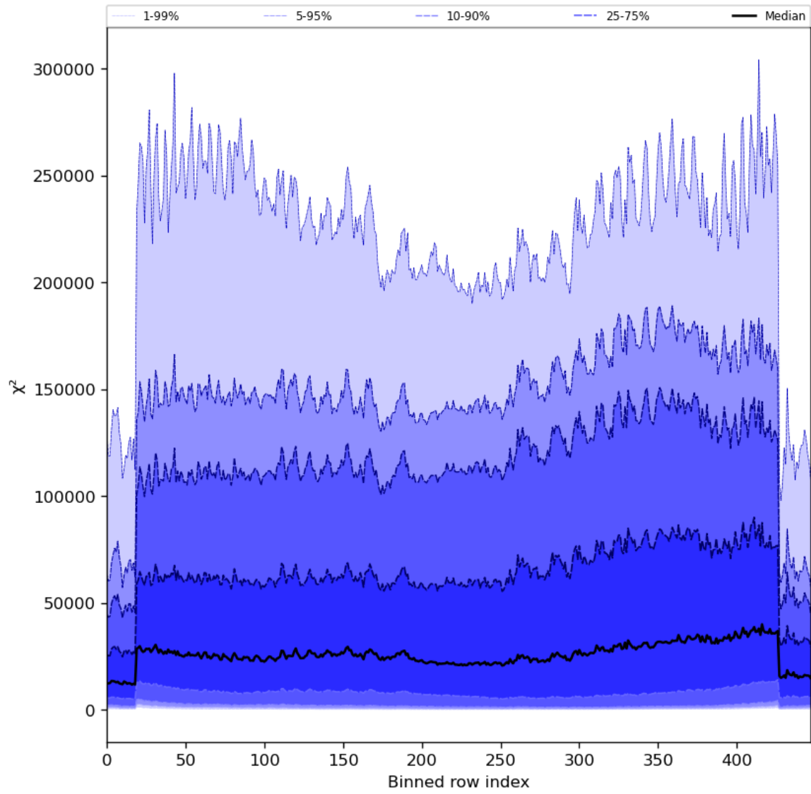
Figure 55: Along track statistics of “ \chi^2 ” for 2024-06-04 to 2024-06-06
