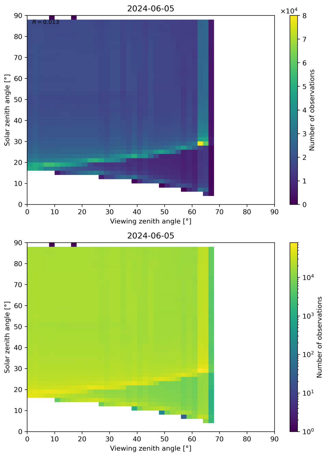
Figure 127: Scatter density plot of “Viewing zenith angle” against “Solar zenith angle” for 2024-06-04 to 2024-06-06.
