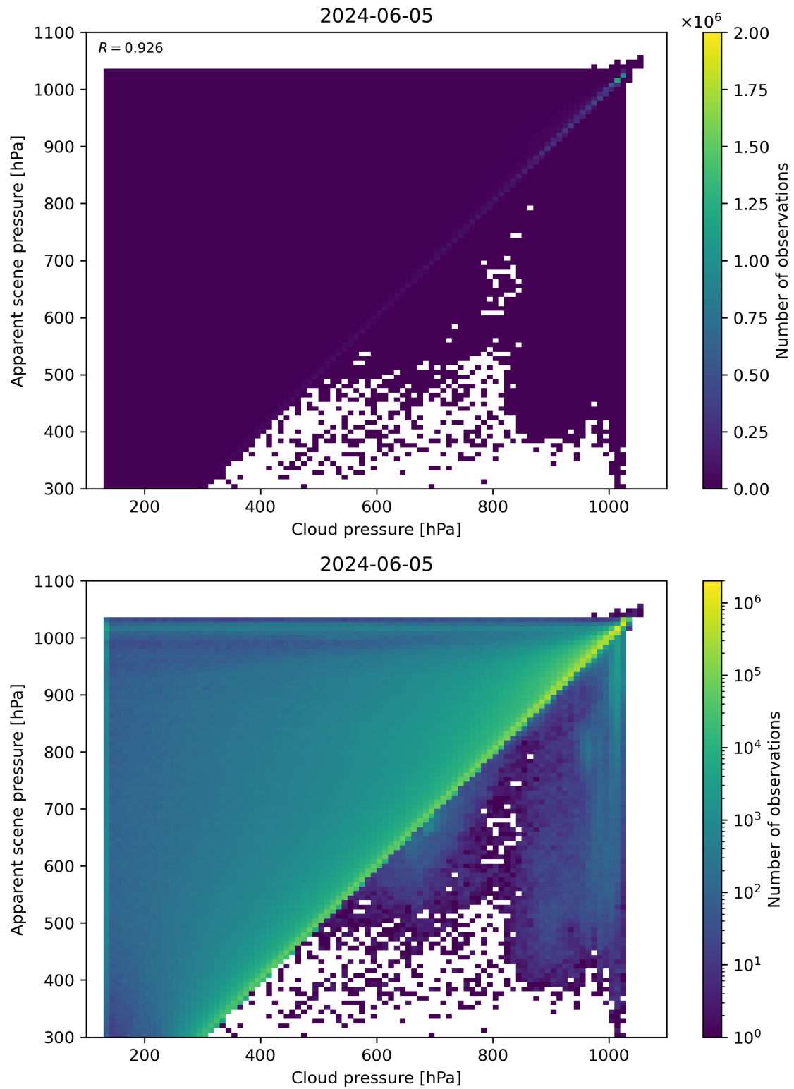
Figure 77: Scatter density plot of “Cloud pressure” against “Apparent scene pressure” for 2024-06-04 to 2024-06-06.
