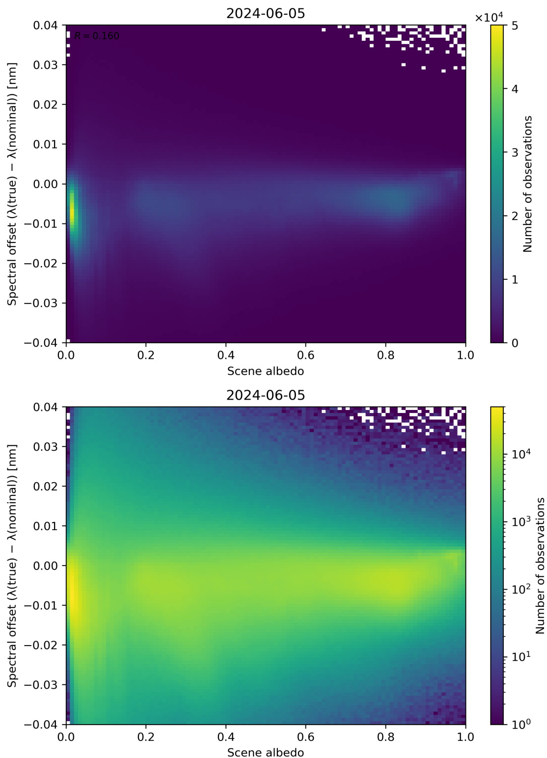
Figure 107: Scatter density plot of “Scene albedo” against “Spectral offset ( \lambda(\text{true}) - \lambda(\text{nominal}) )” for 2024-06-04 to 2024-06-06.
