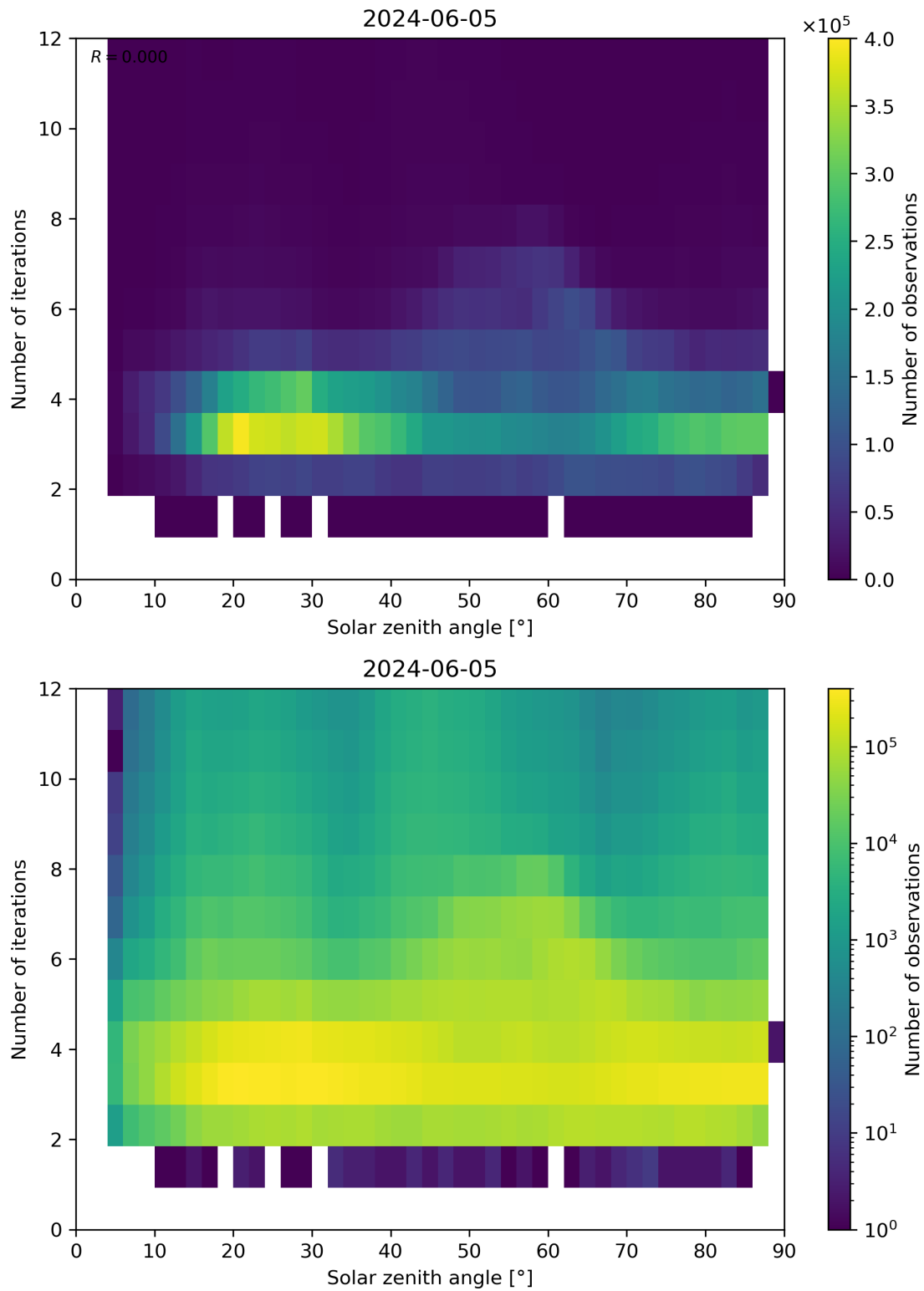
Figure 114: Scatter density plot of “Solar zenith angle” against “Number of iterations” for 2024-06-04 to 2024-06-06.
