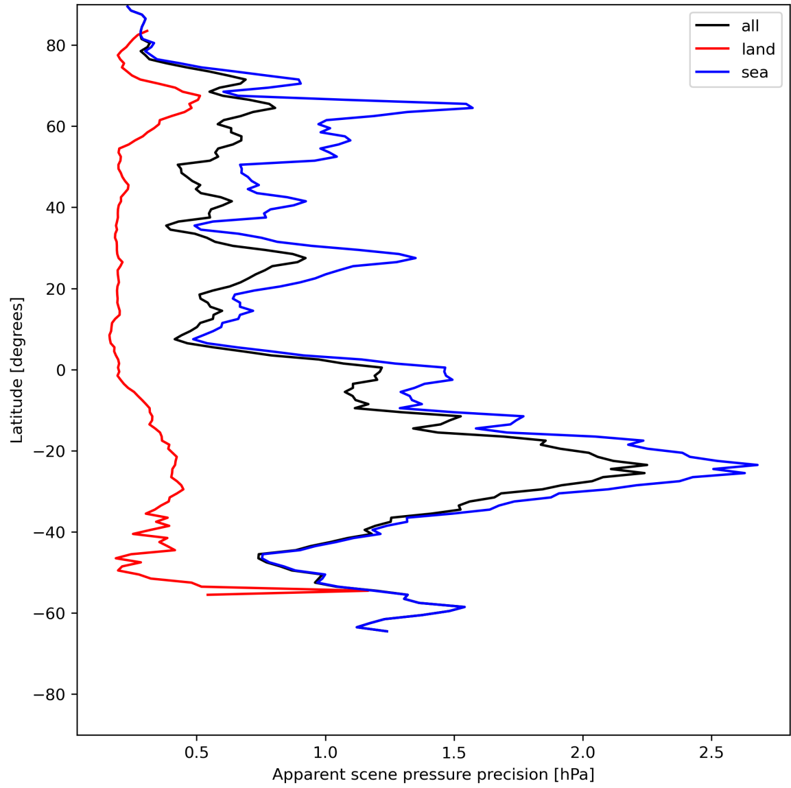
Figure 20: Zonal average of “Apparent scene pressure precision” for 2024-06-04 to 2024-06-06.
