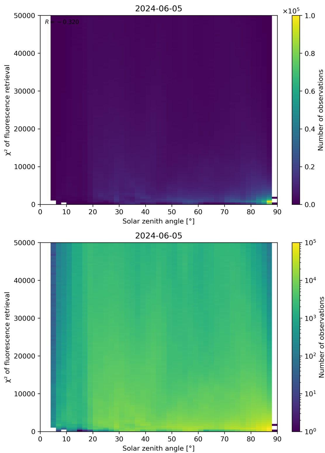
Figure 109: Scatter density plot of “Solar zenith angle” against “ \chi^2 of fluorescence retrieval” for 2024-06-04 to 2024-06-06.
