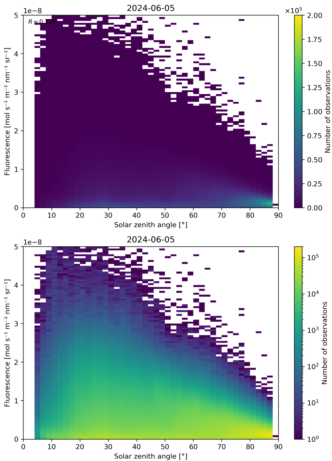
Figure 112: Scatter density plot of “Solar zenith angle” against “Fluorescence” for 2024-06-04 to 2024-06-06.
