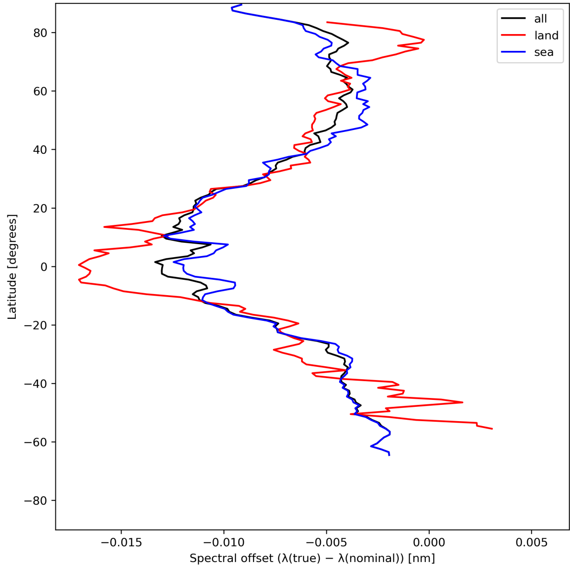
Figure 28: Zonal average of “Spectral offset ( \lambda(\text{true}) - \lambda(\text{nominal}) )” for 2024-06-04 to 2024-06-06.
