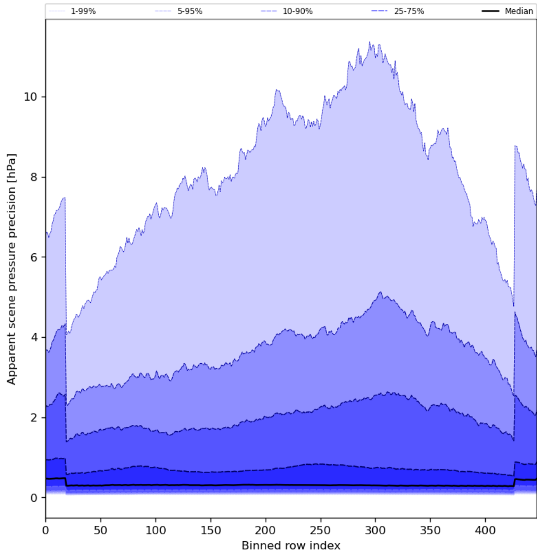
Figure 54: Along track statistics of “Apparent scene pressure precision” for 2024-06-04 to 2024-06-06
