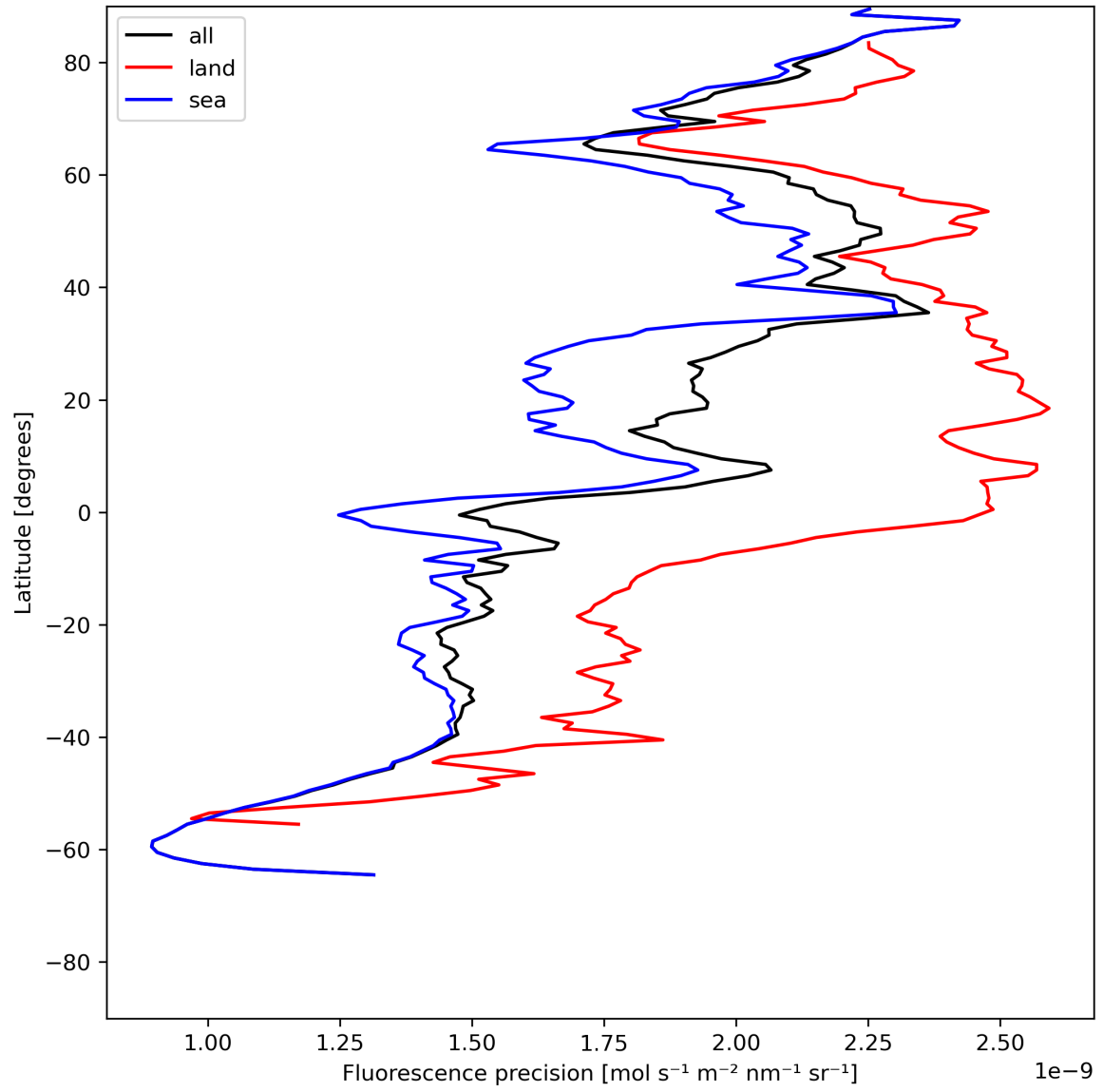
Figure 24: Zonal average of “Fluorescence precision” for 2024-06-04 to 2024-06-06.
