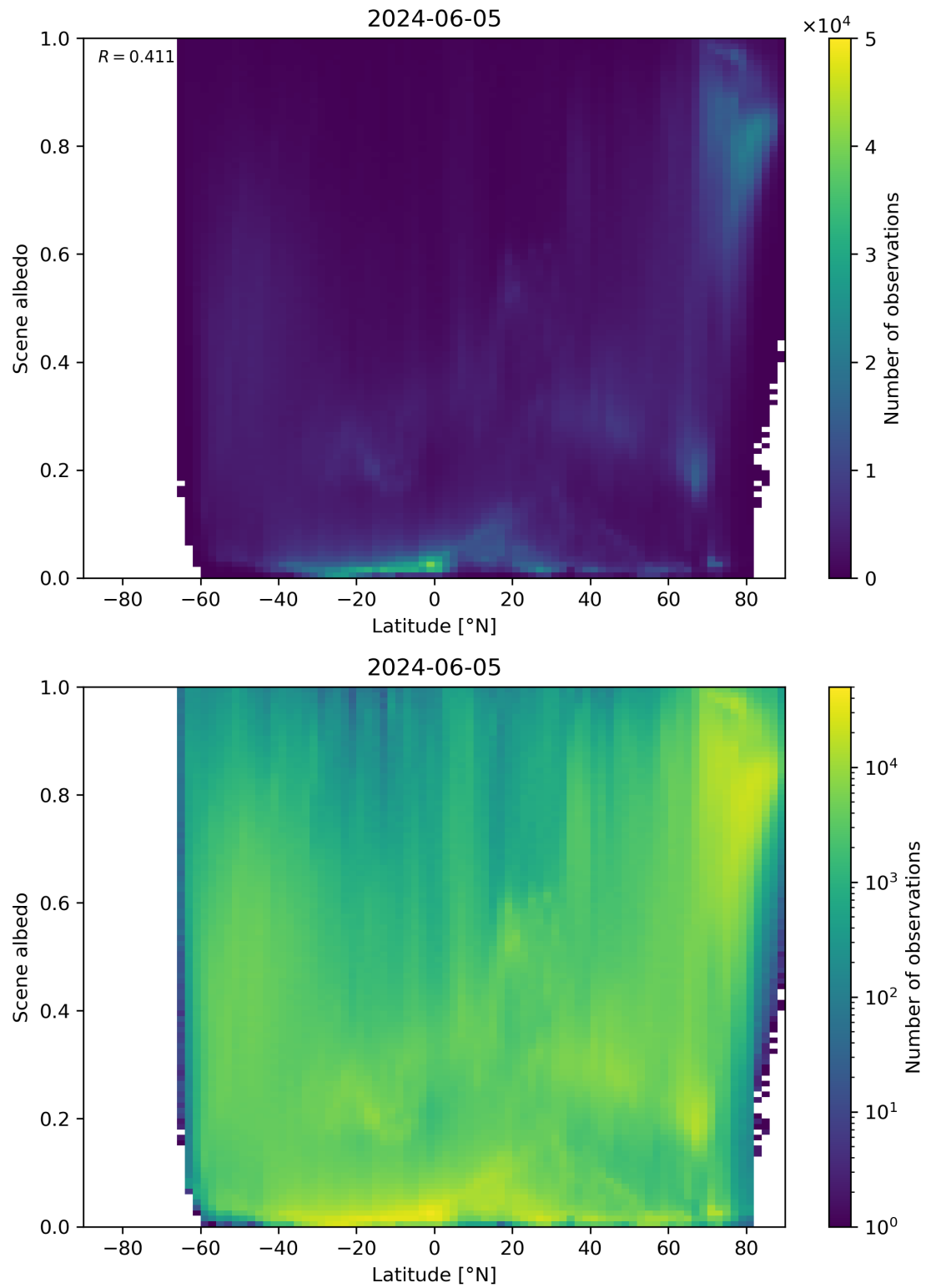
Figure 95: Scatter density plot of “Latitude” against “Scene albedo” for 2024-06-04 to 2024-06-06.
