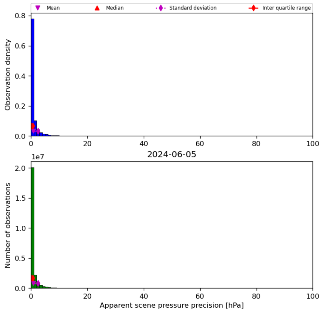
Figure 37: Histogram of “Apparent scene pressure precision” for 2024-06-04 to 2024-06-06
