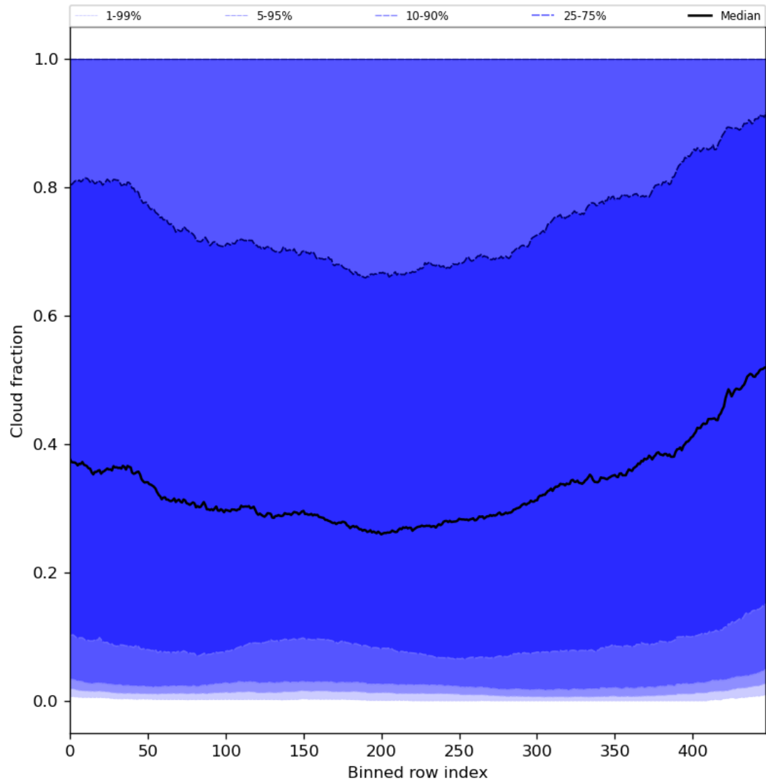
Figure 49: Along track statistics of “Cloud fraction” for 2024-06-04 to 2024-06-06
