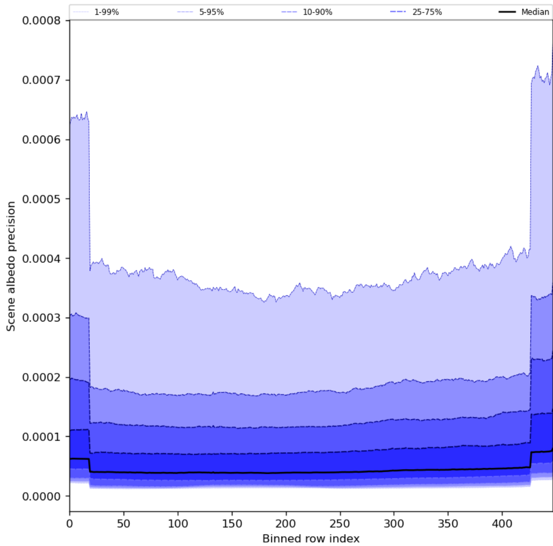
Figure 52: Along track statistics of “Scene albedo precision” for 2024-06-04 to 2024-06-06
