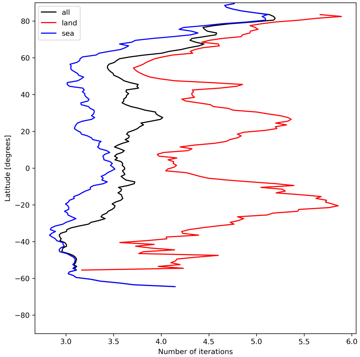
Figure 22: Zonal average of “Number of iterations” for 2024-06-04 to 2024-06-06.
