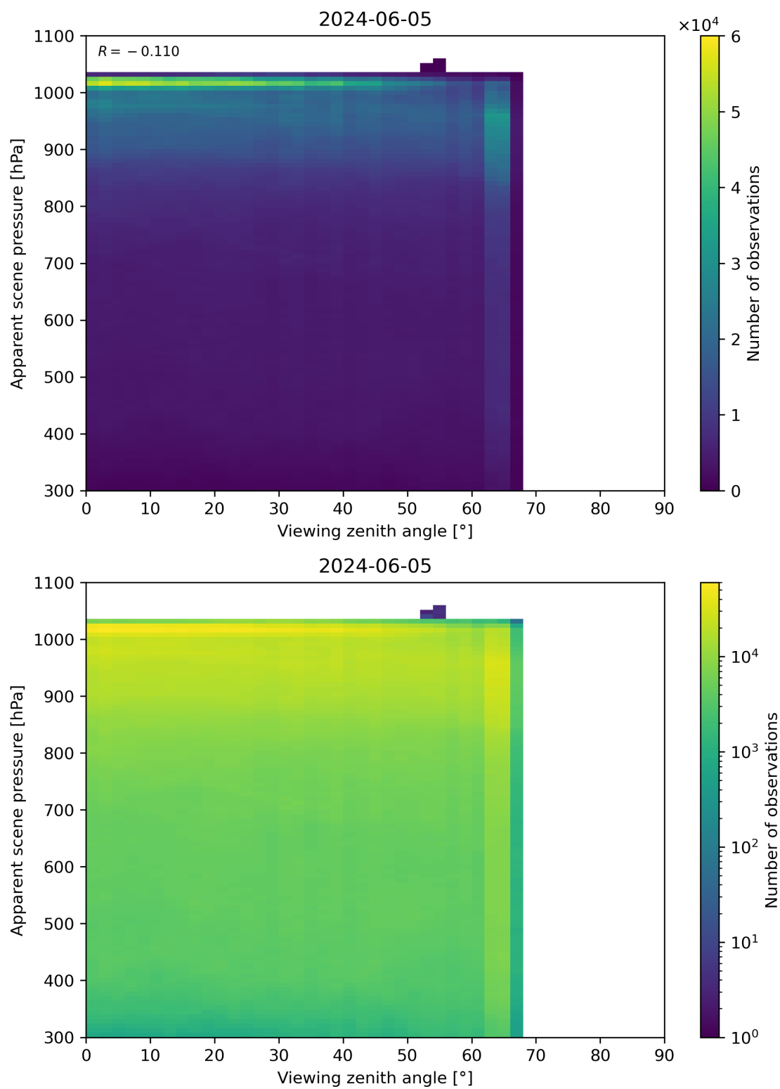
Figure 118: Scatter density plot of “Viewing zenith angle” against “Apparent scene pressure” for 2024-06-04 to 2024-06-06.
