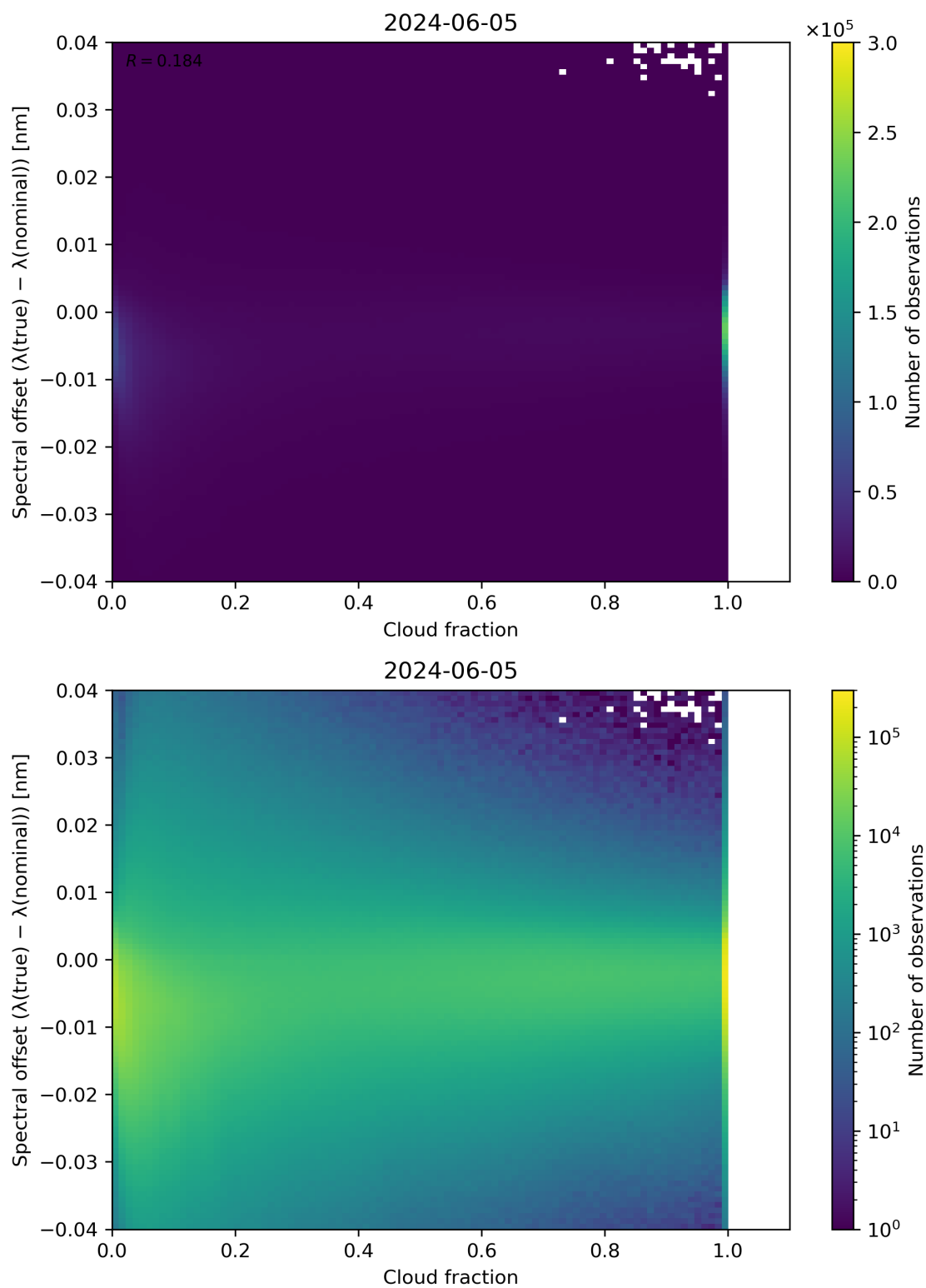
Figure 76: Scatter density plot of “Cloud fraction” against “Spectral offset ( \lambda(\text{true}) - \lambda(\text{nominal}) )” for 2024-06-04 to 2024-06-06.
