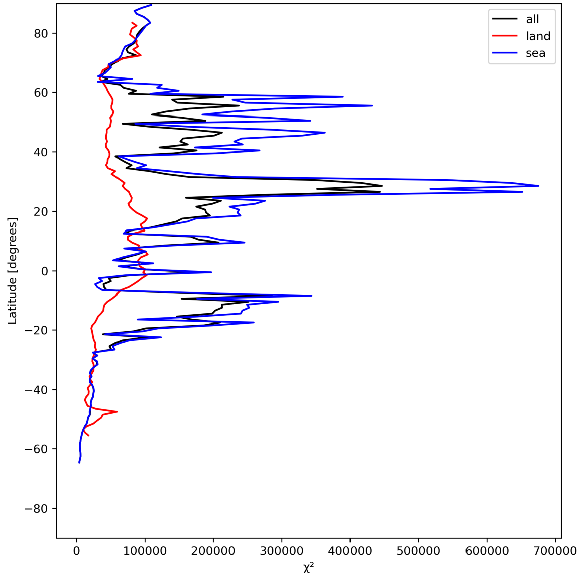
Figure 21: Zonal average of “ \chi^2 ” for 2024-06-04 to 2024-06-06.
