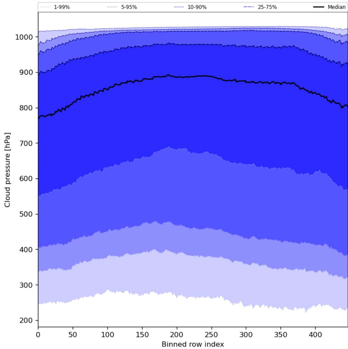
Figure 47: Along track statistics of “Cloud pressure” for 2024-06-04 to 2024-06-06
