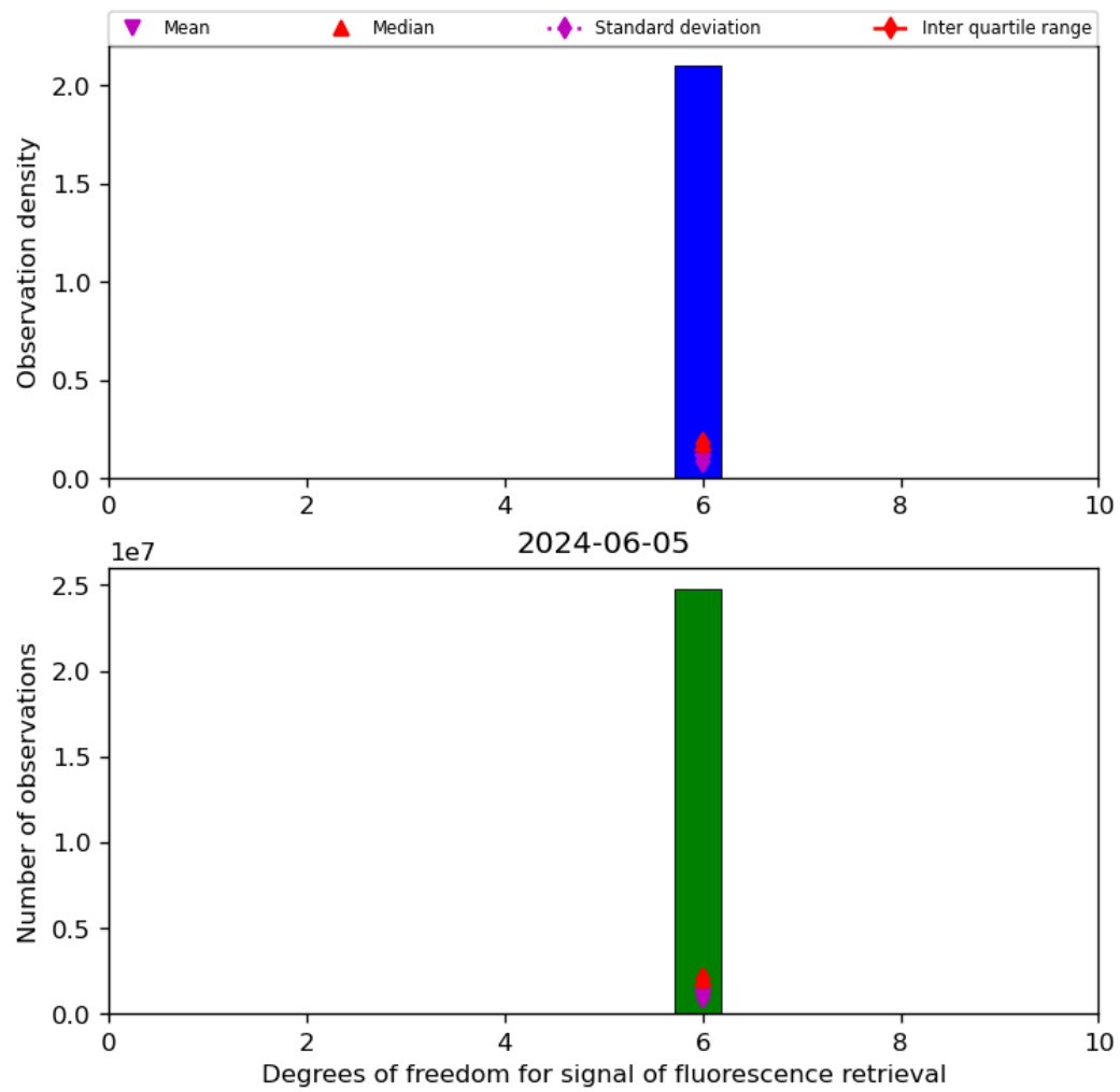
Figure 43: Histogram of “Degrees of freedom for signal of fluorescence retrieval” for 2024-06-04 to 2024-06-06
