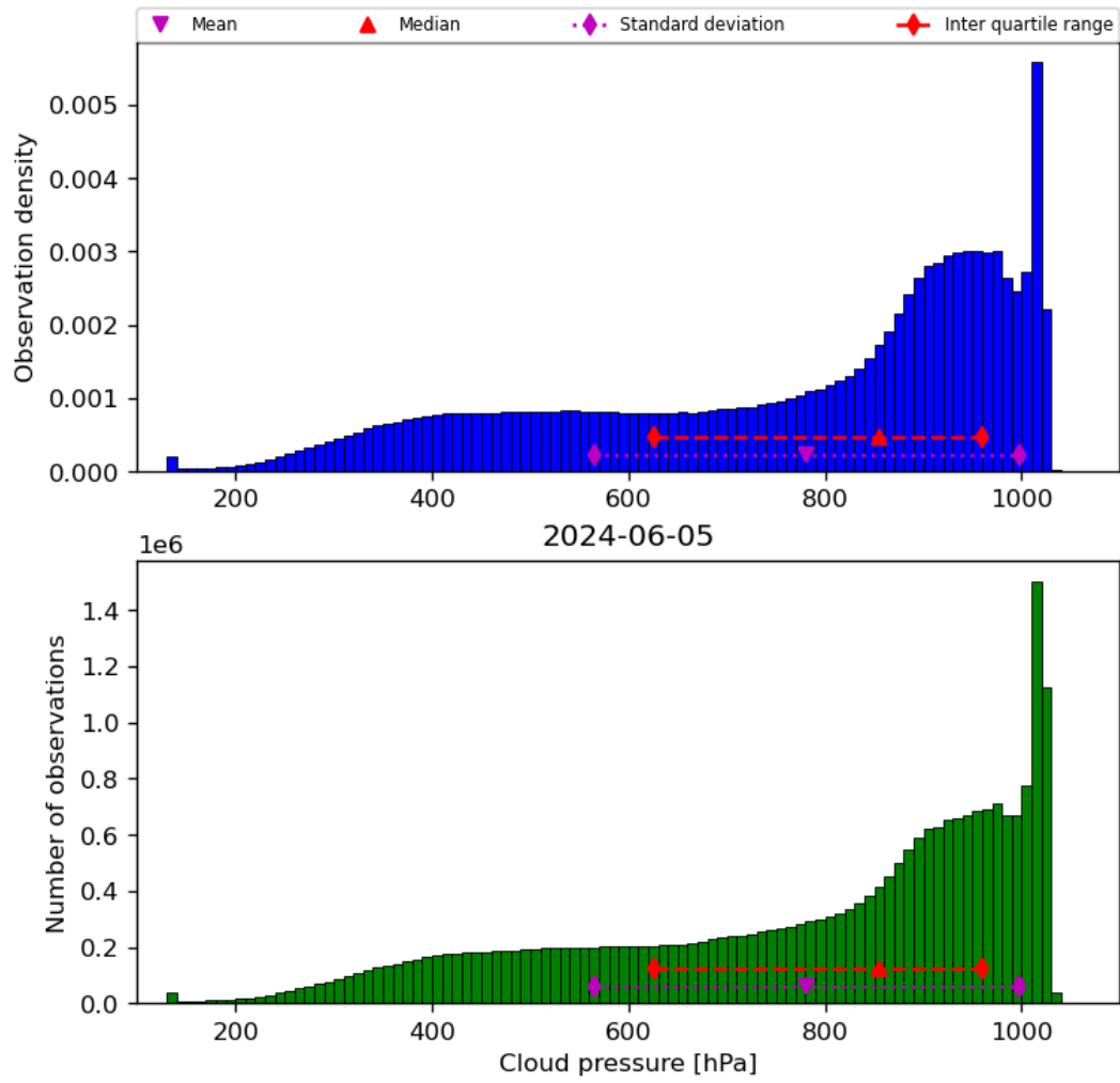
Figure 30: Histogram of “Cloud pressure” for 2024-06-04 to 2024-06-06
