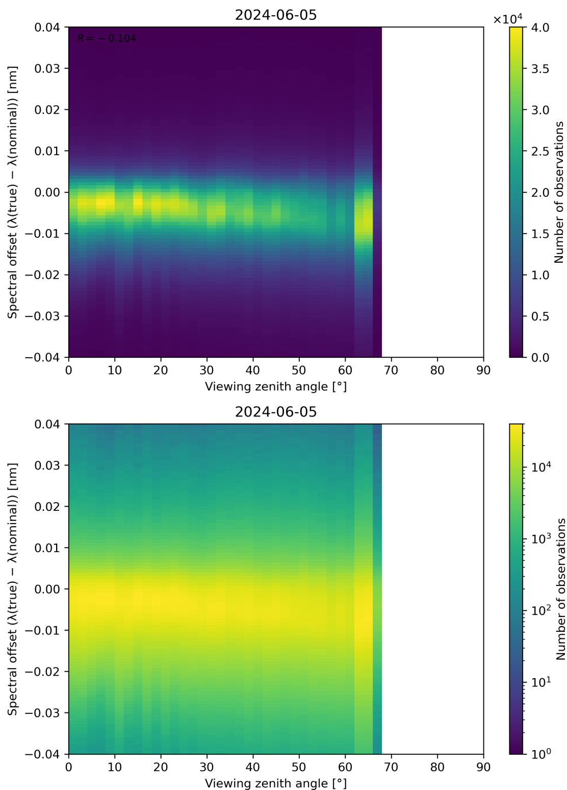
Figure 128: Scatter density plot of “Viewing zenith angle” against “Spectral offset ( \lambda(\text{true}) - \lambda(\text{nominal}) )” for 2024-06-04 to 2024-06-06.
