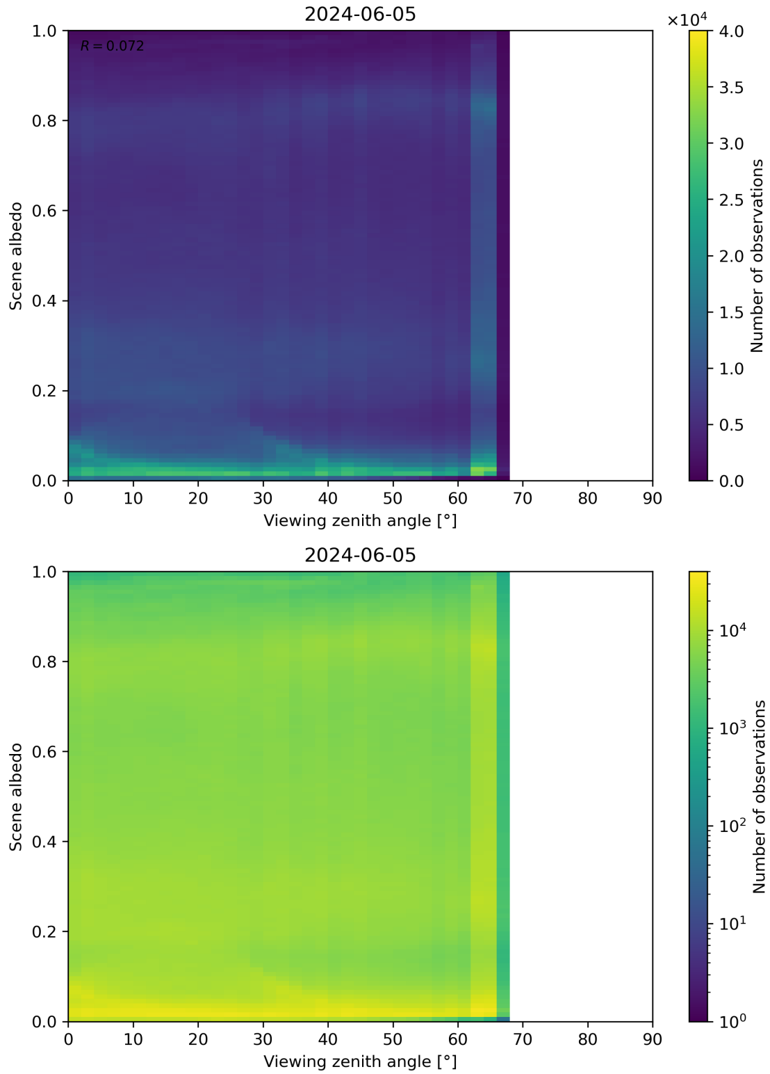
Figure 126: Scatter density plot of “Viewing zenith angle” against “Scene albedo” for 2024-06-04 to 2024-06-06.
