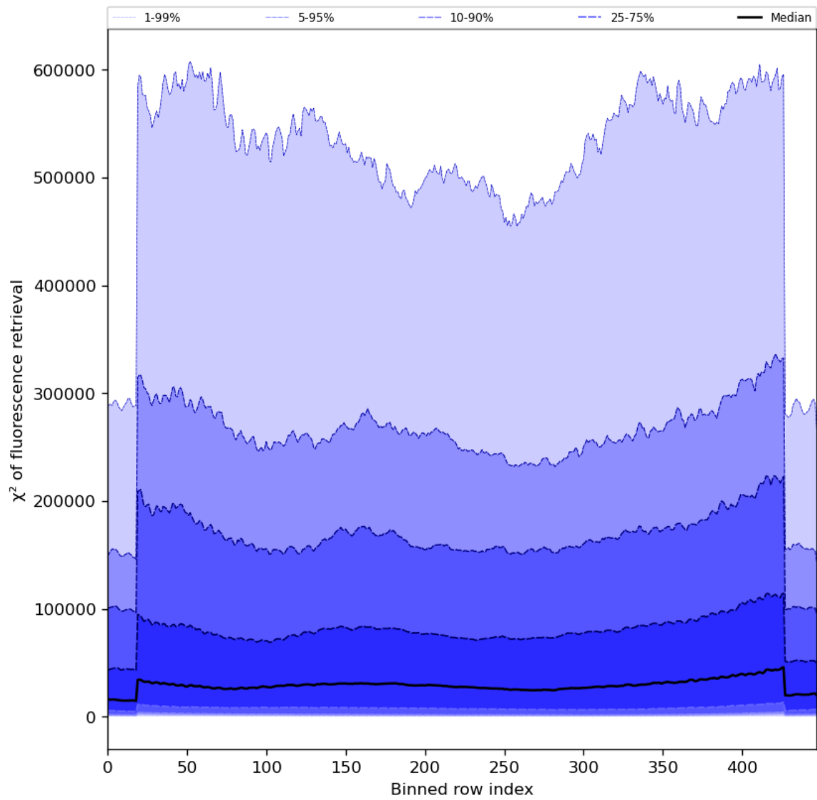
Figure 59: Along track statistics of “ \chi^2 of fluorescence retrieval” for 2024-06-04 to 2024-06-06
