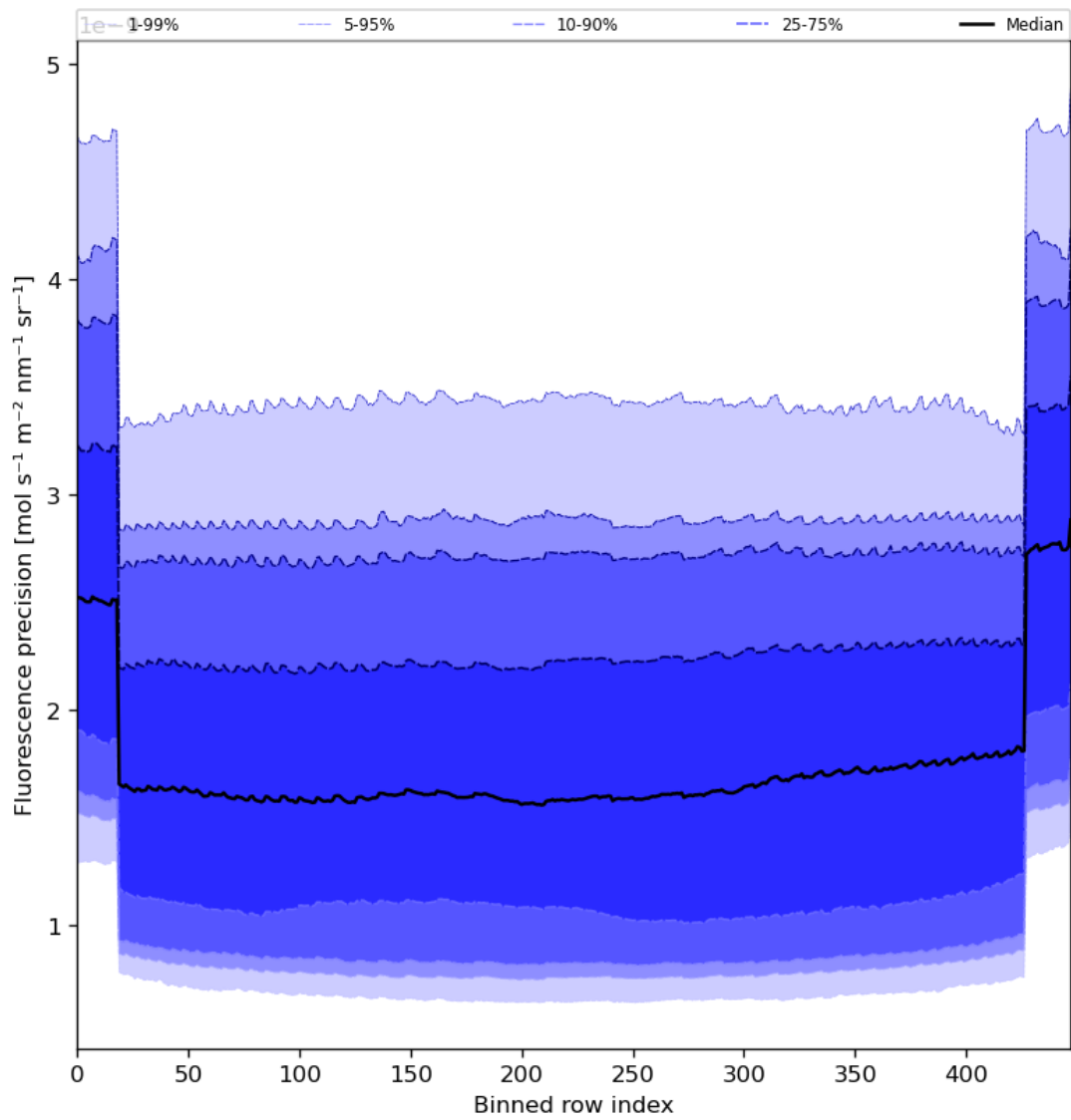
Figure 58: Along track statistics of “Fluorescence precision” for 2024-06-04 to 2024-06-06
