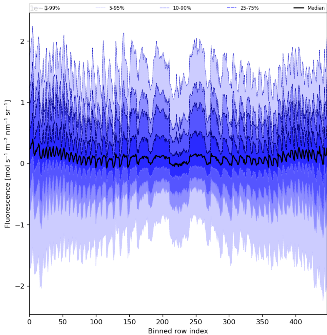
Figure 57: Along track statistics of “Fluorescence” for 2024-06-04 to 2024-06-06
