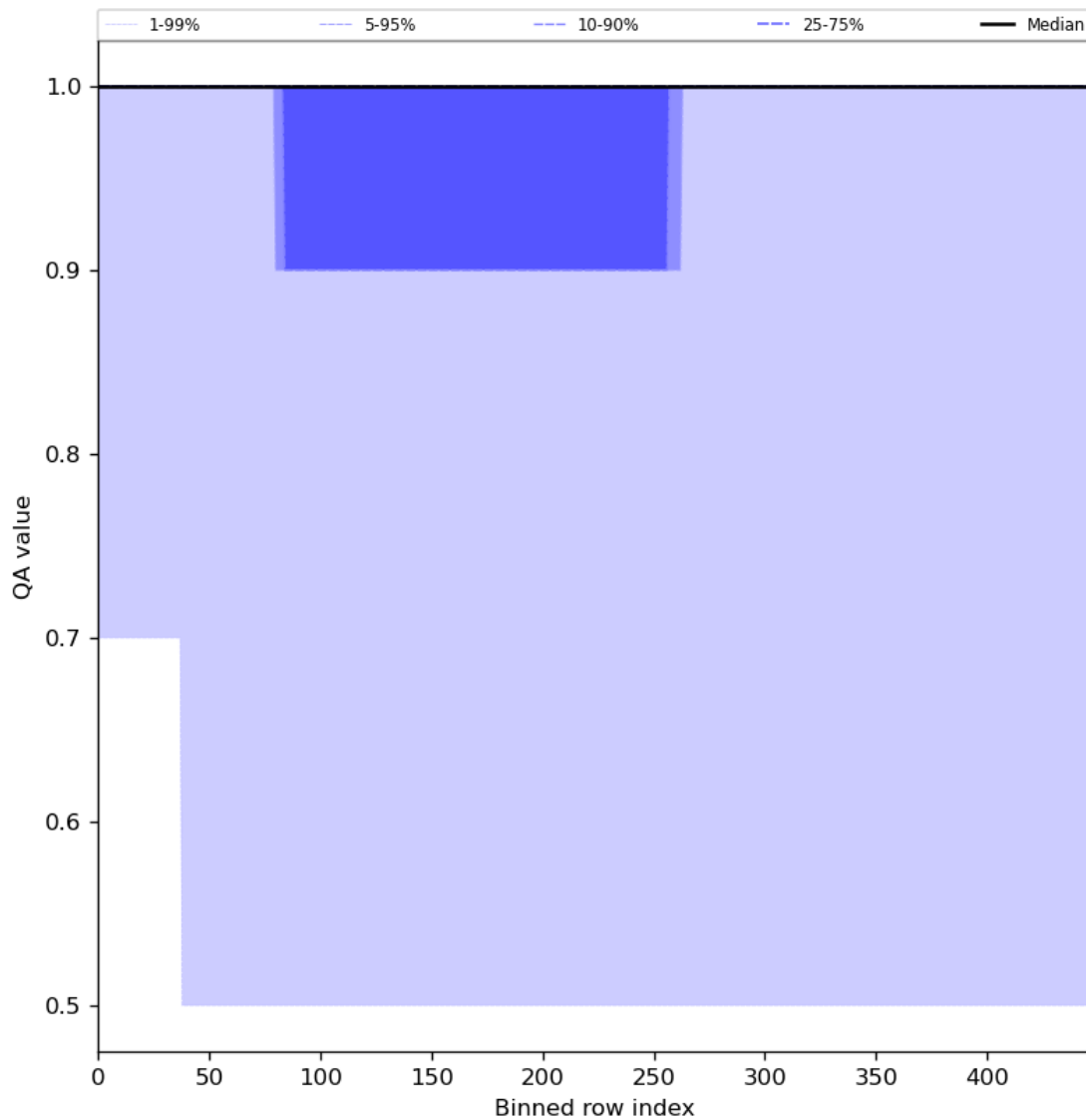
Figure 46: Along track statistics of “QA value” for 2024-06-04 to 2024-06-06
