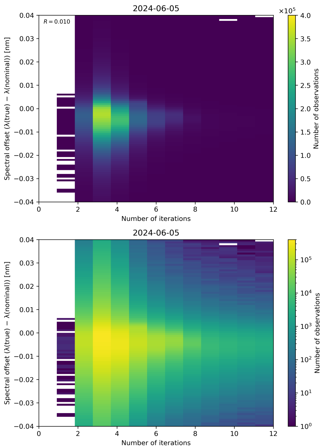
Figure 100: Scatter density plot of “Number of iterations” against “Spectral offset ( \lambda(\text{true}) - \lambda(\text{nominal}) )” for 2024-06-04 to 2024-06-06.
