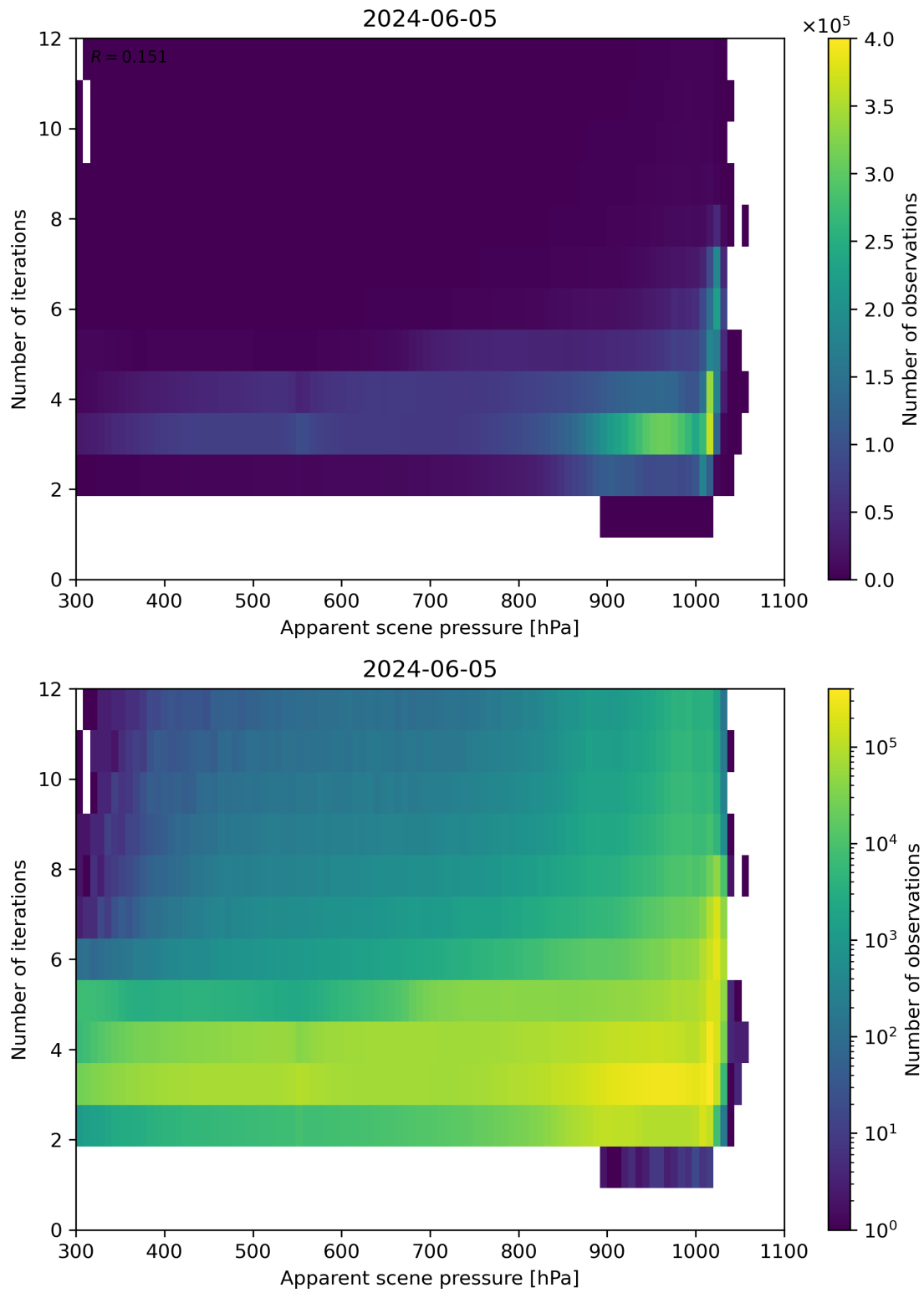
Figure 65: Scatter density plot of “Apparent scene pressure” against “Number of iterations” for 2024-06-04 to 2024-06-06.
