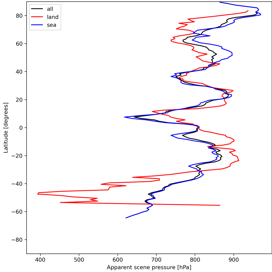
Figure 19: Zonal average of “Apparent scene pressure” for 2024-06-04 to 2024-06-06.
