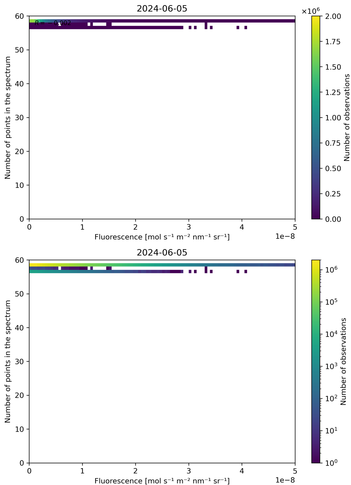
Figure 86: Scatter density plot of “Fluorescence” against “Number of points in the spectrum” for 2024-06-04 to 2024-06-06.
