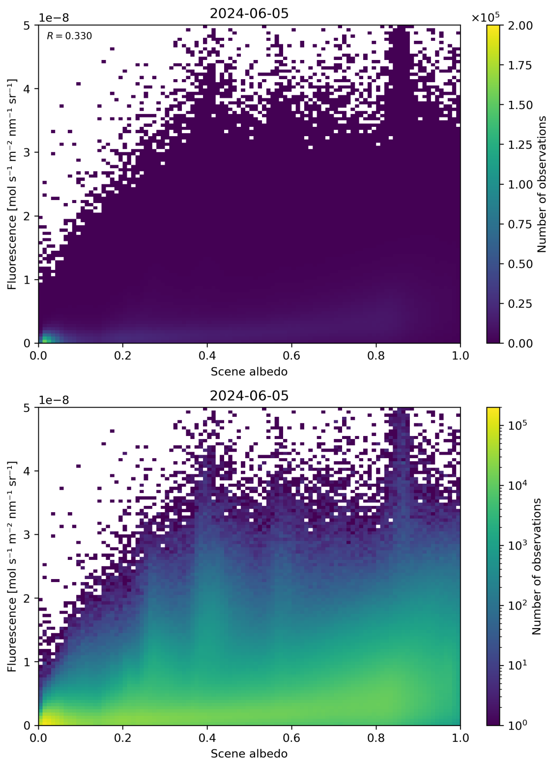
Figure 104: Scatter density plot of “Scene albedo” against “Fluorescence” for 2024-06-04 to 2024-06-06.
