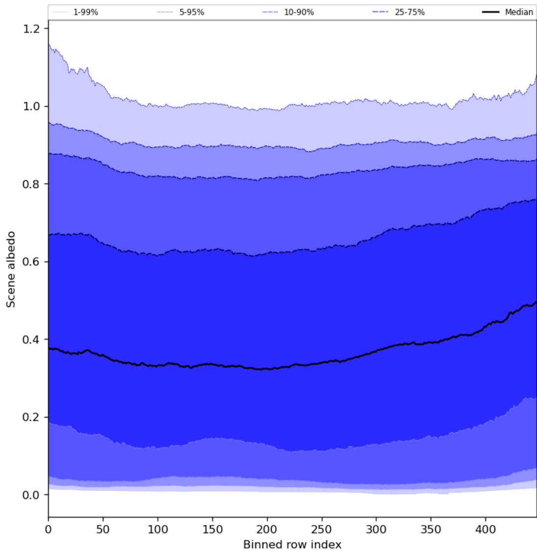
Figure 51: Along track statistics of “Scene albedo” for 2024-06-04 to 2024-06-06
