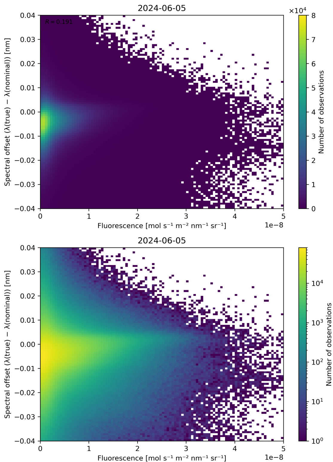
Figure 87: Scatter density plot of “Fluorescence” against “Spectral offset ( \lambda(\text{true}) - \lambda(\text{nominal}) )” for 2024-06-04 to 2024-06-06.
