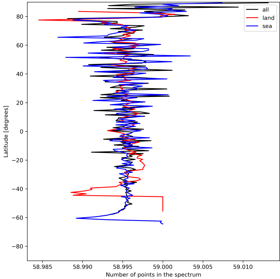
Figure 27: Zonal average of “Number of points in the spectrum” for 2024-06-04 to 2024-06-06.
