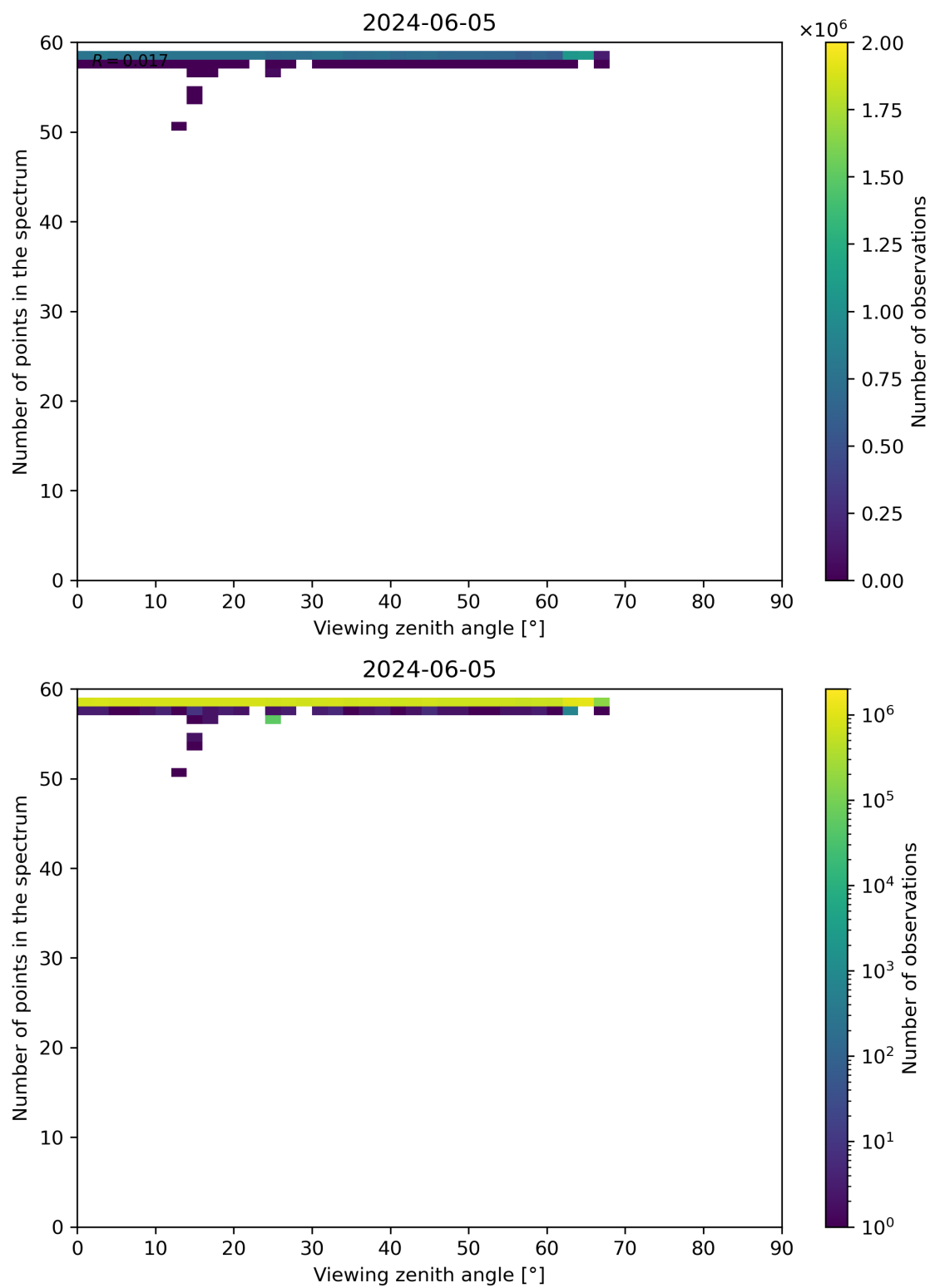
Figure 125: Scatter density plot of “Viewing zenith angle” against “Number of points in the spectrum” for 2024-06-04 to 2024-06-06.
