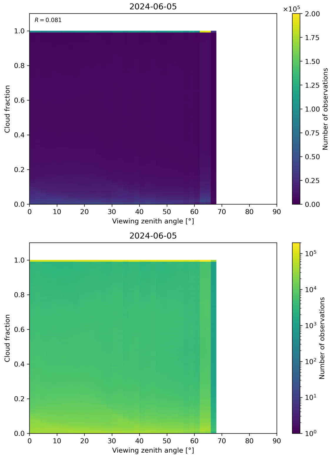
Figure 120: Scatter density plot of “Viewing zenith angle” against “Cloud fraction” for 2024-06-04 to 2024-06-06.
