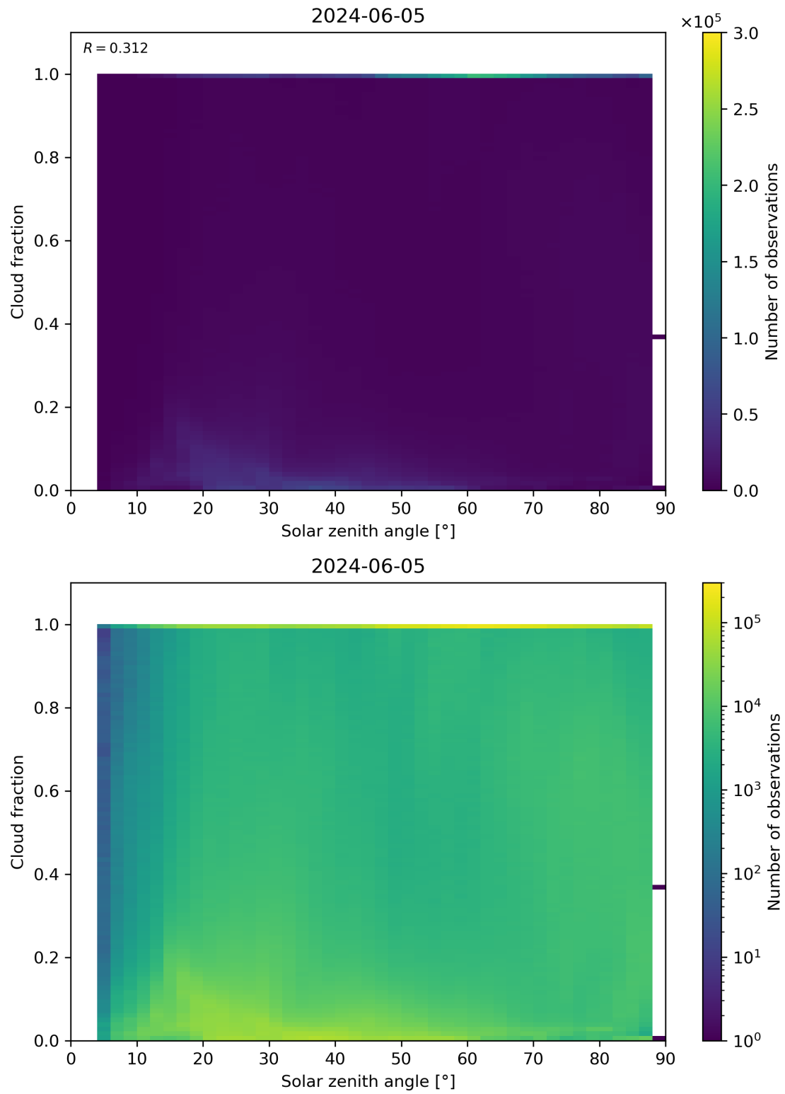
Figure 110: Scatter density plot of “Solar zenith angle” against “Cloud fraction” for 2024-06-04 to 2024-06-06.
