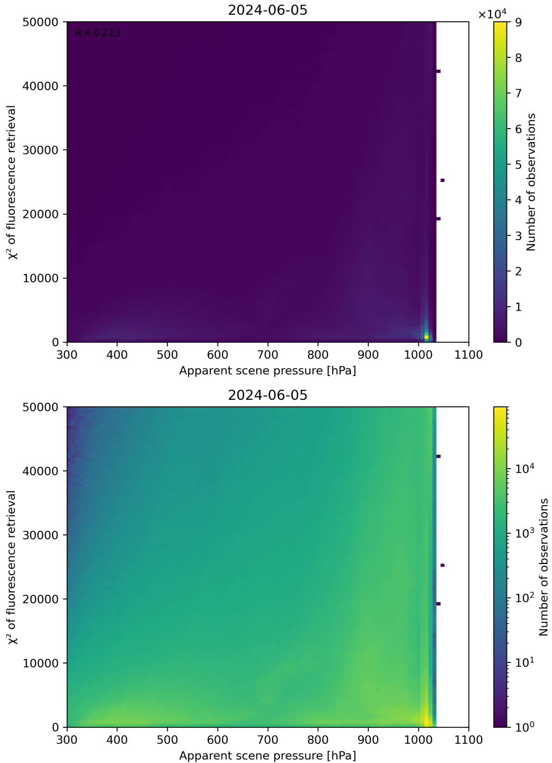
Figure 63: Scatter density plot of “Apparent scene pressure” against “ \chi^2 of fluorescence retrieval” for 2024-06-04 to 2024-06-06.
