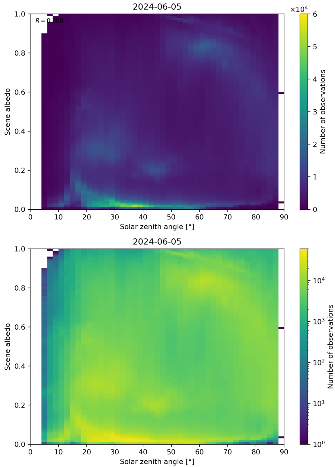
Figure 116: Scatter density plot of “Solar zenith angle” against “Scene albedo” for 2024-06-04 to 2024-06-06.
