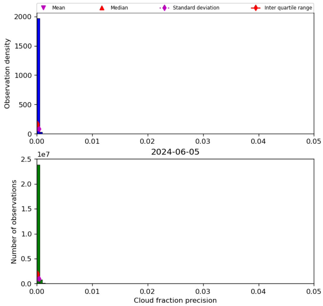
Figure 33: Histogram of “Cloud fraction precision” for 2024-06-04 to 2024-06-06
