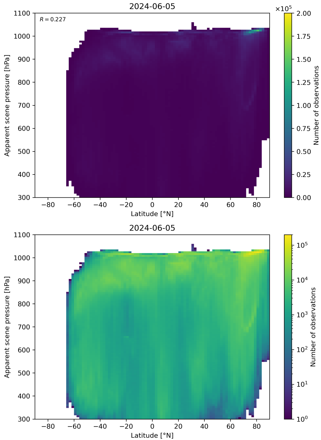
Figure 88: Scatter density plot of “Latitude” against “Apparent scene pressure” for 2024-06-04 to 2024-06-06.
