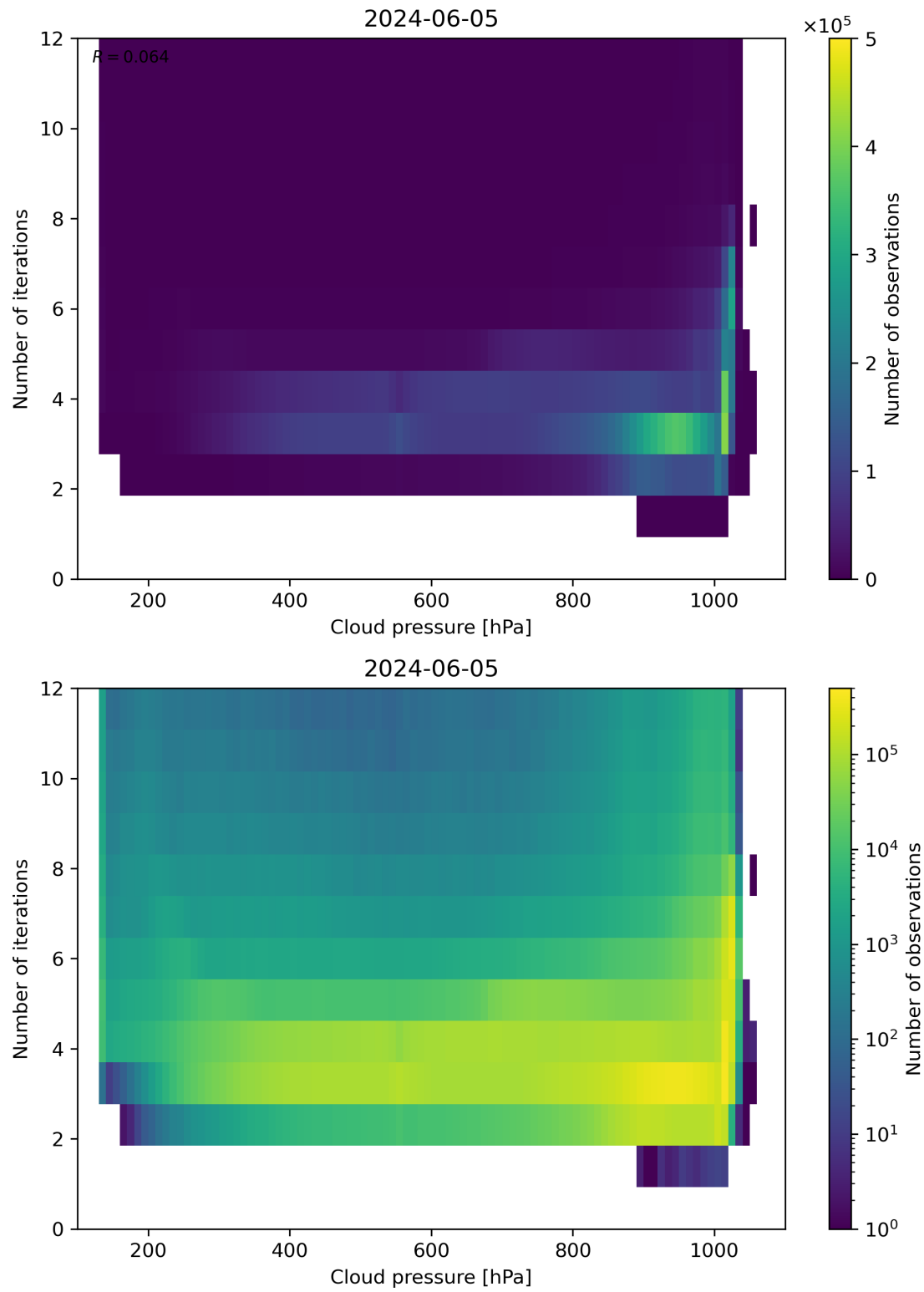
Figure 81: Scatter density plot of “Cloud pressure” against “Number of iterations” for 2024-06-04 to 2024-06-06.
