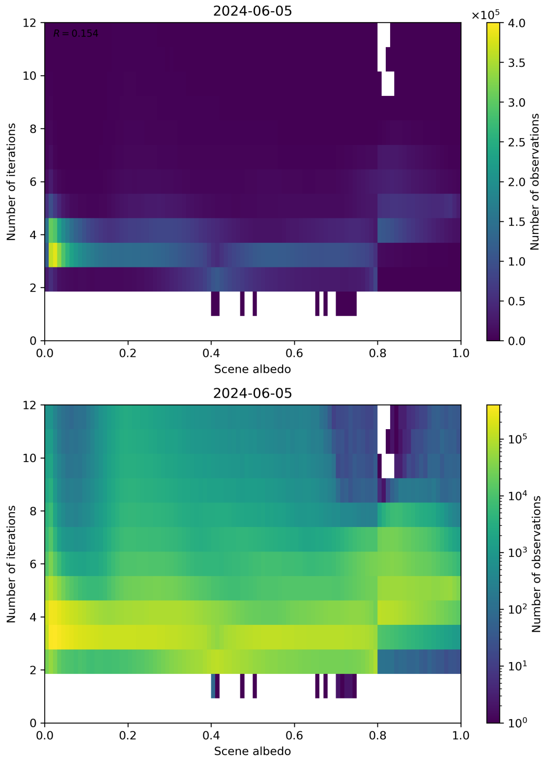
Figure 105: Scatter density plot of “Scene albedo” against “Number of iterations” for 2024-06-04 to 2024-06-06.
