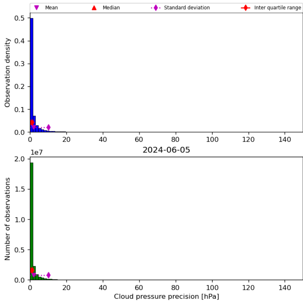
Figure 31: Histogram of “Cloud pressure precision” for 2024-06-04 to 2024-06-06
