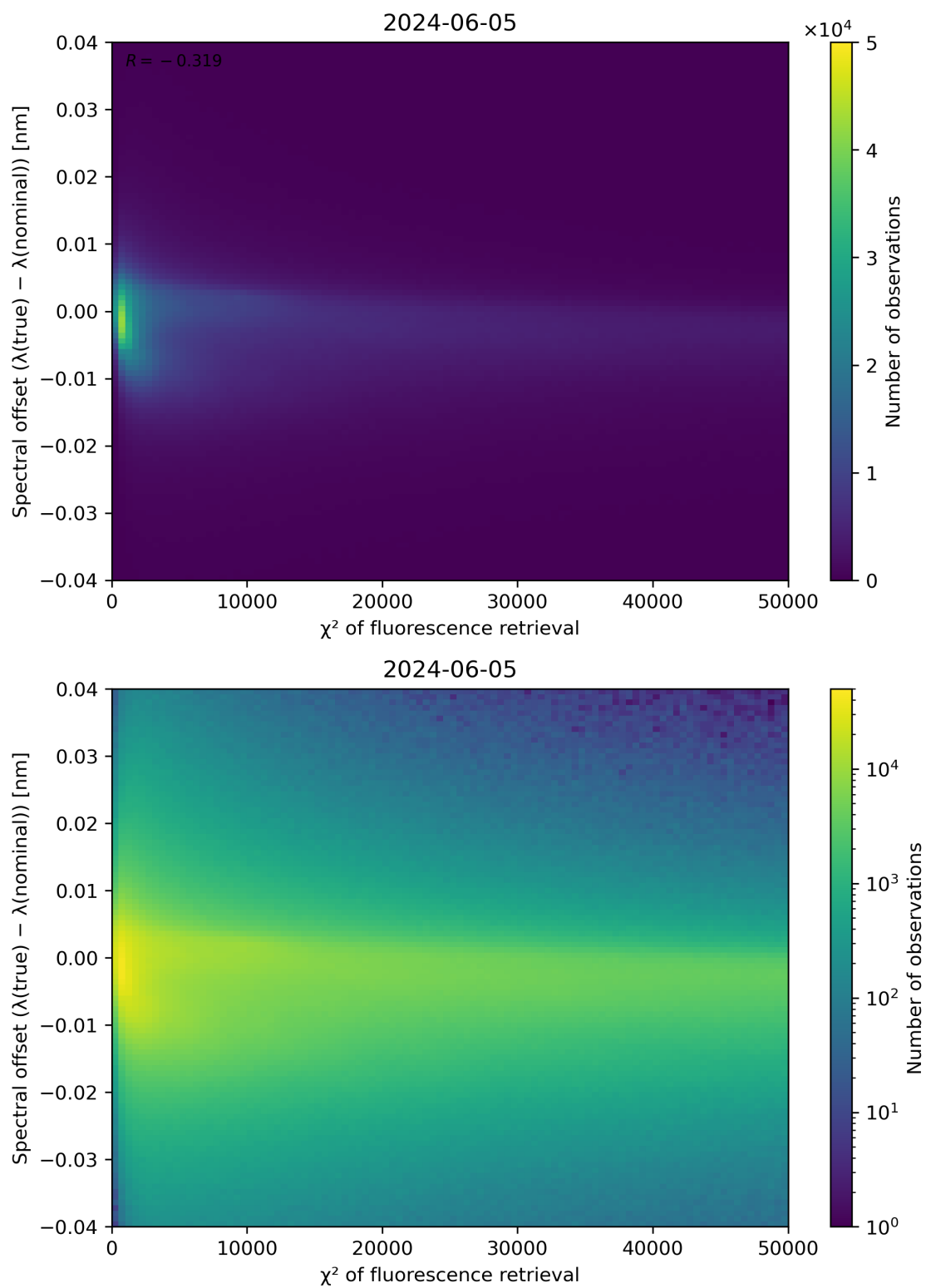
Figure 69: Scatter density plot of “ \chi^2 of fluorescence retrieval” against “Spectral offset ( \lambda(\text{true}) - \lambda(\text{nominal}) )” for 2024-06-04 to 2024-06-06.
