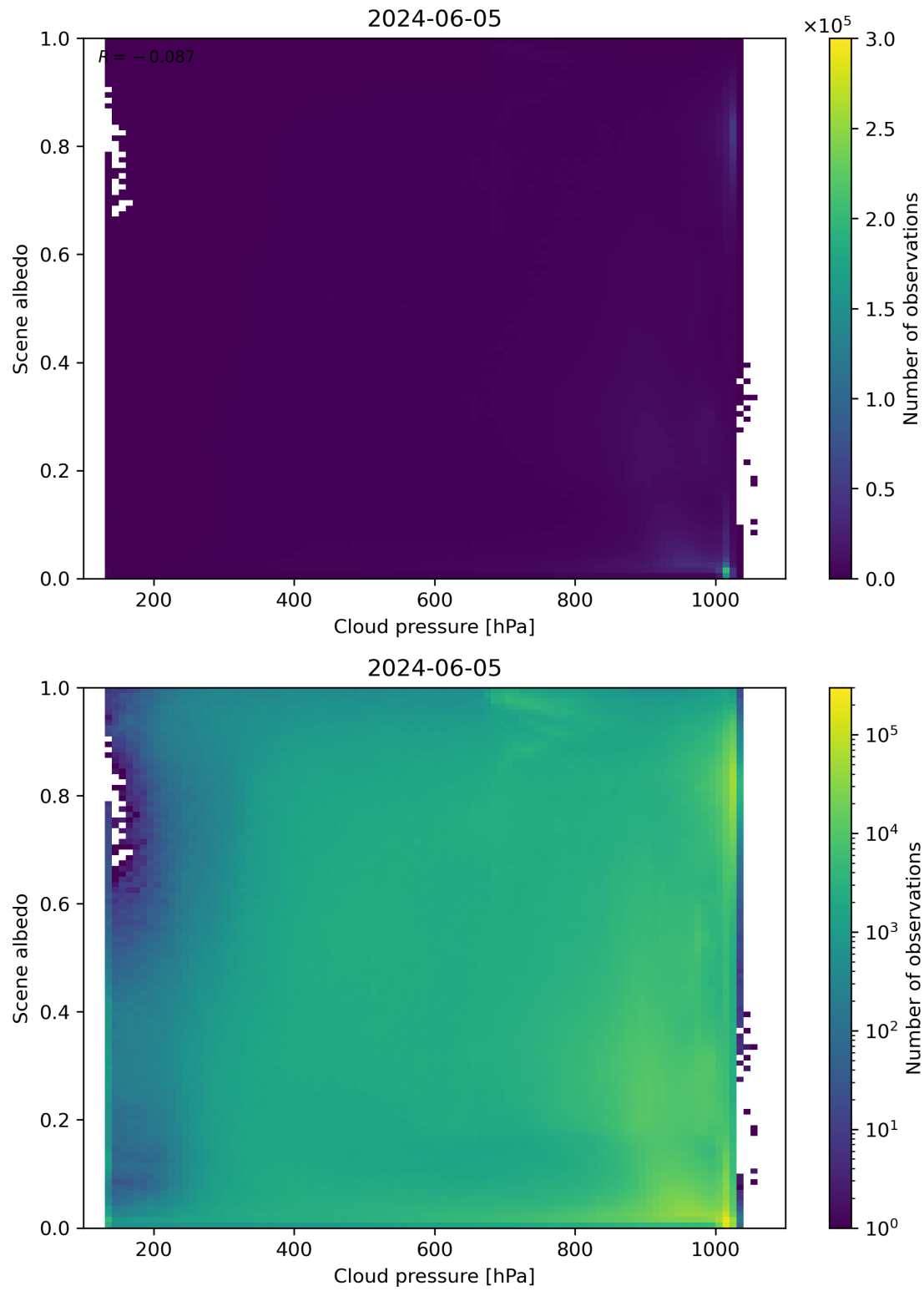
Figure 83: Scatter density plot of “Cloud pressure” against “Scene albedo” for 2024-06-04 to 2024-06-06.
