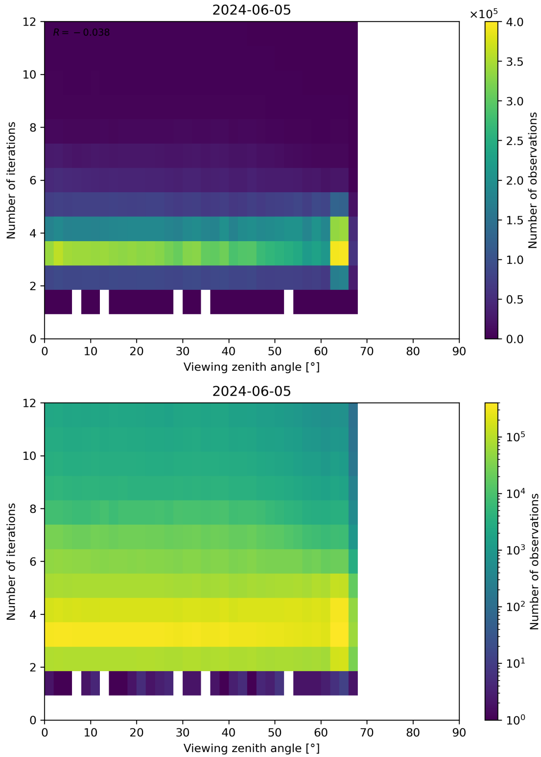
Figure 124: Scatter density plot of “Viewing zenith angle” against “Number of iterations” for 2024-06-04 to 2024-06-06.
