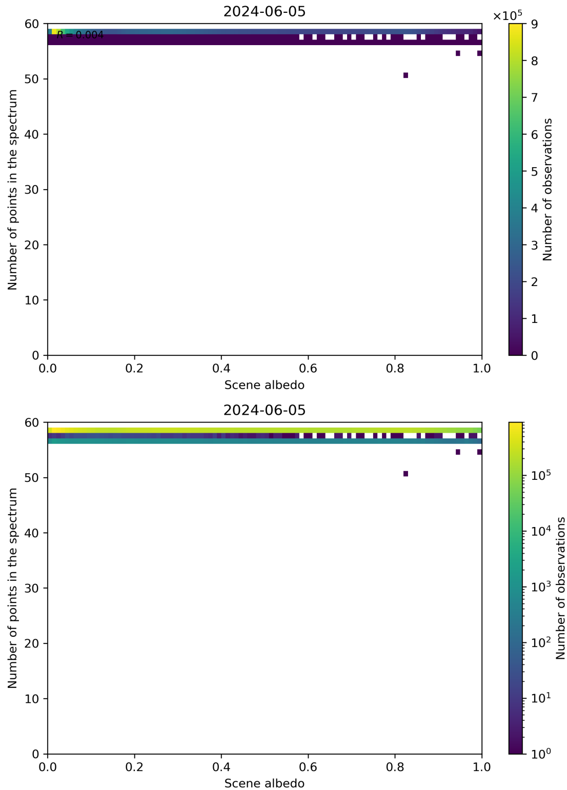
Figure 106: Scatter density plot of “Scene albedo” against “Number of points in the spectrum” for 2024-06-04 to 2024-06-06.
