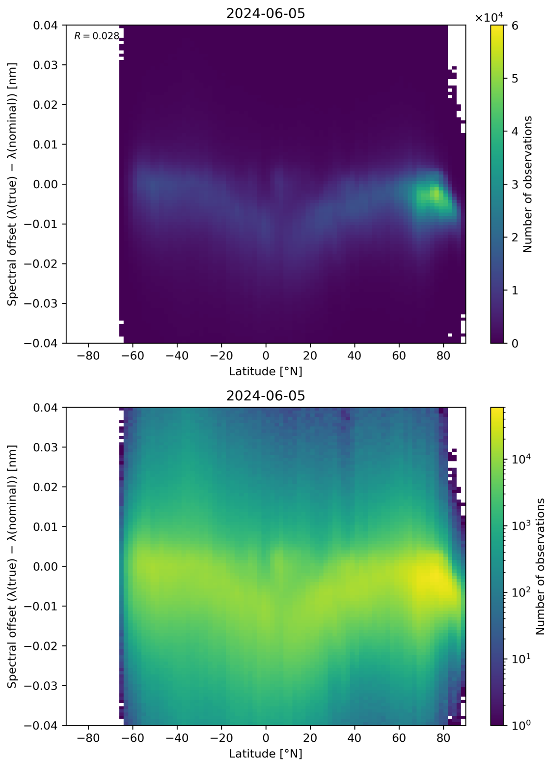
Figure 96: Scatter density plot of “Latitude” against “Spectral offset ( \lambda(\text{true}) - \lambda(\text{nominal}) )” for 2024-06-04 to 2024-06-06.
