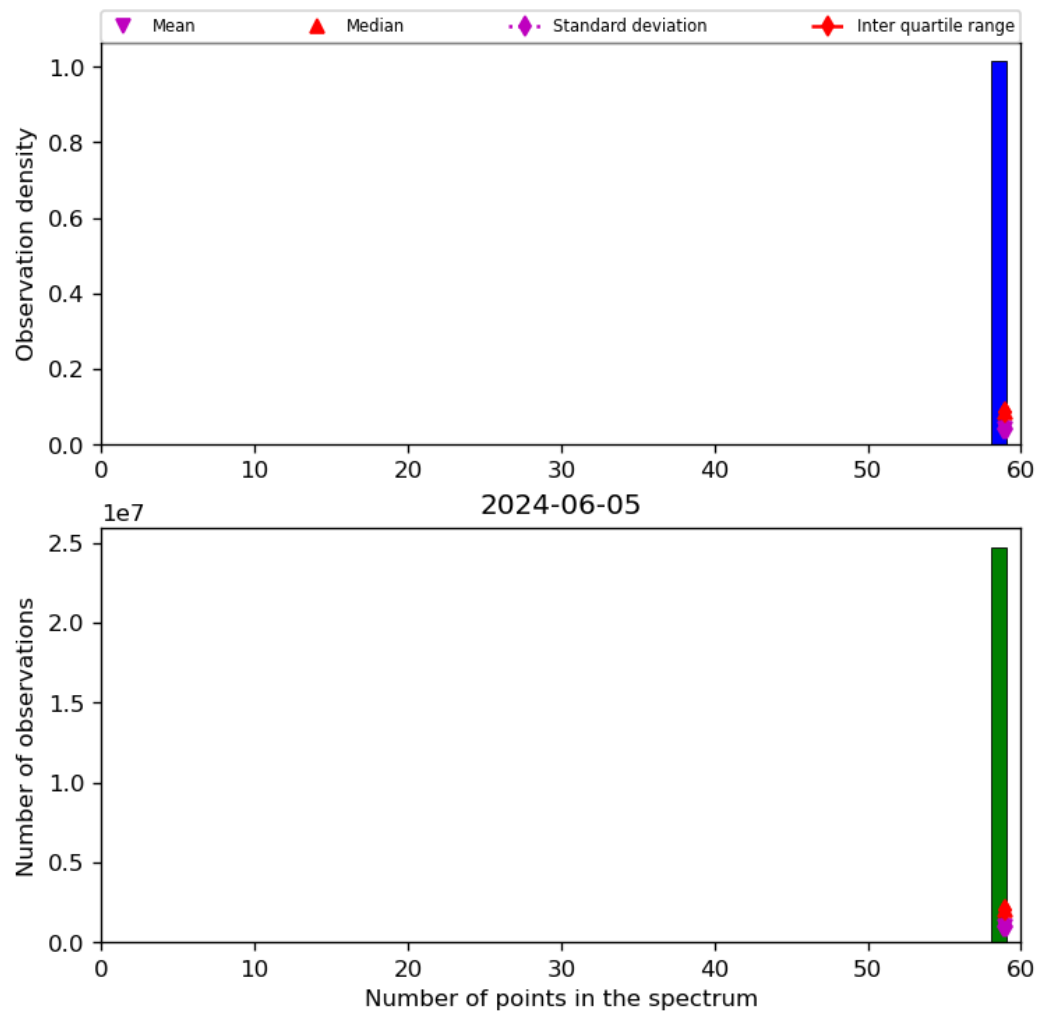
Figure 44: Histogram of “Number of points in the spectrum” for 2024-06-04 to 2024-06-06
