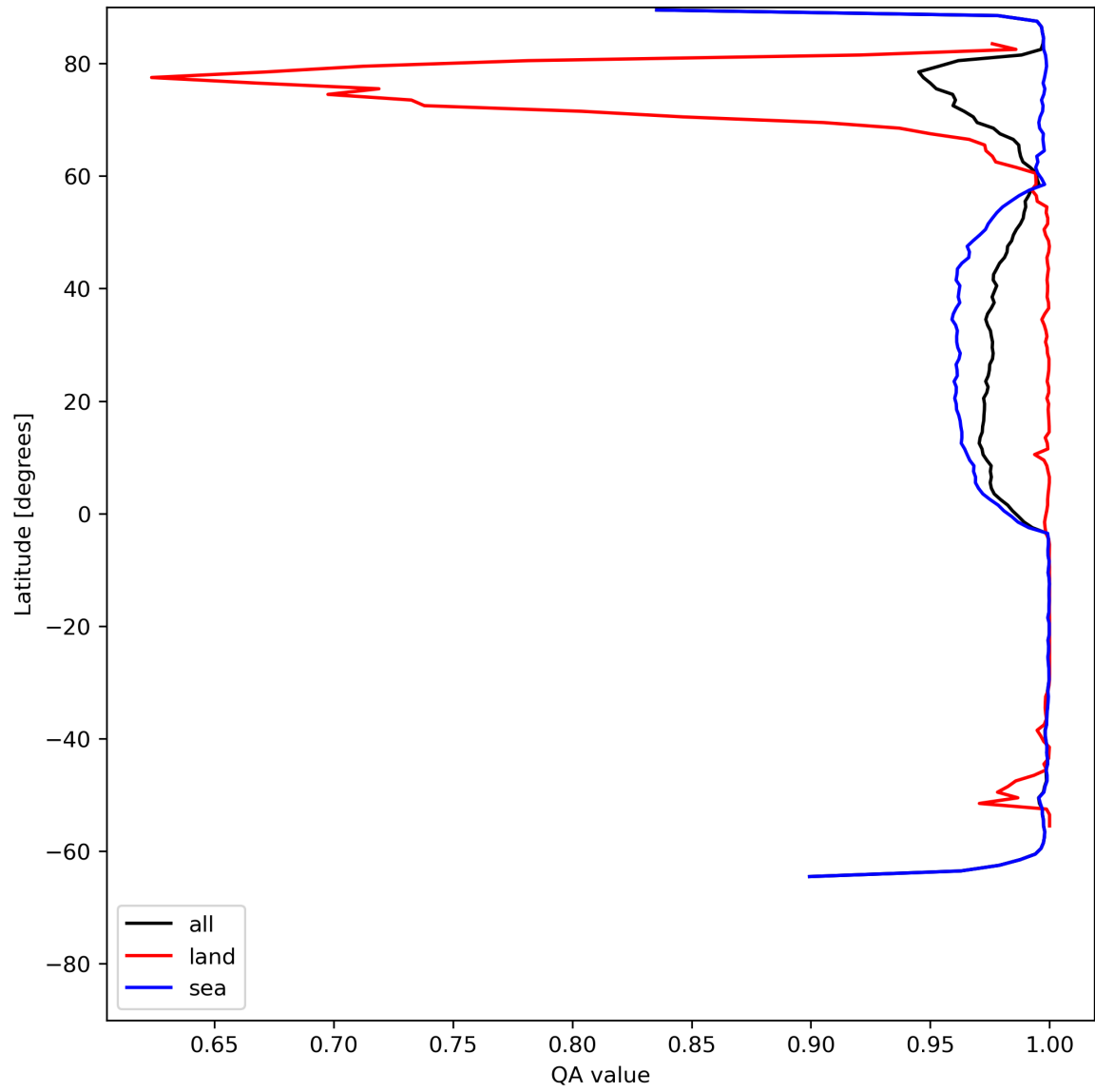
Figure 12: Zonal average of “QA value” for 2024-06-04 to 2024-06-06.
