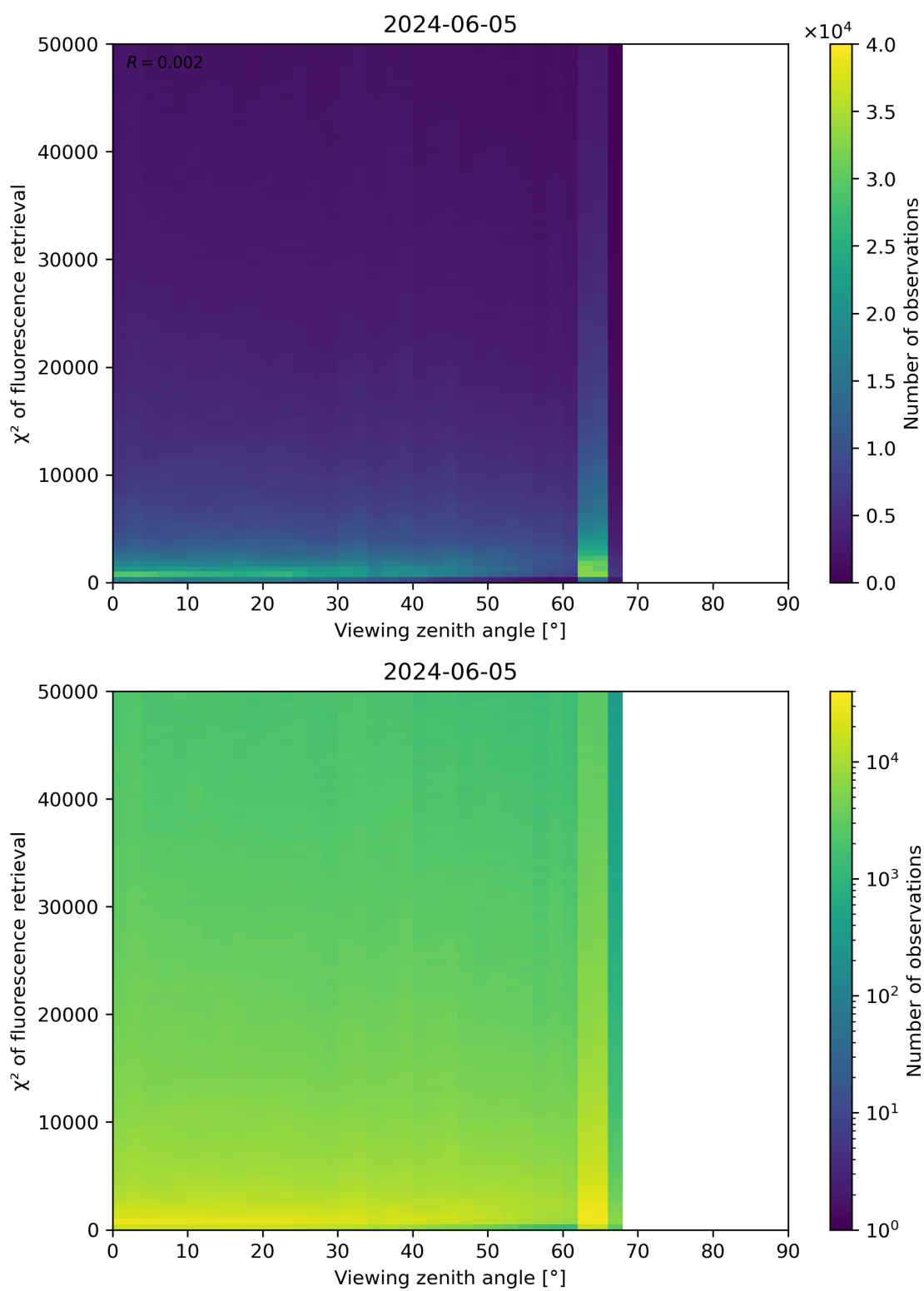
Figure 119: Scatter density plot of “Viewing zenith angle” against “ \chi^2 of fluorescence retrieval” for 2024-06-04 to 2024-06-06.
