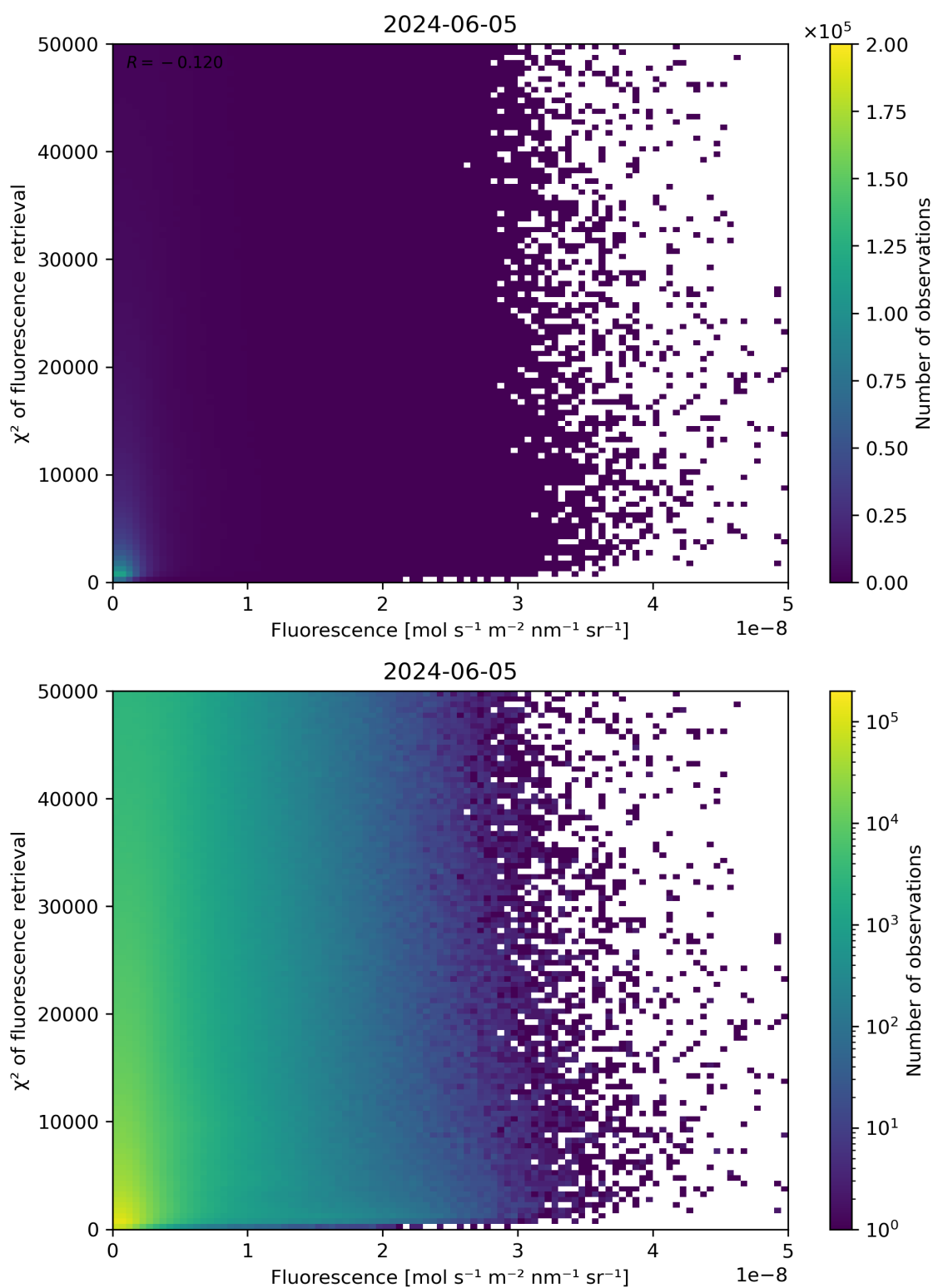
Figure 85: Scatter density plot of “Fluorescence” against “ \chi^2 of fluorescence retrieval” for 2024-06-04 to 2024-06-06.
