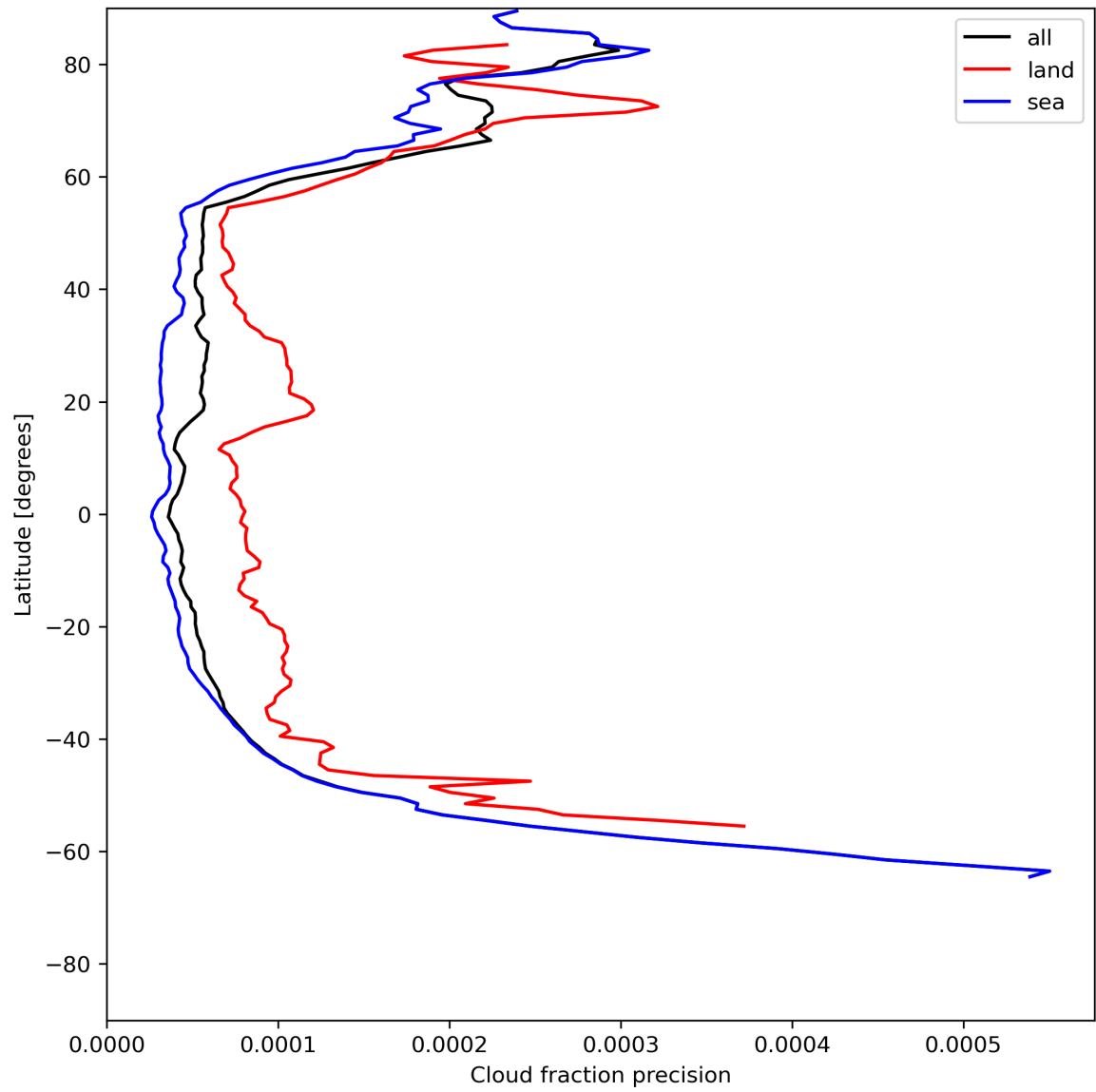
Figure 16: Zonal average of “Cloud fraction precision” for 2024-06-04 to 2024-06-06.
