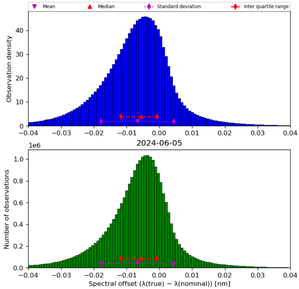
Figure 45: Histogram of “Spectral offset ( \lambda(\text{true}) - \lambda(\text{nominal}) )” for 2024-06-04 to 2024-06-06
