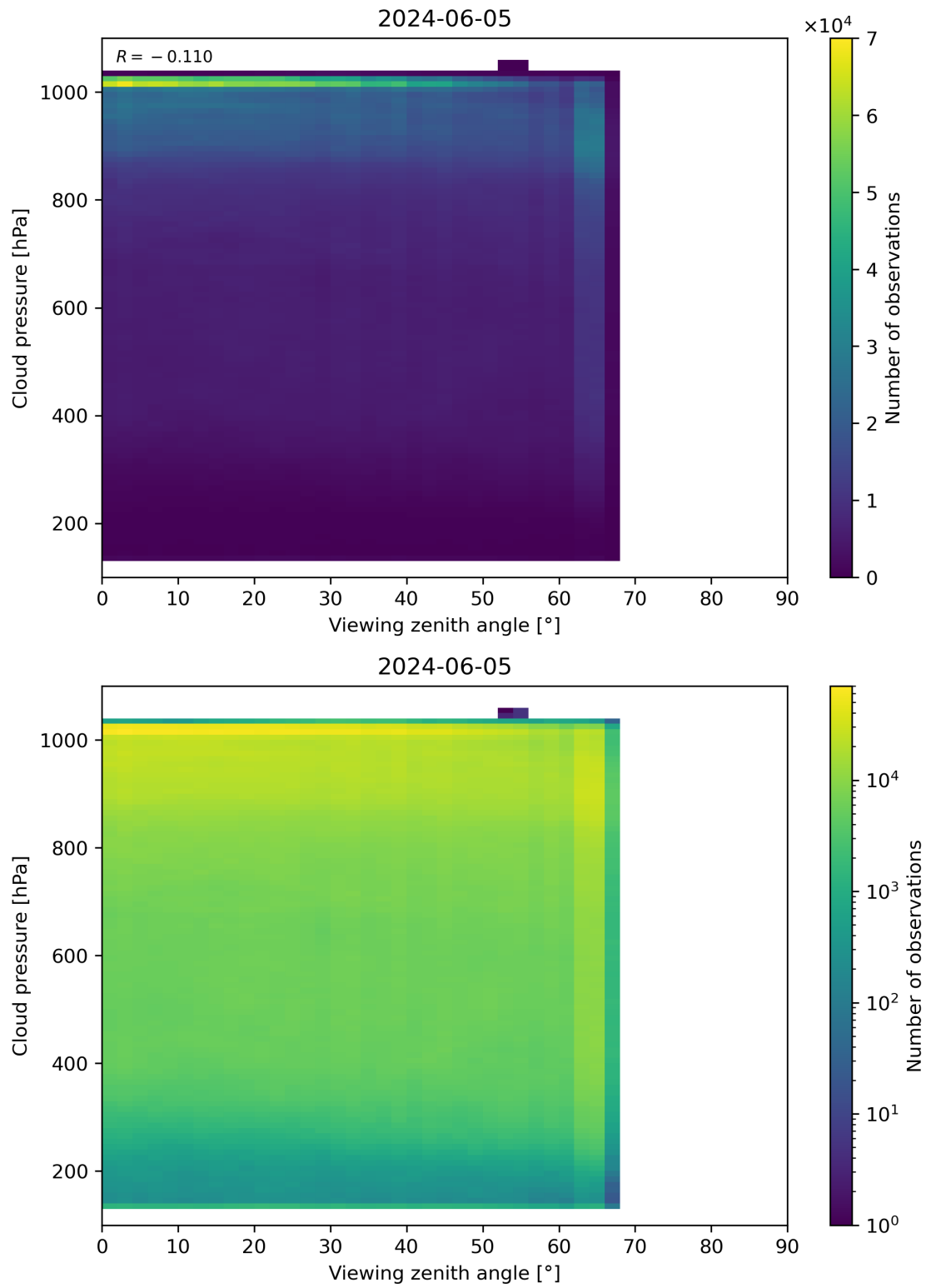
Figure 121: Scatter density plot of “Viewing zenith angle” against “Cloud pressure” for 2024-06-04 to 2024-06-06.
