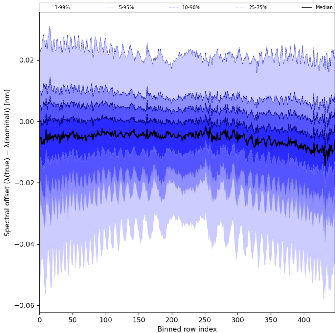
Figure 62: Along track statistics of “Spectral offset ( \lambda(\text{true}) - \lambda(\text{nominal}) )” for 2024-06-04 to 2024-06-06
