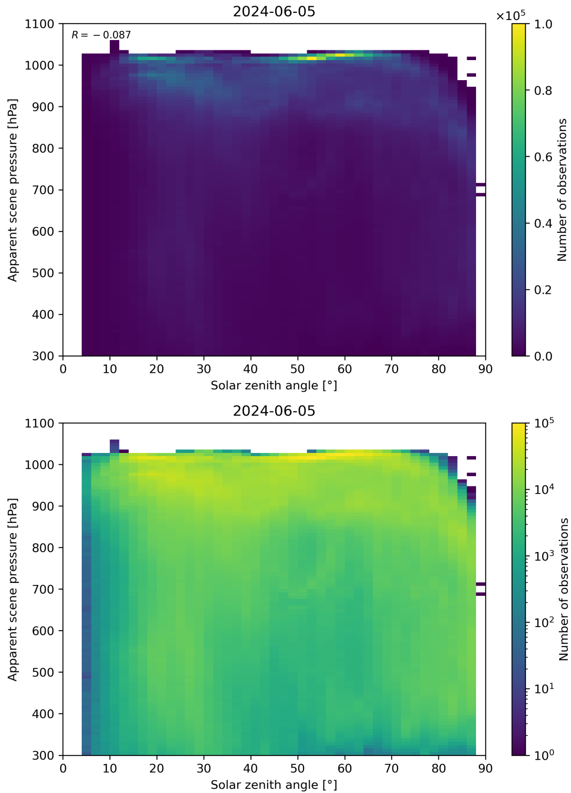
Figure 108: Scatter density plot of “Solar zenith angle” against “Apparent scene pressure” for 2024-06-04 to 2024-06-06.
