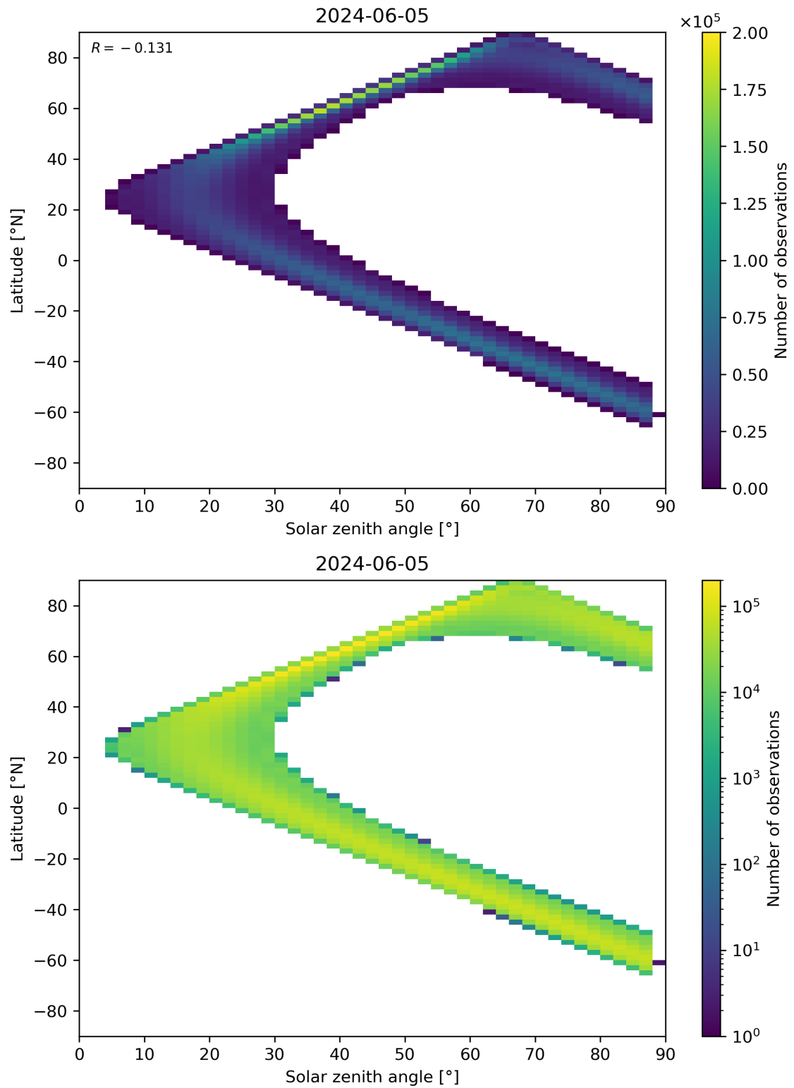
Figure 113: Scatter density plot of “Solar zenith angle” against “Latitude” for 2024-06-04 to 2024-06-06.
