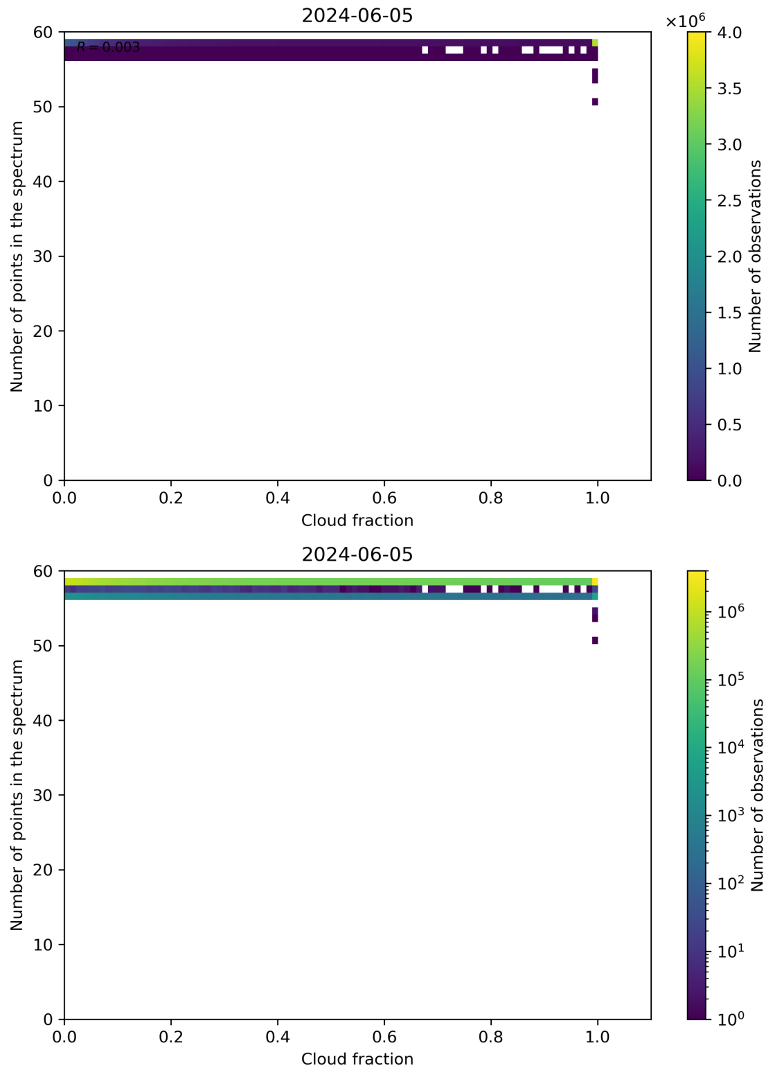
Figure 74: Scatter density plot of “Cloud fraction” against “Number of points in the spectrum” for 2024-06-04 to 2024-06-06.
