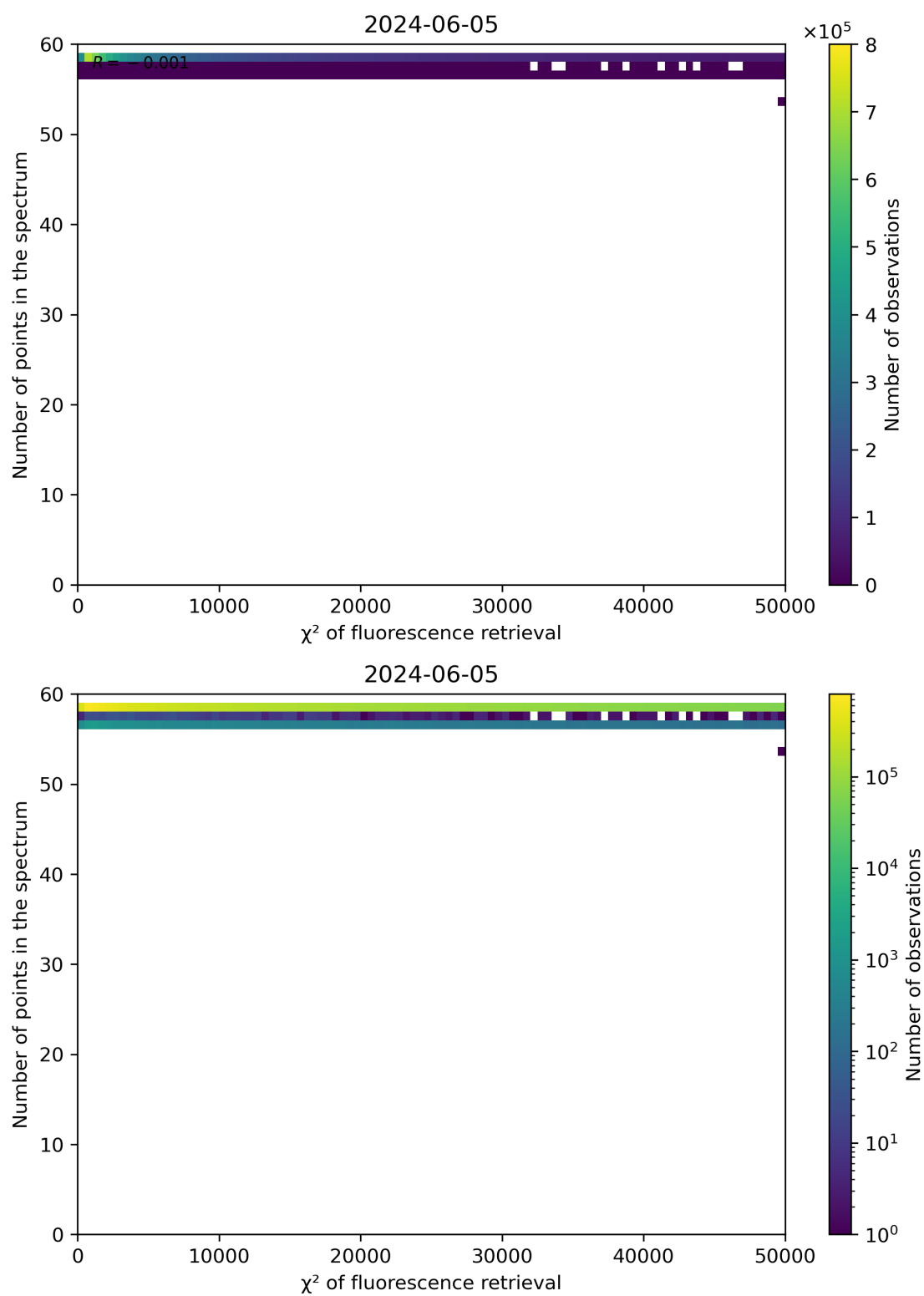
Figure 68: Scatter density plot of " \chi^2 of fluorescence retrieval" against "Number of points in the spectrum" for 2024-06-04 to 2024-06-06.
