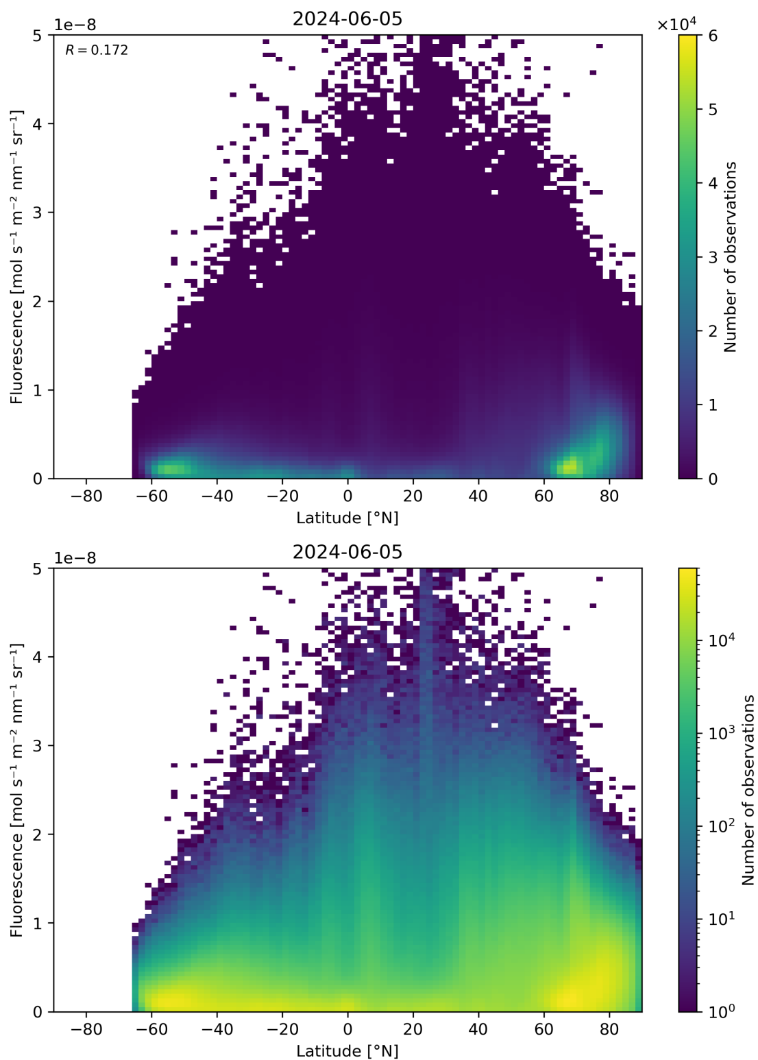
Figure 92: Scatter density plot of “Latitude” against “Fluorescence” for 2024-06-04 to 2024-06-06.
