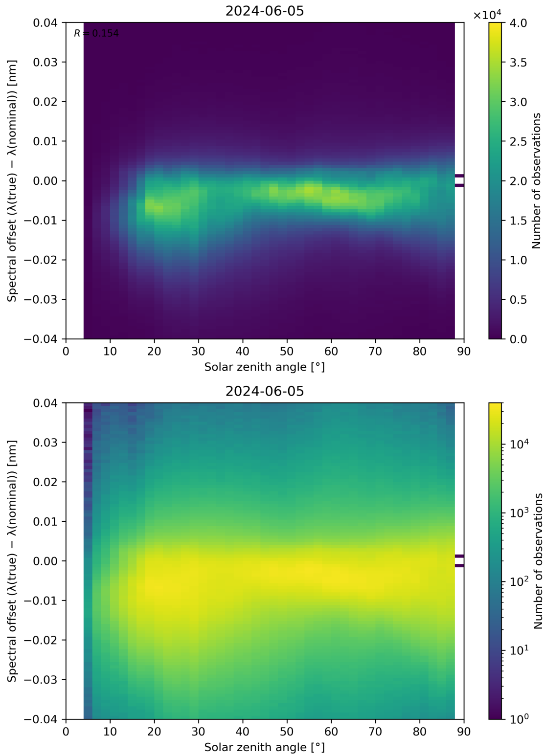
Figure 117: Scatter density plot of “Solar zenith angle” against “Spectral offset ( \lambda(\text{true}) - \lambda(\text{nominal}) )” for 2024-06-04 to 2024-06-06.
