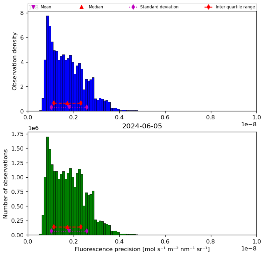
Figure 41: Histogram of “Fluorescence precision” for 2024-06-04 to 2024-06-06
