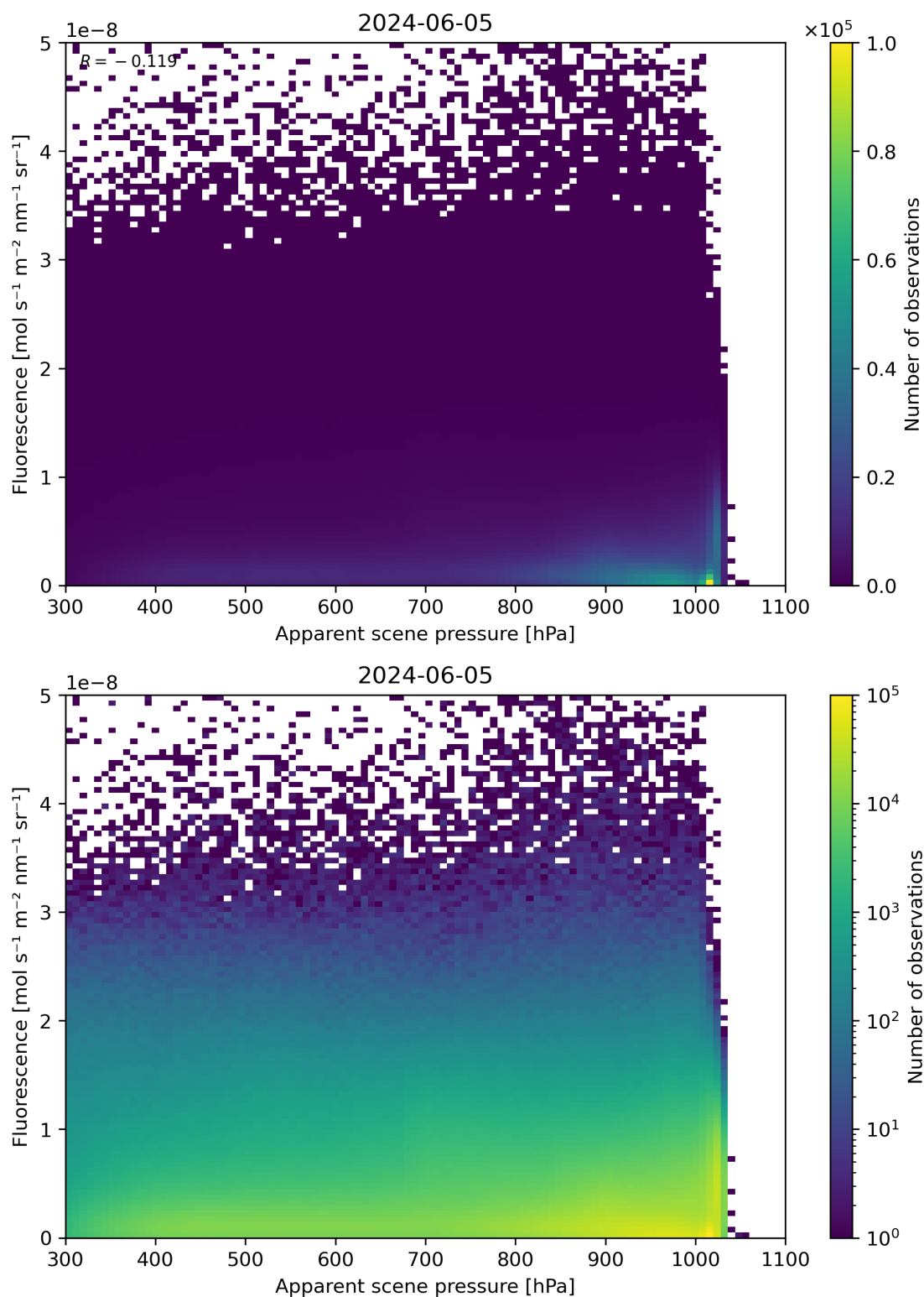
Figure 64: Scatter density plot of “Apparent scene pressure” against “Fluorescence” for 2024-06-04 to 2024-06-06.
