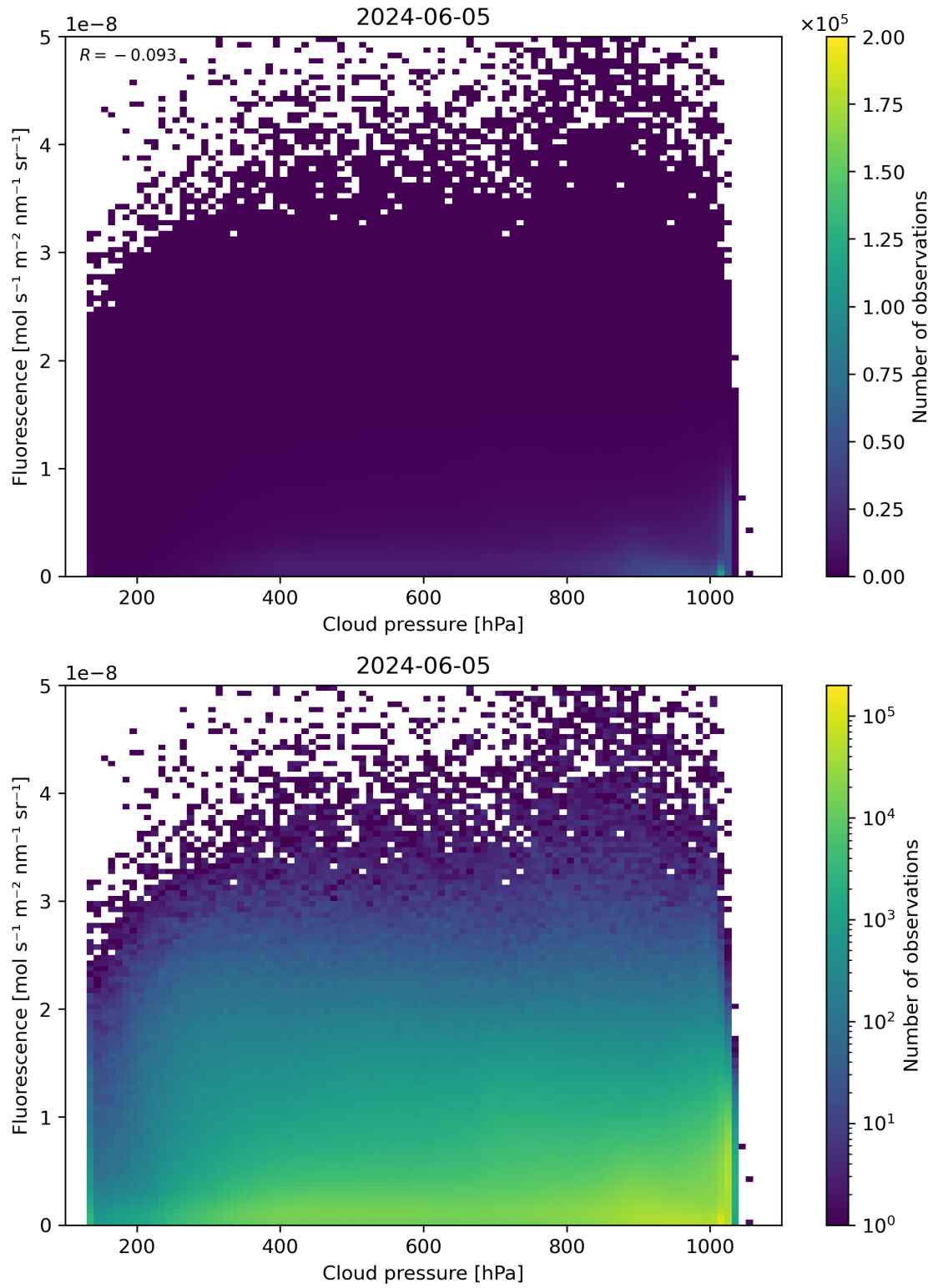
Figure 80: Scatter density plot of “Cloud pressure” against “Fluorescence” for 2024-06-04 to 2024-06-06.
