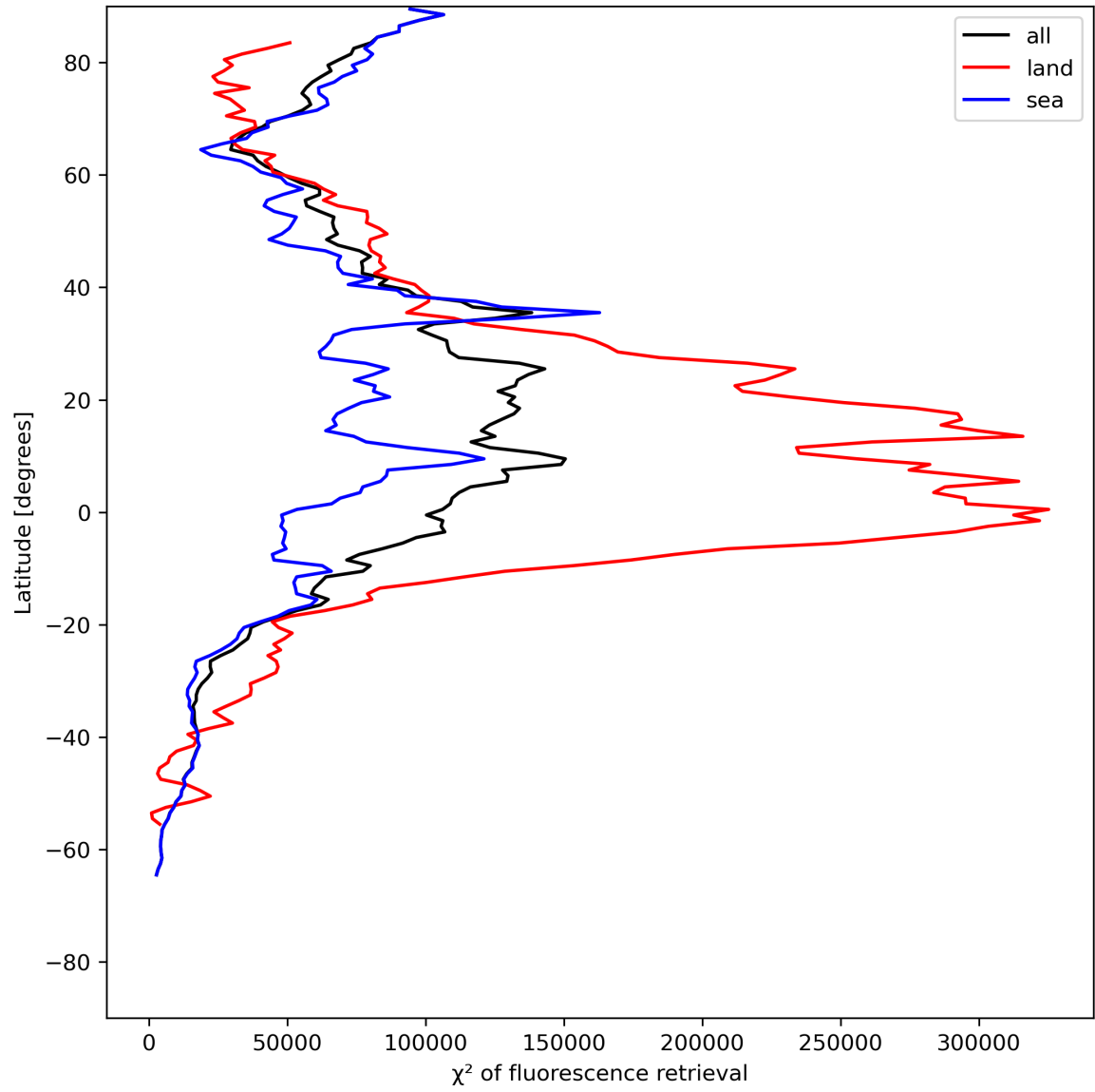
Figure 25: Zonal average of “ \chi^2 of fluorescence retrieval” for 2024-06-04 to 2024-06-06.
