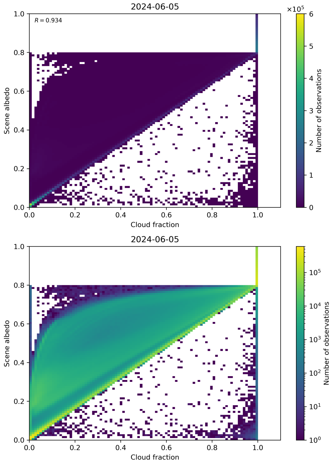
Figure 75: Scatter density plot of “Cloud fraction” against “Scene albedo” for 2024-06-04 to 2024-06-06.
