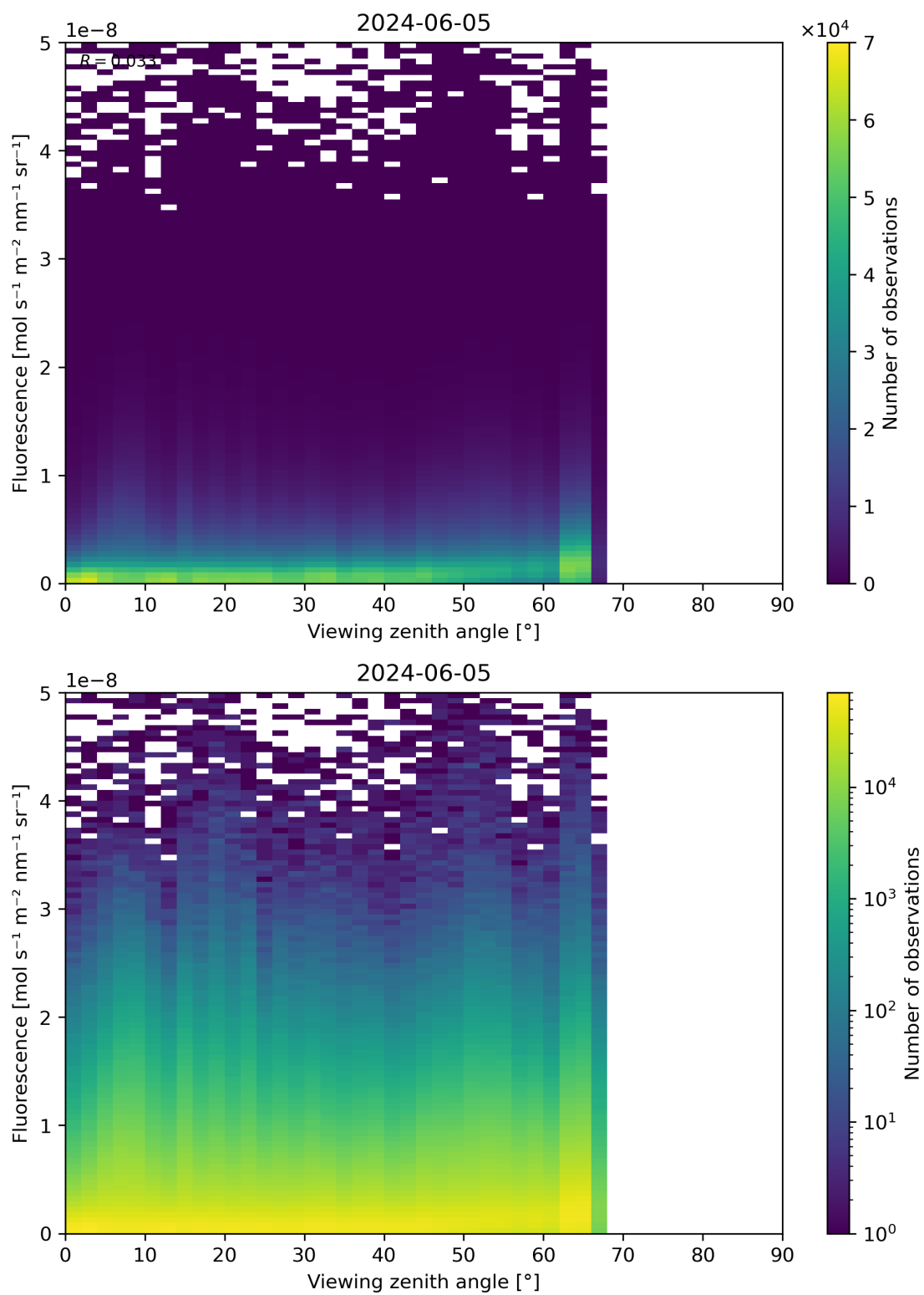
Figure 122: Scatter density plot of “Viewing zenith angle” against “Fluorescence” for 2024-06-04 to 2024-06-06.
