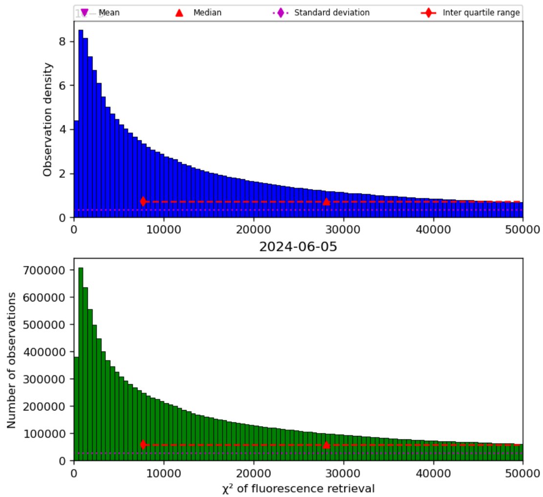
Figure 42: Histogram of “ \chi^2 of fluorescence retrieval” for 2024-06-04 to 2024-06-06
