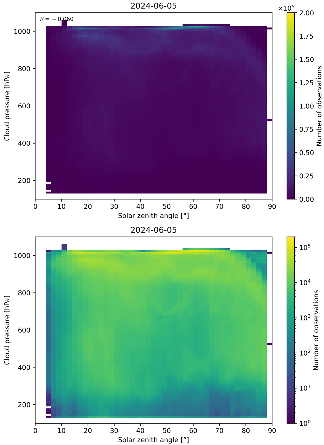
Figure 111: Scatter density plot of “Solar zenith angle” against “Cloud pressure” for 2024-06-04 to 2024-06-06.
