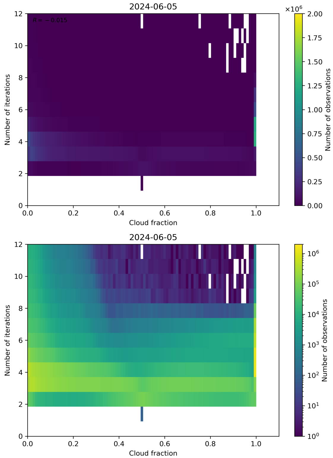
Figure 73: Scatter density plot of “Cloud fraction” against “Number of iterations” for 2024-06-04 to 2024-06-06.
