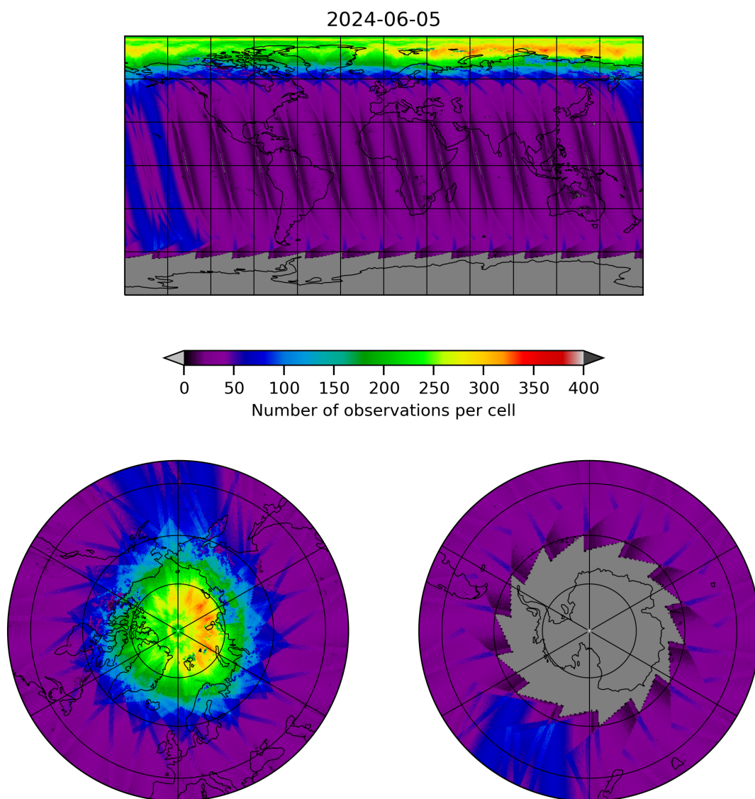
Figure 11: Map of the number of observations for 2024-06-04 to 2024-06-06
