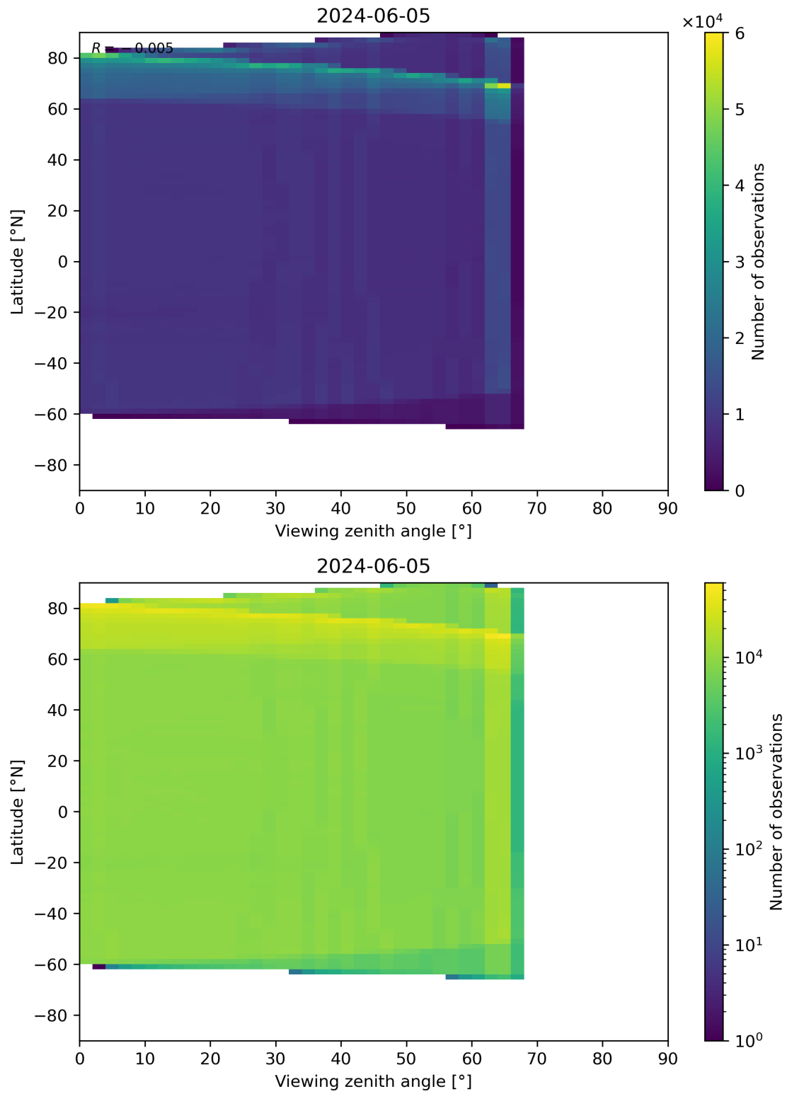
Figure 123: Scatter density plot of “Viewing zenith angle” against “Latitude” for 2024-06-04 to 2024-06-06.
