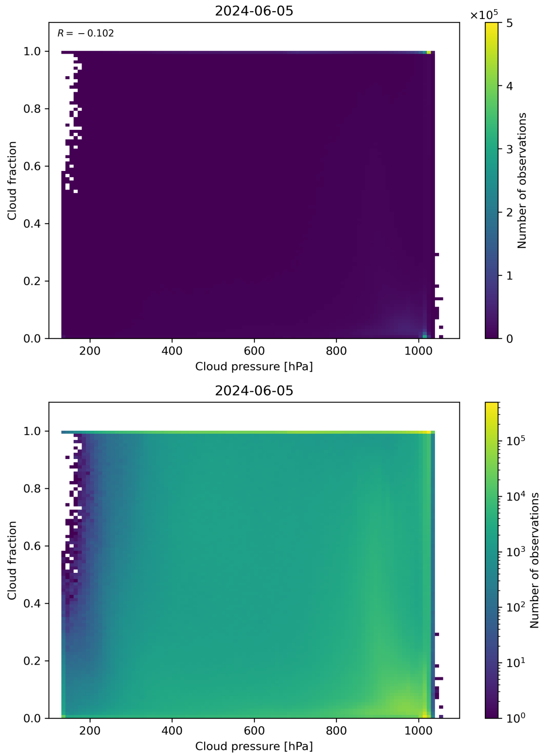
Figure 79: Scatter density plot of “Cloud pressure” against “Cloud fraction” for 2024-06-04 to 2024-06-06.
