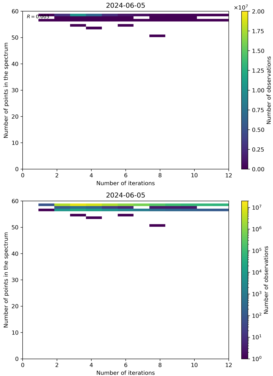
Figure 99: Scatter density plot of “Number of iterations” against “Number of points in the spectrum” for 2024-06-04 to 2024-06-06.
