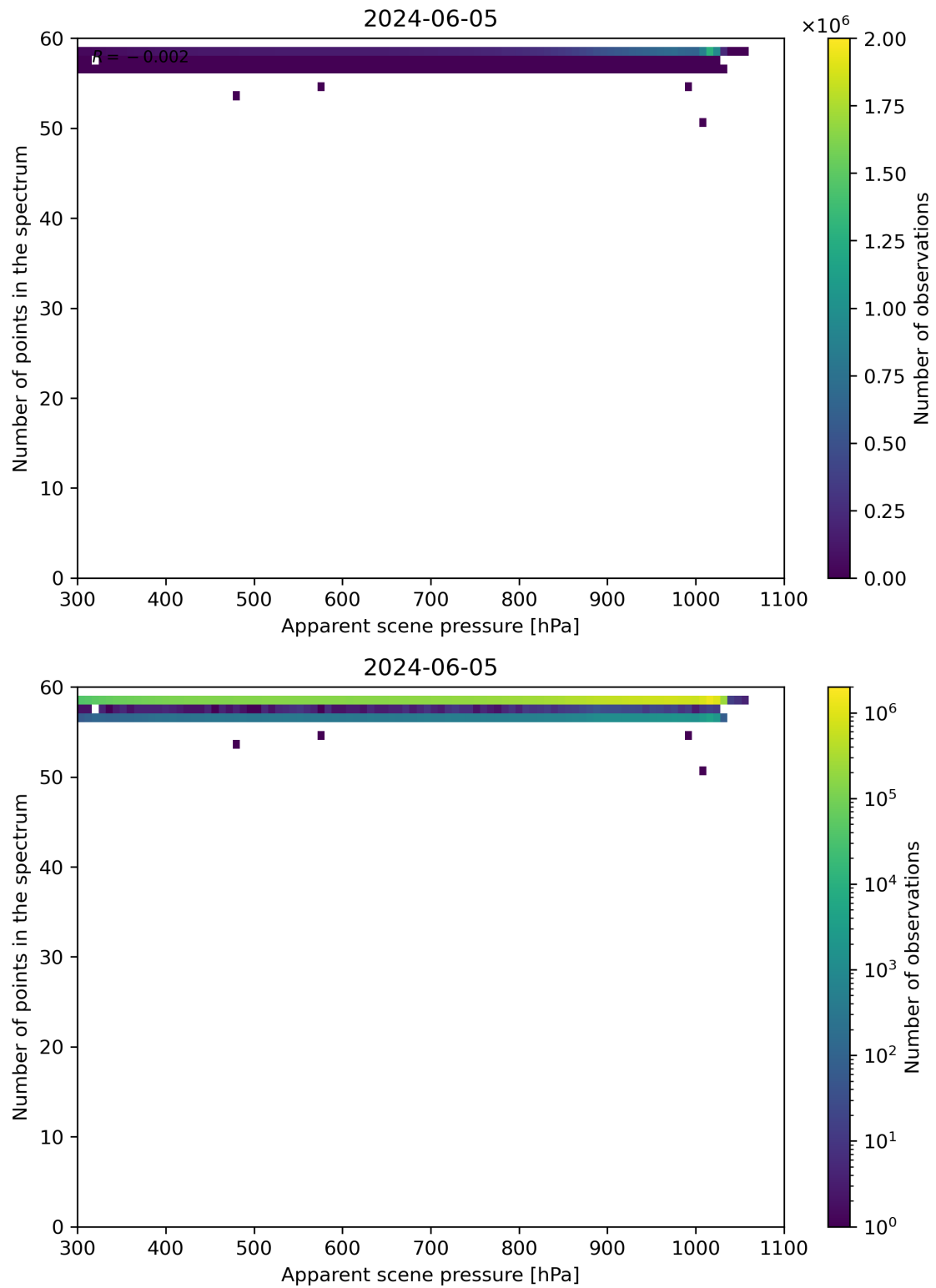
Figure 66: Scatter density plot of “Apparent scene pressure” against “Number of points in the spectrum” for 2024-06-04 to 2024-06-06.
