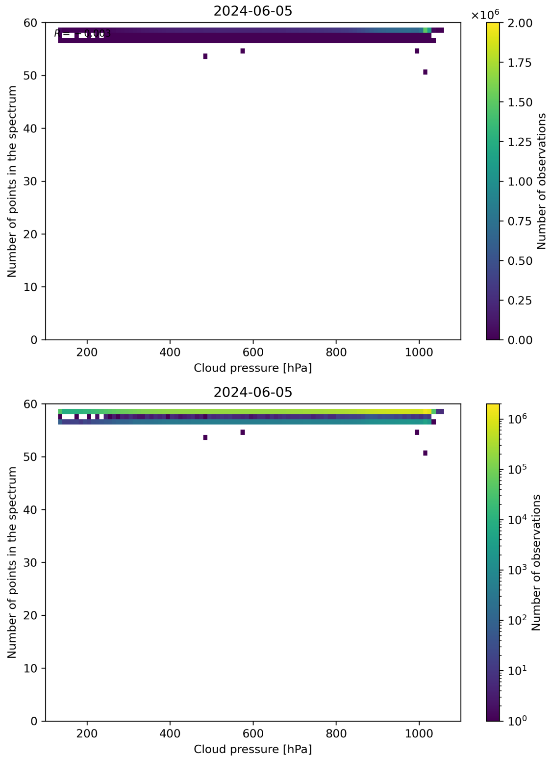
Figure 82: Scatter density plot of “Cloud pressure” against “Number of points in the spectrum” for 2024-06-04 to 2024-06-06.
