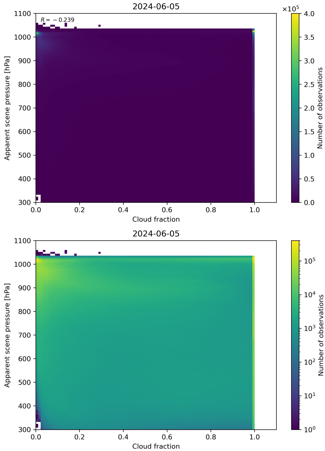
Figure 70: Scatter density plot of “Cloud fraction” against “Apparent scene pressure” for 2024-06-04 to 2024-06-06.
