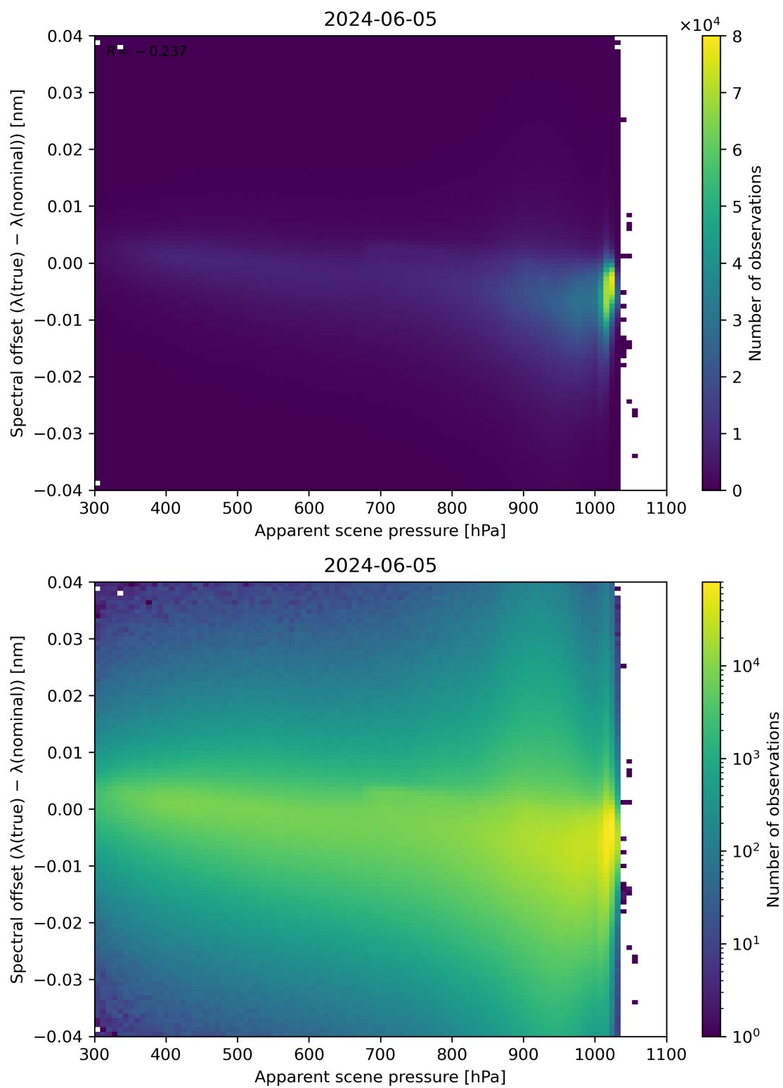
Figure 67: Scatter density plot of “Apparent scene pressure” against “Spectral offset ( \lambda(\text{true}) - \lambda(\text{nominal}) )” for 2024-06-04 to 2024-06-06.
