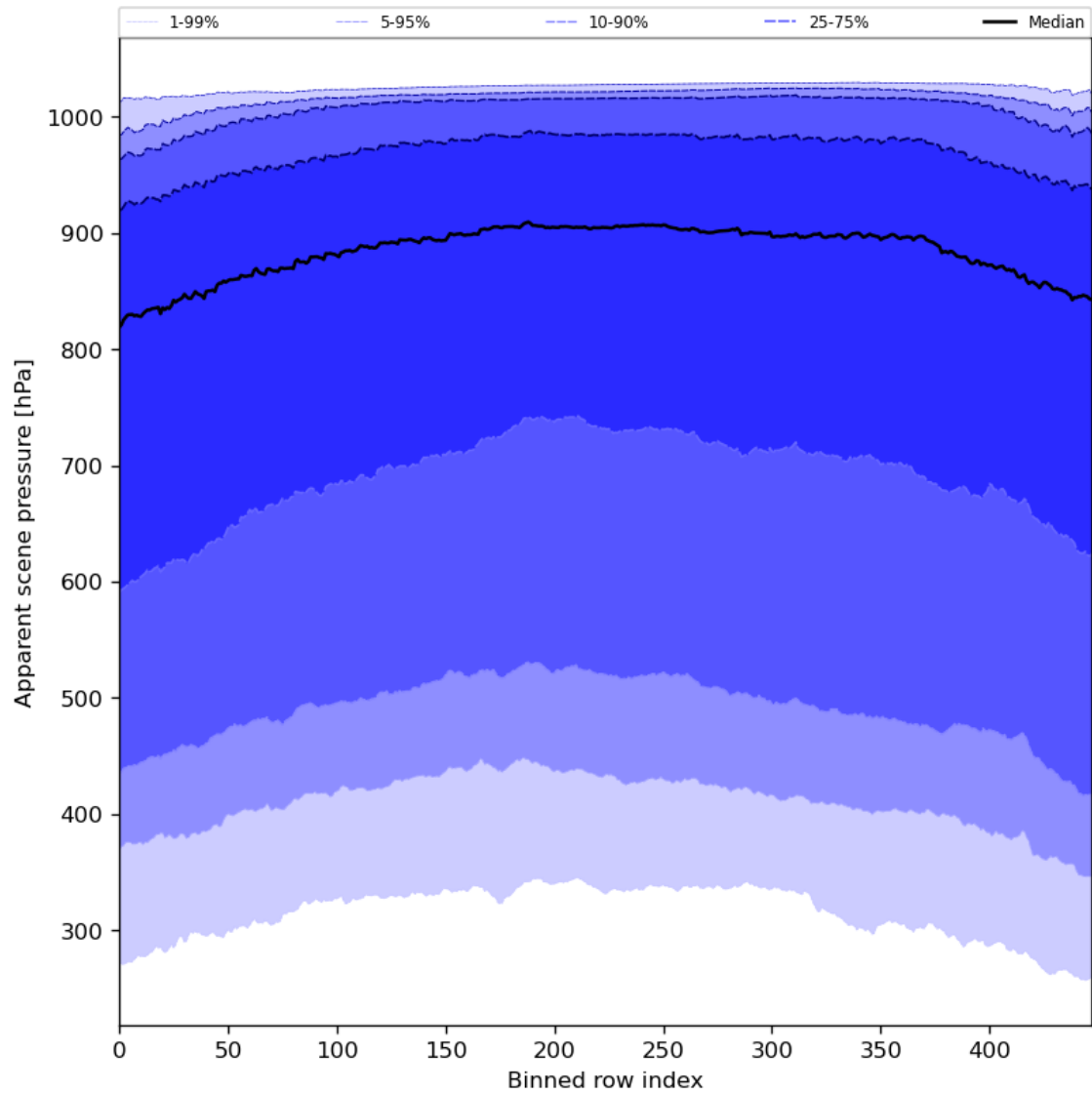
Figure 53: Along track statistics of “Apparent scene pressure” for 2024-06-04 to 2024-06-06
