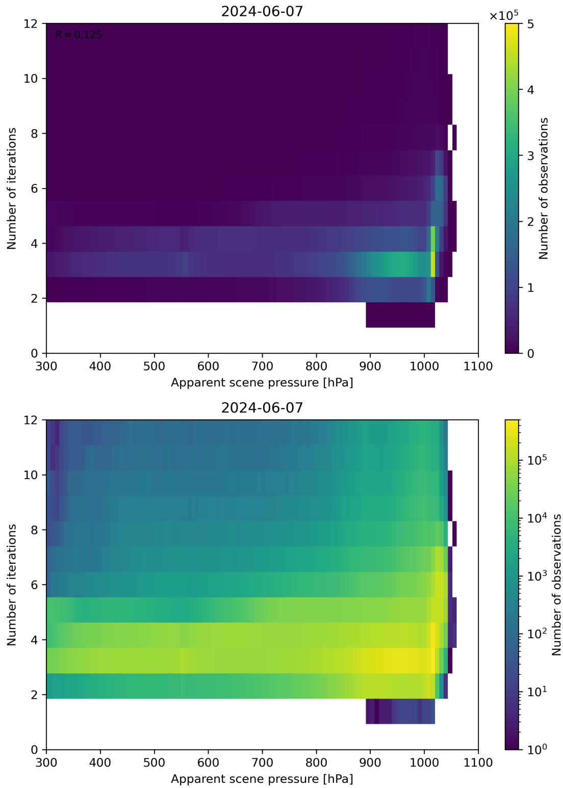
Figure 65: Scatter density plot of “Apparent scene pressure” against “Number of iterations” for 2024-06-06 to 2024-06-08.
