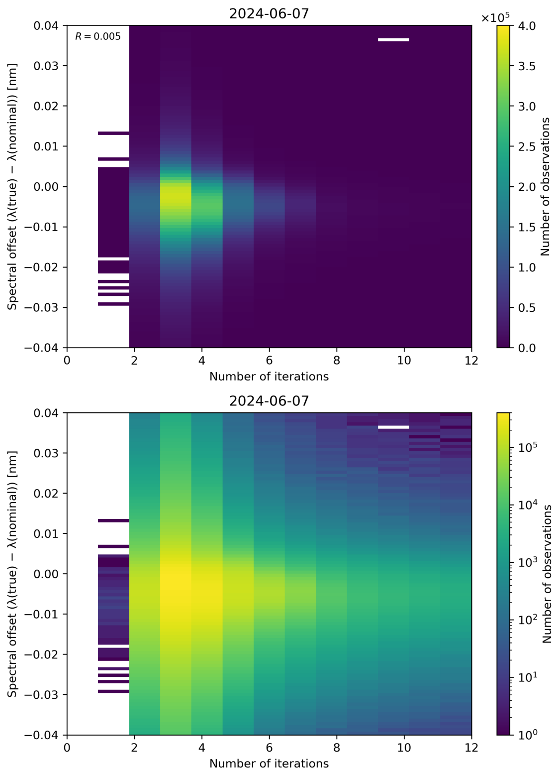
Figure 100: Scatter density plot of “Number of iterations” against “Spectral offset ( \lambda(\text{true}) - \lambda(\text{nominal}) )” for 2024-06-06 to 2024-06-08.
