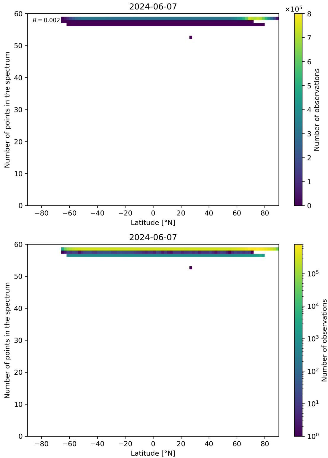
Figure 94: Scatter density plot of “Latitude” against “Number of points in the spectrum” for 2024-06-06 to 2024-06-08.
