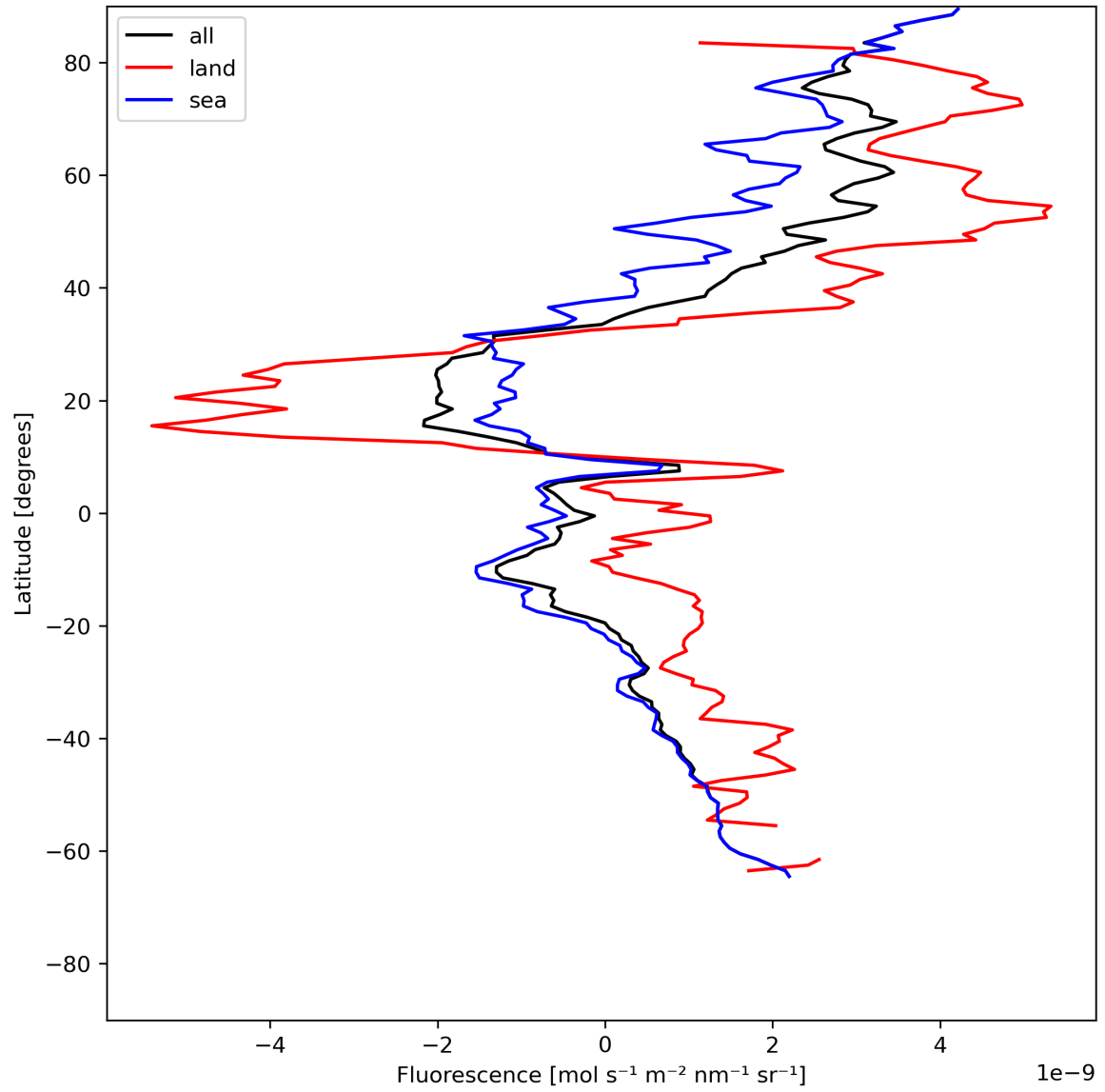
Figure 23: Zonal average of “Fluorescence” for 2024-06-06 to 2024-06-08.
