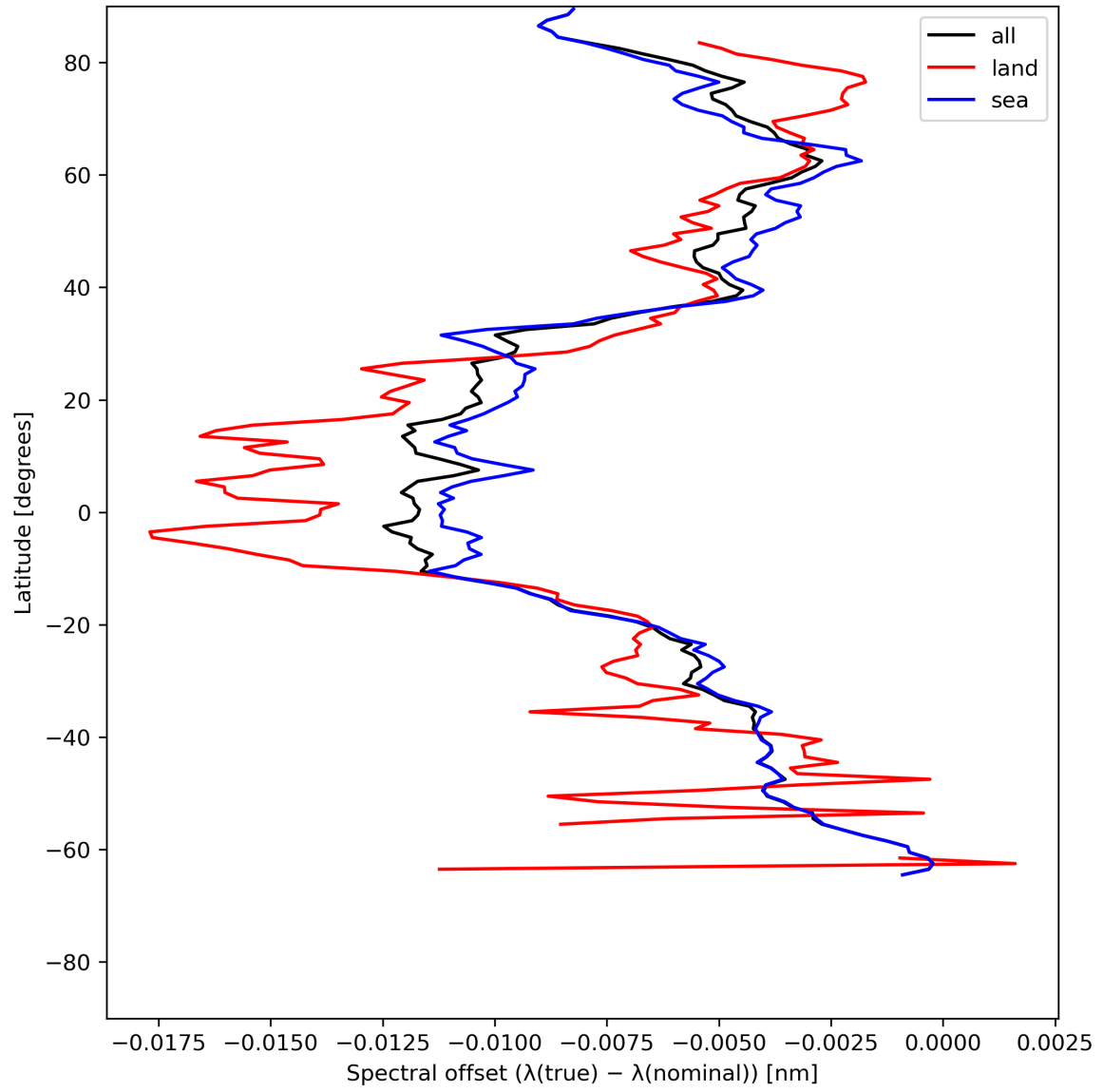
Figure 28: Zonal average of “Spectral offset ( \lambda(\text{true}) - \lambda(\text{nominal}) )” for 2024-06-06 to 2024-06-08.
