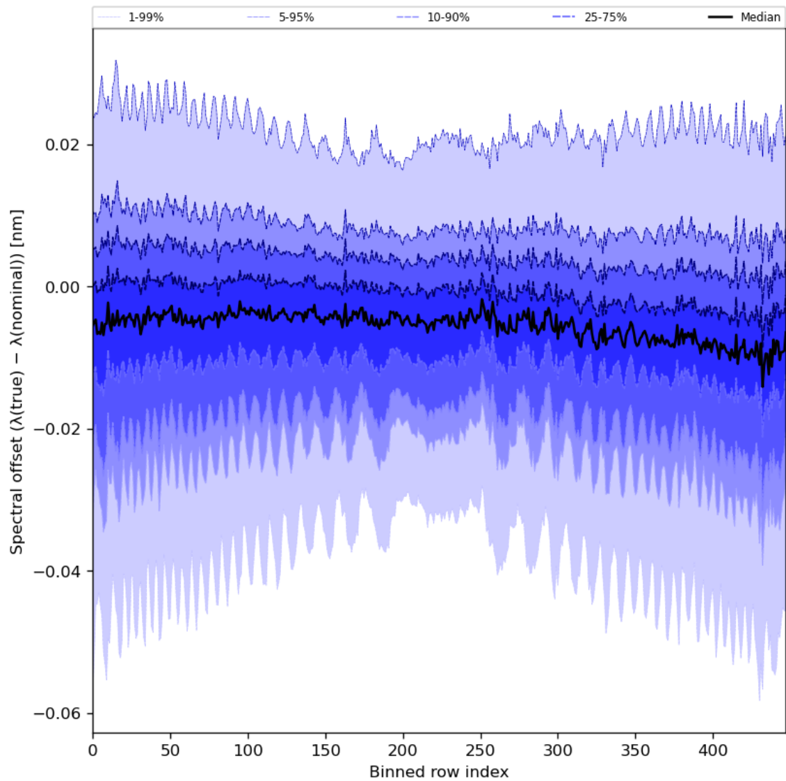
Figure 62: Along track statistics of “Spectral offset ( \lambda(\text{true}) - \lambda(\text{nominal}) )” for 2024-06-06 to 2024-06-08
