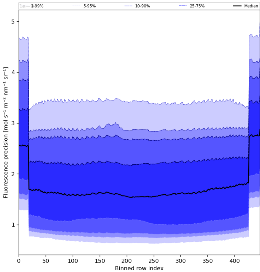
Figure 58: Along track statistics of “Fluorescence precision” for 2024-06-06 to 2024-06-08
