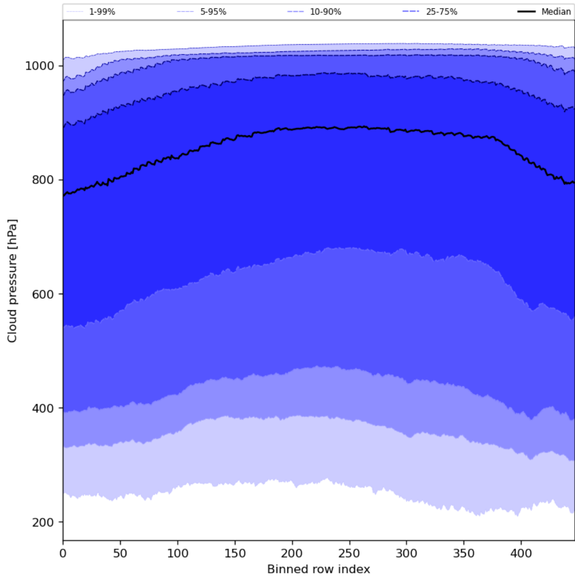
Figure 47: Along track statistics of “Cloud pressure” for 2024-06-06 to 2024-06-08
