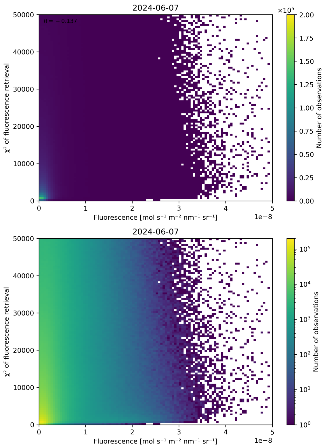
Figure 85: Scatter density plot of “Fluorescence” against “ \chi^2 of fluorescence retrieval” for 2024-06-06 to 2024-06-08.
