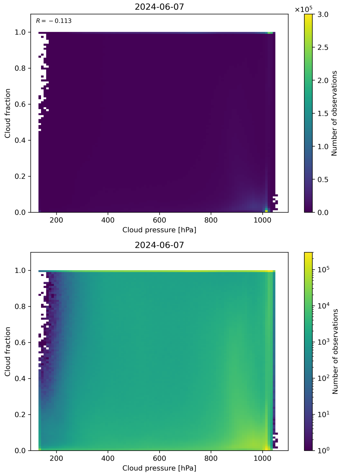
Figure 79: Scatter density plot of “Cloud pressure” against “Cloud fraction” for 2024-06-06 to 2024-06-08.
