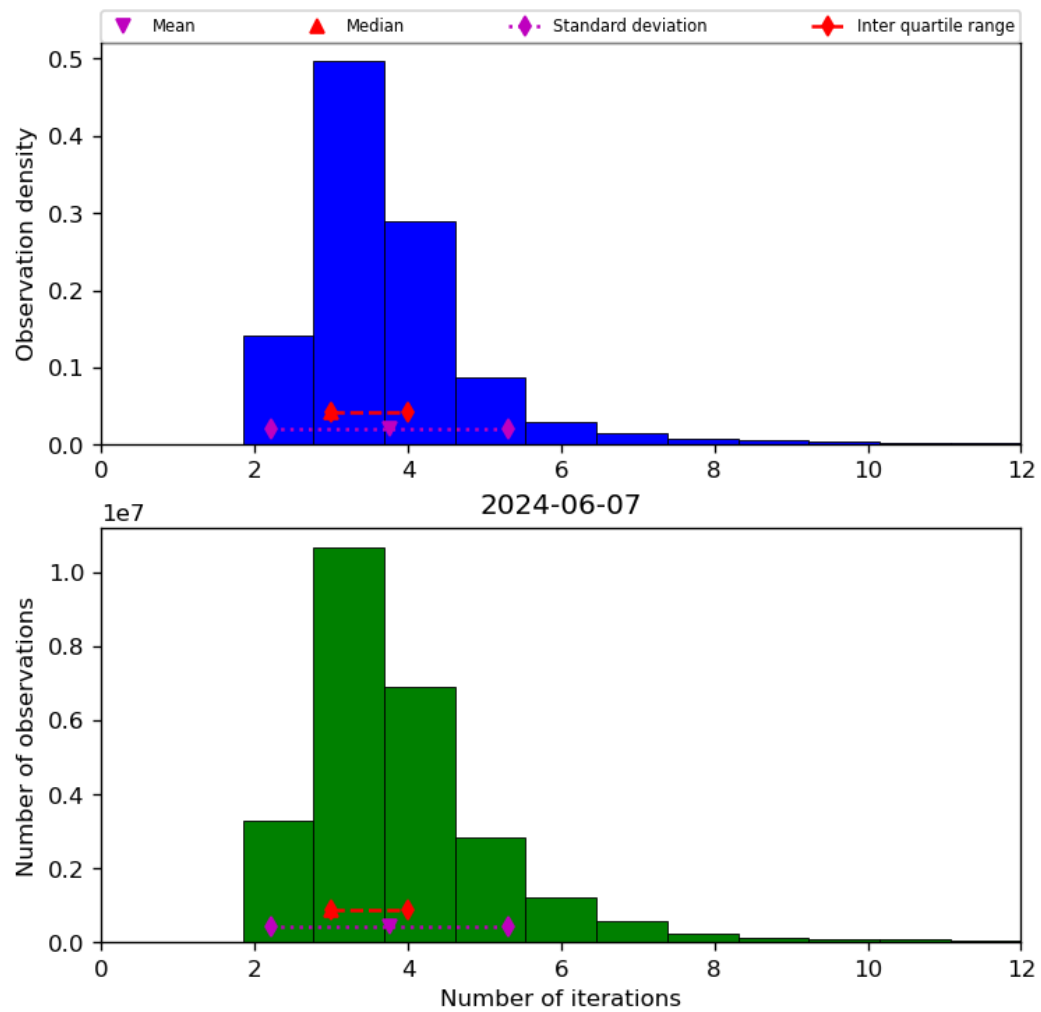
Figure 39: Histogram of “Number of iterations” for 2024-06-06 to 2024-06-08
