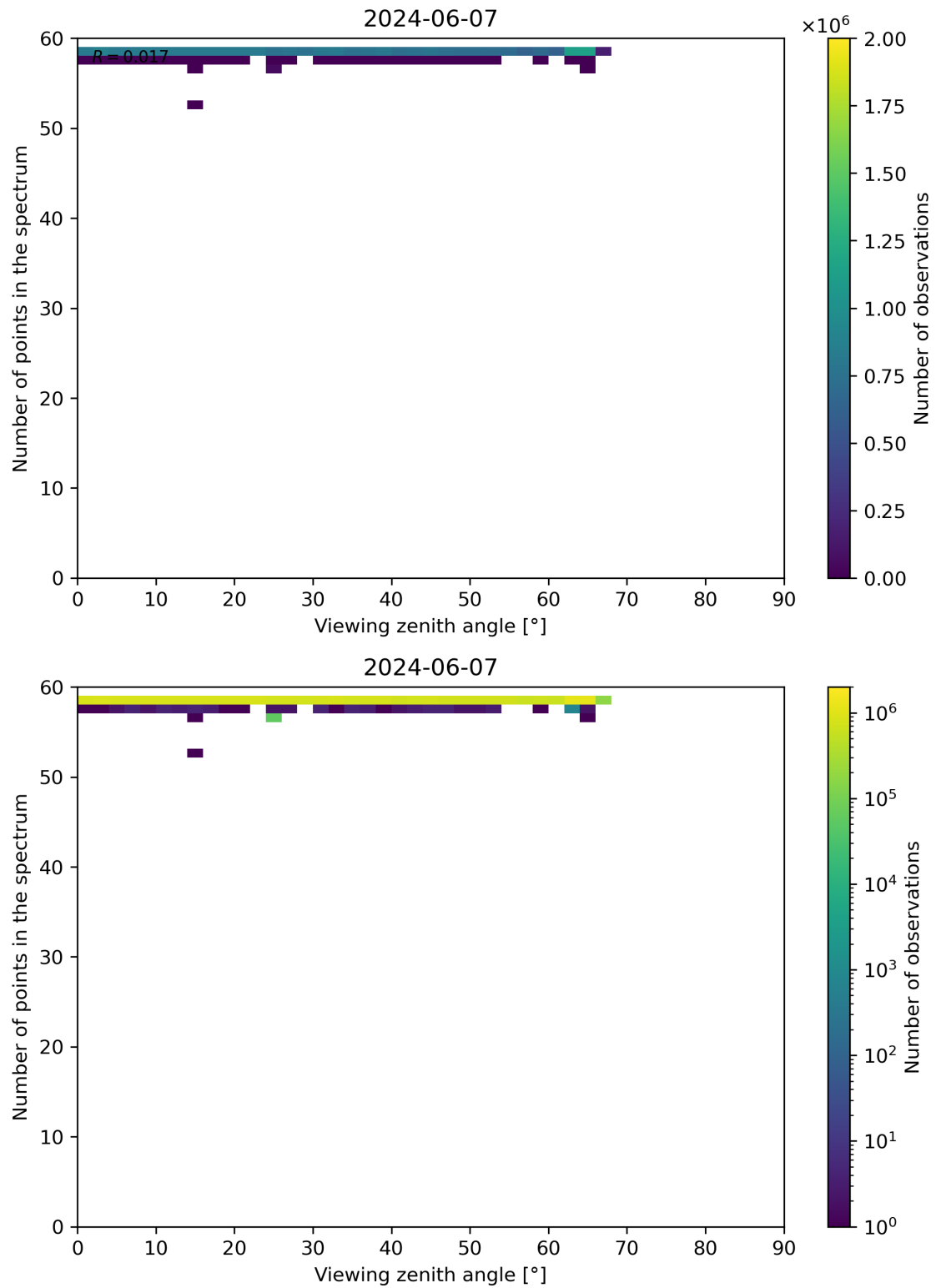
Figure 125: Scatter density plot of “Viewing zenith angle” against “Number of points in the spectrum” for 2024-06-06 to 2024-06-08.
