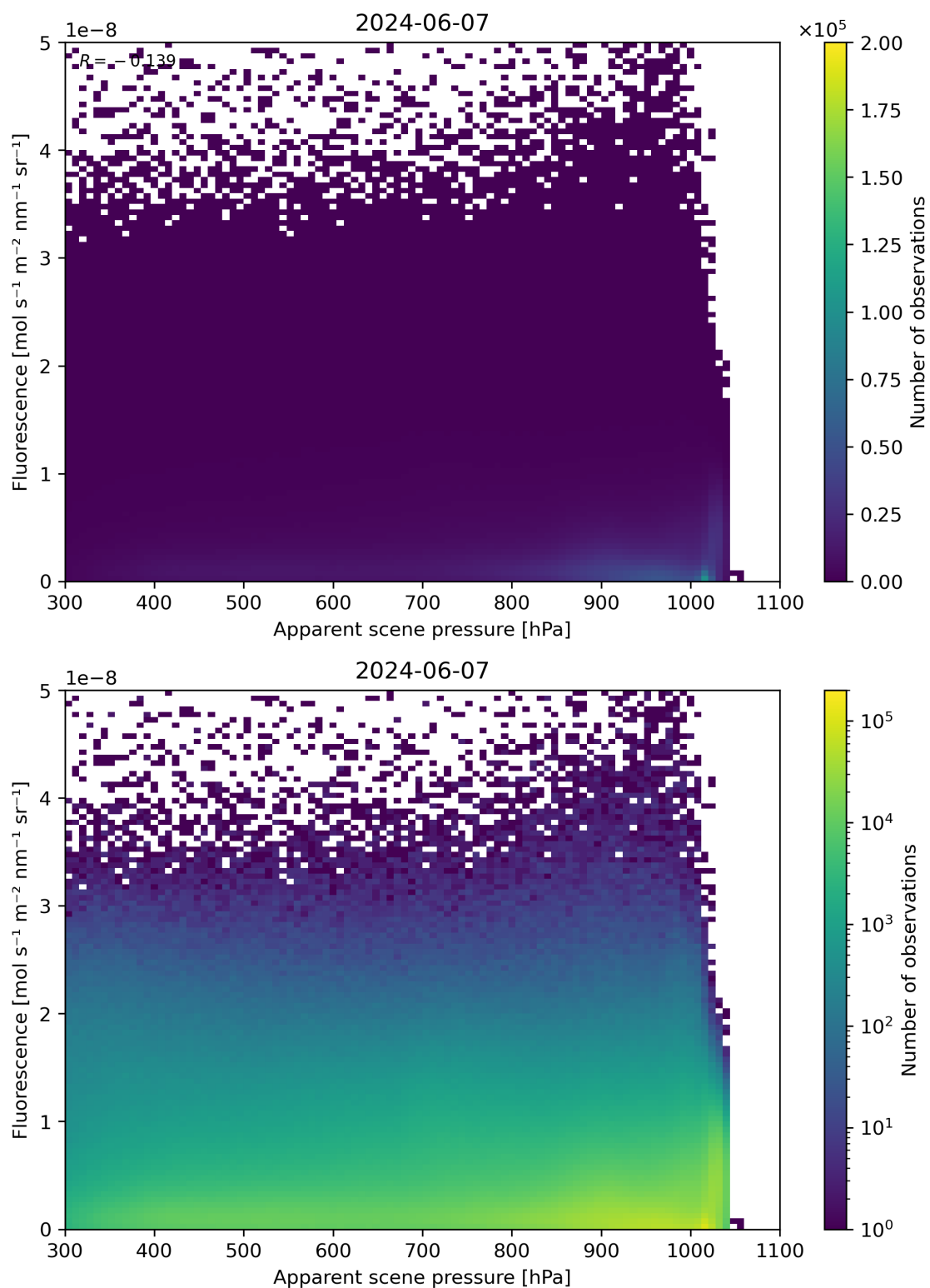
Figure 64: Scatter density plot of “Apparent scene pressure” against “Fluorescence” for 2024-06-06 to 2024-06-08.
