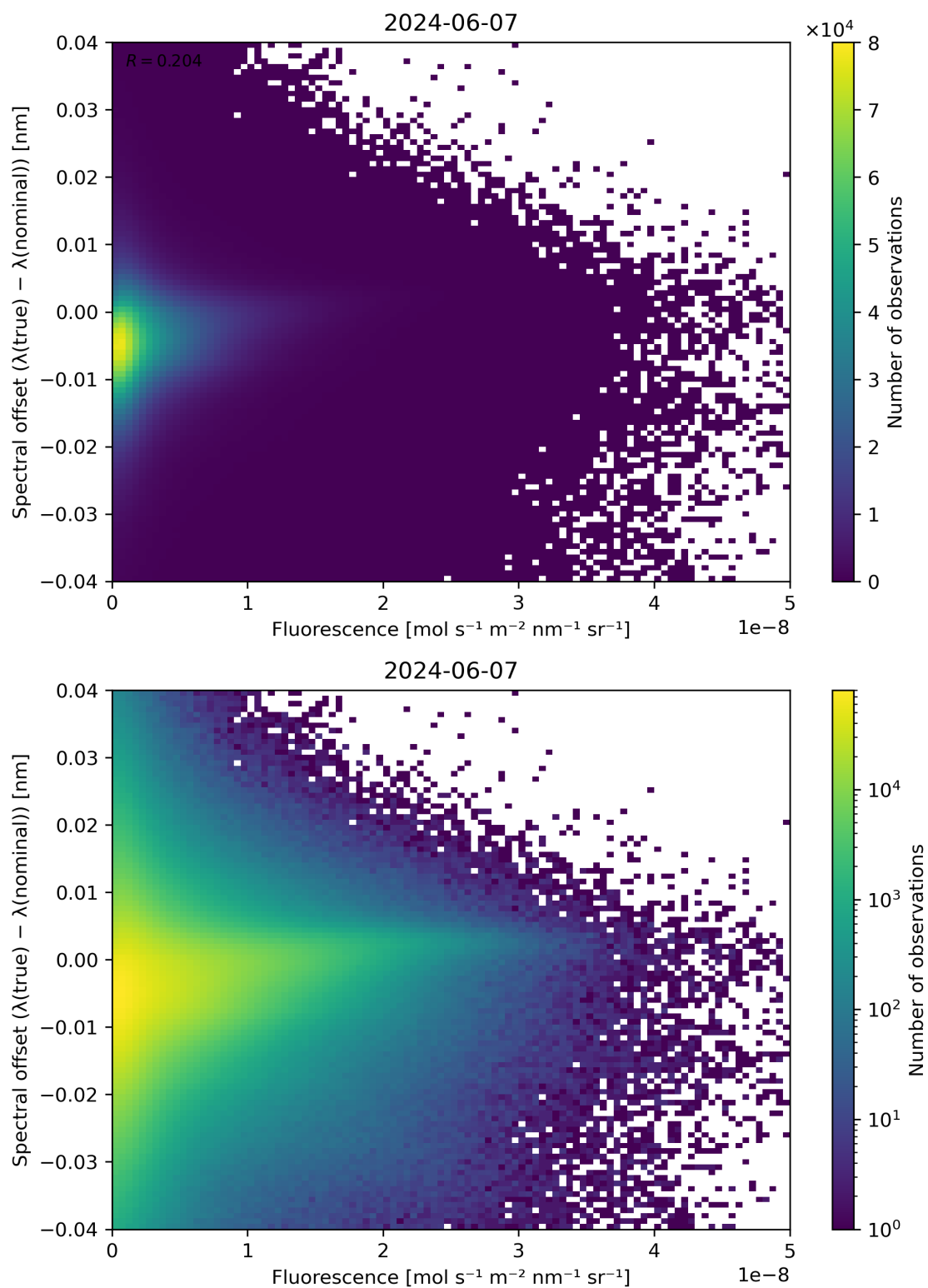
Figure 87: Scatter density plot of “Fluorescence” against “Spectral offset ( \lambda(\text{true}) - \lambda(\text{nominal}) )” for 2024-06-06 to 2024-06-08.
