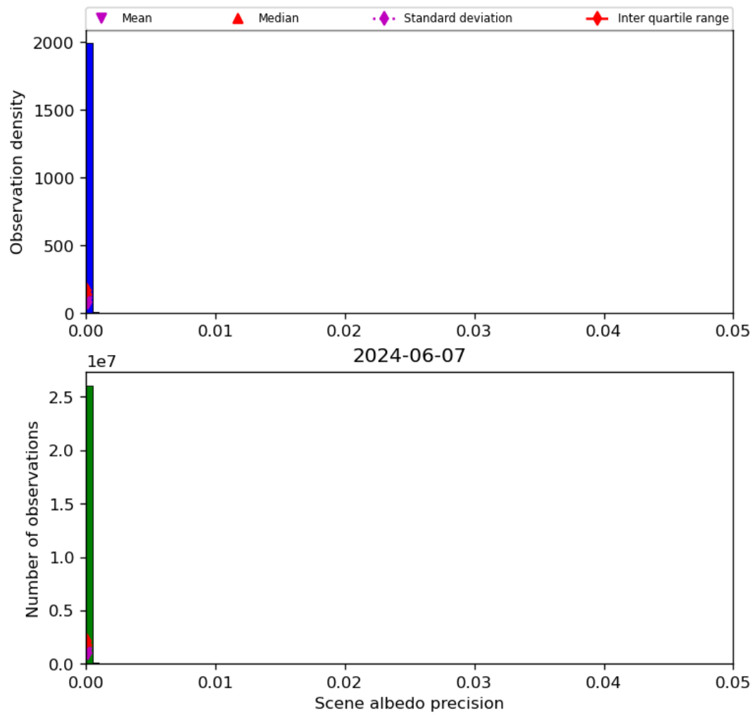
Figure 35: Histogram of “Scene albedo precision” for 2024-06-06 to 2024-06-08
