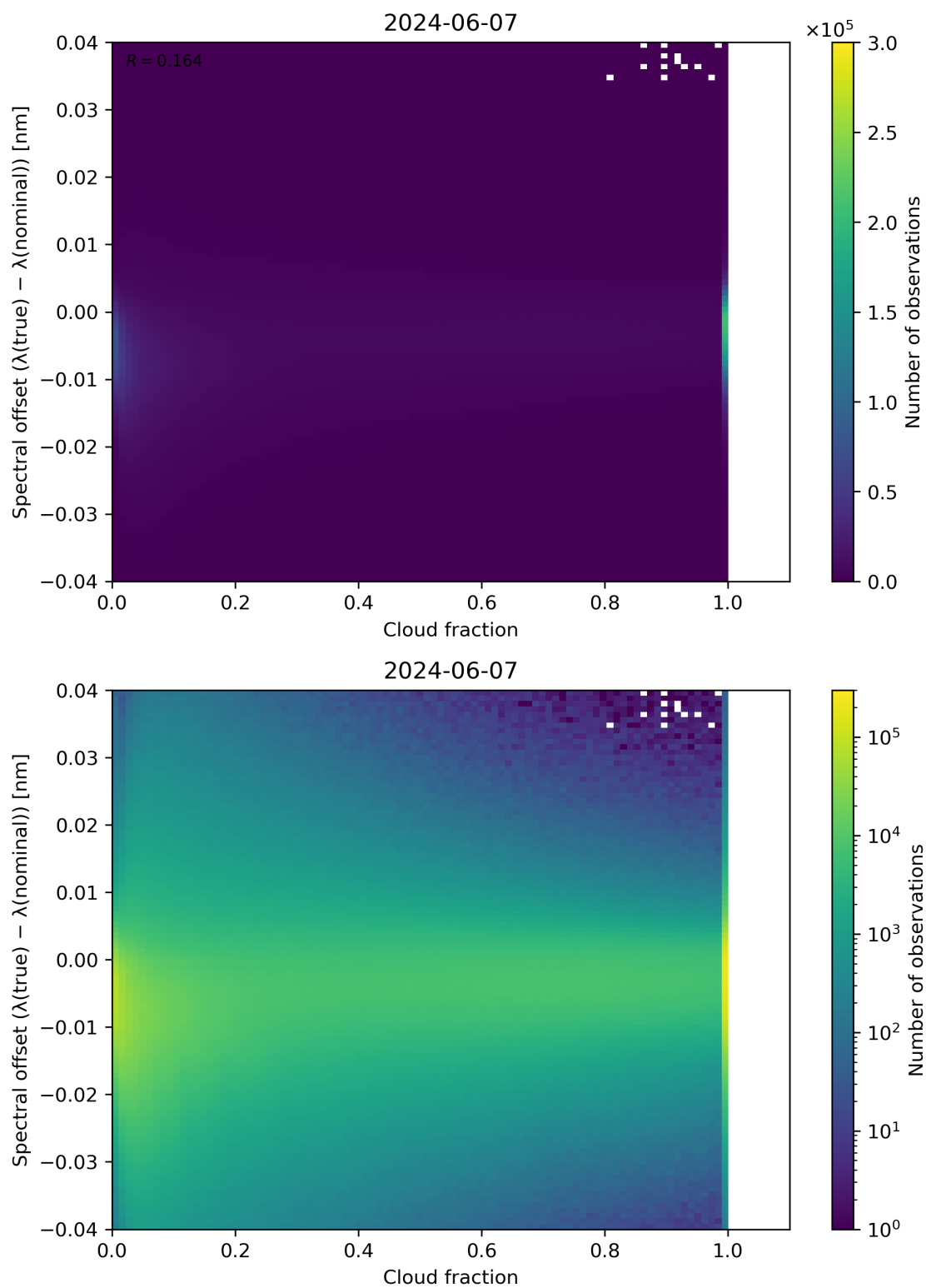
Figure 76: Scatter density plot of “Cloud fraction” against “Spectral offset ( \lambda(\text{true}) - \lambda(\text{nominal}) )” for 2024-06-06 to 2024-06-08.
