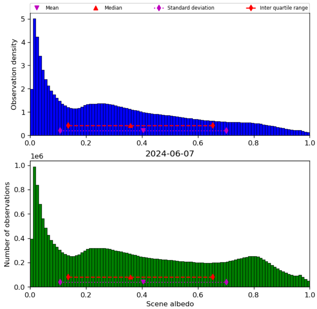
Figure 34: Histogram of “Scene albedo” for 2024-06-06 to 2024-06-08
