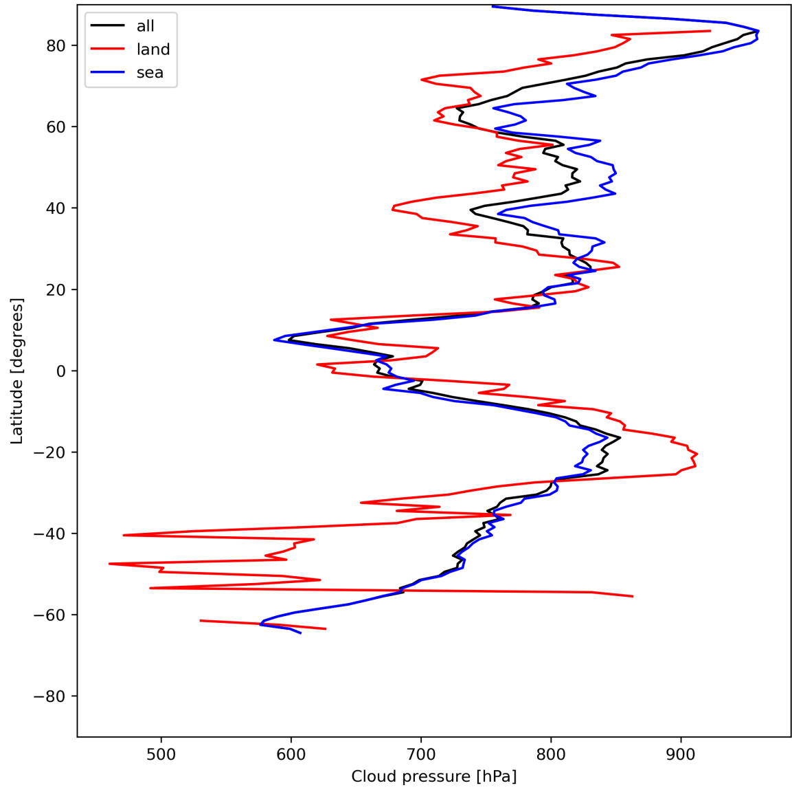
Figure 13: Zonal average of “Cloud pressure” for 2024-06-06 to 2024-06-08.
