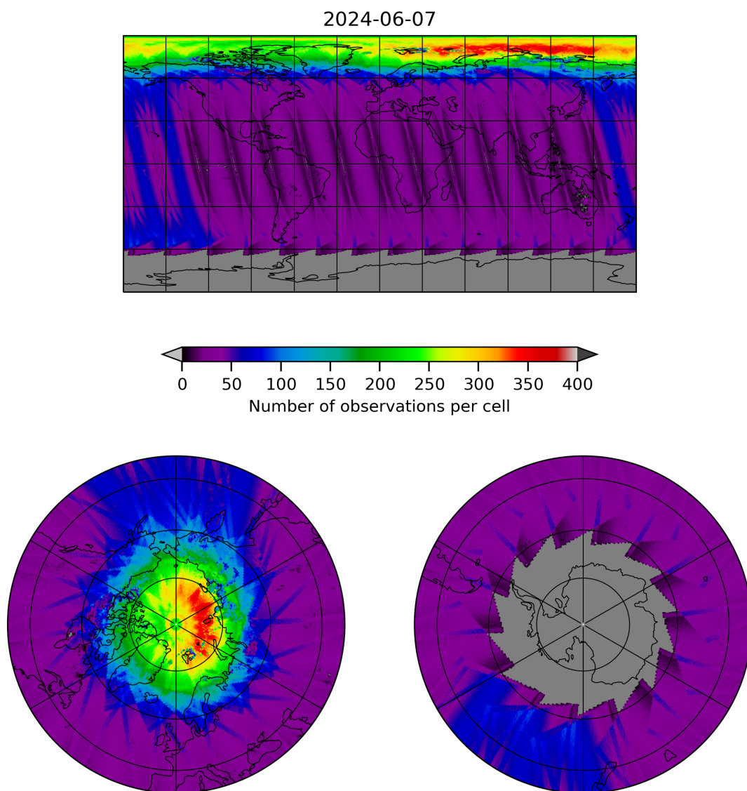
Figure 11: Map of the number of observations for 2024-06-06 to 2024-06-08
