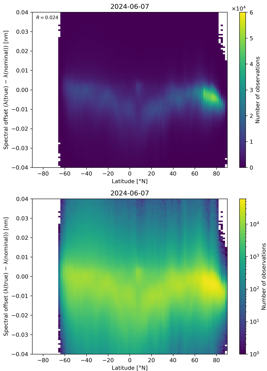
Figure 96: Scatter density plot of “Latitude” against “Spectral offset ( \lambda(\text{true}) - \lambda(\text{nominal}) )” for 2024-06-06 to 2024-06-08.
