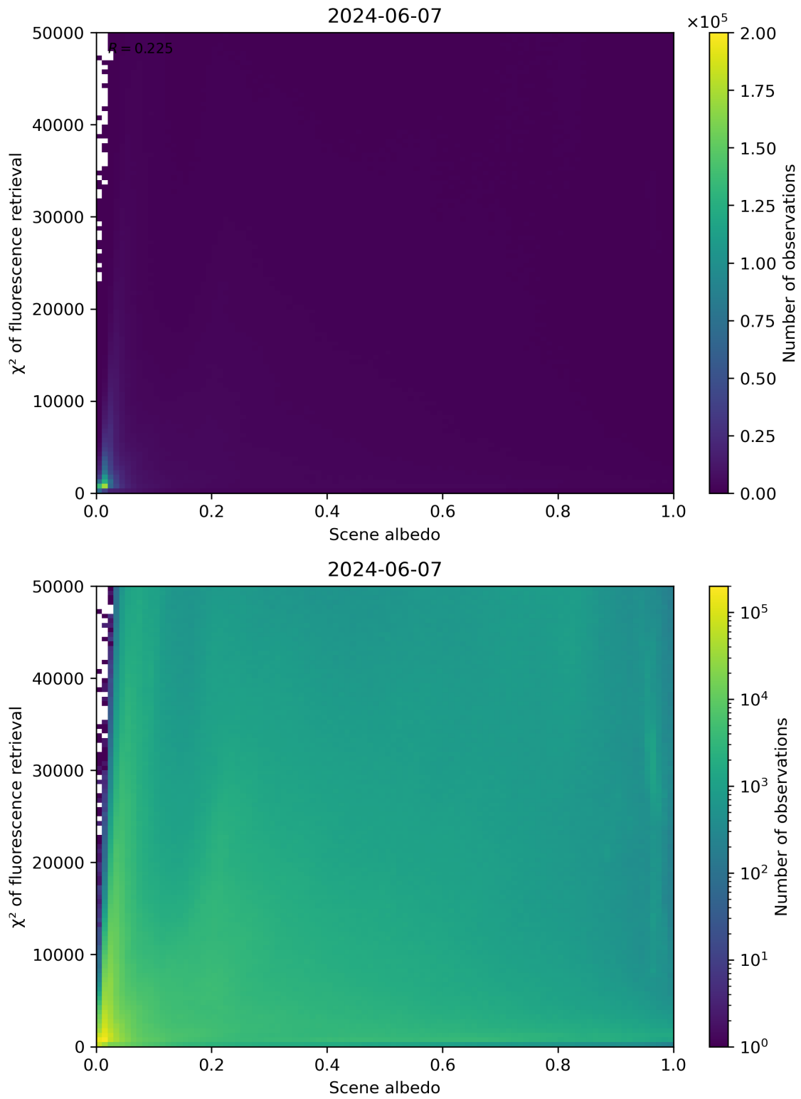
Figure 103: Scatter density plot of “Scene albedo” against “ \chi^2 of fluorescence retrieval” for 2024-06-06 to 2024-06-08.
