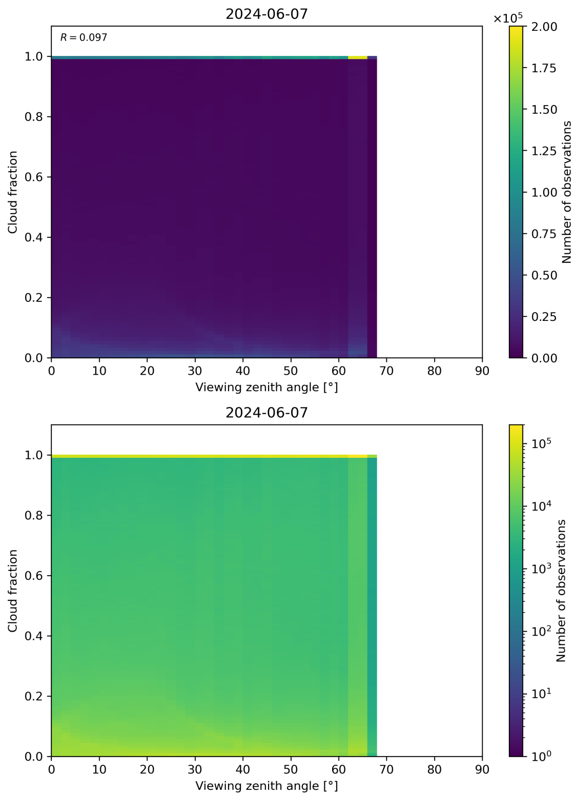
Figure 120: Scatter density plot of “Viewing zenith angle” against “Cloud fraction” for 2024-06-06 to 2024-06-08.
