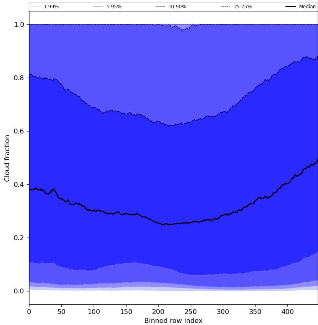
Figure 49: Along track statistics of “Cloud fraction” for 2024-06-06 to 2024-06-08
