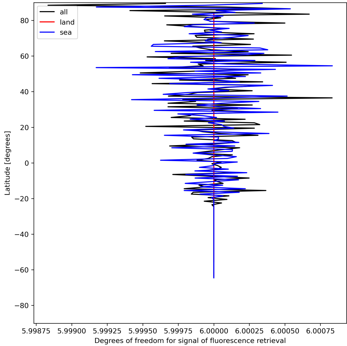
Figure 26: Zonal average of “Degrees of freedom for signal of fluorescence retrieval” for 2024-06-06 to 2024-06-08.
