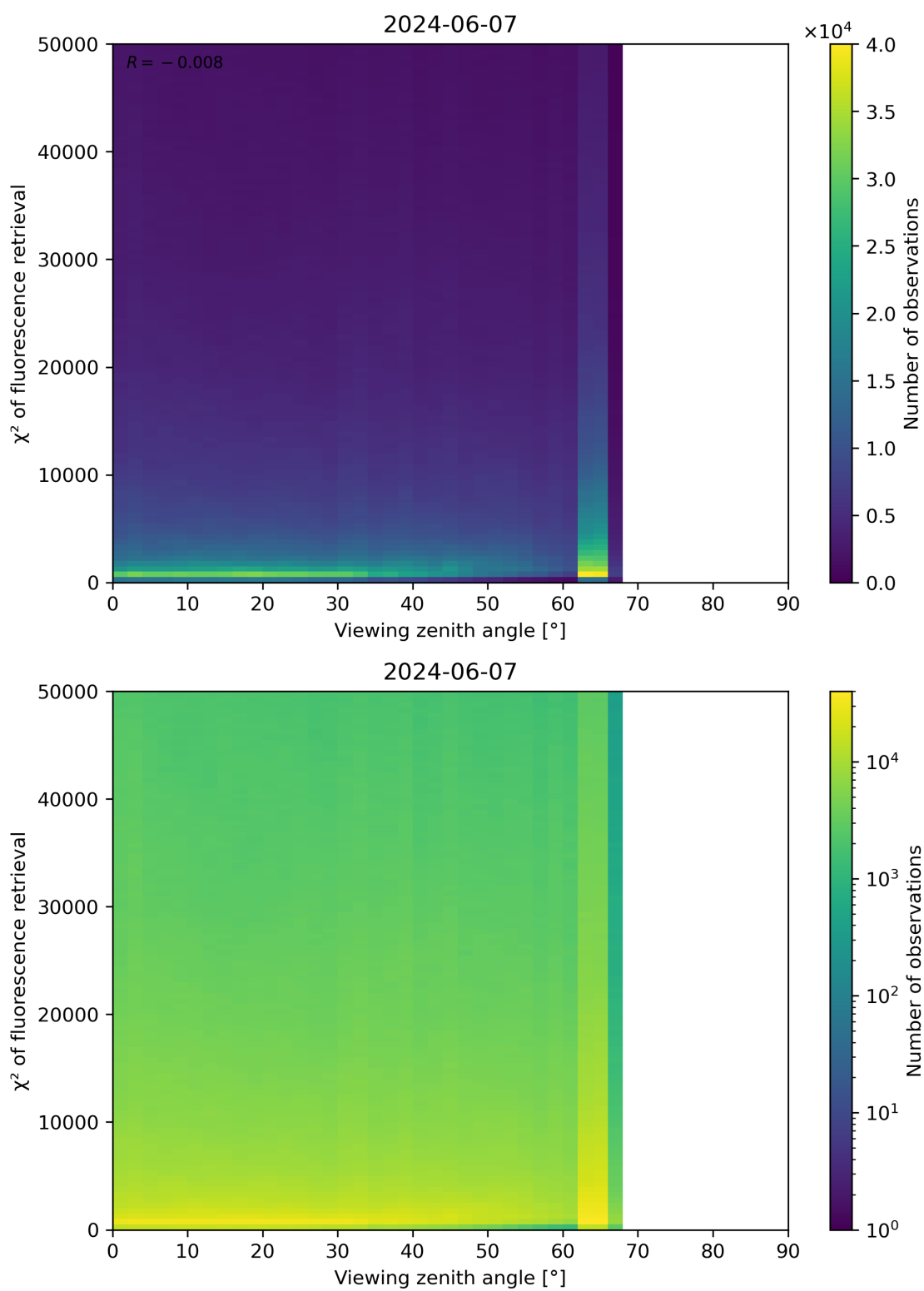
Figure 119: Scatter density plot of “Viewing zenith angle” against “ \chi^2 of fluorescence retrieval” for 2024-06-06 to 2024-06-08.
