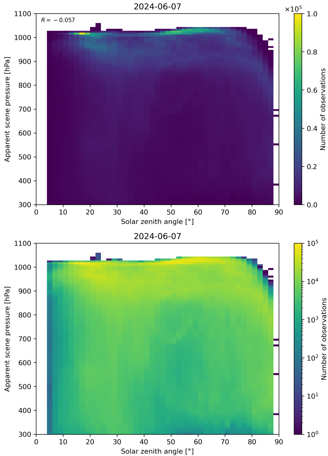
Figure 108: Scatter density plot of “Solar zenith angle” against “Apparent scene pressure” for 2024-06-06 to 2024-06-08.
