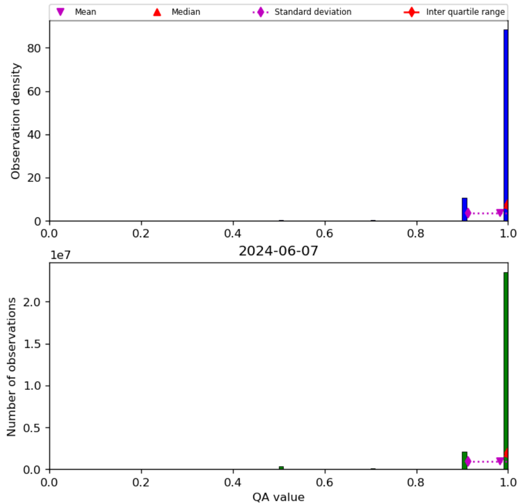
Figure 29: Histogram of “QA value” for 2024-06-06 to 2024-06-08
