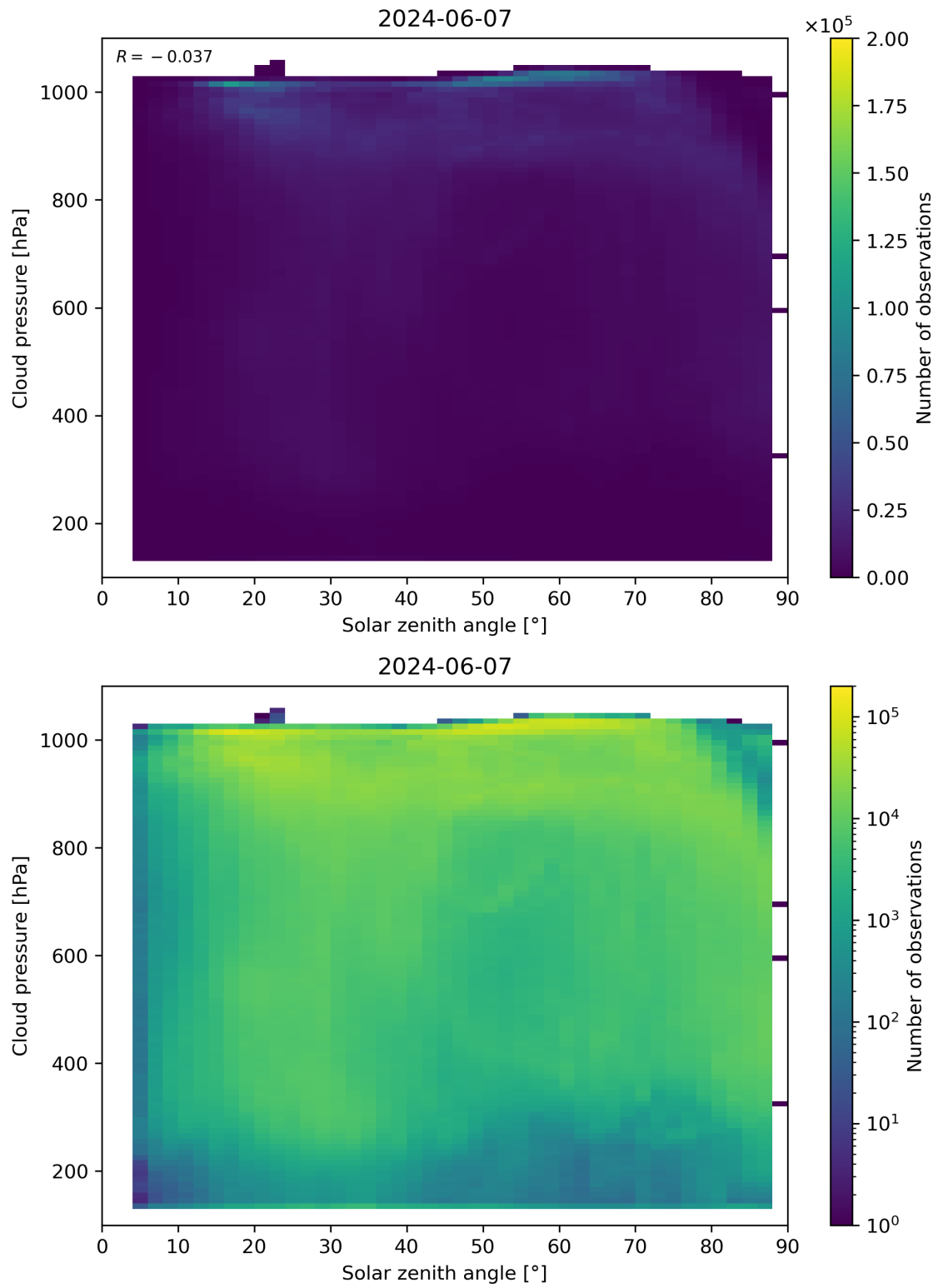
Figure 111: Scatter density plot of “Solar zenith angle” against “Cloud pressure” for 2024-06-06 to 2024-06-08.
