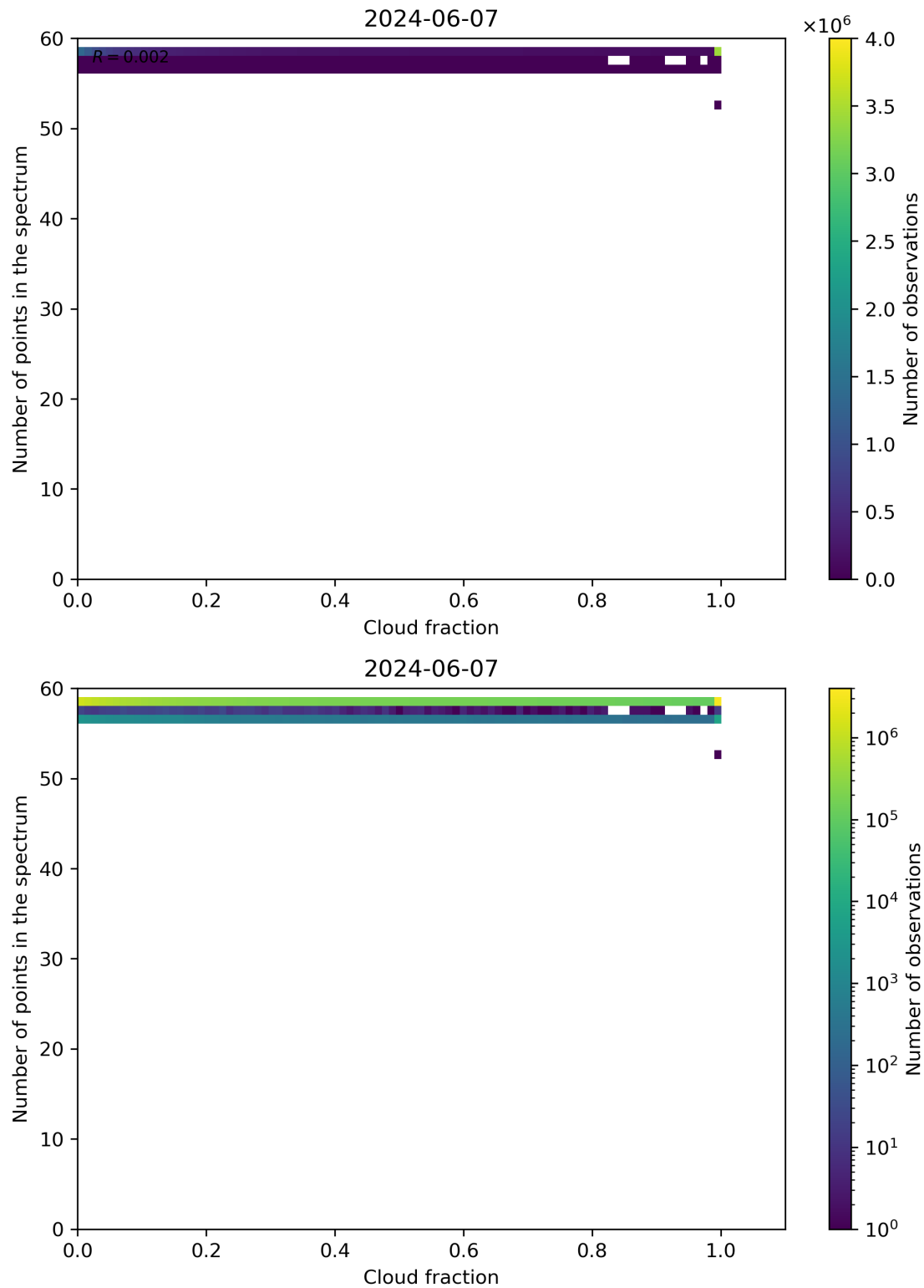
Figure 74: Scatter density plot of “Cloud fraction” against “Number of points in the spectrum” for 2024-06-06 to 2024-06-08.
