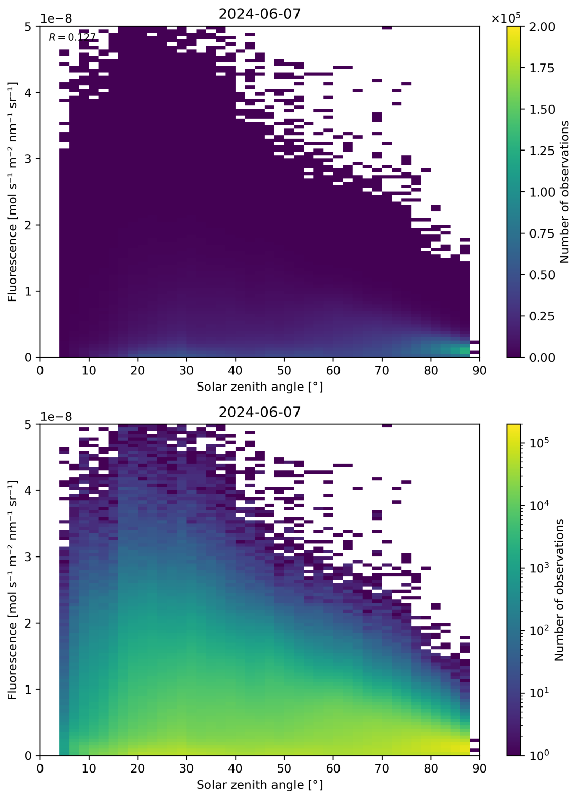
Figure 112: Scatter density plot of “Solar zenith angle” against “Fluorescence” for 2024-06-06 to 2024-06-08.
