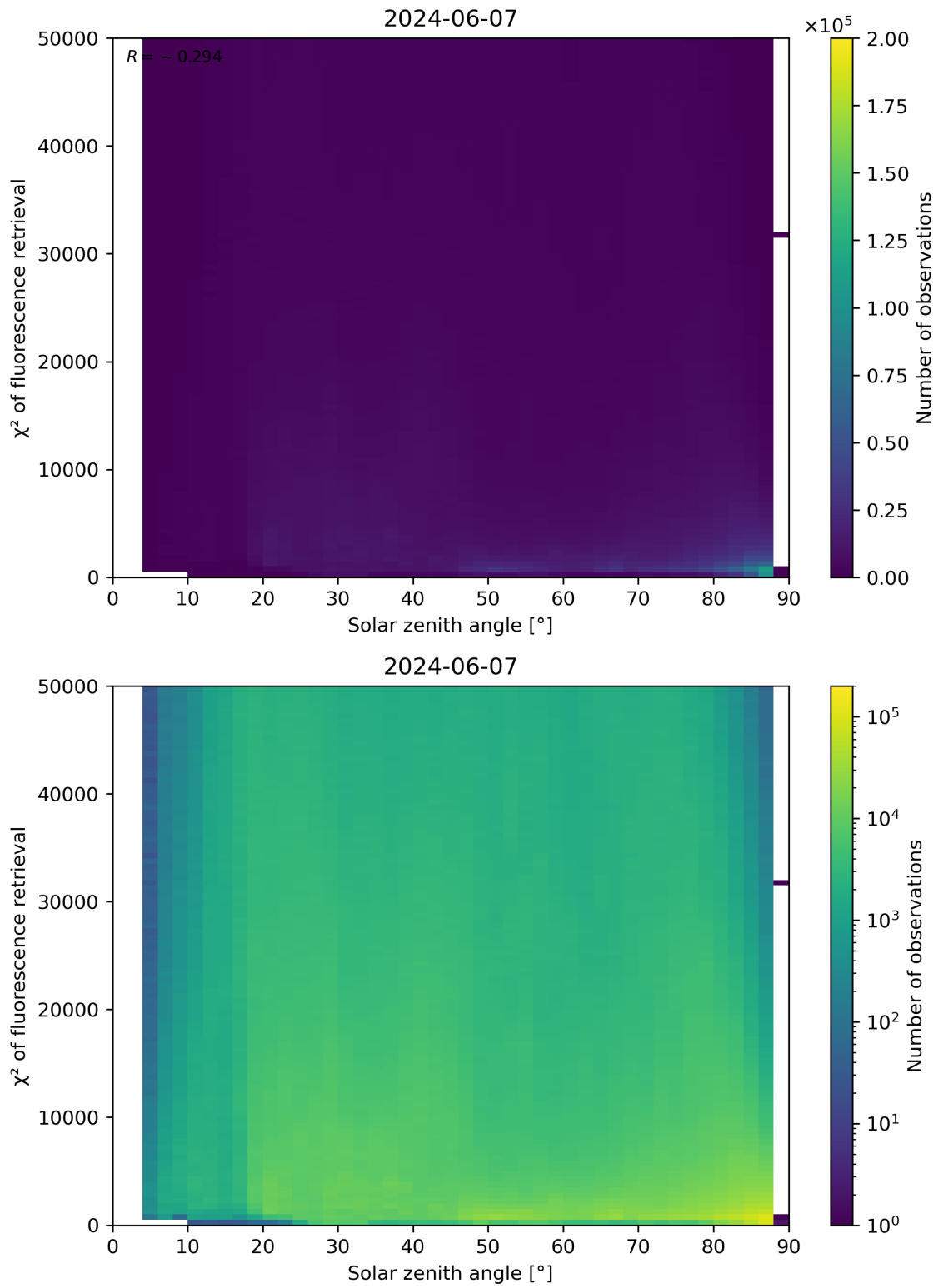
Figure 109: Scatter density plot of “Solar zenith angle” against “ \chi^2 of fluorescence retrieval” for 2024-06-06 to 2024-06-08.
