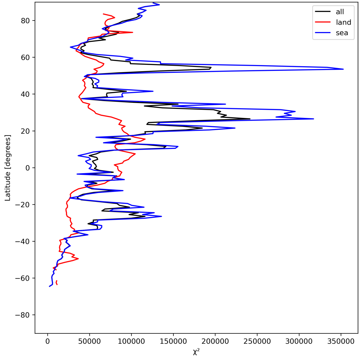
Figure 21: Zonal average of “ \chi^2 ” for 2024-06-06 to 2024-06-08.
