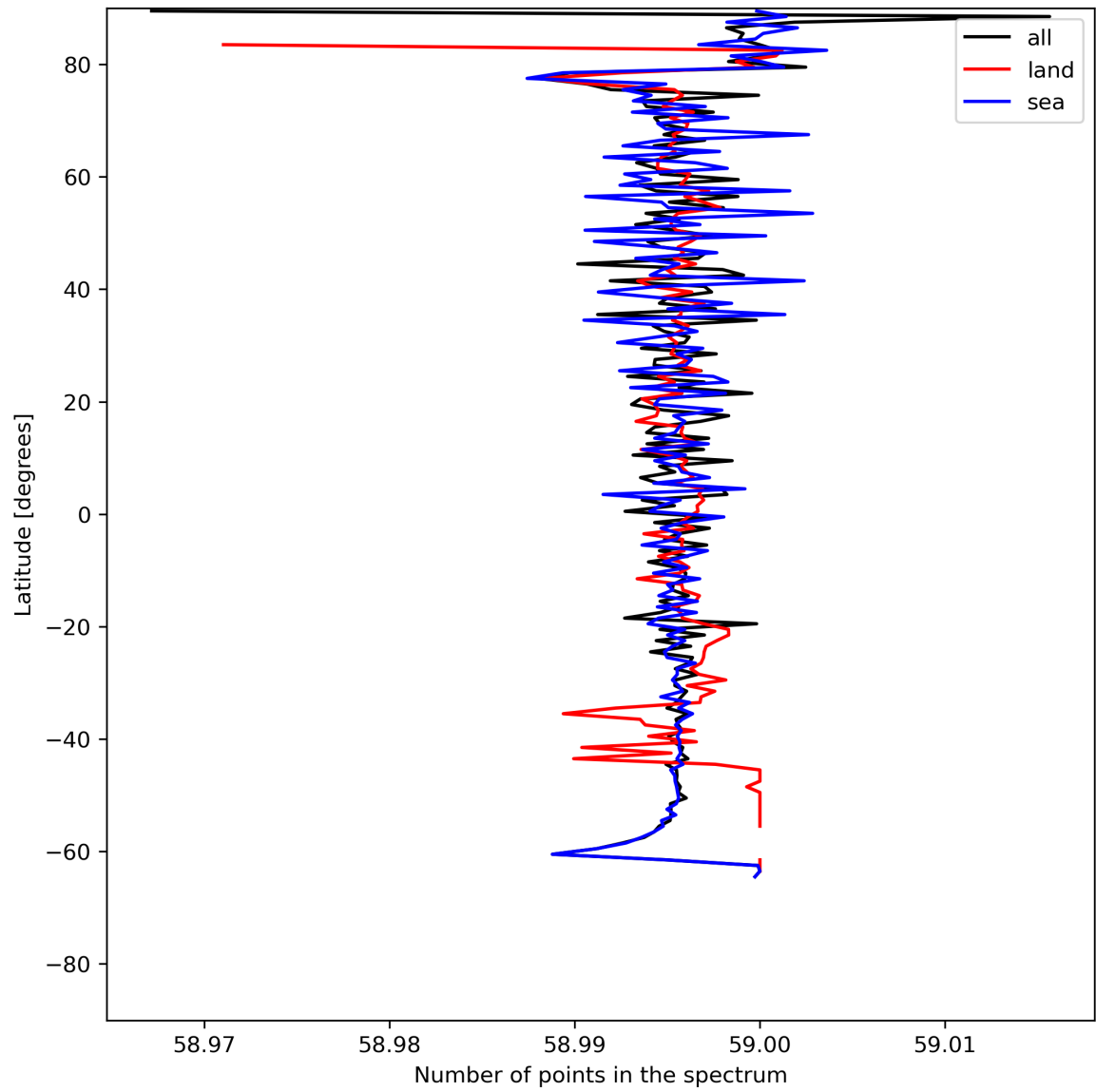
Figure 27: Zonal average of “Number of points in the spectrum” for 2024-06-06 to 2024-06-08.
