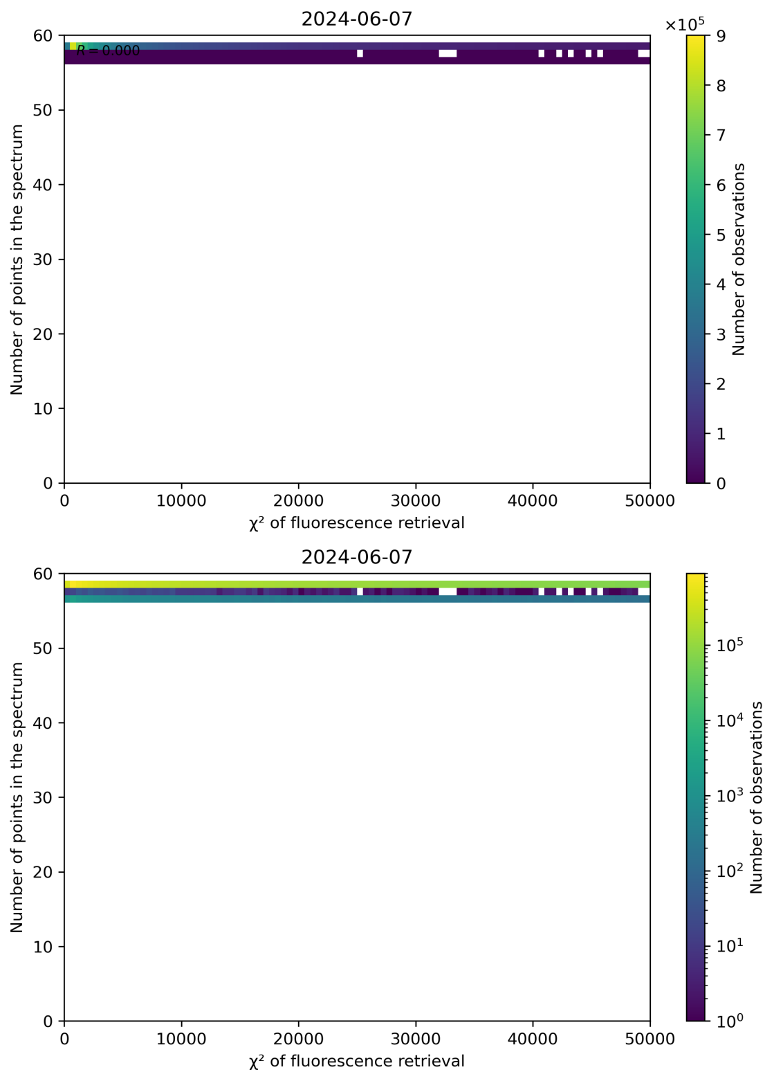
Figure 68: Scatter density plot of " \chi^2 of fluorescence retrieval" against "Number of points in the spectrum" for 2024-06-06 to 2024-06-08.
