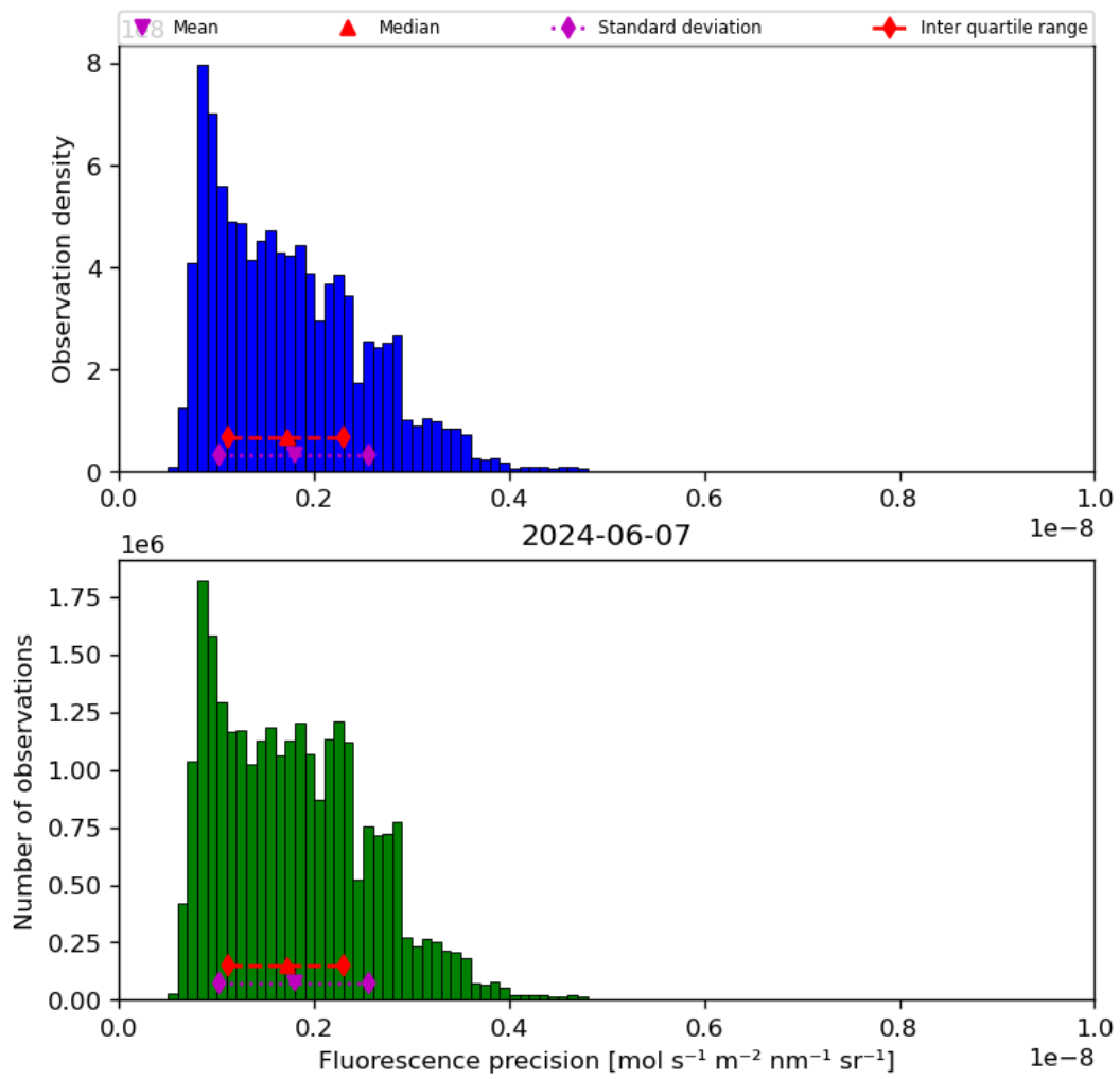
Figure 41: Histogram of “Fluorescence precision” for 2024-06-06 to 2024-06-08
