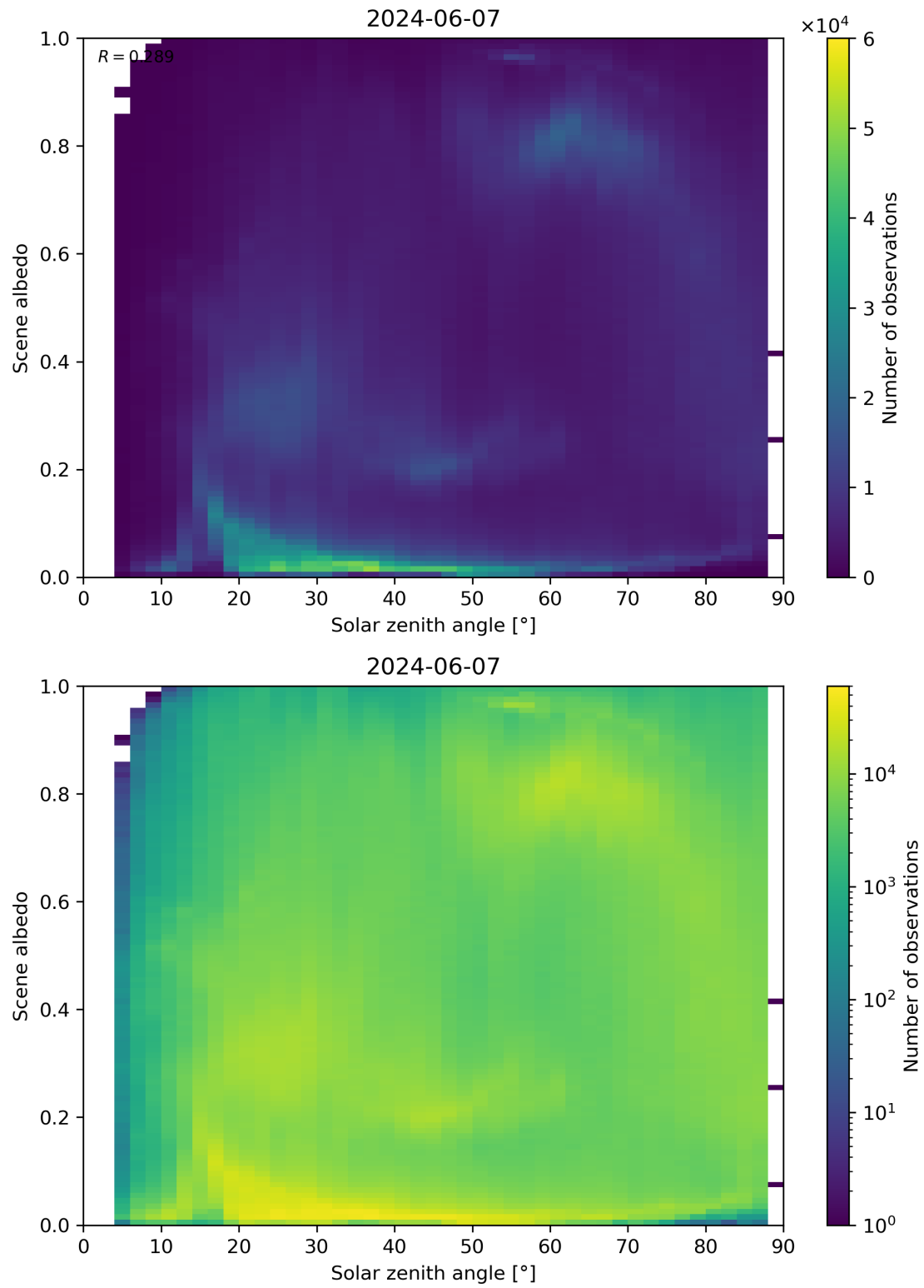
Figure 116: Scatter density plot of “Solar zenith angle” against “Scene albedo” for 2024-06-06 to 2024-06-08.
