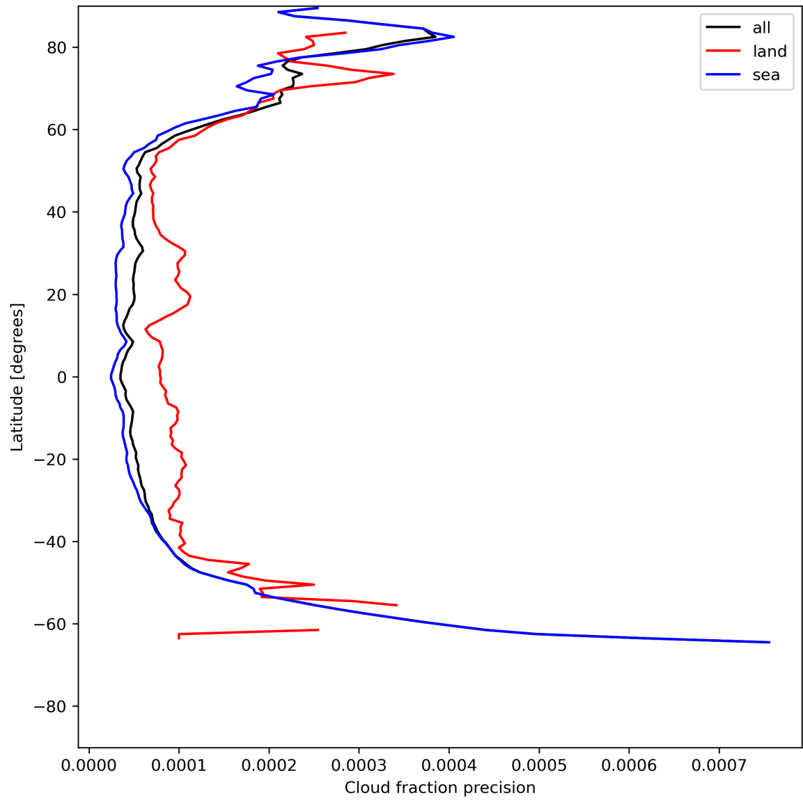
Figure 16: Zonal average of “Cloud fraction precision” for 2024-06-06 to 2024-06-08.
