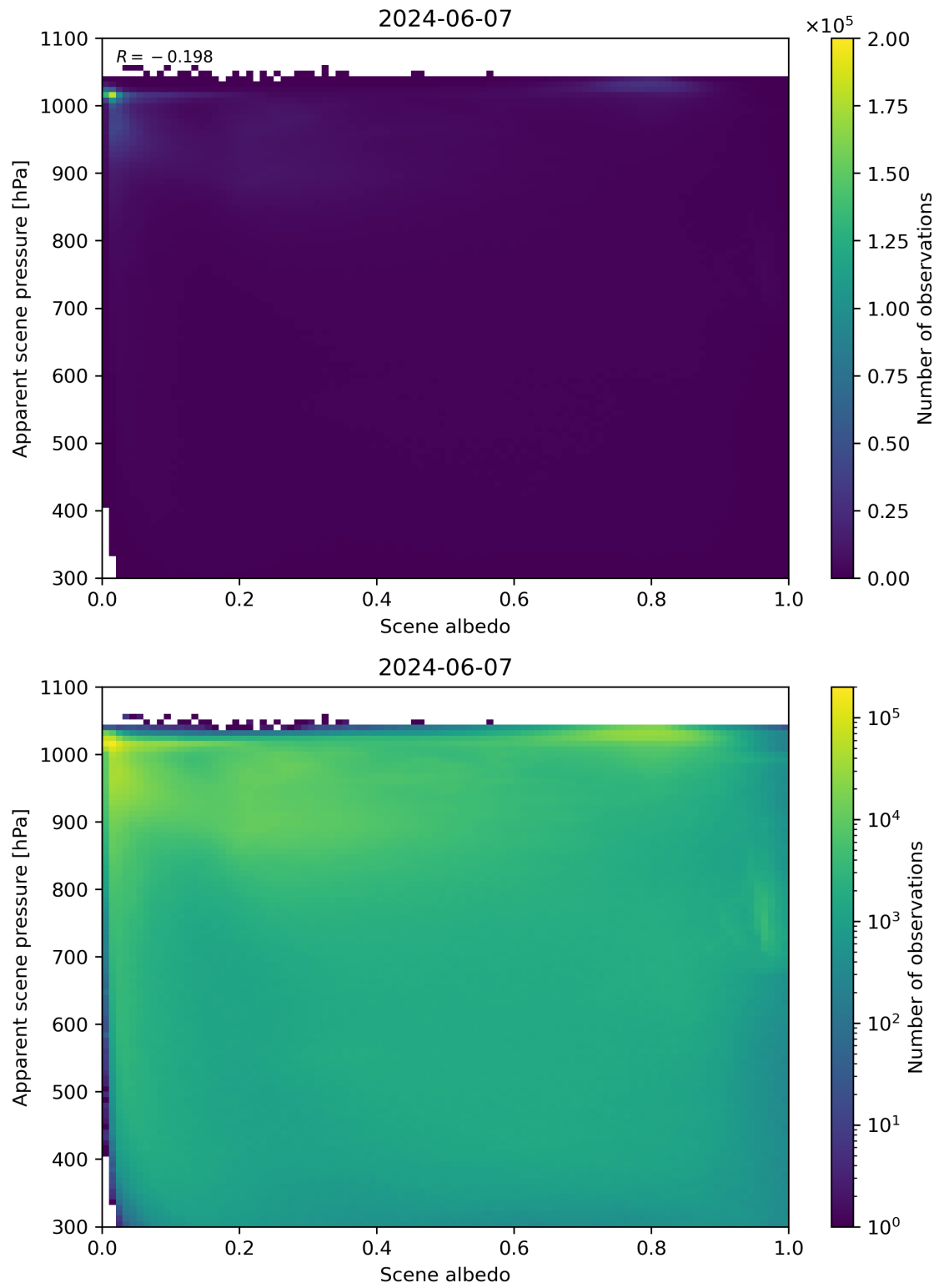
Figure 102: Scatter density plot of “Scene albedo” against “Apparent scene pressure” for 2024-06-06 to 2024-06-08.
