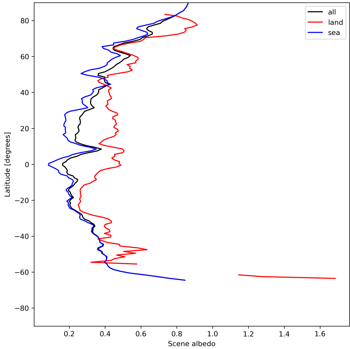
Figure 17: Zonal average of “Scene albedo” for 2024-06-06 to 2024-06-08.
