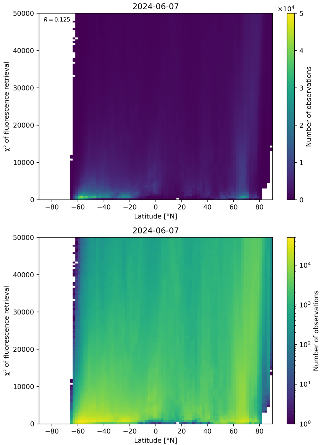
Figure 89: Scatter density plot of “Latitude” against “ \chi^2 of fluorescence retrieval” for 2024-06-06 to 2024-06-08.
