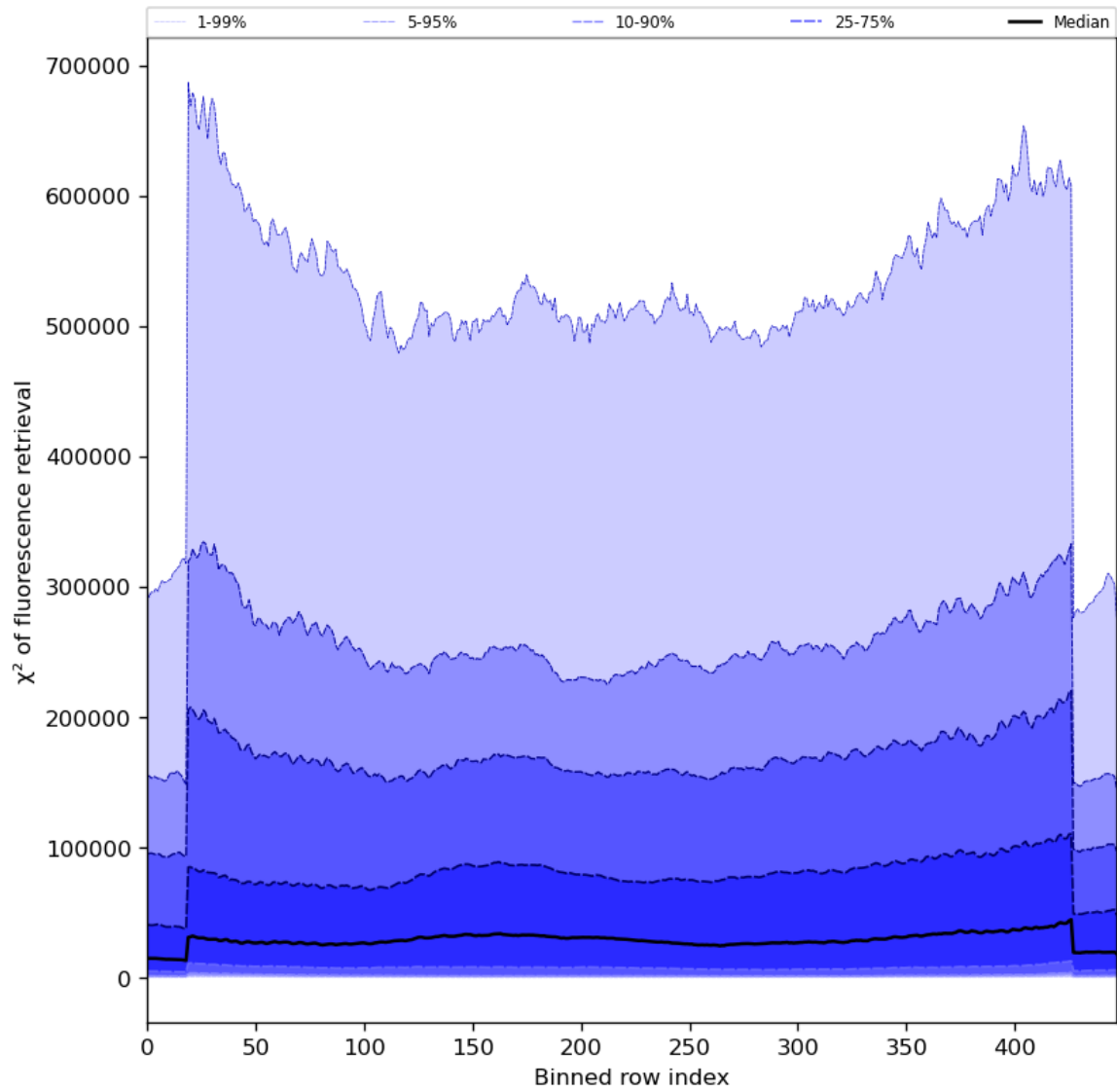
Figure 59: Along track statistics of “ \chi^2 of fluorescence retrieval” for 2024-06-06 to 2024-06-08
