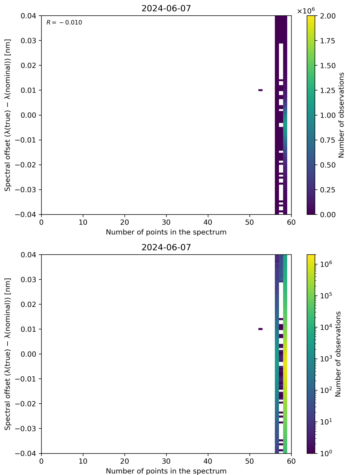
Figure 101: Scatter density plot of “Number of points in the spectrum” against “Spectral offset ( \lambda(\text{true}) - \lambda(\text{nominal}) )” for 2024-06-06 to 2024-06-08.
