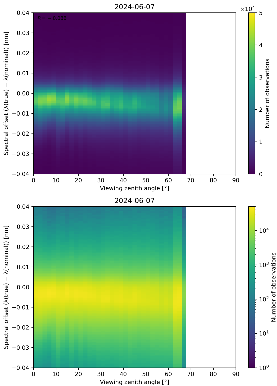
Figure 128: Scatter density plot of “Viewing zenith angle” against “Spectral offset ( \lambda(\text{true}) - \lambda(\text{nominal}) )” for 2024-06-06 to 2024-06-08.
