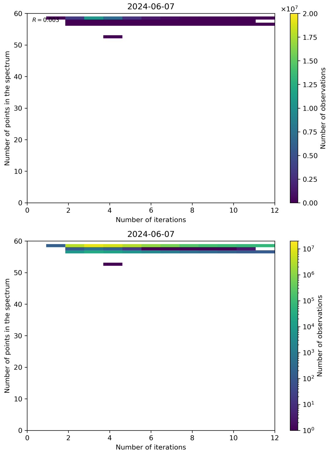
Figure 99: Scatter density plot of “Number of iterations” against “Number of points in the spectrum” for 2024-06-06 to 2024-06-08.
