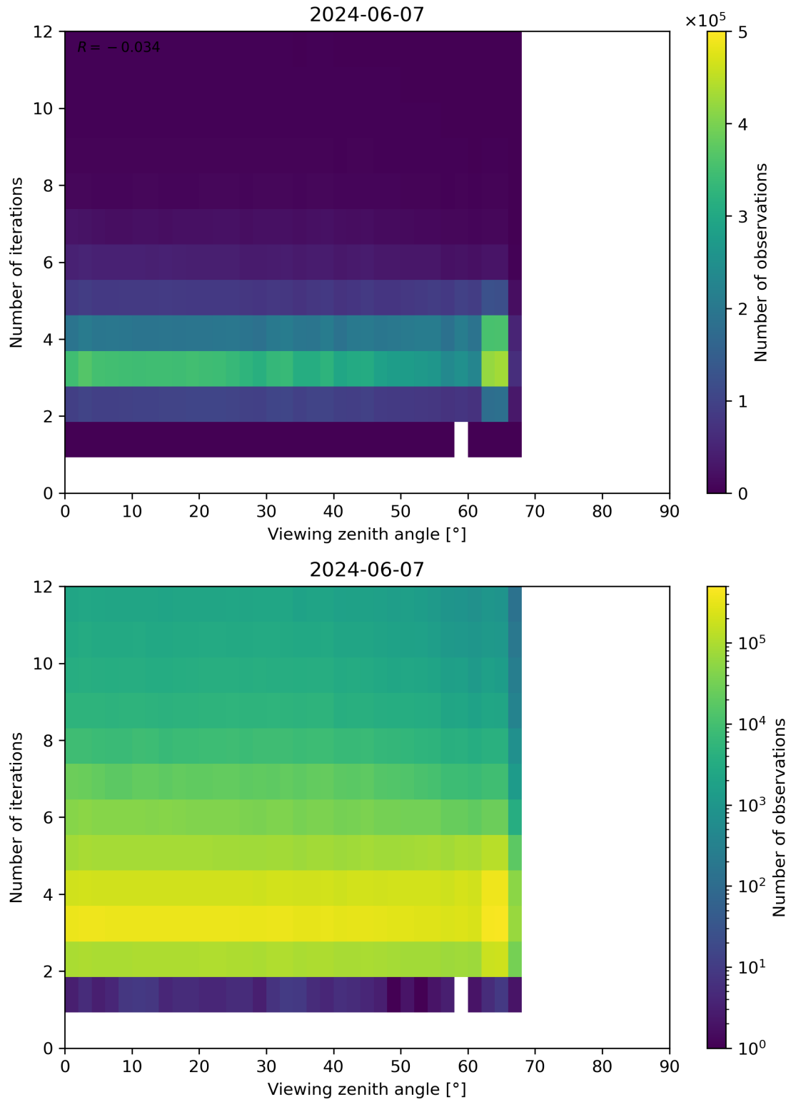
Figure 124: Scatter density plot of “Viewing zenith angle” against “Number of iterations” for 2024-06-06 to 2024-06-08.
