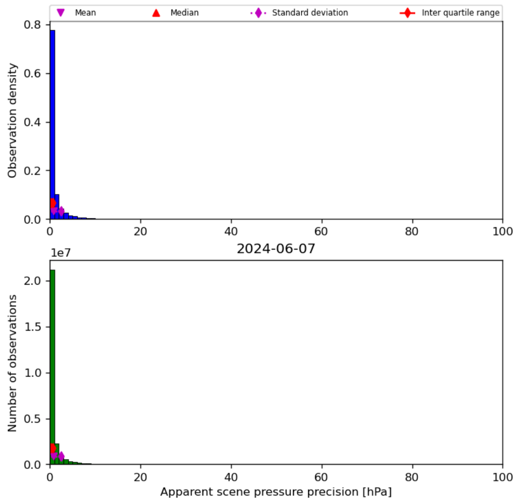
Figure 37: Histogram of “Apparent scene pressure precision” for 2024-06-06 to 2024-06-08
