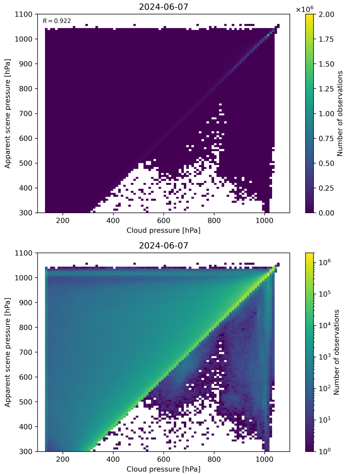
Figure 77: Scatter density plot of “Cloud pressure” against “Apparent scene pressure” for 2024-06-06 to 2024-06-08.
