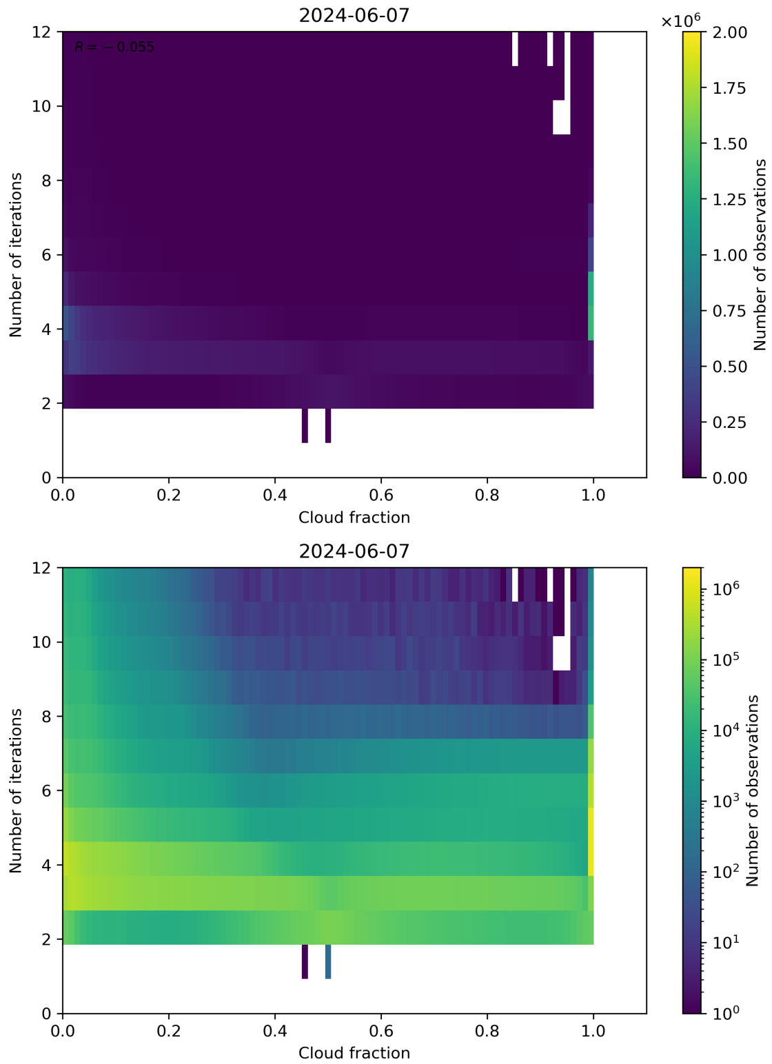
Figure 73: Scatter density plot of “Cloud fraction” against “Number of iterations” for 2024-06-06 to 2024-06-08.
