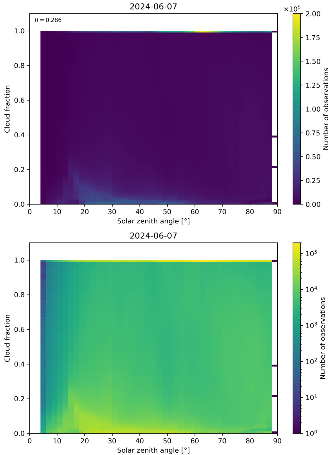
Figure 110: Scatter density plot of “Solar zenith angle” against “Cloud fraction” for 2024-06-06 to 2024-06-08.
