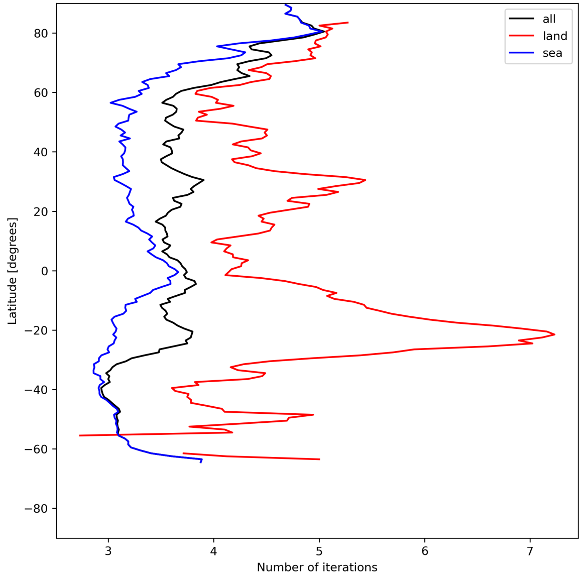
Figure 22: Zonal average of “Number of iterations” for 2024-06-06 to 2024-06-08.
