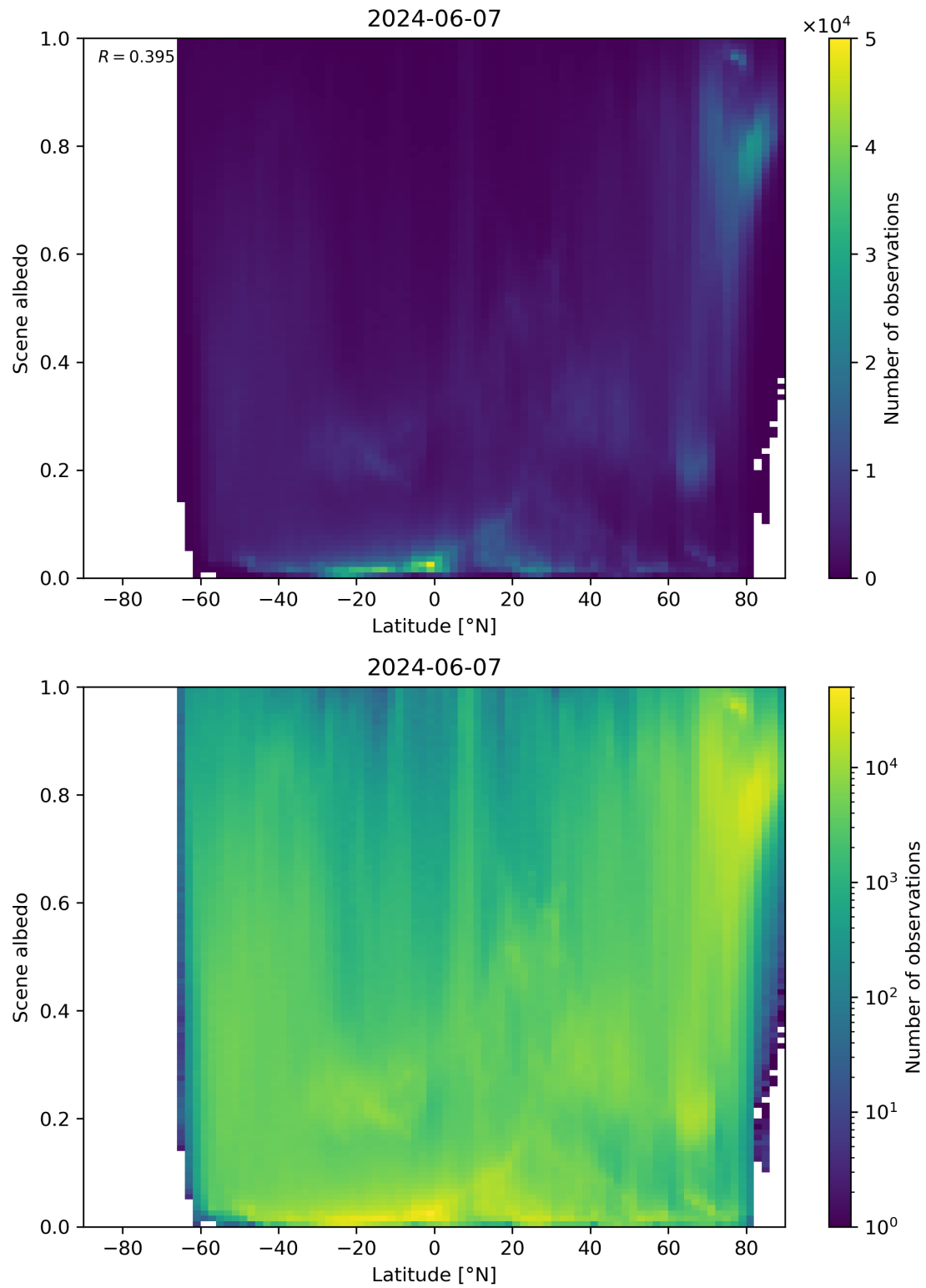
Figure 95: Scatter density plot of “Latitude” against “Scene albedo” for 2024-06-06 to 2024-06-08.
