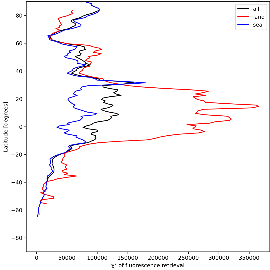
Figure 25: Zonal average of “ \chi^2 of fluorescence retrieval” for 2024-06-06 to 2024-06-08.
