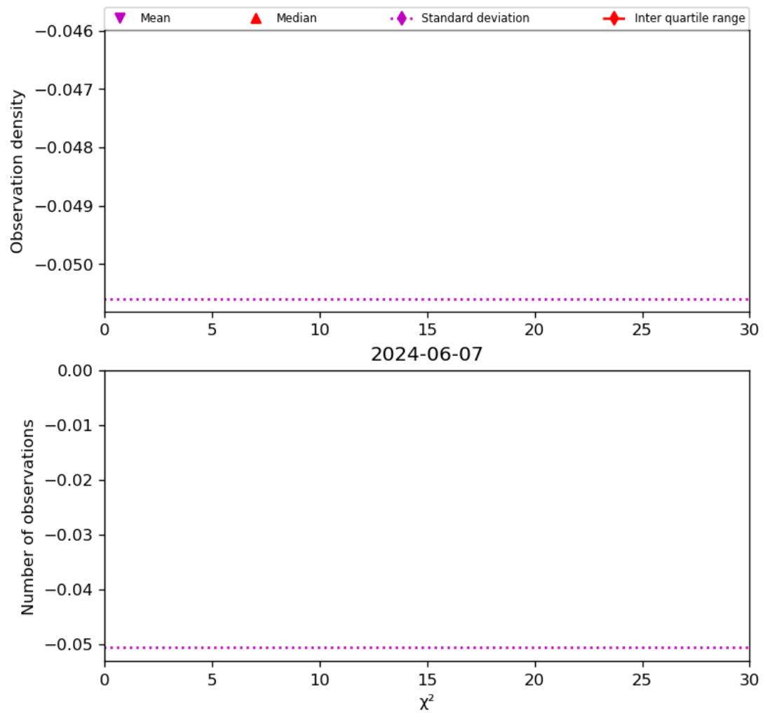
Figure 38: Histogram of “ \chi^2 ” for 2024-06-06 to 2024-06-08
