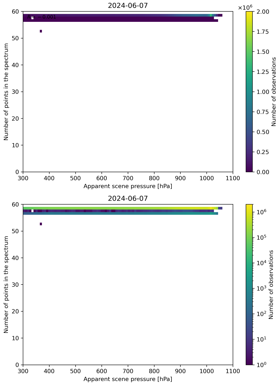
Figure 66: Scatter density plot of “Apparent scene pressure” against “Number of points in the spectrum” for 2024-06-06 to 2024-06-08.
