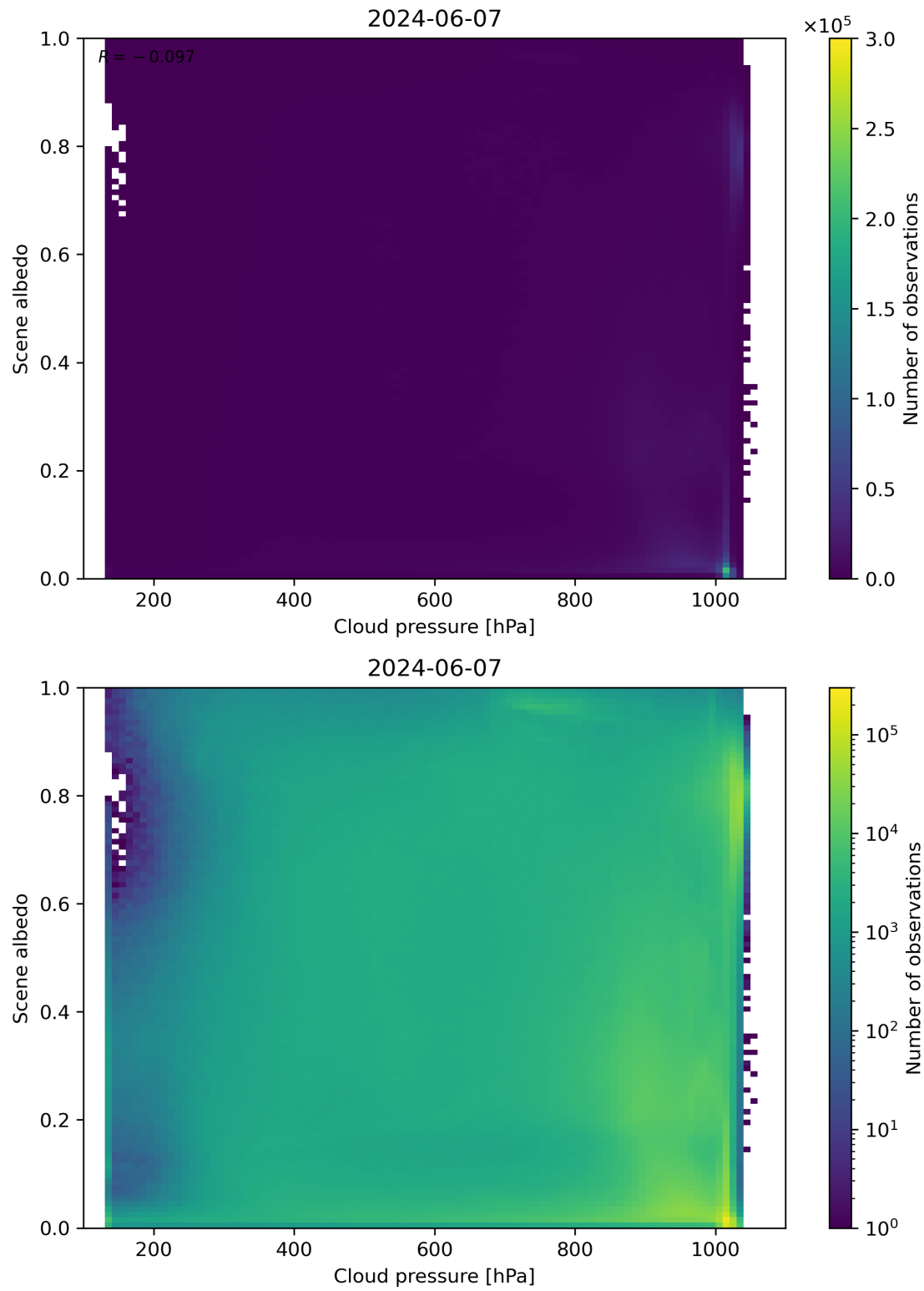
Figure 83: Scatter density plot of “Cloud pressure” against “Scene albedo” for 2024-06-06 to 2024-06-08.
