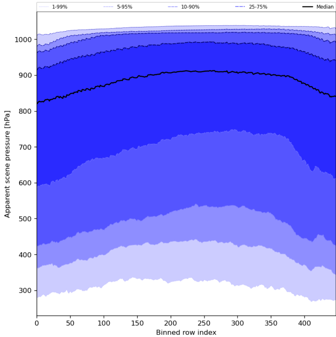
Figure 53: Along track statistics of “Apparent scene pressure” for 2024-06-06 to 2024-06-08
