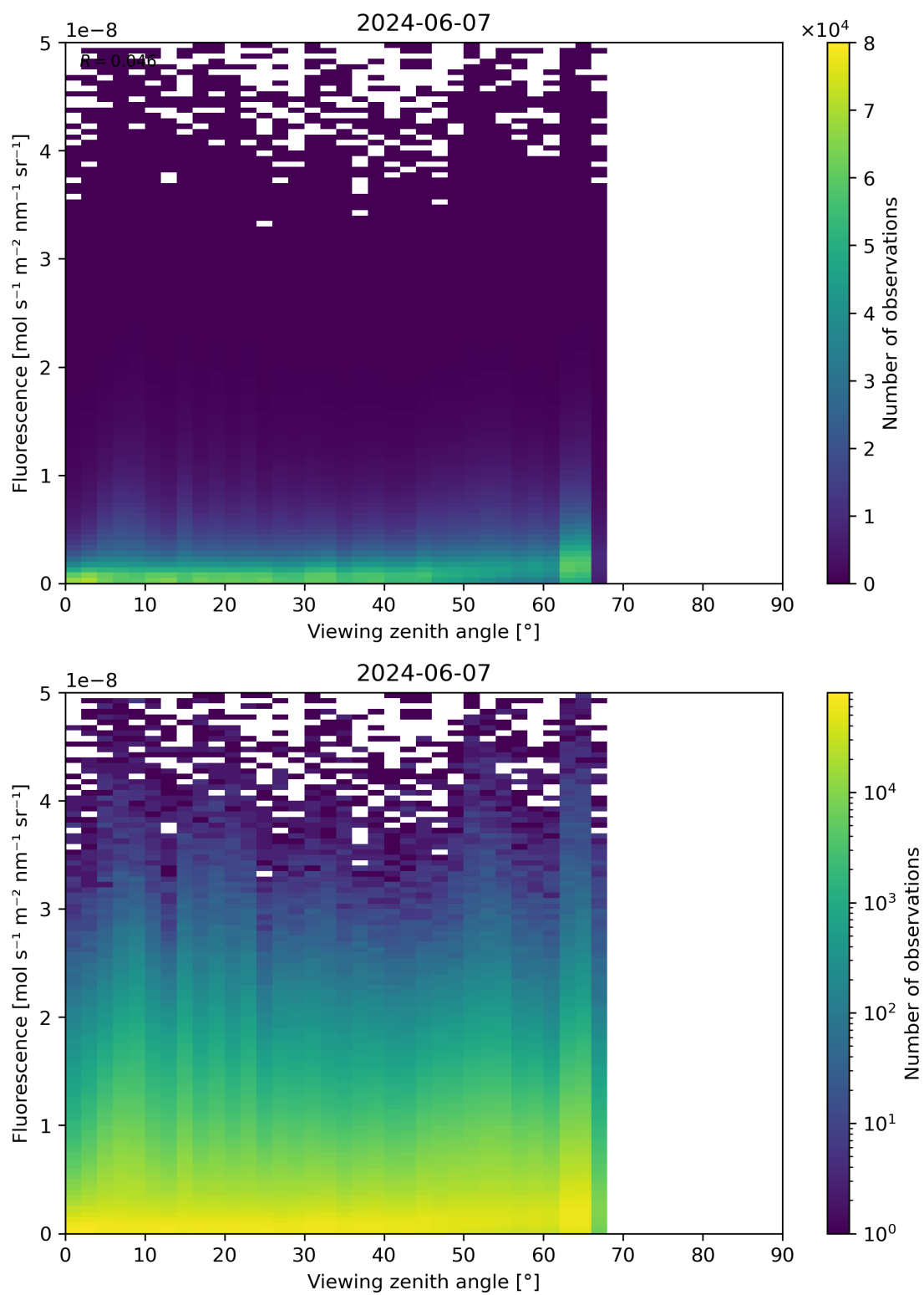
Figure 122: Scatter density plot of “Viewing zenith angle” against “Fluorescence” for 2024-06-06 to 2024-06-08.
