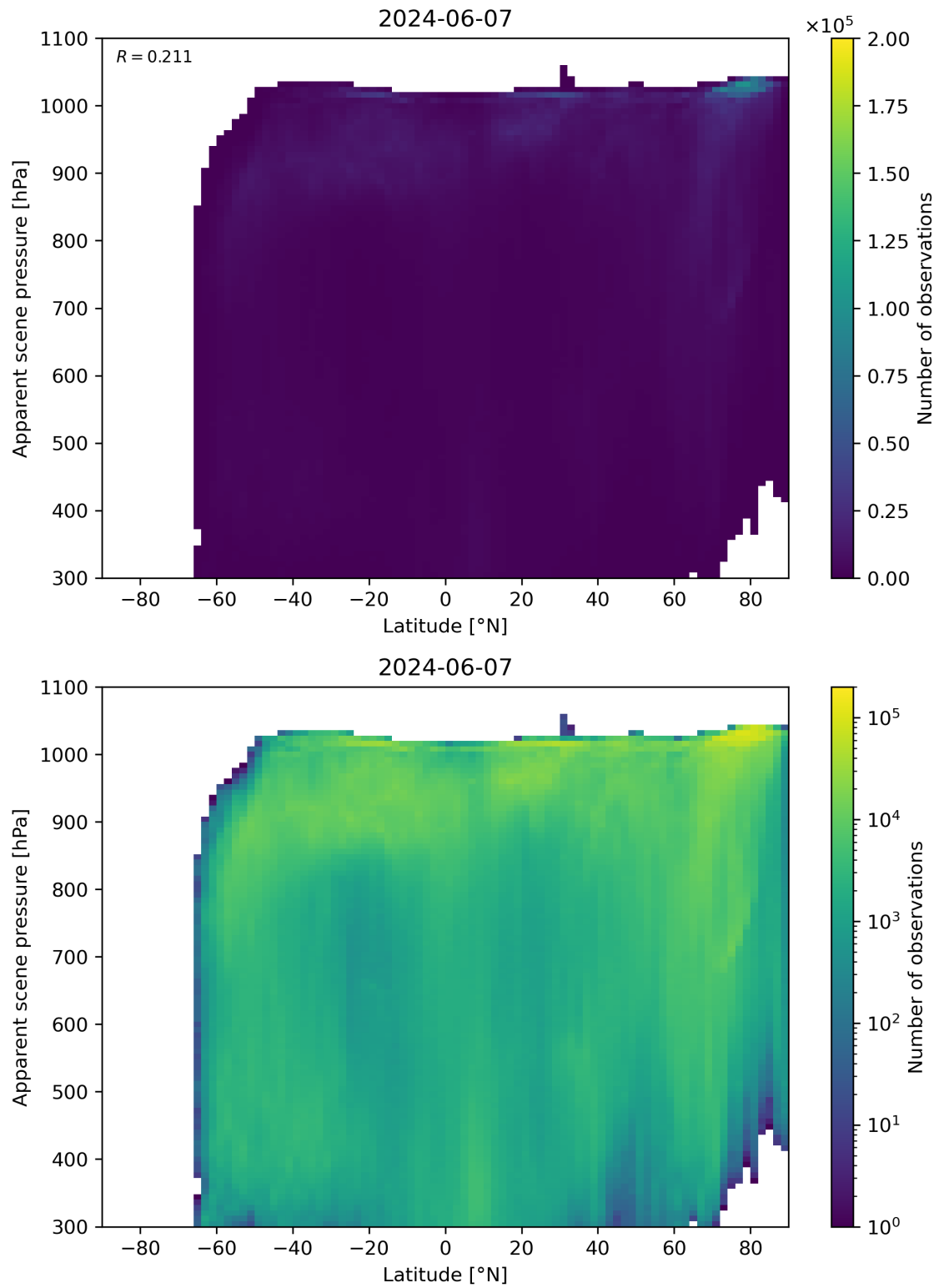
Figure 88: Scatter density plot of “Latitude” against “Apparent scene pressure” for 2024-06-06 to 2024-06-08.
