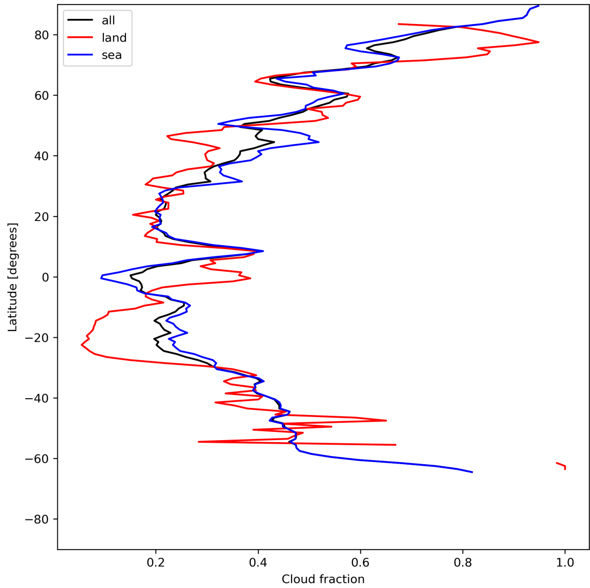
Figure 15: Zonal average of “Cloud fraction” for 2024-06-06 to 2024-06-08.
