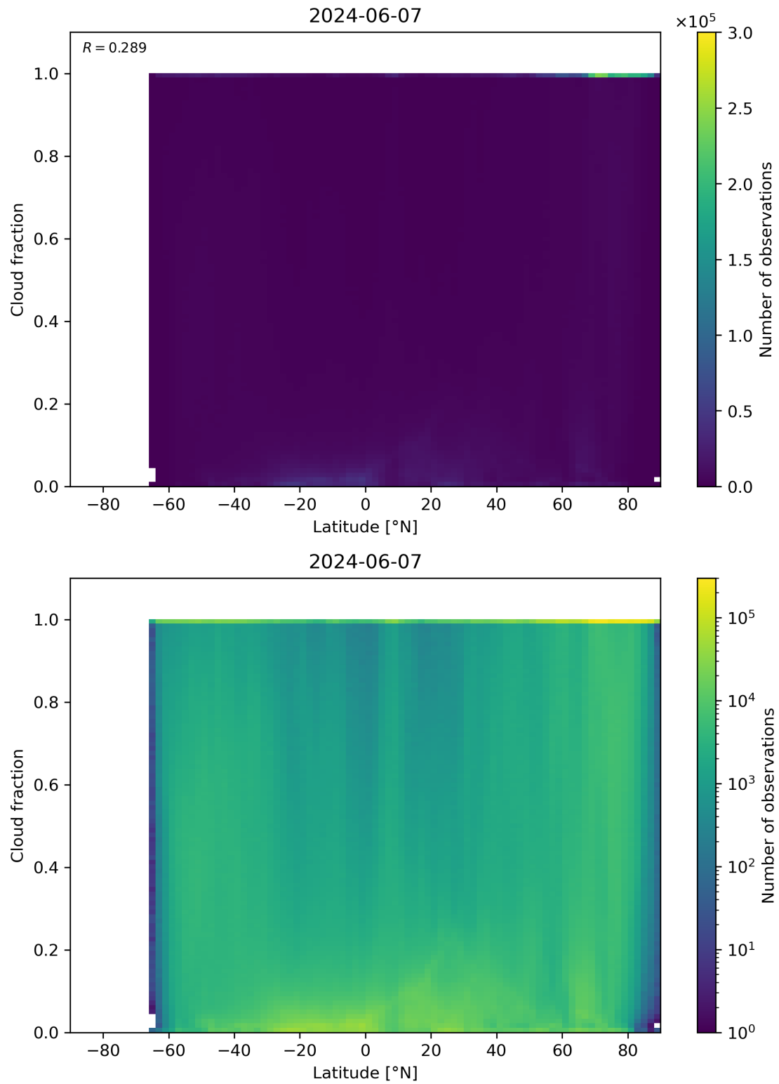
Figure 90: Scatter density plot of “Latitude” against “Cloud fraction” for 2024-06-06 to 2024-06-08.
