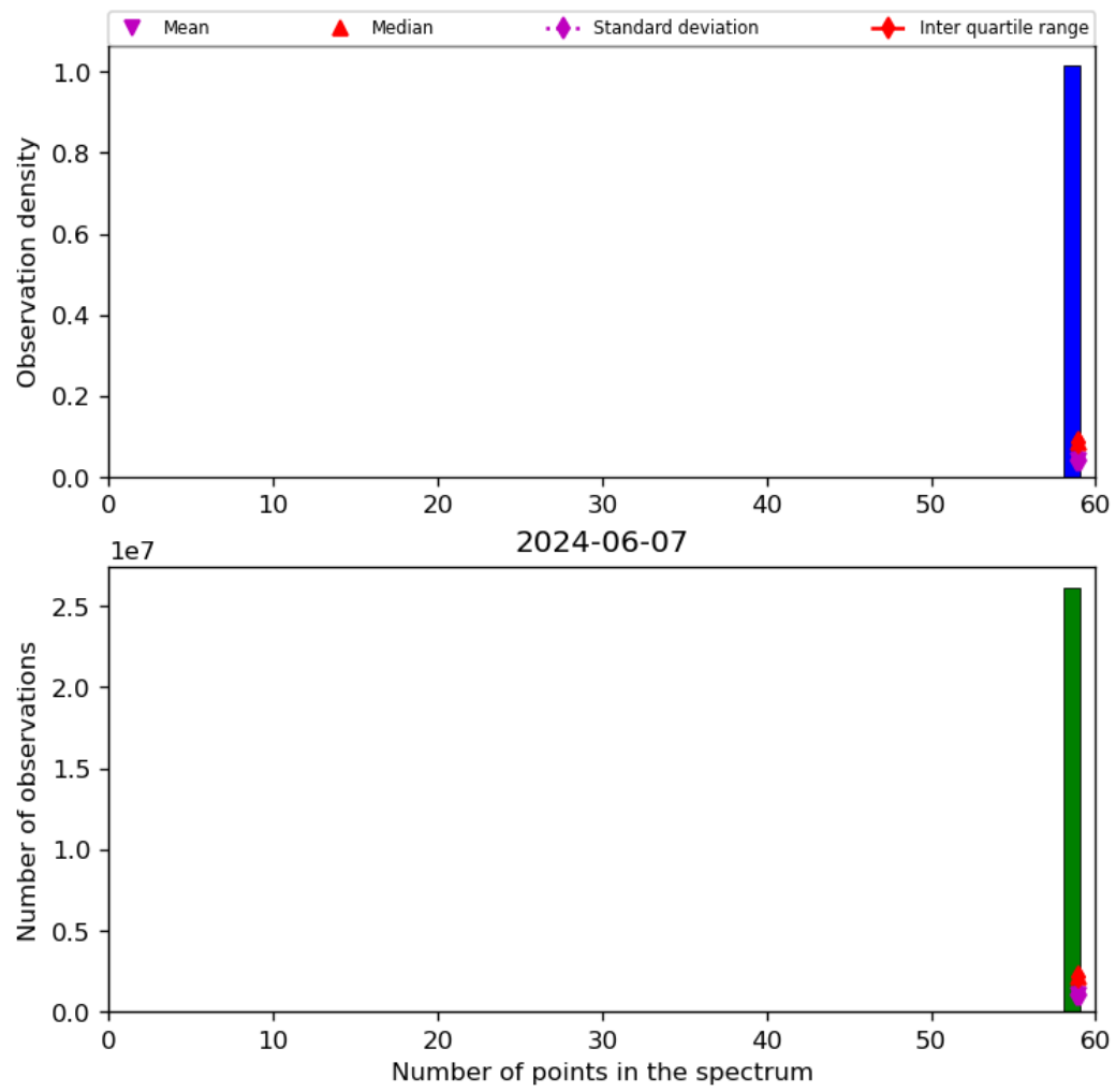
Figure 44: Histogram of “Number of points in the spectrum” for 2024-06-06 to 2024-06-08
