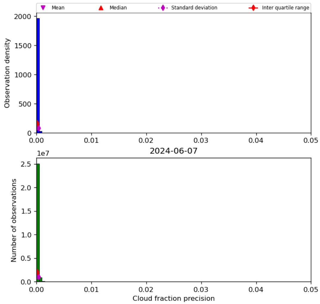
Figure 33: Histogram of “Cloud fraction precision” for 2024-06-06 to 2024-06-08
