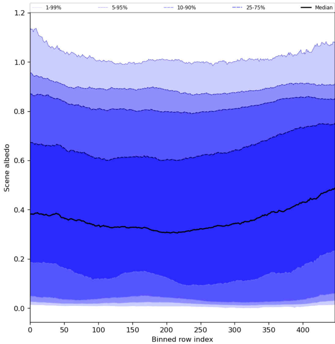
Figure 51: Along track statistics of “Scene albedo” for 2024-06-06 to 2024-06-08
