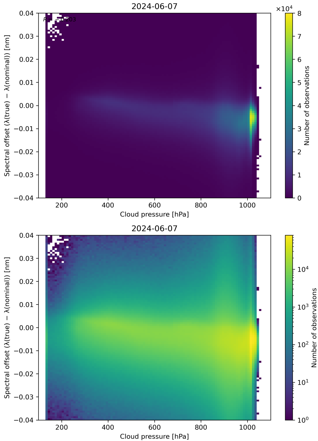
Figure 84: Scatter density plot of “Cloud pressure” against “Spectral offset ( \lambda(\text{true}) - \lambda(\text{nominal}) )” for 2024-06-06 to 2024-06-08.
