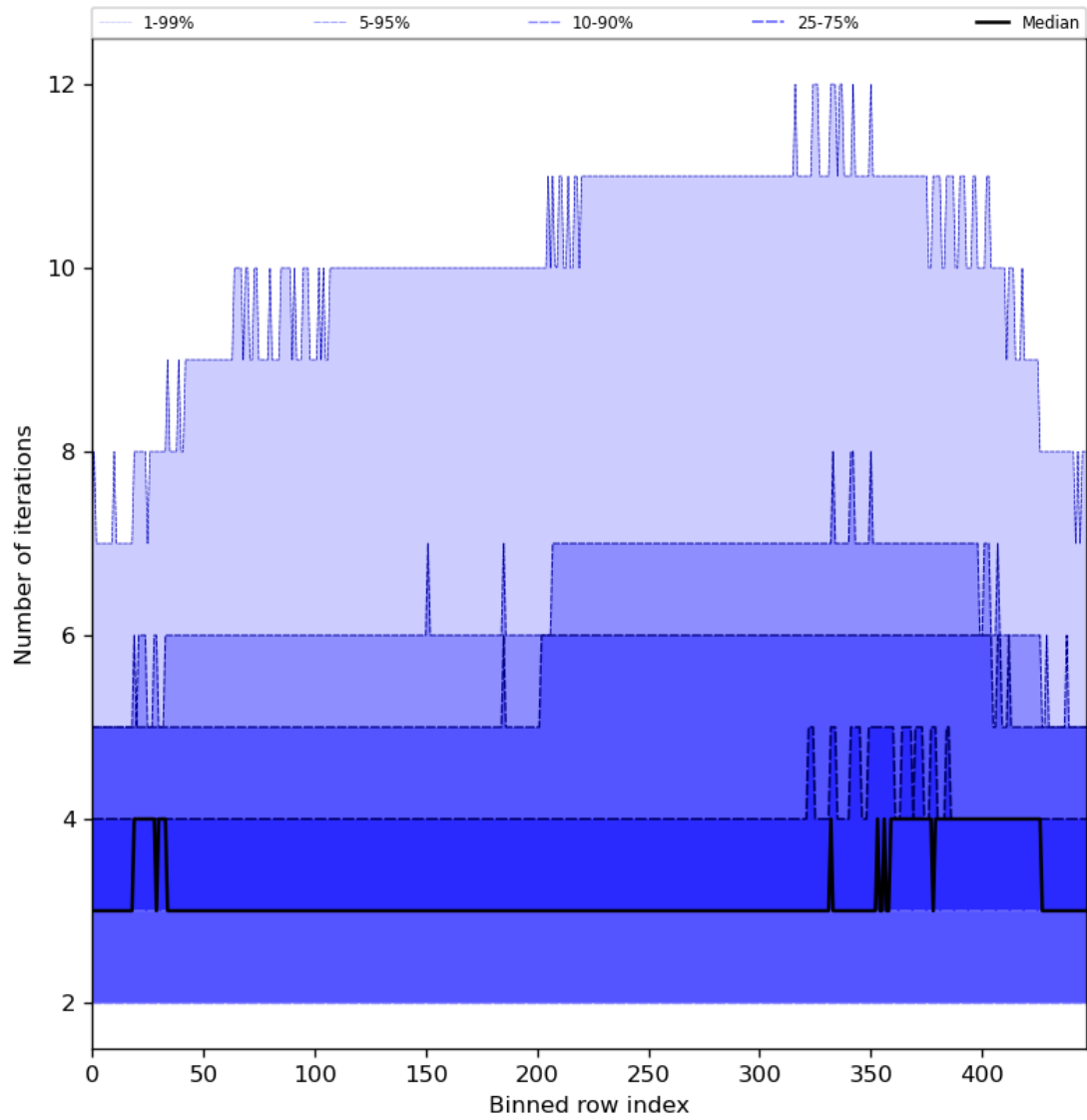
Figure 56: Along track statistics of “Number of iterations” for 2024-06-06 to 2024-06-08
