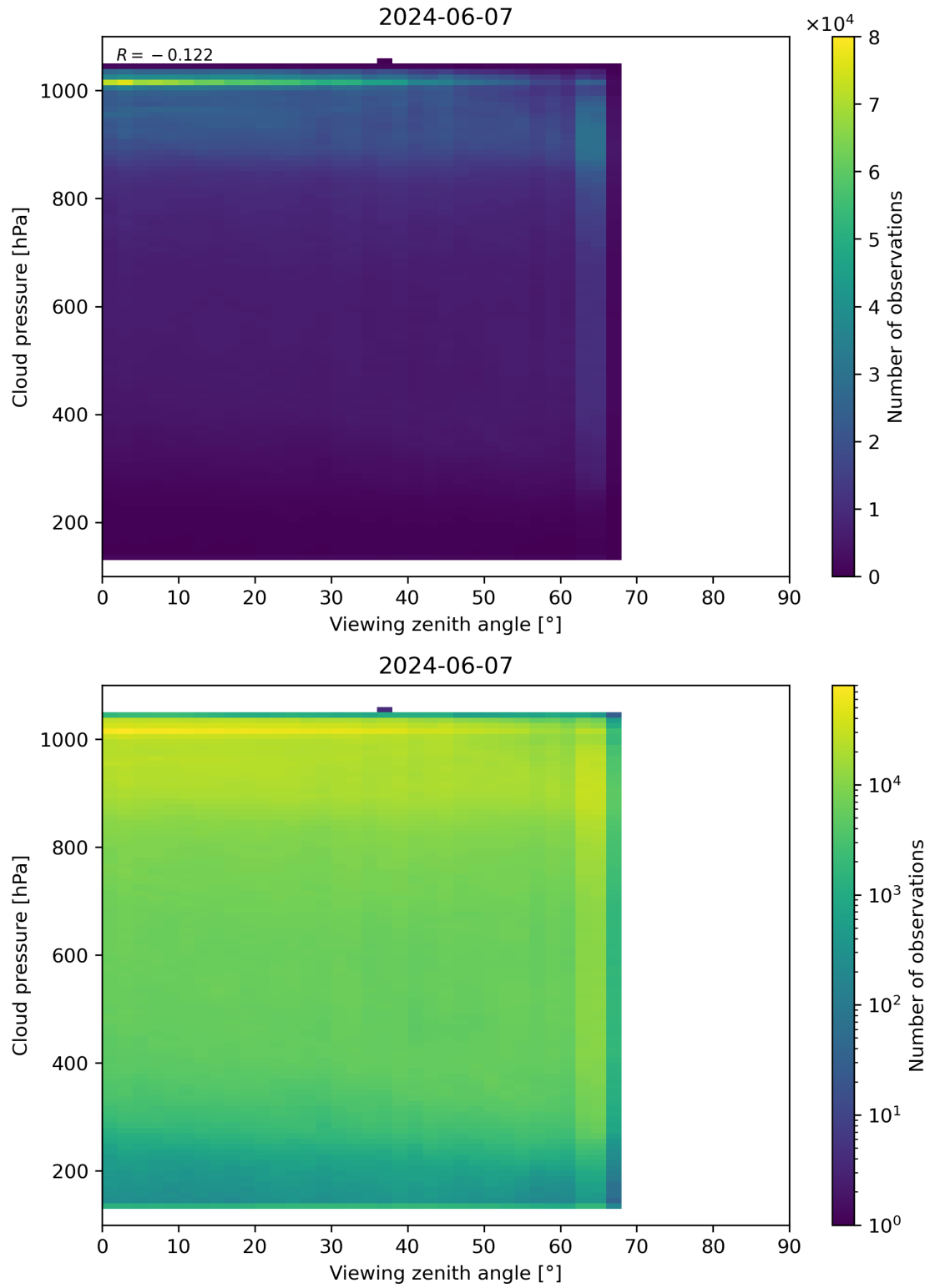
Figure 121: Scatter density plot of “Viewing zenith angle” against “Cloud pressure” for 2024-06-06 to 2024-06-08.
