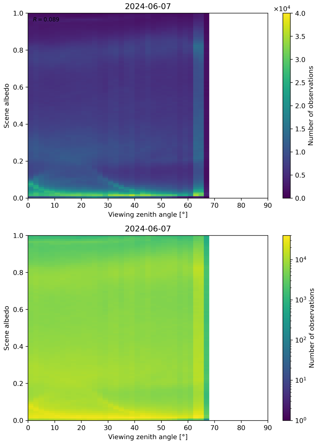
Figure 126: Scatter density plot of “Viewing zenith angle” against “Scene albedo” for 2024-06-06 to 2024-06-08.
