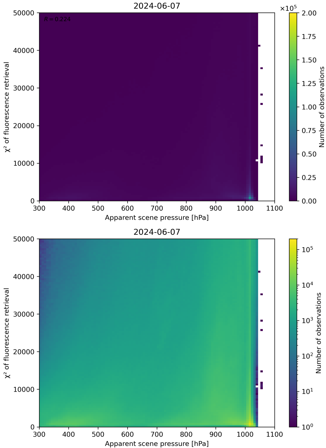
Figure 63: Scatter density plot of “Apparent scene pressure” against “ \chi^2 of fluorescence retrieval” for 2024-06-06 to 2024-06-08.
