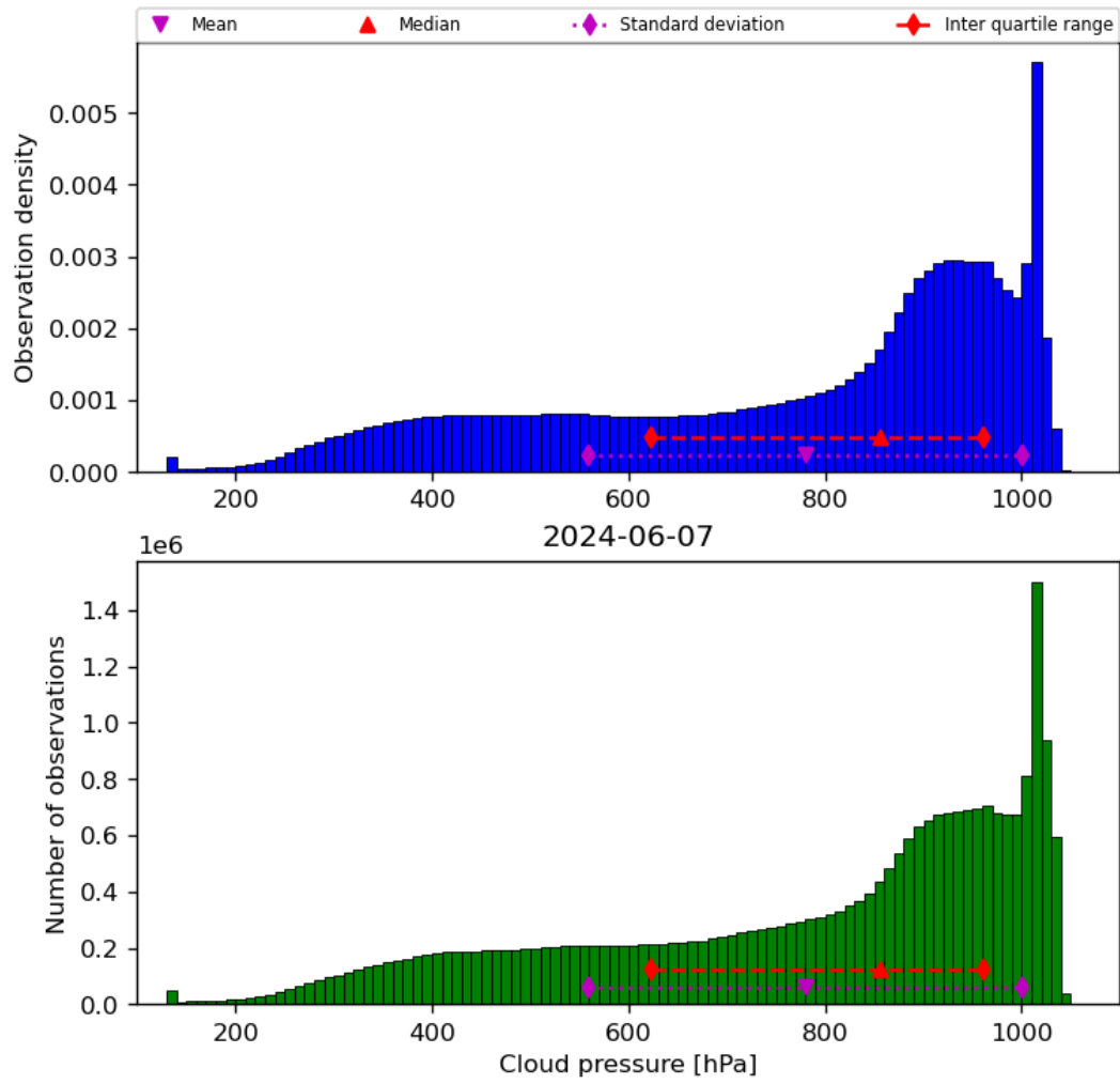
Figure 30: Histogram of “Cloud pressure” for 2024-06-06 to 2024-06-08
