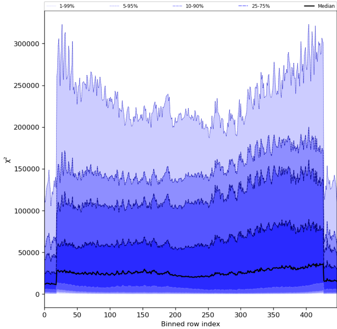
Figure 55: Along track statistics of “ \chi^2 ” for 2024-06-06 to 2024-06-08
