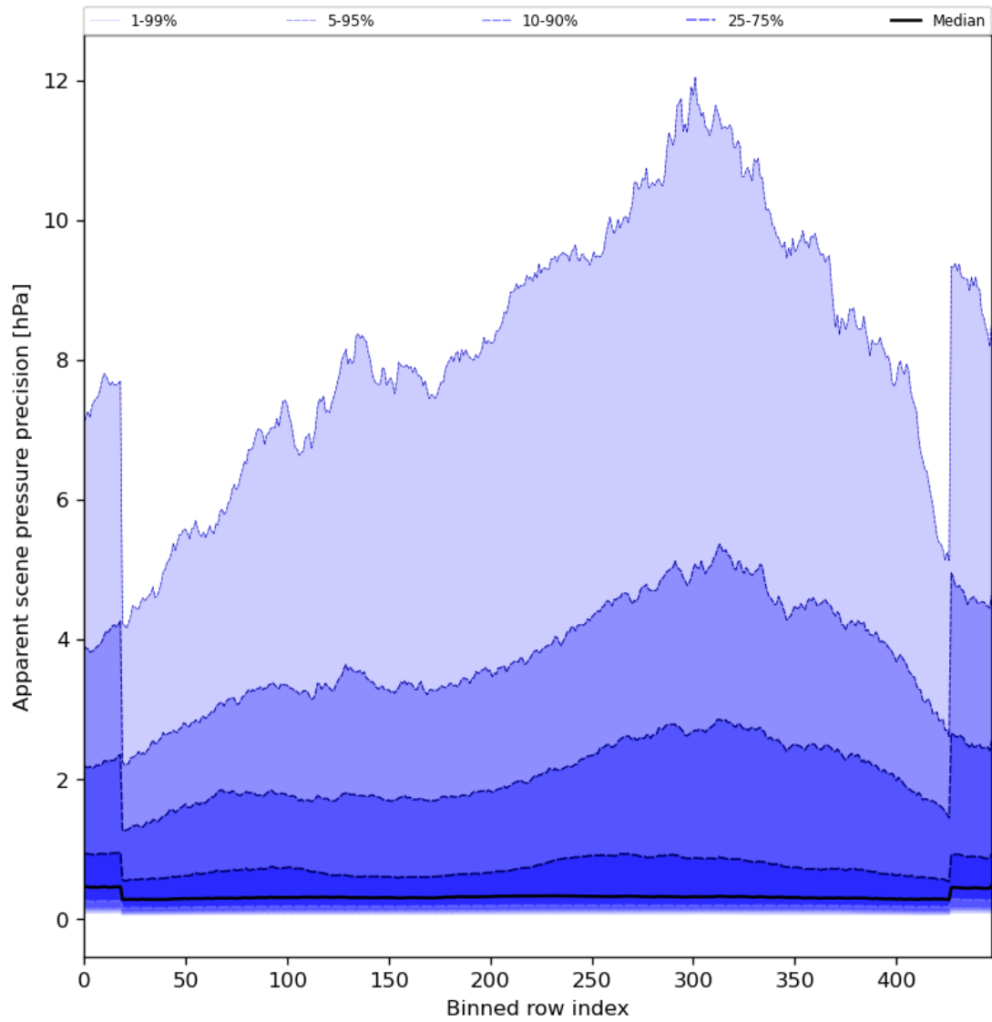
Figure 54: Along track statistics of “Apparent scene pressure precision” for 2024-06-06 to 2024-06-08
