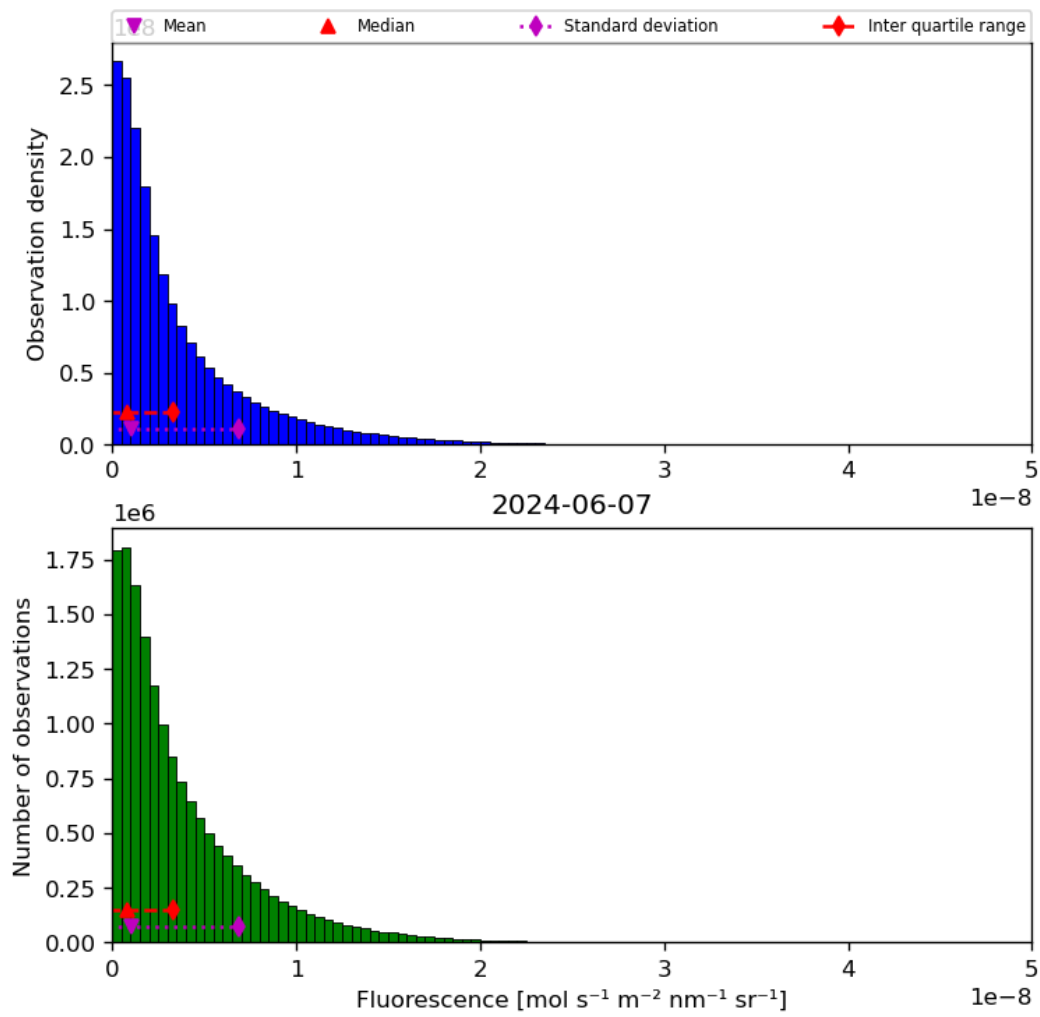
Figure 40: Histogram of “Fluorescence” for 2024-06-06 to 2024-06-08
