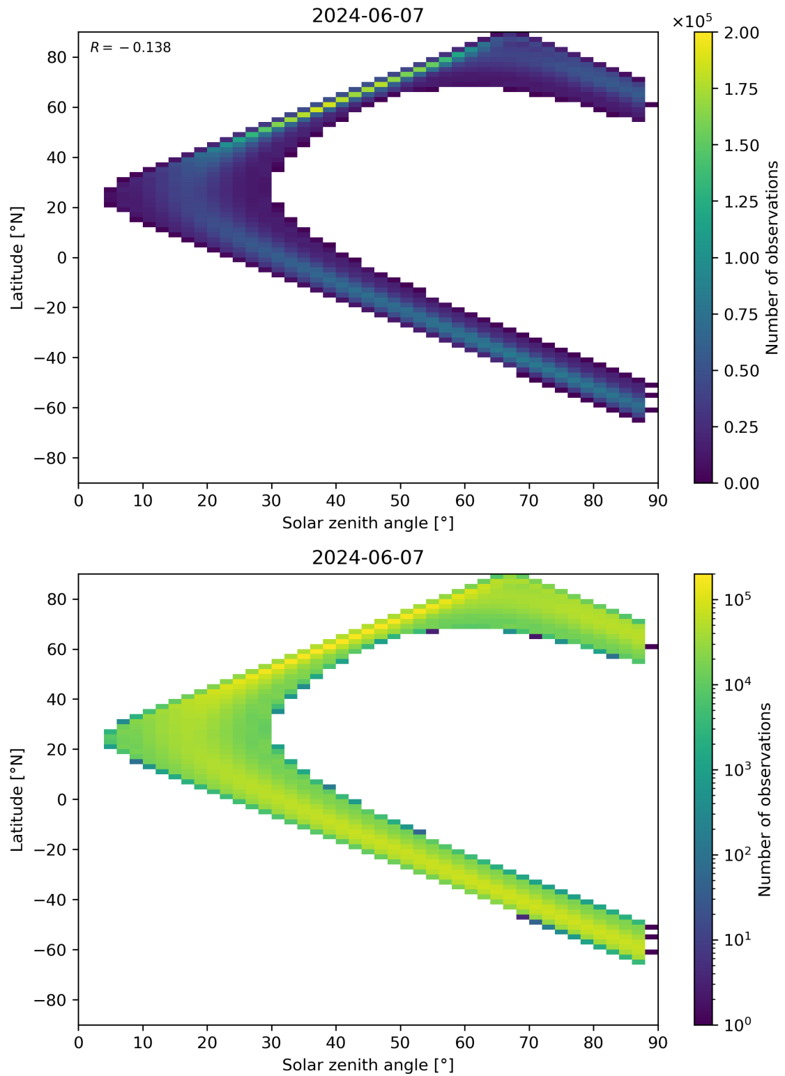
Figure 113: Scatter density plot of “Solar zenith angle” against “Latitude” for 2024-06-06 to 2024-06-08.
