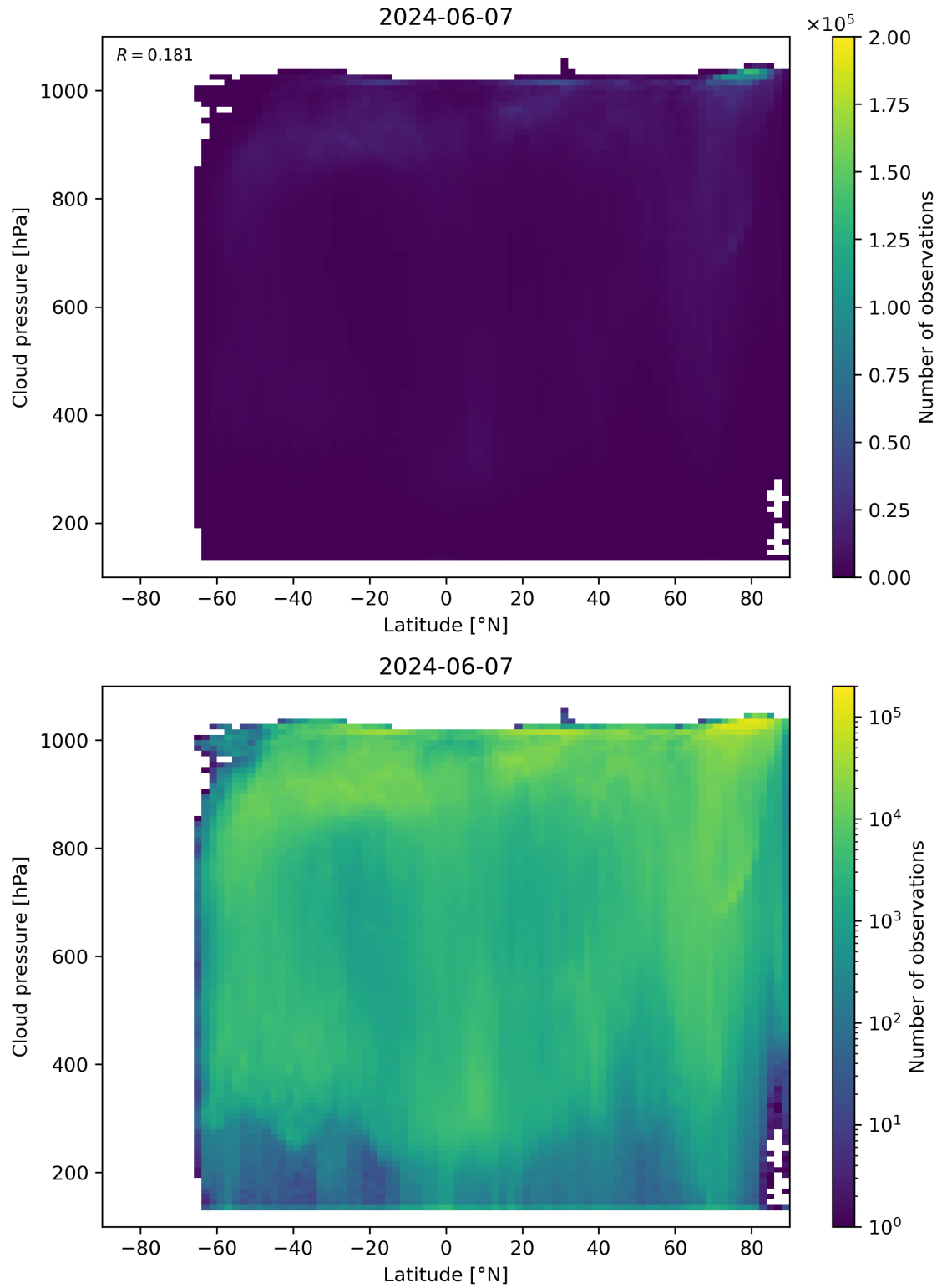
Figure 91: Scatter density plot of “Latitude” against “Cloud pressure” for 2024-06-06 to 2024-06-08.
