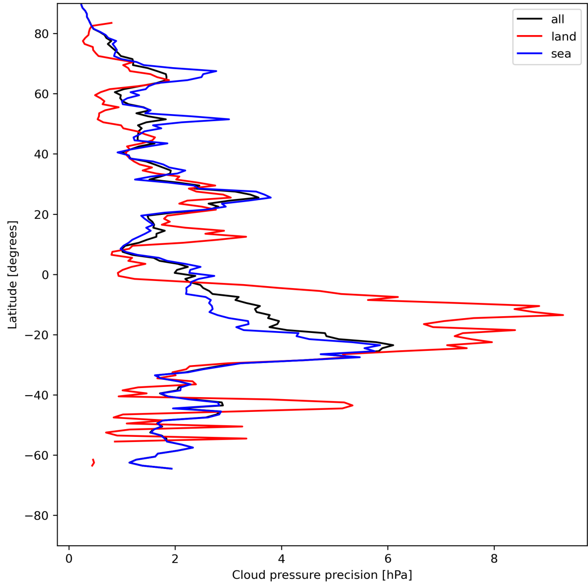
Figure 14: Zonal average of “Cloud pressure precision” for 2024-06-06 to 2024-06-08.
