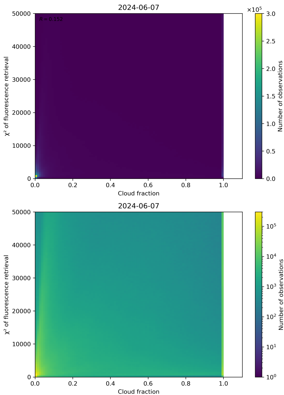
Figure 71: Scatter density plot of “Cloud fraction” against “ \chi^2 of fluorescence retrieval” for 2024-06-06 to 2024-06-08.
