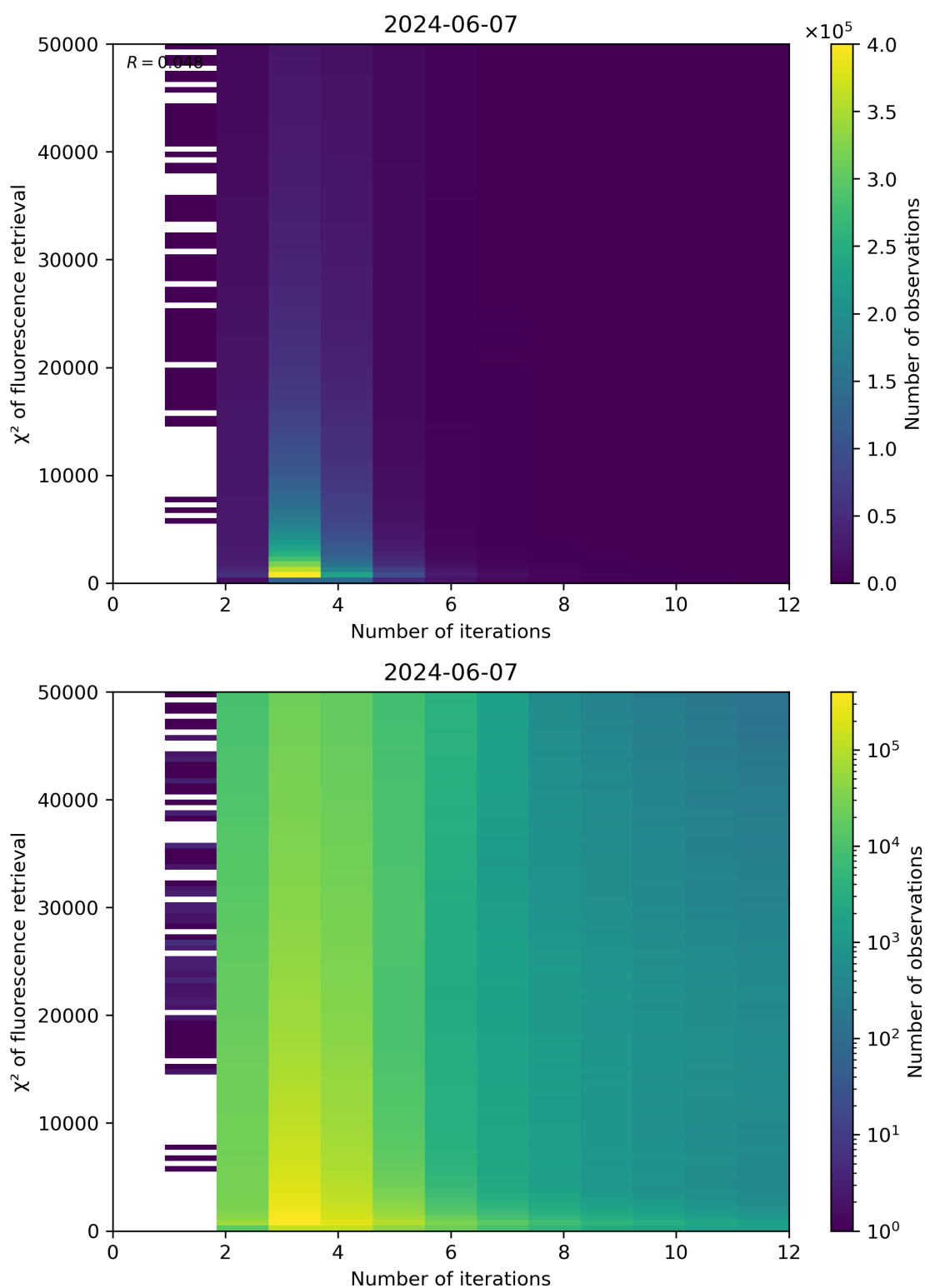
Figure 97: Scatter density plot of “Number of iterations” against “ \chi^2 of fluorescence retrieval” for 2024-06-06 to 2024-06-08.
