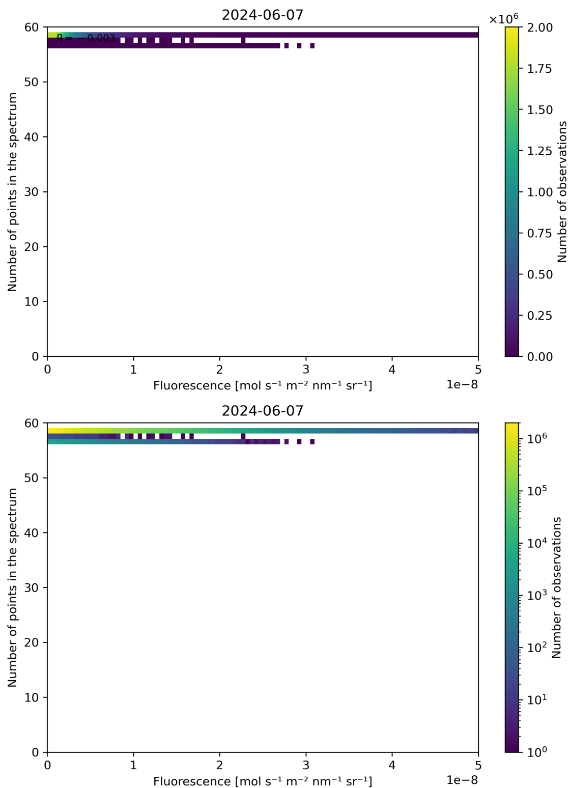
Figure 86: Scatter density plot of “Fluorescence” against “Number of points in the spectrum” for 2024-06-06 to 2024-06-08.
