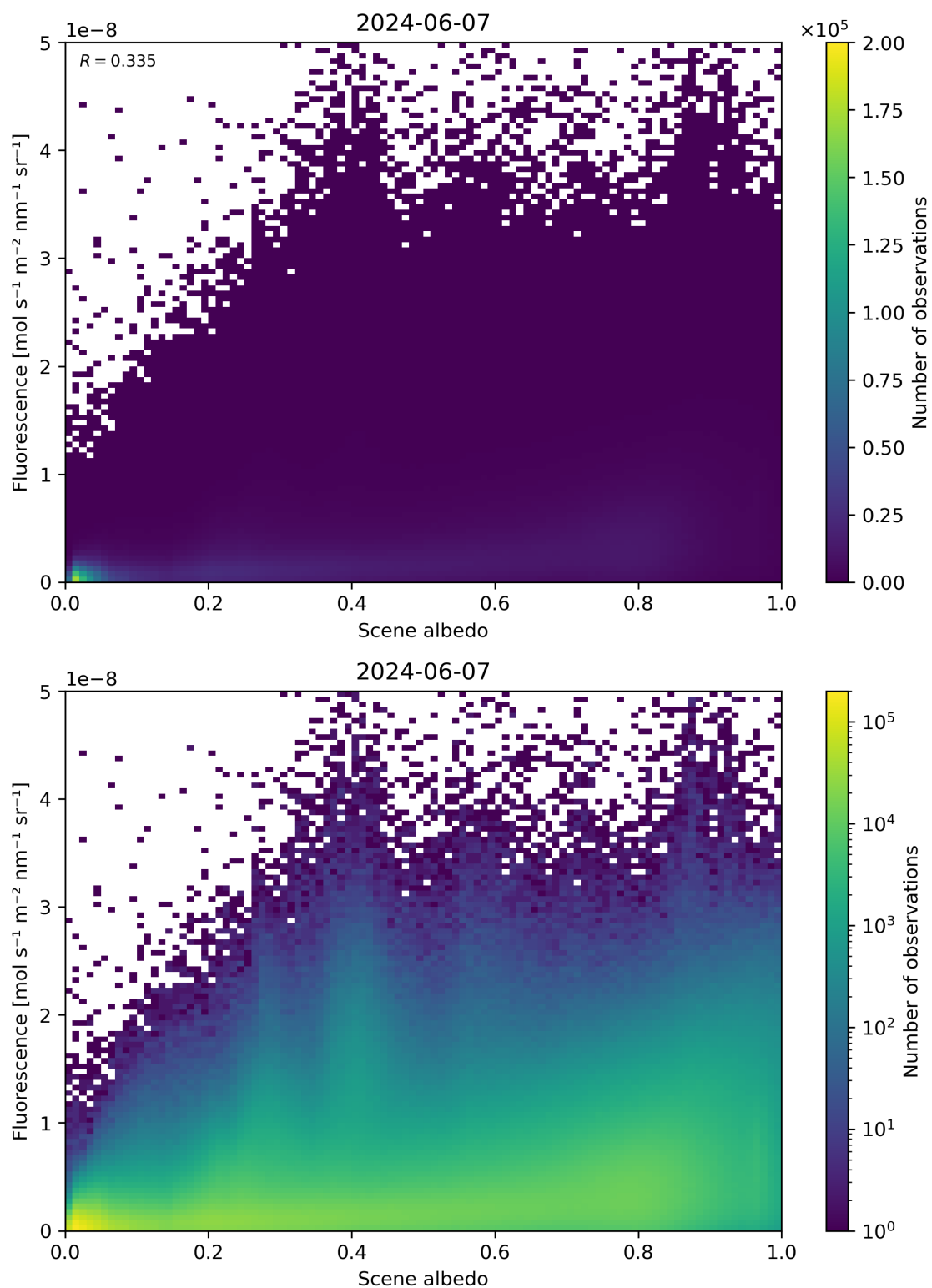
Figure 104: Scatter density plot of “Scene albedo” against “Fluorescence” for 2024-06-06 to 2024-06-08.
