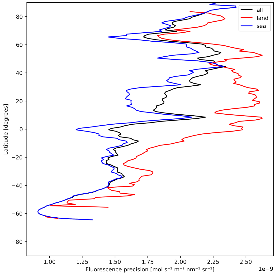
Figure 24: Zonal average of “Fluorescence precision” for 2024-06-06 to 2024-06-08.
