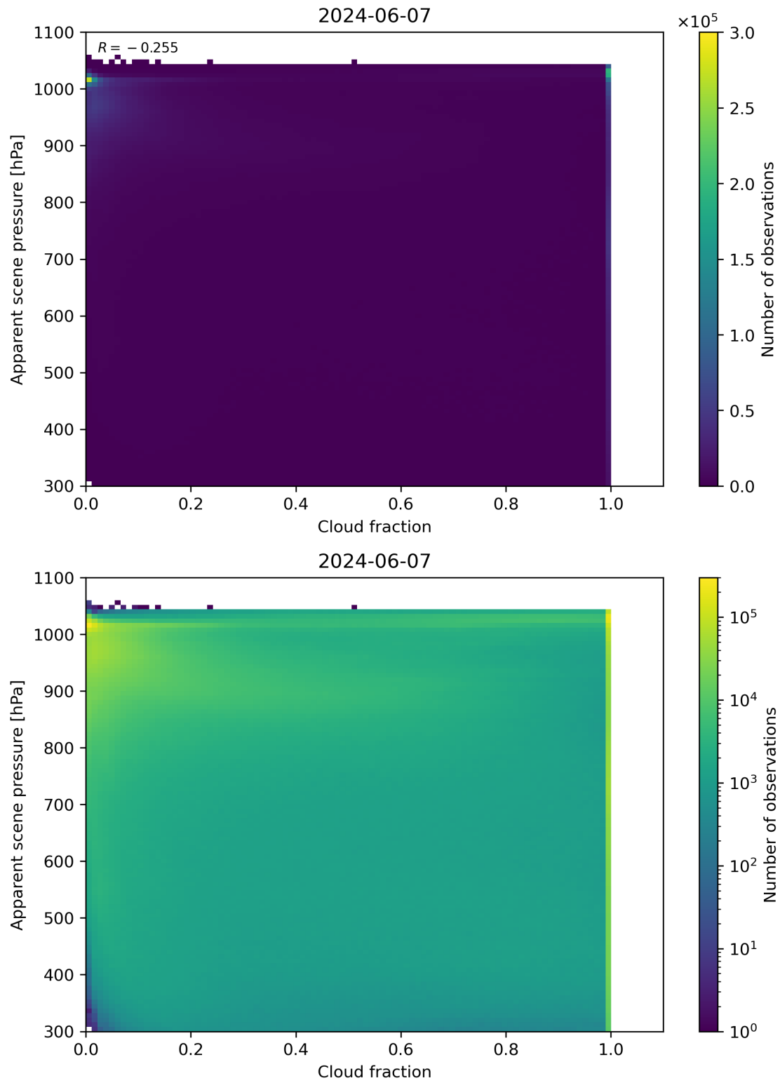
Figure 70: Scatter density plot of “Cloud fraction” against “Apparent scene pressure” for 2024-06-06 to 2024-06-08.
