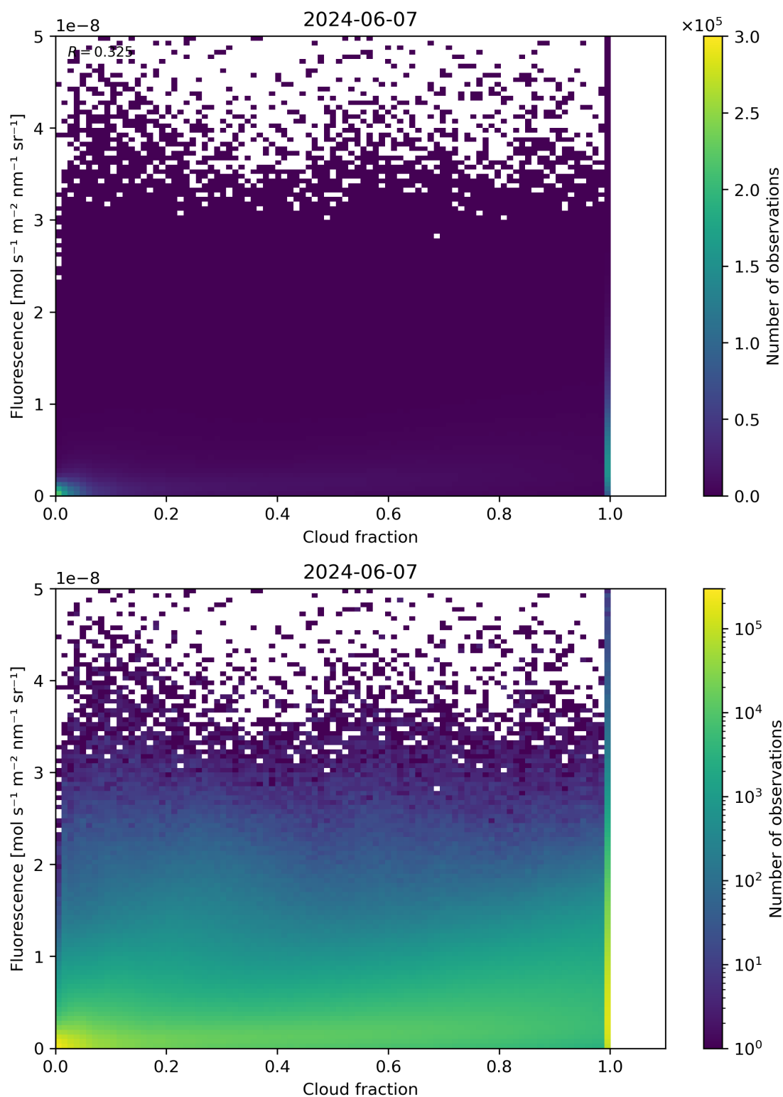
Figure 72: Scatter density plot of “Cloud fraction” against “Fluorescence” for 2024-06-06 to 2024-06-08.
