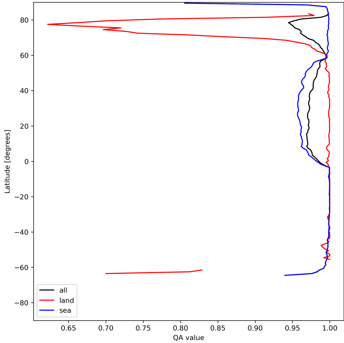
Figure 12: Zonal average of “QA value” for 2024-06-06 to 2024-06-08.
