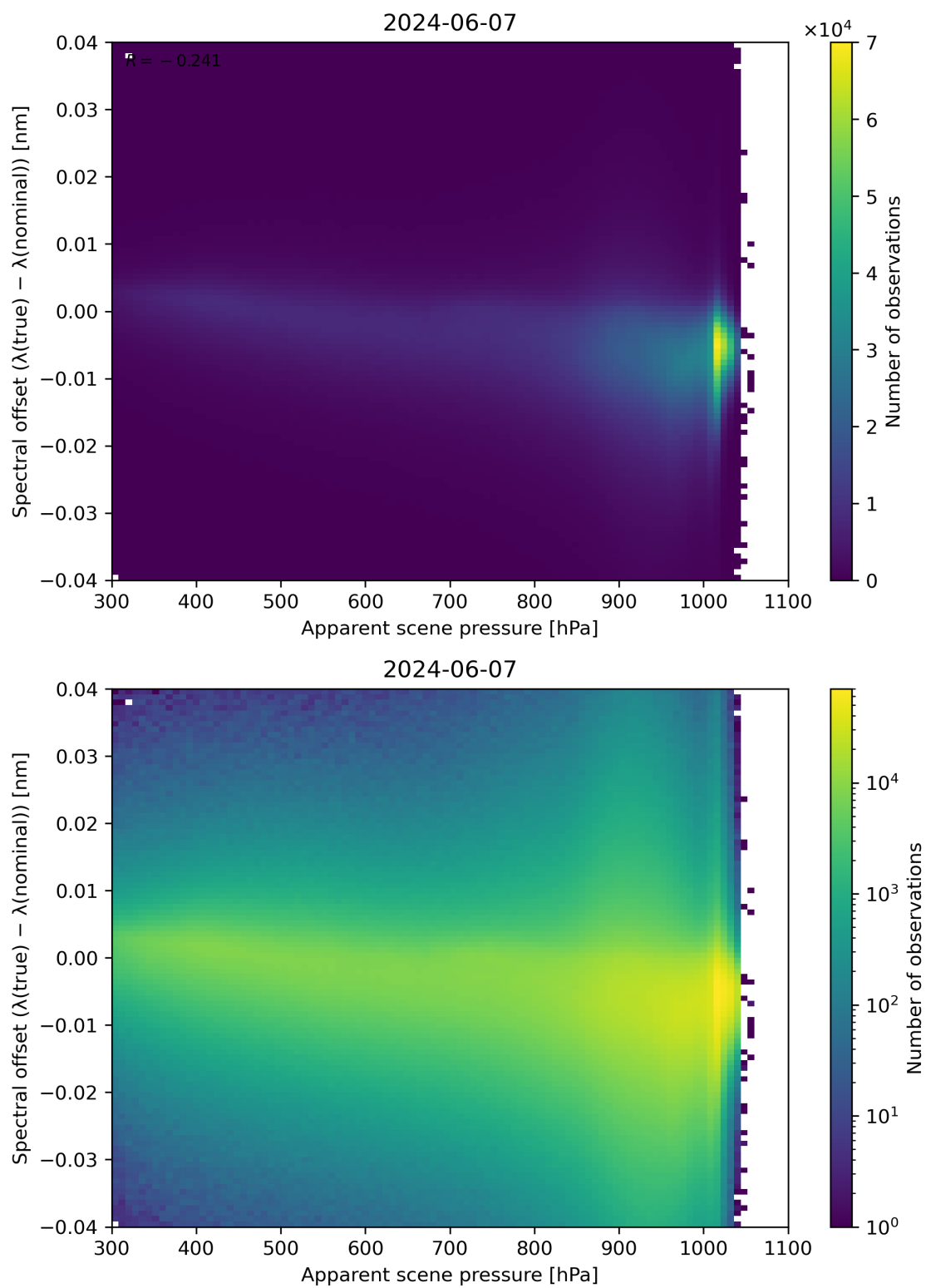
Figure 67: Scatter density plot of “Apparent scene pressure” against “Spectral offset ( \lambda(\text{true}) - \lambda(\text{nominal}) )” for 2024-06-06 to 2024-06-08.
