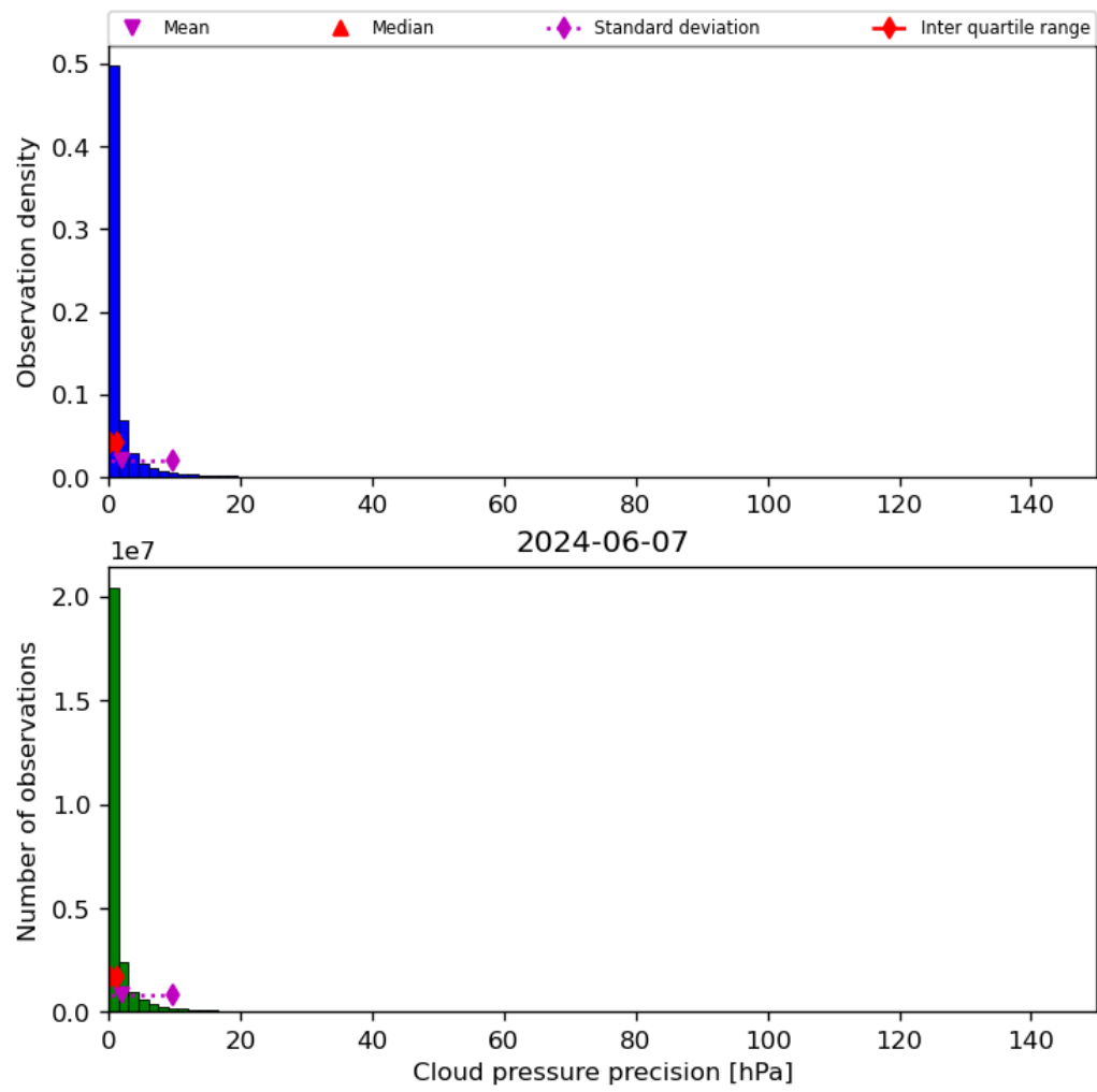
Figure 31: Histogram of “Cloud pressure precision” for 2024-06-06 to 2024-06-08
