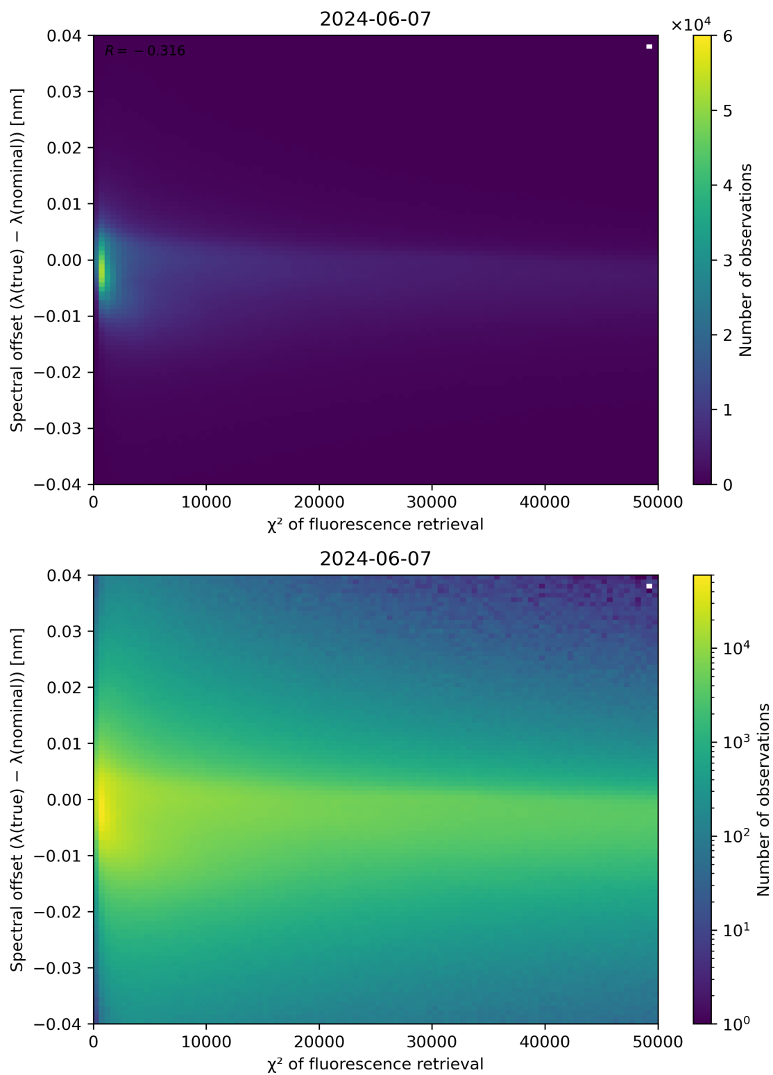
Figure 69: Scatter density plot of " \chi^2 of fluorescence retrieval" against "Spectral offset ( \lambda(\text{true}) - \lambda(\text{nominal}) )" for 2024-06-06 to 2024-06-08.
