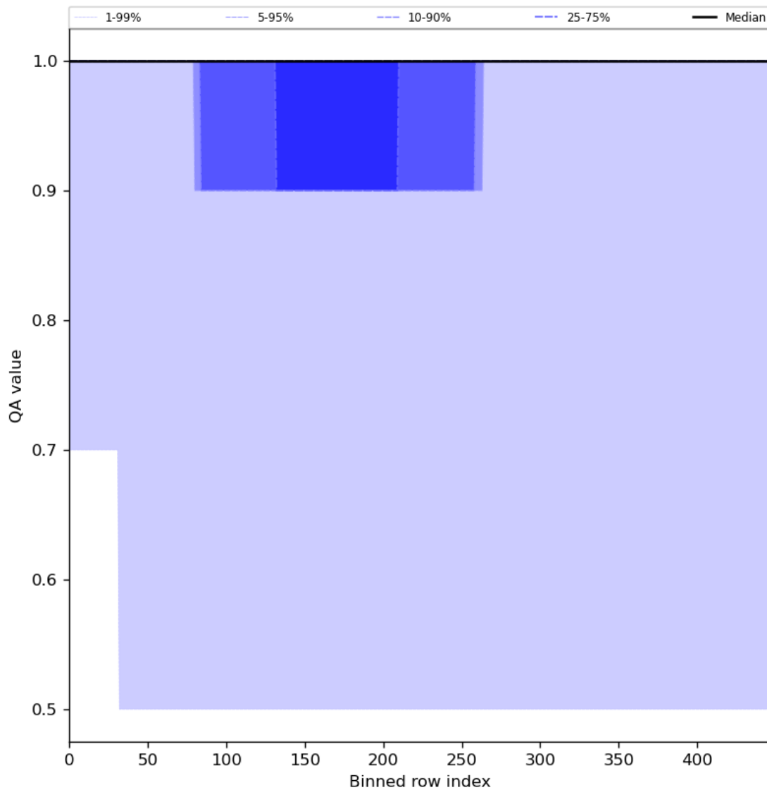
Figure 46: Along track statistics of “QA value” for 2024-06-06 to 2024-06-08
