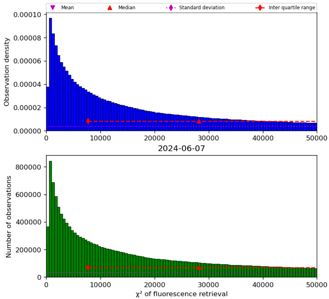
Figure 42: Histogram of “ \chi^2 of fluorescence retrieval” for 2024-06-06 to 2024-06-08
