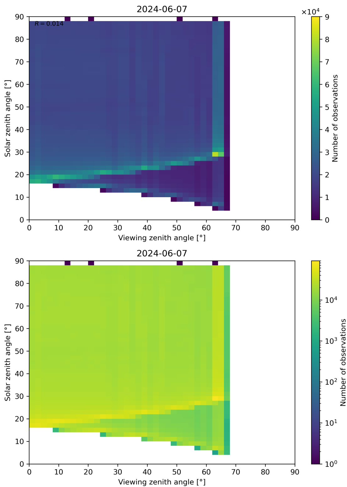
Figure 127: Scatter density plot of “Viewing zenith angle” against “Solar zenith angle” for 2024-06-06 to 2024-06-08.
