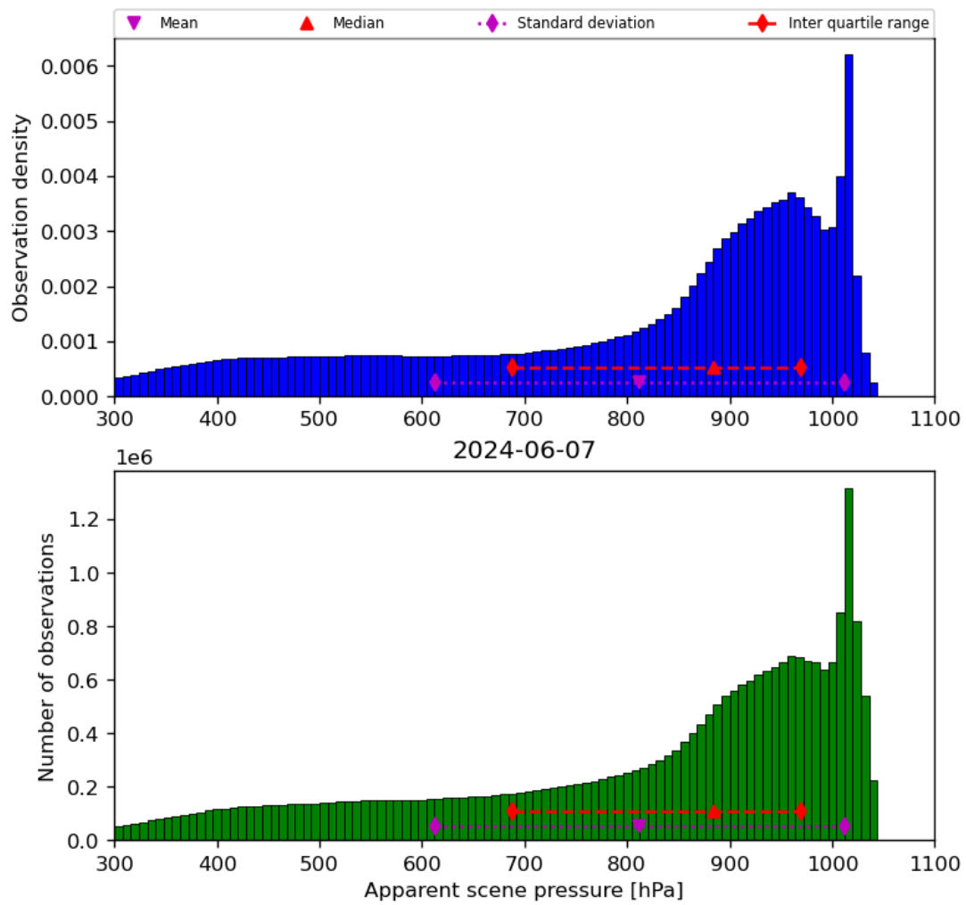
Figure 36: Histogram of “Apparent scene pressure” for 2024-06-06 to 2024-06-08
