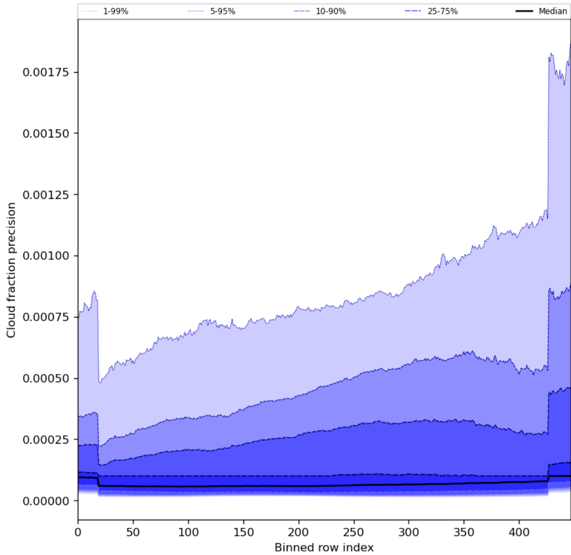
Figure 50: Along track statistics of “Cloud fraction precision” for 2024-06-06 to 2024-06-08
