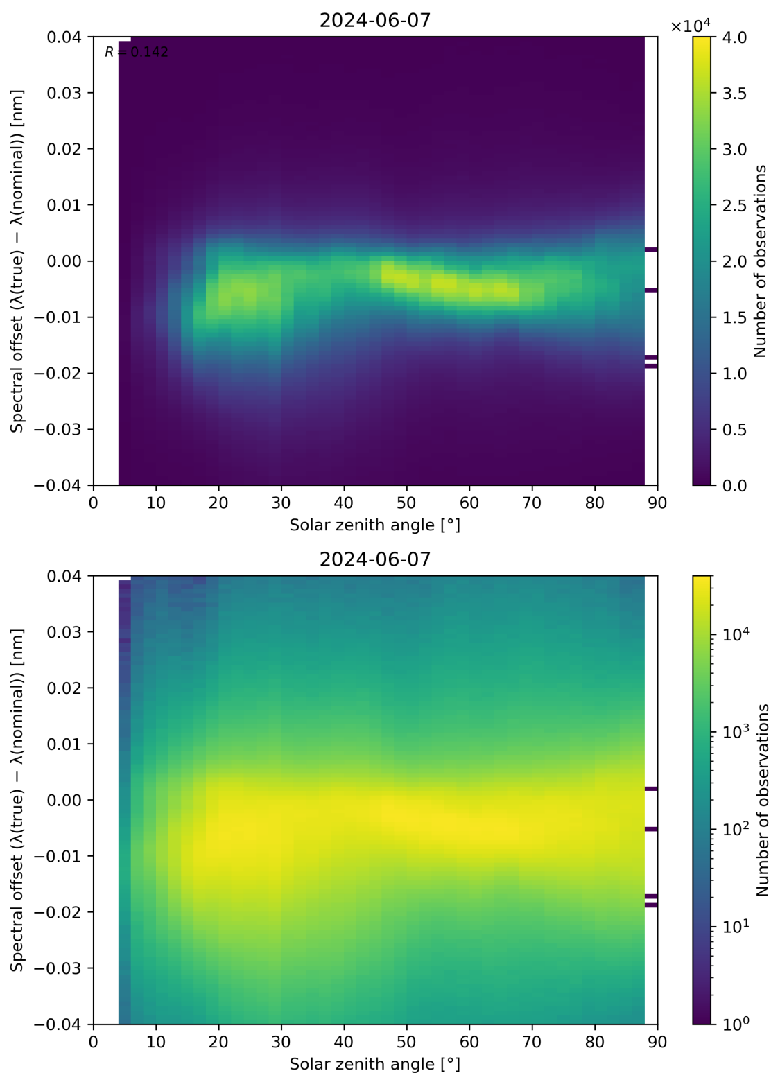
Figure 117: Scatter density plot of “Solar zenith angle” against “Spectral offset ( \lambda(\text{true}) - \lambda(\text{nominal}) )” for 2024-06-06 to 2024-06-08.
