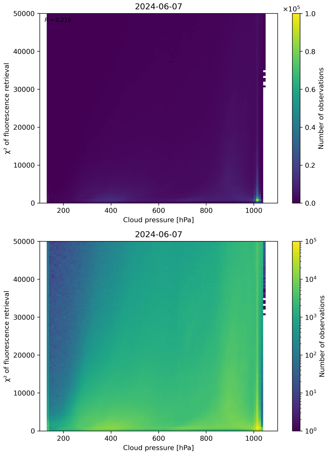
Figure 78: Scatter density plot of “Cloud pressure” against “ \chi^2 of fluorescence retrieval” for 2024-06-06 to 2024-06-08.
