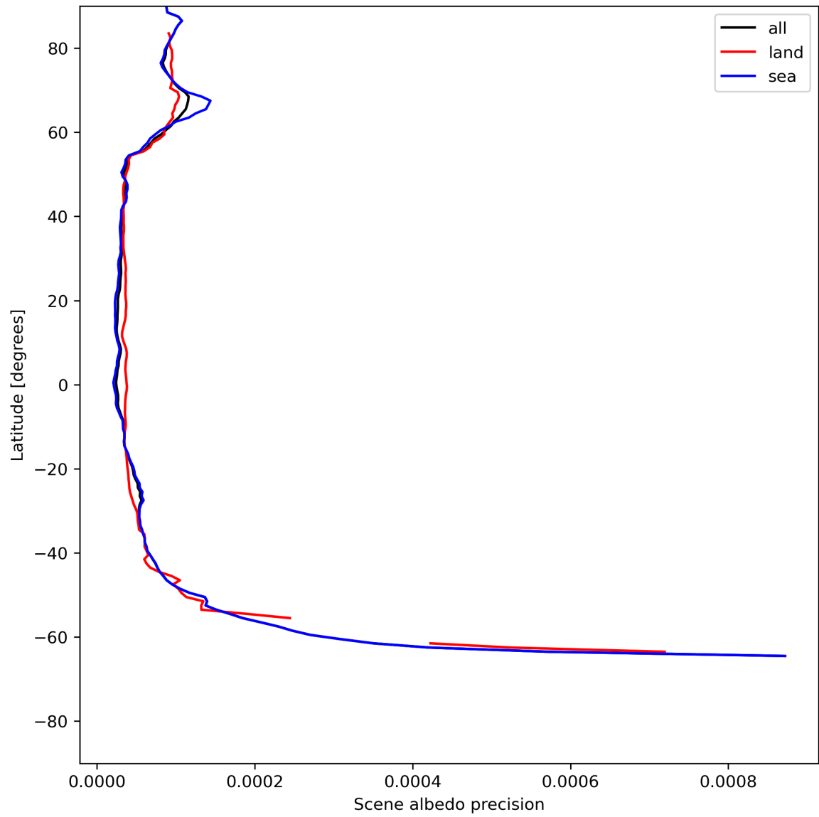
Figure 18: Zonal average of “Scene albedo precision” for 2024-06-06 to 2024-06-08.
