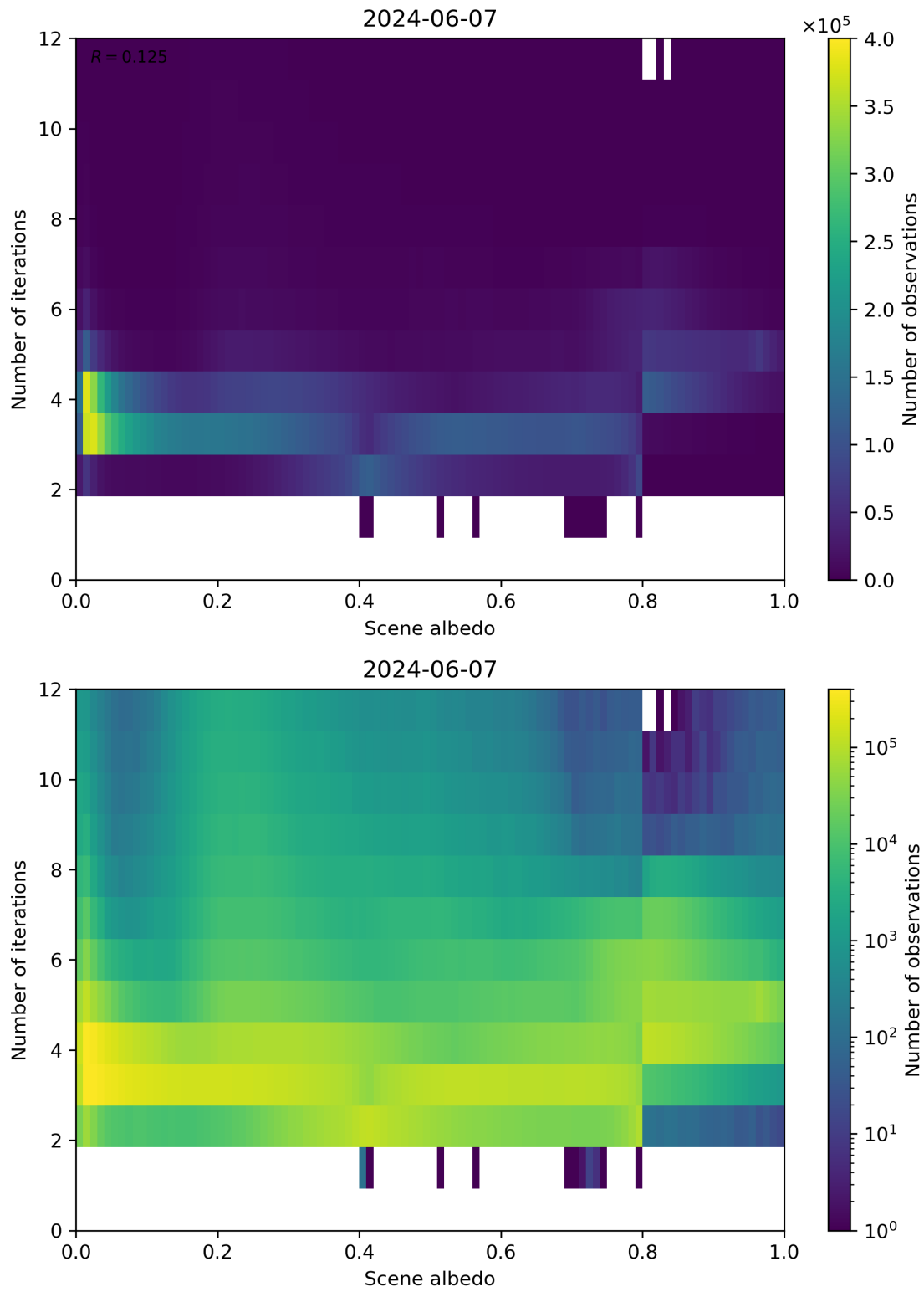
Figure 105: Scatter density plot of “Scene albedo” against “Number of iterations” for 2024-06-06 to 2024-06-08.
