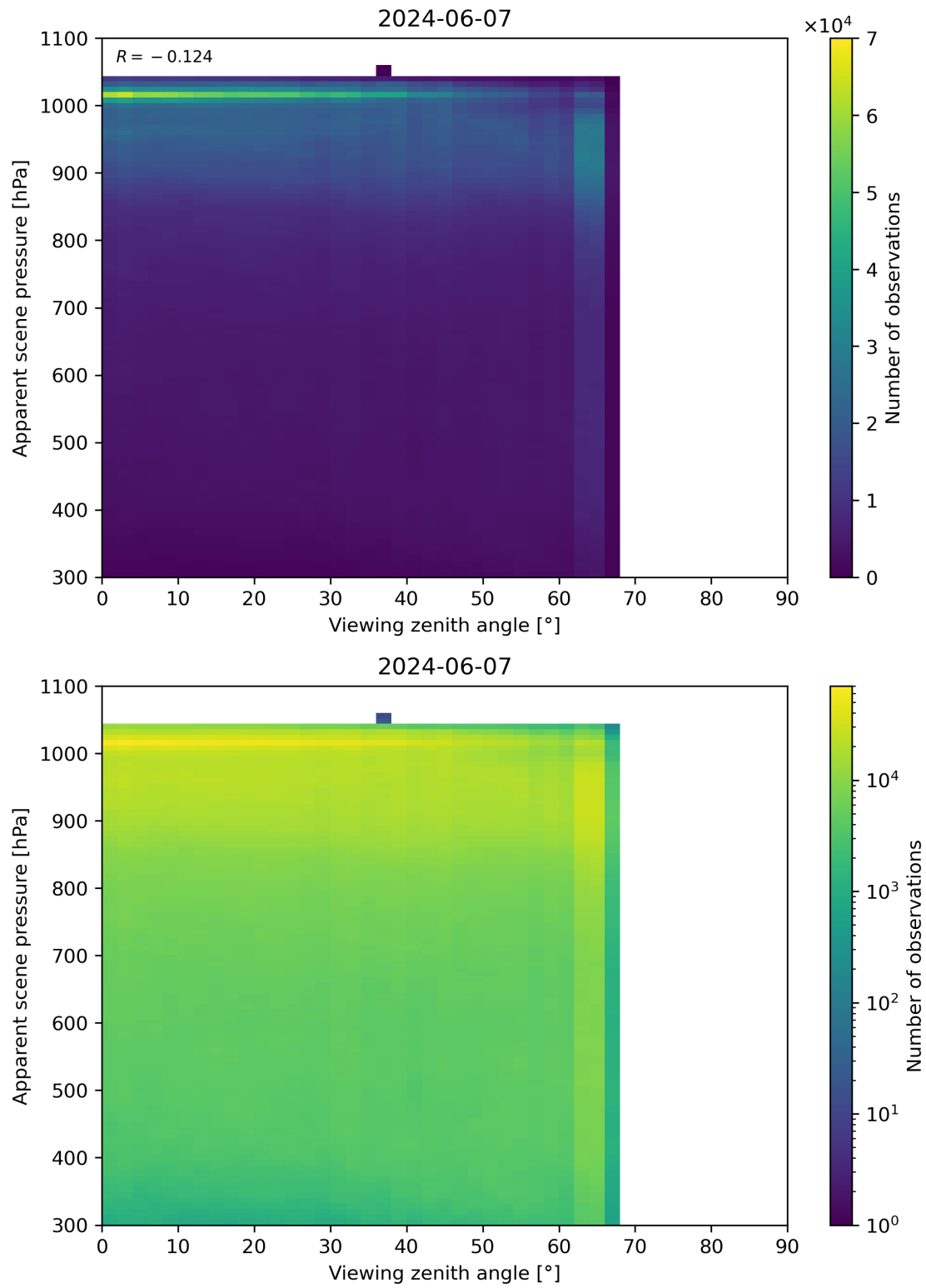
Figure 118: Scatter density plot of “Viewing zenith angle” against “Apparent scene pressure” for 2024-06-06 to 2024-06-08.
