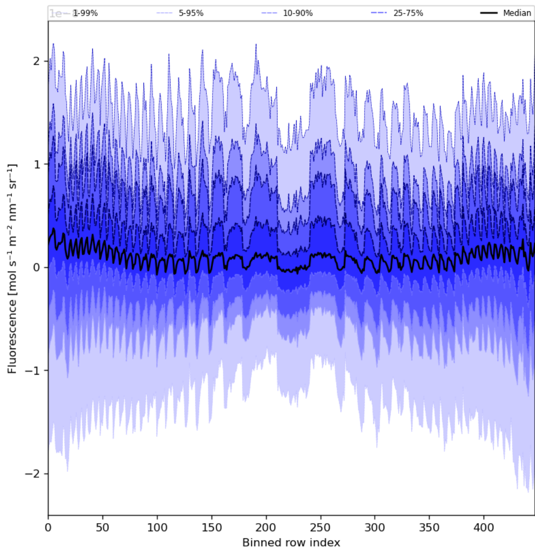
Figure 57: Along track statistics of “Fluorescence” for 2024-06-06 to 2024-06-08
