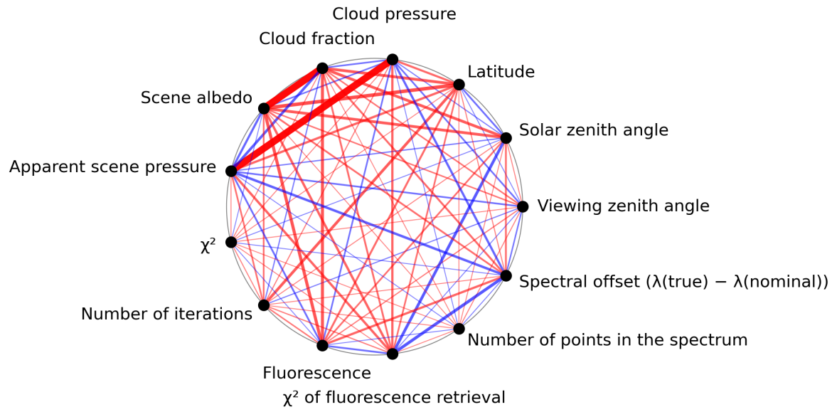
Figure 1: Map of correlation graph for 2024-06-06 to 2024-06-08.
