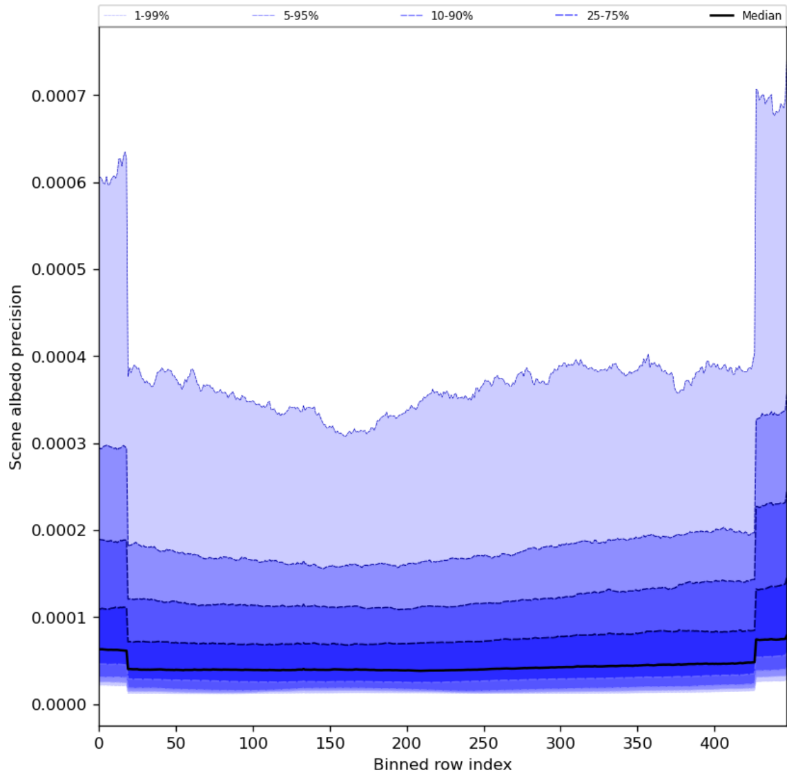
Figure 52: Along track statistics of “Scene albedo precision” for 2024-06-06 to 2024-06-08
