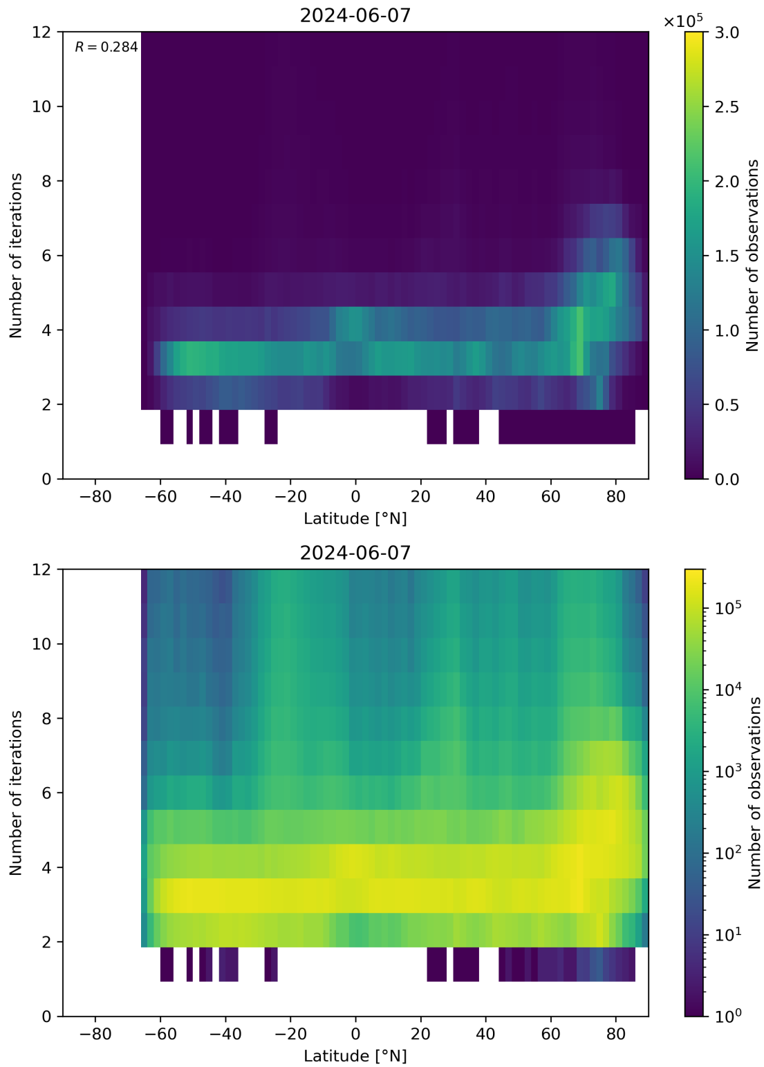
Figure 93: Scatter density plot of “Latitude” against “Number of iterations” for 2024-06-06 to 2024-06-08.
