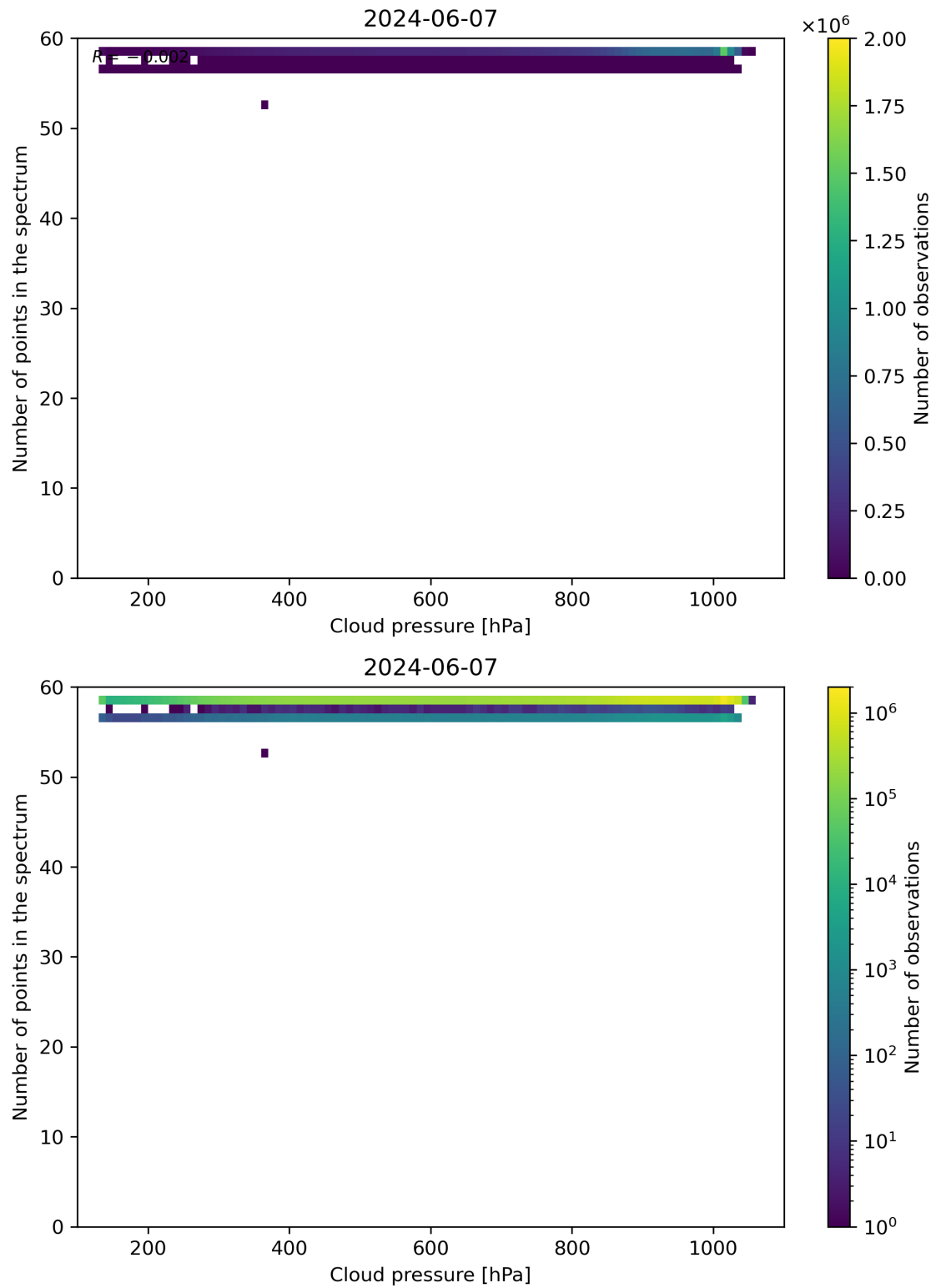
Figure 82: Scatter density plot of “Cloud pressure” against “Number of points in the spectrum” for 2024-06-06 to 2024-06-08.
