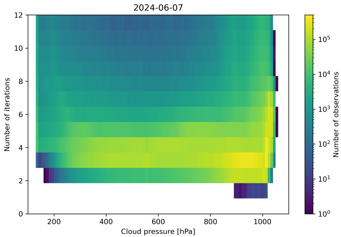
Figure 81: Scatter density plot of “Cloud pressure” against “Number of iterations” for 2024-06-06 to 2024-06-08.
