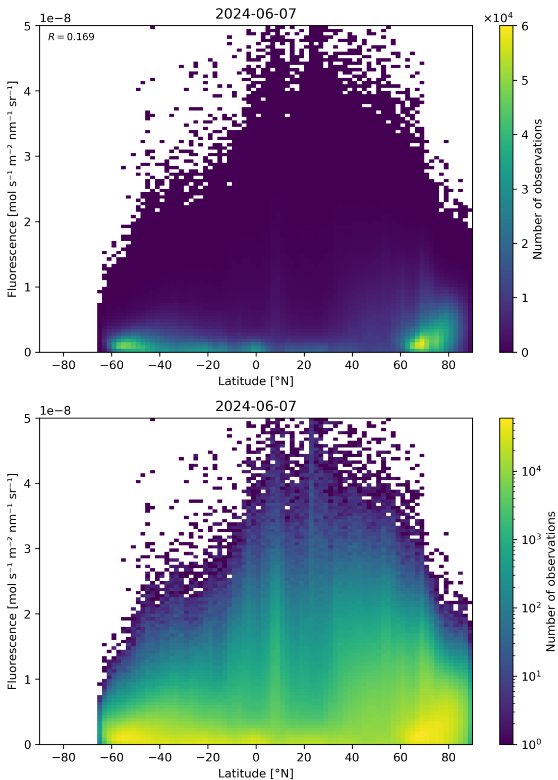
Figure 92: Scatter density plot of “Latitude” against “Fluorescence” for 2024-06-06 to 2024-06-08.
