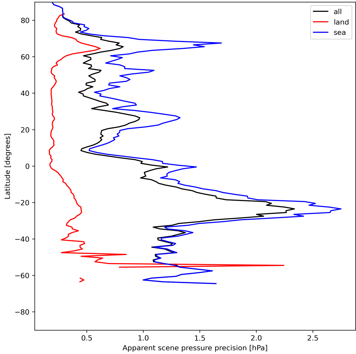
Figure 20: Zonal average of “Apparent scene pressure precision” for 2024-06-06 to 2024-06-08.
