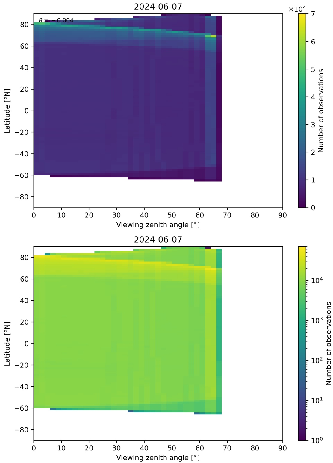
Figure 123: Scatter density plot of “Viewing zenith angle” against “Latitude” for 2024-06-06 to 2024-06-08.
