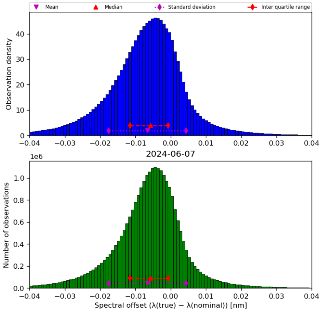
Figure 45: Histogram of “Spectral offset ( \lambda(\text{true}) - \lambda(\text{nominal}) )” for 2024-06-06 to 2024-06-08
