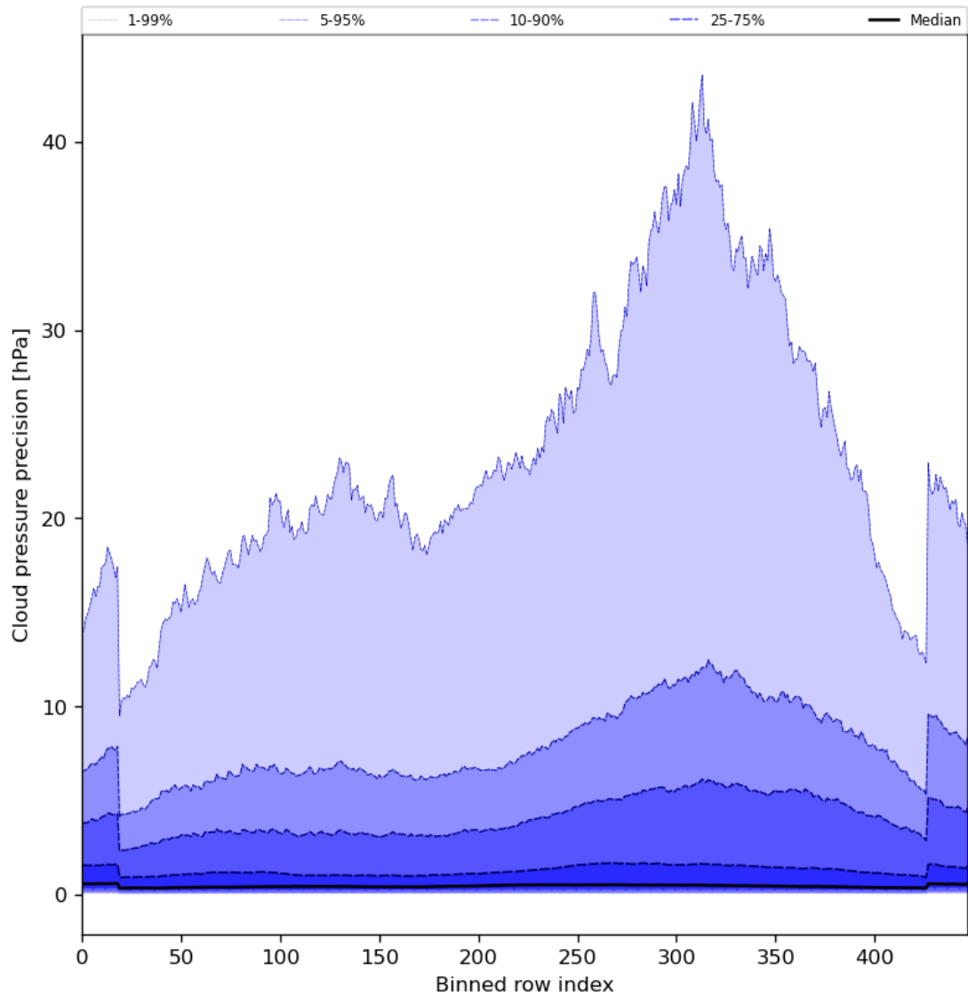
Figure 48: Along track statistics of “Cloud pressure precision” for 2024-06-06 to 2024-06-08
