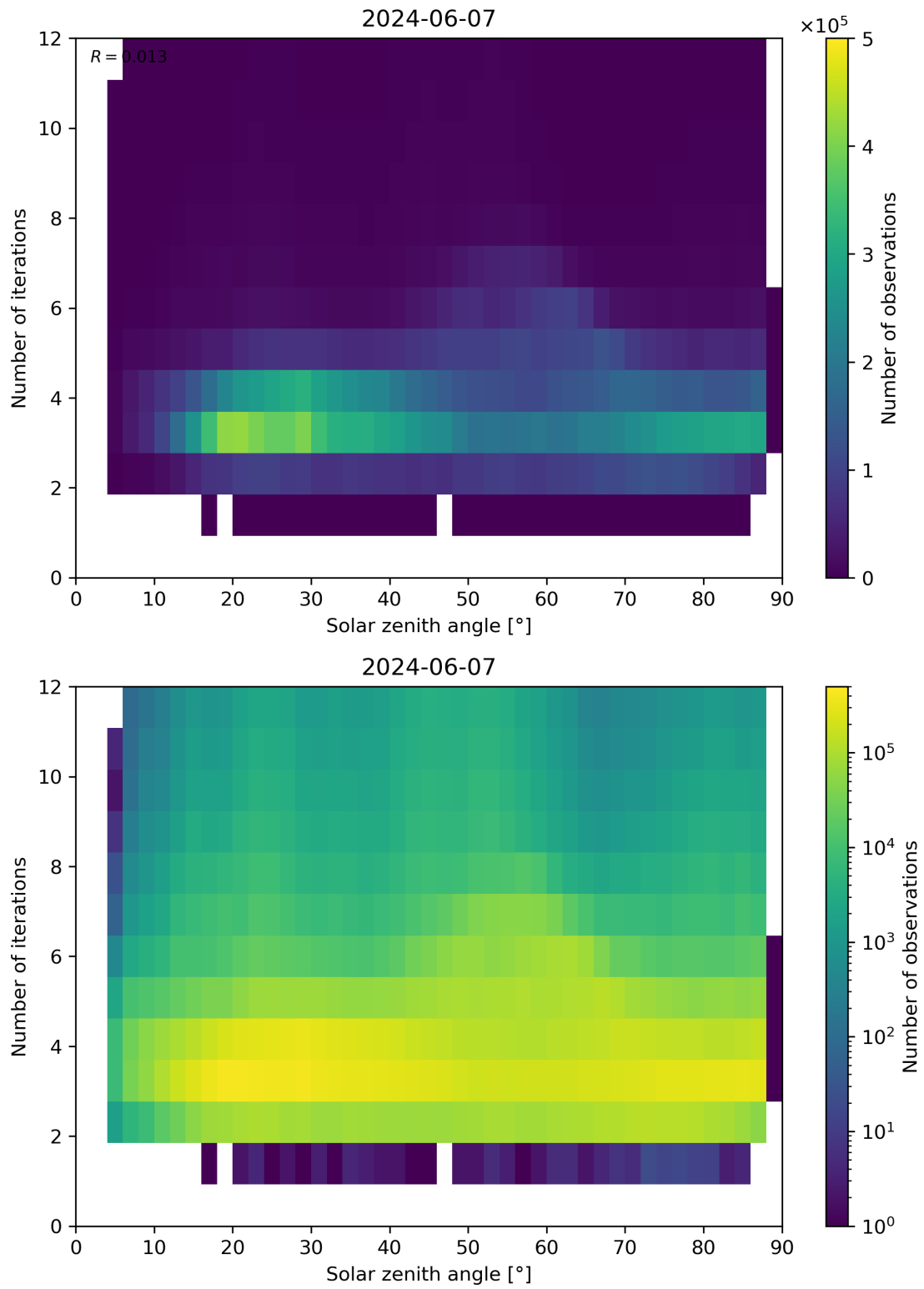
Figure 114: Scatter density plot of “Solar zenith angle” against “Number of iterations” for 2024-06-06 to 2024-06-08.
