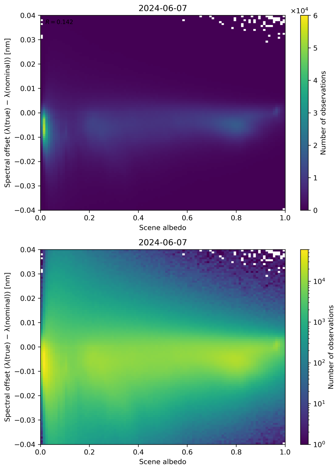
Figure 107: Scatter density plot of “Scene albedo” against “Spectral offset ( \lambda(\text{true}) - \lambda(\text{nominal}) )” for 2024-06-06 to 2024-06-08.
