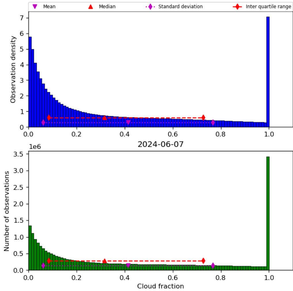
Figure 32: Histogram of “Cloud fraction” for 2024-06-06 to 2024-06-08
