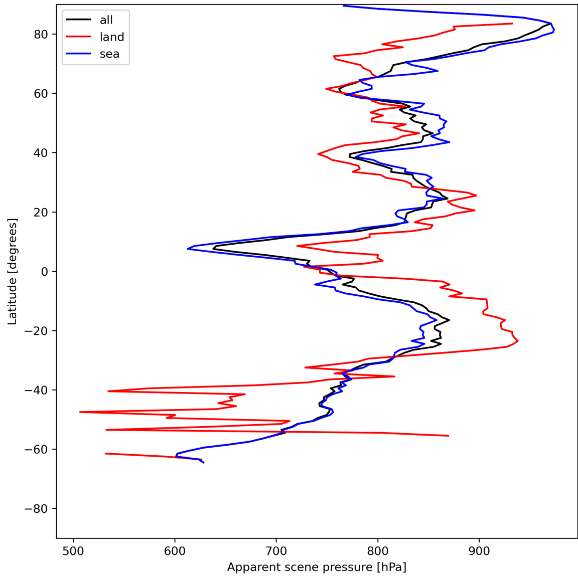
Figure 19: Zonal average of “Apparent scene pressure” for 2024-06-06 to 2024-06-08.
