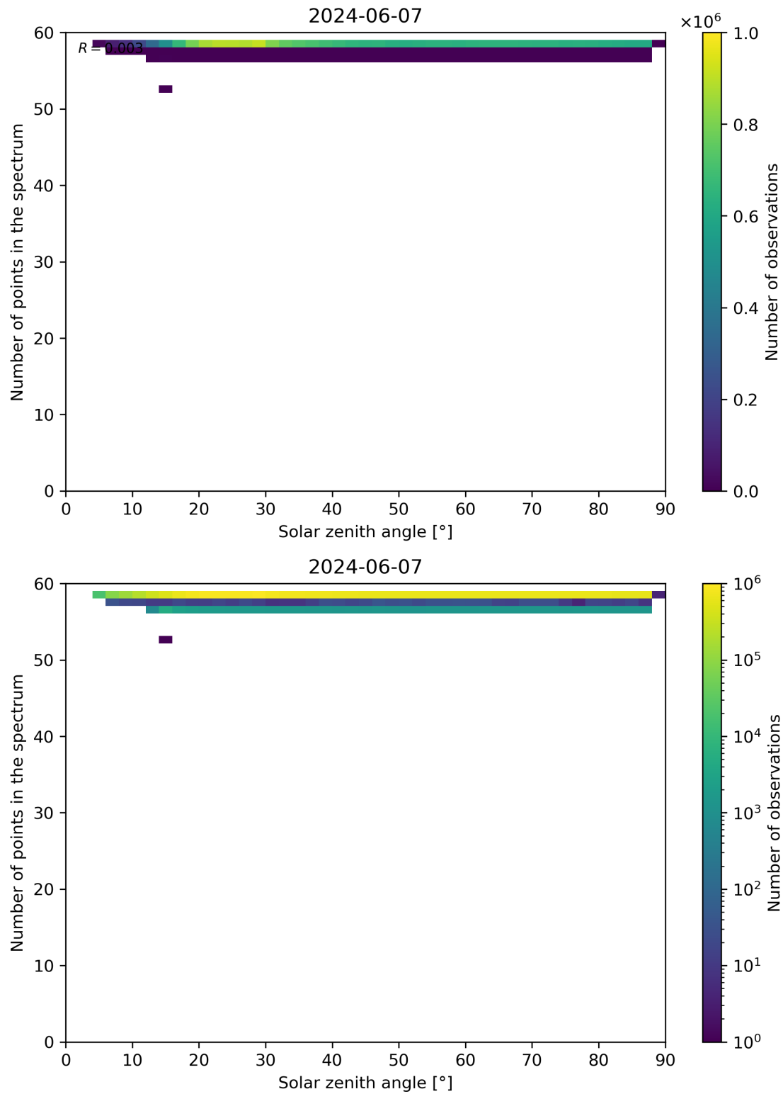
Figure 115: Scatter density plot of “Solar zenith angle” against “Number of points in the spectrum” for 2024-06-06 to 2024-06-08.
