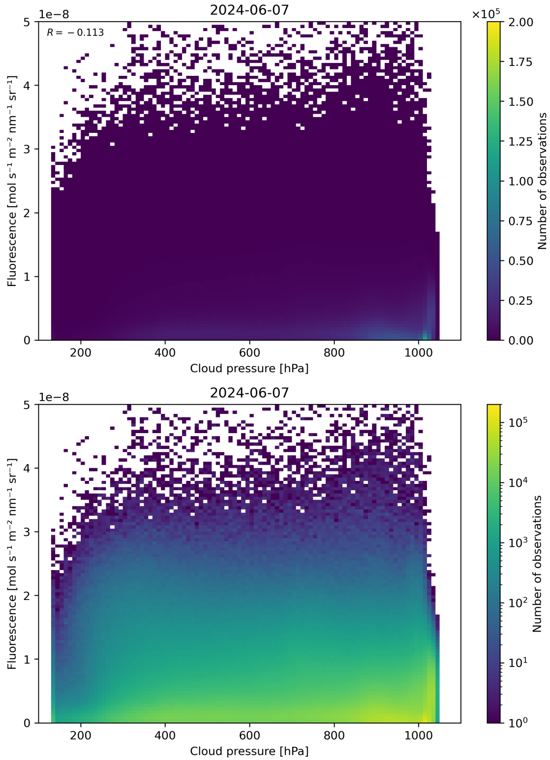
Figure 80: Scatter density plot of “Cloud pressure” against “Fluorescence” for 2024-06-06 to 2024-06-08.
