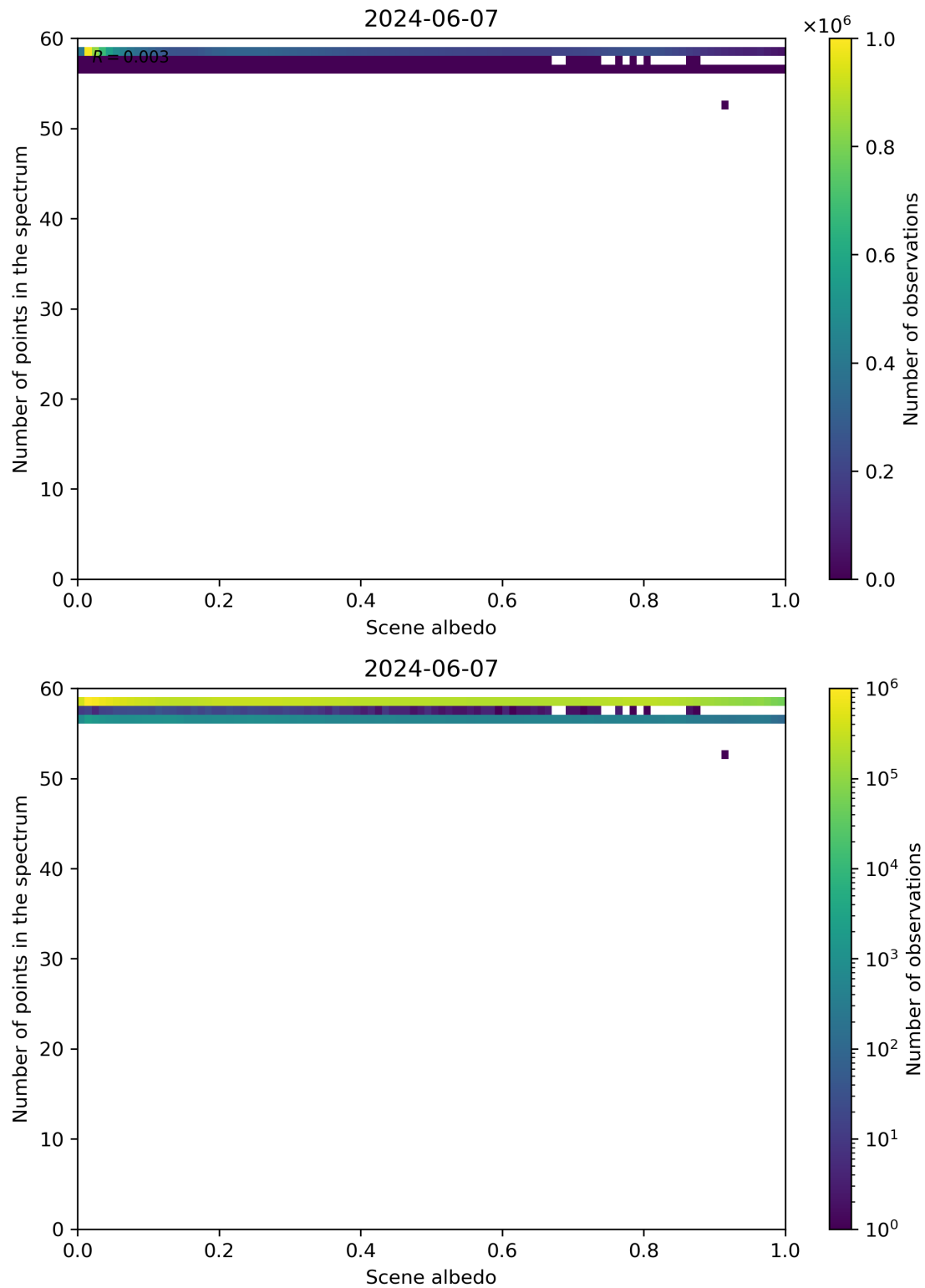
Figure 106: Scatter density plot of “Scene albedo” against “Number of points in the spectrum” for 2024-06-06 to 2024-06-08.
