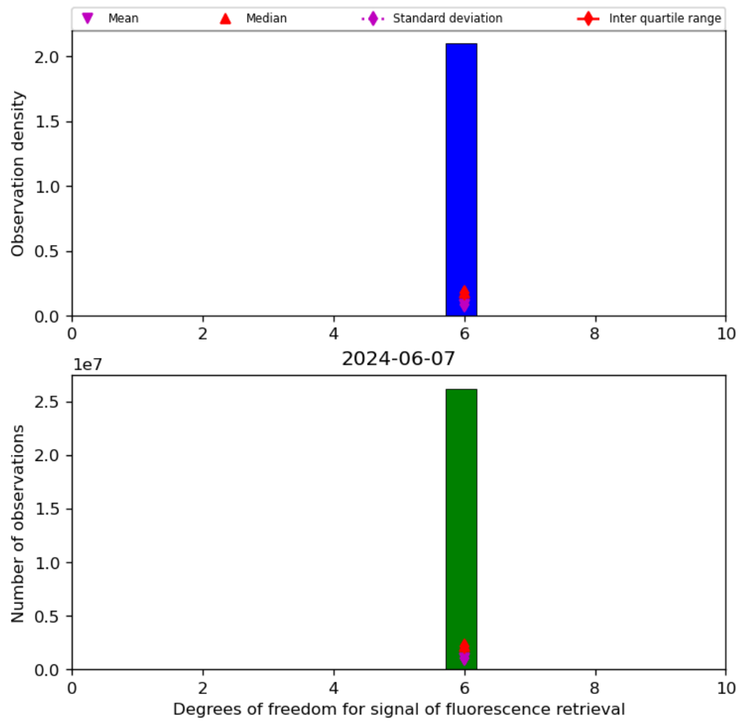
Figure 43: Histogram of “Degrees of freedom for signal of fluorescence retrieval” for 2024-06-06 to 2024-06-08
