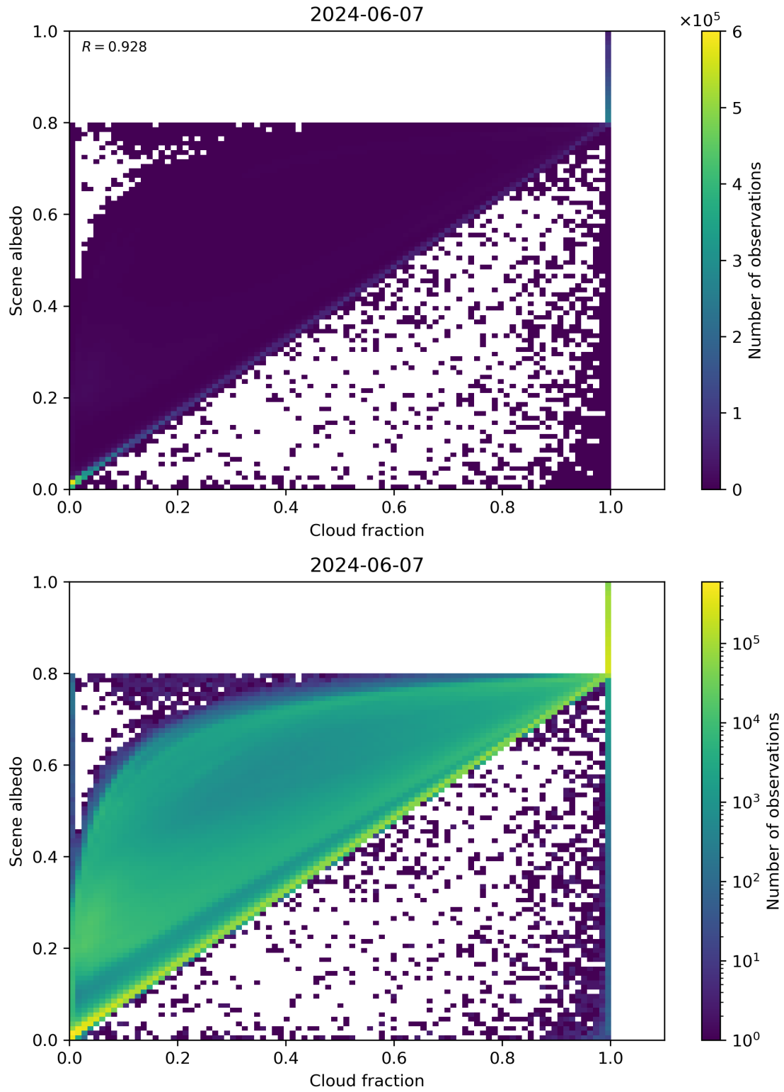
Figure 75: Scatter density plot of “Cloud fraction” against “Scene albedo” for 2024-06-06 to 2024-06-08.
