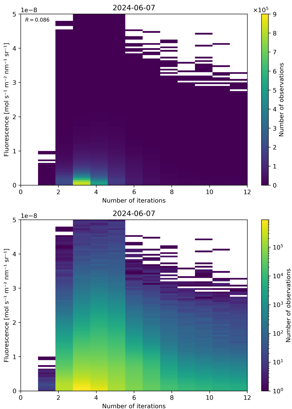
Figure 98: Scatter density plot of “Number of iterations” against “Fluorescence” for 2024-06-06 to 2024-06-08.
