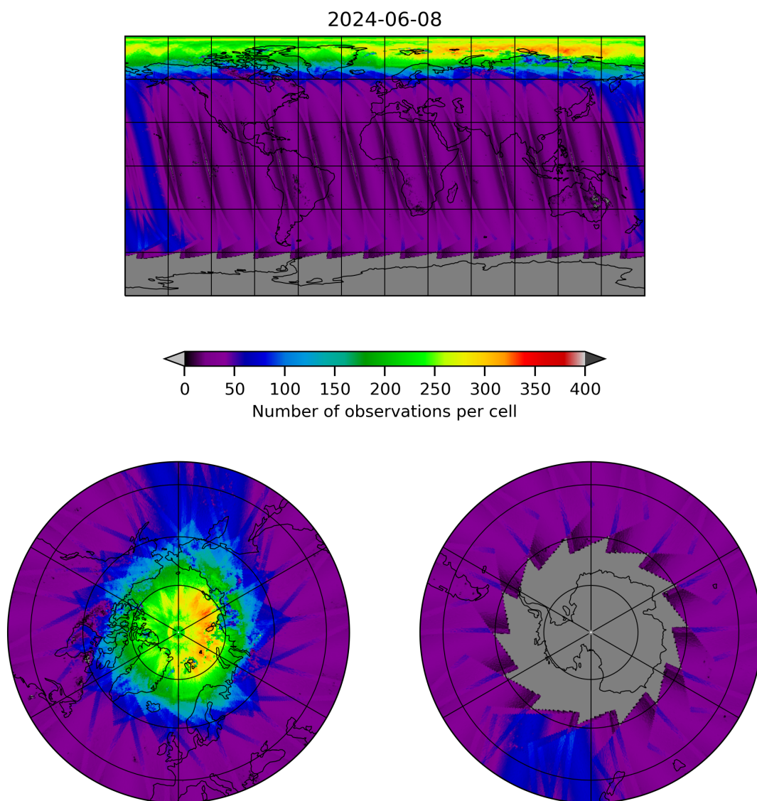
Figure 11: Map of the number of observations for 2024-06-08 to 2024-06-09
