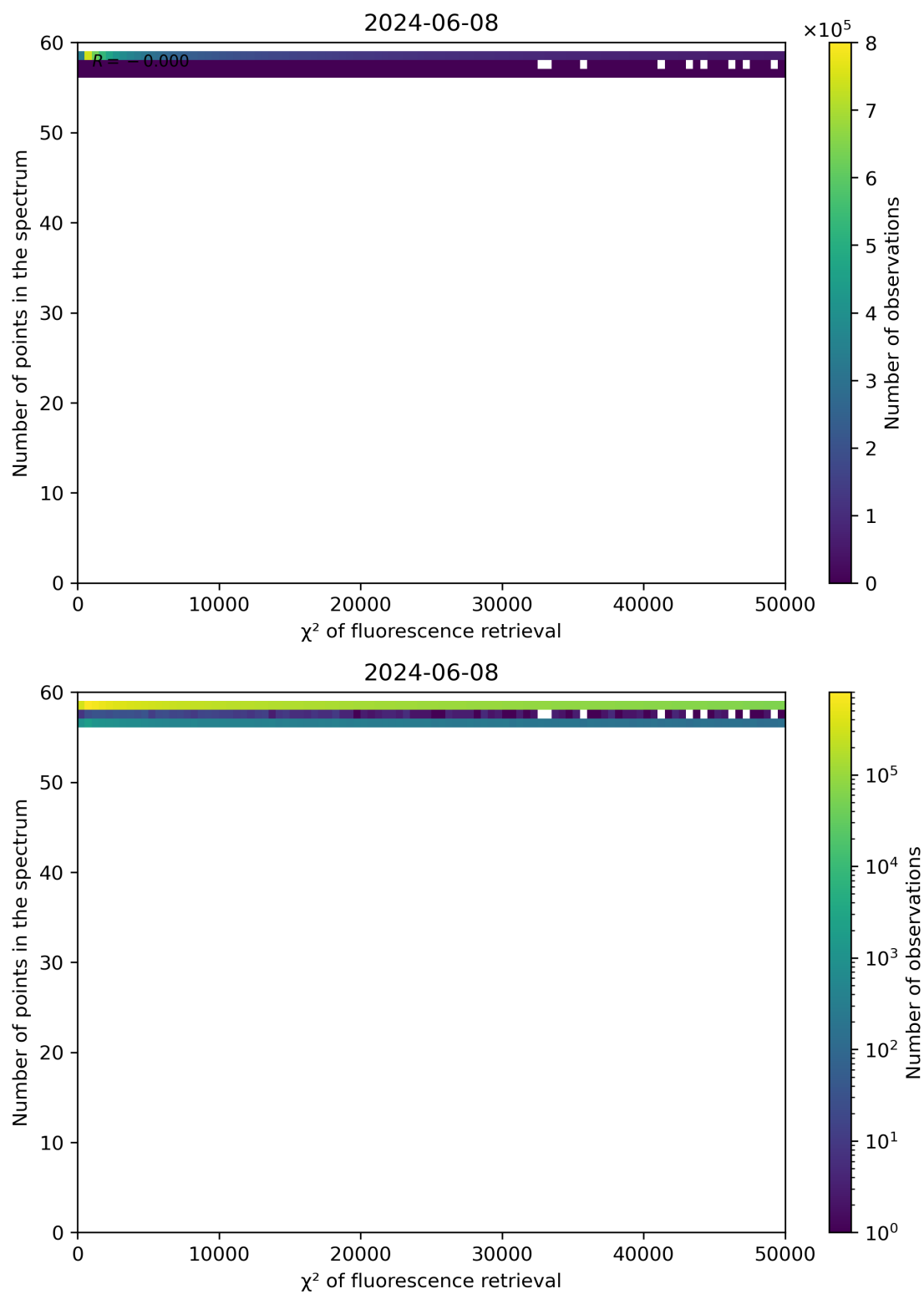
Figure 68: Scatter density plot of " \chi^2 of fluorescence retrieval" against "Number of points in the spectrum" for 2024-06-08 to 2024-06-09.
