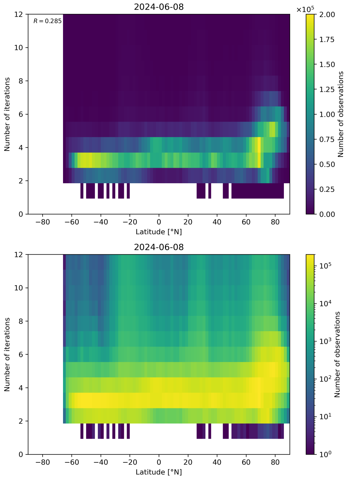
Figure 93: Scatter density plot of “Latitude” against “Number of iterations” for 2024-06-08 to 2024-06-09.
