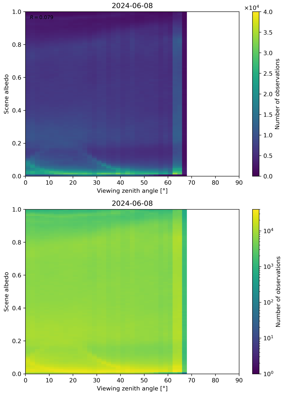
Figure 126: Scatter density plot of “Viewing zenith angle” against “Scene albedo” for 2024-06-08 to 2024-06-09.
