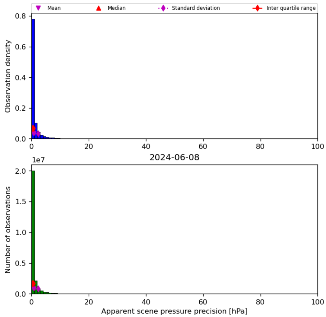
Figure 37: Histogram of “Apparent scene pressure precision” for 2024-06-08 to 2024-06-09
