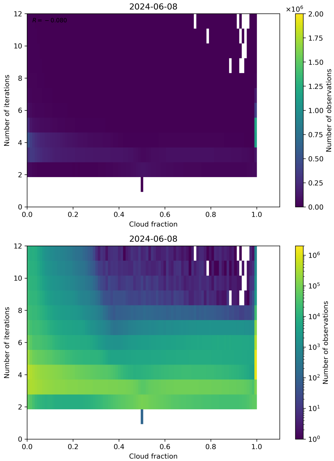
Figure 73: Scatter density plot of “Cloud fraction” against “Number of iterations” for 2024-06-08 to 2024-06-09.
