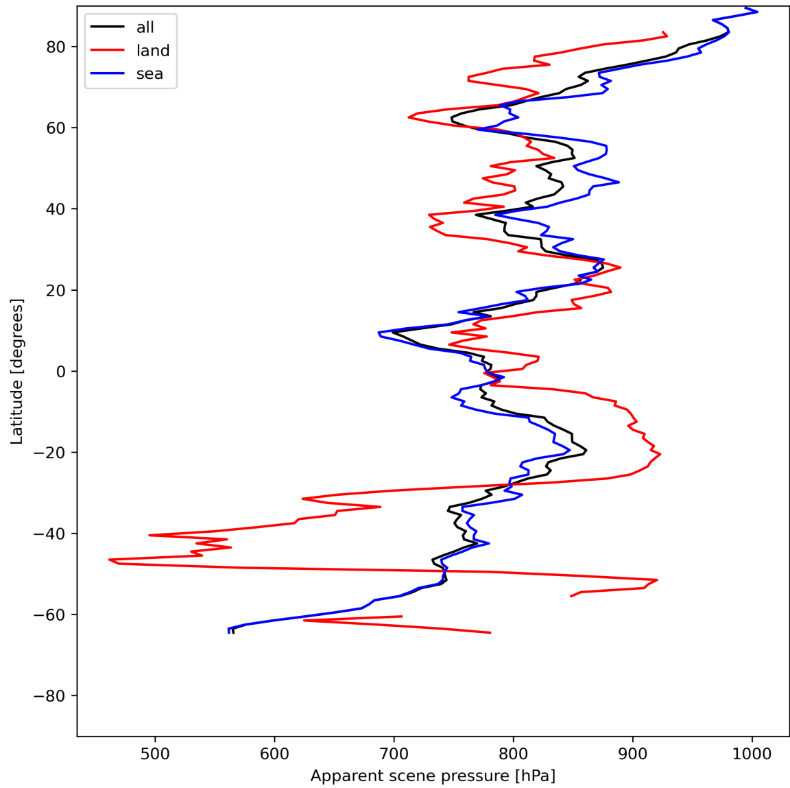
Figure 19: Zonal average of “Apparent scene pressure” for 2024-06-08 to 2024-06-09.
