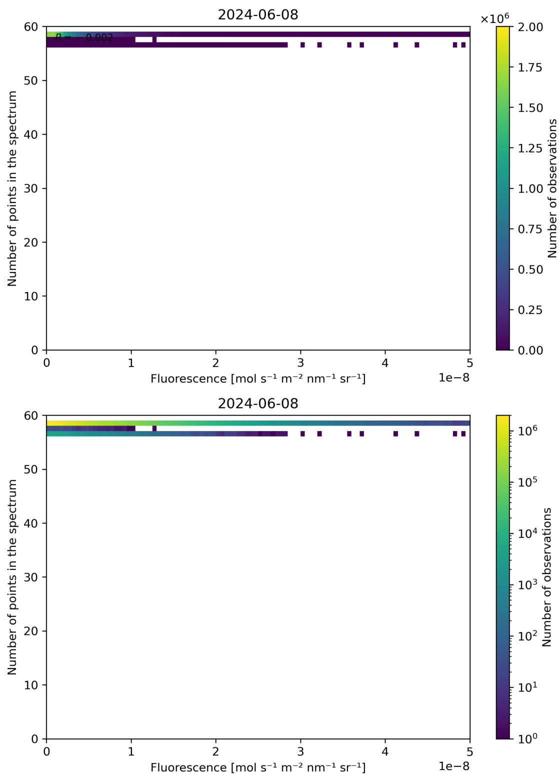
Figure 86: Scatter density plot of “Fluorescence” against “Number of points in the spectrum” for 2024-06-08 to 2024-06-09.
