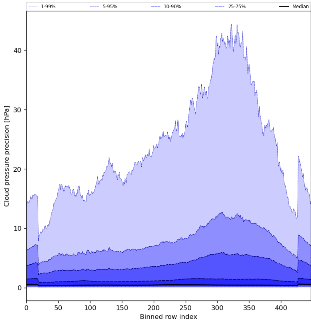
Figure 48: Along track statistics of “Cloud pressure precision” for 2024-06-08 to 2024-06-09
