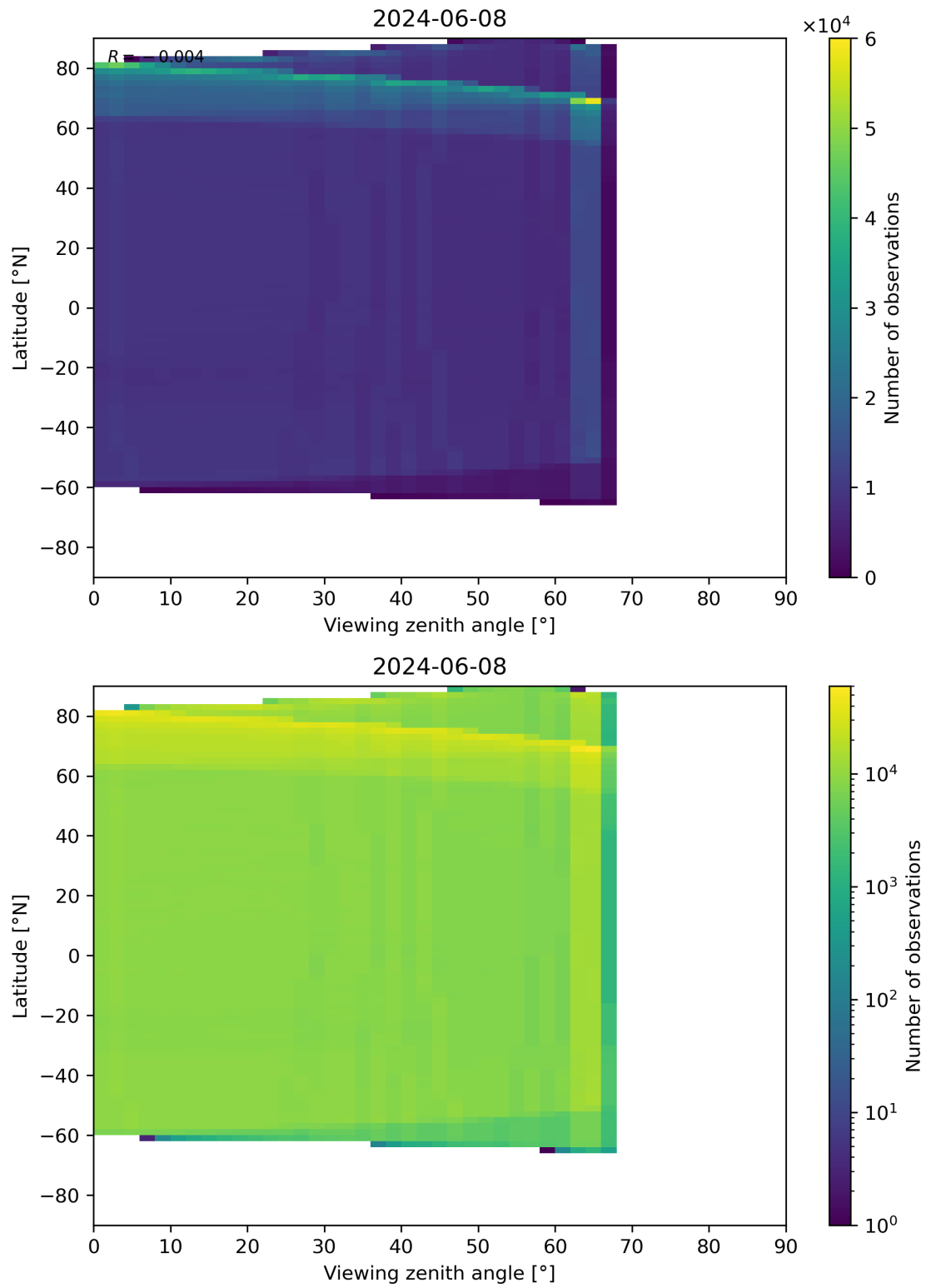
Figure 123: Scatter density plot of “Viewing zenith angle” against “Latitude” for 2024-06-08 to 2024-06-09.
