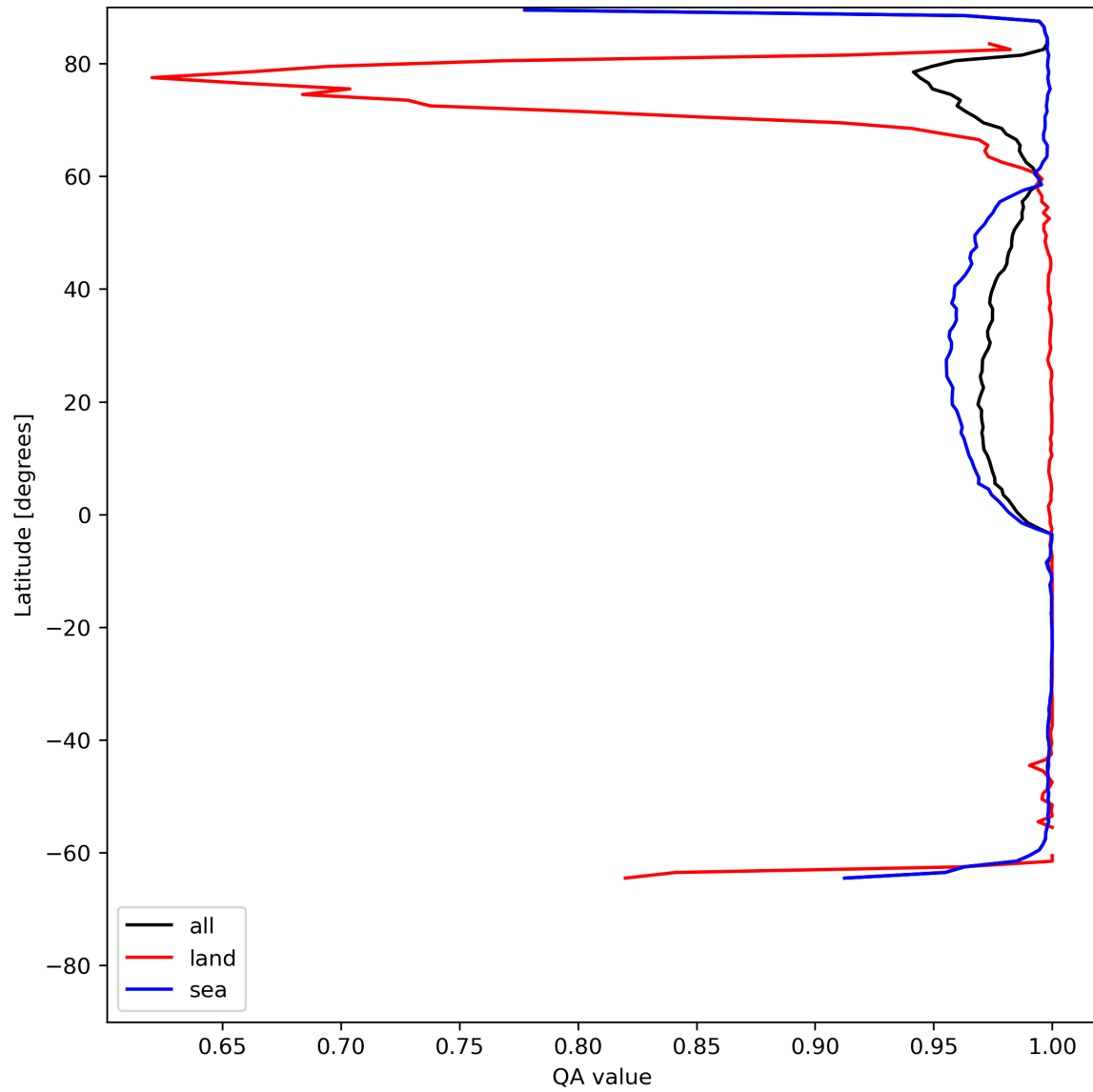
Figure 12: Zonal average of “QA value” for 2024-06-08 to 2024-06-09.
