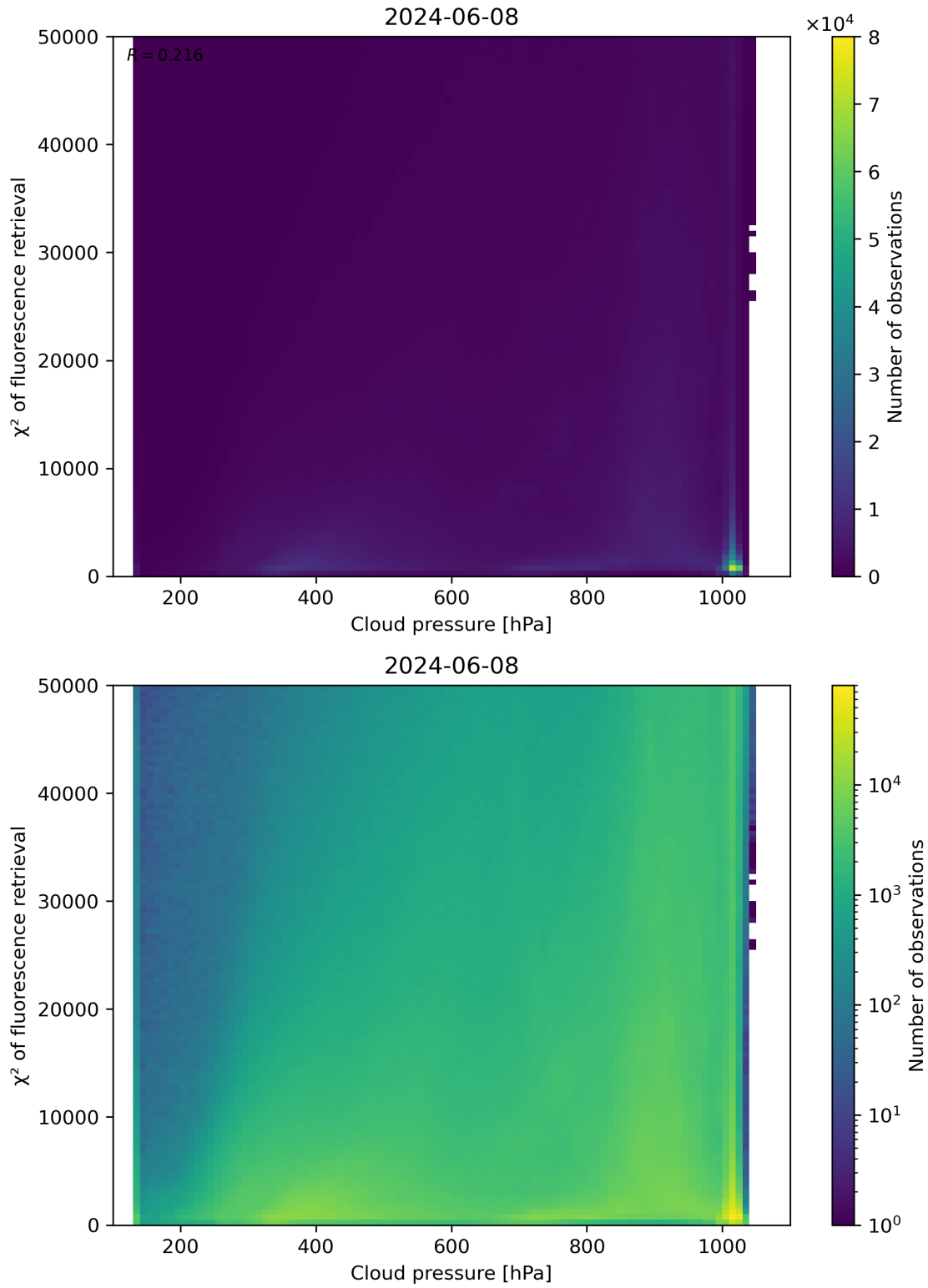
Figure 78: Scatter density plot of “Cloud pressure” against “ \chi^2 of fluorescence retrieval” for 2024-06-08 to 2024-06-09.
