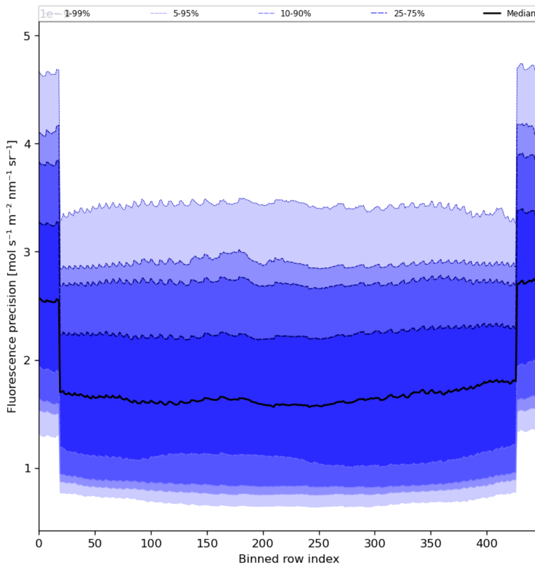
Figure 58: Along track statistics of “Fluorescence precision” for 2024-06-08 to 2024-06-09
