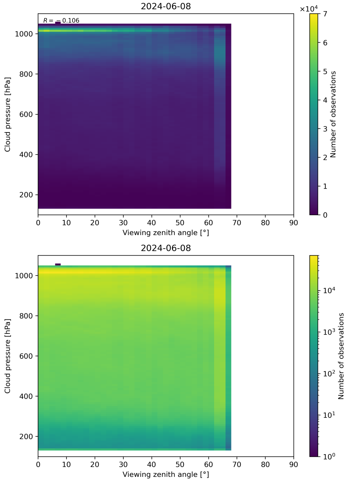
Figure 121: Scatter density plot of “Viewing zenith angle” against “Cloud pressure” for 2024-06-08 to 2024-06-09.
