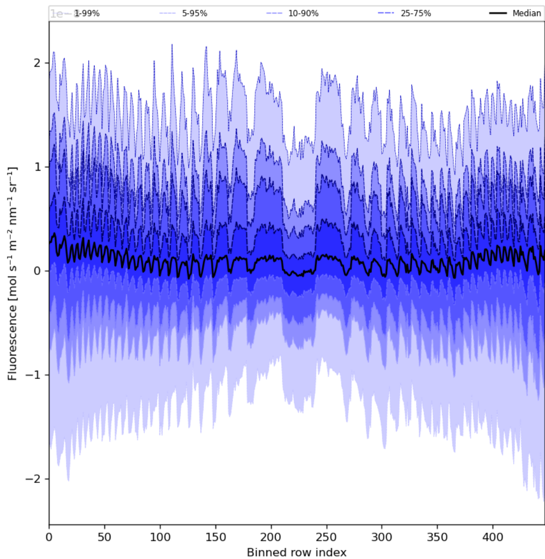
Figure 57: Along track statistics of “Fluorescence” for 2024-06-08 to 2024-06-09
