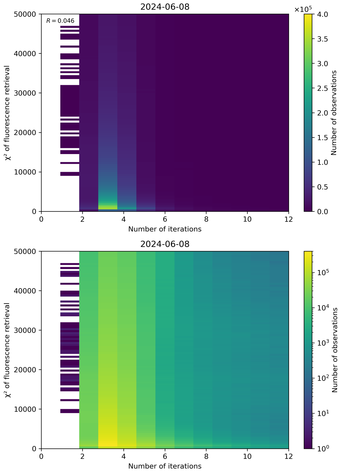
Figure 97: Scatter density plot of “Number of iterations” against “ \chi^2 of fluorescence retrieval” for 2024-06-08 to 2024-06-09.
