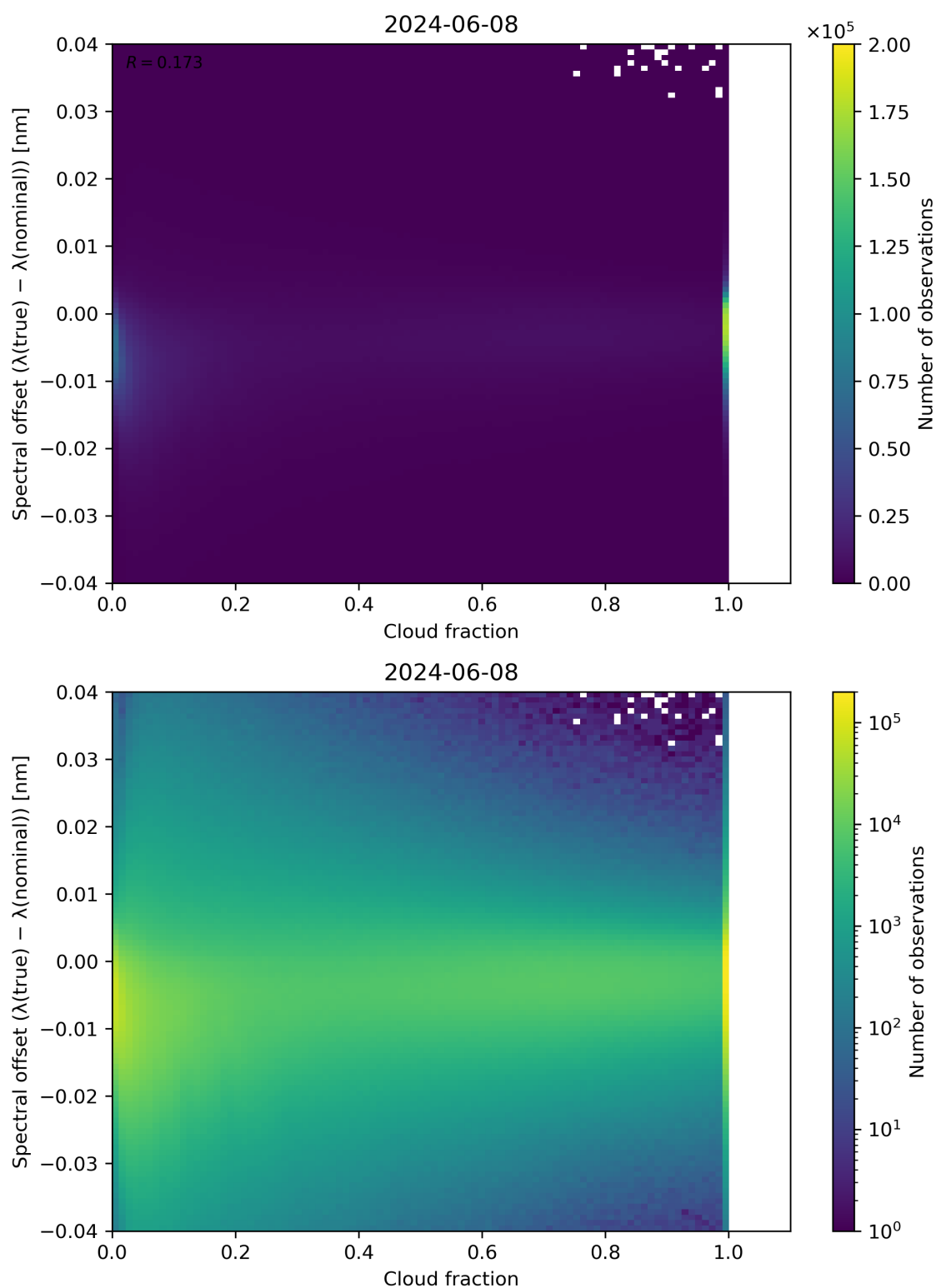
Figure 76: Scatter density plot of “Cloud fraction” against “Spectral offset ( \lambda(\text{true}) - \lambda(\text{nominal}) )” for 2024-06-08 to 2024-06-09.
