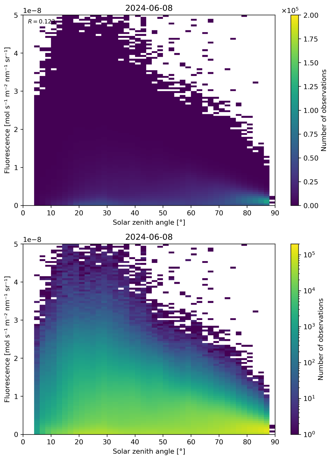
Figure 112: Scatter density plot of “Solar zenith angle” against “Fluorescence” for 2024-06-08 to 2024-06-09.
