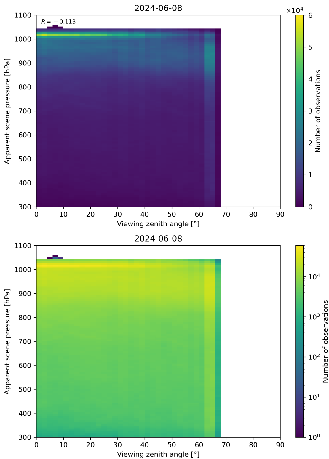
Figure 118: Scatter density plot of “Viewing zenith angle” against “Apparent scene pressure” for 2024-06-08 to 2024-06-09.
