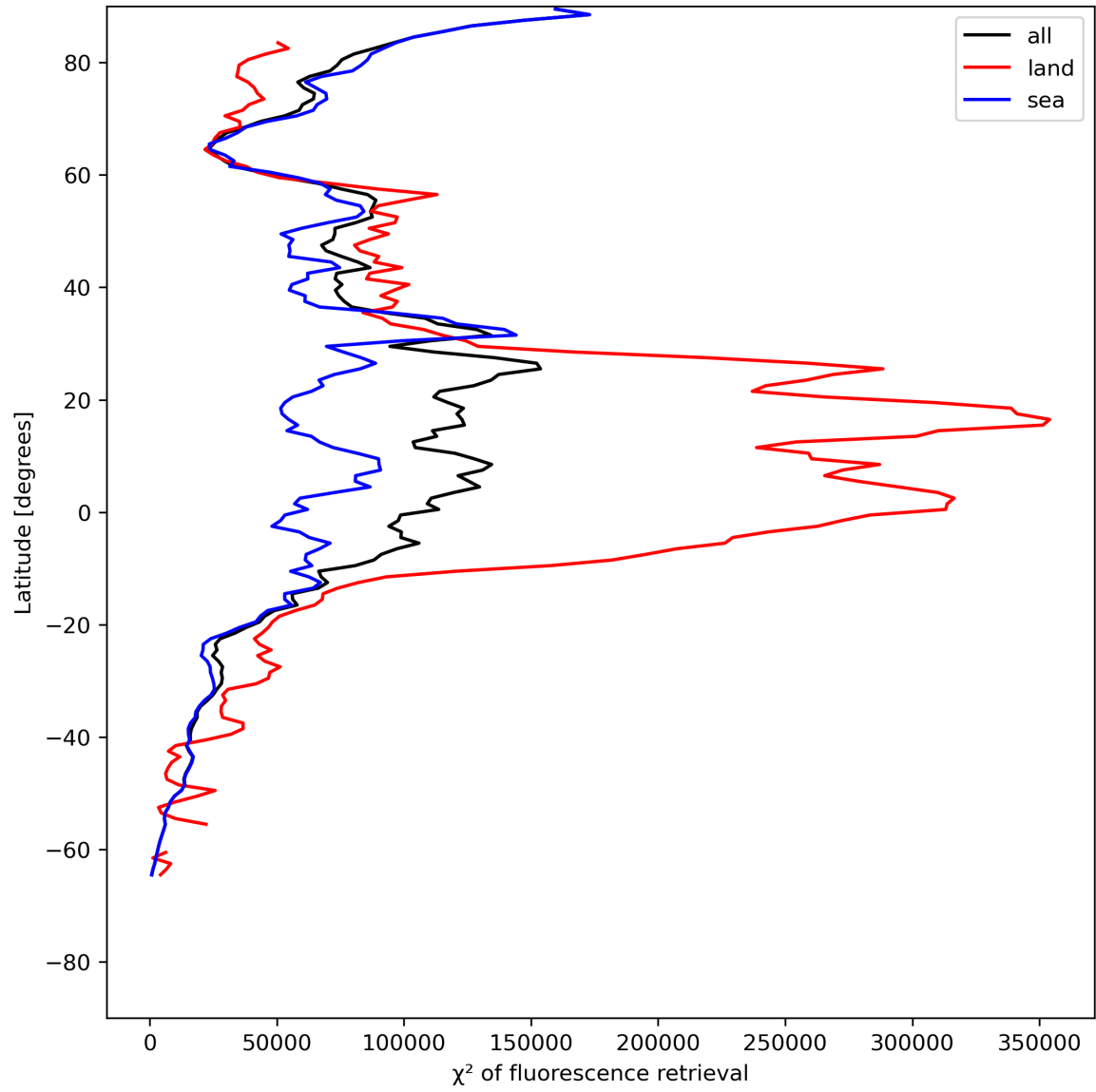
Figure 25: Zonal average of “ \chi^2 of fluorescence retrieval” for 2024-06-08 to 2024-06-09.
