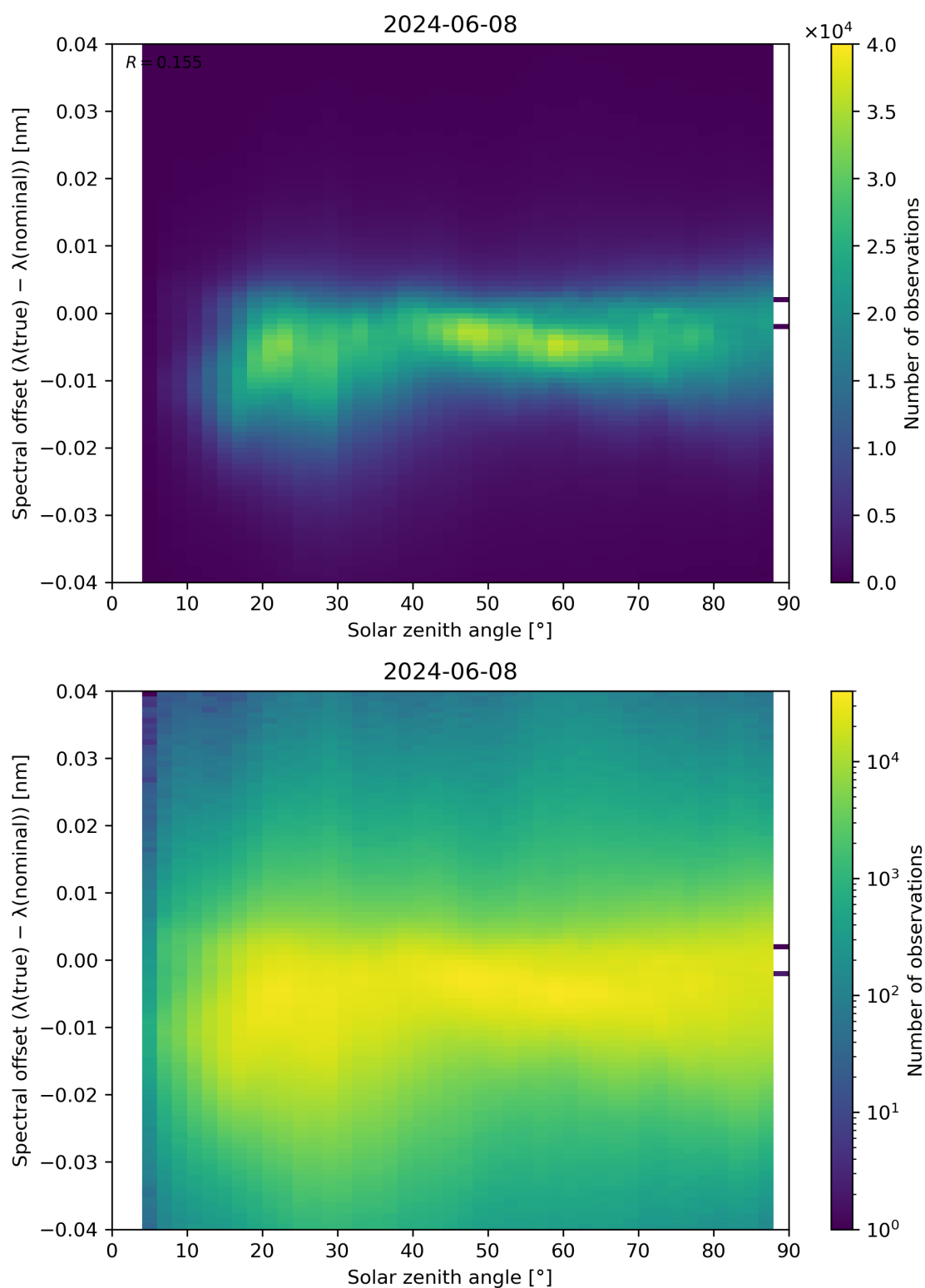
Figure 117: Scatter density plot of “Solar zenith angle” against “Spectral offset ( \lambda(\text{true}) - \lambda(\text{nominal}) )” for 2024-06-08 to 2024-06-09.
