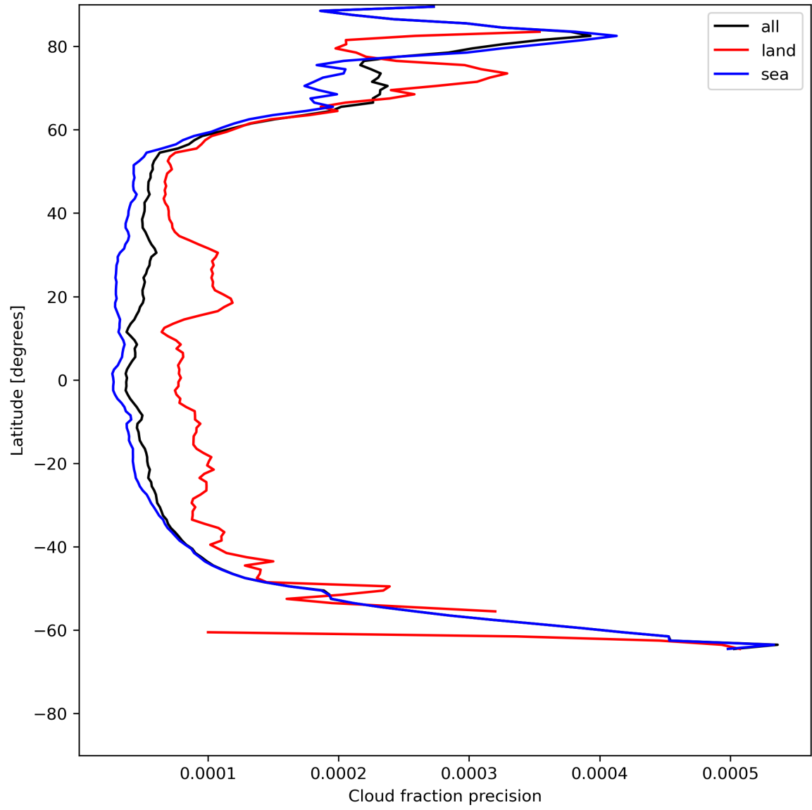
Figure 16: Zonal average of “Cloud fraction precision” for 2024-06-08 to 2024-06-09.
