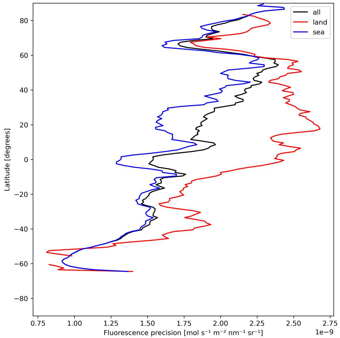
Figure 24: Zonal average of “Fluorescence precision” for 2024-06-08 to 2024-06-09.
