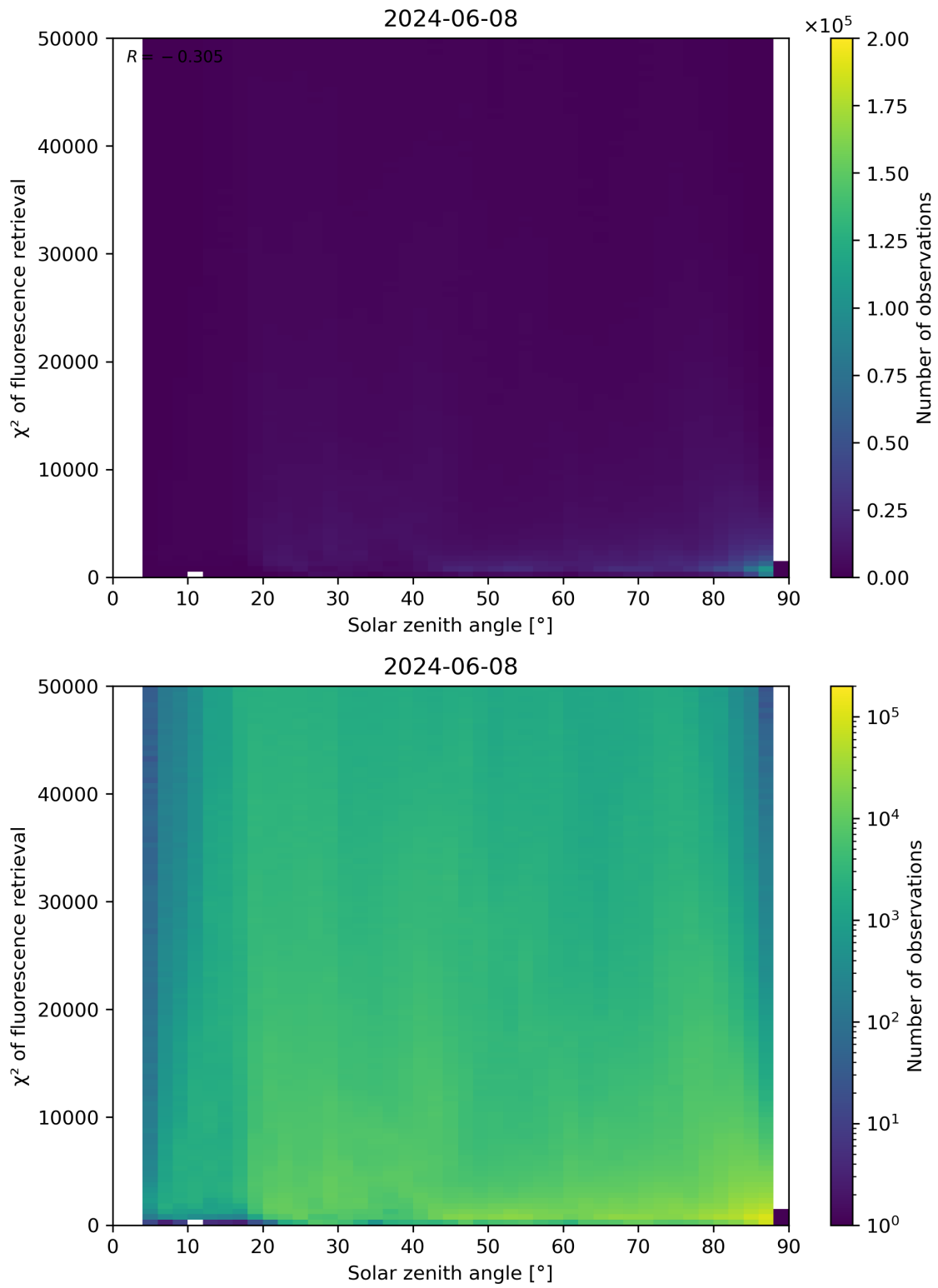
Figure 109: Scatter density plot of “Solar zenith angle” against “ \chi^2 of fluorescence retrieval” for 2024-06-08 to 2024-06-09.
