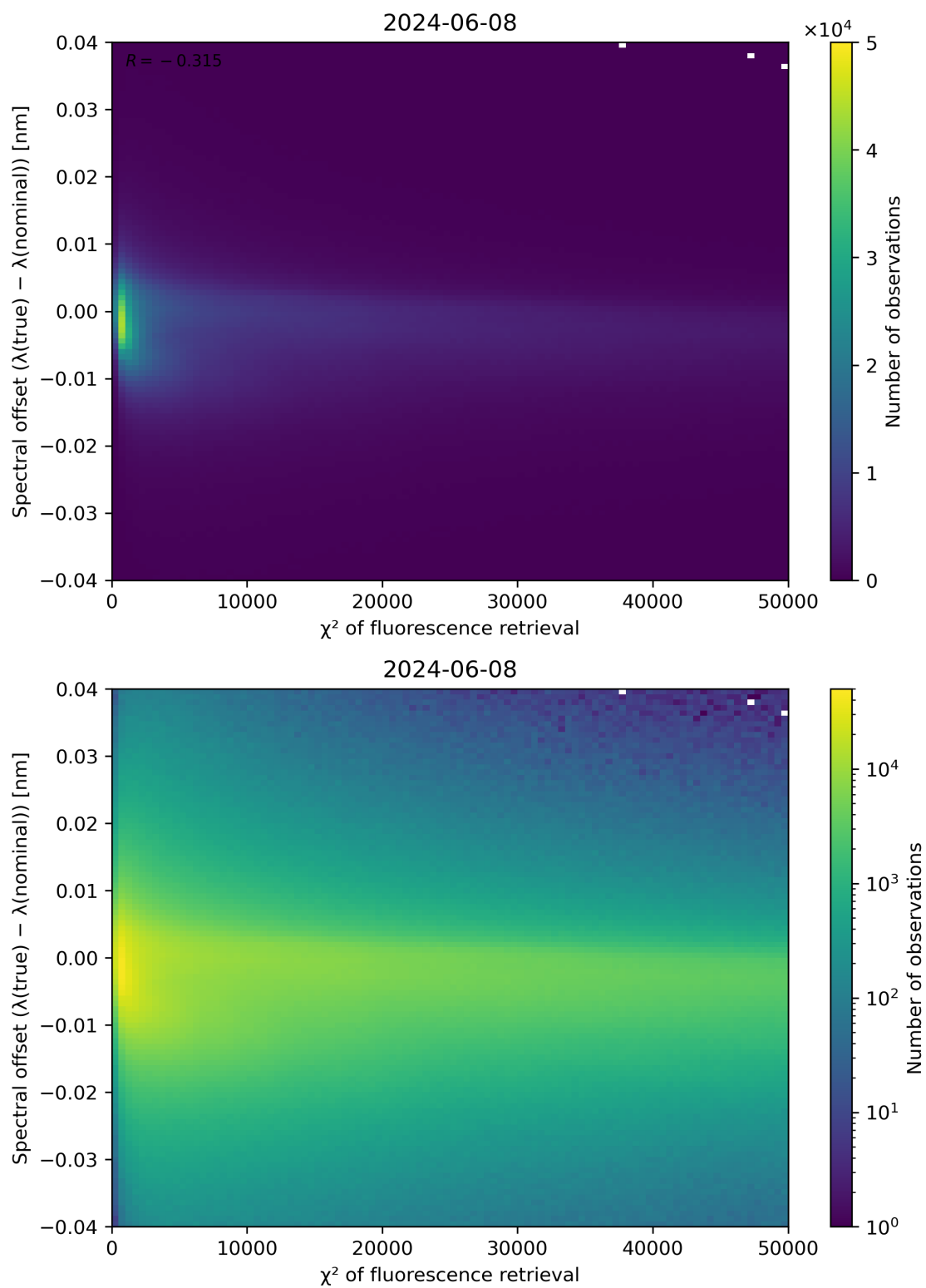
Figure 69: Scatter density plot of " \chi^2 of fluorescence retrieval" against "Spectral offset ( \lambda(\text{true}) - \lambda(\text{nominal})) " for 2024-06-08 to 2024-06-09.
