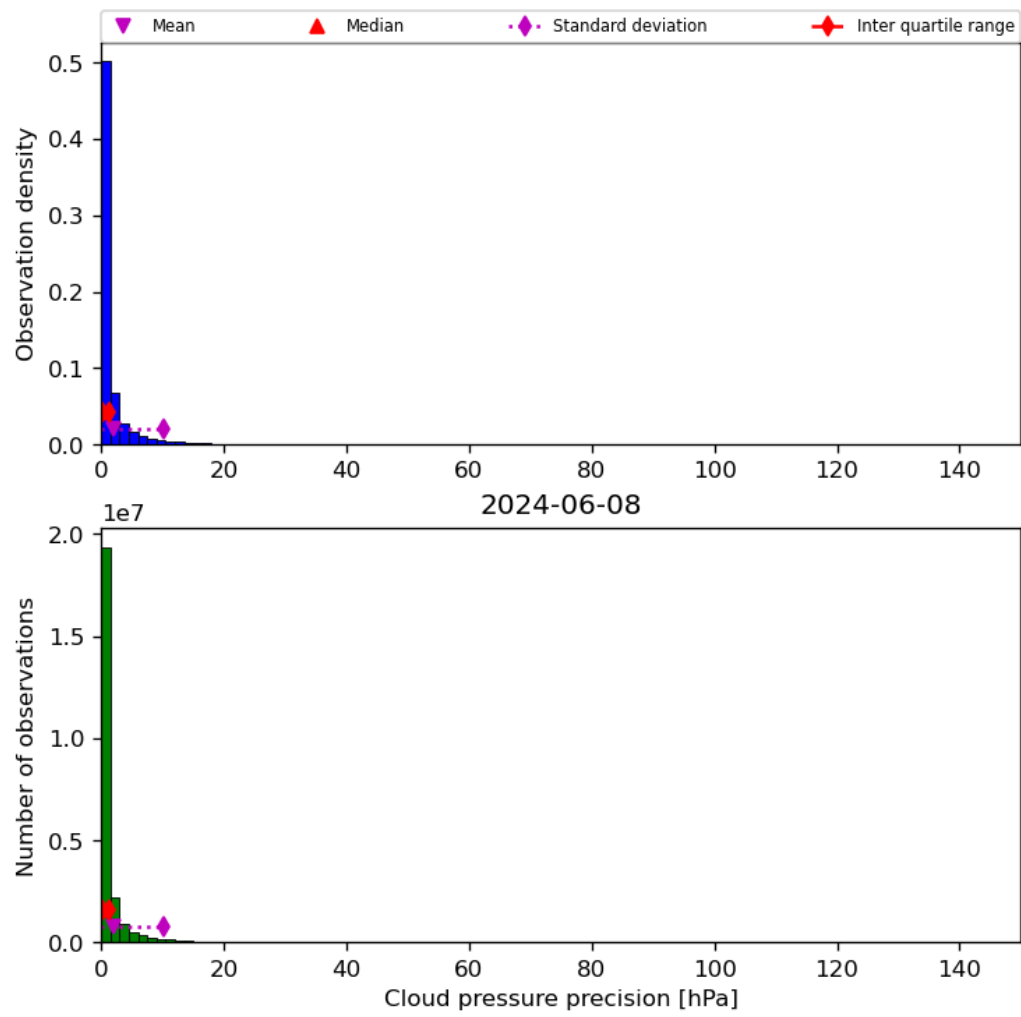
Figure 31: Histogram of “Cloud pressure precision” for 2024-06-08 to 2024-06-09
