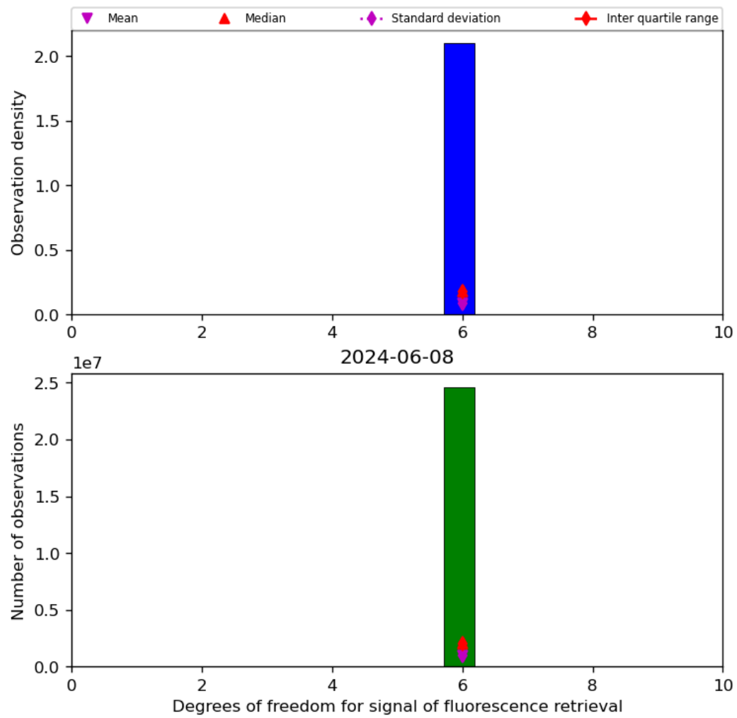
Figure 43: Histogram of “Degrees of freedom for signal of fluorescence retrieval” for 2024-06-08 to 2024-06-09
