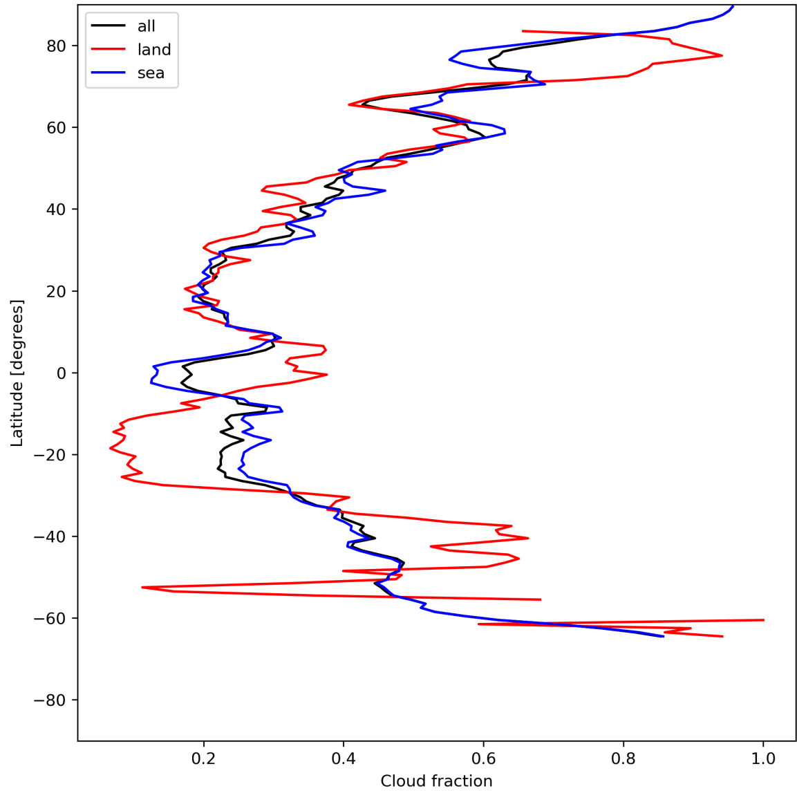
Figure 15: Zonal average of “Cloud fraction” for 2024-06-08 to 2024-06-09.
