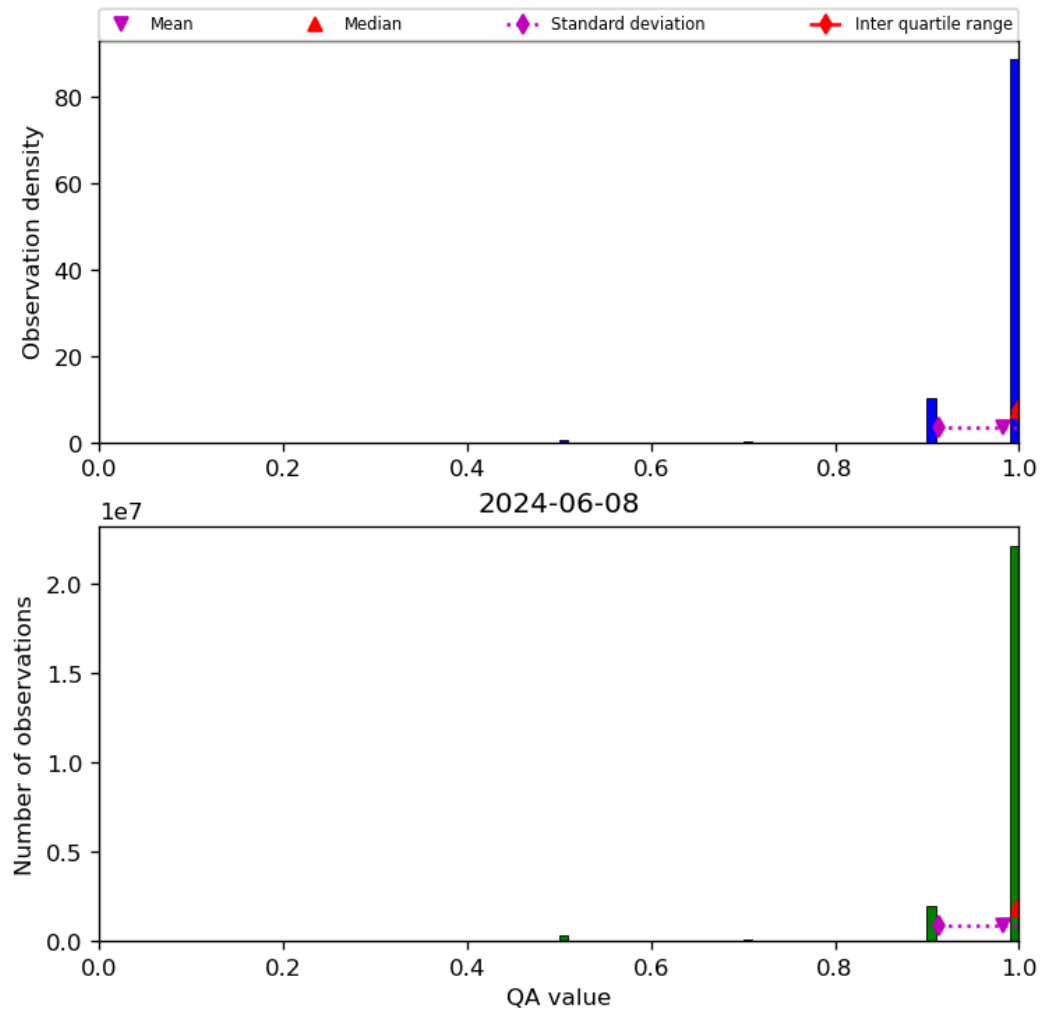
Figure 29: Histogram of “QA value” for 2024-06-08 to 2024-06-09
