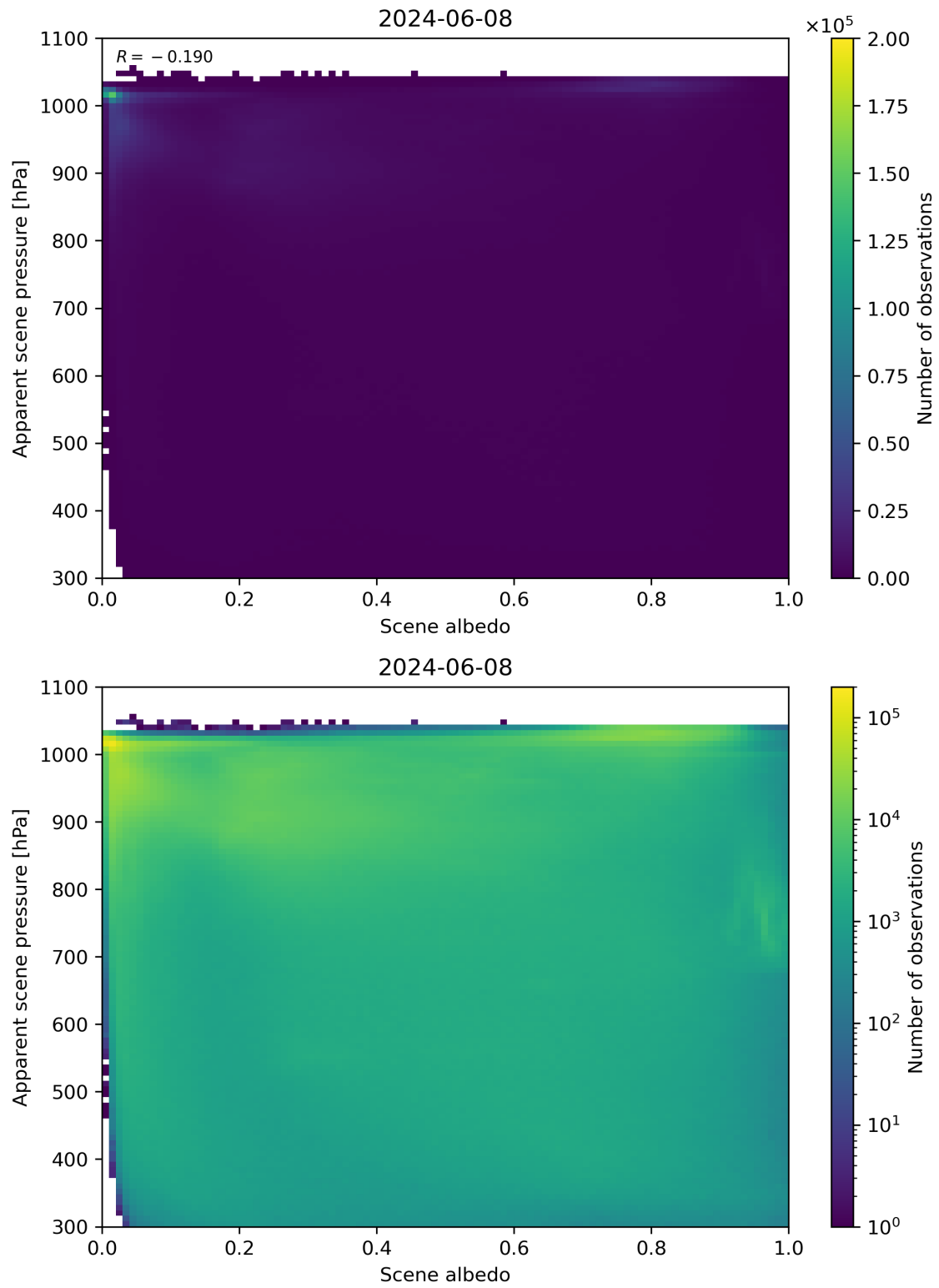
Figure 102: Scatter density plot of “Scene albedo” against “Apparent scene pressure” for 2024-06-08 to 2024-06-09.
