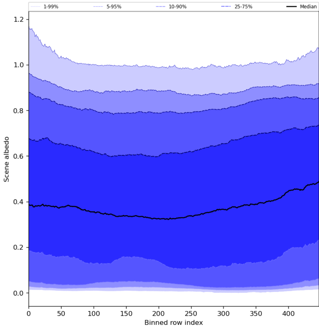
Figure 51: Along track statistics of “Scene albedo” for 2024-06-08 to 2024-06-09
