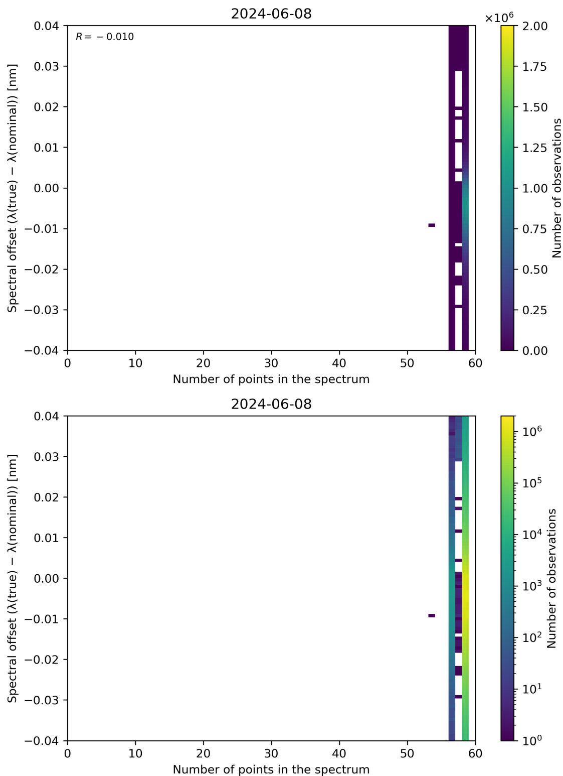
Figure 101: Scatter density plot of “Number of points in the spectrum” against “Spectral offset ( \lambda(\text{true}) - \lambda(\text{nominal}) )” for 2024-06-08 to 2024-06-09.
