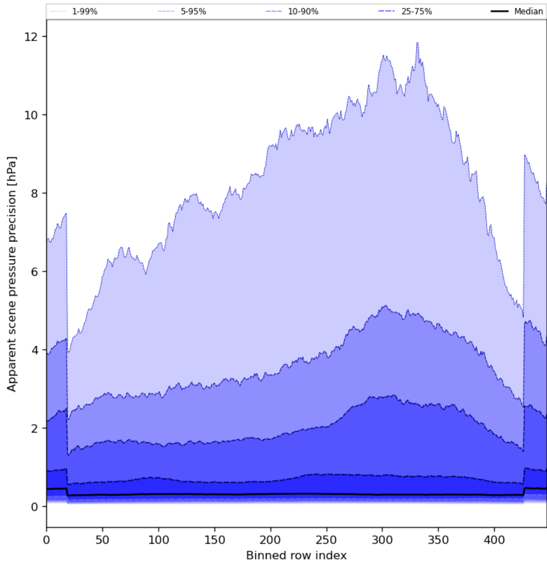
Figure 54: Along track statistics of “Apparent scene pressure precision” for 2024-06-08 to 2024-06-09
