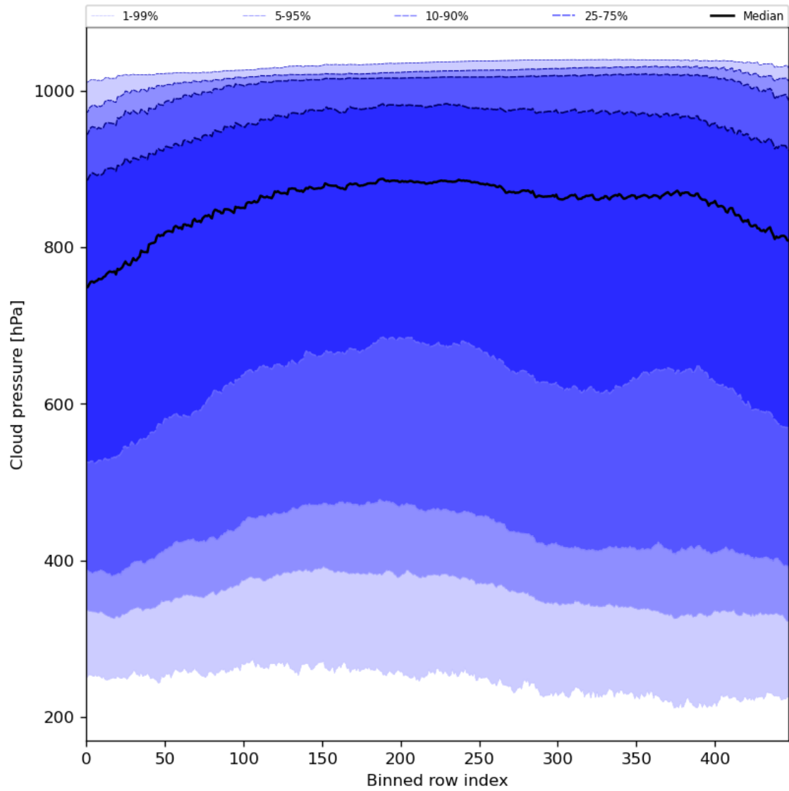
Figure 47: Along track statistics of “Cloud pressure” for 2024-06-08 to 2024-06-09
