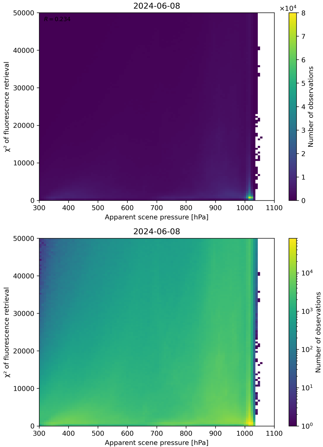
Figure 63: Scatter density plot of “Apparent scene pressure” against “ \chi^2 of fluorescence retrieval” for 2024-06-08 to 2024-06-09.
