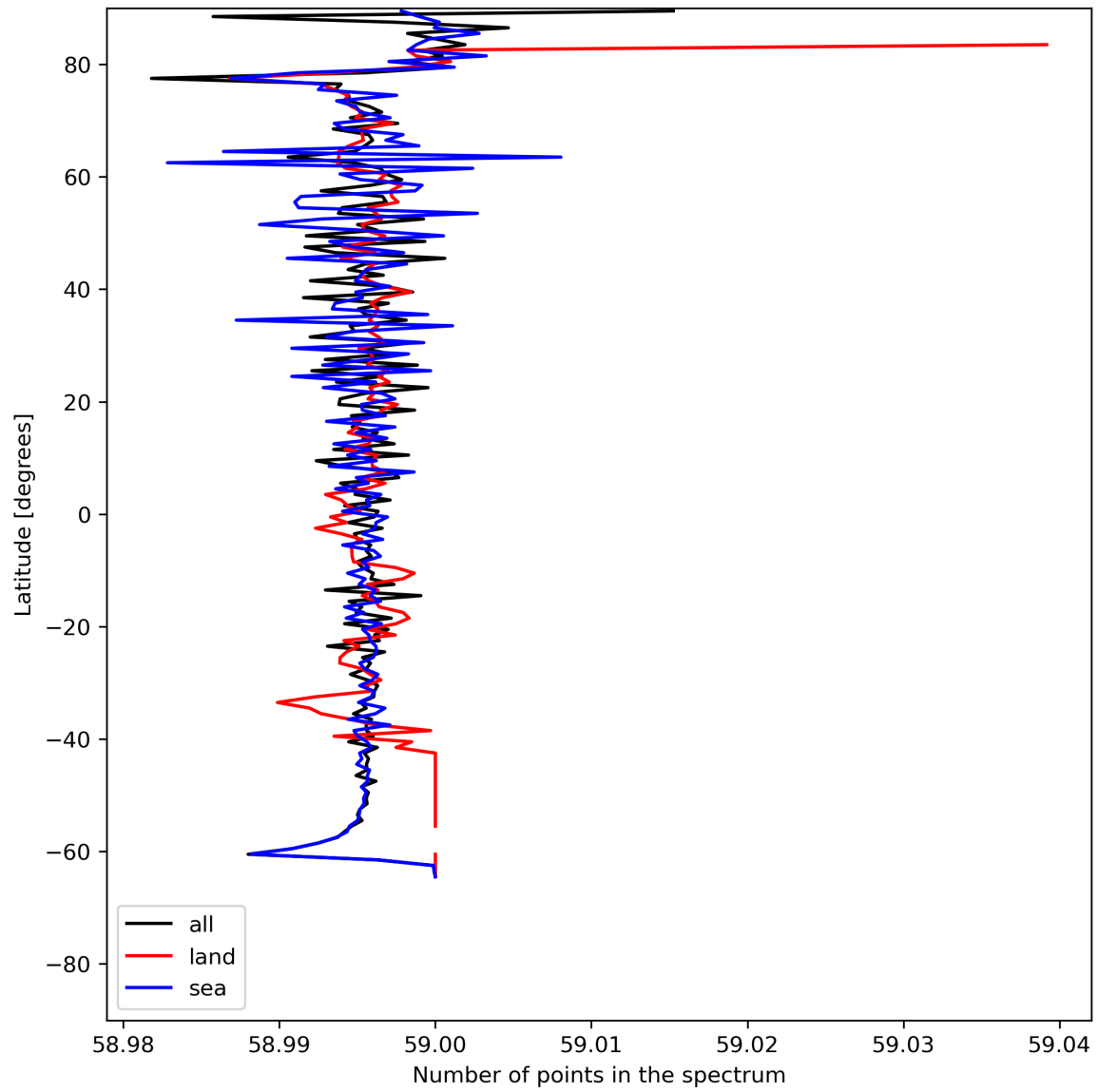
Figure 27: Zonal average of “Number of points in the spectrum” for 2024-06-08 to 2024-06-09.
