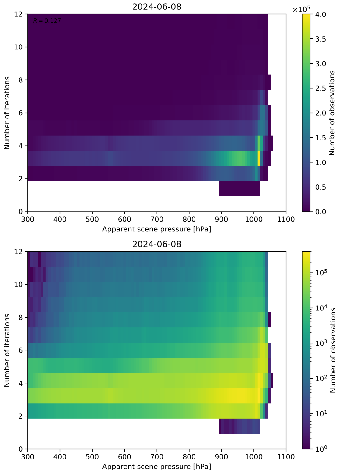
Figure 65: Scatter density plot of “Apparent scene pressure” against “Number of iterations” for 2024-06-08 to 2024-06-09.
