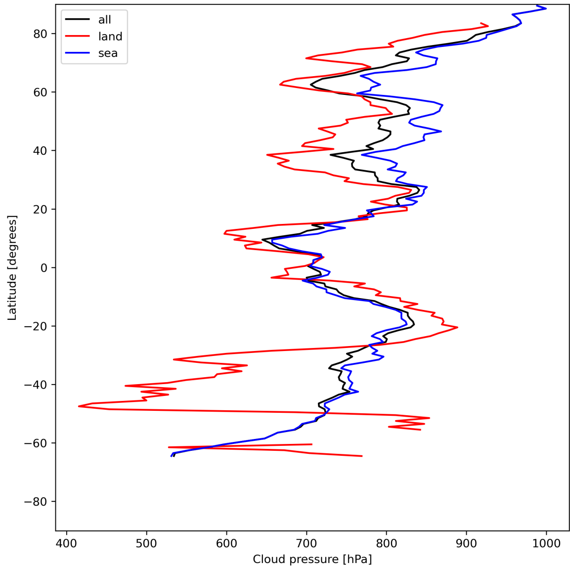
Figure 13: Zonal average of “Cloud pressure” for 2024-06-08 to 2024-06-09.
