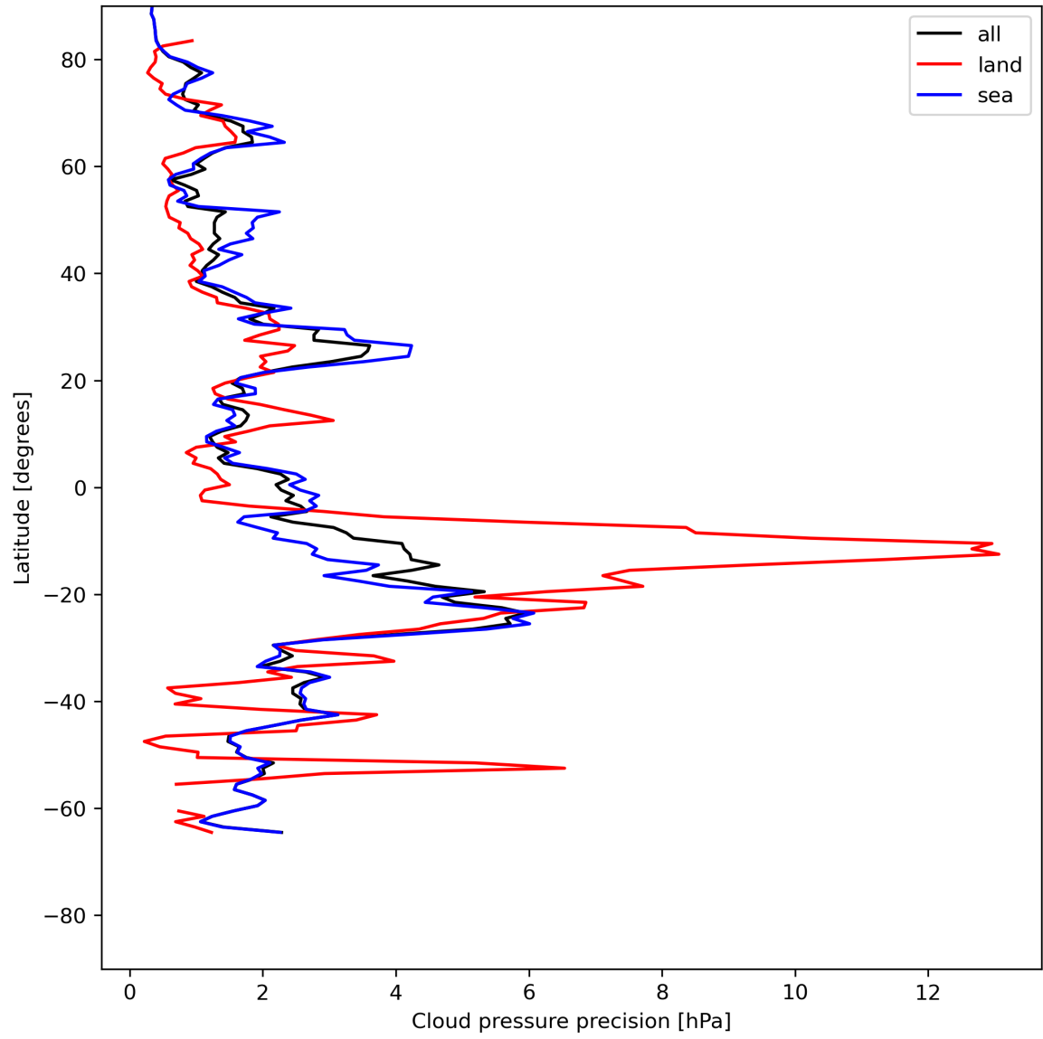
Figure 14: Zonal average of “Cloud pressure precision” for 2024-06-08 to 2024-06-09.
