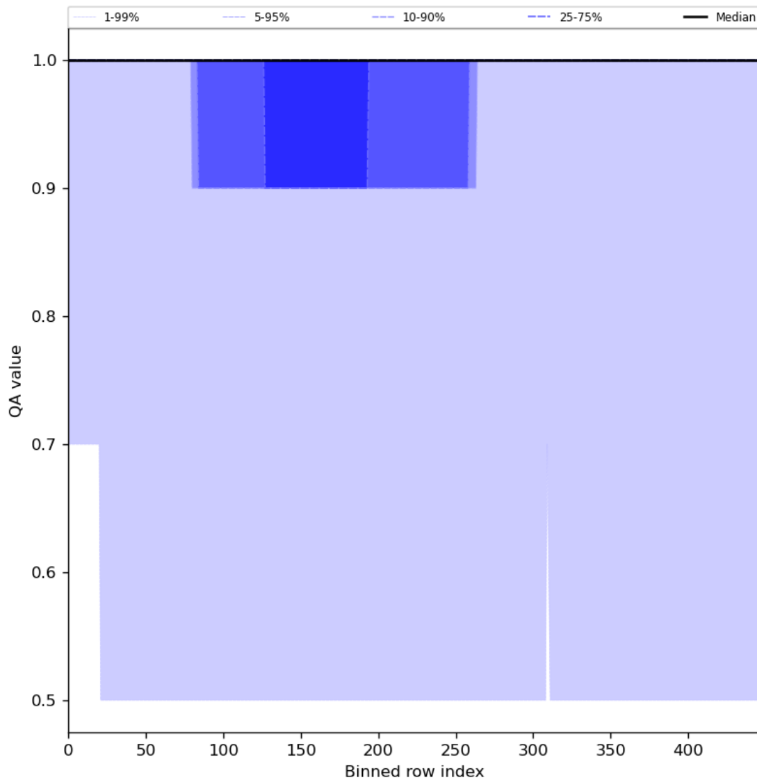
Figure 46: Along track statistics of “QA value” for 2024-06-08 to 2024-06-09
