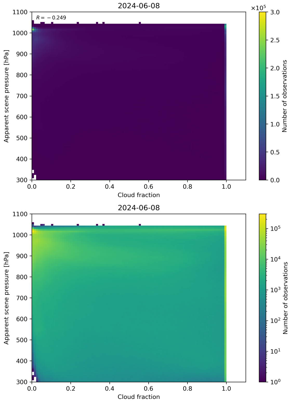
Figure 70: Scatter density plot of “Cloud fraction” against “Apparent scene pressure” for 2024-06-08 to 2024-06-09.
