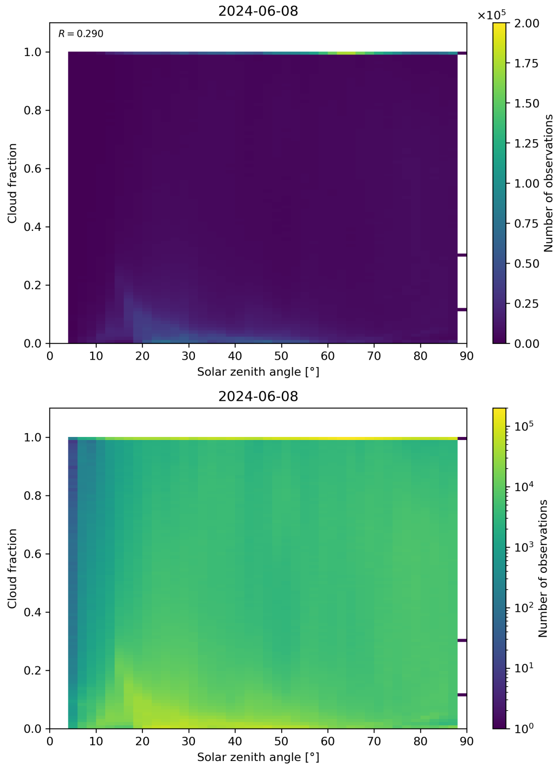
Figure 110: Scatter density plot of “Solar zenith angle” against “Cloud fraction” for 2024-06-08 to 2024-06-09.
