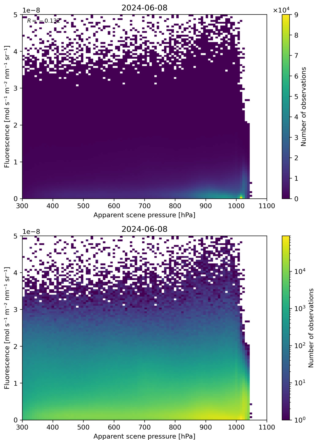
Figure 64: Scatter density plot of “Apparent scene pressure” against “Fluorescence” for 2024-06-08 to 2024-06-09.
