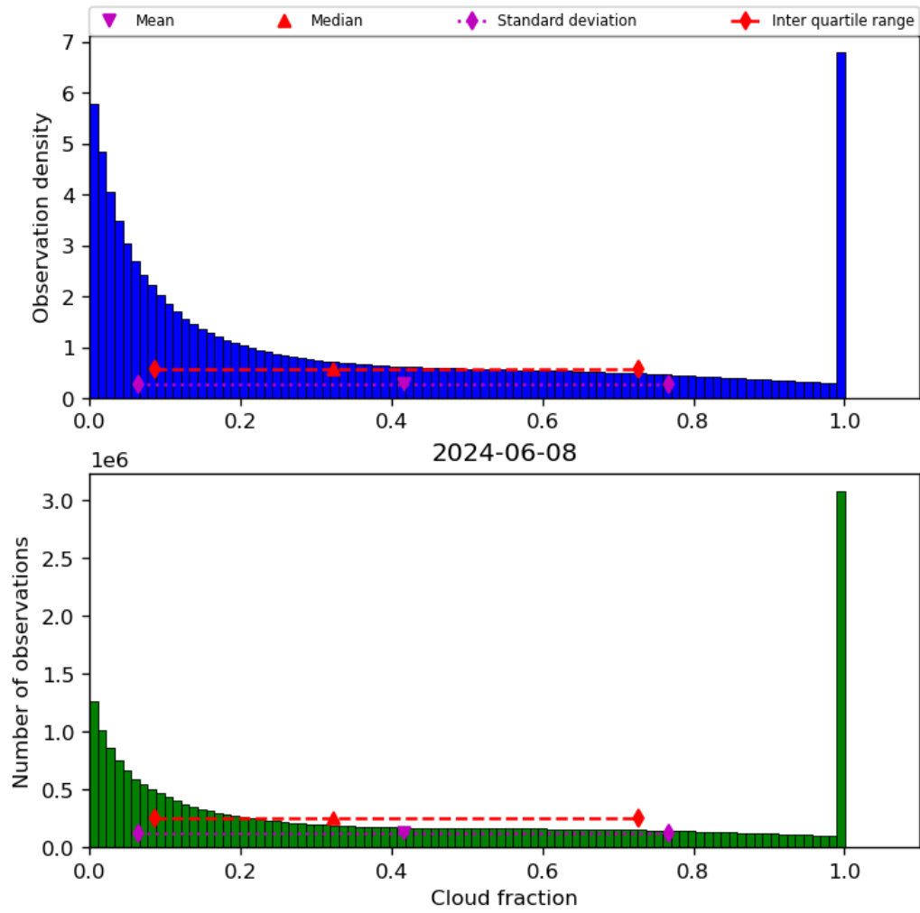
Figure 32: Histogram of “Cloud fraction” for 2024-06-08 to 2024-06-09
