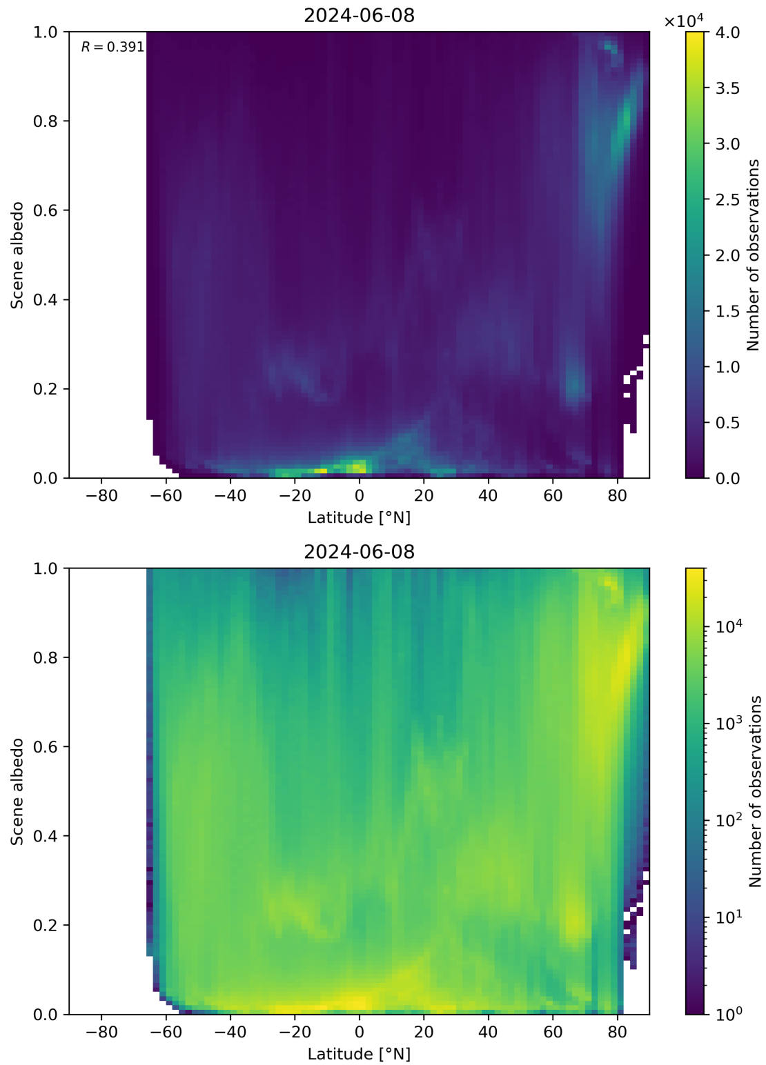
Figure 95: Scatter density plot of “Latitude” against “Scene albedo” for 2024-06-08 to 2024-06-09.
