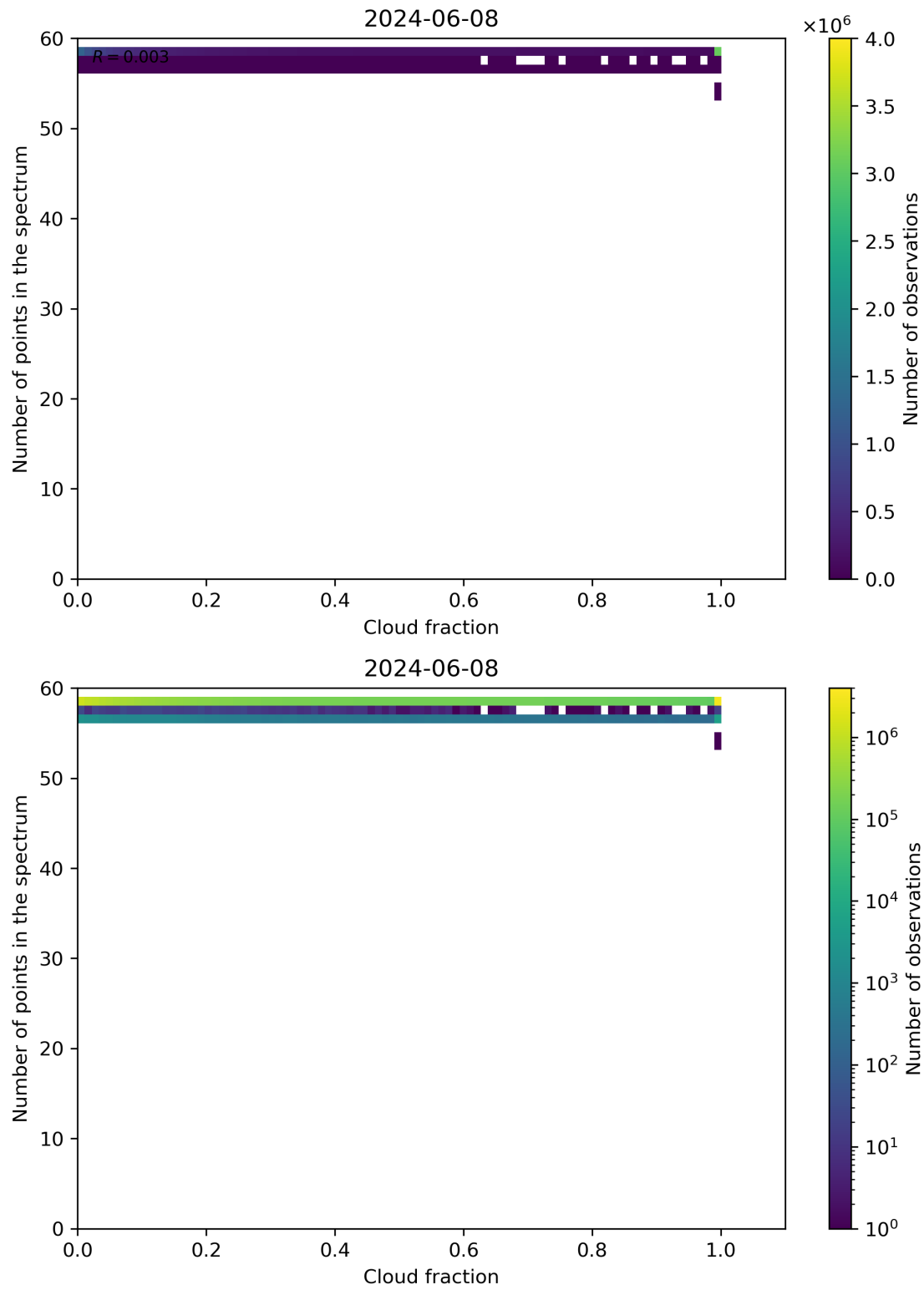
Figure 74: Scatter density plot of “Cloud fraction” against “Number of points in the spectrum” for 2024-06-08 to 2024-06-09.
