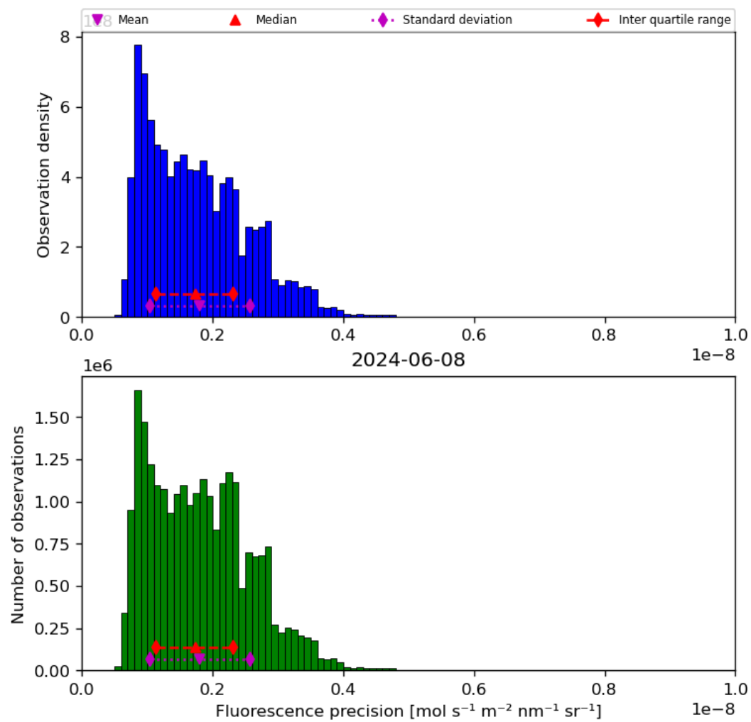
Figure 41: Histogram of “Fluorescence precision” for 2024-06-08 to 2024-06-09
