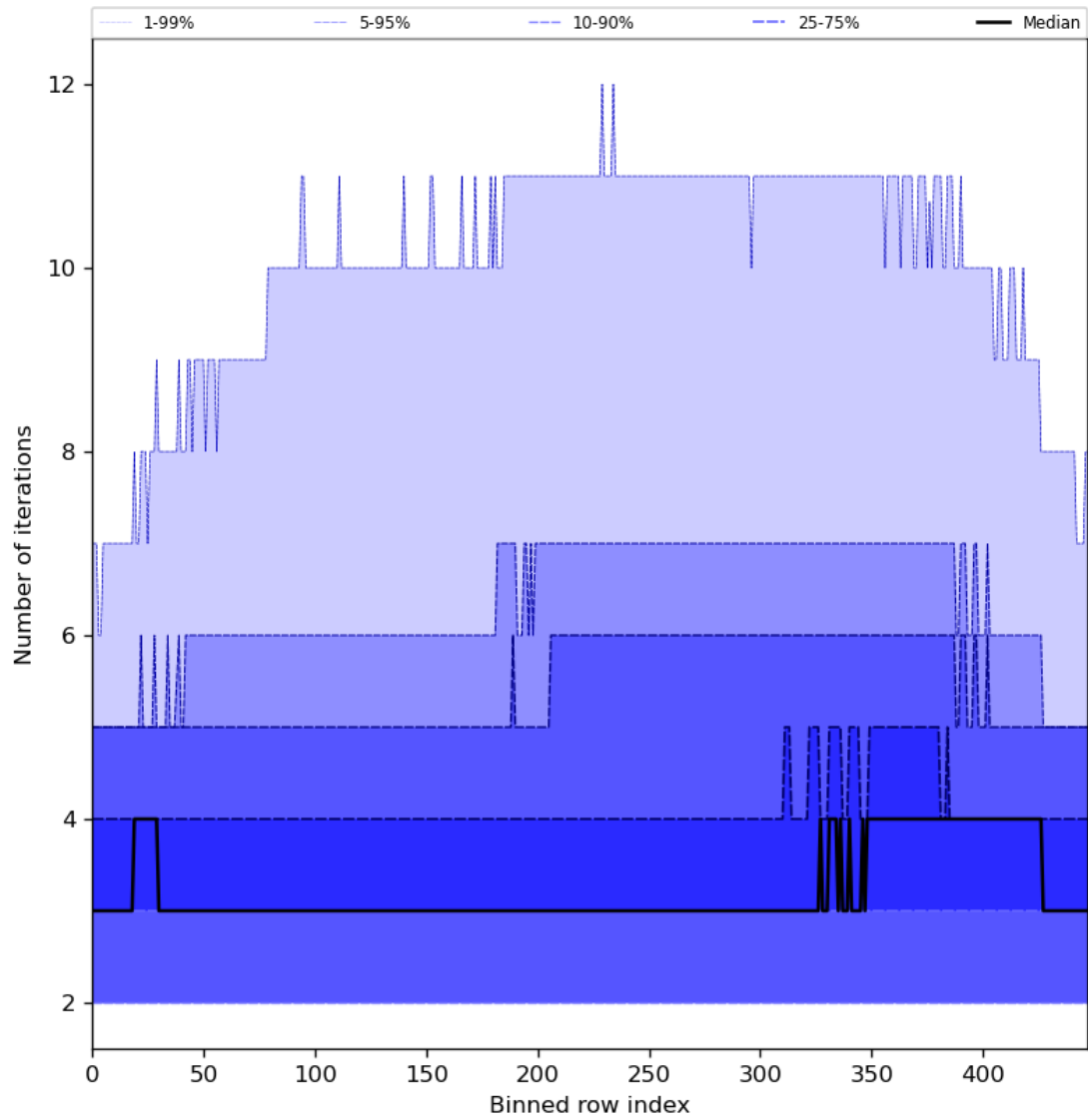
Figure 56: Along track statistics of “Number of iterations” for 2024-06-08 to 2024-06-09
