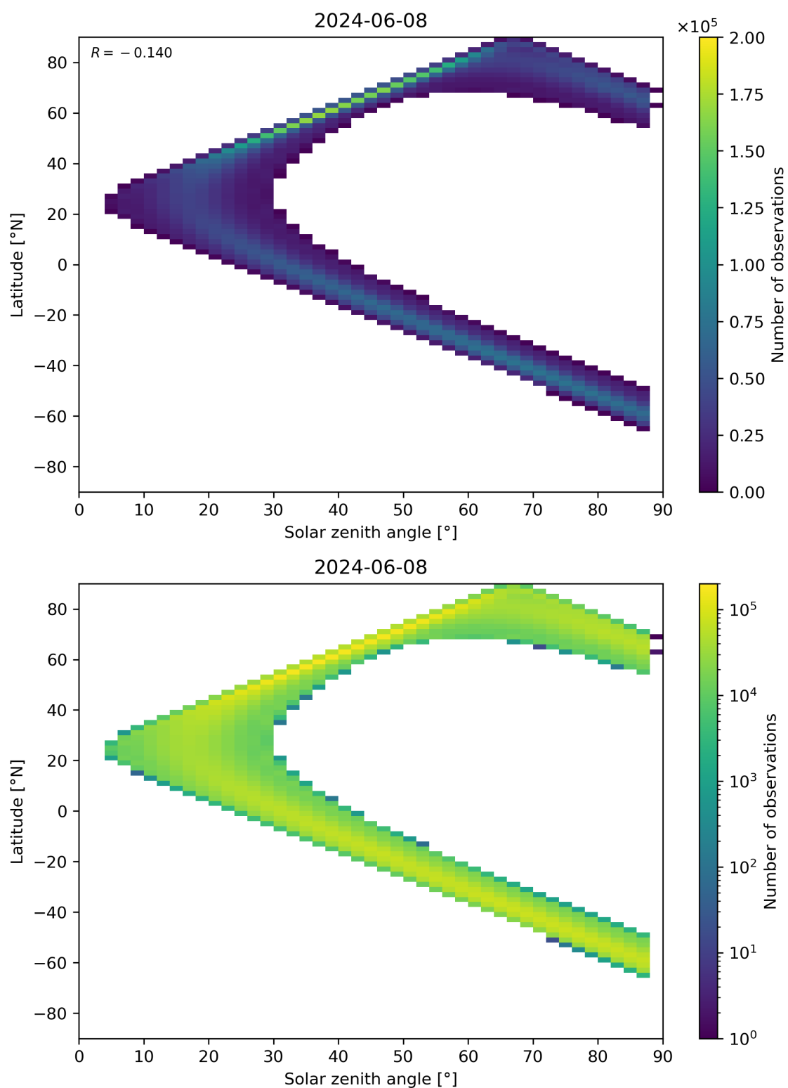
Figure 113: Scatter density plot of “Solar zenith angle” against “Latitude” for 2024-06-08 to 2024-06-09.
