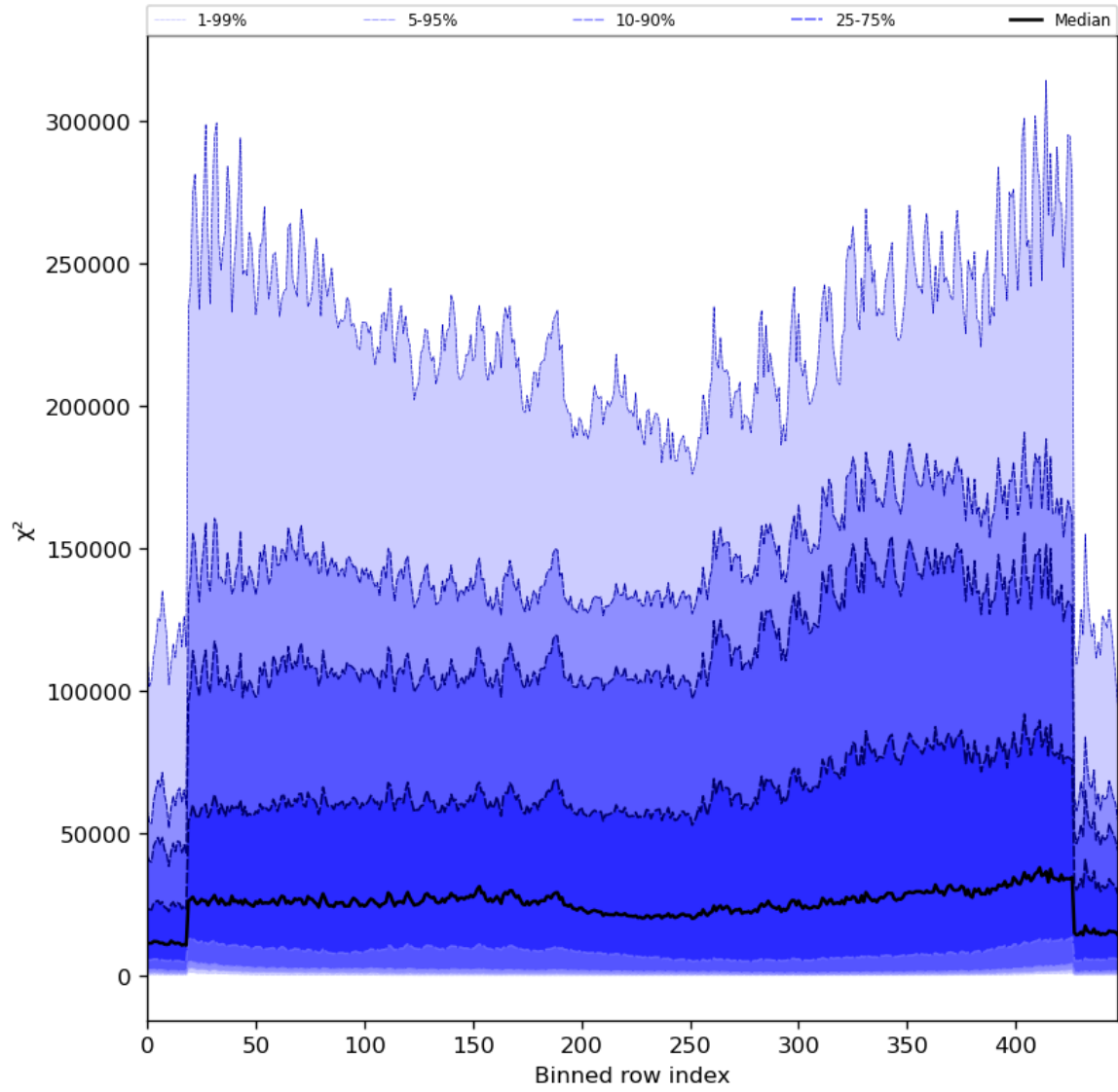
Figure 55: Along track statistics of “ \chi^2 ” for 2024-06-08 to 2024-06-09
