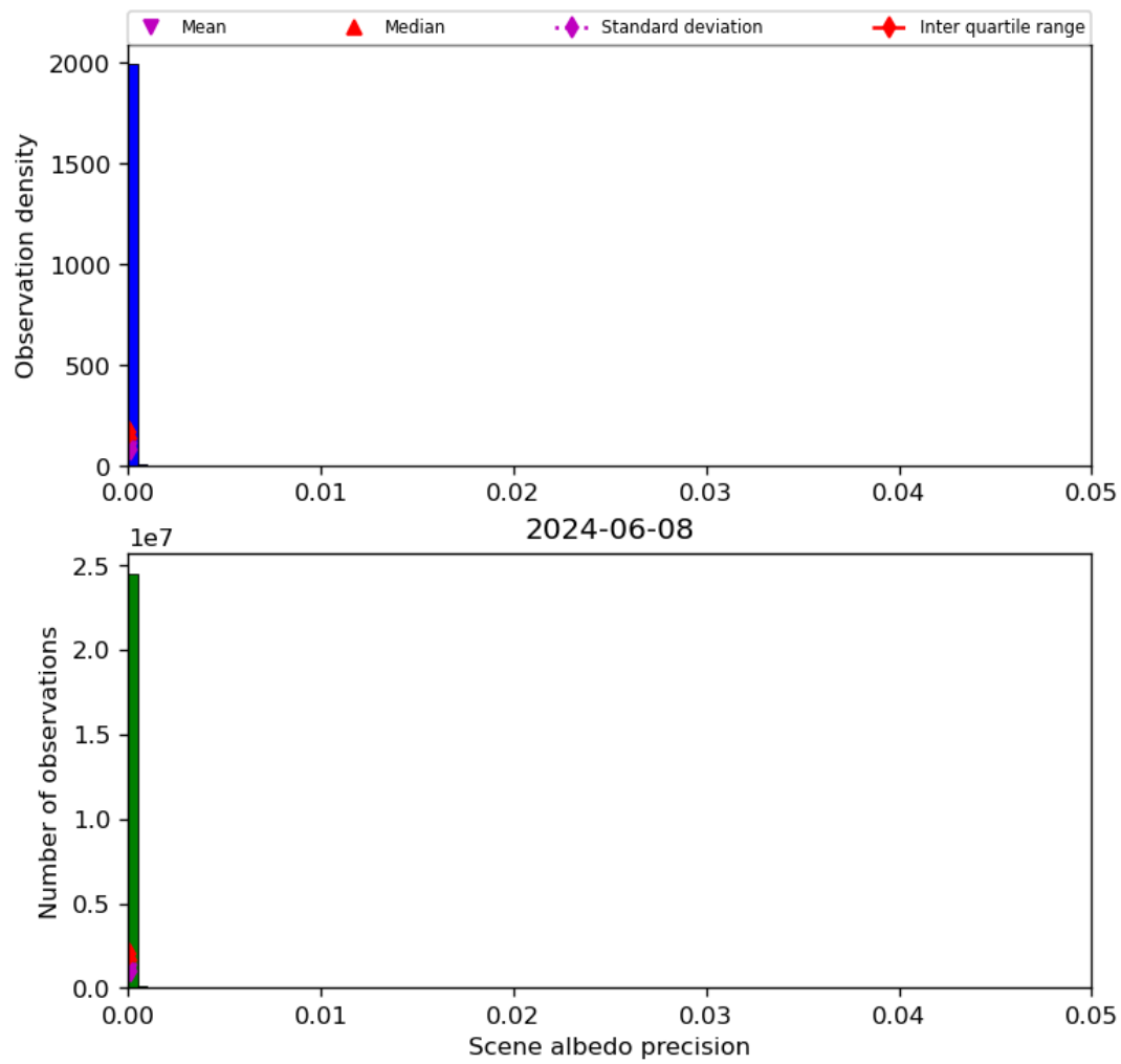
Figure 35: Histogram of “Scene albedo precision” for 2024-06-08 to 2024-06-09
