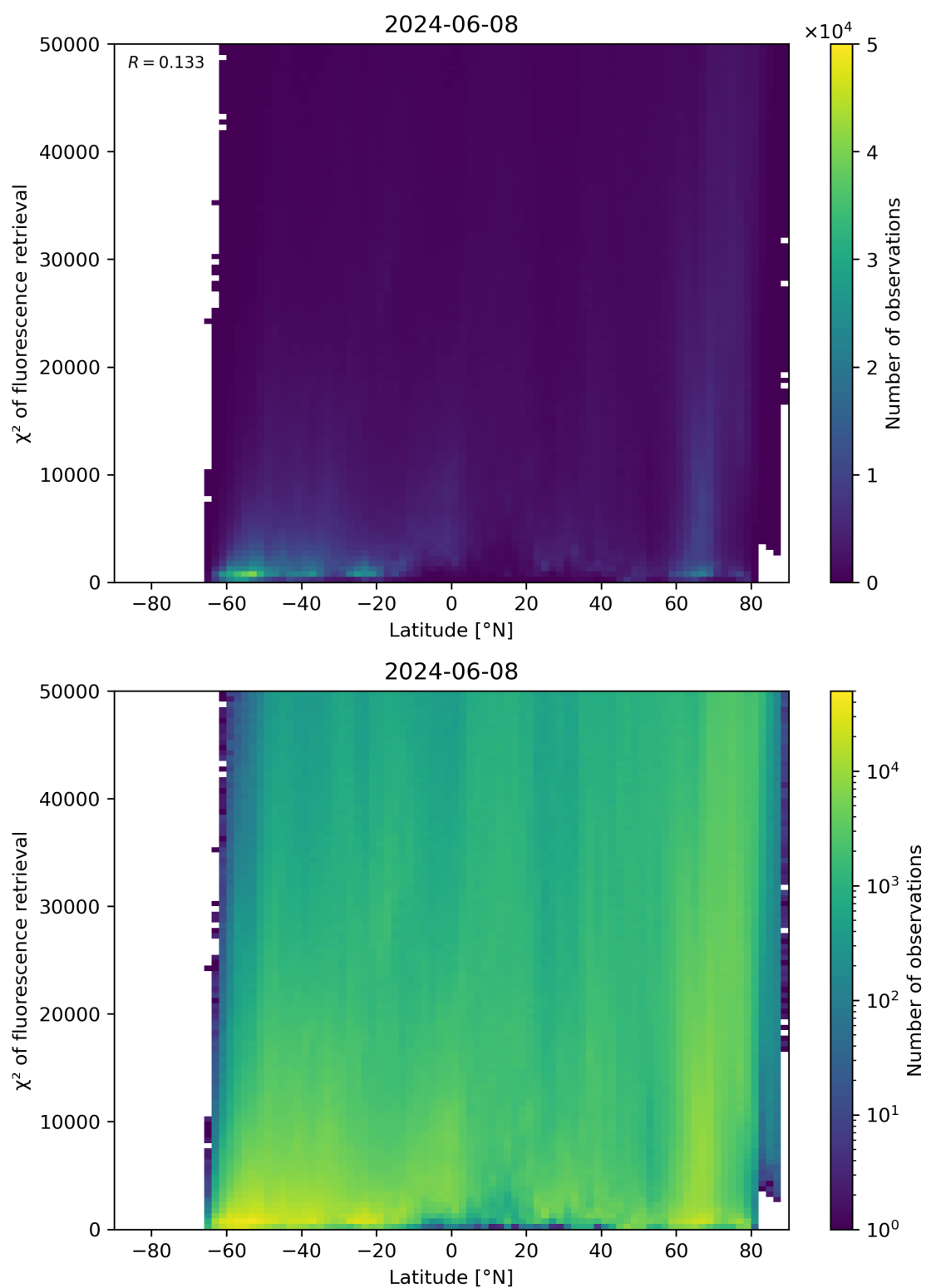
Figure 89: Scatter density plot of “Latitude” against “ \chi^2 of fluorescence retrieval” for 2024-06-08 to 2024-06-09.
