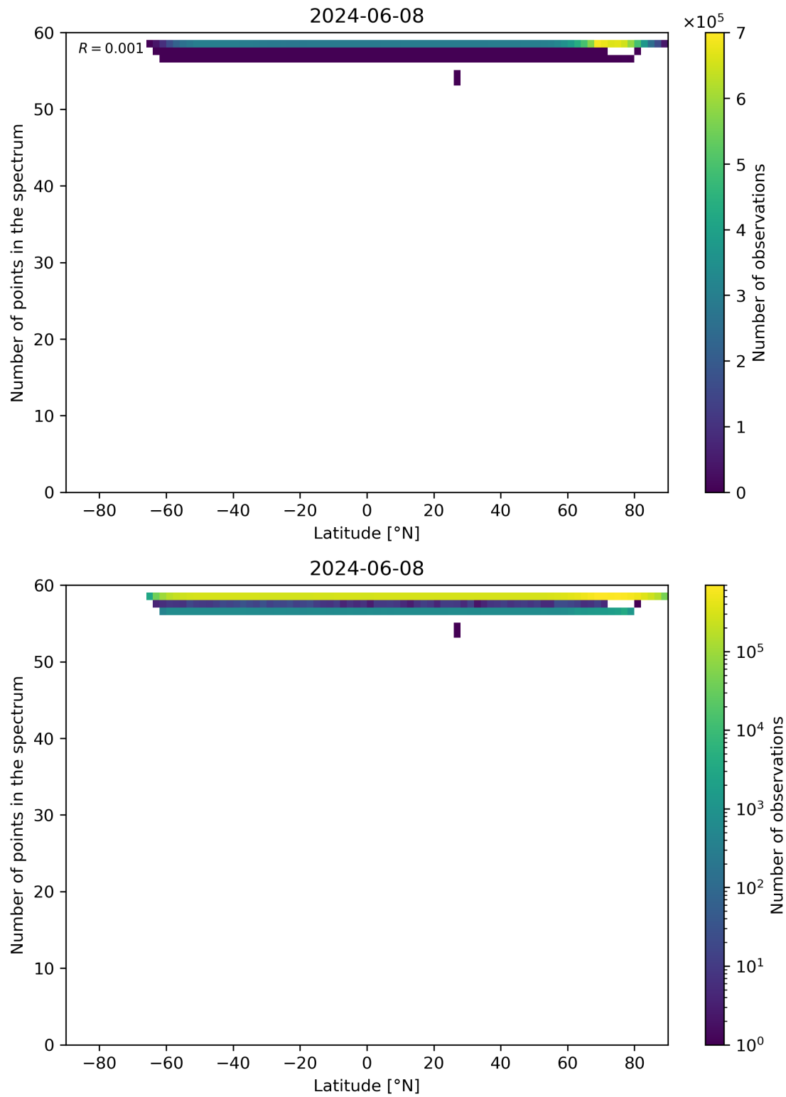
Figure 94: Scatter density plot of “Latitude” against “Number of points in the spectrum” for 2024-06-08 to 2024-06-09.
