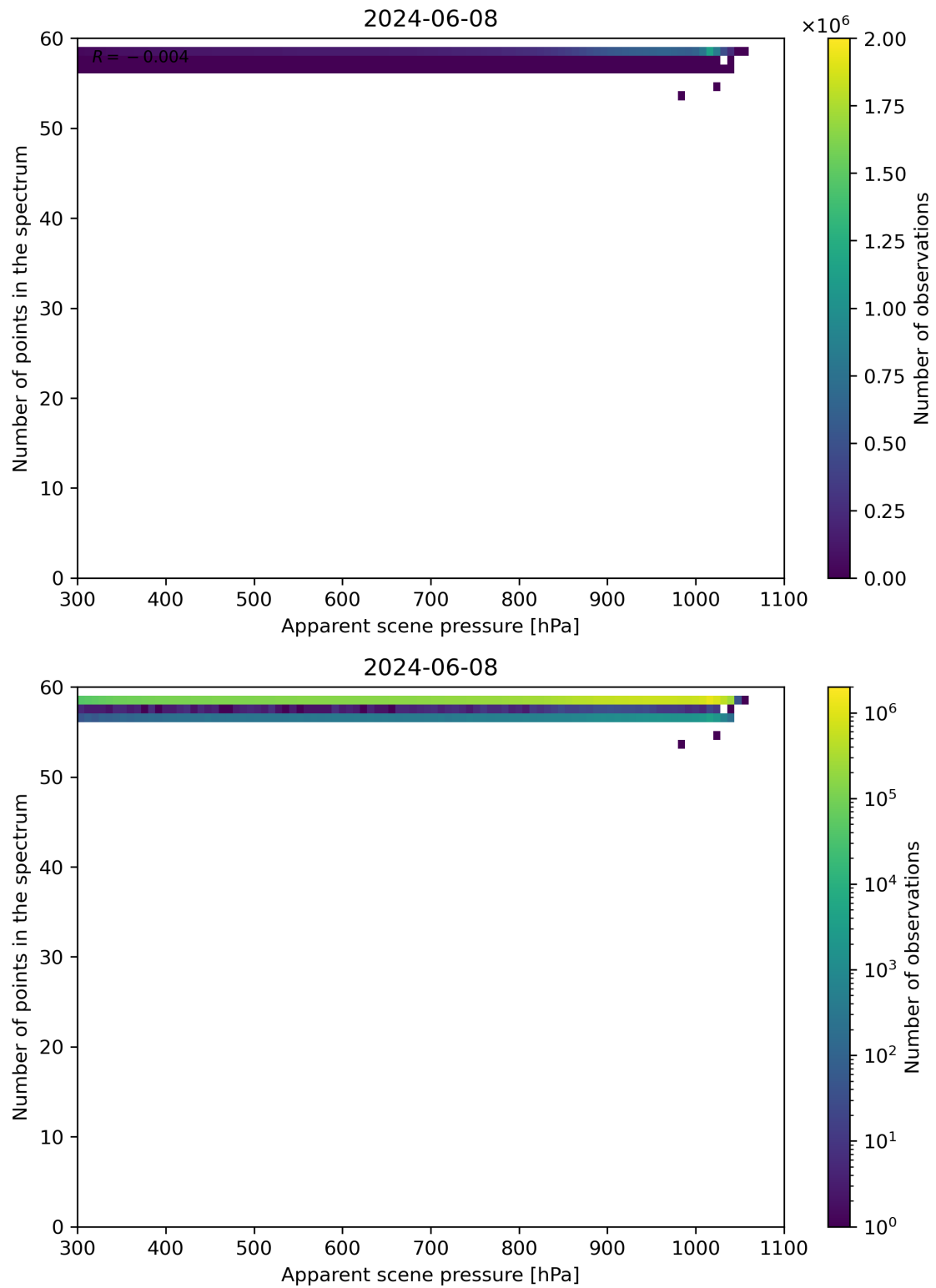
Figure 66: Scatter density plot of “Apparent scene pressure” against “Number of points in the spectrum” for 2024-06-08 to 2024-06-09.
