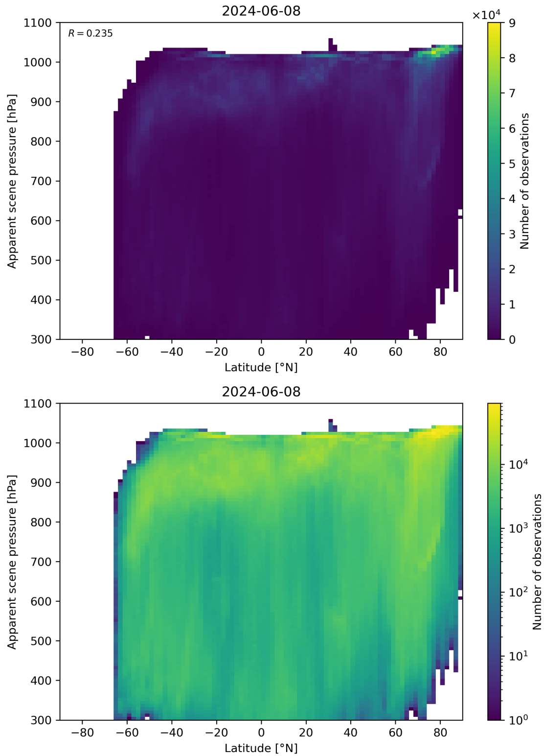
Figure 88: Scatter density plot of “Latitude” against “Apparent scene pressure” for 2024-06-08 to 2024-06-09.
