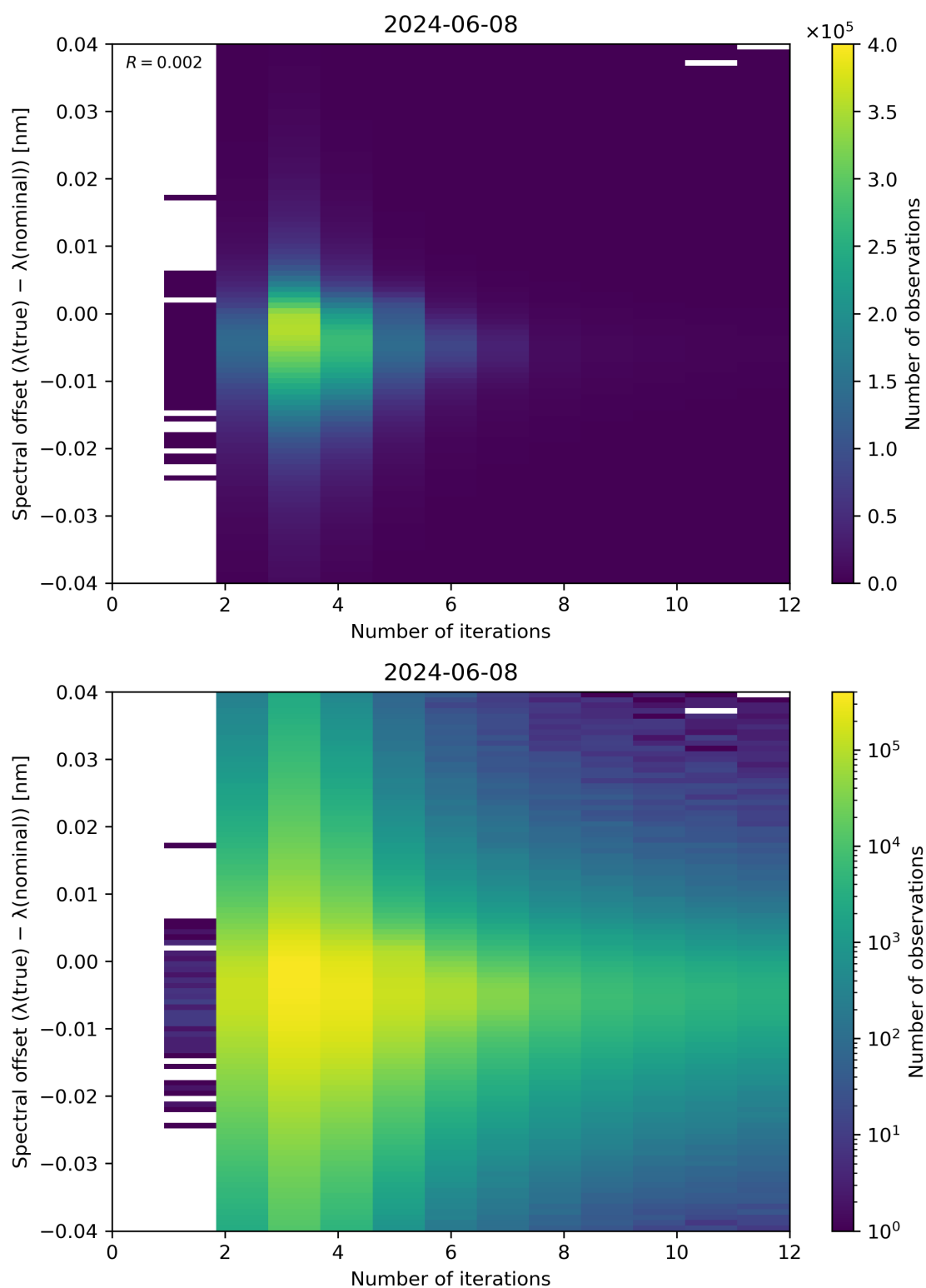
Figure 100: Scatter density plot of “Number of iterations” against “Spectral offset ( \lambda(\text{true}) - \lambda(\text{nominal}) )” for 2024-06-08 to 2024-06-09.
