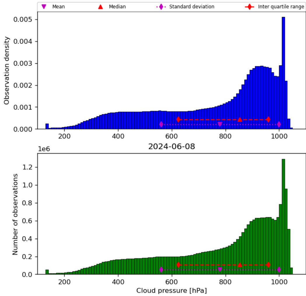
Figure 30: Histogram of “Cloud pressure” for 2024-06-08 to 2024-06-09
