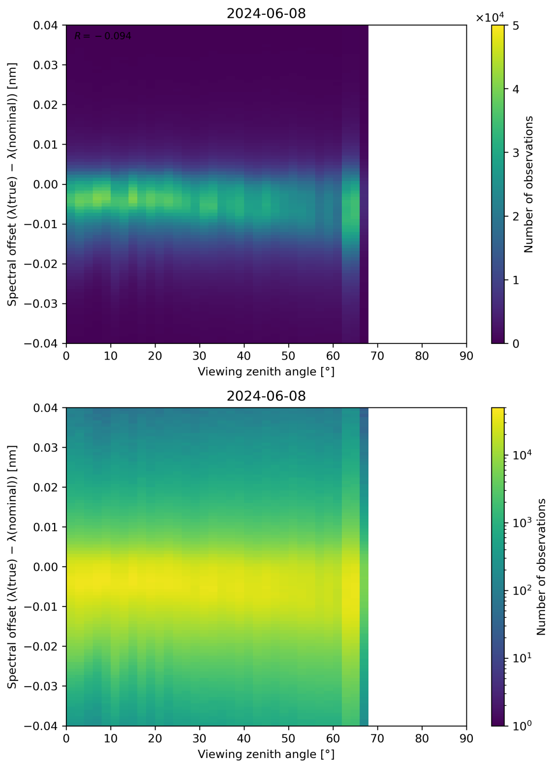
Figure 128: Scatter density plot of “Viewing zenith angle” against “Spectral offset ( \lambda(\text{true}) - \lambda(\text{nominal}) )” for 2024-06-08 to 2024-06-09.
