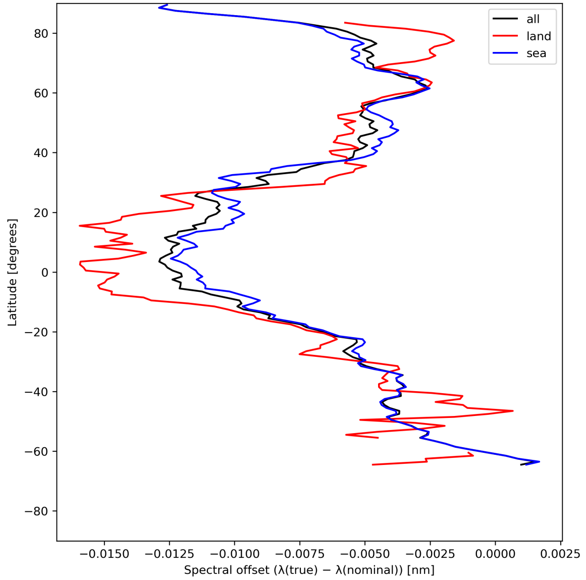
Figure 28: Zonal average of “Spectral offset ( \lambda(\text{true}) - \lambda(\text{nominal}) )” for 2024-06-08 to 2024-06-09.
