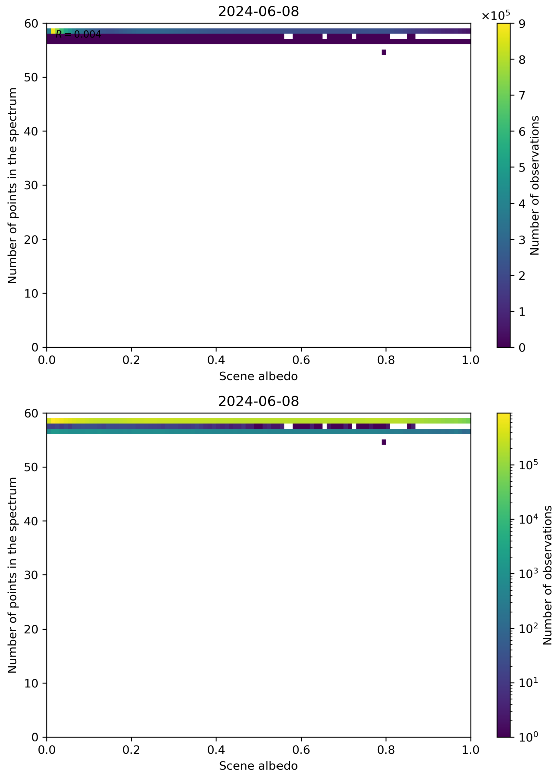
Figure 106: Scatter density plot of “Scene albedo” against “Number of points in the spectrum” for 2024-06-08 to 2024-06-09.
