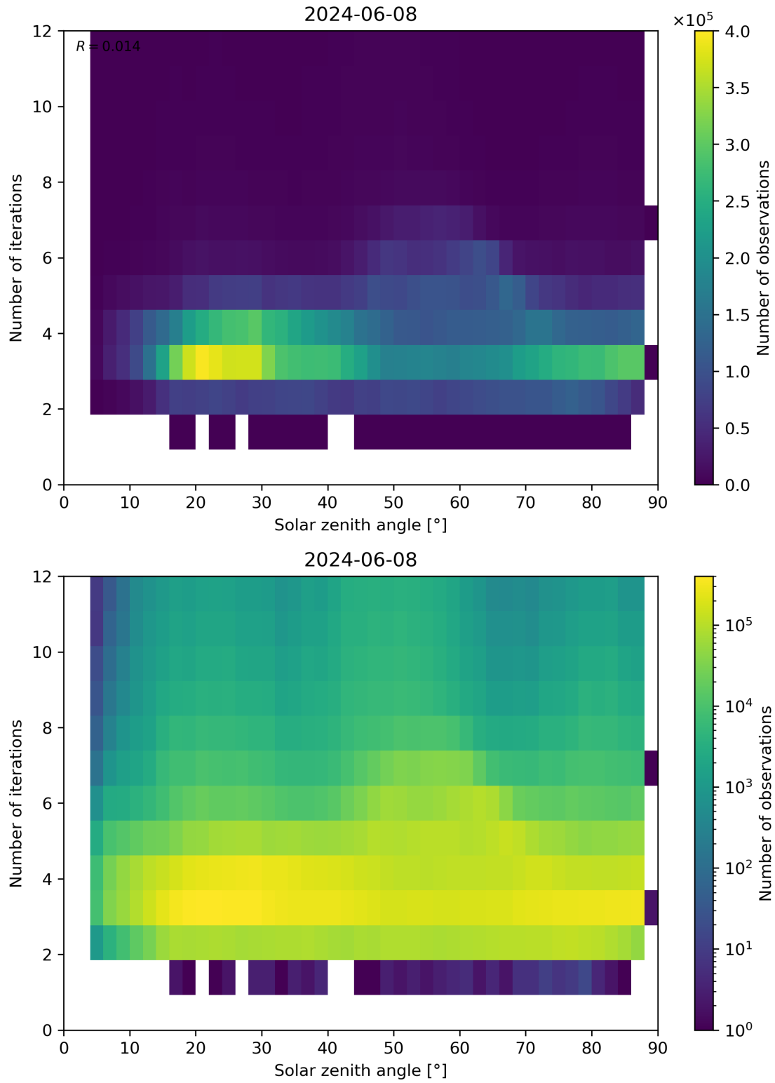
Figure 114: Scatter density plot of “Solar zenith angle” against “Number of iterations” for 2024-06-08 to 2024-06-09.
