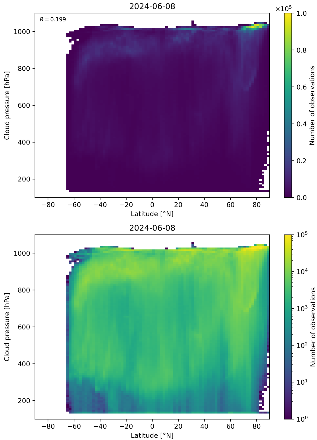
Figure 91: Scatter density plot of “Latitude” against “Cloud pressure” for 2024-06-08 to 2024-06-09.
