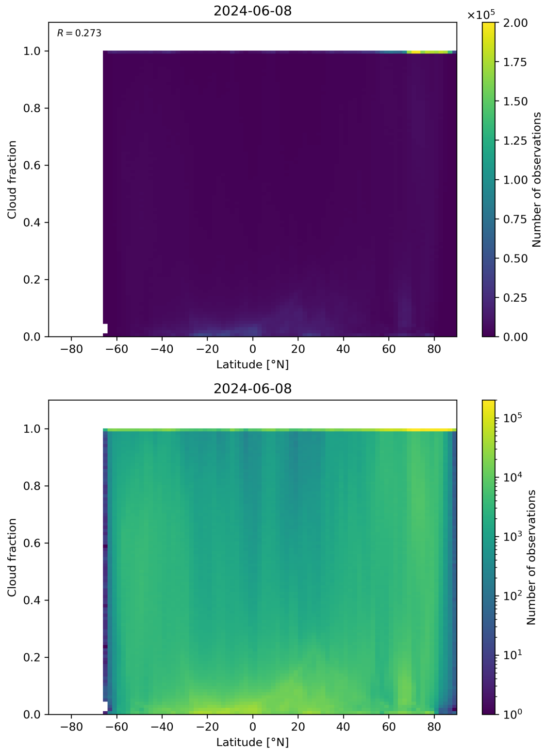
Figure 90: Scatter density plot of “Latitude” against “Cloud fraction” for 2024-06-08 to 2024-06-09.
