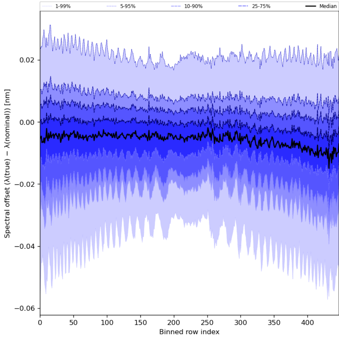
Figure 62: Along track statistics of “Spectral offset ( \lambda(\text{true}) - \lambda(\text{nominal}) )” for 2024-06-08 to 2024-06-09
