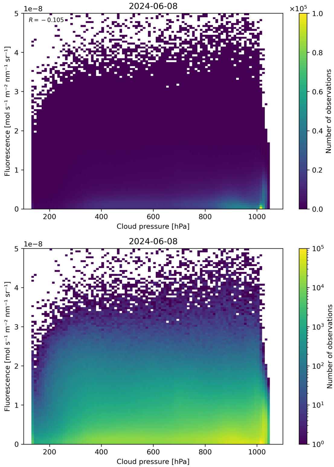
Figure 80: Scatter density plot of “Cloud pressure” against “Fluorescence” for 2024-06-08 to 2024-06-09.
