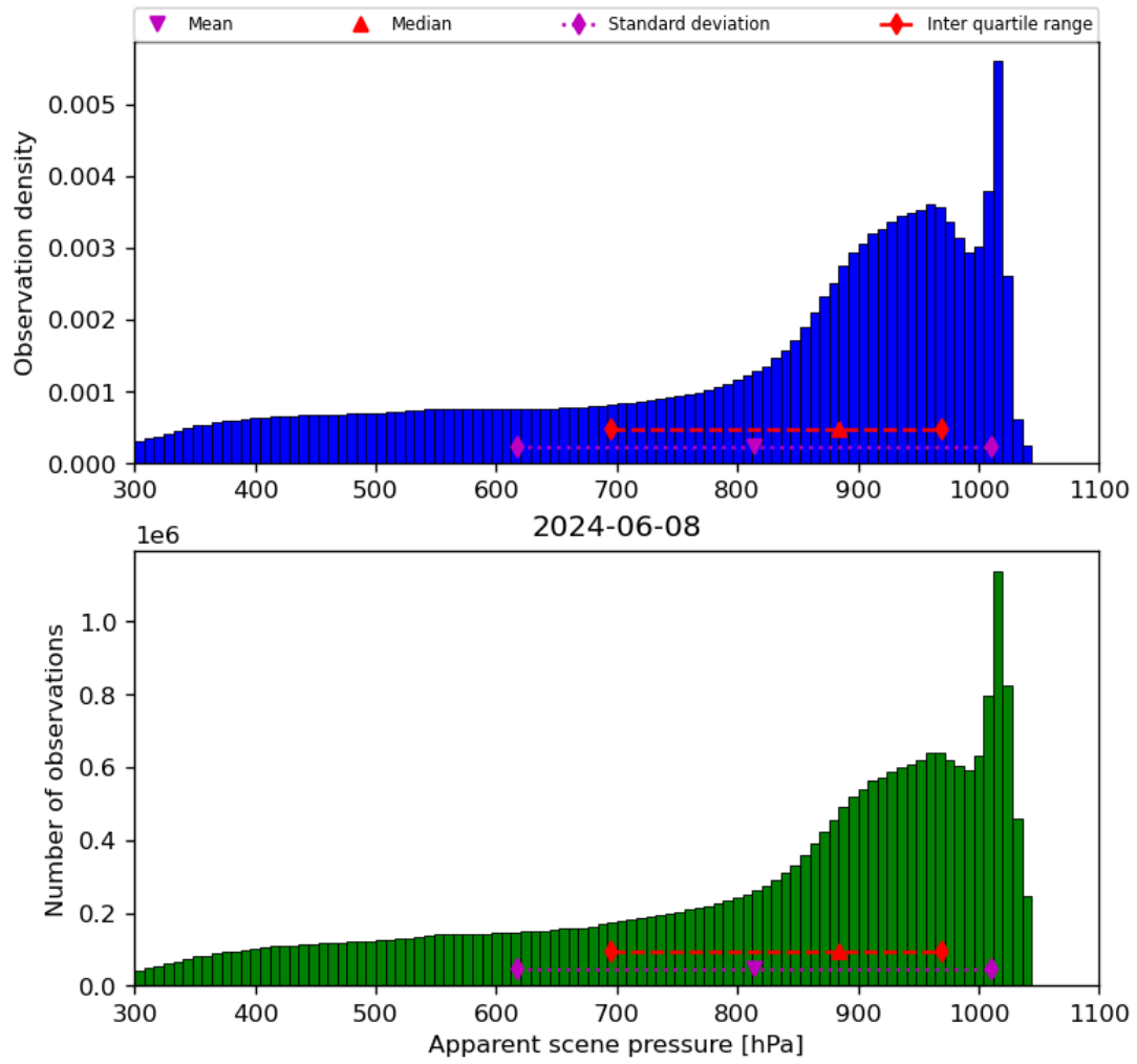
Figure 36: Histogram of “Apparent scene pressure” for 2024-06-08 to 2024-06-09
