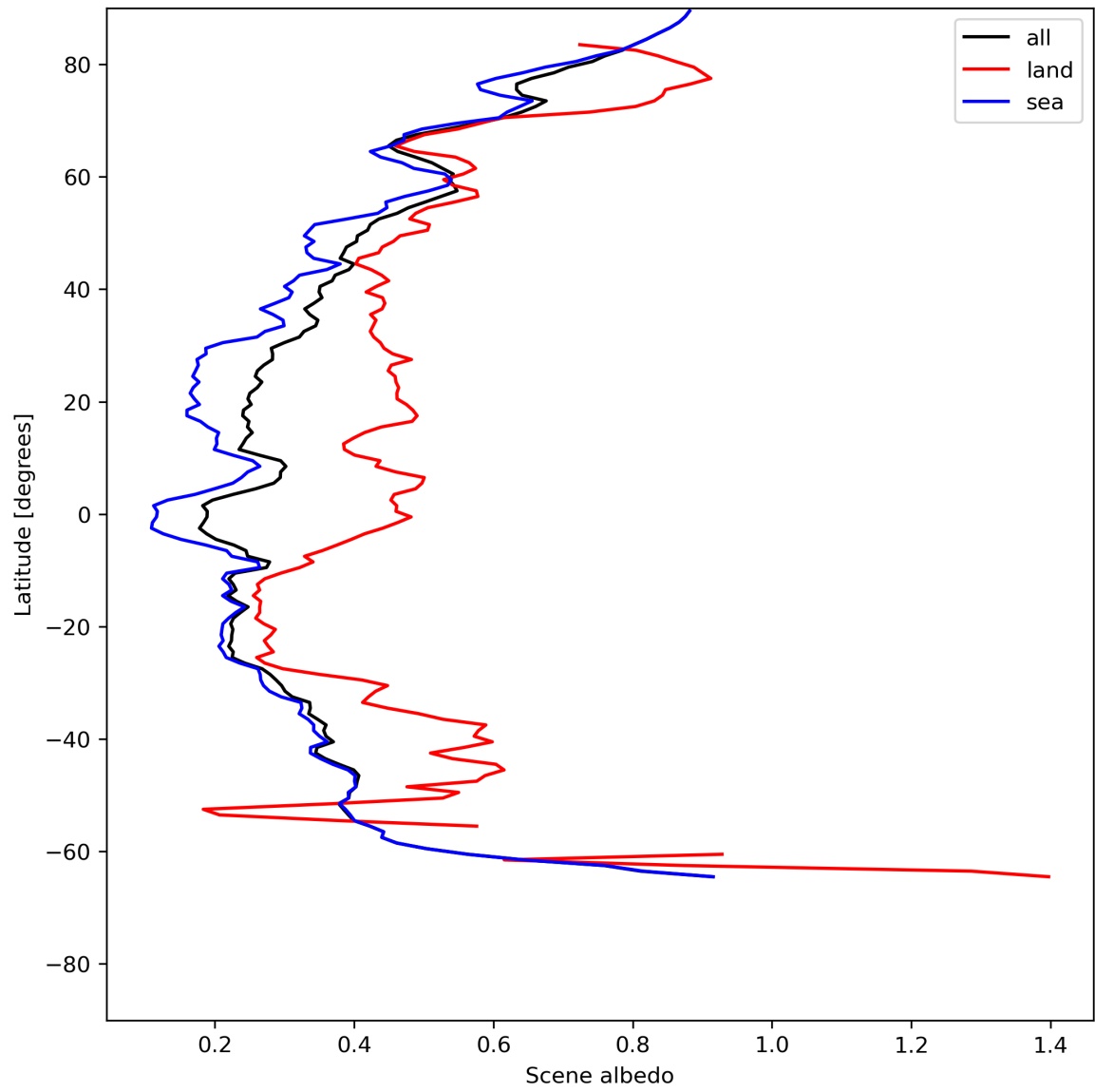
Figure 17: Zonal average of “Scene albedo” for 2024-06-08 to 2024-06-09.
