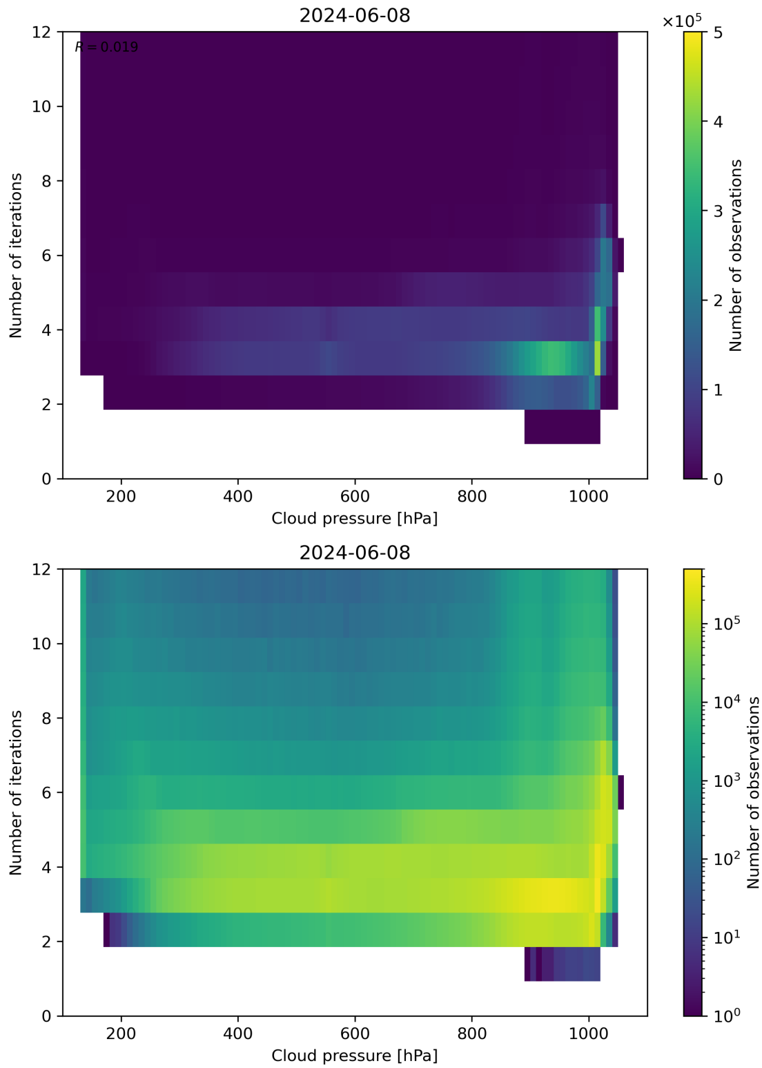
Figure 81: Scatter density plot of “Cloud pressure” against “Number of iterations” for 2024-06-08 to 2024-06-09.
