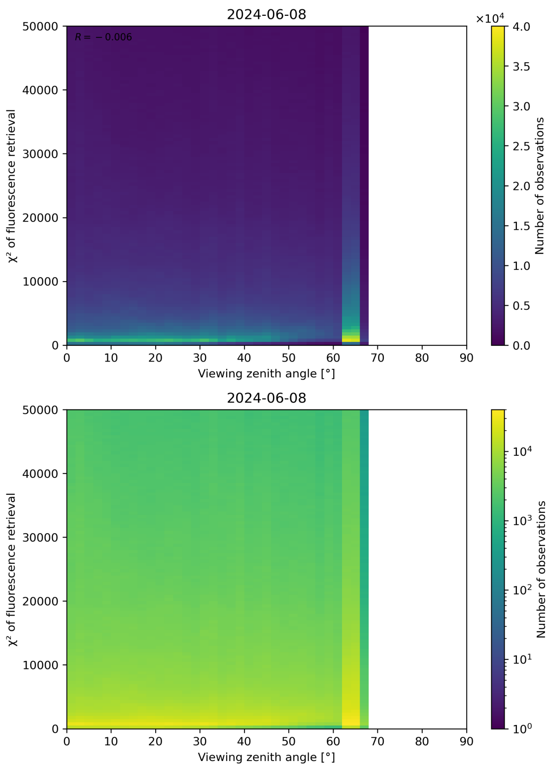
Figure 119: Scatter density plot of “Viewing zenith angle” against “ \chi^2 of fluorescence retrieval” for 2024-06-08 to 2024-06-09.
