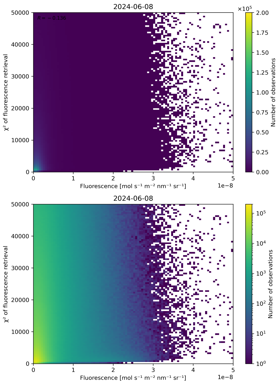
Figure 85: Scatter density plot of “Fluorescence” against “ \chi^2 of fluorescence retrieval” for 2024-06-08 to 2024-06-09.
