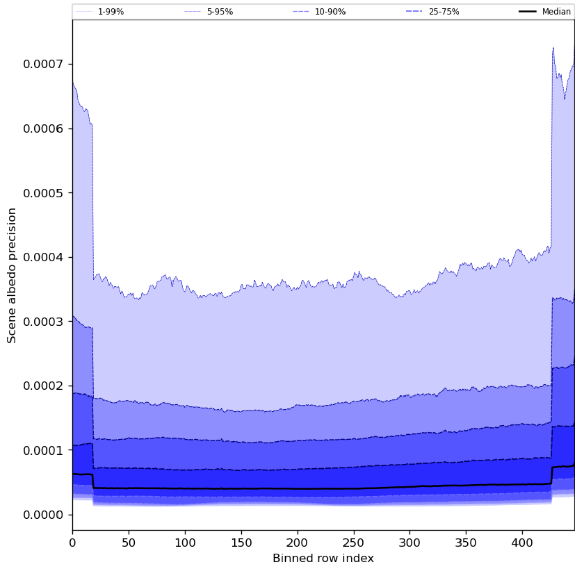
Figure 52: Along track statistics of “Scene albedo precision” for 2024-06-08 to 2024-06-09
