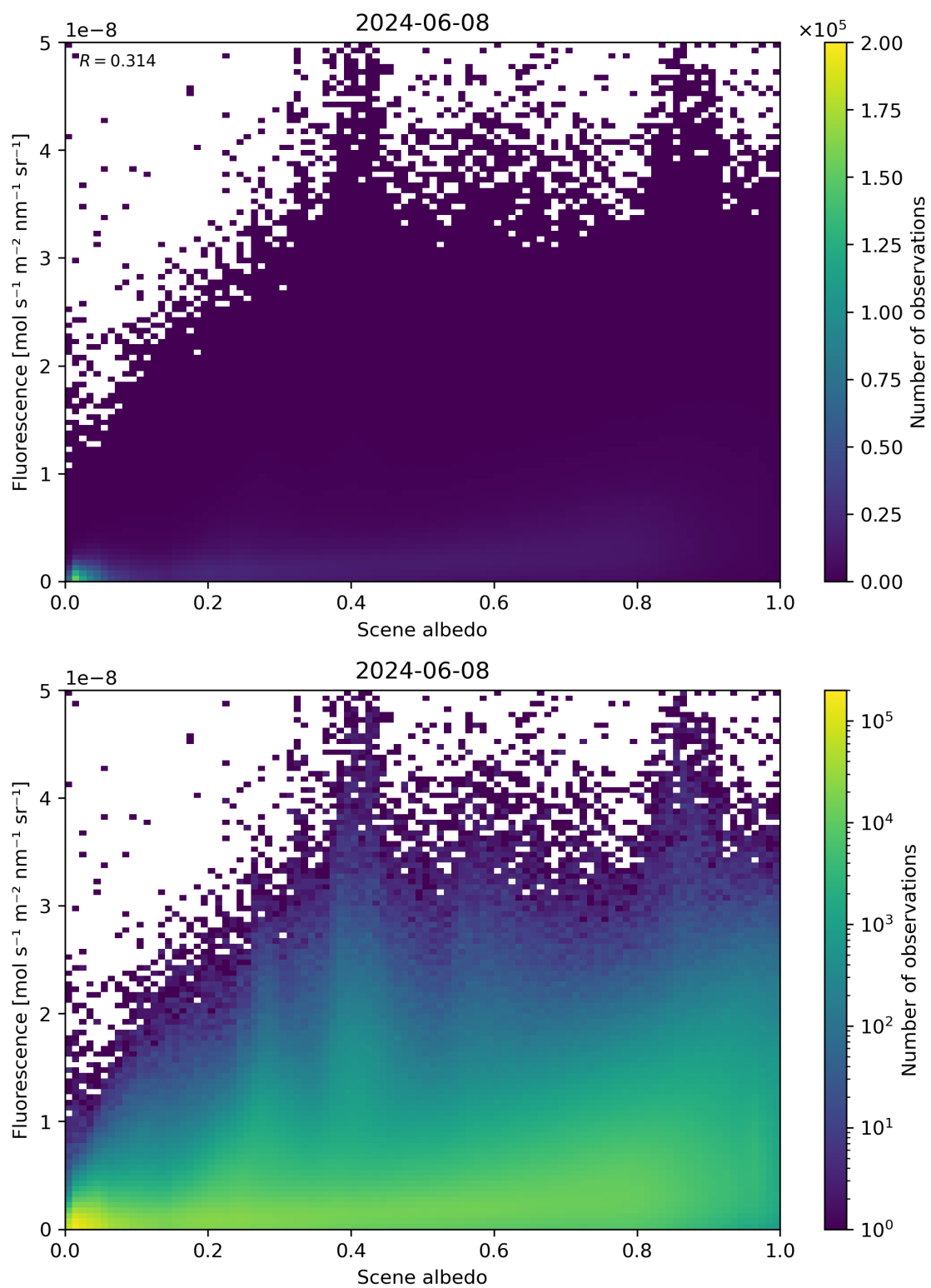
Figure 104: Scatter density plot of “Scene albedo” against “Fluorescence” for 2024-06-08 to 2024-06-09.
