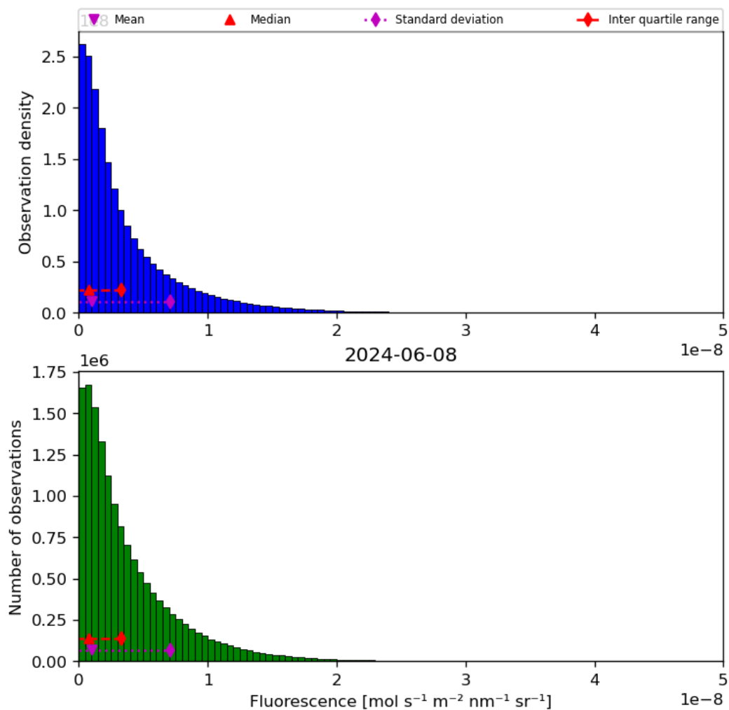
Figure 40: Histogram of “Fluorescence” for 2024-06-08 to 2024-06-09
