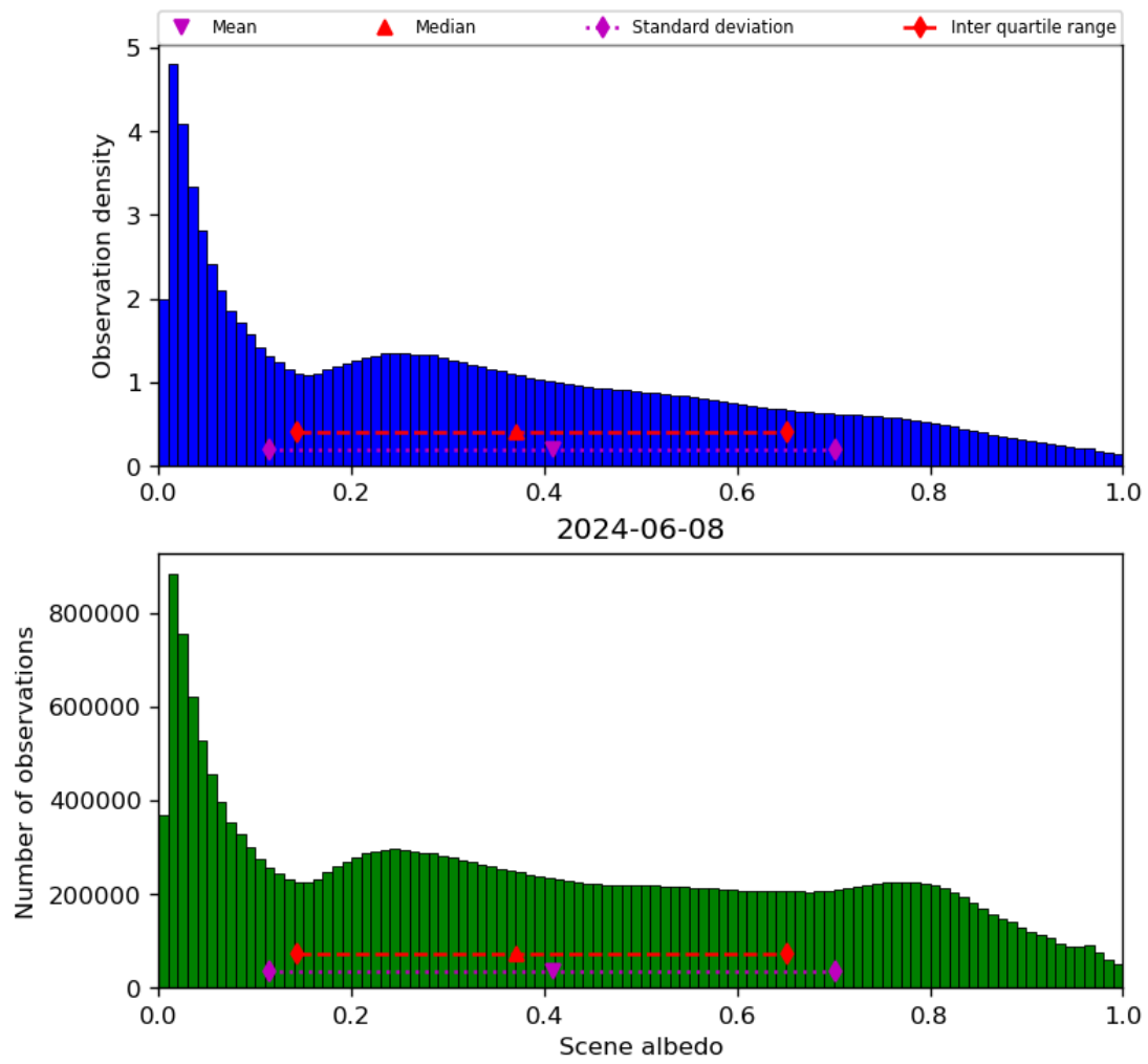
Figure 34: Histogram of “Scene albedo” for 2024-06-08 to 2024-06-09
