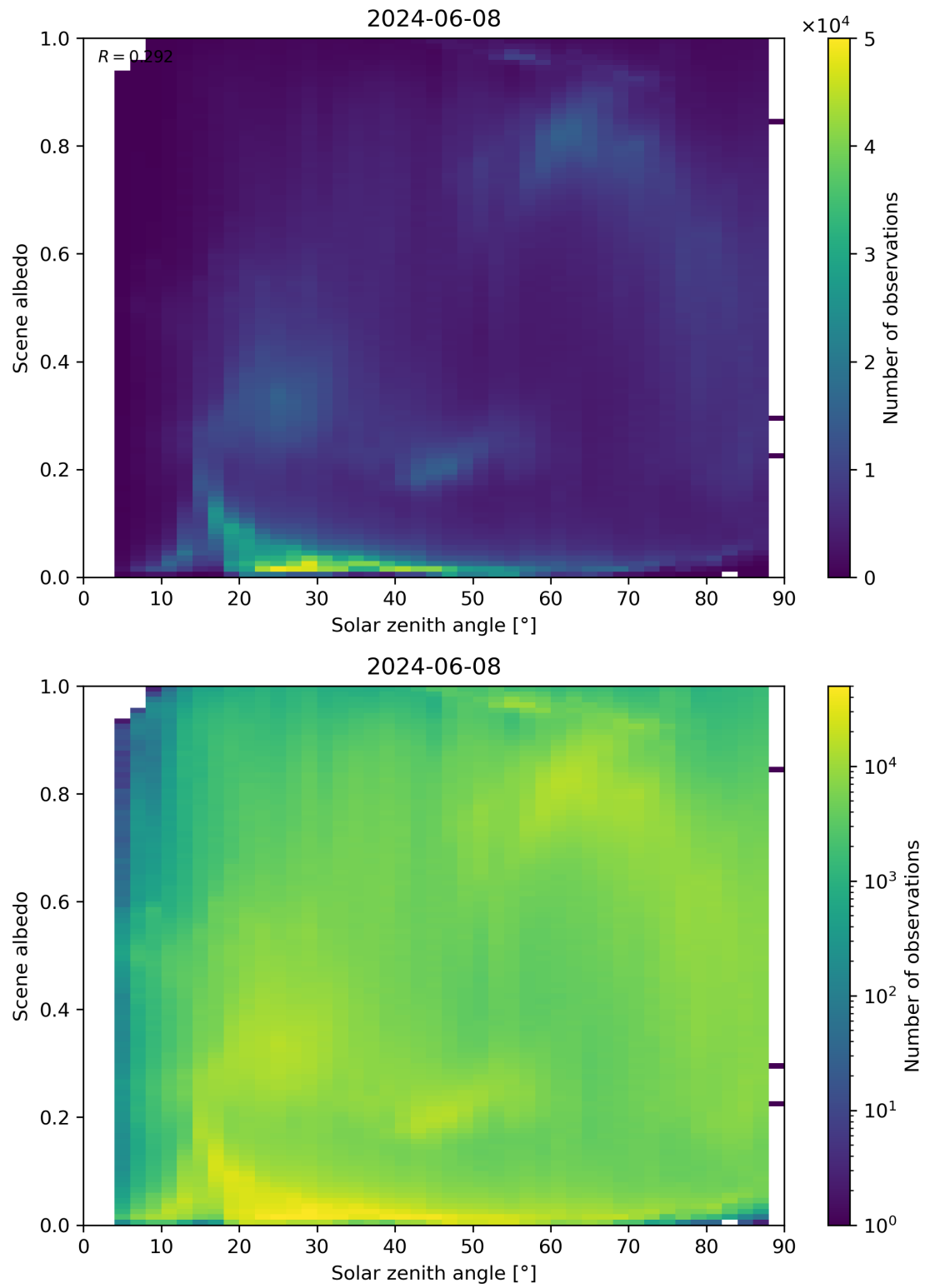
Figure 116: Scatter density plot of “Solar zenith angle” against “Scene albedo” for 2024-06-08 to 2024-06-09.
