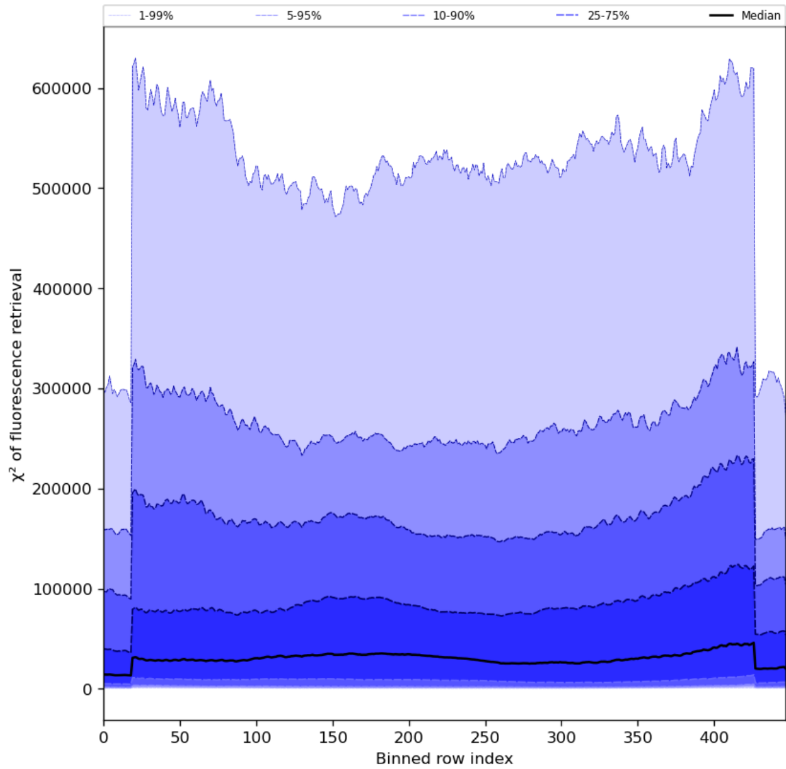
Figure 59: Along track statistics of “ \chi^2 of fluorescence retrieval” for 2024-06-08 to 2024-06-09
