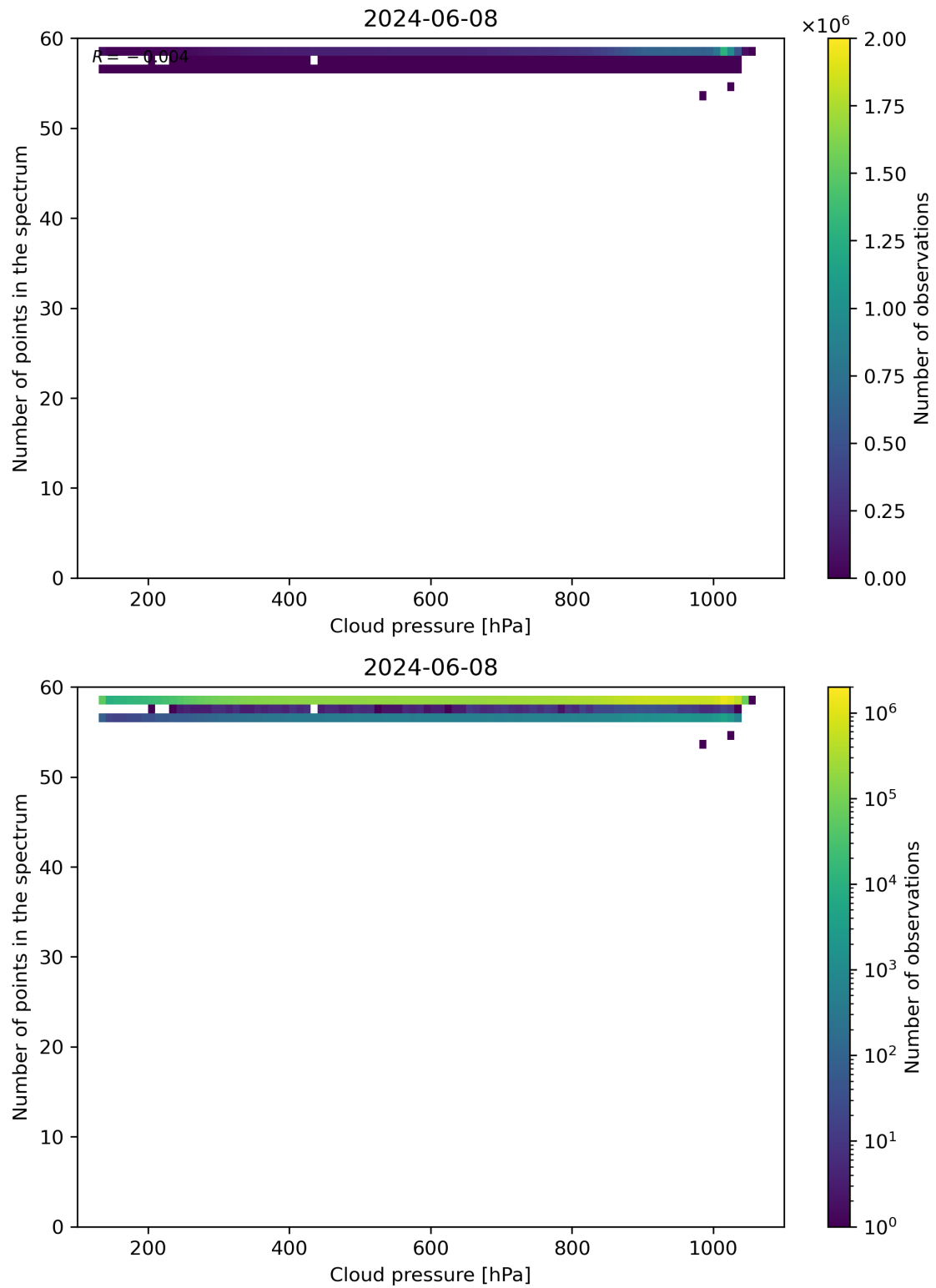
Figure 82: Scatter density plot of “Cloud pressure” against “Number of points in the spectrum” for 2024-06-08 to 2024-06-09.
