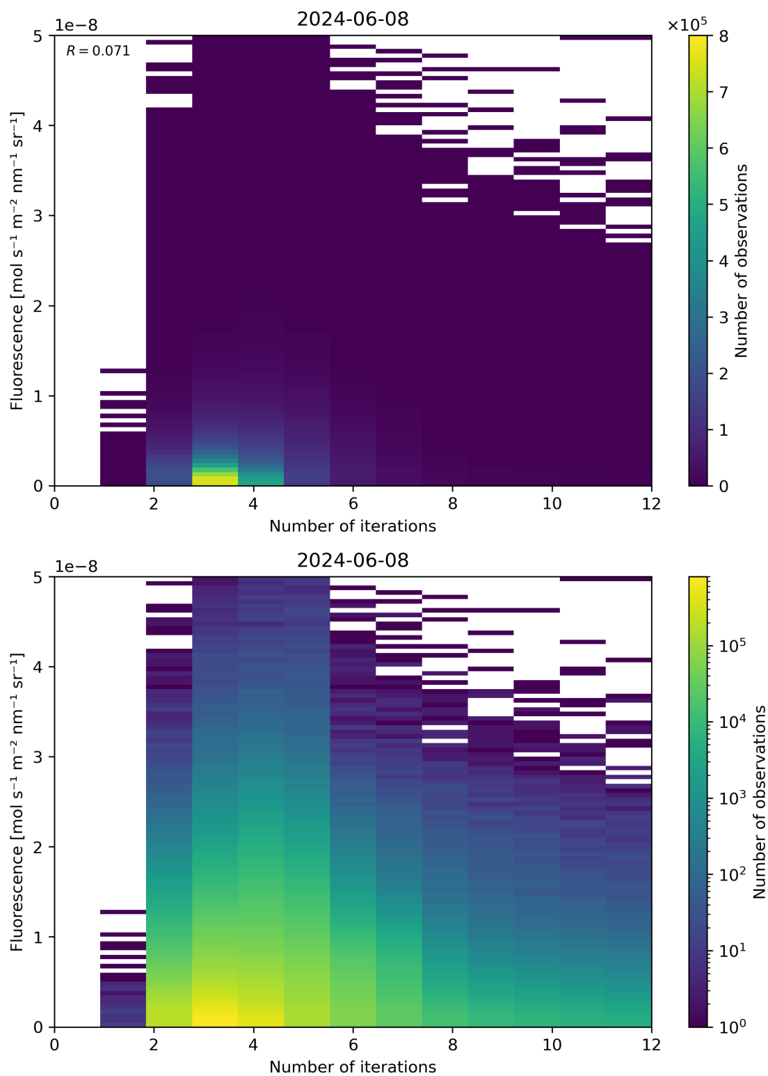
Figure 98: Scatter density plot of “Number of iterations” against “Fluorescence” for 2024-06-08 to 2024-06-09.
