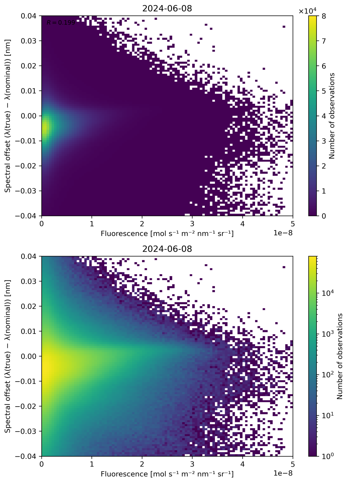
Figure 87: Scatter density plot of “Fluorescence” against “Spectral offset ( \lambda(\text{true}) - \lambda(\text{nominal}) )” for 2024-06-08 to 2024-06-09.
