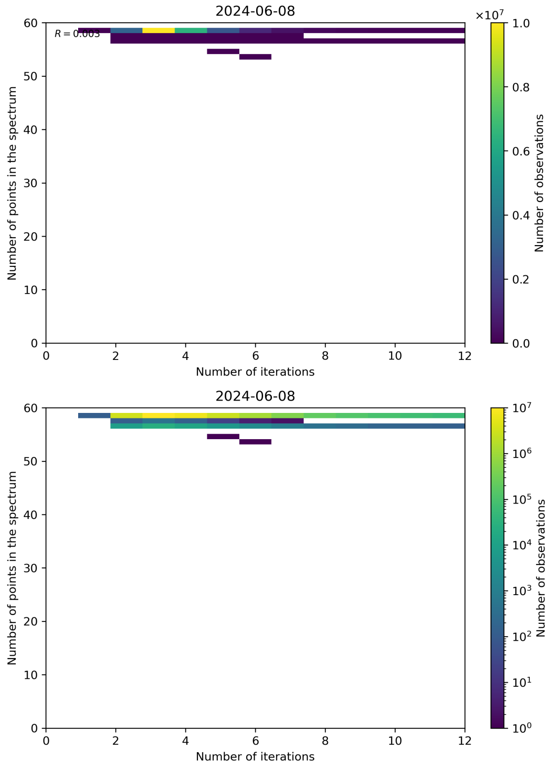
Figure 99: Scatter density plot of “Number of iterations” against “Number of points in the spectrum” for 2024-06-08 to 2024-06-09.
