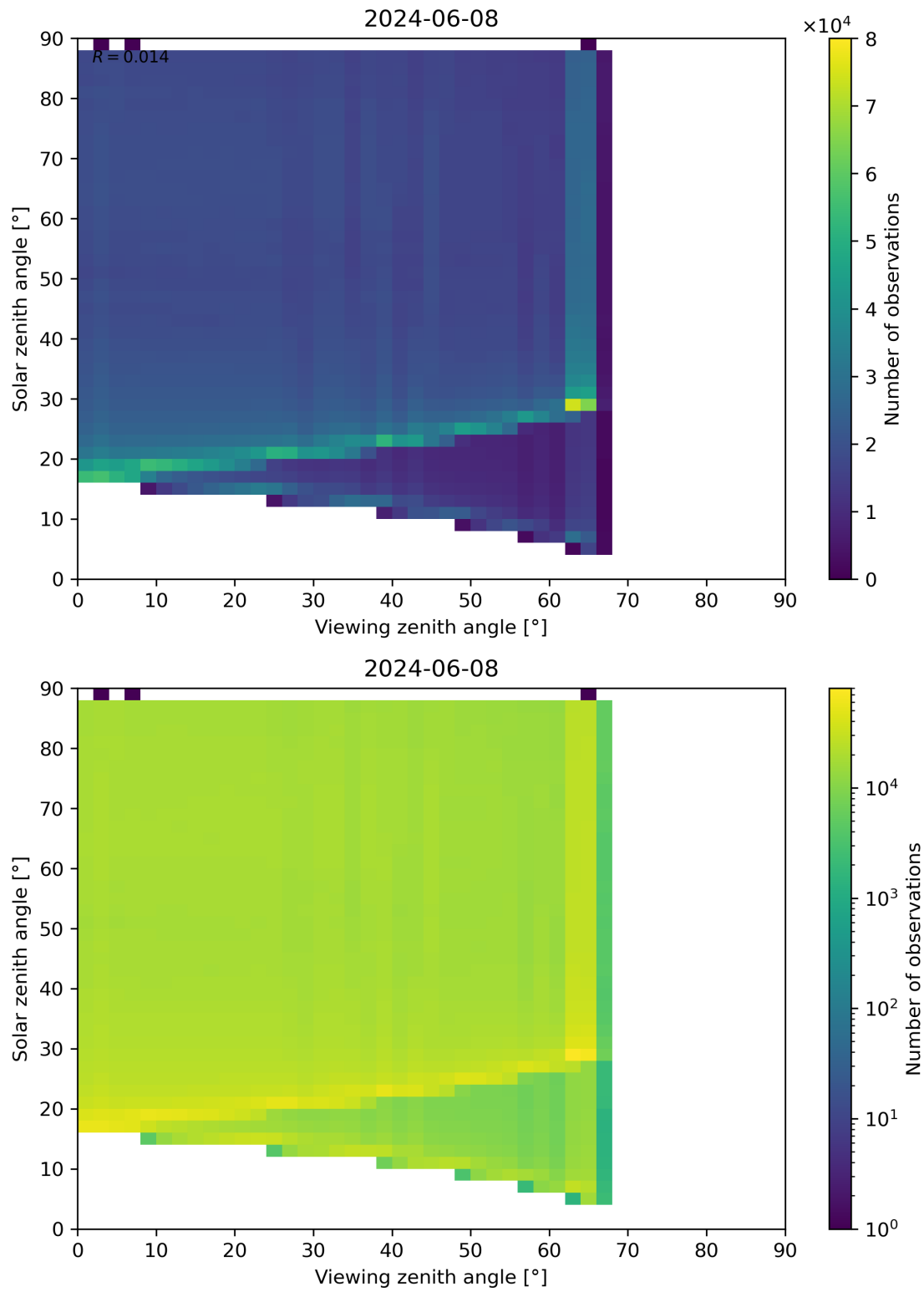
Figure 127: Scatter density plot of “Viewing zenith angle” against “Solar zenith angle” for 2024-06-08 to 2024-06-09.
