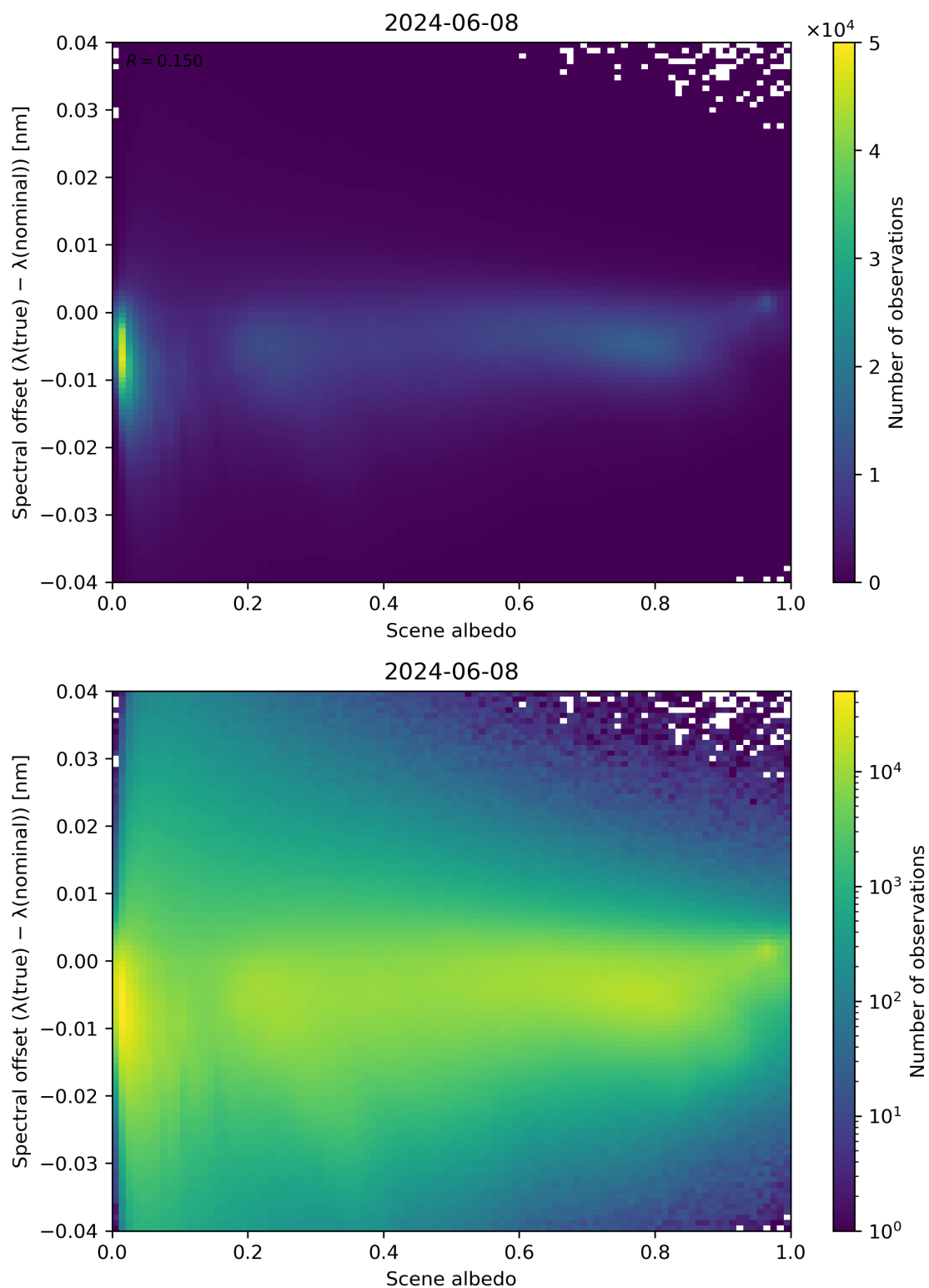
Figure 107: Scatter density plot of “Scene albedo” against “Spectral offset ( \lambda(\text{true}) - \lambda(\text{nominal}) )” for 2024-06-08 to 2024-06-09.
