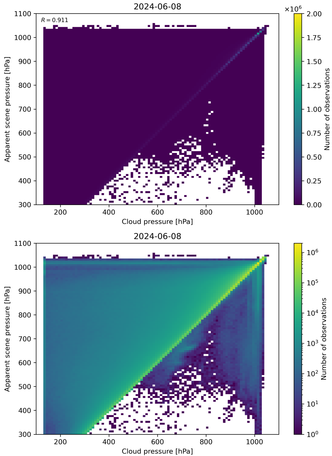
Figure 77: Scatter density plot of “Cloud pressure” against “Apparent scene pressure” for 2024-06-08 to 2024-06-09.
