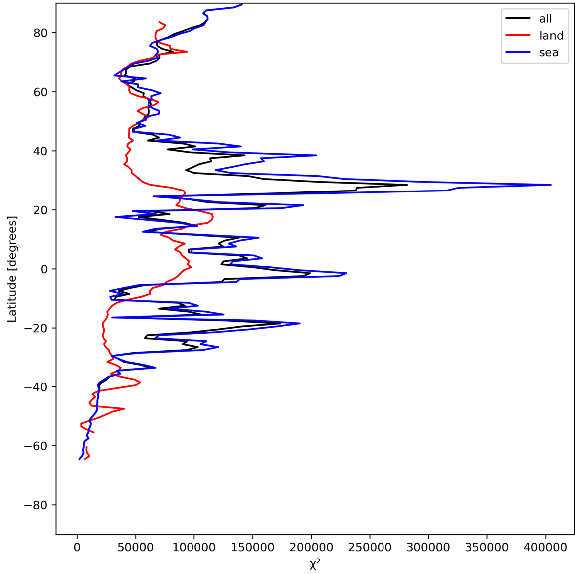
Figure 21: Zonal average of “ \chi^2 ” for 2024-06-08 to 2024-06-09.
