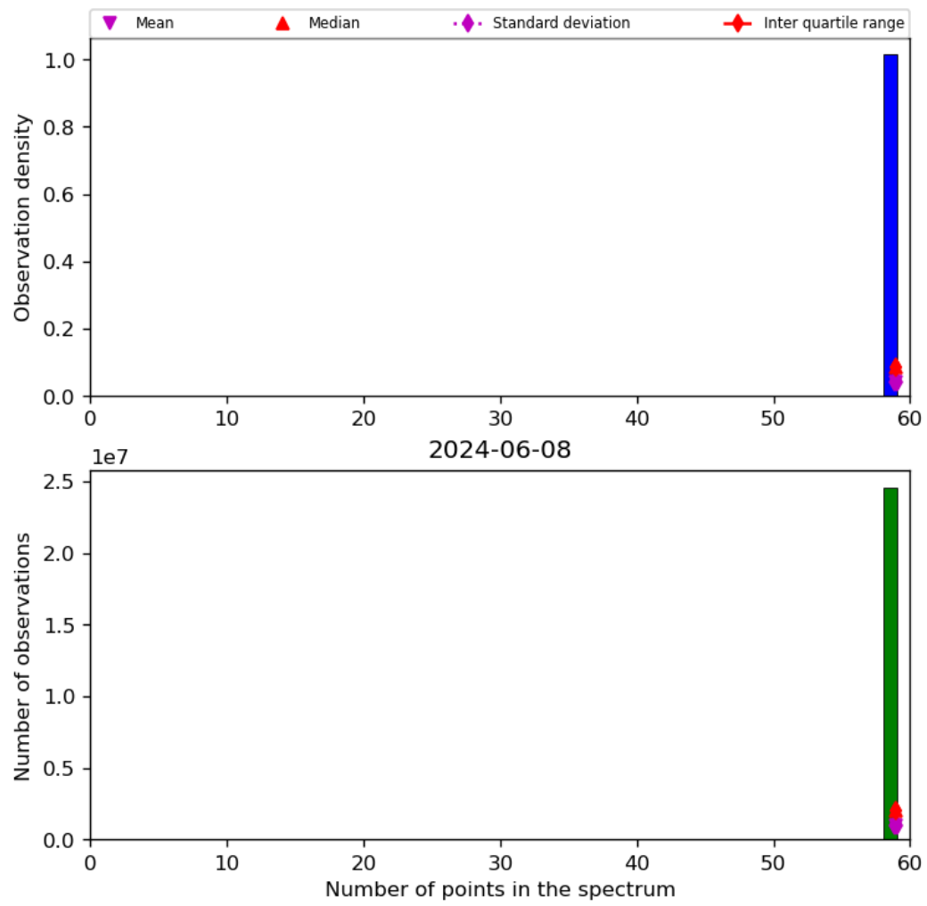
Figure 44: Histogram of “Number of points in the spectrum” for 2024-06-08 to 2024-06-09
