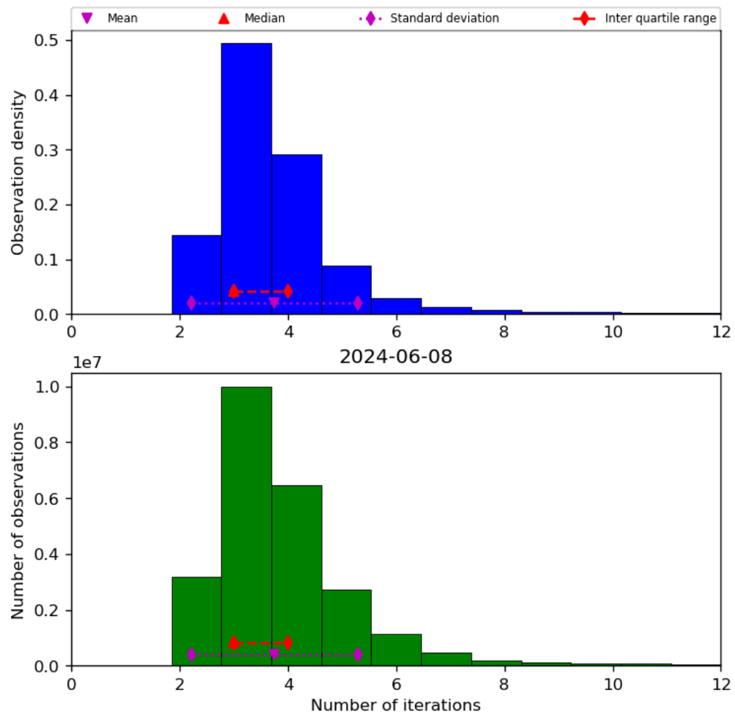
Figure 39: Histogram of “Number of iterations” for 2024-06-08 to 2024-06-09
