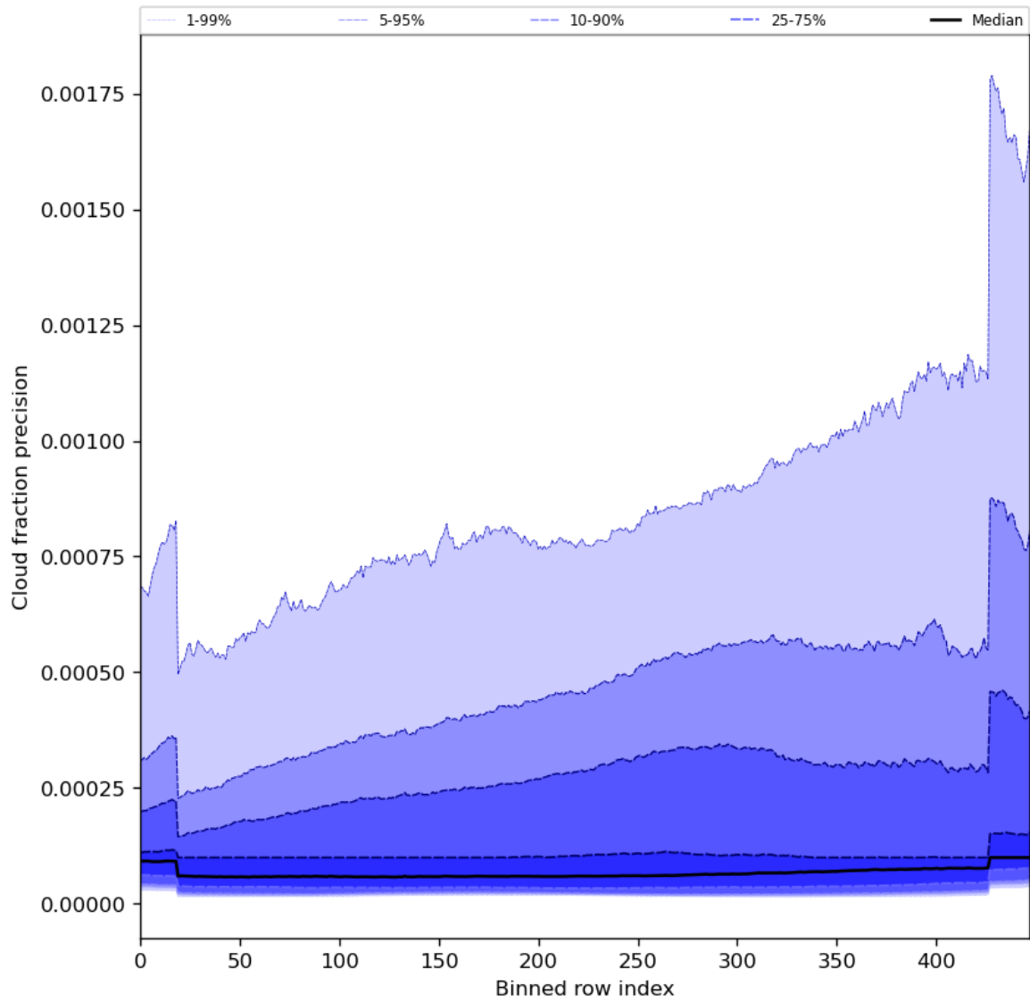
Figure 50: Along track statistics of “Cloud fraction precision” for 2024-06-08 to 2024-06-09
