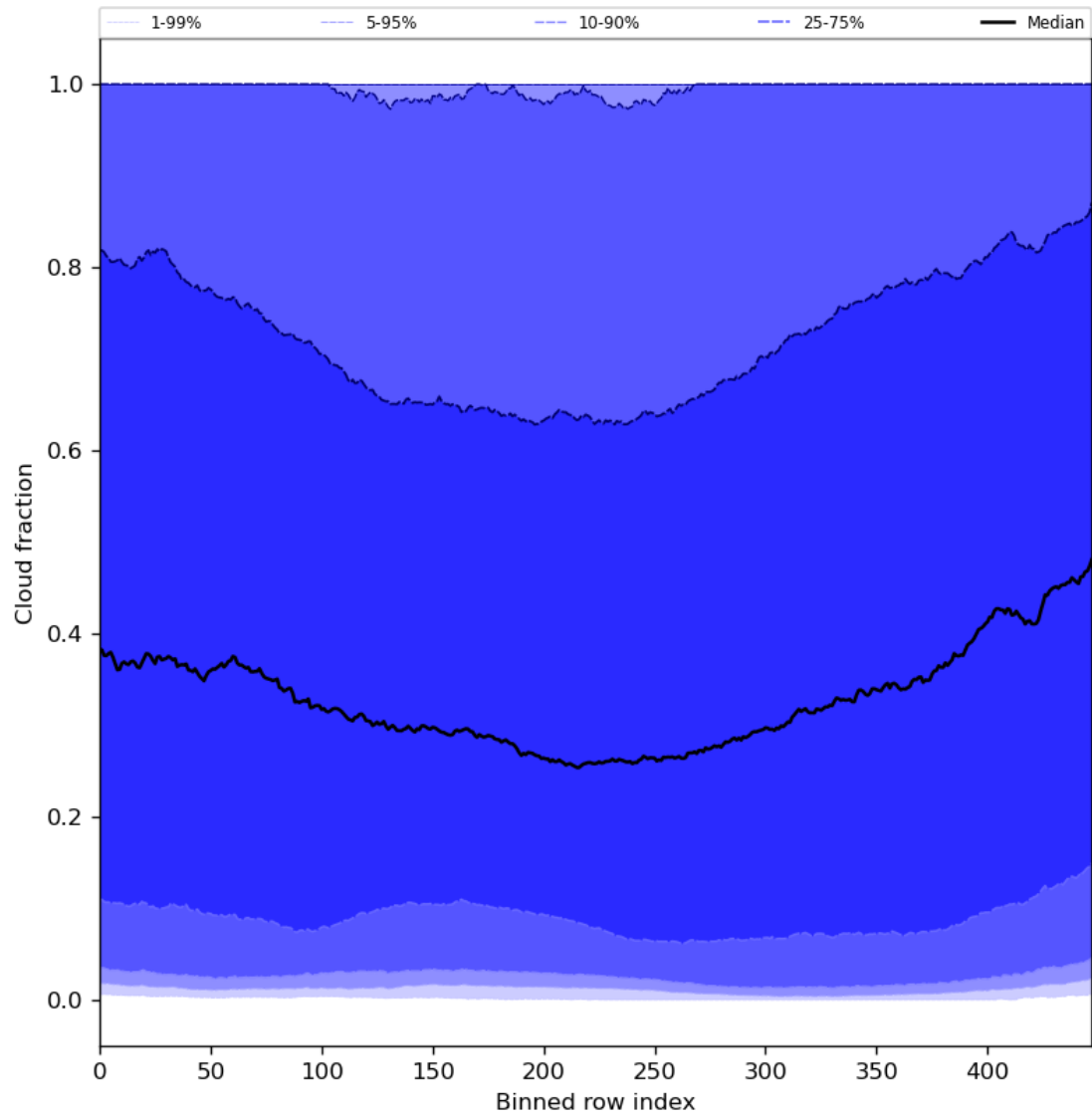
Figure 49: Along track statistics of “Cloud fraction” for 2024-06-08 to 2024-06-09
