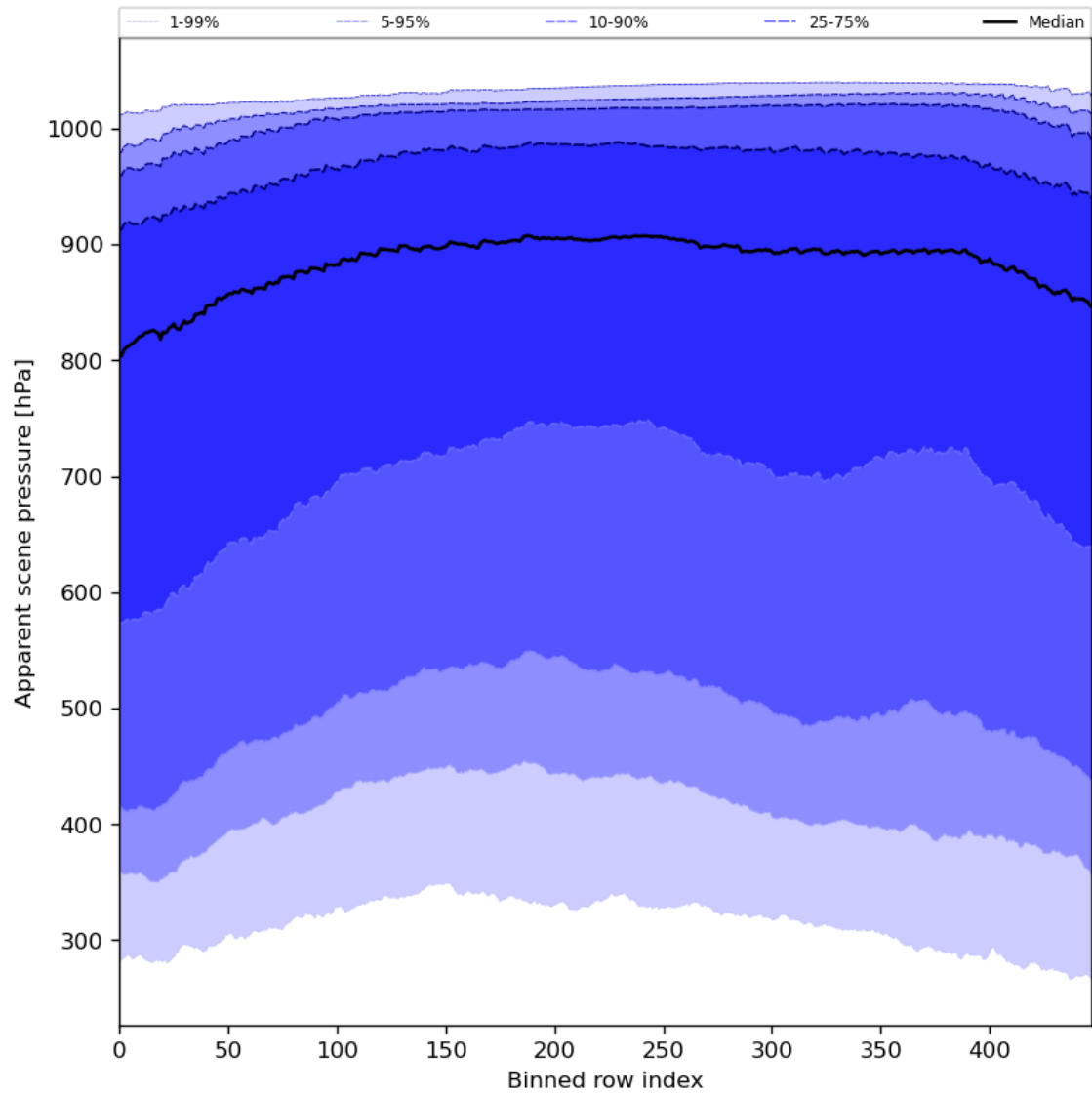
Figure 53: Along track statistics of “Apparent scene pressure” for 2024-06-08 to 2024-06-09
