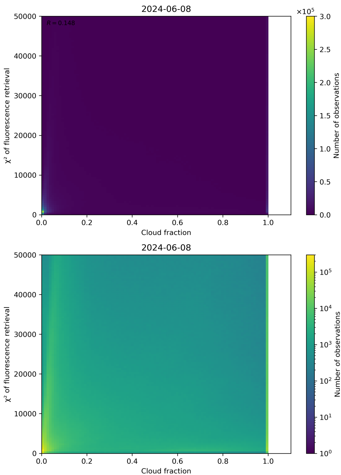
Figure 71: Scatter density plot of “Cloud fraction” against “ \chi^2 of fluorescence retrieval” for 2024-06-08 to 2024-06-09.
