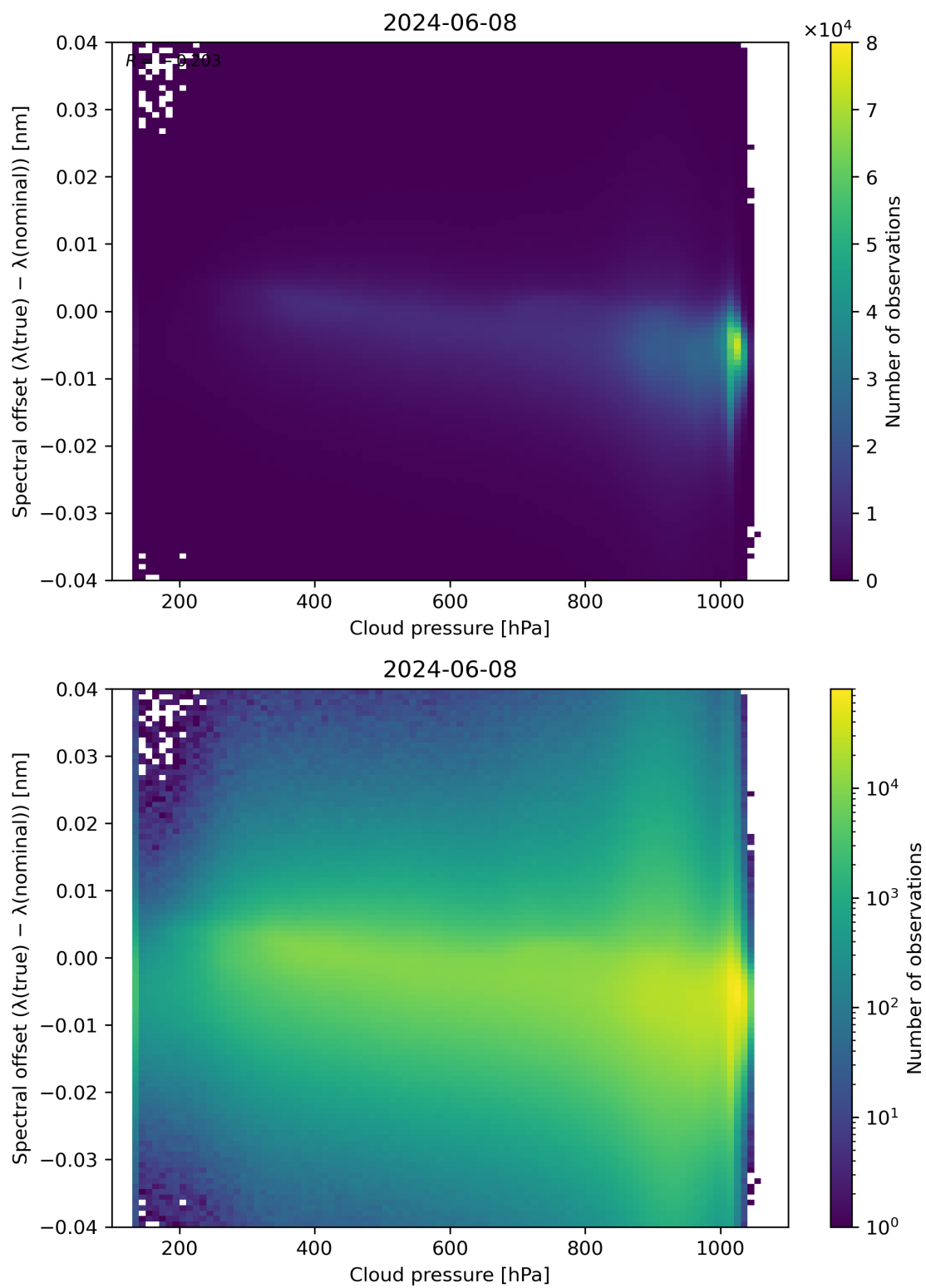
Figure 84: Scatter density plot of “Cloud pressure” against “Spectral offset ( \lambda(\text{true}) - \lambda(\text{nominal}) )” for 2024-06-08 to 2024-06-09.
