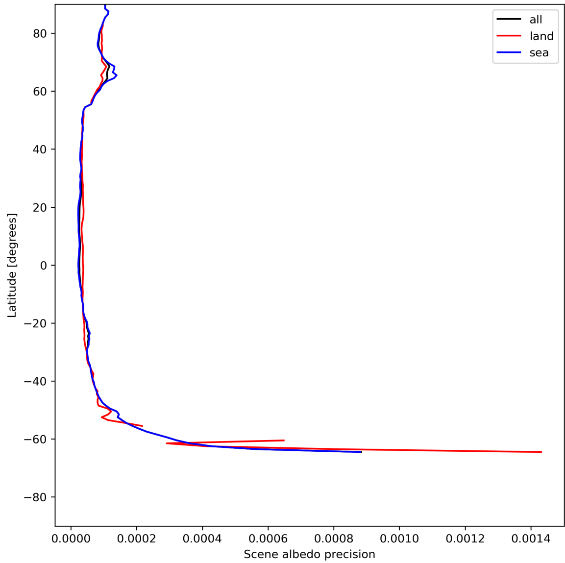
Figure 18: Zonal average of “Scene albedo precision” for 2024-06-08 to 2024-06-09.
