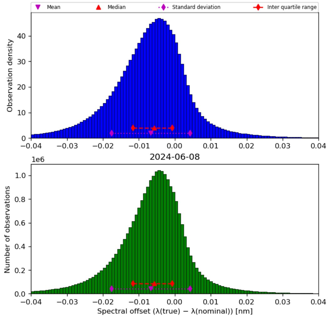
Figure 45: Histogram of “Spectral offset ( \lambda(\text{true}) - \lambda(\text{nominal}) )” for 2024-06-08 to 2024-06-09
