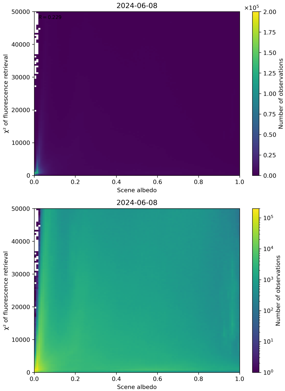
Figure 103: Scatter density plot of “Scene albedo” against “ \chi^2 of fluorescence retrieval” for 2024-06-08 to 2024-06-09.
