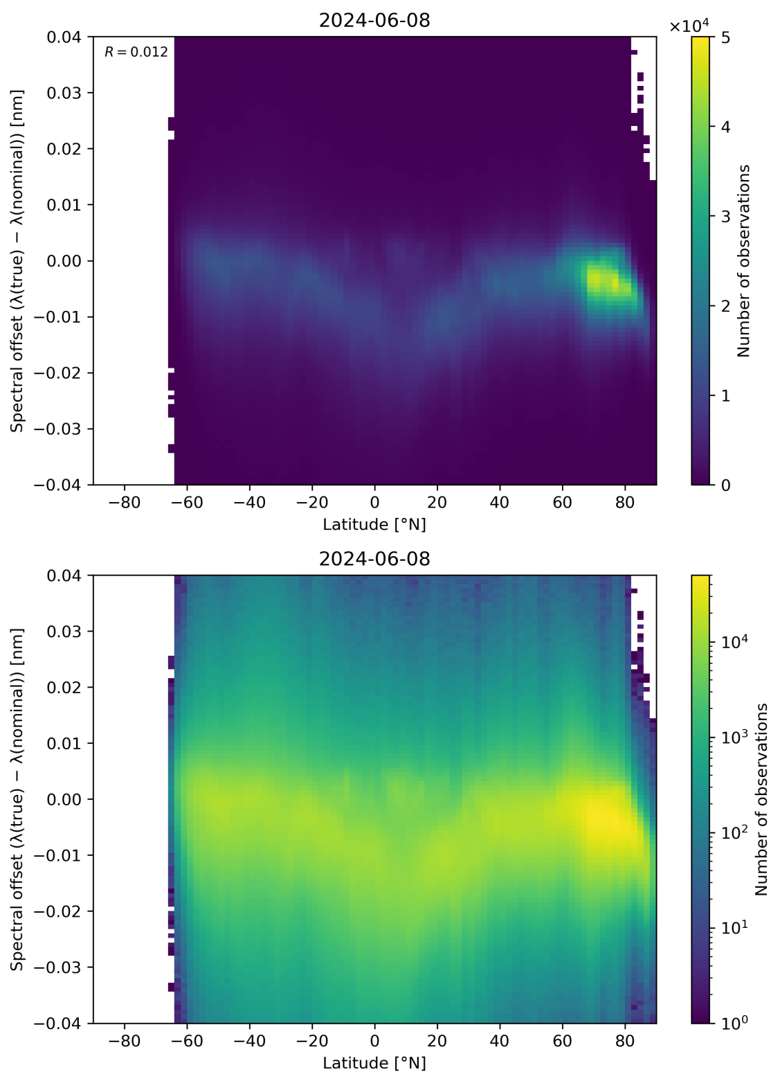
Figure 96: Scatter density plot of “Latitude” against “Spectral offset ( \lambda(\text{true}) - \lambda(\text{nominal}) )” for 2024-06-08 to 2024-06-09.
