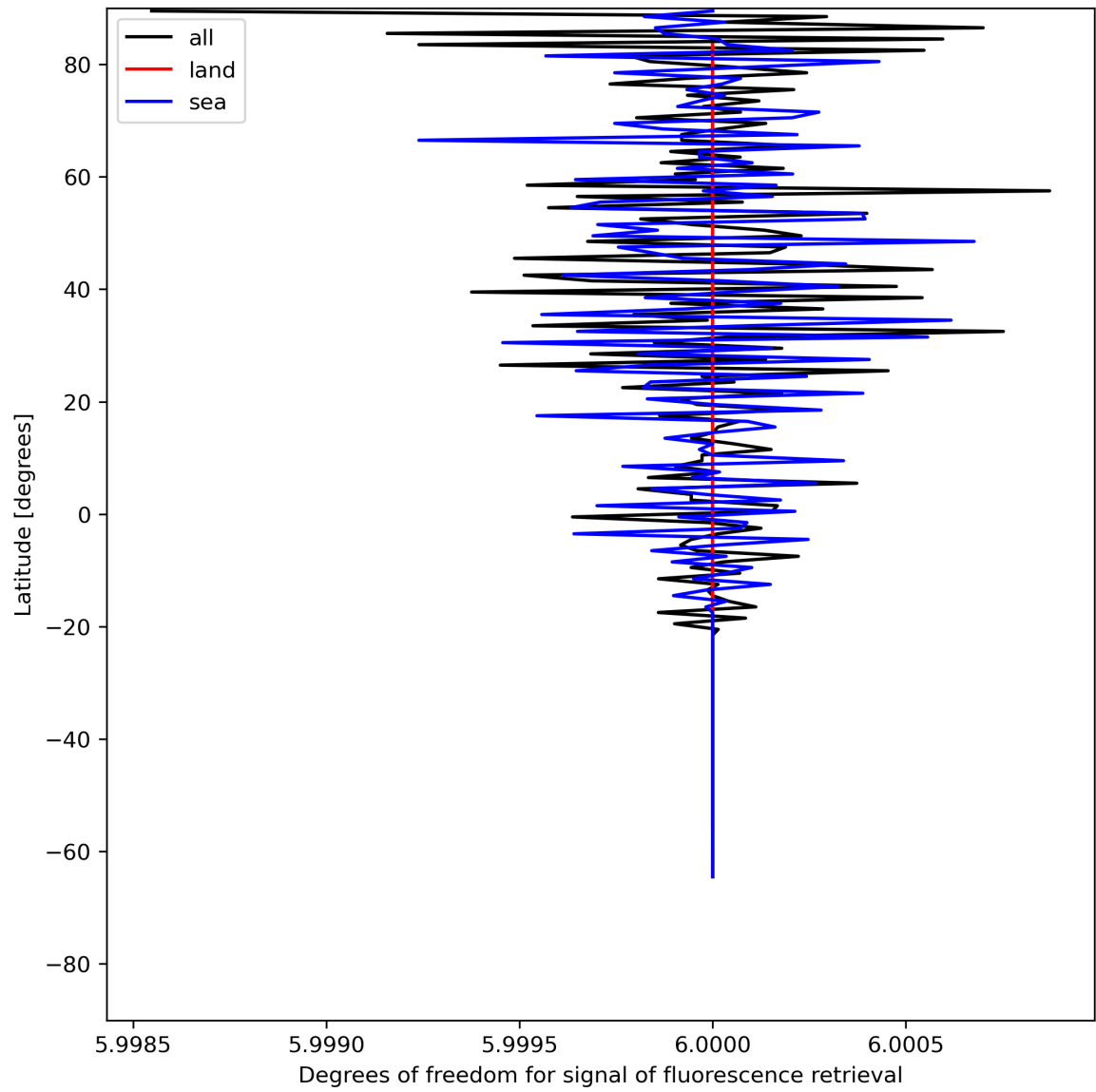
Figure 26: Zonal average of “Degrees of freedom for signal of fluorescence retrieval” for 2024-06-08 to 2024-06-09.
