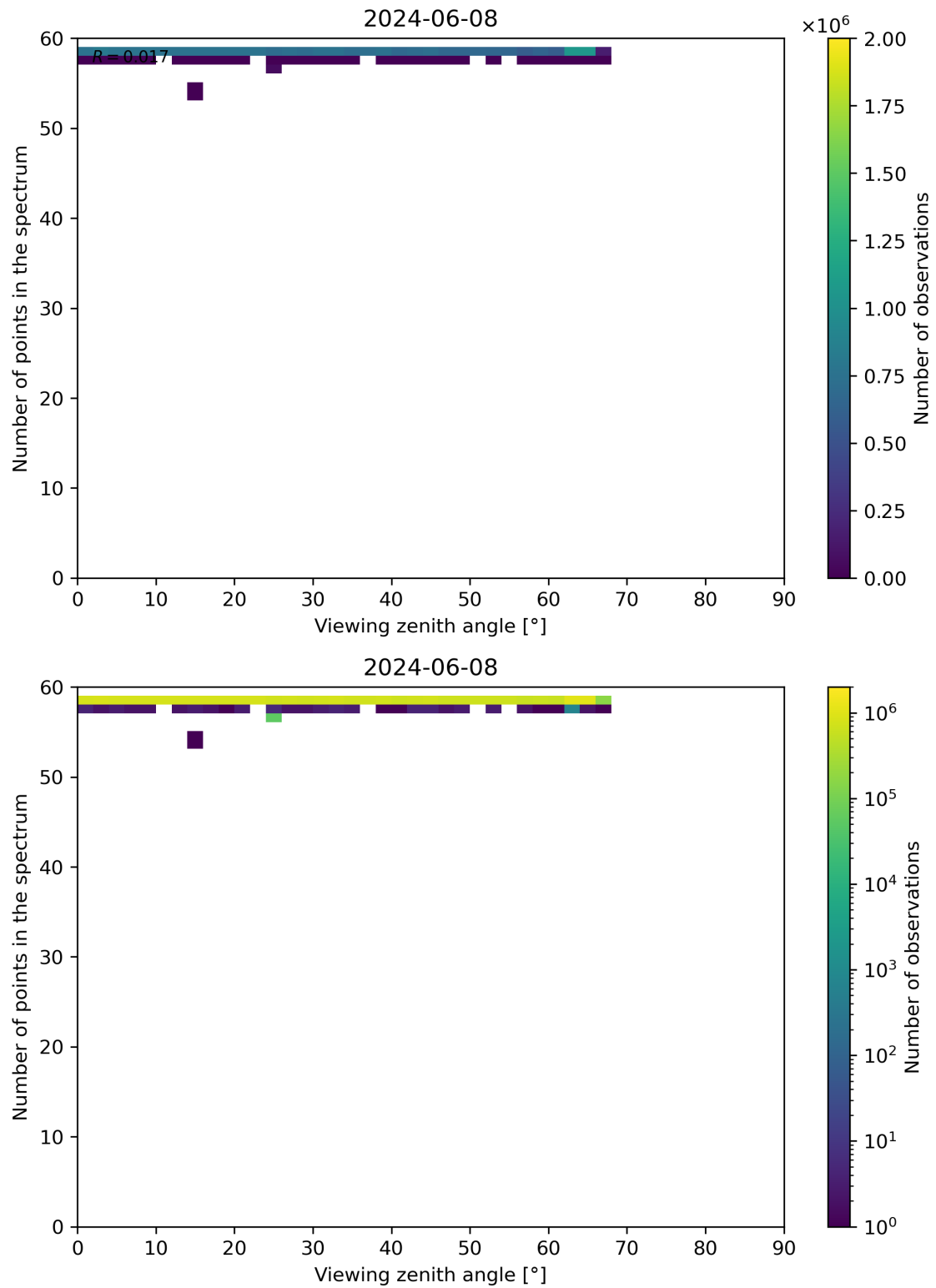
Figure 125: Scatter density plot of “Viewing zenith angle” against “Number of points in the spectrum” for 2024-06-08 to 2024-06-09.
