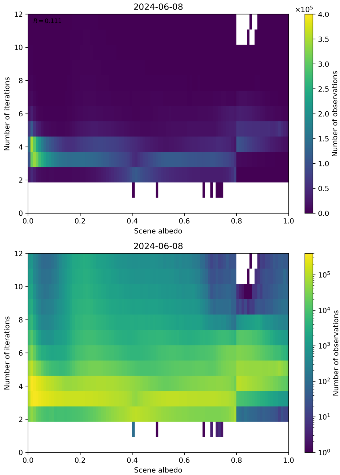
Figure 105: Scatter density plot of “Scene albedo” against “Number of iterations” for 2024-06-08 to 2024-06-09.
