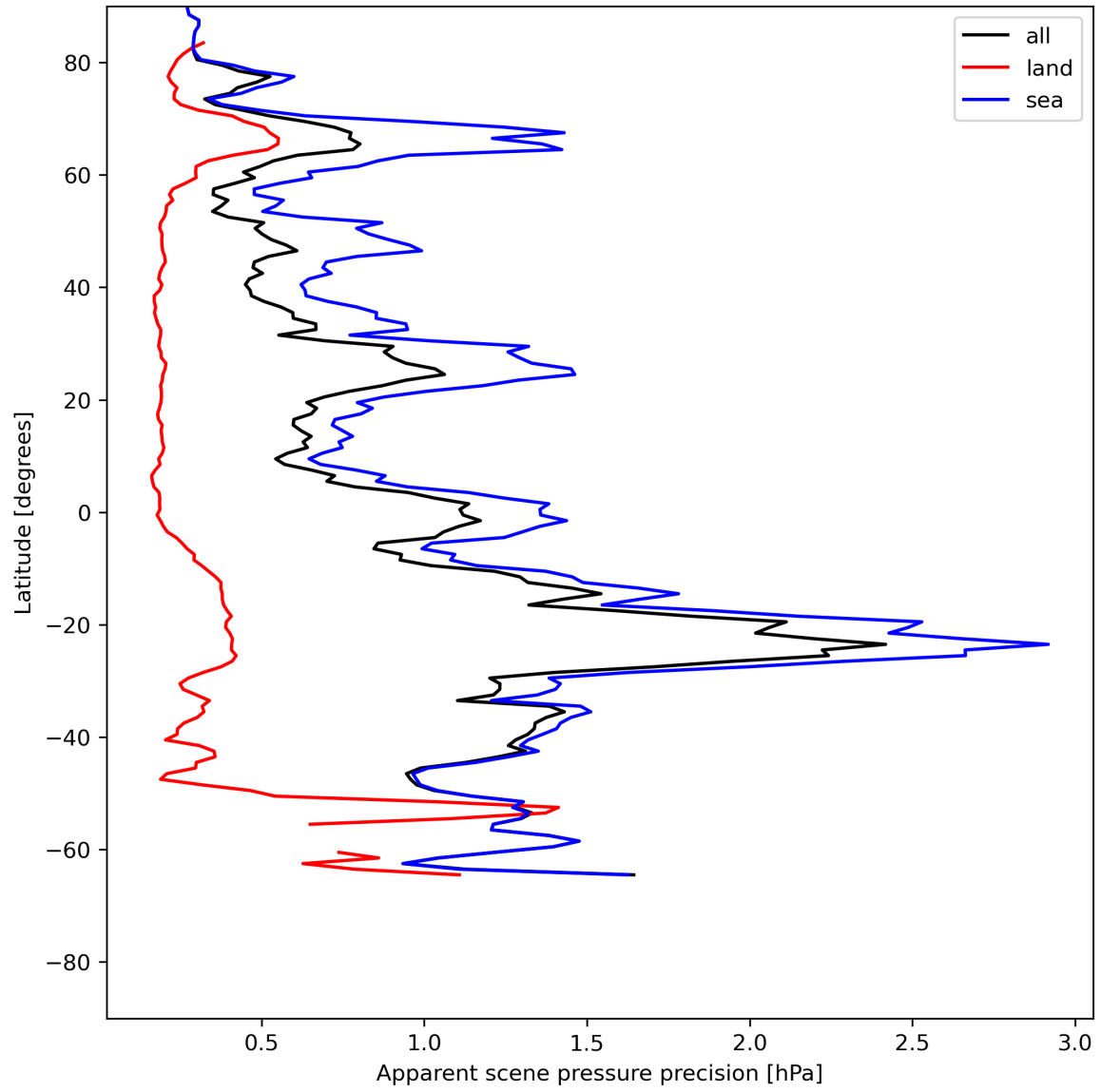
Figure 20: Zonal average of “Apparent scene pressure precision” for 2024-06-08 to 2024-06-09.
