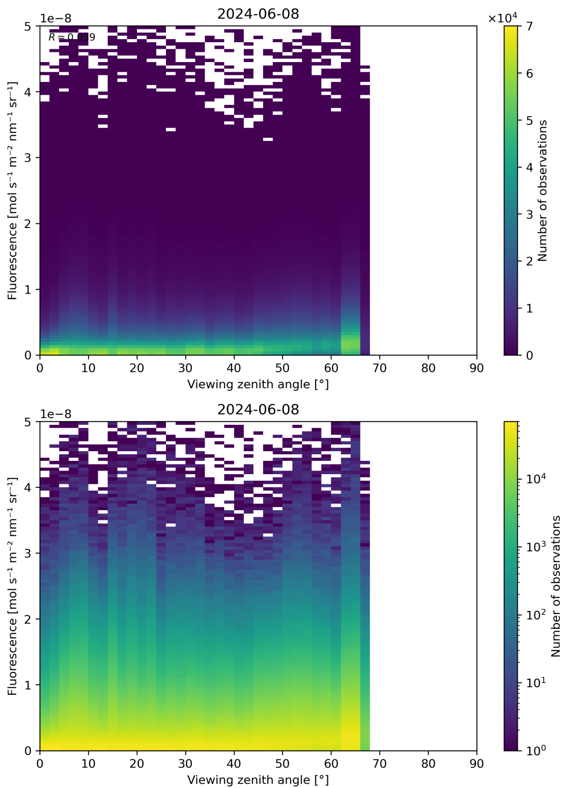
Figure 122: Scatter density plot of “Viewing zenith angle” against “Fluorescence” for 2024-06-08 to 2024-06-09.
