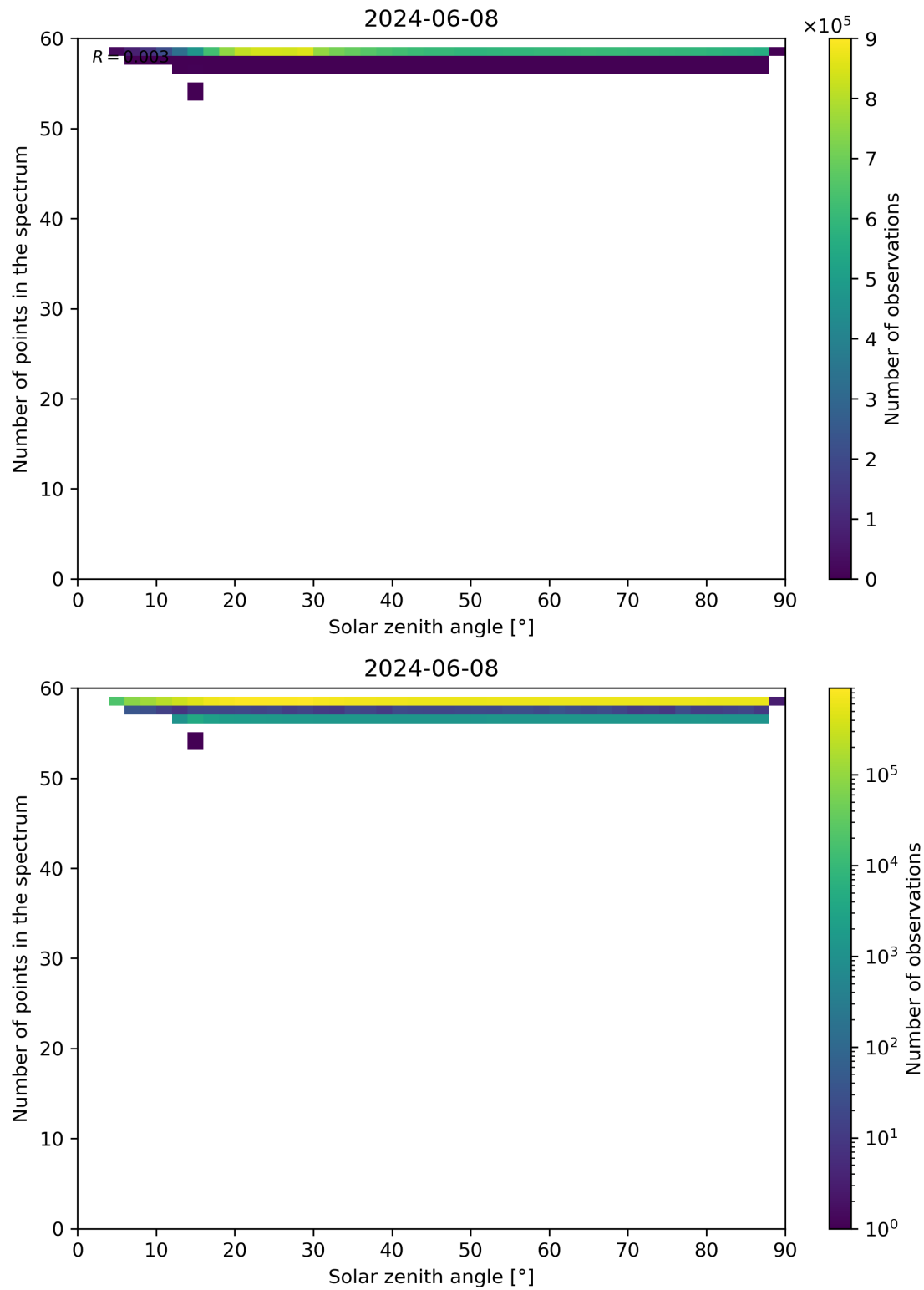
Figure 115: Scatter density plot of “Solar zenith angle” against “Number of points in the spectrum” for 2024-06-08 to 2024-06-09.
