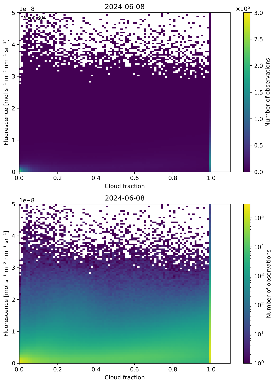
Figure 72: Scatter density plot of "Cloud fraction" against "Fluorescence" for 2024-06-08 to 2024-06-09.
