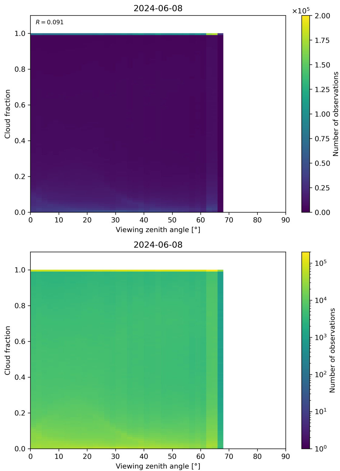
Figure 120: Scatter density plot of “Viewing zenith angle” against “Cloud fraction” for 2024-06-08 to 2024-06-09.
