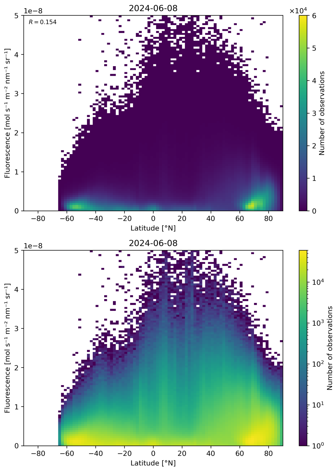
Figure 92: Scatter density plot of “Latitude” against “Fluorescence” for 2024-06-08 to 2024-06-09.
