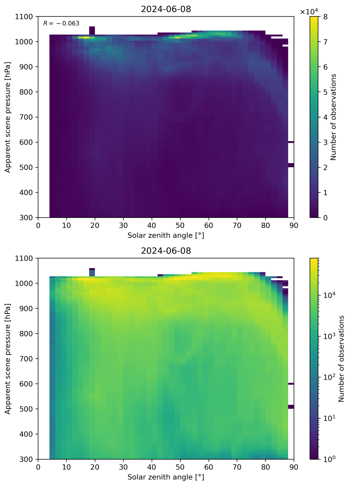
Figure 108: Scatter density plot of “Solar zenith angle” against “Apparent scene pressure” for 2024-06-08 to 2024-06-09.
