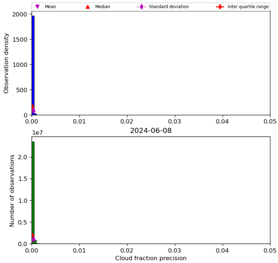
Figure 33: Histogram of “Cloud fraction precision” for 2024-06-08 to 2024-06-09
