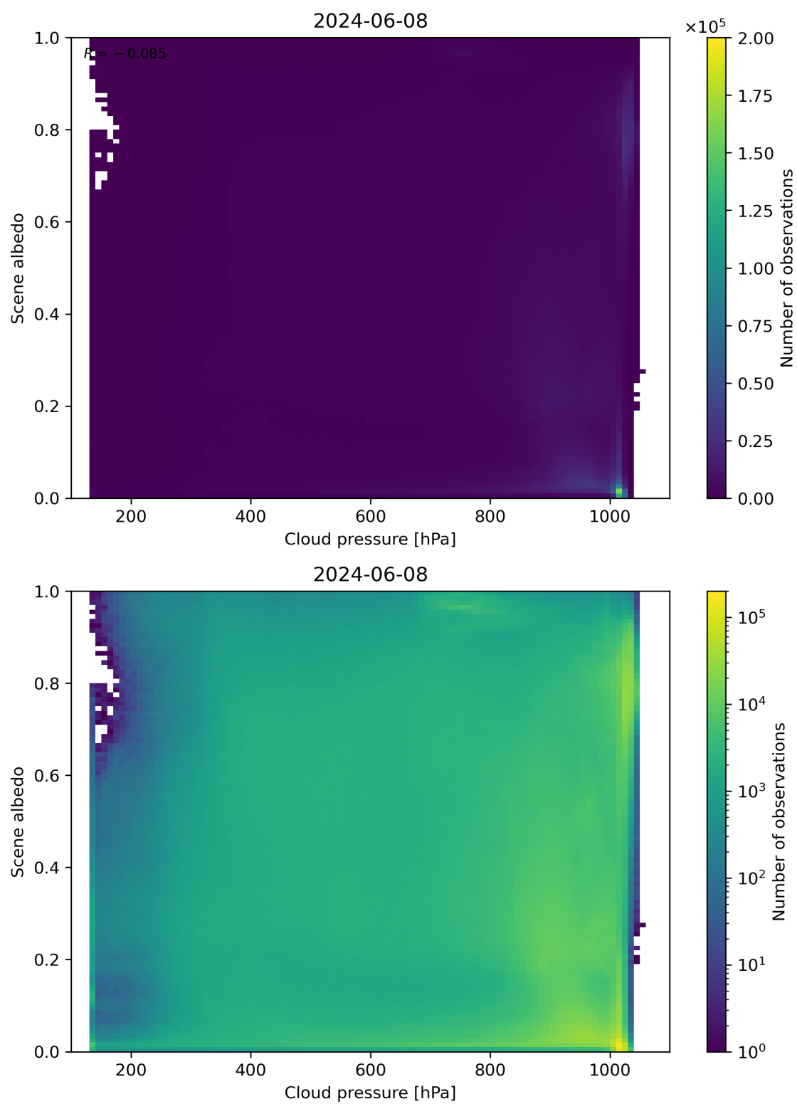
Figure 83: Scatter density plot of “Cloud pressure” against “Scene albedo” for 2024-06-08 to 2024-06-09.
