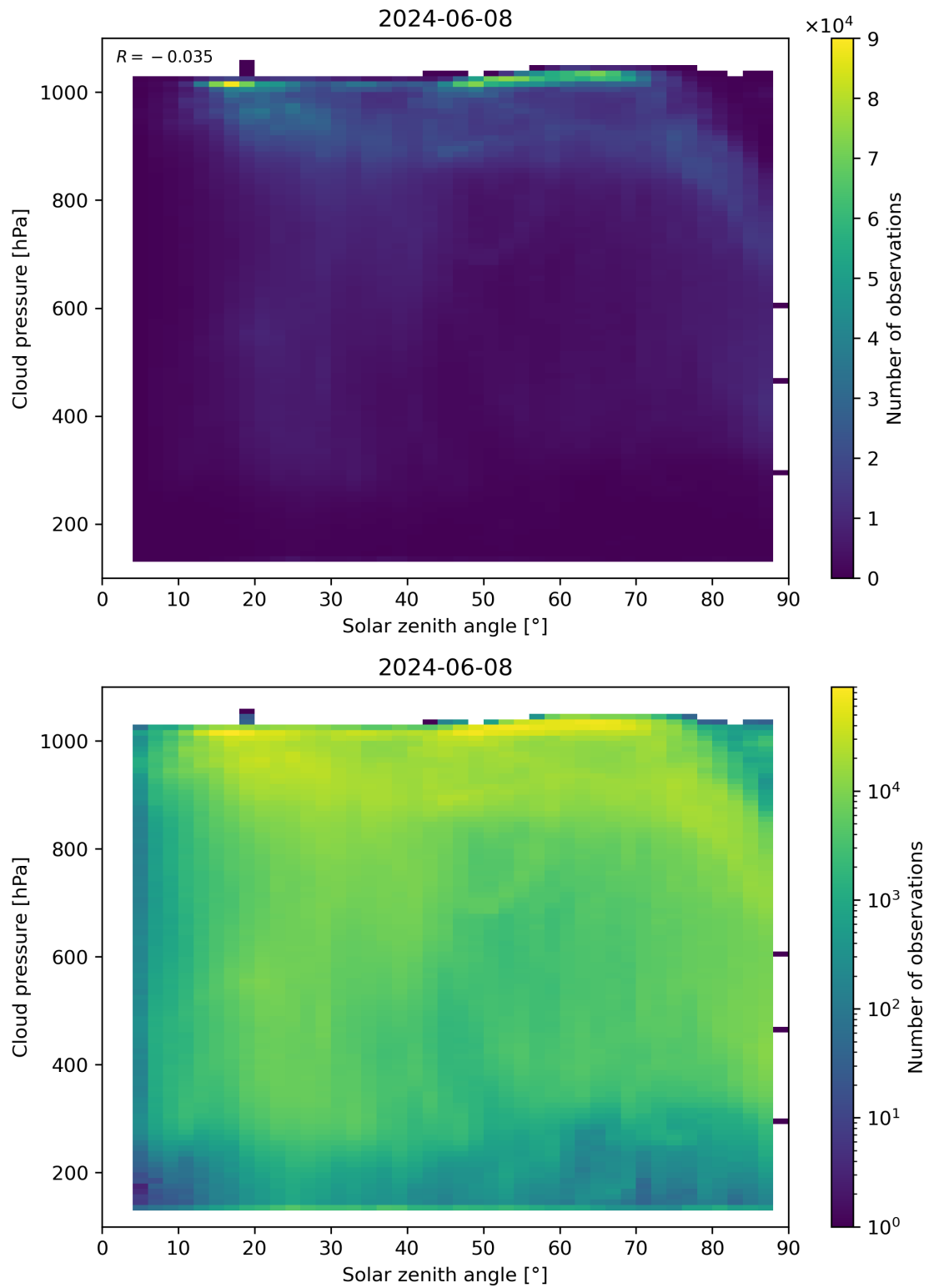
Figure 111: Scatter density plot of “Solar zenith angle” against “Cloud pressure” for 2024-06-08 to 2024-06-09.
