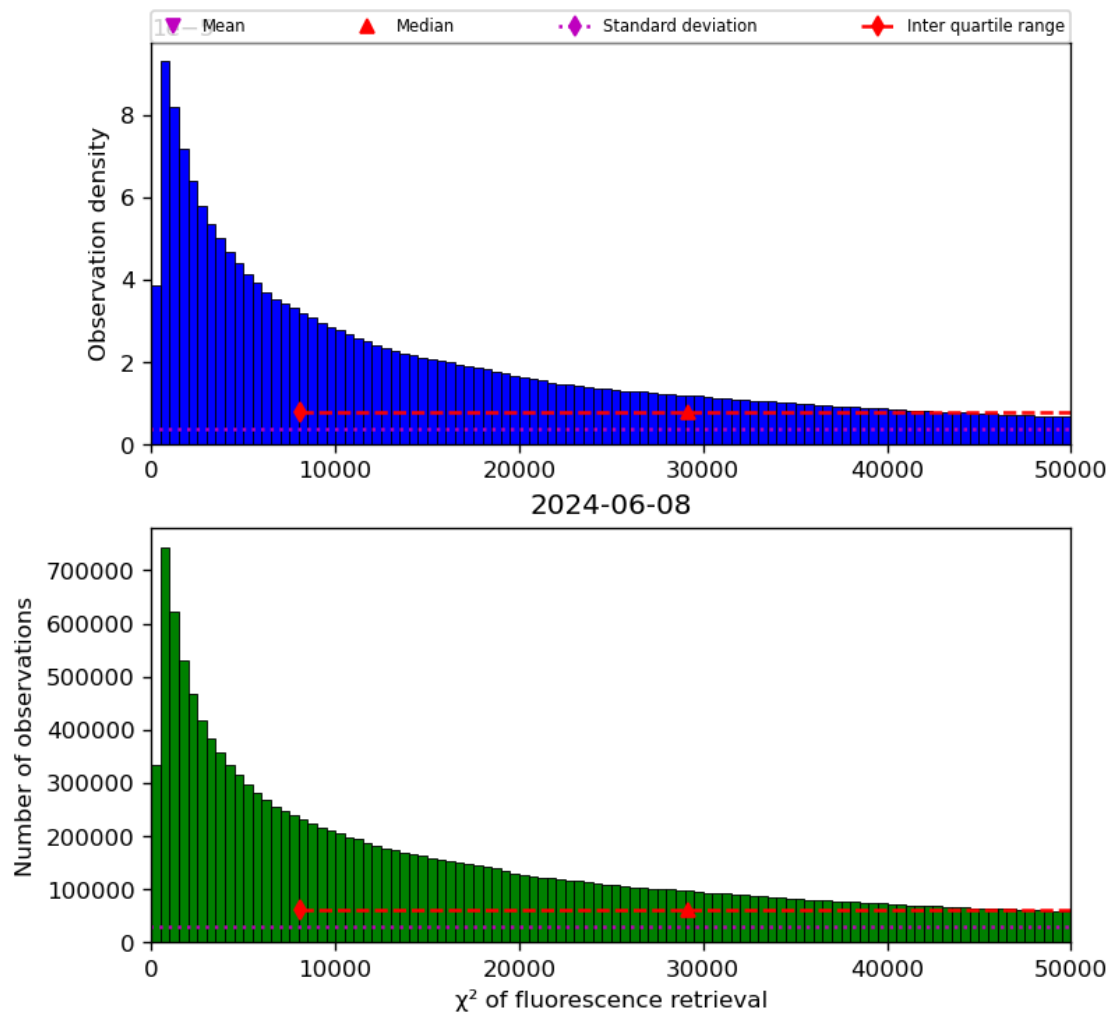
Figure 42: Histogram of “ \chi^2 of fluorescence retrieval” for 2024-06-08 to 2024-06-09
