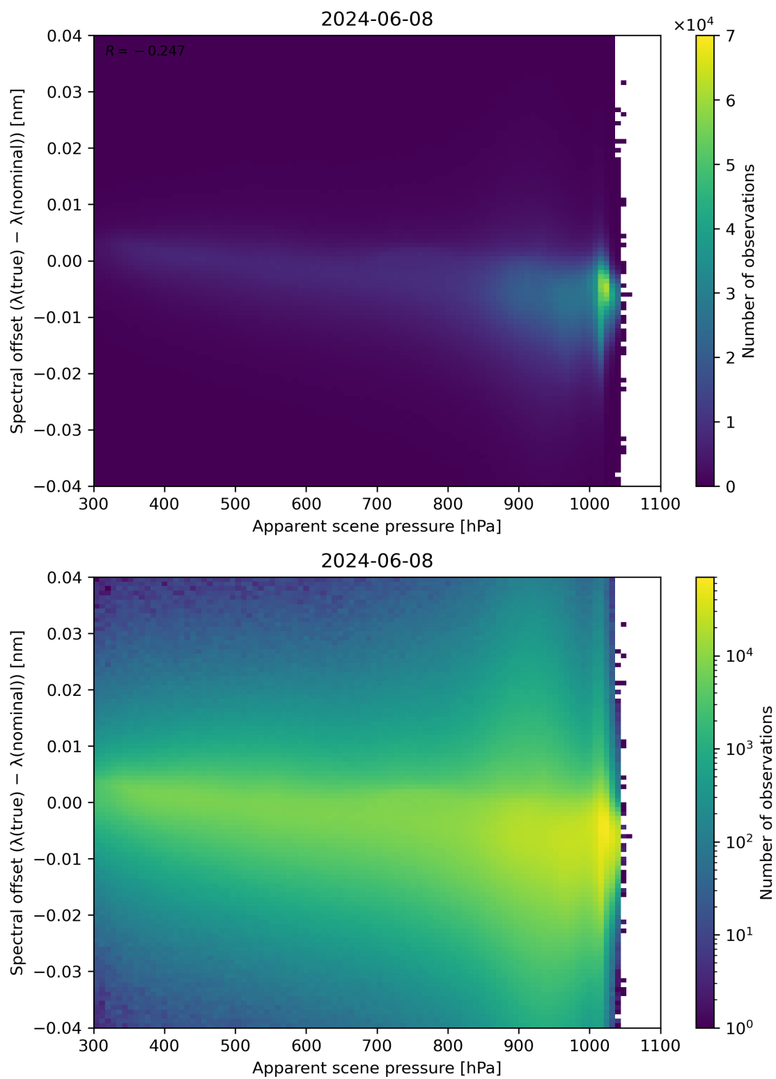
Figure 67: Scatter density plot of “Apparent scene pressure” against “Spectral offset ( \lambda(\text{true}) - \lambda(\text{nominal}) )” for 2024-06-08 to 2024-06-09.
