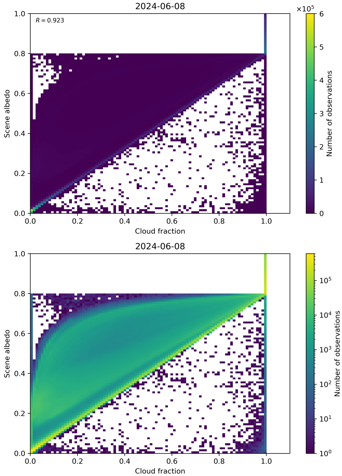
Figure 75: Scatter density plot of “Cloud fraction” against “Scene albedo” for 2024-06-08 to 2024-06-09.
