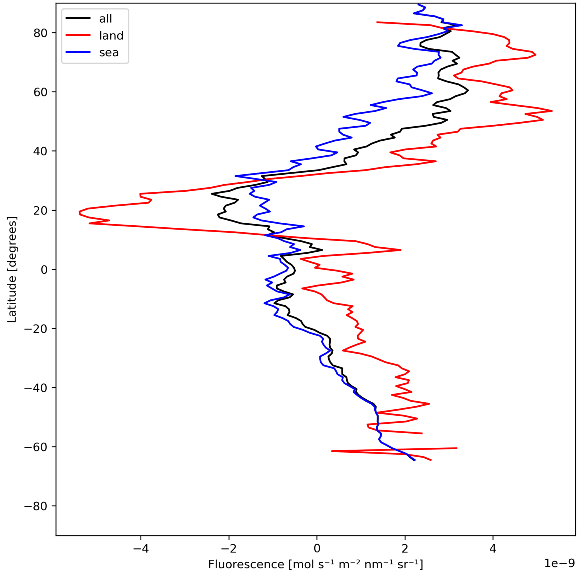
Figure 23: Zonal average of “Fluorescence” for 2024-06-08 to 2024-06-09.
