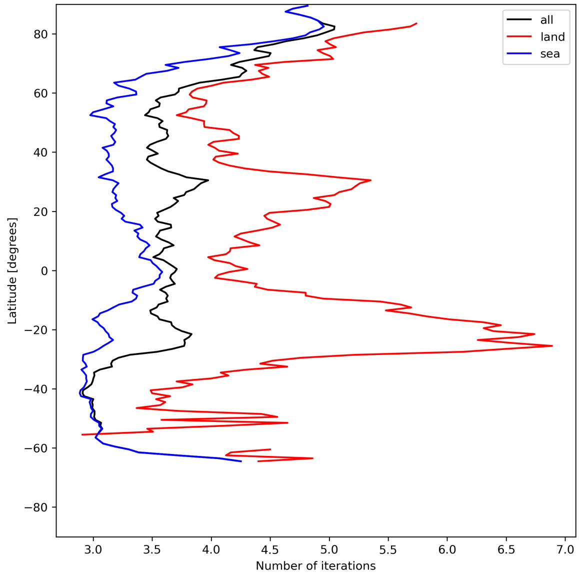
Figure 22: Zonal average of “Number of iterations” for 2024-06-08 to 2024-06-09.
