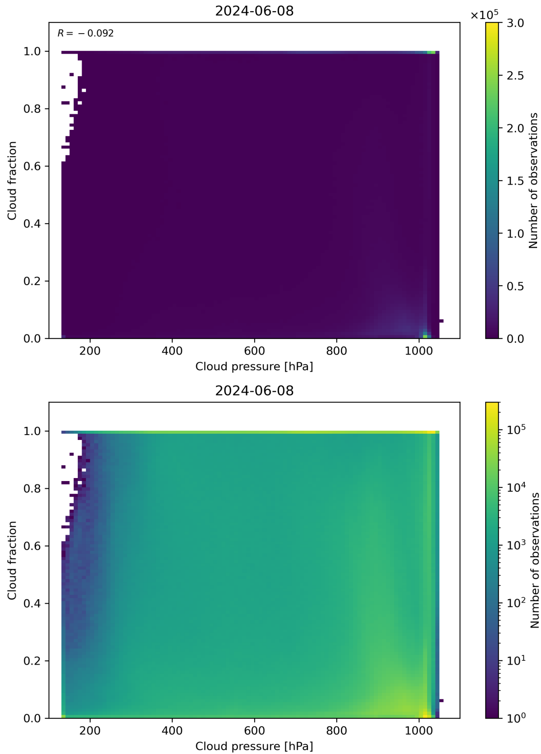
Figure 79: Scatter density plot of “Cloud pressure” against “Cloud fraction” for 2024-06-08 to 2024-06-09.
