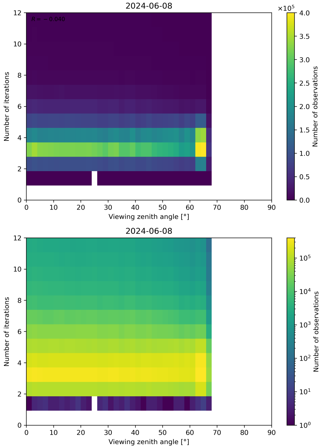
Figure 124: Scatter density plot of “Viewing zenith angle” against “Number of iterations” for 2024-06-08 to 2024-06-09.
