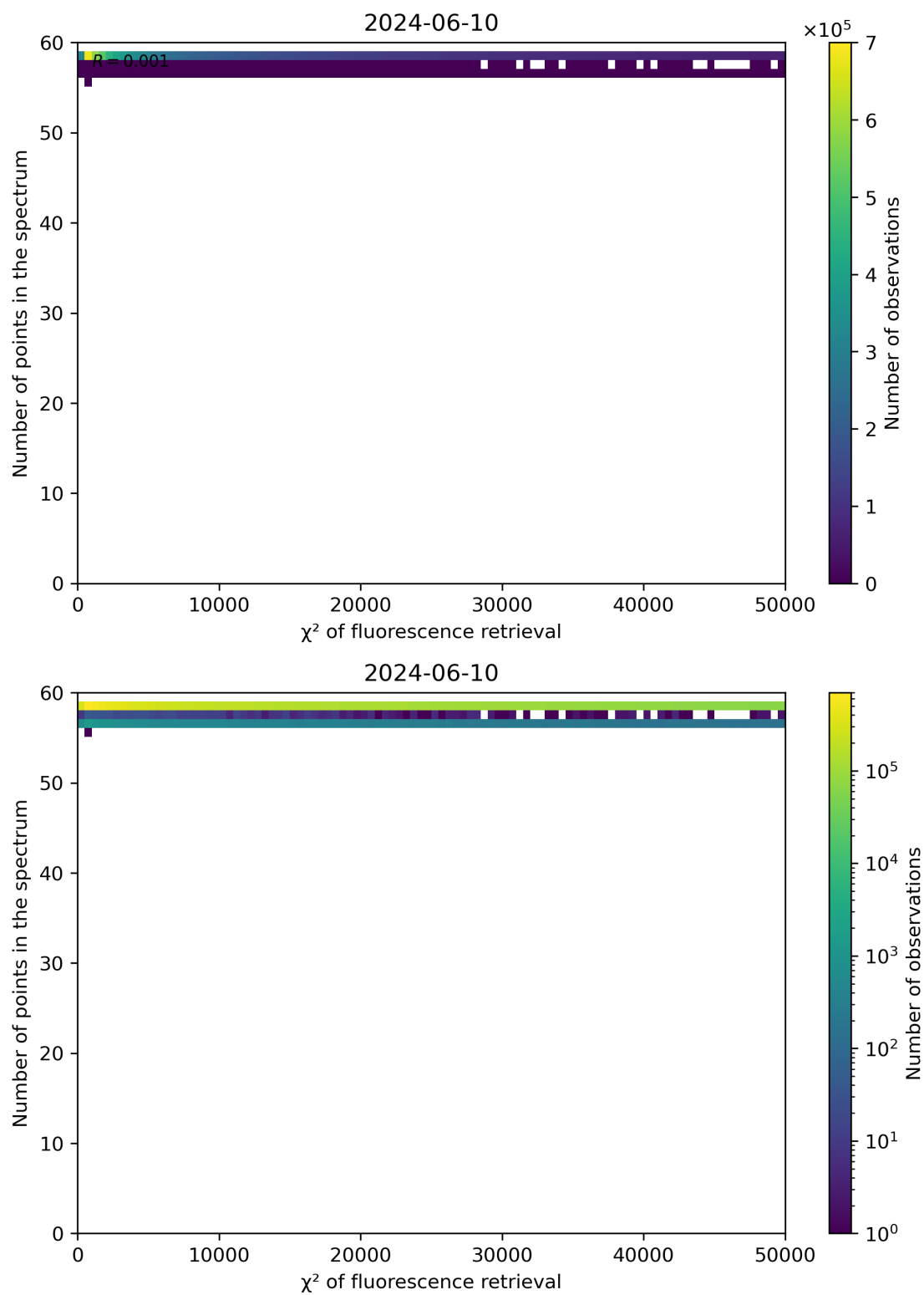
Figure 68: Scatter density plot of " \chi^2 of fluorescence retrieval" against "Number of points in the spectrum" for 2024-06-09 to 2024-06-11.
