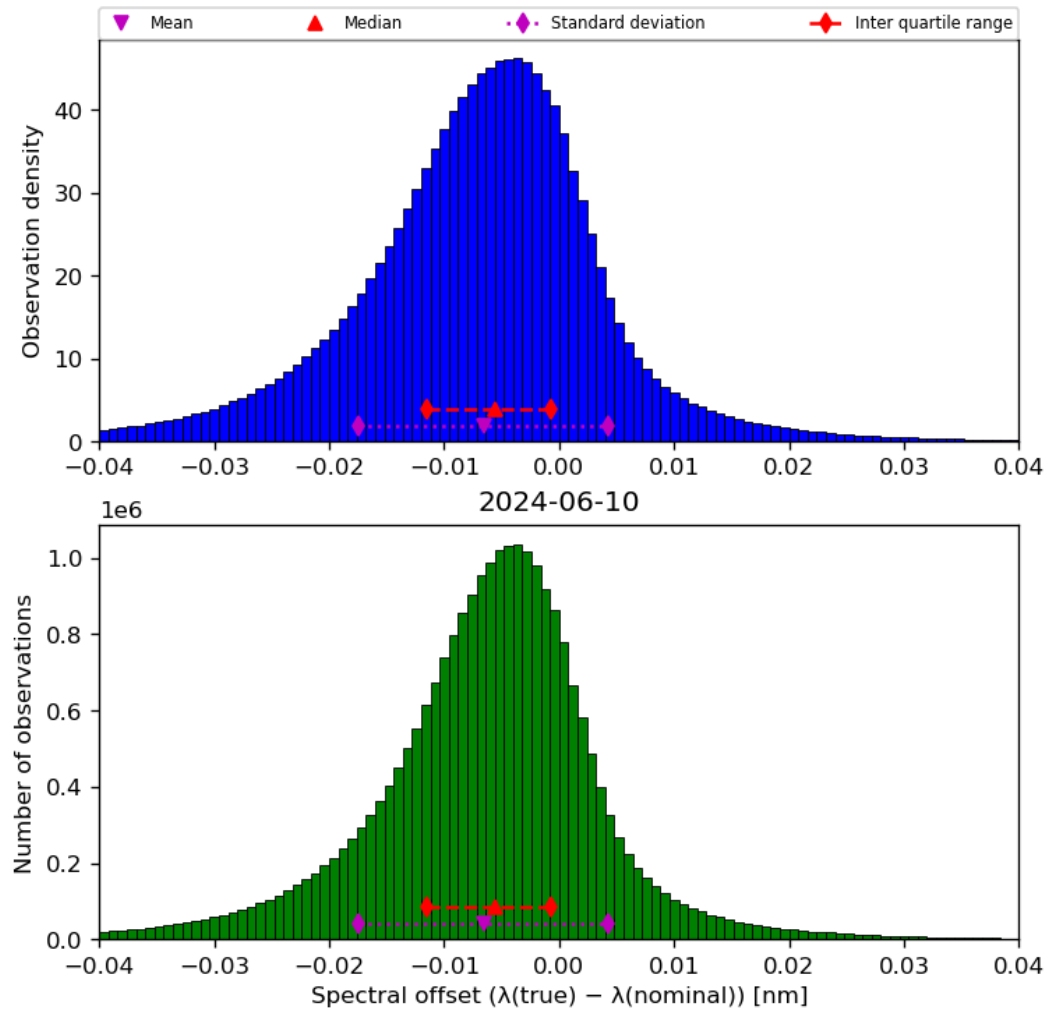
Figure 45: Histogram of “Spectral offset ( \lambda(\text{true}) - \lambda(\text{nominal}) )” for 2024-06-09 to 2024-06-11
