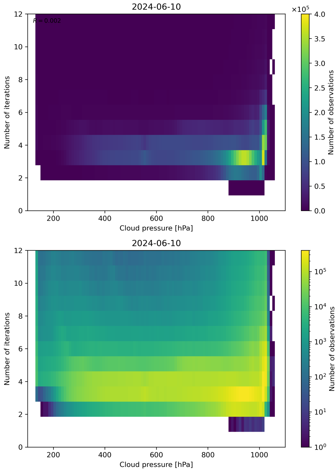
Figure 81: Scatter density plot of “Cloud pressure” against “Number of iterations” for 2024-06-09 to 2024-06-11.
