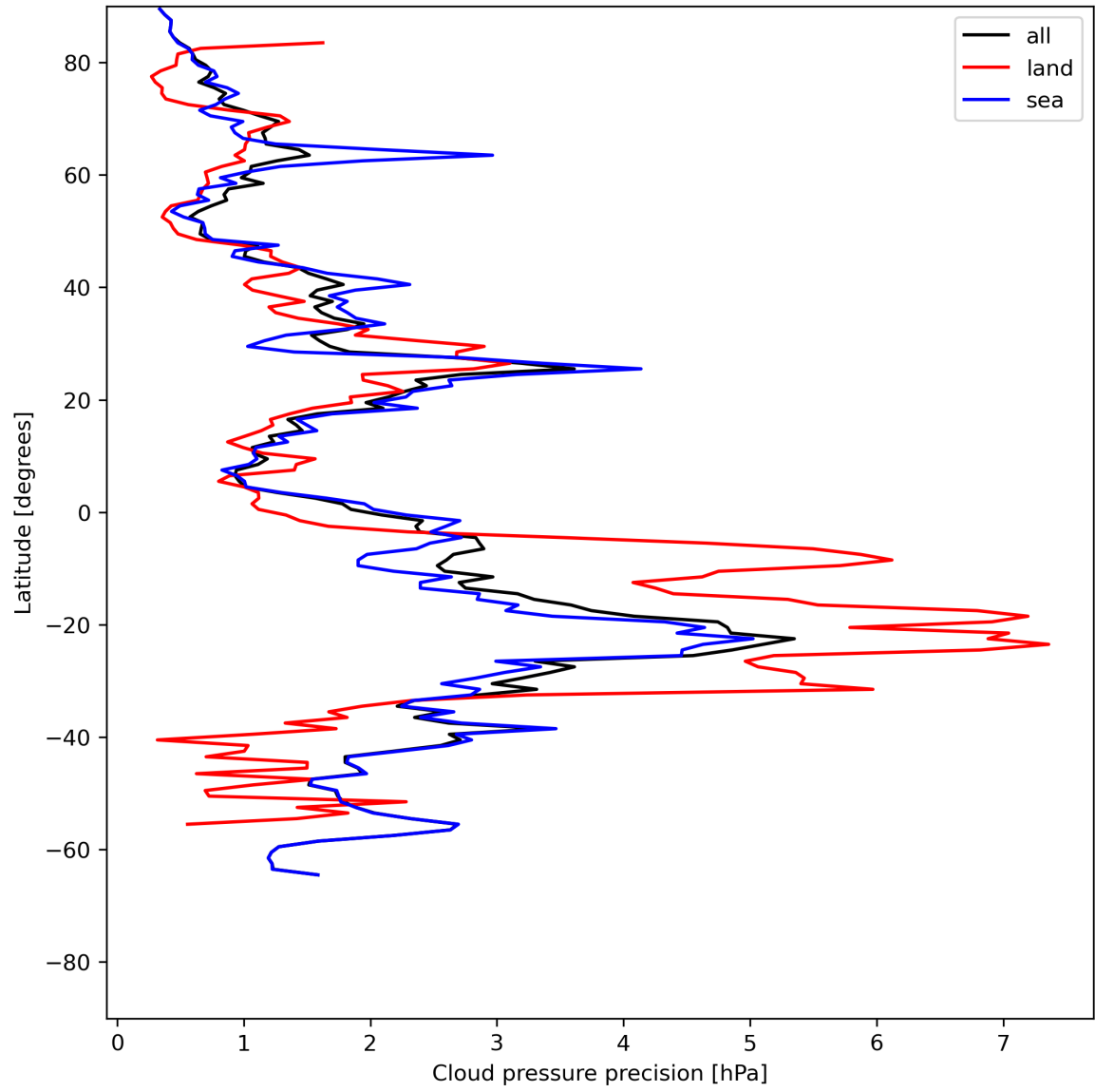
Figure 14: Zonal average of “Cloud pressure precision” for 2024-06-09 to 2024-06-11.
