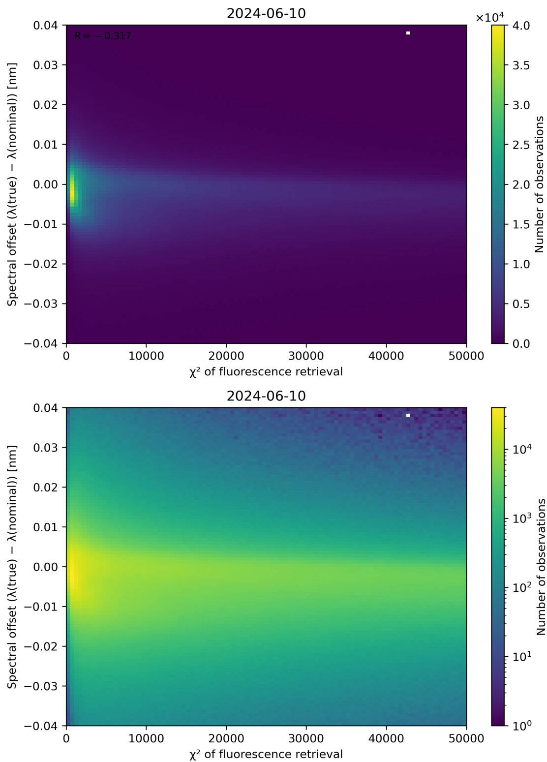
Figure 69: Scatter density plot of " \chi^2 of fluorescence retrieval" against "Spectral offset ( \lambda(\text{true}) - \lambda(\text{nominal}) )" for 2024-06-09 to 2024-06-11.
