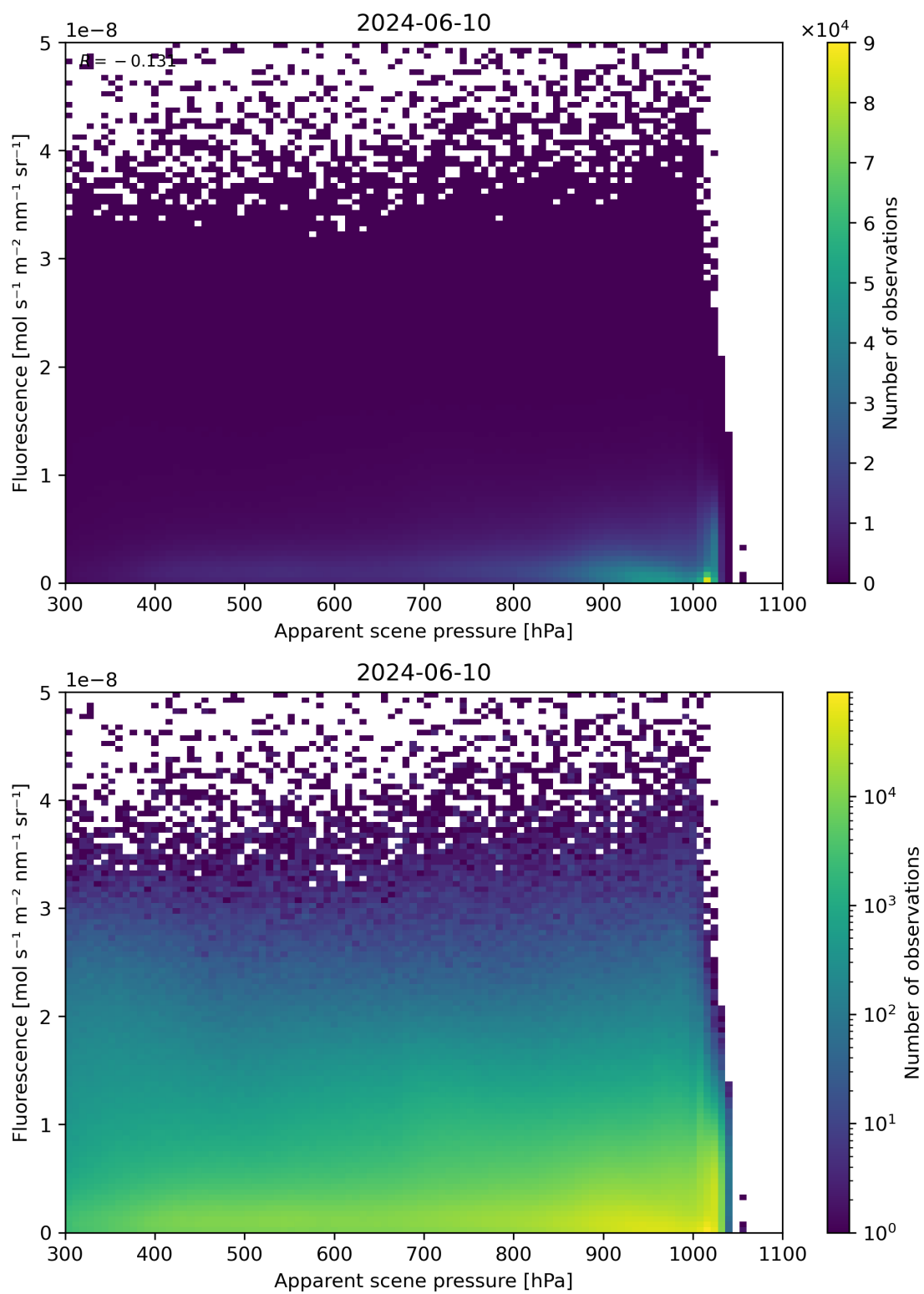
Figure 64: Scatter density plot of “Apparent scene pressure” against “Fluorescence” for 2024-06-09 to 2024-06-11.
