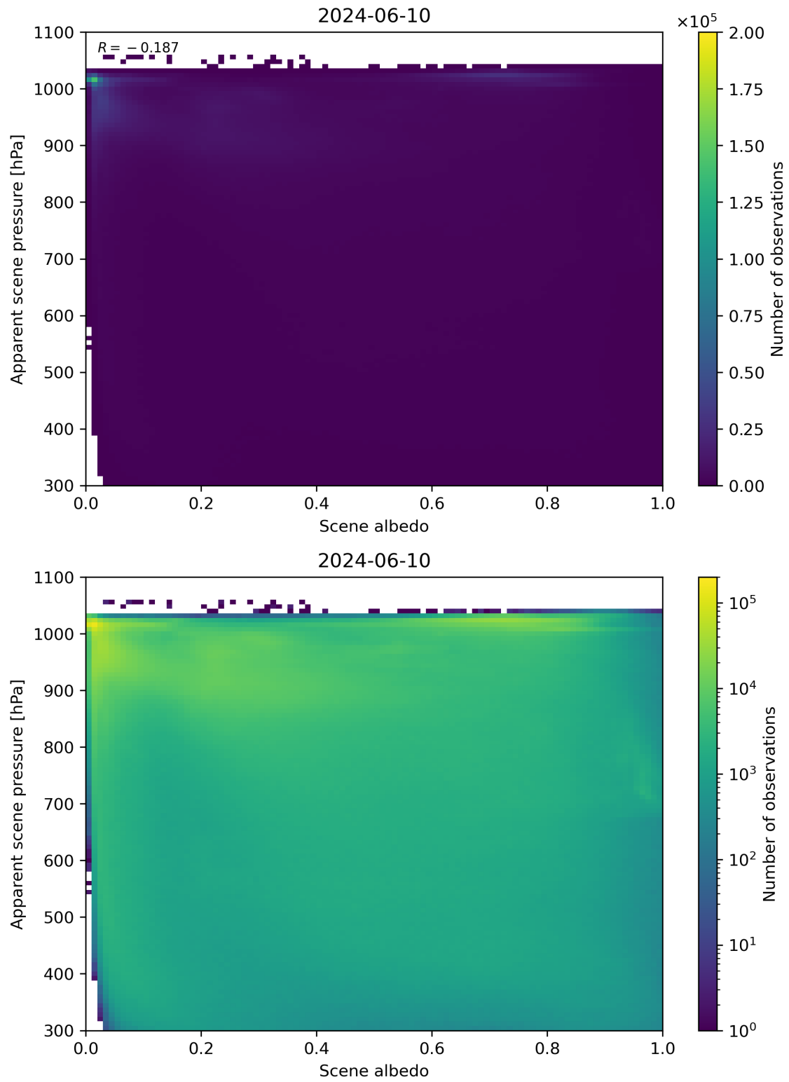
Figure 102: Scatter density plot of “Scene albedo” against “Apparent scene pressure” for 2024-06-09 to 2024-06-11.
