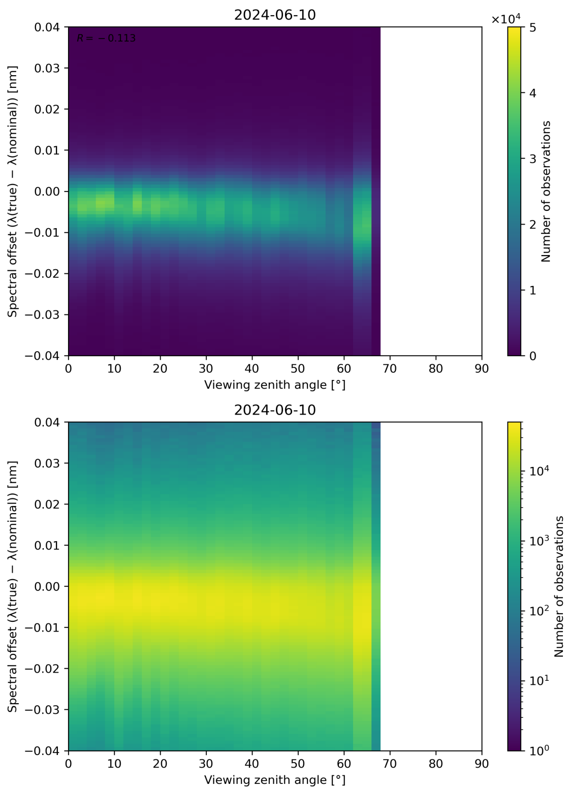
Figure 128: Scatter density plot of “Viewing zenith angle” against “Spectral offset ( \lambda(\text{true}) - \lambda(\text{nominal}) )” for 2024-06-09 to 2024-06-11.
