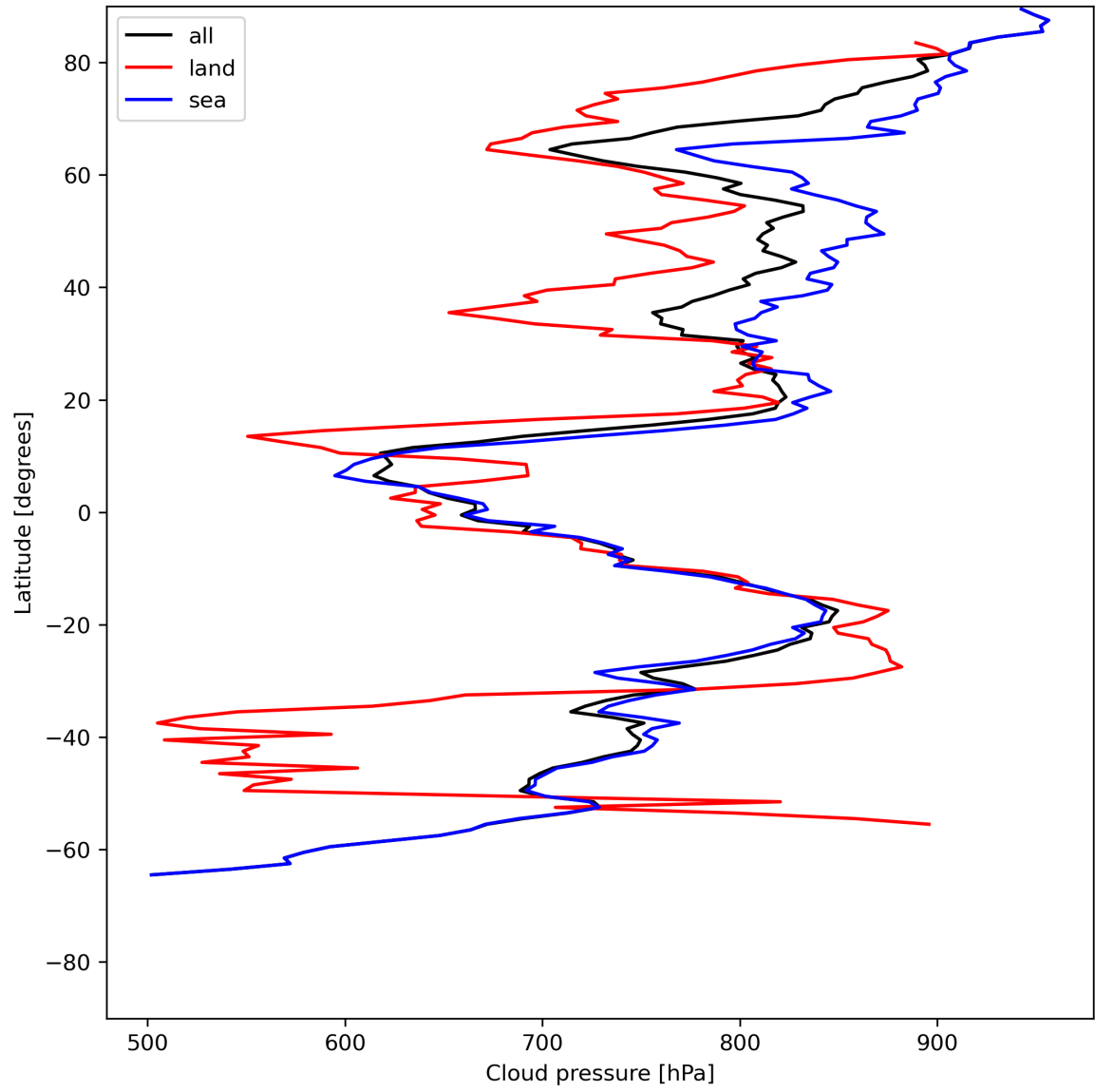
Figure 13: Zonal average of “Cloud pressure” for 2024-06-09 to 2024-06-11.
