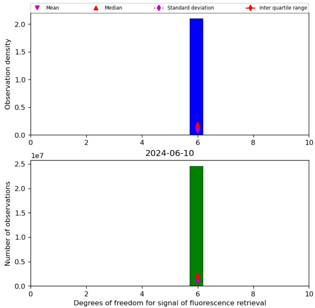
Figure 43: Histogram of "Degrees of freedom for signal of fluorescence retrieval" for 2024-06-09 to 2024-06-11
