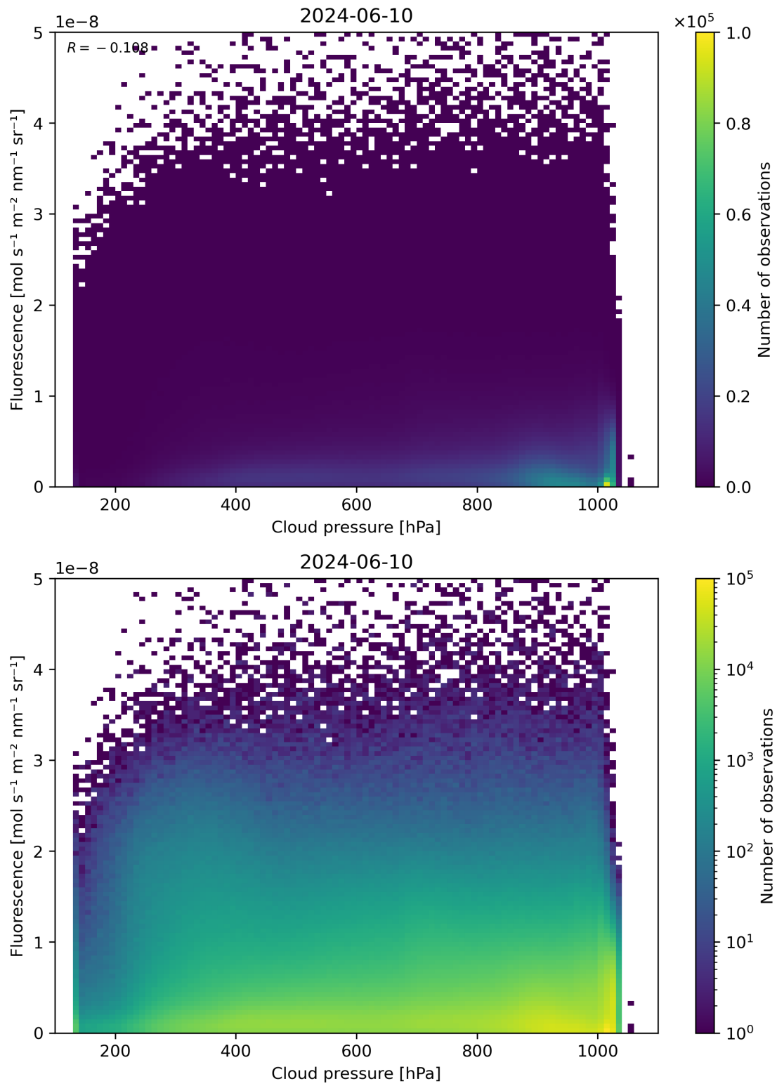
Figure 80: Scatter density plot of “Cloud pressure” against “Fluorescence” for 2024-06-09 to 2024-06-11.
