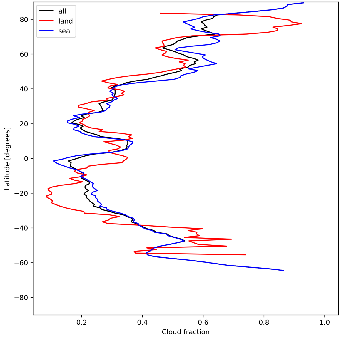
Figure 15: Zonal average of “Cloud fraction” for 2024-06-09 to 2024-06-11.
