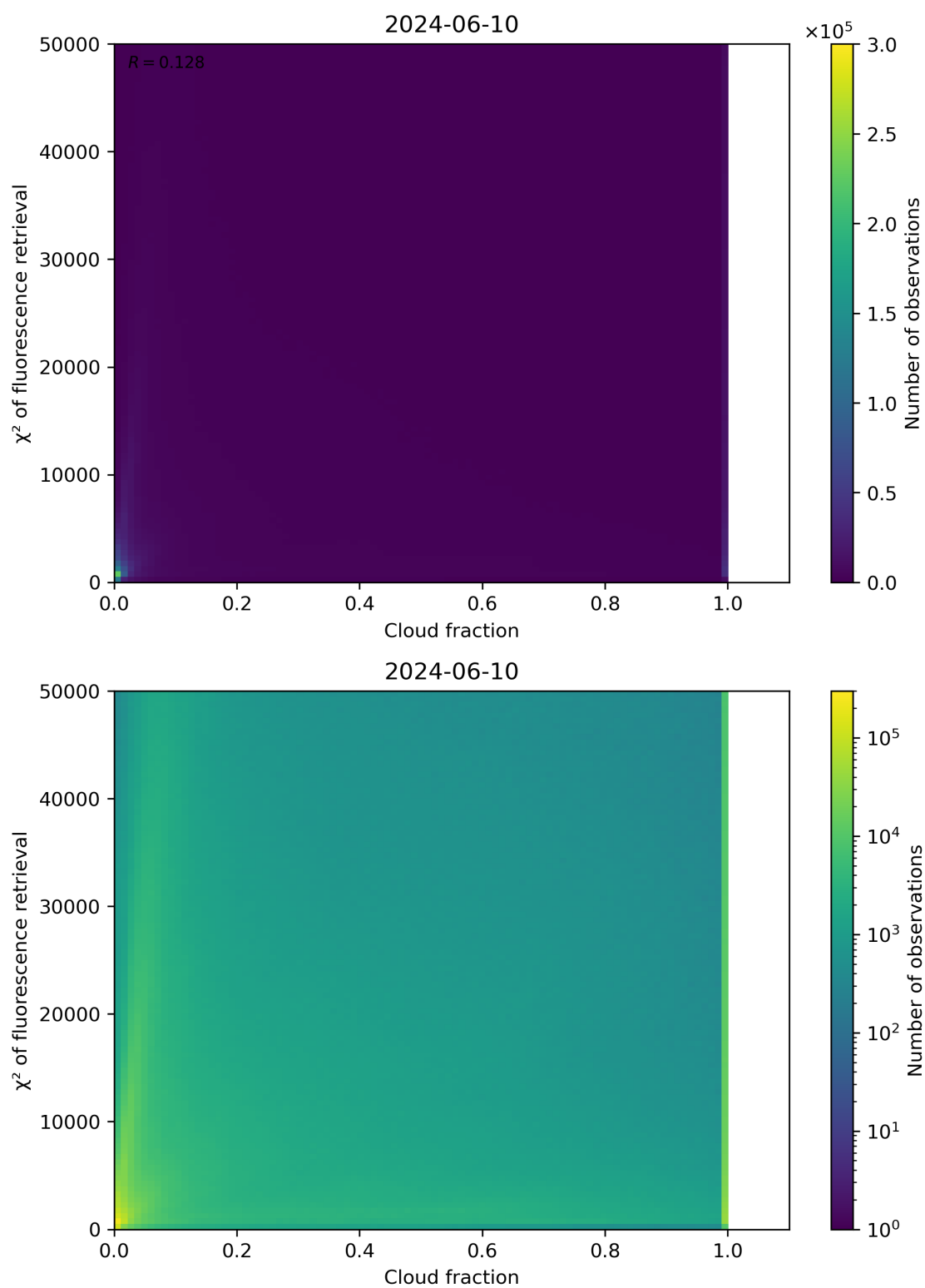
Figure 71: Scatter density plot of “Cloud fraction” against “ \chi^2 of fluorescence retrieval” for 2024-06-09 to 2024-06-11.
