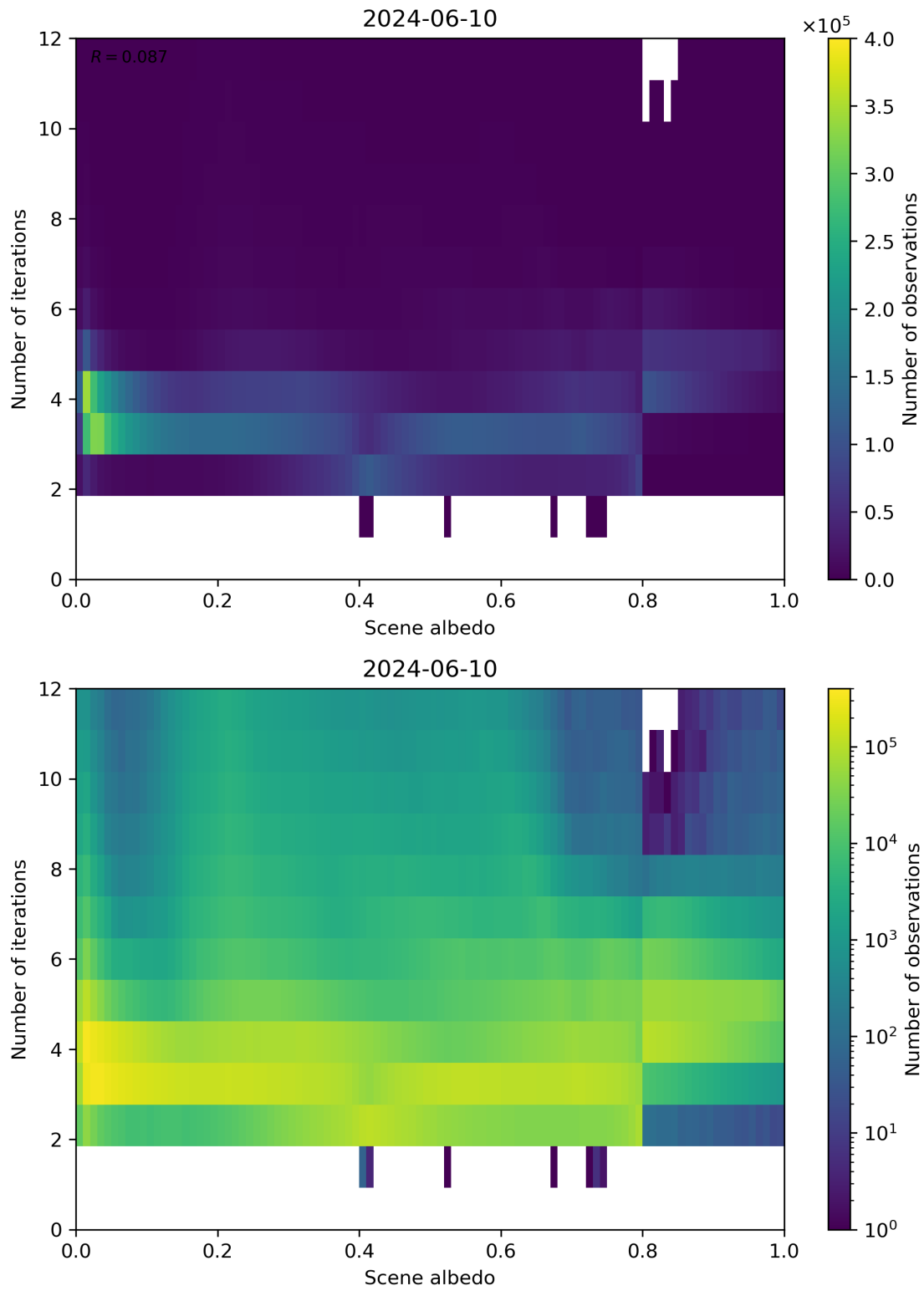
Figure 105: Scatter density plot of “Scene albedo” against “Number of iterations” for 2024-06-09 to 2024-06-11.
