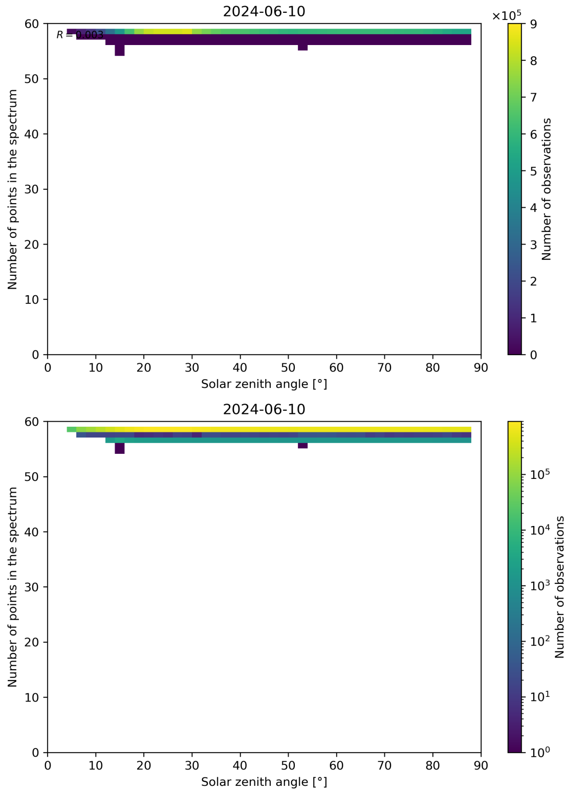
Figure 115: Scatter density plot of “Solar zenith angle” against “Number of points in the spectrum” for 2024-06-09 to 2024-06-11.
