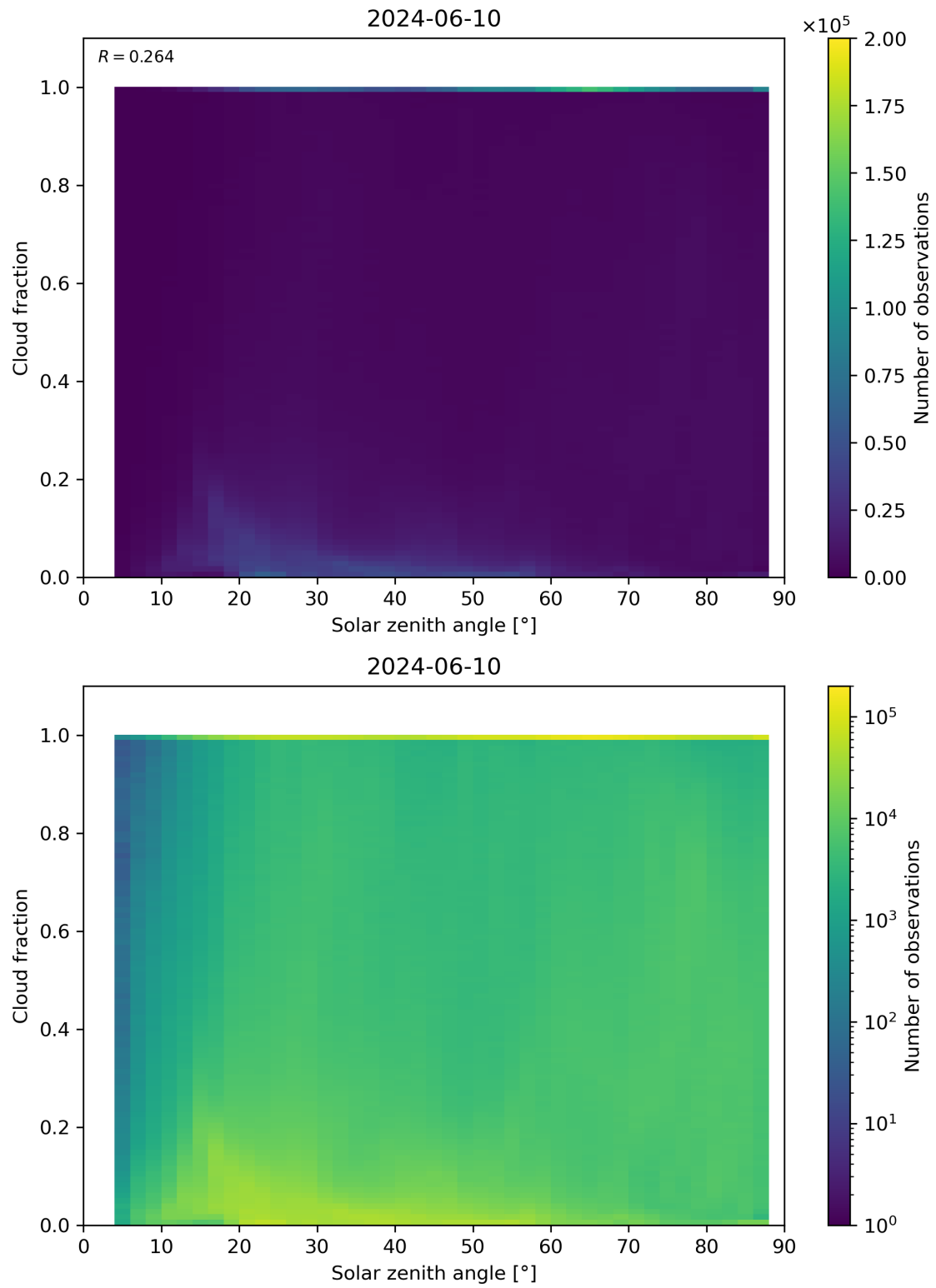
Figure 110: Scatter density plot of “Solar zenith angle” against “Cloud fraction” for 2024-06-09 to 2024-06-11.
