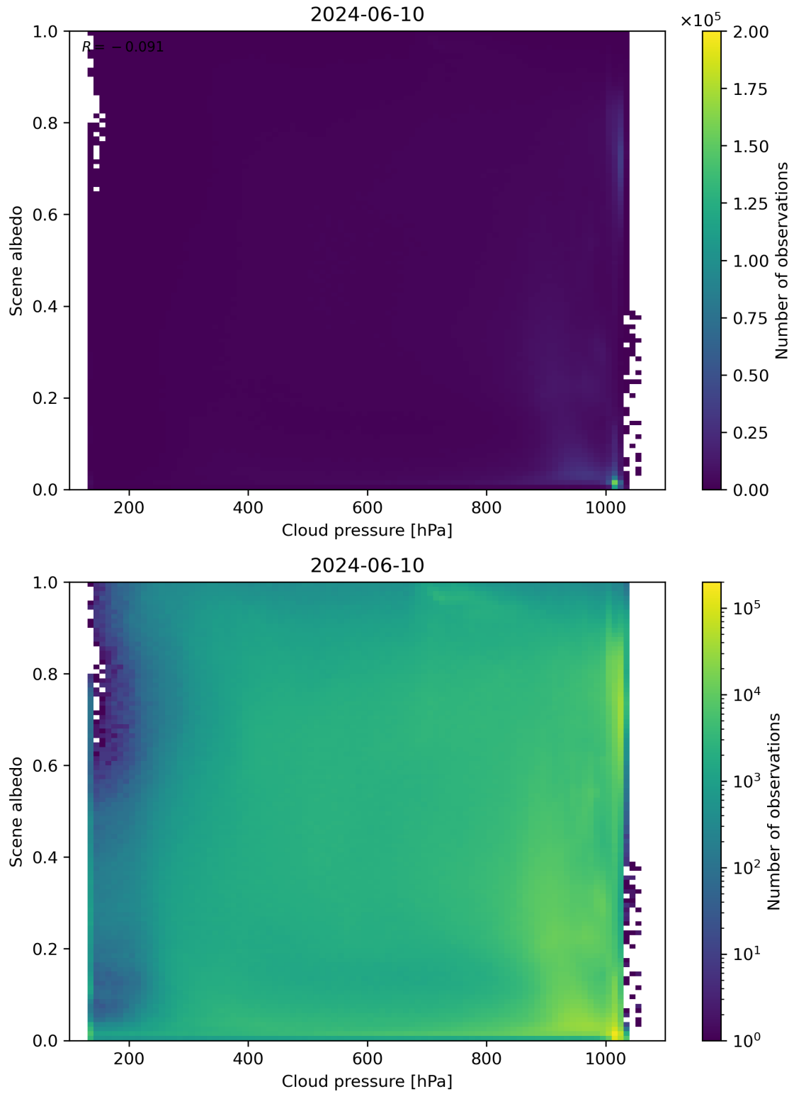
Figure 83: Scatter density plot of “Cloud pressure” against “Scene albedo” for 2024-06-09 to 2024-06-11.
