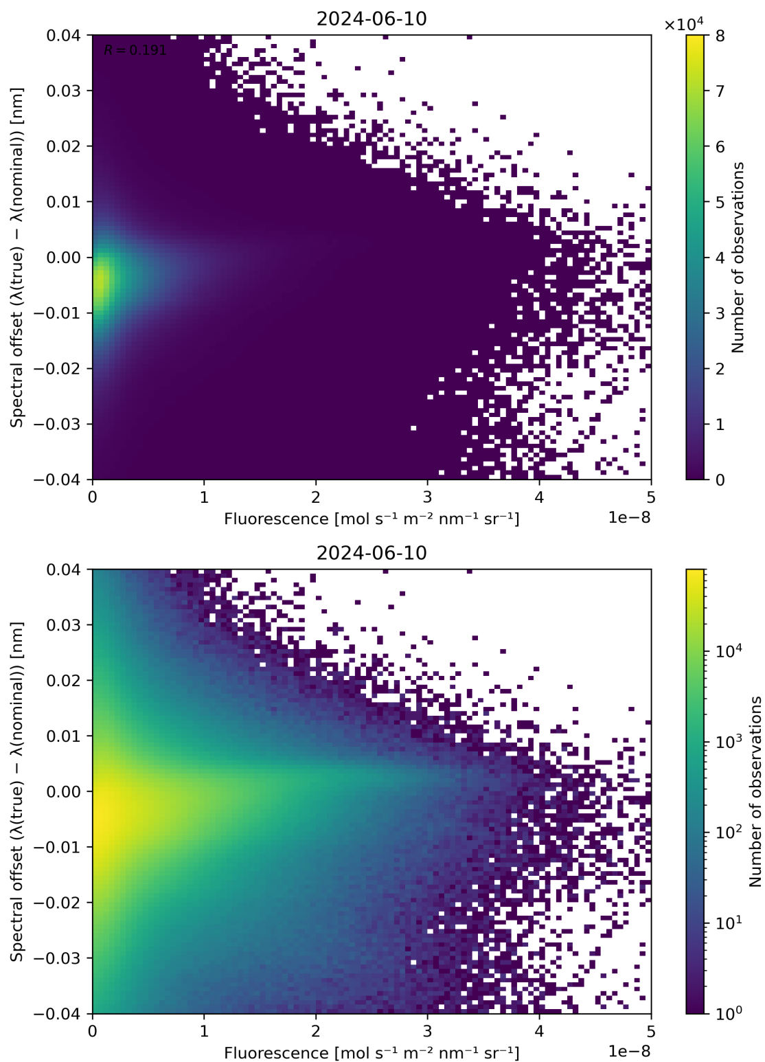
Figure 87: Scatter density plot of “Fluorescence” against “Spectral offset ( \lambda(\text{true}) - \lambda(\text{nominal}) )” for 2024-06-09 to 2024-06-11.
