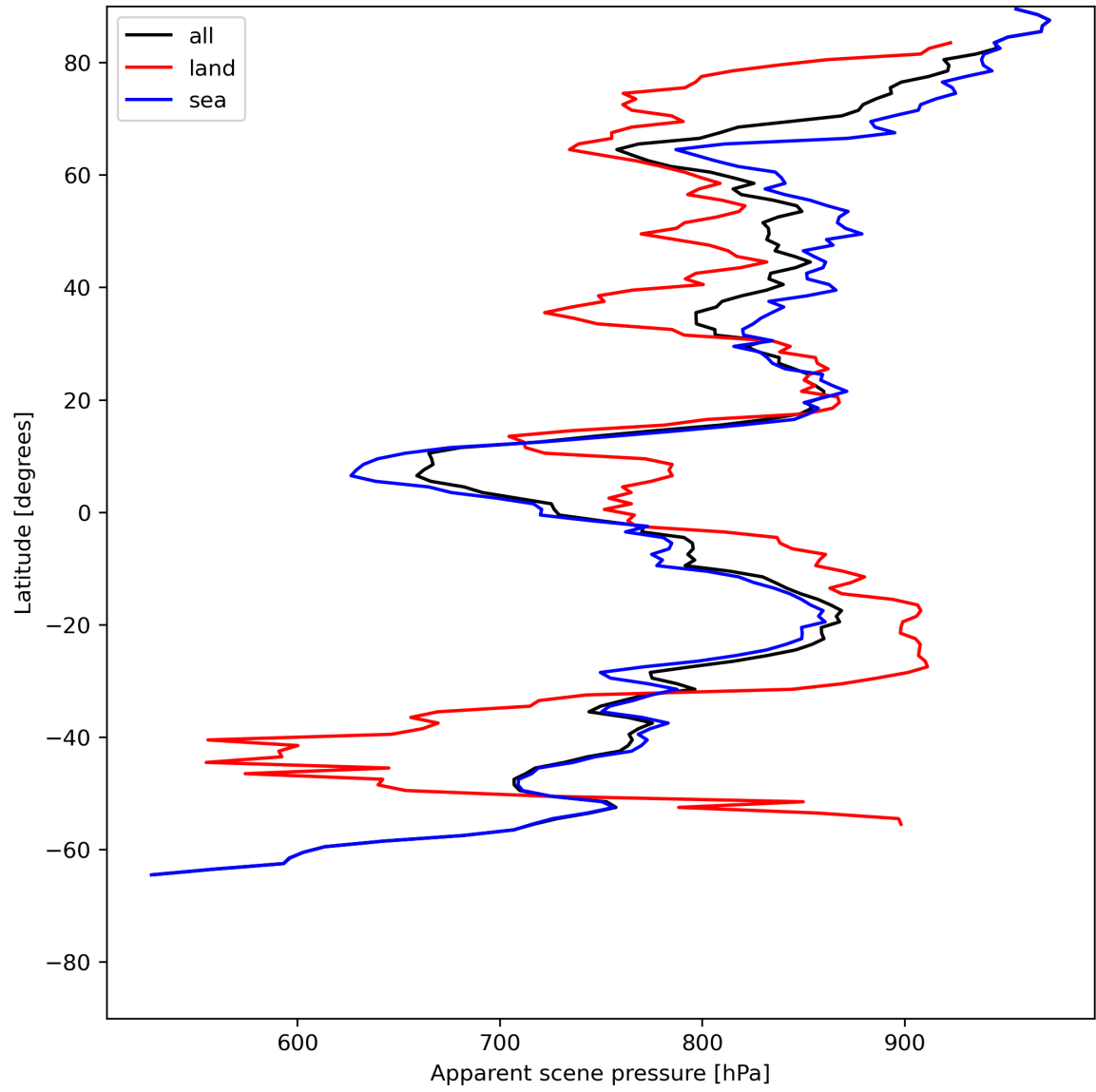
Figure 19: Zonal average of “Apparent scene pressure” for 2024-06-09 to 2024-06-11.
