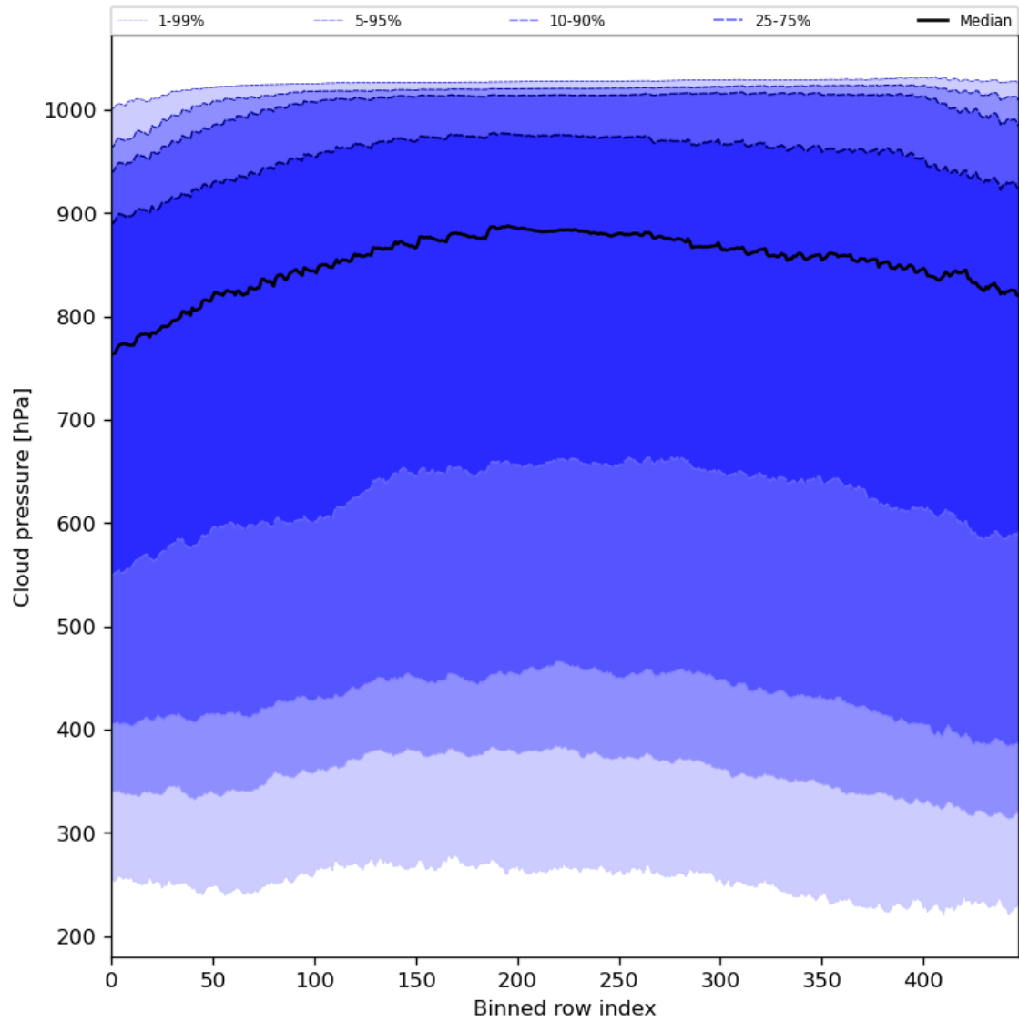
Figure 47: Along track statistics of “Cloud pressure” for 2024-06-09 to 2024-06-11
