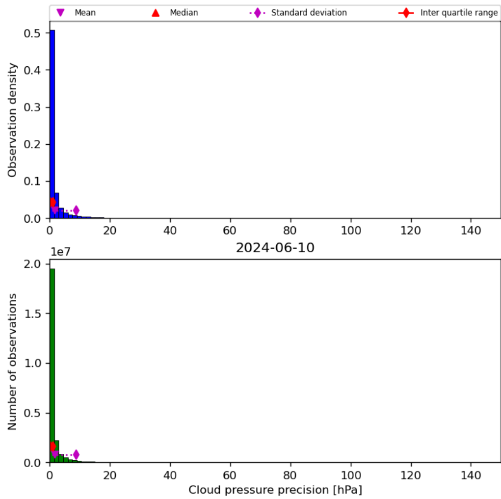
Figure 31: Histogram of “Cloud pressure precision” for 2024-06-09 to 2024-06-11
