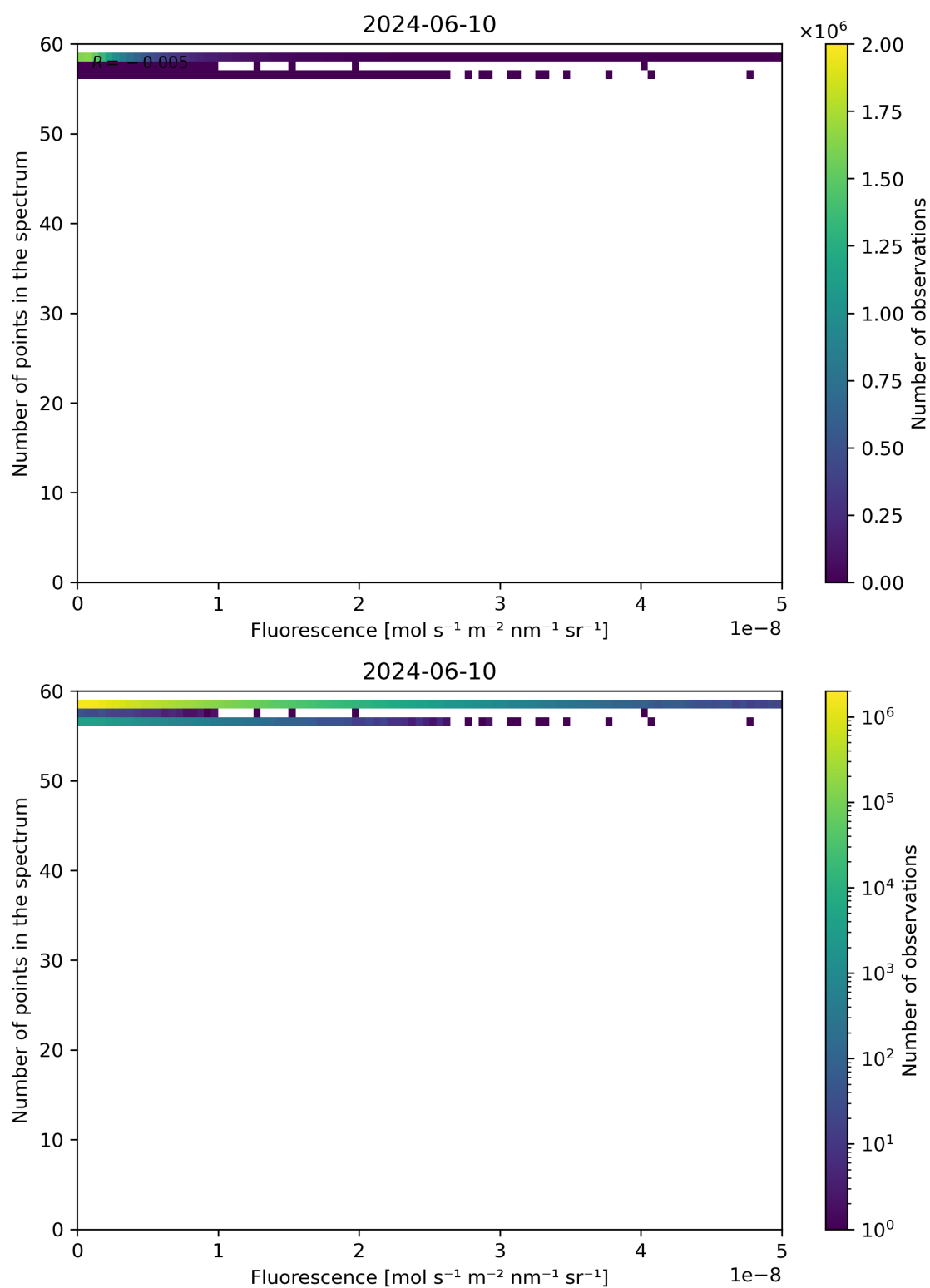
Figure 86: Scatter density plot of “Fluorescence” against “Number of points in the spectrum” for 2024-06-09 to 2024-06-11.
