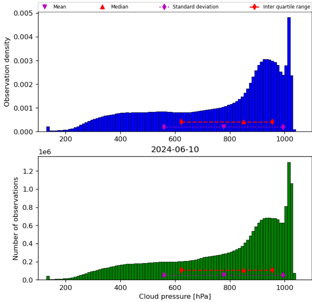
Figure 30: Histogram of “Cloud pressure” for 2024-06-09 to 2024-06-11
