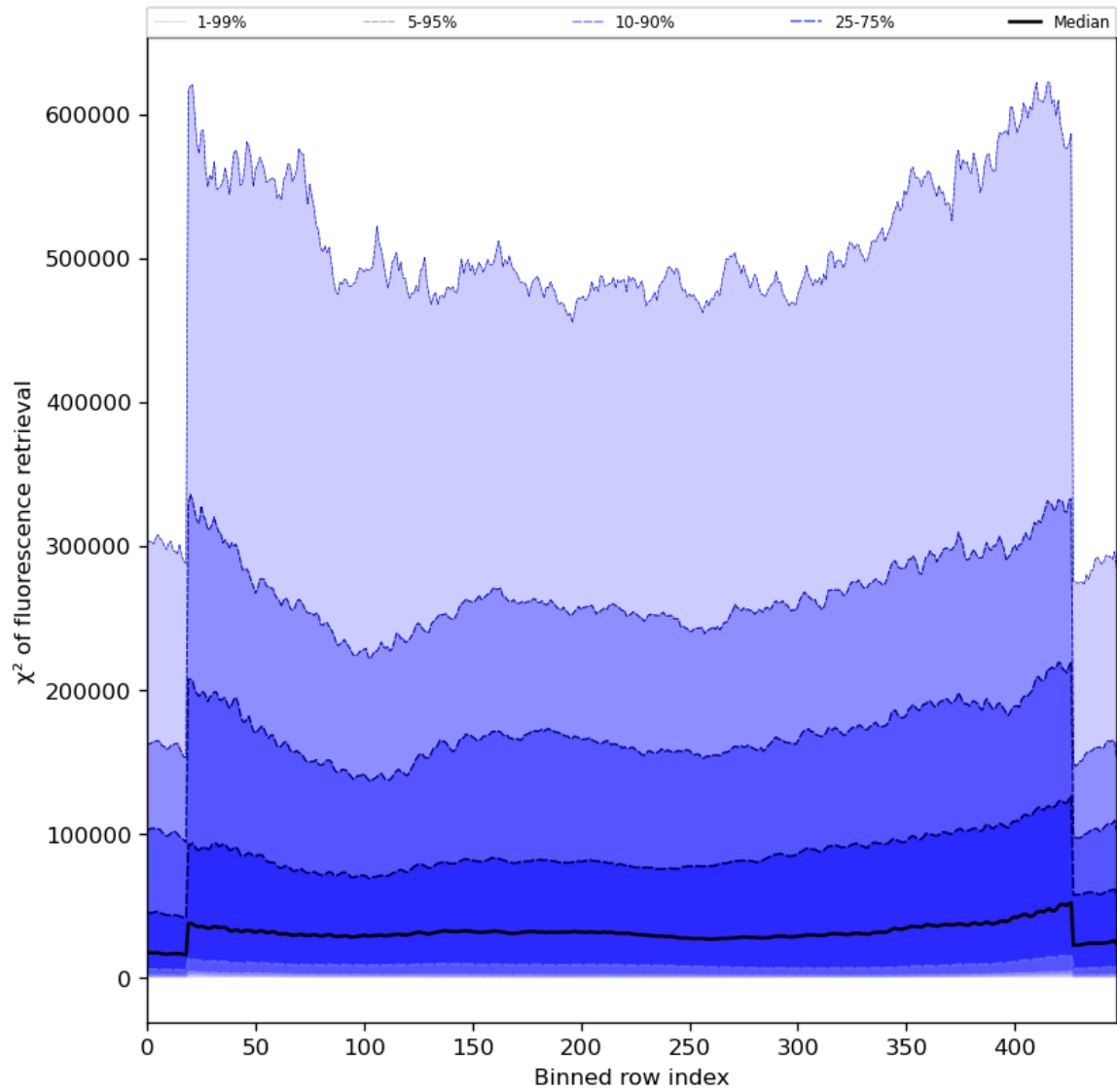
Figure 59: Along track statistics of “ \chi^2 of fluorescence retrieval” for 2024-06-09 to 2024-06-11
