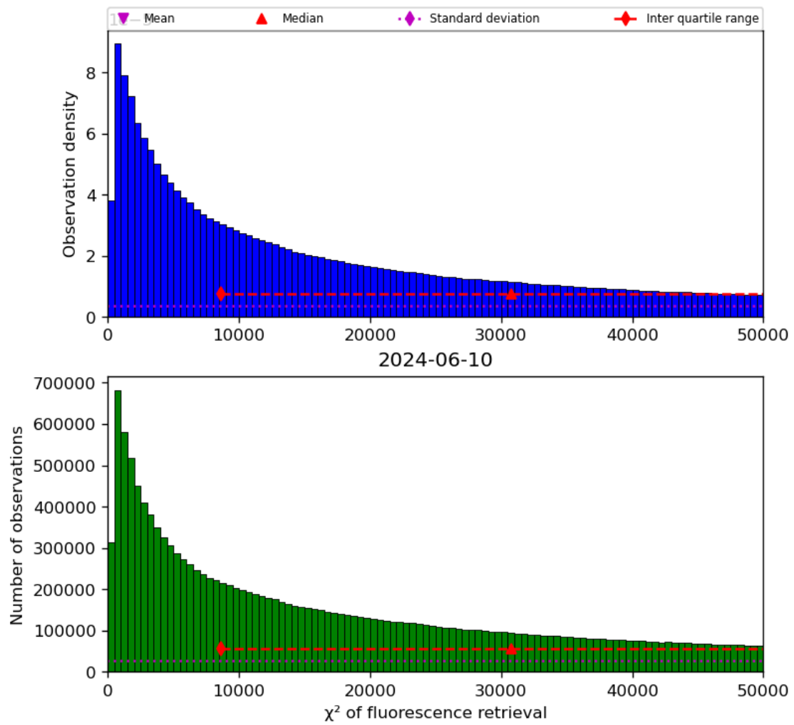
Figure 42: Histogram of “ \chi^2 of fluorescence retrieval” for 2024-06-09 to 2024-06-11
