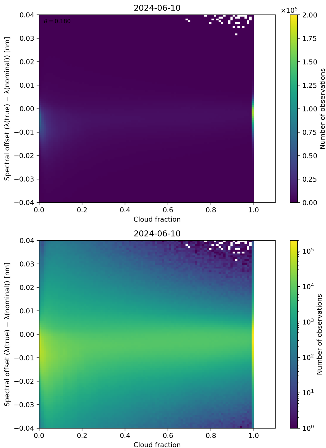
Figure 76: Scatter density plot of “Cloud fraction” against “Spectral offset ( \lambda(\text{true}) - \lambda(\text{nominal}) )” for 2024-06-09 to 2024-06-11.
