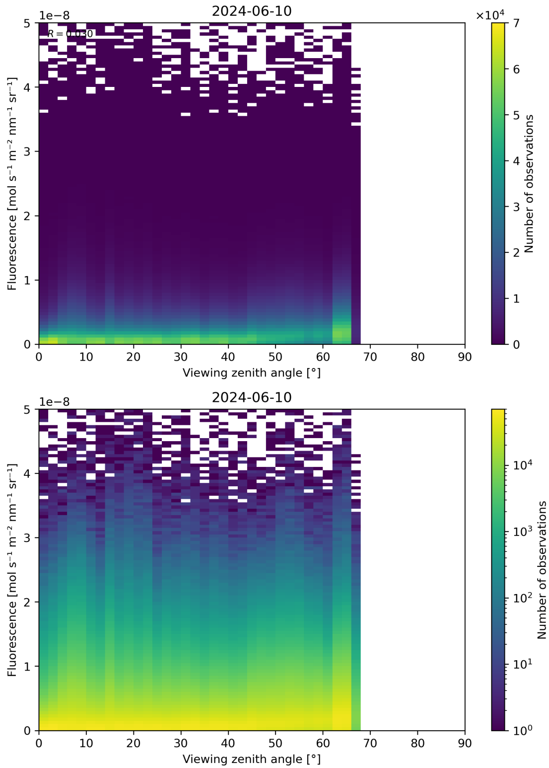
Figure 122: Scatter density plot of “Viewing zenith angle” against “Fluorescence” for 2024-06-09 to 2024-06-11.
