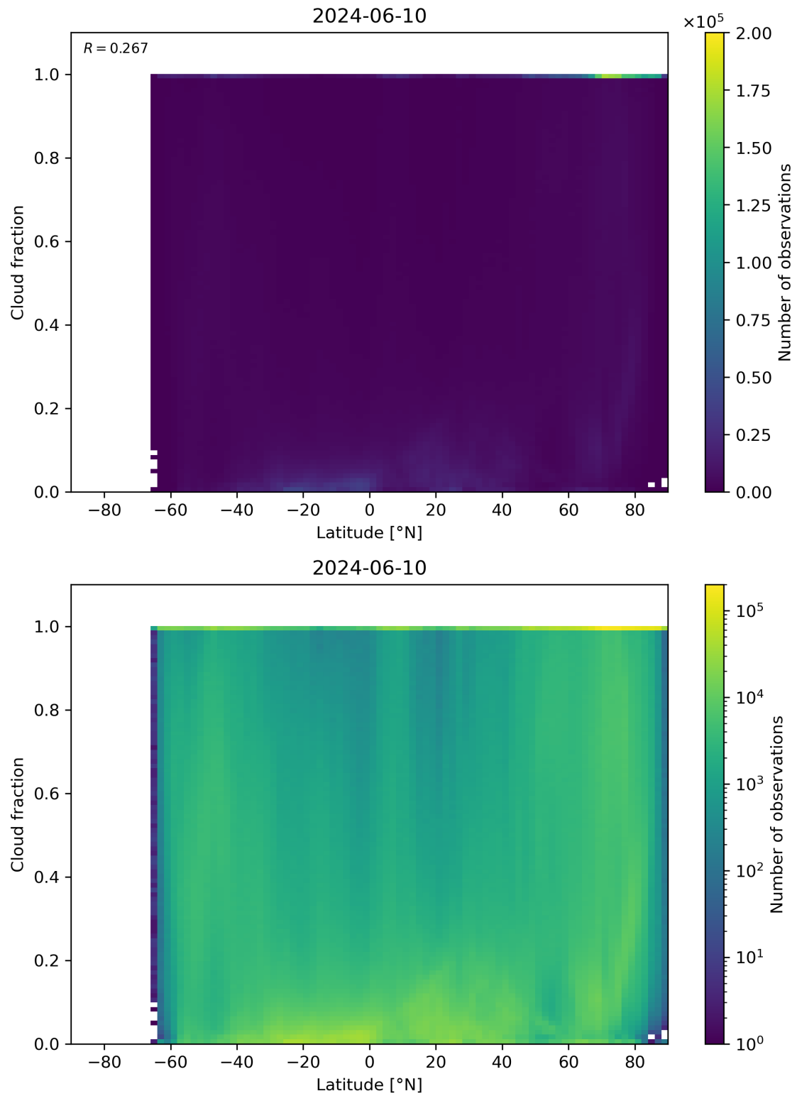
Figure 90: Scatter density plot of “Latitude” against “Cloud fraction” for 2024-06-09 to 2024-06-11.
