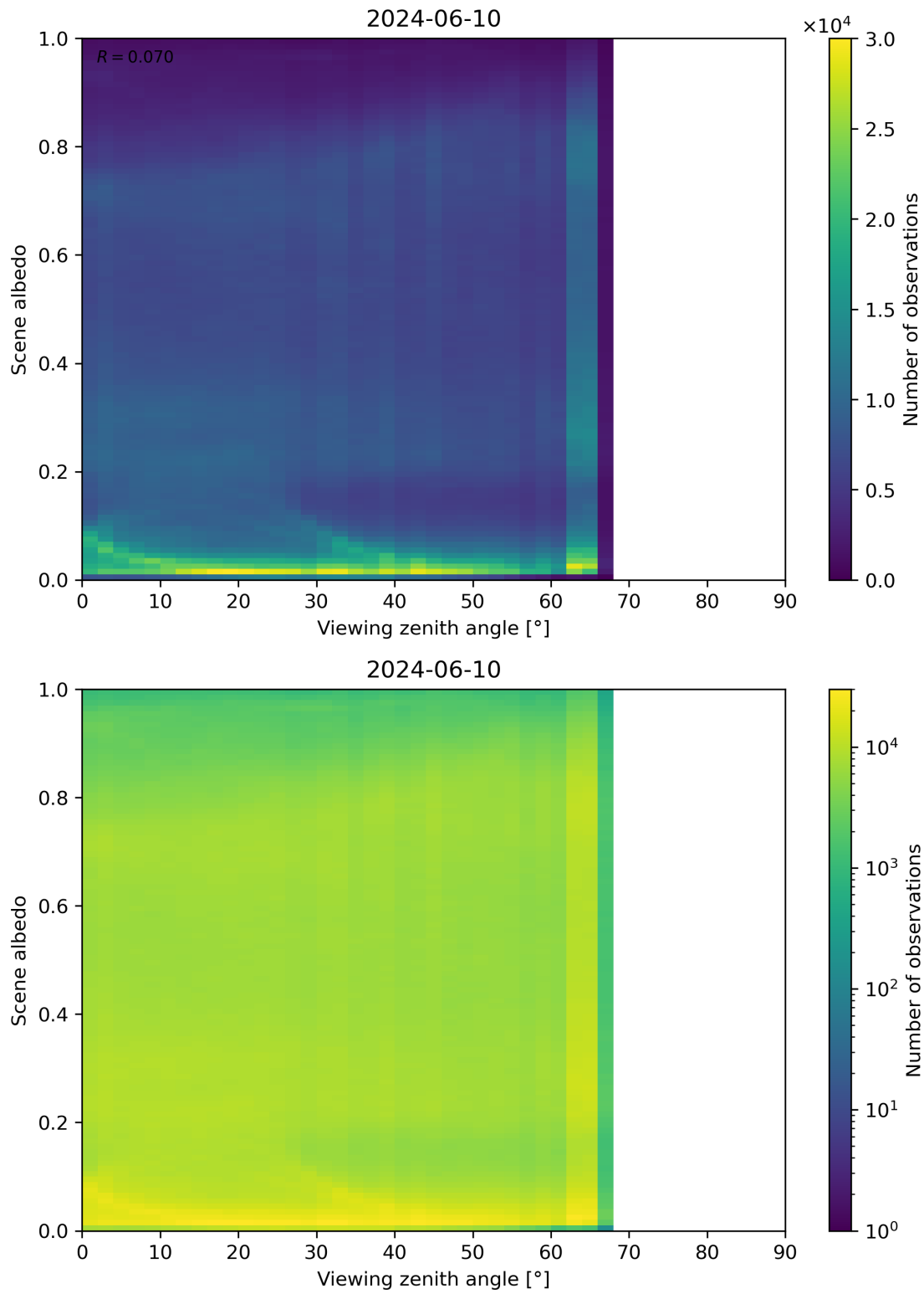
Figure 126: Scatter density plot of “Viewing zenith angle” against “Scene albedo” for 2024-06-09 to 2024-06-11.
