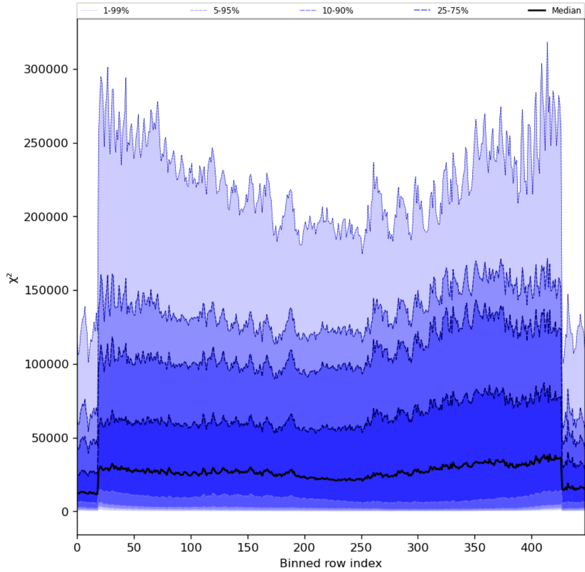
Figure 55: Along track statistics of “ \chi^2 ” for 2024-06-09 to 2024-06-11
