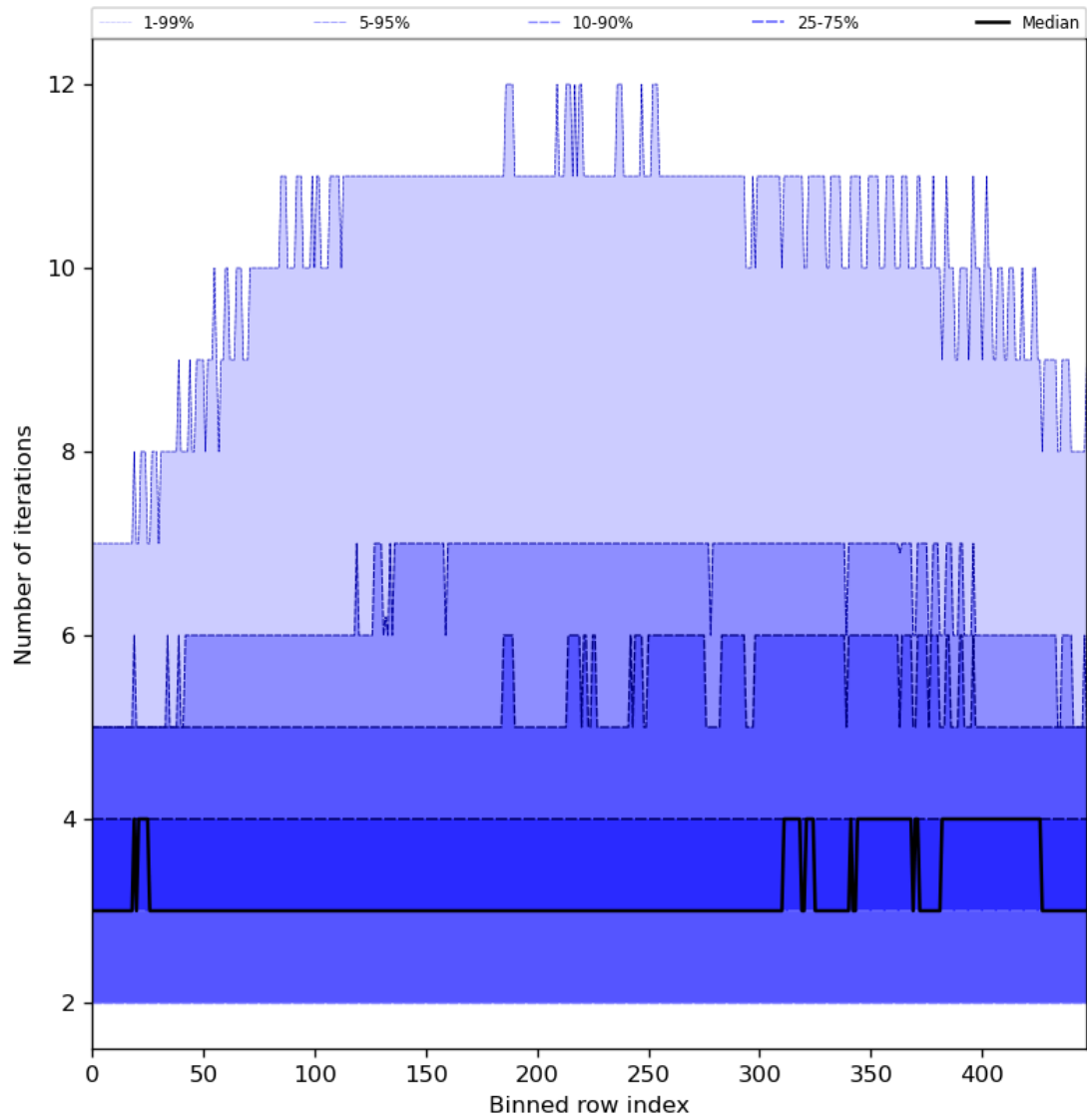
Figure 56: Along track statistics of “Number of iterations” for 2024-06-09 to 2024-06-11
