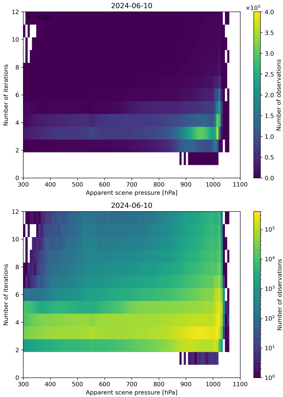
Figure 65: Scatter density plot of “Apparent scene pressure” against “Number of iterations” for 2024-06-09 to 2024-06-11.
