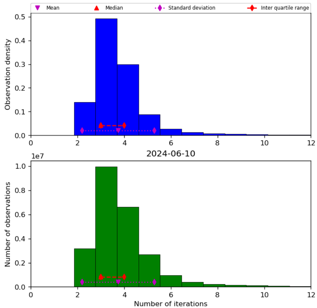
Figure 39: Histogram of “Number of iterations” for 2024-06-09 to 2024-06-11
