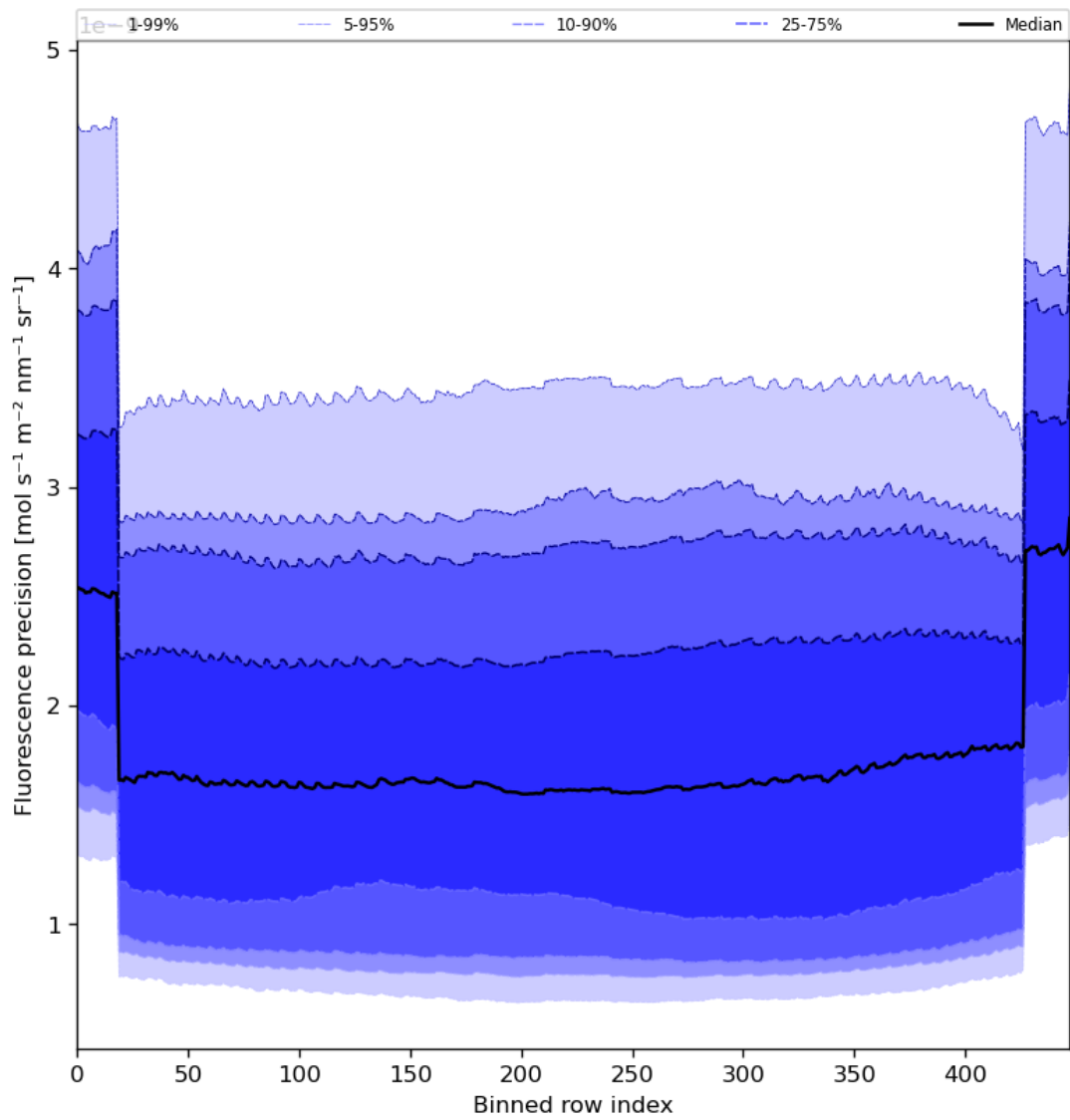
Figure 58: Along track statistics of “Fluorescence precision” for 2024-06-09 to 2024-06-11
