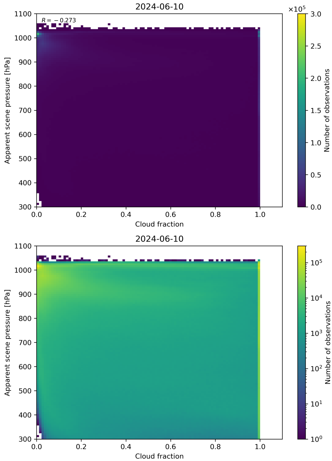
Figure 70: Scatter density plot of “Cloud fraction” against “Apparent scene pressure” for 2024-06-09 to 2024-06-11.
