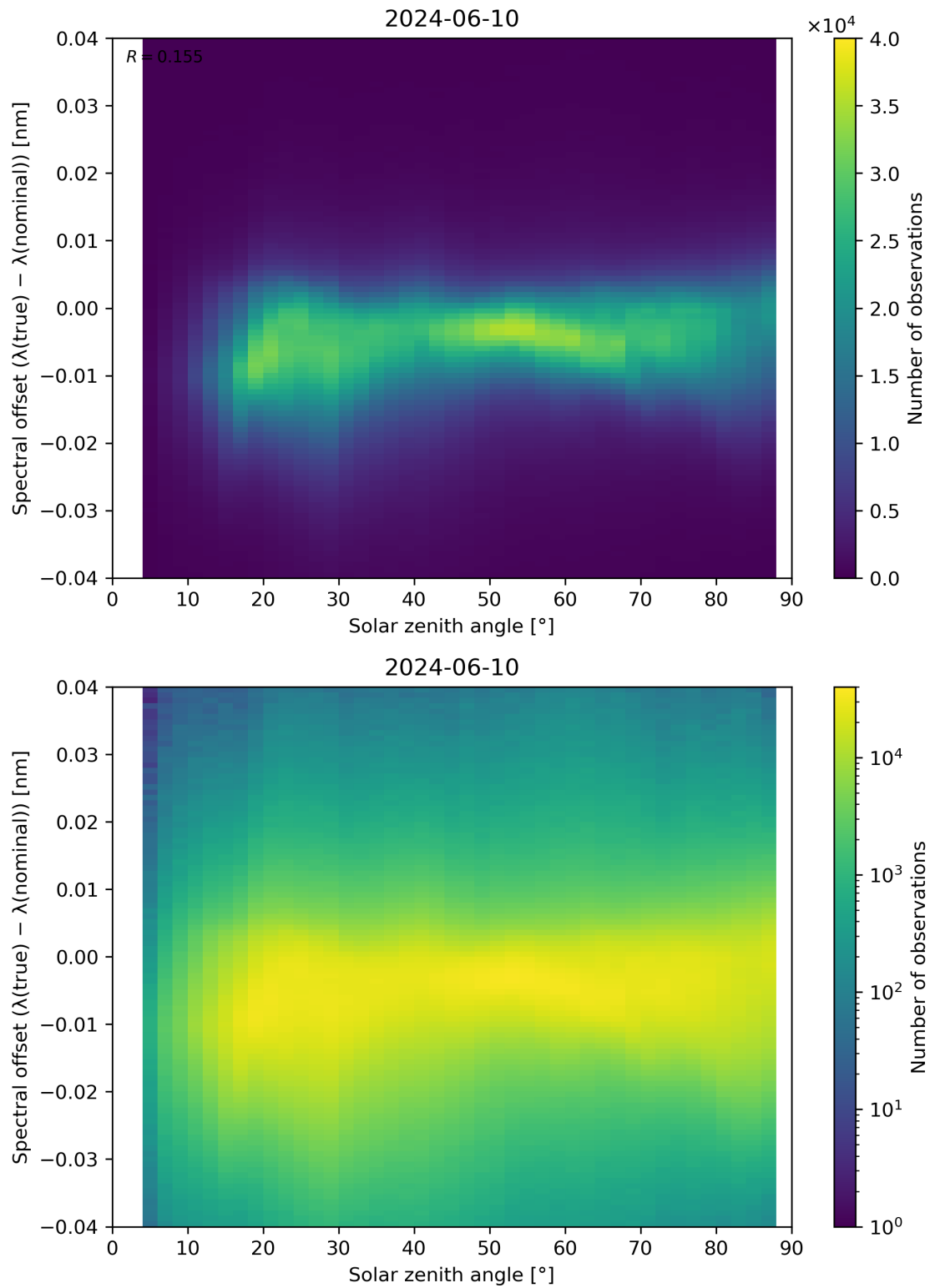
Figure 117: Scatter density plot of “Solar zenith angle” against “Spectral offset ( \lambda(\text{true}) - \lambda(\text{nominal}) )” for 2024-06-09 to 2024-06-11.
