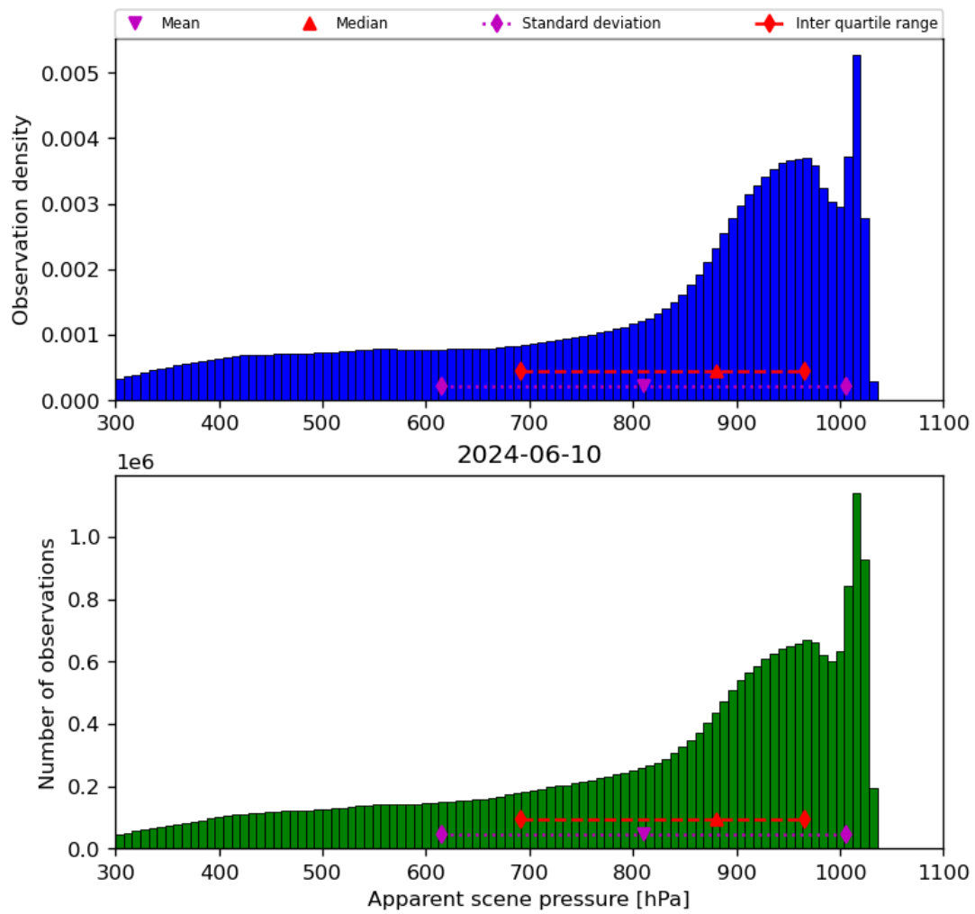
Figure 36: Histogram of “Apparent scene pressure” for 2024-06-09 to 2024-06-11
