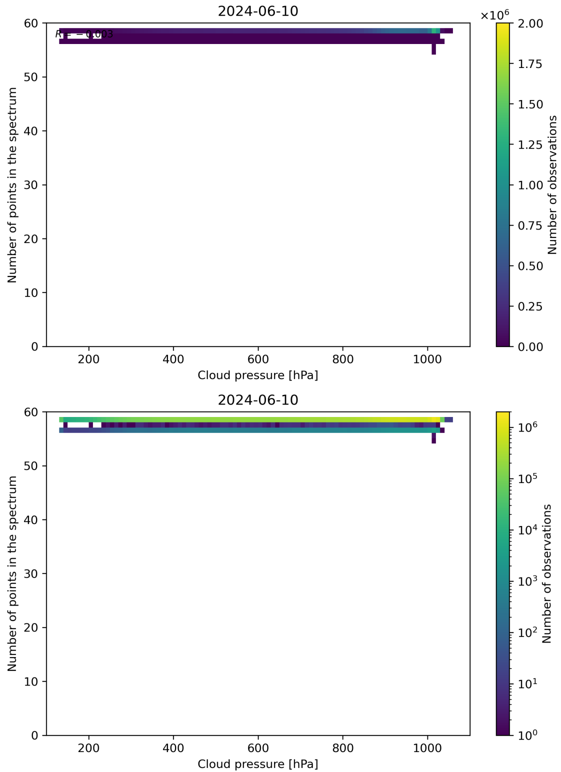
Figure 82: Scatter density plot of “Cloud pressure” against “Number of points in the spectrum” for 2024-06-09 to 2024-06-11.
