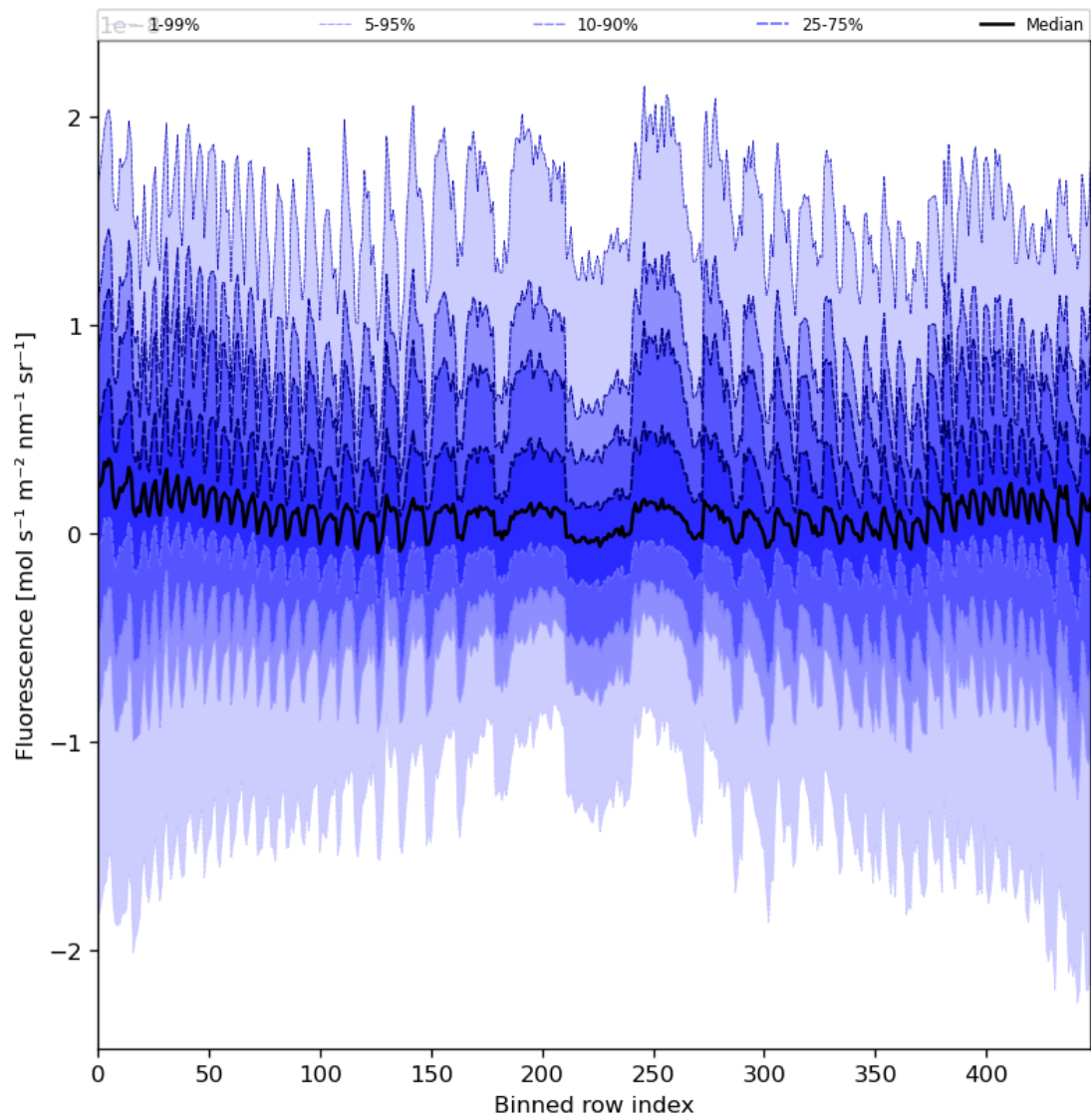
Figure 57: Along track statistics of “Fluorescence” for 2024-06-09 to 2024-06-11
