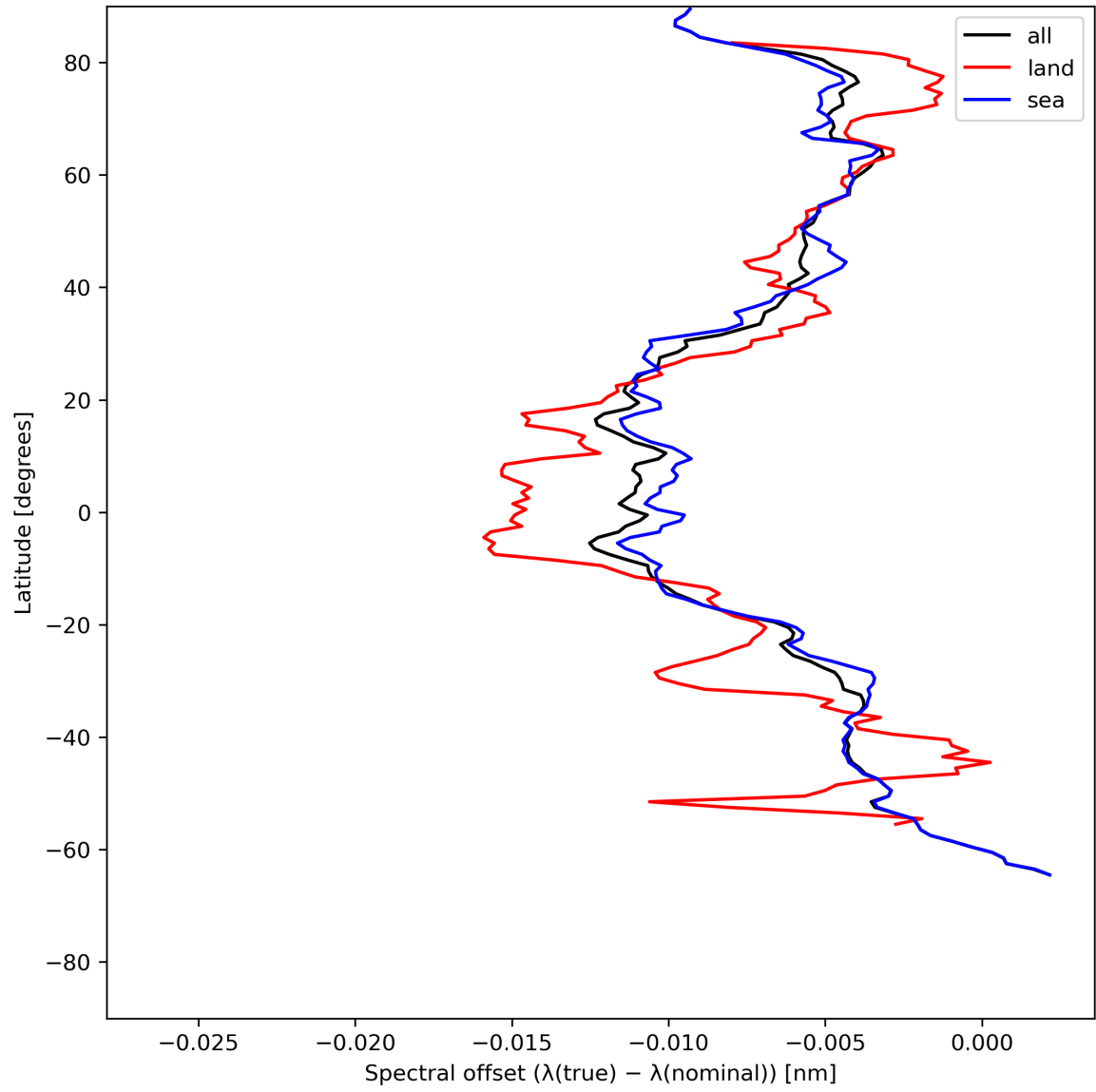
Figure 28: Zonal average of “Spectral offset ( \lambda(\text{true}) - \lambda(\text{nominal}) )” for 2024-06-09 to 2024-06-11.
