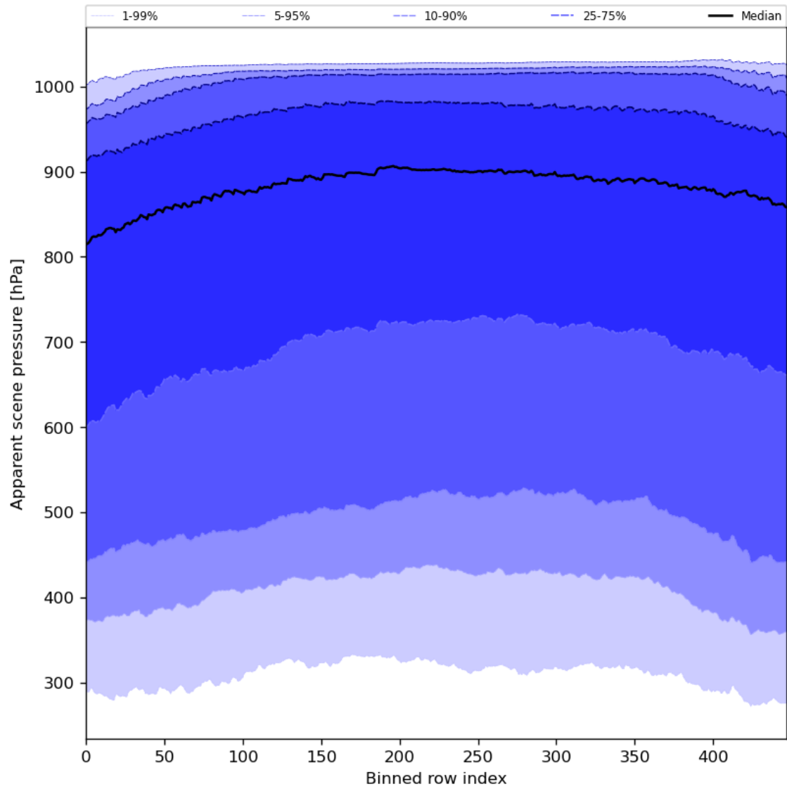
Figure 53: Along track statistics of “Apparent scene pressure” for 2024-06-09 to 2024-06-11
