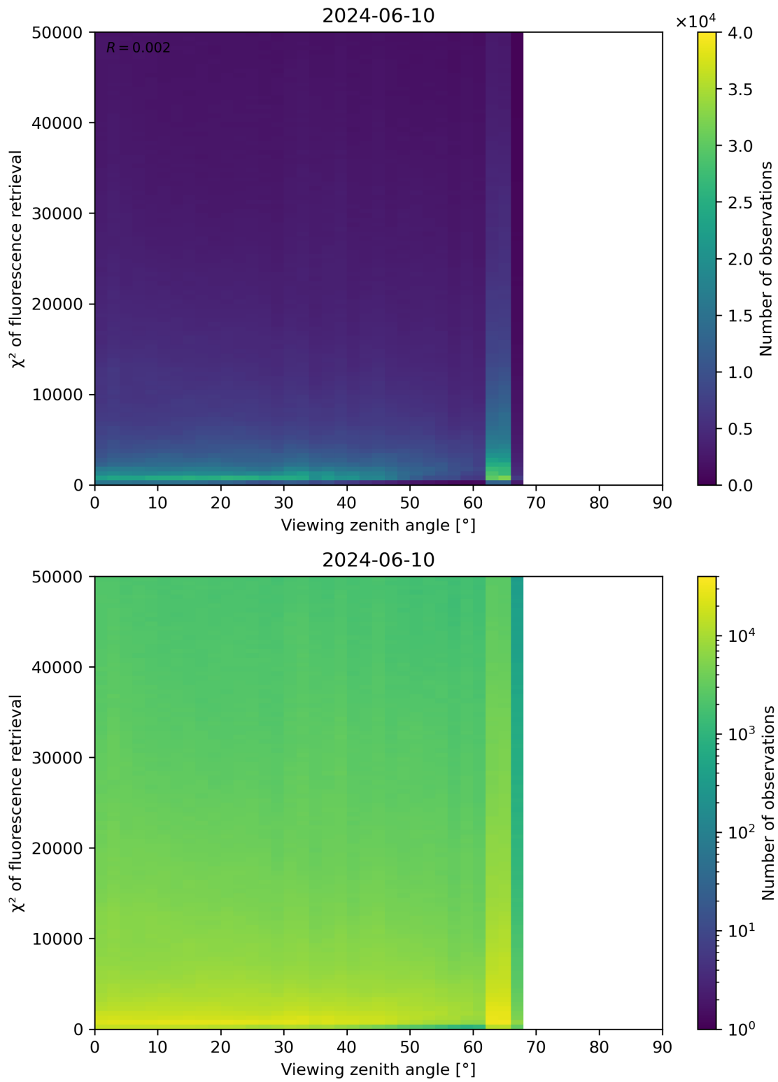
Figure 119: Scatter density plot of “Viewing zenith angle” against “ \chi^2 of fluorescence retrieval” for 2024-06-09 to 2024-06-11.
