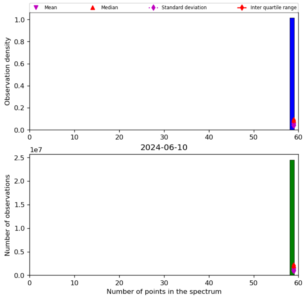
Figure 44: Histogram of “Number of points in the spectrum” for 2024-06-09 to 2024-06-11
