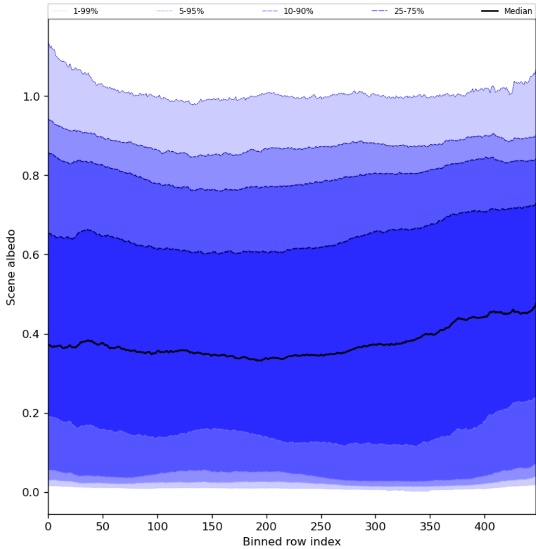
Figure 51: Along track statistics of “Scene albedo” for 2024-06-09 to 2024-06-11
