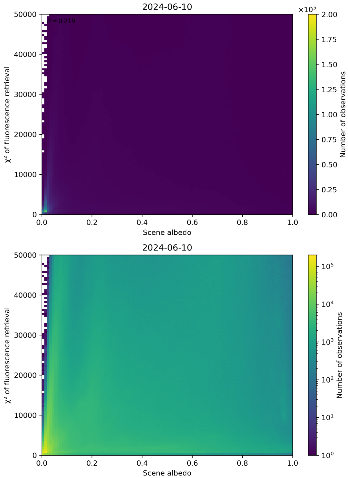
Figure 103: Scatter density plot of “Scene albedo” against “ \chi^2 of fluorescence retrieval” for 2024-06-09 to 2024-06-11.
