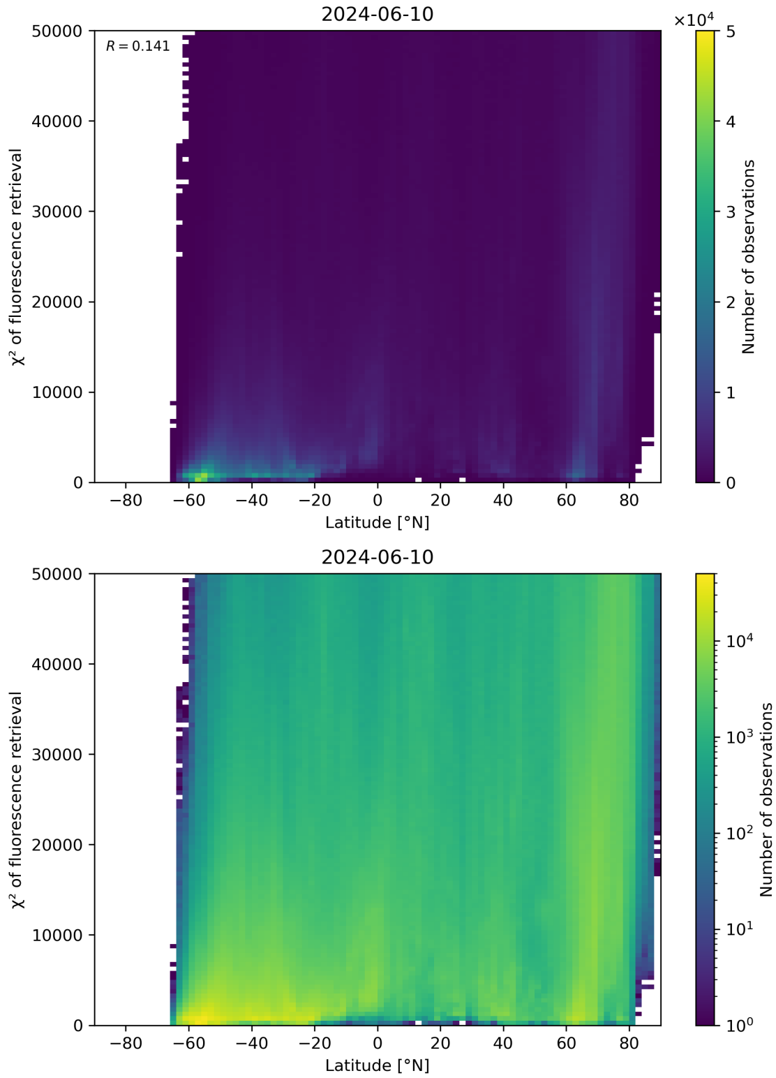
Figure 89: Scatter density plot of “Latitude” against “ \chi^2 of fluorescence retrieval” for 2024-06-09 to 2024-06-11.
