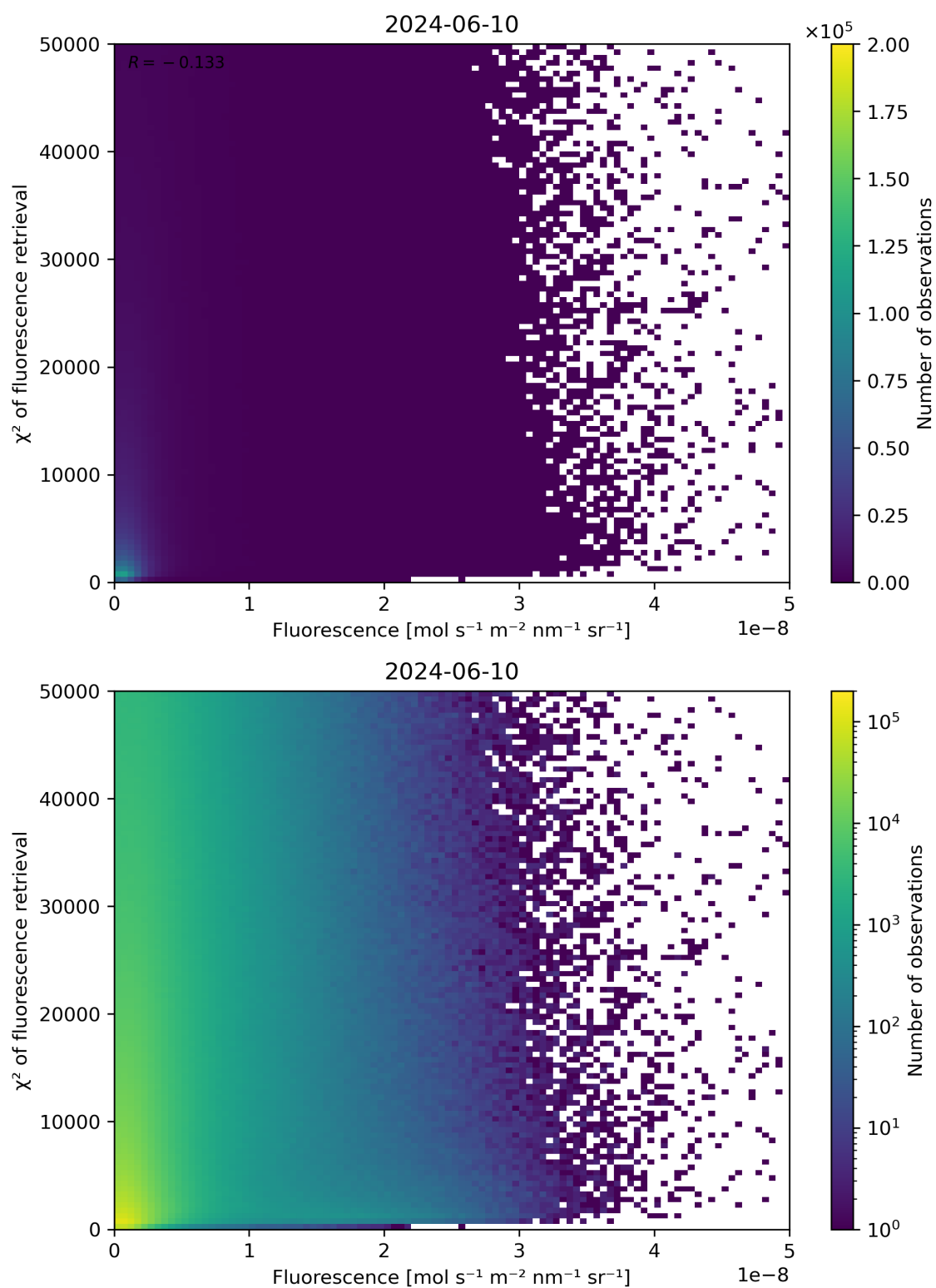
Figure 85: Scatter density plot of “Fluorescence” against “ \chi^2 of fluorescence retrieval” for 2024-06-09 to 2024-06-11.
