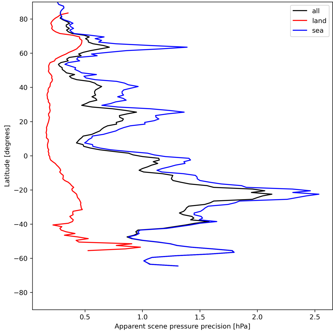
Figure 20: Zonal average of “Apparent scene pressure precision” for 2024-06-09 to 2024-06-11.
