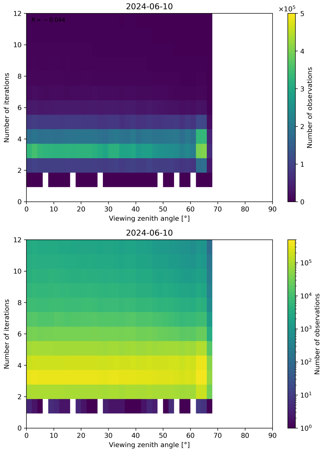
Figure 124: Scatter density plot of “Viewing zenith angle” against “Number of iterations” for 2024-06-09 to 2024-06-11.
