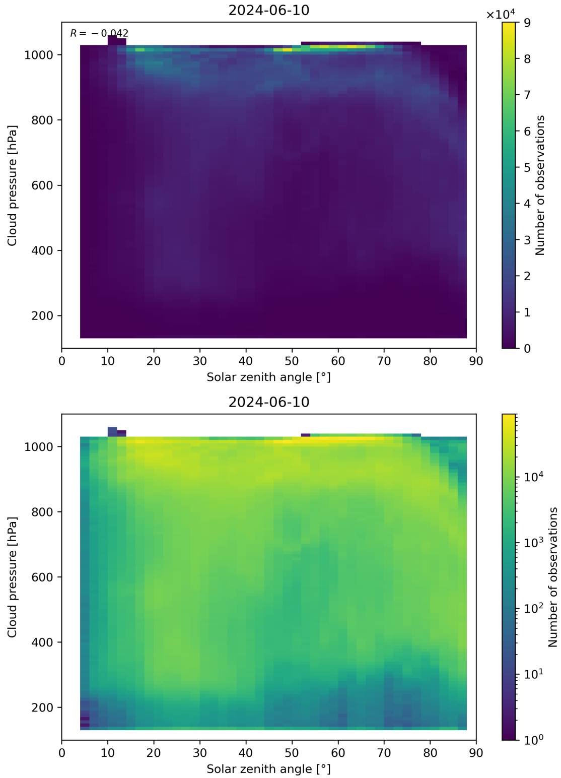
Figure 111: Scatter density plot of “Solar zenith angle” against “Cloud pressure” for 2024-06-09 to 2024-06-11.
