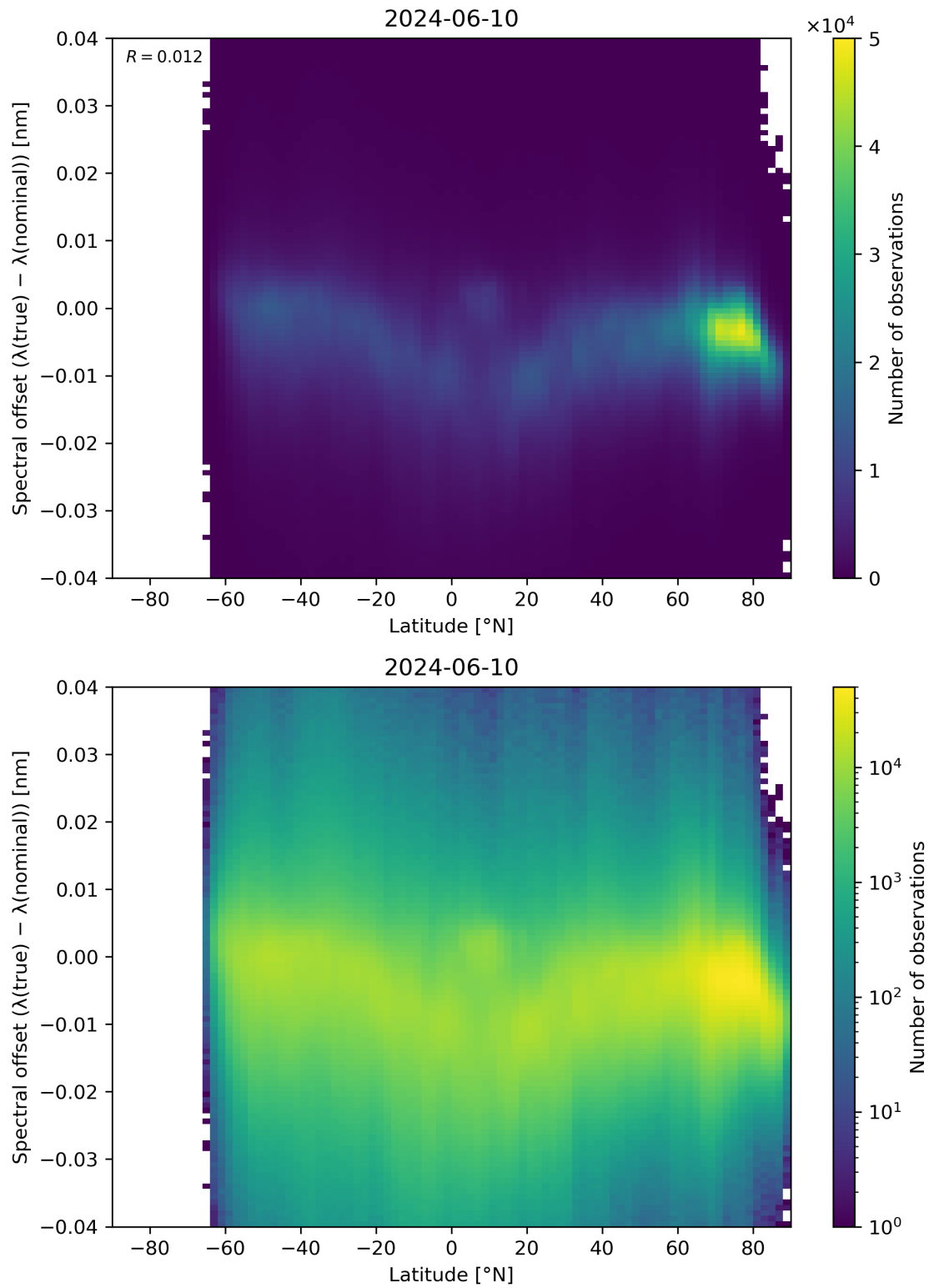
Figure 96: Scatter density plot of “Latitude” against “Spectral offset ( \lambda(\text{true}) - \lambda(\text{nominal}) )” for 2024-06-09 to 2024-06-11.
