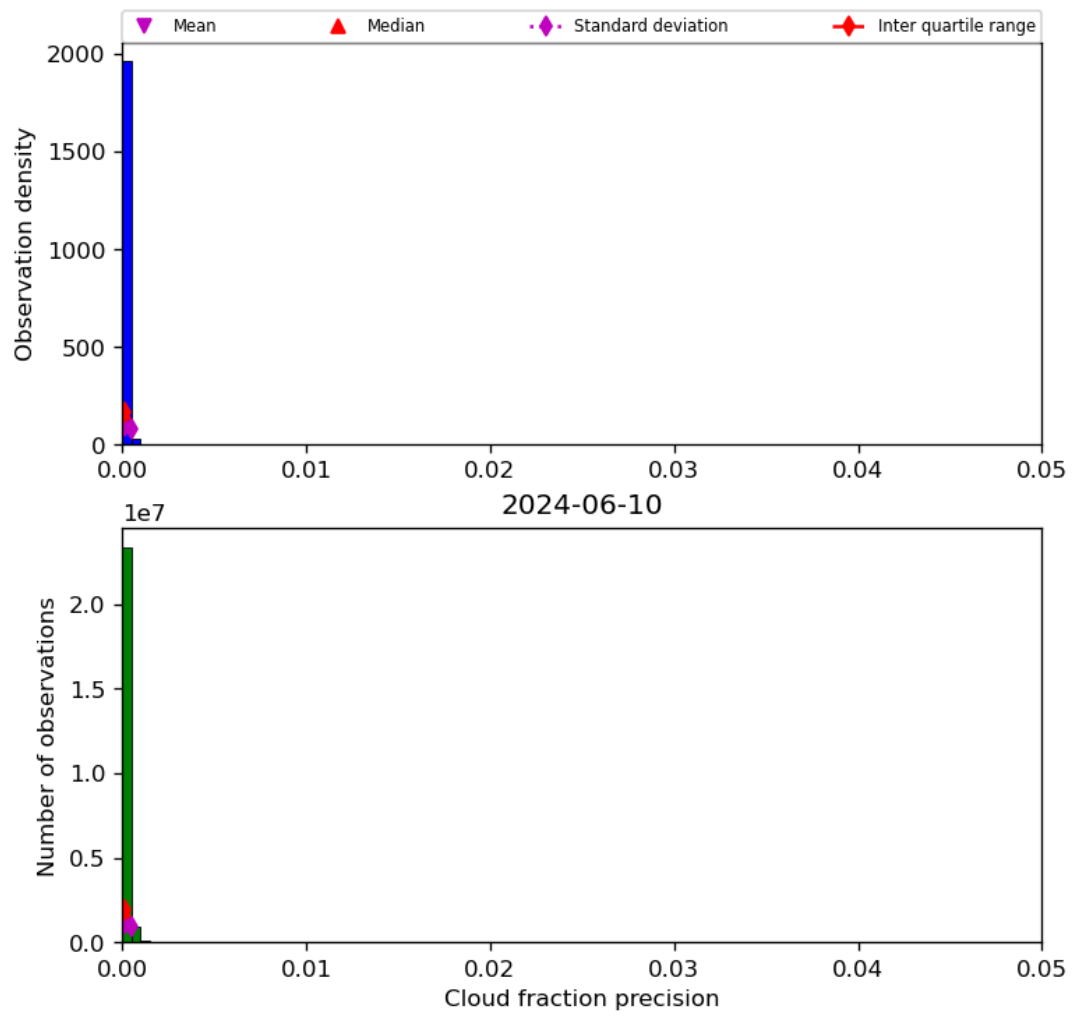
Figure 33: Histogram of “Cloud fraction precision” for 2024-06-09 to 2024-06-11
