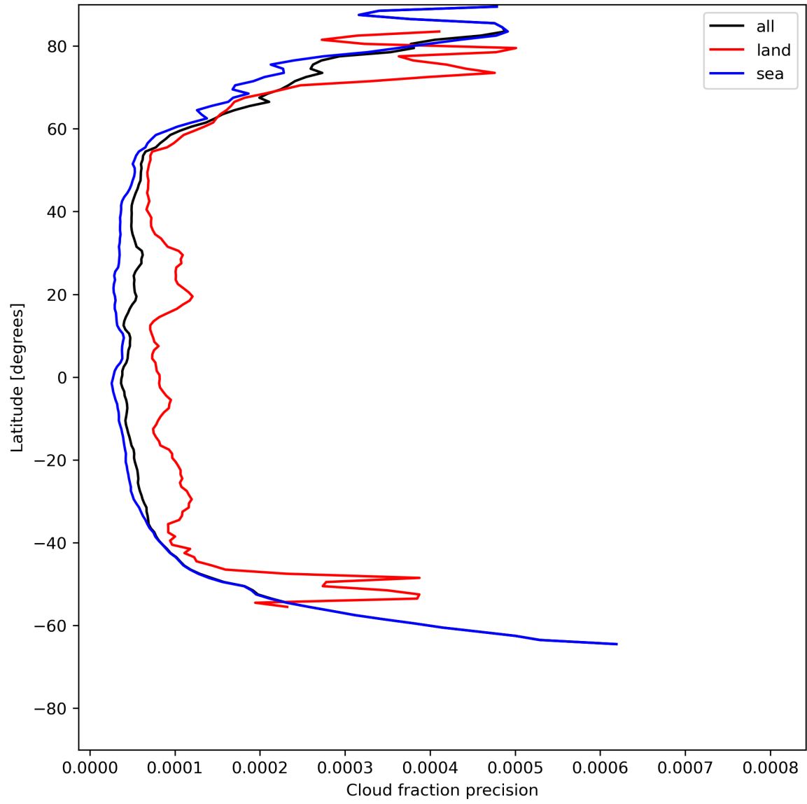
Figure 16: Zonal average of “Cloud fraction precision” for 2024-06-09 to 2024-06-11.
