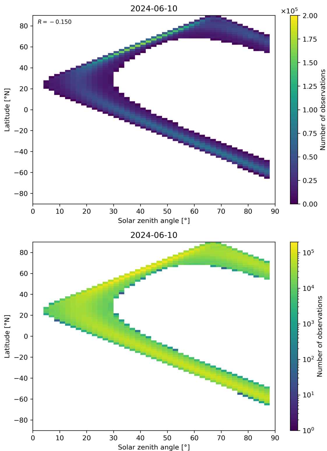
Figure 113: Scatter density plot of “Solar zenith angle” against “Latitude” for 2024-06-09 to 2024-06-11.
