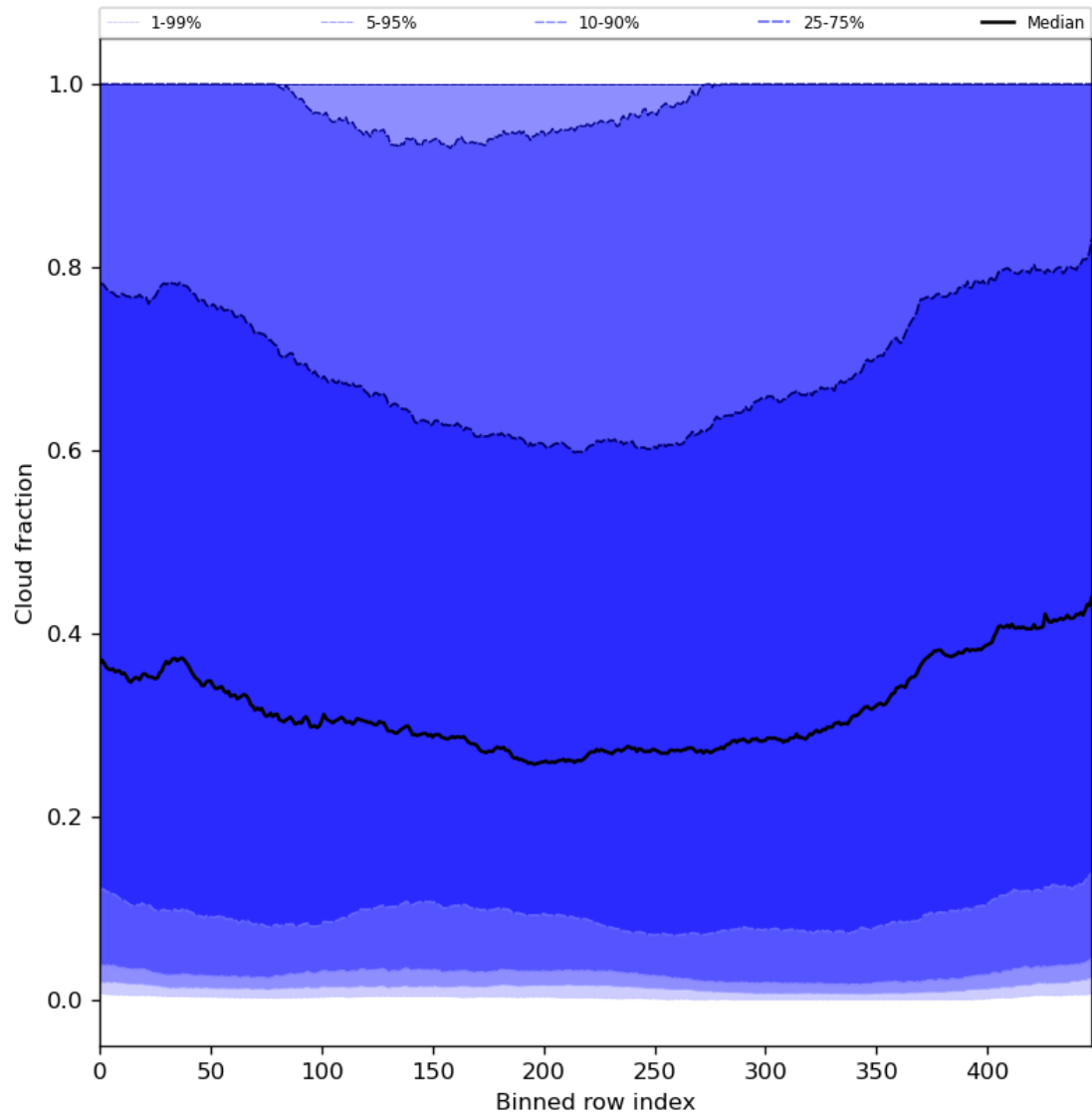
Figure 49: Along track statistics of “Cloud fraction” for 2024-06-09 to 2024-06-11
