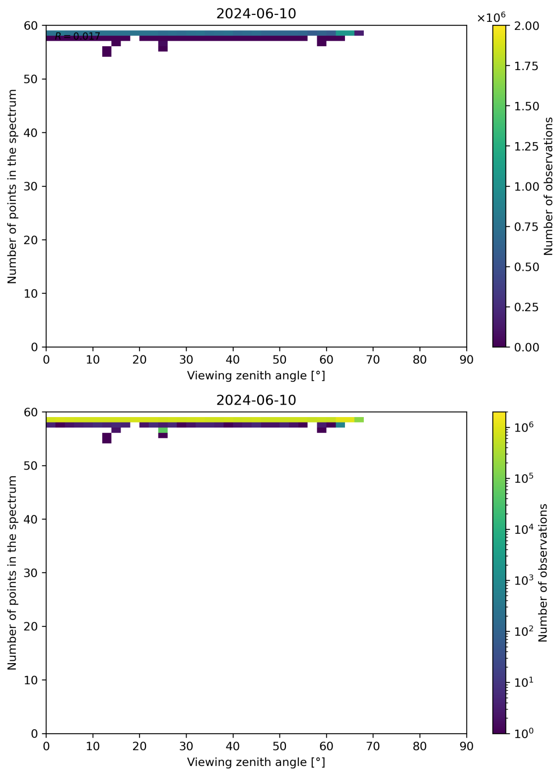
Figure 125: Scatter density plot of “Viewing zenith angle” against “Number of points in the spectrum” for 2024-06-09 to 2024-06-11.
