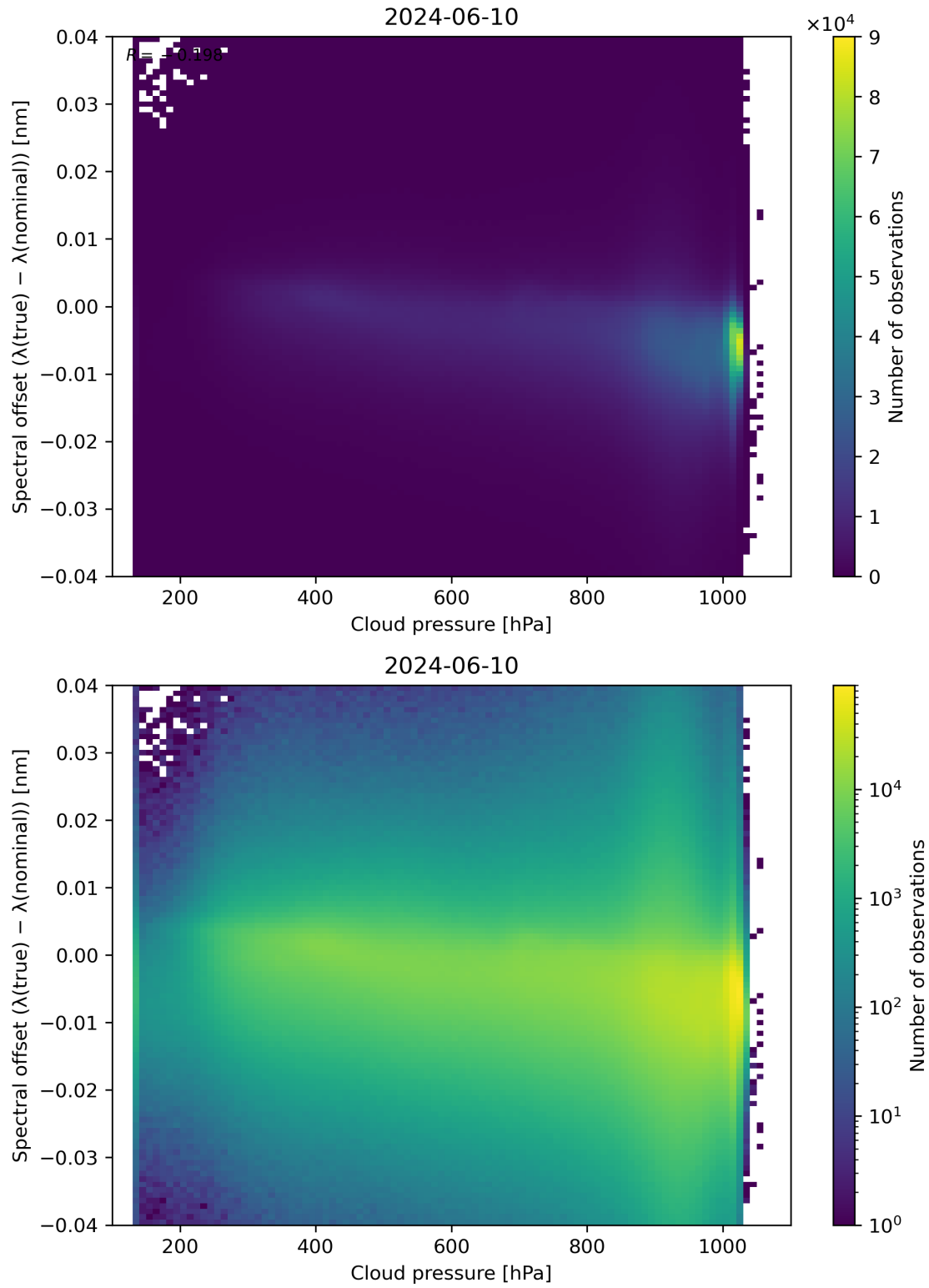
Figure 84: Scatter density plot of “Cloud pressure” against “Spectral offset ( \lambda(\text{true}) - \lambda(\text{nominal}) )” for 2024-06-09 to 2024-06-11.
