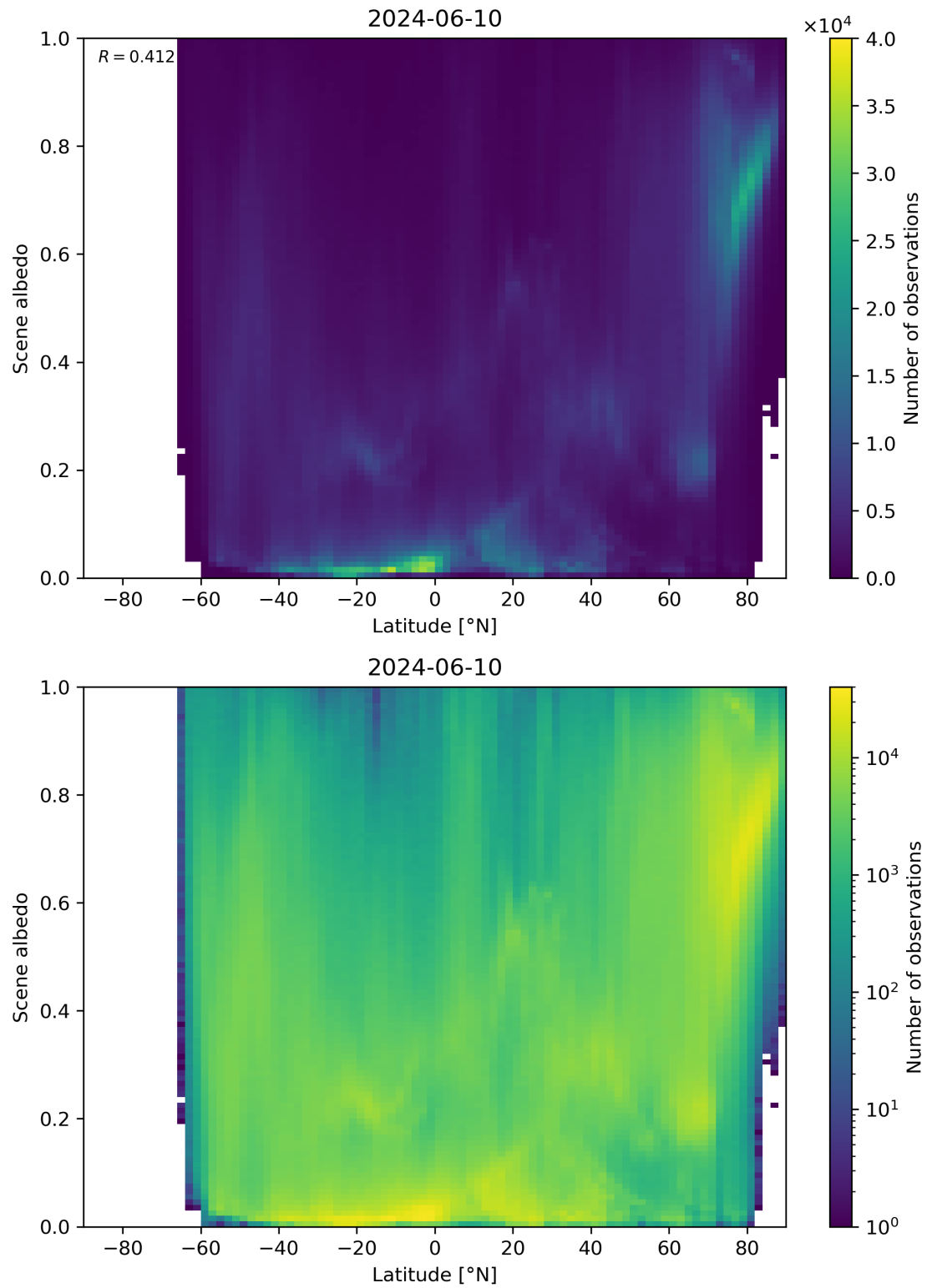
Figure 95: Scatter density plot of “Latitude” against “Scene albedo” for 2024-06-09 to 2024-06-11.
