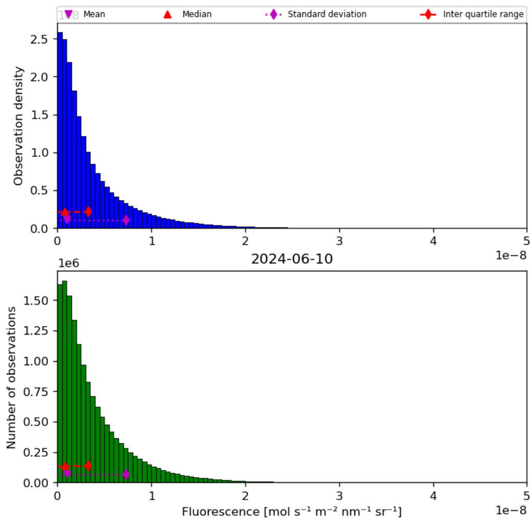
Figure 40: Histogram of “Fluorescence” for 2024-06-09 to 2024-06-11
