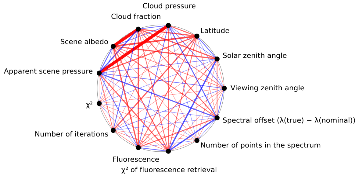
Figure 1: Map of correlation graph for 2024-06-09 to 2024-06-11.
