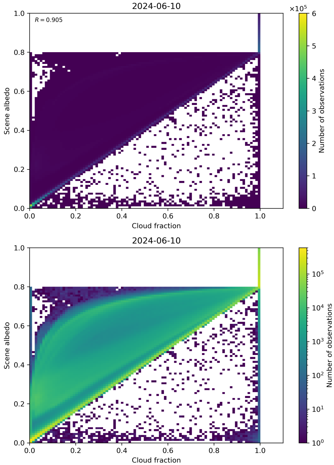
Figure 75: Scatter density plot of “Cloud fraction” against “Scene albedo” for 2024-06-09 to 2024-06-11.
