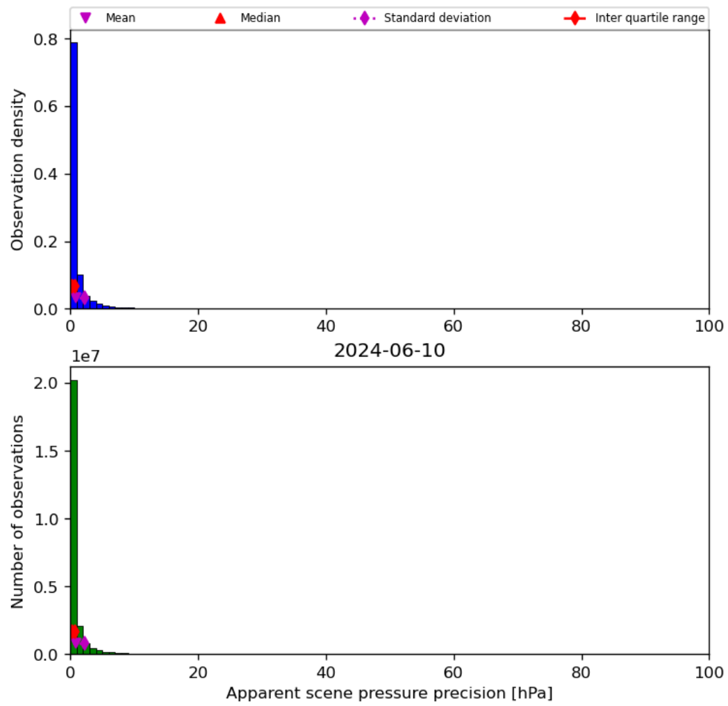
Figure 37: Histogram of “Apparent scene pressure precision” for 2024-06-09 to 2024-06-11
