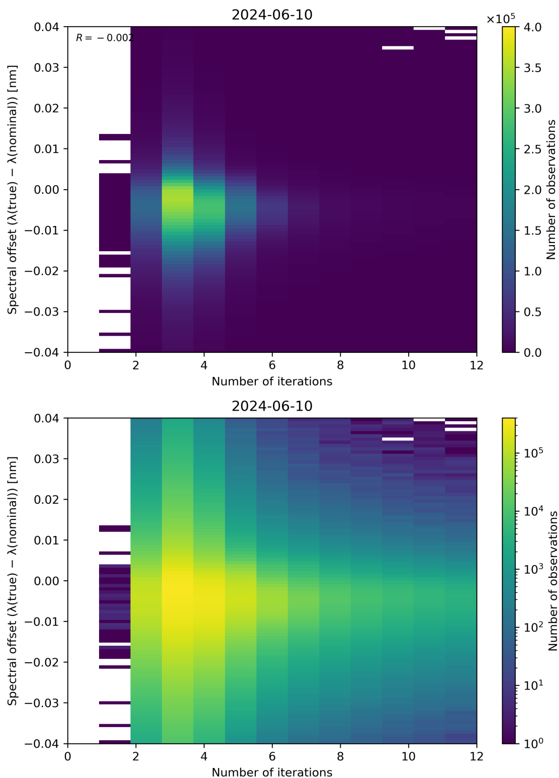
Figure 100: Scatter density plot of “Number of iterations” against “Spectral offset ( \lambda(\text{true}) - \lambda(\text{nominal}) )” for 2024-06-09 to 2024-06-11.
