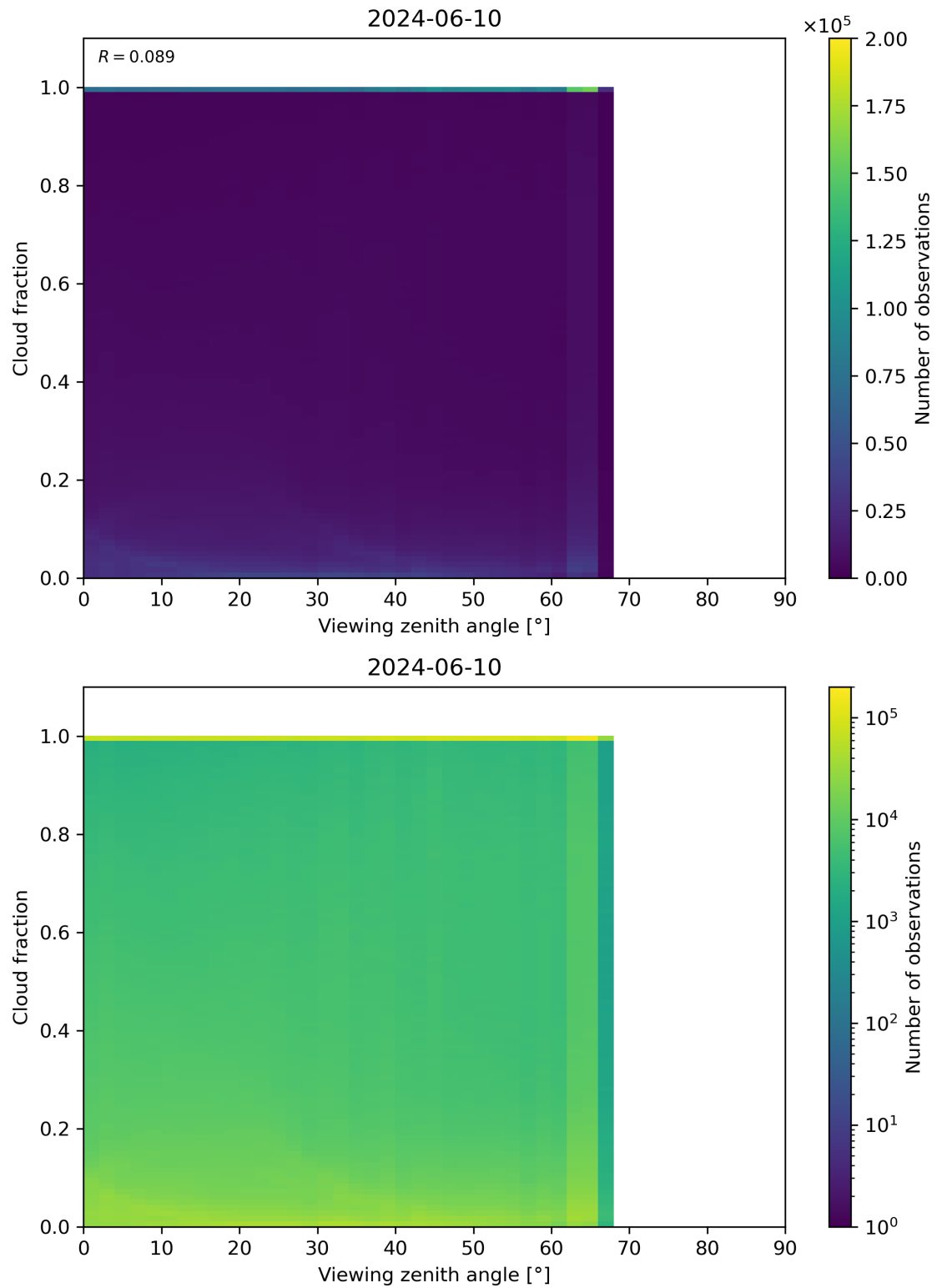
Figure 120: Scatter density plot of “Viewing zenith angle” against “Cloud fraction” for 2024-06-09 to 2024-06-11.
