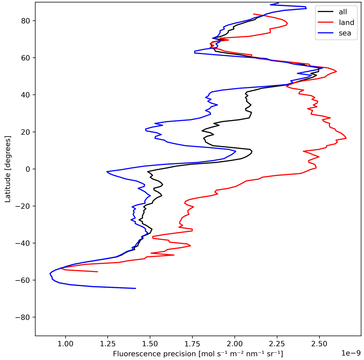
Figure 24: Zonal average of “Fluorescence precision” for 2024-06-09 to 2024-06-11.
