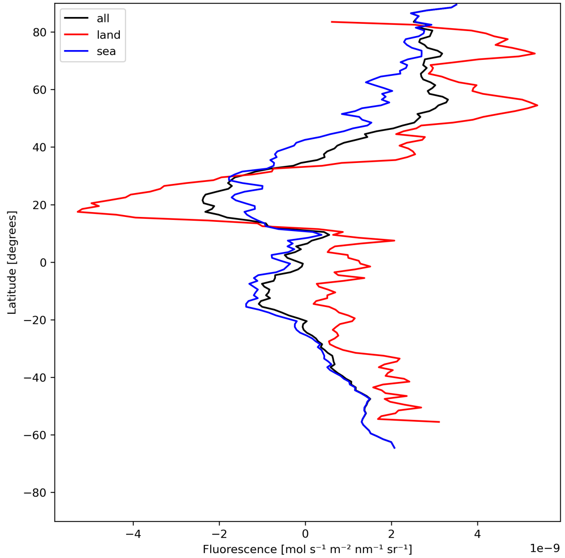
Figure 23: Zonal average of “Fluorescence” for 2024-06-09 to 2024-06-11.
