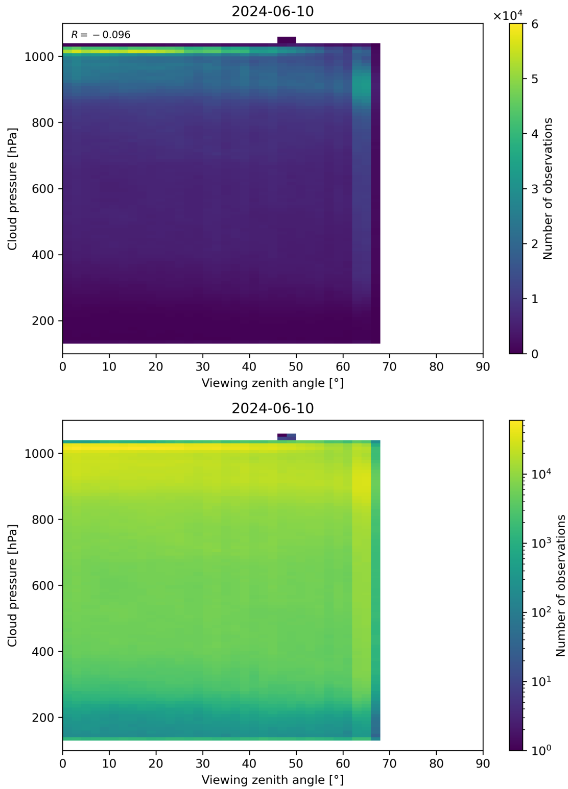
Figure 121: Scatter density plot of “Viewing zenith angle” against “Cloud pressure” for 2024-06-09 to 2024-06-11.
