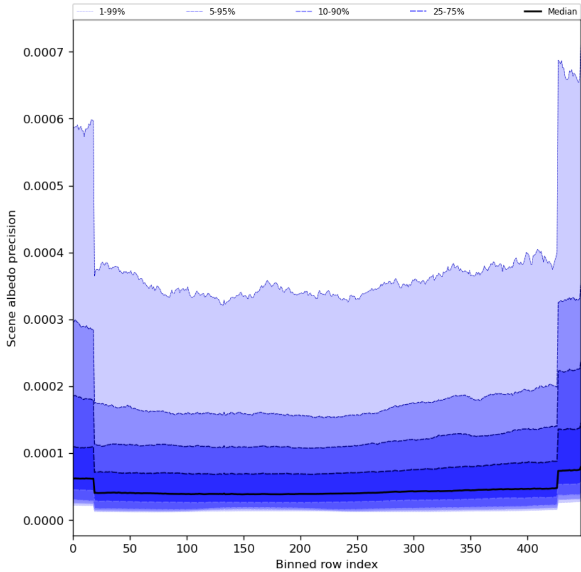
Figure 52: Along track statistics of “Scene albedo precision” for 2024-06-09 to 2024-06-11
