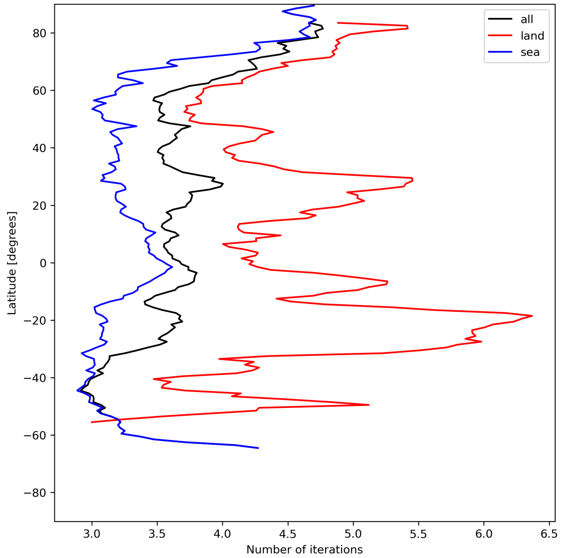
Figure 22: Zonal average of “Number of iterations” for 2024-06-09 to 2024-06-11.
