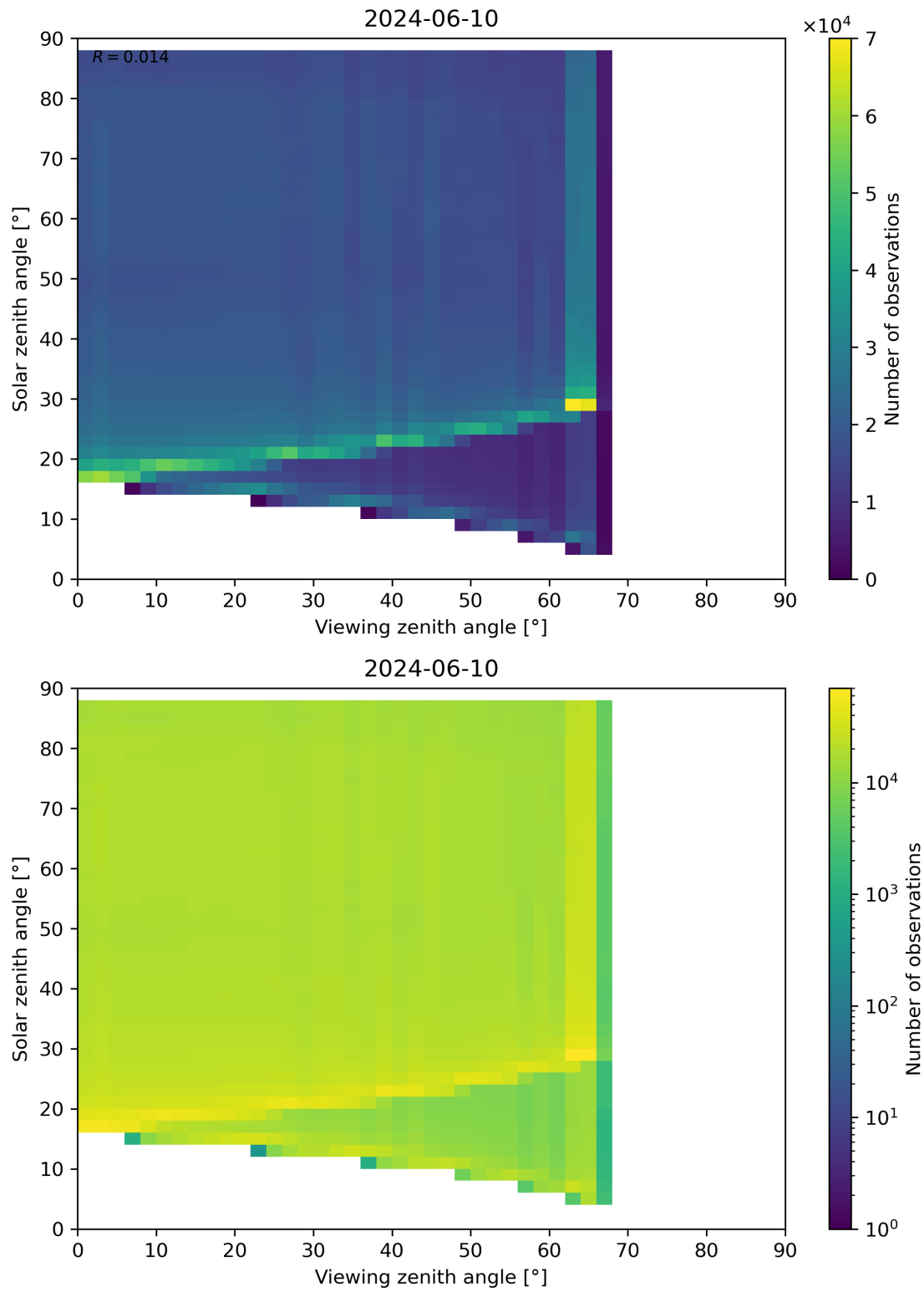
Figure 127: Scatter density plot of “Viewing zenith angle” against “Solar zenith angle” for 2024-06-09 to 2024-06-11.
