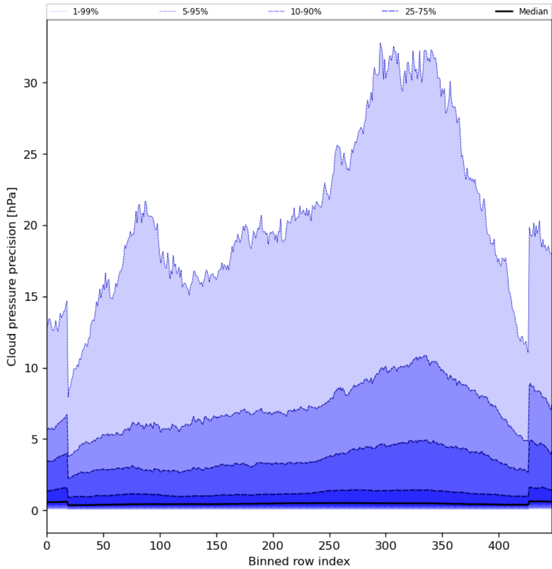
Figure 48: Along track statistics of “Cloud pressure precision” for 2024-06-09 to 2024-06-11
