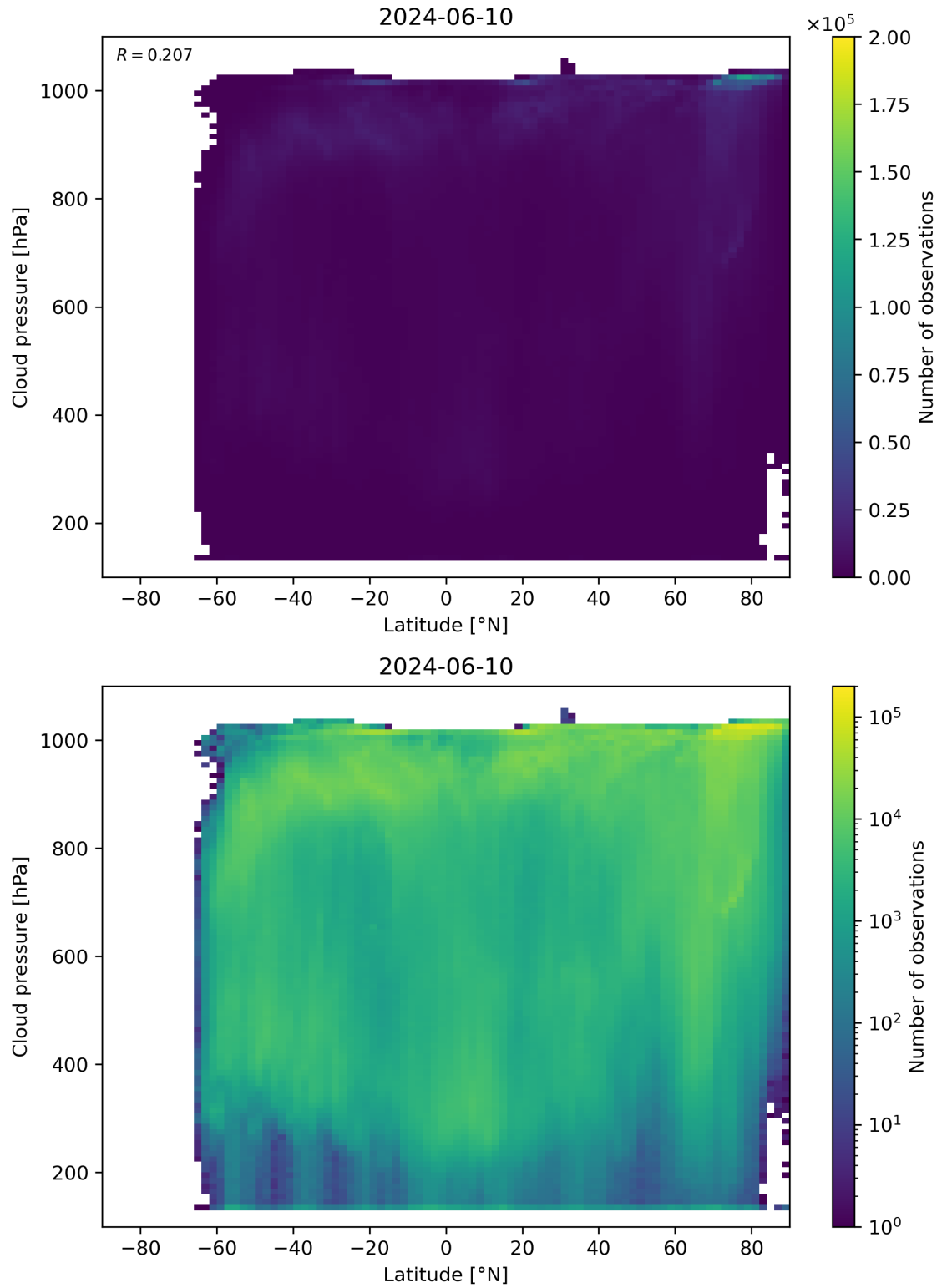
Figure 91: Scatter density plot of “Latitude” against “Cloud pressure” for 2024-06-09 to 2024-06-11.
