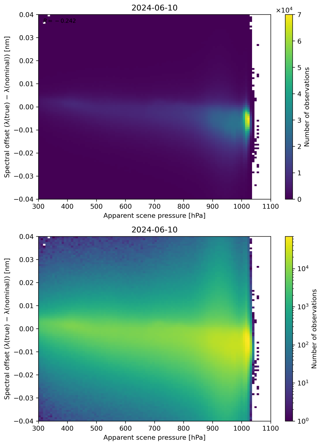
Figure 67: Scatter density plot of “Apparent scene pressure” against “Spectral offset ( \lambda(\text{true}) - \lambda(\text{nominal}) )” for 2024-06-09 to 2024-06-11.
