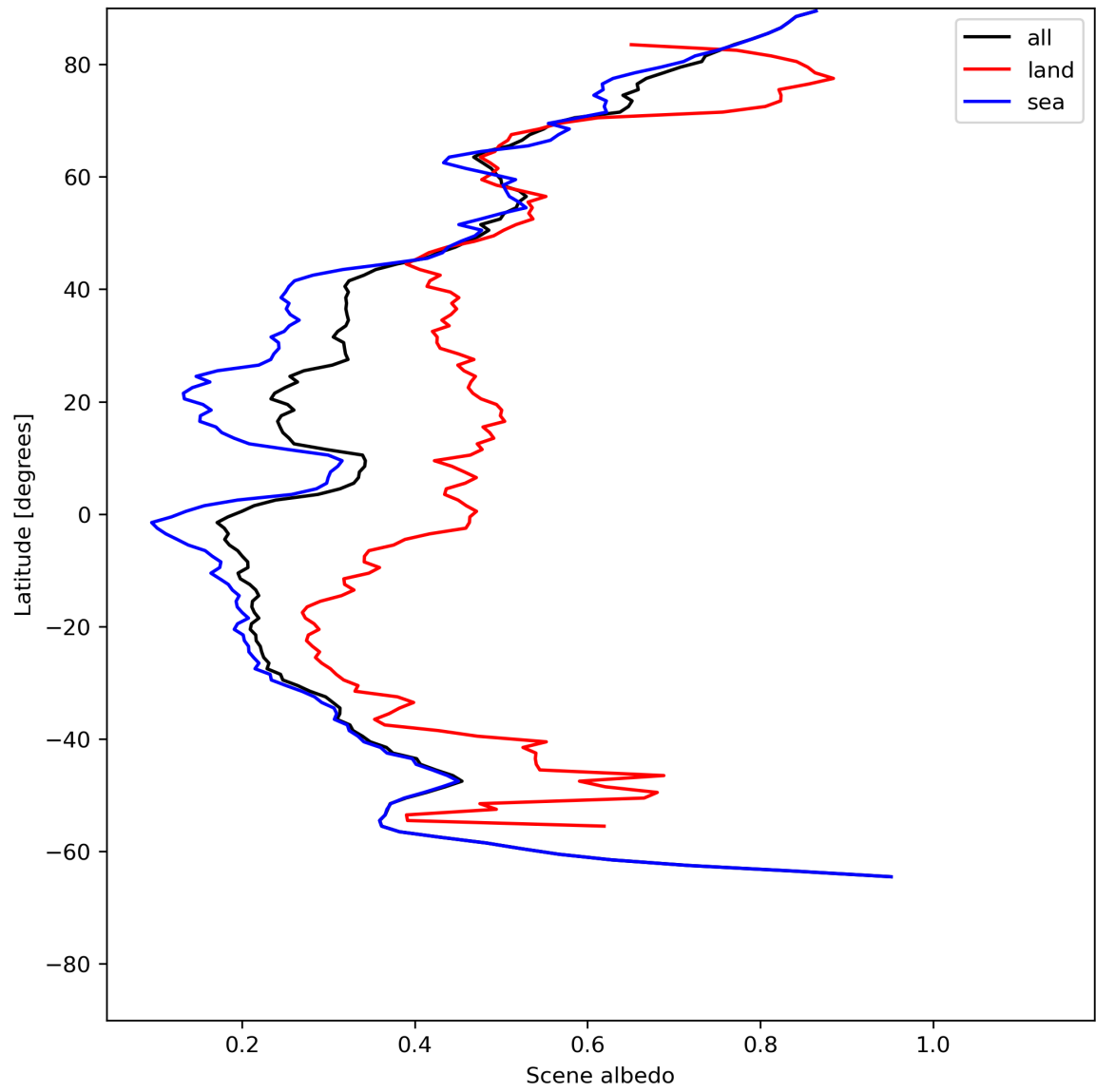
Figure 17: Zonal average of “Scene albedo” for 2024-06-09 to 2024-06-11.
