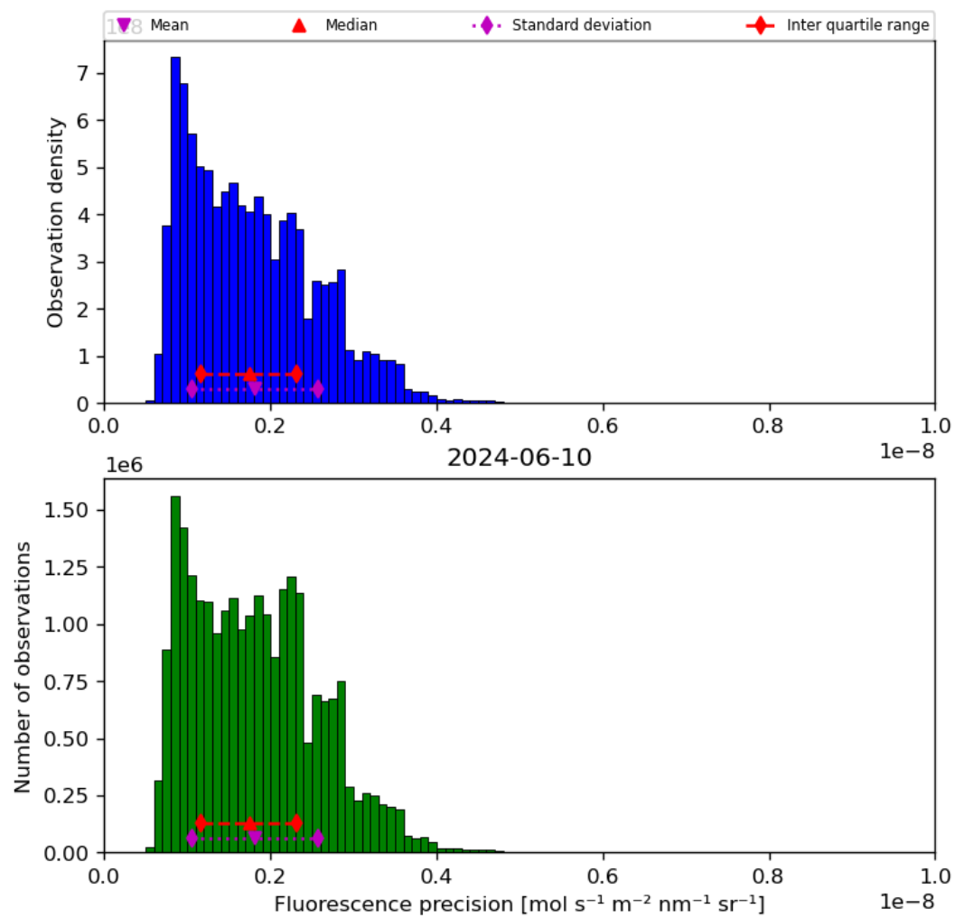
Figure 41: Histogram of “Fluorescence precision” for 2024-06-09 to 2024-06-11
