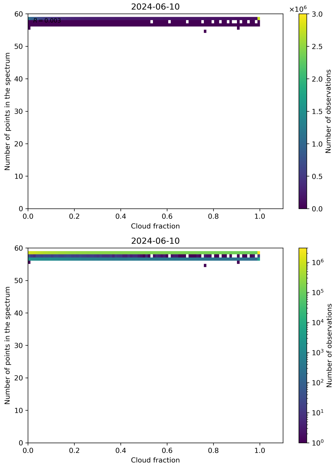
Figure 74: Scatter density plot of “Cloud fraction” against “Number of points in the spectrum” for 2024-06-09 to 2024-06-11.
