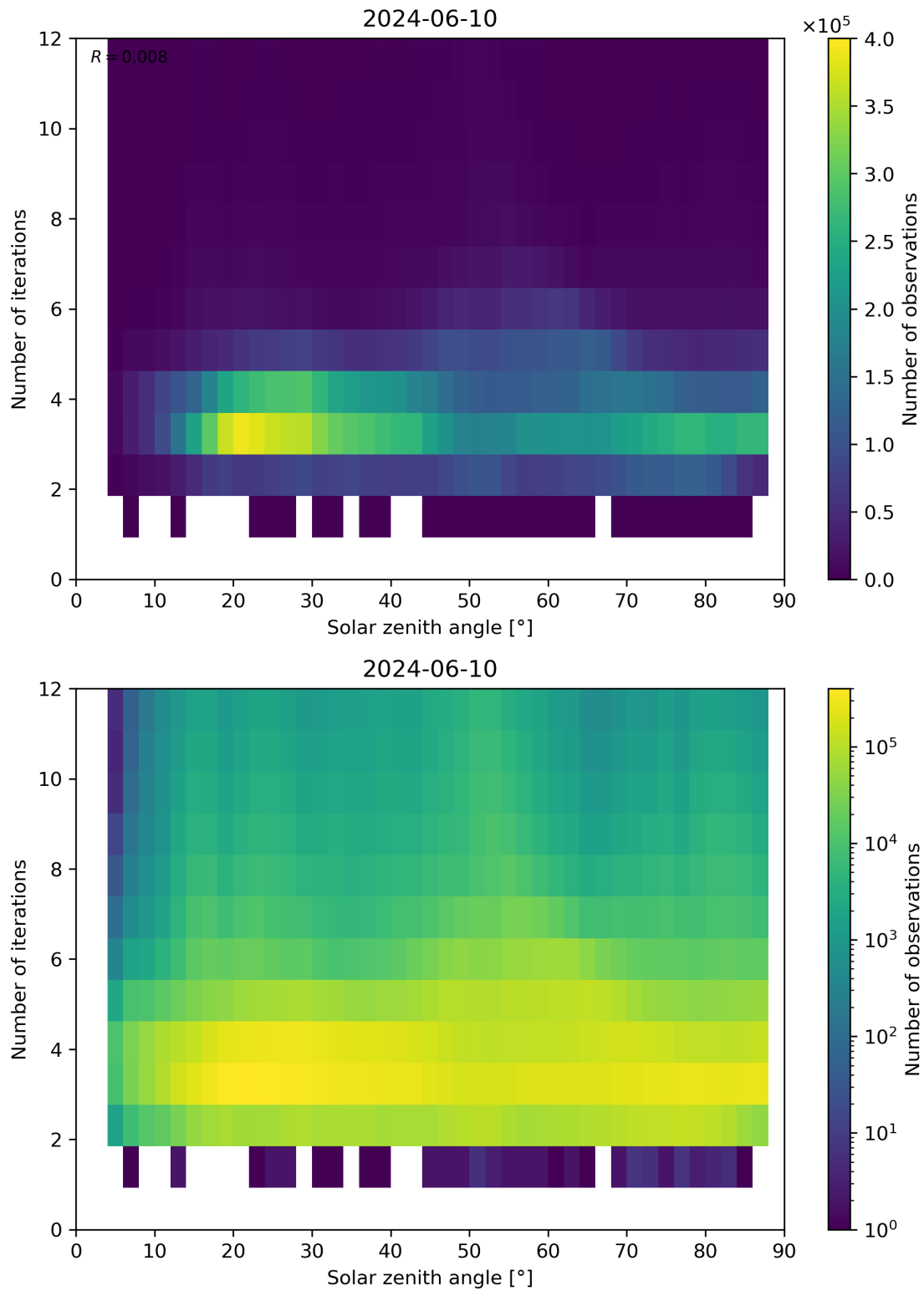
Figure 114: Scatter density plot of “Solar zenith angle” against “Number of iterations” for 2024-06-09 to 2024-06-11.
