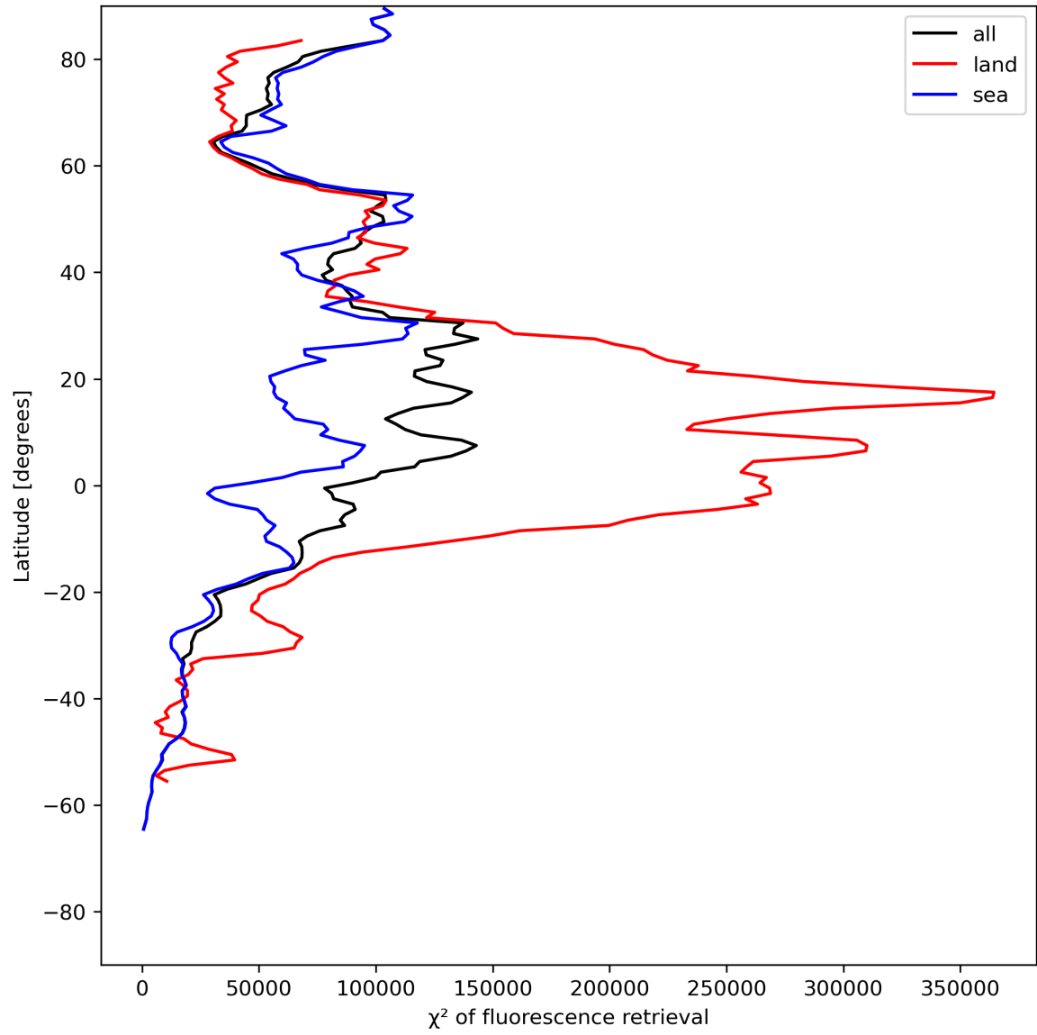
Figure 25: Zonal average of “ \chi^2 of fluorescence retrieval” for 2024-06-09 to 2024-06-11.
