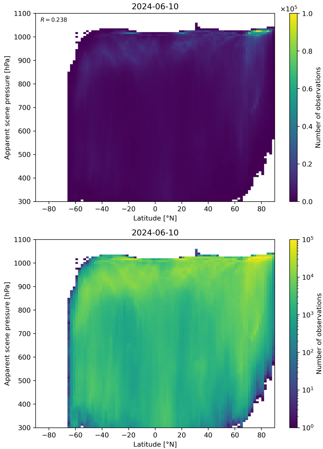
Figure 88: Scatter density plot of “Latitude” against “Apparent scene pressure” for 2024-06-09 to 2024-06-11.
