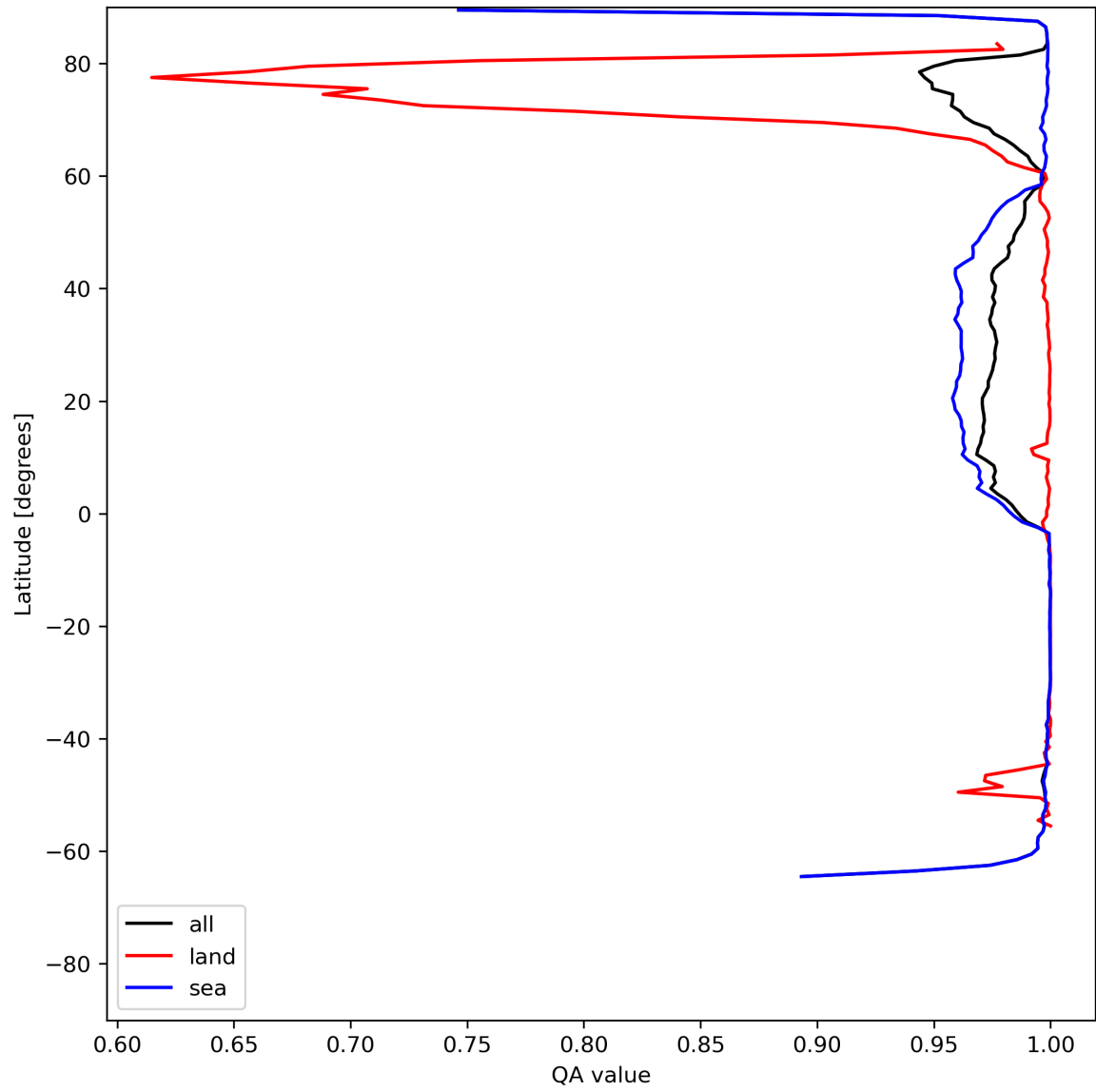
Figure 12: Zonal average of “QA value” for 2024-06-09 to 2024-06-11.
