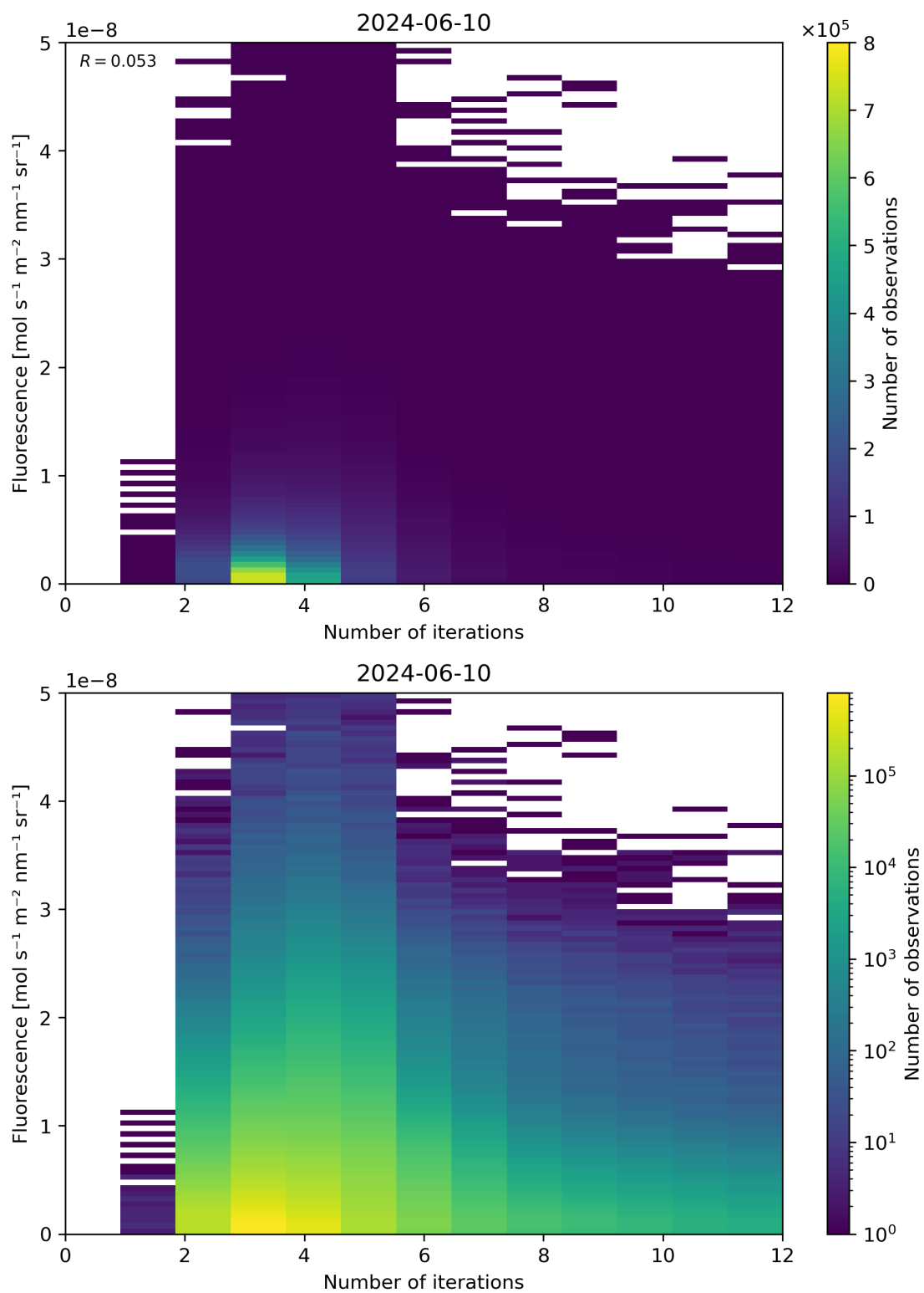
Figure 98: Scatter density plot of “Number of iterations” against “Fluorescence” for 2024-06-09 to 2024-06-11.
