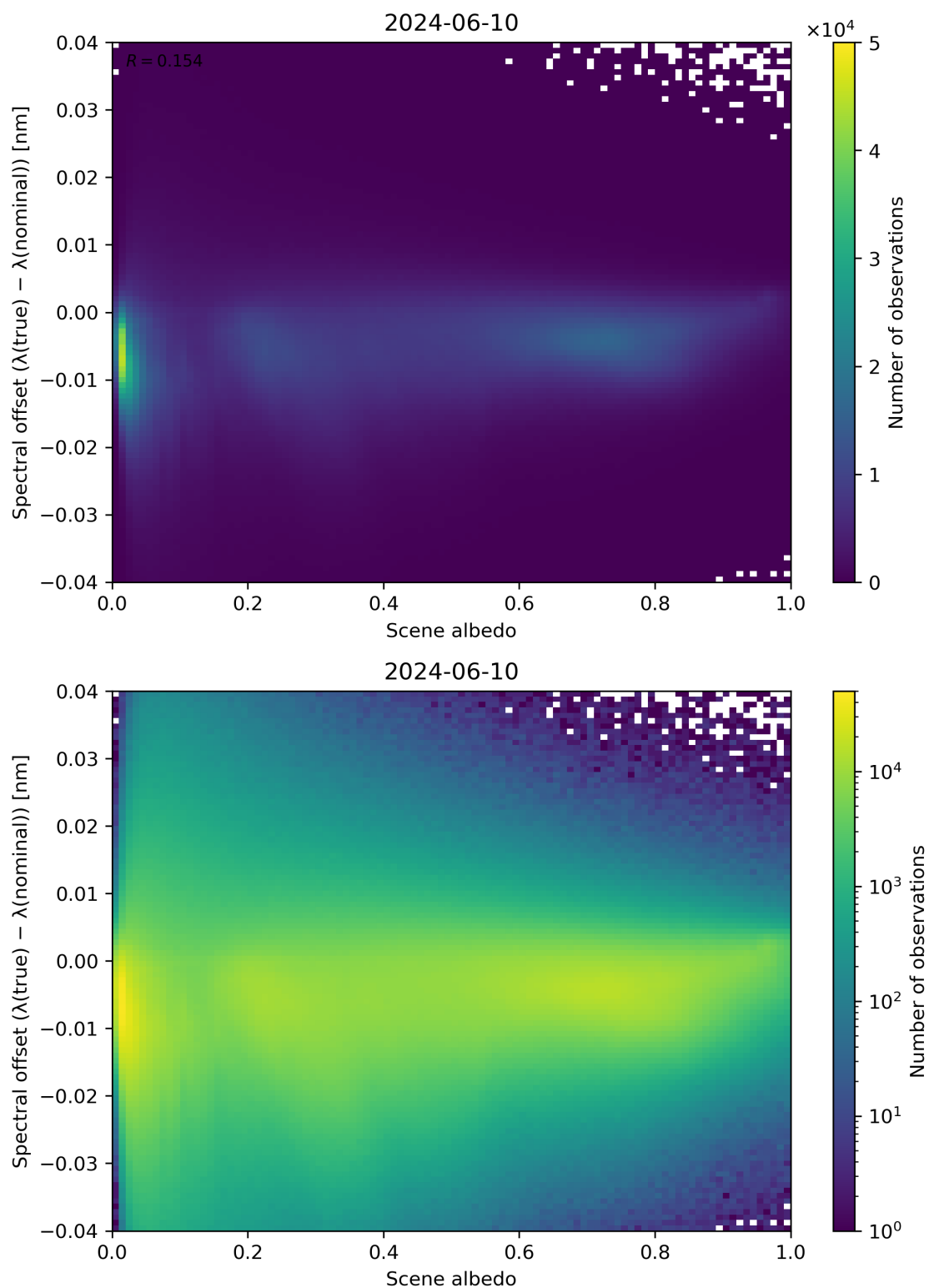
Figure 107: Scatter density plot of “Scene albedo” against “Spectral offset ( \lambda(\text{true}) - \lambda(\text{nominal}) )” for 2024-06-09 to 2024-06-11.
