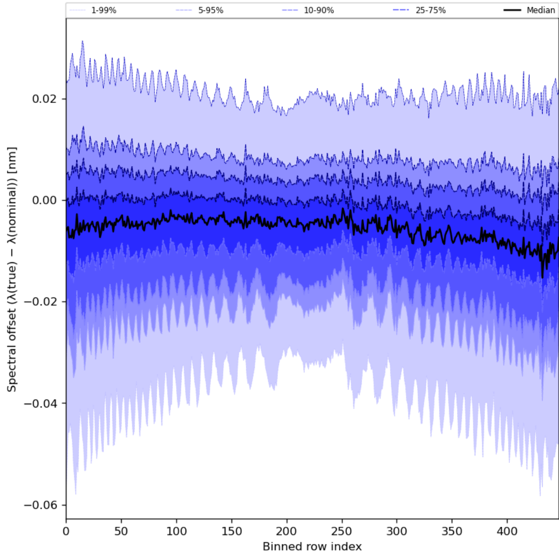
Figure 62: Along track statistics of “Spectral offset ( \lambda(\text{true}) - \lambda(\text{nominal}) )” for 2024-06-09 to 2024-06-11
