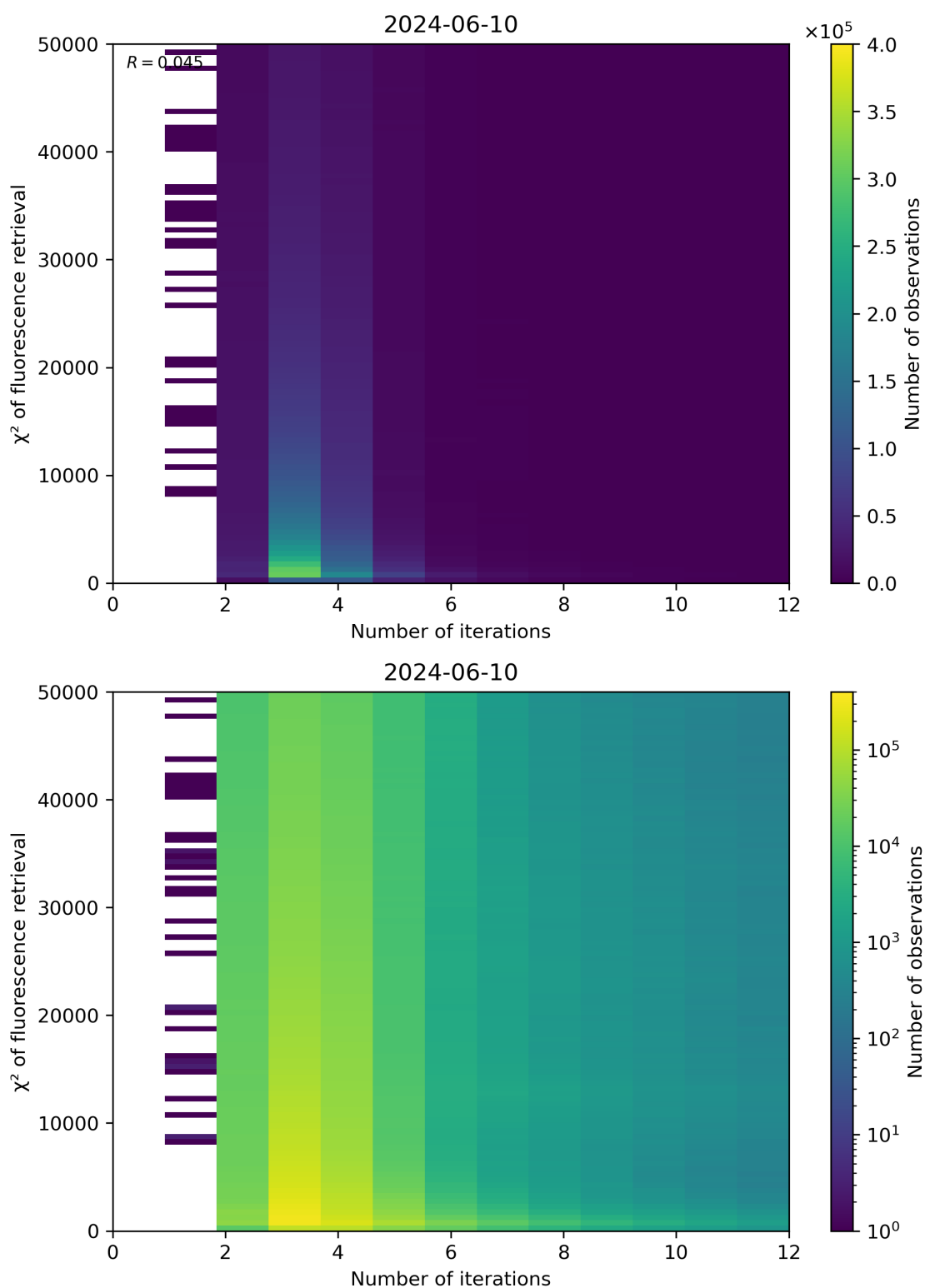
Figure 97: Scatter density plot of “Number of iterations” against “ \chi^2 of fluorescence retrieval” for 2024-06-09 to 2024-06-11.
