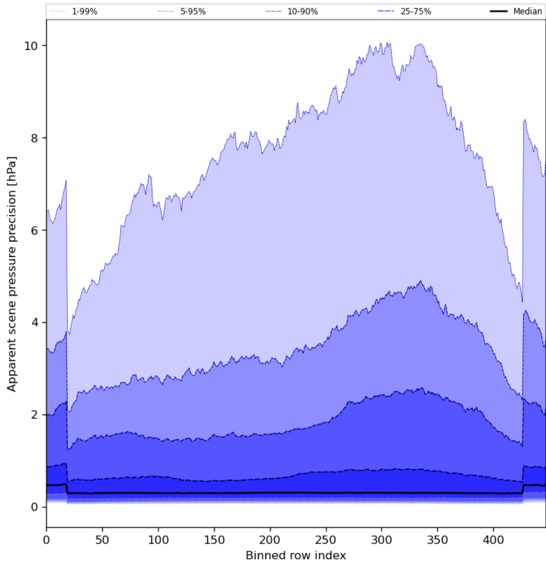
Figure 54: Along track statistics of “Apparent scene pressure precision” for 2024-06-09 to 2024-06-11
