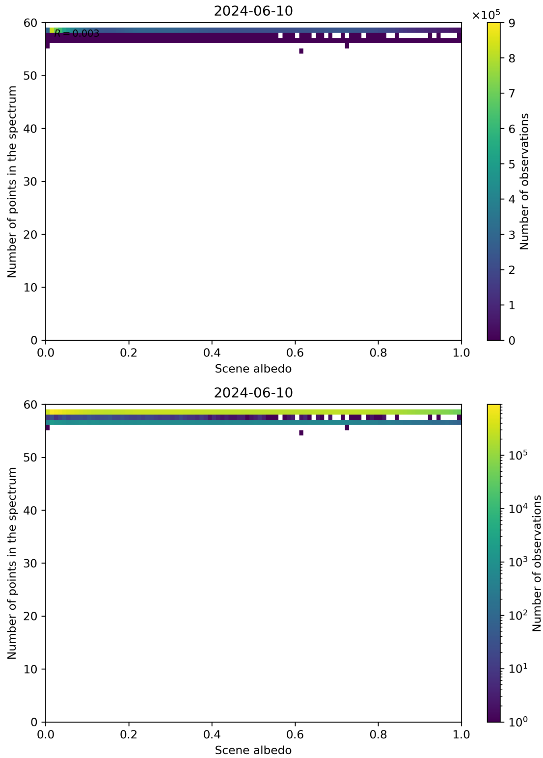
Figure 106: Scatter density plot of “Scene albedo” against “Number of points in the spectrum” for 2024-06-09 to 2024-06-11.
