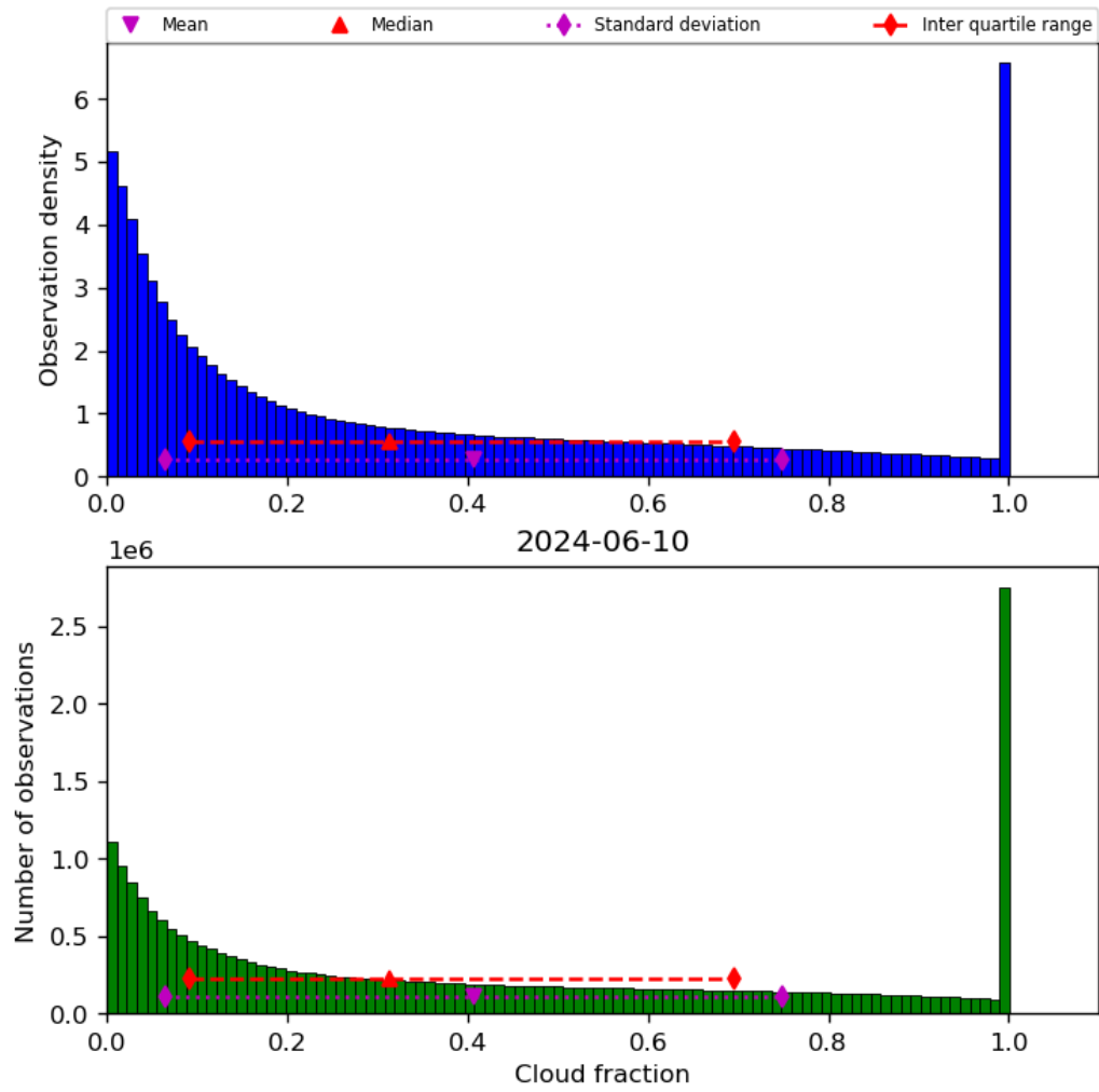
Figure 32: Histogram of “Cloud fraction” for 2024-06-09 to 2024-06-11
