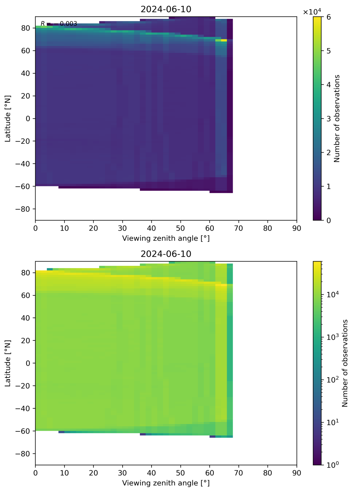
Figure 123: Scatter density plot of “Viewing zenith angle” against “Latitude” for 2024-06-09 to 2024-06-11.
