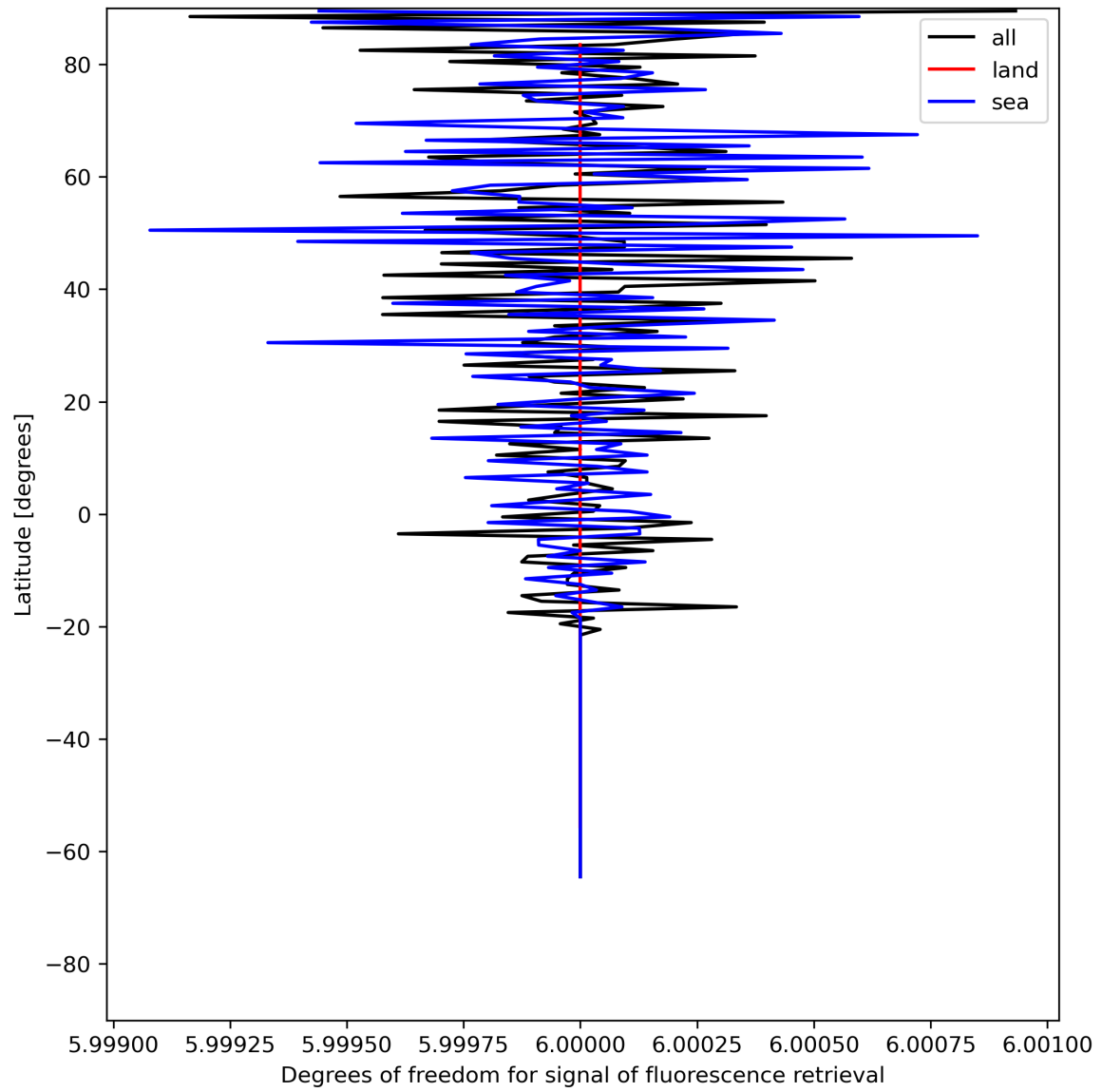
Figure 26: Zonal average of “Degrees of freedom for signal of fluorescence retrieval” for 2024-06-09 to 2024-06-11.
