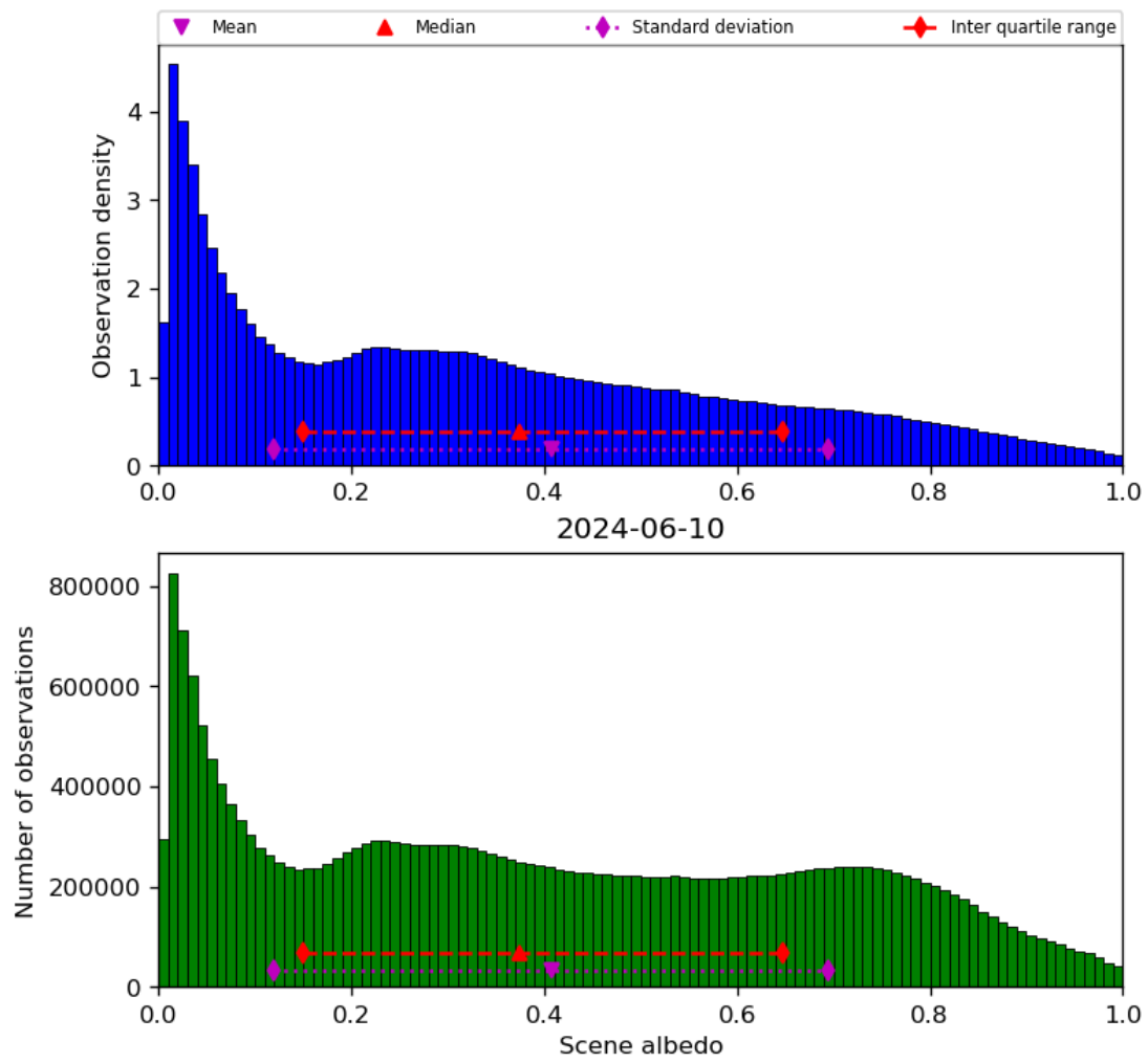
Figure 34: Histogram of “Scene albedo” for 2024-06-09 to 2024-06-11
