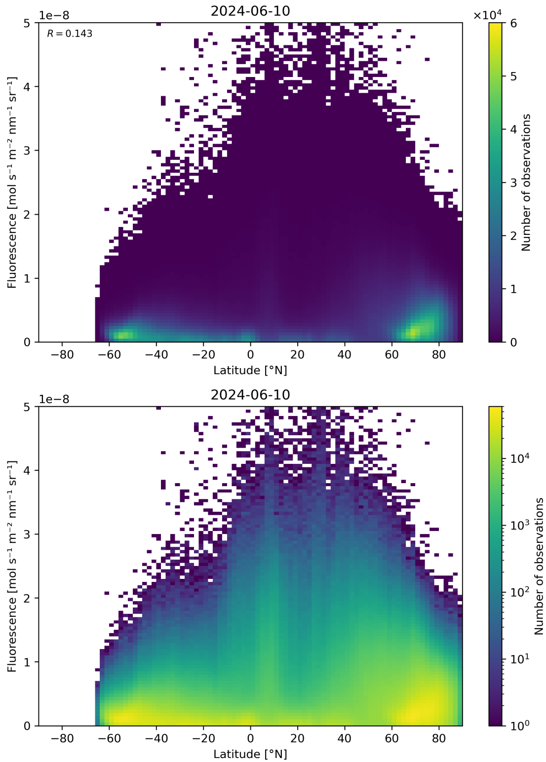
Figure 92: Scatter density plot of “Latitude” against “Fluorescence” for 2024-06-09 to 2024-06-11.
