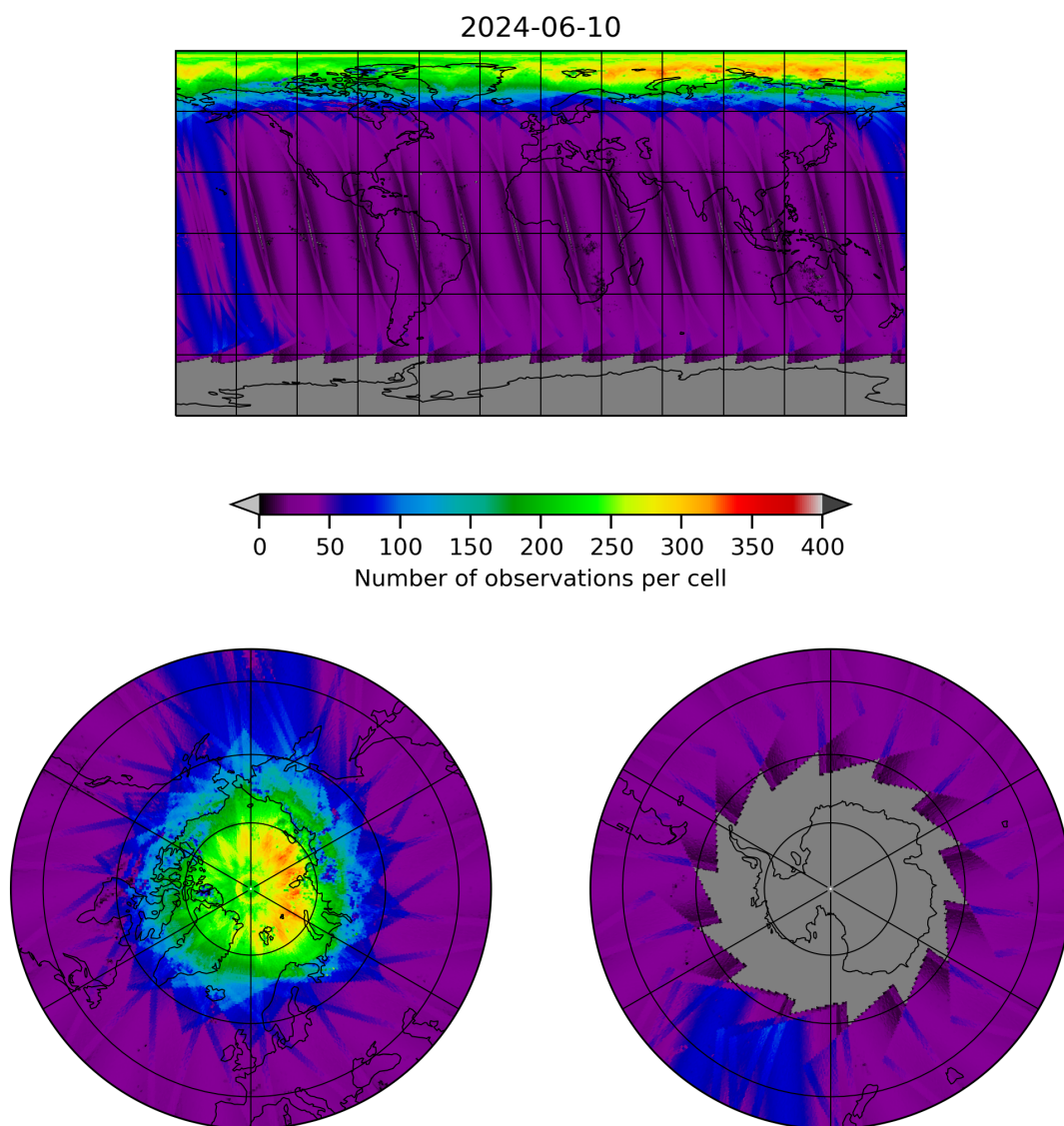
Figure 11: Map of the number of observations for 2024-06-09 to 2024-06-11
