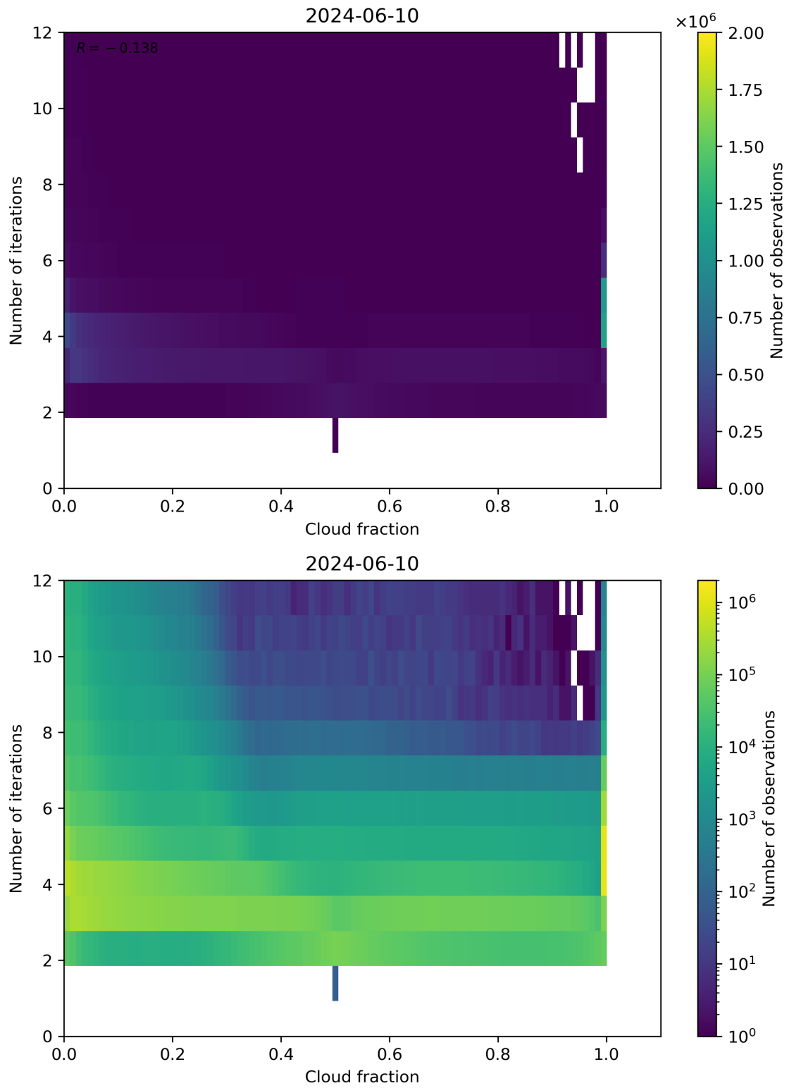
Figure 73: Scatter density plot of “Cloud fraction” against “Number of iterations” for 2024-06-09 to 2024-06-11.
