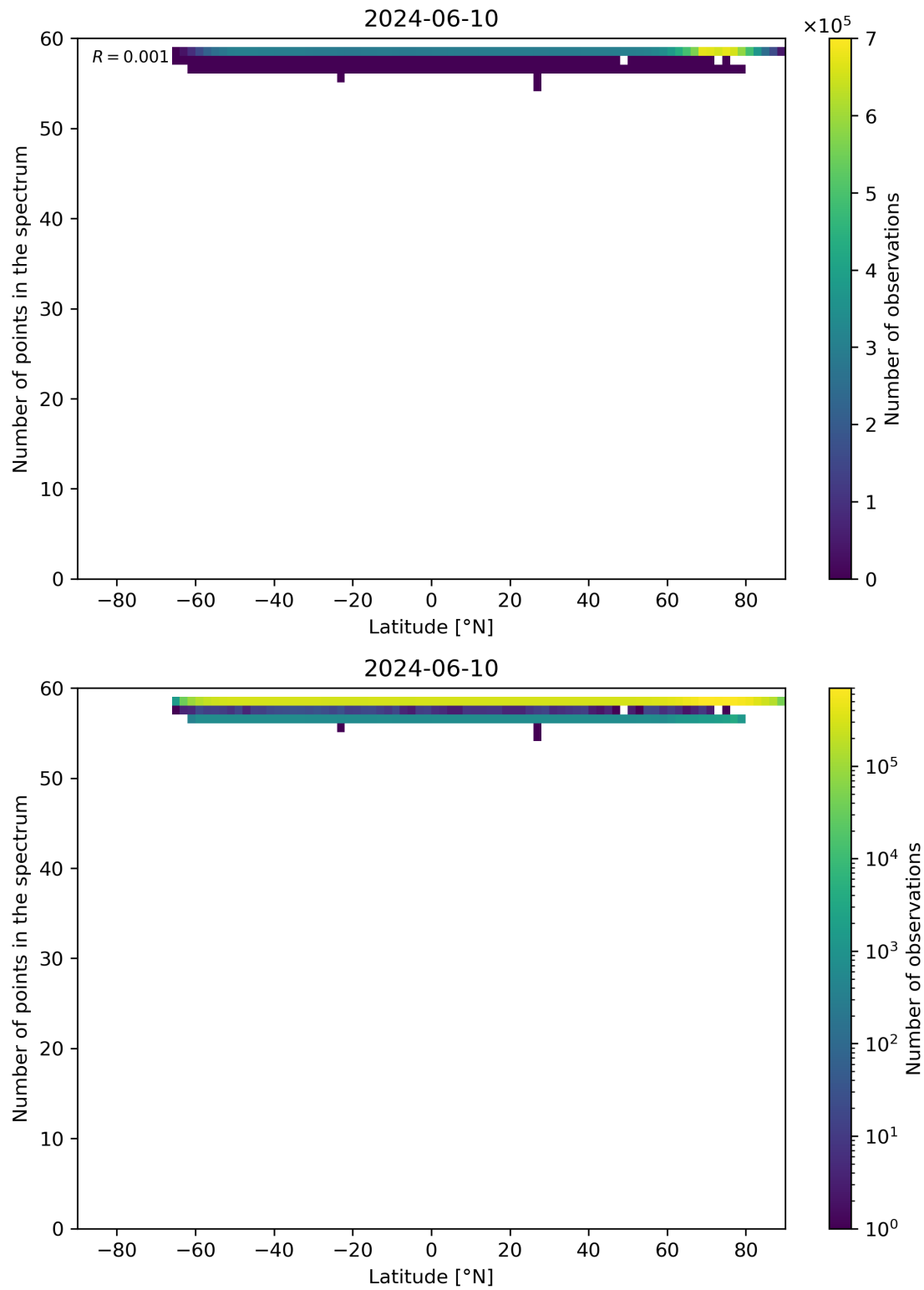
Figure 94: Scatter density plot of “Latitude” against “Number of points in the spectrum” for 2024-06-09 to 2024-06-11.
