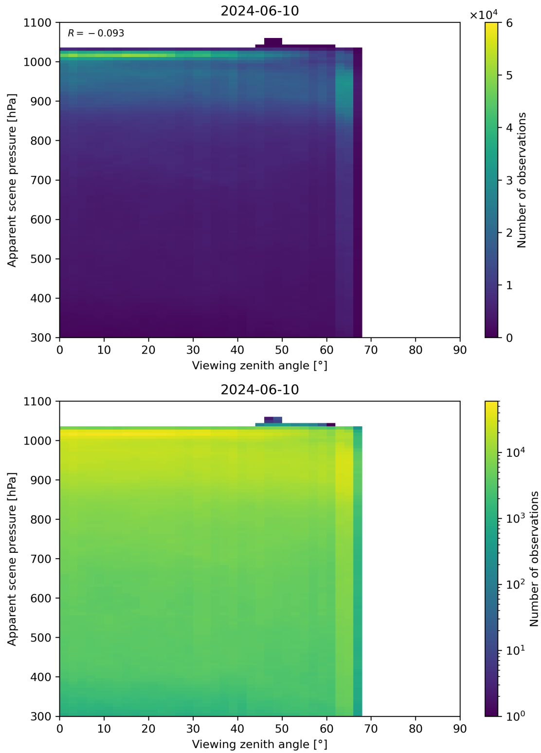
Figure 118: Scatter density plot of “Viewing zenith angle” against “Apparent scene pressure” for 2024-06-09 to 2024-06-11.
