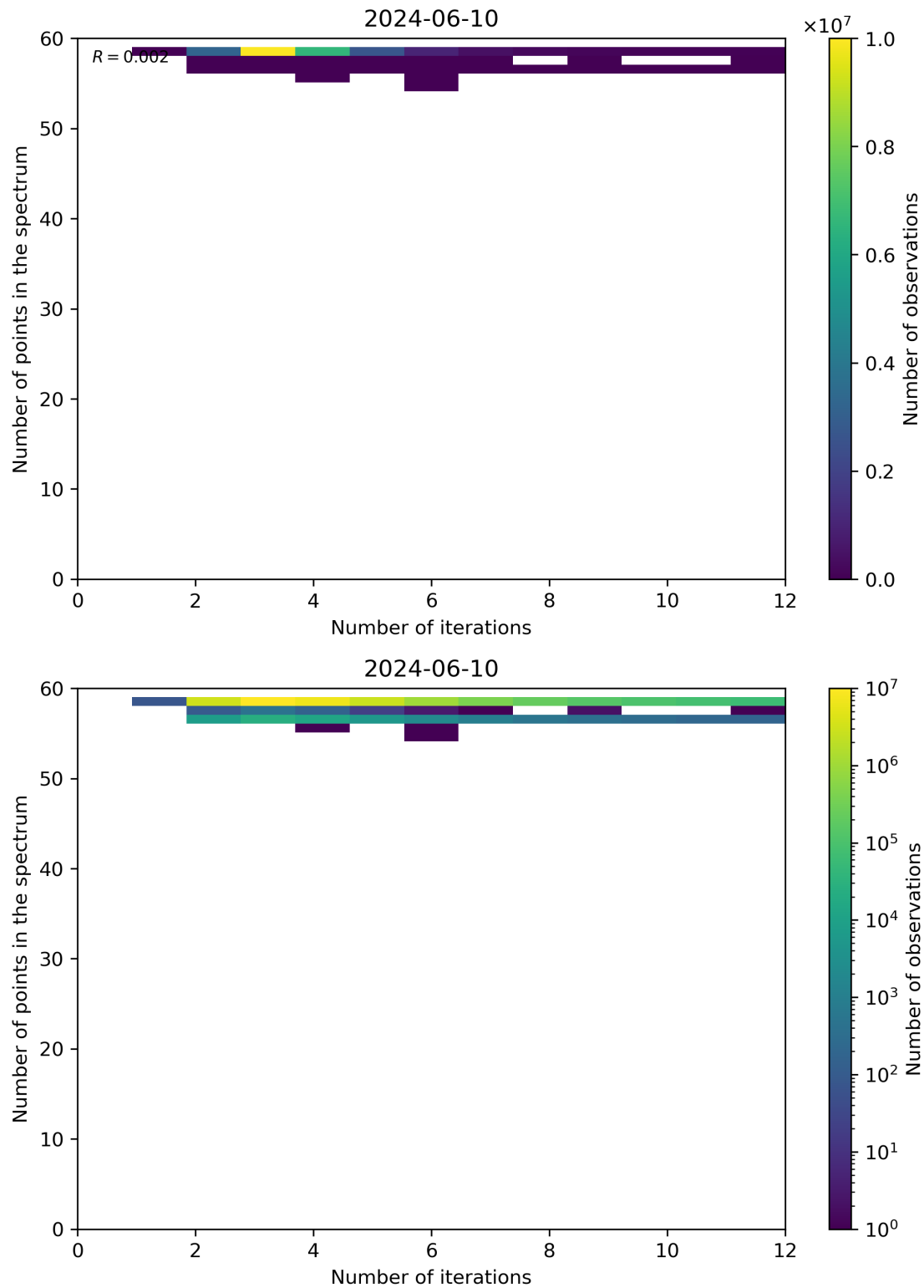
Figure 99: Scatter density plot of “Number of iterations” against “Number of points in the spectrum” for 2024-06-09 to 2024-06-11.
