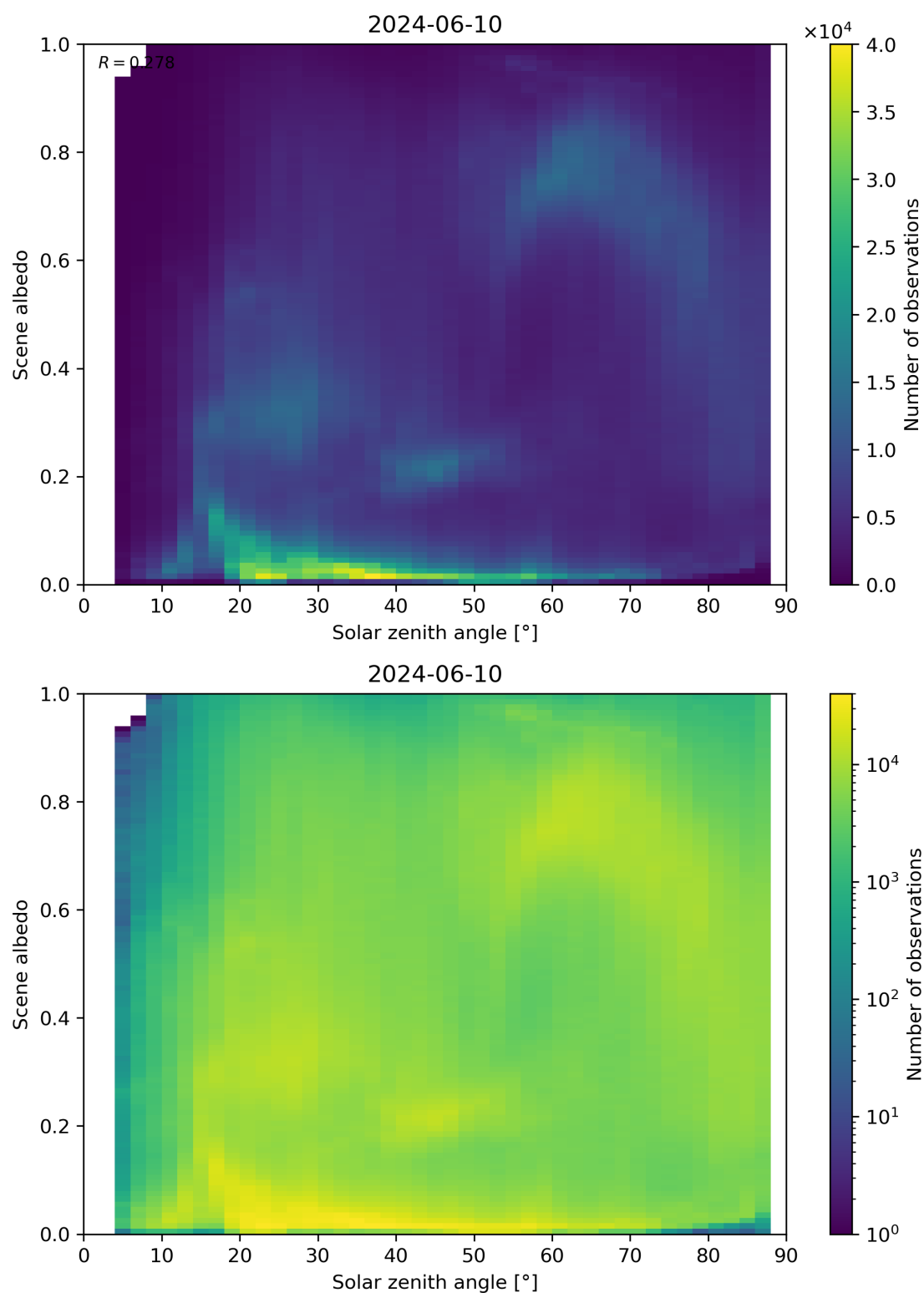
Figure 116: Scatter density plot of “Solar zenith angle” against “Scene albedo” for 2024-06-09 to 2024-06-11.
