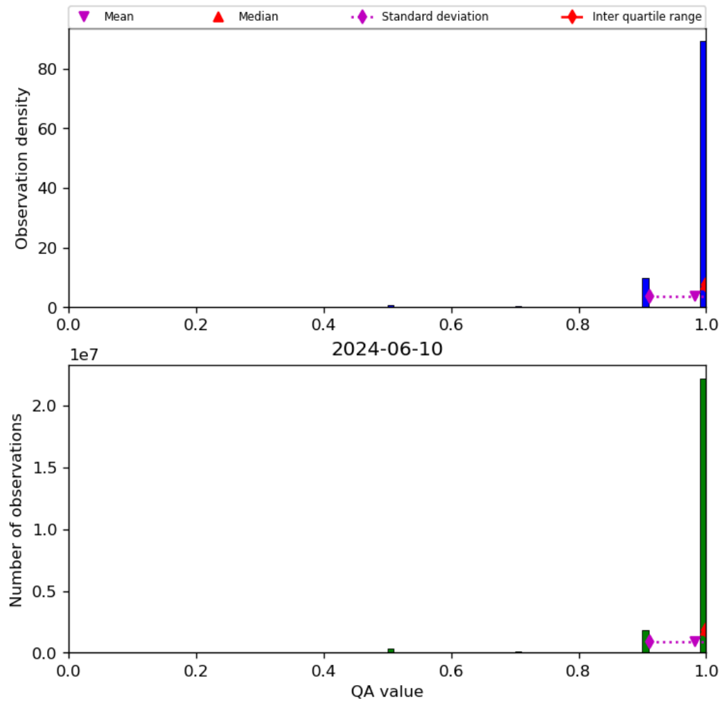
Figure 29: Histogram of “QA value” for 2024-06-09 to 2024-06-11
