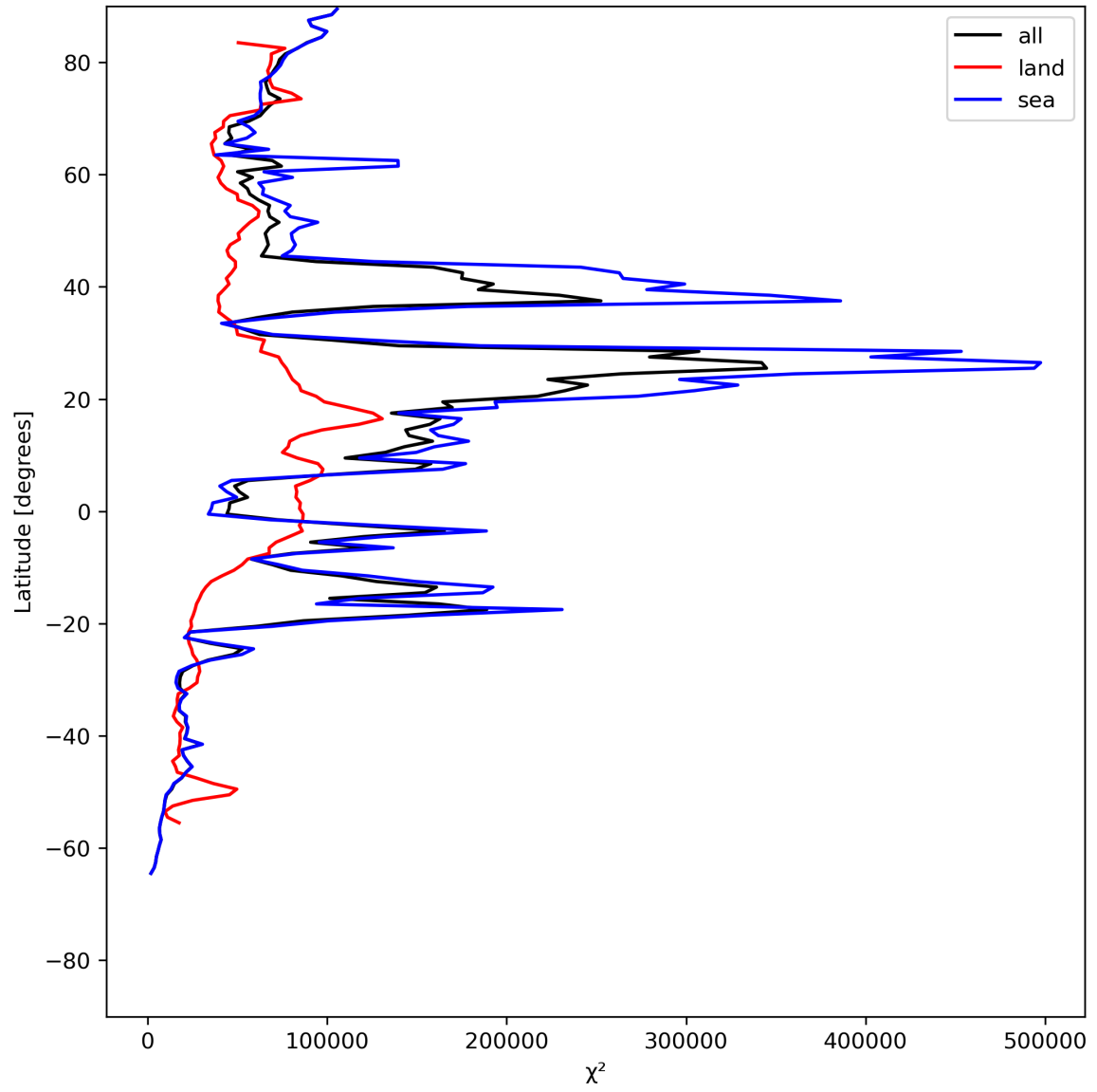
Figure 21: Zonal average of “ \chi^2 ” for 2024-06-09 to 2024-06-11.
