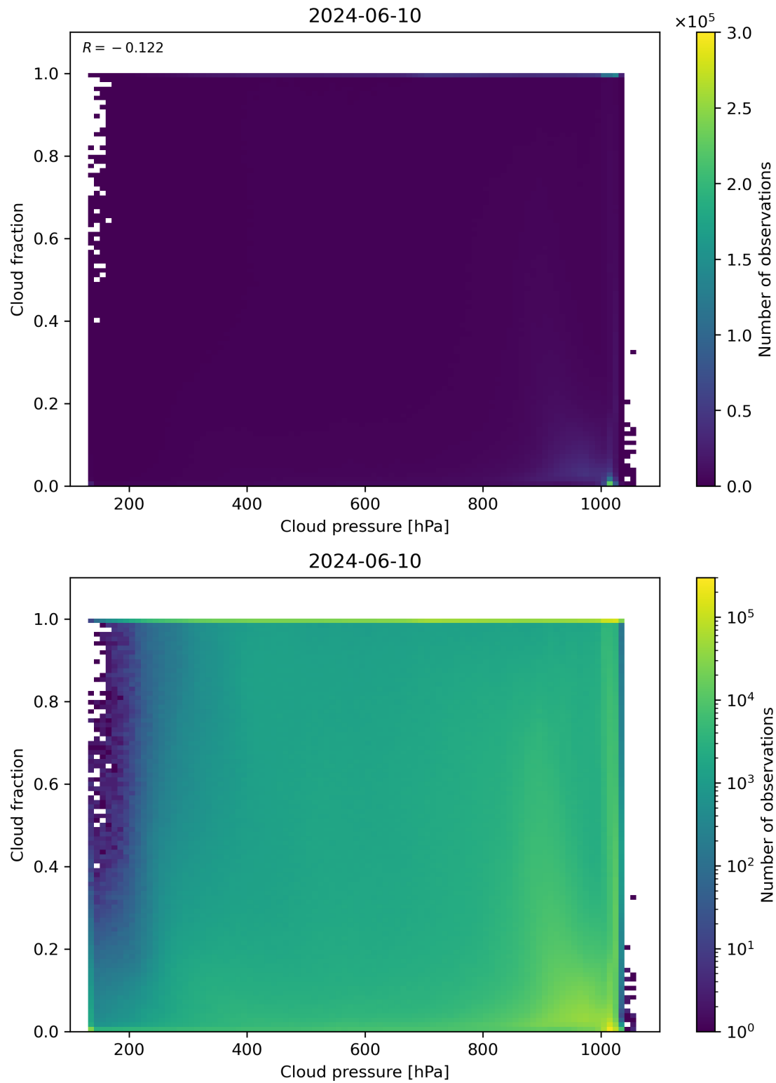
Figure 79: Scatter density plot of “Cloud pressure” against “Cloud fraction” for 2024-06-09 to 2024-06-11.
