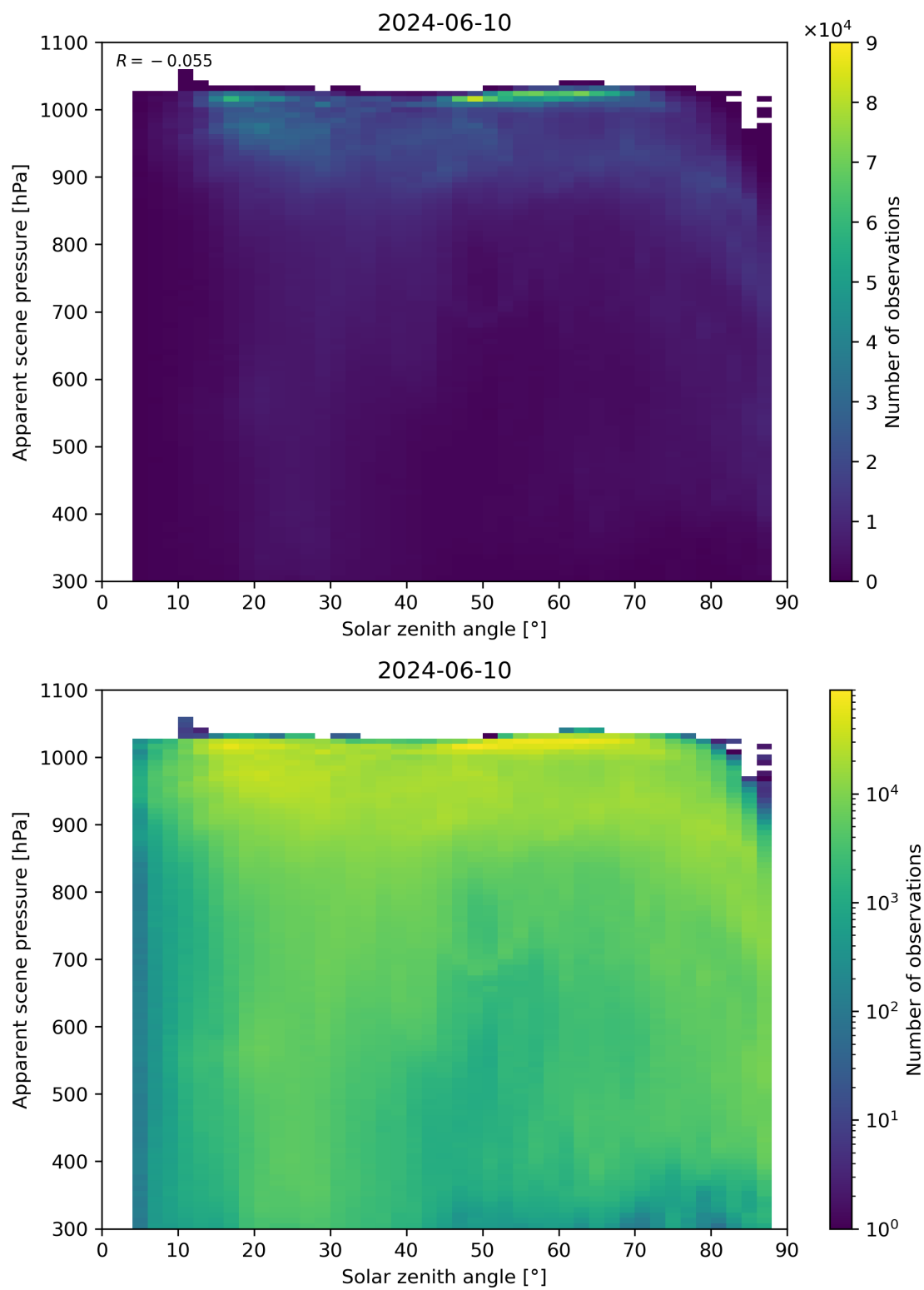
Figure 108: Scatter density plot of “Solar zenith angle” against “Apparent scene pressure” for 2024-06-09 to 2024-06-11.
