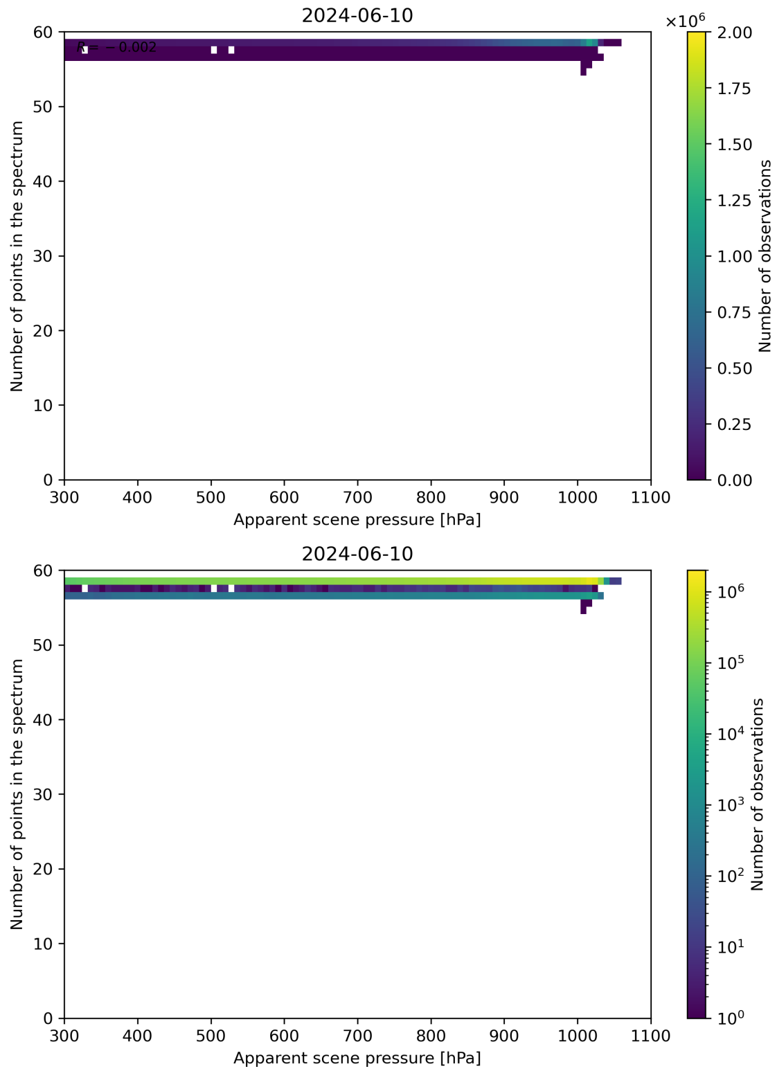
Figure 66: Scatter density plot of “Apparent scene pressure” against “Number of points in the spectrum” for 2024-06-09 to 2024-06-11.
