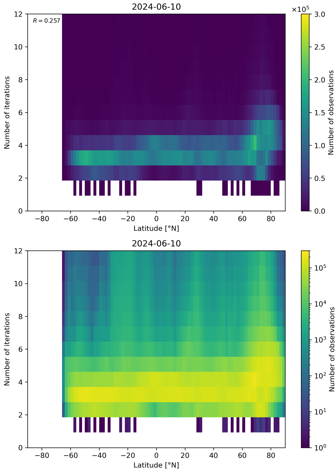
Figure 93: Scatter density plot of “Latitude” against “Number of iterations” for 2024-06-09 to 2024-06-11.
