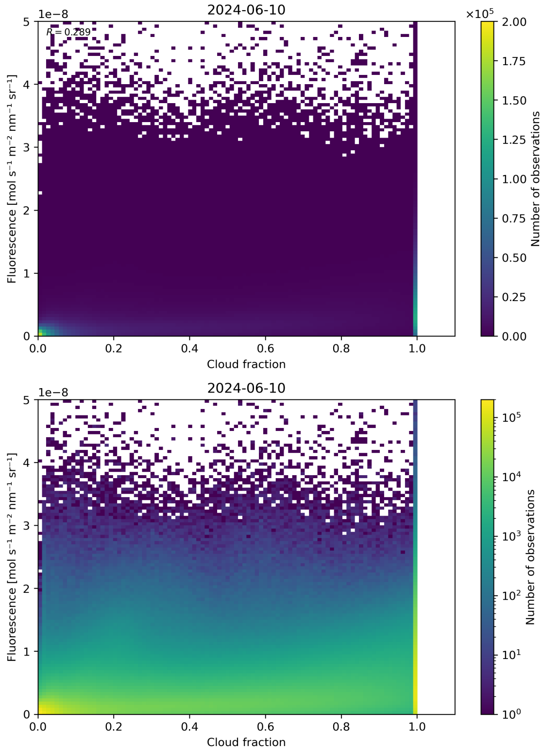
Figure 72: Scatter density plot of “Cloud fraction” against “Fluorescence” for 2024-06-09 to 2024-06-11.
