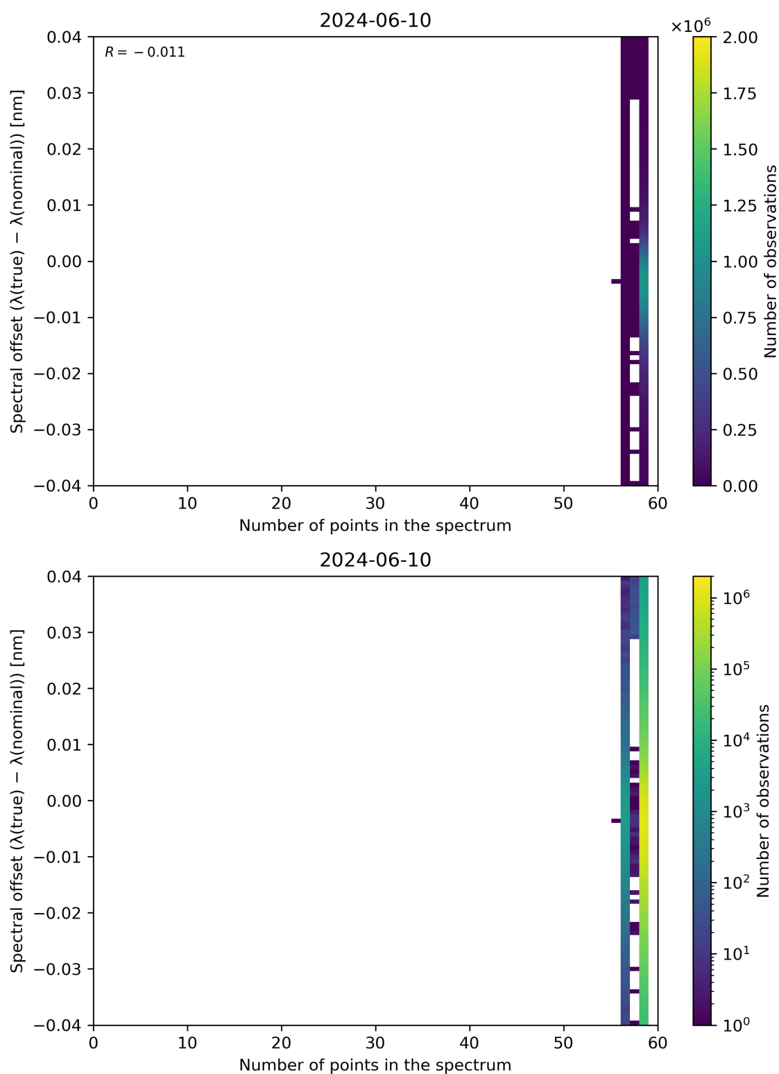
Figure 101: Scatter density plot of “Number of points in the spectrum” against “Spectral offset ( \lambda(\text{true}) - \lambda(\text{nominal}) )” for 2024-06-09 to 2024-06-11.
