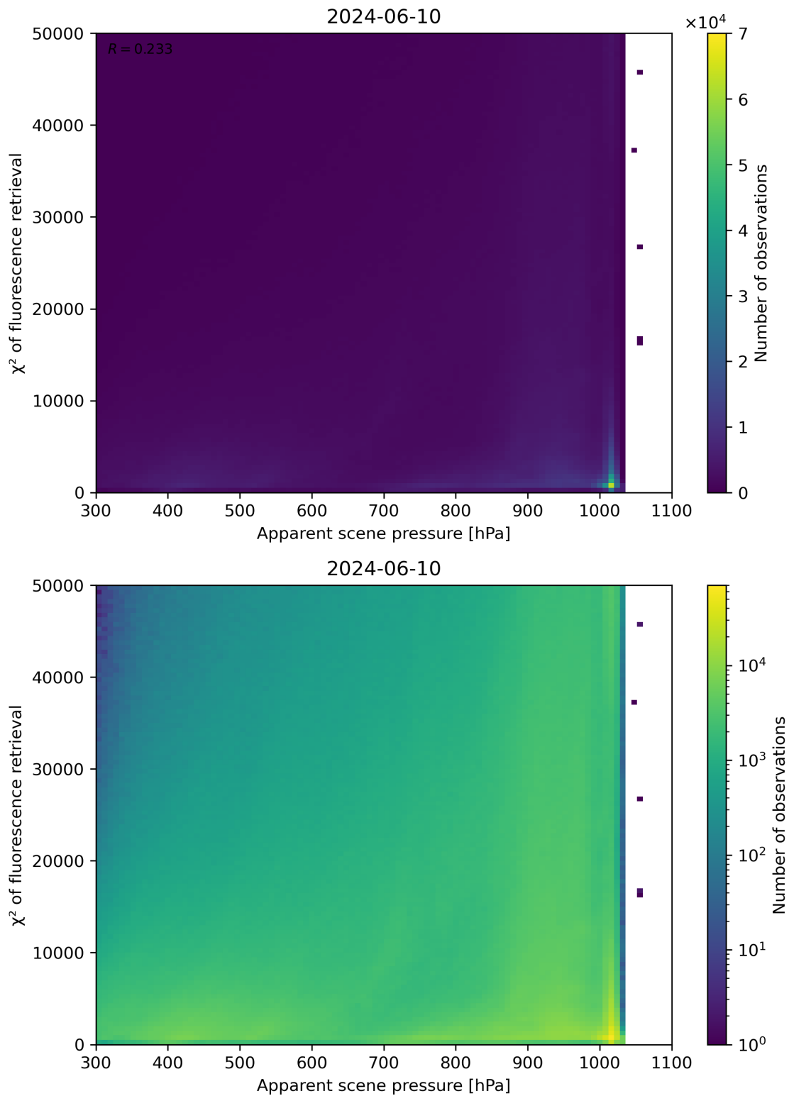
Figure 63: Scatter density plot of “Apparent scene pressure” against “ \chi^2 of fluorescence retrieval” for 2024-06-09 to 2024-06-11.
