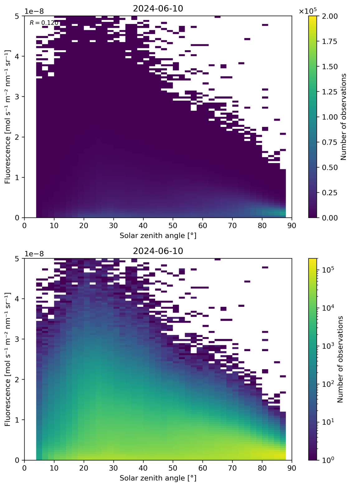
Figure 112: Scatter density plot of “Solar zenith angle” against “Fluorescence” for 2024-06-09 to 2024-06-11.
