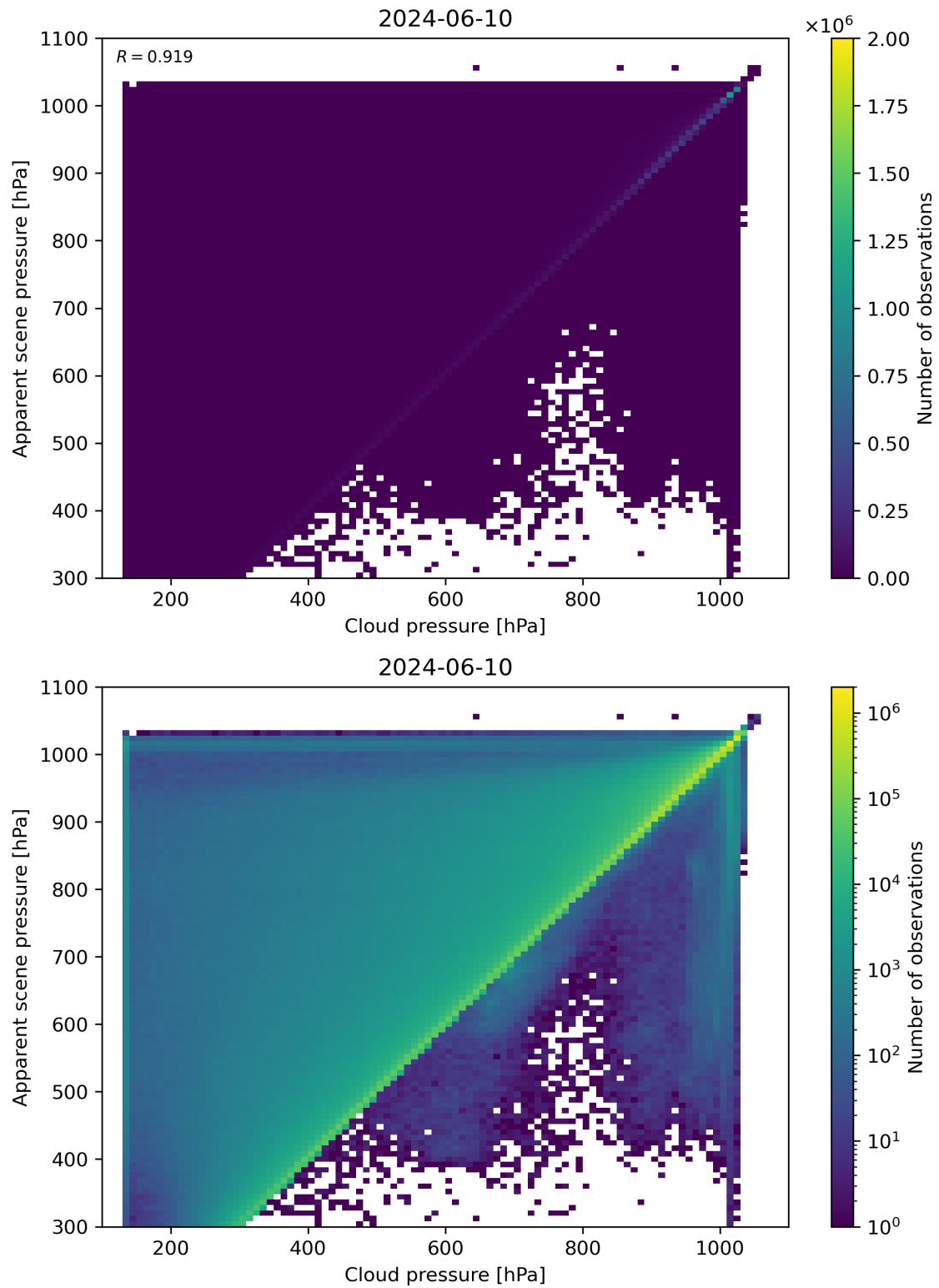
Figure 77: Scatter density plot of “Cloud pressure” against “Apparent scene pressure” for 2024-06-09 to 2024-06-11.
