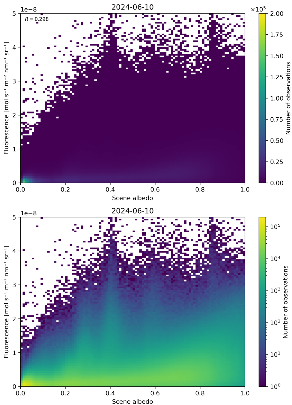
Figure 104: Scatter density plot of “Scene albedo” against “Fluorescence” for 2024-06-09 to 2024-06-11.
