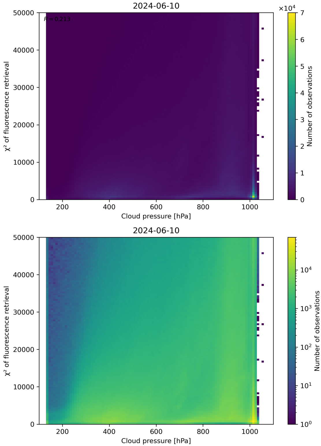
Figure 78: Scatter density plot of “Cloud pressure” against “ \chi^2 of fluorescence retrieval” for 2024-06-09 to 2024-06-11.
