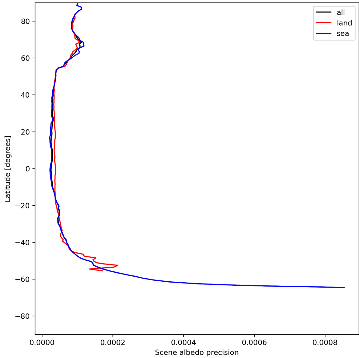
Figure 18: Zonal average of “Scene albedo precision” for 2024-06-09 to 2024-06-11.
