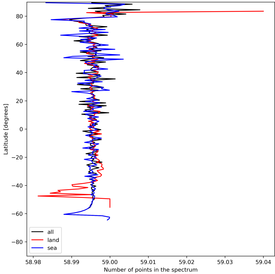
Figure 27: Zonal average of “Number of points in the spectrum” for 2024-06-09 to 2024-06-11.
