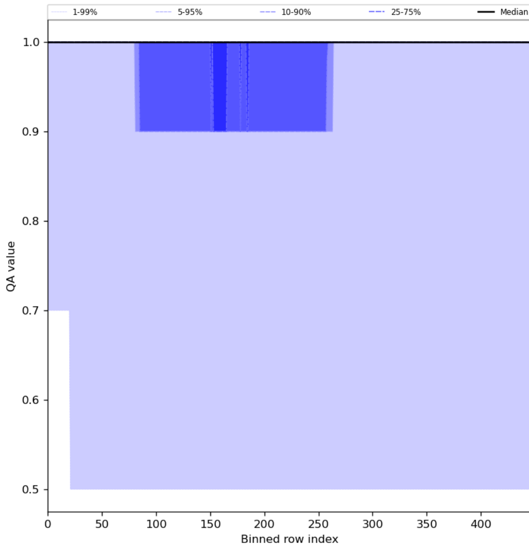
Figure 46: Along track statistics of “QA value” for 2024-06-09 to 2024-06-11
