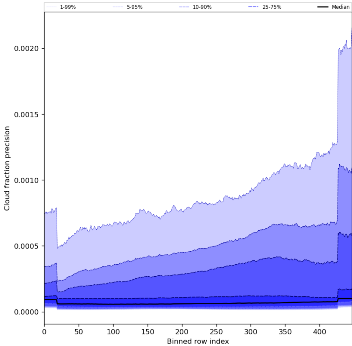
Figure 50: Along track statistics of “Cloud fraction precision” for 2024-06-09 to 2024-06-11
