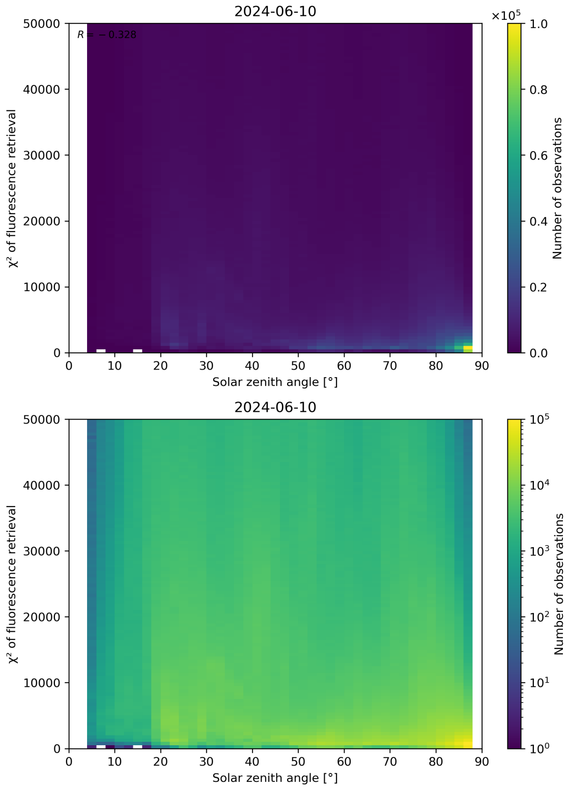
Figure 109: Scatter density plot of “Solar zenith angle” against “ \chi^2 of fluorescence retrieval” for 2024-06-09 to 2024-06-11.
