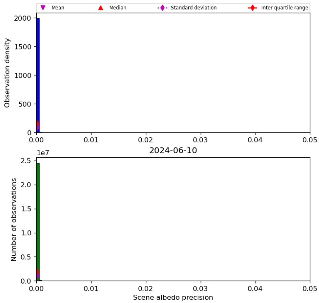
Figure 35: Histogram of “Scene albedo precision” for 2024-06-09 to 2024-06-11
