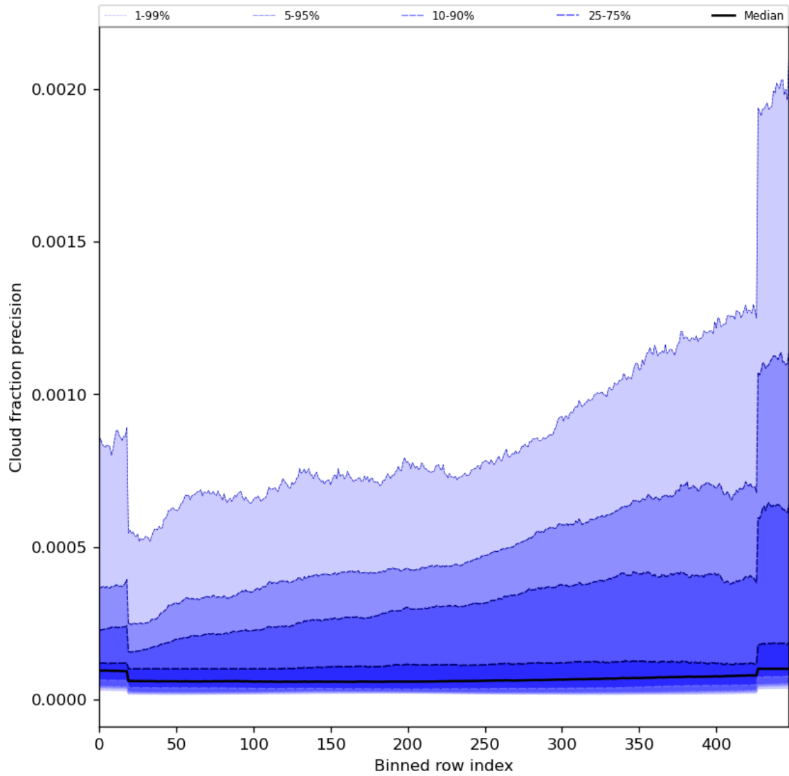
Figure 50: Along track statistics of “Cloud fraction precision” for 2024-06-10 to 2024-06-12
