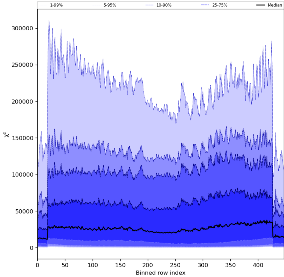
Figure 55: Along track statistics of “ \chi^2 ” for 2024-06-10 to 2024-06-12
