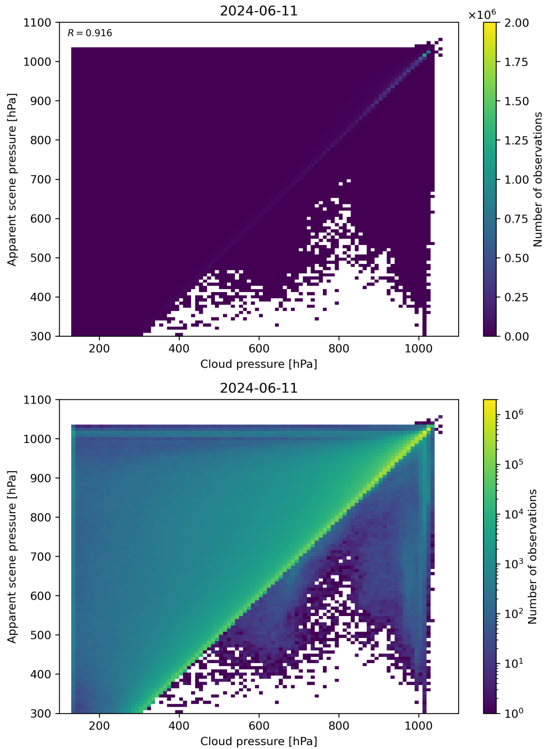
Figure 77: Scatter density plot of “Cloud pressure” against “Apparent scene pressure” for 2024-06-10 to 2024-06-12.
