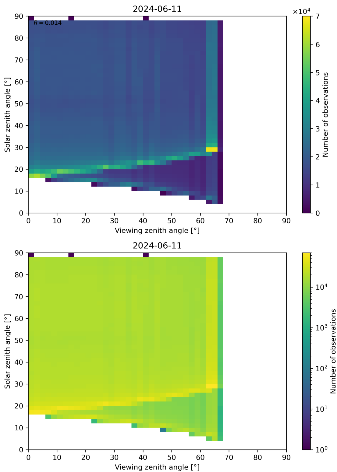
Figure 127: Scatter density plot of “Viewing zenith angle” against “Solar zenith angle” for 2024-06-10 to 2024-06-12.
