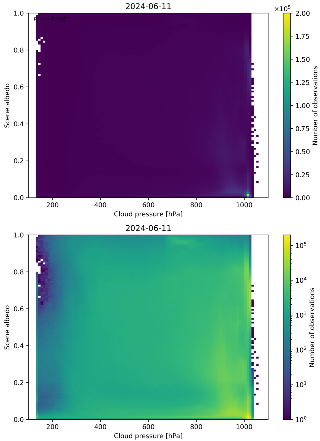
Figure 83: Scatter density plot of “Cloud pressure” against “Scene albedo” for 2024-06-10 to 2024-06-12.
