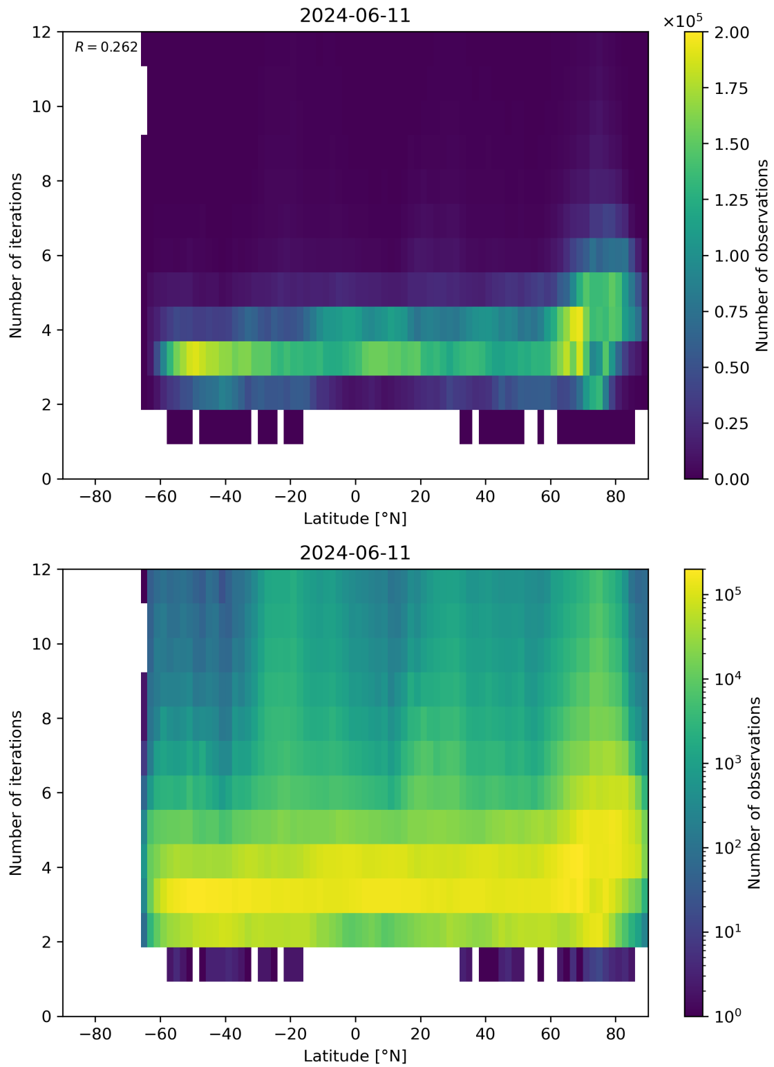
Figure 93: Scatter density plot of “Latitude” against “Number of iterations” for 2024-06-10 to 2024-06-12.
