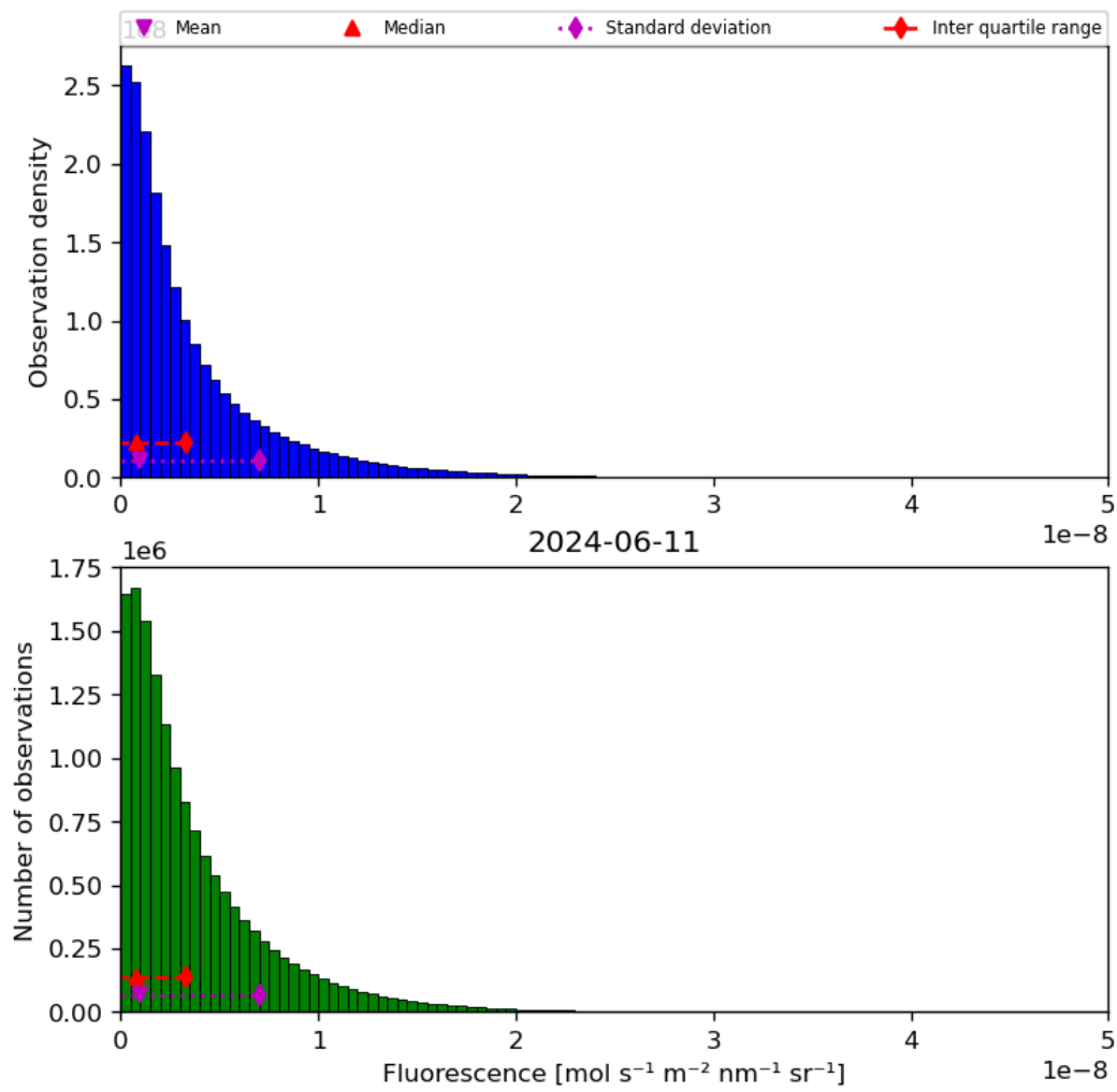
Figure 40: Histogram of “Fluorescence” for 2024-06-10 to 2024-06-12
