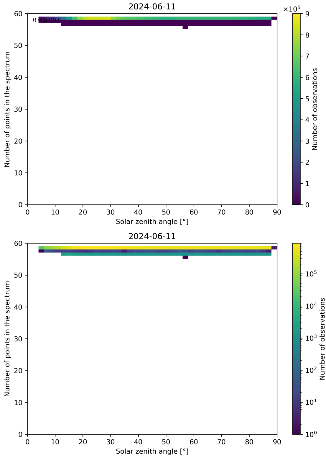
Figure 115: Scatter density plot of “Solar zenith angle” against “Number of points in the spectrum” for 2024-06-10 to 2024-06-12.
