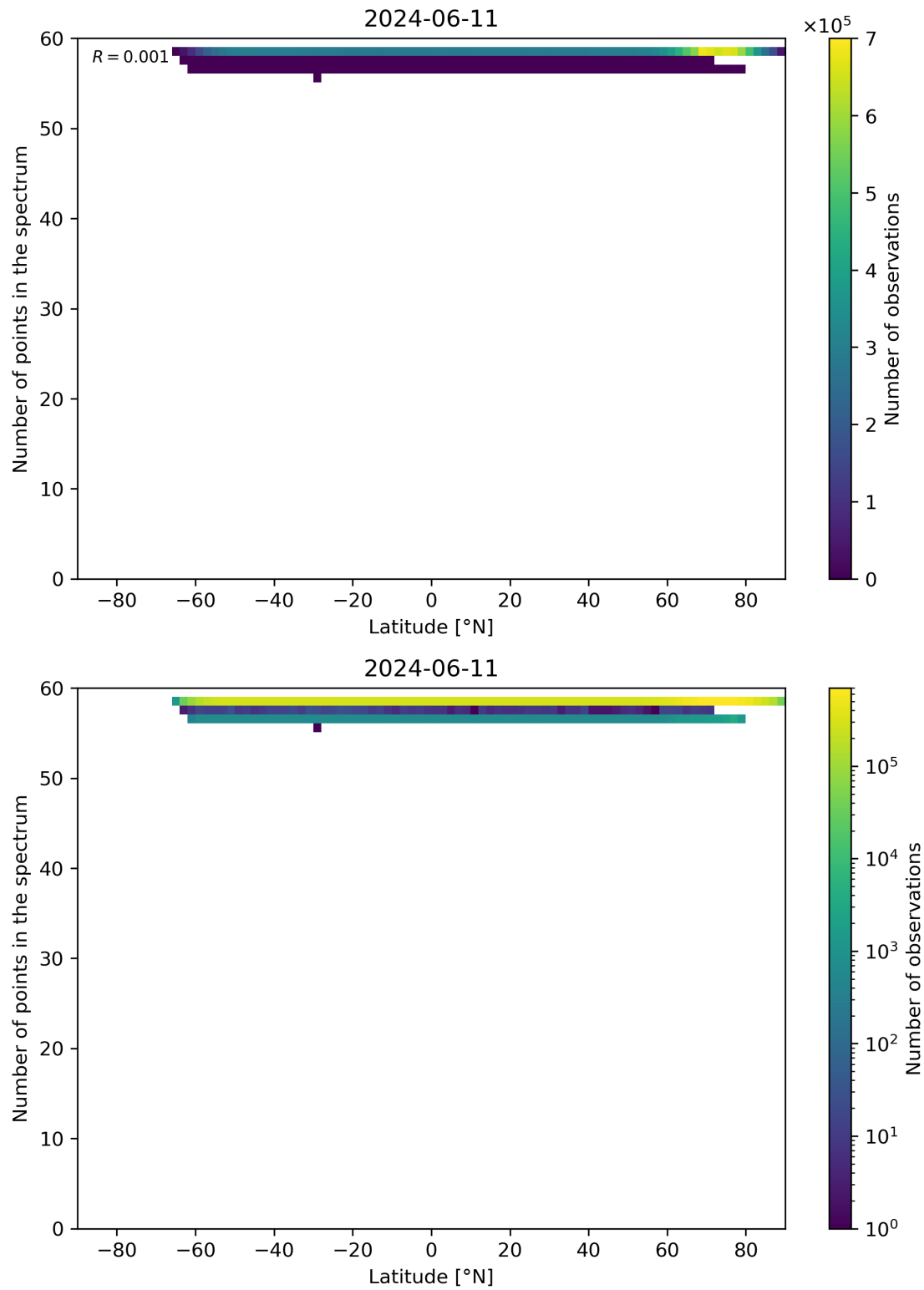
Figure 94: Scatter density plot of “Latitude” against “Number of points in the spectrum” for 2024-06-10 to 2024-06-12.
