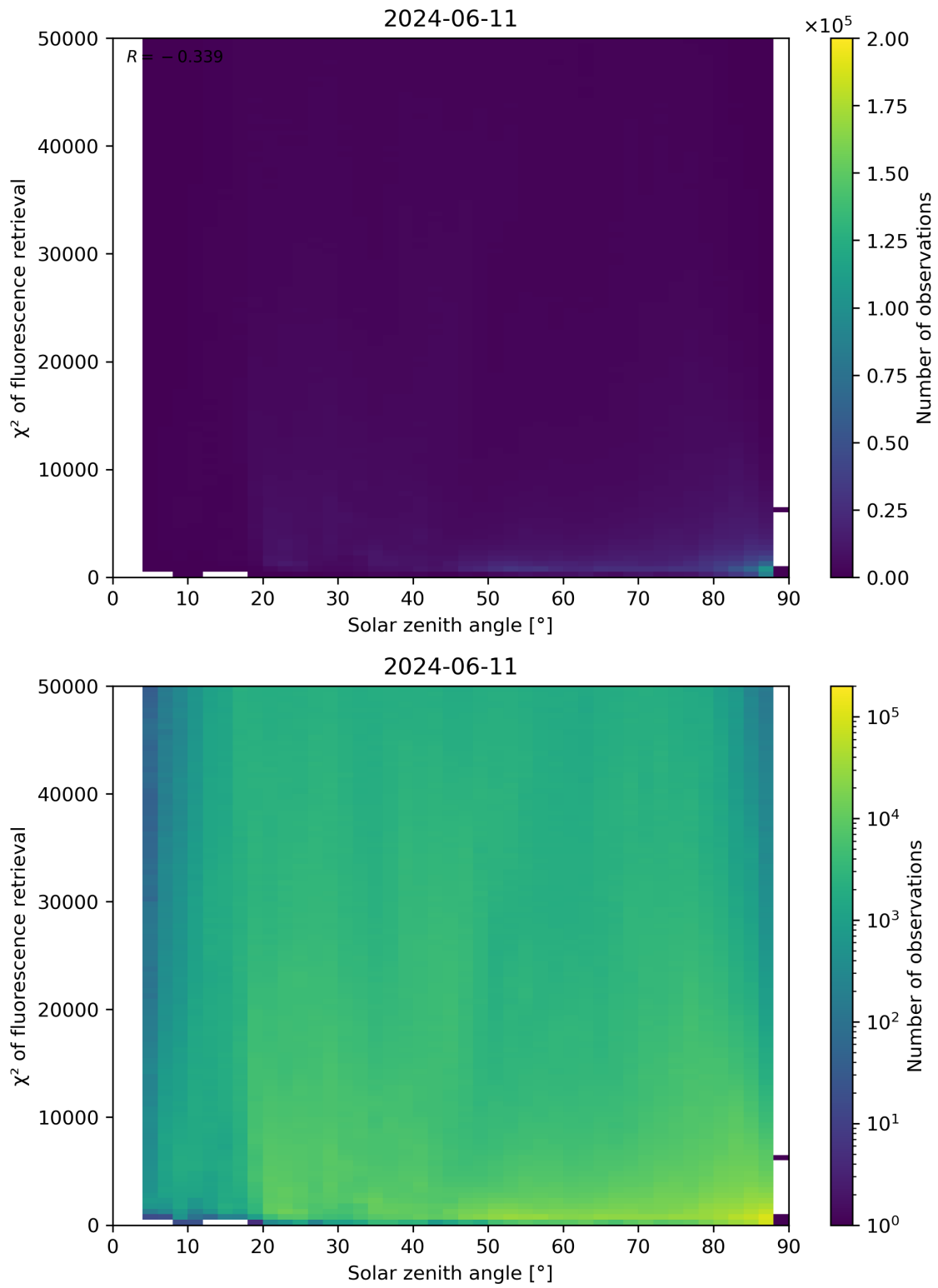
Figure 109: Scatter density plot of “Solar zenith angle” against “ \chi^2 of fluorescence retrieval” for 2024-06-10 to 2024-06-12.
