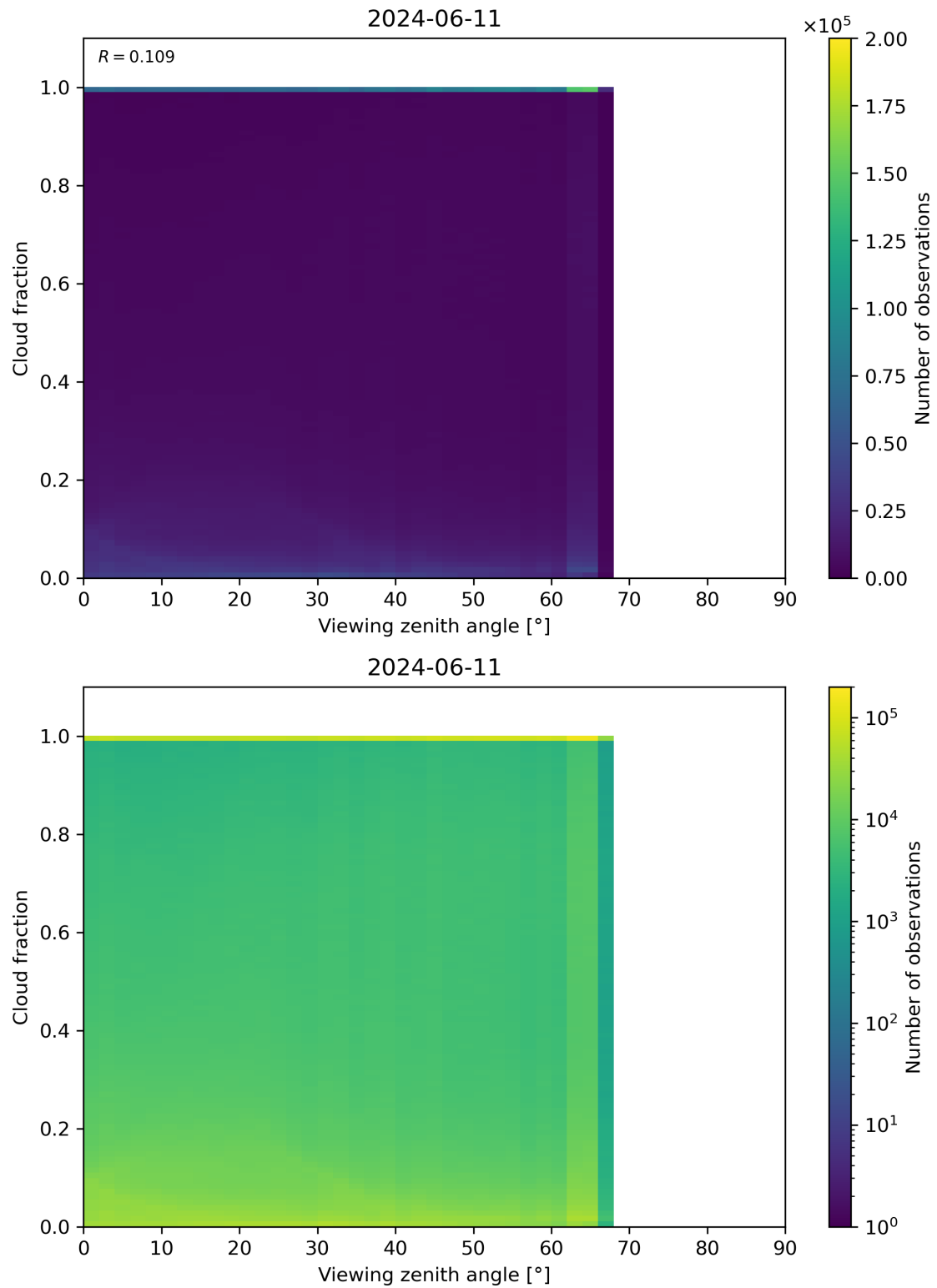
Figure 120: Scatter density plot of “Viewing zenith angle” against “Cloud fraction” for 2024-06-10 to 2024-06-12.
