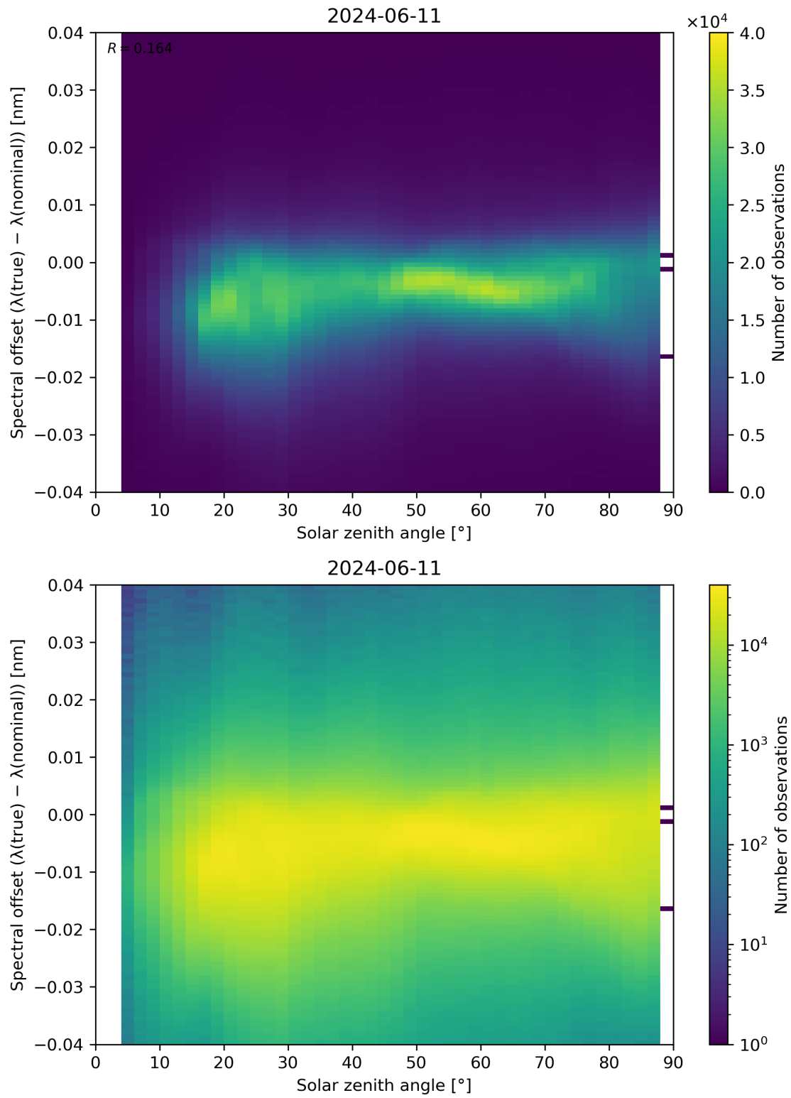
Figure 117: Scatter density plot of “Solar zenith angle” against “Spectral offset ( \lambda(\text{true}) - \lambda(\text{nominal}) )” for 2024-06-10 to 2024-06-12.
