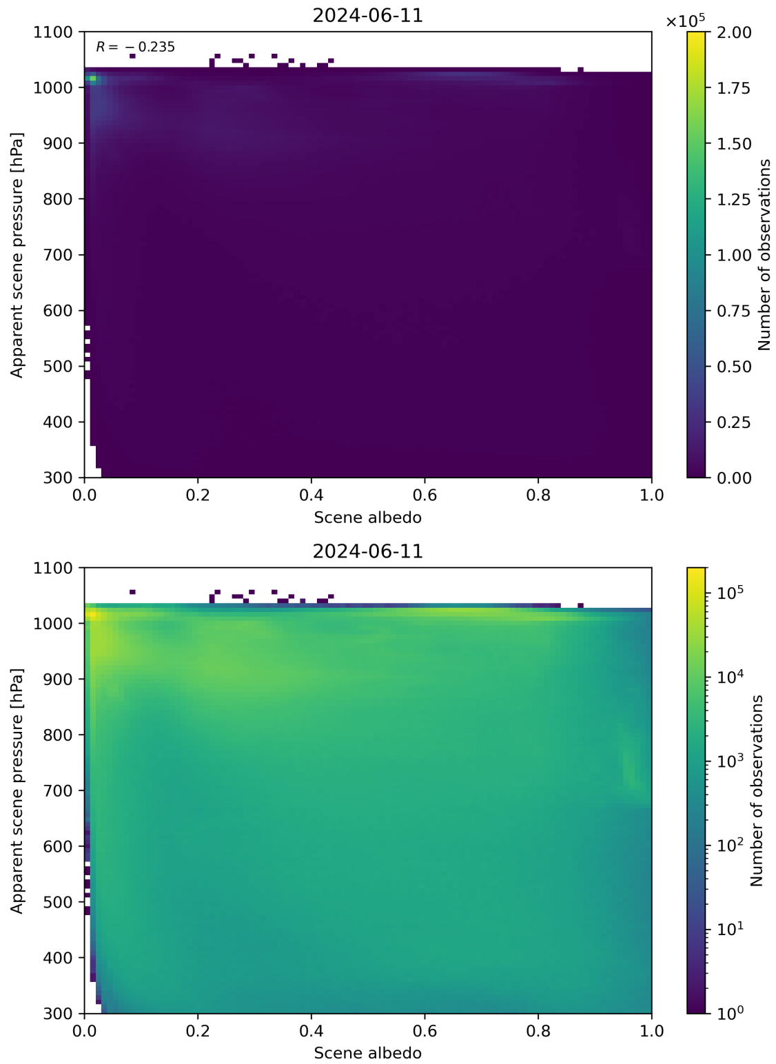
Figure 102: Scatter density plot of “Scene albedo” against “Apparent scene pressure” for 2024-06-10 to 2024-06-12.
