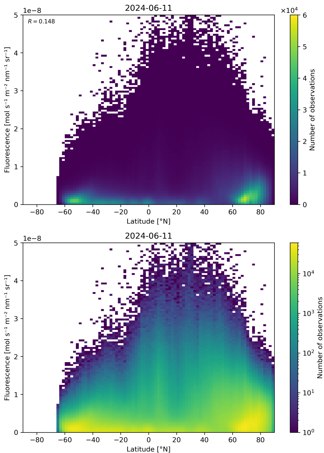
Figure 92: Scatter density plot of “Latitude” against “Fluorescence” for 2024-06-10 to 2024-06-12.
