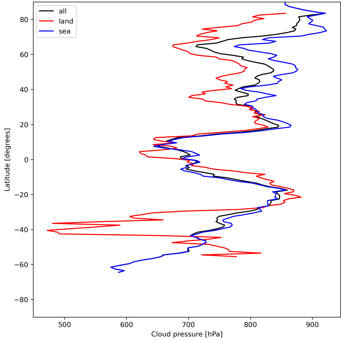
Figure 13: Zonal average of “Cloud pressure” for 2024-06-10 to 2024-06-12.
