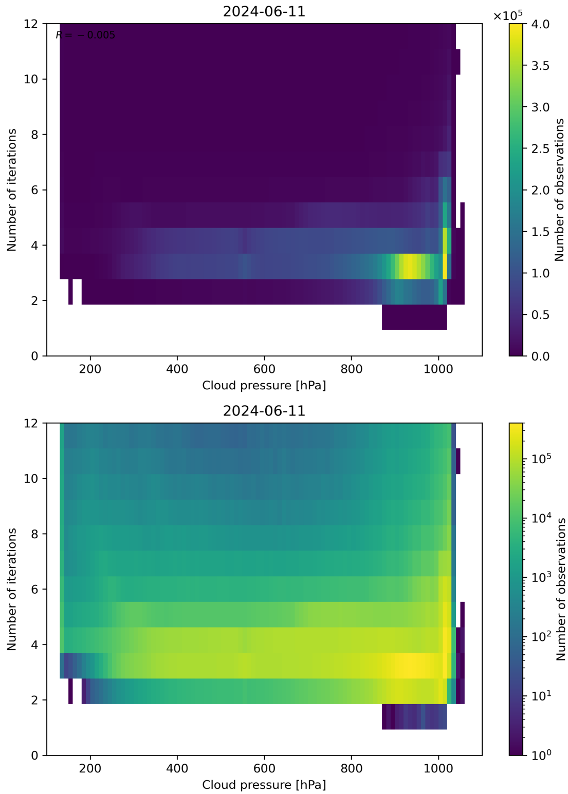
Figure 81: Scatter density plot of “Cloud pressure” against “Number of iterations” for 2024-06-10 to 2024-06-12.
