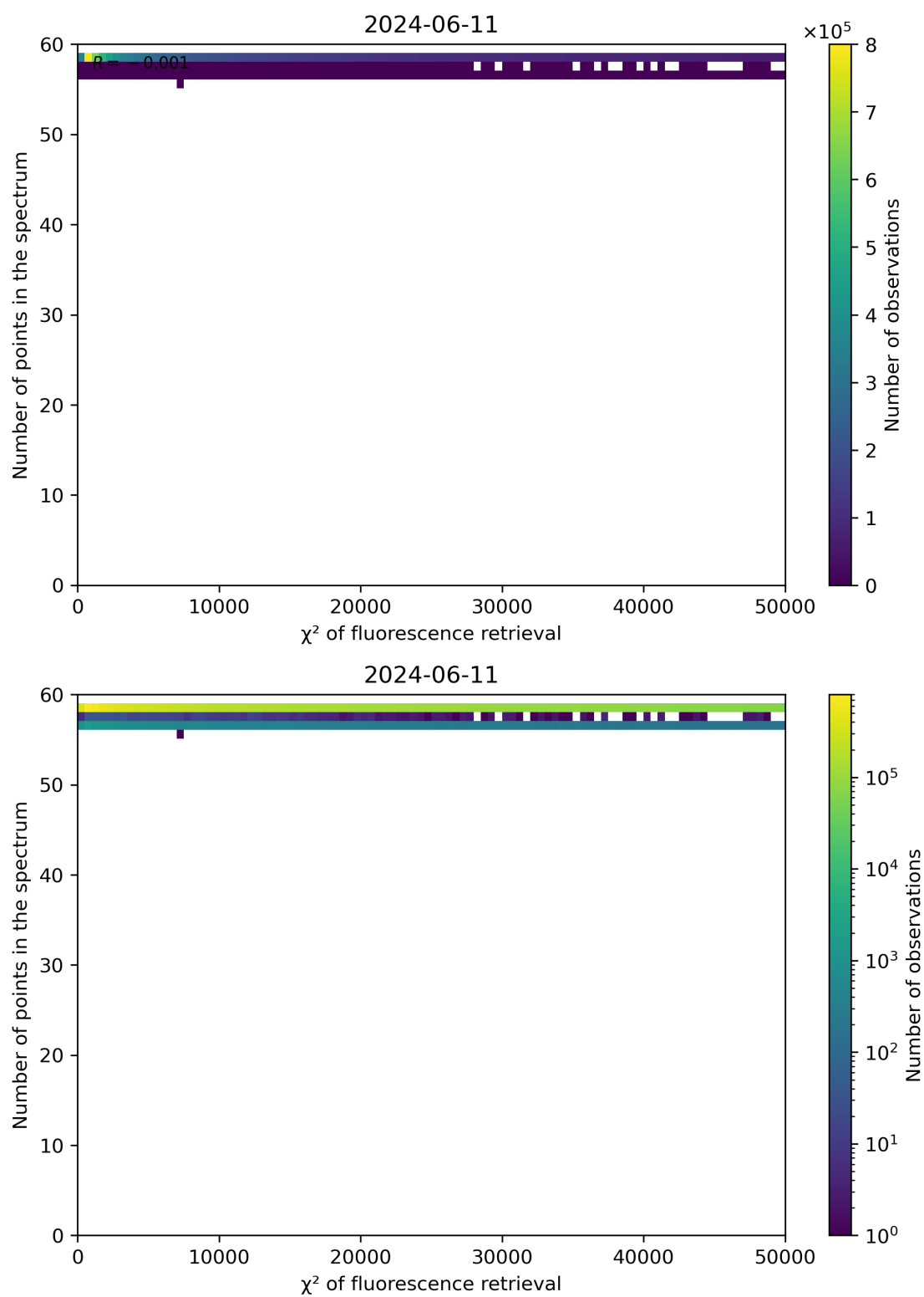
Figure 68: Scatter density plot of " \chi^2 of fluorescence retrieval" against "Number of points in the spectrum" for 2024-06-10 to 2024-06-12.
