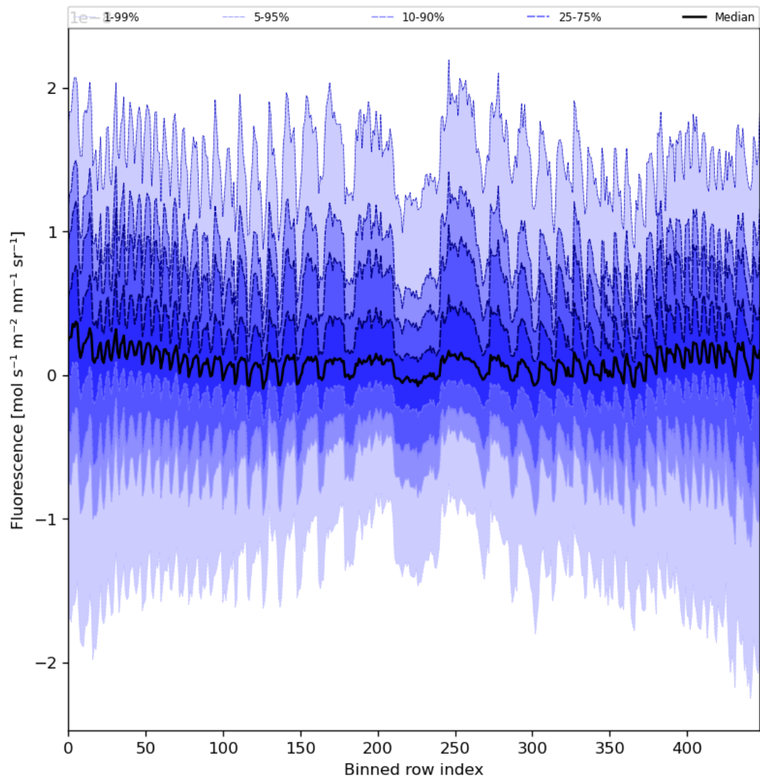
Figure 57: Along track statistics of “Fluorescence” for 2024-06-10 to 2024-06-12
