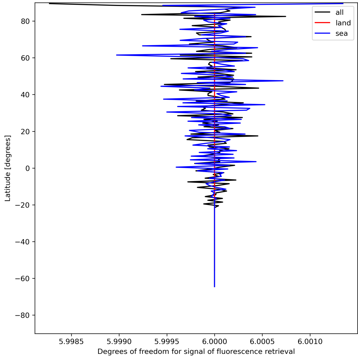
Figure 26: Zonal average of “Degrees of freedom for signal of fluorescence retrieval” for 2024-06-10 to 2024-06-12.
