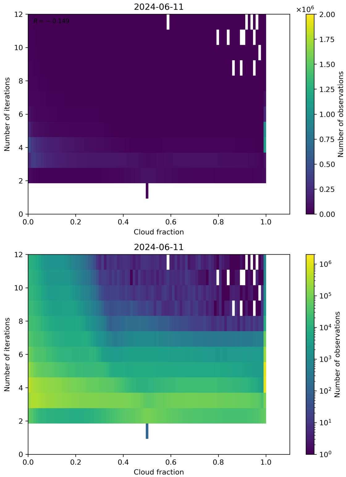
Figure 73: Scatter density plot of “Cloud fraction” against “Number of iterations” for 2024-06-10 to 2024-06-12.
