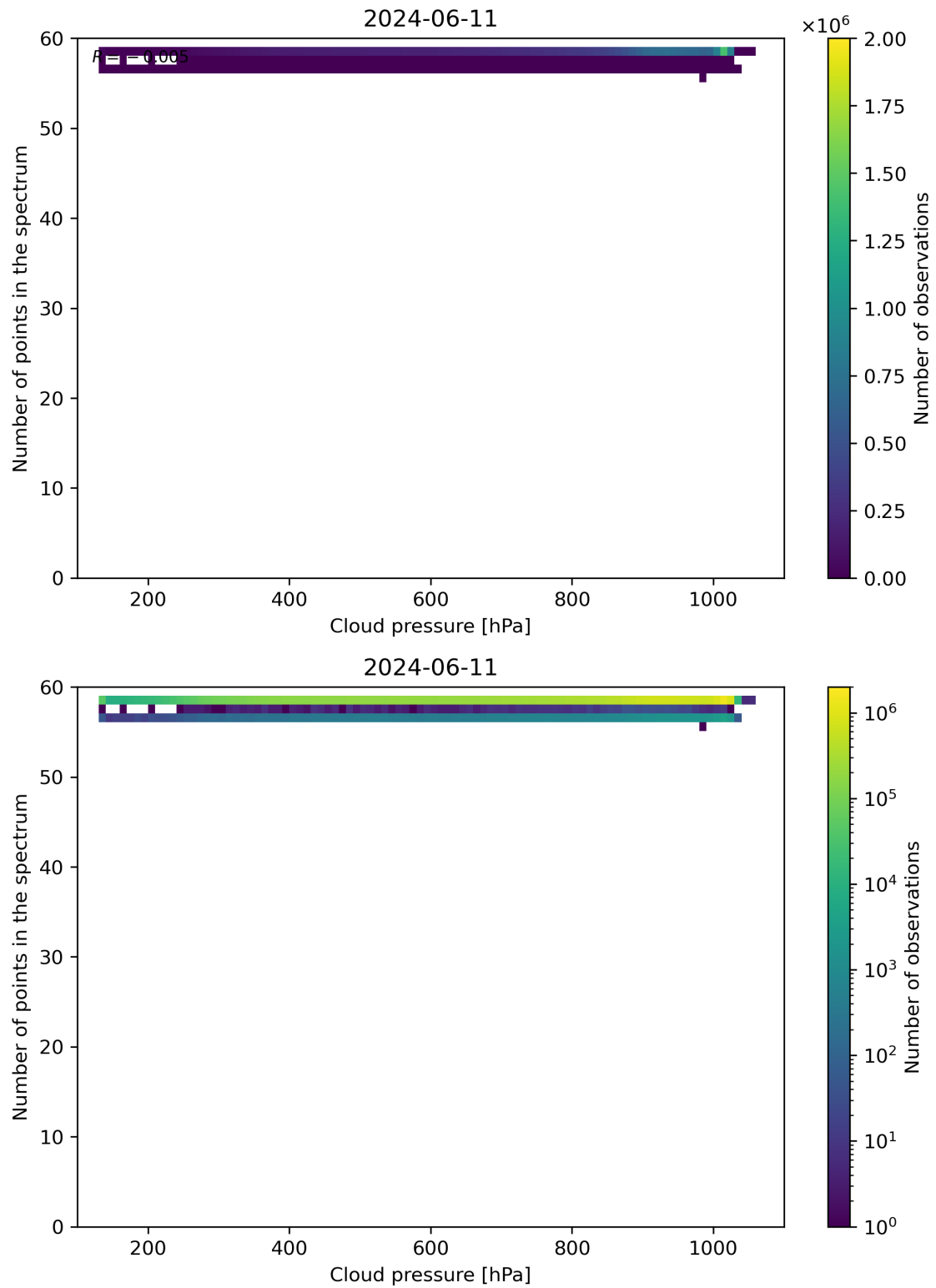
Figure 82: Scatter density plot of “Cloud pressure” against “Number of points in the spectrum” for 2024-06-10 to 2024-06-12.
