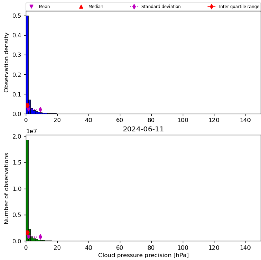
Figure 31: Histogram of “Cloud pressure precision” for 2024-06-10 to 2024-06-12
