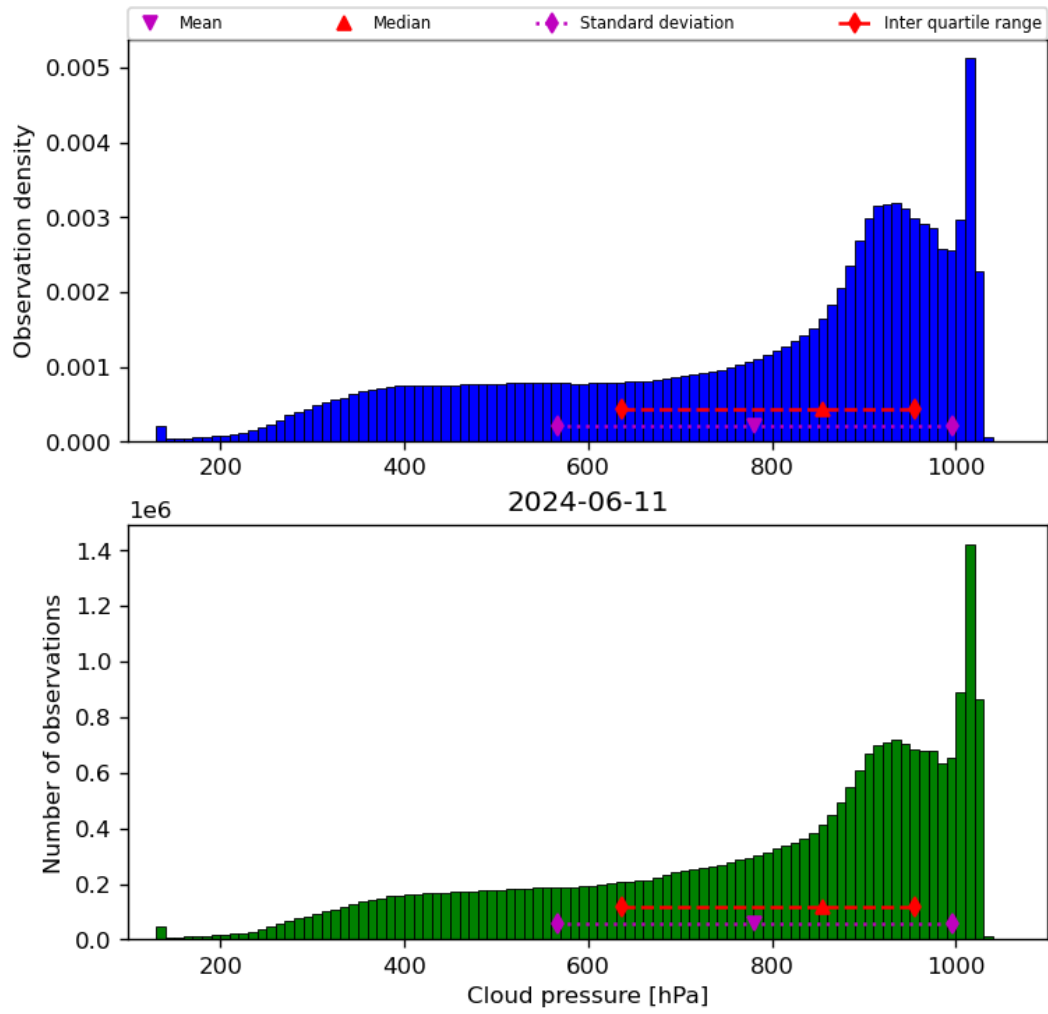
Figure 30: Histogram of “Cloud pressure” for 2024-06-10 to 2024-06-12
