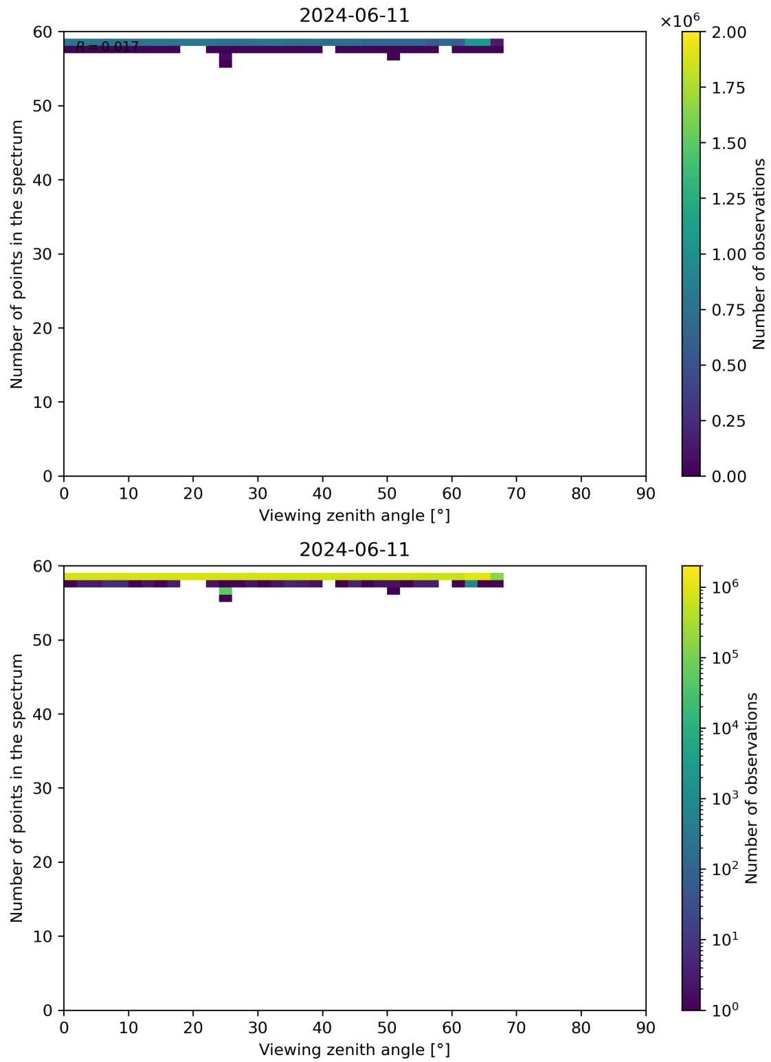
Figure 125: Scatter density plot of “Viewing zenith angle” against “Number of points in the spectrum” for 2024-06-10 to 2024-06-12.
