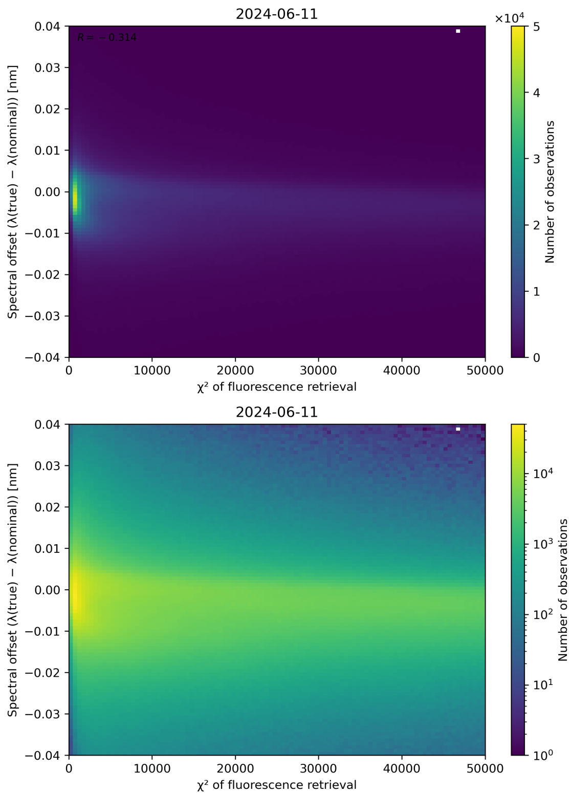
Figure 69: Scatter density plot of “ \chi^2 of fluorescence retrieval” against “Spectral offset ( \lambda(\text{true}) - \lambda(\text{nominal}) )” for 2024-06-10 to 2024-06-12.
