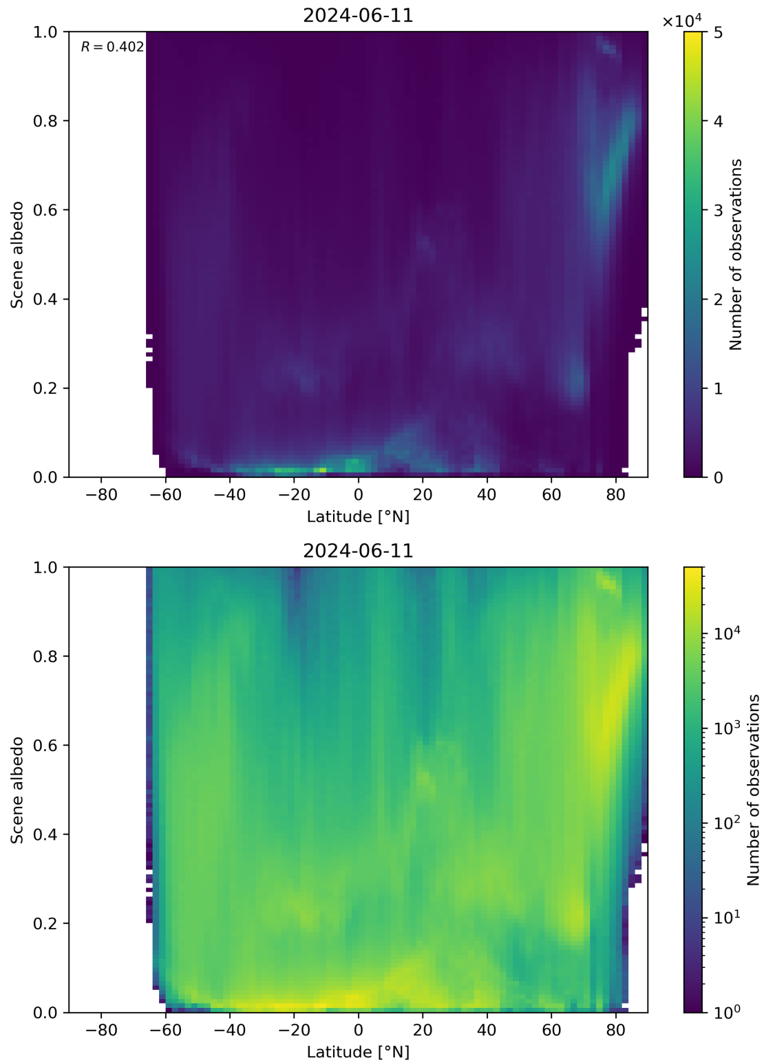
Figure 95: Scatter density plot of “Latitude” against “Scene albedo” for 2024-06-10 to 2024-06-12.
