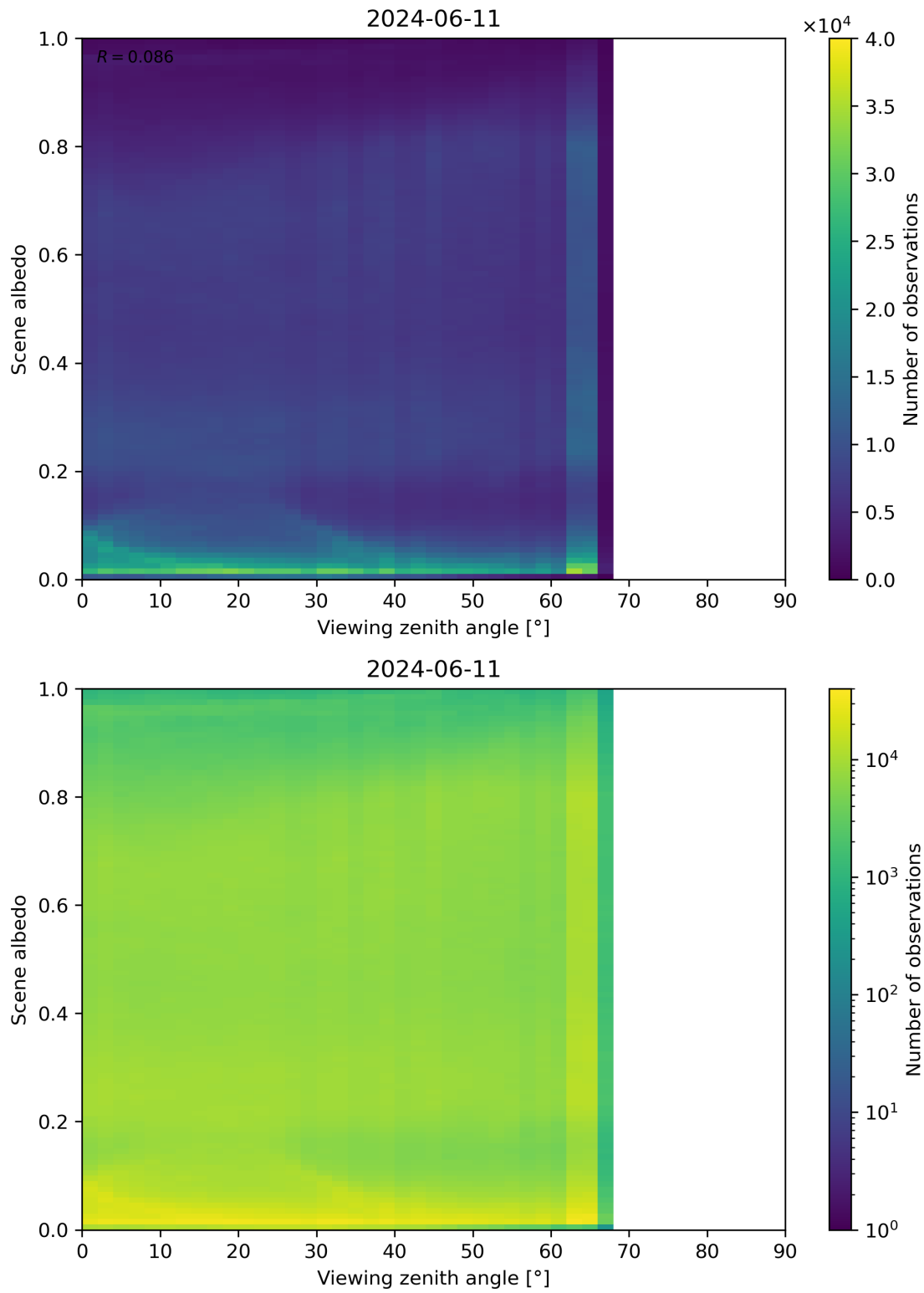
Figure 126: Scatter density plot of “Viewing zenith angle” against “Scene albedo” for 2024-06-10 to 2024-06-12.
