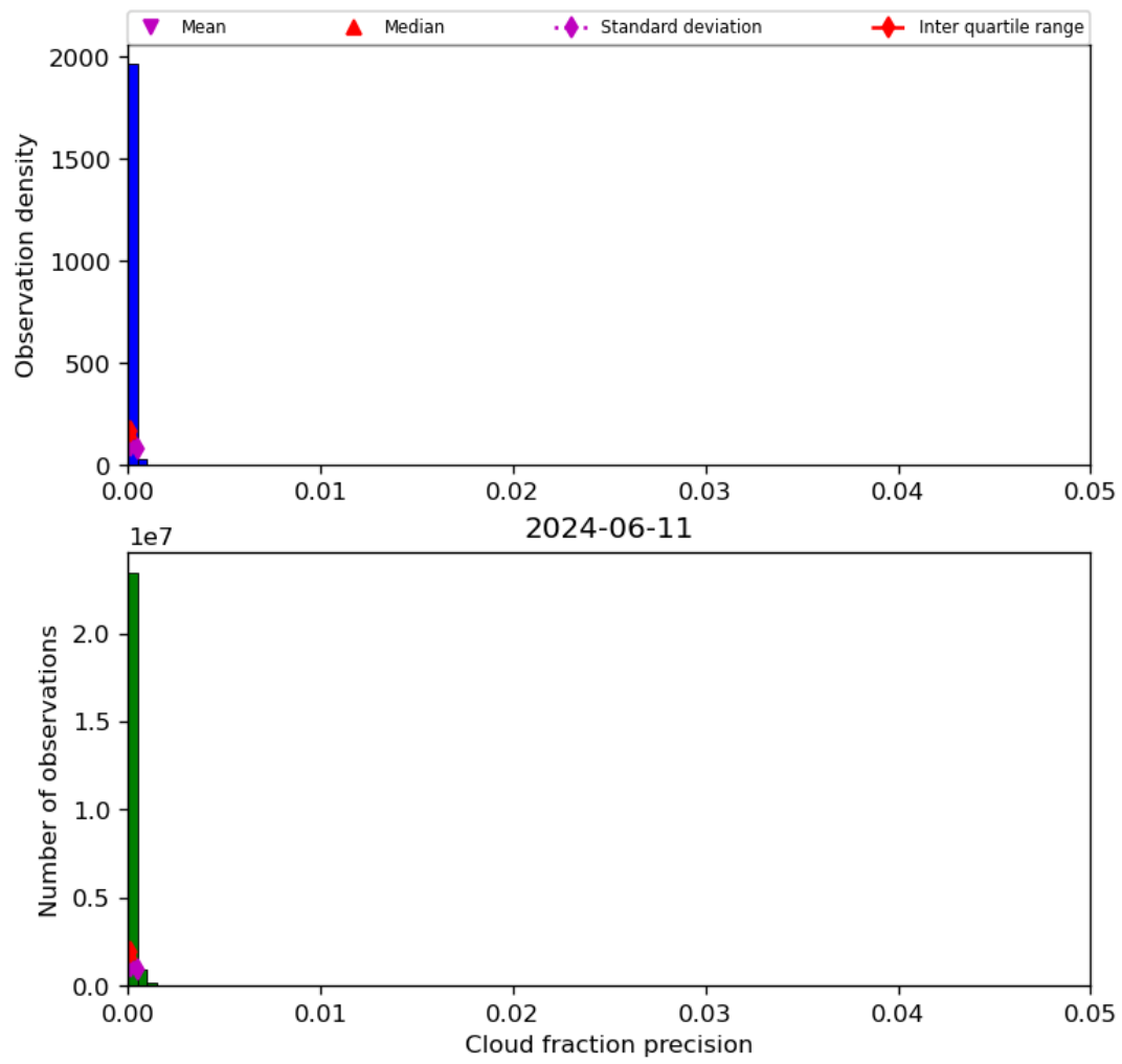
Figure 33: Histogram of “Cloud fraction precision” for 2024-06-10 to 2024-06-12
