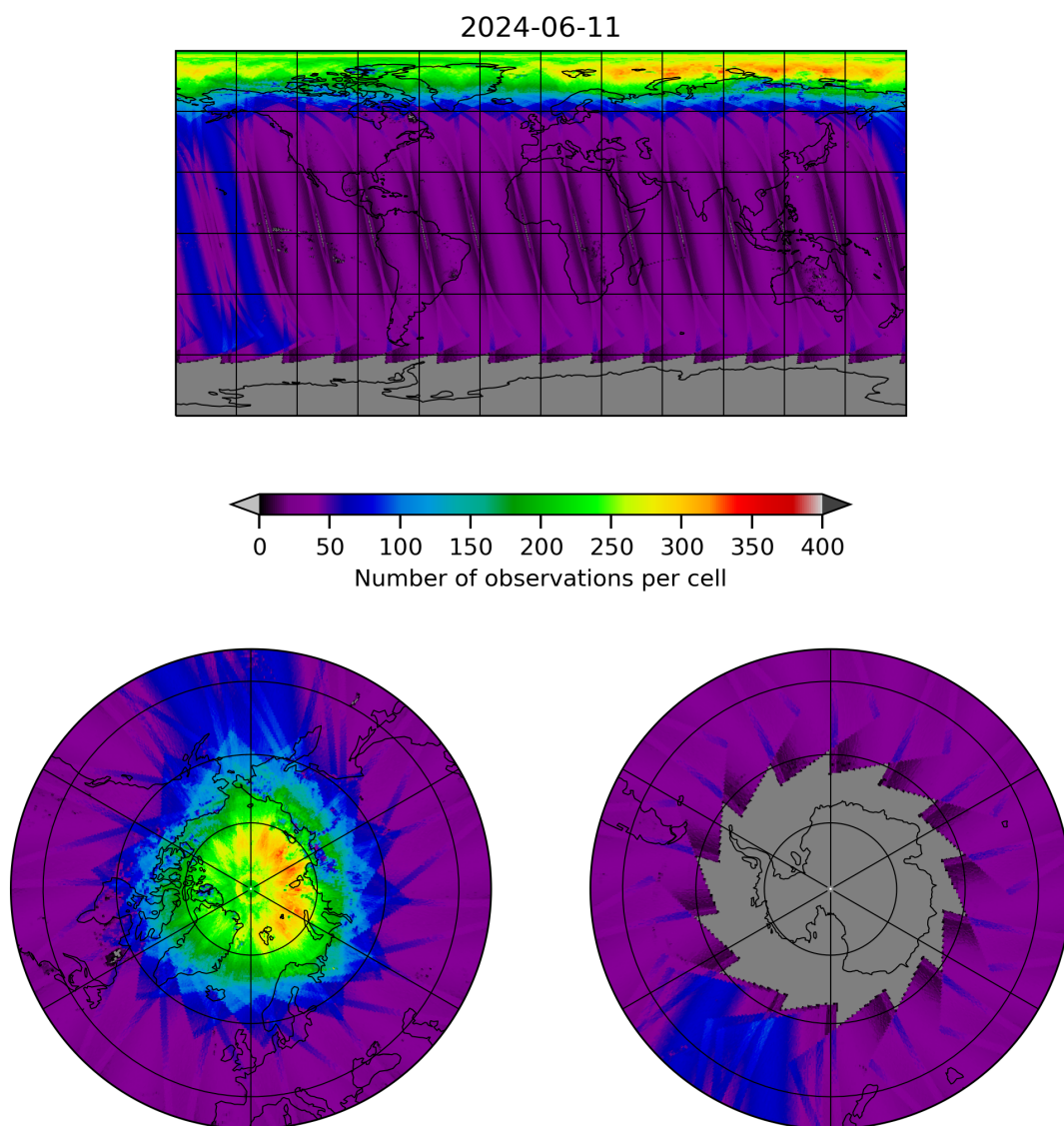
Figure 11: Map of the number of observations for 2024-06-10 to 2024-06-12
