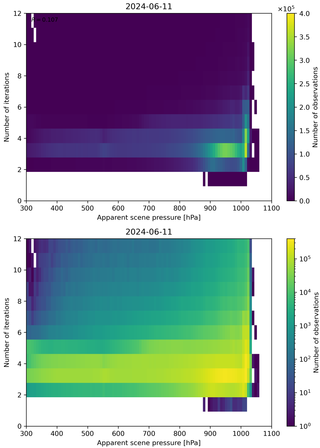
Figure 65: Scatter density plot of “Apparent scene pressure” against “Number of iterations” for 2024-06-10 to 2024-06-12.
