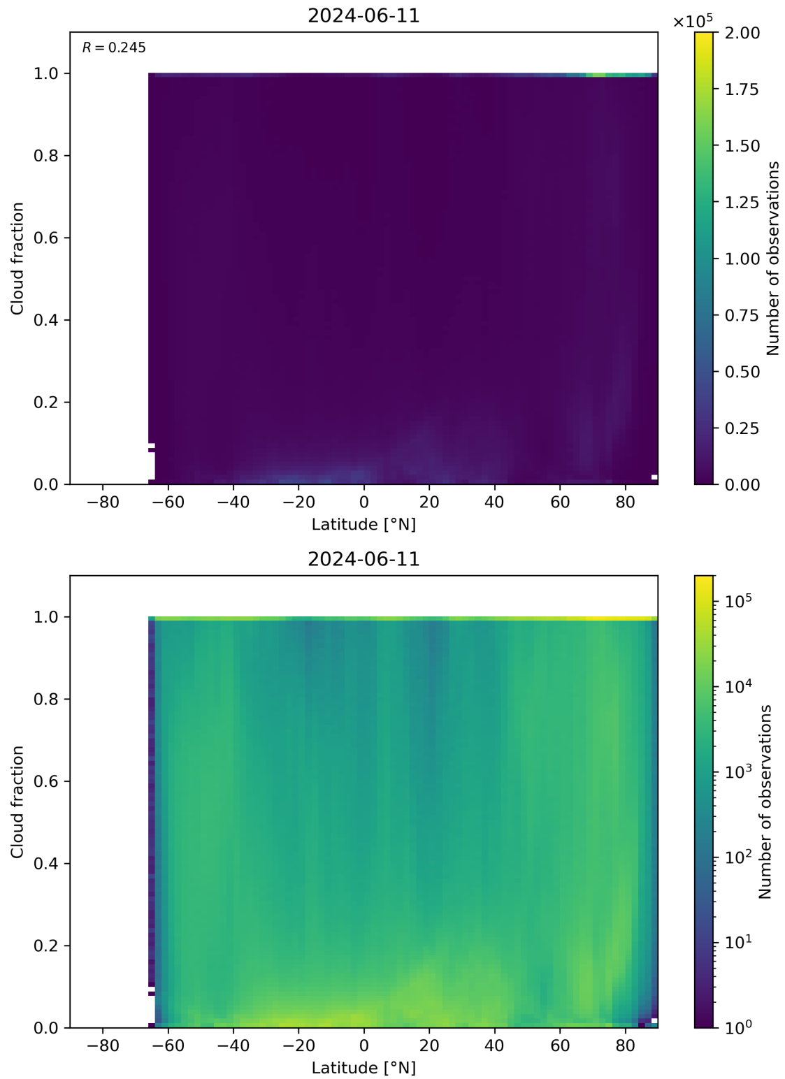
Figure 90: Scatter density plot of “Latitude” against “Cloud fraction” for 2024-06-10 to 2024-06-12.
