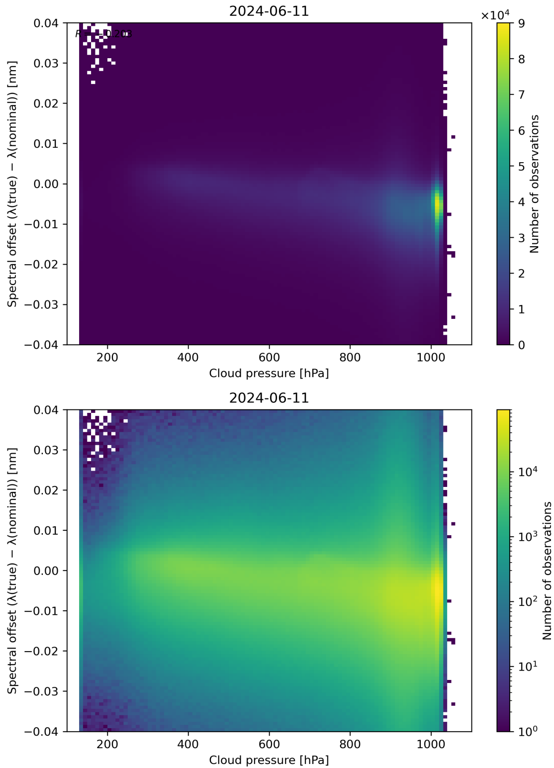
Figure 84: Scatter density plot of “Cloud pressure” against “Spectral offset ( \lambda(\text{true}) - \lambda(\text{nominal}) )” for 2024-06-10 to 2024-06-12.
