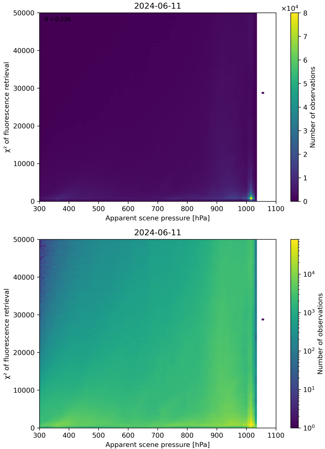
Figure 63: Scatter density plot of “Apparent scene pressure” against “ \chi^2 of fluorescence retrieval” for 2024-06-10 to 2024-06-12.
