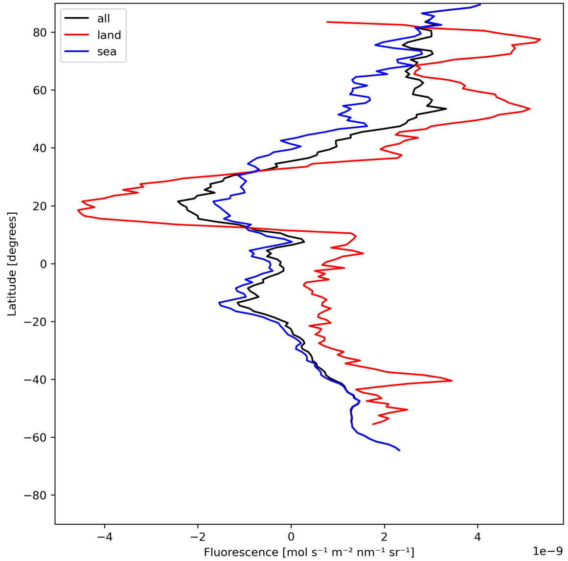
Figure 23: Zonal average of “Fluorescence” for 2024-06-10 to 2024-06-12.
