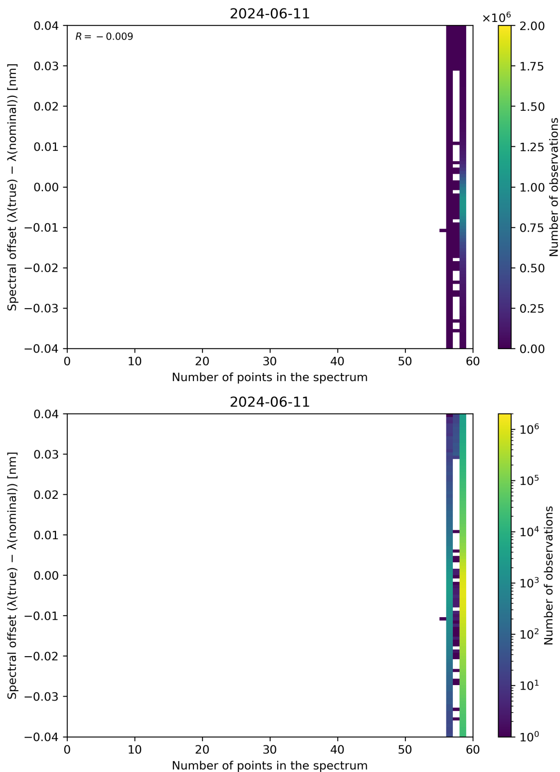
Figure 101: Scatter density plot of “Number of points in the spectrum” against “Spectral offset ( \lambda(\text{true}) - \lambda(\text{nominal}) )” for 2024-06-10 to 2024-06-12.
