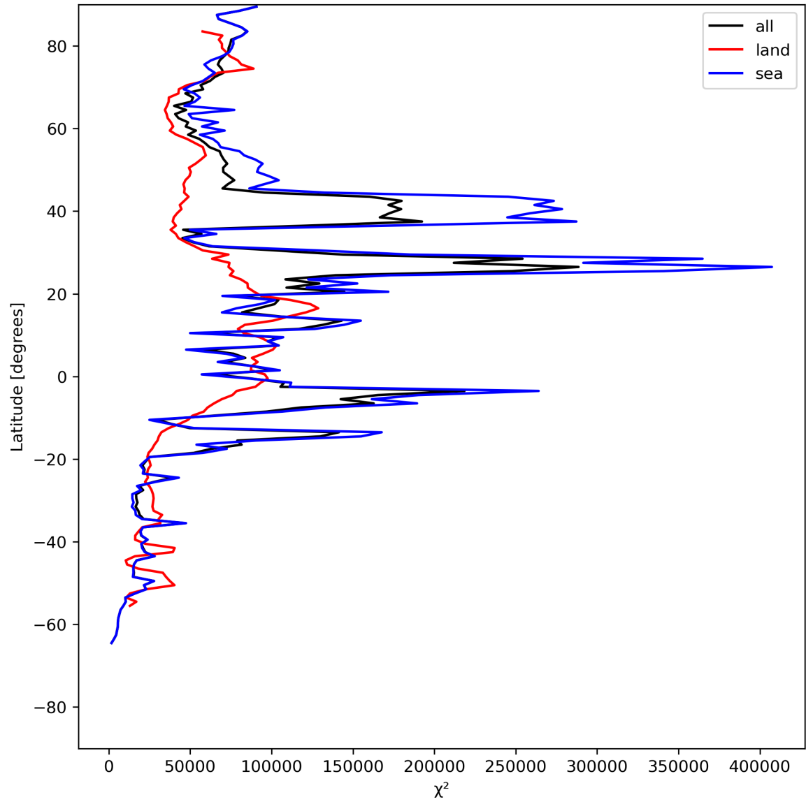
Figure 21: Zonal average of “ \chi^2 ” for 2024-06-10 to 2024-06-12.
