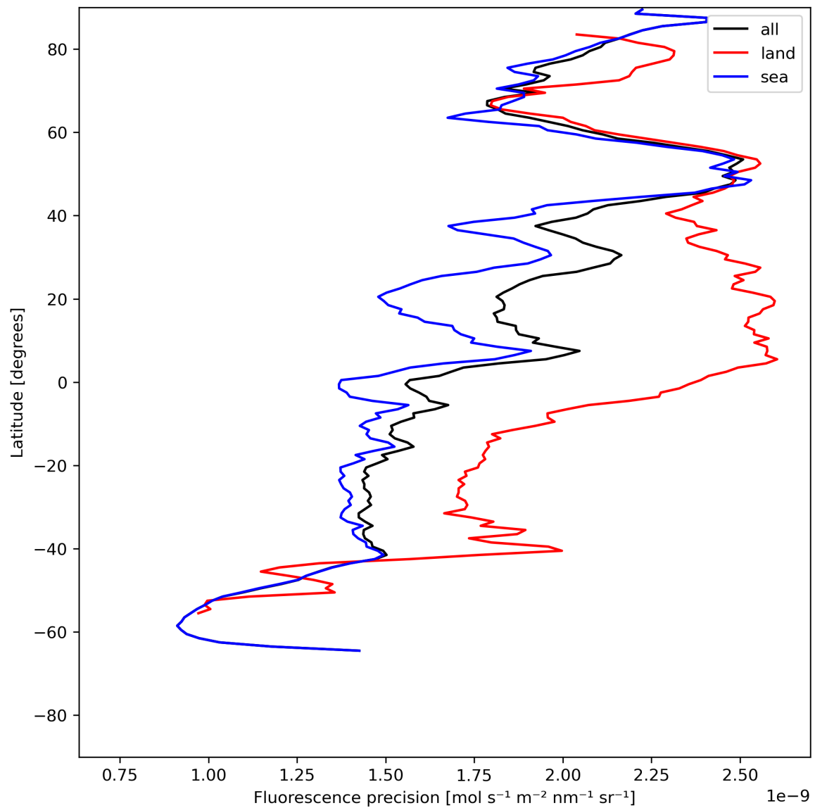
Figure 24: Zonal average of “Fluorescence precision” for 2024-06-10 to 2024-06-12.
