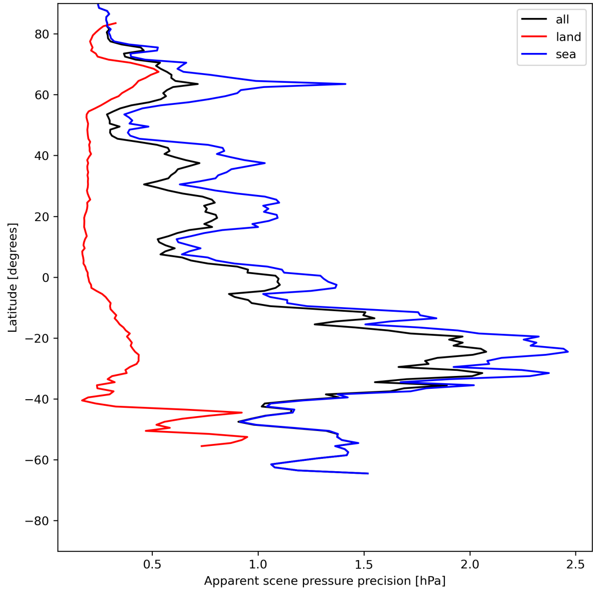
Figure 20: Zonal average of “Apparent scene pressure precision” for 2024-06-10 to 2024-06-12.
