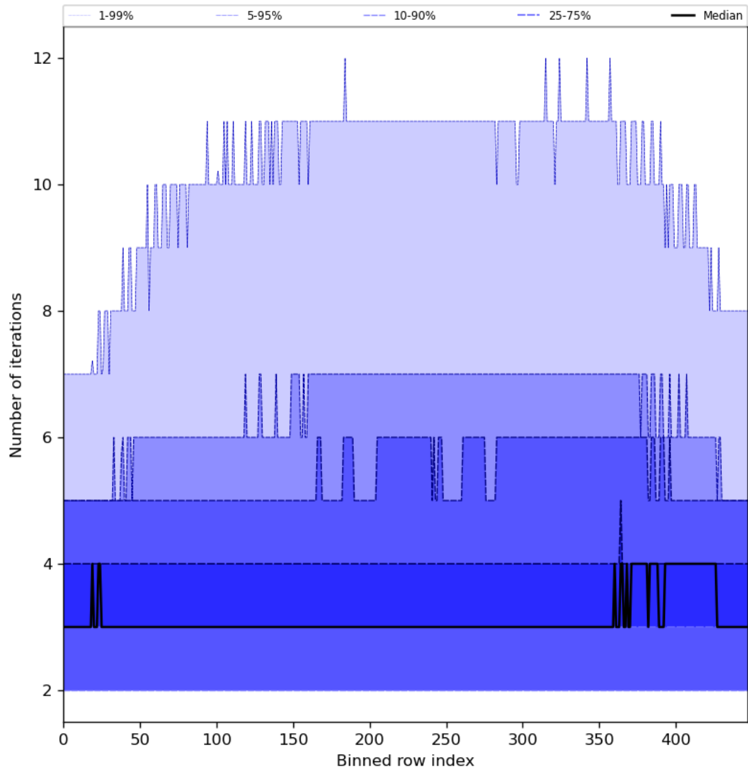
Figure 56: Along track statistics of “Number of iterations” for 2024-06-10 to 2024-06-12
