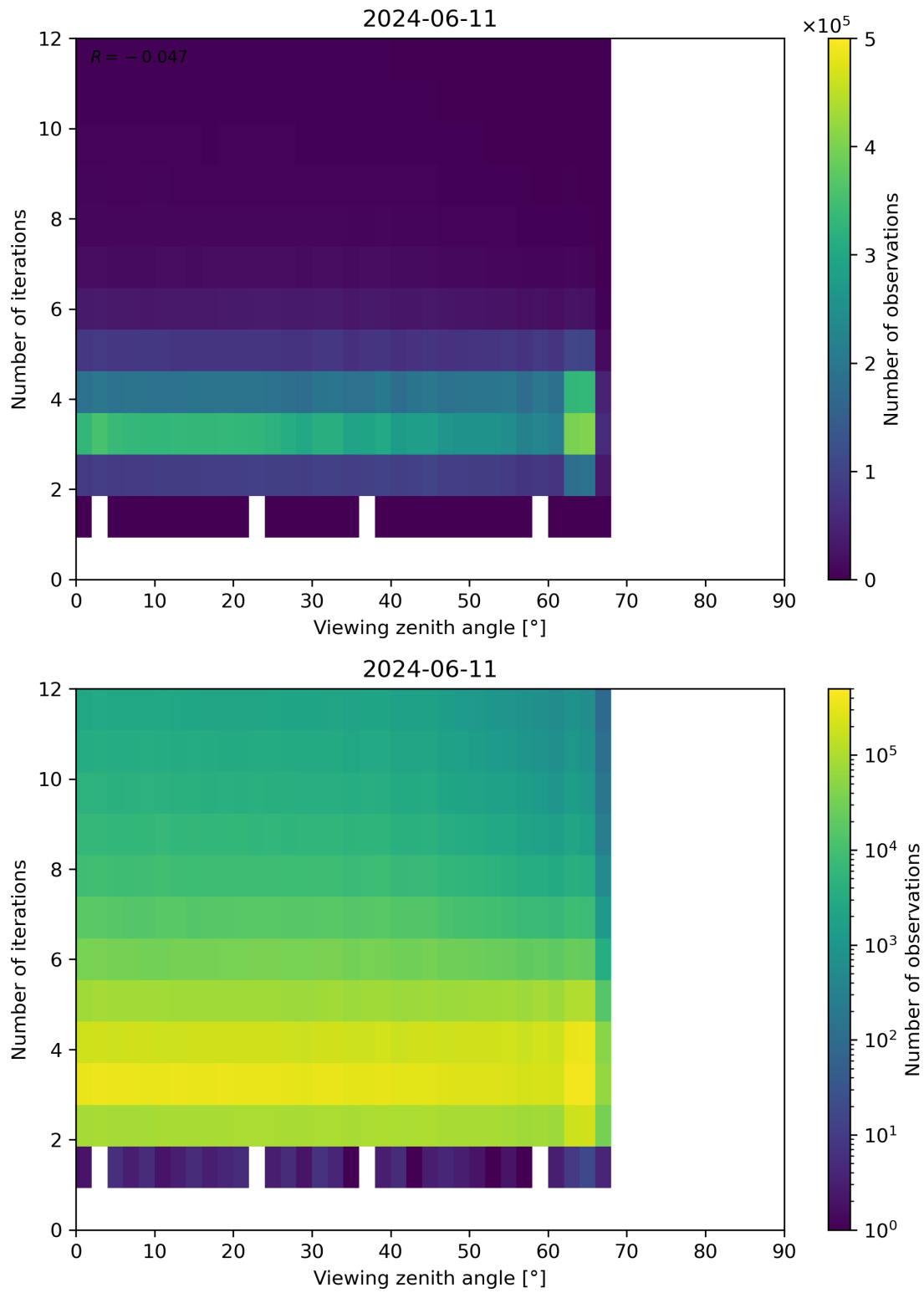
Figure 124: Scatter density plot of “Viewing zenith angle” against “Number of iterations” for 2024-06-10 to 2024-06-12.
