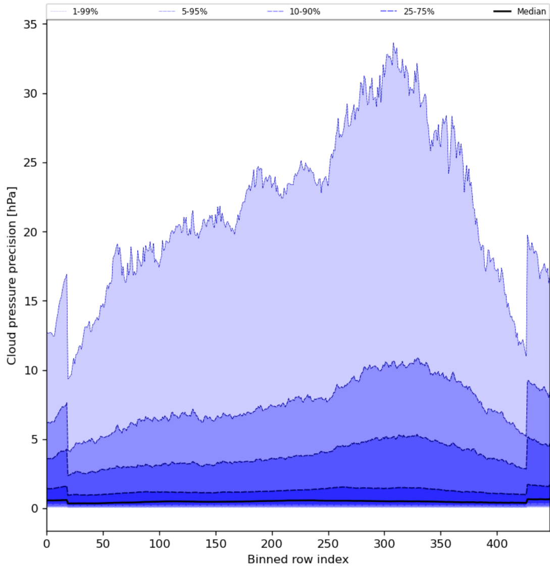
Figure 48: Along track statistics of “Cloud pressure precision” for 2024-06-10 to 2024-06-12
