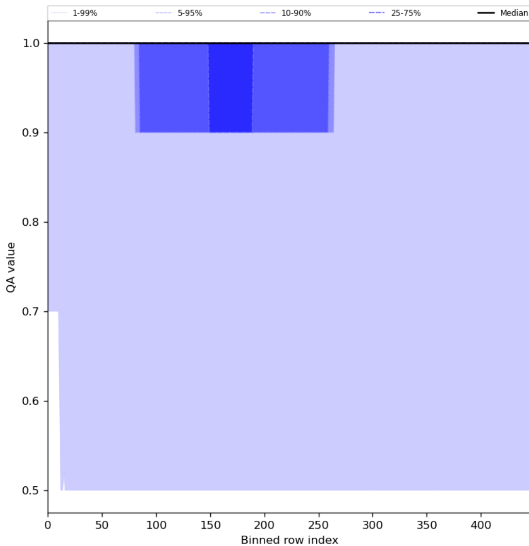
Figure 46: Along track statistics of “QA value” for 2024-06-10 to 2024-06-12
