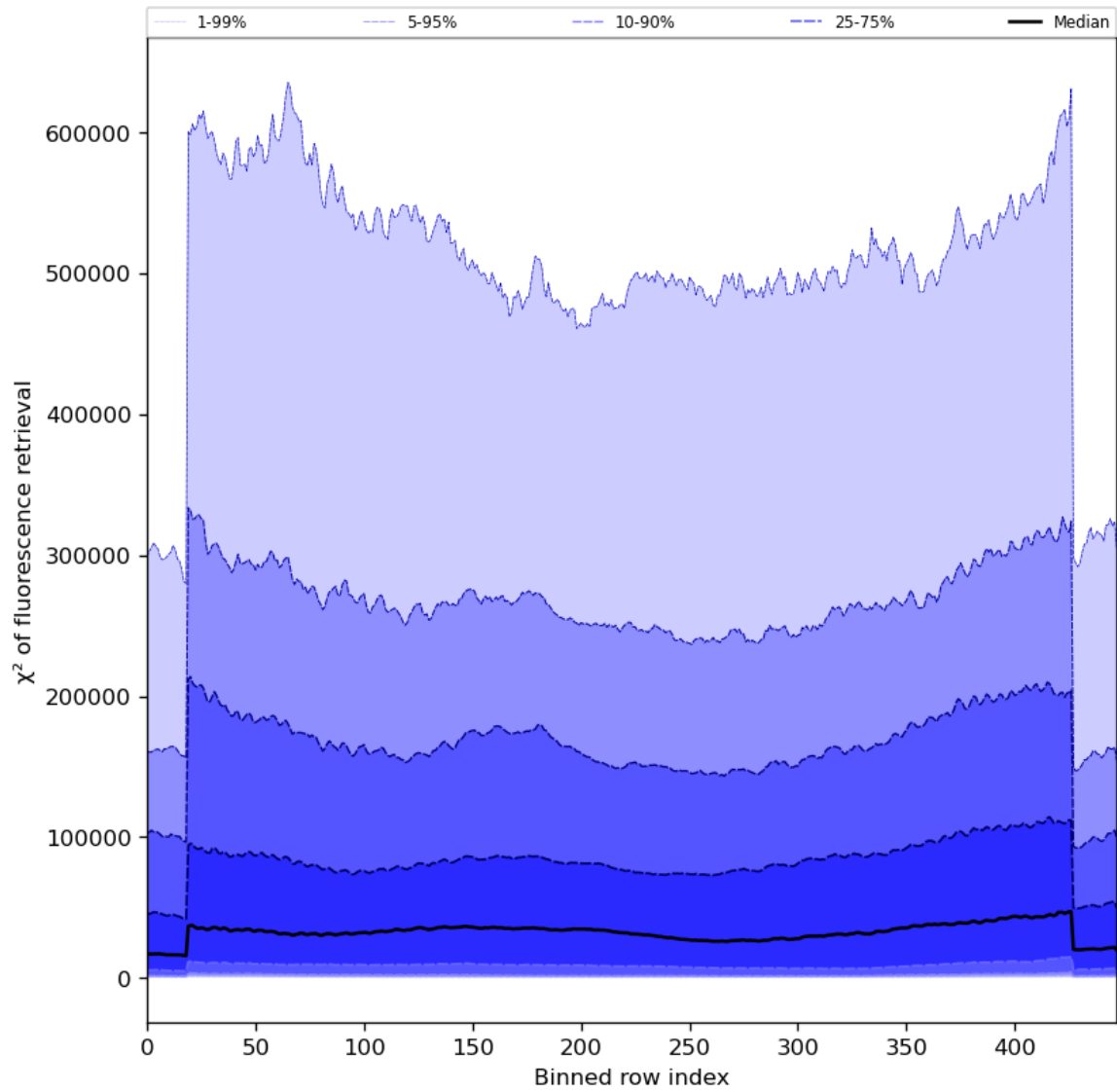
Figure 59: Along track statistics of “ \chi^2 of fluorescence retrieval” for 2024-06-10 to 2024-06-12
