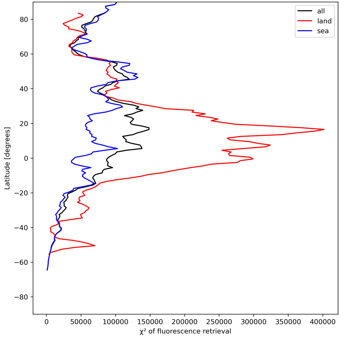
Figure 25: Zonal average of “ \chi^2 of fluorescence retrieval” for 2024-06-10 to 2024-06-12.
