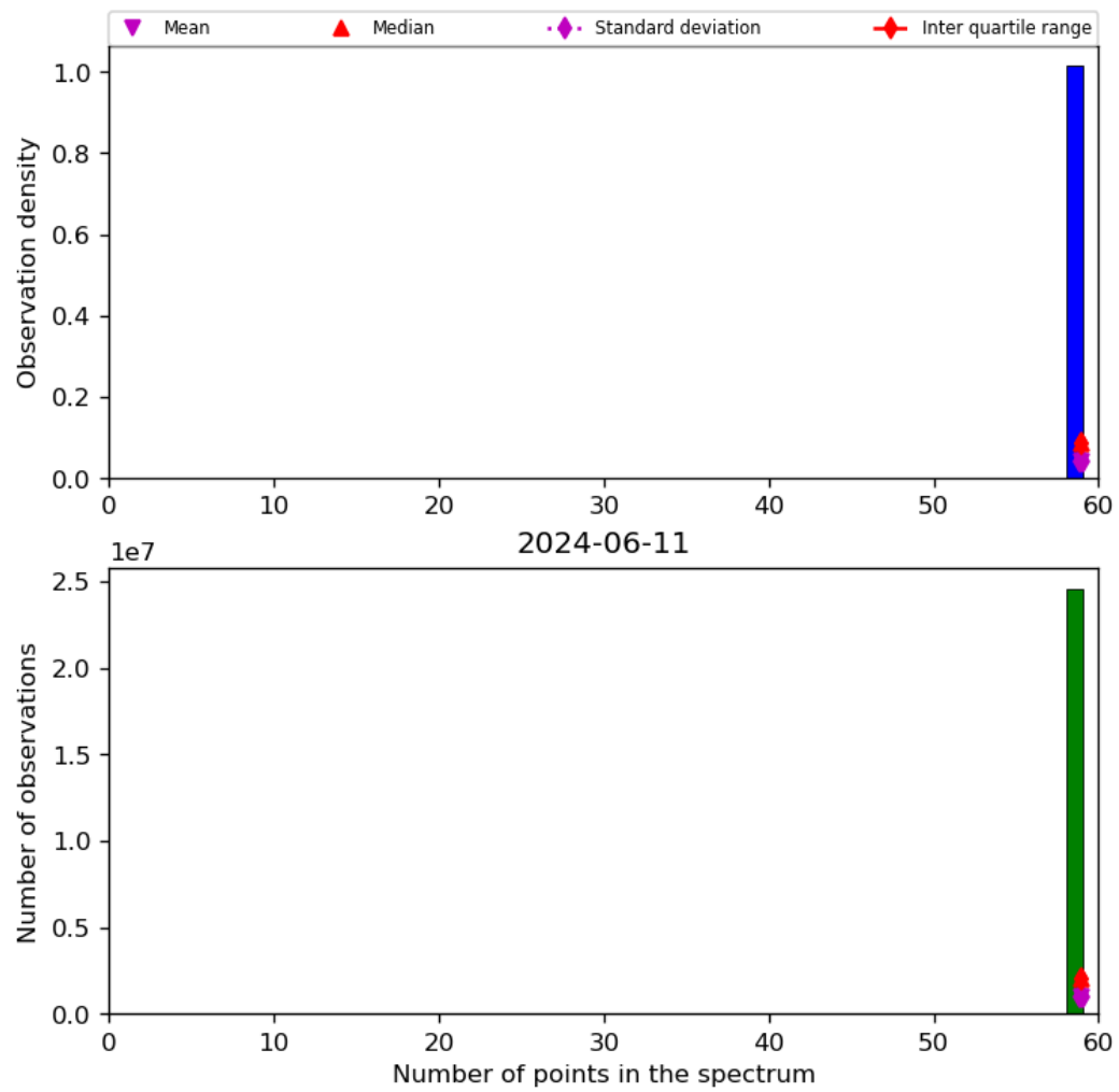
Figure 44: Histogram of “Number of points in the spectrum” for 2024-06-10 to 2024-06-12
