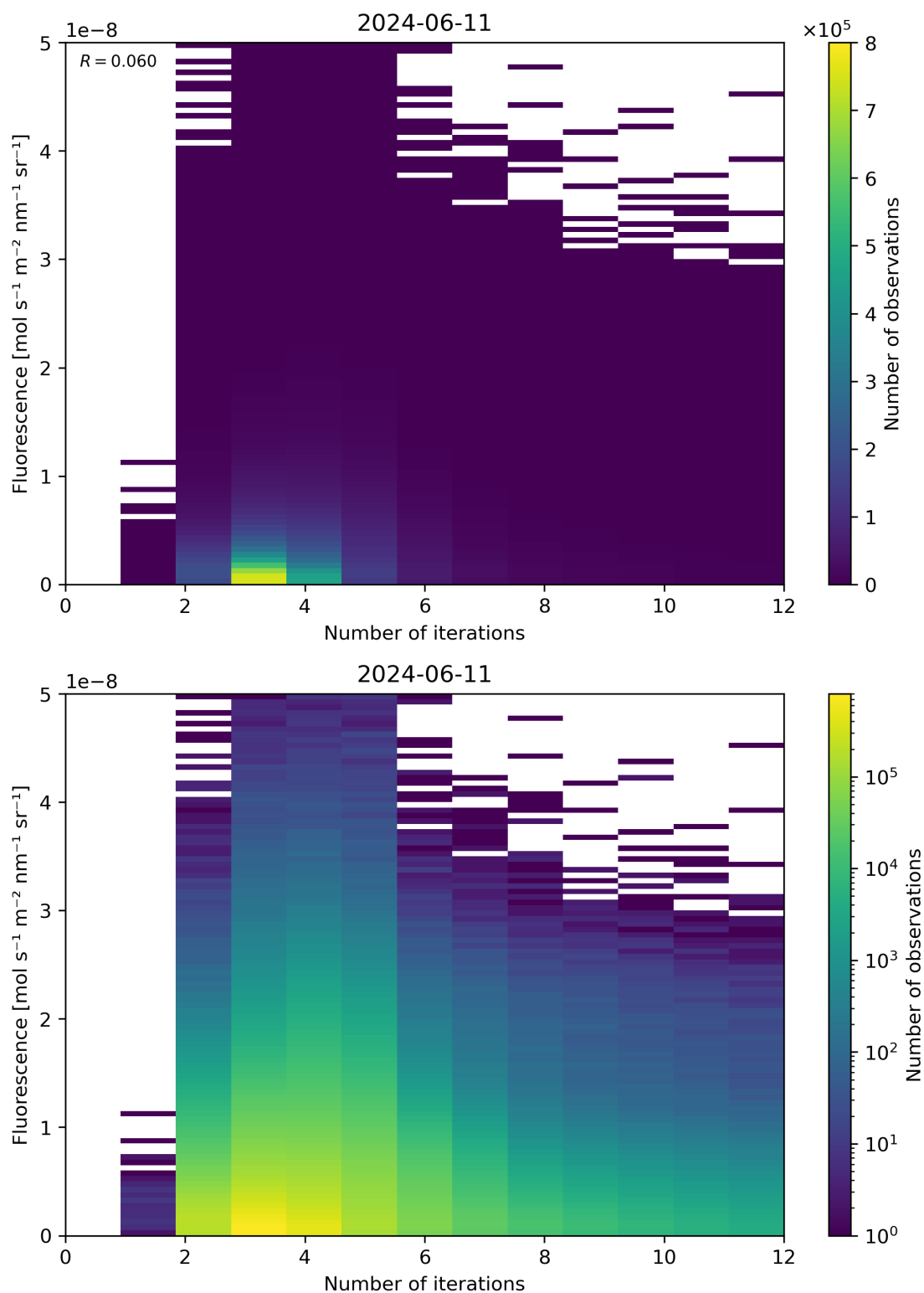
Figure 98: Scatter density plot of “Number of iterations” against “Fluorescence” for 2024-06-10 to 2024-06-12.
