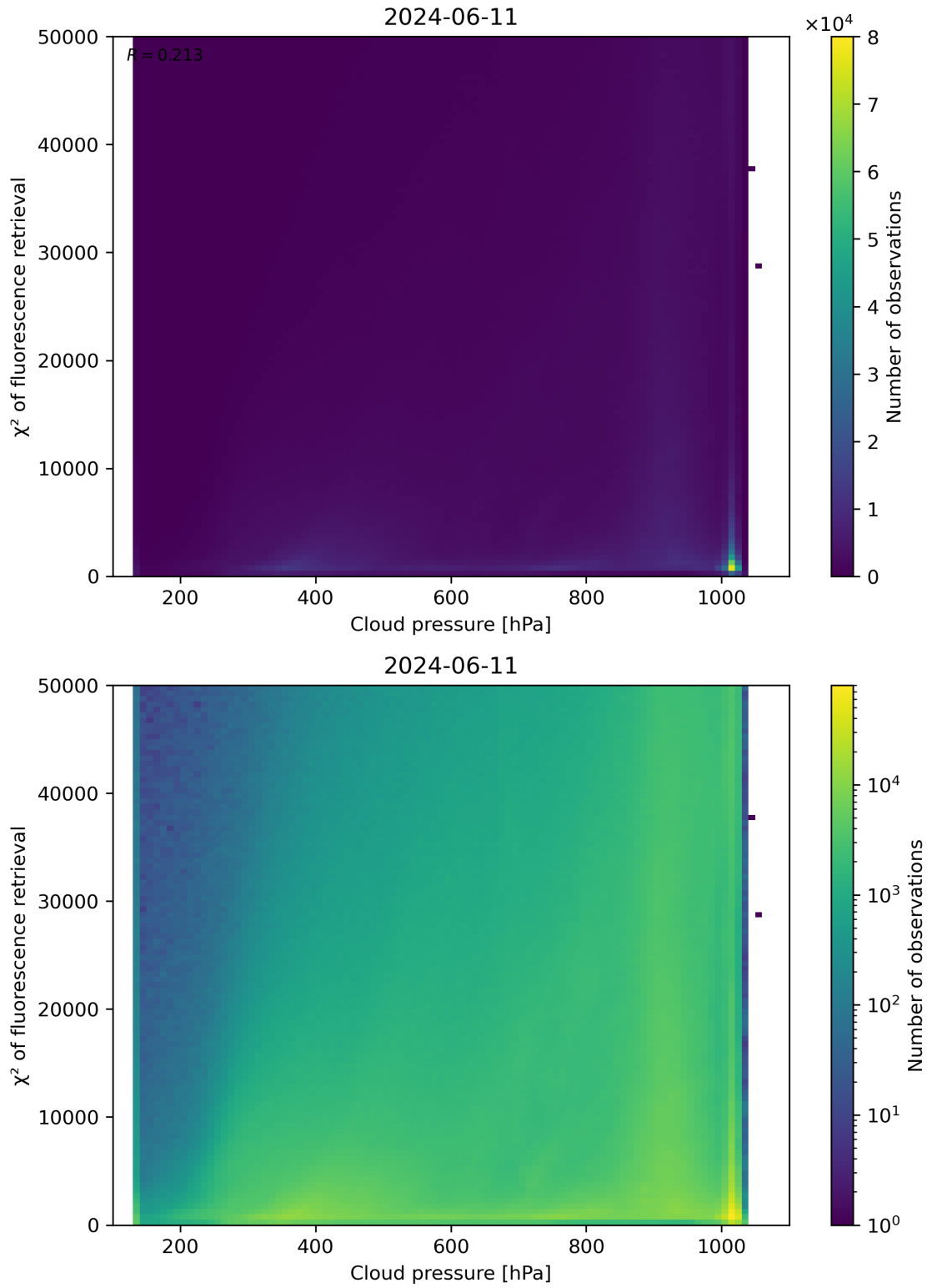
Figure 78: Scatter density plot of “Cloud pressure” against “ \chi^2 of fluorescence retrieval” for 2024-06-10 to 2024-06-12.
