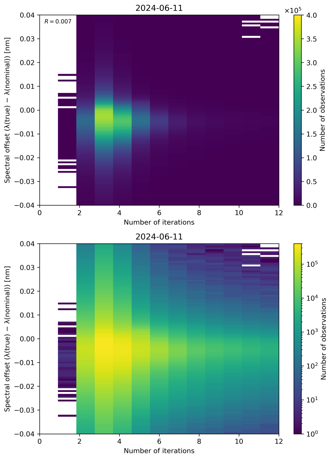
Figure 100: Scatter density plot of “Number of iterations” against “Spectral offset ( \lambda(\text{true}) - \lambda(\text{nominal}) )” for 2024-06-10 to 2024-06-12.
