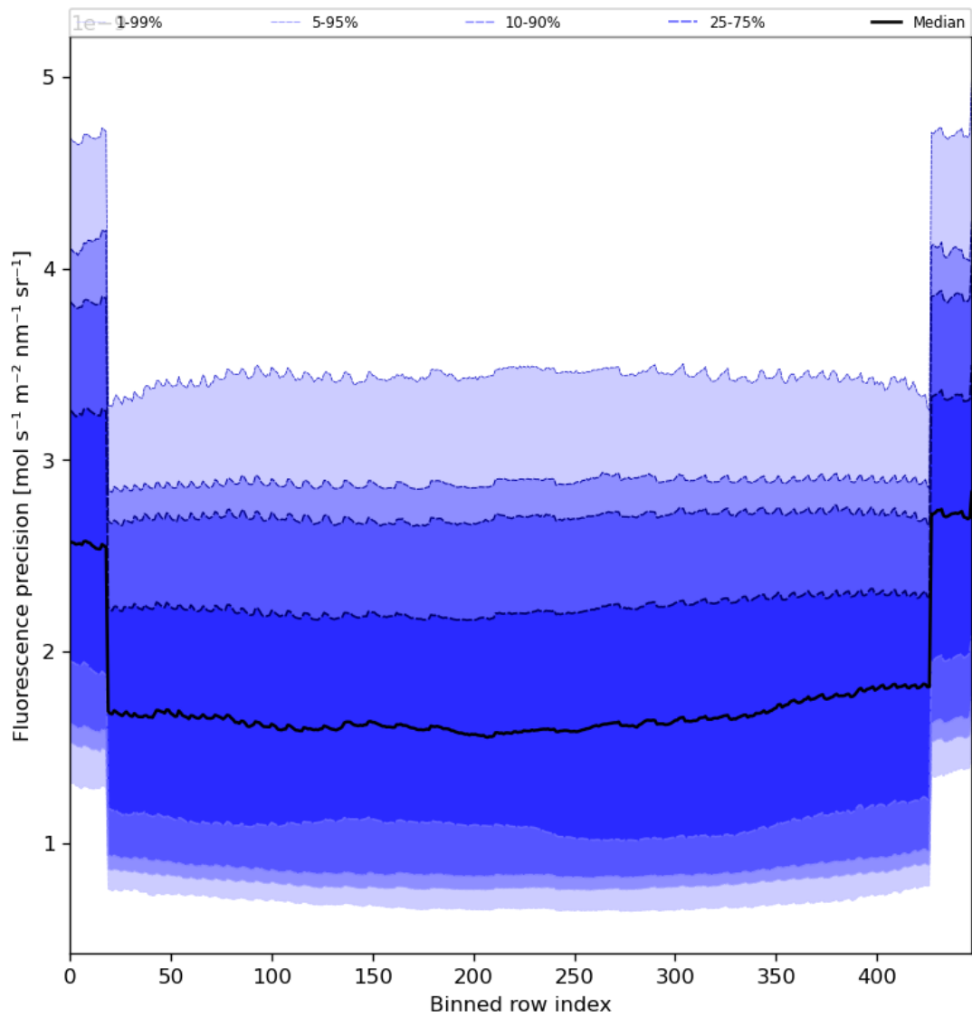
Figure 58: Along track statistics of “Fluorescence precision” for 2024-06-10 to 2024-06-12
