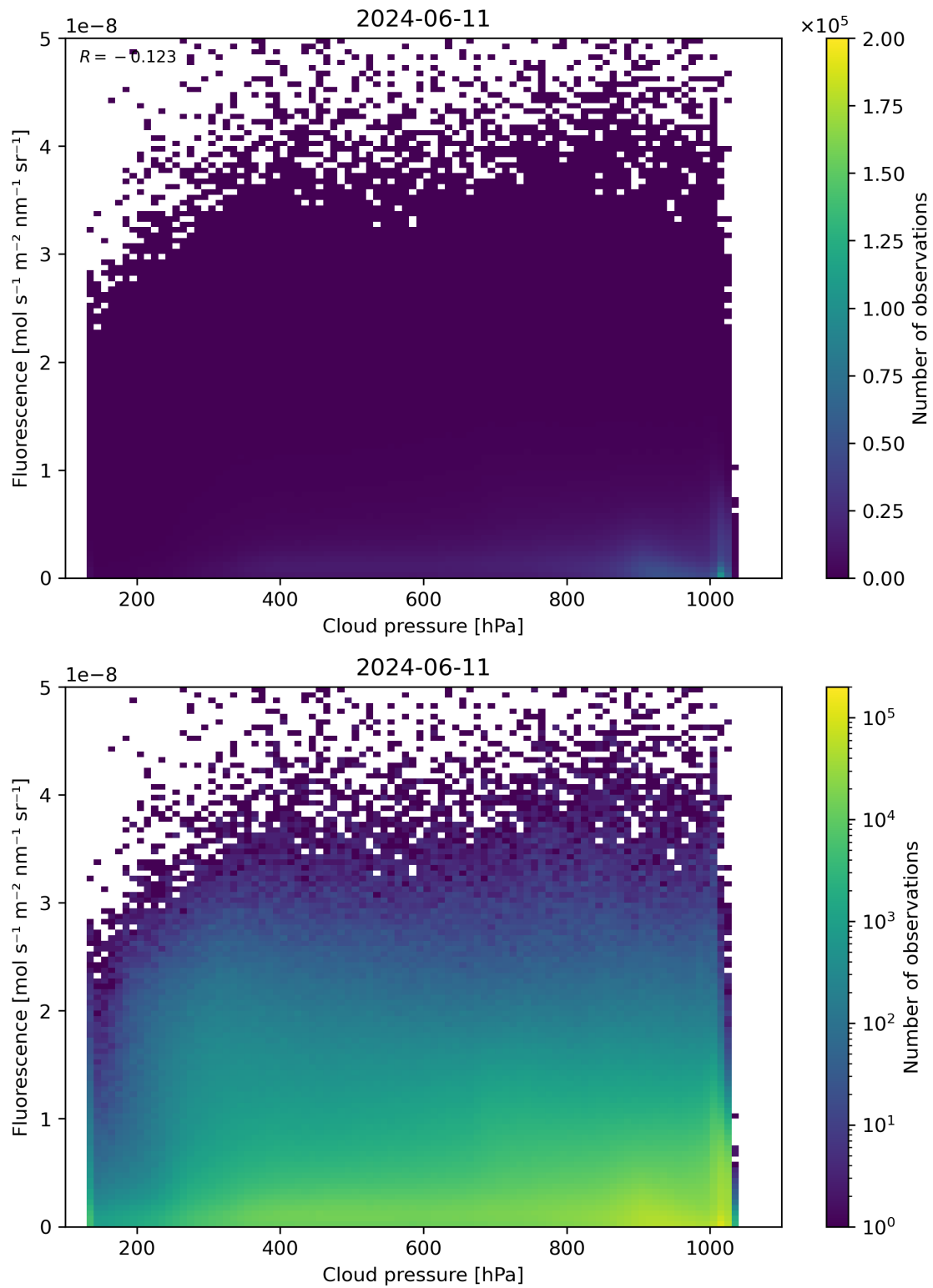
Figure 80: Scatter density plot of “Cloud pressure” against “Fluorescence” for 2024-06-10 to 2024-06-12.
