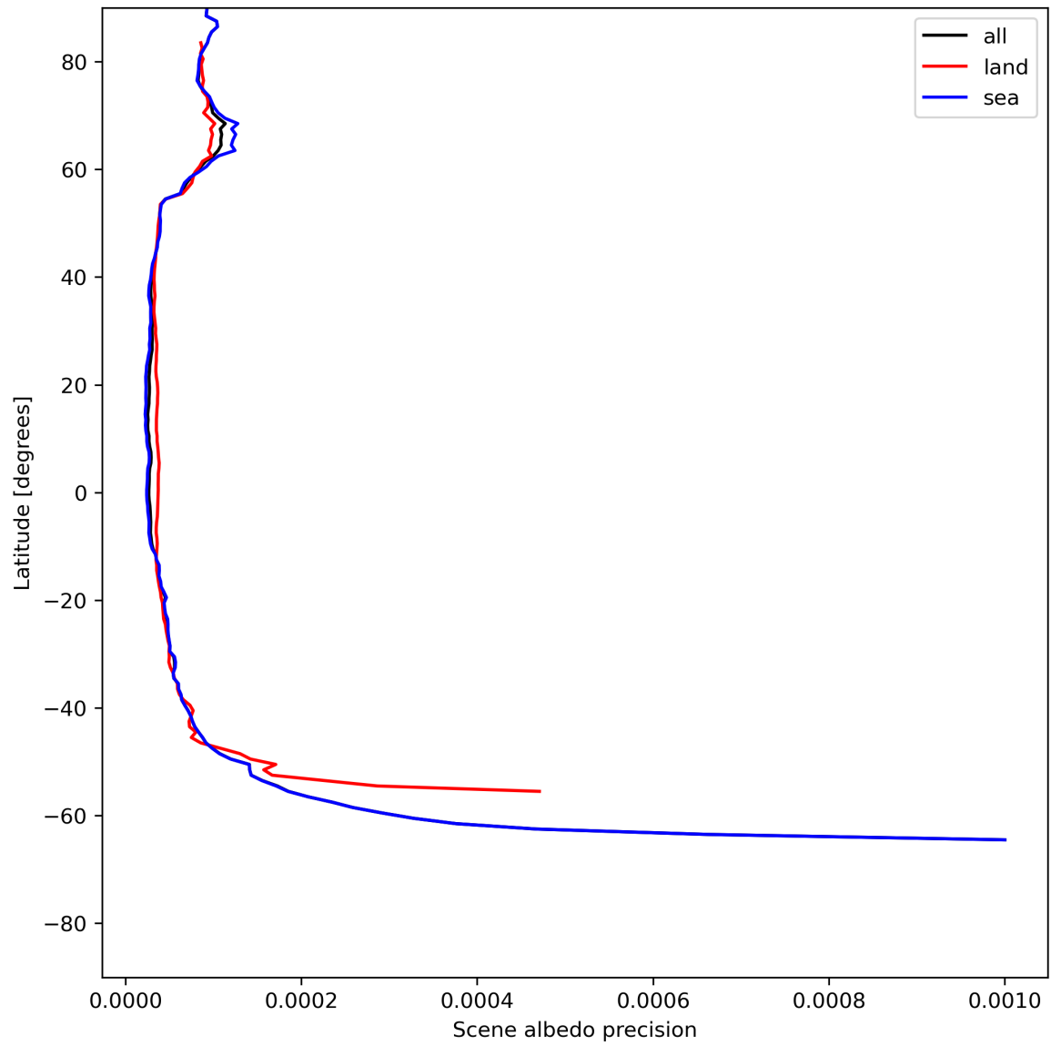
Figure 18: Zonal average of “Scene albedo precision” for 2024-06-10 to 2024-06-12.
