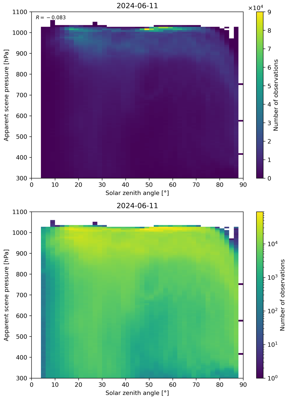
Figure 108: Scatter density plot of “Solar zenith angle” against “Apparent scene pressure” for 2024-06-10 to 2024-06-12.
