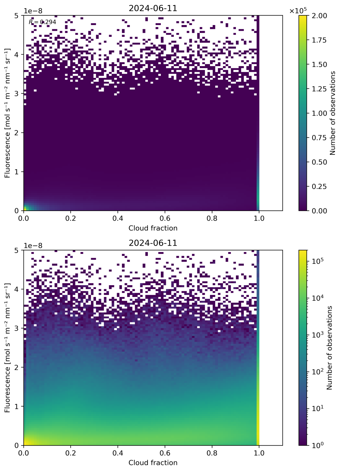
Figure 72: Scatter density plot of “Cloud fraction” against “Fluorescence” for 2024-06-10 to 2024-06-12.
