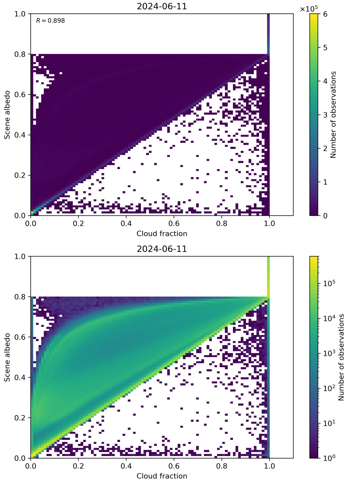
Figure 75: Scatter density plot of “Cloud fraction” against “Scene albedo” for 2024-06-10 to 2024-06-12.
