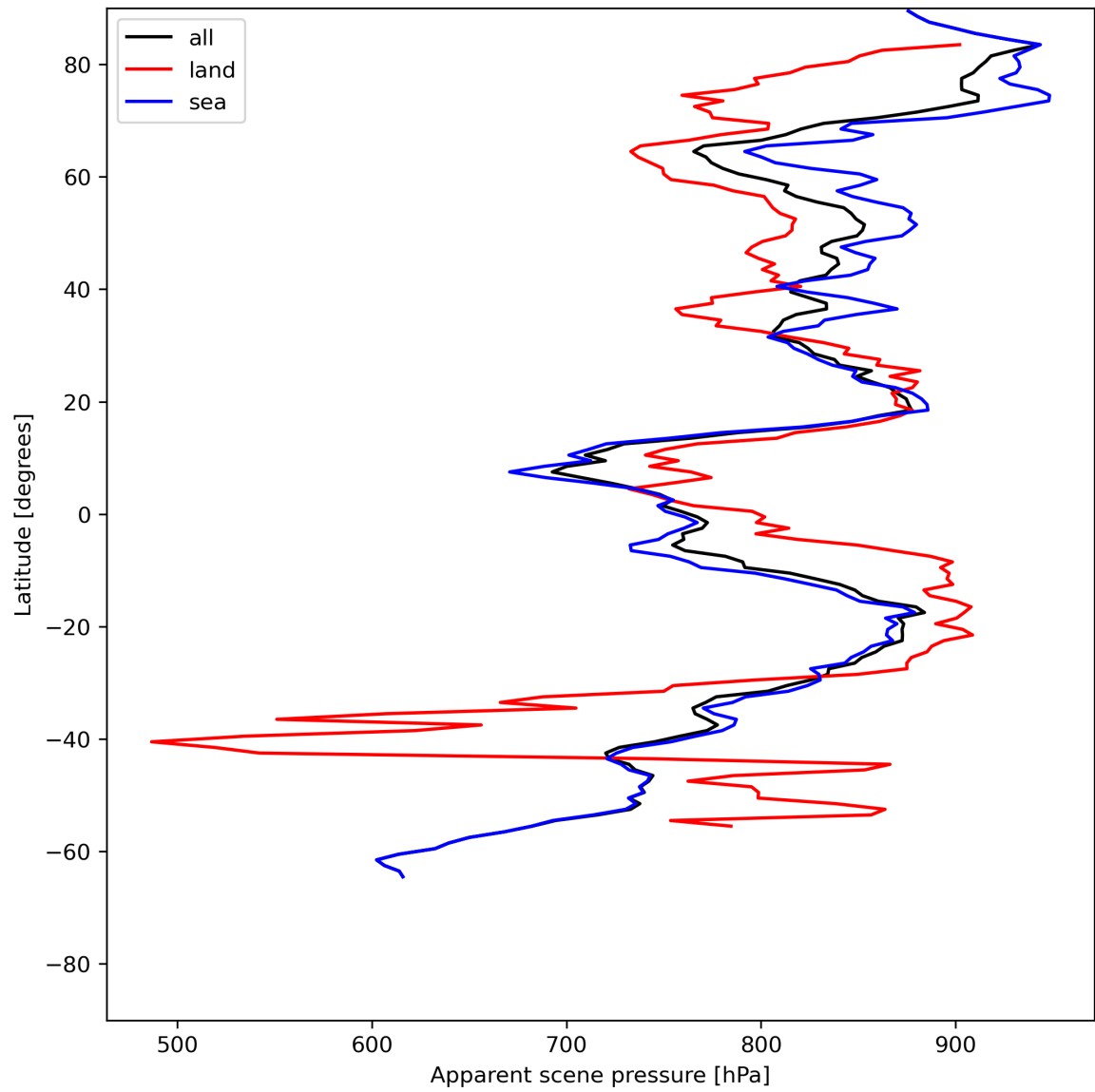
Figure 19: Zonal average of “Apparent scene pressure” for 2024-06-10 to 2024-06-12.
