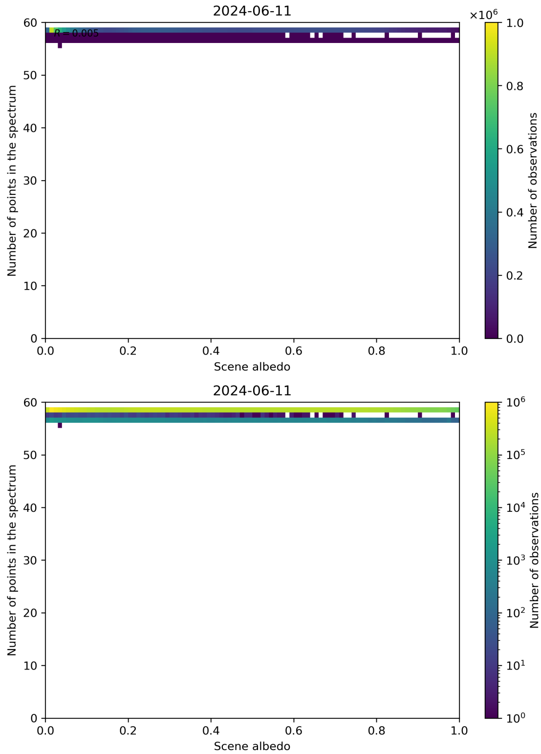
Figure 106: Scatter density plot of “Scene albedo” against “Number of points in the spectrum” for 2024-06-10 to 2024-06-12.
