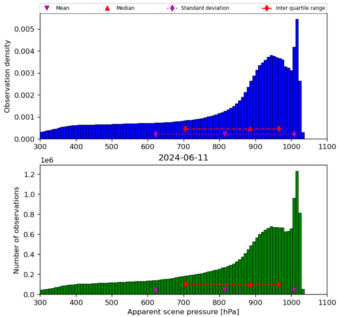
Figure 36: Histogram of “Apparent scene pressure” for 2024-06-10 to 2024-06-12
