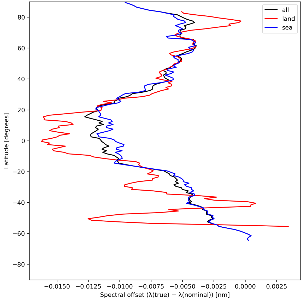
Figure 28: Zonal average of “Spectral offset ( \lambda(\text{true}) - \lambda(\text{nominal}) )” for 2024-06-10 to 2024-06-12.
