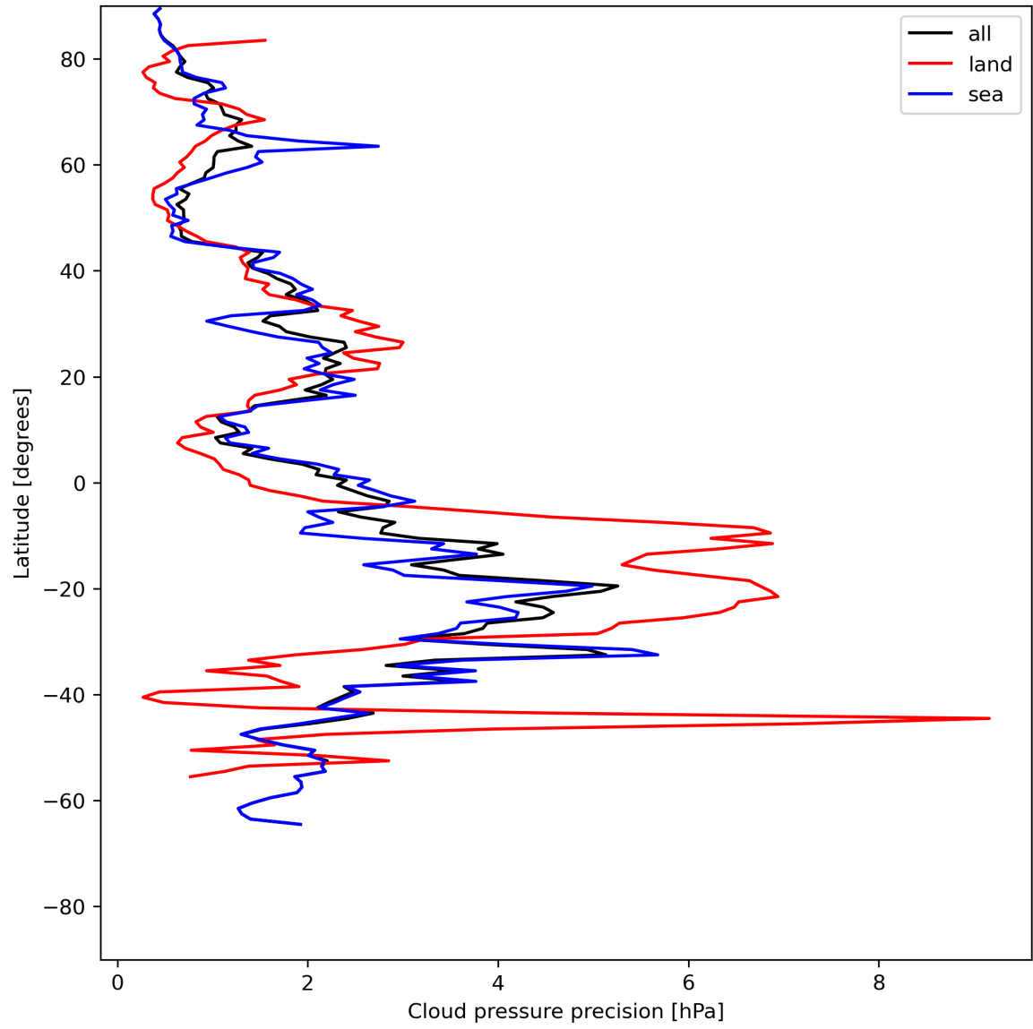
Figure 14: Zonal average of “Cloud pressure precision” for 2024-06-10 to 2024-06-12.
