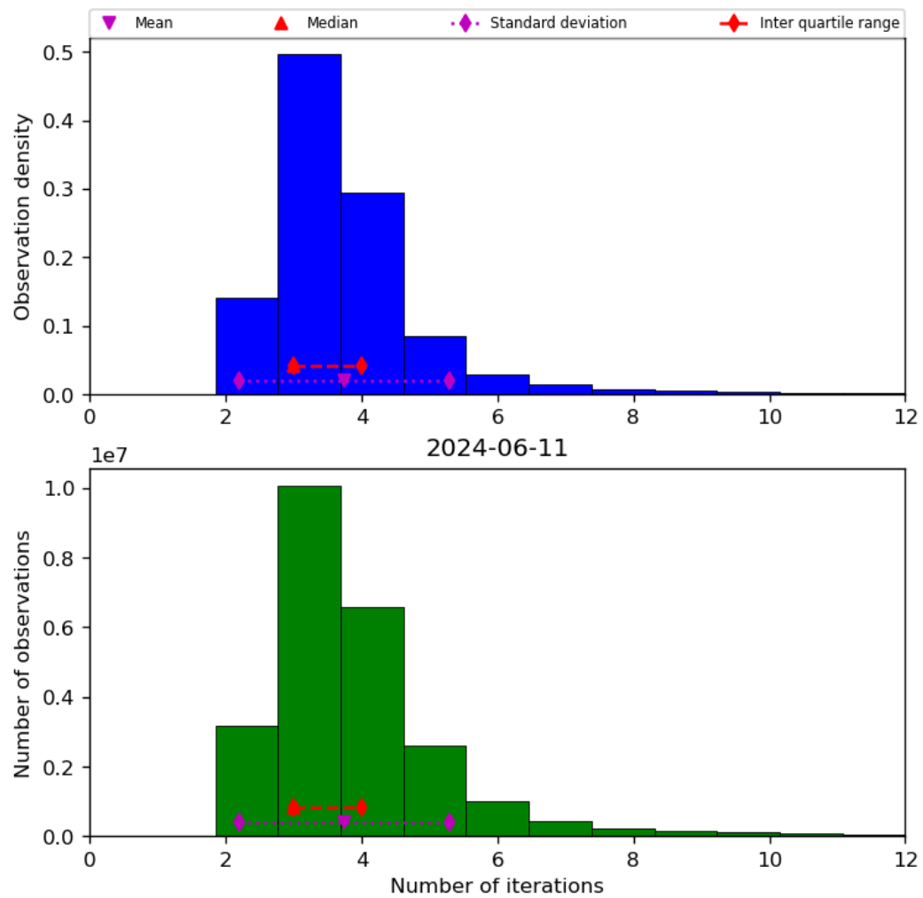
Figure 39: Histogram of “Number of iterations” for 2024-06-10 to 2024-06-12
