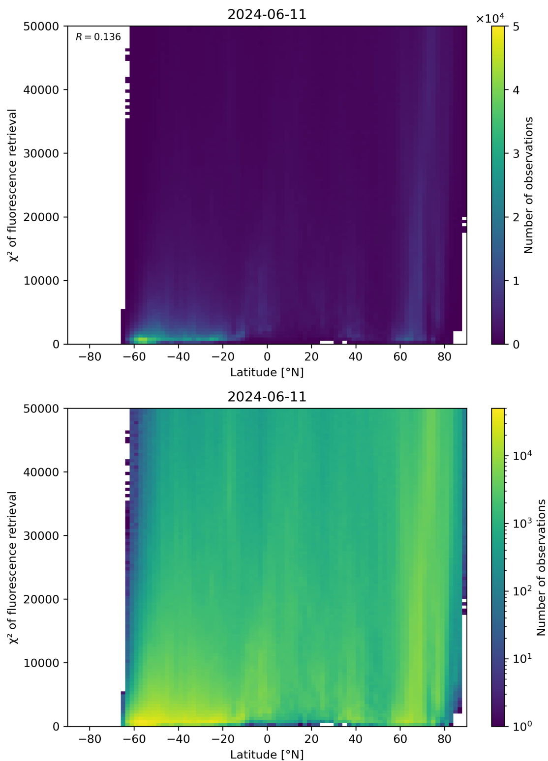
Figure 89: Scatter density plot of “Latitude” against “ \chi^2 of fluorescence retrieval” for 2024-06-10 to 2024-06-12.
