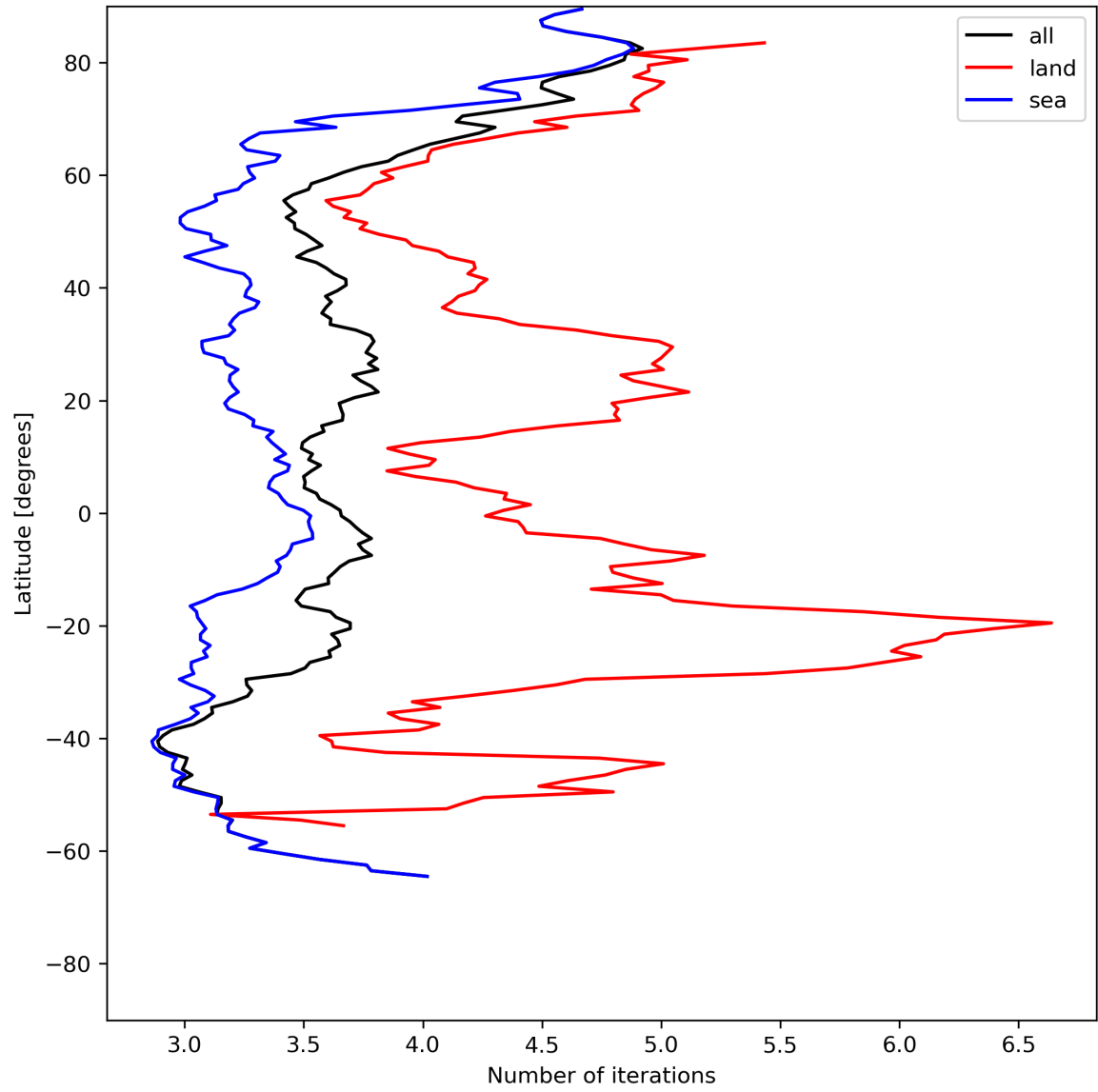
Figure 22: Zonal average of “Number of iterations” for 2024-06-10 to 2024-06-12.
