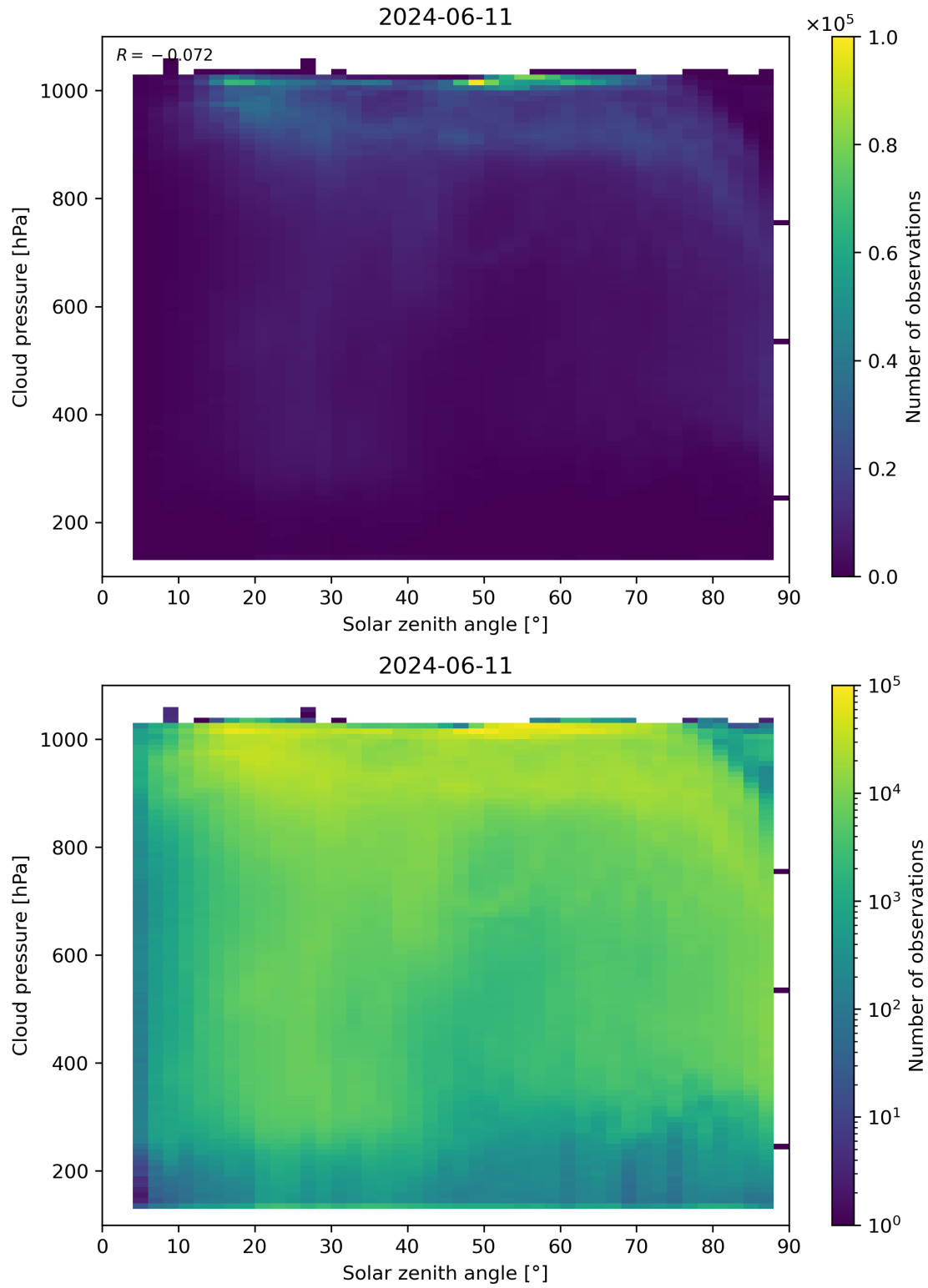
Figure 111: Scatter density plot of “Solar zenith angle” against “Cloud pressure” for 2024-06-10 to 2024-06-12.
