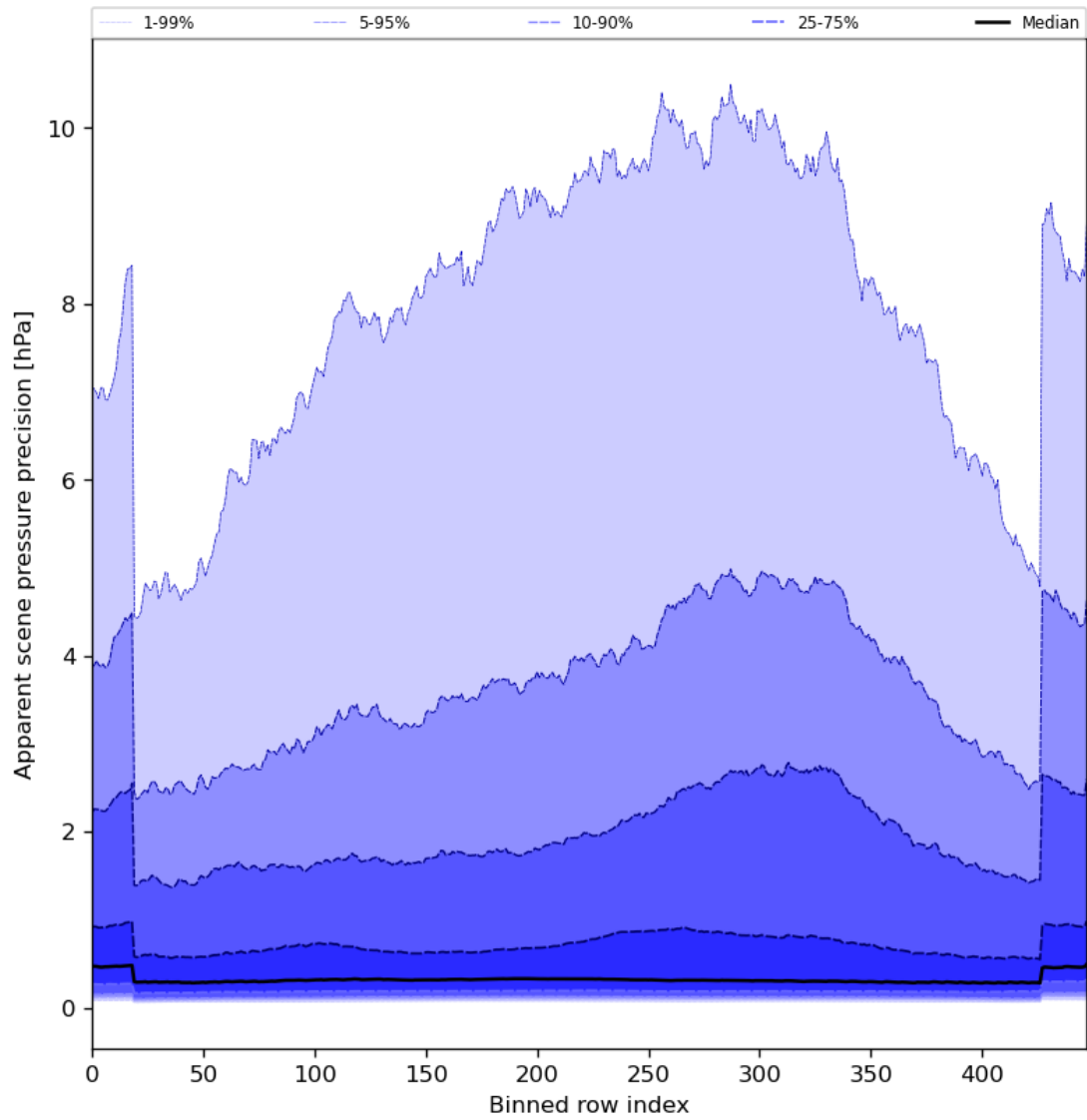
Figure 54: Along track statistics of “Apparent scene pressure precision” for 2024-06-10 to 2024-06-12
