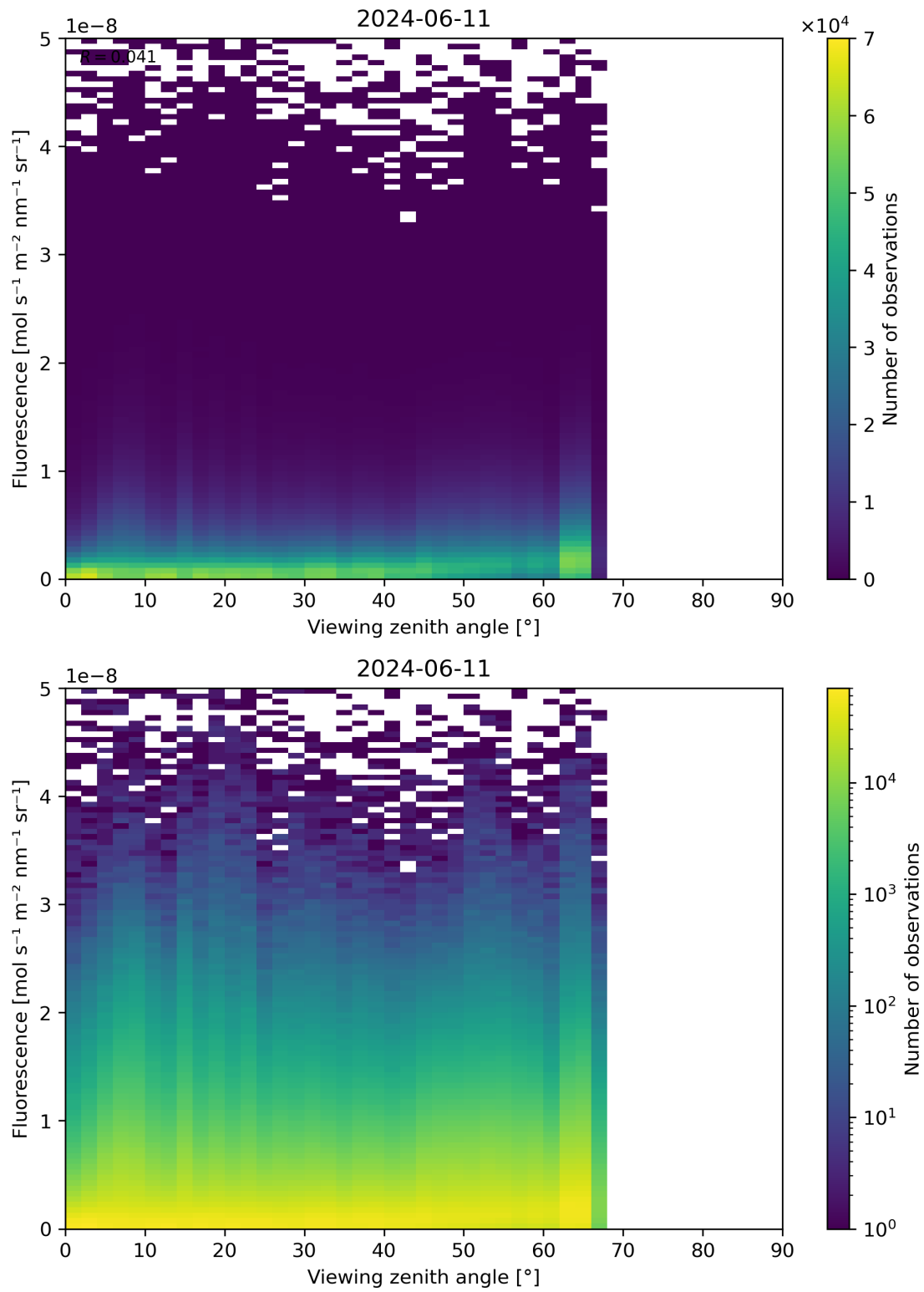
Figure 122: Scatter density plot of “Viewing zenith angle” against “Fluorescence” for 2024-06-10 to 2024-06-12.
