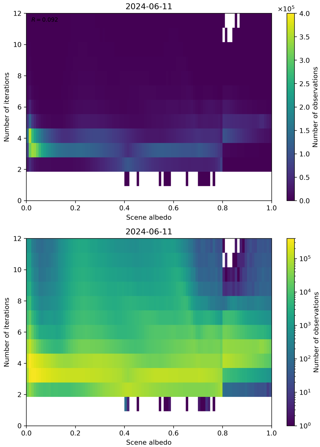
Figure 105: Scatter density plot of “Scene albedo” against “Number of iterations” for 2024-06-10 to 2024-06-12.
