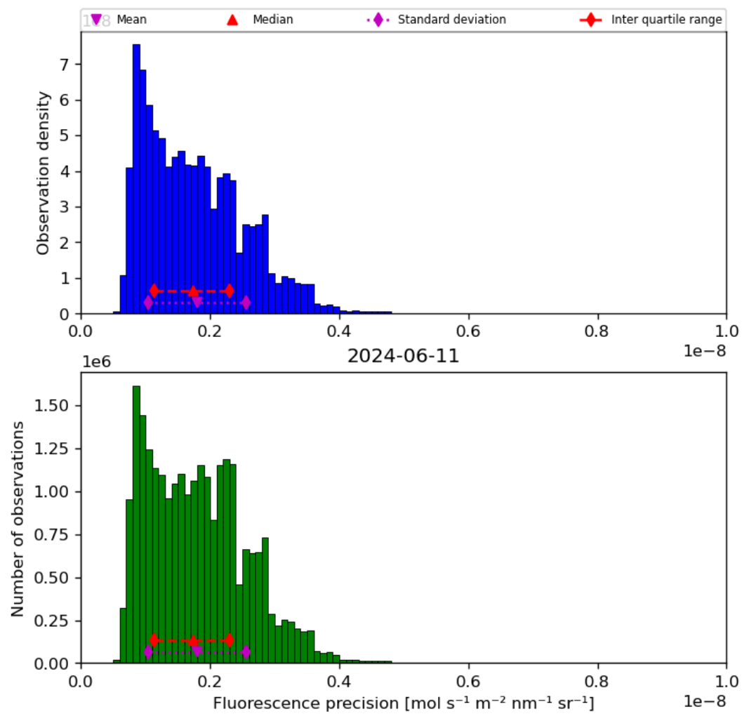
Figure 41: Histogram of “Fluorescence precision” for 2024-06-10 to 2024-06-12
