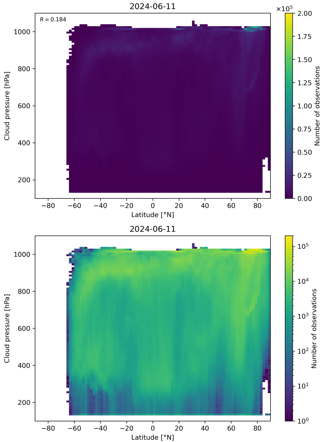
Figure 91: Scatter density plot of “Latitude” against “Cloud pressure” for 2024-06-10 to 2024-06-12.
