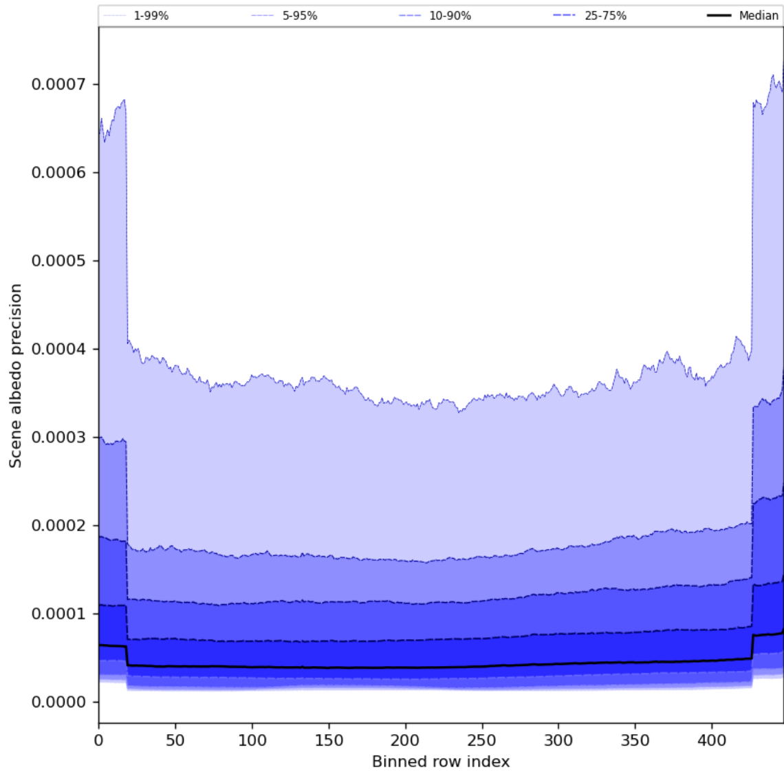
Figure 52: Along track statistics of “Scene albedo precision” for 2024-06-10 to 2024-06-12
