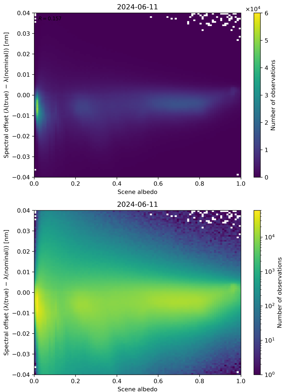
Figure 107: Scatter density plot of “Scene albedo” against “Spectral offset ( \lambda(\text{true}) - \lambda(\text{nominal}) )” for 2024-06-10 to 2024-06-12.
