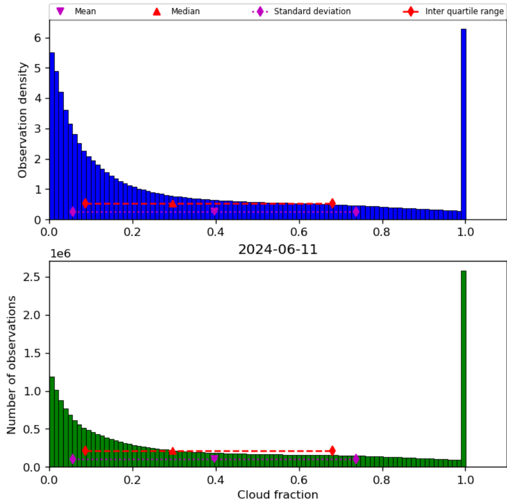
Figure 32: Histogram of “Cloud fraction” for 2024-06-10 to 2024-06-12
