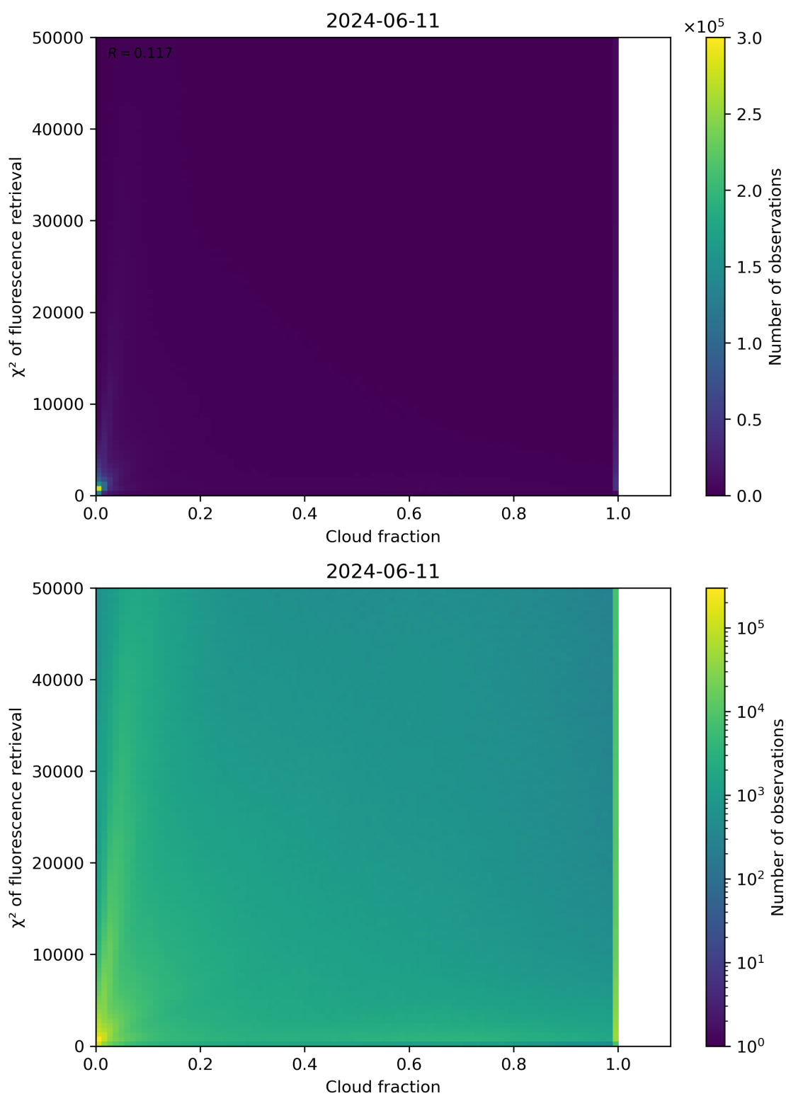
Figure 71: Scatter density plot of “Cloud fraction” against “ \chi^2 of fluorescence retrieval” for 2024-06-10 to 2024-06-12.
