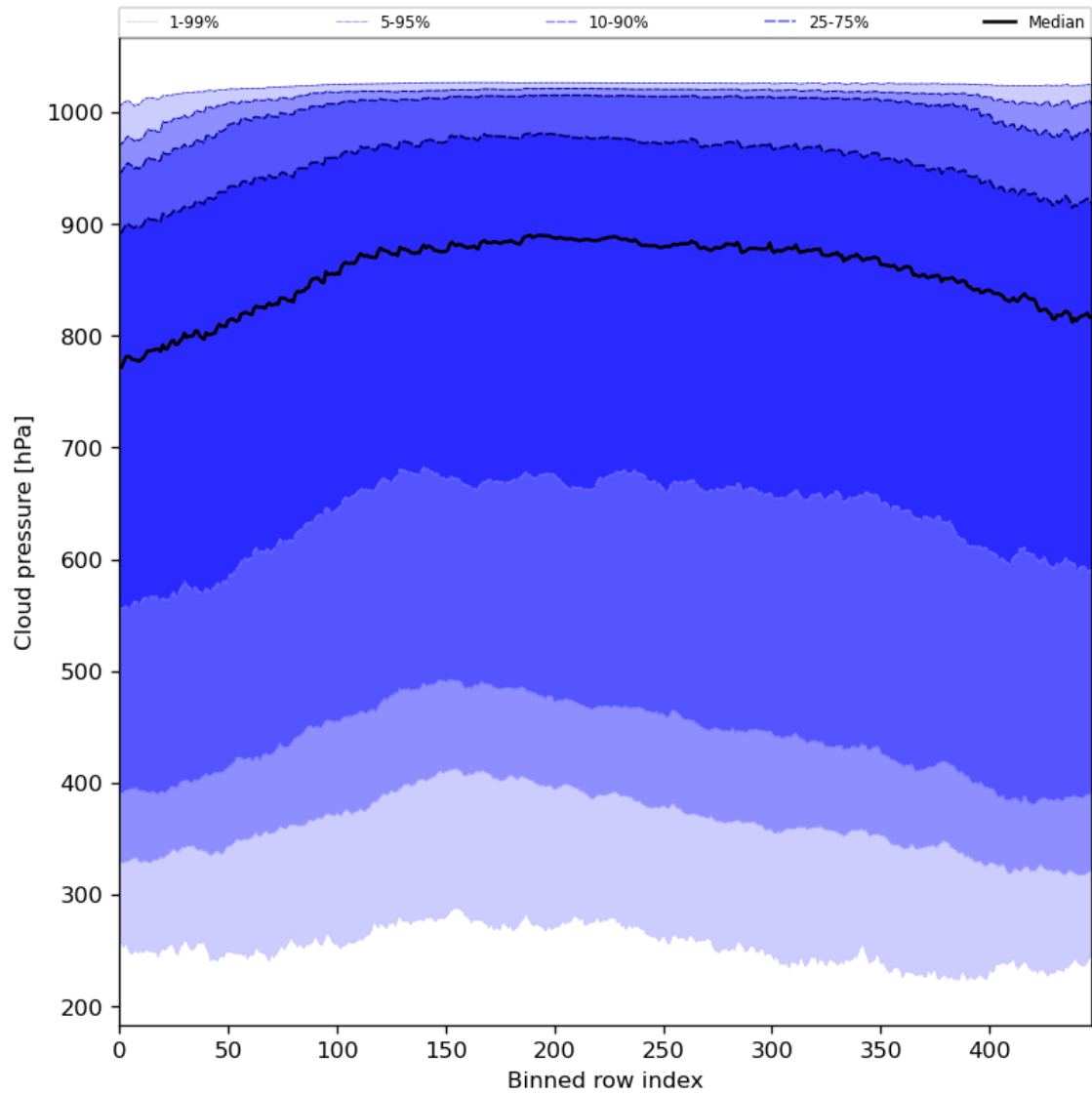
Figure 47: Along track statistics of “Cloud pressure” for 2024-06-10 to 2024-06-12
