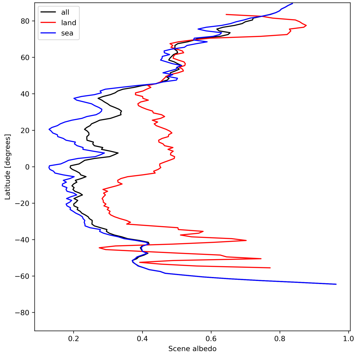
Figure 17: Zonal average of “Scene albedo” for 2024-06-10 to 2024-06-12.
