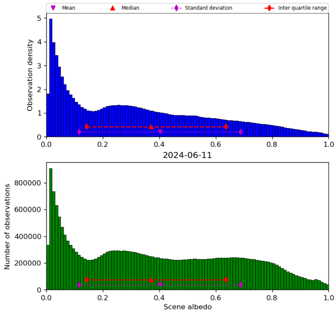
Figure 34: Histogram of “Scene albedo” for 2024-06-10 to 2024-06-12
