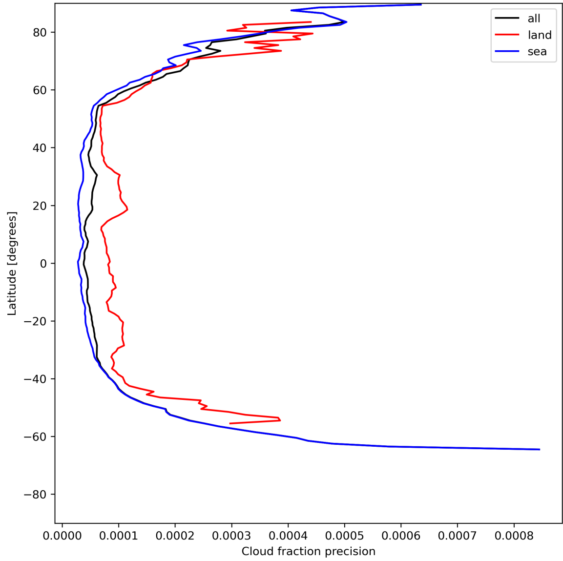
Figure 16: Zonal average of “Cloud fraction precision” for 2024-06-10 to 2024-06-12.
