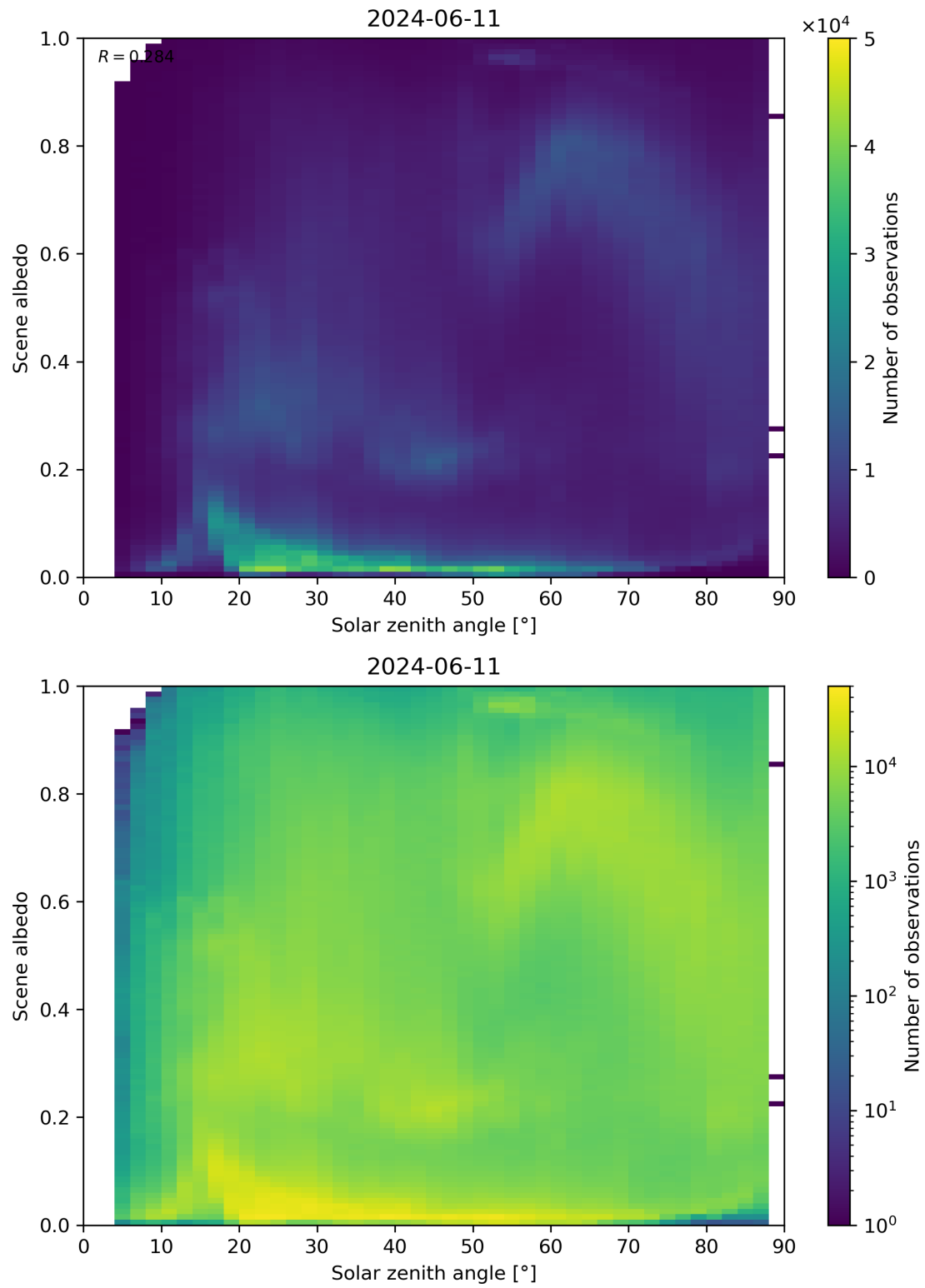
Figure 116: Scatter density plot of “Solar zenith angle” against “Scene albedo” for 2024-06-10 to 2024-06-12.
