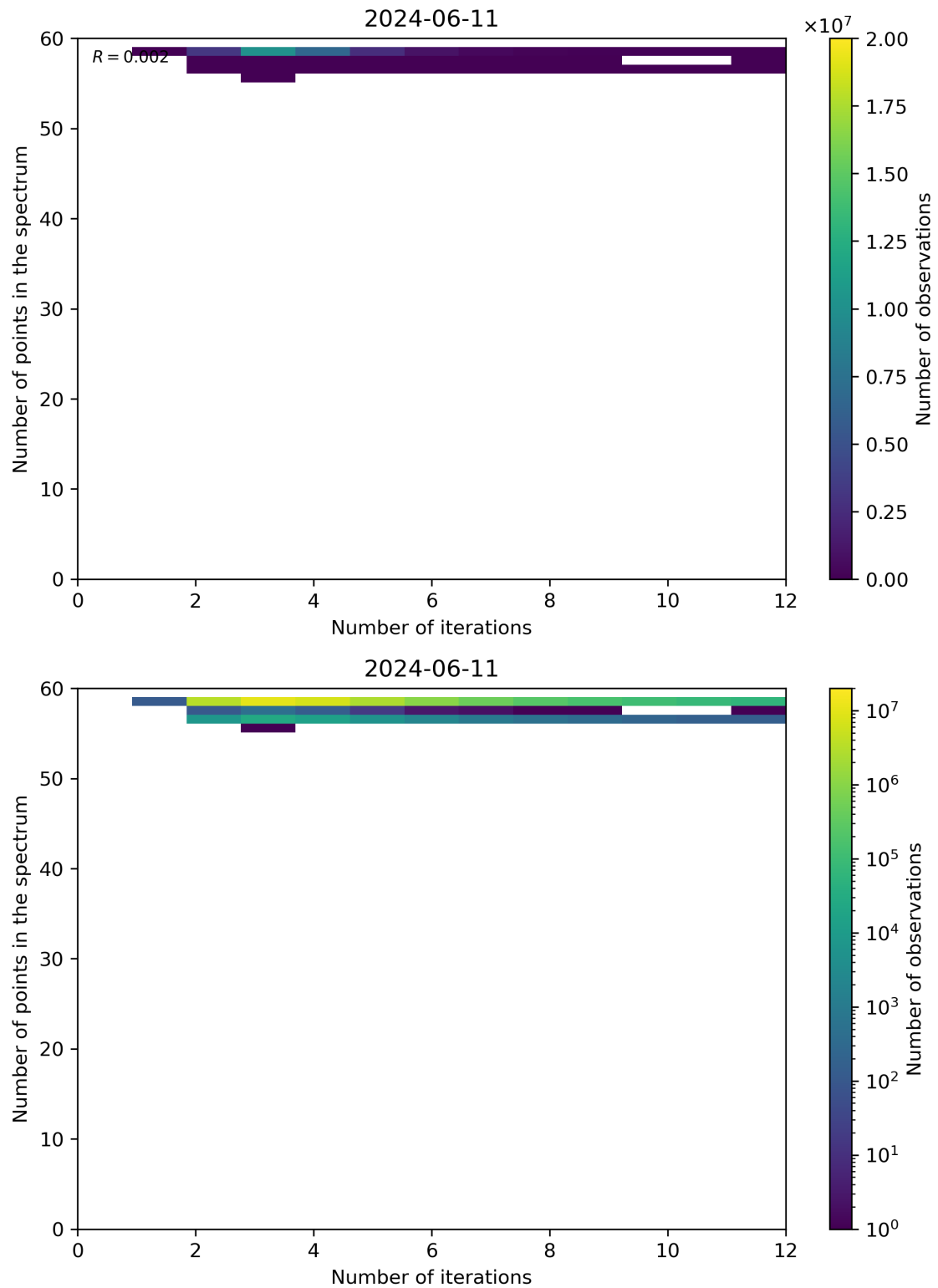
Figure 99: Scatter density plot of “Number of iterations” against “Number of points in the spectrum” for 2024-06-10 to 2024-06-12.
