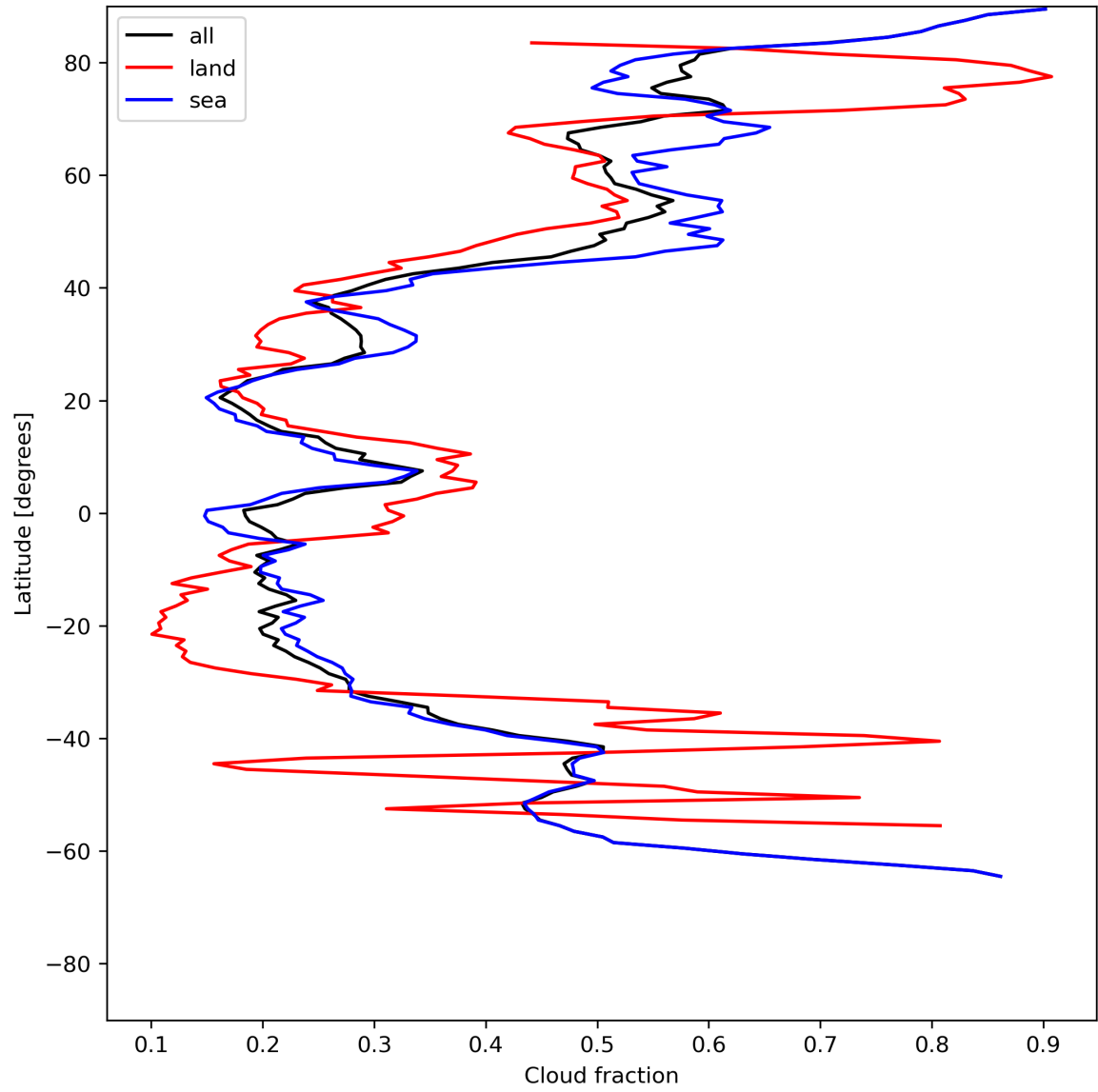
Figure 15: Zonal average of “Cloud fraction” for 2024-06-10 to 2024-06-12.
