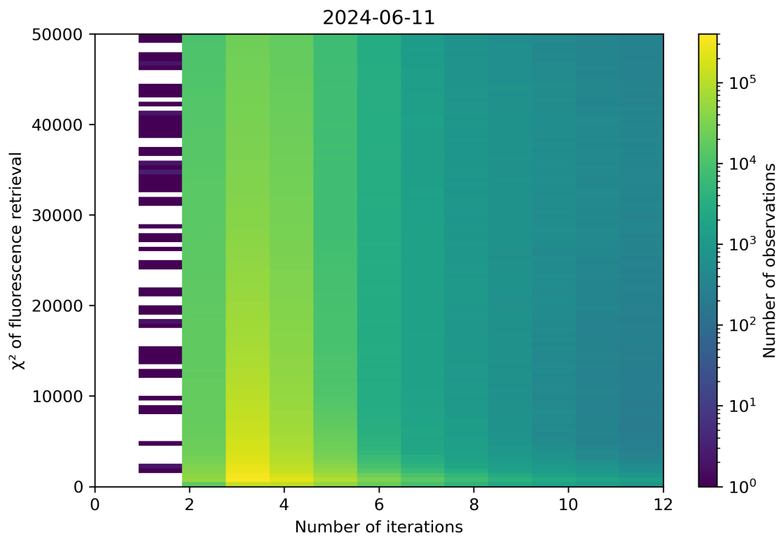
Figure 97: Scatter density plot of “Number of iterations” against “ \chi^2 of fluorescence retrieval” for 2024-06-10 to 2024-06-12.
