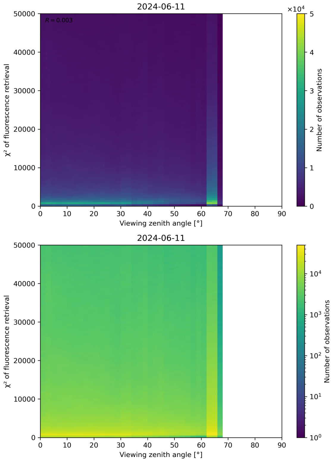
Figure 119: Scatter density plot of “Viewing zenith angle” against “ \chi^2 of fluorescence retrieval” for 2024-06-10 to 2024-06-12.
