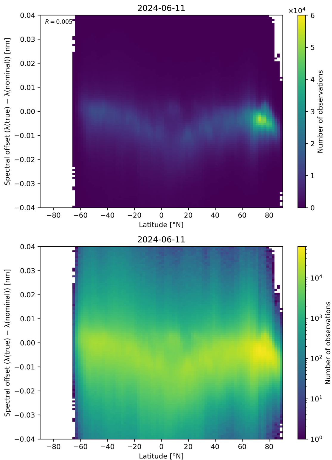
Figure 96: Scatter density plot of “Latitude” against “Spectral offset ( \lambda(\text{true}) - \lambda(\text{nominal}) )” for 2024-06-10 to 2024-06-12.
