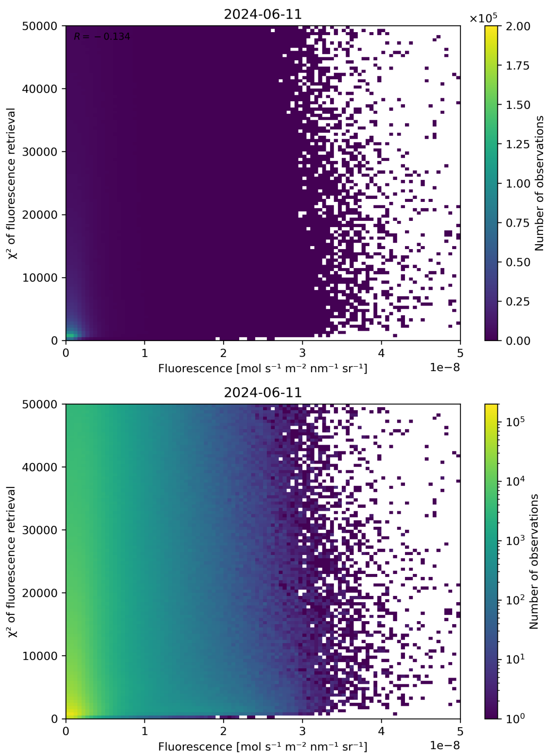
Figure 85: Scatter density plot of “Fluorescence” against “ \chi^2 of fluorescence retrieval” for 2024-06-10 to 2024-06-12.
