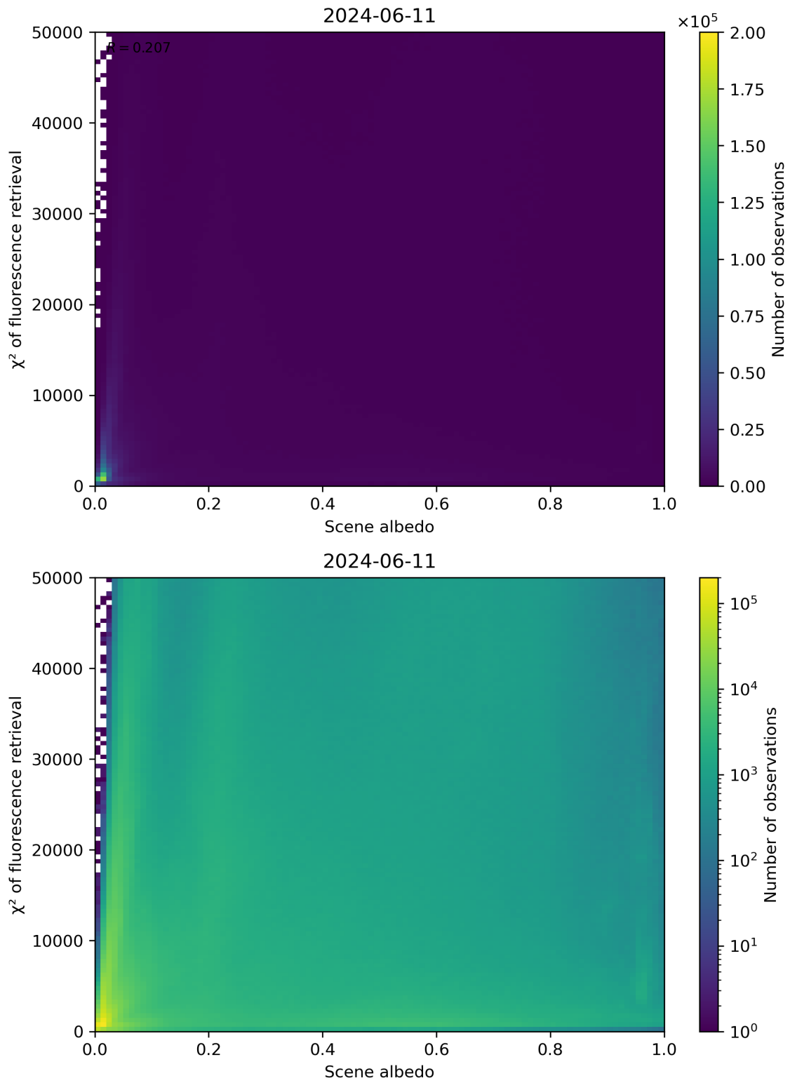
Figure 103: Scatter density plot of “Scene albedo” against “ \chi^2 of fluorescence retrieval” for 2024-06-10 to 2024-06-12.
