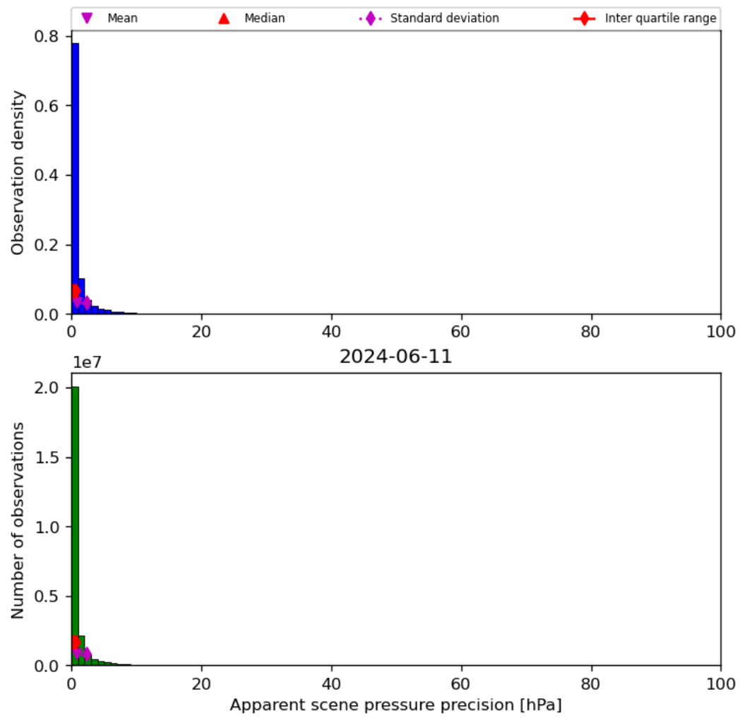
Figure 37: Histogram of “Apparent scene pressure precision” for 2024-06-10 to 2024-06-12
