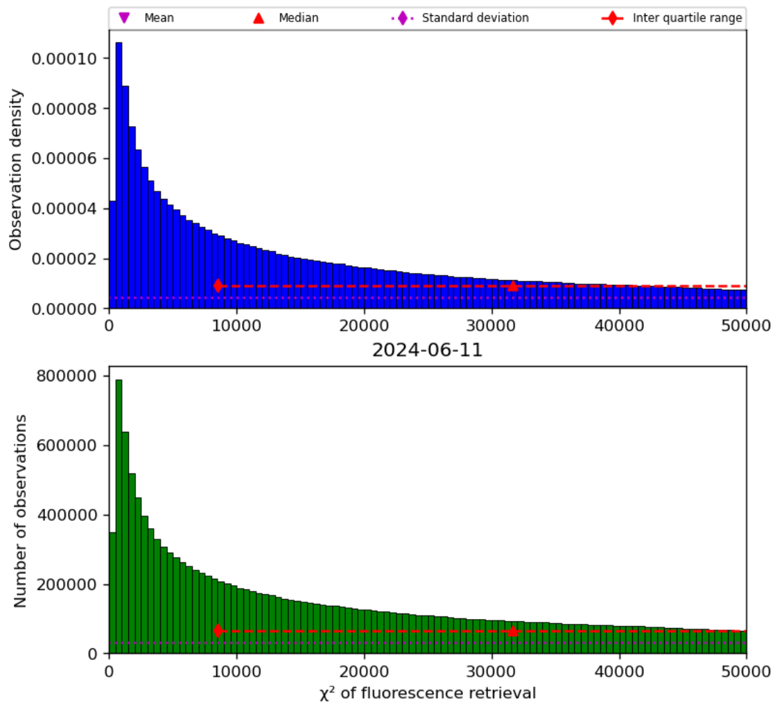
Figure 42: Histogram of “ \chi^2 of fluorescence retrieval” for 2024-06-10 to 2024-06-12
