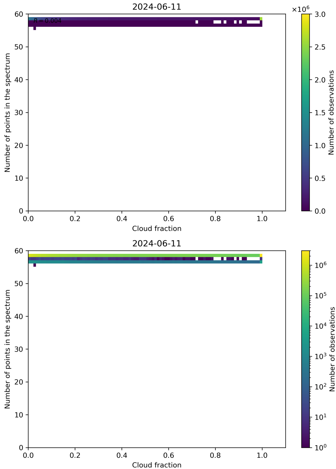
Figure 74: Scatter density plot of “Cloud fraction” against “Number of points in the spectrum” for 2024-06-10 to 2024-06-12.
