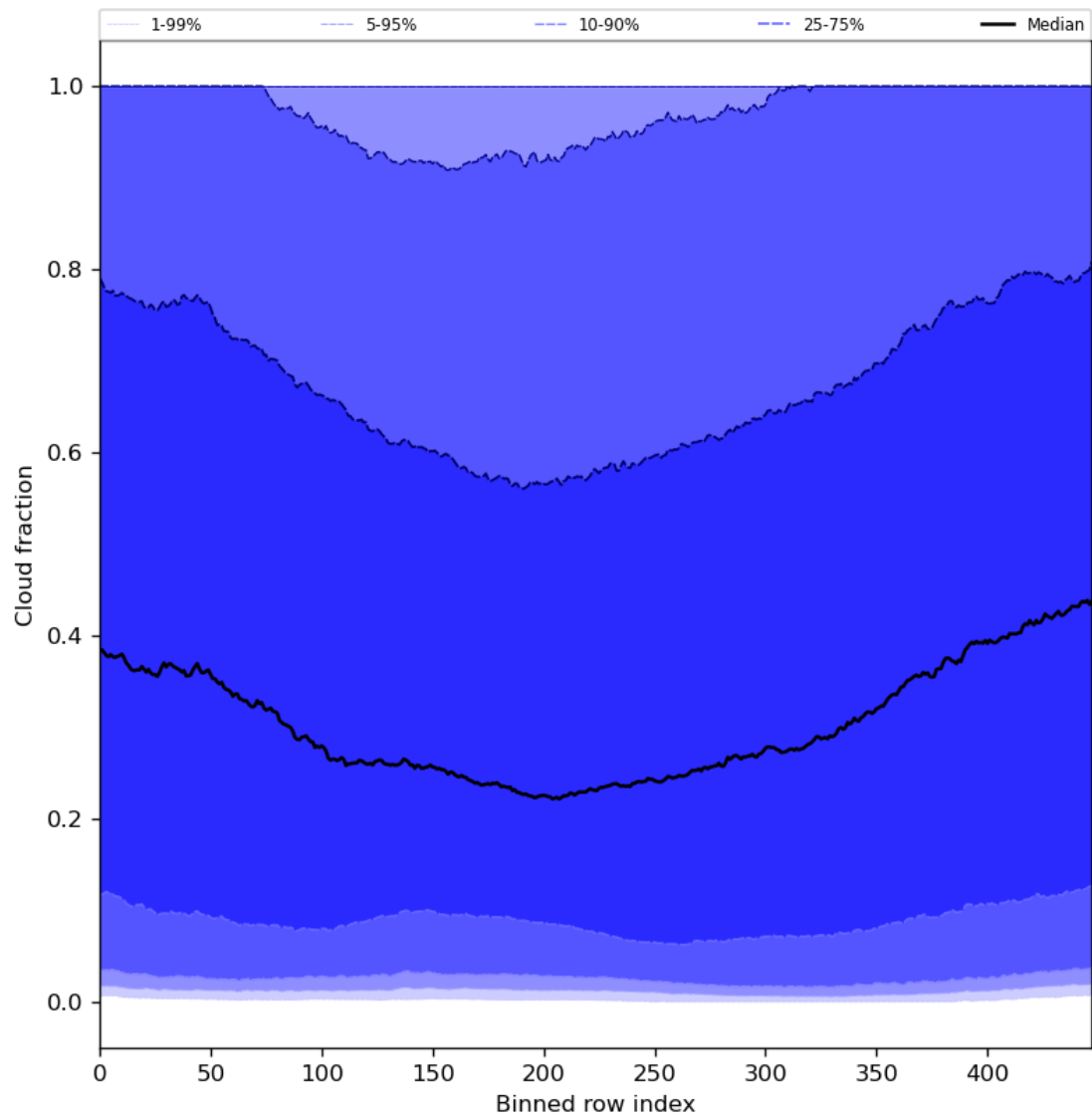
Figure 49: Along track statistics of “Cloud fraction” for 2024-06-10 to 2024-06-12
