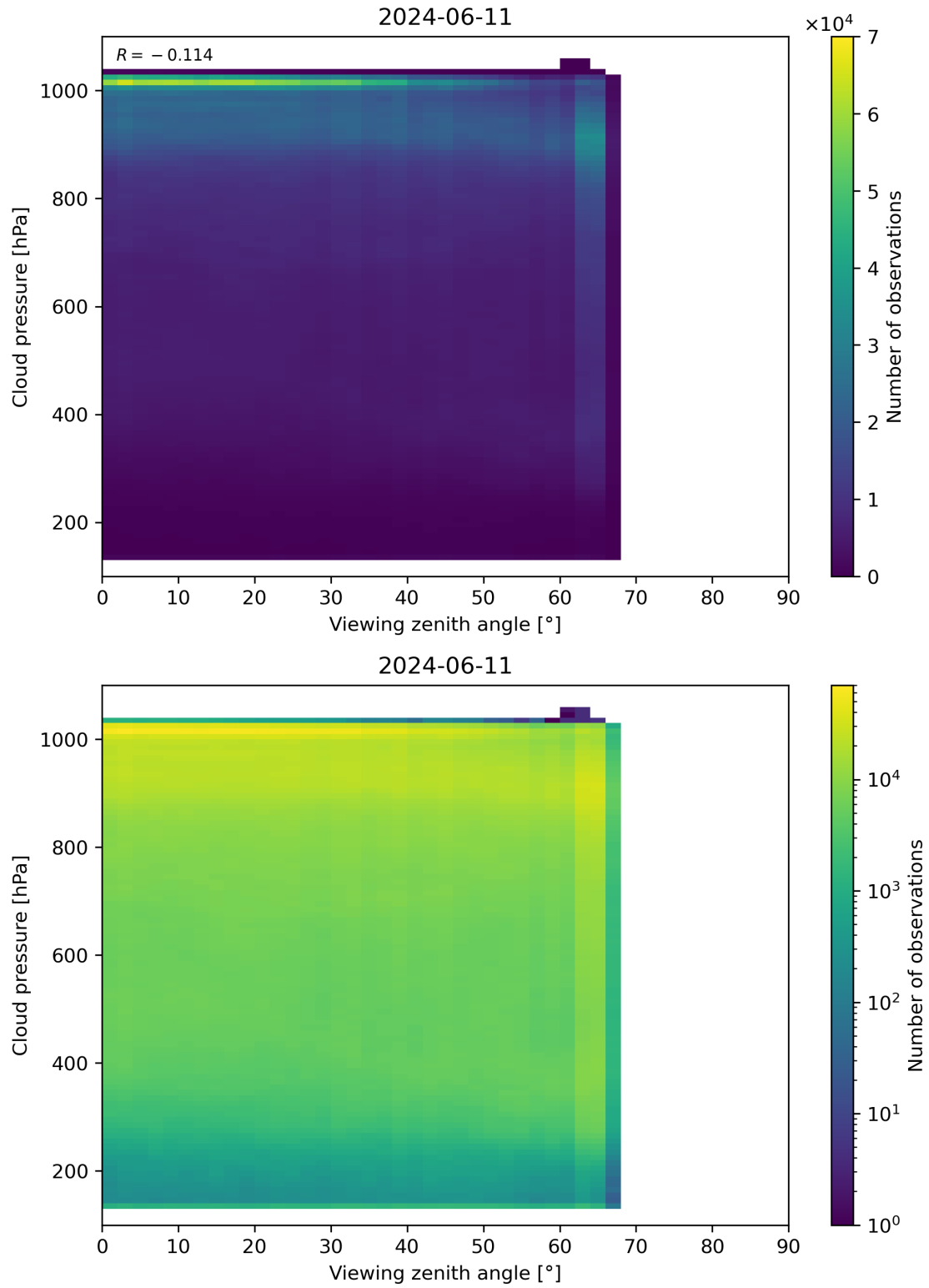
Figure 121: Scatter density plot of “Viewing zenith angle” against “Cloud pressure” for 2024-06-10 to 2024-06-12.
