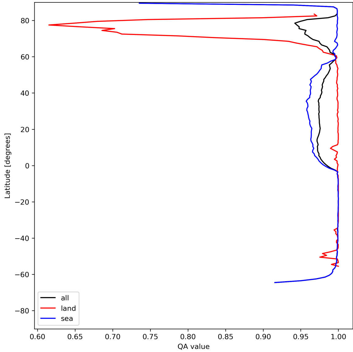
Figure 12: Zonal average of “QA value” for 2024-06-10 to 2024-06-12.
