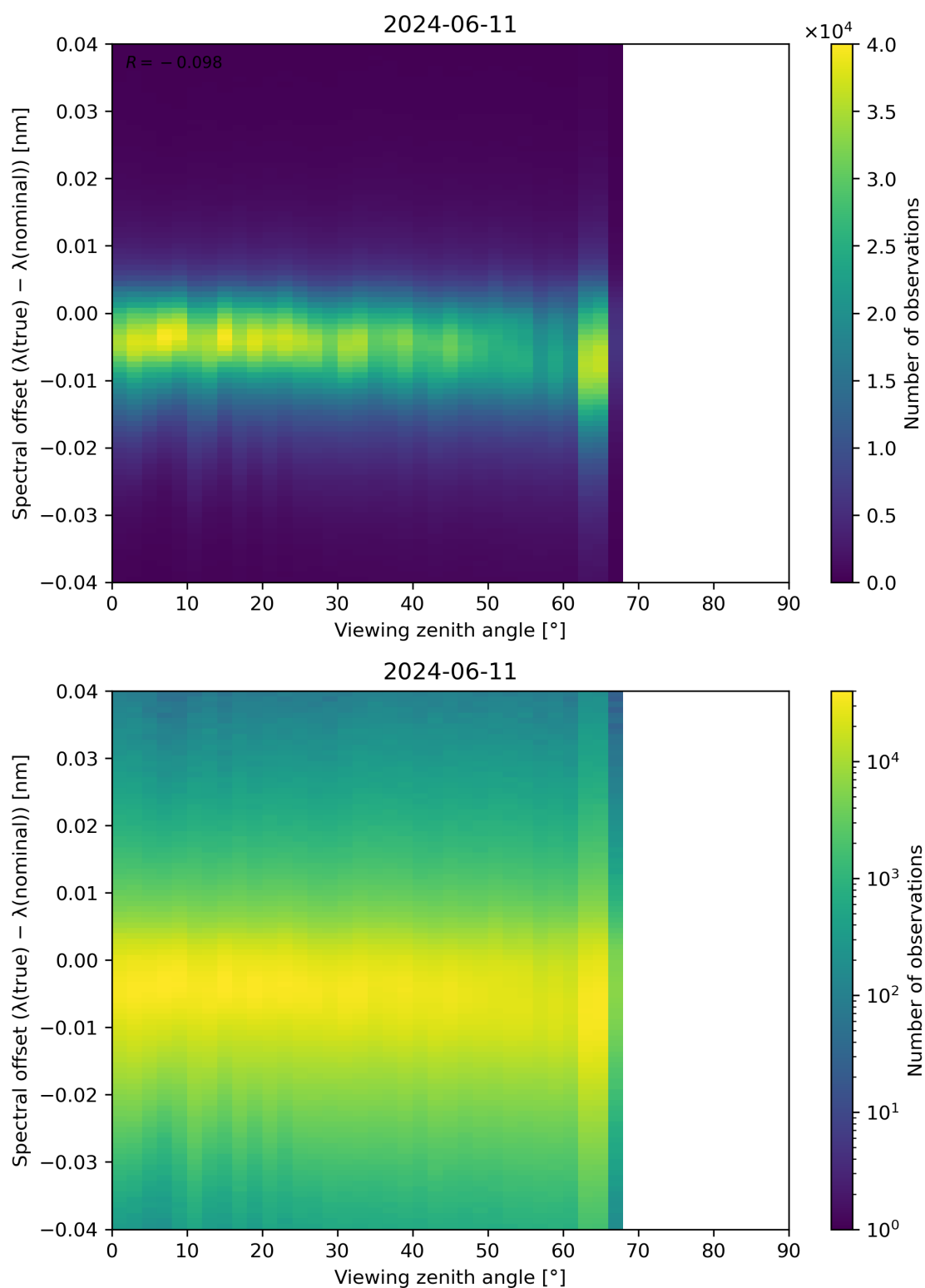
Figure 128: Scatter density plot of “Viewing zenith angle” against “Spectral offset ( \lambda(\text{true}) - \lambda(\text{nominal}) )” for 2024-06-10 to 2024-06-12.
