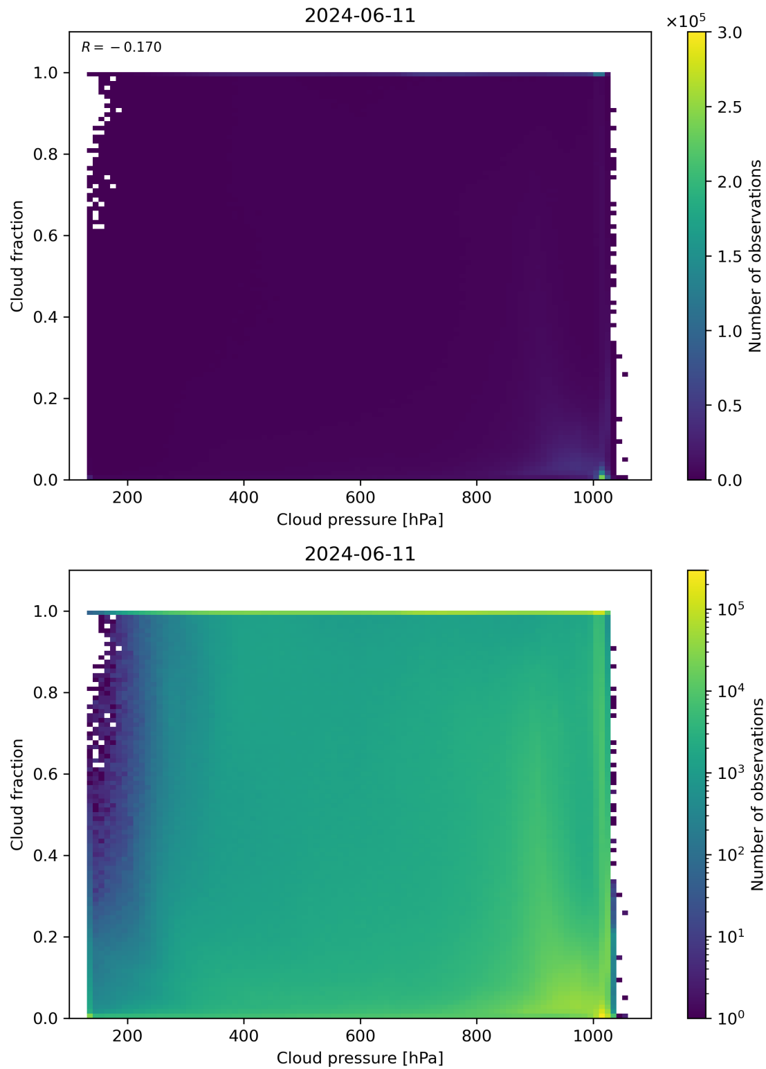
Figure 79: Scatter density plot of “Cloud pressure” against “Cloud fraction” for 2024-06-10 to 2024-06-12.
