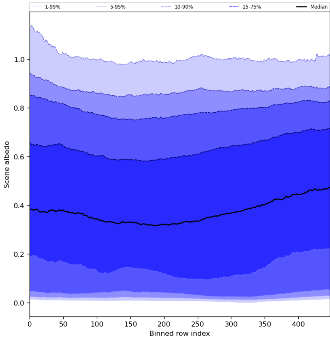
Figure 51: Along track statistics of “Scene albedo” for 2024-06-10 to 2024-06-12
