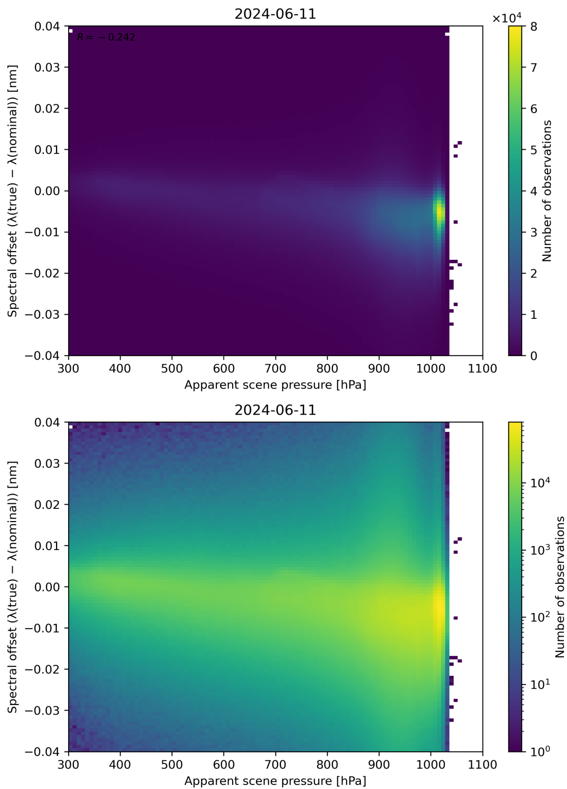
Figure 67: Scatter density plot of “Apparent scene pressure” against “Spectral offset ( \lambda(\text{true}) - \lambda(\text{nominal}) )” for 2024-06-10 to 2024-06-12.
