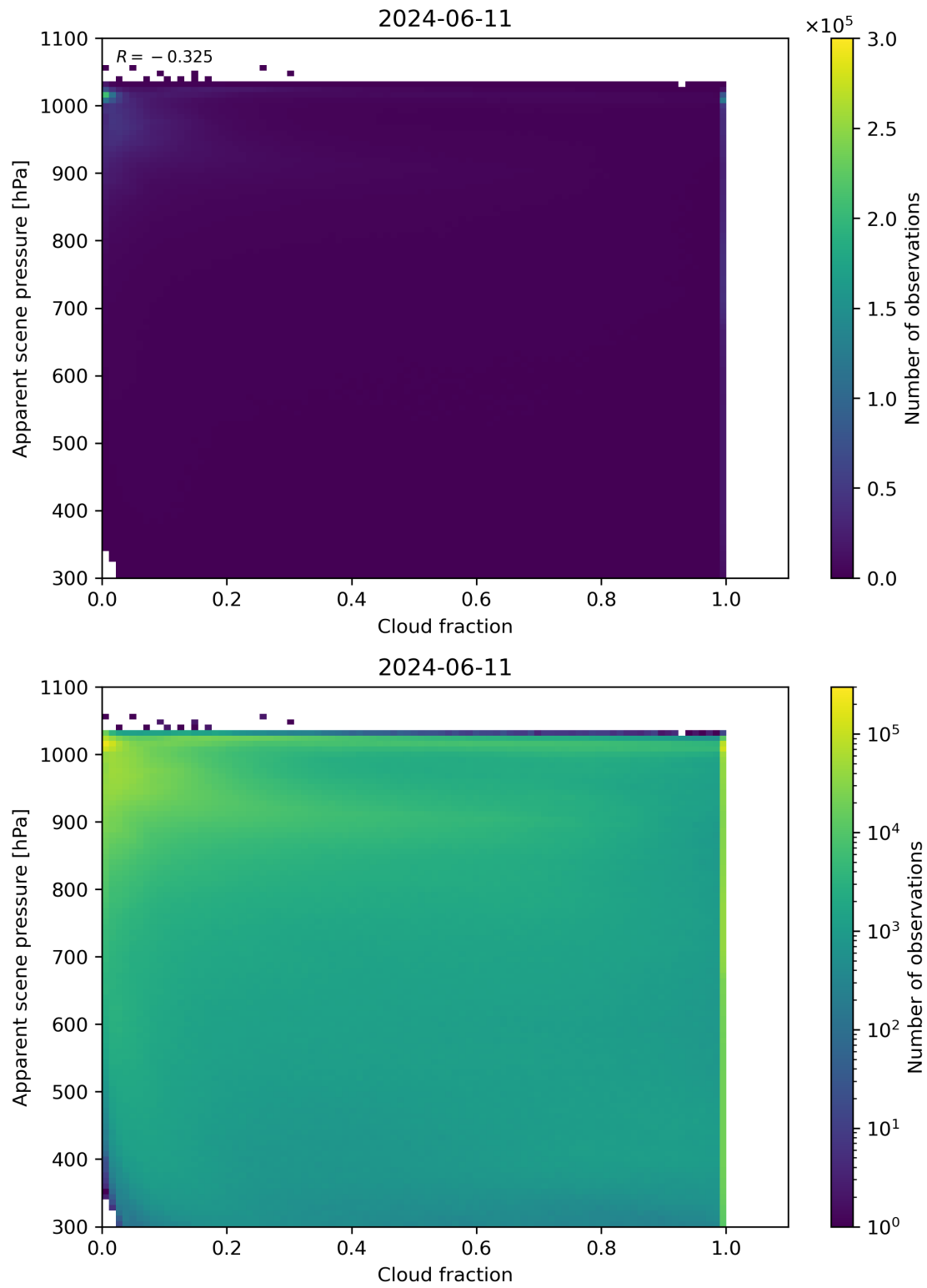
Figure 70: Scatter density plot of “Cloud fraction” against “Apparent scene pressure” for 2024-06-10 to 2024-06-12.
