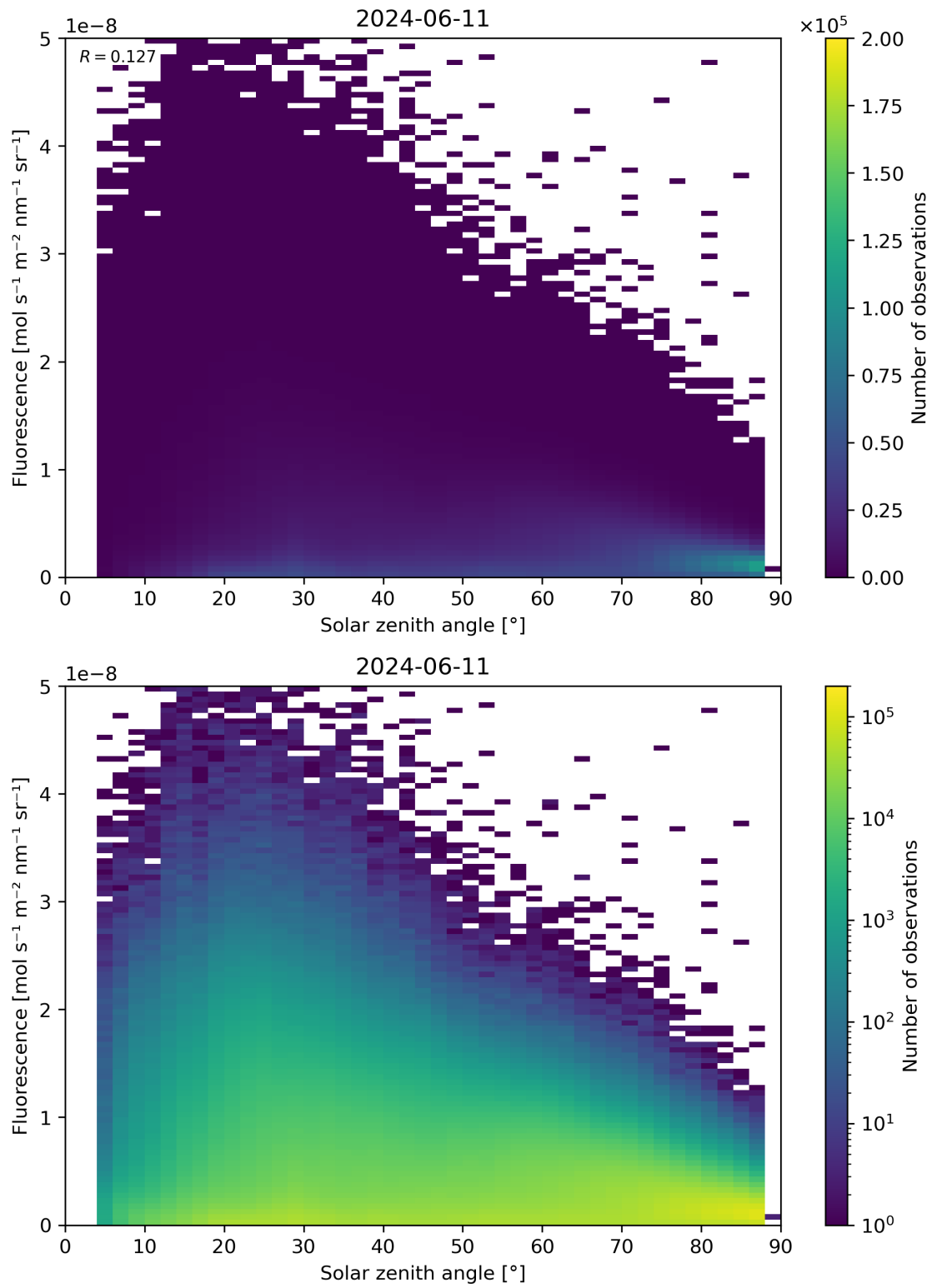
Figure 112: Scatter density plot of “Solar zenith angle” against “Fluorescence” for 2024-06-10 to 2024-06-12.
