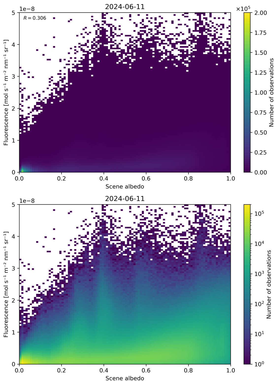
Figure 104: Scatter density plot of “Scene albedo” against “Fluorescence” for 2024-06-10 to 2024-06-12.
