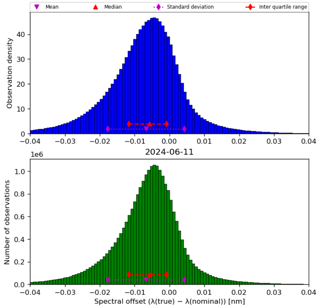
Figure 45: Histogram of “Spectral offset ( \lambda(\text{true}) - \lambda(\text{nominal}) )” for 2024-06-10 to 2024-06-12
