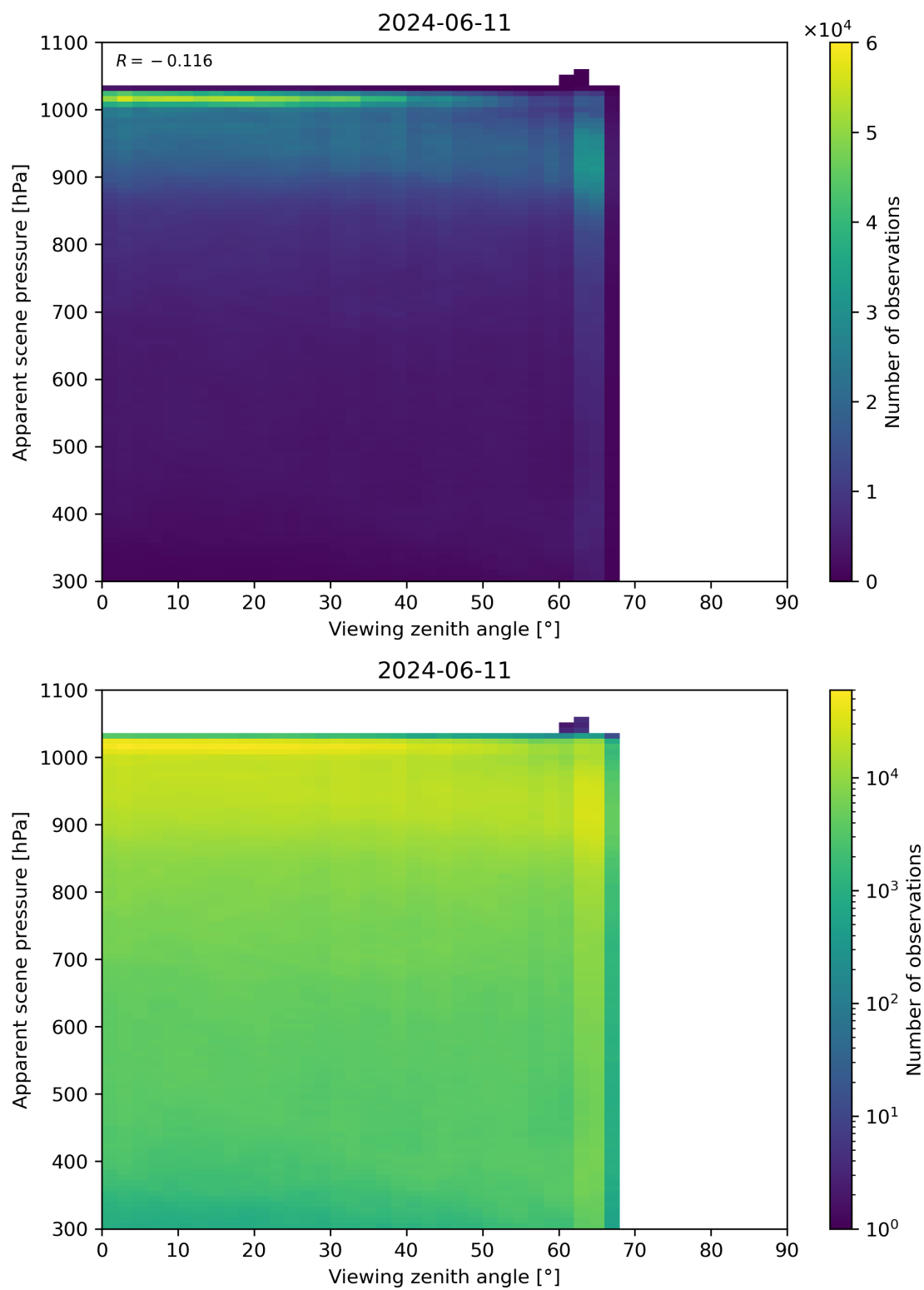
Figure 118: Scatter density plot of “Viewing zenith angle” against “Apparent scene pressure” for 2024-06-10 to 2024-06-12.
