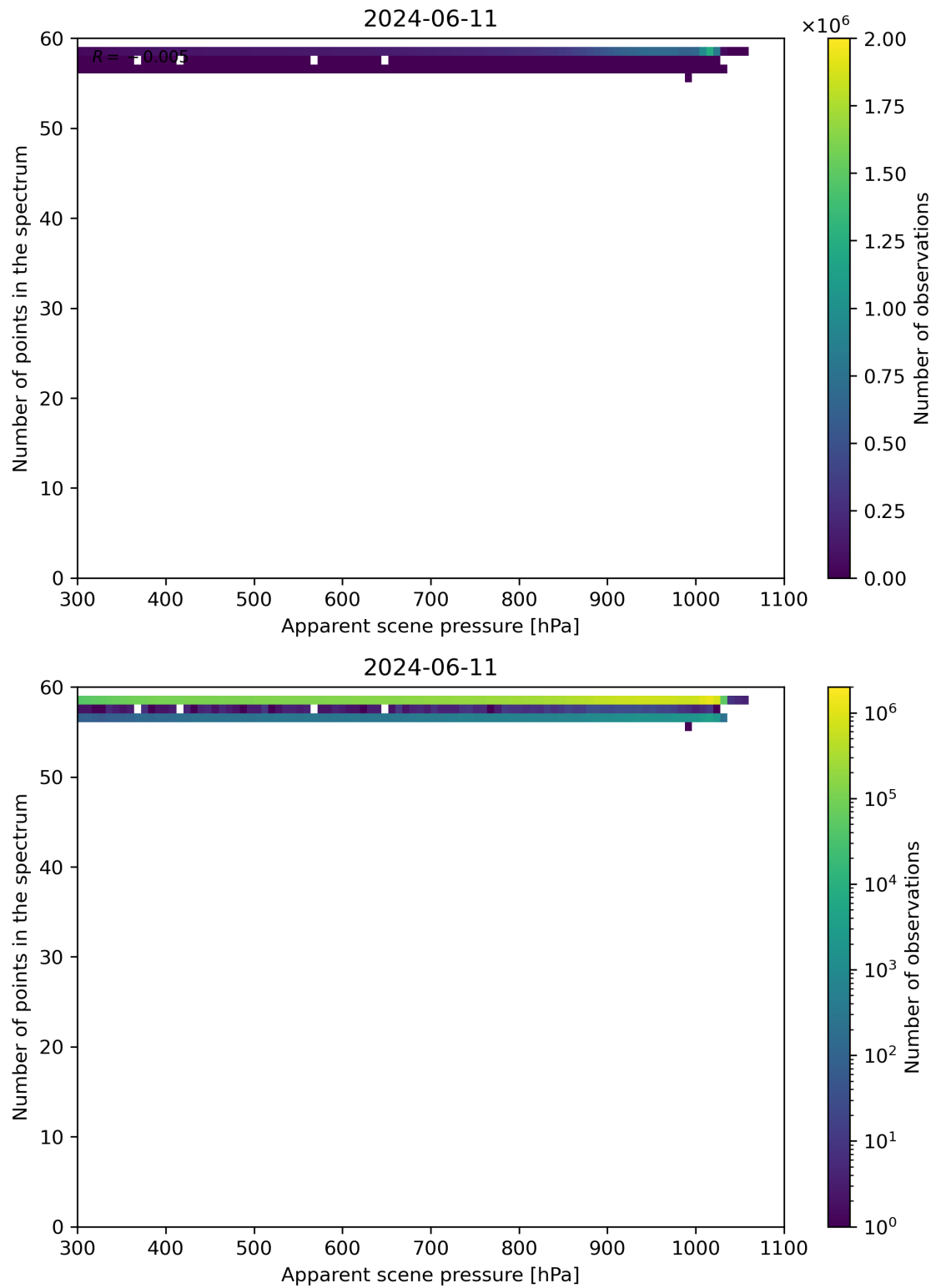
Figure 66: Scatter density plot of “Apparent scene pressure” against “Number of points in the spectrum” for 2024-06-10 to 2024-06-12.
