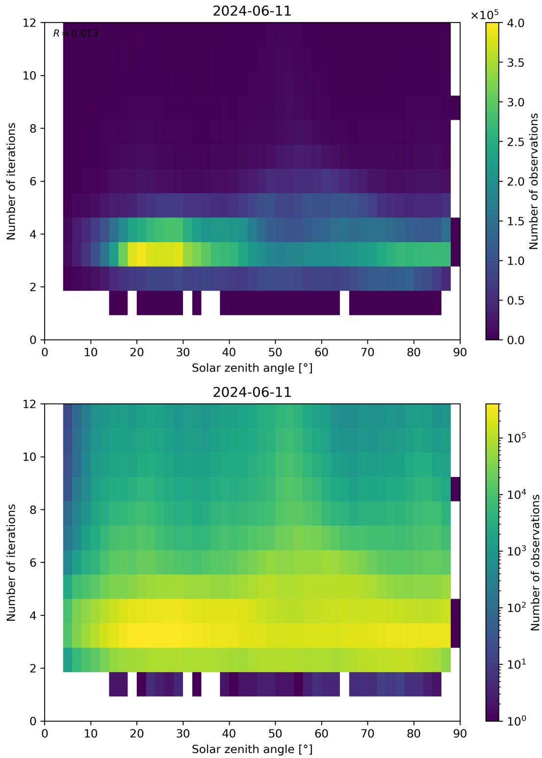
Figure 114: Scatter density plot of “Solar zenith angle” against “Number of iterations” for 2024-06-10 to 2024-06-12.
