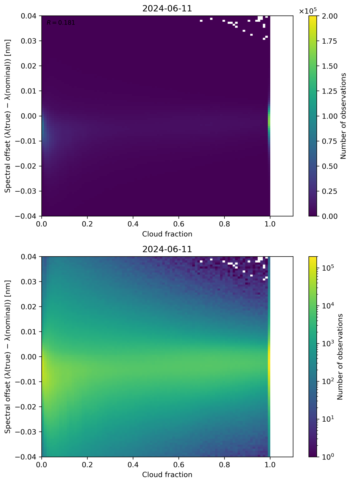
Figure 76: Scatter density plot of “Cloud fraction” against “Spectral offset ( \lambda(\text{true}) - \lambda(\text{nominal}) )” for 2024-06-10 to 2024-06-12.
