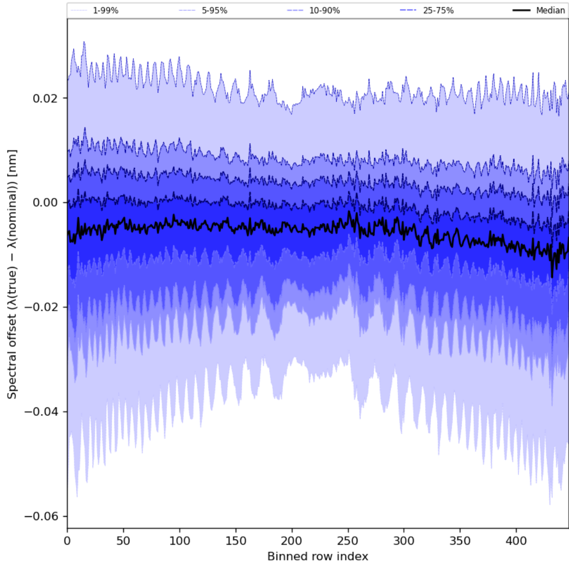
Figure 62: Along track statistics of “Spectral offset ( \lambda(\text{true}) - \lambda(\text{nominal}) )” for 2024-06-10 to 2024-06-12
