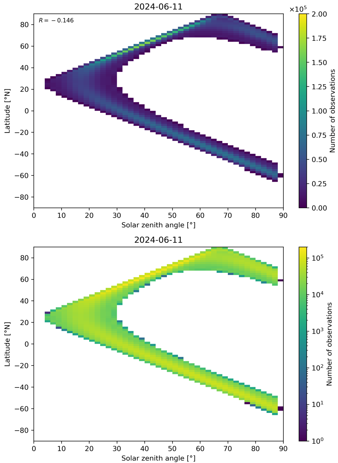
Figure 113: Scatter density plot of “Solar zenith angle” against “Latitude” for 2024-06-10 to 2024-06-12.
