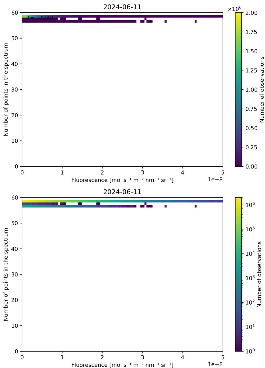
Figure 86: Scatter density plot of “Fluorescence” against “Number of points in the spectrum” for 2024-06-10 to 2024-06-12.
