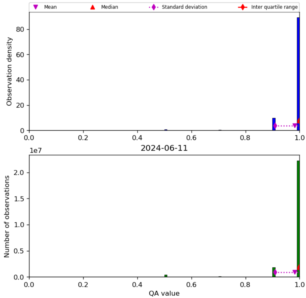
Figure 29: Histogram of “QA value” for 2024-06-10 to 2024-06-12
