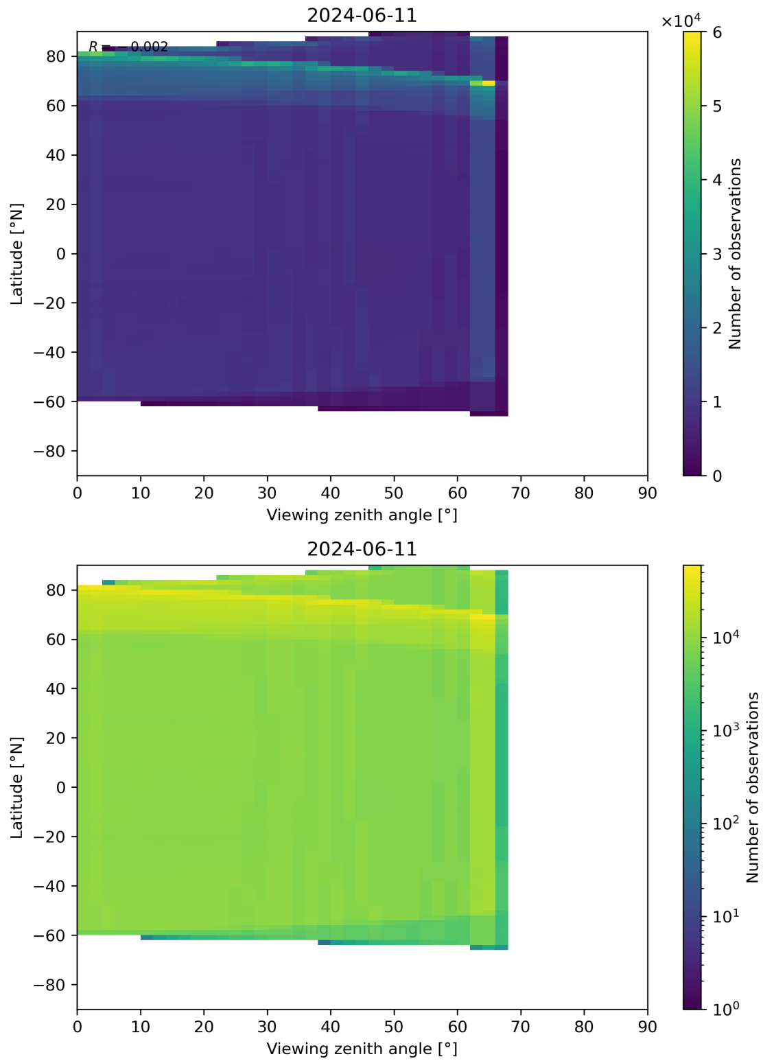
Figure 123: Scatter density plot of “Viewing zenith angle” against “Latitude” for 2024-06-10 to 2024-06-12.
