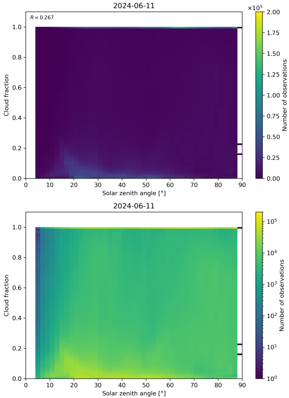
Figure 110: Scatter density plot of “Solar zenith angle” against “Cloud fraction” for 2024-06-10 to 2024-06-12.
