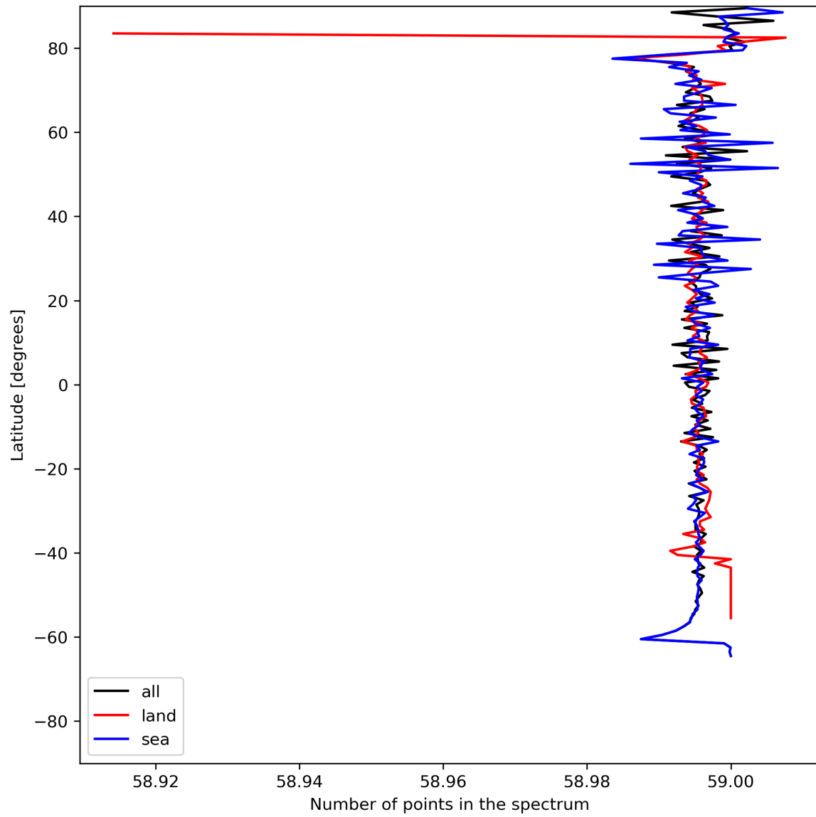
Figure 27: Zonal average of “Number of points in the spectrum” for 2024-06-10 to 2024-06-12.
