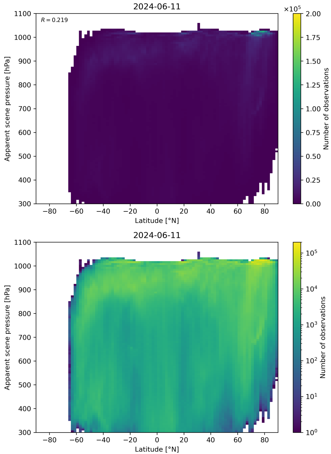
Figure 88: Scatter density plot of “Latitude” against “Apparent scene pressure” for 2024-06-10 to 2024-06-12.
