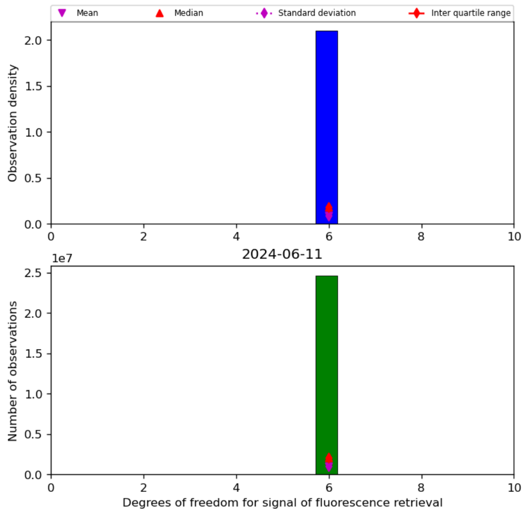
Figure 43: Histogram of “Degrees of freedom for signal of fluorescence retrieval” for 2024-06-10 to 2024-06-12
