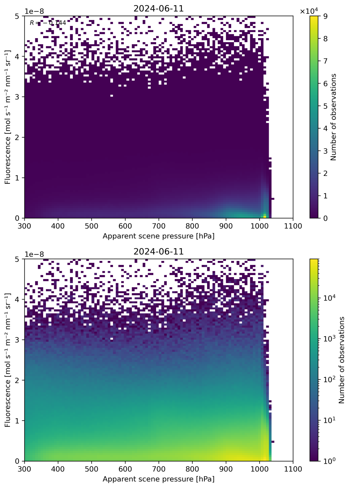
Figure 64: Scatter density plot of “Apparent scene pressure” against “Fluorescence” for 2024-06-10 to 2024-06-12.
