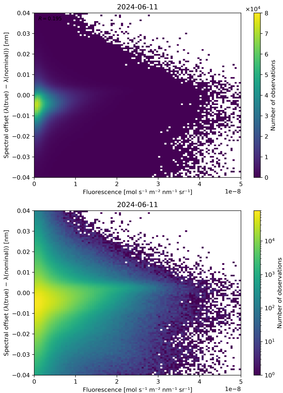
Figure 87: Scatter density plot of “Fluorescence” against “Spectral offset ( \lambda(\text{true}) - \lambda(\text{nominal}) )” for 2024-06-10 to 2024-06-12.
