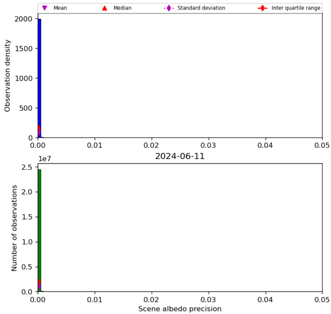
Figure 35: Histogram of “Scene albedo precision” for 2024-06-10 to 2024-06-12
