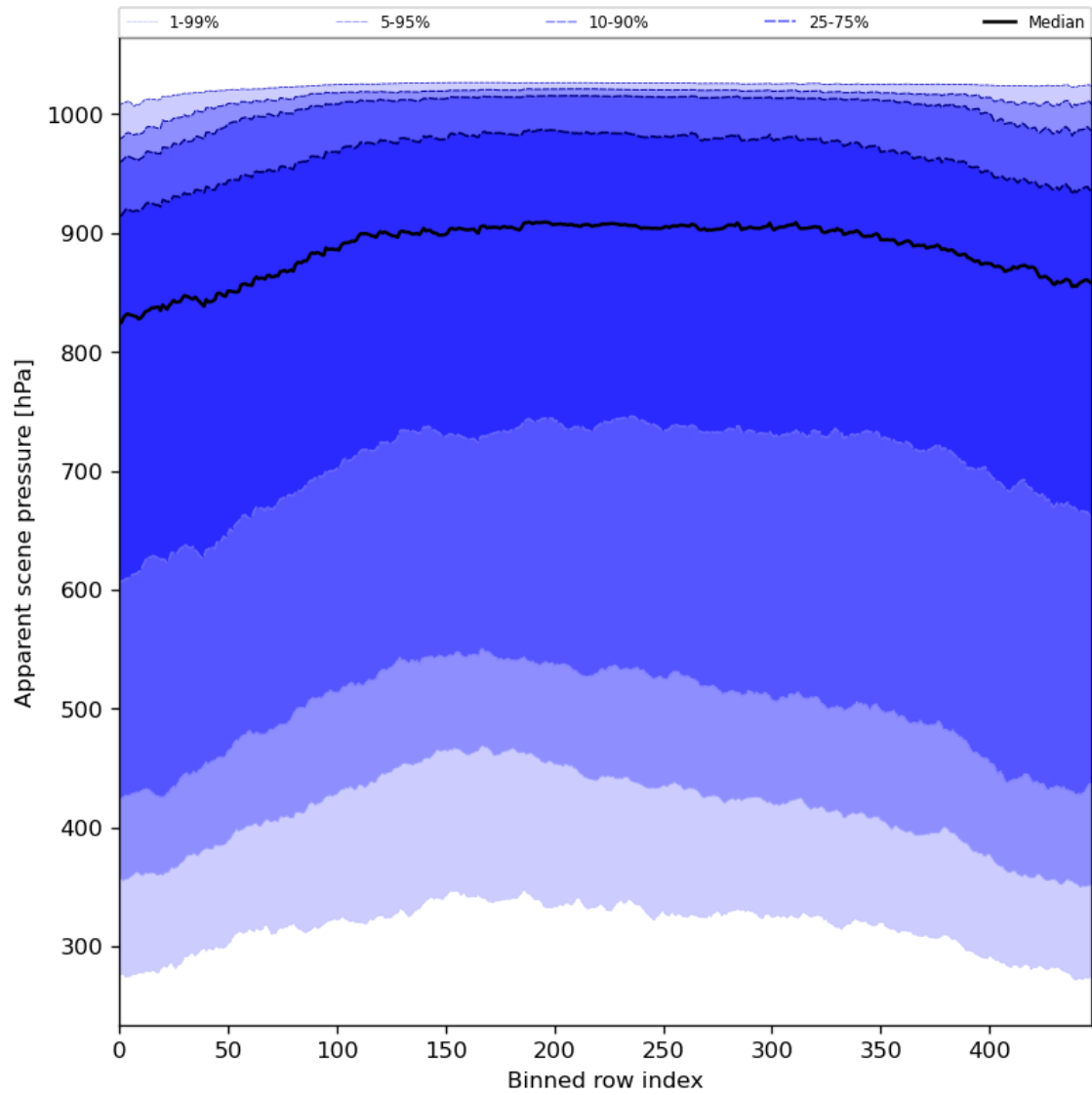
Figure 53: Along track statistics of “Apparent scene pressure” for 2024-06-10 to 2024-06-12
