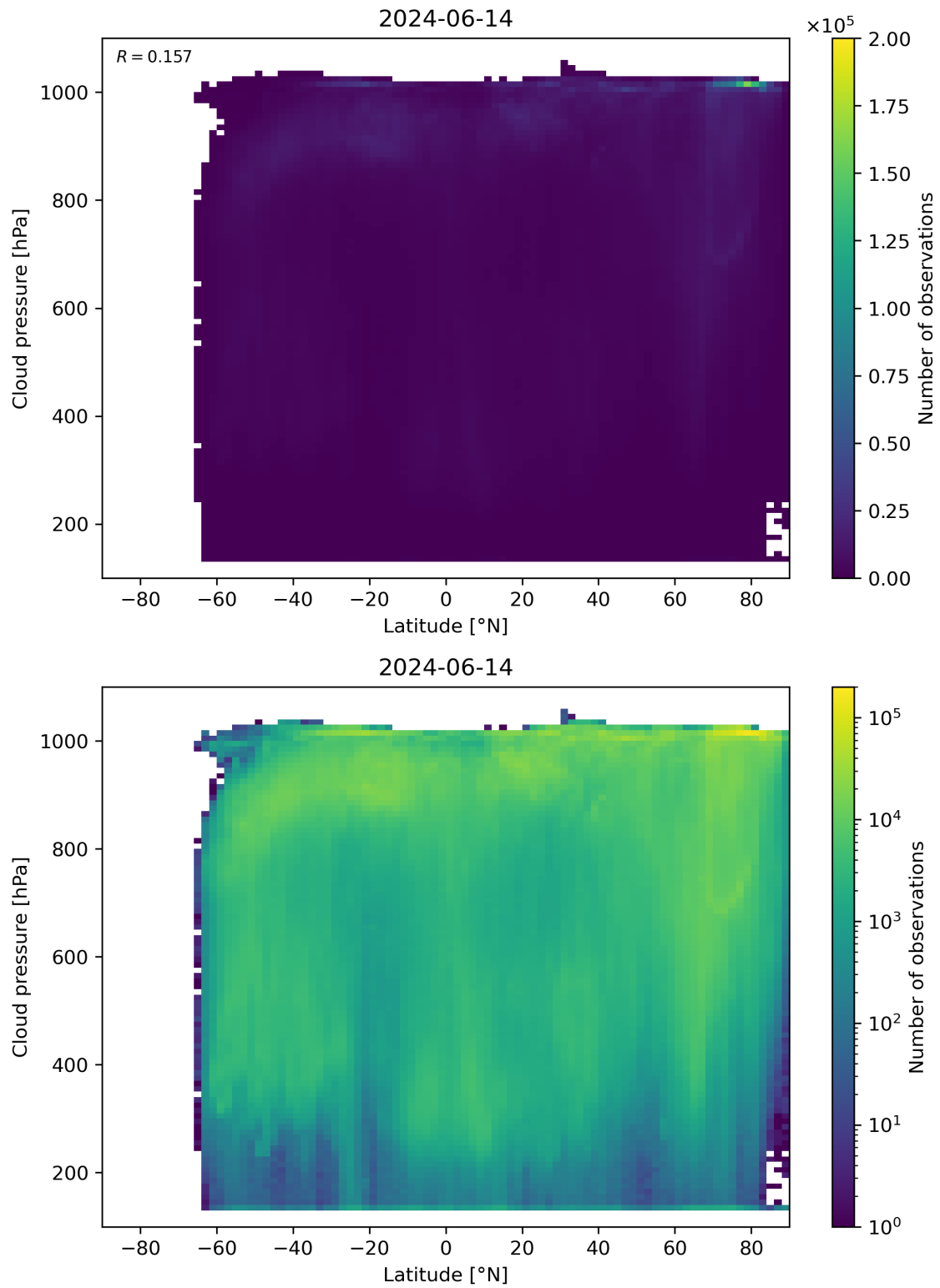
Figure 91: Scatter density plot of “Latitude” against “Cloud pressure” for 2024-06-13 to 2024-06-15.
