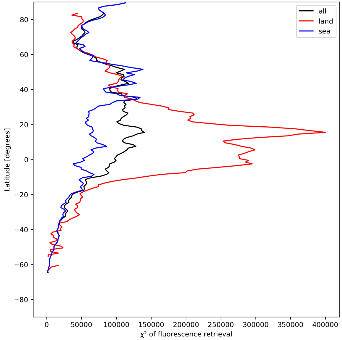
Figure 25: Zonal average of “ \chi^2 of fluorescence retrieval” for 2024-06-13 to 2024-06-15.
