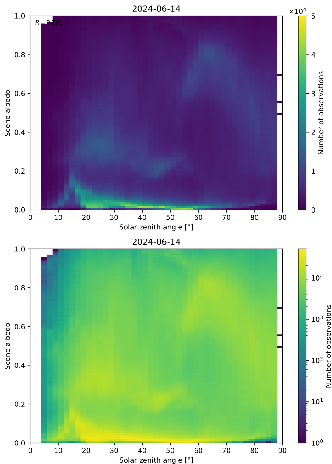
Figure 116: Scatter density plot of “Solar zenith angle” against “Scene albedo” for 2024-06-13 to 2024-06-15.
