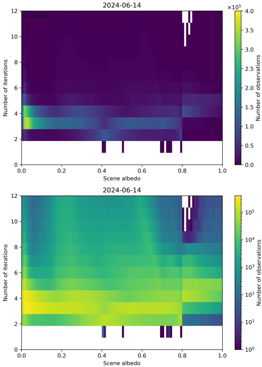
Figure 105: Scatter density plot of “Scene albedo” against “Number of iterations” for 2024-06-13 to 2024-06-15.
