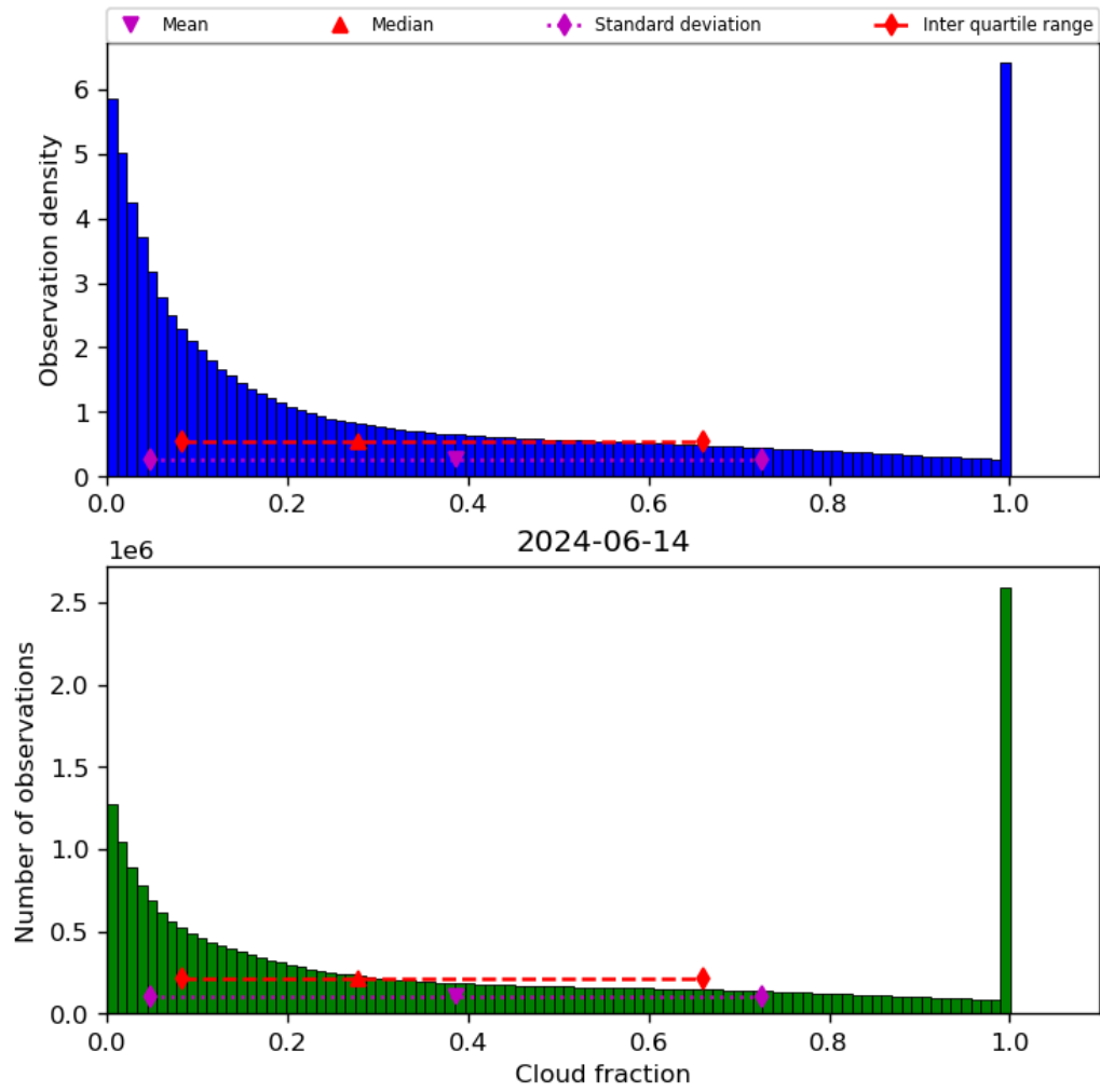
Figure 32: Histogram of “Cloud fraction” for 2024-06-13 to 2024-06-15
