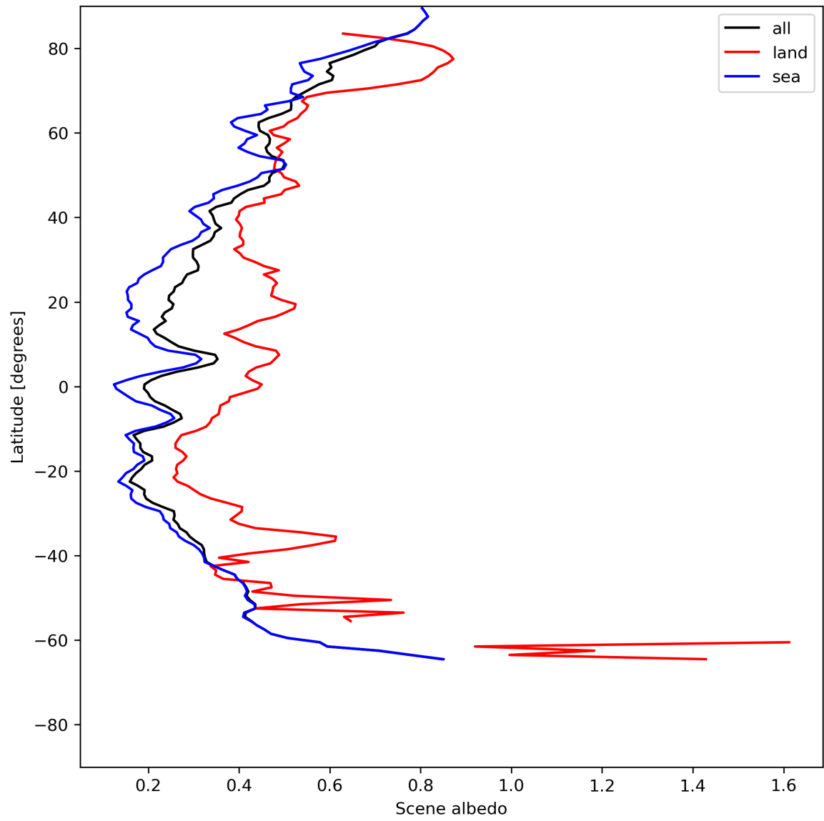
Figure 17: Zonal average of “Scene albedo” for 2024-06-13 to 2024-06-15.
