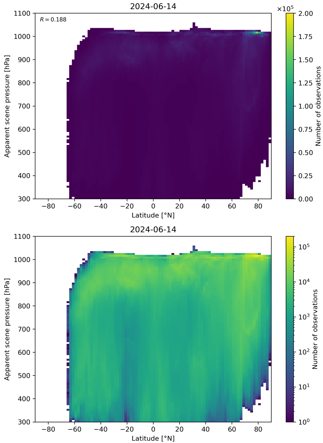
Figure 88: Scatter density plot of “Latitude” against “Apparent scene pressure” for 2024-06-13 to 2024-06-15.
