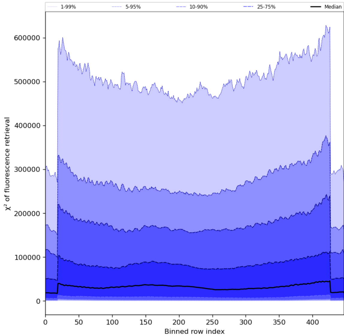
Figure 59: Along track statistics of “ \chi^2 of fluorescence retrieval” for 2024-06-13 to 2024-06-15
