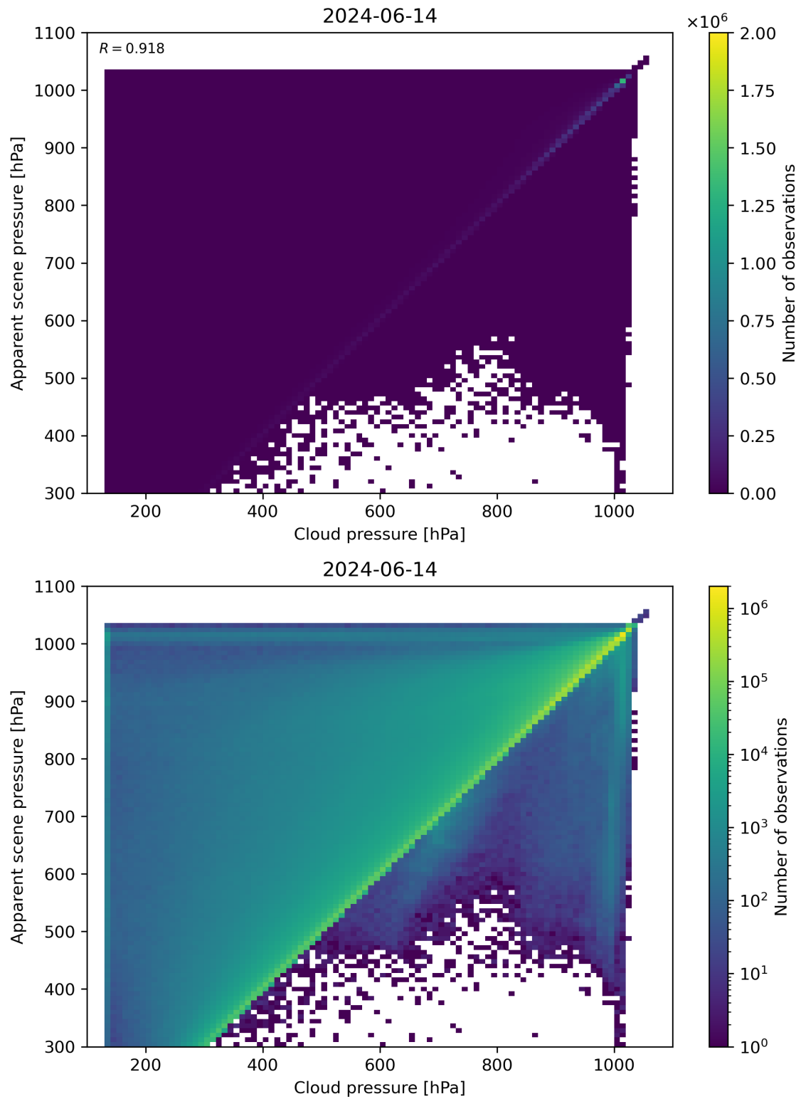
Figure 77: Scatter density plot of “Cloud pressure” against “Apparent scene pressure” for 2024-06-13 to 2024-06-15.
