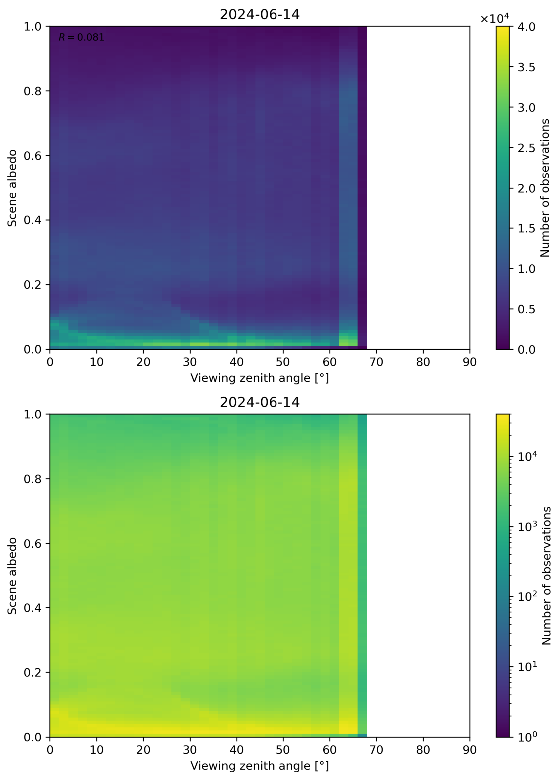
Figure 126: Scatter density plot of “Viewing zenith angle” against “Scene albedo” for 2024-06-13 to 2024-06-15.
