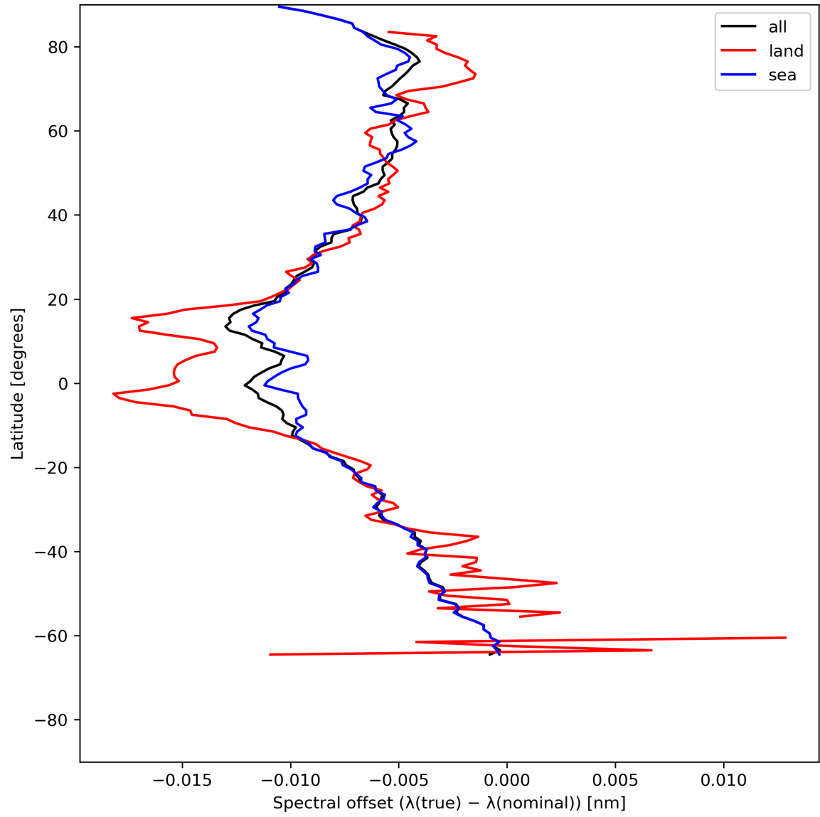
Figure 28: Zonal average of “Spectral offset ( \lambda(\text{true}) - \lambda(\text{nominal}) )” for 2024-06-13 to 2024-06-15.
