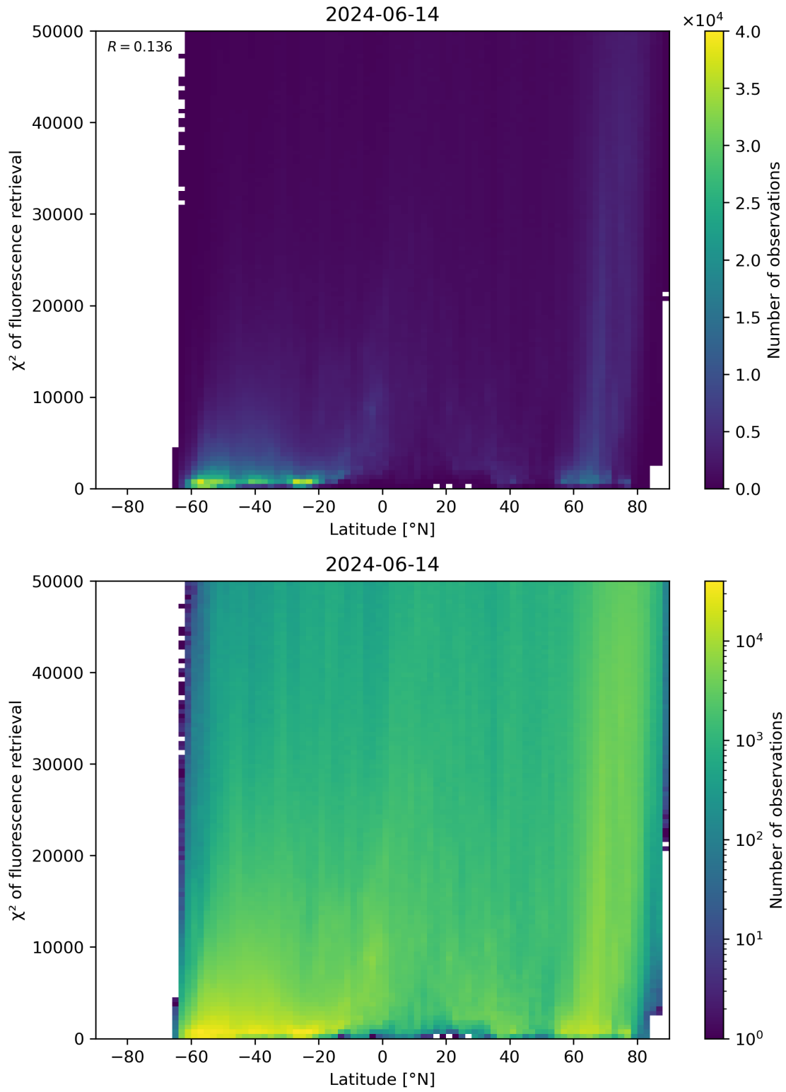
Figure 89: Scatter density plot of “Latitude” against “ \chi^2 of fluorescence retrieval” for 2024-06-13 to 2024-06-15.
