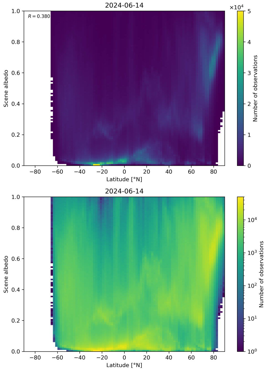
Figure 95: Scatter density plot of “Latitude” against “Scene albedo” for 2024-06-13 to 2024-06-15.
