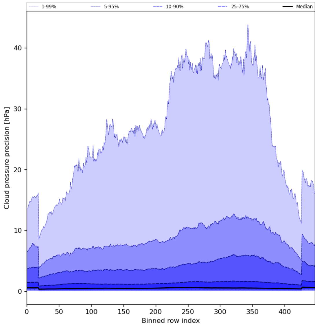
Figure 48: Along track statistics of “Cloud pressure precision” for 2024-06-13 to 2024-06-15
