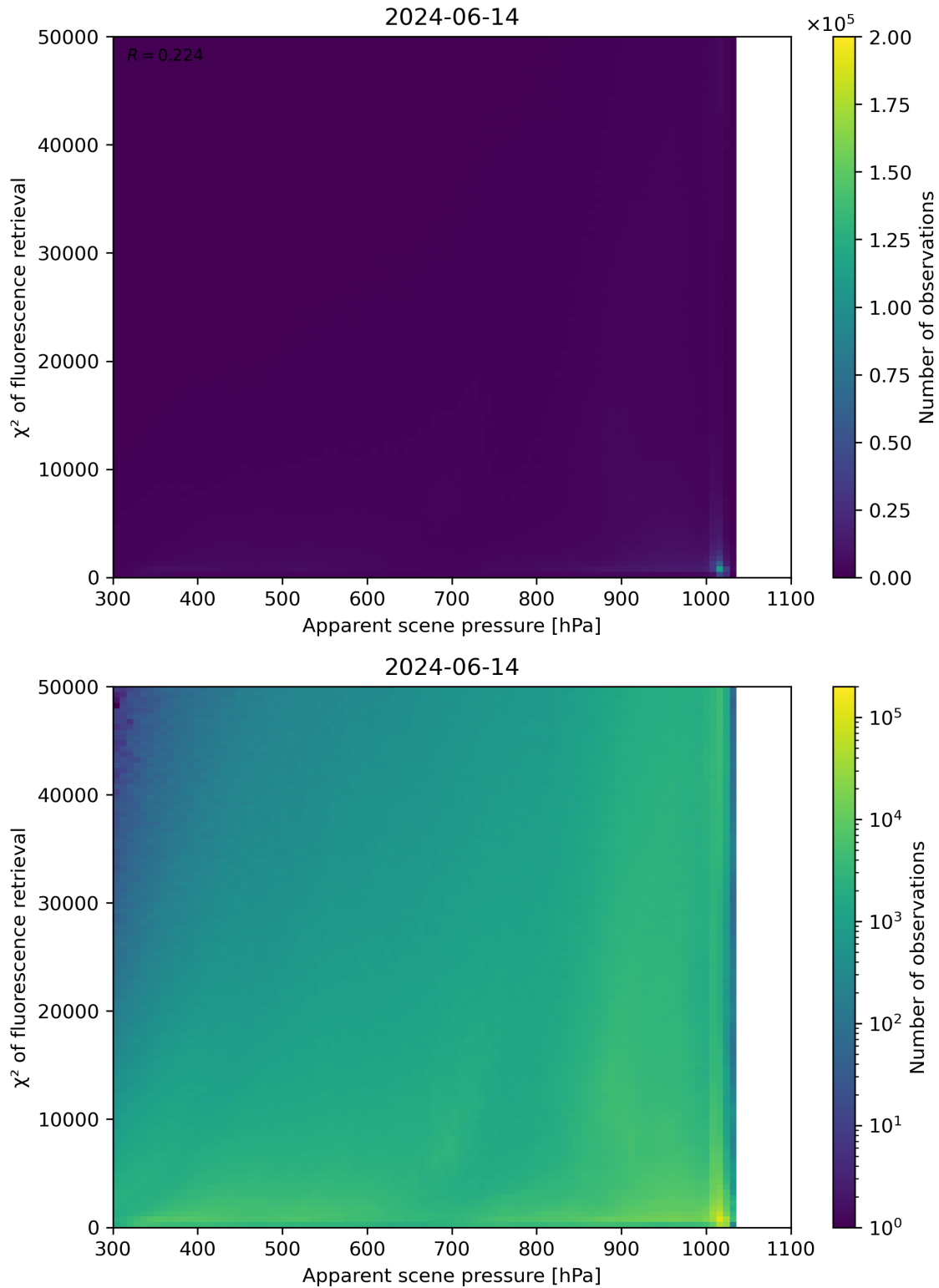
Figure 63: Scatter density plot of “Apparent scene pressure” against “ \chi^2 of fluorescence retrieval” for 2024-06-13 to 2024-06-15.
