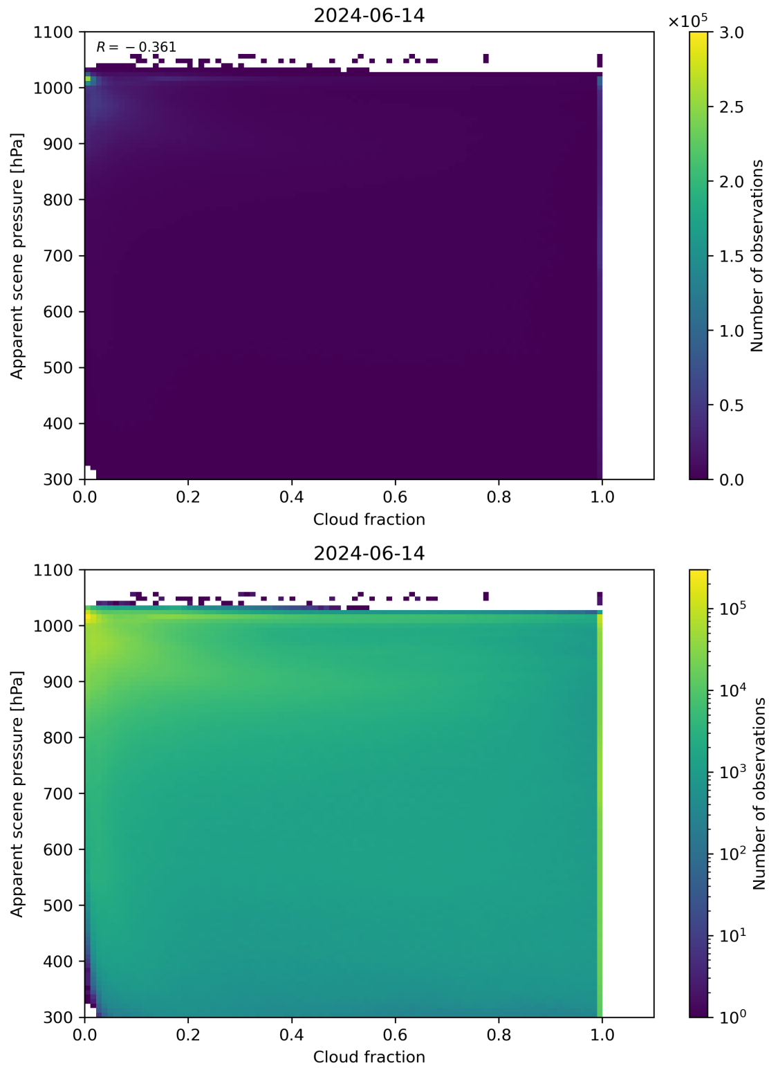
Figure 70: Scatter density plot of “Cloud fraction” against “Apparent scene pressure” for 2024-06-13 to 2024-06-15.
