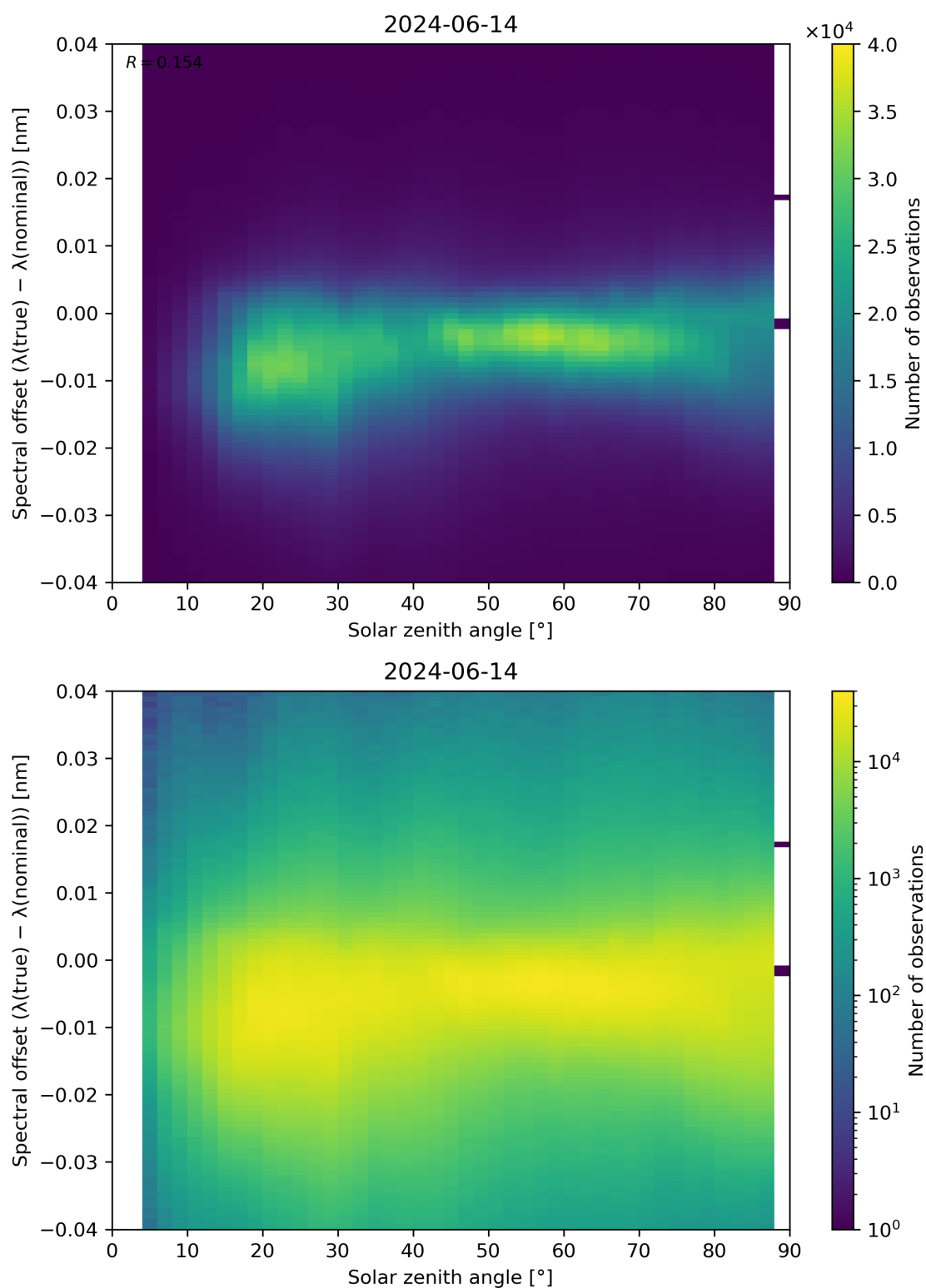
Figure 117: Scatter density plot of “Solar zenith angle” against “Spectral offset ( \lambda(\text{true}) - \lambda(\text{nominal}) )” for 2024-06-13 to 2024-06-15.
