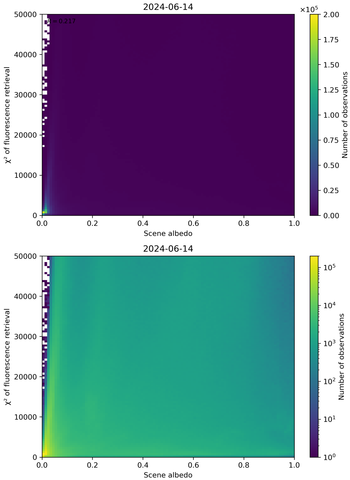
Figure 103: Scatter density plot of “Scene albedo” against “ \chi^2 of fluorescence retrieval” for 2024-06-13 to 2024-06-15.
