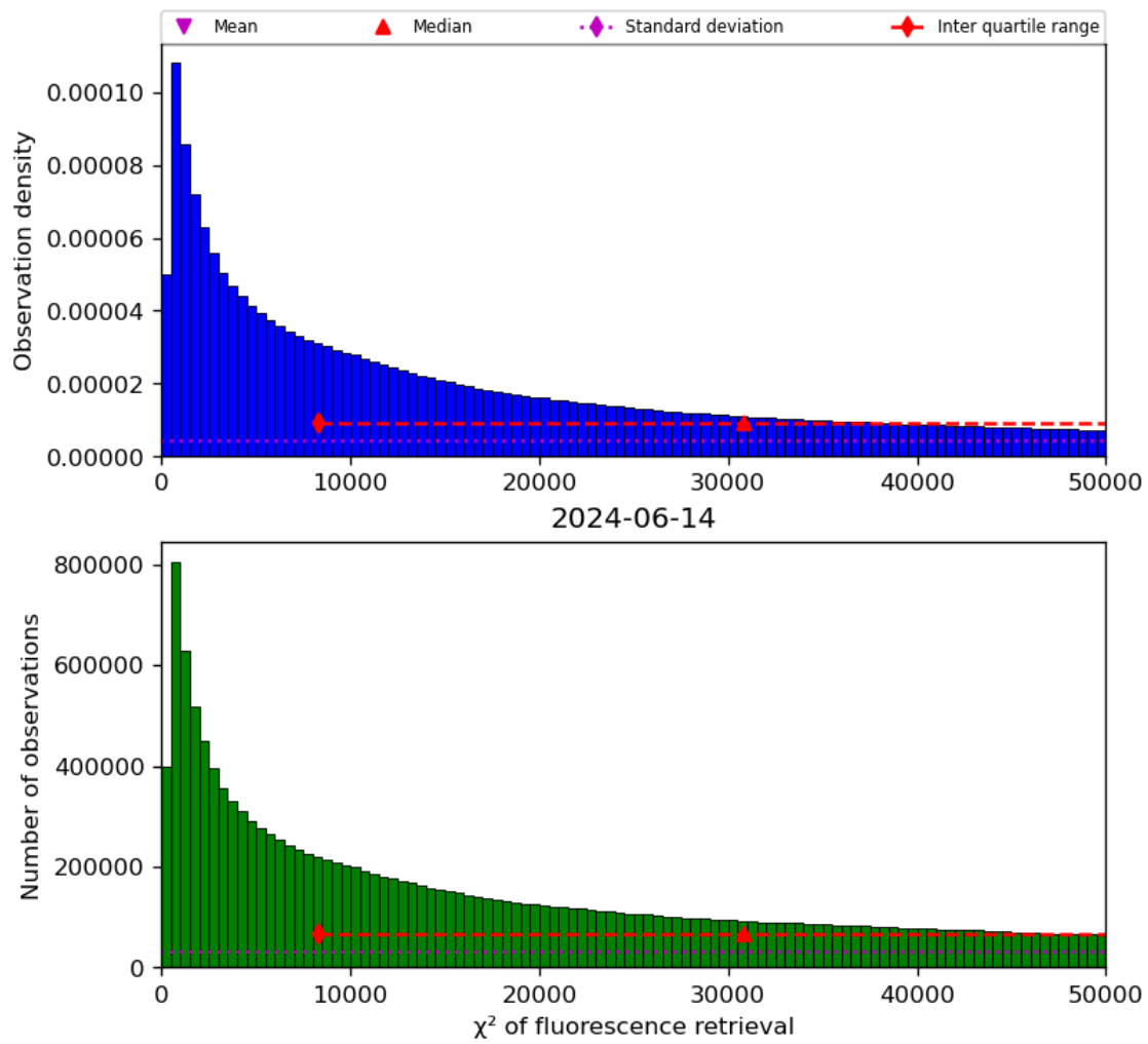
Figure 42: Histogram of “ \chi^2 of fluorescence retrieval” for 2024-06-13 to 2024-06-15
