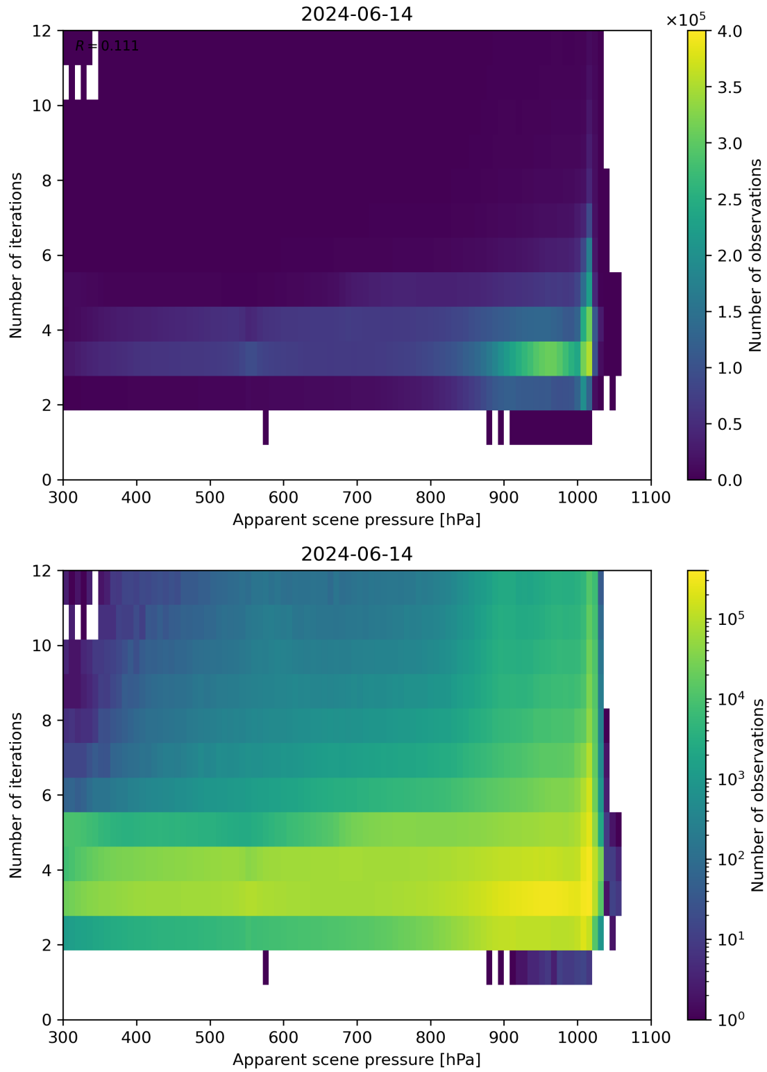
Figure 65: Scatter density plot of “Apparent scene pressure” against “Number of iterations” for 2024-06-13 to 2024-06-15.
