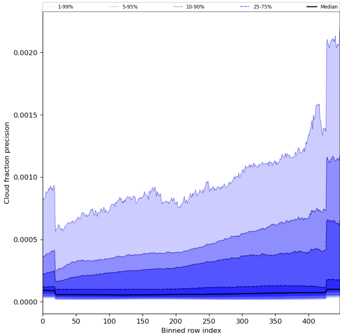
Figure 50: Along track statistics of “Cloud fraction precision” for 2024-06-13 to 2024-06-15
