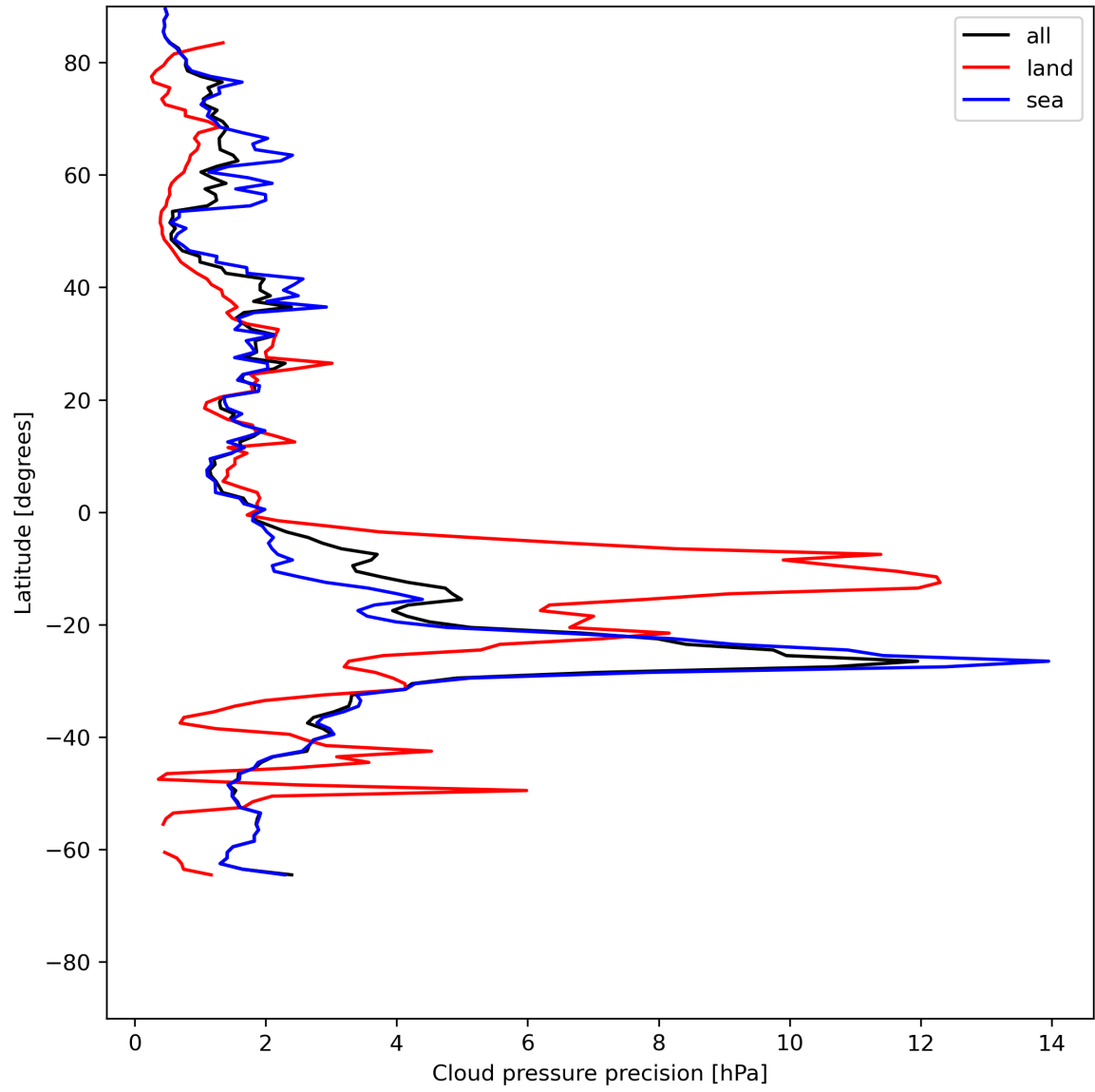
Figure 14: Zonal average of “Cloud pressure precision” for 2024-06-13 to 2024-06-15.
