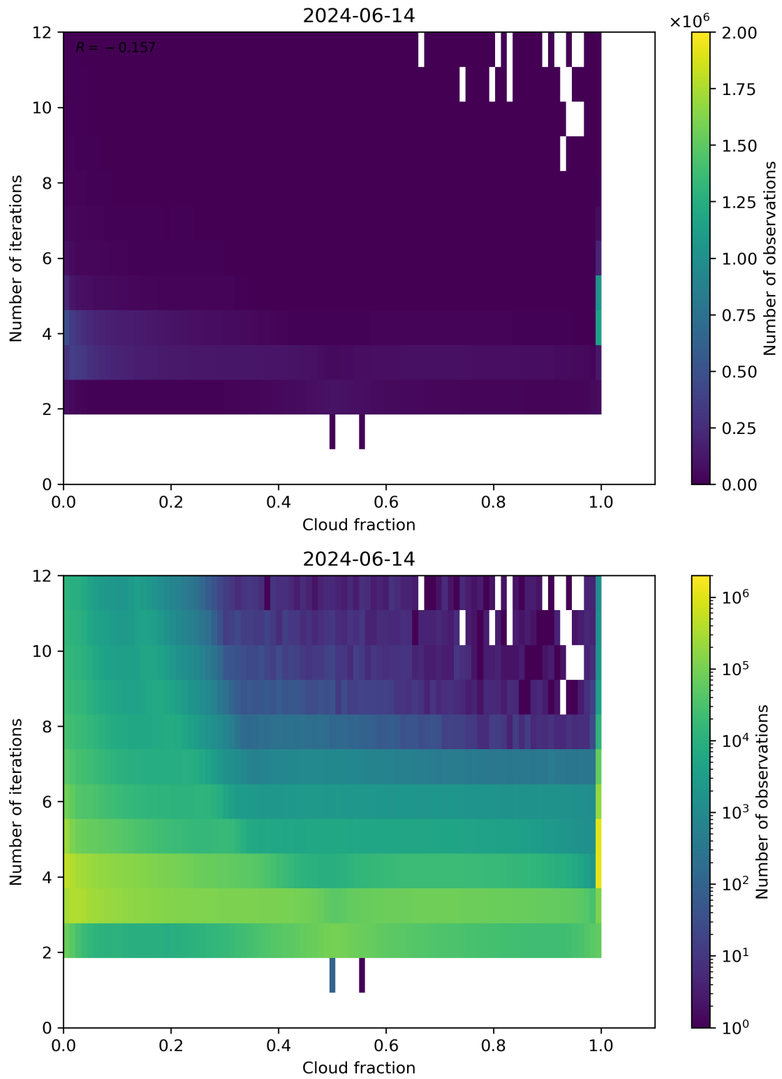
Figure 73: Scatter density plot of “Cloud fraction” against “Number of iterations” for 2024-06-13 to 2024-06-15.
