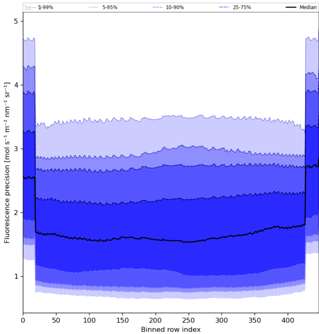
Figure 58: Along track statistics of “Fluorescence precision” for 2024-06-13 to 2024-06-15
