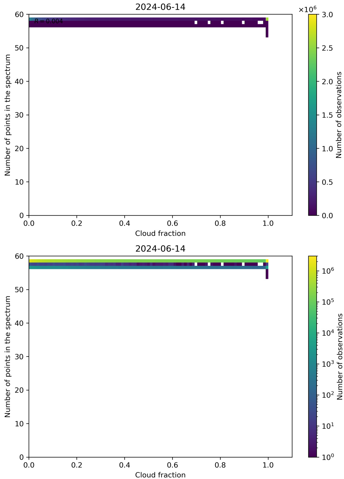
Figure 74: Scatter density plot of “Cloud fraction” against “Number of points in the spectrum” for 2024-06-13 to 2024-06-15.
