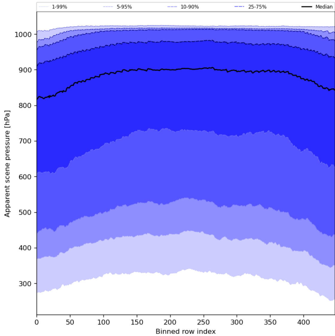
Figure 53: Along track statistics of “Apparent scene pressure” for 2024-06-13 to 2024-06-15
