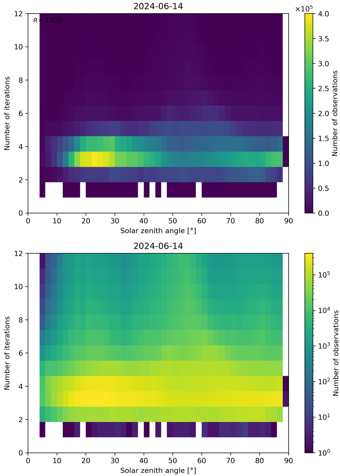
Figure 114: Scatter density plot of “Solar zenith angle” against “Number of iterations” for 2024-06-13 to 2024-06-15.
