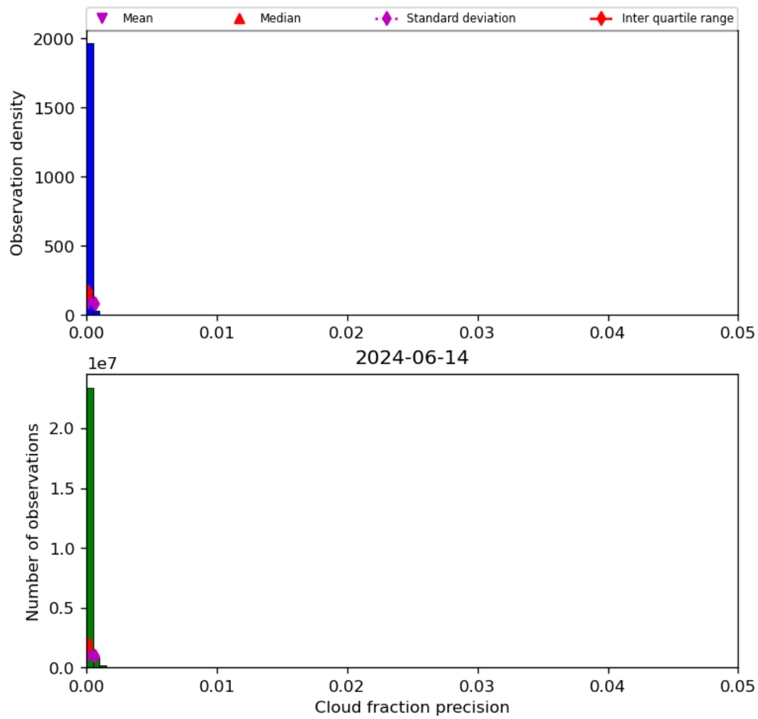
Figure 33: Histogram of “Cloud fraction precision” for 2024-06-13 to 2024-06-15
