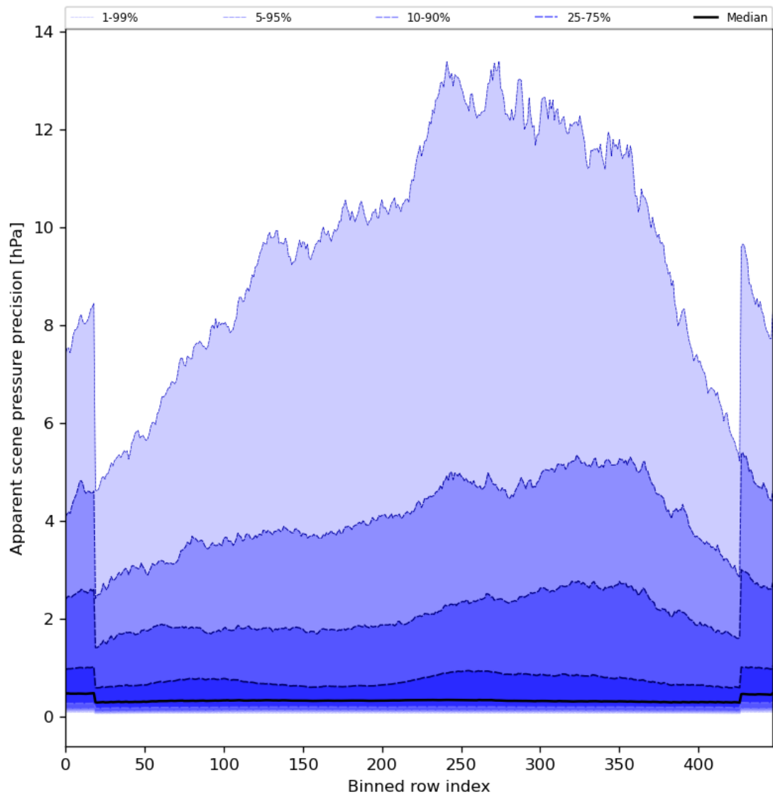
Figure 54: Along track statistics of “Apparent scene pressure precision” for 2024-06-13 to 2024-06-15
