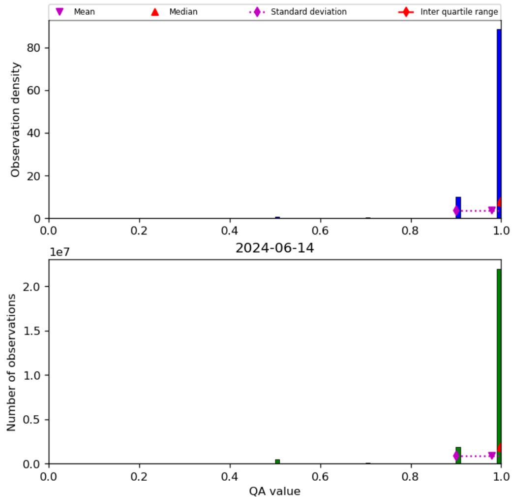
Figure 29: Histogram of “QA value” for 2024-06-13 to 2024-06-15
