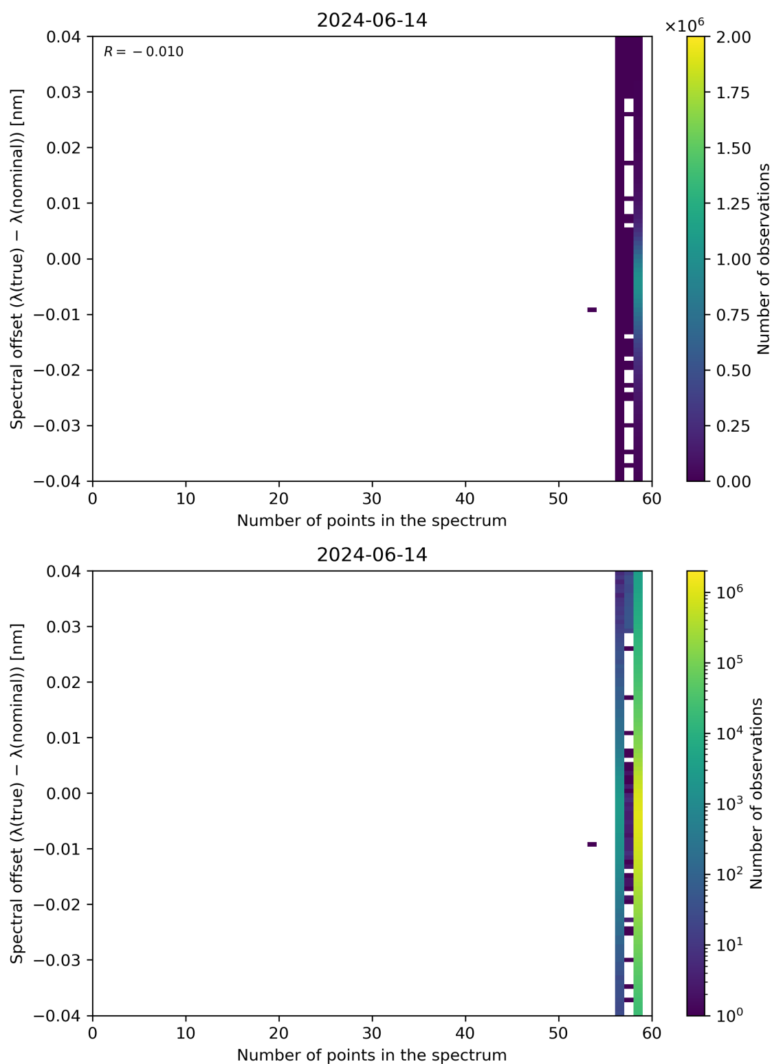
Figure 101: Scatter density plot of “Number of points in the spectrum” against “Spectral offset ( \lambda(\text{true}) - \lambda(\text{nominal}) )” for 2024-06-13 to 2024-06-15.
