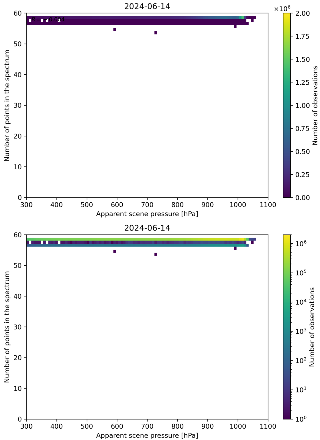
Figure 66: Scatter density plot of “Apparent scene pressure” against “Number of points in the spectrum” for 2024-06-13 to 2024-06-15.
