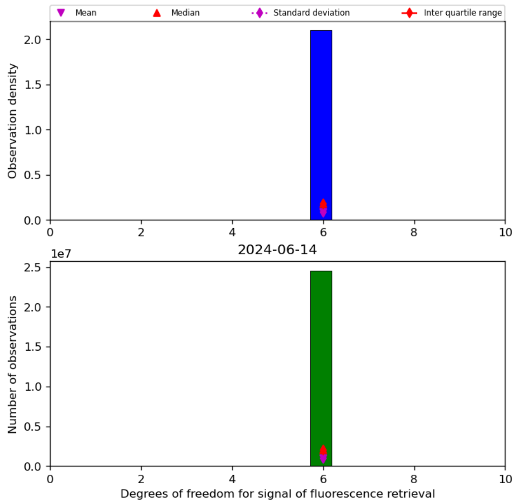
Figure 43: Histogram of “Degrees of freedom for signal of fluorescence retrieval” for 2024-06-13 to 2024-06-15
