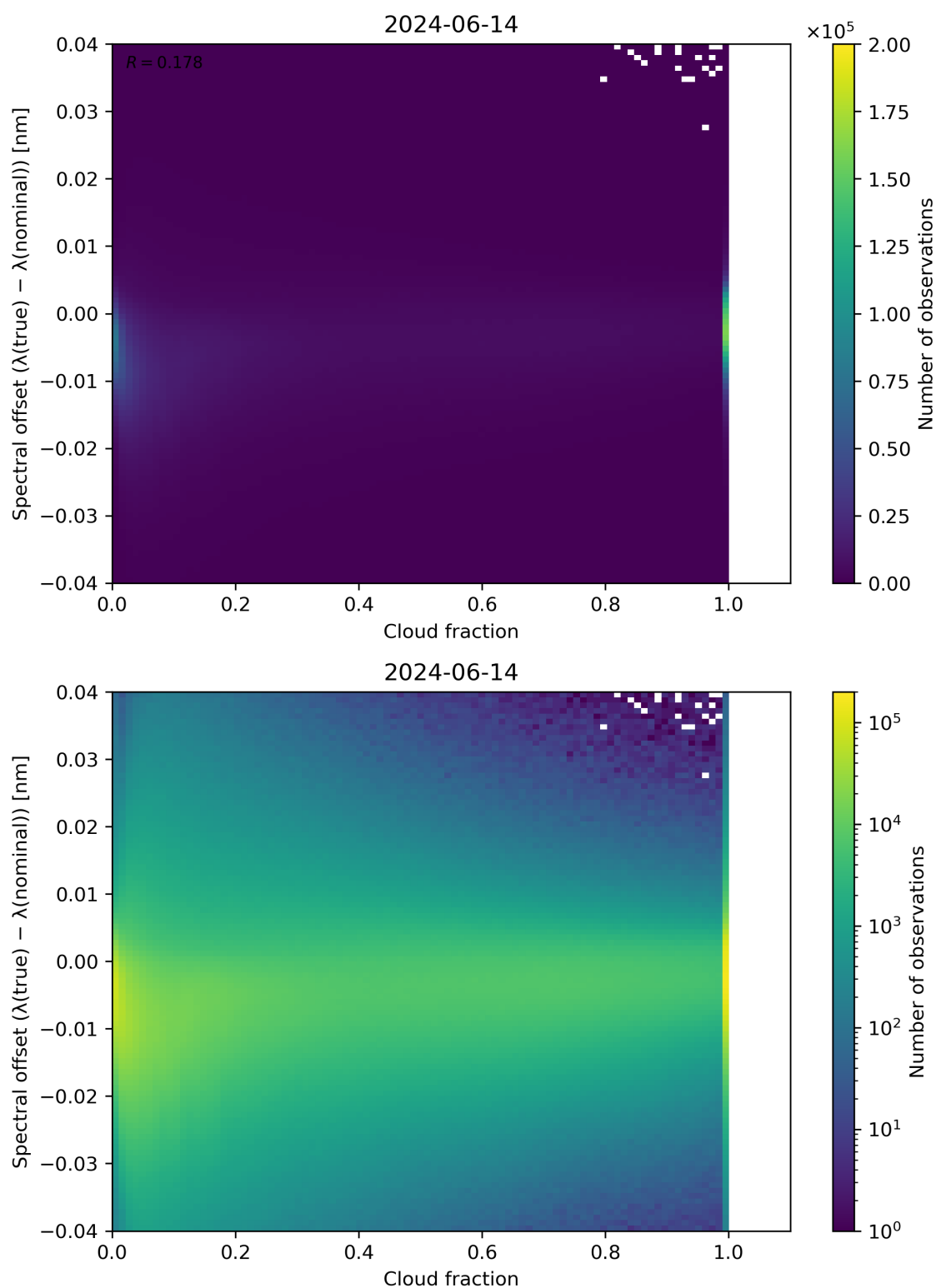
Figure 76: Scatter density plot of “Cloud fraction” against “Spectral offset ( \lambda(\text{true}) - \lambda(\text{nominal}) )” for 2024-06-13 to 2024-06-15.
