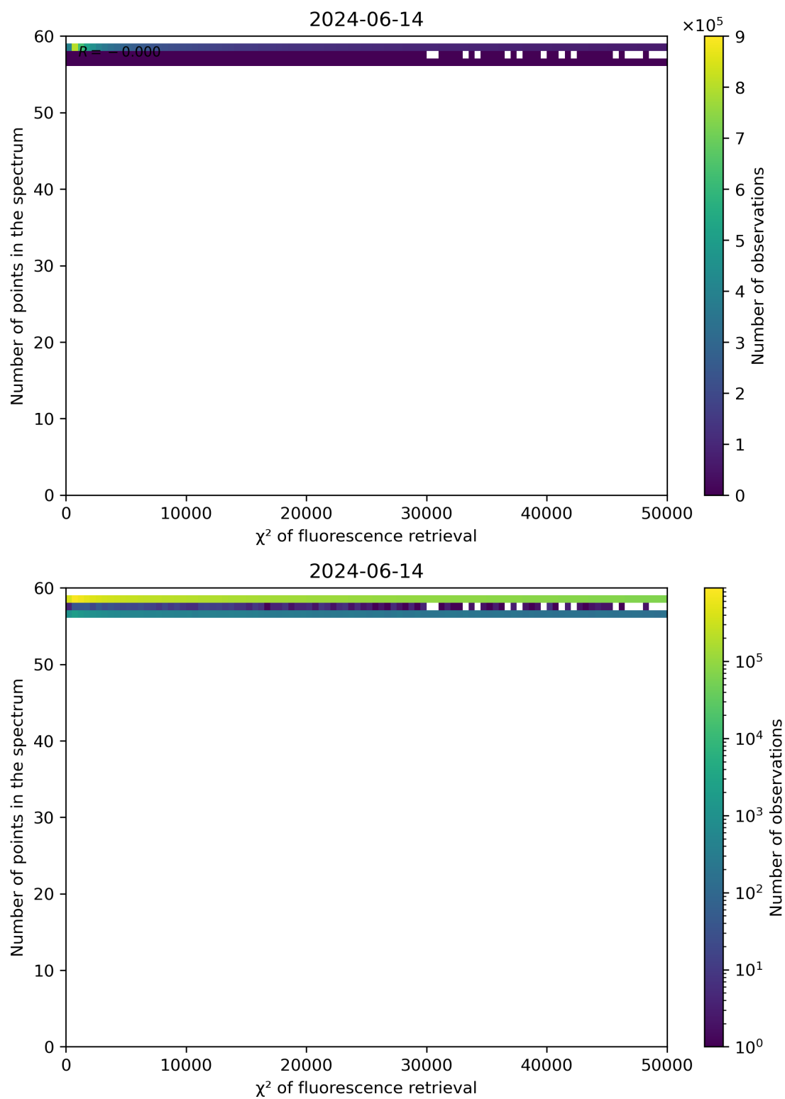
Figure 68: Scatter density plot of " \chi^2 of fluorescence retrieval" against "Number of points in the spectrum" for 2024-06-13 to 2024-06-15.
