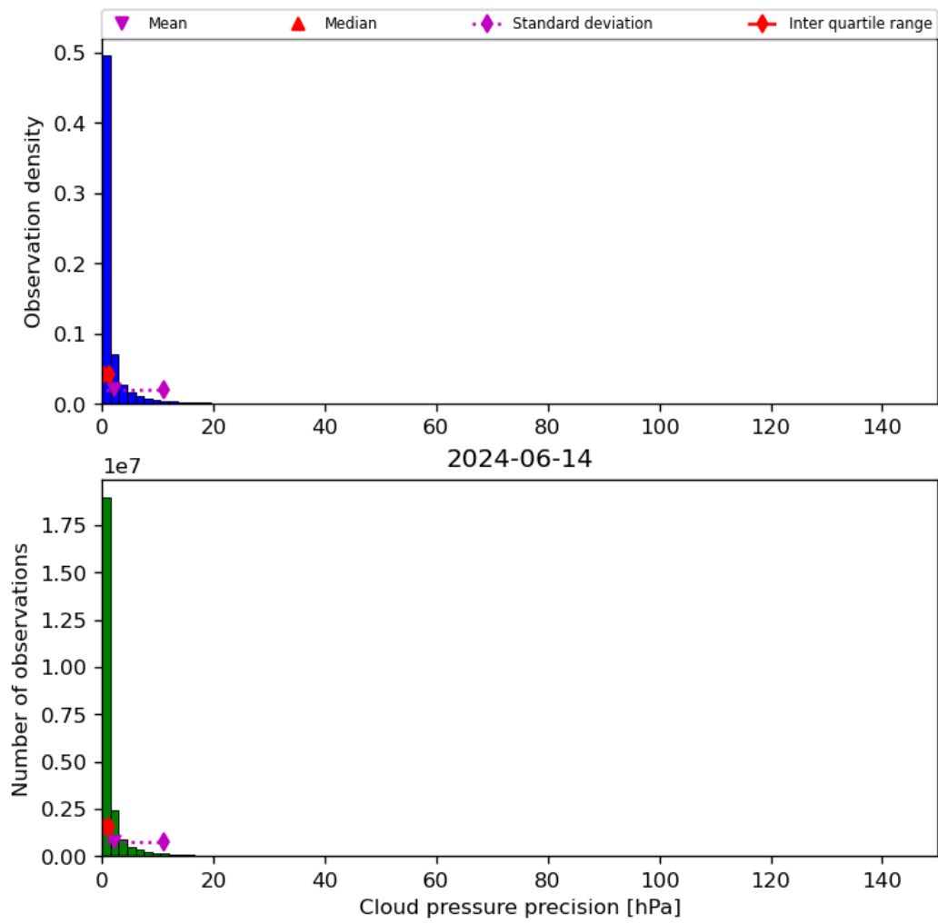
Figure 31: Histogram of “Cloud pressure precision” for 2024-06-13 to 2024-06-15
