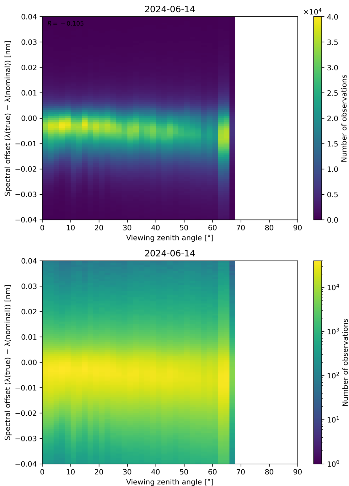
Figure 128: Scatter density plot of “Viewing zenith angle” against “Spectral offset ( \lambda(\text{true}) - \lambda(\text{nominal}) )” for 2024-06-13 to 2024-06-15.
