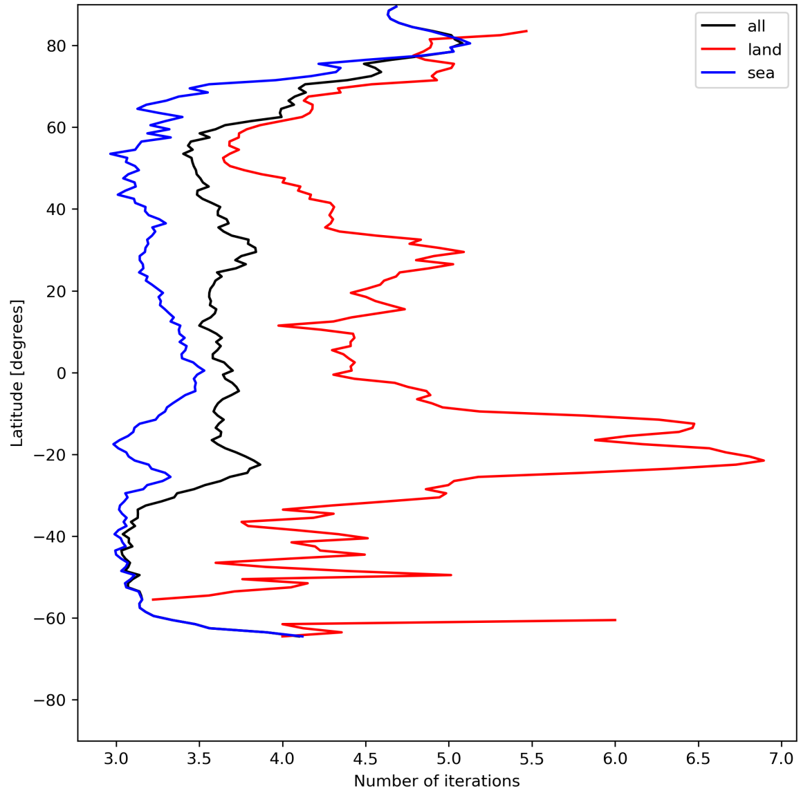
Figure 22: Zonal average of “Number of iterations” for 2024-06-13 to 2024-06-15.
