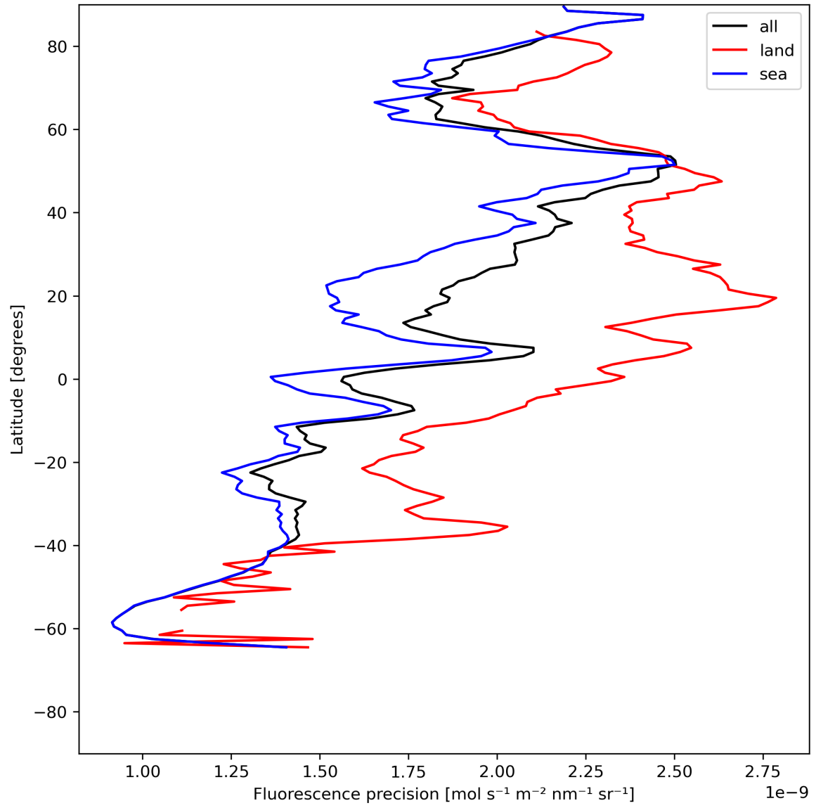
Figure 24: Zonal average of “Fluorescence precision” for 2024-06-13 to 2024-06-15.
