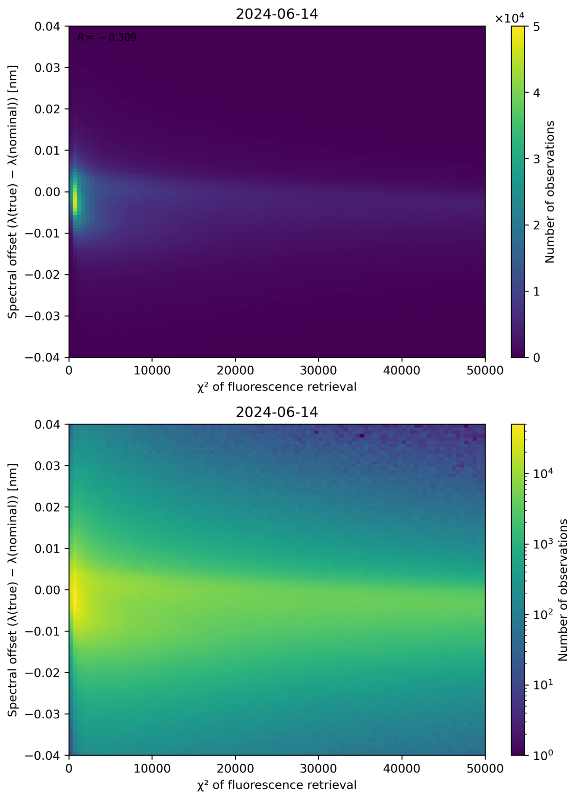
Figure 69: Scatter density plot of “ \chi^2 of fluorescence retrieval” against “Spectral offset ( \lambda(\text{true}) - \lambda(\text{nominal}) )” for 2024-06-13 to 2024-06-15.
