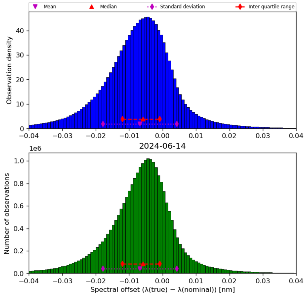
Figure 45: Histogram of “Spectral offset ( \lambda(\text{true}) - \lambda(\text{nominal}) )” for 2024-06-13 to 2024-06-15
