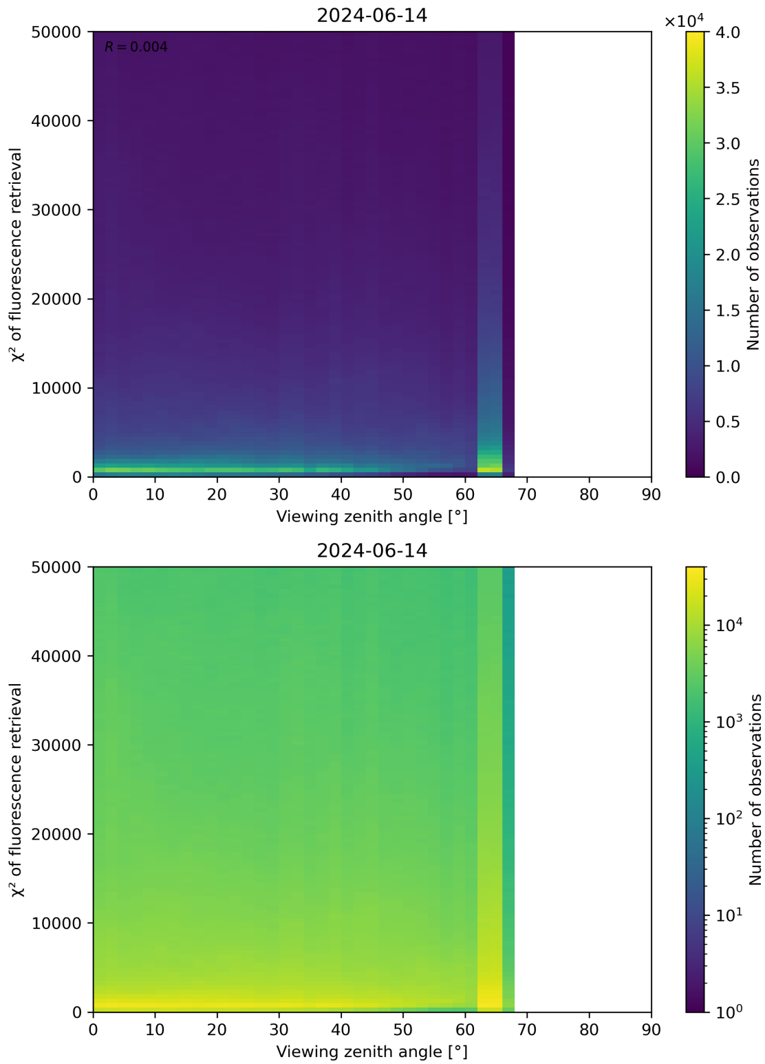
Figure 119: Scatter density plot of “Viewing zenith angle” against “ \chi^2 of fluorescence retrieval” for 2024-06-13 to 2024-06-15.
