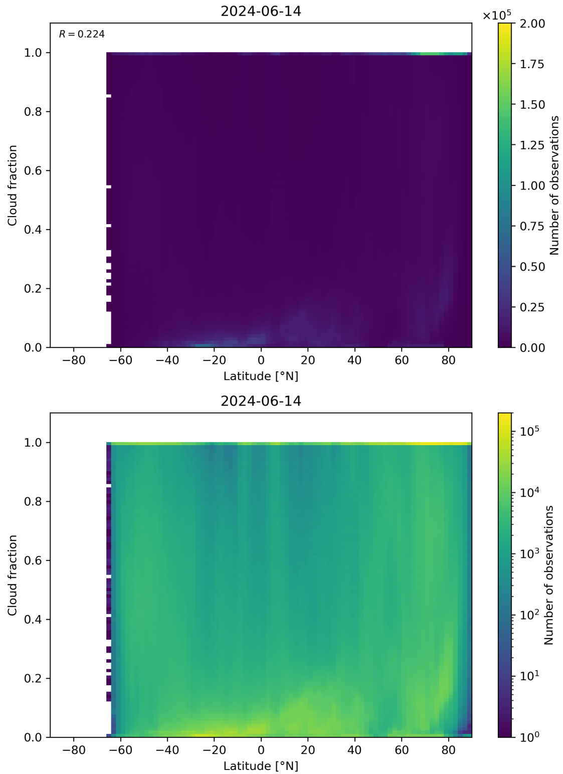
Figure 90: Scatter density plot of “Latitude” against “Cloud fraction” for 2024-06-13 to 2024-06-15.
