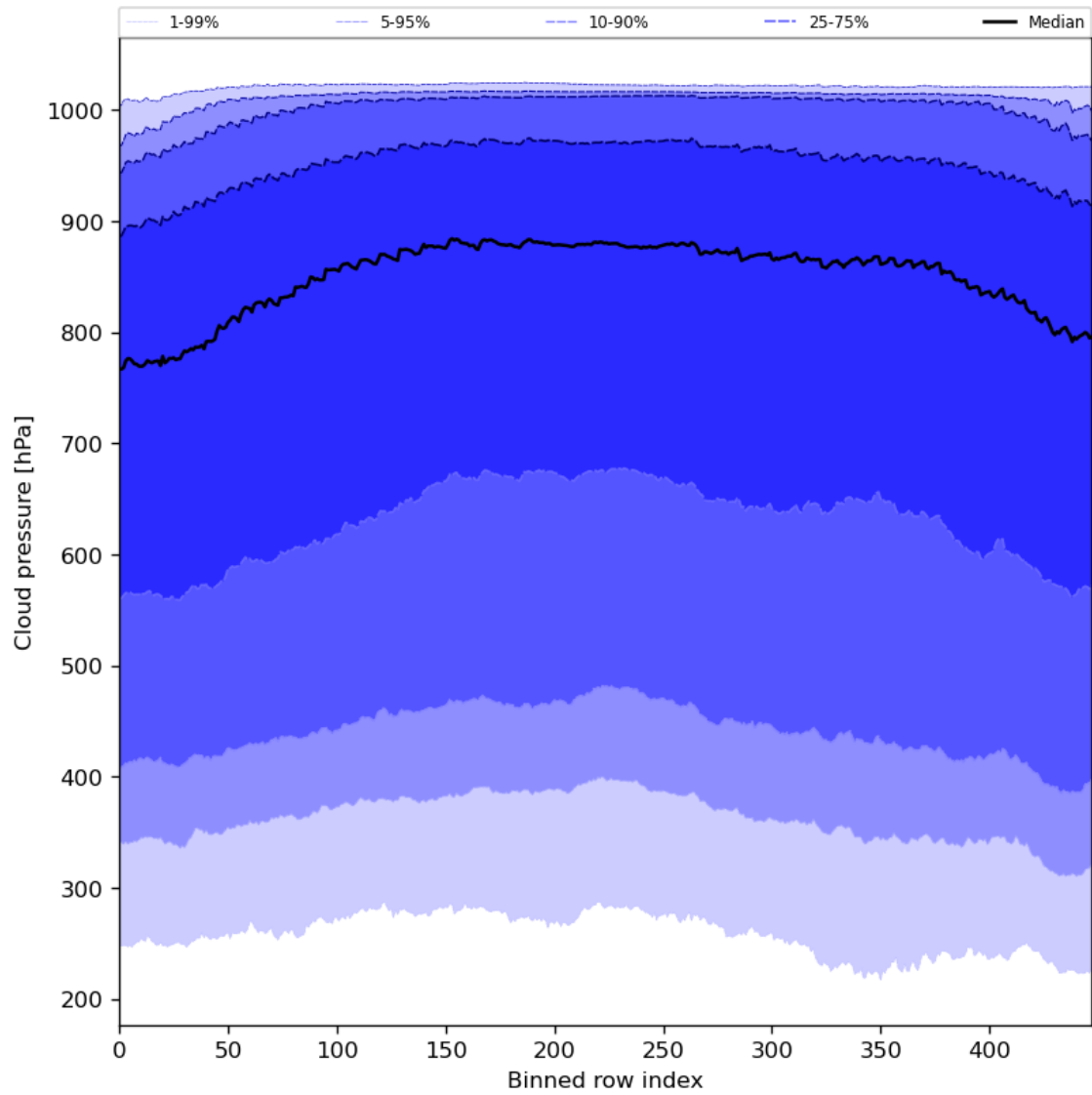
Figure 47: Along track statistics of “Cloud pressure” for 2024-06-13 to 2024-06-15
