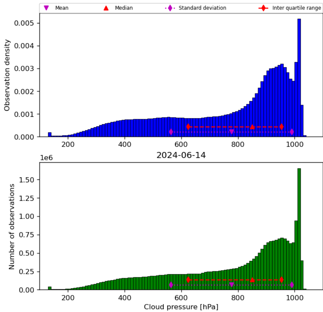
Figure 30: Histogram of “Cloud pressure” for 2024-06-13 to 2024-06-15
