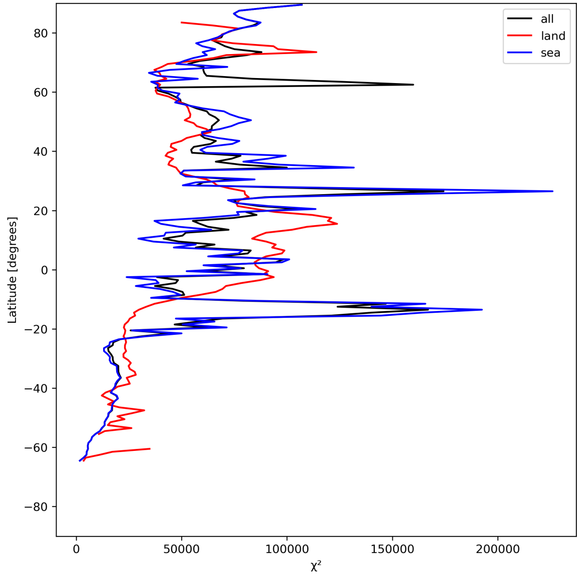
Figure 21: Zonal average of “ \chi^2 ” for 2024-06-13 to 2024-06-15.
