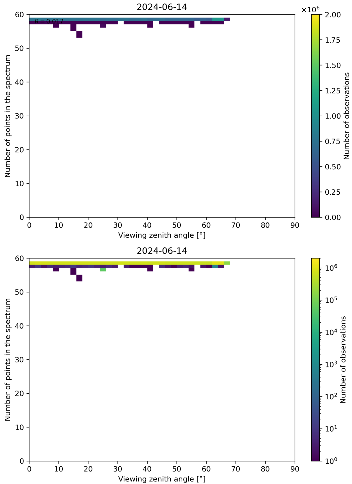
Figure 125: Scatter density plot of “Viewing zenith angle” against “Number of points in the spectrum” for 2024-06-13 to 2024-06-15.
