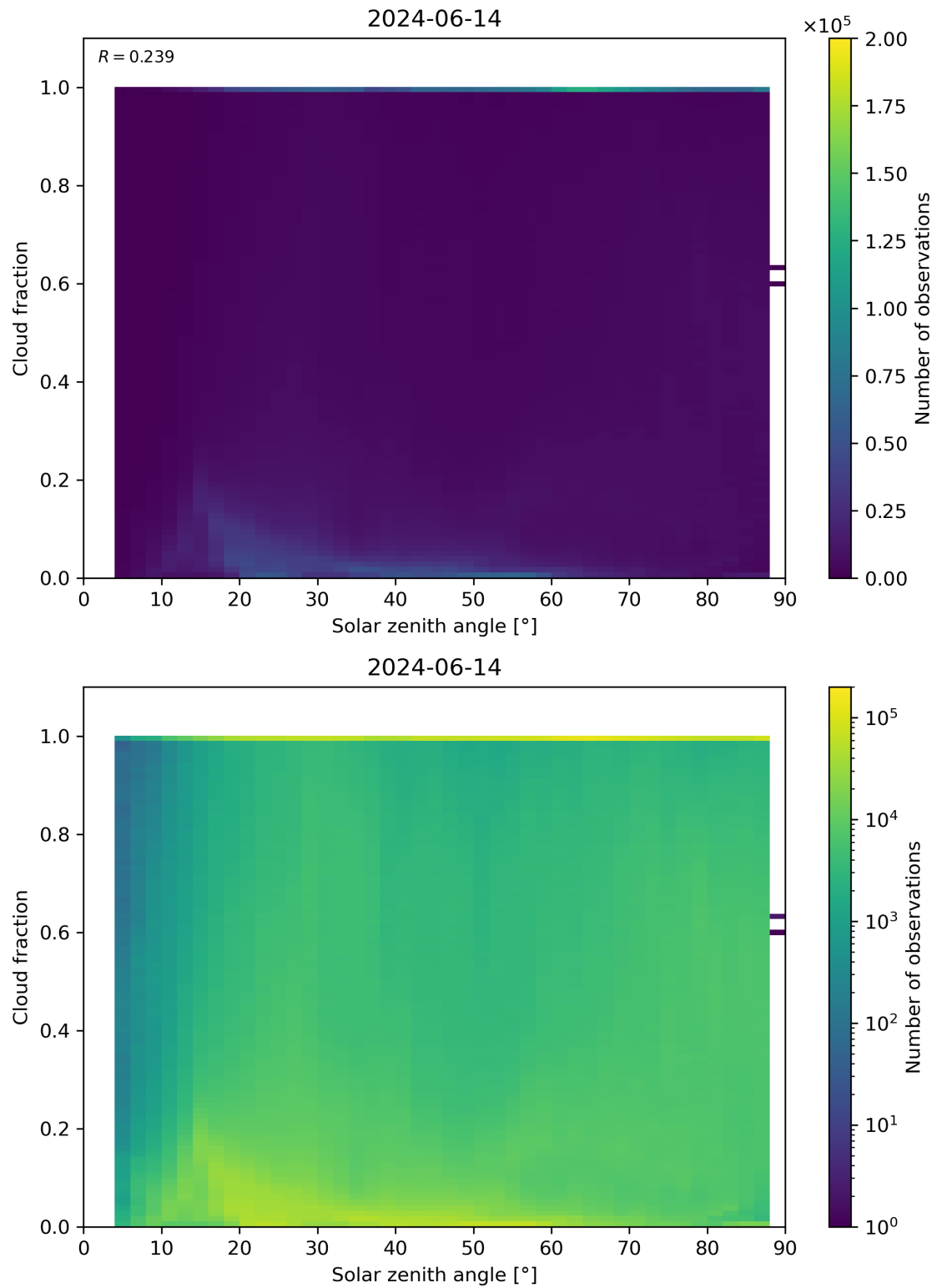
Figure 110: Scatter density plot of “Solar zenith angle” against “Cloud fraction” for 2024-06-13 to 2024-06-15.
