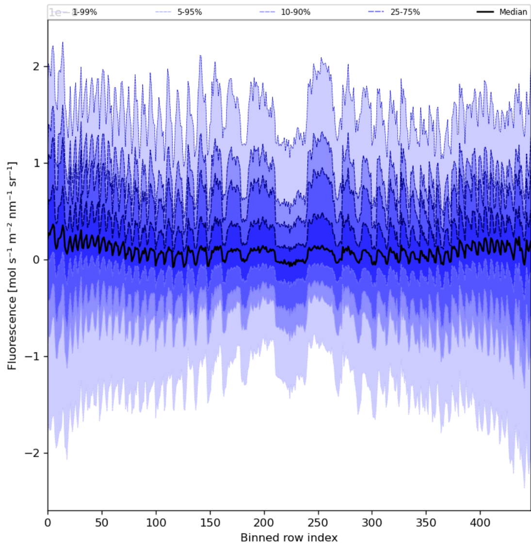
Figure 57: Along track statistics of “Fluorescence” for 2024-06-13 to 2024-06-15
