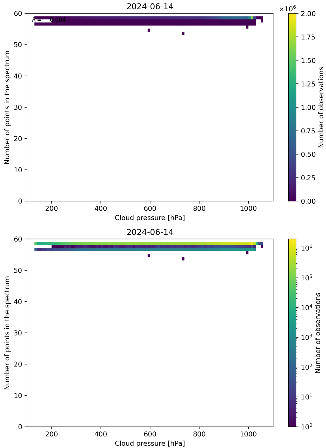
Figure 82: Scatter density plot of “Cloud pressure” against “Number of points in the spectrum” for 2024-06-13 to 2024-06-15.
