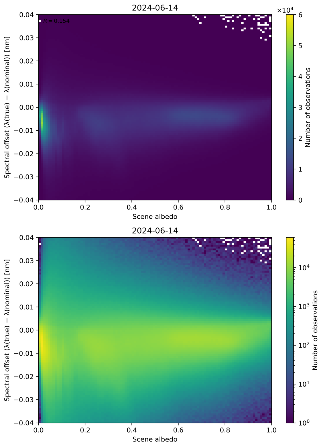
Figure 107: Scatter density plot of “Scene albedo” against “Spectral offset ( \lambda(\text{true}) - \lambda(\text{nominal}) )” for 2024-06-13 to 2024-06-15.
