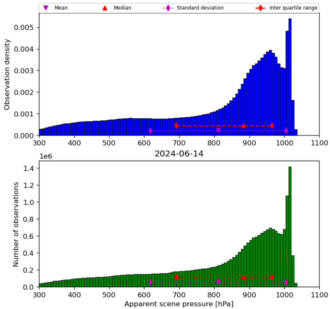
Figure 36: Histogram of “Apparent scene pressure” for 2024-06-13 to 2024-06-15
