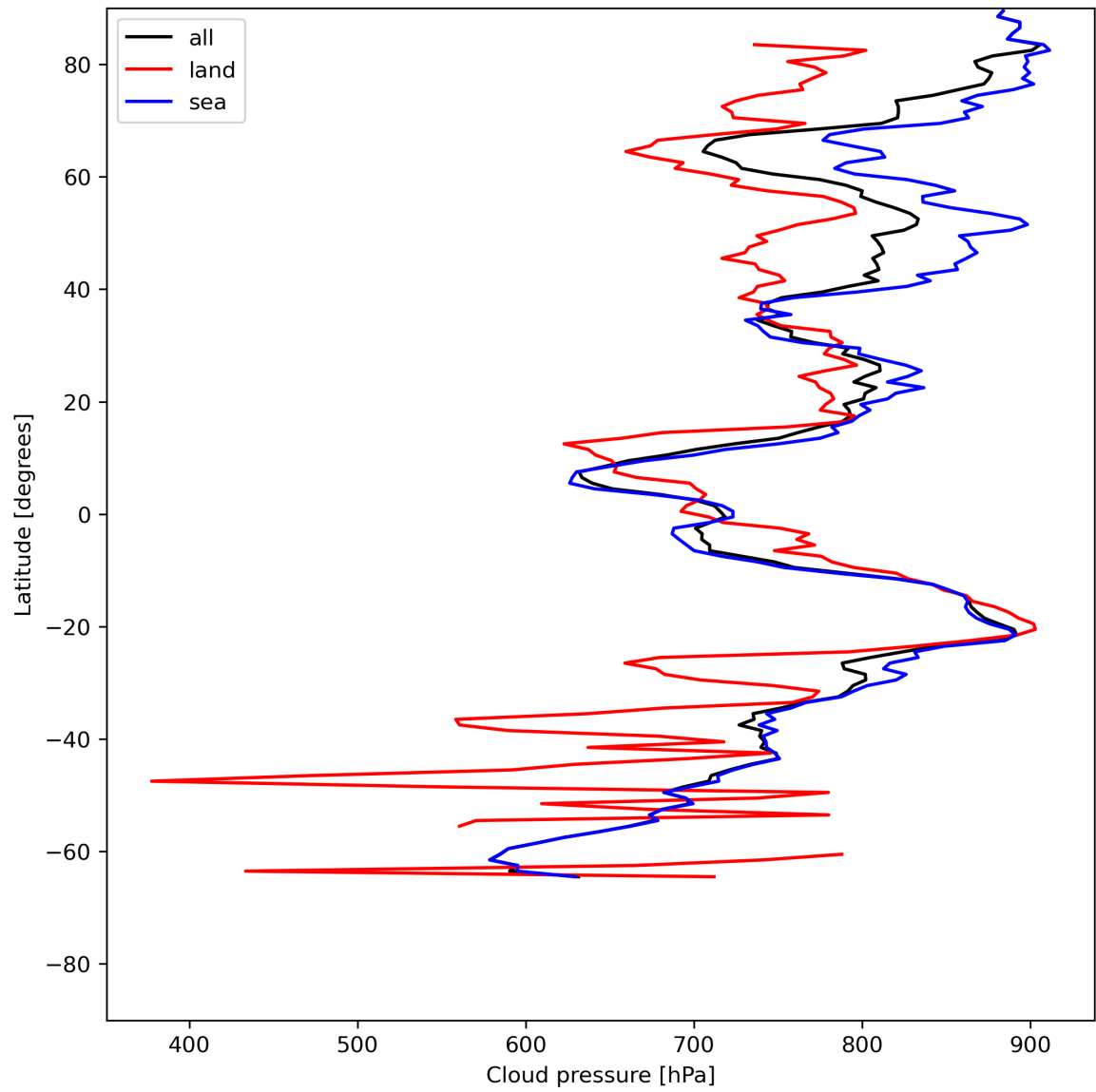
Figure 13: Zonal average of “Cloud pressure” for 2024-06-13 to 2024-06-15.
