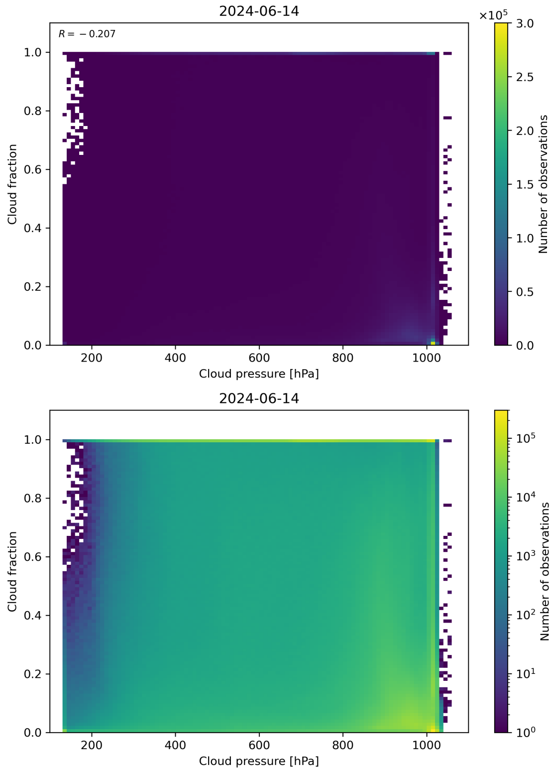
Figure 79: Scatter density plot of “Cloud pressure” against “Cloud fraction” for 2024-06-13 to 2024-06-15.
