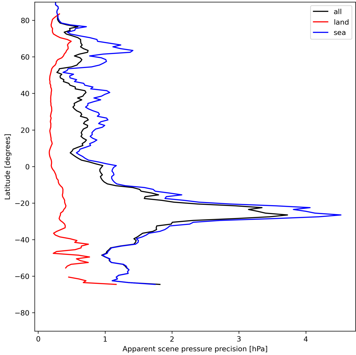
Figure 20: Zonal average of “Apparent scene pressure precision” for 2024-06-13 to 2024-06-15.
