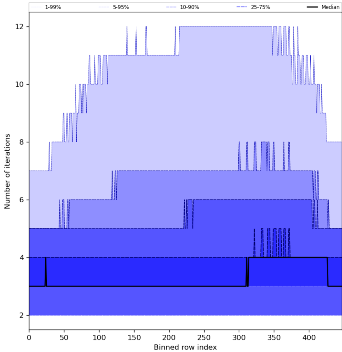
Figure 56: Along track statistics of “Number of iterations” for 2024-06-13 to 2024-06-15
