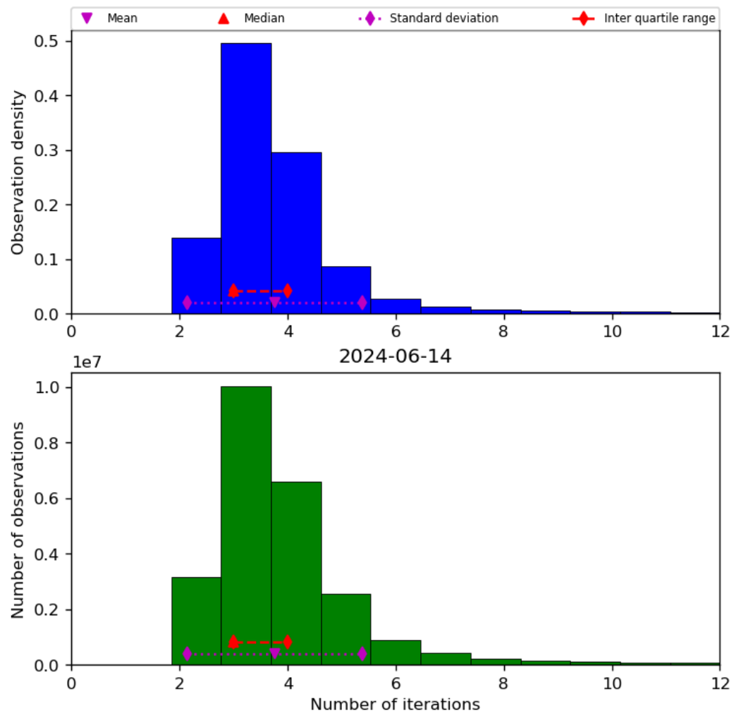
Figure 39: Histogram of “Number of iterations” for 2024-06-13 to 2024-06-15
