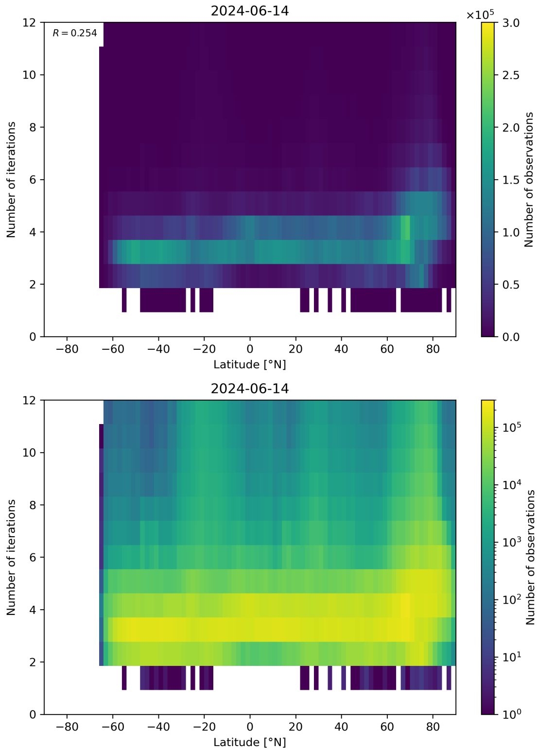
Figure 93: Scatter density plot of “Latitude” against “Number of iterations” for 2024-06-13 to 2024-06-15.
