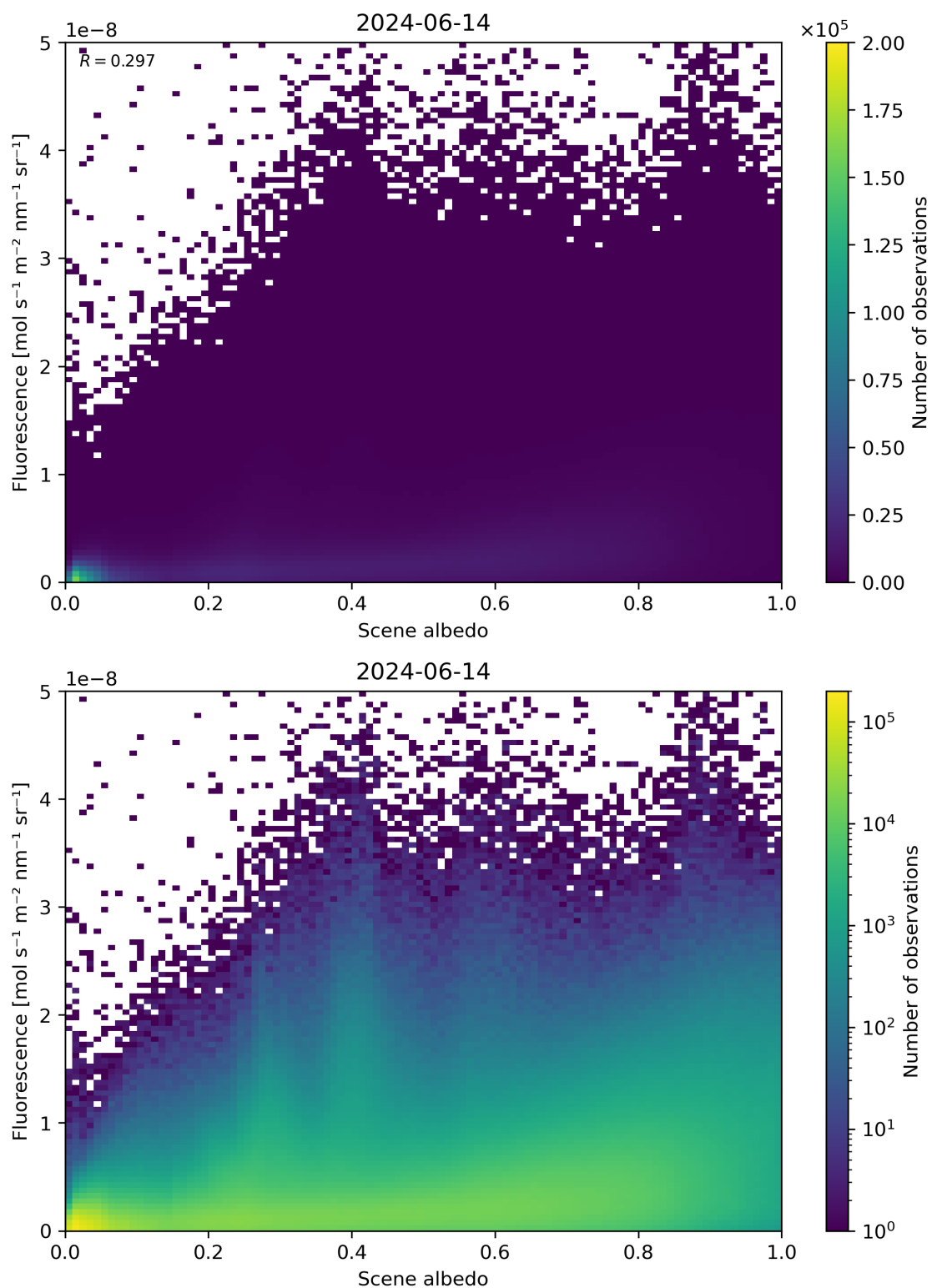
Figure 104: Scatter density plot of “Scene albedo” against “Fluorescence” for 2024-06-13 to 2024-06-15.
