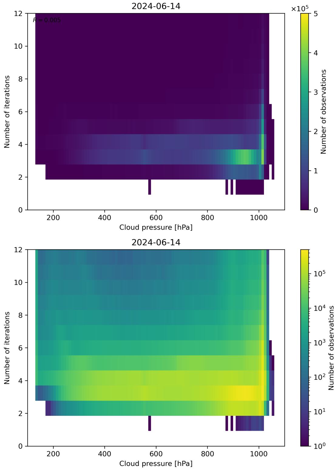
Figure 81: Scatter density plot of “Cloud pressure” against “Number of iterations” for 2024-06-13 to 2024-06-15.
