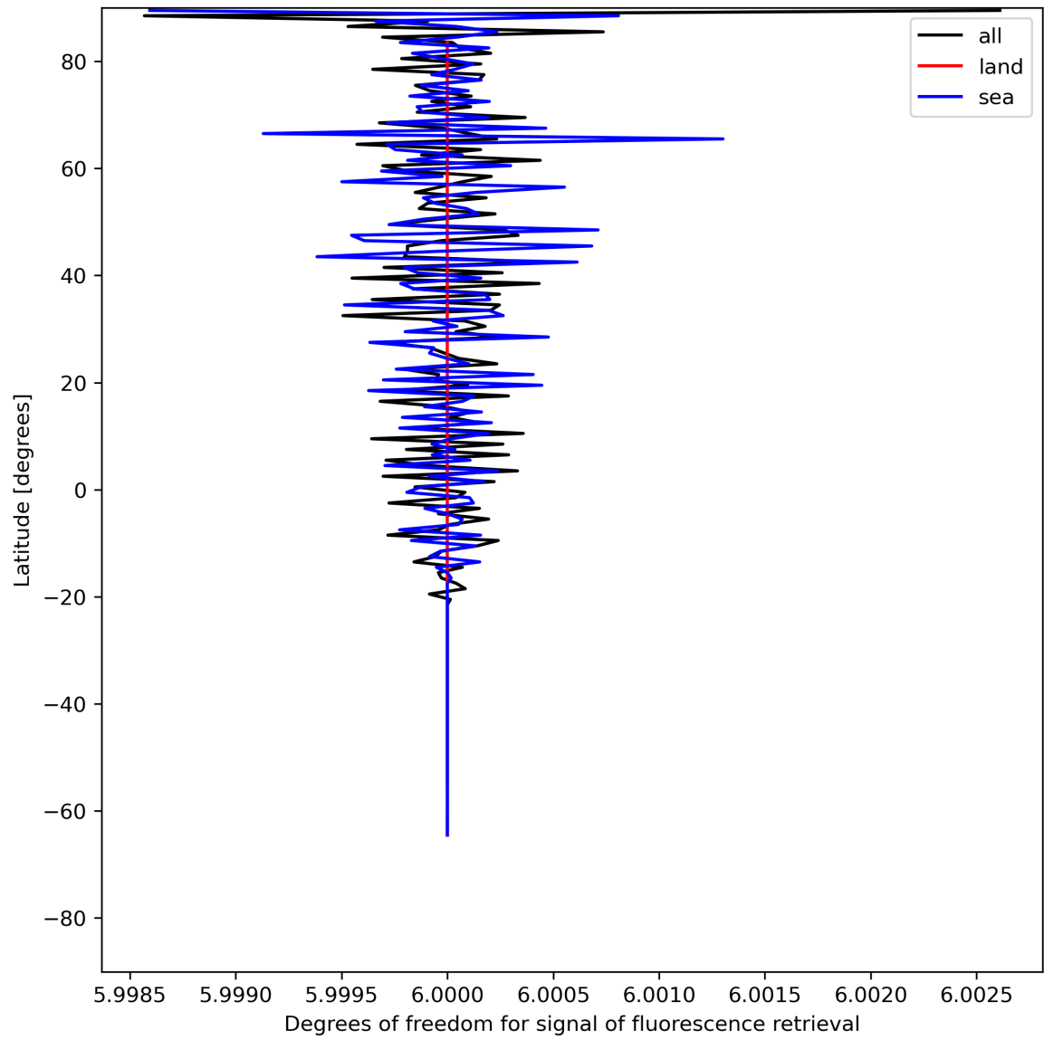
Figure 26: Zonal average of “Degrees of freedom for signal of fluorescence retrieval” for 2024-06-13 to 2024-06-15.
