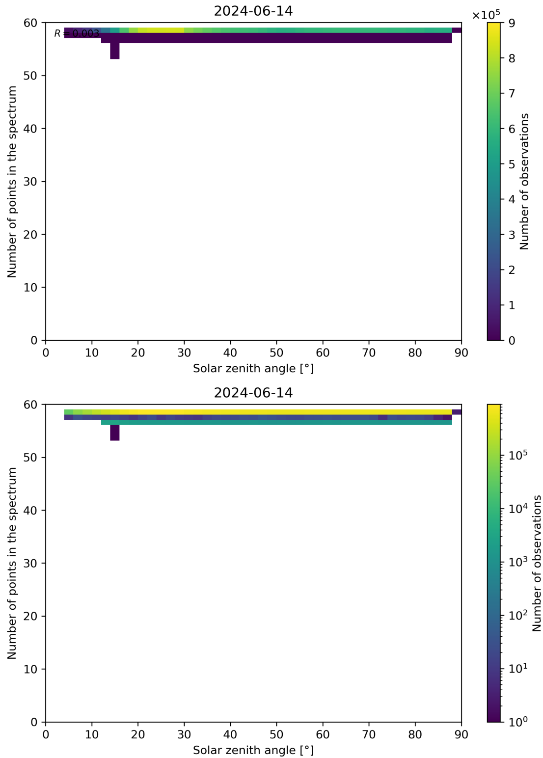
Figure 115: Scatter density plot of “Solar zenith angle” against “Number of points in the spectrum” for 2024-06-13 to 2024-06-15.
