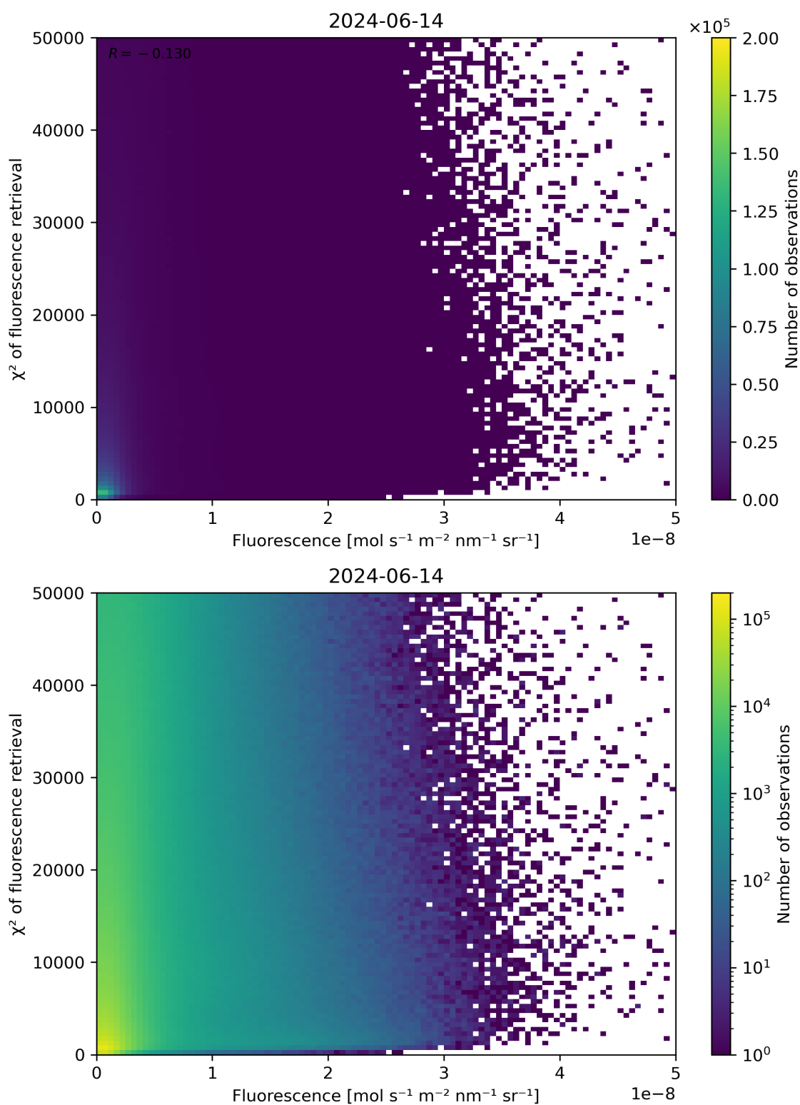
Figure 85: Scatter density plot of “Fluorescence” against “ \chi^2 of fluorescence retrieval” for 2024-06-13 to 2024-06-15.
