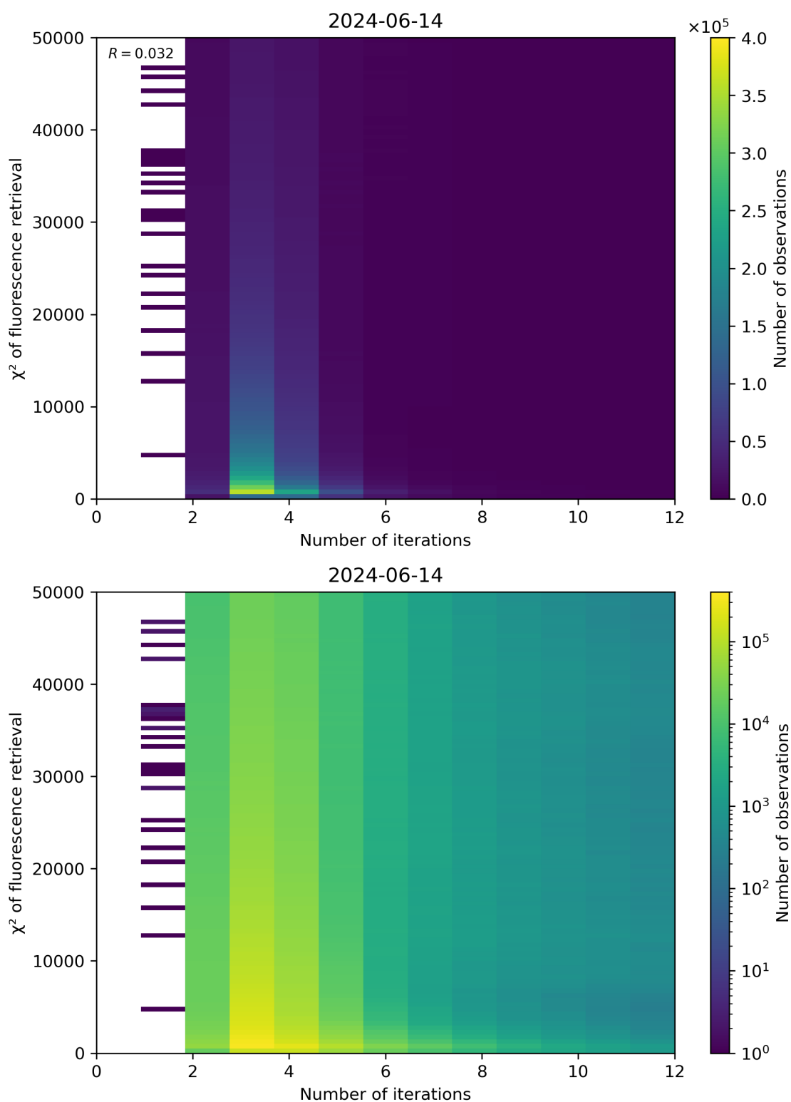
Figure 97: Scatter density plot of “Number of iterations” against “ \chi^2 of fluorescence retrieval” for 2024-06-13 to 2024-06-15.
