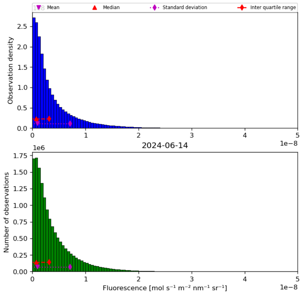
Figure 40: Histogram of “Fluorescence” for 2024-06-13 to 2024-06-15
