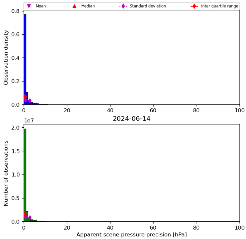
Figure 37: Histogram of “Apparent scene pressure precision” for 2024-06-13 to 2024-06-15
