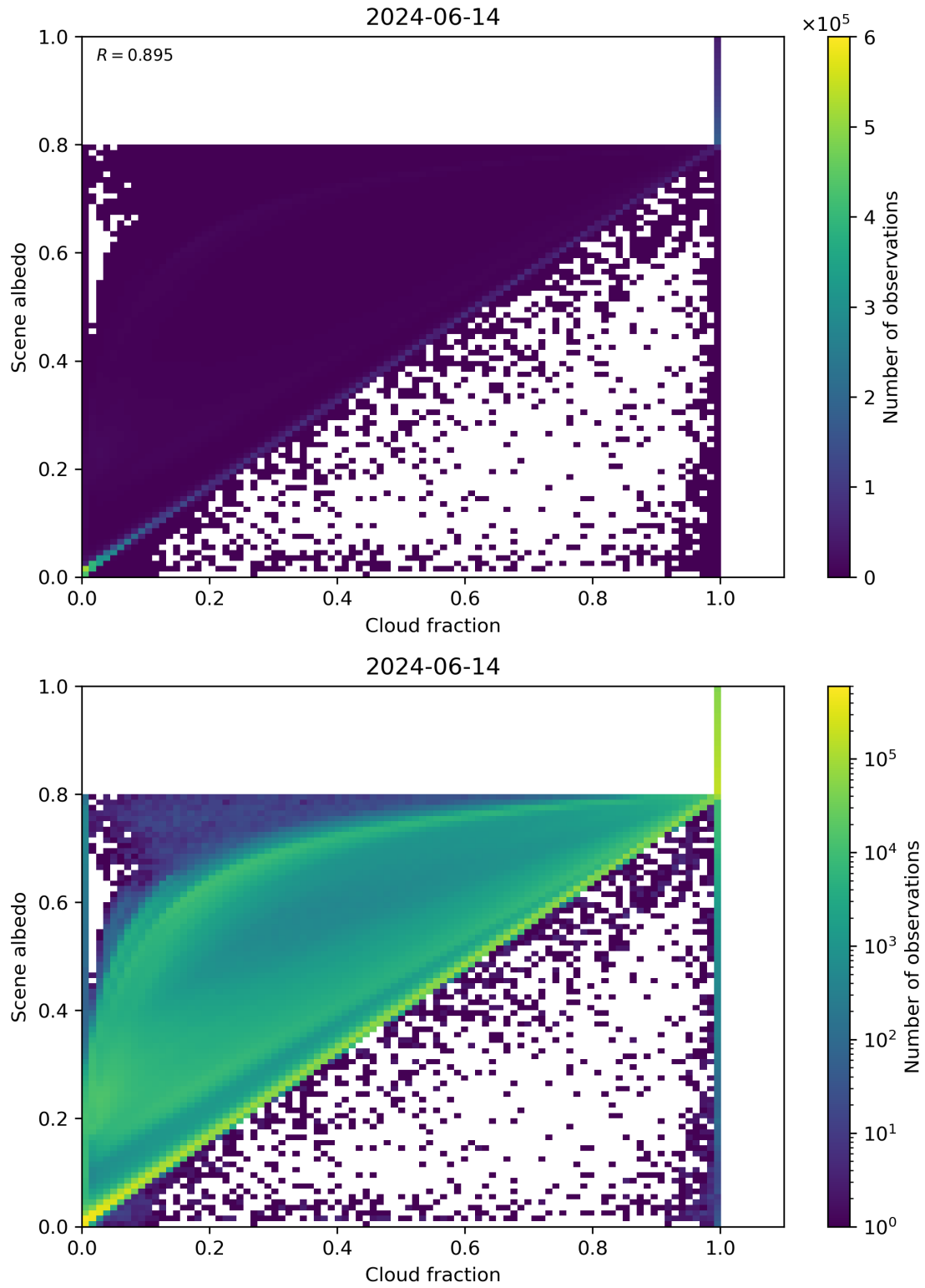
Figure 75: Scatter density plot of “Cloud fraction” against “Scene albedo” for 2024-06-13 to 2024-06-15.
