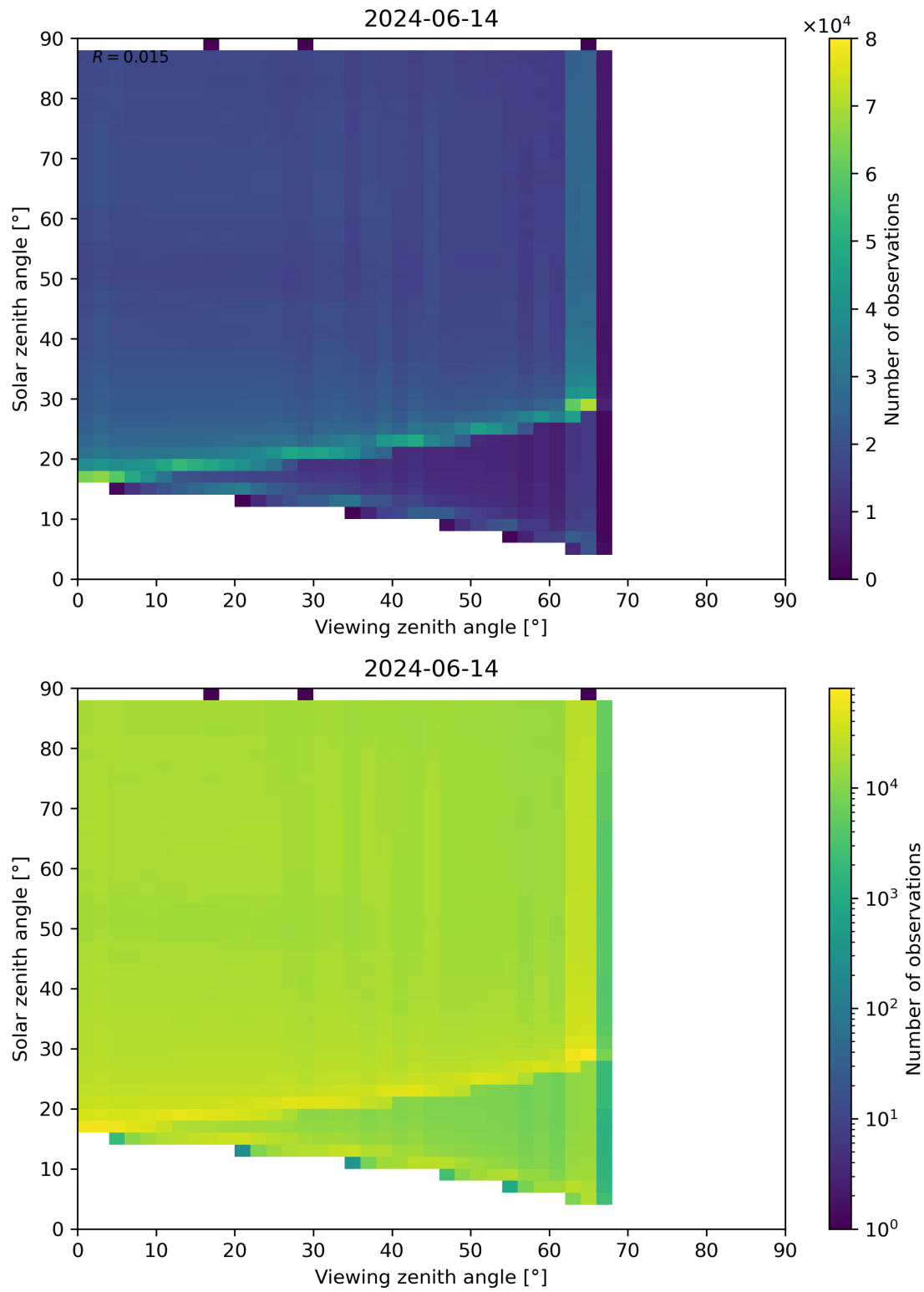
Figure 127: Scatter density plot of “Viewing zenith angle” against “Solar zenith angle” for 2024-06-13 to 2024-06-15.
