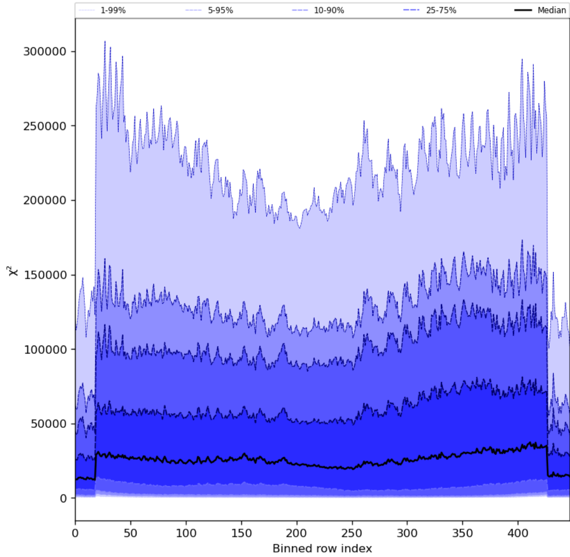
Figure 55: Along track statistics of “ \chi^2 ” for 2024-06-13 to 2024-06-15
