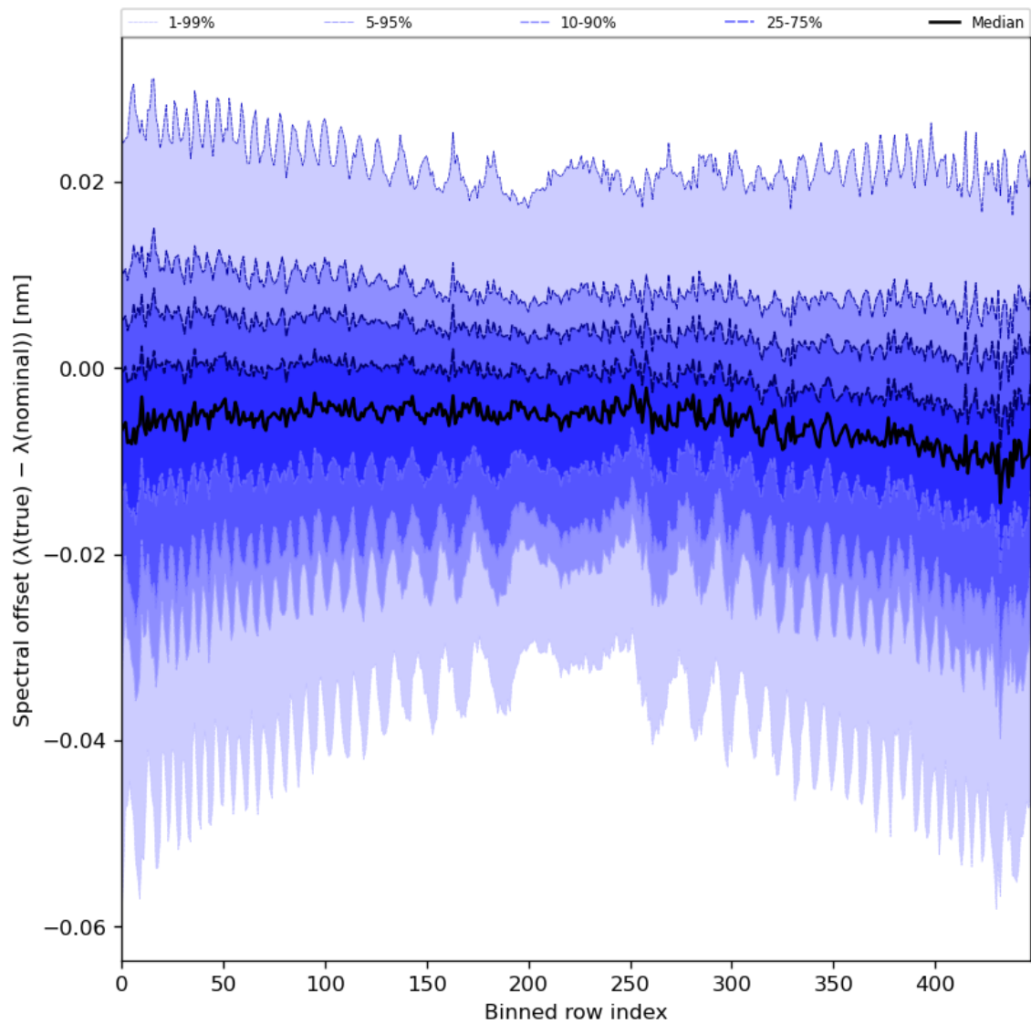
Figure 62: Along track statistics of “Spectral offset ( \lambda(\text{true}) - \lambda(\text{nominal}) )” for 2024-06-13 to 2024-06-15
