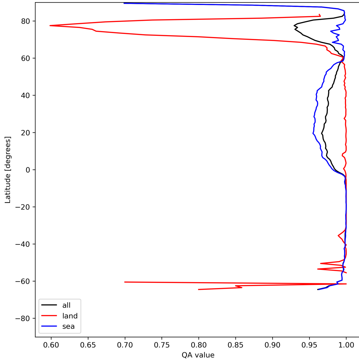
Figure 12: Zonal average of “QA value” for 2024-06-13 to 2024-06-15.
