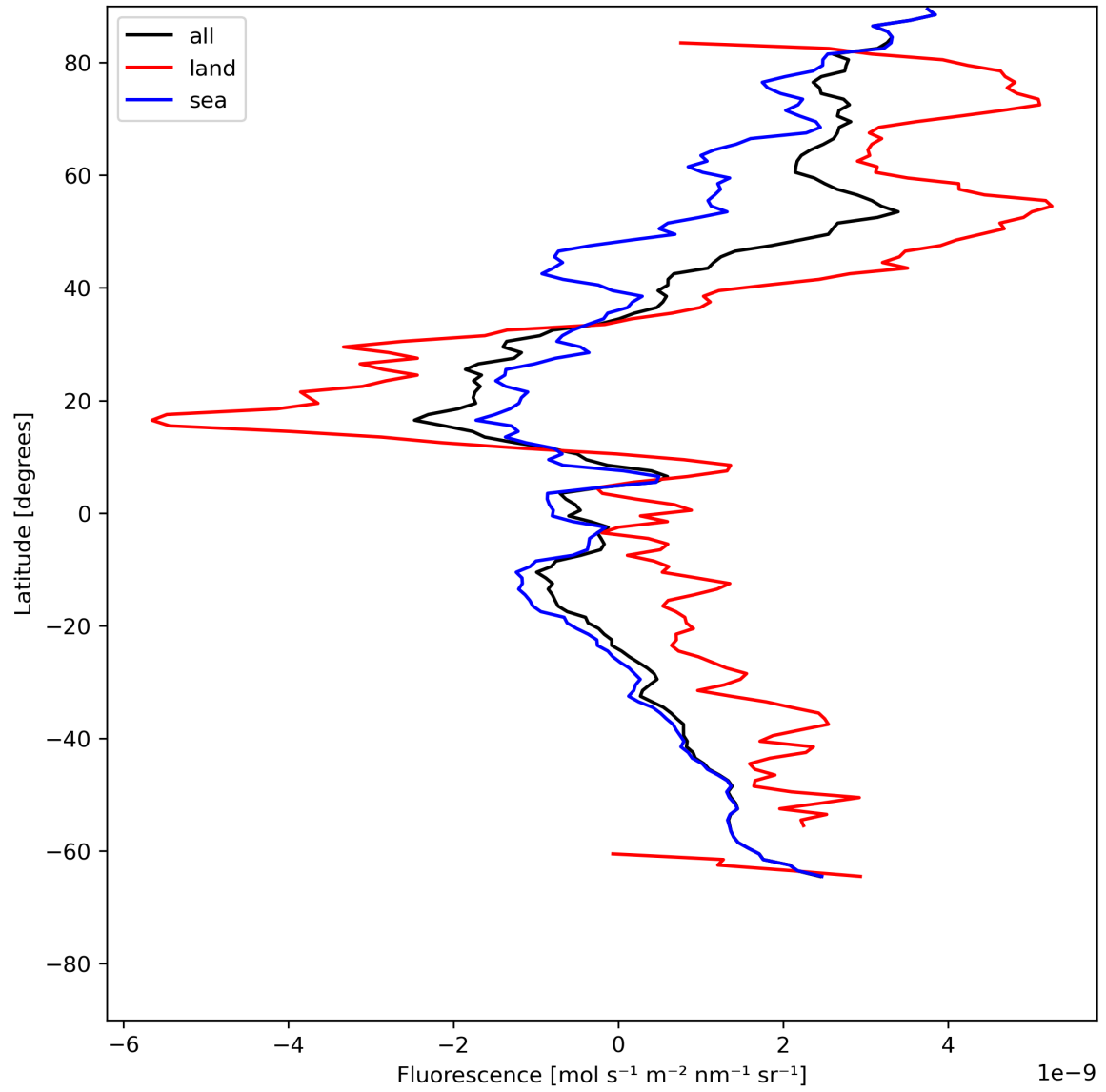
Figure 23: Zonal average of “Fluorescence” for 2024-06-13 to 2024-06-15.
