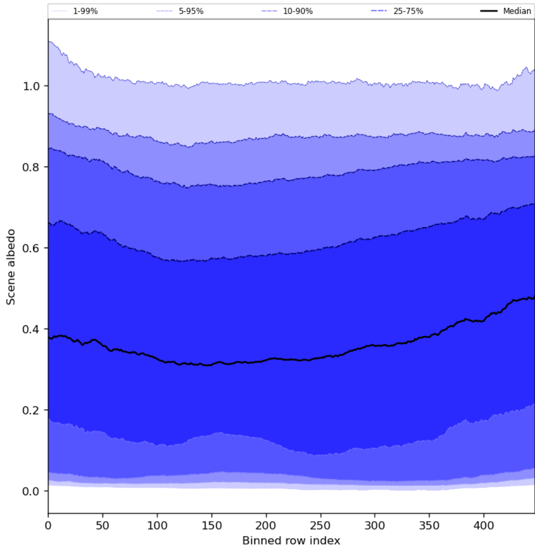
Figure 51: Along track statistics of “Scene albedo” for 2024-06-13 to 2024-06-15
