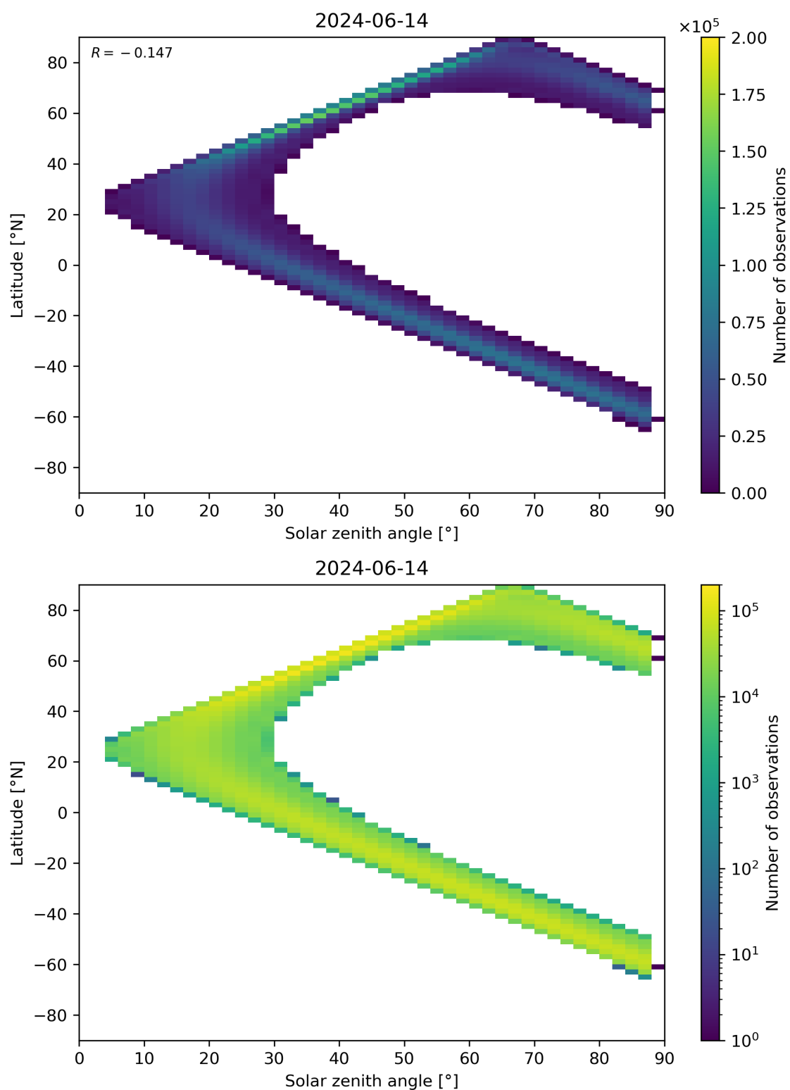
Figure 113: Scatter density plot of “Solar zenith angle” against “Latitude” for 2024-06-13 to 2024-06-15.
