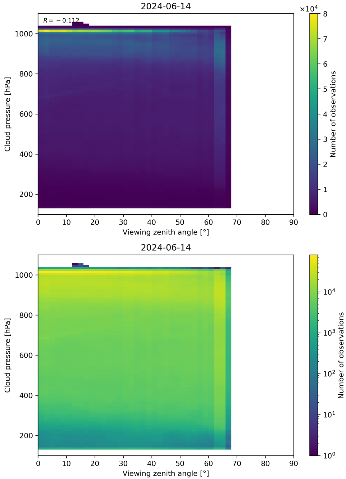
Figure 121: Scatter density plot of “Viewing zenith angle” against “Cloud pressure” for 2024-06-13 to 2024-06-15.
