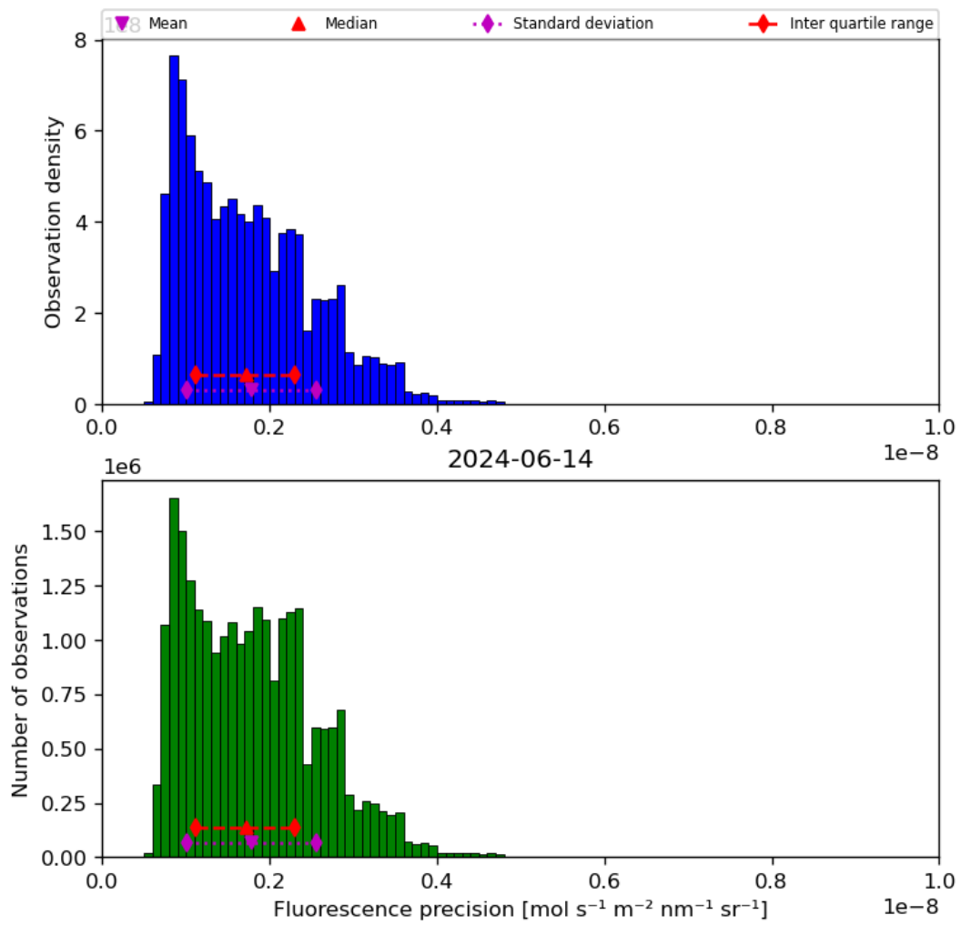
Figure 41: Histogram of “Fluorescence precision” for 2024-06-13 to 2024-06-15
