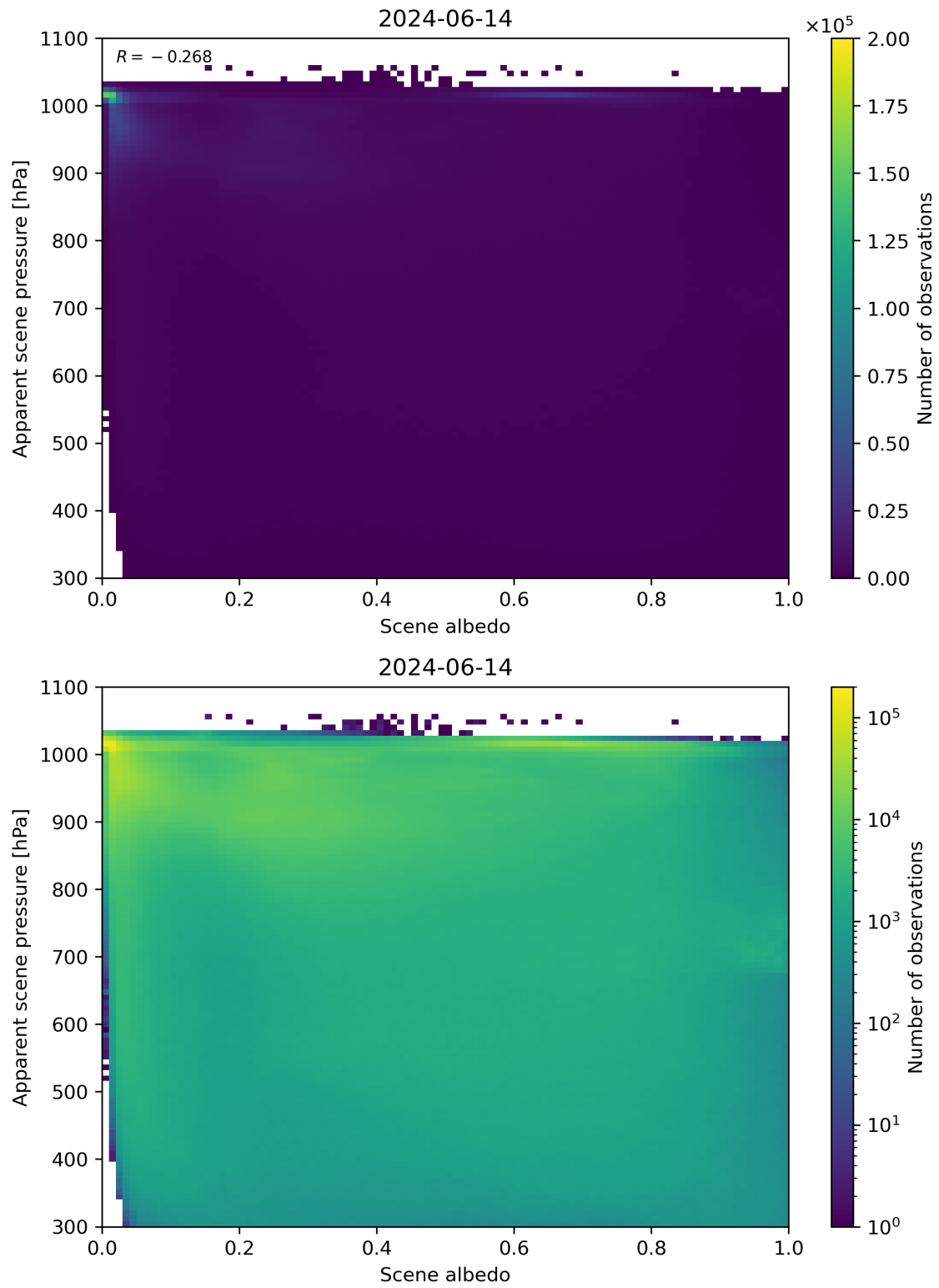
Figure 102: Scatter density plot of “Scene albedo” against “Apparent scene pressure” for 2024-06-13 to 2024-06-15.
