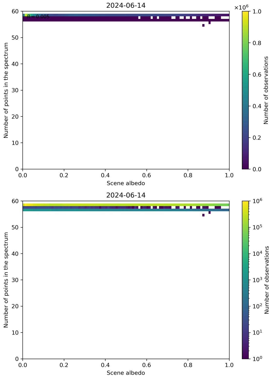
Figure 106: Scatter density plot of “Scene albedo” against “Number of points in the spectrum” for 2024-06-13 to 2024-06-15.
