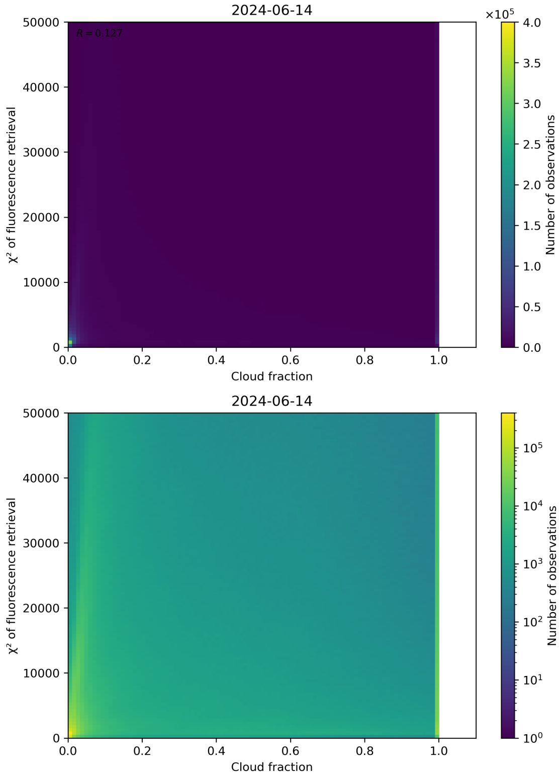
Figure 71: Scatter density plot of “Cloud fraction” against “ \chi^2 of fluorescence retrieval” for 2024-06-13 to 2024-06-15.
