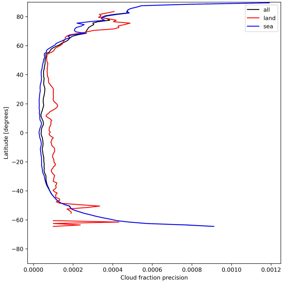
Figure 16: Zonal average of “Cloud fraction precision” for 2024-06-13 to 2024-06-15.
