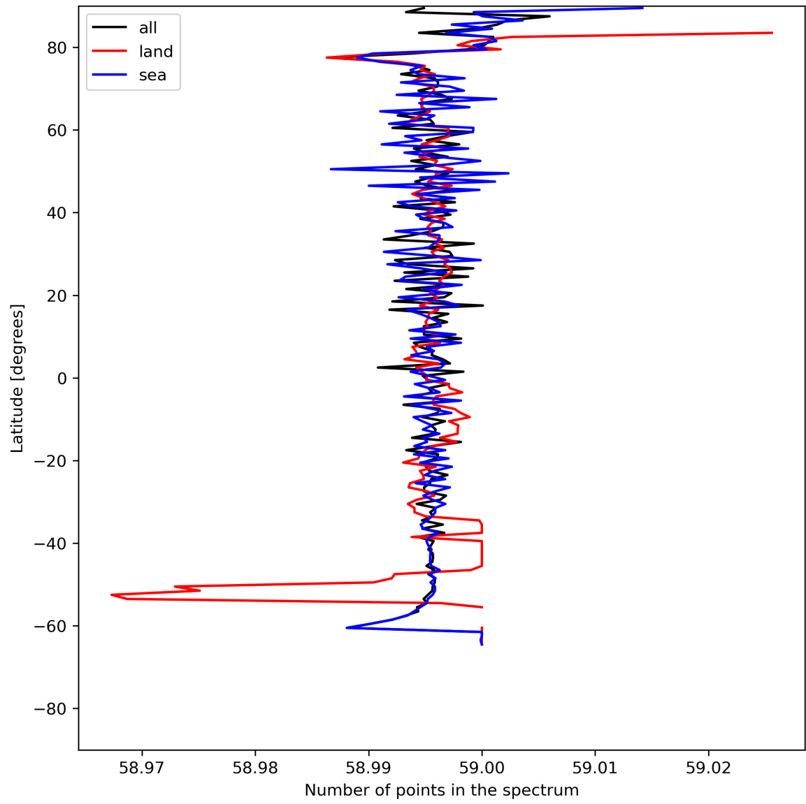
Figure 27: Zonal average of “Number of points in the spectrum” for 2024-06-13 to 2024-06-15.
