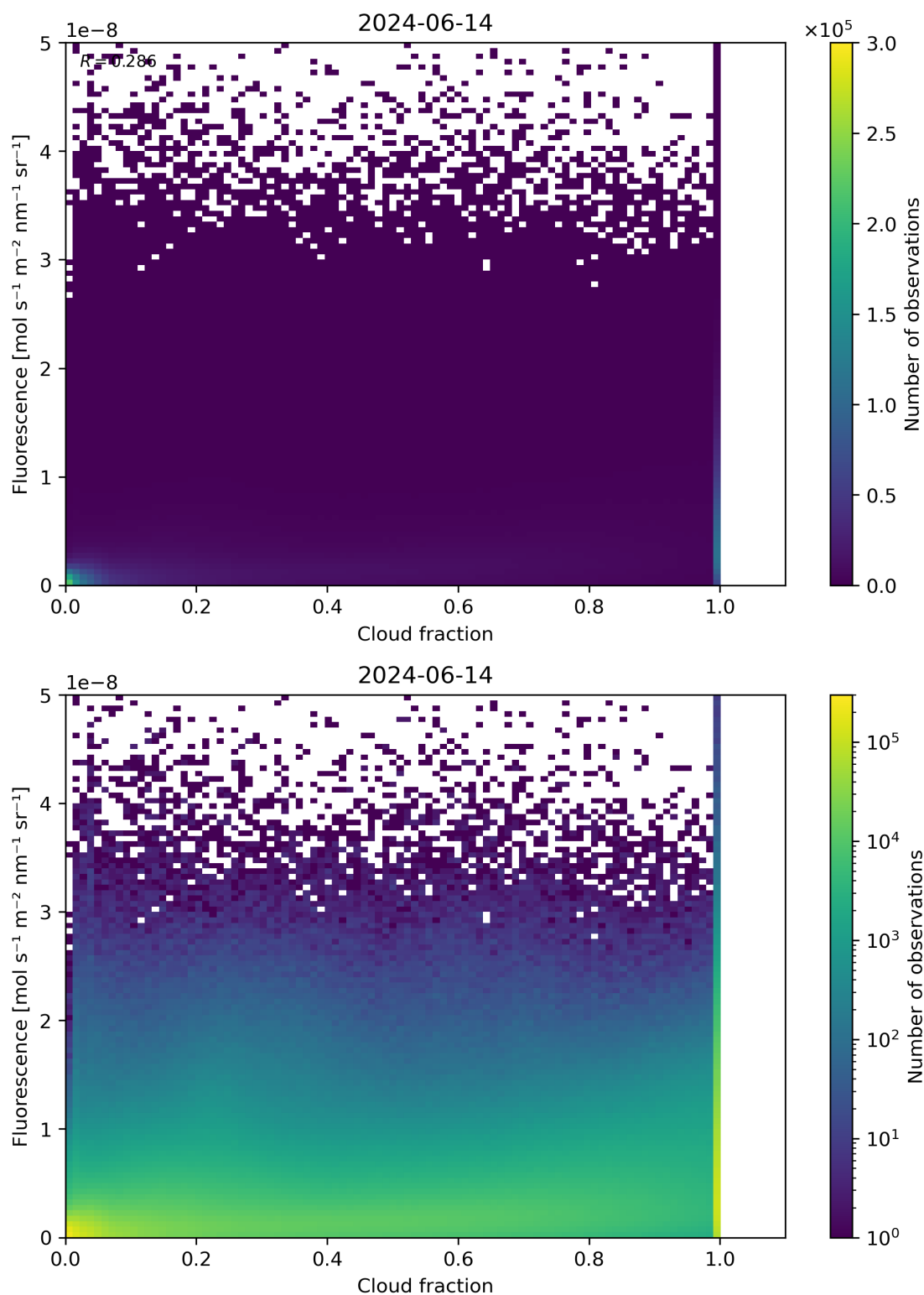
Figure 72: Scatter density plot of “Cloud fraction” against “Fluorescence” for 2024-06-13 to 2024-06-15.
