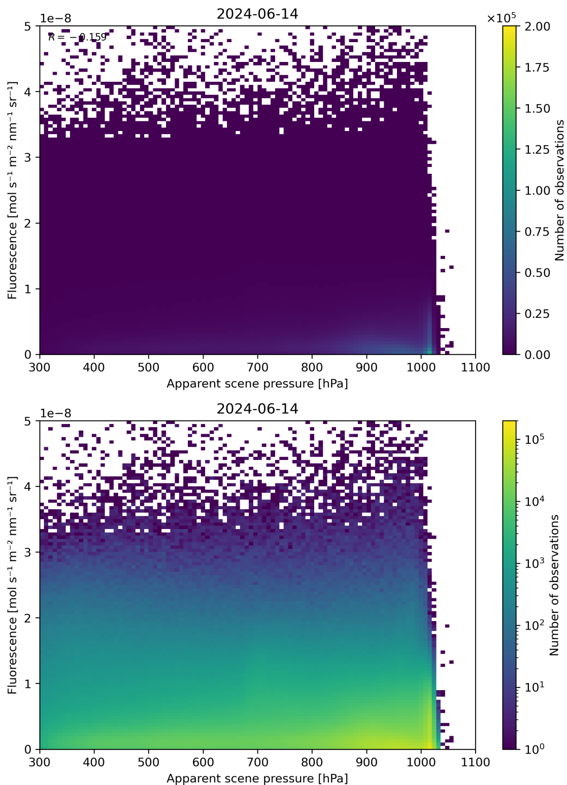
Figure 64: Scatter density plot of “Apparent scene pressure” against “Fluorescence” for 2024-06-13 to 2024-06-15.
