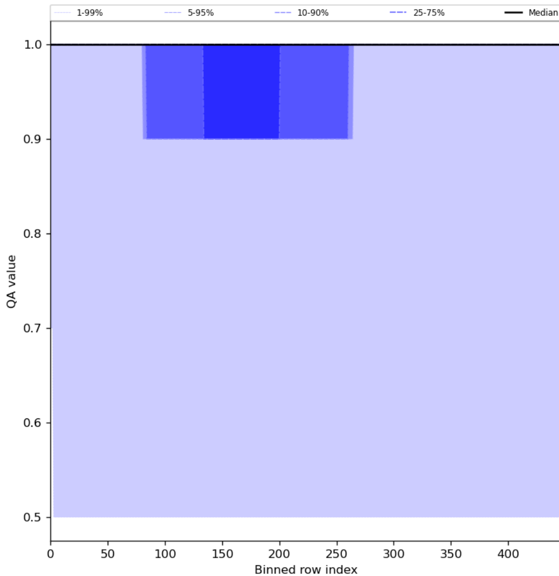
Figure 46: Along track statistics of “QA value” for 2024-06-13 to 2024-06-15
