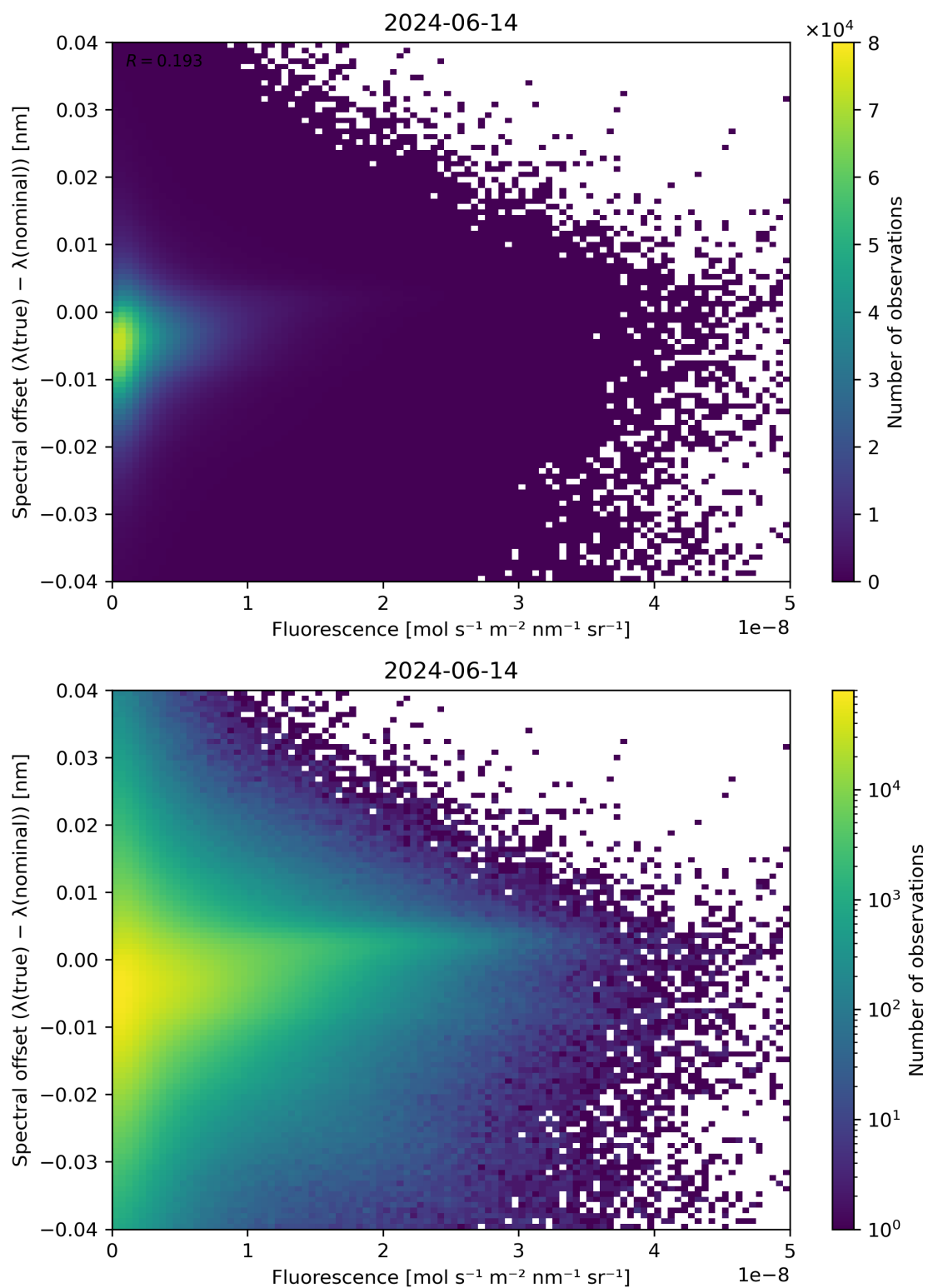
Figure 87: Scatter density plot of “Fluorescence” against “Spectral offset ( \lambda(\text{true}) - \lambda(\text{nominal}) )” for 2024-06-13 to 2024-06-15.
