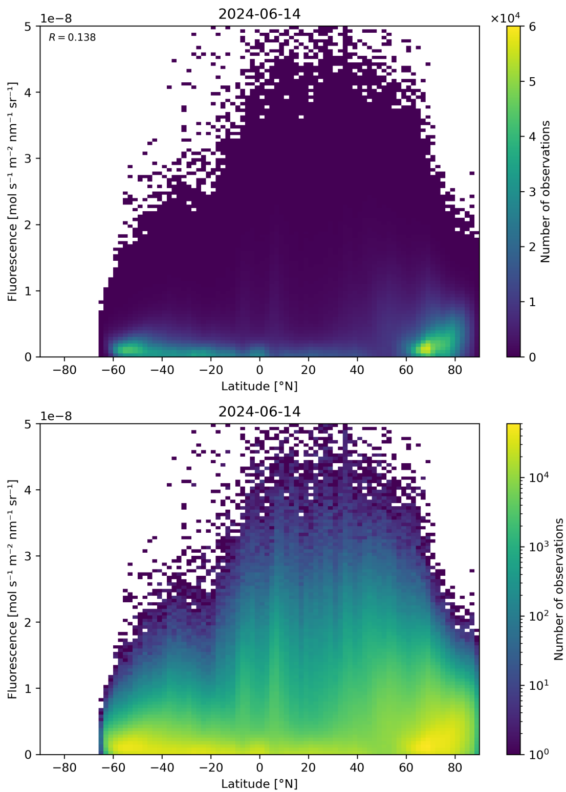
Figure 92: Scatter density plot of “Latitude” against “Fluorescence” for 2024-06-13 to 2024-06-15.
