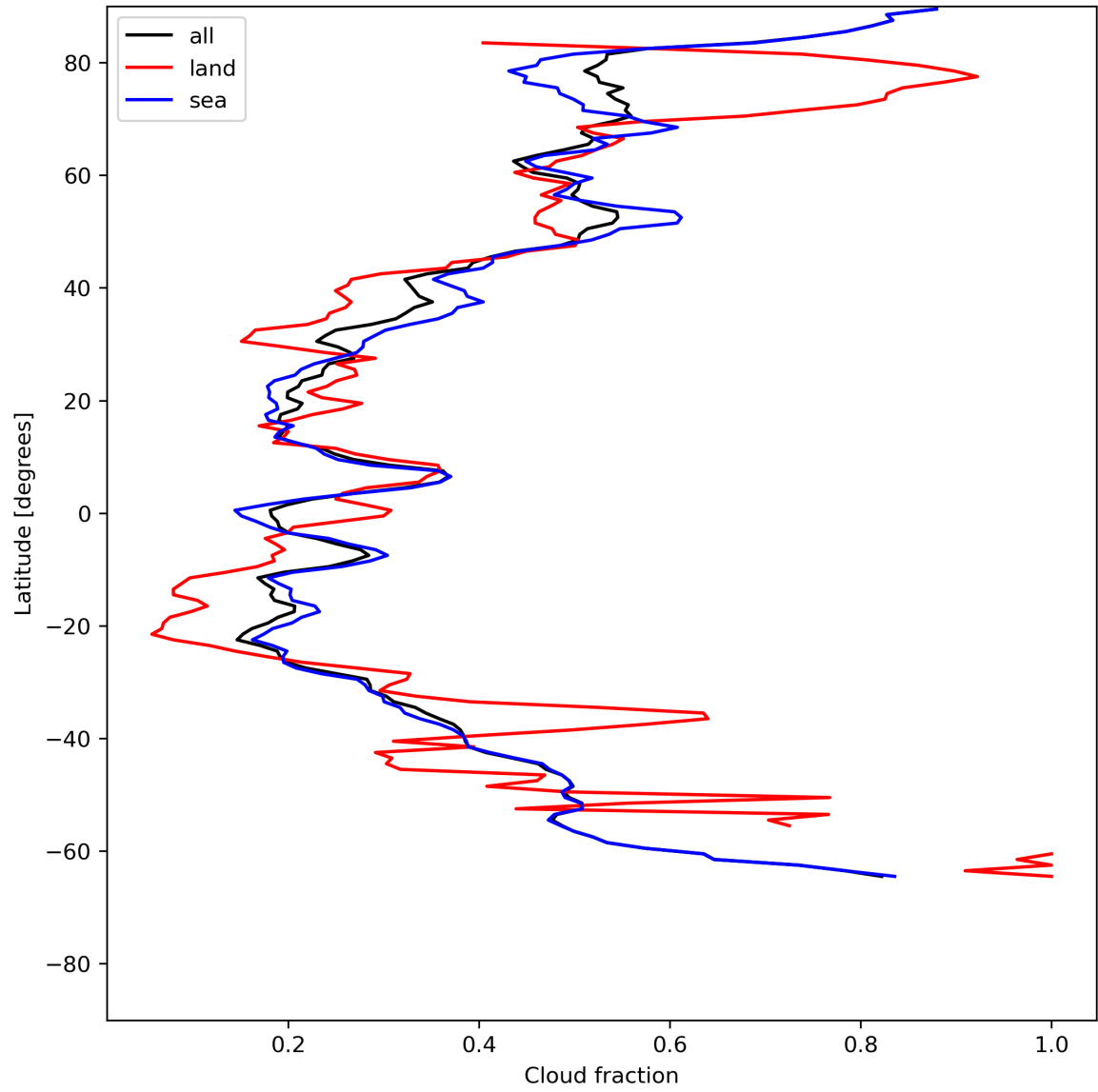
Figure 15: Zonal average of “Cloud fraction” for 2024-06-13 to 2024-06-15.
