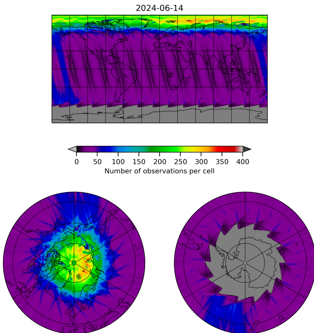
Figure 11: Map of the number of observations for 2024-06-13 to 2024-06-15
