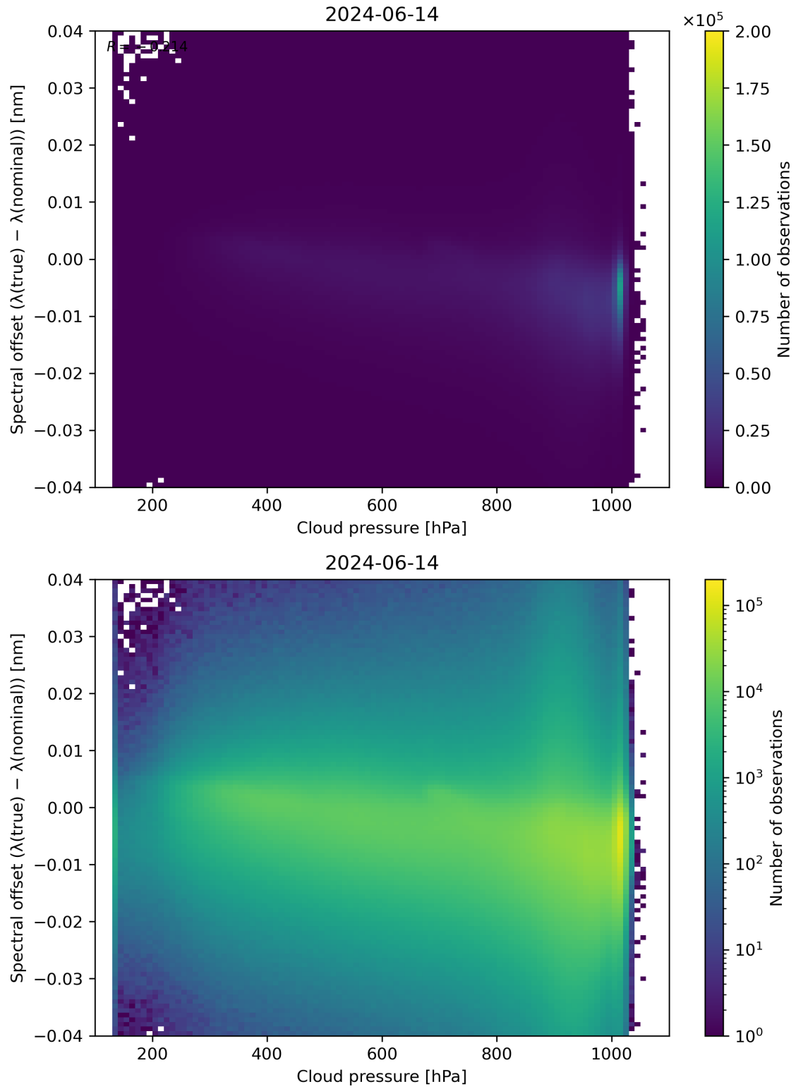
Figure 84: Scatter density plot of “Cloud pressure” against “Spectral offset ( \lambda(\text{true}) - \lambda(\text{nominal}) )” for 2024-06-13 to 2024-06-15.
