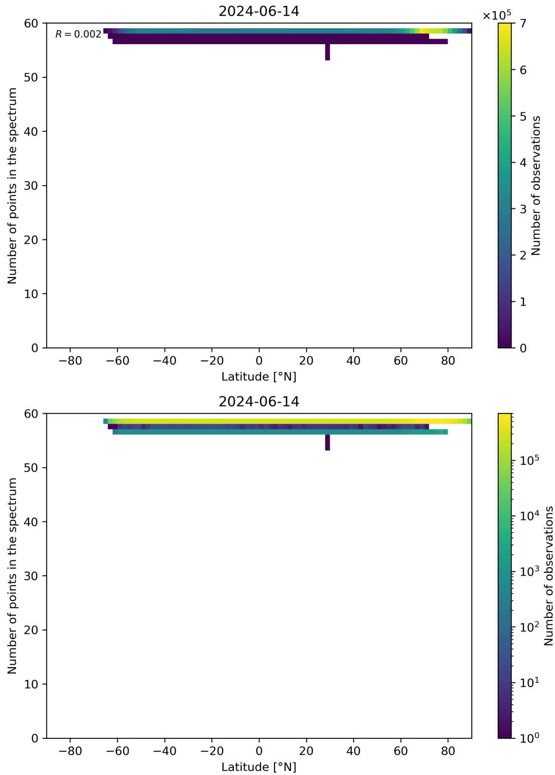
Figure 94: Scatter density plot of “Latitude” against “Number of points in the spectrum” for 2024-06-13 to 2024-06-15.
