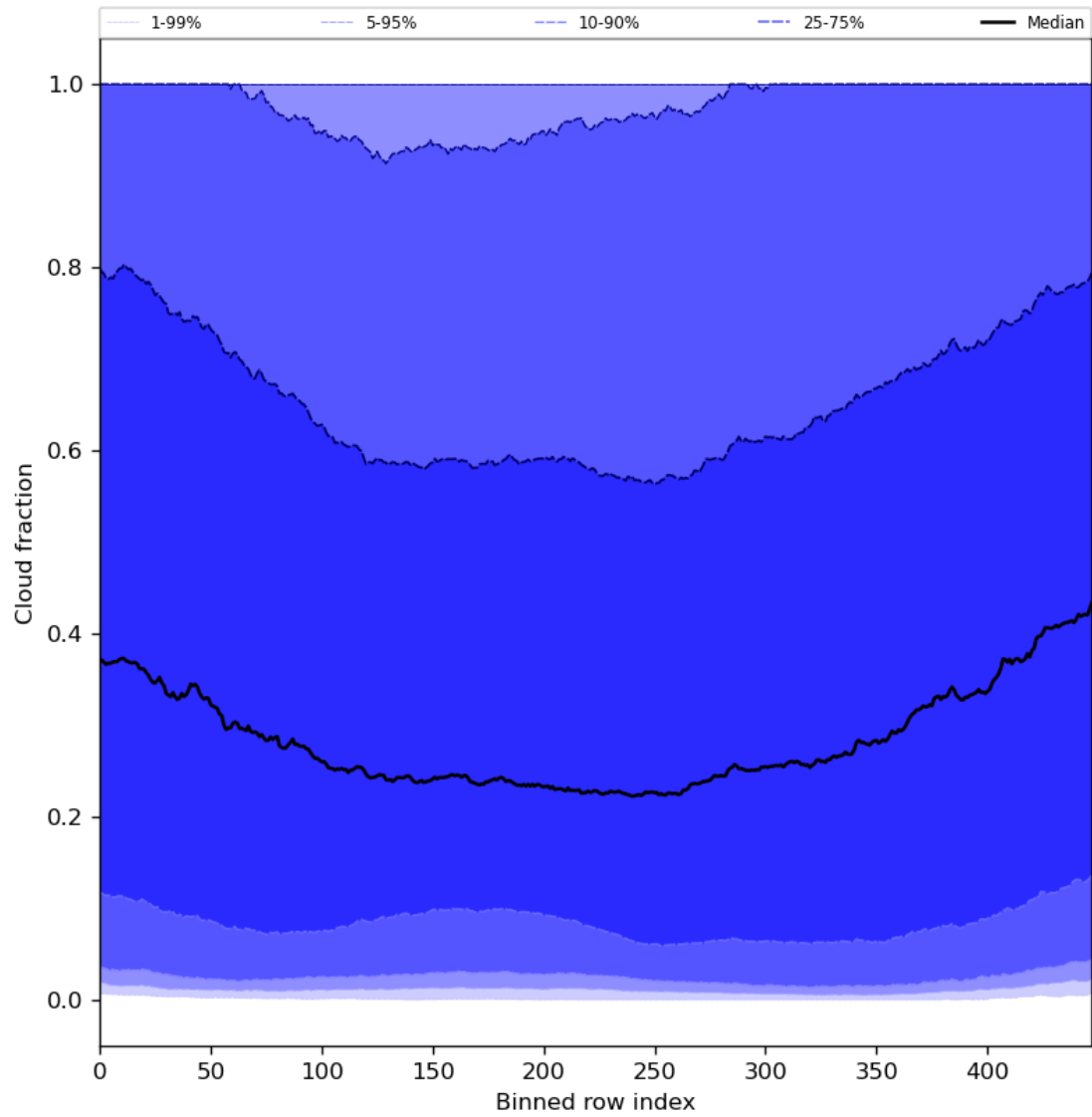
Figure 49: Along track statistics of “Cloud fraction” for 2024-06-13 to 2024-06-15
