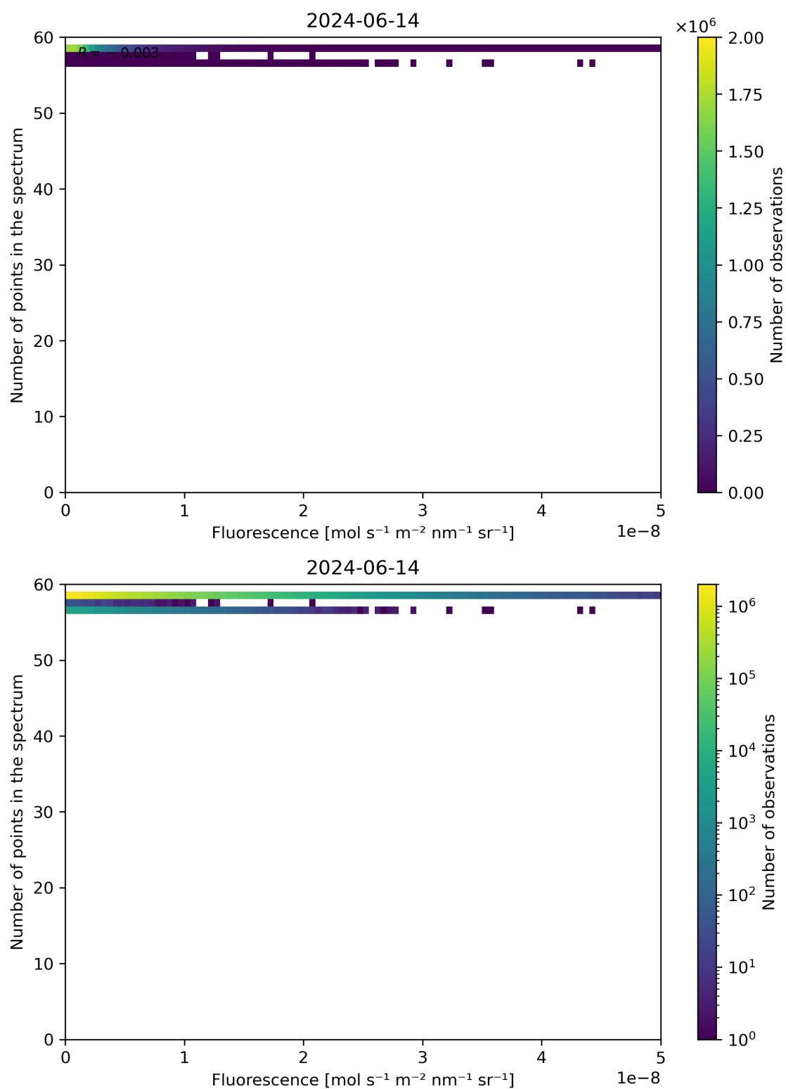
Figure 86: Scatter density plot of “Fluorescence” against “Number of points in the spectrum” for 2024-06-13 to 2024-06-15.
