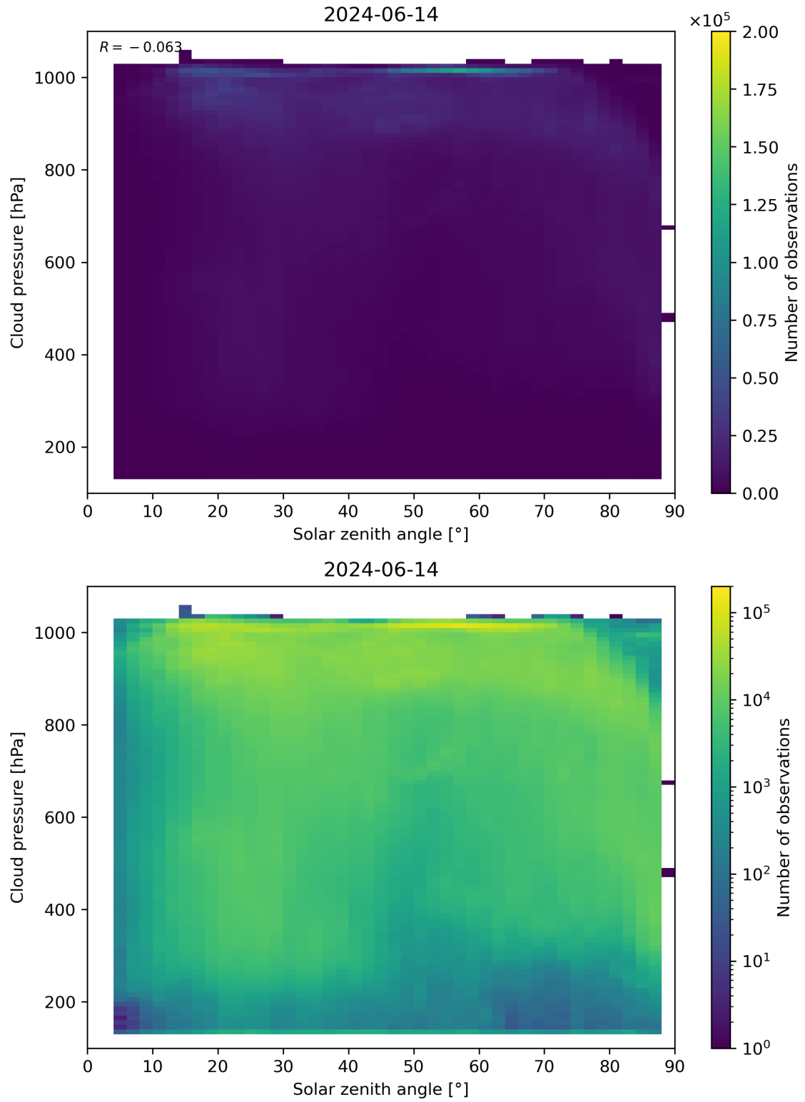
Figure 111: Scatter density plot of “Solar zenith angle” against “Cloud pressure” for 2024-06-13 to 2024-06-15.
