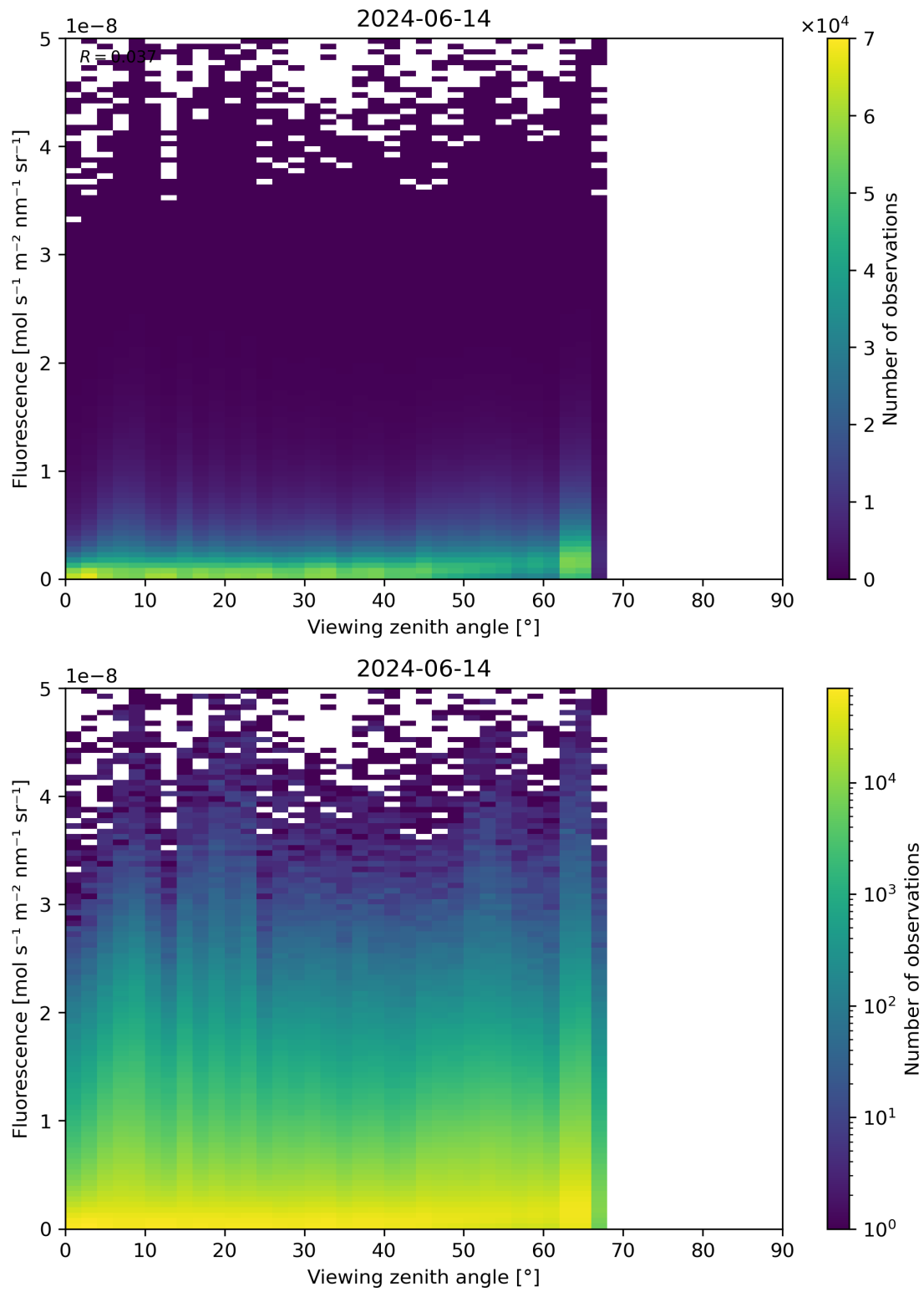
Figure 122: Scatter density plot of “Viewing zenith angle” against “Fluorescence” for 2024-06-13 to 2024-06-15.
