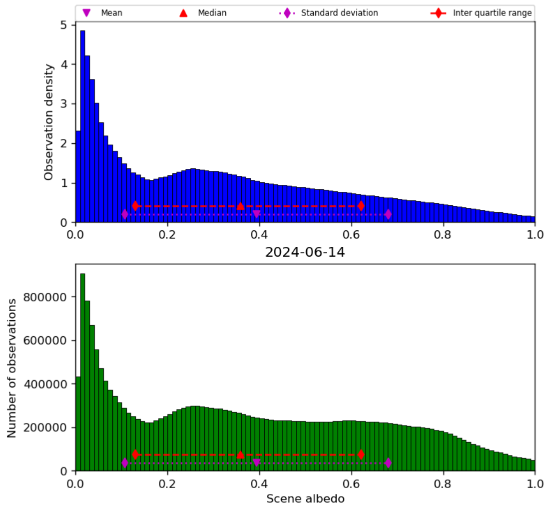
Figure 34: Histogram of “Scene albedo” for 2024-06-13 to 2024-06-15
