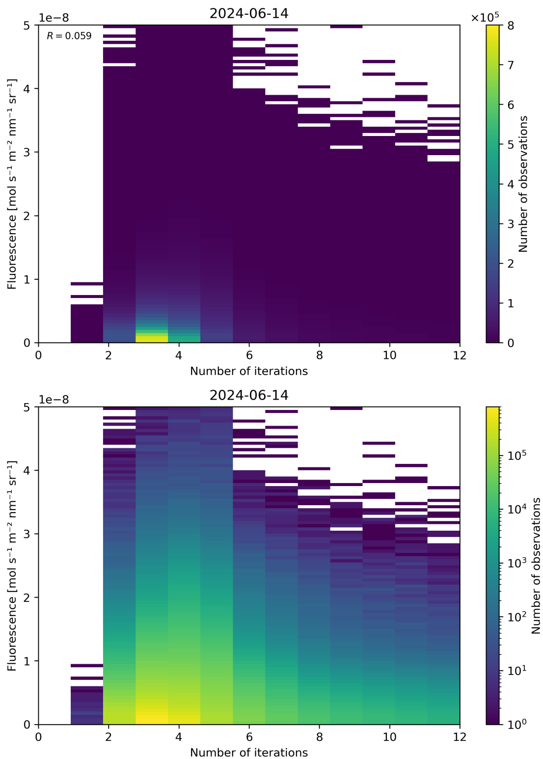
Figure 98: Scatter density plot of “Number of iterations” against “Fluorescence” for 2024-06-13 to 2024-06-15.
