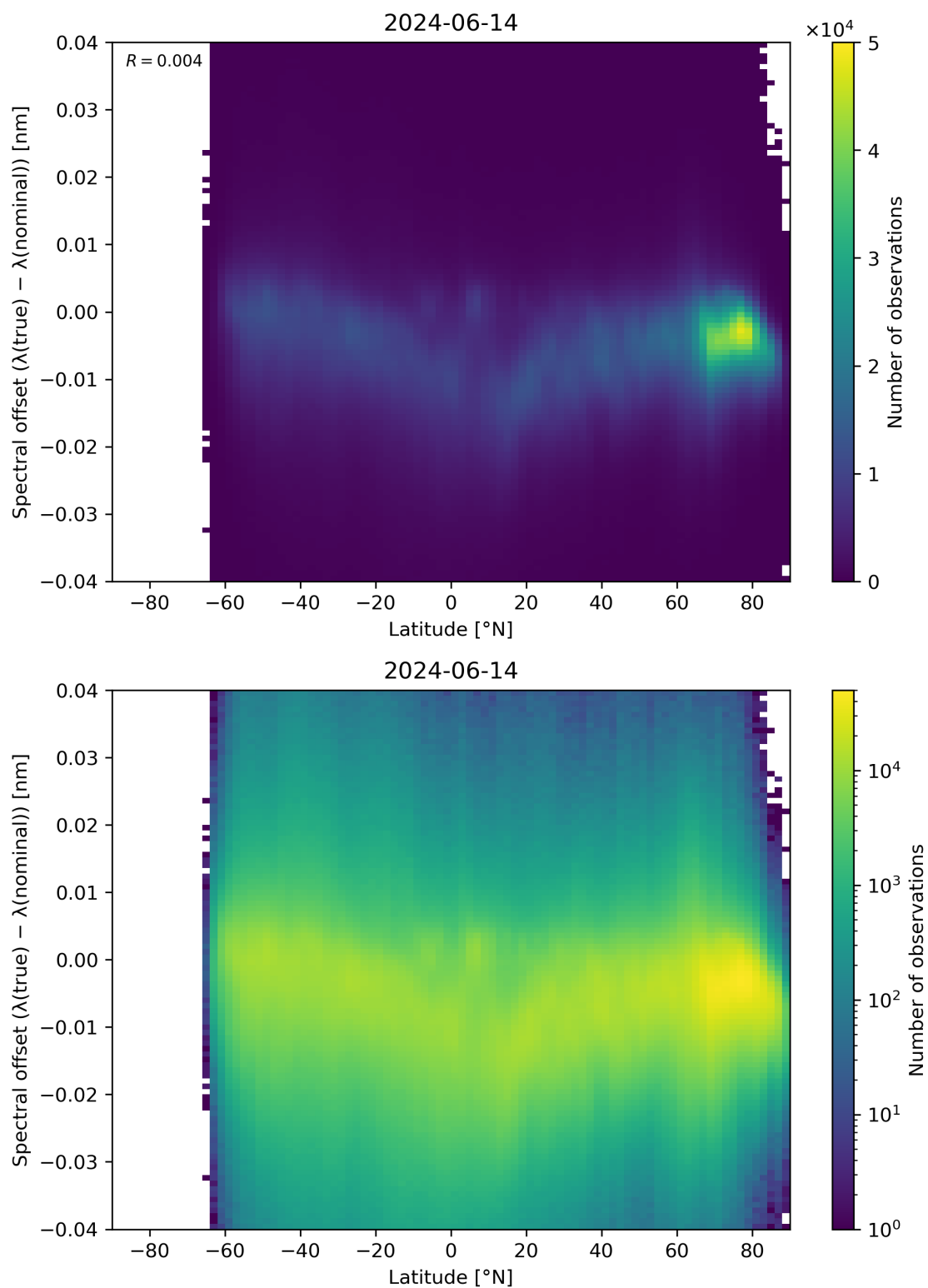
Figure 96: Scatter density plot of “Latitude” against “Spectral offset ( \lambda(\text{true}) - \lambda(\text{nominal}) )” for 2024-06-13 to 2024-06-15.
