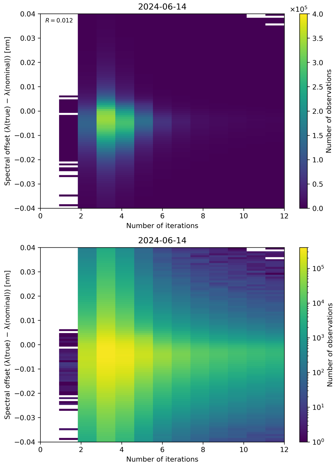
Figure 100: Scatter density plot of “Number of iterations” against “Spectral offset ( \lambda(\text{true}) - \lambda(\text{nominal}) )” for 2024-06-13 to 2024-06-15.
