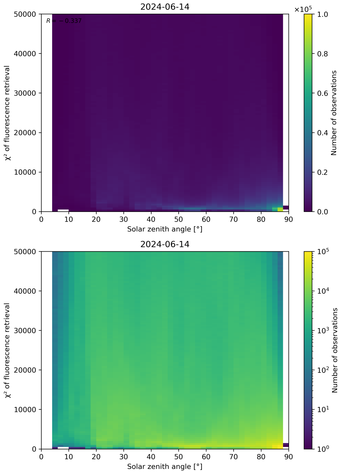
Figure 109: Scatter density plot of “Solar zenith angle” against “ \chi^2 of fluorescence retrieval” for 2024-06-13 to 2024-06-15.
