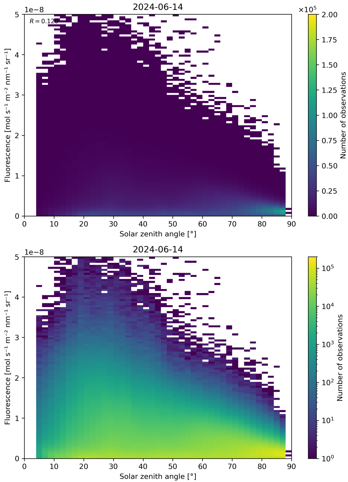
Figure 112: Scatter density plot of “Solar zenith angle” against “Fluorescence” for 2024-06-13 to 2024-06-15.
