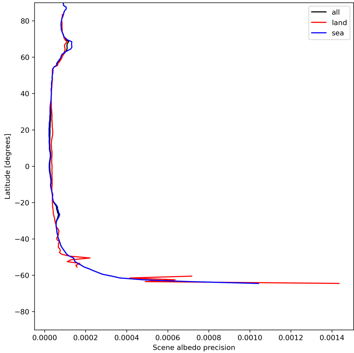
Figure 18: Zonal average of “Scene albedo precision” for 2024-06-13 to 2024-06-15.
