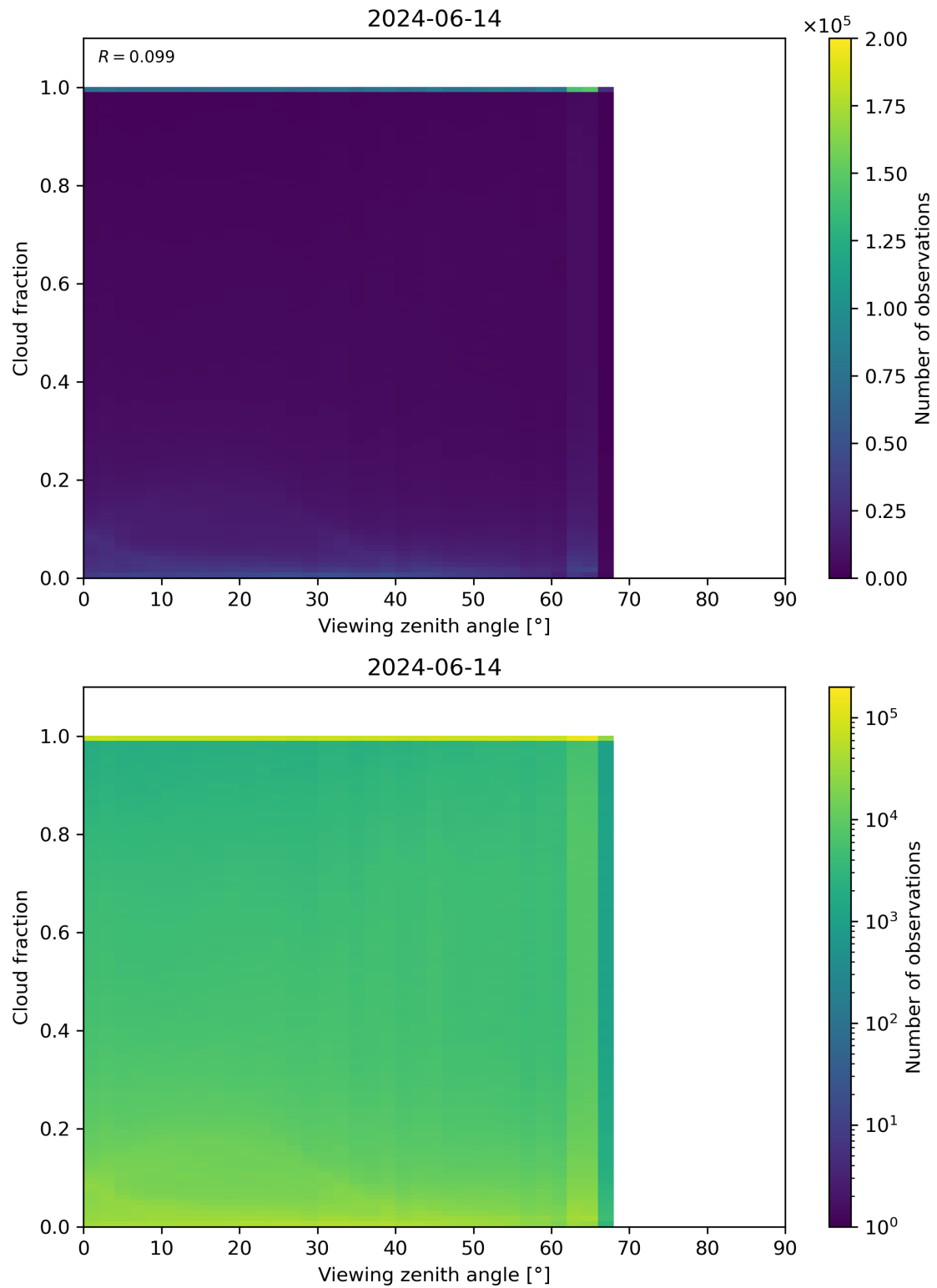
Figure 120: Scatter density plot of “Viewing zenith angle” against “Cloud fraction” for 2024-06-13 to 2024-06-15.
