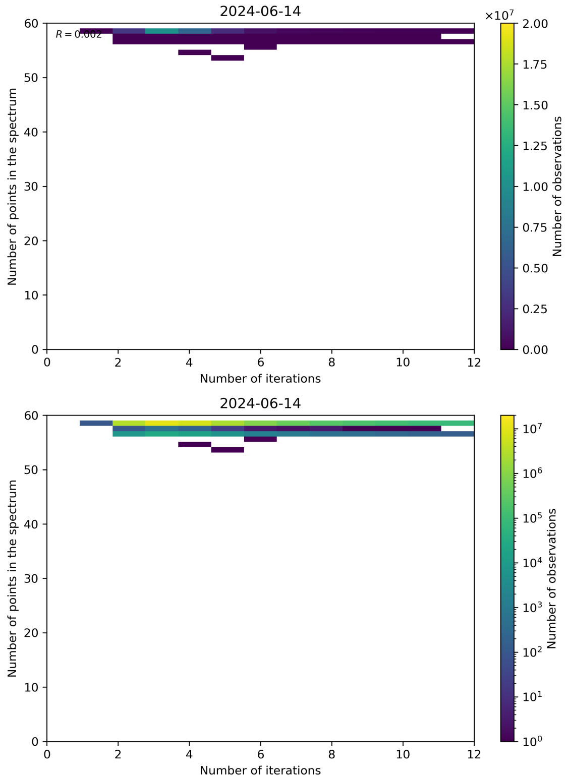
Figure 99: Scatter density plot of “Number of iterations” against “Number of points in the spectrum” for 2024-06-13 to 2024-06-15.
