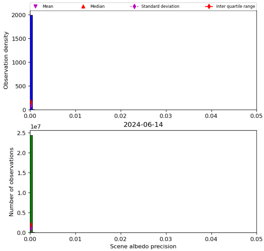
Figure 35: Histogram of “Scene albedo precision” for 2024-06-13 to 2024-06-15
