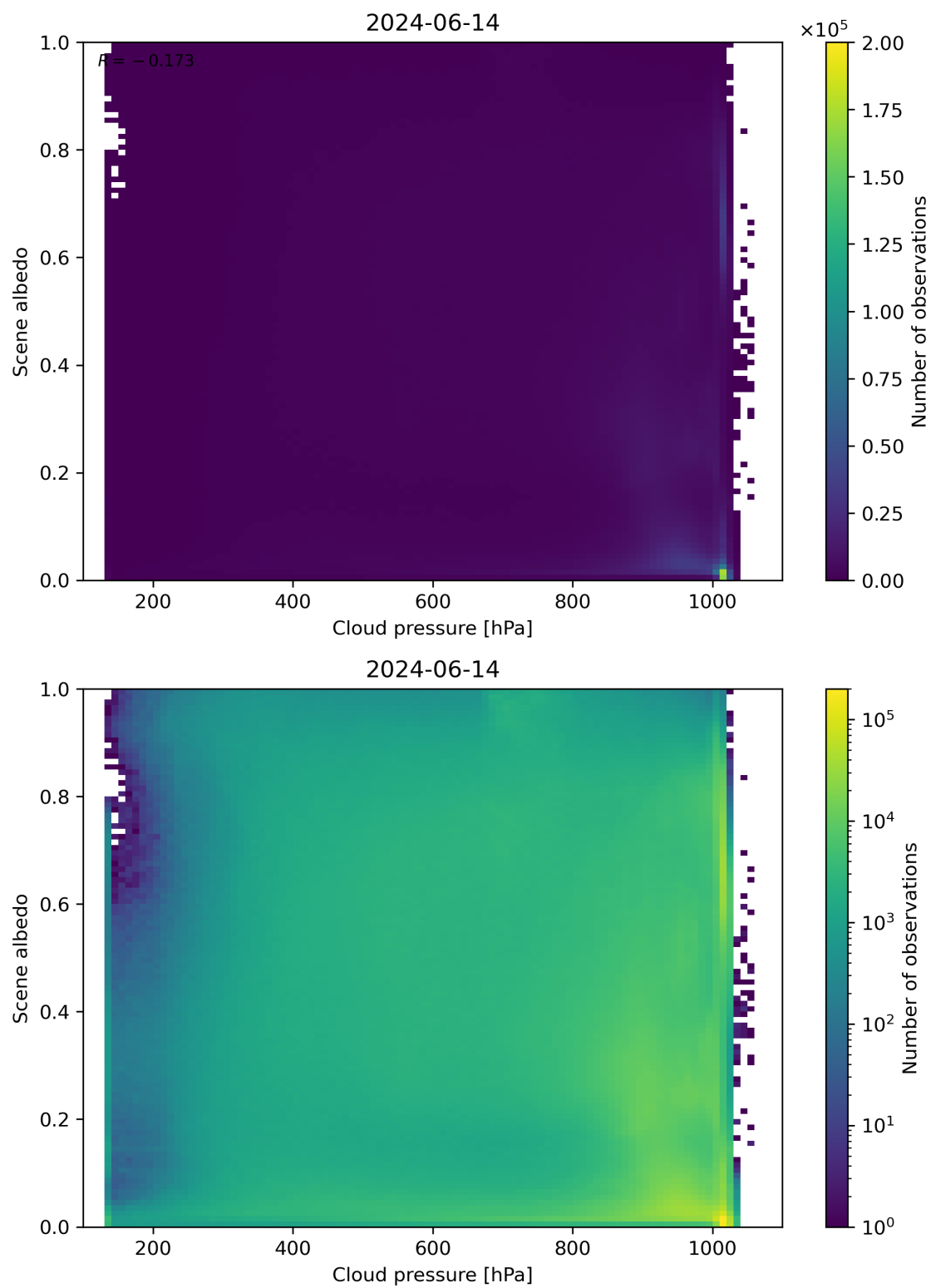
Figure 83: Scatter density plot of “Cloud pressure” against “Scene albedo” for 2024-06-13 to 2024-06-15.
