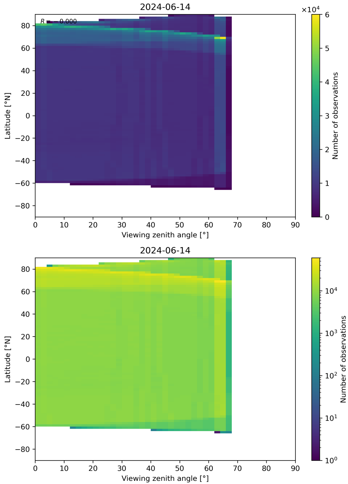
Figure 123: Scatter density plot of “Viewing zenith angle” against “Latitude” for 2024-06-13 to 2024-06-15.
