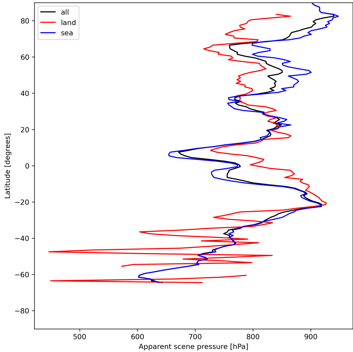
Figure 19: Zonal average of “Apparent scene pressure” for 2024-06-13 to 2024-06-15.
