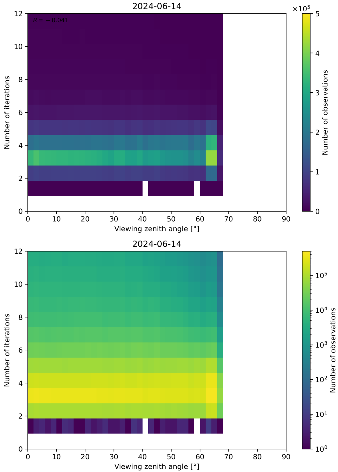
Figure 124: Scatter density plot of “Viewing zenith angle” against “Number of iterations” for 2024-06-13 to 2024-06-15.
