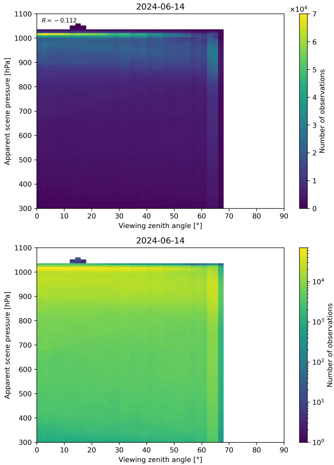
Figure 118: Scatter density plot of “Viewing zenith angle” against “Apparent scene pressure” for 2024-06-13 to 2024-06-15.
