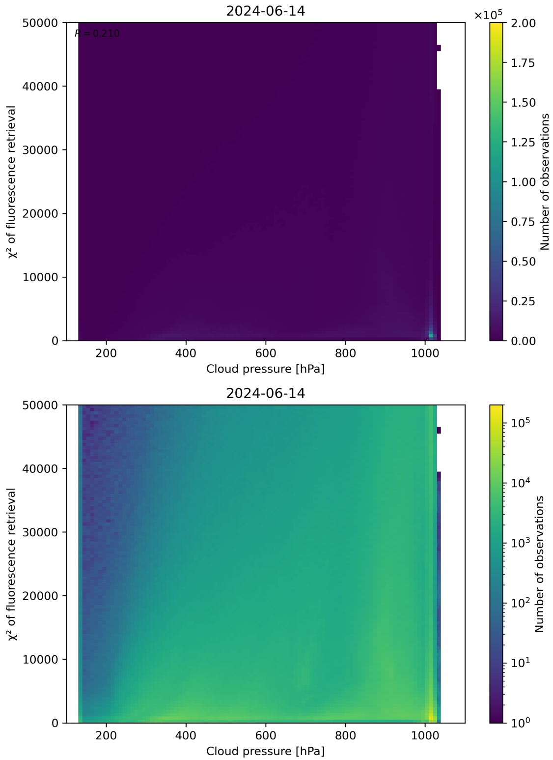
Figure 78: Scatter density plot of “Cloud pressure” against “ \chi^2 of fluorescence retrieval” for 2024-06-13 to 2024-06-15.
