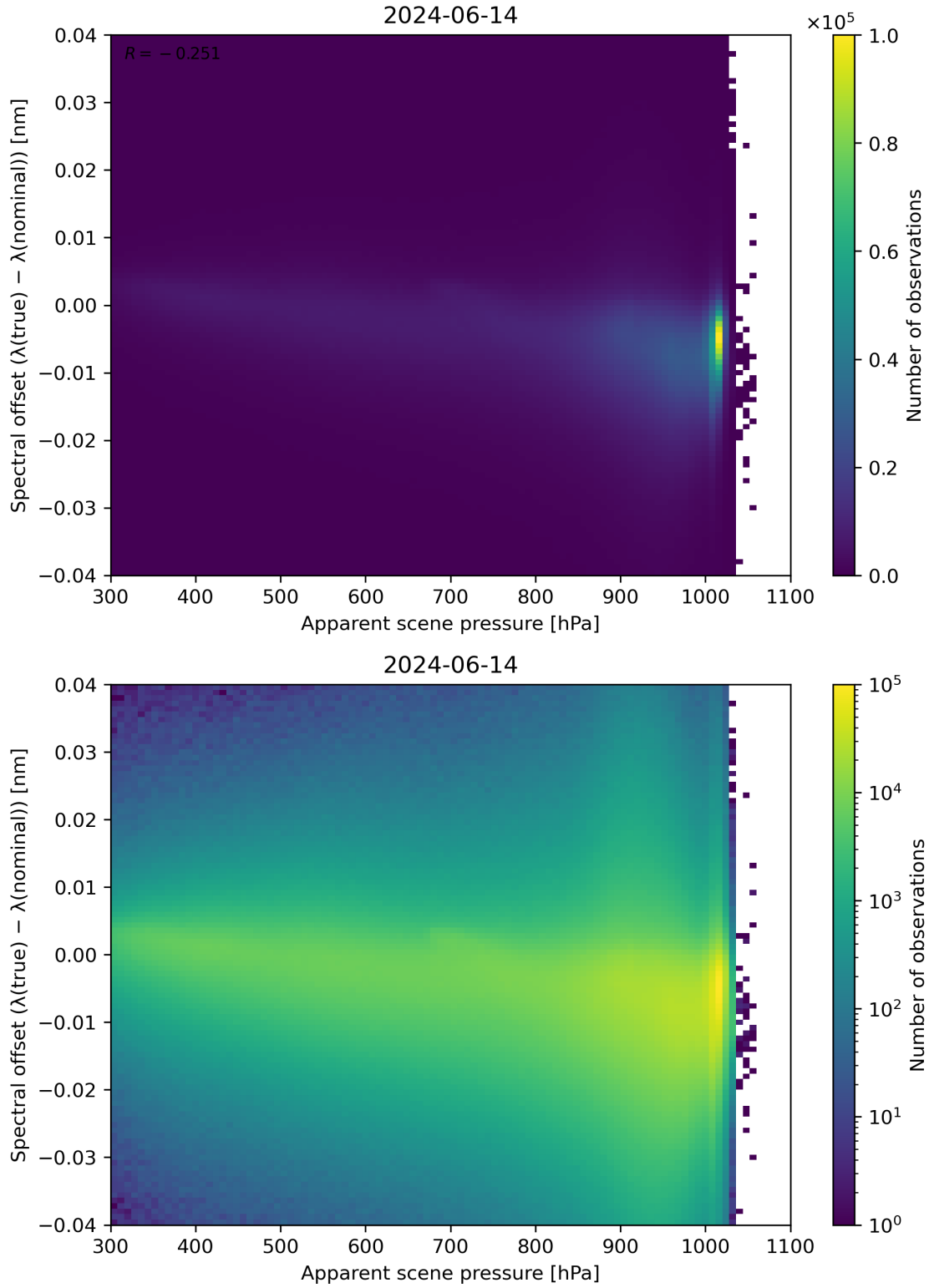
Figure 67: Scatter density plot of “Apparent scene pressure” against “Spectral offset ( \lambda(\text{true}) - \lambda(\text{nominal}) )” for 2024-06-13 to 2024-06-15.
