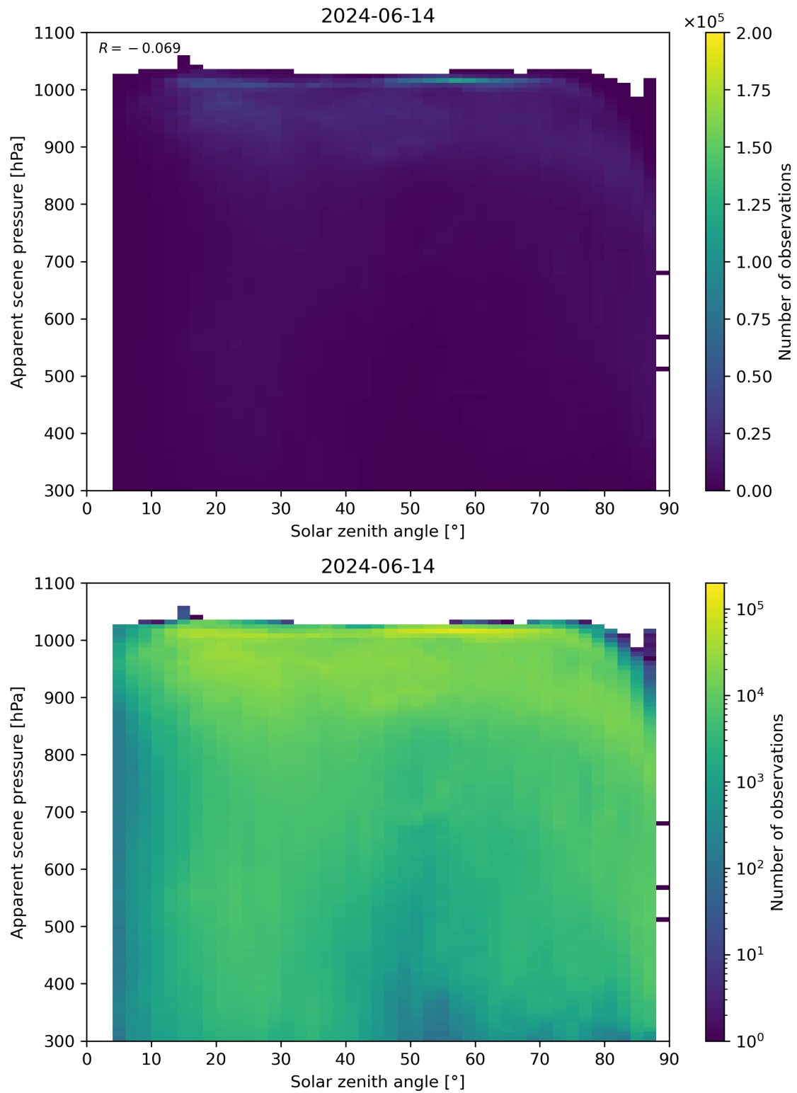
Figure 108: Scatter density plot of “Solar zenith angle” against “Apparent scene pressure” for 2024-06-13 to 2024-06-15.
