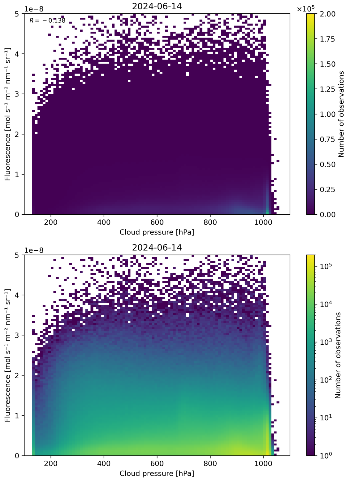
Figure 80: Scatter density plot of “Cloud pressure” against “Fluorescence” for 2024-06-13 to 2024-06-15.
