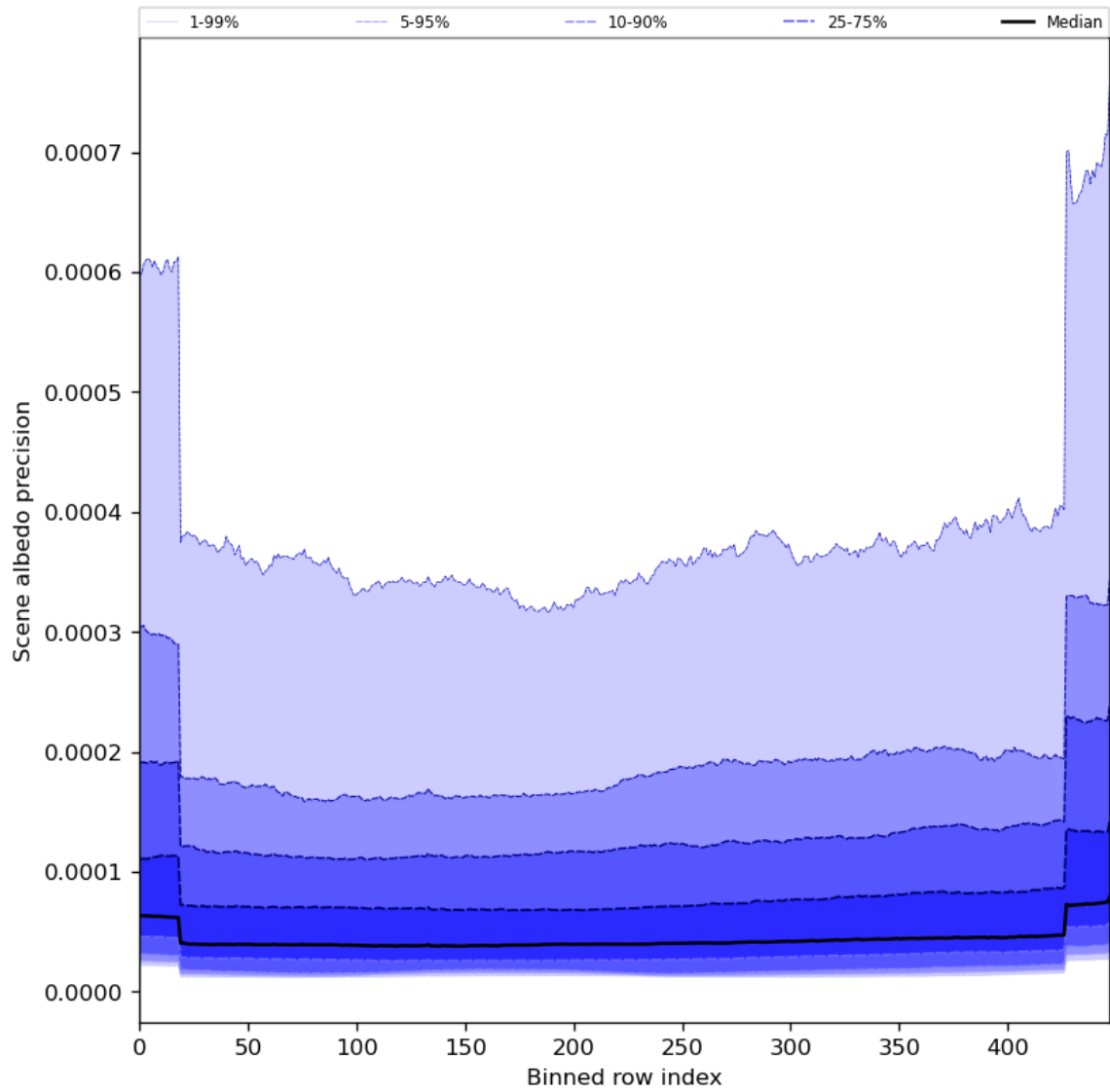
Figure 52: Along track statistics of “Scene albedo precision” for 2024-06-13 to 2024-06-15
