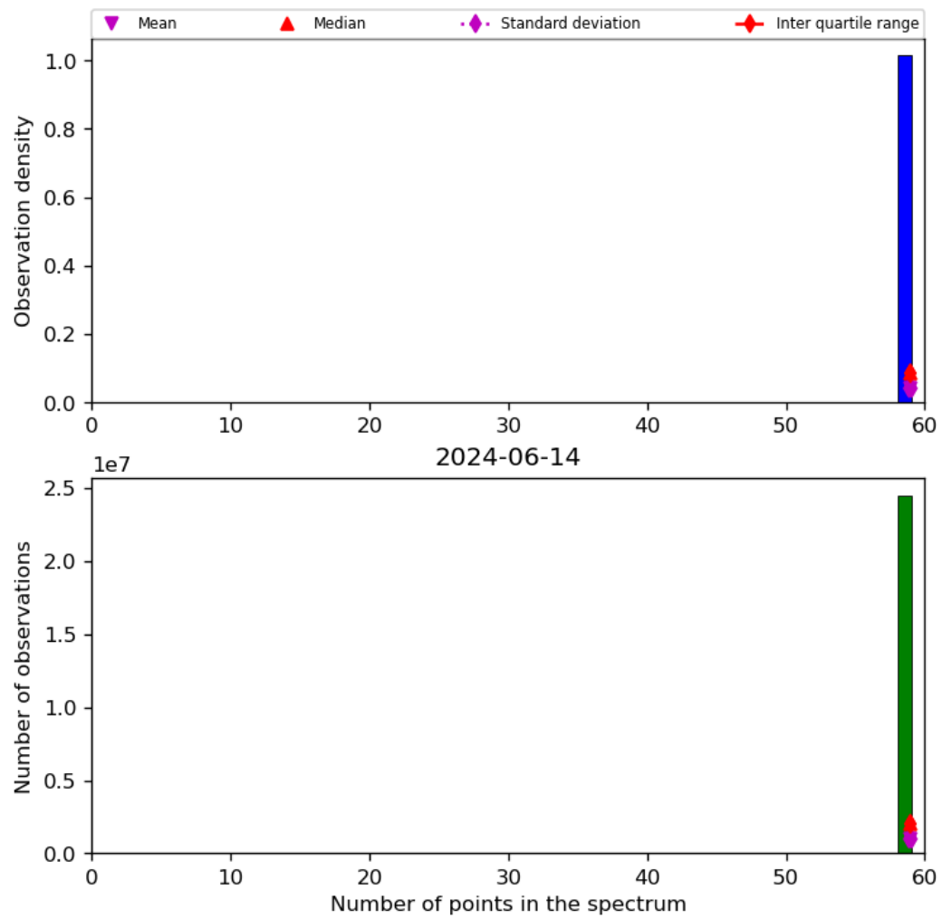
Figure 44: Histogram of “Number of points in the spectrum” for 2024-06-13 to 2024-06-15
