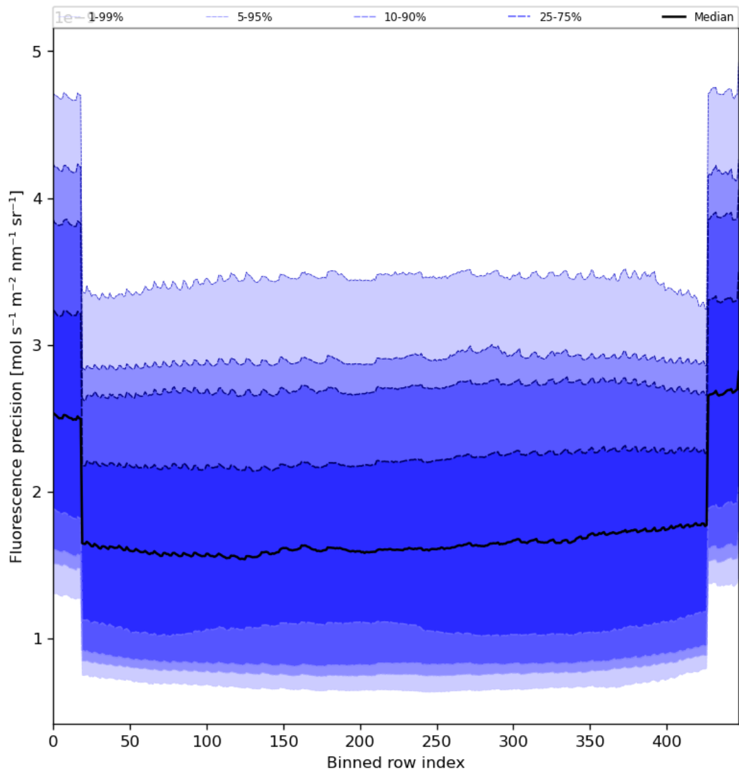
Figure 58: Along track statistics of “Fluorescence precision” for 2024-06-14 to 2024-06-16
