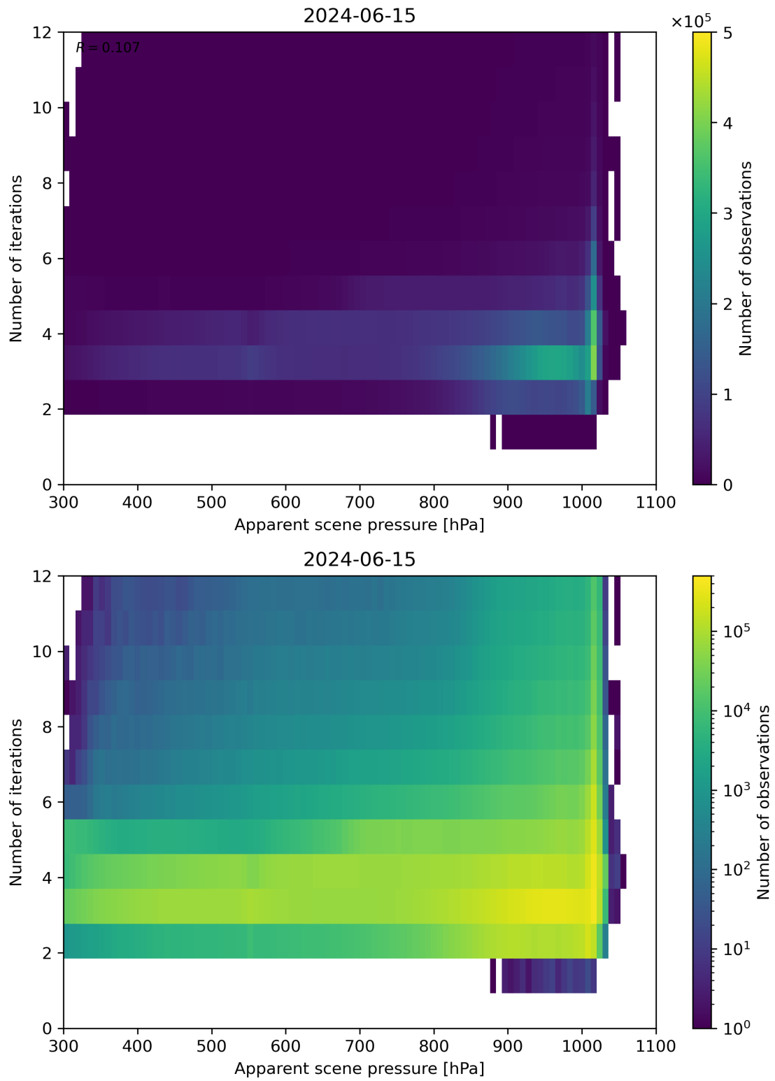
Figure 65: Scatter density plot of “Apparent scene pressure” against “Number of iterations” for 2024-06-14 to 2024-06-16.
