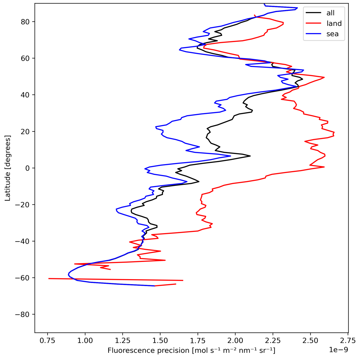
Figure 24: Zonal average of “Fluorescence precision” for 2024-06-14 to 2024-06-16.
