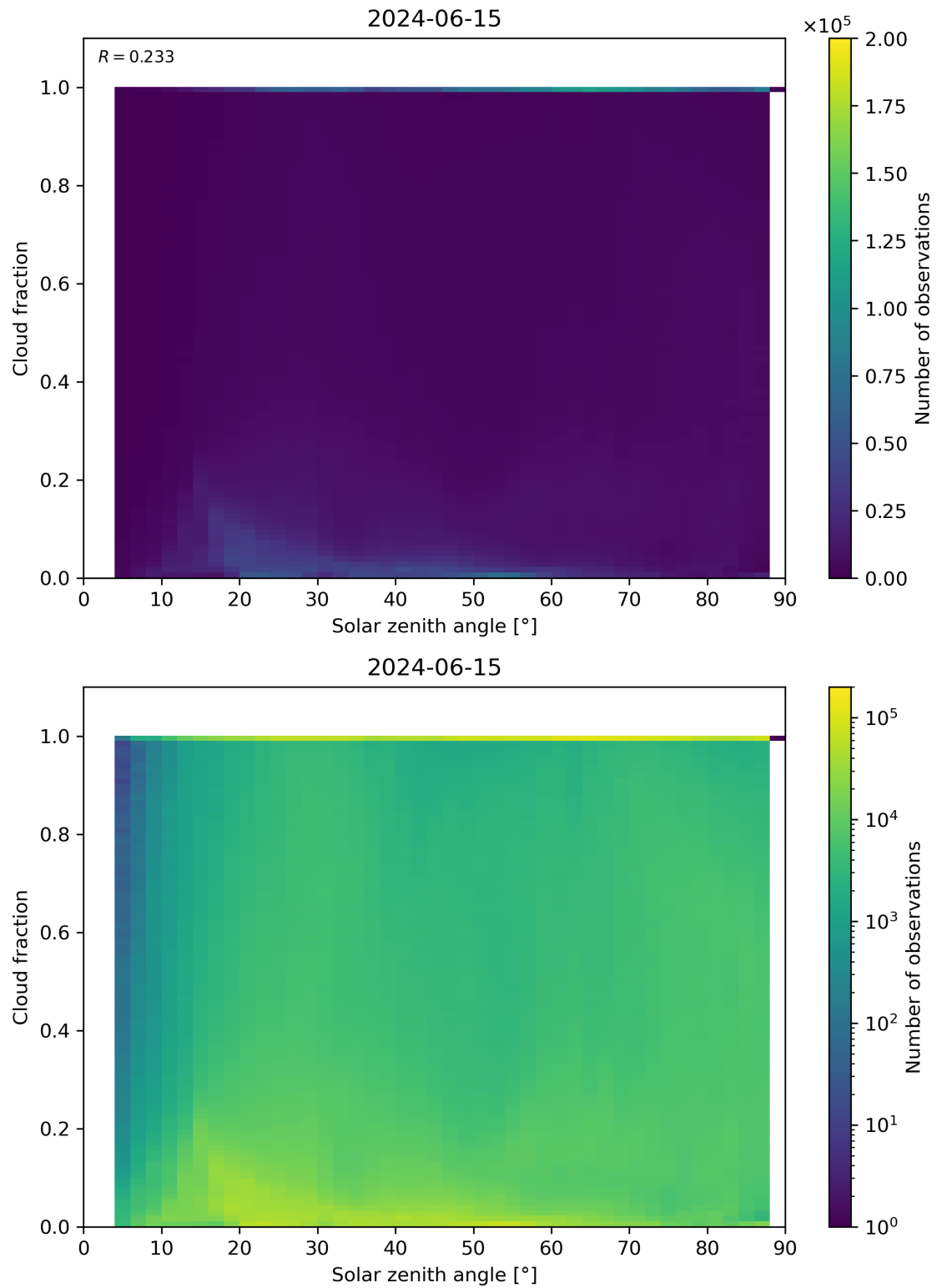
Figure 110: Scatter density plot of “Solar zenith angle” against “Cloud fraction” for 2024-06-14 to 2024-06-16.
