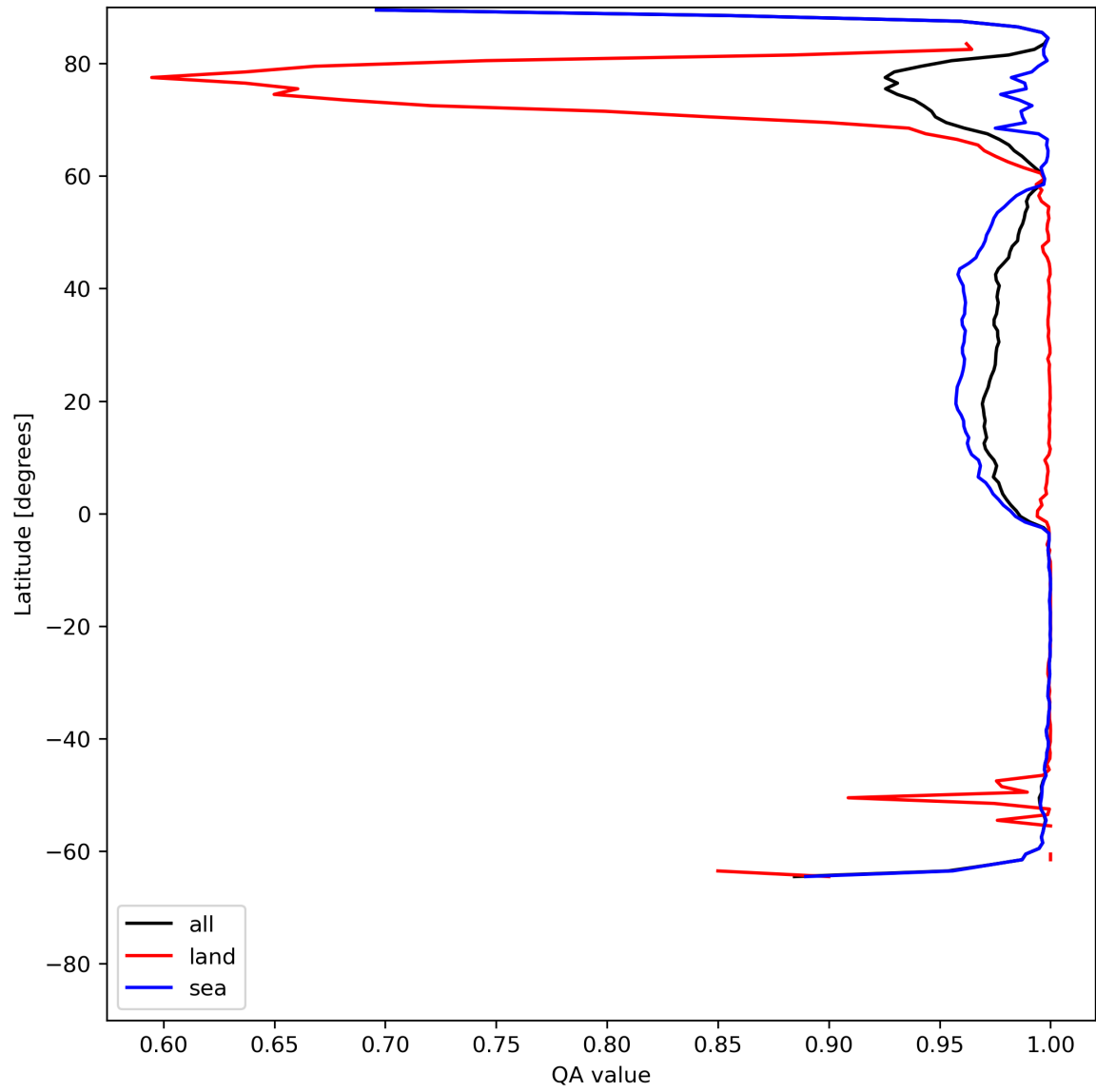
Figure 12: Zonal average of “QA value” for 2024-06-14 to 2024-06-16.
