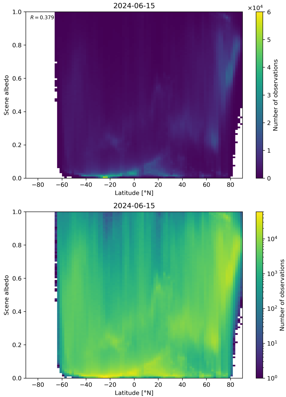
Figure 95: Scatter density plot of “Latitude” against “Scene albedo” for 2024-06-14 to 2024-06-16.
