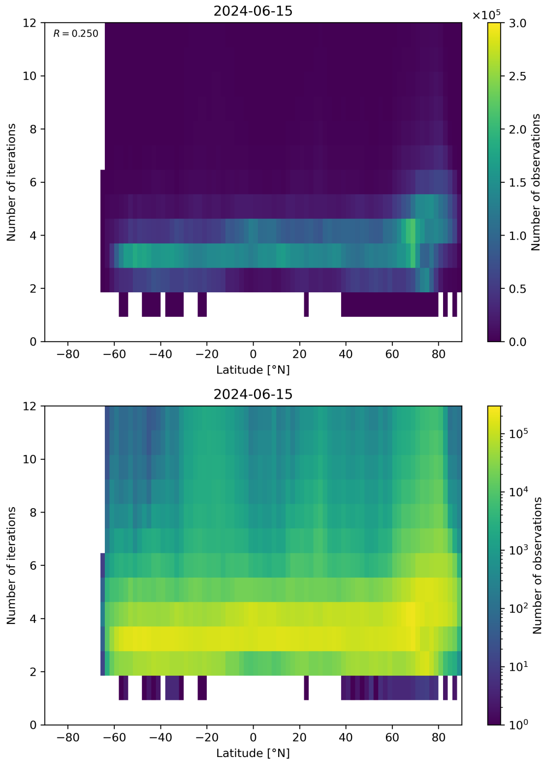
Figure 93: Scatter density plot of “Latitude” against “Number of iterations” for 2024-06-14 to 2024-06-16.
