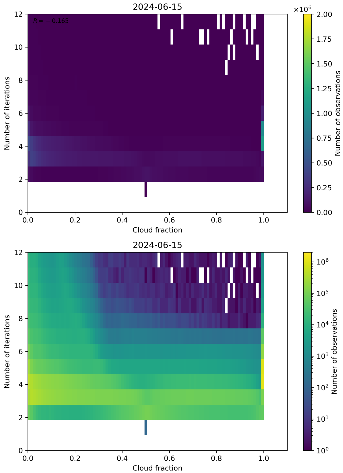
Figure 73: Scatter density plot of “Cloud fraction” against “Number of iterations” for 2024-06-14 to 2024-06-16.
