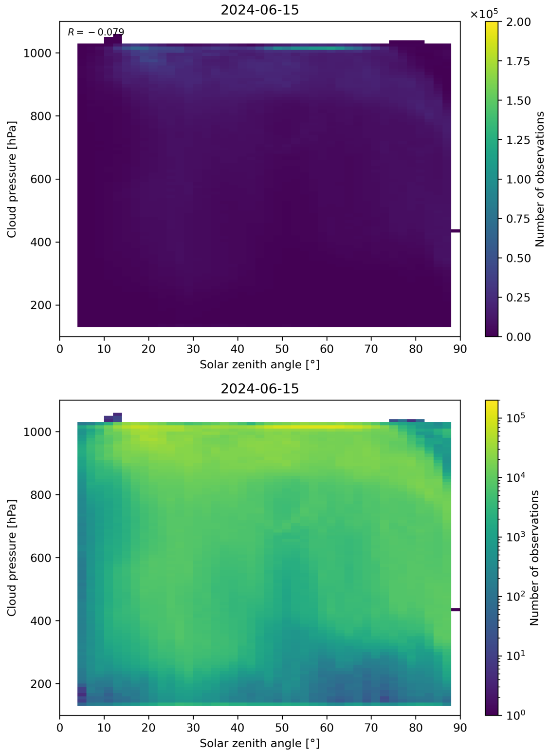
Figure 111: Scatter density plot of “Solar zenith angle” against “Cloud pressure” for 2024-06-14 to 2024-06-16.
