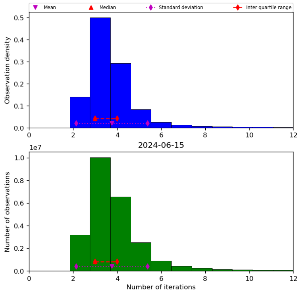
Figure 39: Histogram of “Number of iterations” for 2024-06-14 to 2024-06-16
