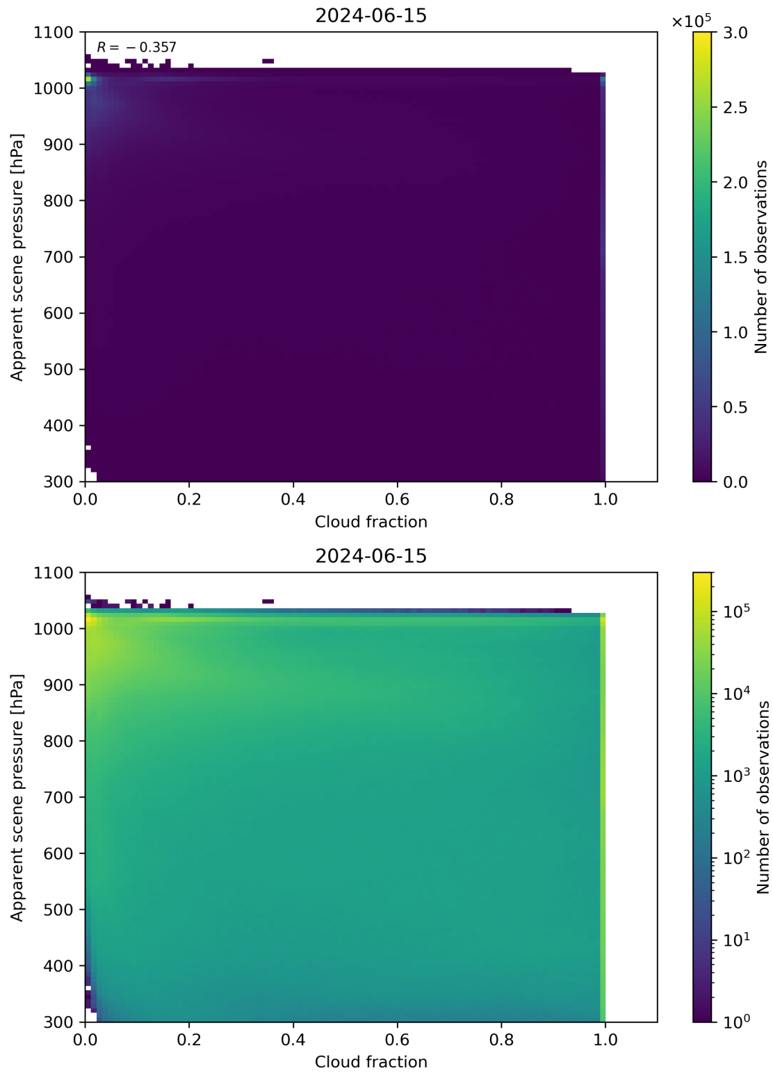
Figure 70: Scatter density plot of “Cloud fraction” against “Apparent scene pressure” for 2024-06-14 to 2024-06-16.
