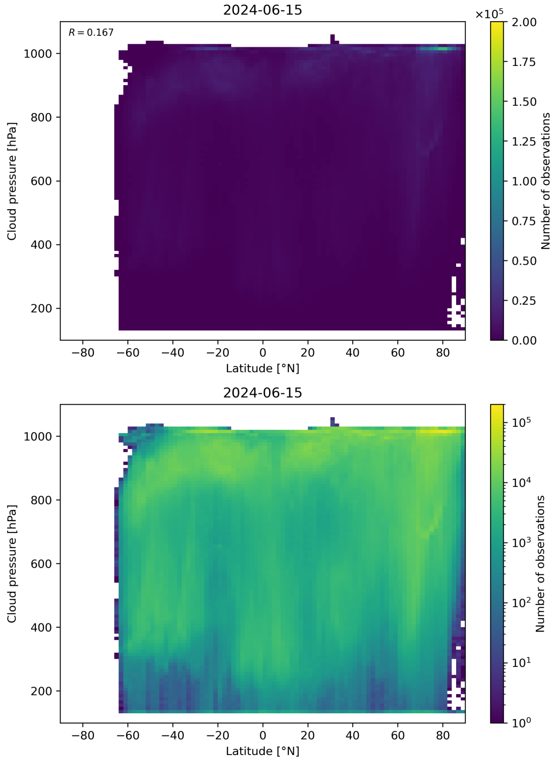
Figure 91: Scatter density plot of “Latitude” against “Cloud pressure” for 2024-06-14 to 2024-06-16.
