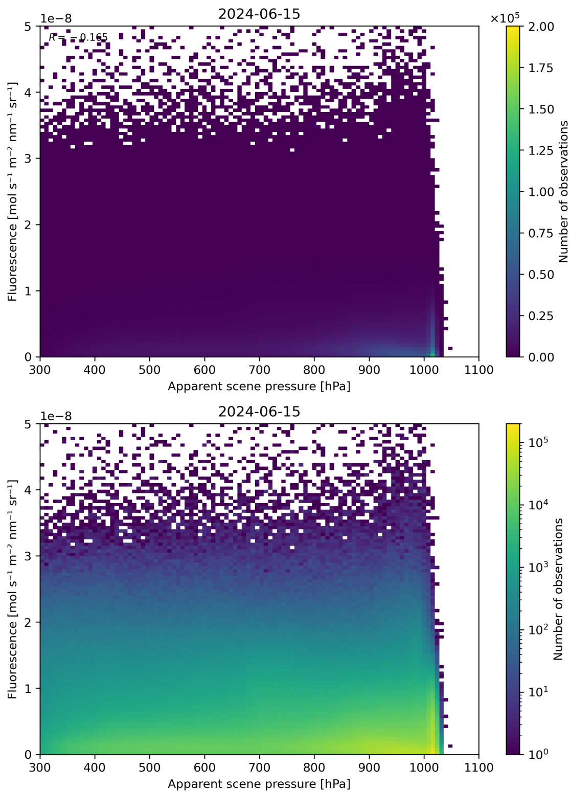
Figure 64: Scatter density plot of “Apparent scene pressure” against “Fluorescence” for 2024-06-14 to 2024-06-16.
