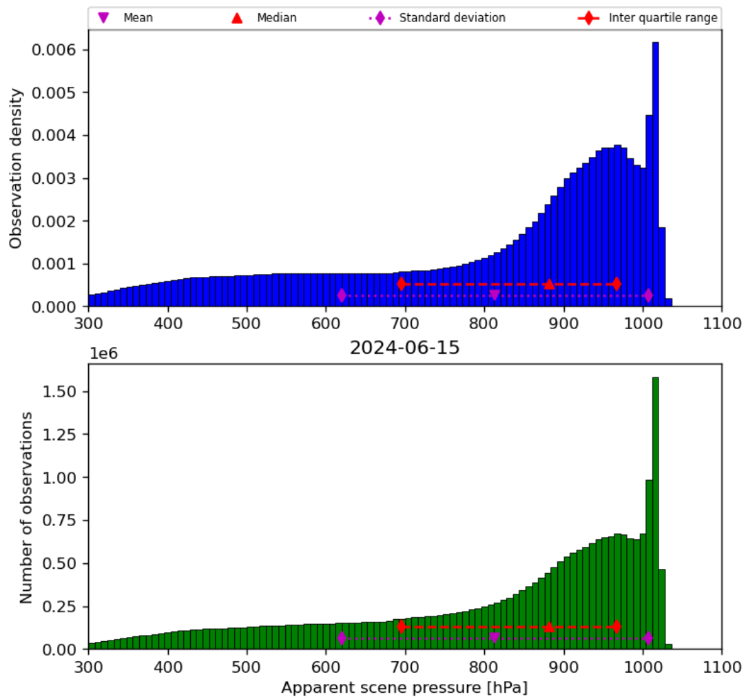
Figure 36: Histogram of “Apparent scene pressure” for 2024-06-14 to 2024-06-16
