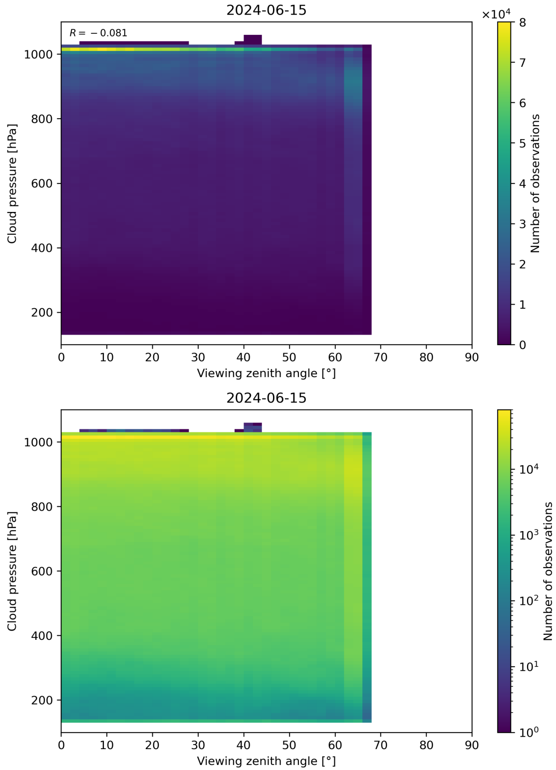
Figure 121: Scatter density plot of “Viewing zenith angle” against “Cloud pressure” for 2024-06-14 to 2024-06-16.
