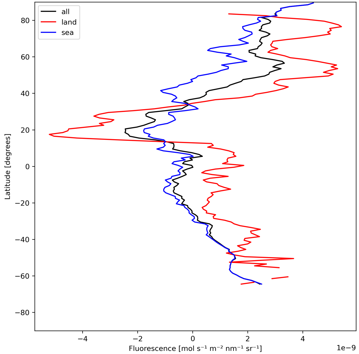
Figure 23: Zonal average of “Fluorescence” for 2024-06-14 to 2024-06-16.
