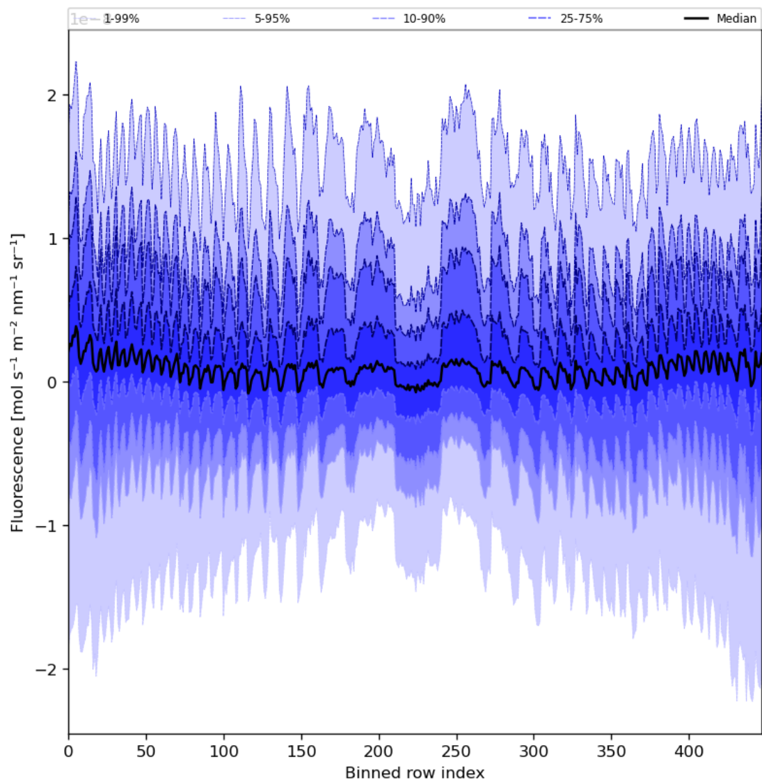
Figure 57: Along track statistics of “Fluorescence” for 2024-06-14 to 2024-06-16
