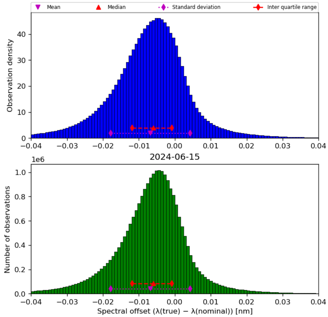
Figure 45: Histogram of “Spectral offset ( \lambda(\text{true}) - \lambda(\text{nominal}) )” for 2024-06-14 to 2024-06-16
