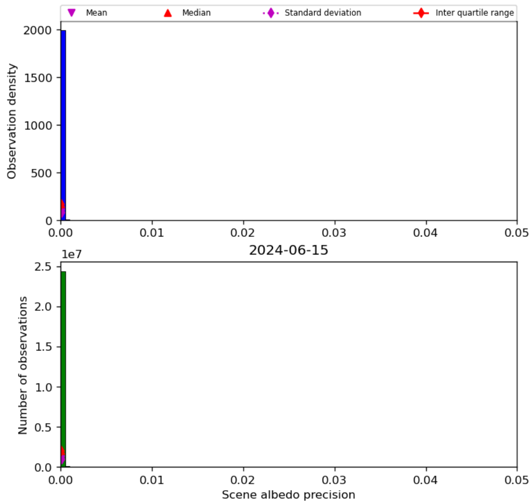
Figure 35: Histogram of “Scene albedo precision” for 2024-06-14 to 2024-06-16
