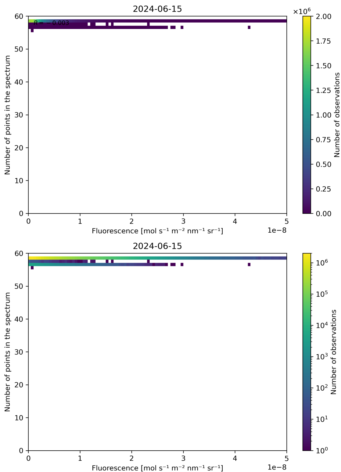
Figure 86: Scatter density plot of “Fluorescence” against “Number of points in the spectrum” for 2024-06-14 to 2024-06-16.
