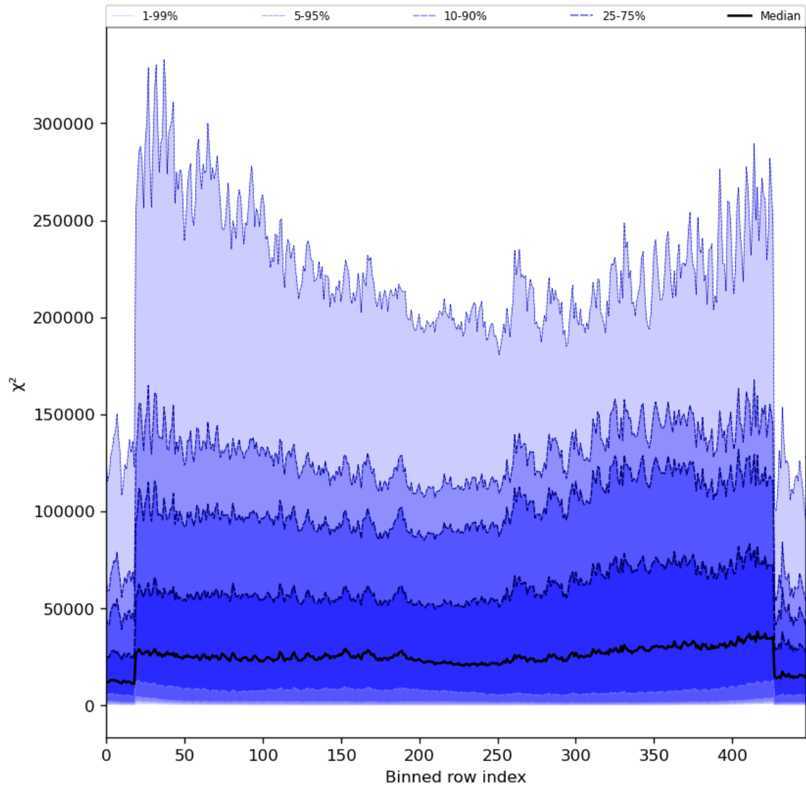
Figure 55: Along track statistics of “ \chi^2 ” for 2024-06-14 to 2024-06-16
