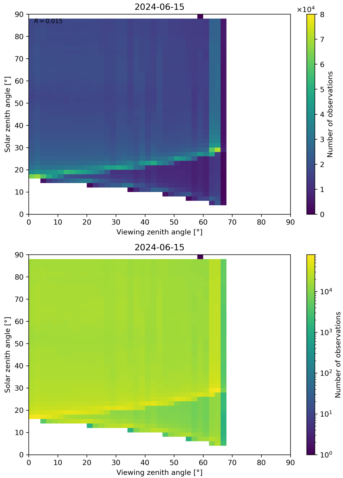
Figure 127: Scatter density plot of “Viewing zenith angle” against “Solar zenith angle” for 2024-06-14 to 2024-06-16.
