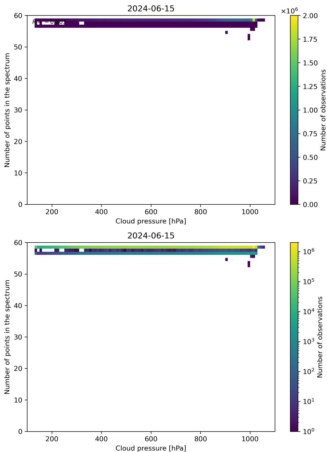
Figure 82: Scatter density plot of “Cloud pressure” against “Number of points in the spectrum” for 2024-06-14 to 2024-06-16.
