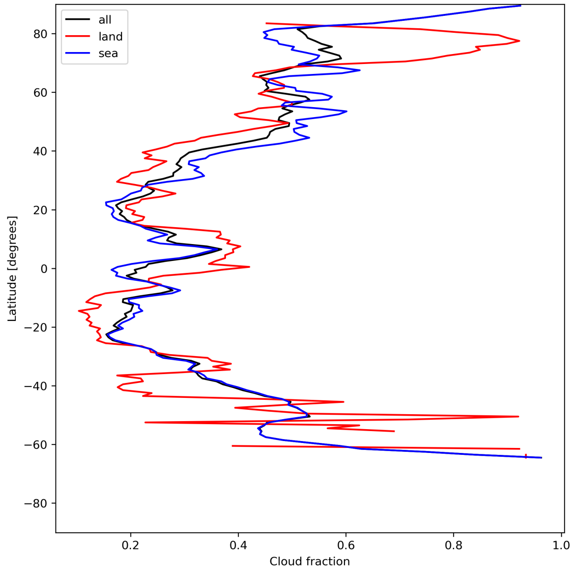
Figure 15: Zonal average of “Cloud fraction” for 2024-06-14 to 2024-06-16.
