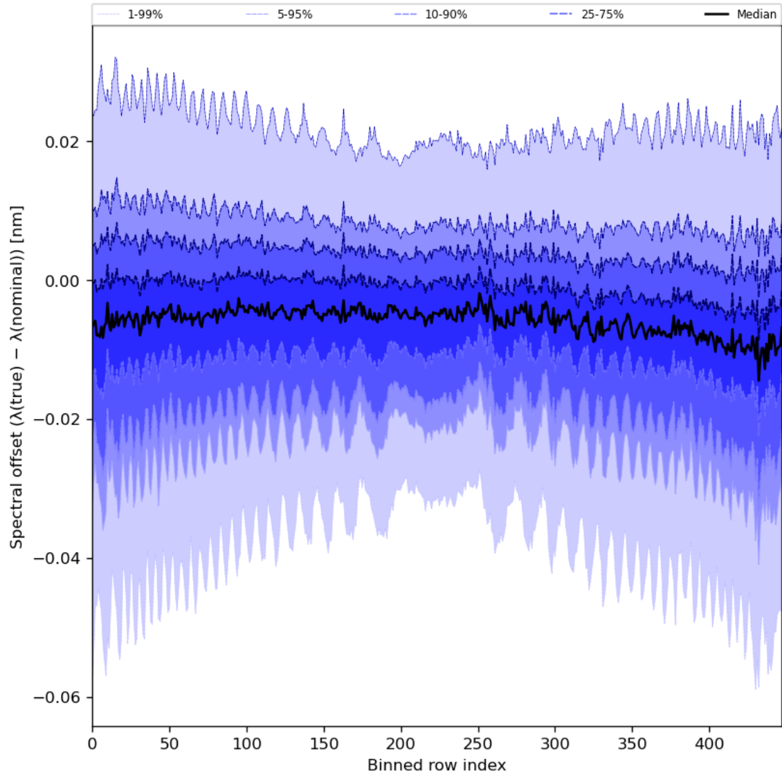
Figure 62: Along track statistics of “Spectral offset ( \lambda(\text{true}) - \lambda(\text{nominal}) )” for 2024-06-14 to 2024-06-16
