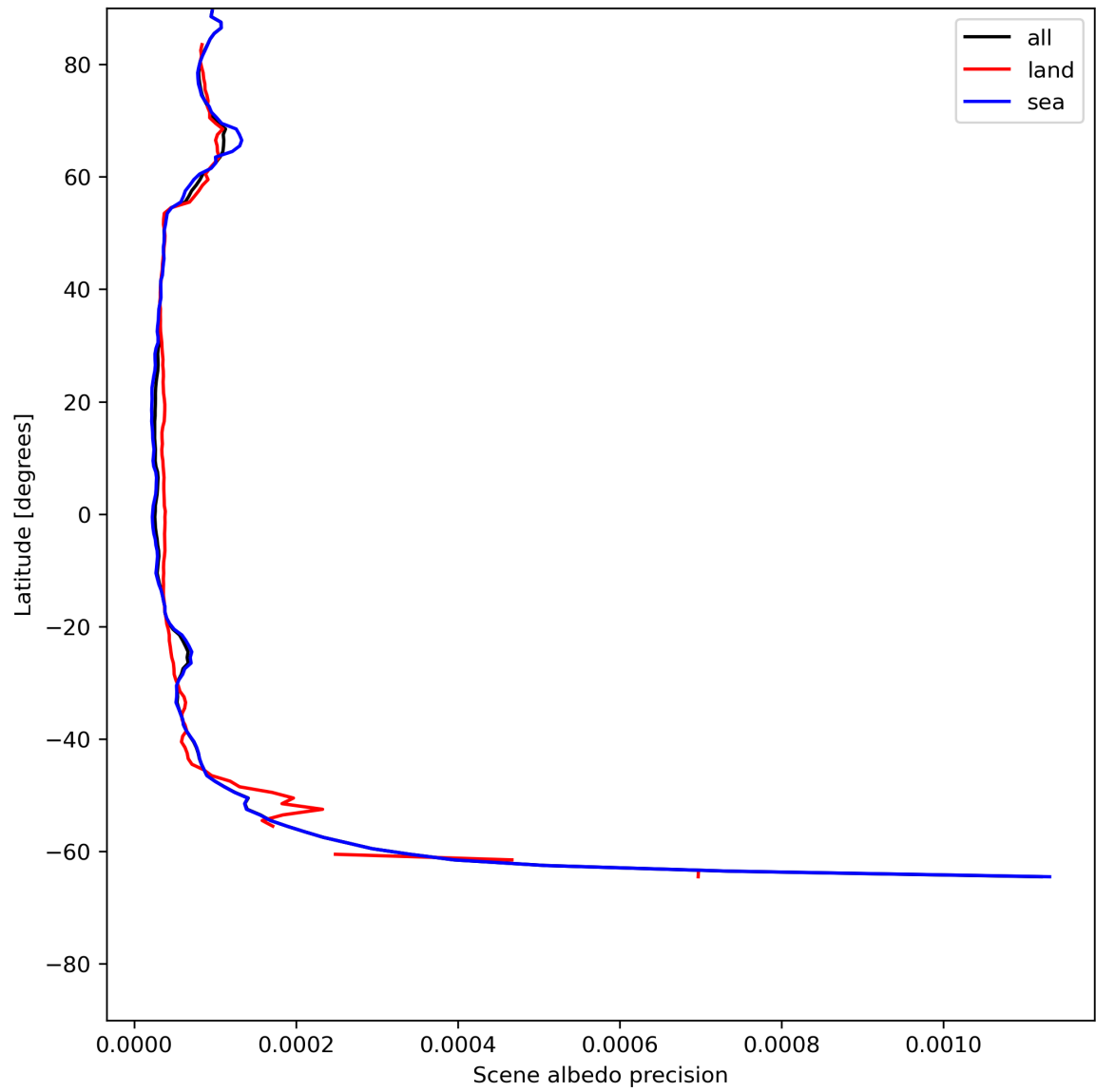
Figure 18: Zonal average of “Scene albedo precision” for 2024-06-14 to 2024-06-16.
