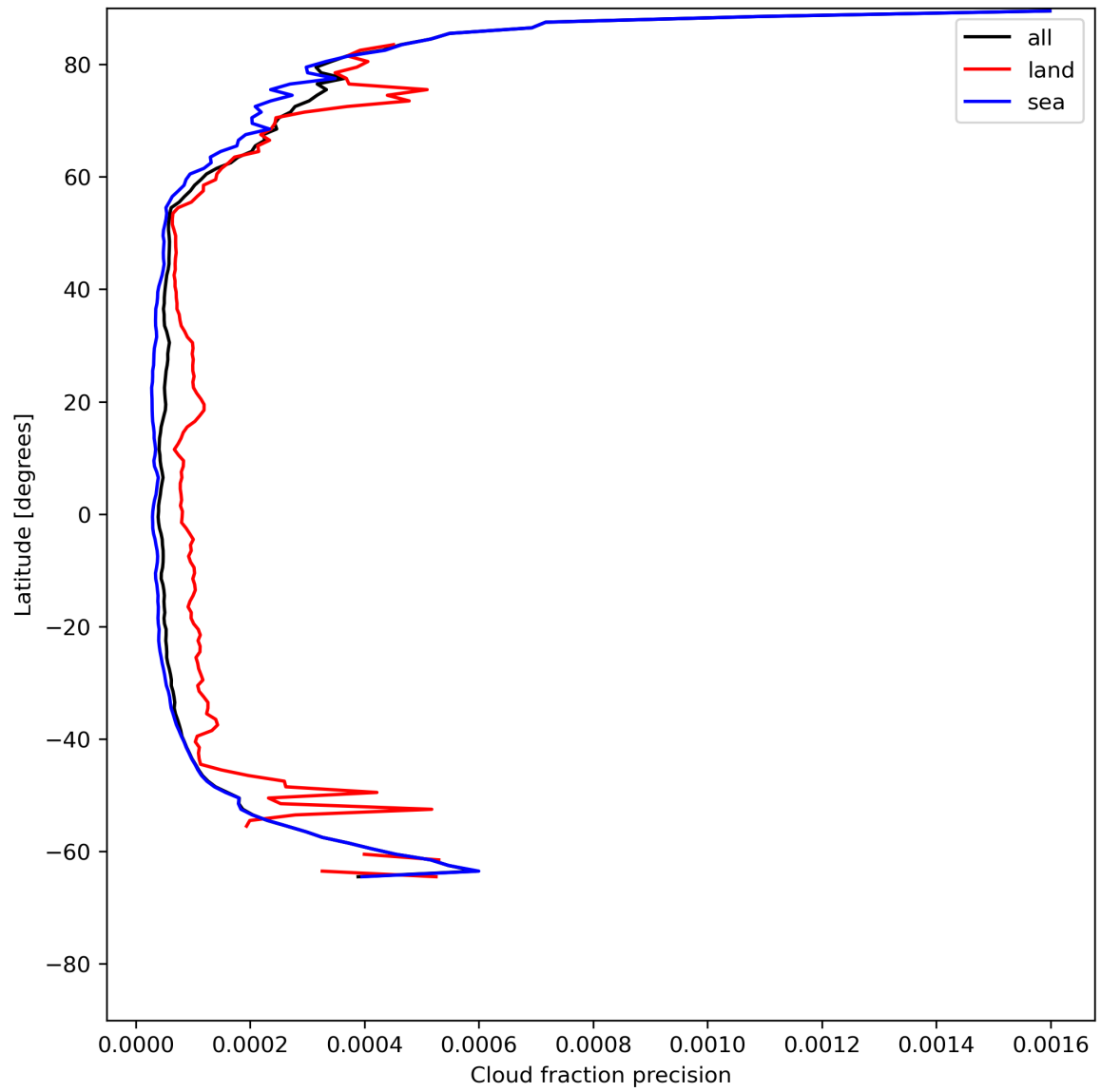
Figure 16: Zonal average of “Cloud fraction precision” for 2024-06-14 to 2024-06-16.
