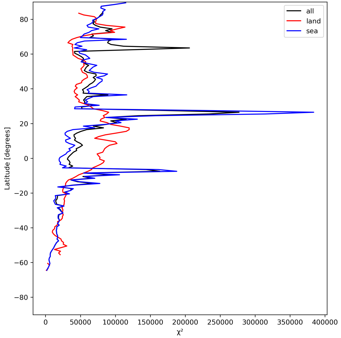
Figure 21: Zonal average of “ \chi^2 ” for 2024-06-14 to 2024-06-16.
