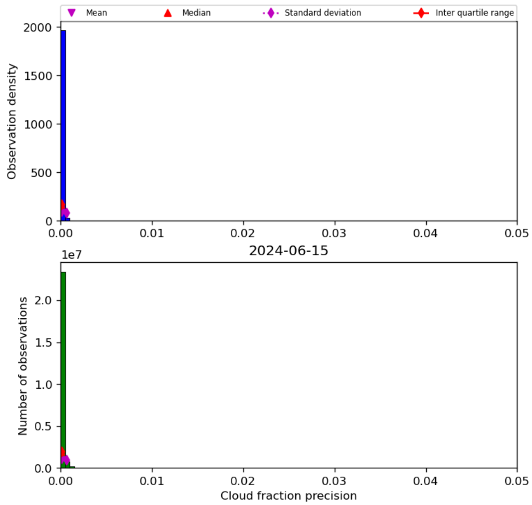
Figure 33: Histogram of “Cloud fraction precision” for 2024-06-14 to 2024-06-16
