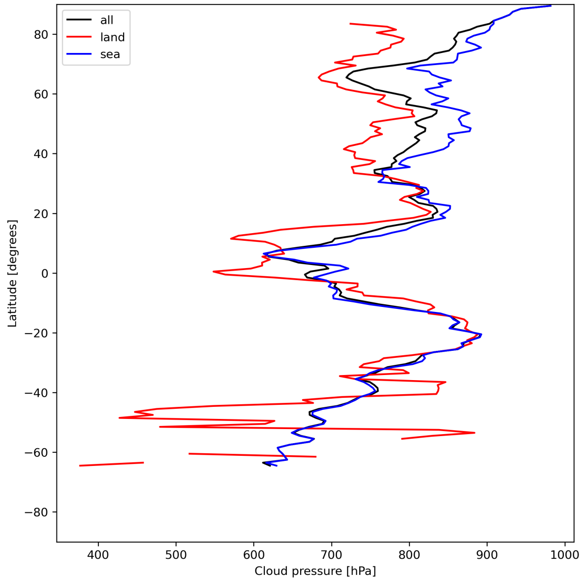
Figure 13: Zonal average of “Cloud pressure” for 2024-06-14 to 2024-06-16.
