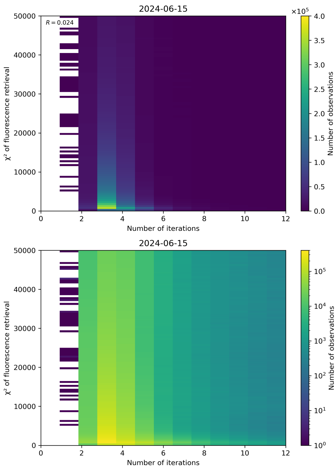
Figure 97: Scatter density plot of “Number of iterations” against “ \chi^2 of fluorescence retrieval” for 2024-06-14 to 2024-06-16.
