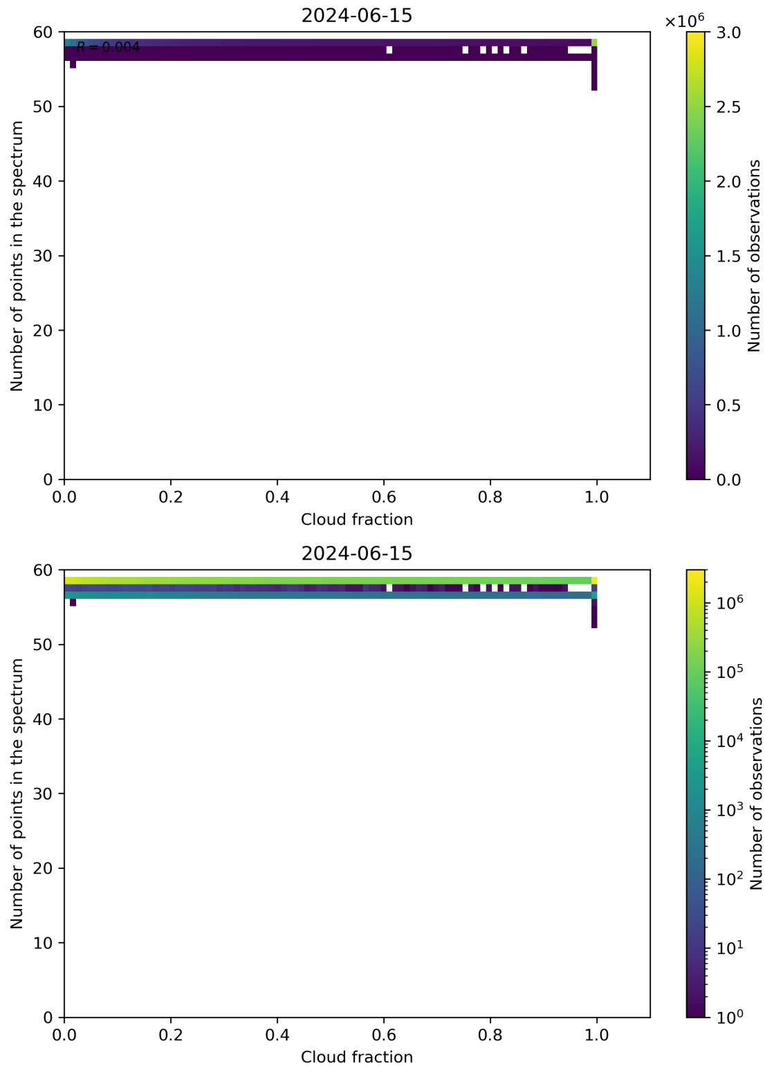
Figure 74: Scatter density plot of “Cloud fraction” against “Number of points in the spectrum” for 2024-06-14 to 2024-06-16.
