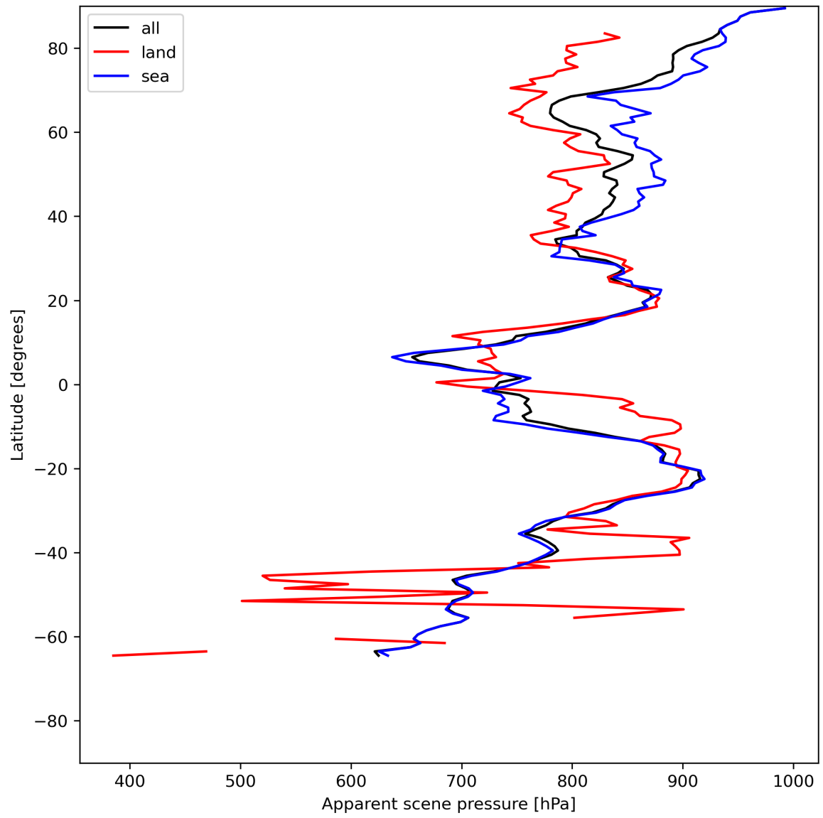
Figure 19: Zonal average of “Apparent scene pressure” for 2024-06-14 to 2024-06-16.
