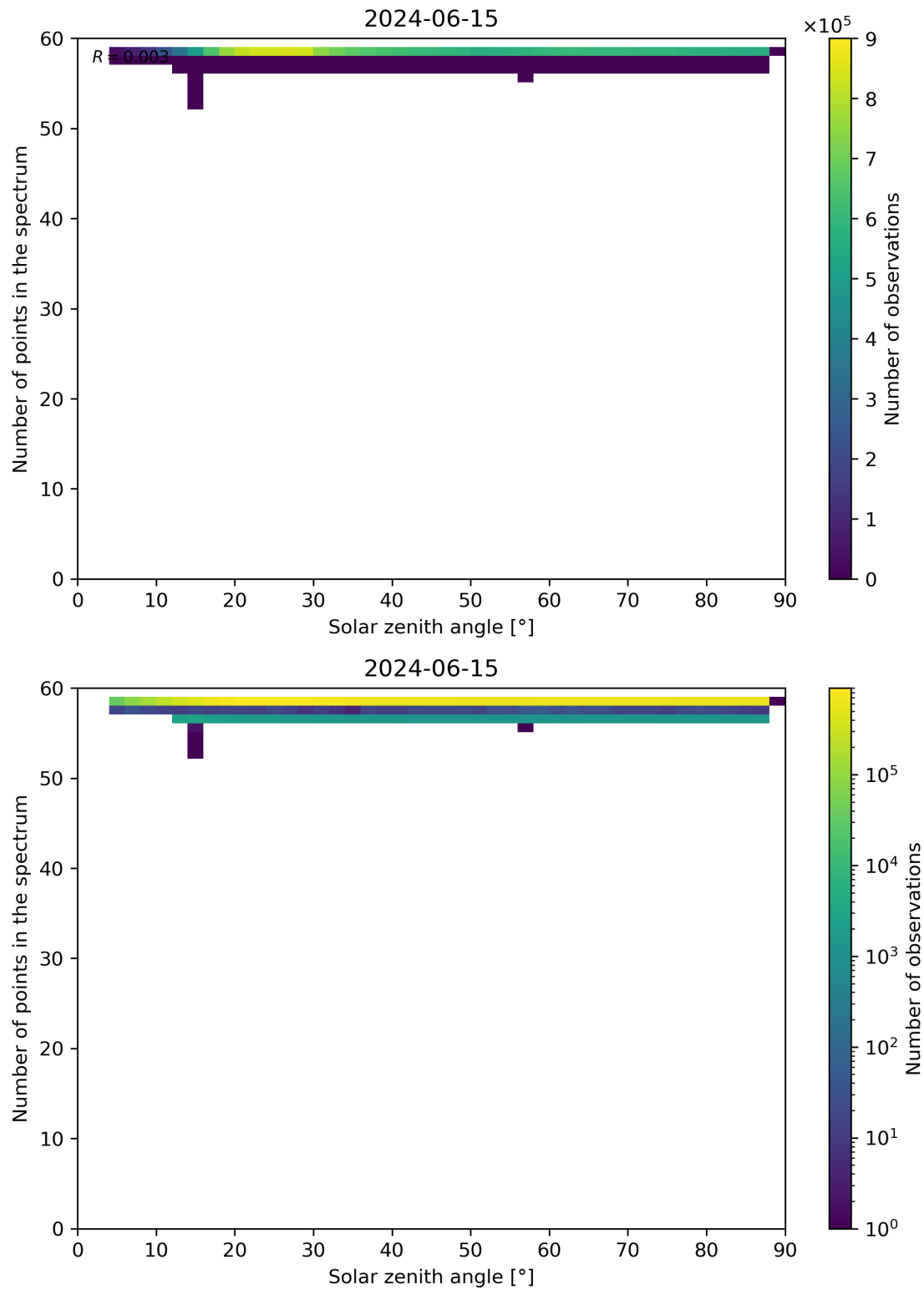
Figure 115: Scatter density plot of “Solar zenith angle” against “Number of points in the spectrum” for 2024-06-14 to 2024-06-16.
