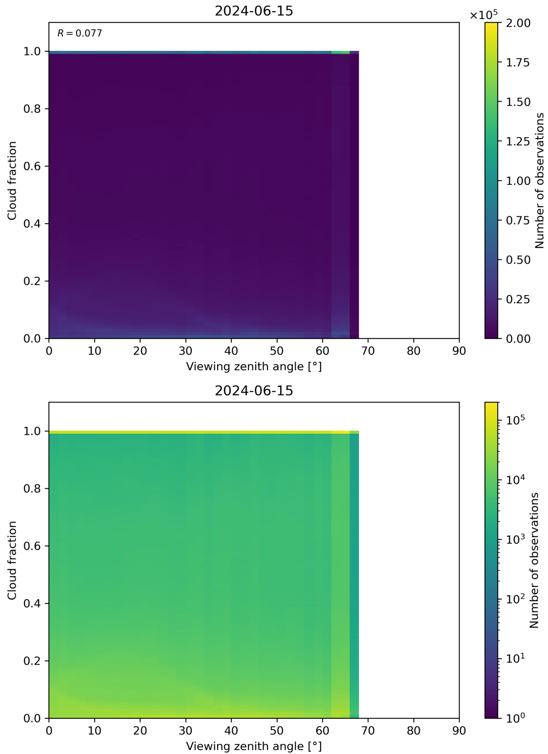
Figure 120: Scatter density plot of “Viewing zenith angle” against “Cloud fraction” for 2024-06-14 to 2024-06-16.
