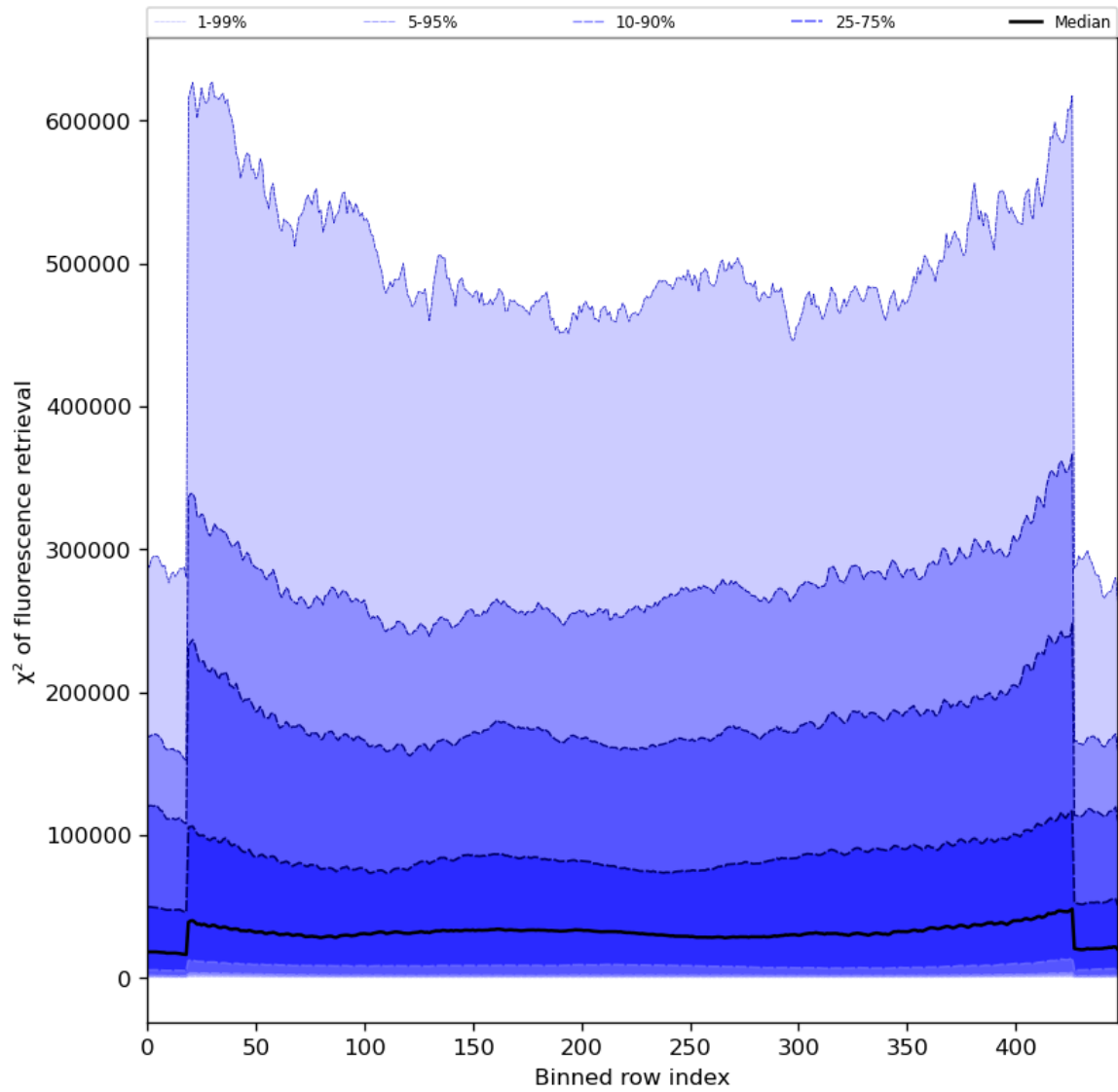
Figure 59: Along track statistics of “ \chi^2 of fluorescence retrieval” for 2024-06-14 to 2024-06-16
