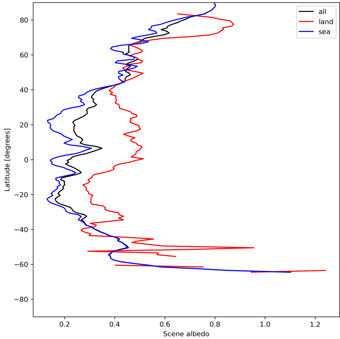
Figure 17: Zonal average of “Scene albedo” for 2024-06-14 to 2024-06-16.
