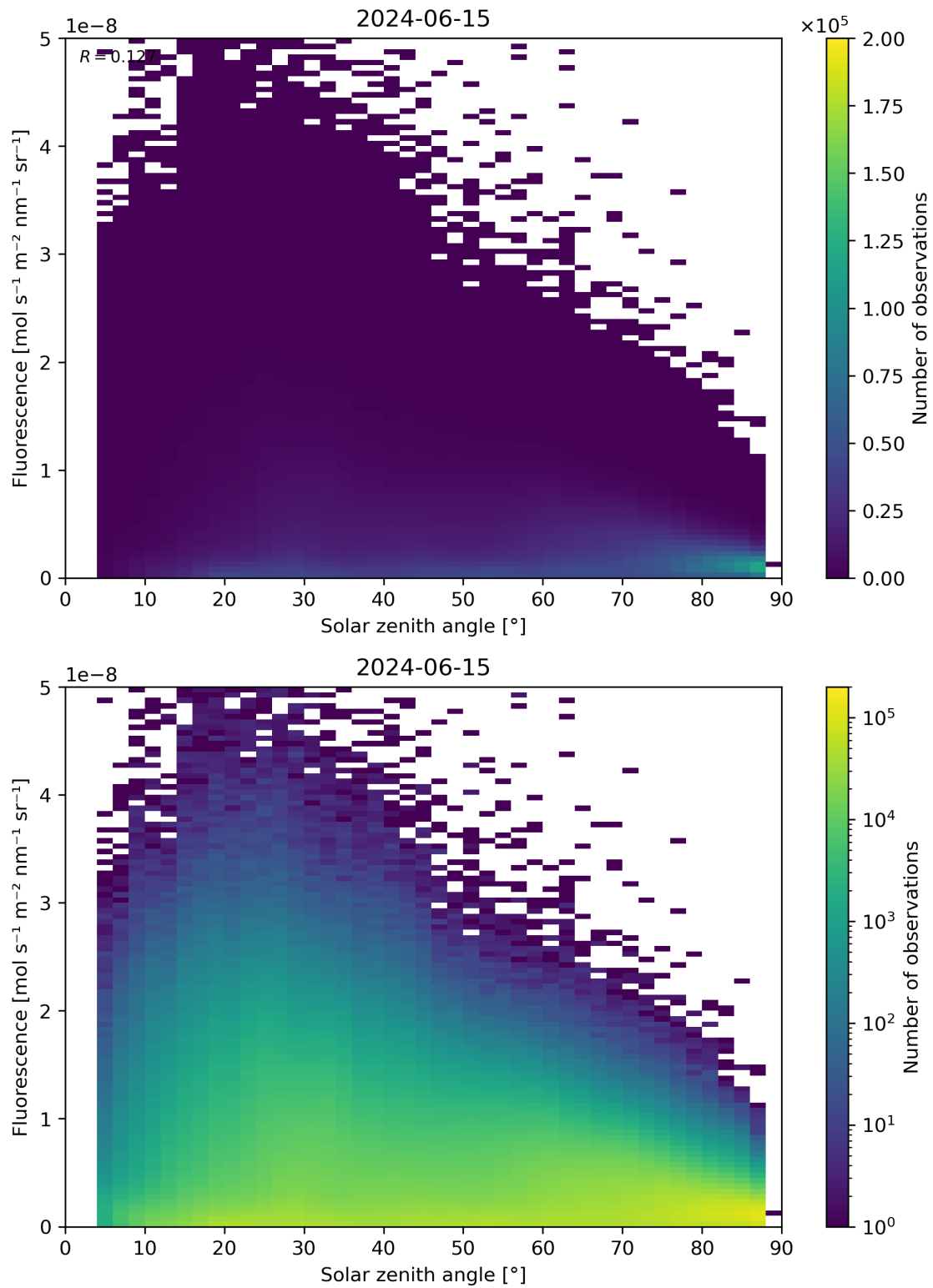
Figure 112: Scatter density plot of “Solar zenith angle” against “Fluorescence” for 2024-06-14 to 2024-06-16.
