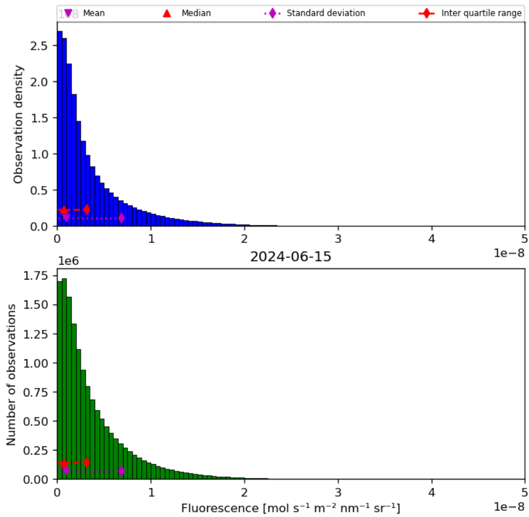
Figure 40: Histogram of “Fluorescence” for 2024-06-14 to 2024-06-16
