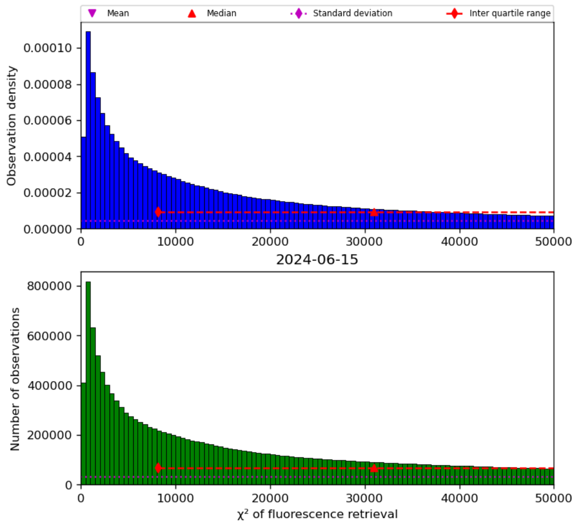
Figure 42: Histogram of “ \chi^2 of fluorescence retrieval” for 2024-06-14 to 2024-06-16
