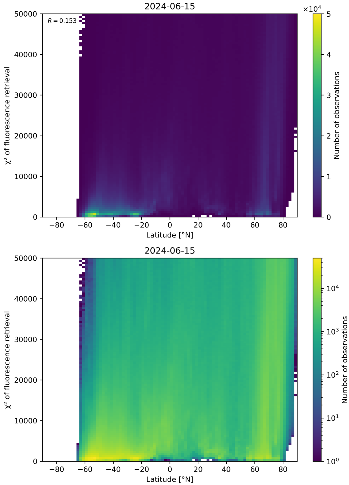
Figure 89: Scatter density plot of “Latitude” against “ \chi^2 of fluorescence retrieval” for 2024-06-14 to 2024-06-16.
