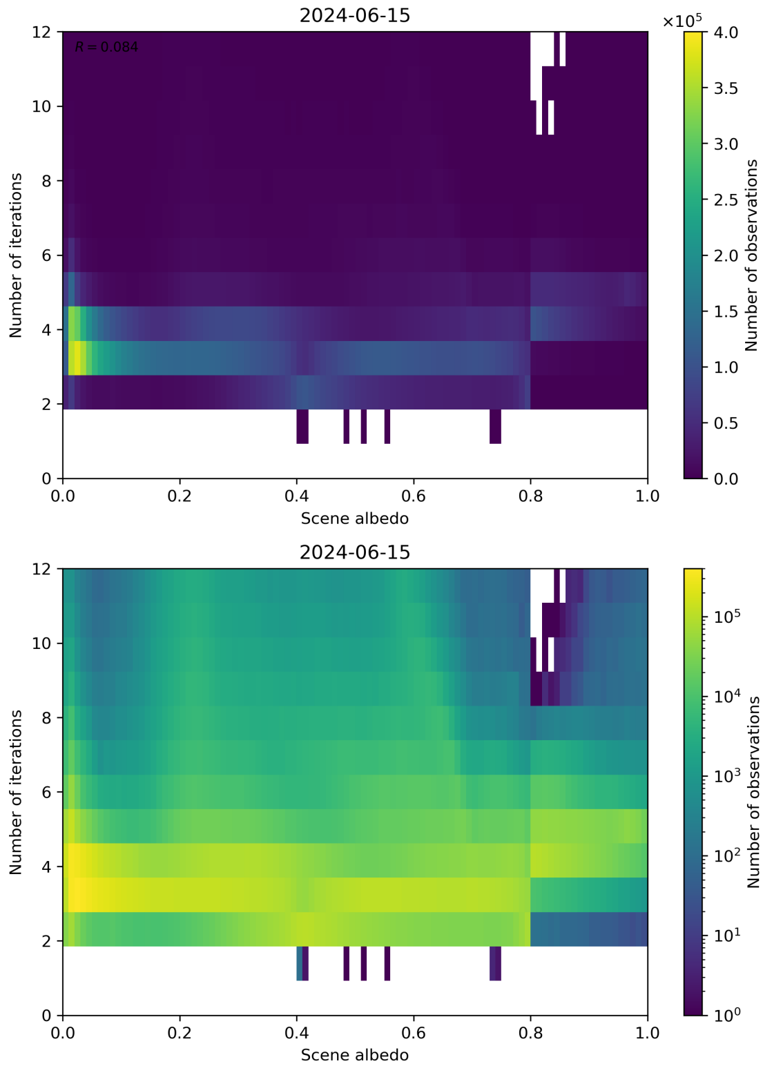
Figure 105: Scatter density plot of “Scene albedo” against “Number of iterations” for 2024-06-14 to 2024-06-16.
