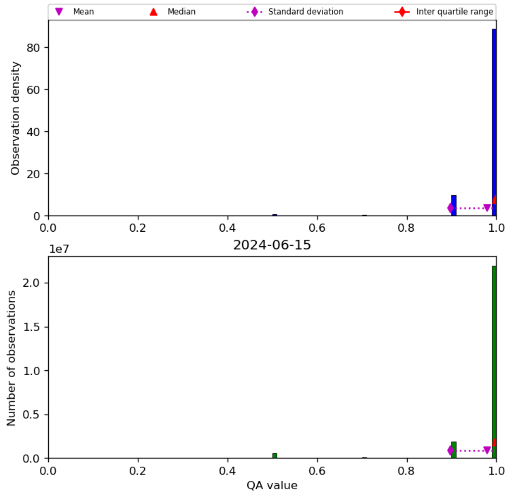
Figure 29: Histogram of “QA value” for 2024-06-14 to 2024-06-16
