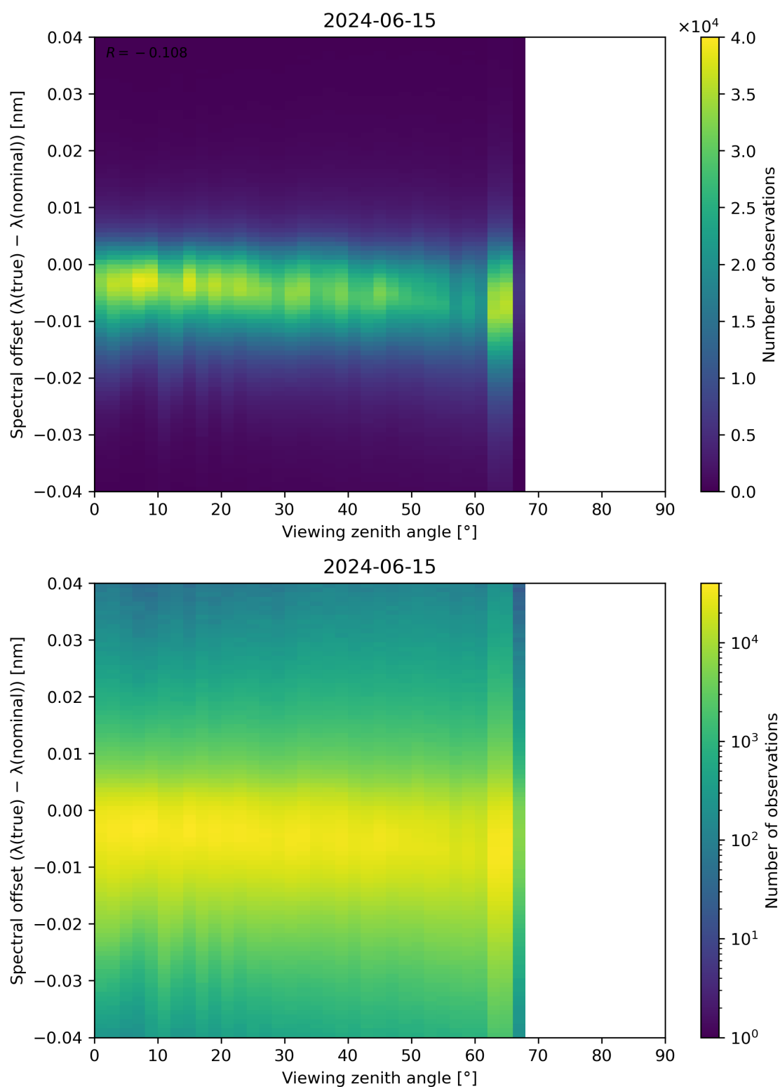
Figure 128: Scatter density plot of “Viewing zenith angle” against “Spectral offset ( \lambda(\text{true}) - \lambda(\text{nominal}) )” for 2024-06-14 to 2024-06-16.
