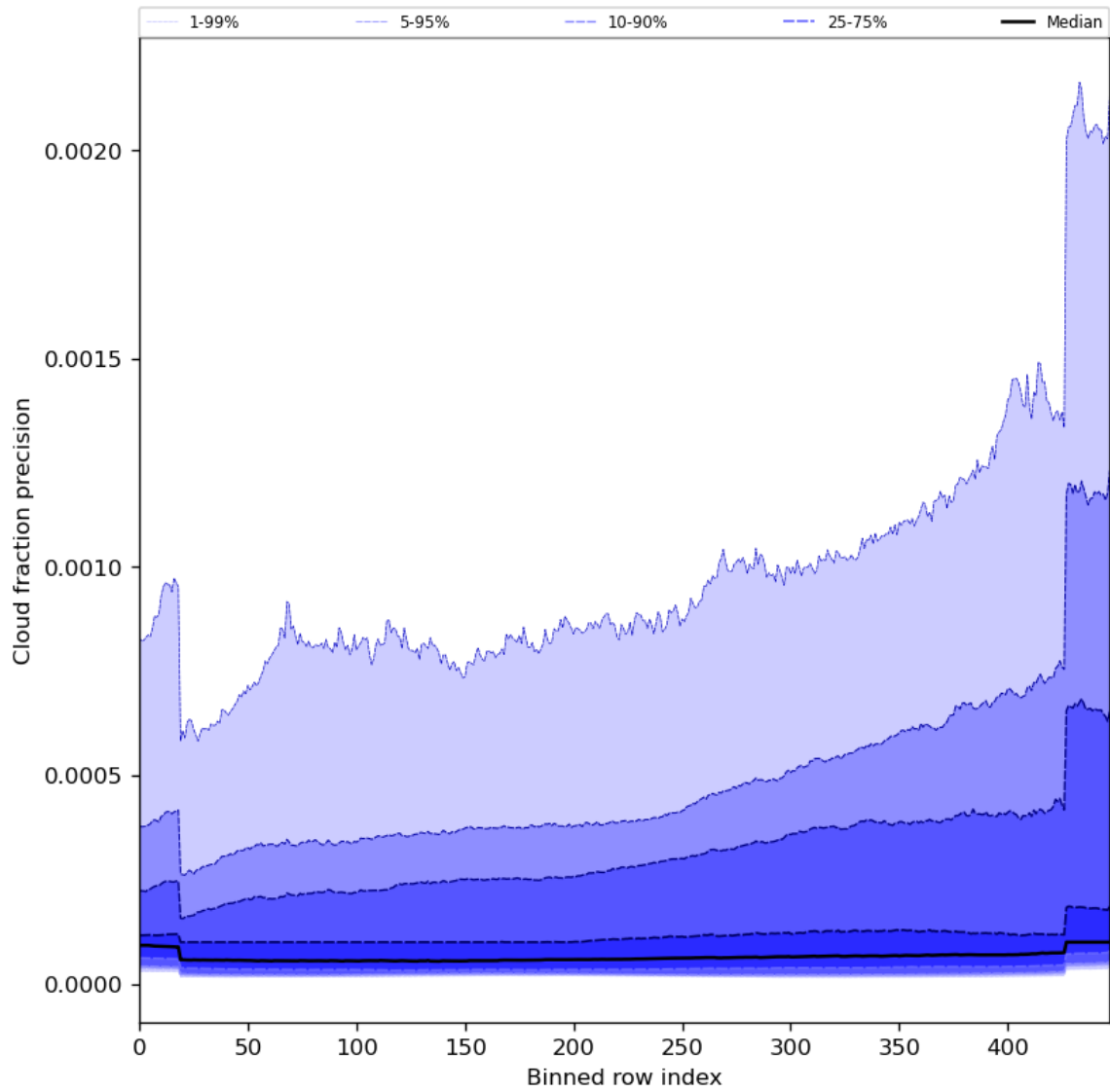
Figure 50: Along track statistics of “Cloud fraction precision” for 2024-06-14 to 2024-06-16
