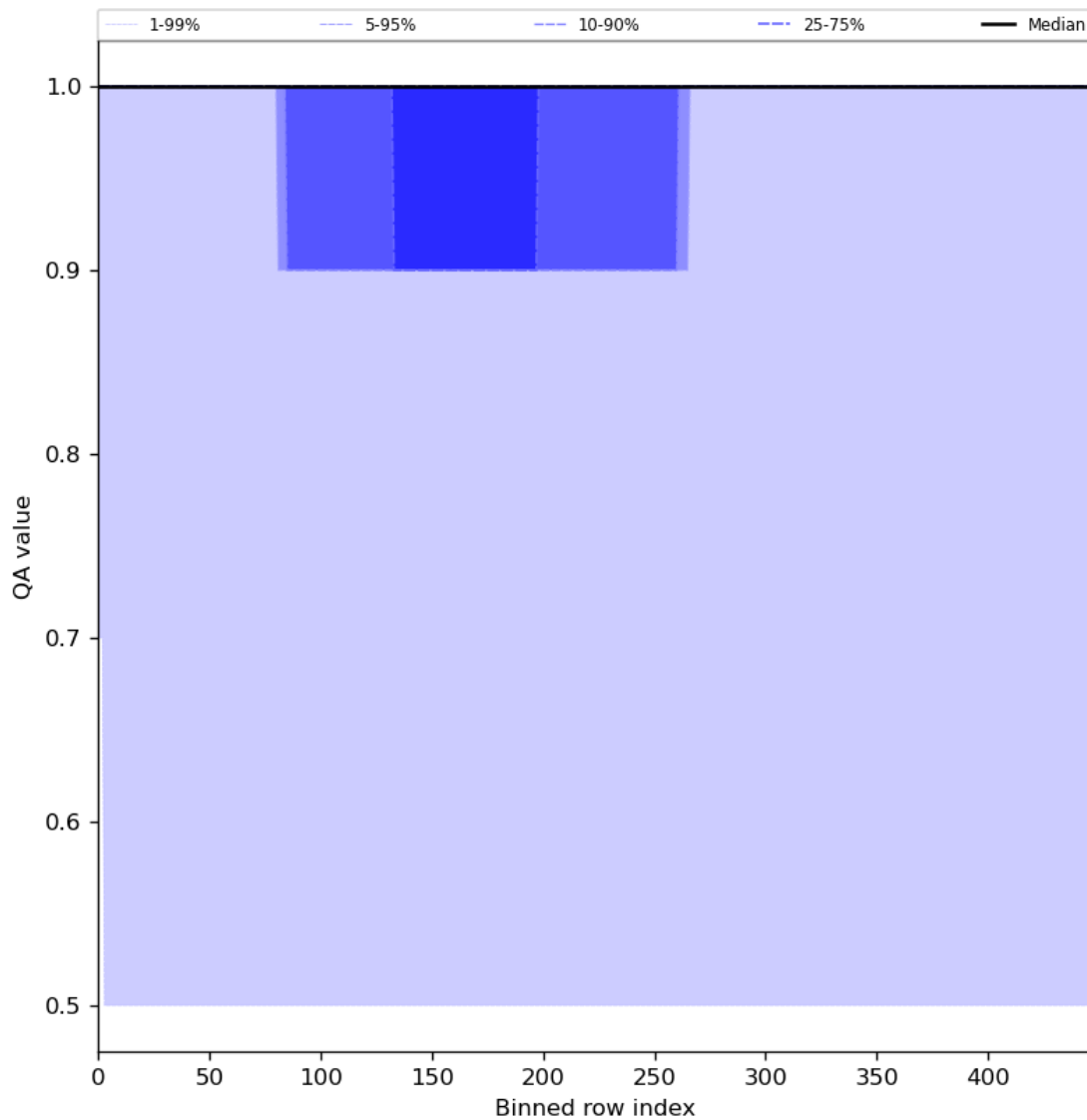
Figure 46: Along track statistics of “QA value” for 2024-06-14 to 2024-06-16
