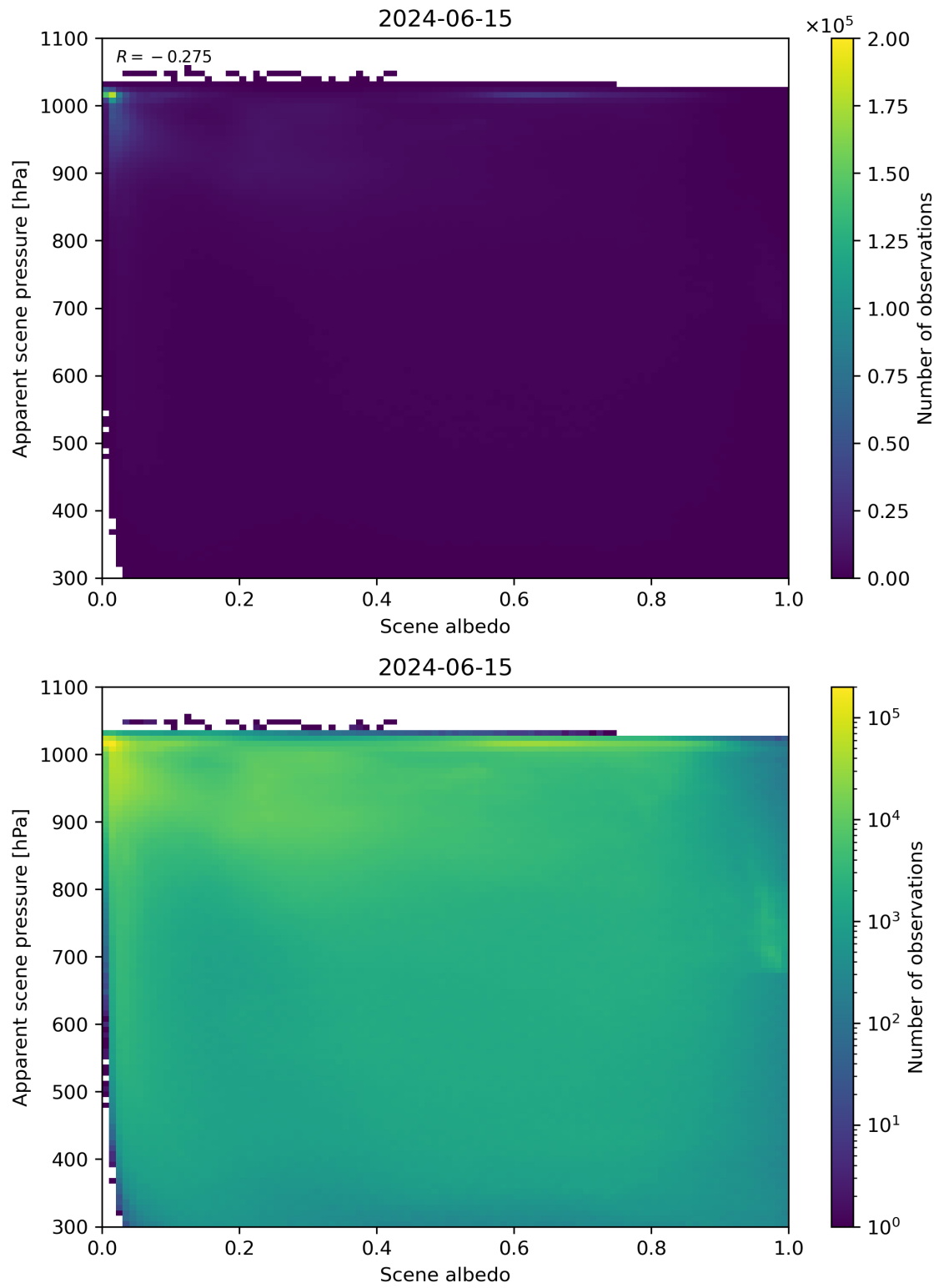
Figure 102: Scatter density plot of “Scene albedo” against “Apparent scene pressure” for 2024-06-14 to 2024-06-16.
