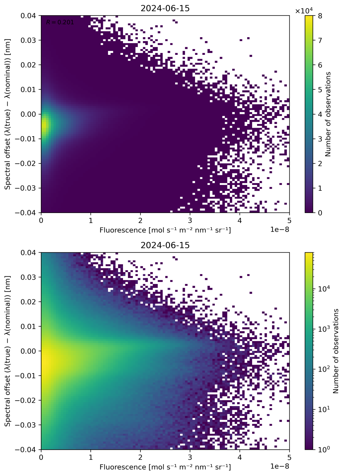
Figure 87: Scatter density plot of “Fluorescence” against “Spectral offset ( \lambda(\text{true}) - \lambda(\text{nominal}) )” for 2024-06-14 to 2024-06-16.
