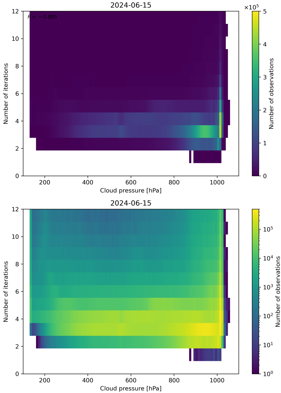
Figure 81: Scatter density plot of “Cloud pressure” against “Number of iterations” for 2024-06-14 to 2024-06-16.
