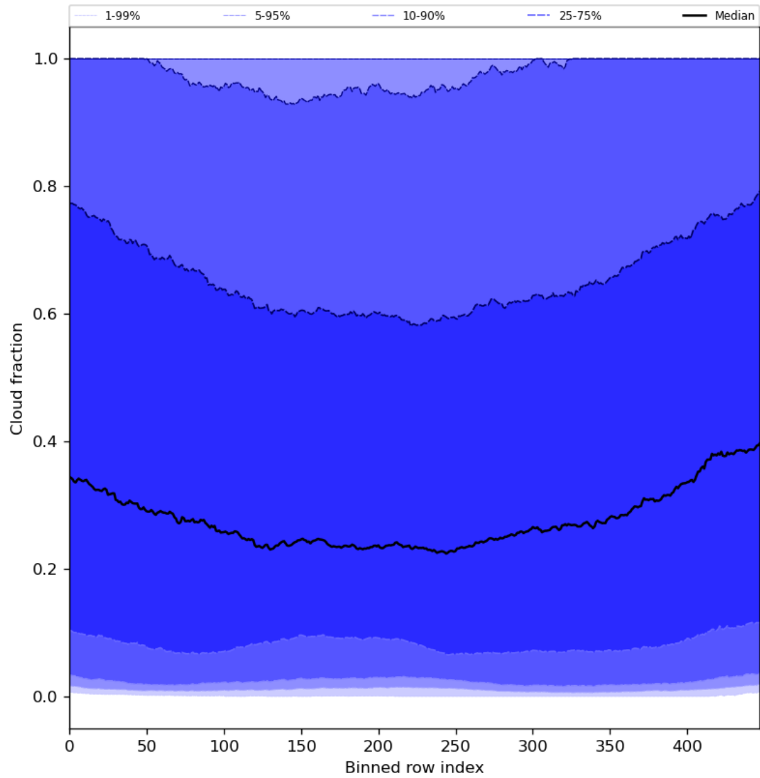
Figure 49: Along track statistics of “Cloud fraction” for 2024-06-14 to 2024-06-16
