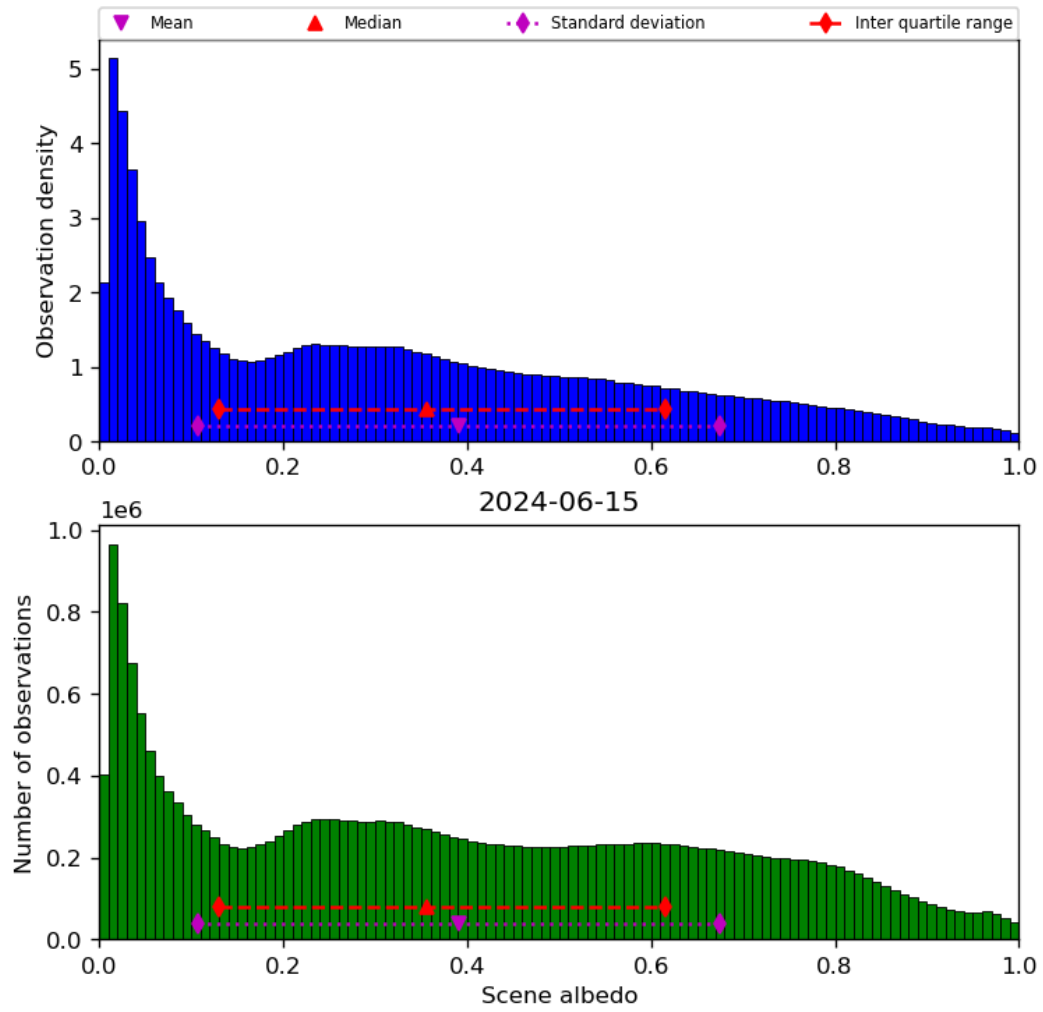
Figure 34: Histogram of “Scene albedo” for 2024-06-14 to 2024-06-16
