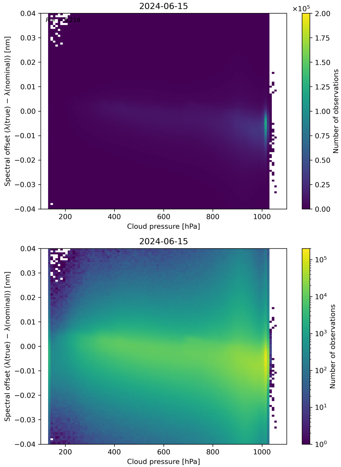
Figure 84: Scatter density plot of “Cloud pressure” against “Spectral offset ( \lambda(\text{true}) - \lambda(\text{nominal}) )” for 2024-06-14 to 2024-06-16.
