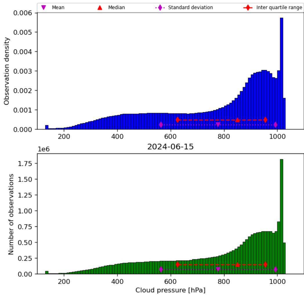
Figure 30: Histogram of “Cloud pressure” for 2024-06-14 to 2024-06-16
