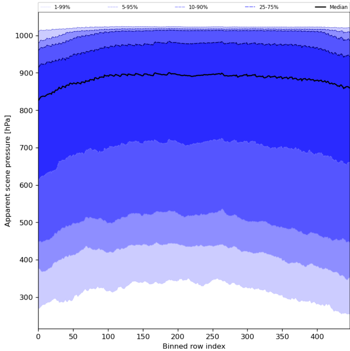
Figure 53: Along track statistics of “Apparent scene pressure” for 2024-06-14 to 2024-06-16
