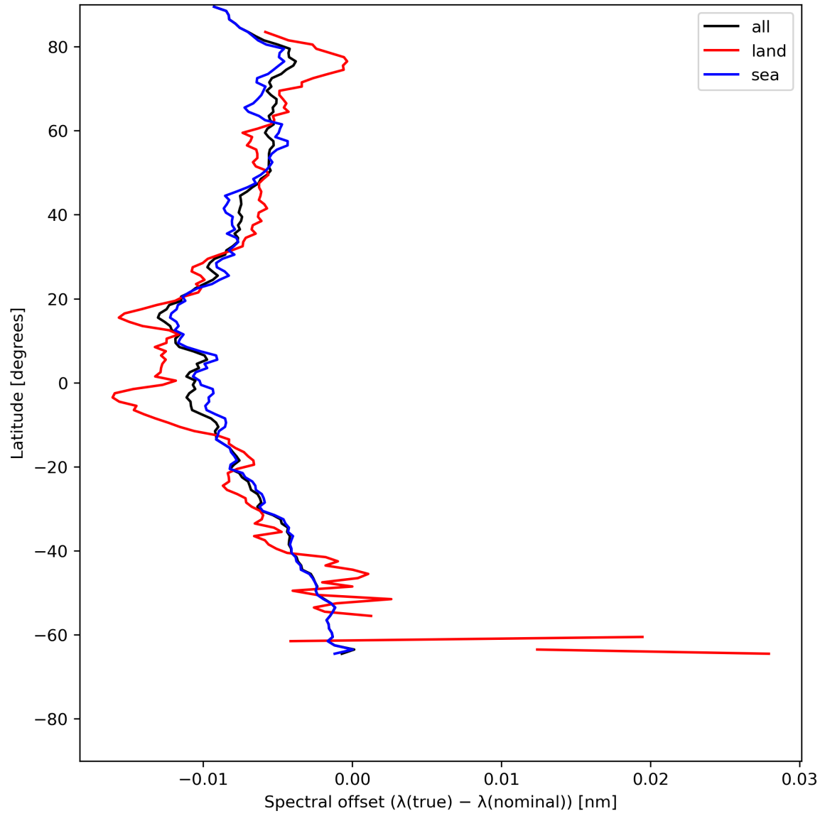
Figure 28: Zonal average of “Spectral offset ( \lambda(\text{true}) - \lambda(\text{nominal}) )” for 2024-06-14 to 2024-06-16.
