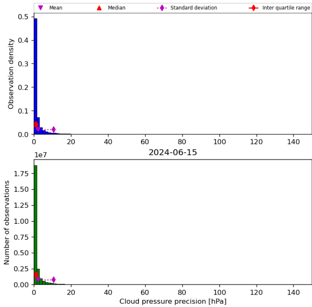
Figure 31: Histogram of “Cloud pressure precision” for 2024-06-14 to 2024-06-16
