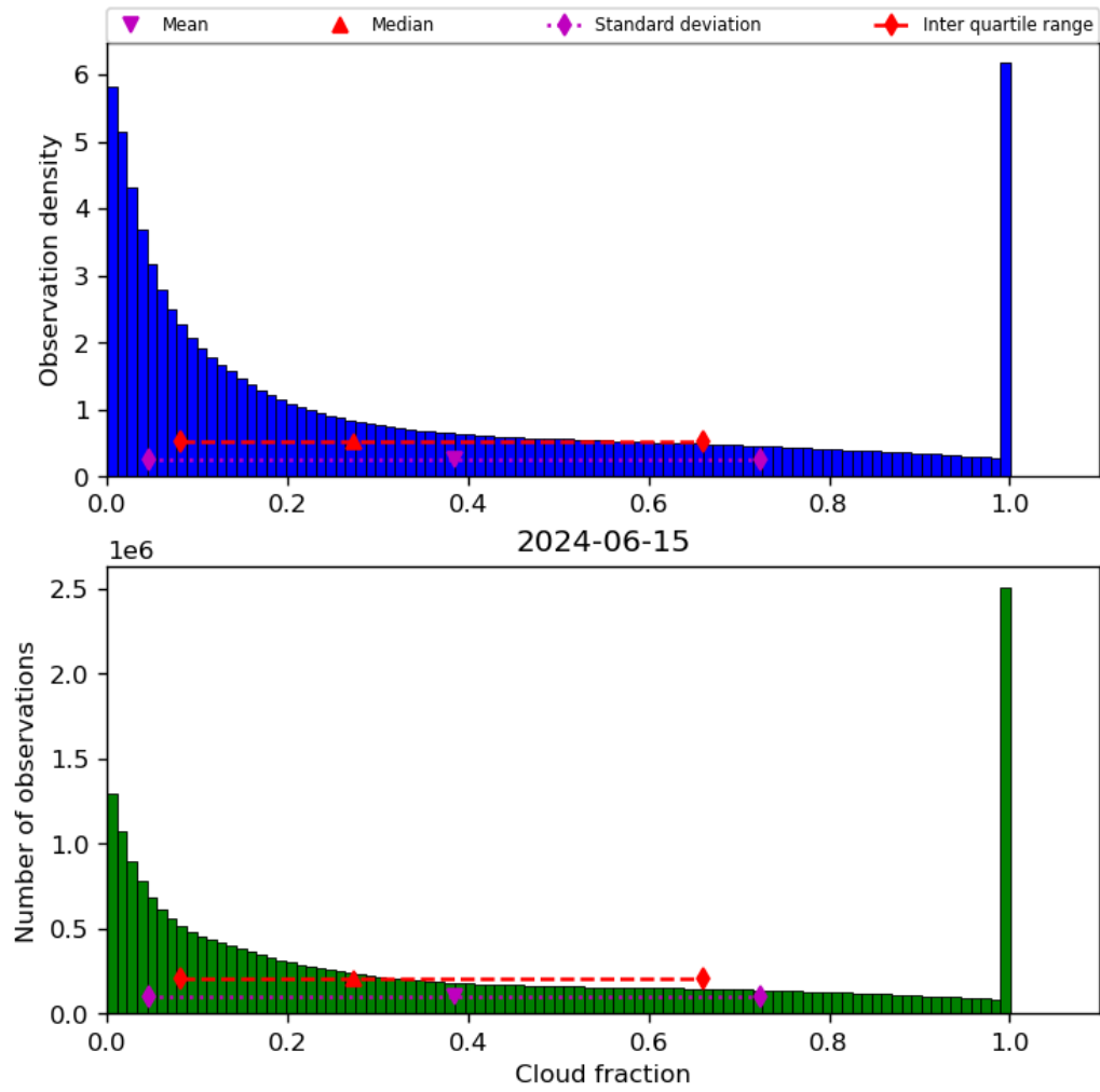
Figure 32: Histogram of “Cloud fraction” for 2024-06-14 to 2024-06-16
