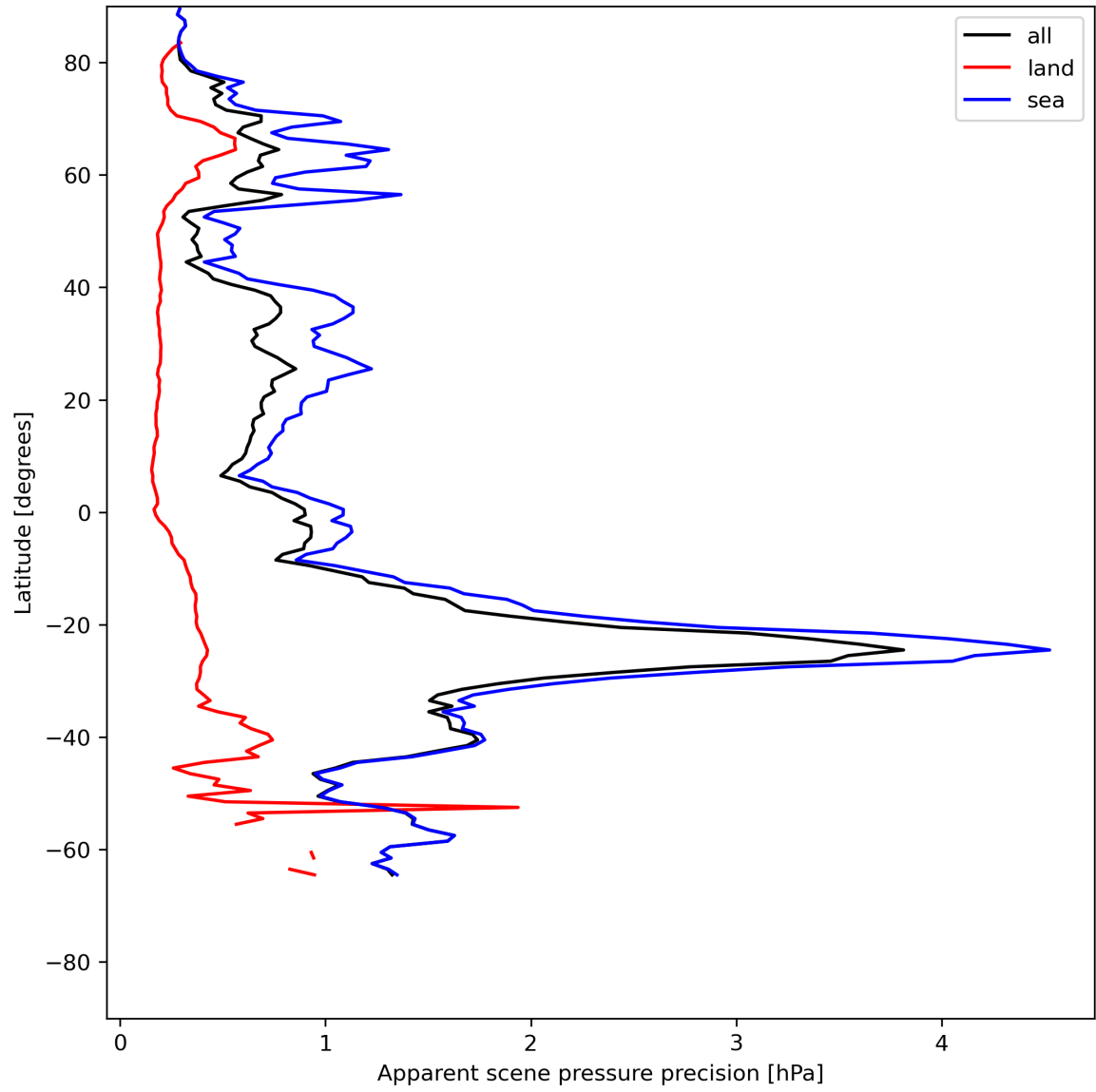
Figure 20: Zonal average of “Apparent scene pressure precision” for 2024-06-14 to 2024-06-16.
