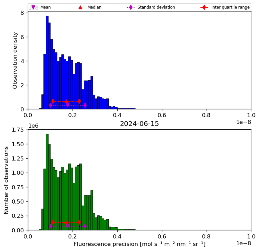
Figure 41: Histogram of “Fluorescence precision” for 2024-06-14 to 2024-06-16
