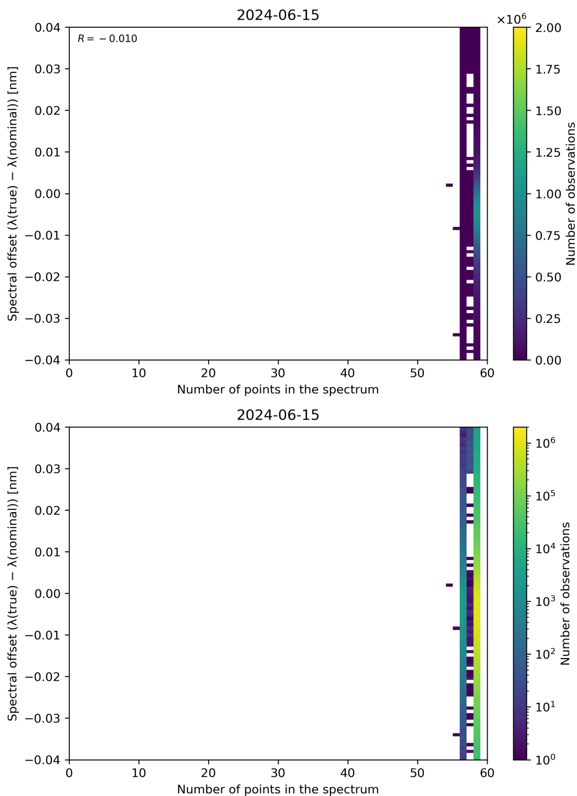
Figure 101: Scatter density plot of “Number of points in the spectrum” against “Spectral offset ( \lambda(\text{true}) - \lambda(\text{nominal}) )” for 2024-06-14 to 2024-06-16.
