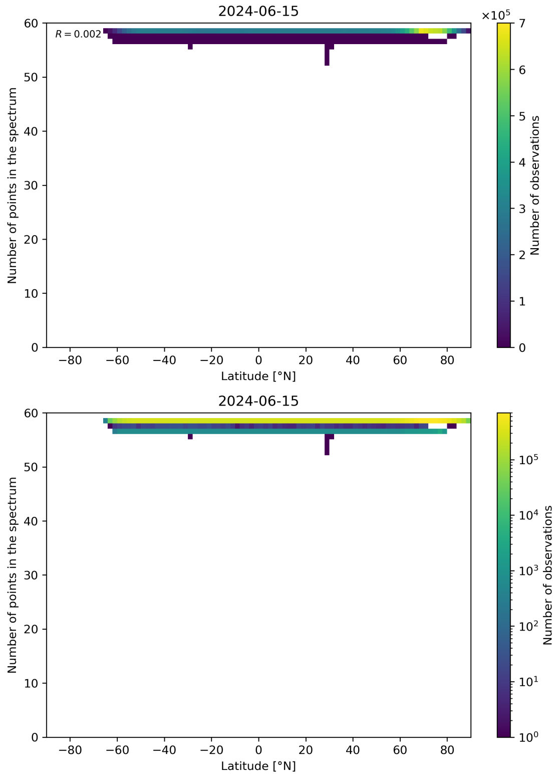
Figure 94: Scatter density plot of “Latitude” against “Number of points in the spectrum” for 2024-06-14 to 2024-06-16.
