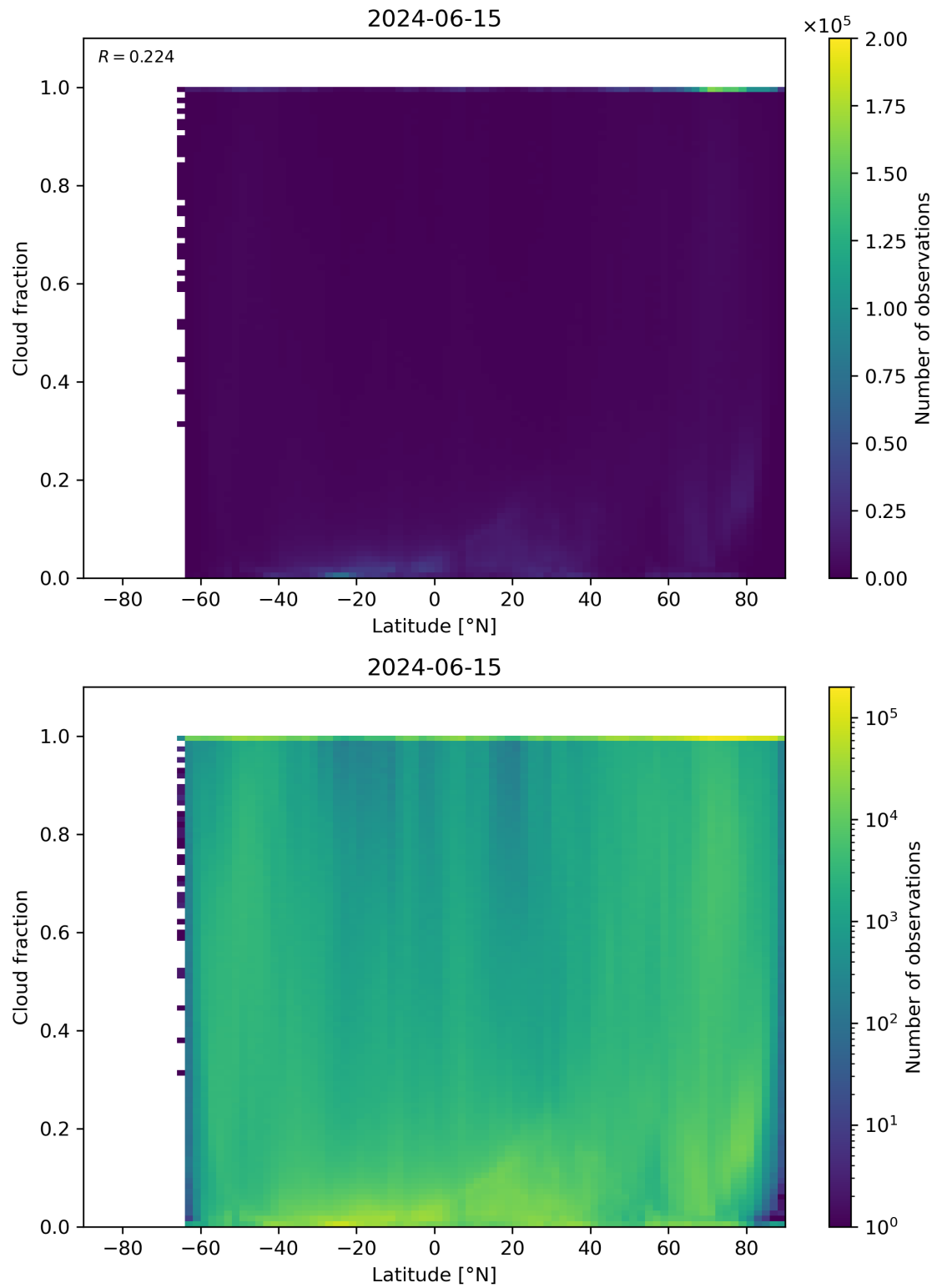
Figure 90: Scatter density plot of “Latitude” against “Cloud fraction” for 2024-06-14 to 2024-06-16.
