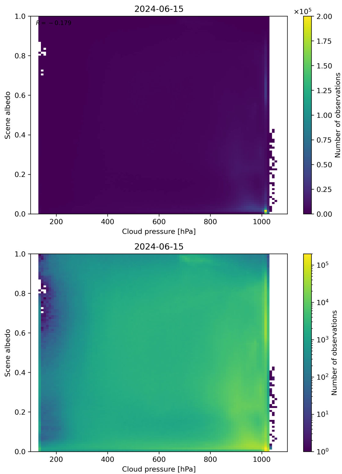
Figure 83: Scatter density plot of “Cloud pressure” against “Scene albedo” for 2024-06-14 to 2024-06-16.
