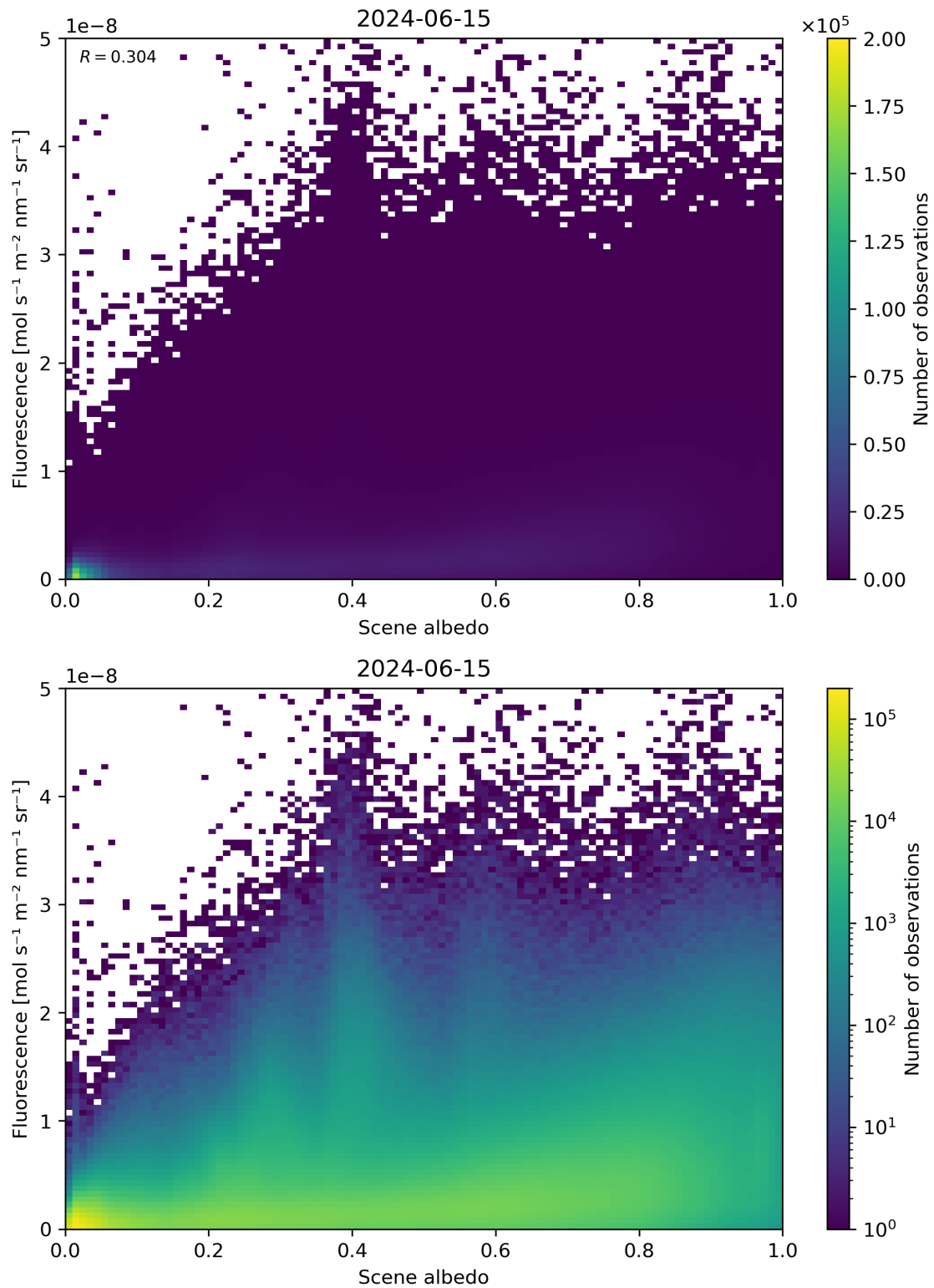
Figure 104: Scatter density plot of “Scene albedo” against “Fluorescence” for 2024-06-14 to 2024-06-16.
