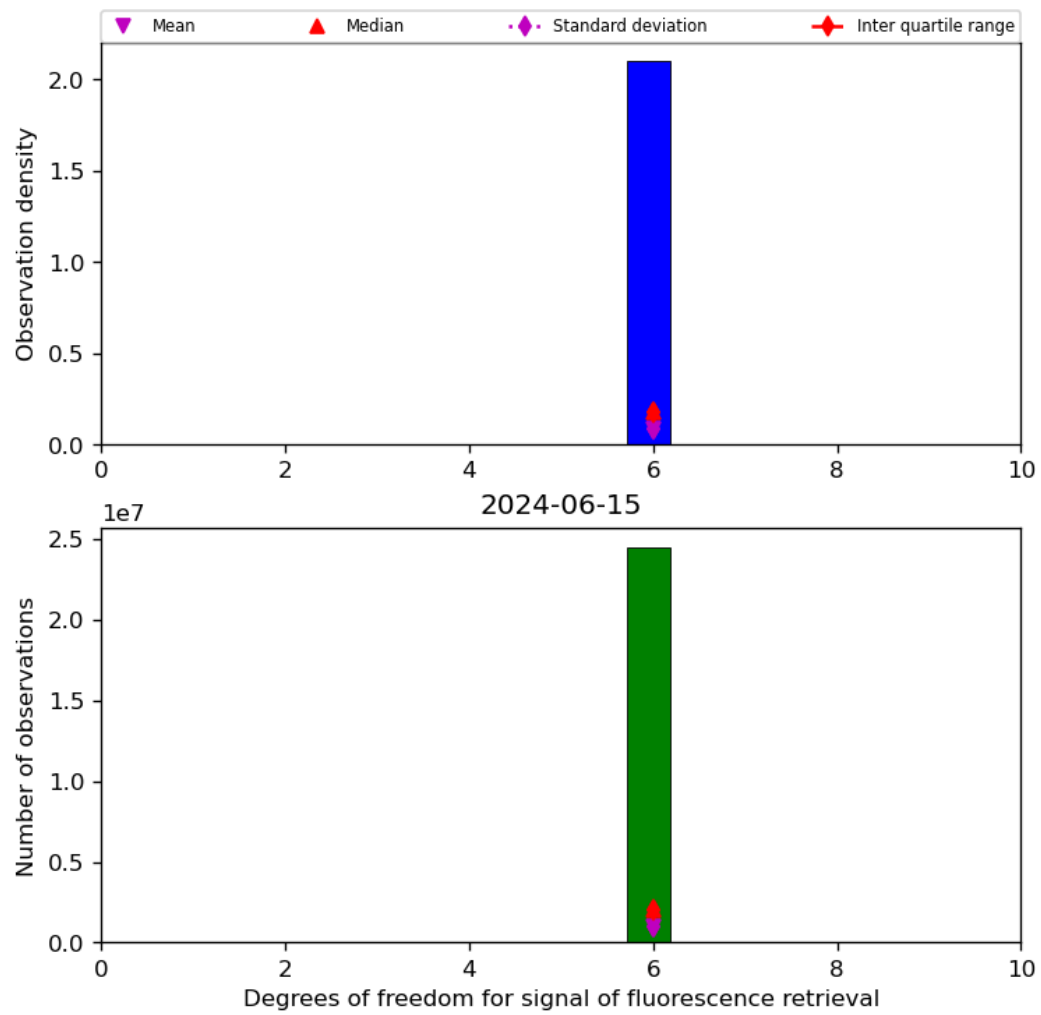
Figure 43: Histogram of “Degrees of freedom for signal of fluorescence retrieval” for 2024-06-14 to 2024-06-16
