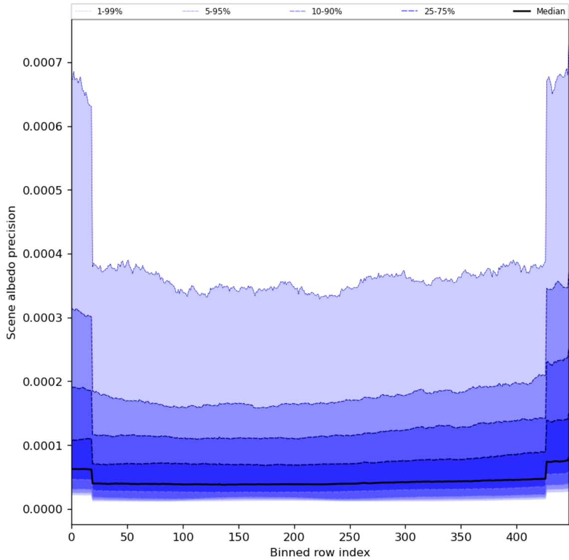
Figure 52: Along track statistics of “Scene albedo precision” for 2024-06-14 to 2024-06-16
