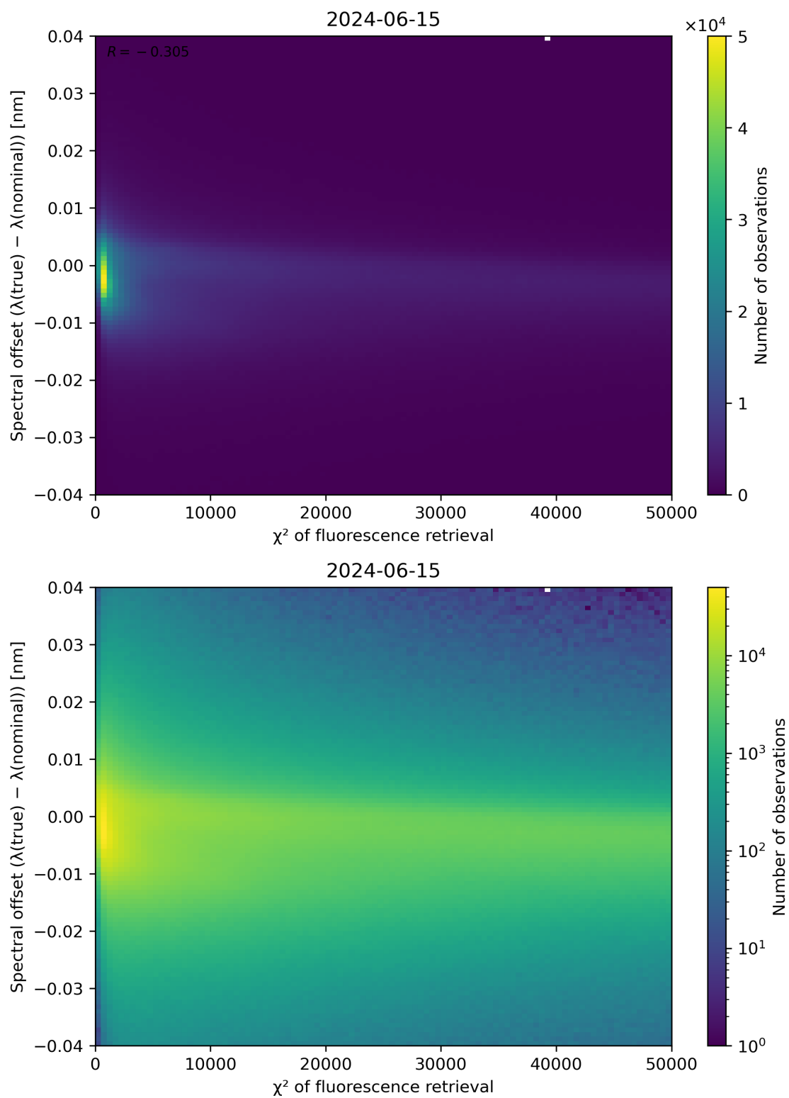
Figure 69: Scatter density plot of " \chi^2 of fluorescence retrieval" against "Spectral offset ( \lambda(\text{true}) - \lambda(\text{nominal})) " for 2024-06-14 to 2024-06-16.
