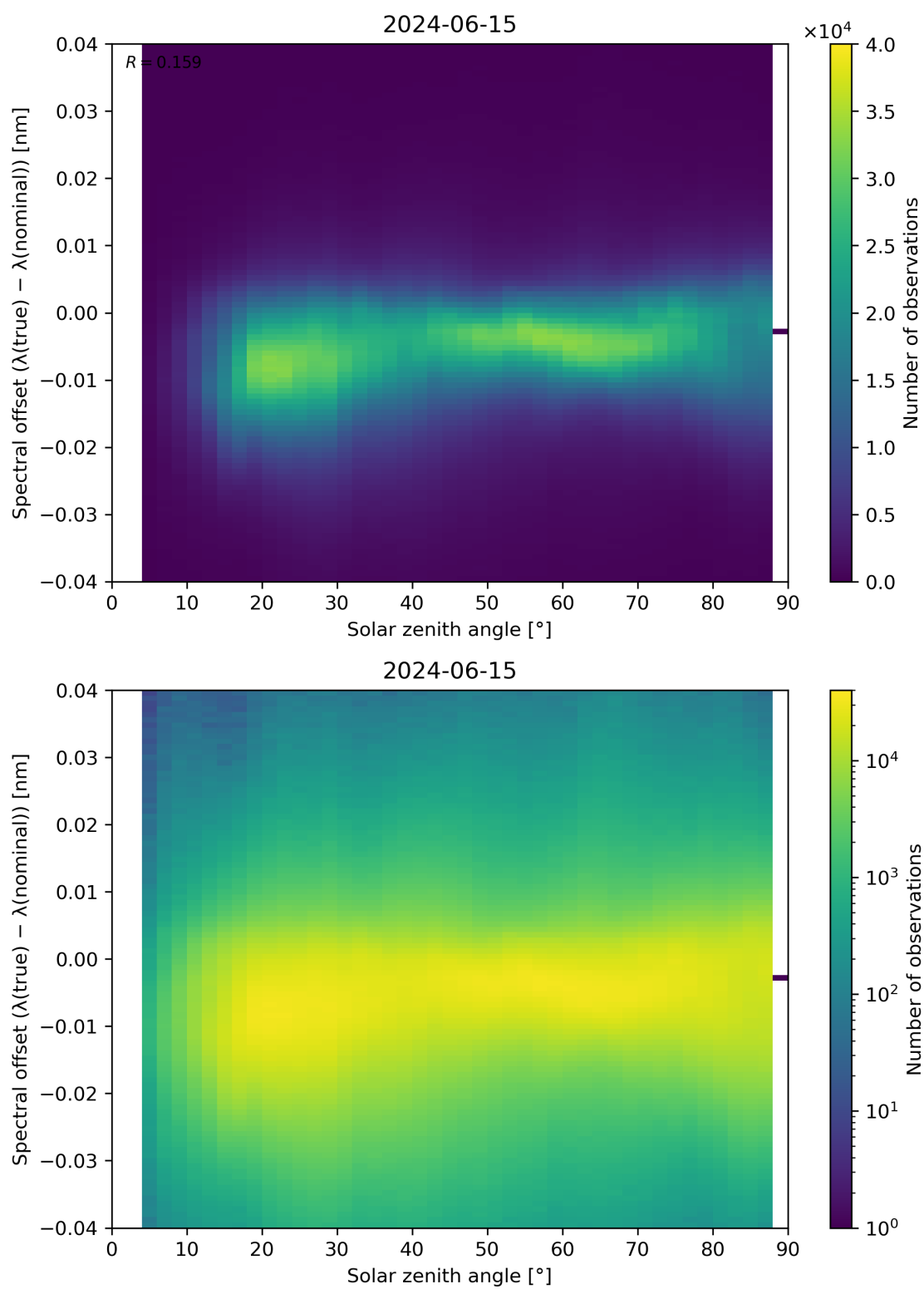
Figure 117: Scatter density plot of “Solar zenith angle” against “Spectral offset ( \lambda(\text{true}) - \lambda(\text{nominal}) )” for 2024-06-14 to 2024-06-16.
