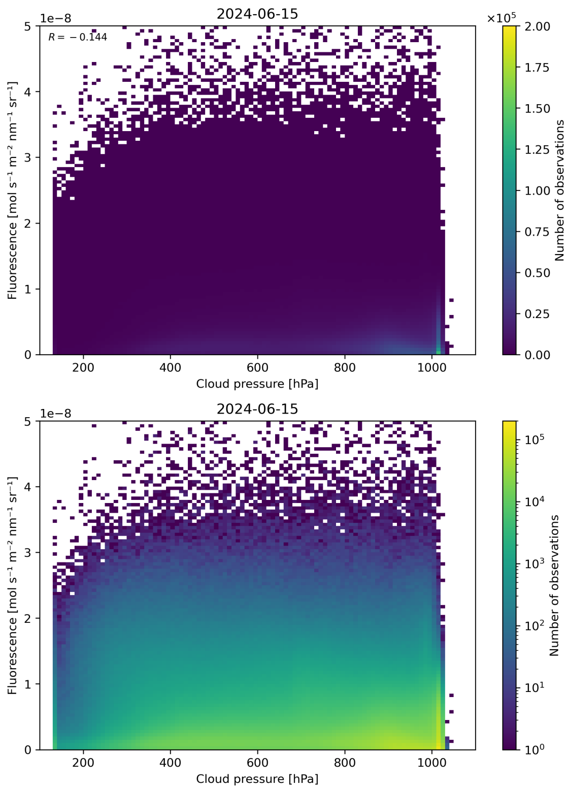
Figure 80: Scatter density plot of “Cloud pressure” against “Fluorescence” for 2024-06-14 to 2024-06-16.
