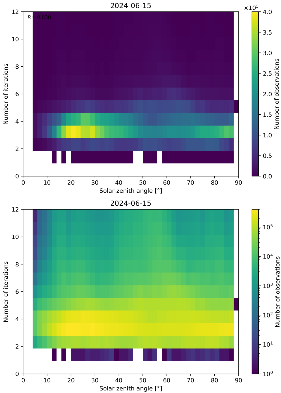
Figure 114: Scatter density plot of “Solar zenith angle” against “Number of iterations” for 2024-06-14 to 2024-06-16.
