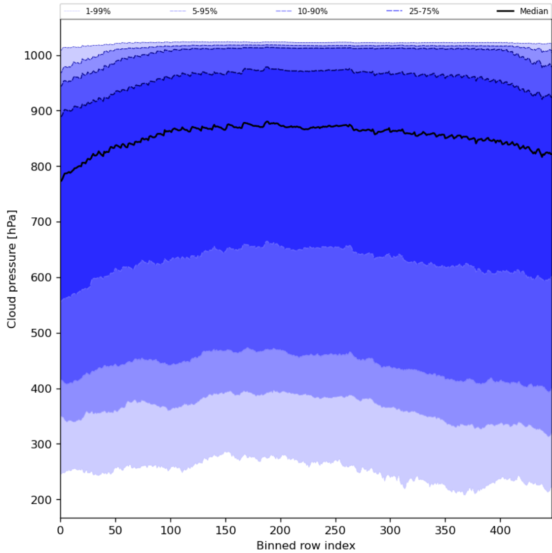
Figure 47: Along track statistics of “Cloud pressure” for 2024-06-14 to 2024-06-16
