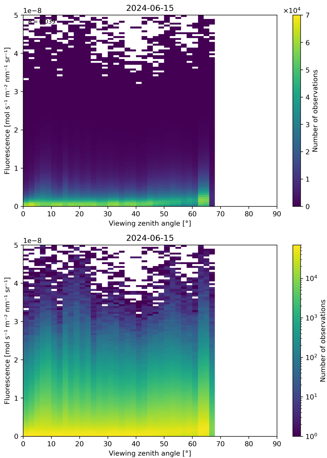
Figure 122: Scatter density plot of “Viewing zenith angle” against “Fluorescence” for 2024-06-14 to 2024-06-16.
