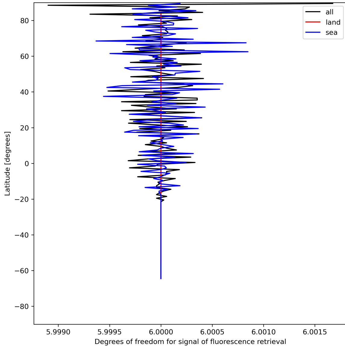
Figure 26: Zonal average of “Degrees of freedom for signal of fluorescence retrieval” for 2024-06-14 to 2024-06-16.
