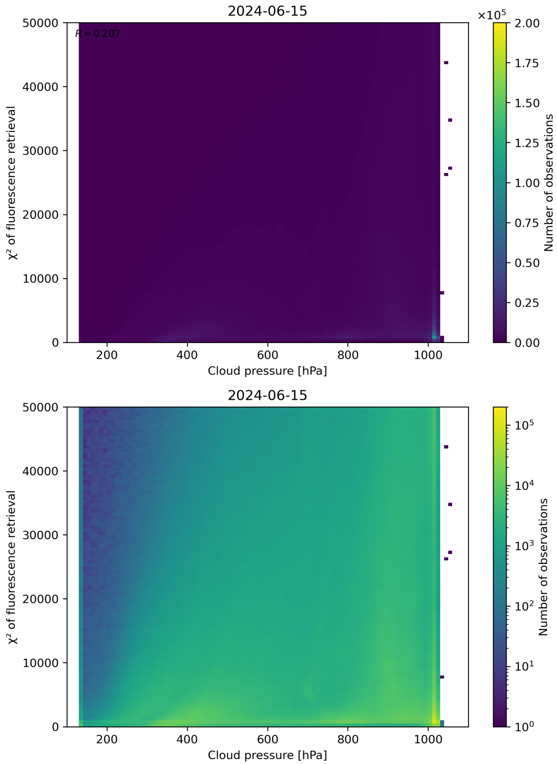
Figure 78: Scatter density plot of “Cloud pressure” against “ \chi^2 of fluorescence retrieval” for 2024-06-14 to 2024-06-16.
