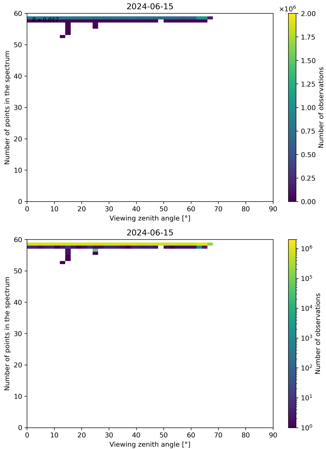
Figure 125: Scatter density plot of “Viewing zenith angle” against “Number of points in the spectrum” for 2024-06-14 to 2024-06-16.
