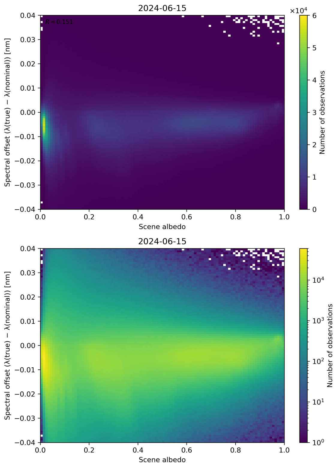
Figure 107: Scatter density plot of “Scene albedo” against “Spectral offset ( \lambda(\text{true}) - \lambda(\text{nominal}) )” for 2024-06-14 to 2024-06-16.
