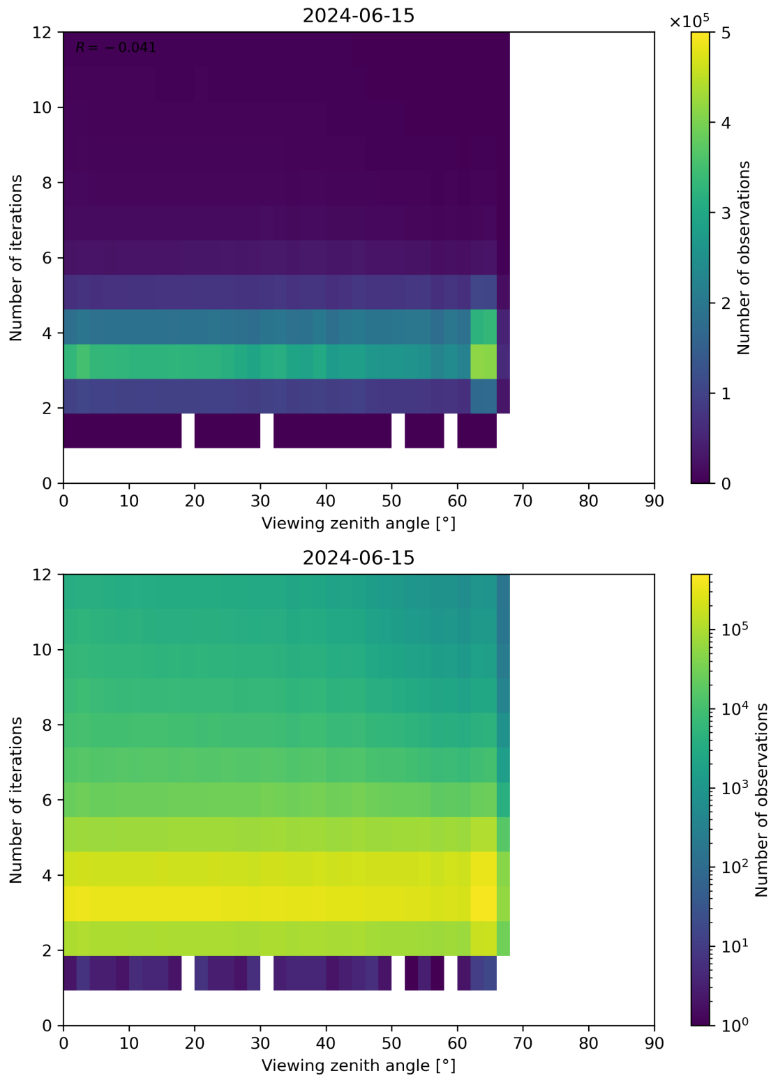
Figure 124: Scatter density plot of “Viewing zenith angle” against “Number of iterations” for 2024-06-14 to 2024-06-16.
