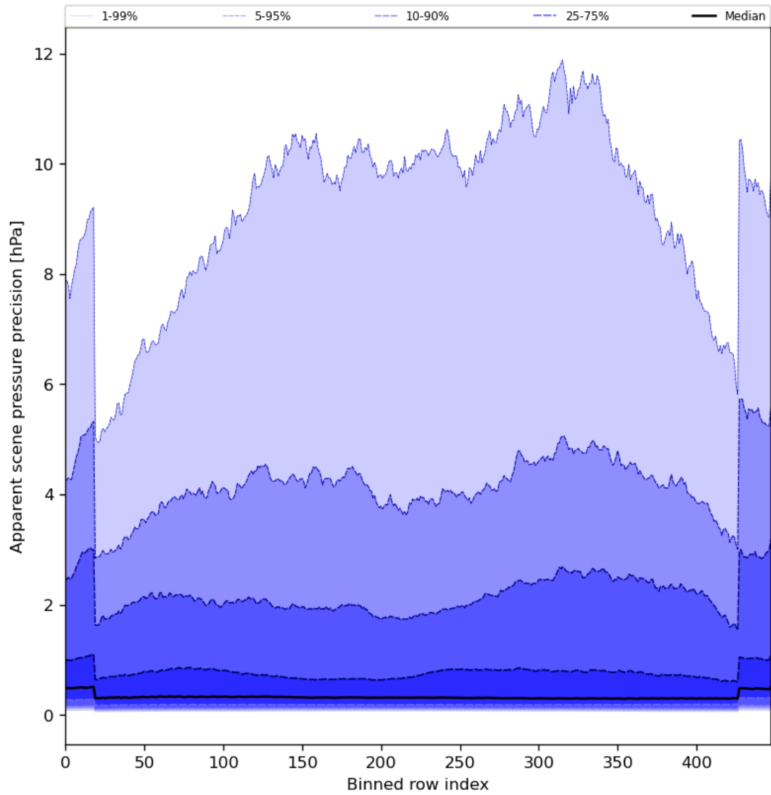
Figure 54: Along track statistics of “Apparent scene pressure precision” for 2024-06-14 to 2024-06-16
