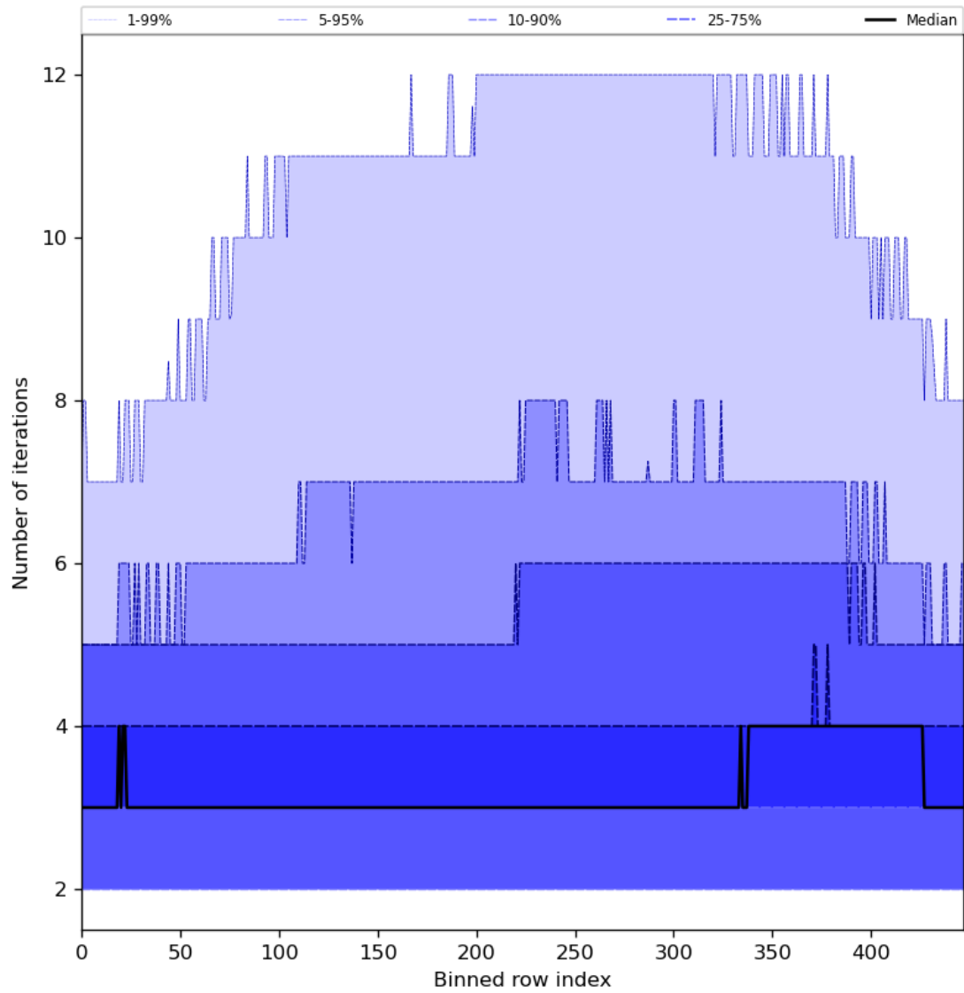
Figure 56: Along track statistics of “Number of iterations” for 2024-06-14 to 2024-06-16
