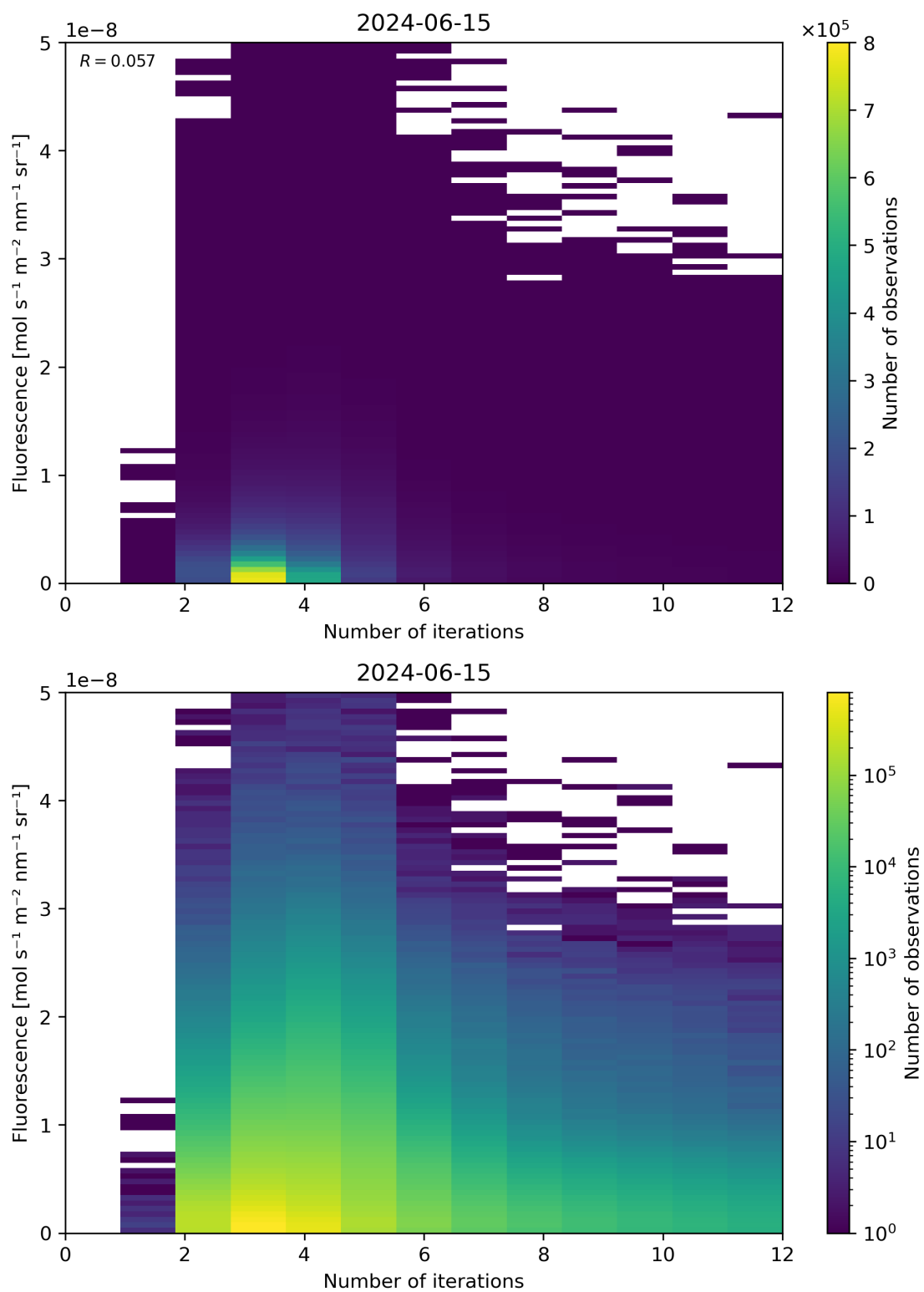
Figure 98: Scatter density plot of “Number of iterations” against “Fluorescence” for 2024-06-14 to 2024-06-16.
