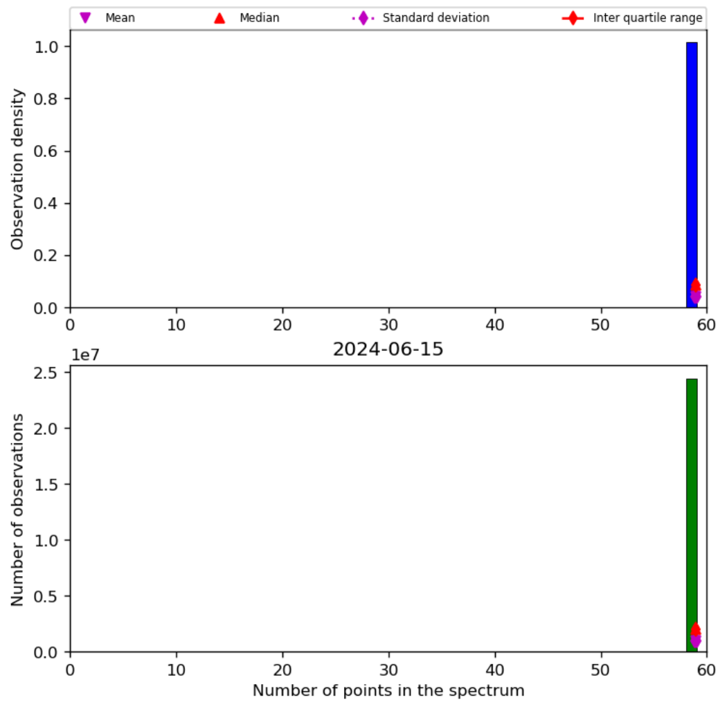
Figure 44: Histogram of “Number of points in the spectrum” for 2024-06-14 to 2024-06-16
