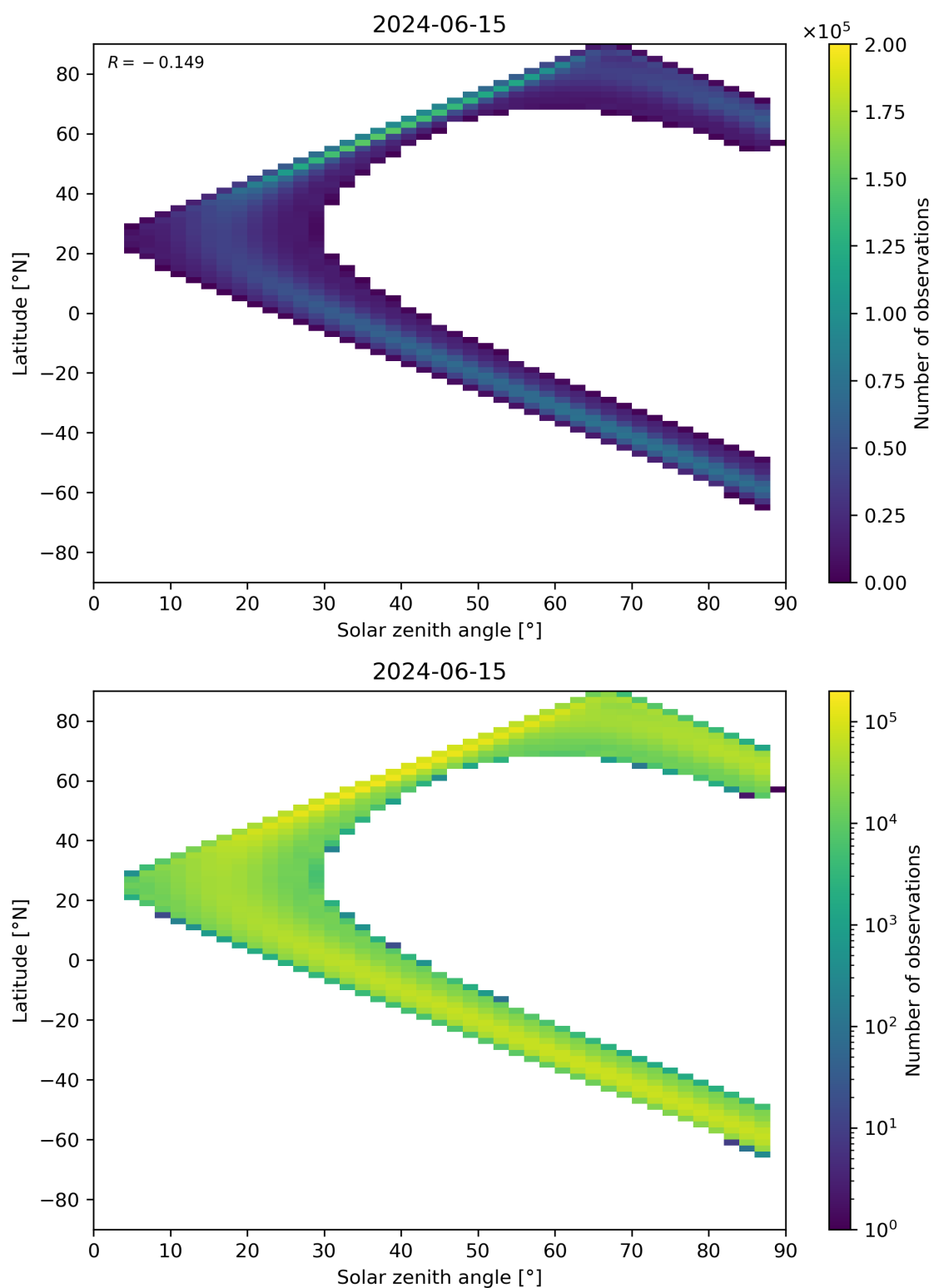
Figure 113: Scatter density plot of “Solar zenith angle” against “Latitude” for 2024-06-14 to 2024-06-16.
