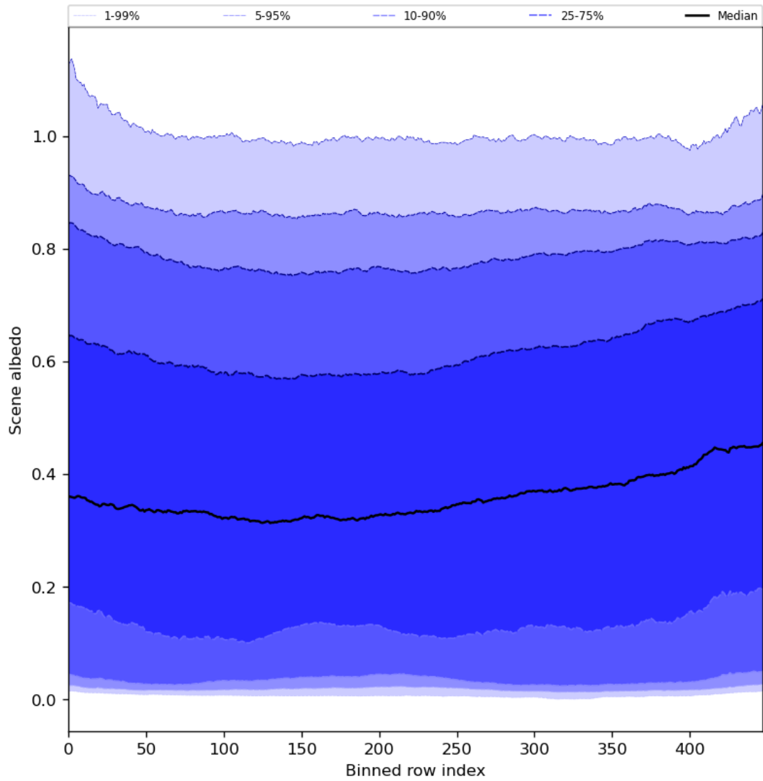
Figure 51: Along track statistics of “Scene albedo” for 2024-06-14 to 2024-06-16
