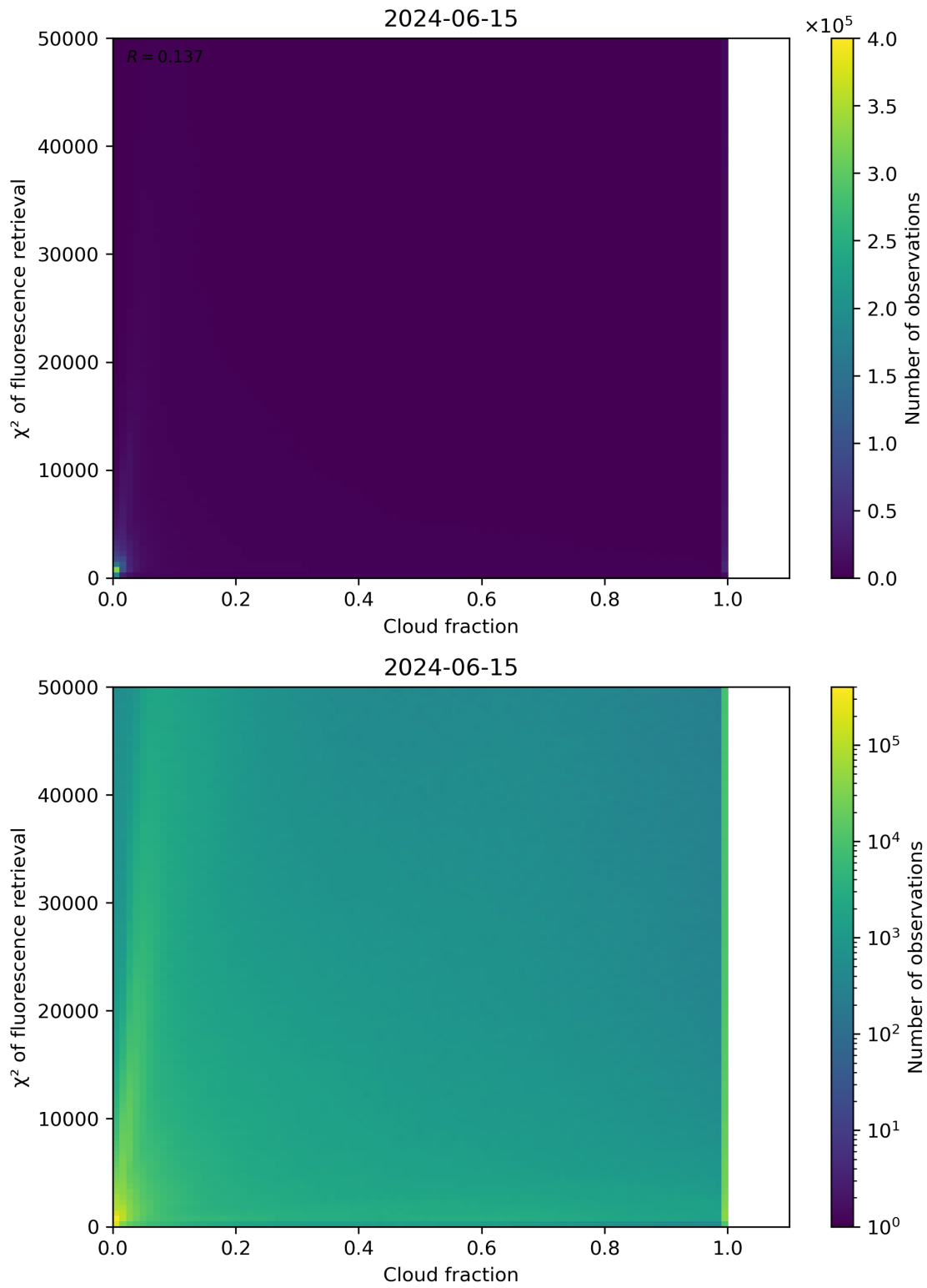
Figure 71: Scatter density plot of “Cloud fraction” against “ \chi^2 of fluorescence retrieval” for 2024-06-14 to 2024-06-16.
