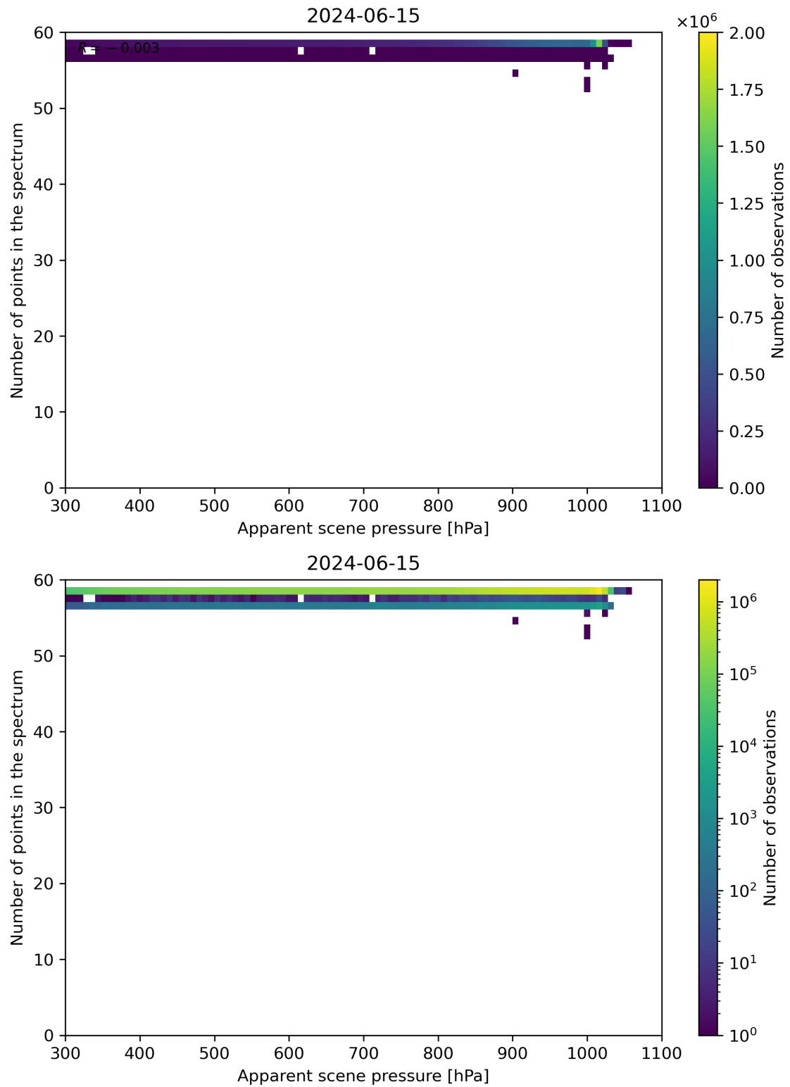
Figure 66: Scatter density plot of “Apparent scene pressure” against “Number of points in the spectrum” for 2024-06-14 to 2024-06-16.
