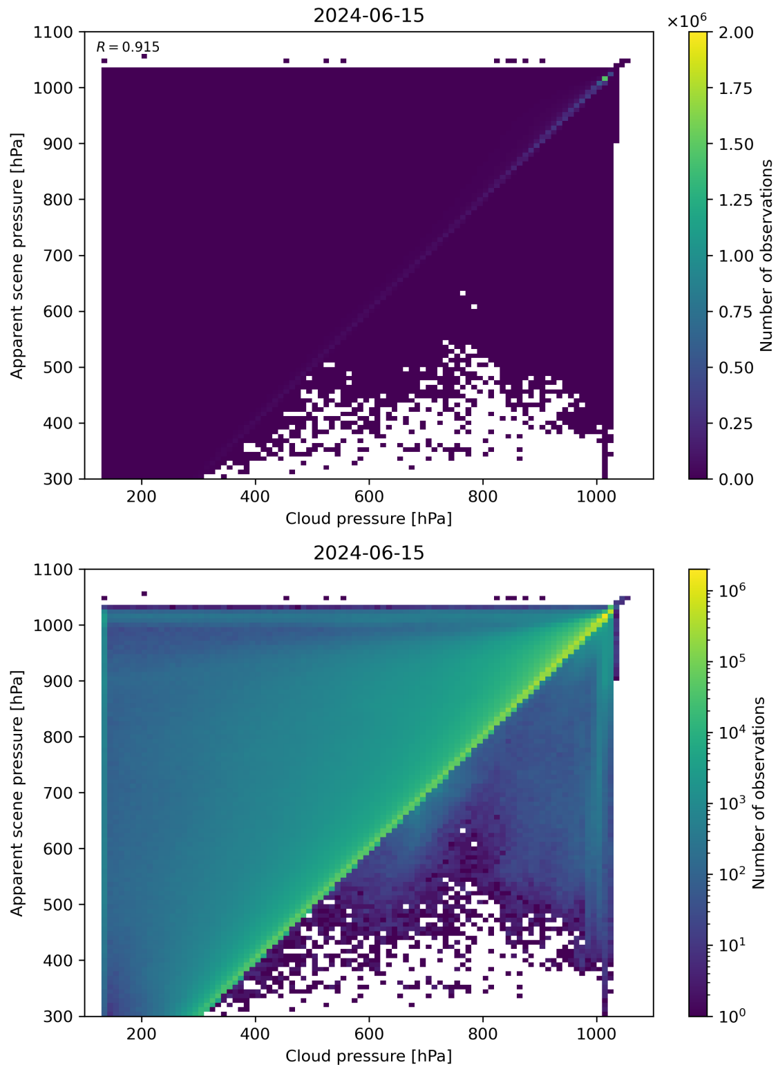
Figure 77: Scatter density plot of “Cloud pressure” against “Apparent scene pressure” for 2024-06-14 to 2024-06-16.
