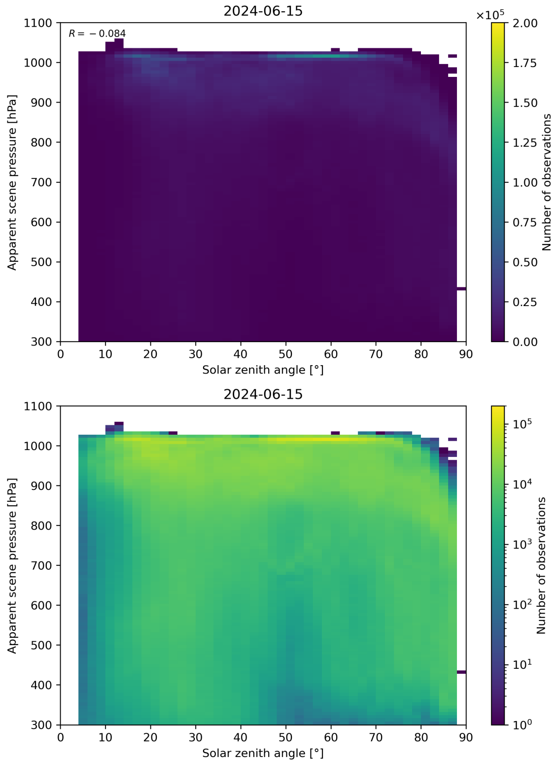
Figure 108: Scatter density plot of “Solar zenith angle” against “Apparent scene pressure” for 2024-06-14 to 2024-06-16.
