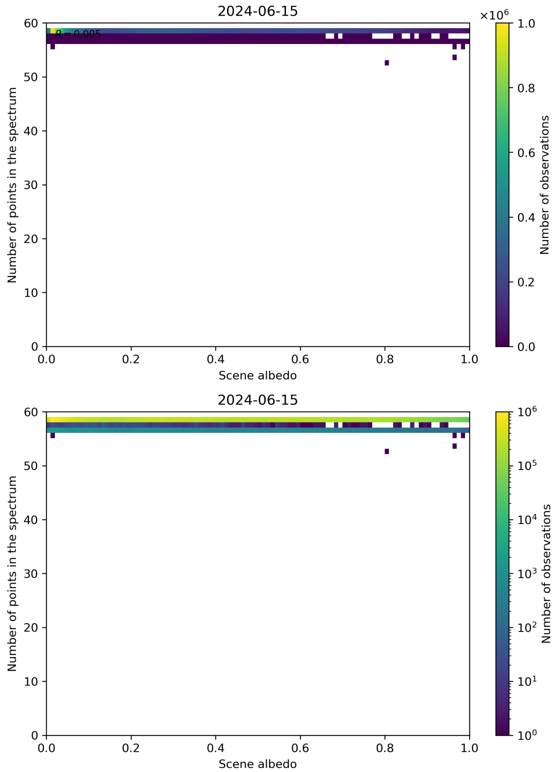
Figure 106: Scatter density plot of “Scene albedo” against “Number of points in the spectrum” for 2024-06-14 to 2024-06-16.
