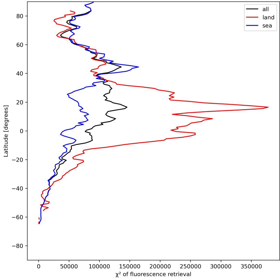
Figure 25: Zonal average of “ \chi^2 of fluorescence retrieval” for 2024-06-14 to 2024-06-16.
