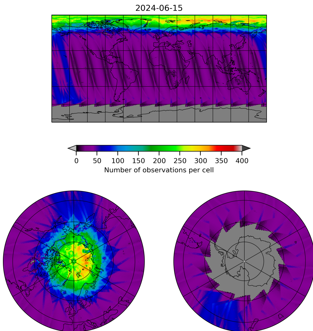
Figure 11: Map of the number of observations for 2024-06-14 to 2024-06-16
