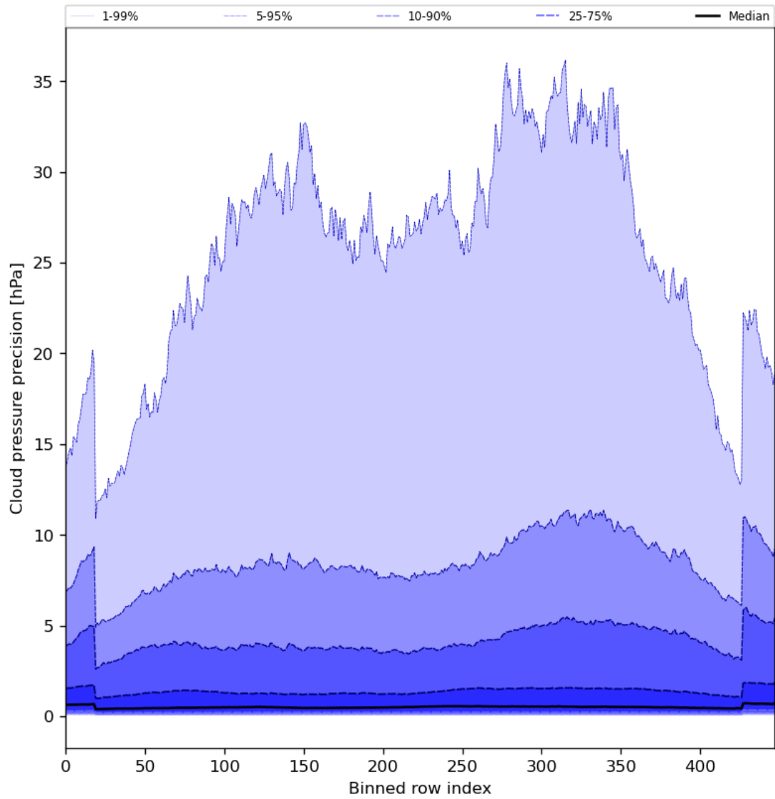
Figure 48: Along track statistics of “Cloud pressure precision” for 2024-06-14 to 2024-06-16
