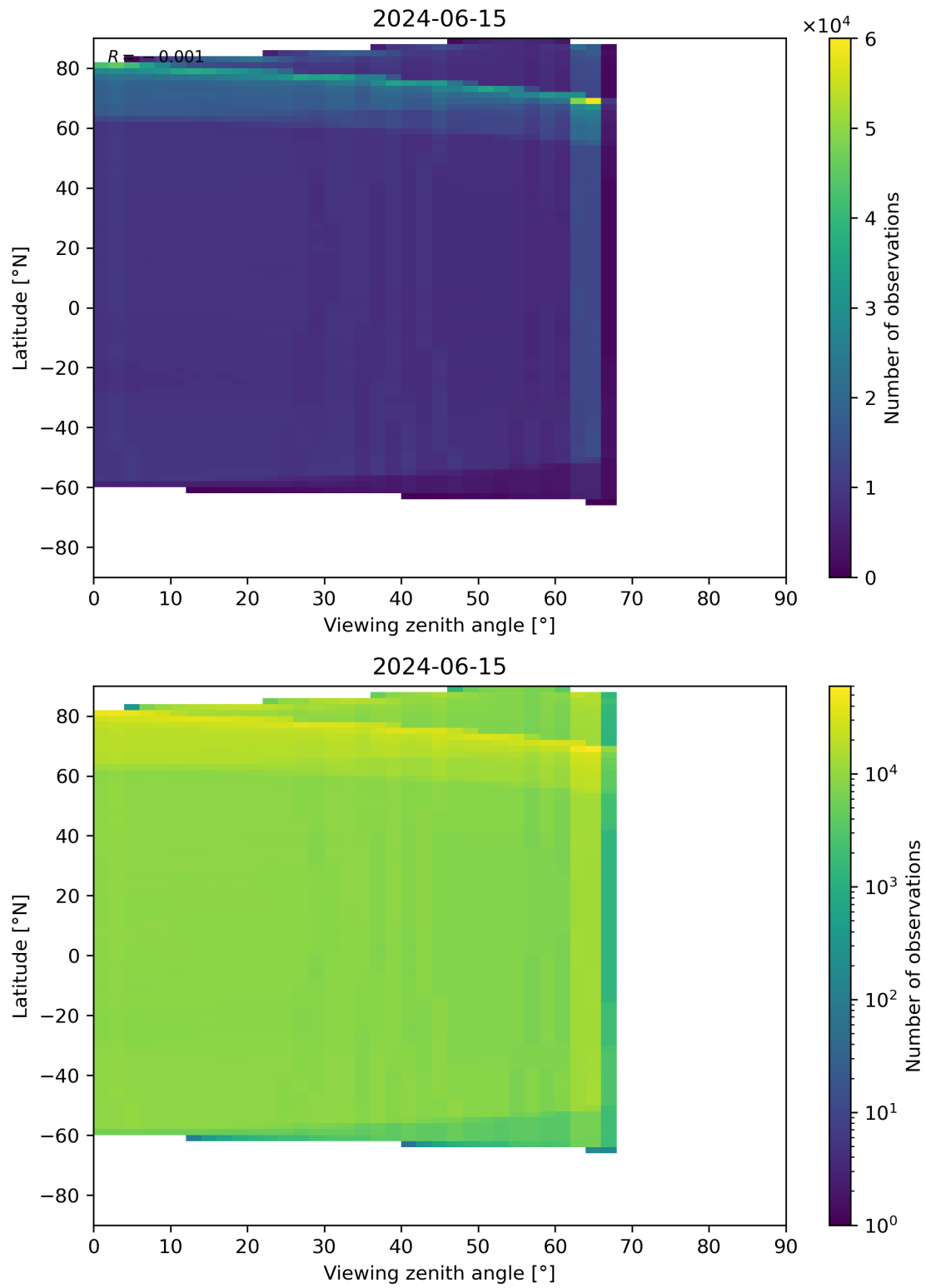
Figure 123: Scatter density plot of “Viewing zenith angle” against “Latitude” for 2024-06-14 to 2024-06-16.
