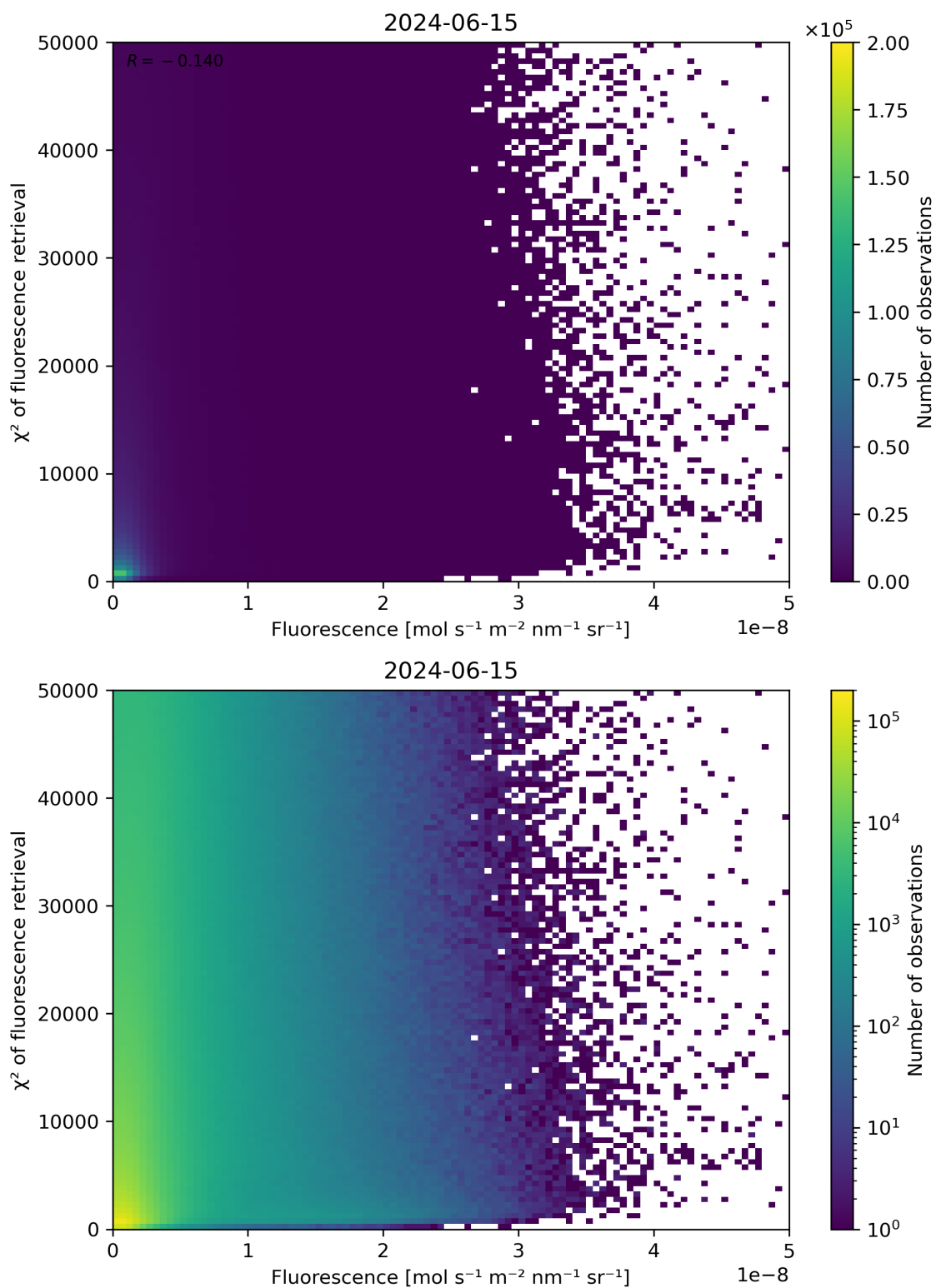
Figure 85: Scatter density plot of “Fluorescence” against “ \chi^2 of fluorescence retrieval” for 2024-06-14 to 2024-06-16.
