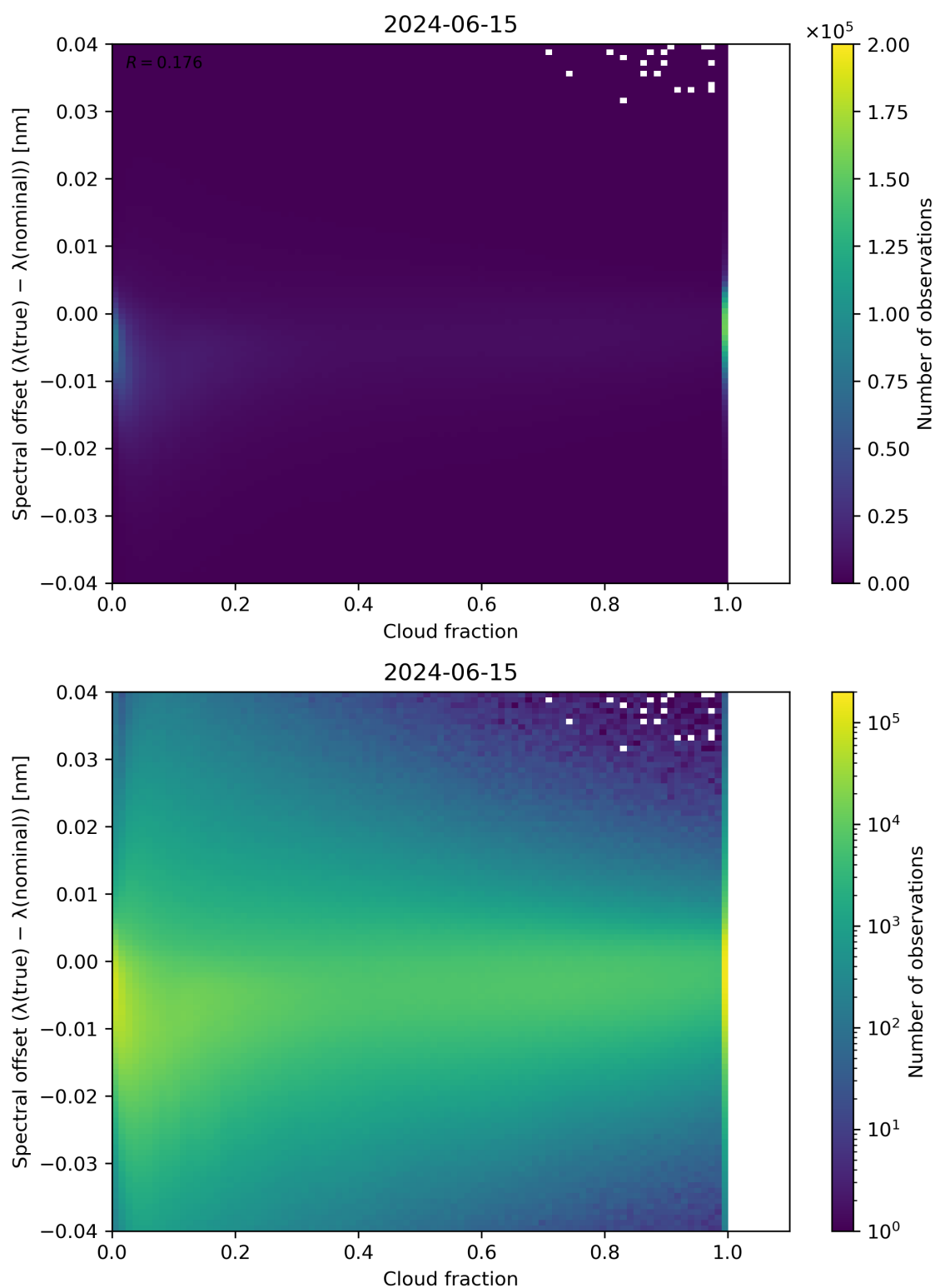
Figure 76: Scatter density plot of “Cloud fraction” against “Spectral offset ( \lambda(\text{true}) - \lambda(\text{nominal}) )” for 2024-06-14 to 2024-06-16.
