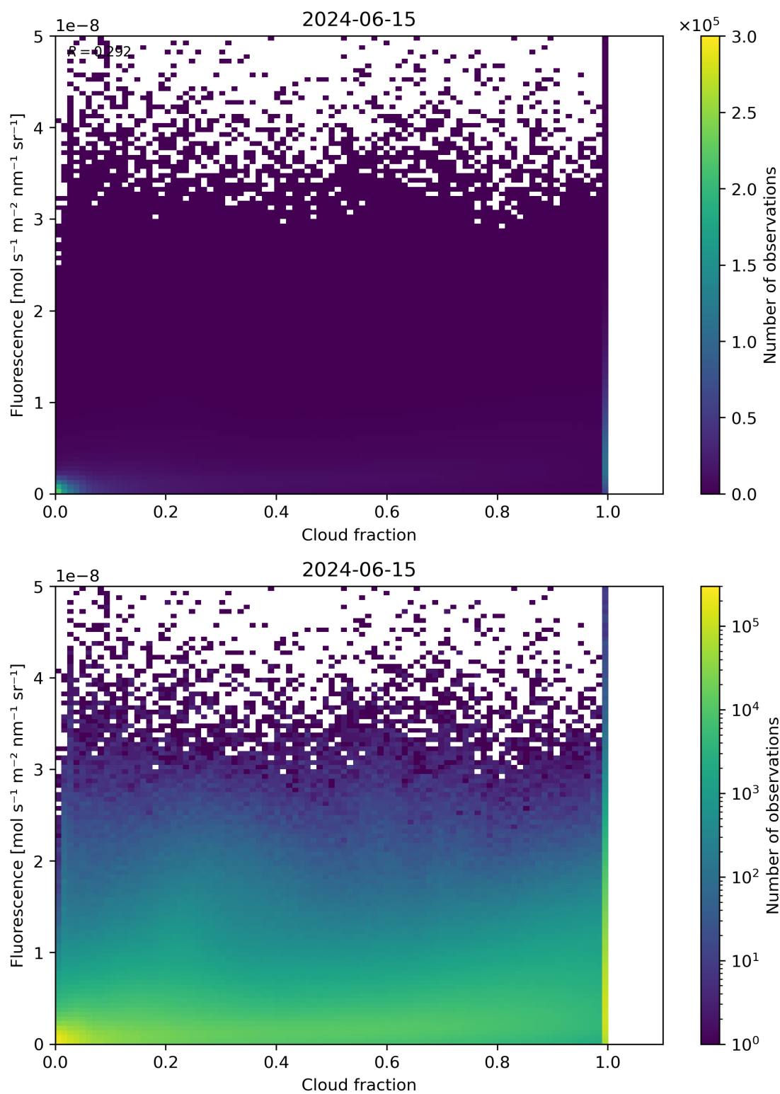
Figure 72: Scatter density plot of "Cloud fraction" against "Fluorescence" for 2024-06-14 to 2024-06-16.
