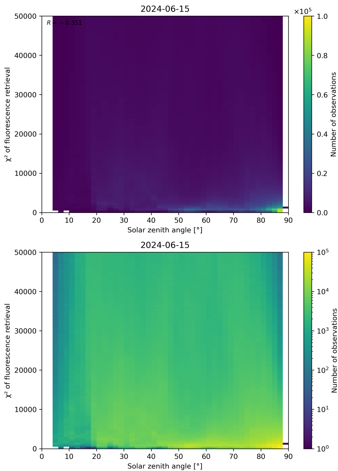
Figure 109: Scatter density plot of “Solar zenith angle” against “ \chi^2 of fluorescence retrieval” for 2024-06-14 to 2024-06-16.
