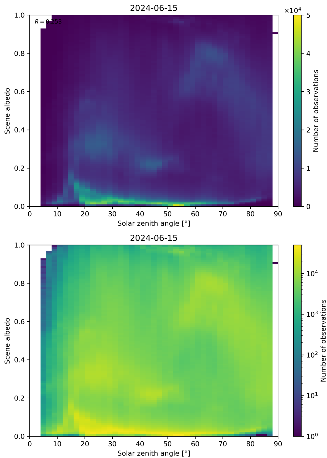
Figure 116: Scatter density plot of “Solar zenith angle” against “Scene albedo” for 2024-06-14 to 2024-06-16.
