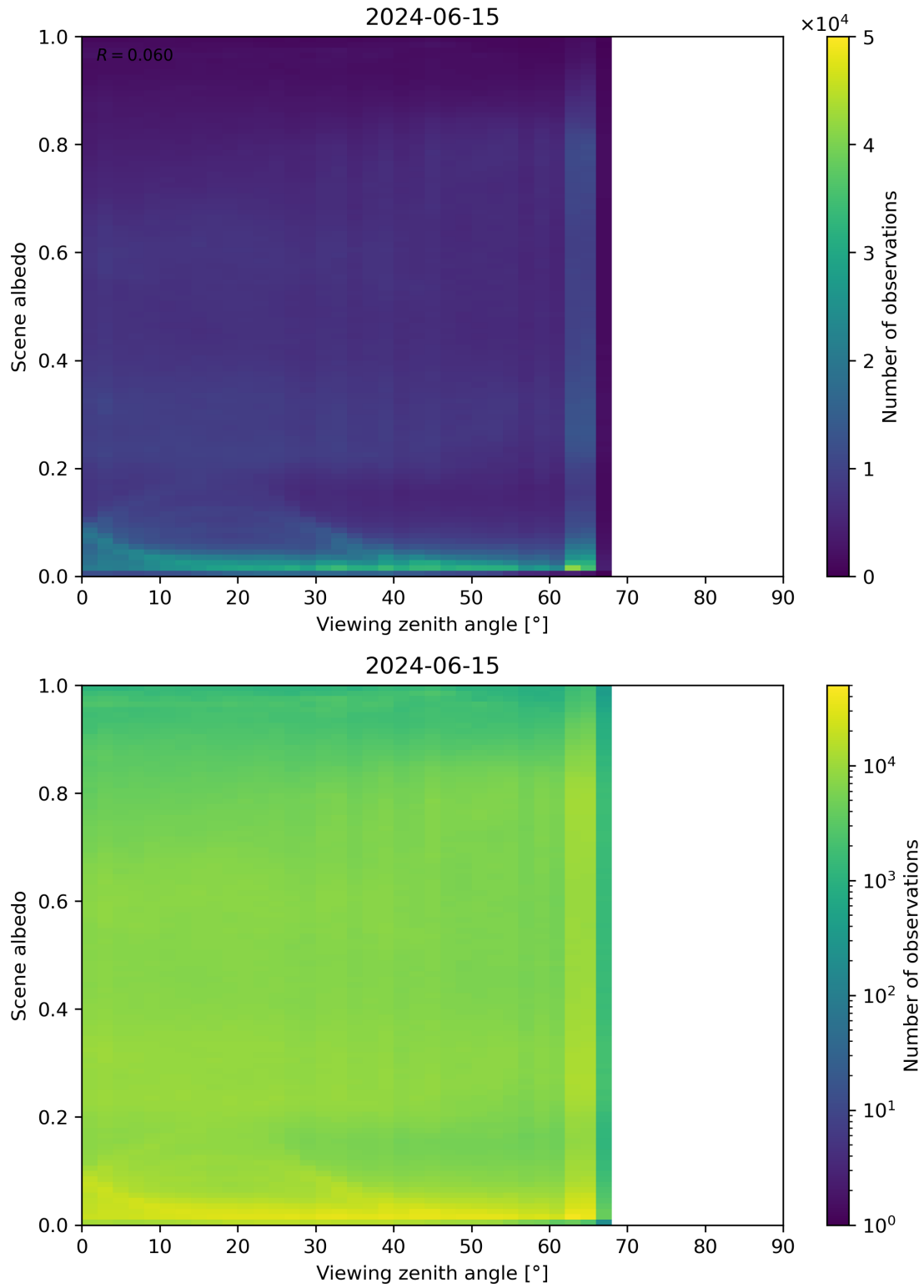
Figure 126: Scatter density plot of “Viewing zenith angle” against “Scene albedo” for 2024-06-14 to 2024-06-16.
