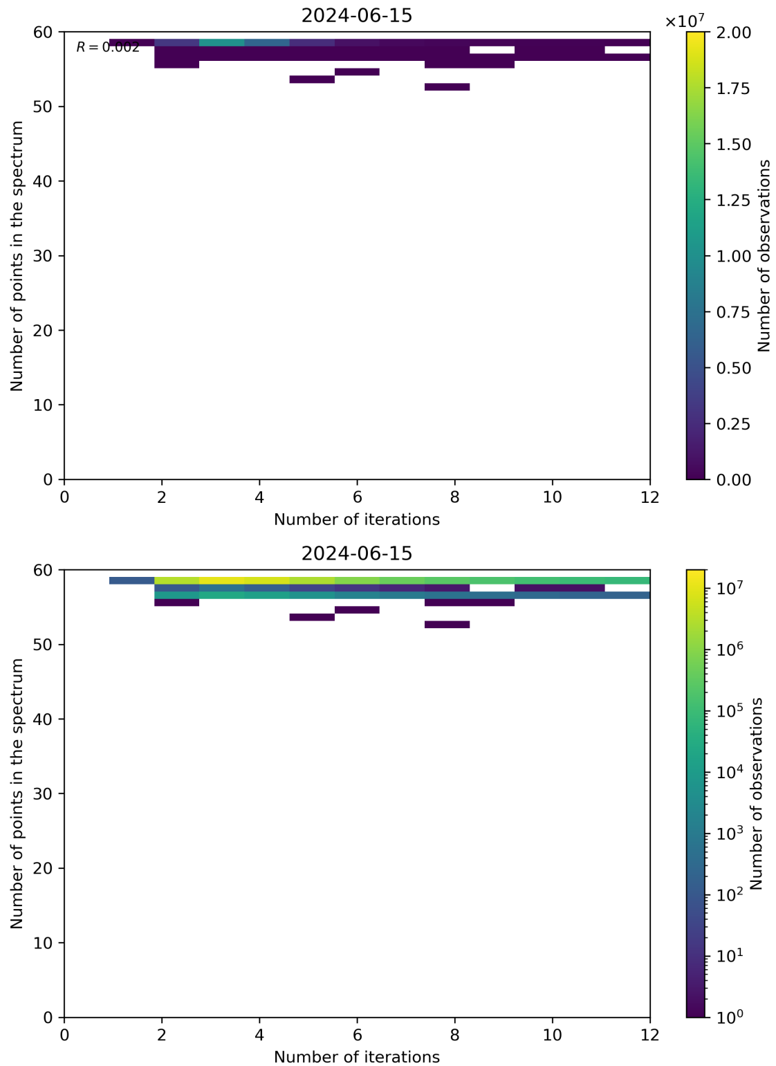
Figure 99: Scatter density plot of “Number of iterations” against “Number of points in the spectrum” for 2024-06-14 to 2024-06-16.
