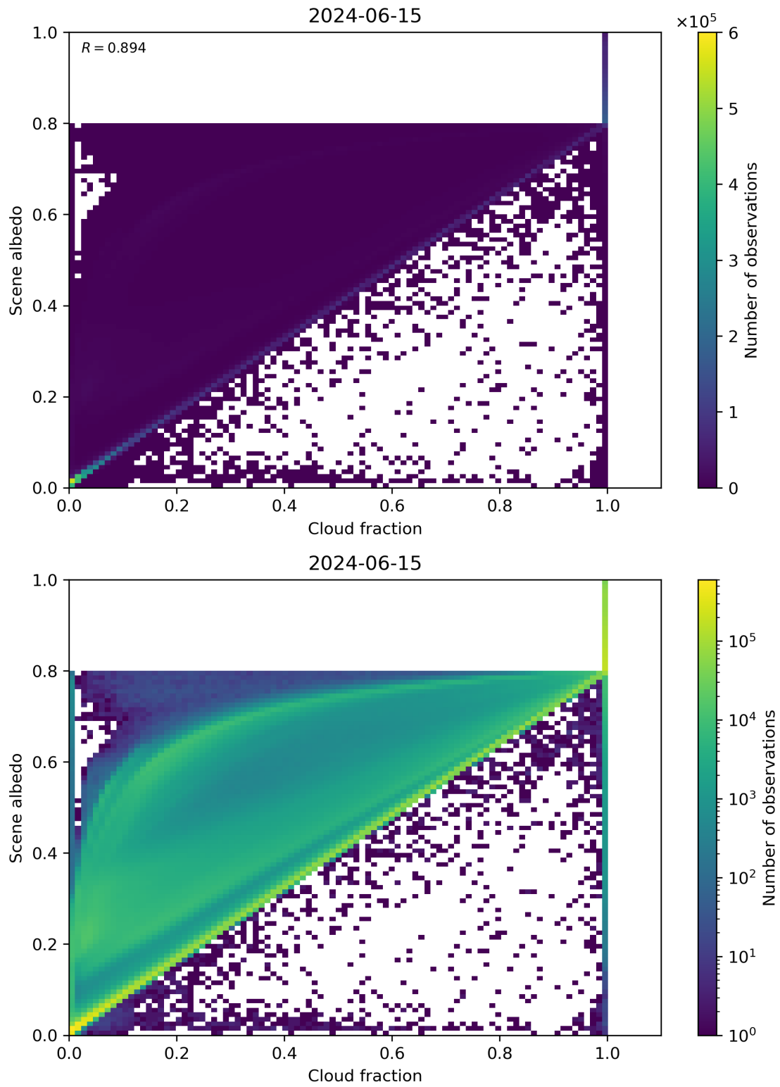
Figure 75: Scatter density plot of “Cloud fraction” against “Scene albedo” for 2024-06-14 to 2024-06-16.
