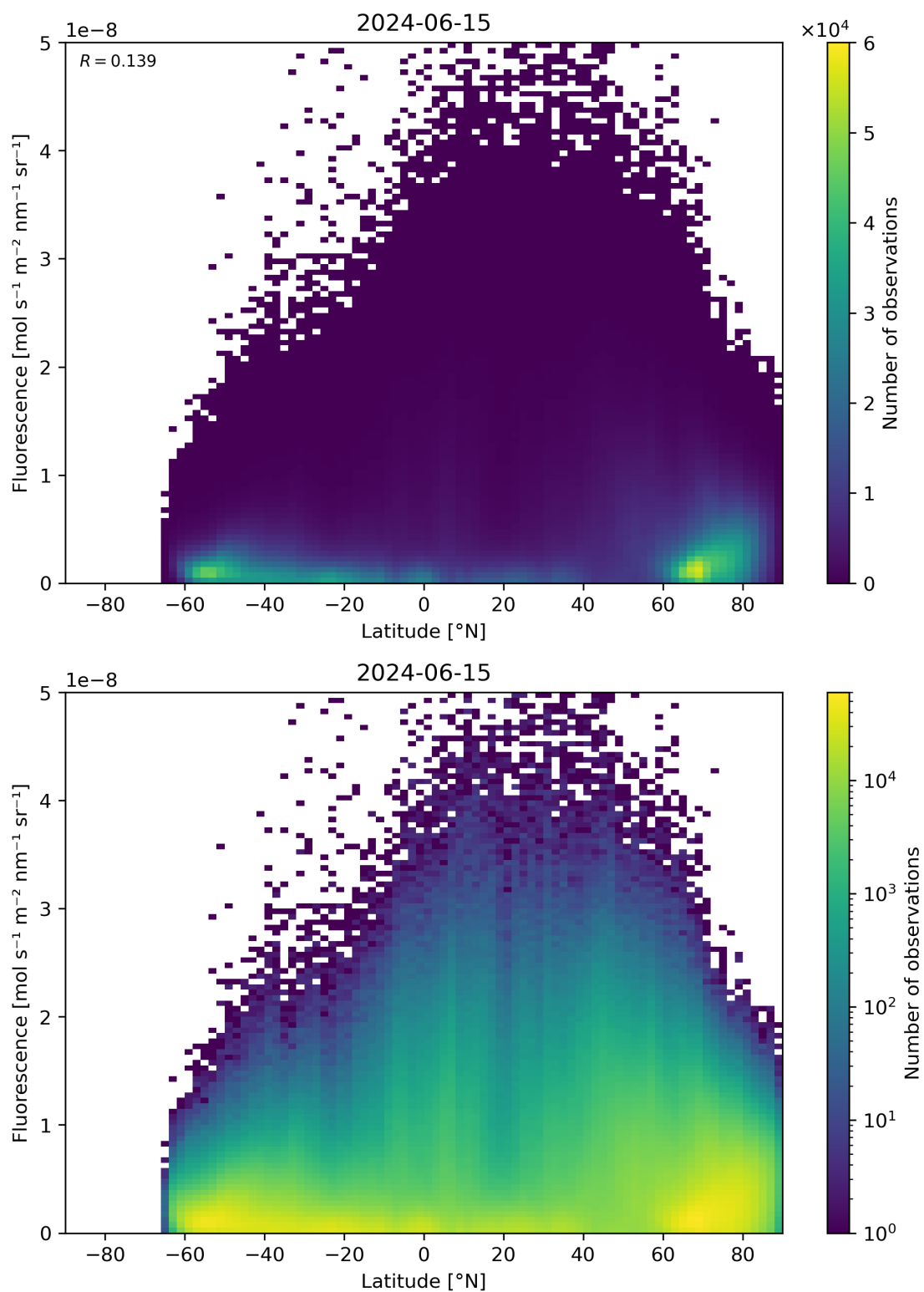
Figure 92: Scatter density plot of “Latitude” against “Fluorescence” for 2024-06-14 to 2024-06-16.
