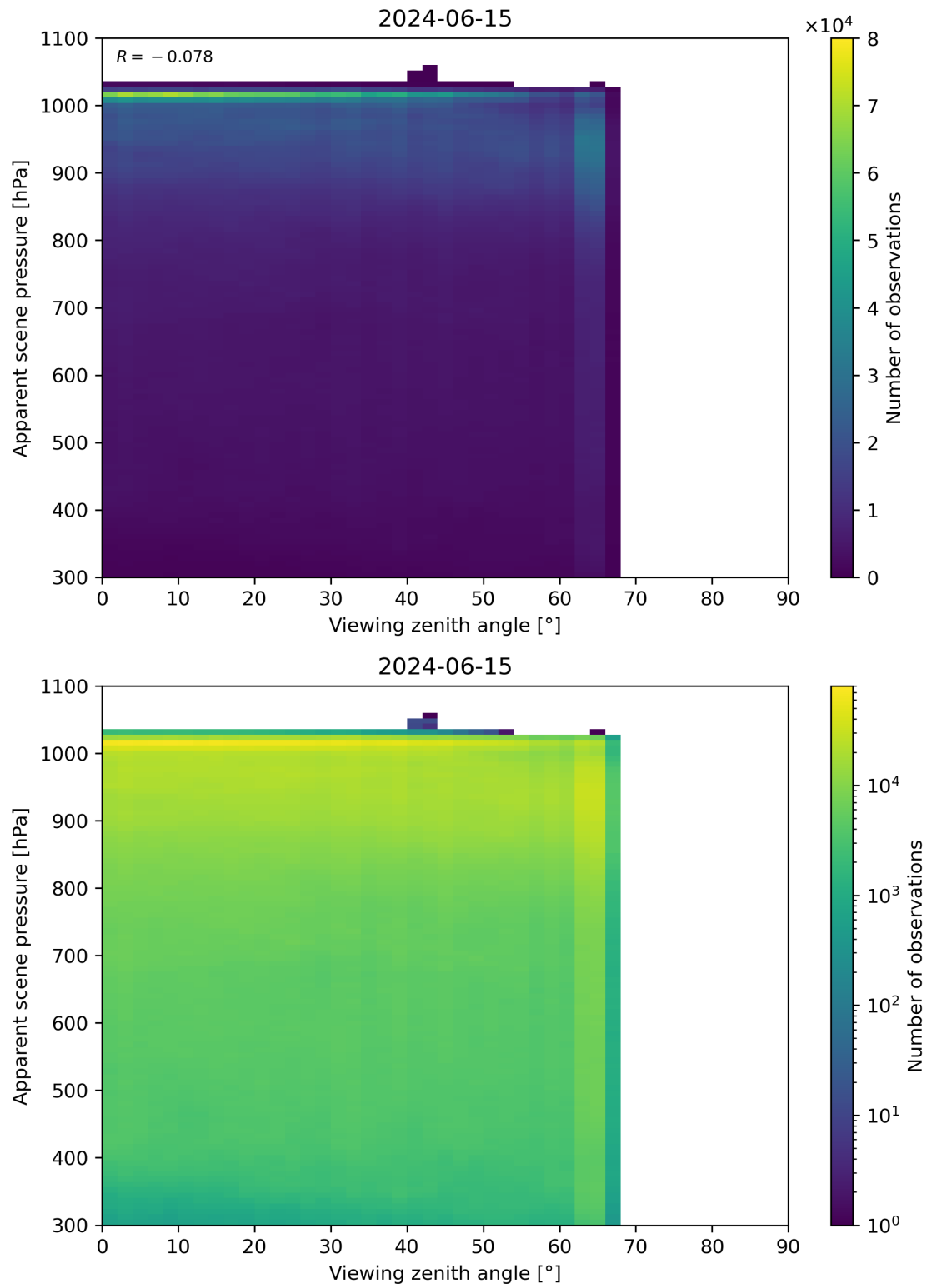
Figure 118: Scatter density plot of “Viewing zenith angle” against “Apparent scene pressure” for 2024-06-14 to 2024-06-16.
