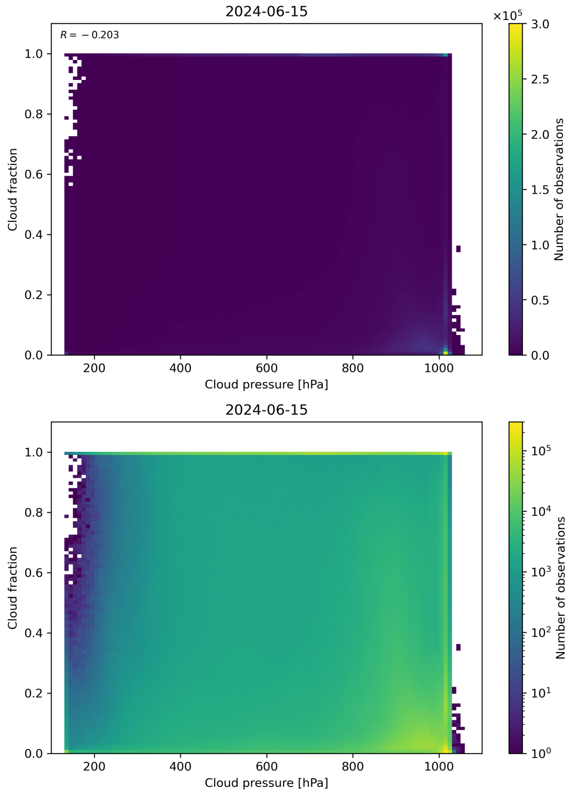
Figure 79: Scatter density plot of “Cloud pressure” against “Cloud fraction” for 2024-06-14 to 2024-06-16.
