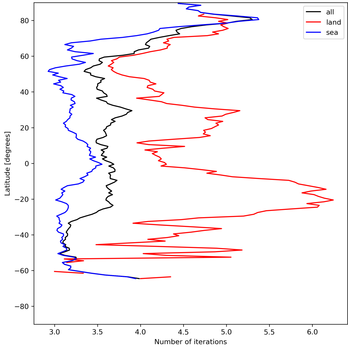
Figure 22: Zonal average of “Number of iterations” for 2024-06-14 to 2024-06-16.
