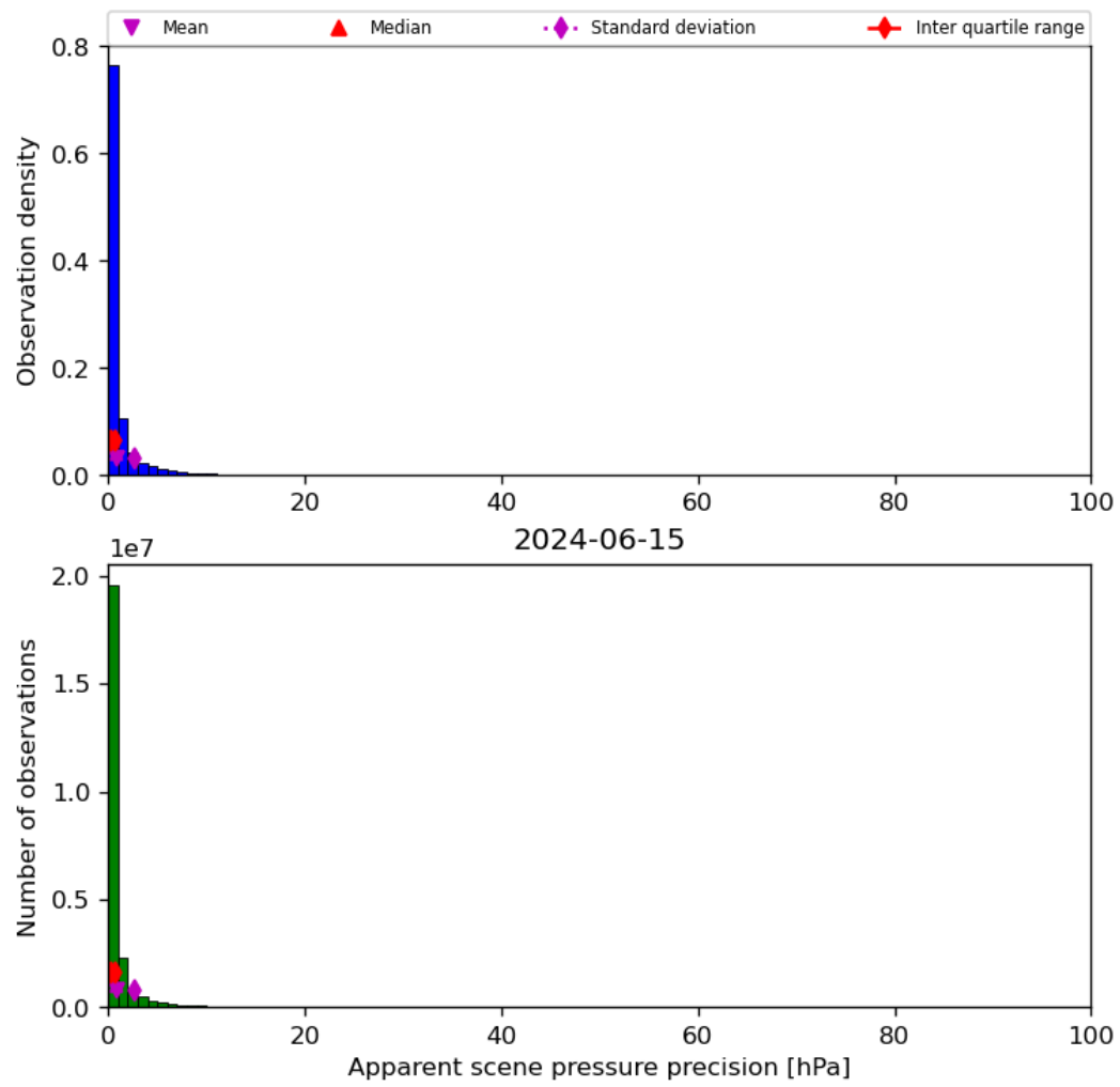
Figure 37: Histogram of “Apparent scene pressure precision” for 2024-06-14 to 2024-06-16
