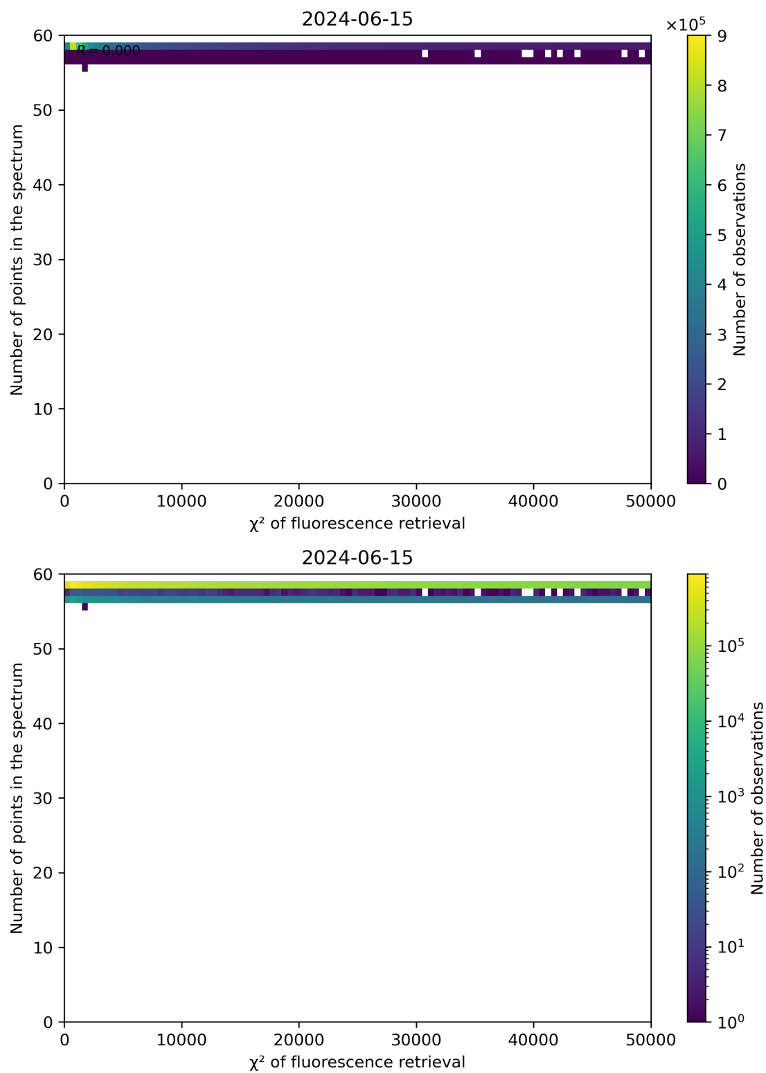
Figure 68: Scatter density plot of “ \chi^2 of fluorescence retrieval” against “Number of points in the spectrum” for 2024-06-14 to 2024-06-16.
