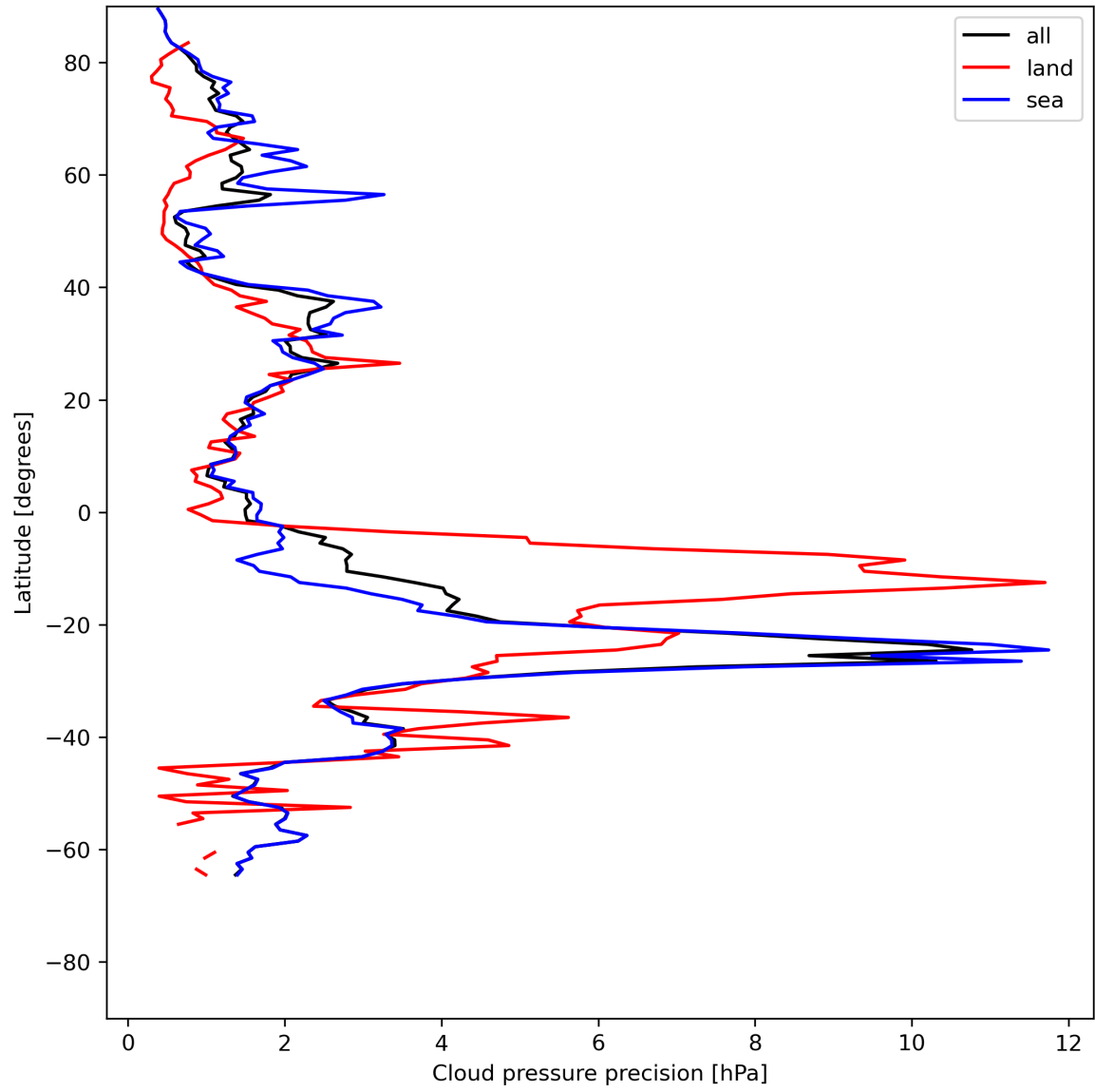
Figure 14: Zonal average of “Cloud pressure precision” for 2024-06-14 to 2024-06-16.
