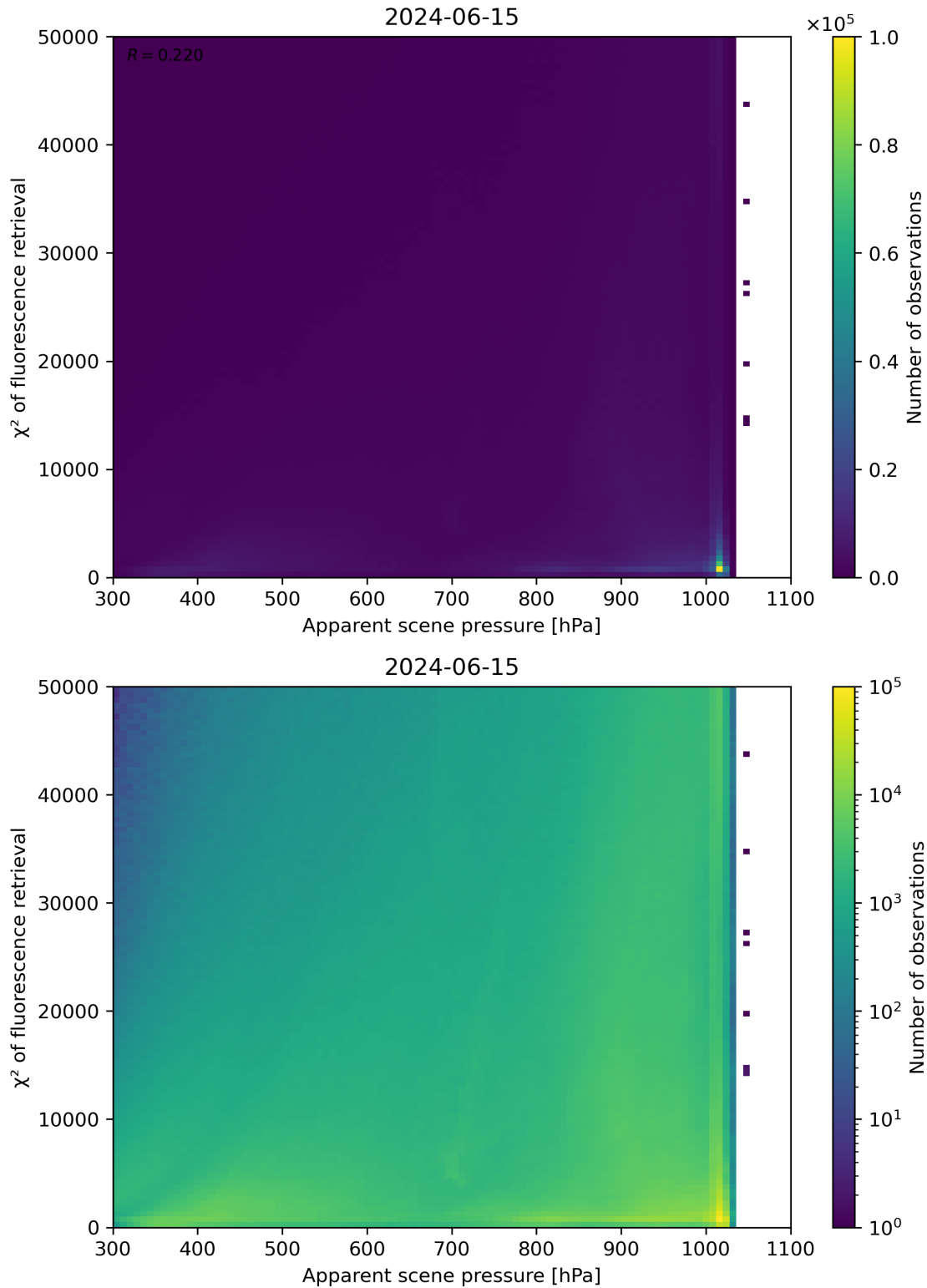
Figure 63: Scatter density plot of “Apparent scene pressure” against “ \chi^2 of fluorescence retrieval” for 2024-06-14 to 2024-06-16.
