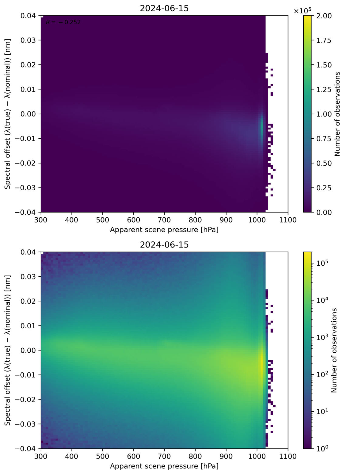
Figure 67: Scatter density plot of “Apparent scene pressure” against “Spectral offset ( \lambda(\text{true}) - \lambda(\text{nominal}) )” for 2024-06-14 to 2024-06-16.
