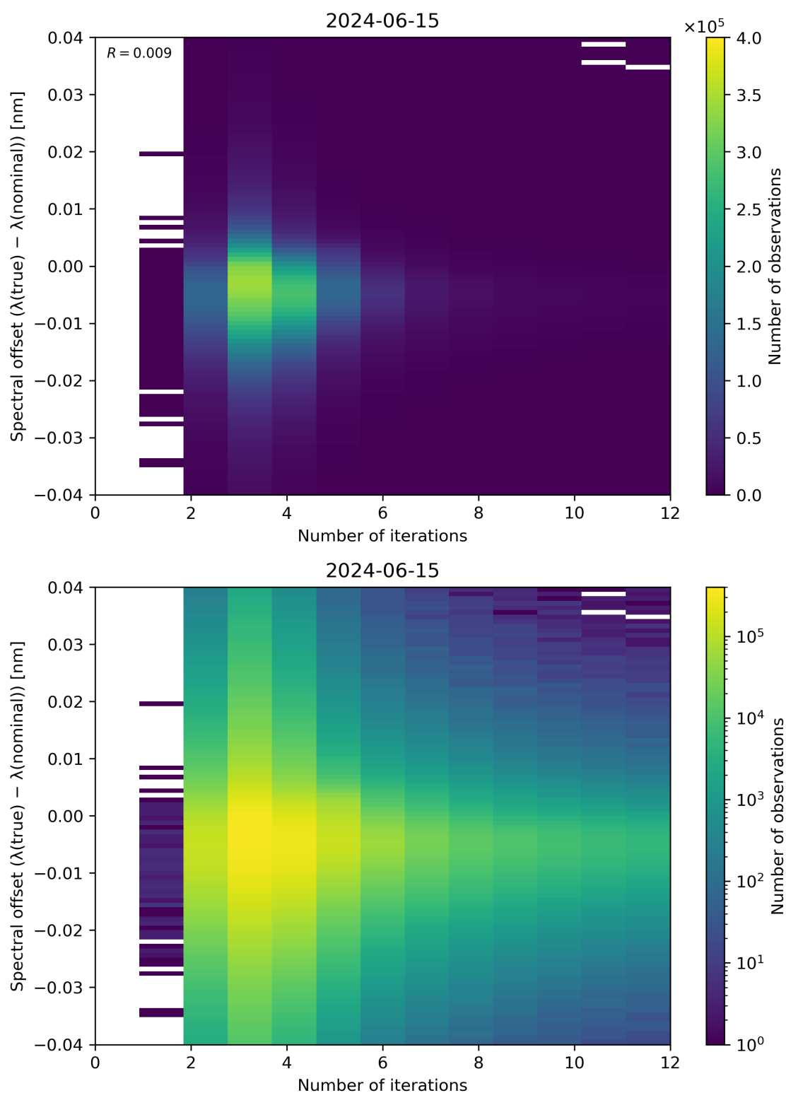
Figure 100: Scatter density plot of “Number of iterations” against “Spectral offset ( \lambda(\text{true}) - \lambda(\text{nominal}) )” for 2024-06-14 to 2024-06-16.
