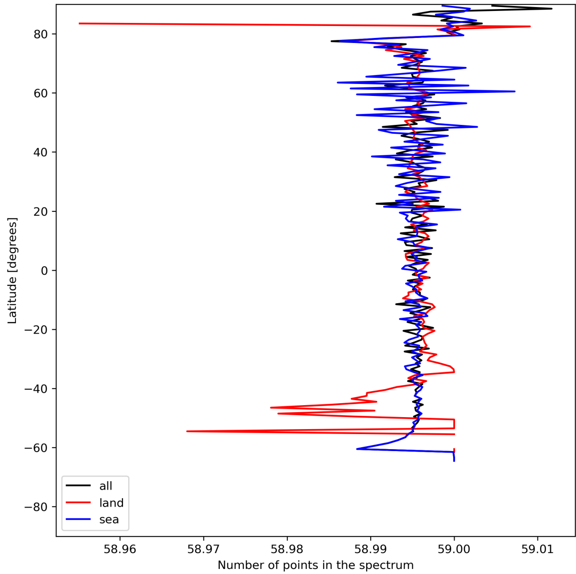
Figure 27: Zonal average of “Number of points in the spectrum” for 2024-06-14 to 2024-06-16.
