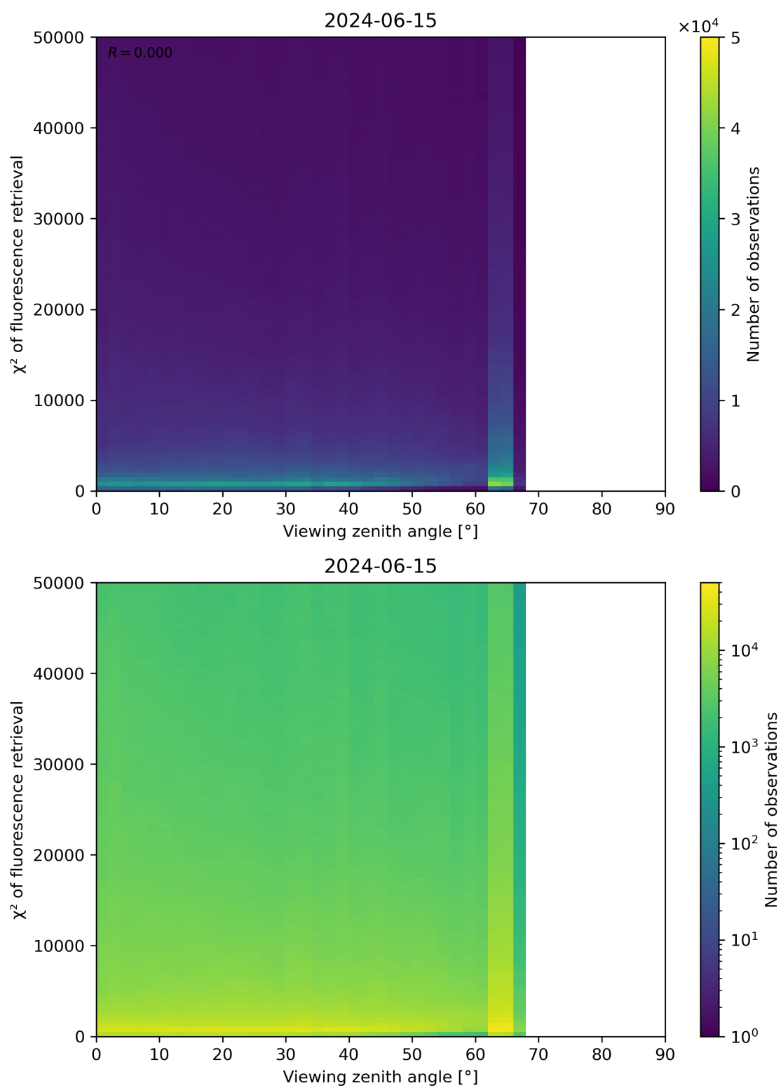
Figure 119: Scatter density plot of “Viewing zenith angle” against “ \chi^2 of fluorescence retrieval” for 2024-06-14 to 2024-06-16.
