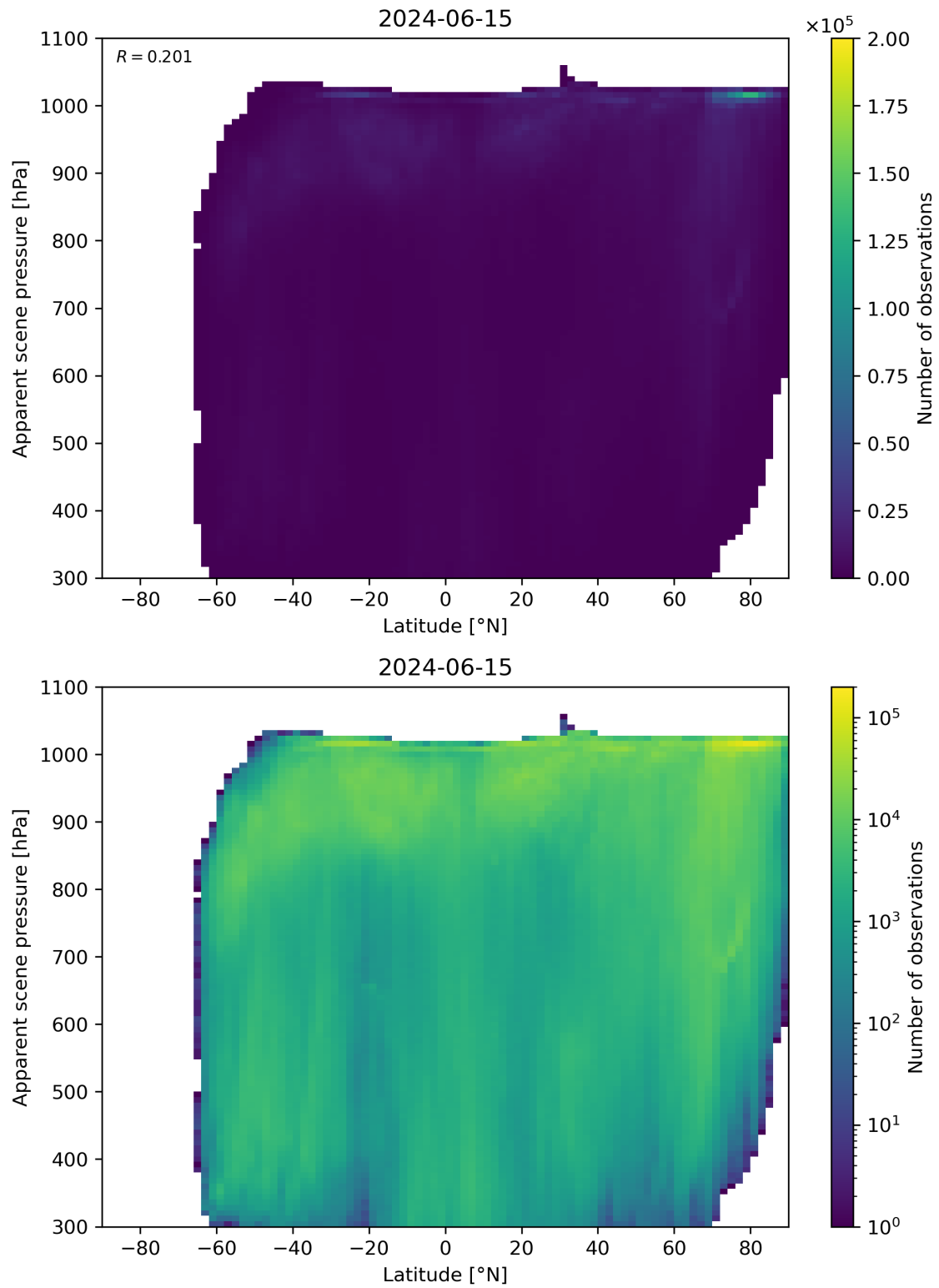
Figure 88: Scatter density plot of “Latitude” against “Apparent scene pressure” for 2024-06-14 to 2024-06-16.
