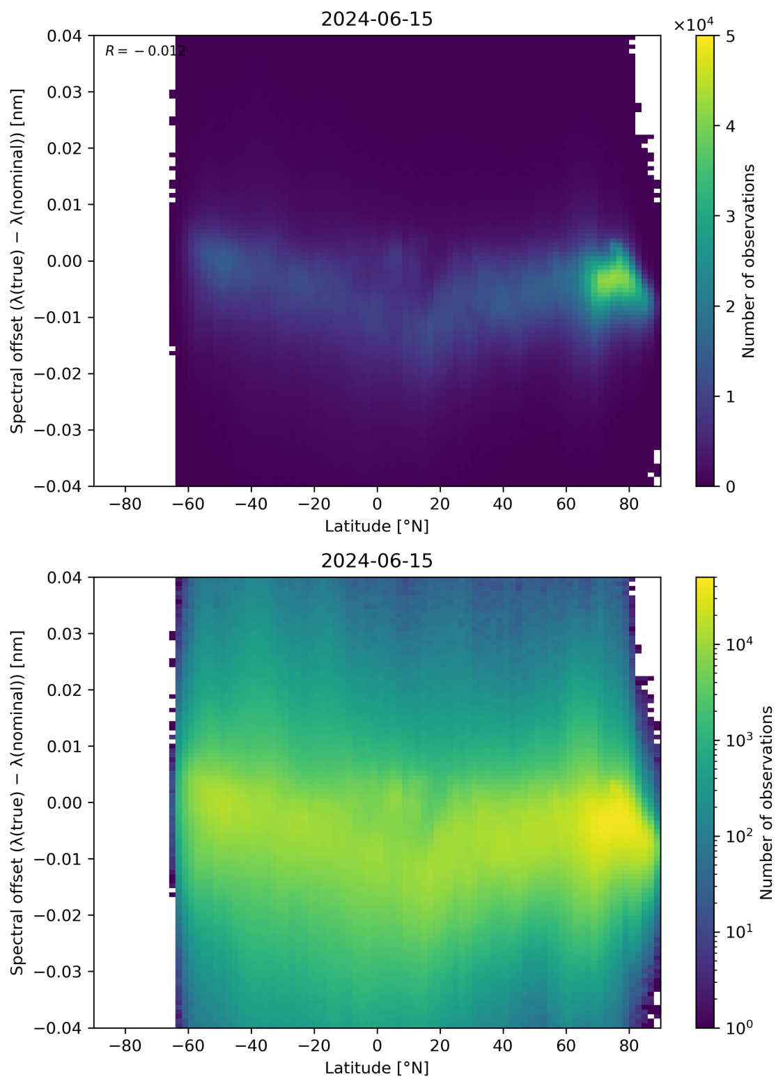
Figure 96: Scatter density plot of “Latitude” against “Spectral offset ( \lambda(\text{true}) - \lambda(\text{nominal}) )” for 2024-06-14 to 2024-06-16.
