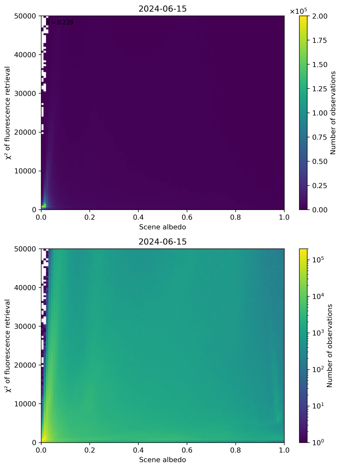
Figure 103: Scatter density plot of “Scene albedo” against “ \chi^2 of fluorescence retrieval” for 2024-06-14 to 2024-06-16.
