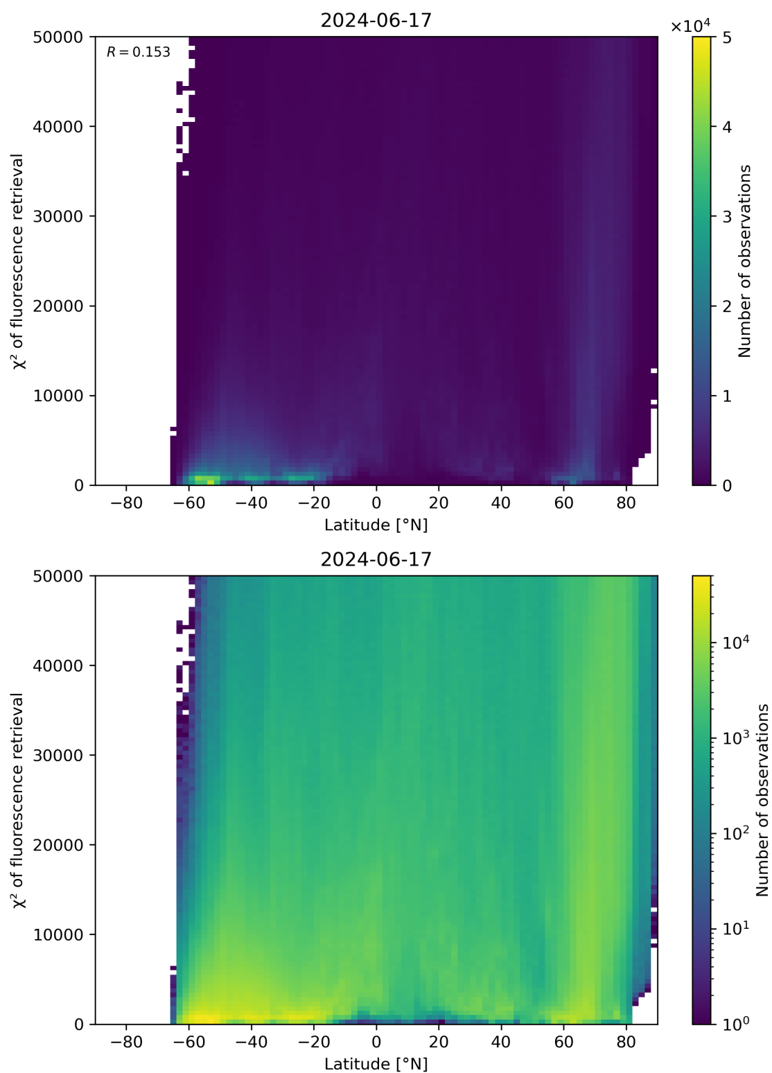
Figure 89: Scatter density plot of “Latitude” against “ \chi^2 of fluorescence retrieval” for 2024-06-16 to 2024-06-18.
