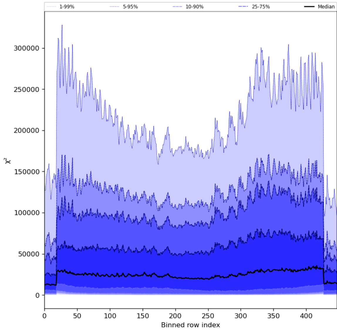
Figure 55: Along track statistics of “ \chi^2 ” for 2024-06-16 to 2024-06-18
