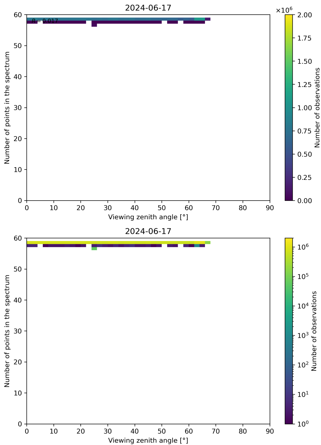
Figure 125: Scatter density plot of “Viewing zenith angle” against “Number of points in the spectrum” for 2024-06-16 to 2024-06-18.
