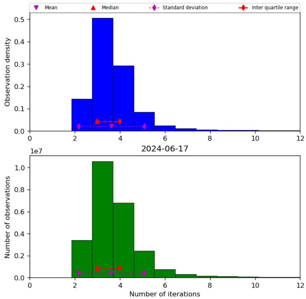
Figure 39: Histogram of “Number of iterations” for 2024-06-16 to 2024-06-18
