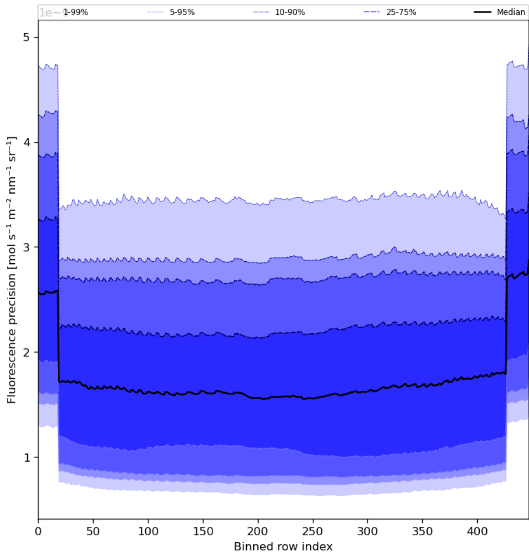
Figure 58: Along track statistics of “Fluorescence precision” for 2024-06-16 to 2024-06-18
