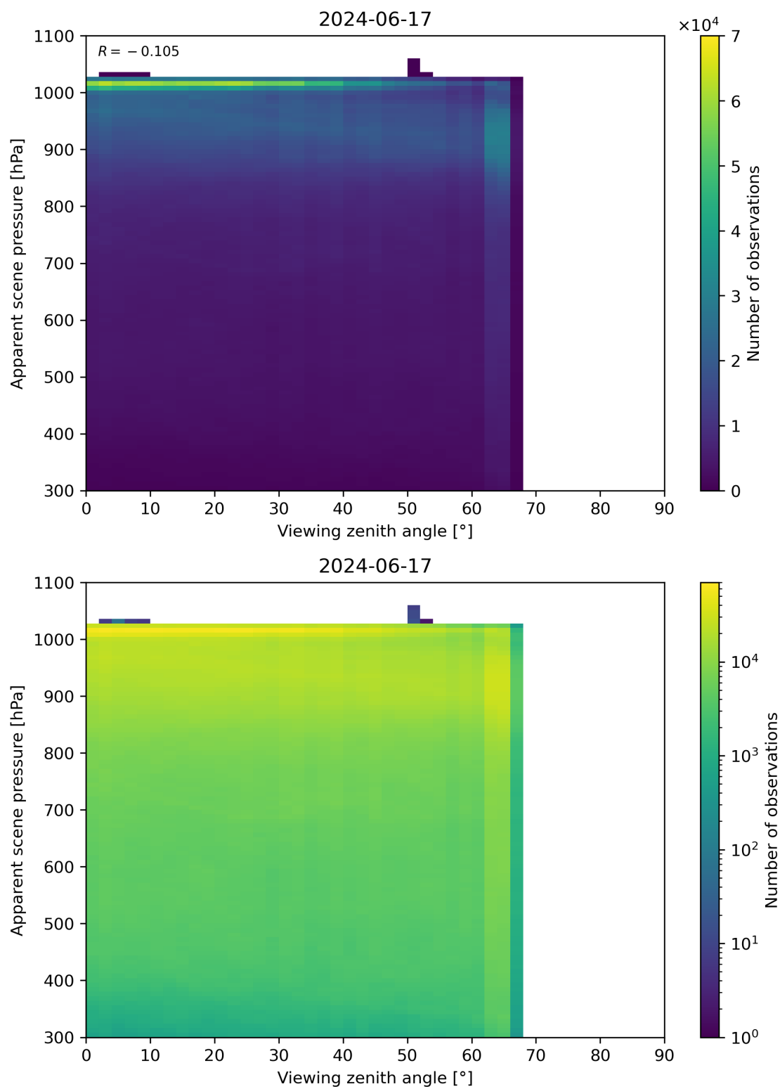
Figure 118: Scatter density plot of “Viewing zenith angle” against “Apparent scene pressure” for 2024-06-16 to 2024-06-18.
