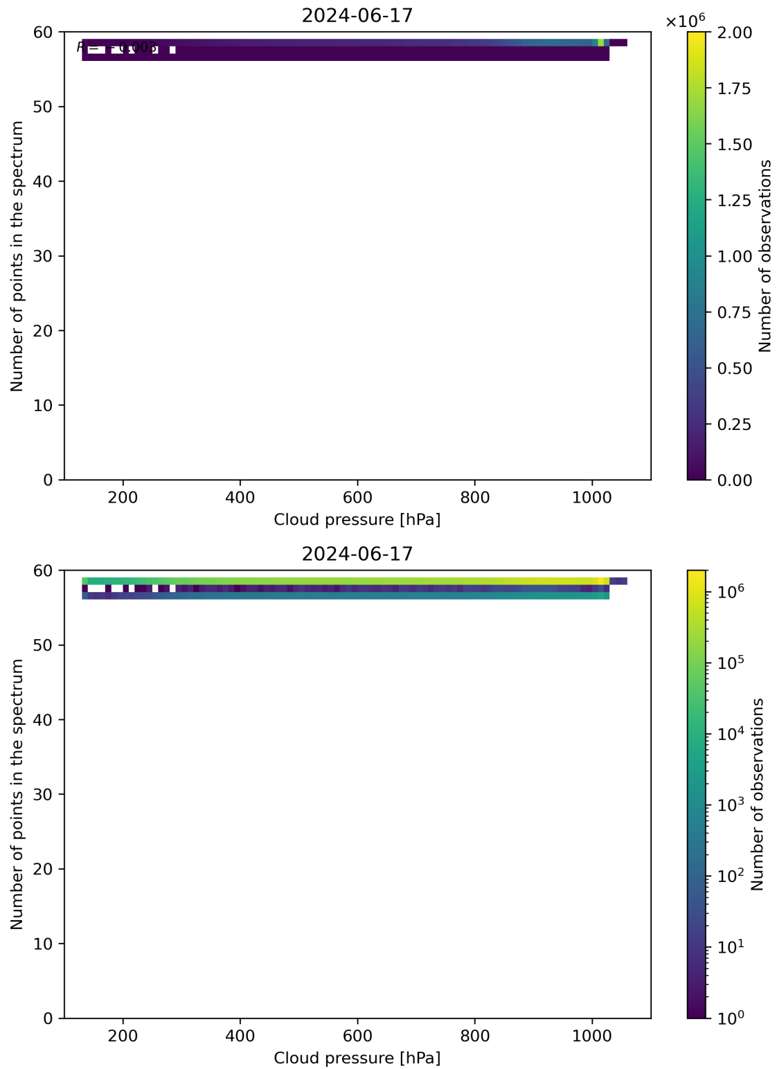
Figure 82: Scatter density plot of “Cloud pressure” against “Number of points in the spectrum” for 2024-06-16 to 2024-06-18.
