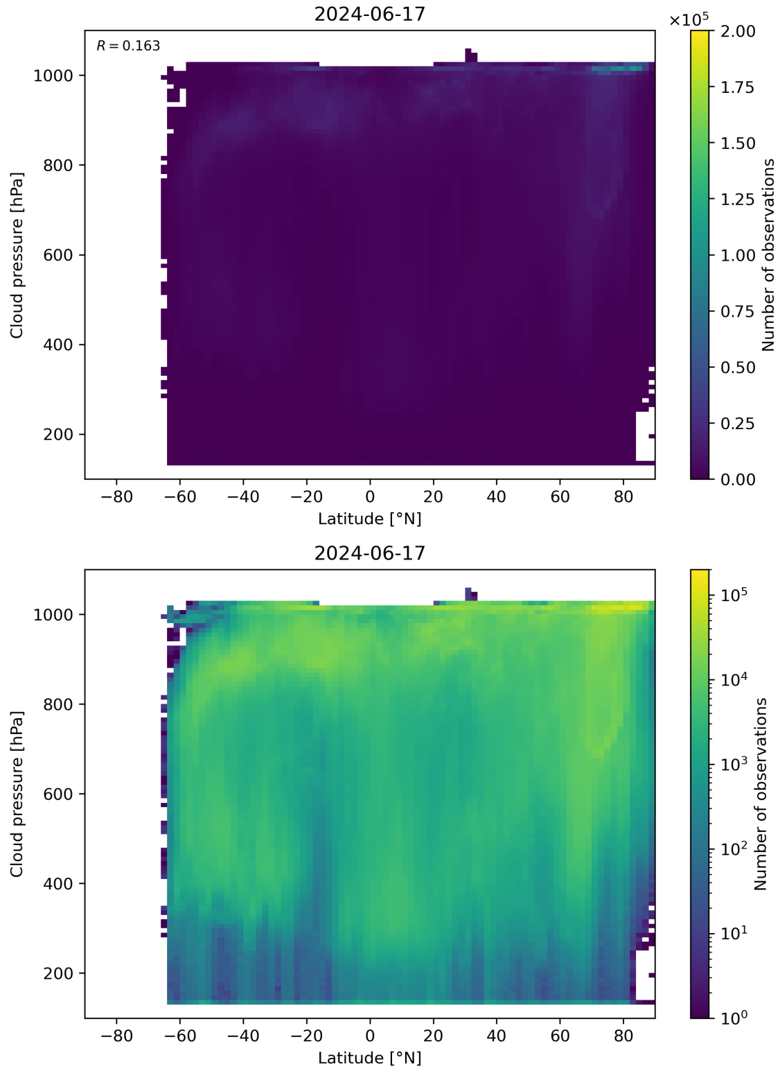
Figure 91: Scatter density plot of “Latitude” against “Cloud pressure” for 2024-06-16 to 2024-06-18.
