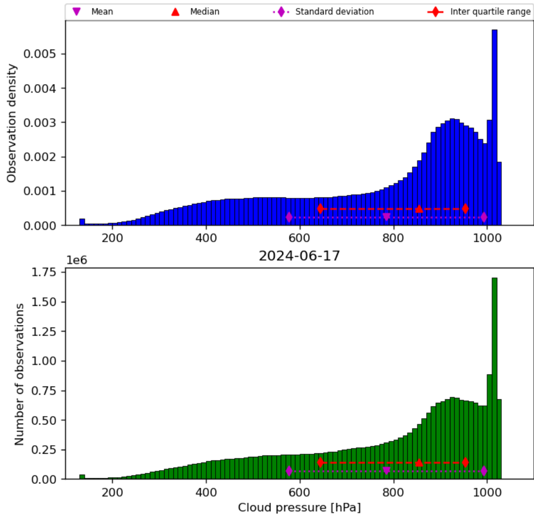
Figure 30: Histogram of “Cloud pressure” for 2024-06-16 to 2024-06-18
