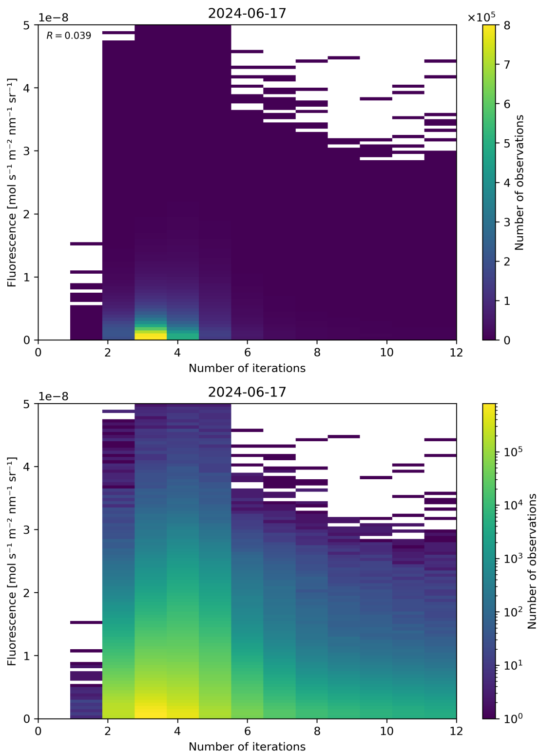
Figure 98: Scatter density plot of “Number of iterations” against “Fluorescence” for 2024-06-16 to 2024-06-18.
