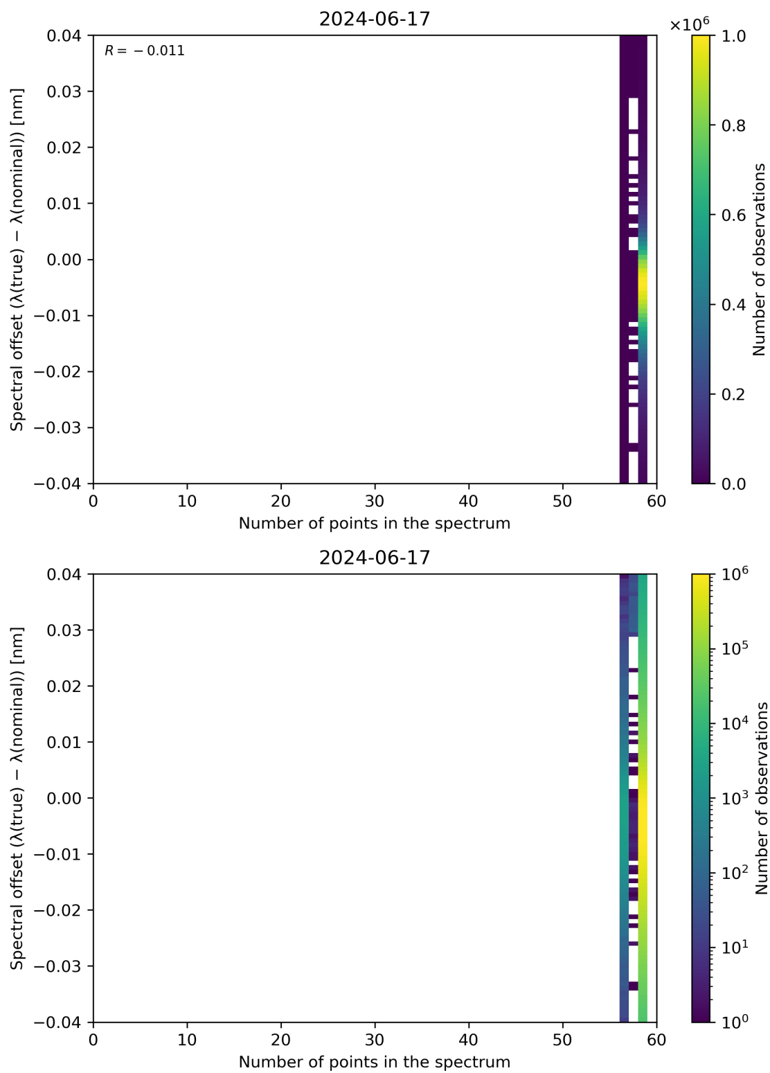
Figure 101: Scatter density plot of “Number of points in the spectrum” against “Spectral offset ( \lambda(\text{true}) - \lambda(\text{nominal}) )” for 2024-06-16 to 2024-06-18.
