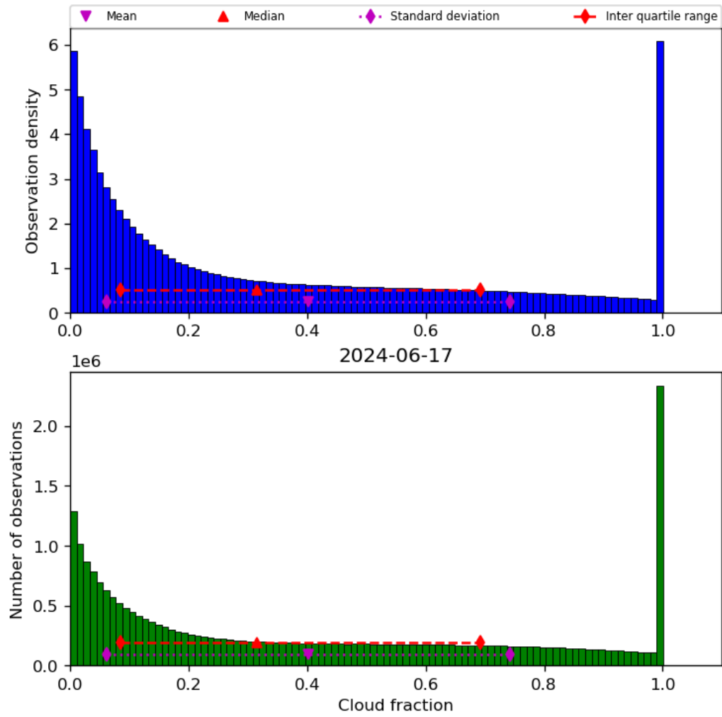
Figure 32: Histogram of “Cloud fraction” for 2024-06-16 to 2024-06-18
