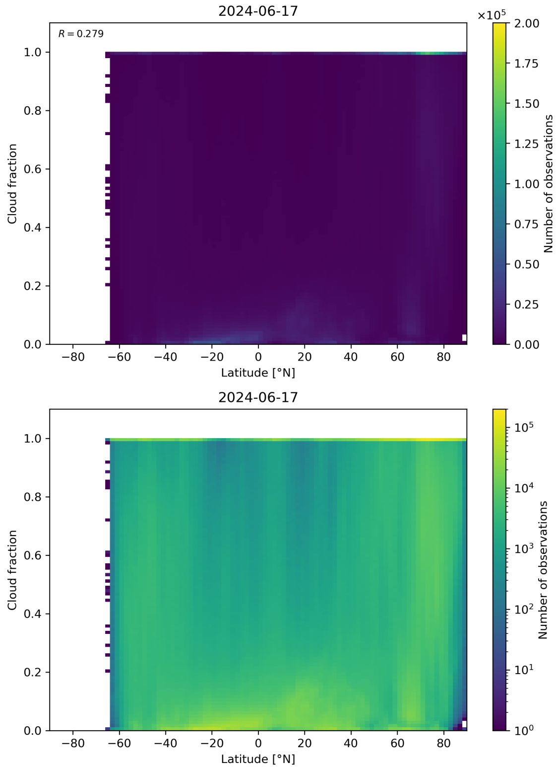
Figure 90: Scatter density plot of “Latitude” against “Cloud fraction” for 2024-06-16 to 2024-06-18.
