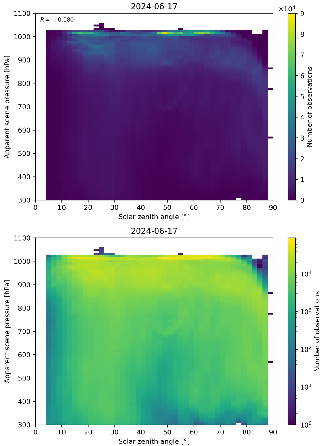
Figure 108: Scatter density plot of “Solar zenith angle” against “Apparent scene pressure” for 2024-06-16 to 2024-06-18.
