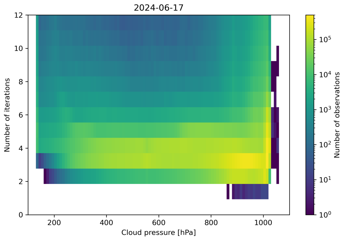
Figure 81: Scatter density plot of “Cloud pressure” against “Number of iterations” for 2024-06-16 to 2024-06-18.
