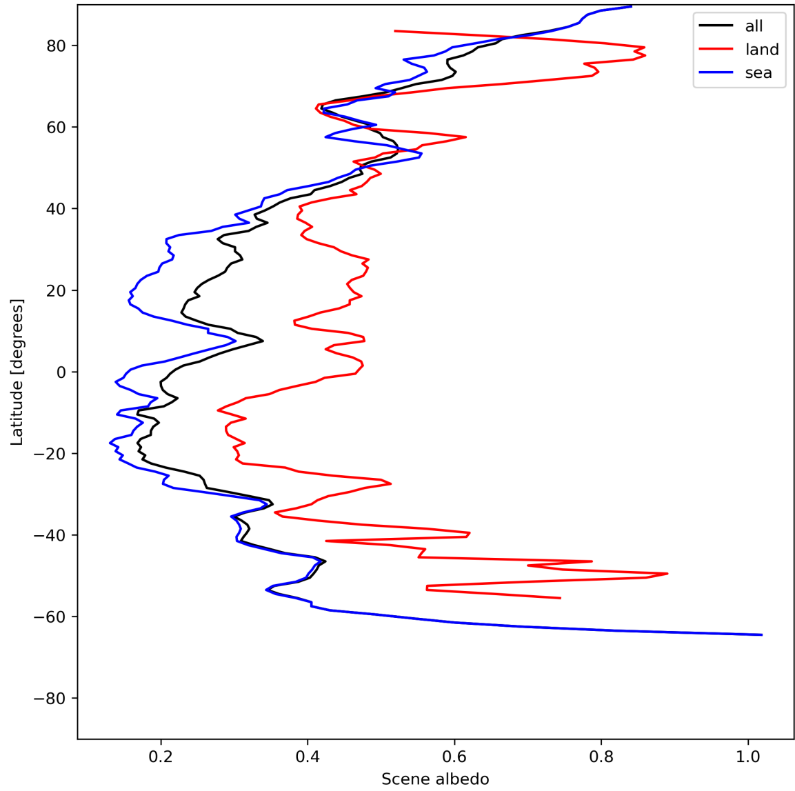
Figure 17: Zonal average of “Scene albedo” for 2024-06-16 to 2024-06-18.
