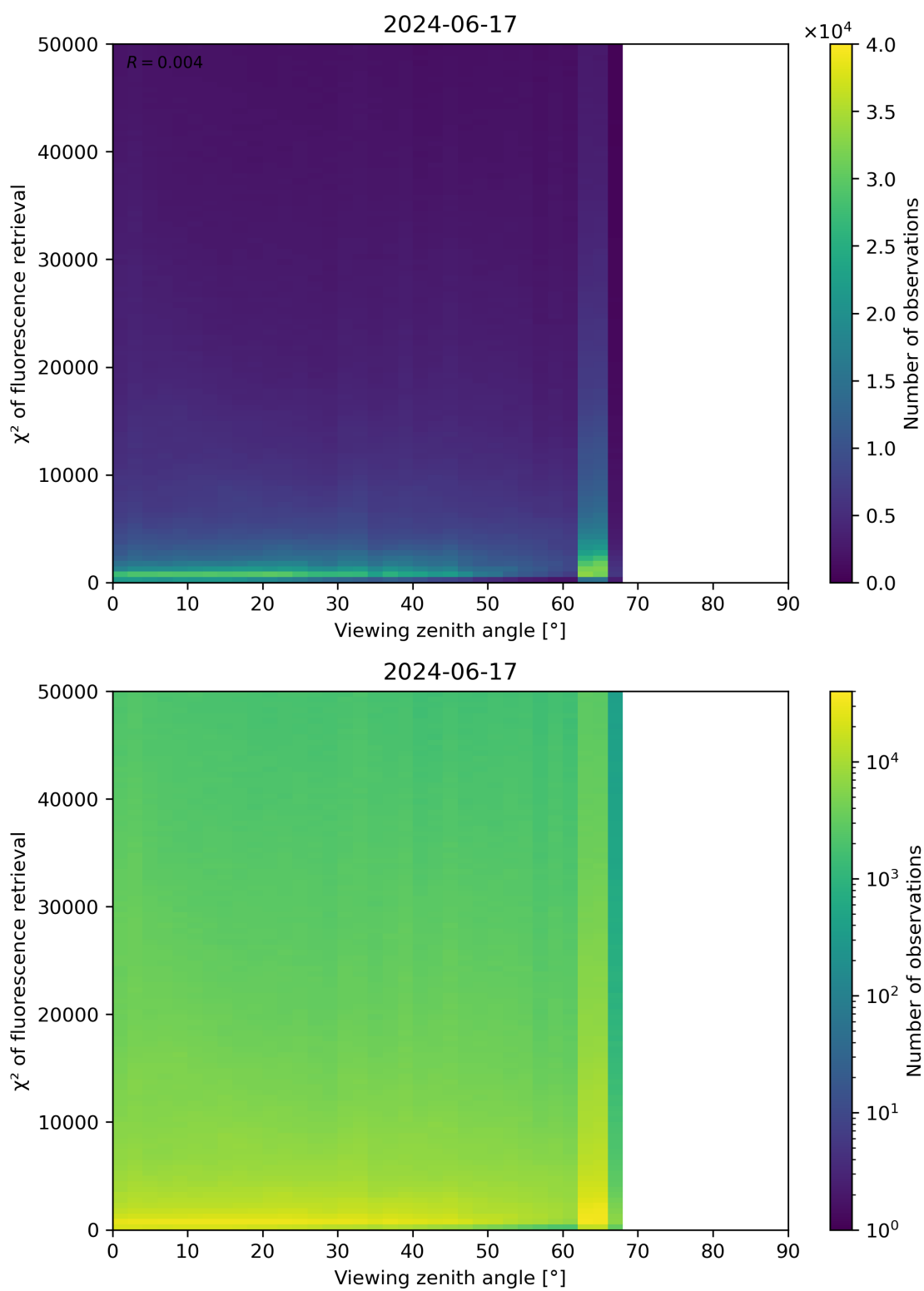
Figure 119: Scatter density plot of “Viewing zenith angle” against “ \chi^2 of fluorescence retrieval” for 2024-06-16 to 2024-06-18.
