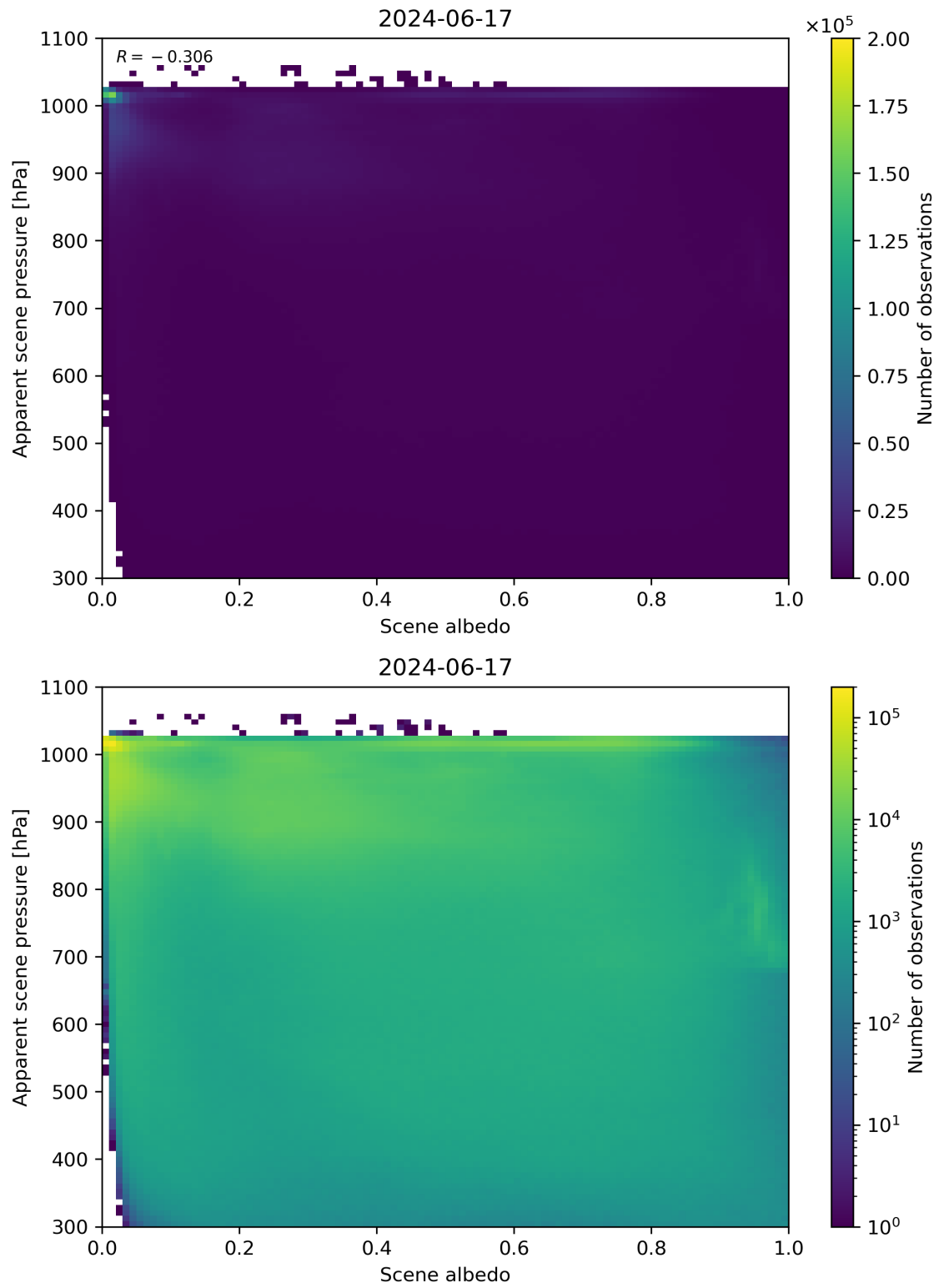
Figure 102: Scatter density plot of “Scene albedo” against “Apparent scene pressure” for 2024-06-16 to 2024-06-18.
