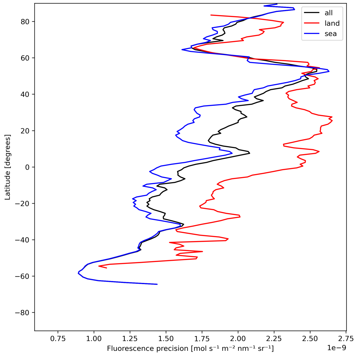
Figure 24: Zonal average of “Fluorescence precision” for 2024-06-16 to 2024-06-18.
