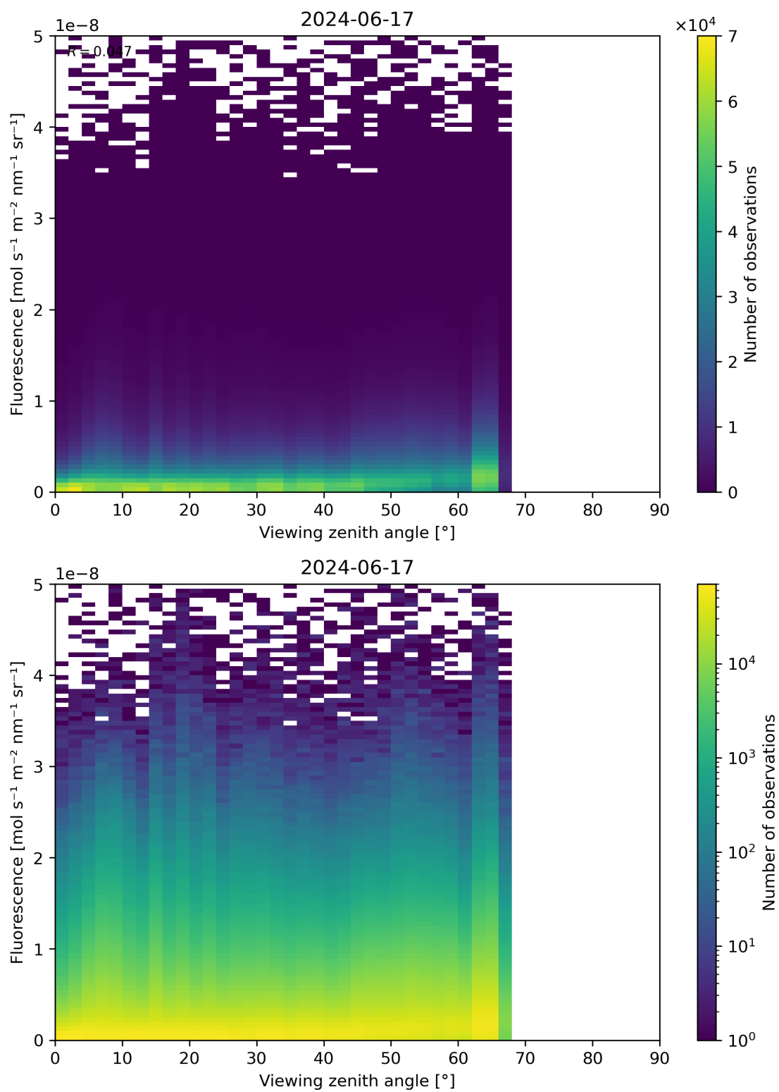
Figure 122: Scatter density plot of “Viewing zenith angle” against “Fluorescence” for 2024-06-16 to 2024-06-18.
