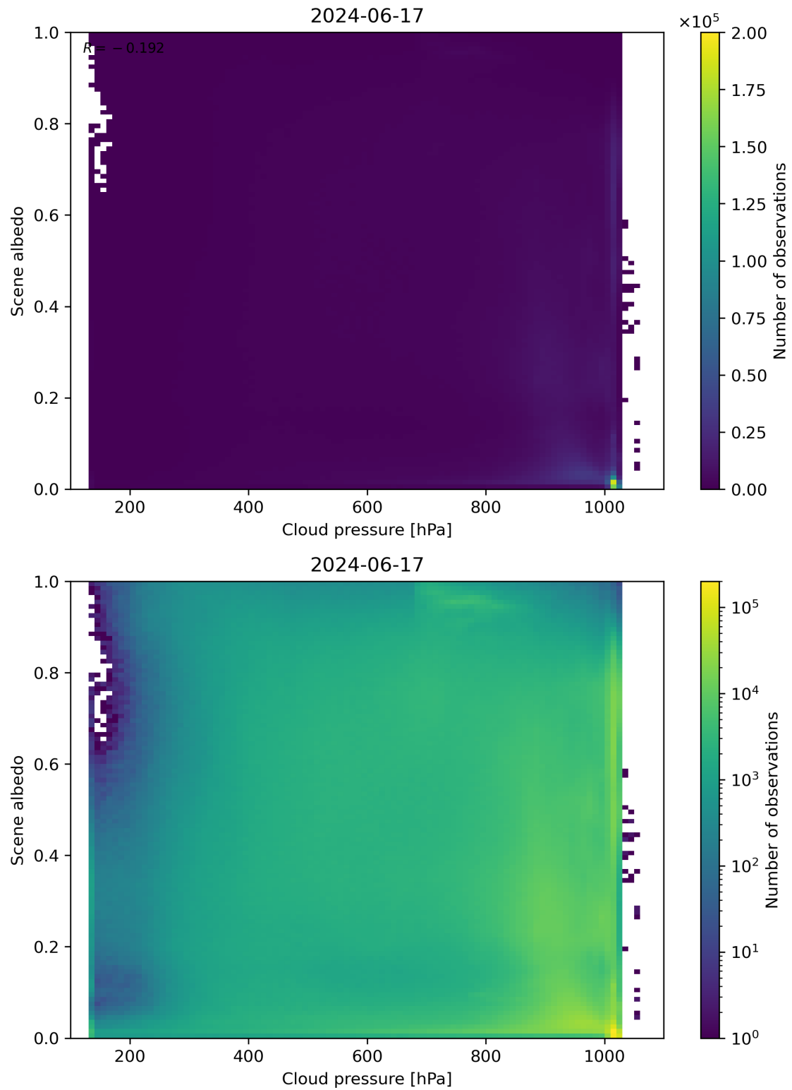
Figure 83: Scatter density plot of “Cloud pressure” against “Scene albedo” for 2024-06-16 to 2024-06-18.
