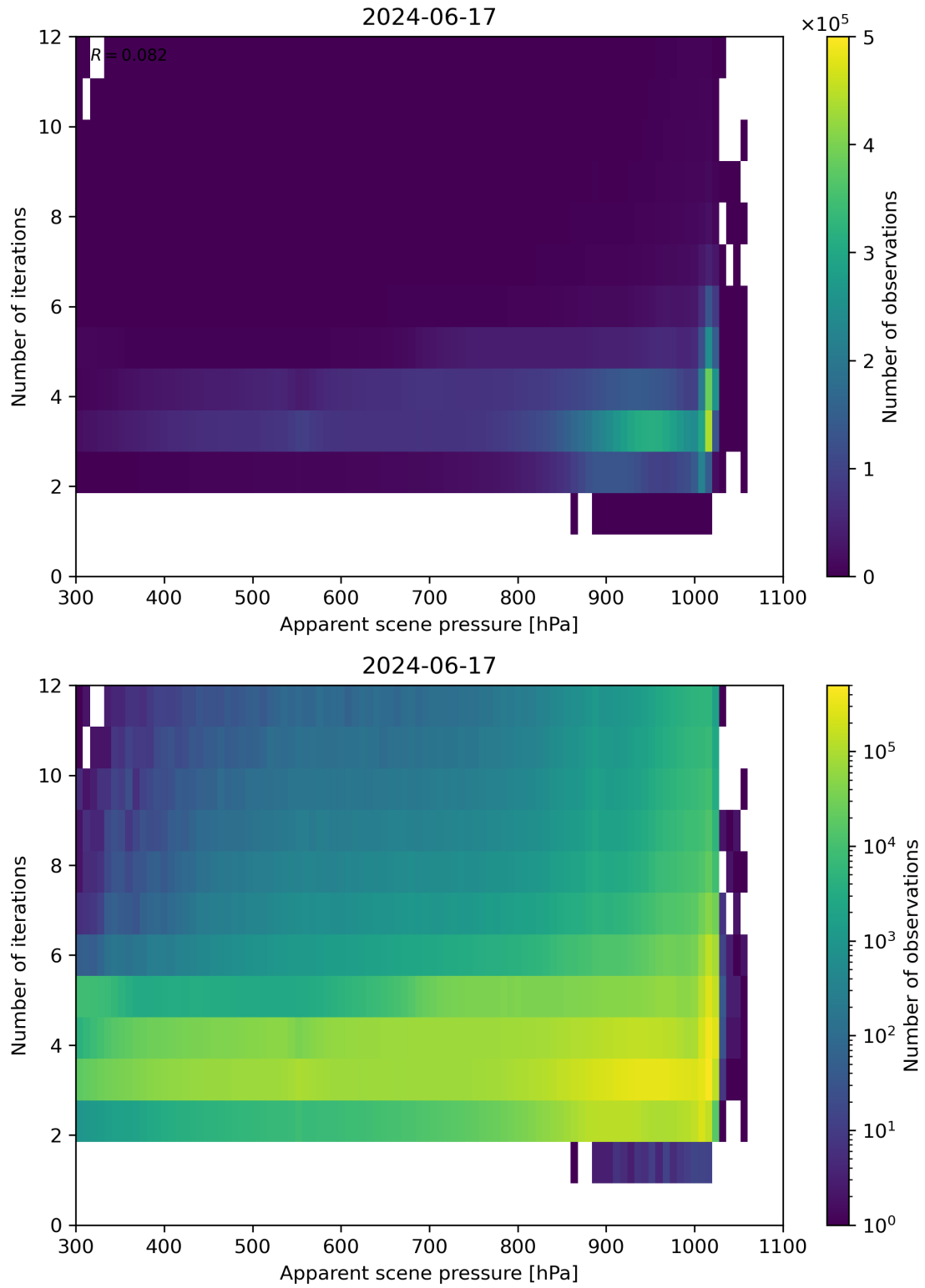
Figure 65: Scatter density plot of “Apparent scene pressure” against “Number of iterations” for 2024-06-16 to 2024-06-18.
