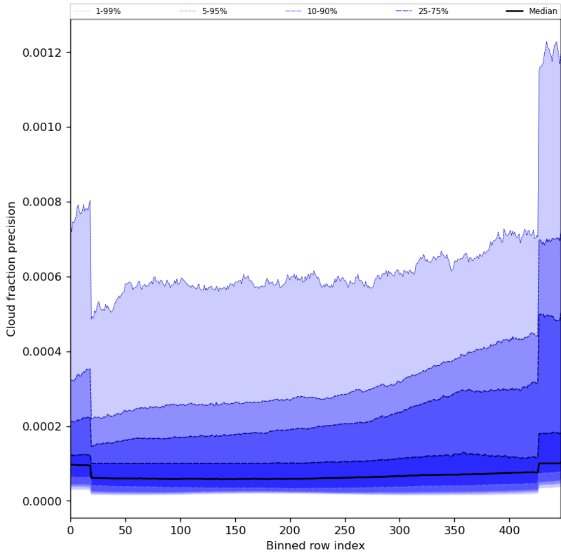
Figure 50: Along track statistics of “Cloud fraction precision” for 2024-06-16 to 2024-06-18
