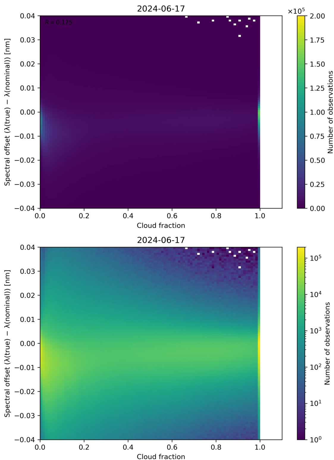
Figure 76: Scatter density plot of “Cloud fraction” against “Spectral offset ( \lambda(\text{true}) - \lambda(\text{nominal}) )” for 2024-06-16 to 2024-06-18.
