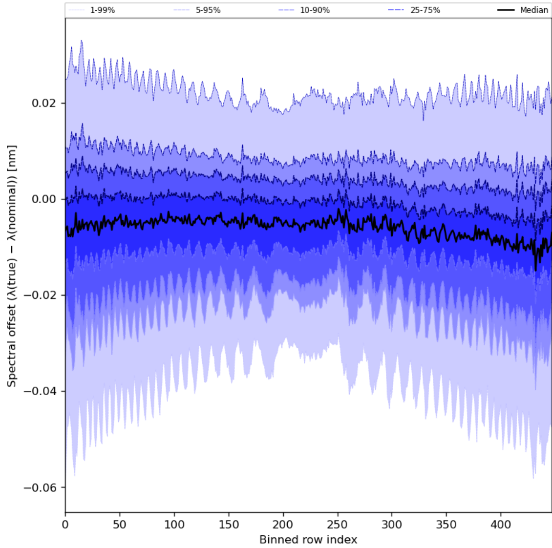
Figure 62: Along track statistics of “Spectral offset ( \lambda(\text{true}) - \lambda(\text{nominal}) )” for 2024-06-16 to 2024-06-18
