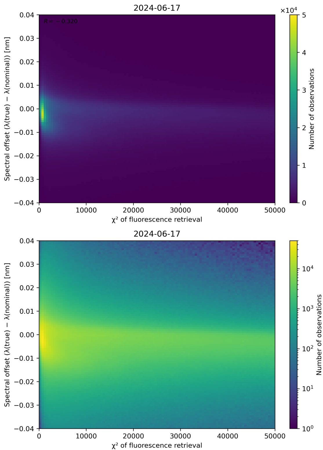
Figure 69: Scatter density plot of “ \chi^2 of fluorescence retrieval” against “Spectral offset ( \lambda(\text{true}) - \lambda(\text{nominal}) )” for 2024-06-16 to 2024-06-18.
