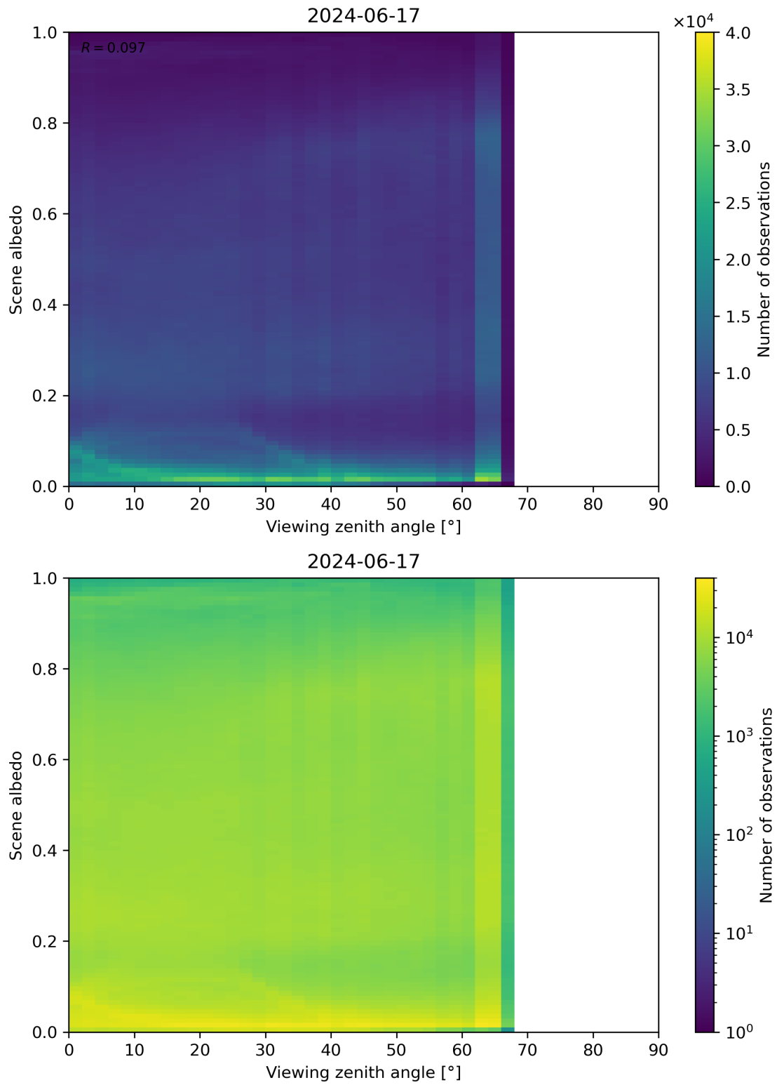
Figure 126: Scatter density plot of “Viewing zenith angle” against “Scene albedo” for 2024-06-16 to 2024-06-18.
