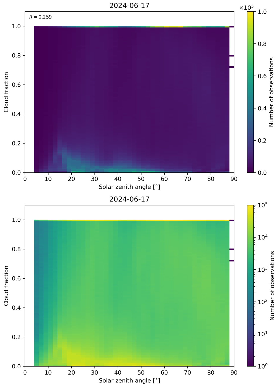
Figure 110: Scatter density plot of “Solar zenith angle” against “Cloud fraction” for 2024-06-16 to 2024-06-18.
