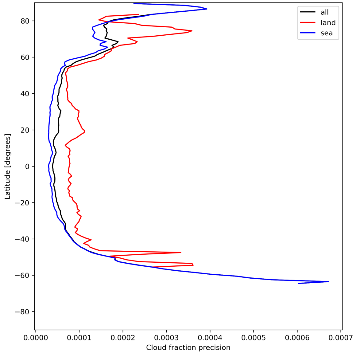
Figure 16: Zonal average of “Cloud fraction precision” for 2024-06-16 to 2024-06-18.
