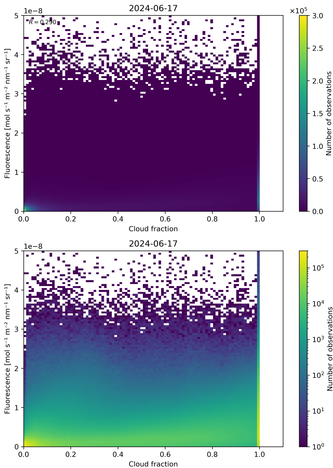
Figure 72: Scatter density plot of “Cloud fraction” against “Fluorescence” for 2024-06-16 to 2024-06-18.
