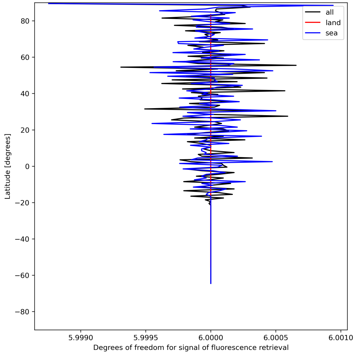
Figure 26: Zonal average of “Degrees of freedom for signal of fluorescence retrieval” for 2024-06-16 to 2024-06-18.
