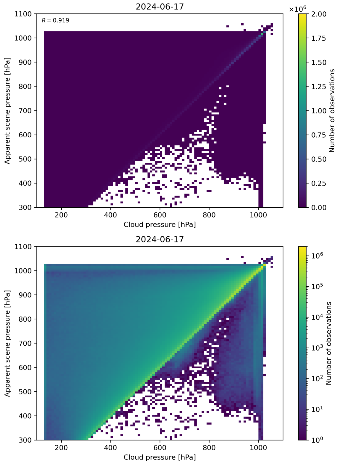
Figure 77: Scatter density plot of “Cloud pressure” against “Apparent scene pressure” for 2024-06-16 to 2024-06-18.
