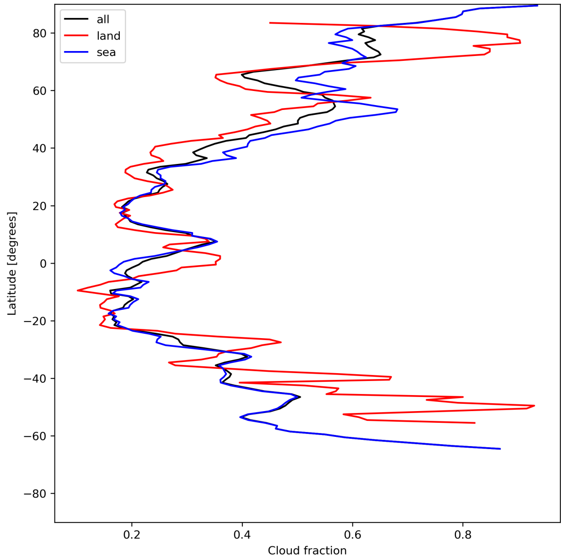
Figure 15: Zonal average of “Cloud fraction” for 2024-06-16 to 2024-06-18.
