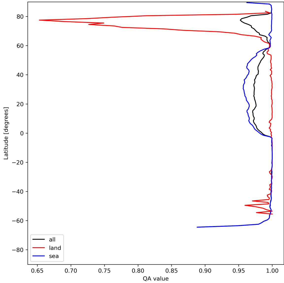
Figure 12: Zonal average of “QA value” for 2024-06-16 to 2024-06-18.
