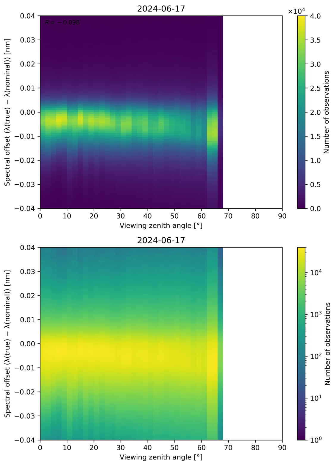
Figure 128: Scatter density plot of “Viewing zenith angle” against “Spectral offset ( \lambda(\text{true}) - \lambda(\text{nominal}) )” for 2024-06-16 to 2024-06-18.
