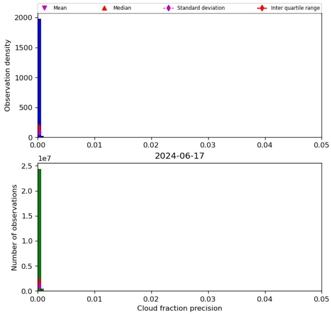
Figure 33: Histogram of “Cloud fraction precision” for 2024-06-16 to 2024-06-18
