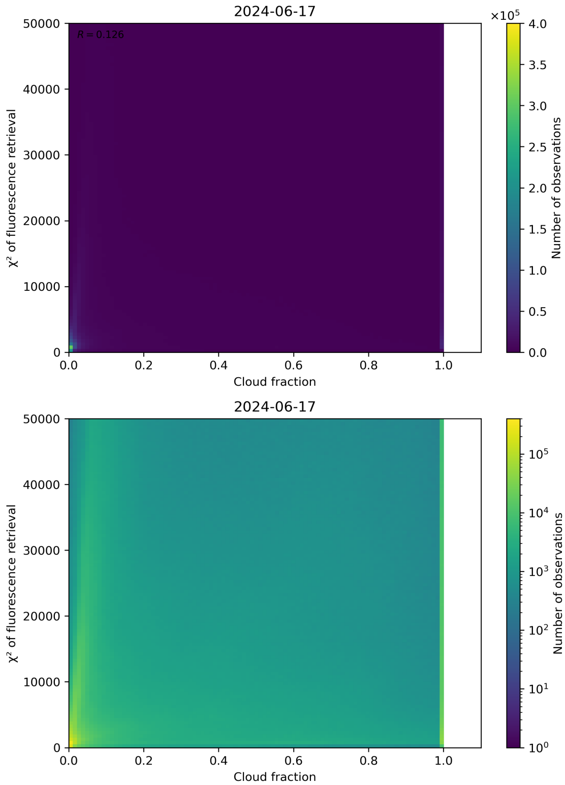
Figure 71: Scatter density plot of “Cloud fraction” against “ \chi^2 of fluorescence retrieval” for 2024-06-16 to 2024-06-18.
