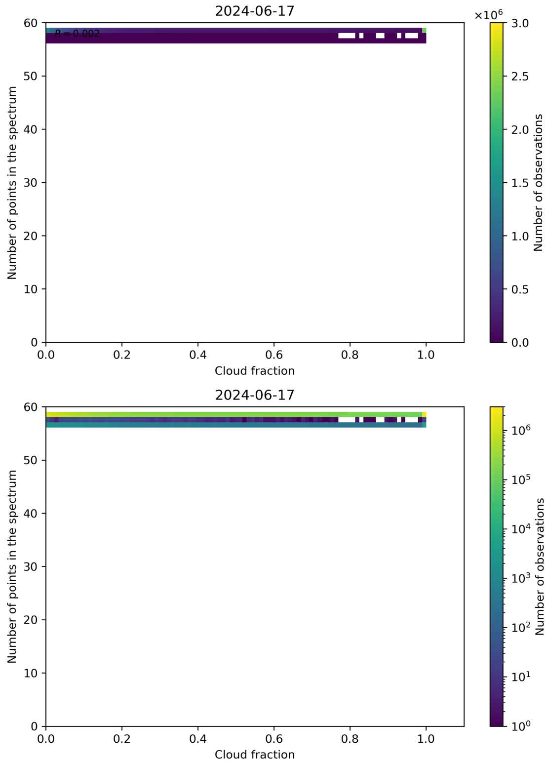
Figure 74: Scatter density plot of “Cloud fraction” against “Number of points in the spectrum” for 2024-06-16 to 2024-06-18.
