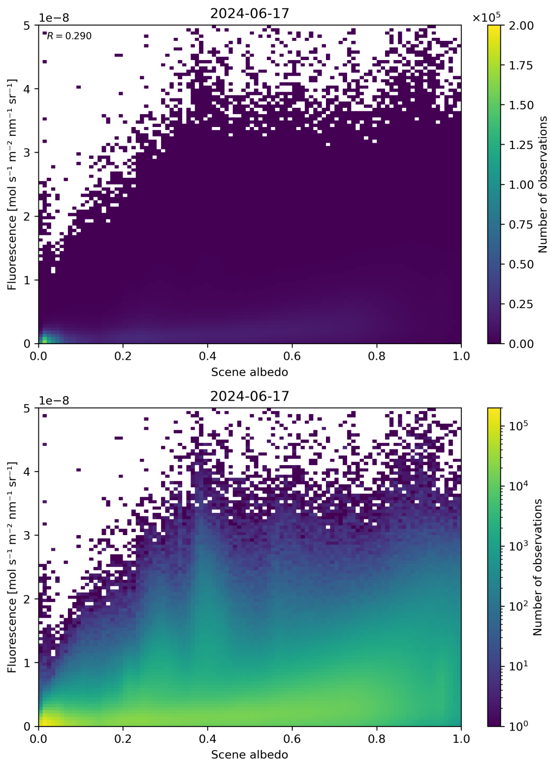
Figure 104: Scatter density plot of “Scene albedo” against “Fluorescence” for 2024-06-16 to 2024-06-18.
