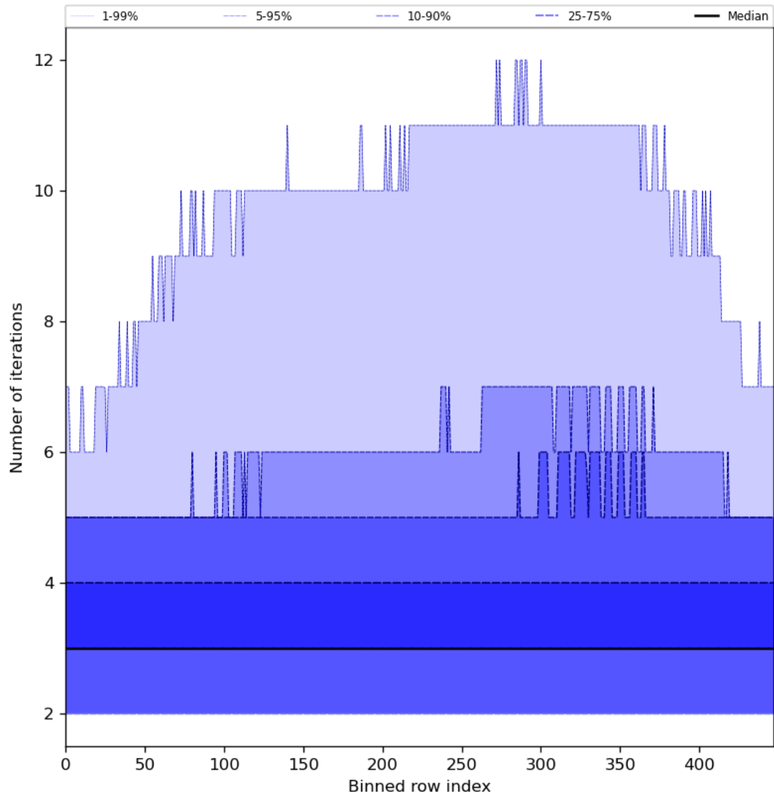
Figure 56: Along track statistics of “Number of iterations” for 2024-06-16 to 2024-06-18
