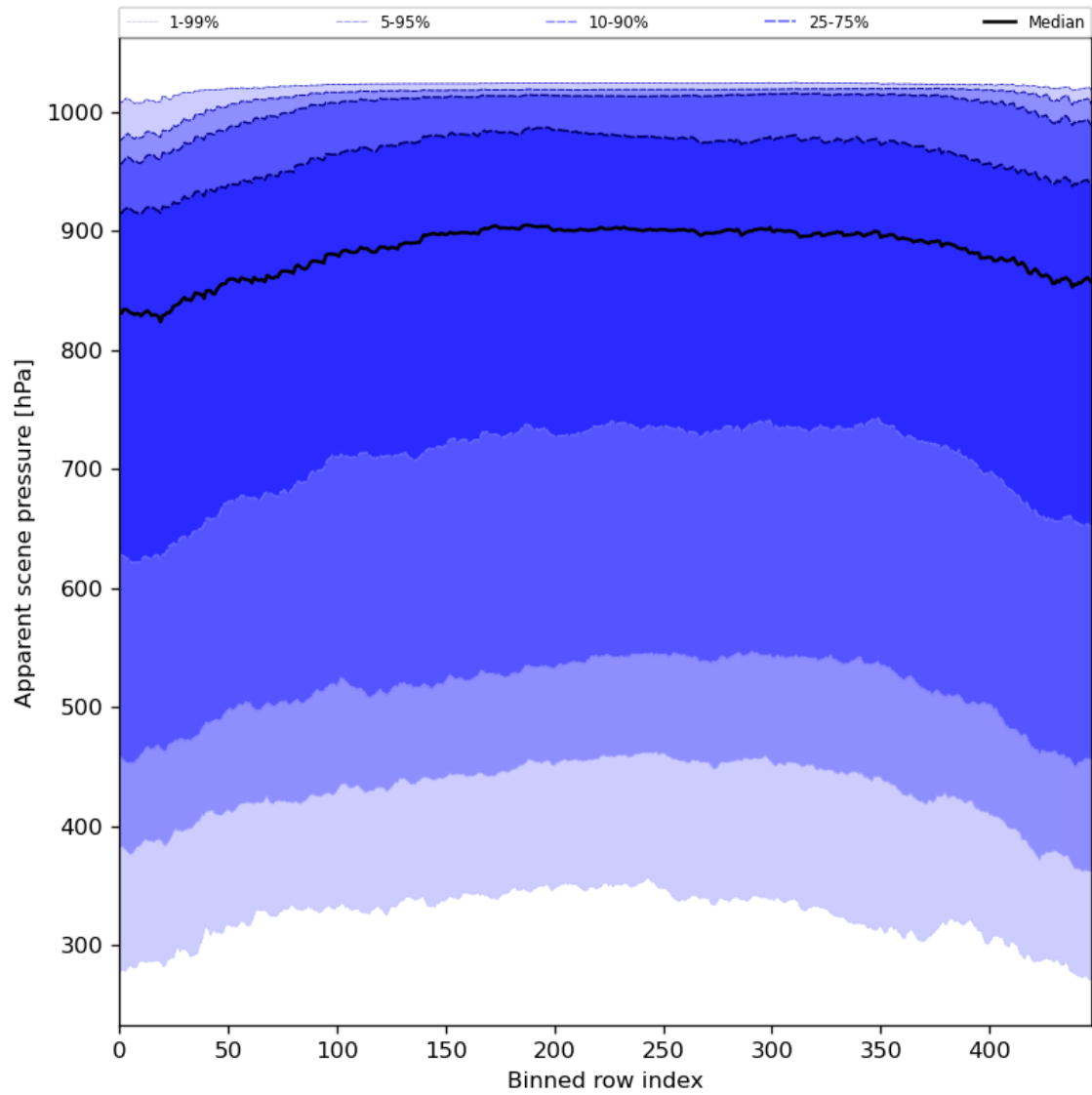
Figure 53: Along track statistics of “Apparent scene pressure” for 2024-06-16 to 2024-06-18
