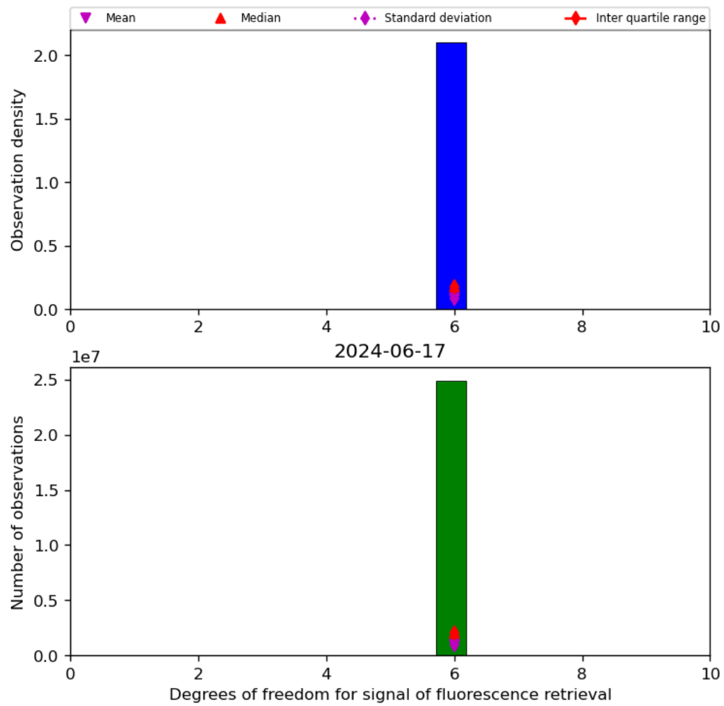
Figure 43: Histogram of “Degrees of freedom for signal of fluorescence retrieval” for 2024-06-16 to 2024-06-18
