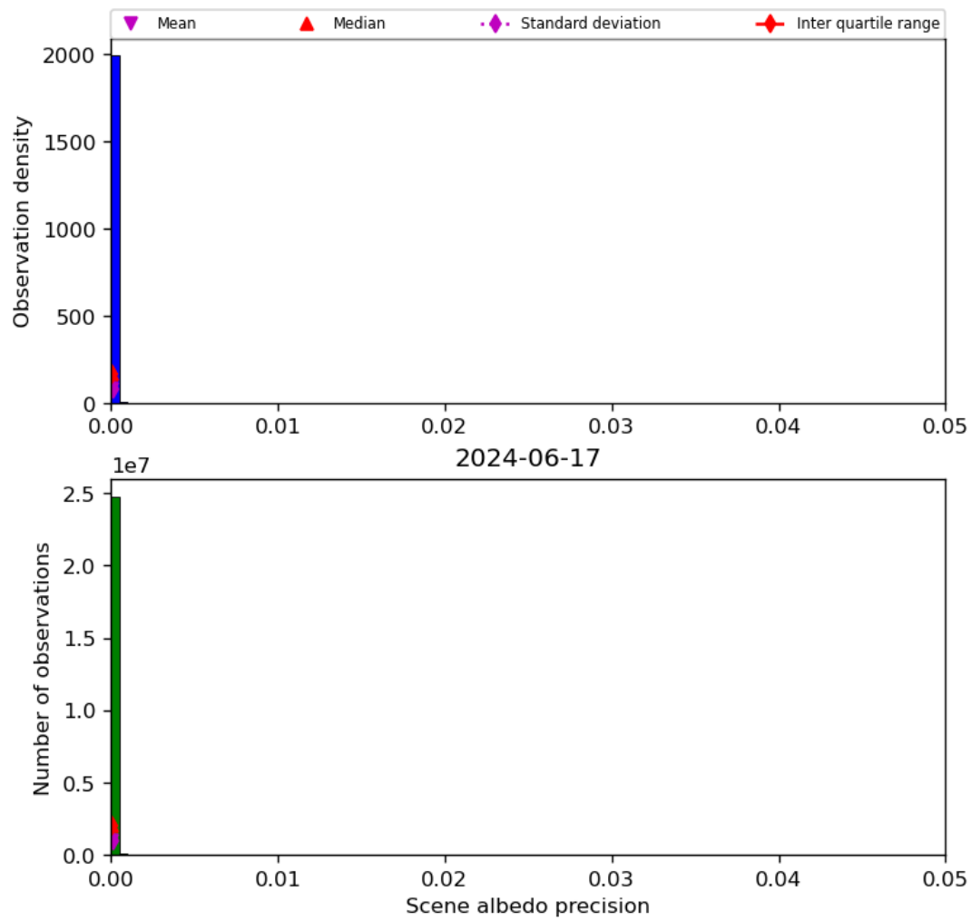
Figure 35: Histogram of “Scene albedo precision” for 2024-06-16 to 2024-06-18
