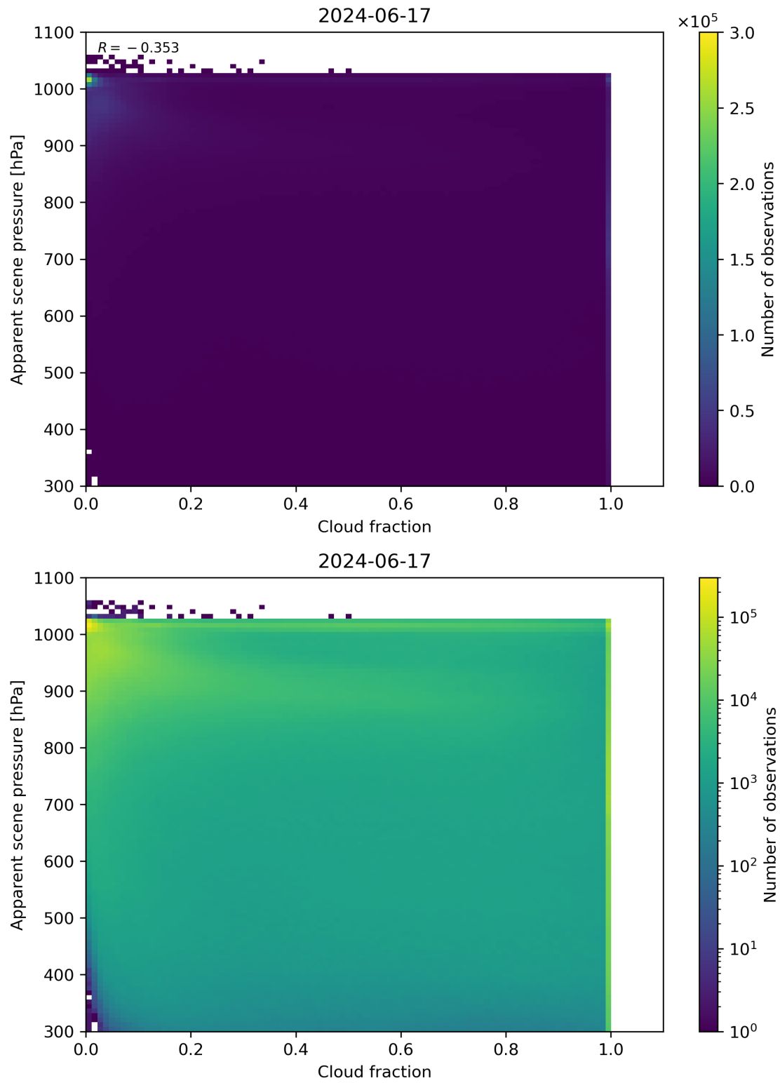
Figure 70: Scatter density plot of “Cloud fraction” against “Apparent scene pressure” for 2024-06-16 to 2024-06-18.
