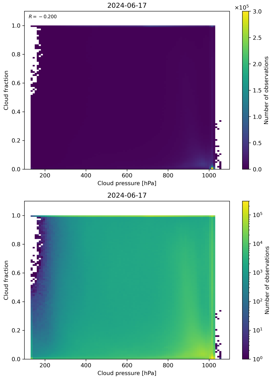
Figure 79: Scatter density plot of “Cloud pressure” against “Cloud fraction” for 2024-06-16 to 2024-06-18.
