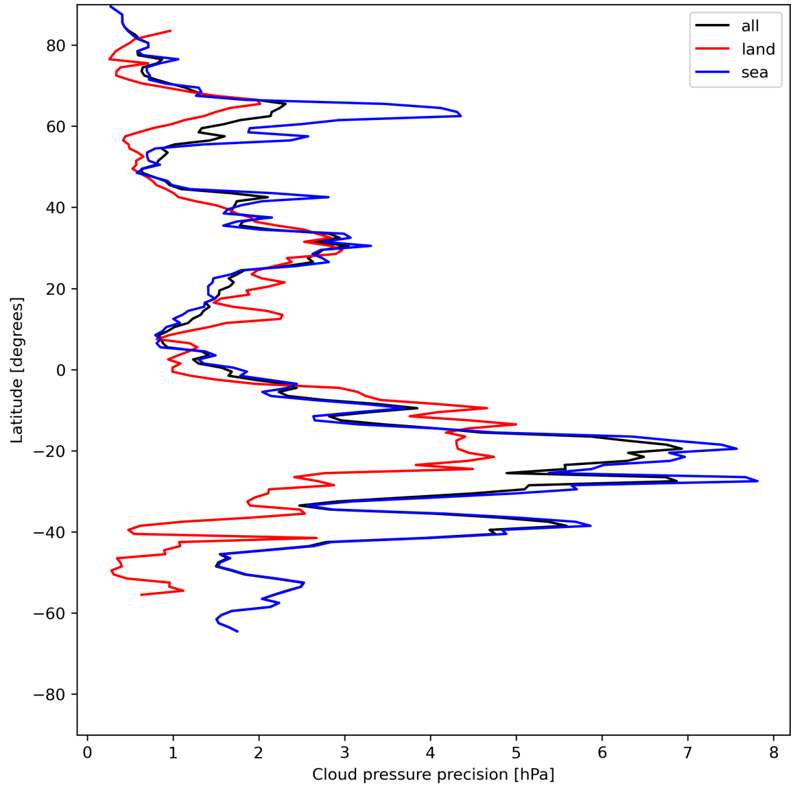
Figure 14: Zonal average of “Cloud pressure precision” for 2024-06-16 to 2024-06-18.
