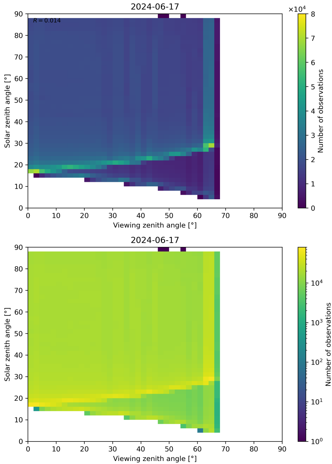
Figure 127: Scatter density plot of “Viewing zenith angle” against “Solar zenith angle” for 2024-06-16 to 2024-06-18.
