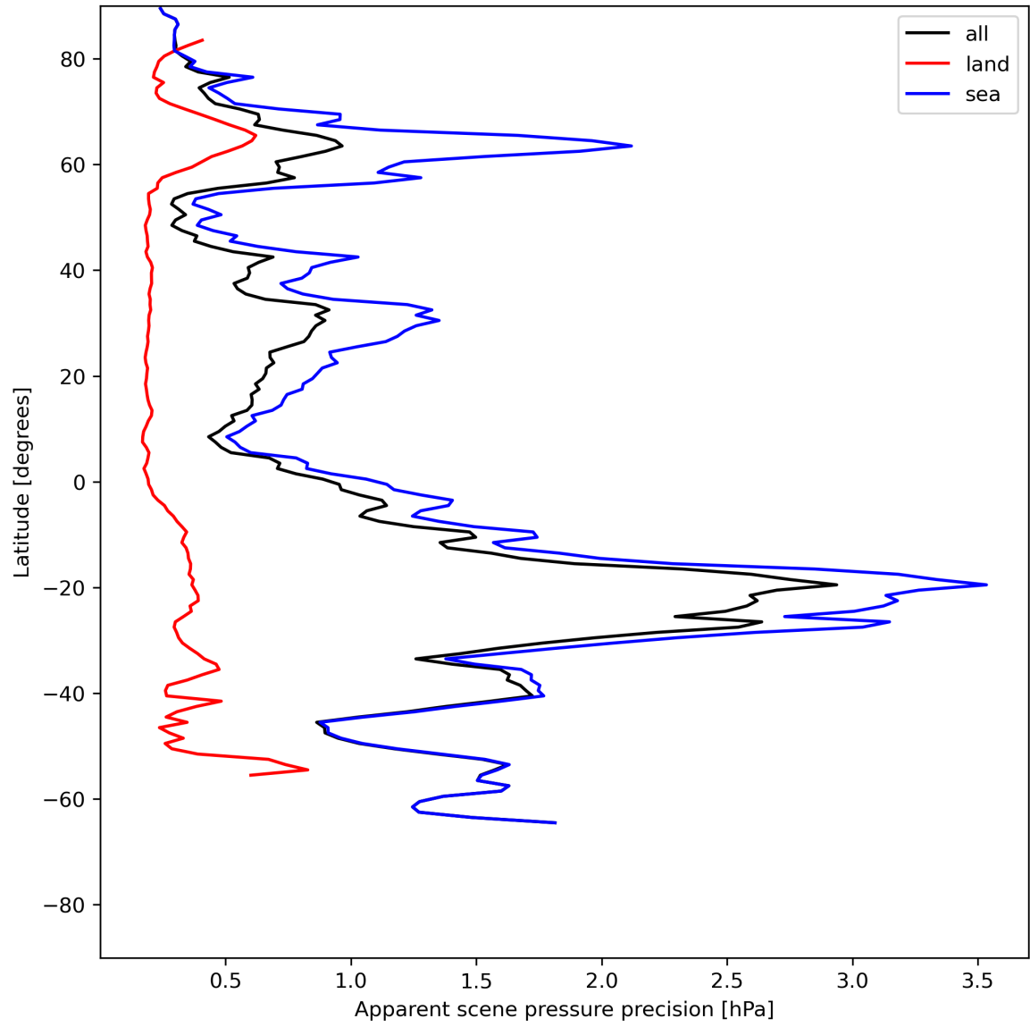
Figure 20: Zonal average of “Apparent scene pressure precision” for 2024-06-16 to 2024-06-18.
