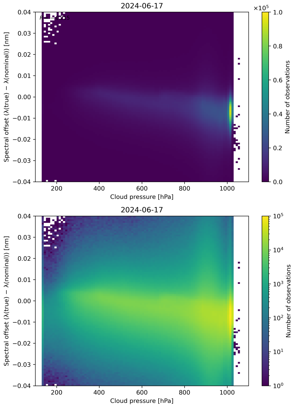
Figure 84: Scatter density plot of “Cloud pressure” against “Spectral offset ( \lambda(\text{true}) - \lambda(\text{nominal}) )” for 2024-06-16 to 2024-06-18.
