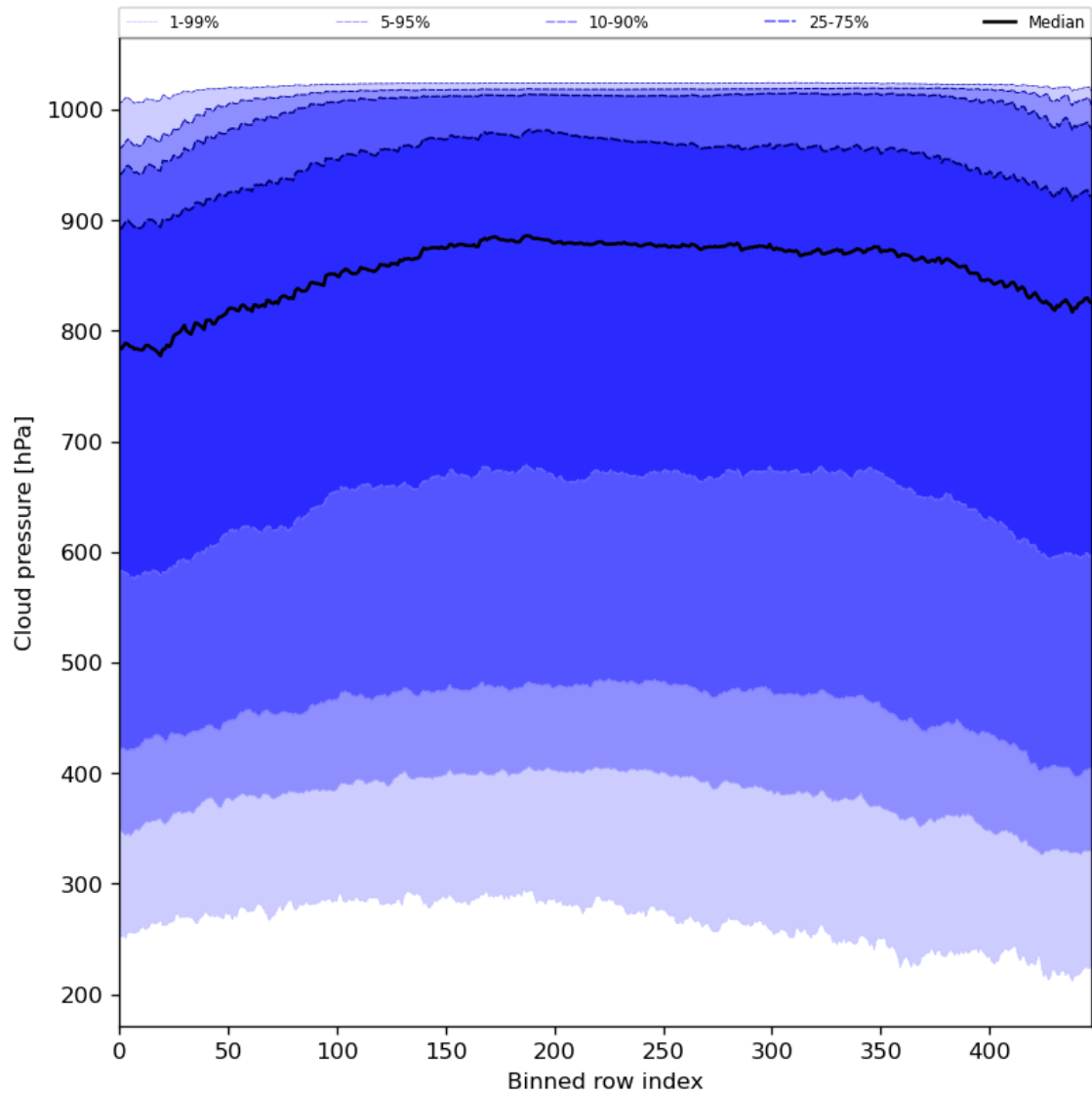
Figure 47: Along track statistics of “Cloud pressure” for 2024-06-16 to 2024-06-18
