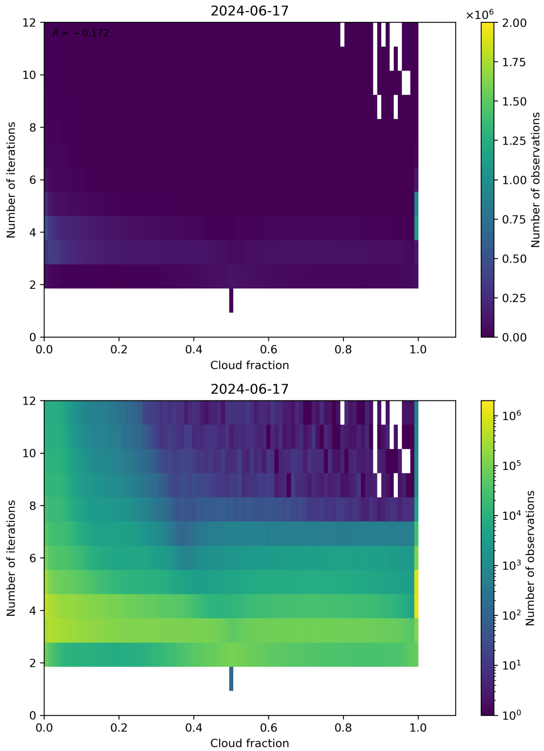
Figure 73: Scatter density plot of “Cloud fraction” against “Number of iterations” for 2024-06-16 to 2024-06-18.
