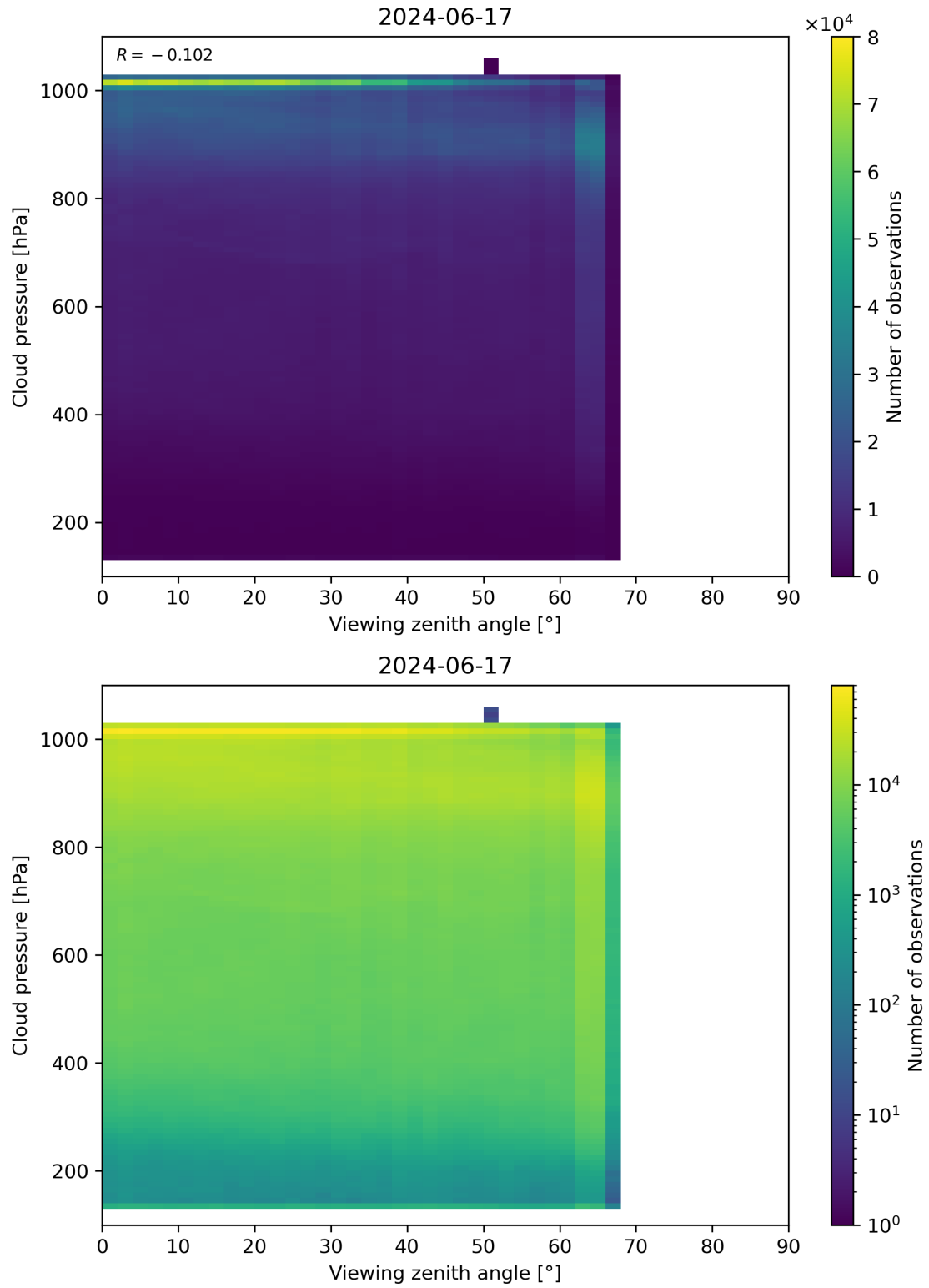
Figure 121: Scatter density plot of “Viewing zenith angle” against “Cloud pressure” for 2024-06-16 to 2024-06-18.
