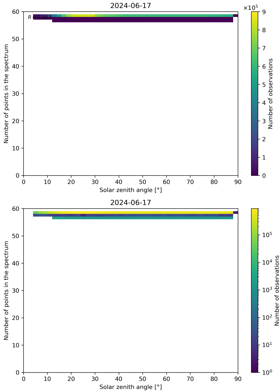
Figure 115: Scatter density plot of “Solar zenith angle” against “Number of points in the spectrum” for 2024-06-16 to 2024-06-18.
