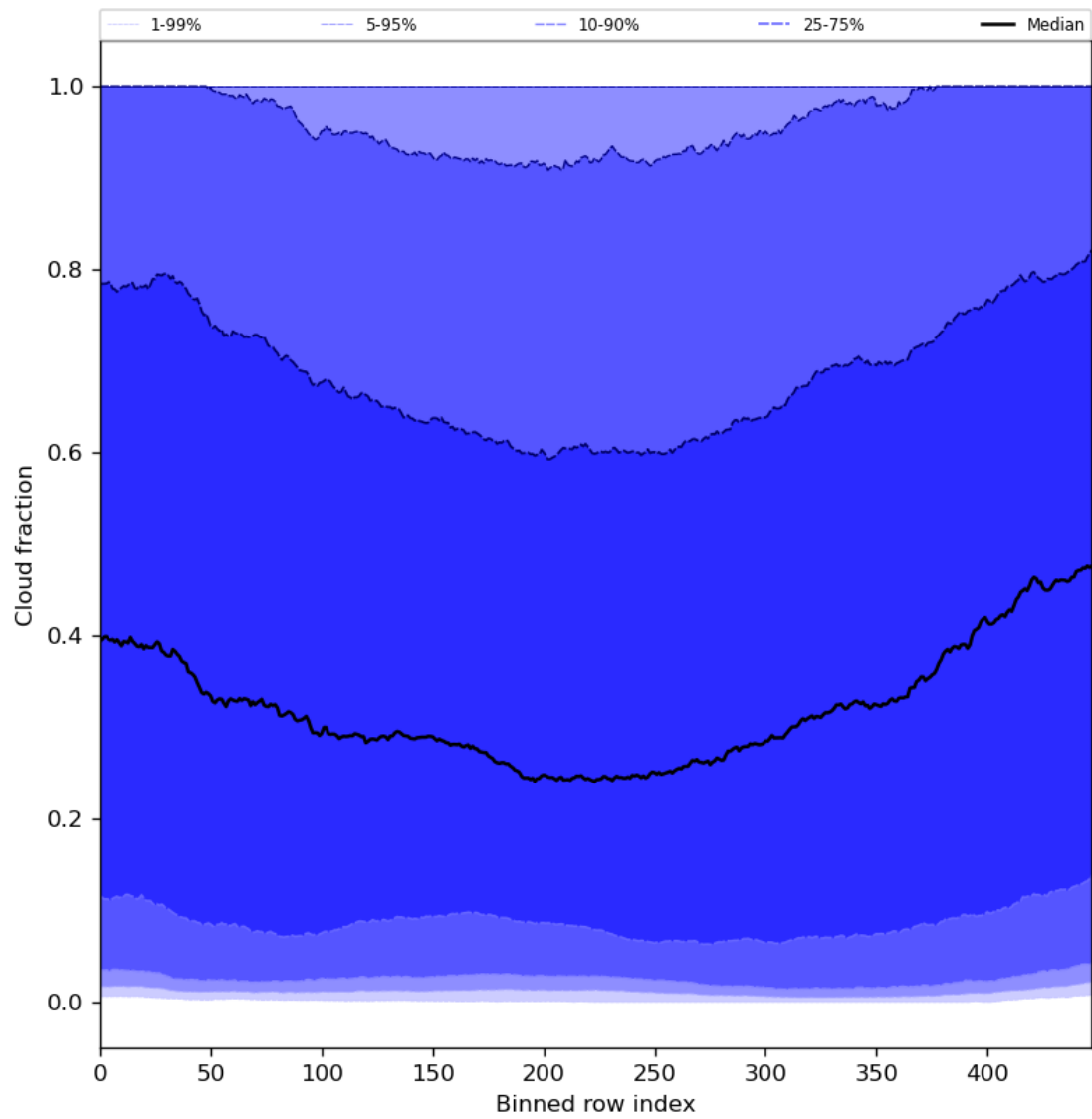
Figure 49: Along track statistics of “Cloud fraction” for 2024-06-16 to 2024-06-18
