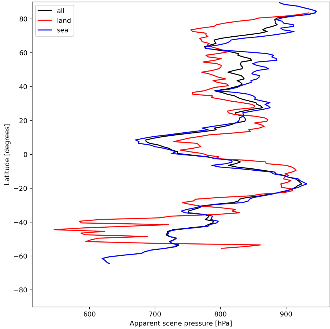
Figure 19: Zonal average of “Apparent scene pressure” for 2024-06-16 to 2024-06-18.
