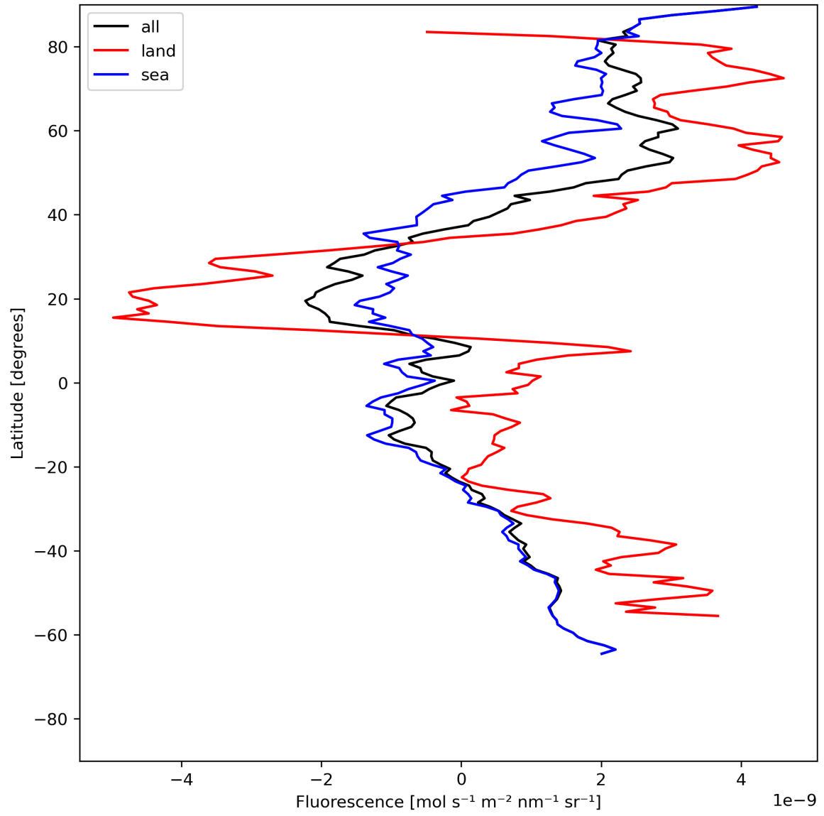
Figure 23: Zonal average of “Fluorescence” for 2024-06-16 to 2024-06-18.
