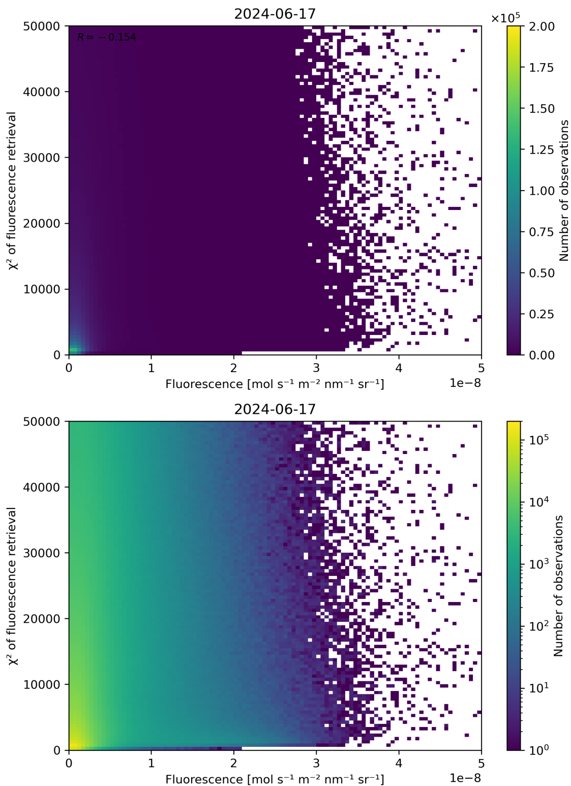
Figure 85: Scatter density plot of “Fluorescence” against “ \chi^2 of fluorescence retrieval” for 2024-06-16 to 2024-06-18.
