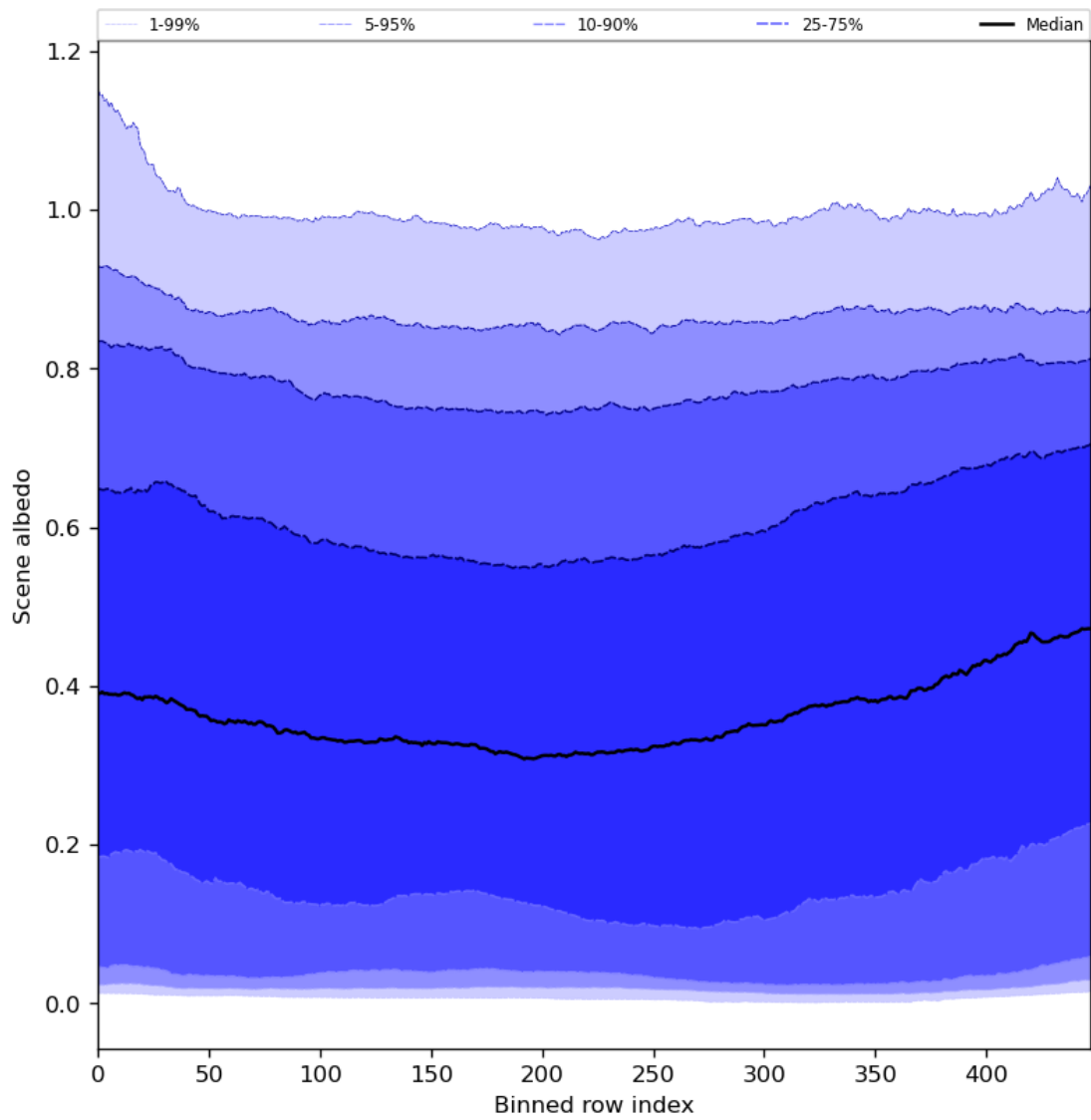
Figure 51: Along track statistics of “Scene albedo” for 2024-06-16 to 2024-06-18
