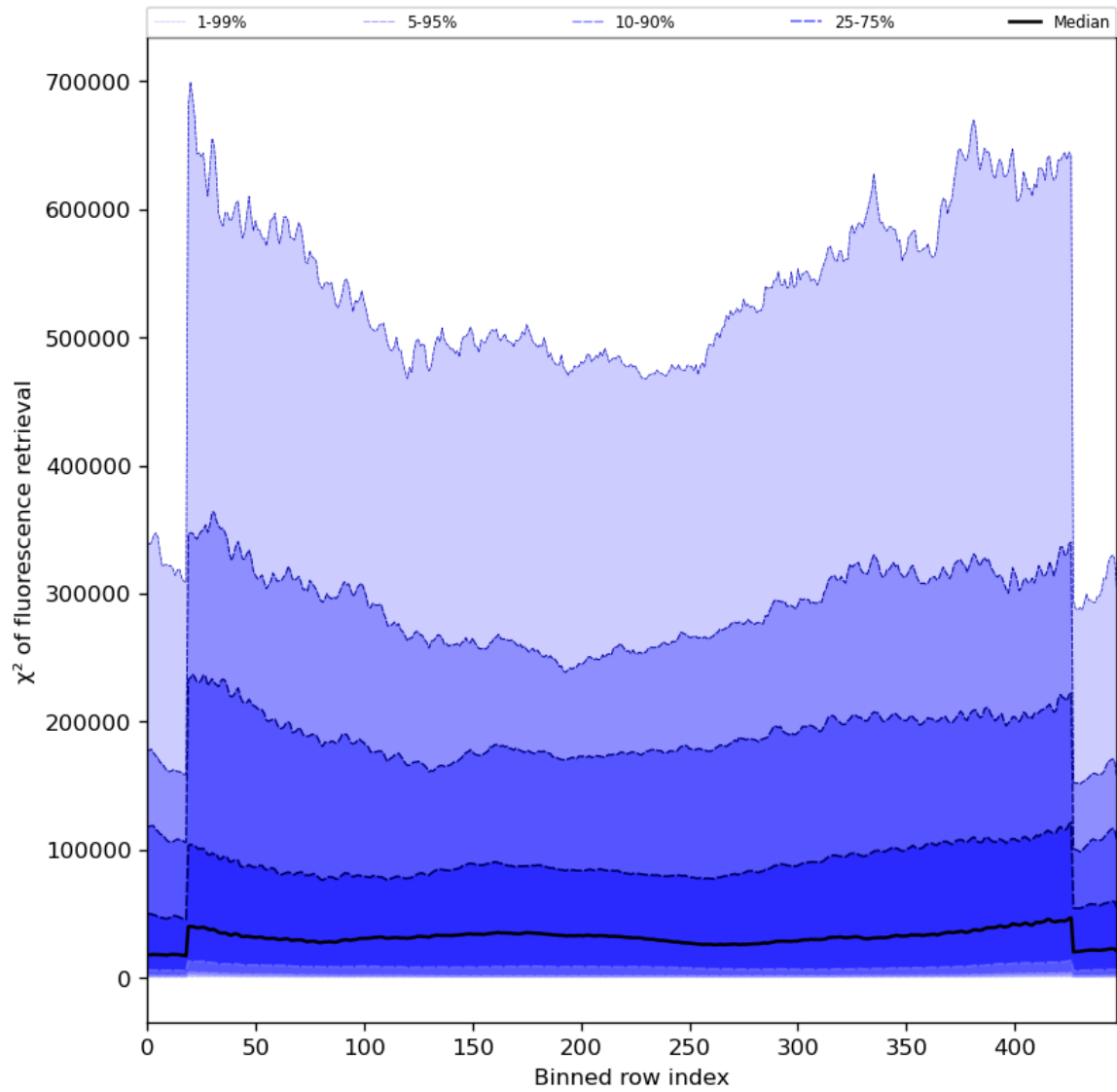
Figure 59: Along track statistics of “ \chi^2 of fluorescence retrieval” for 2024-06-16 to 2024-06-18
