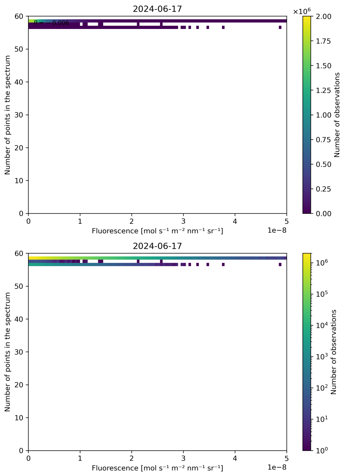
Figure 86: Scatter density plot of “Fluorescence” against “Number of points in the spectrum” for 2024-06-16 to 2024-06-18.
