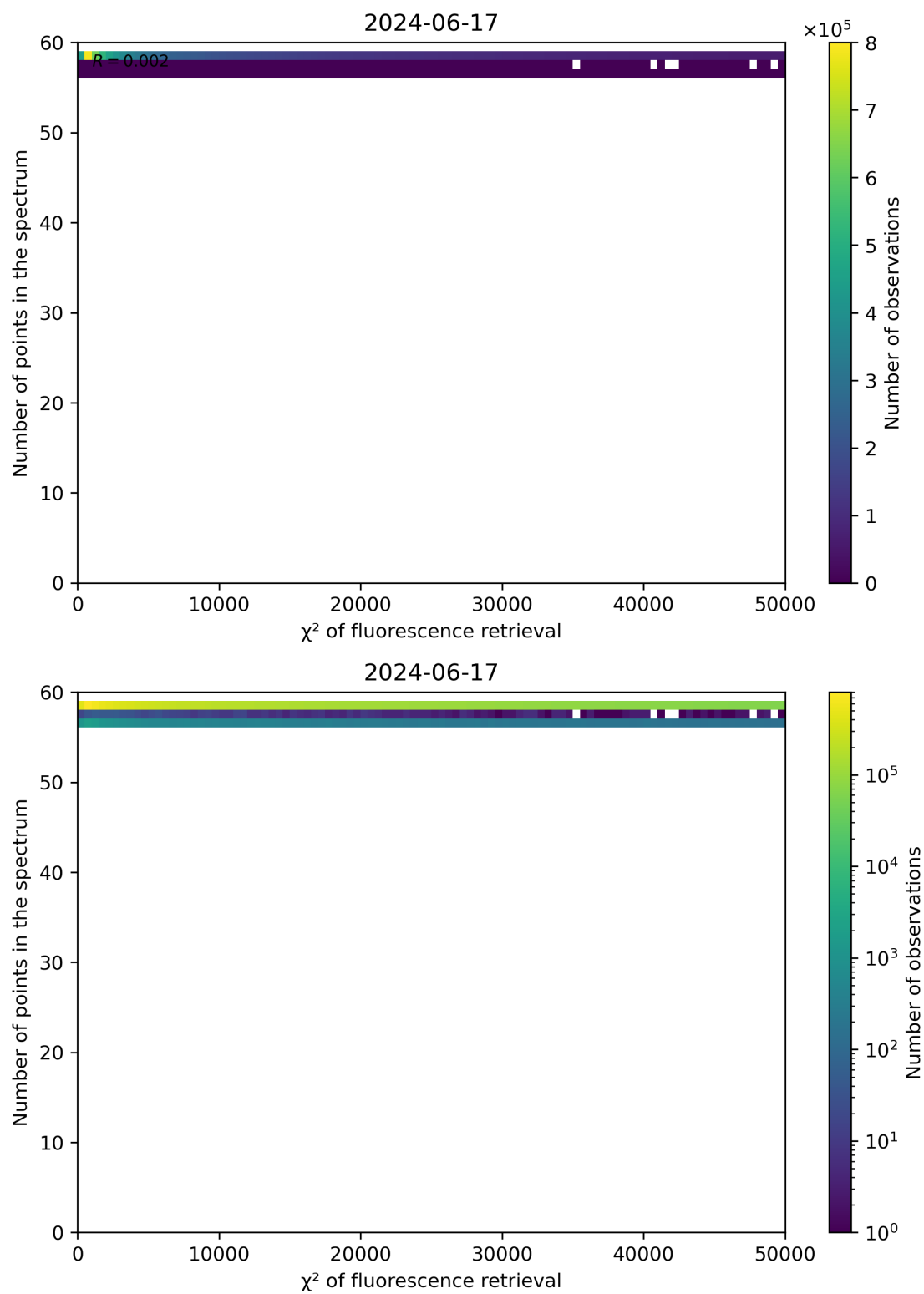
Figure 68: Scatter density plot of “ \chi^2 of fluorescence retrieval” against “Number of points in the spectrum” for 2024-06-16 to 2024-06-18.
