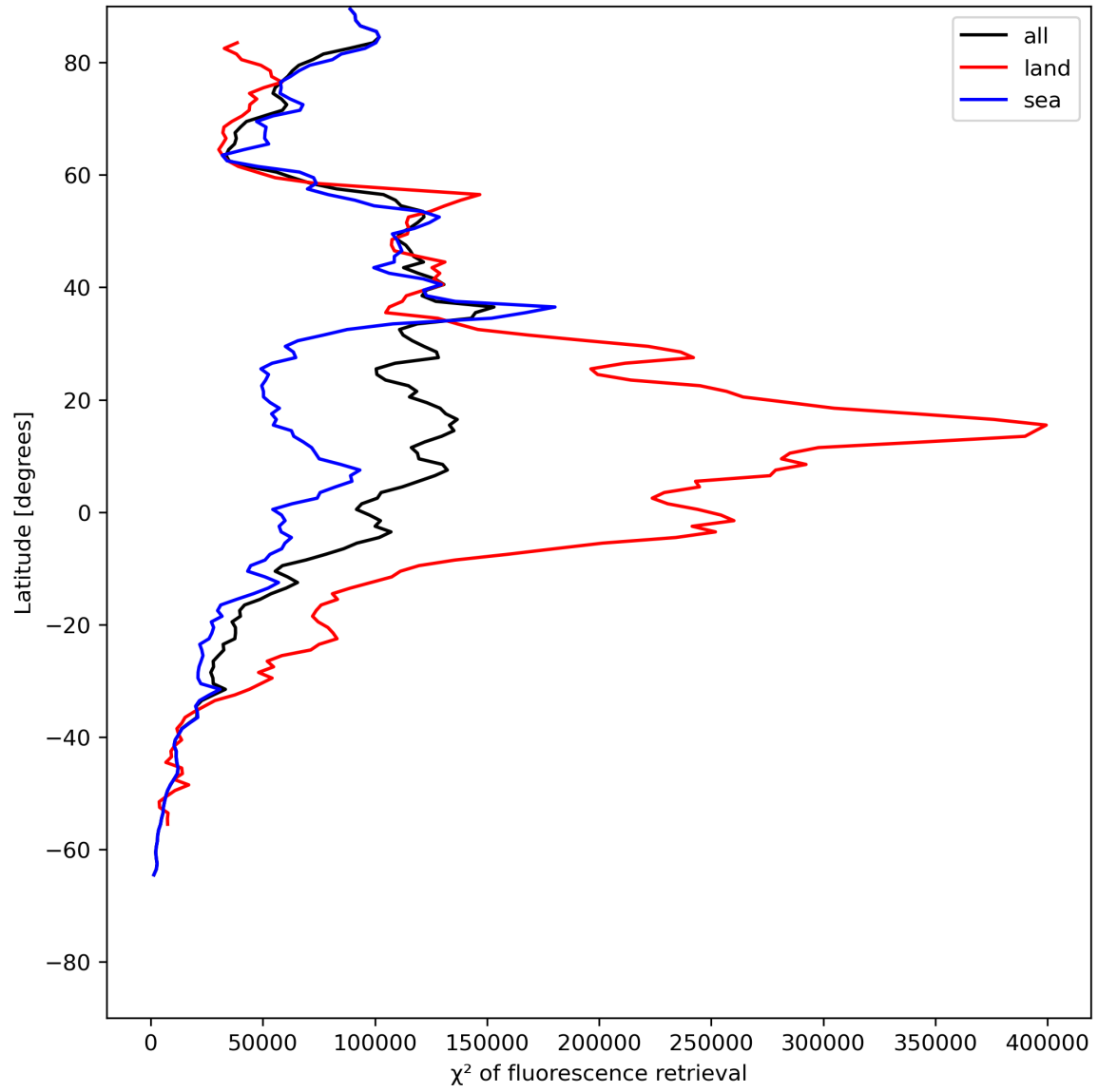
Figure 25: Zonal average of “ \chi^2 of fluorescence retrieval” for 2024-06-16 to 2024-06-18.
