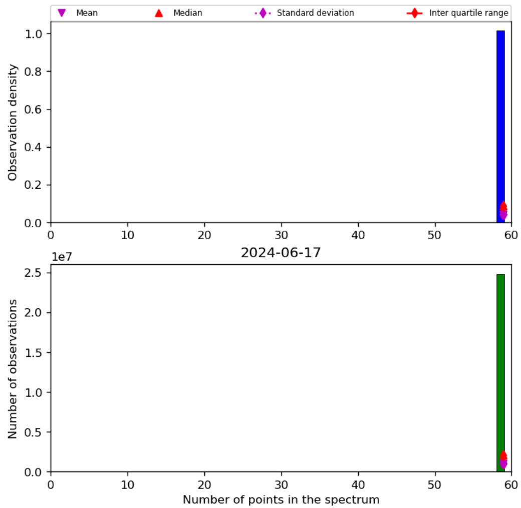
Figure 44: Histogram of “Number of points in the spectrum” for 2024-06-16 to 2024-06-18
