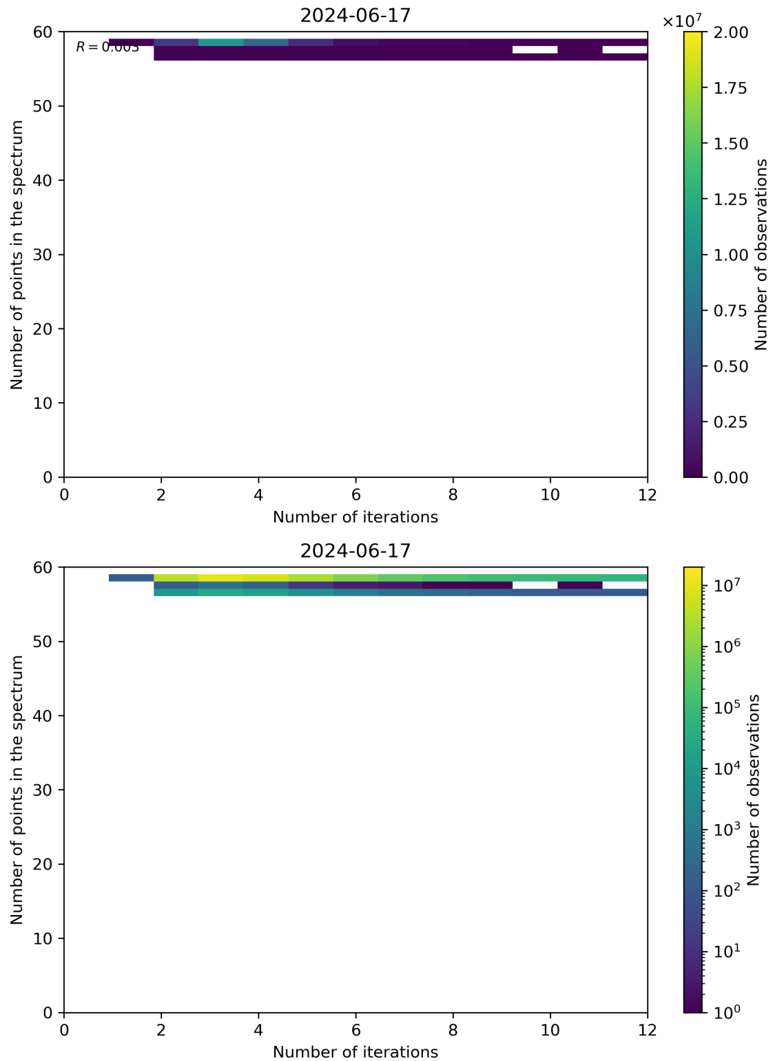
Figure 99: Scatter density plot of “Number of iterations” against “Number of points in the spectrum” for 2024-06-16 to 2024-06-18.
