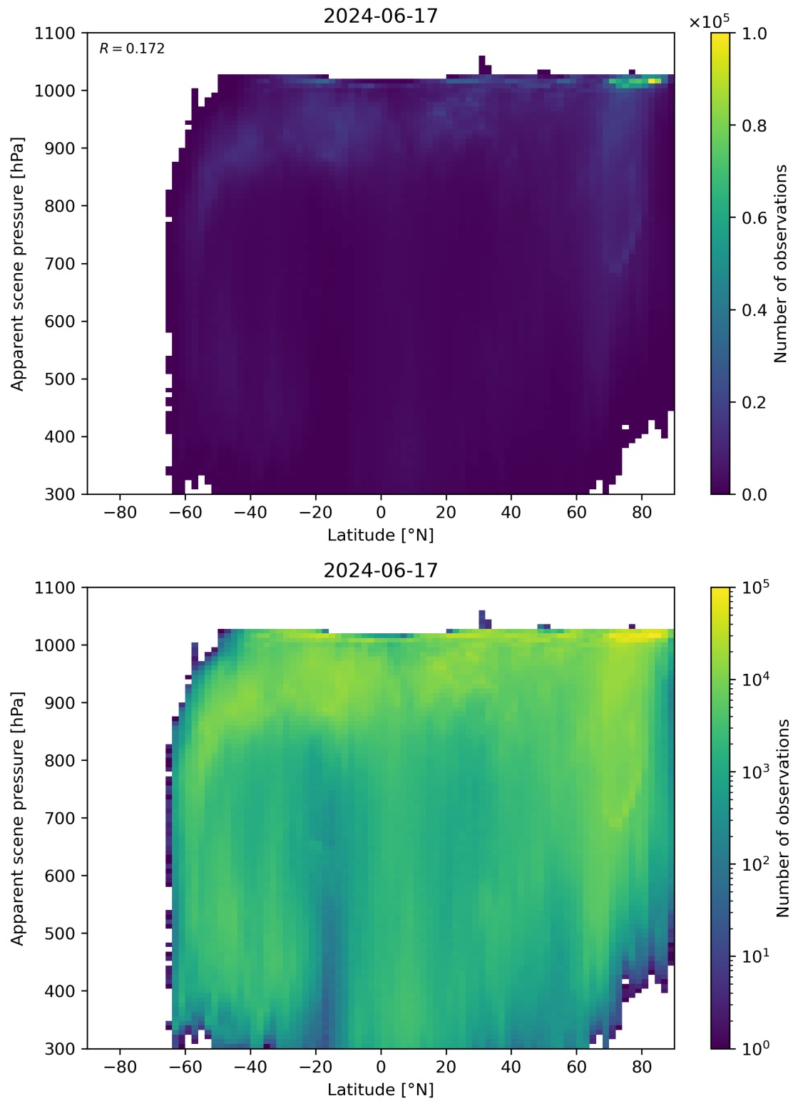
Figure 88: Scatter density plot of “Latitude” against “Apparent scene pressure” for 2024-06-16 to 2024-06-18.
