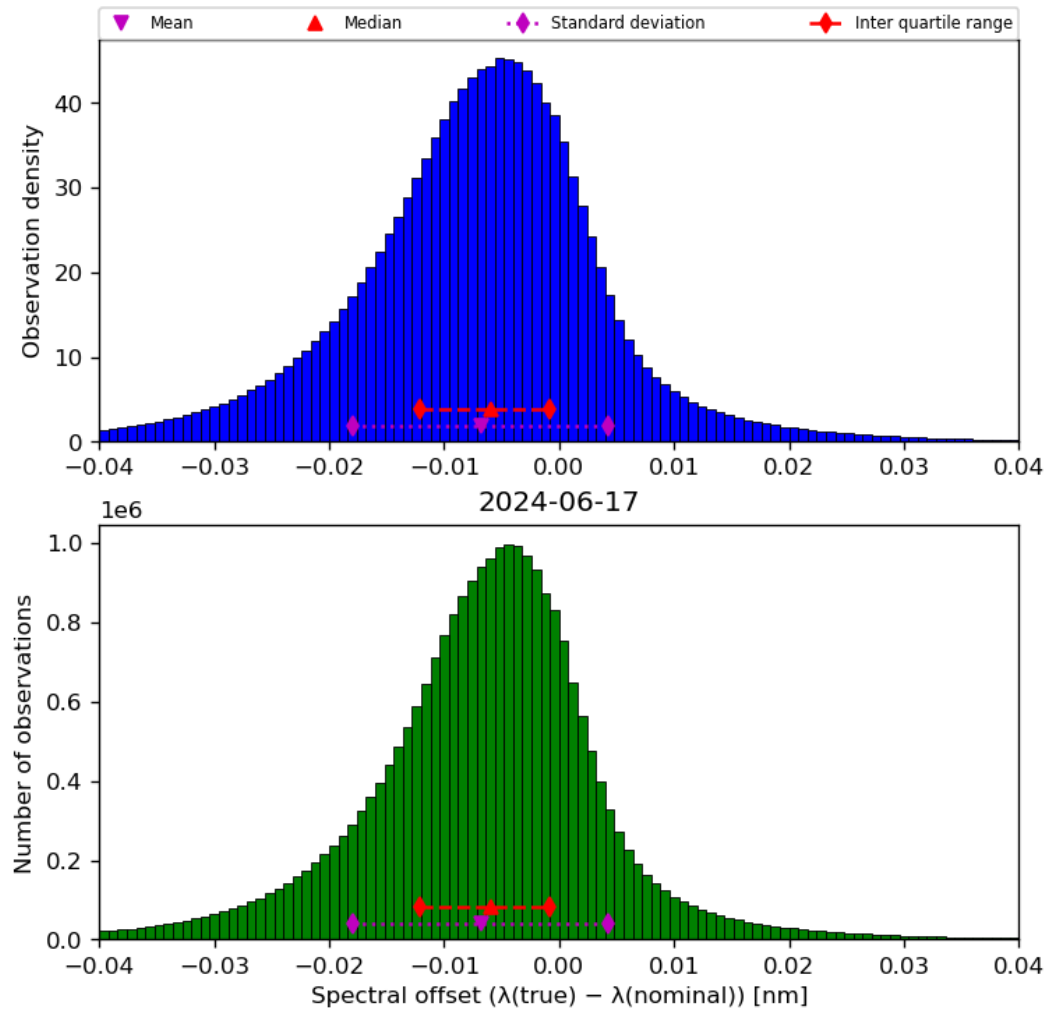
Figure 45: Histogram of “Spectral offset ( \lambda(\text{true}) - \lambda(\text{nominal}) )” for 2024-06-16 to 2024-06-18
