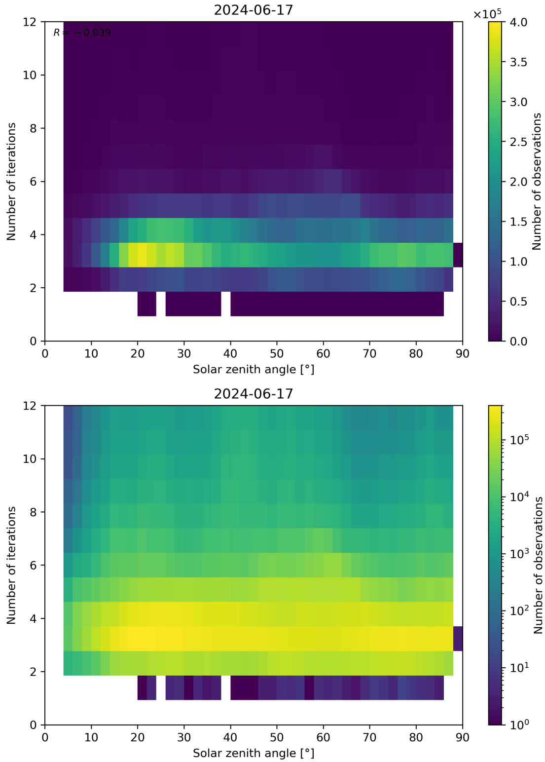
Figure 114: Scatter density plot of “Solar zenith angle” against “Number of iterations” for 2024-06-16 to 2024-06-18.
