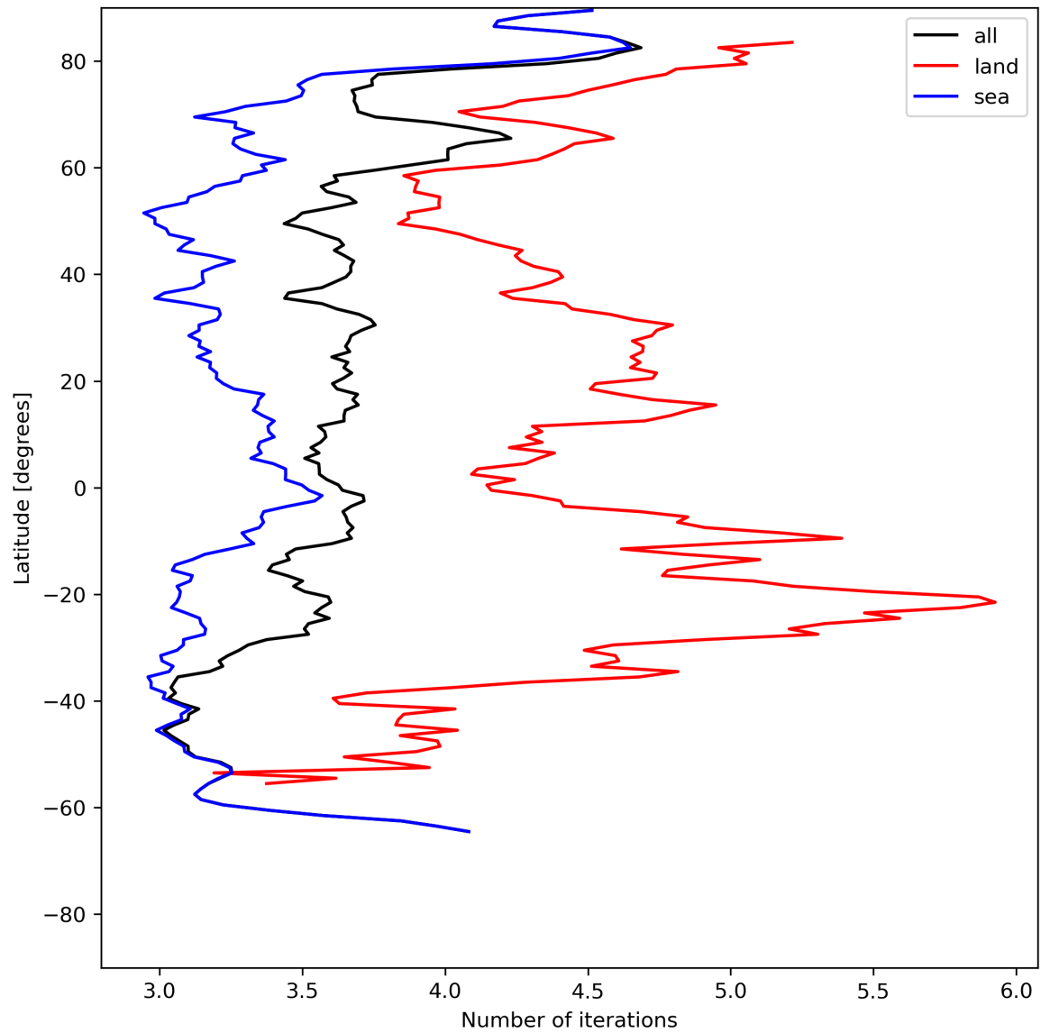
Figure 22: Zonal average of “Number of iterations” for 2024-06-16 to 2024-06-18.
