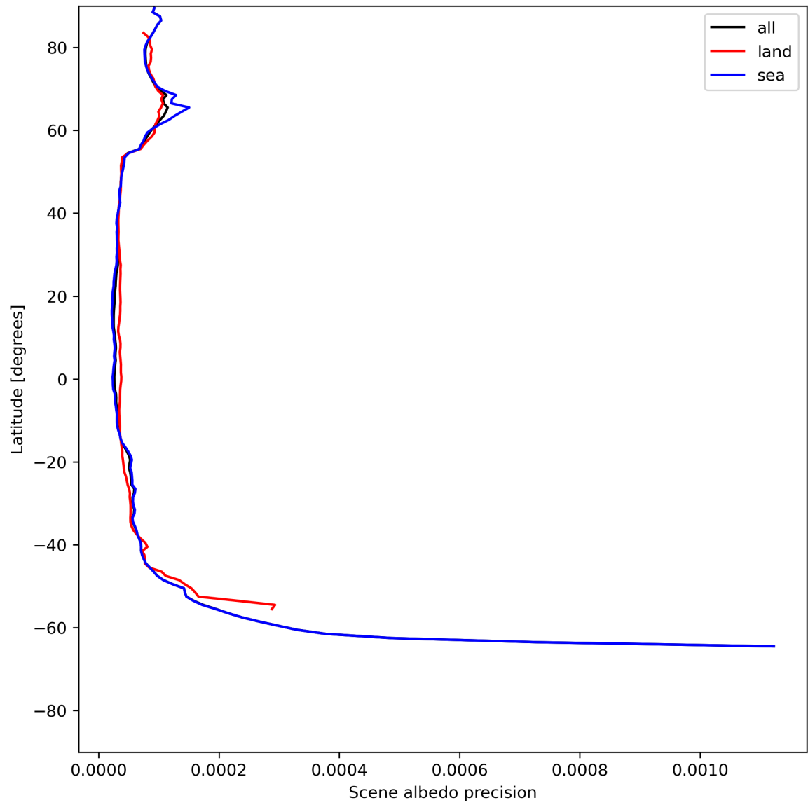
Figure 18: Zonal average of “Scene albedo precision” for 2024-06-16 to 2024-06-18.
