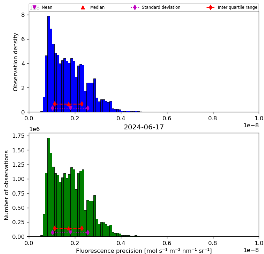
Figure 41: Histogram of “Fluorescence precision” for 2024-06-16 to 2024-06-18
