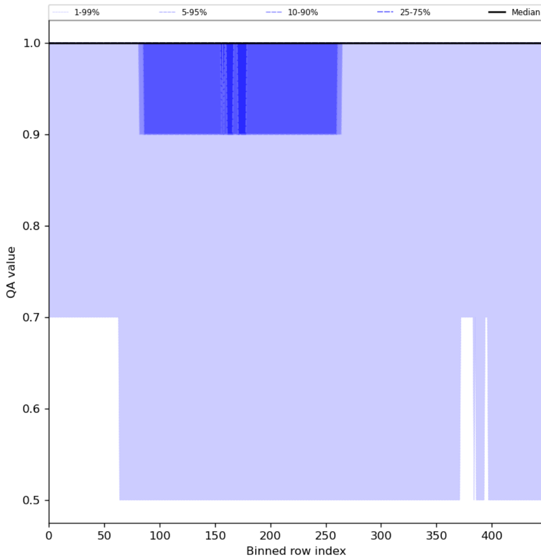
Figure 46: Along track statistics of “QA value” for 2024-06-16 to 2024-06-18
