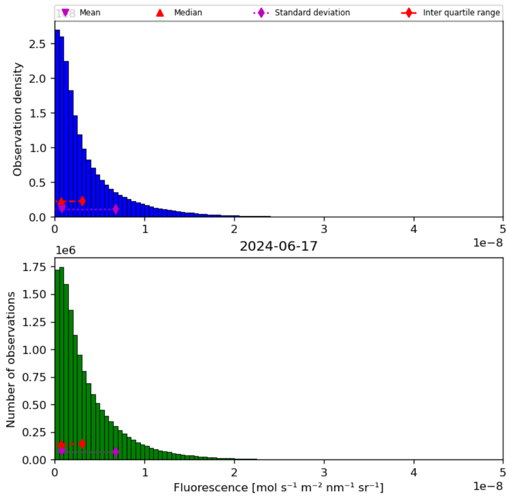
Figure 40: Histogram of “Fluorescence” for 2024-06-16 to 2024-06-18
