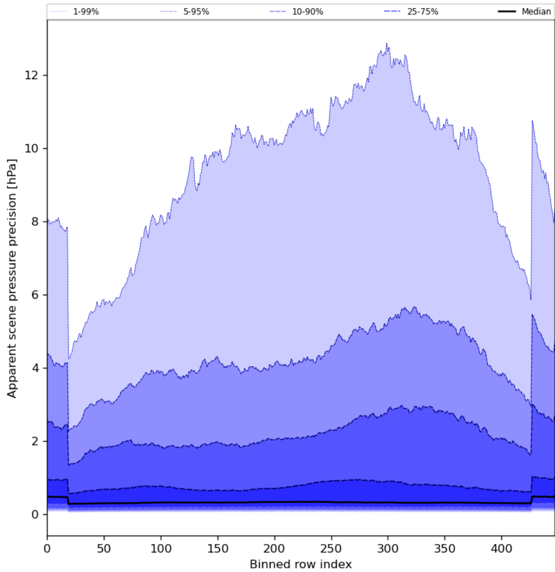
Figure 54: Along track statistics of “Apparent scene pressure precision” for 2024-06-16 to 2024-06-18
