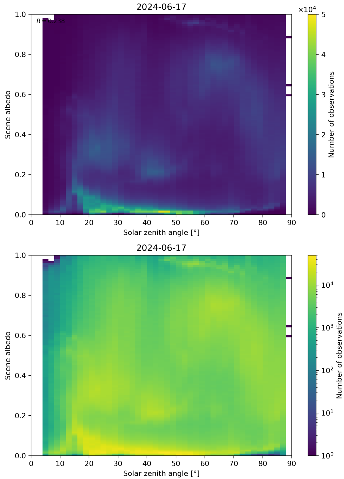
Figure 116: Scatter density plot of “Solar zenith angle” against “Scene albedo” for 2024-06-16 to 2024-06-18.
