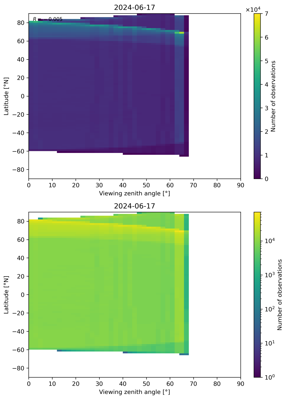
Figure 123: Scatter density plot of “Viewing zenith angle” against “Latitude” for 2024-06-16 to 2024-06-18.
