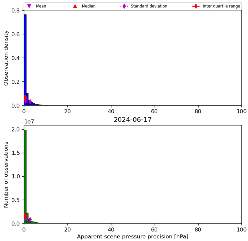
Figure 37: Histogram of “Apparent scene pressure precision” for 2024-06-16 to 2024-06-18
