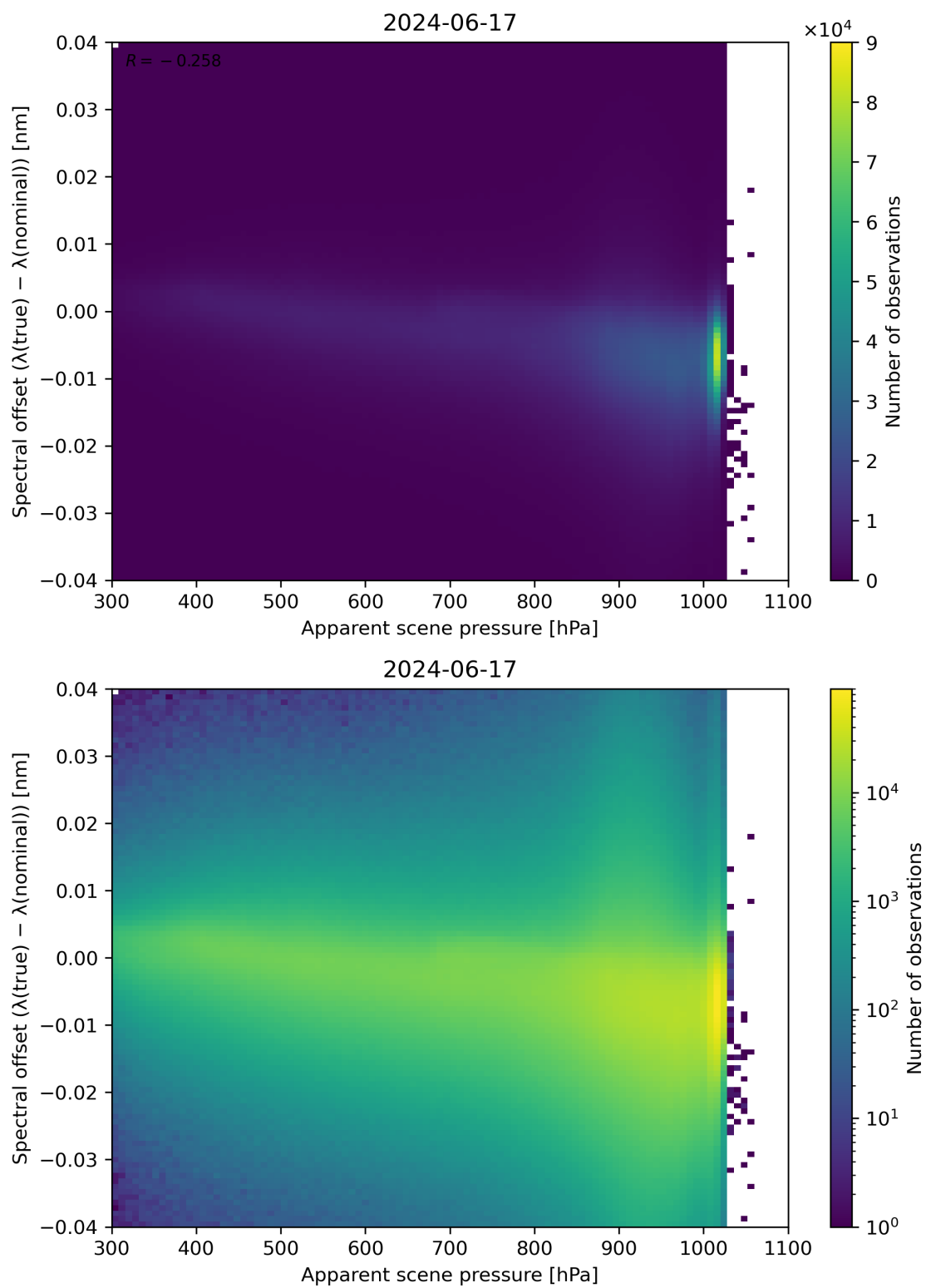
Figure 67: Scatter density plot of “Apparent scene pressure” against “Spectral offset ( \lambda(\text{true}) - \lambda(\text{nominal}) )” for 2024-06-16 to 2024-06-18.
