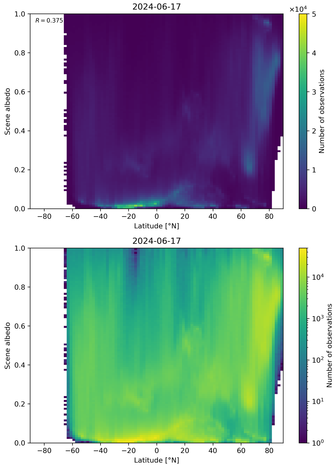
Figure 95: Scatter density plot of “Latitude” against “Scene albedo” for 2024-06-16 to 2024-06-18.
