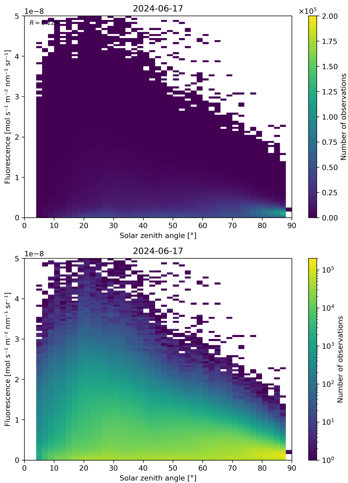
Figure 112: Scatter density plot of “Solar zenith angle” against “Fluorescence” for 2024-06-16 to 2024-06-18.
