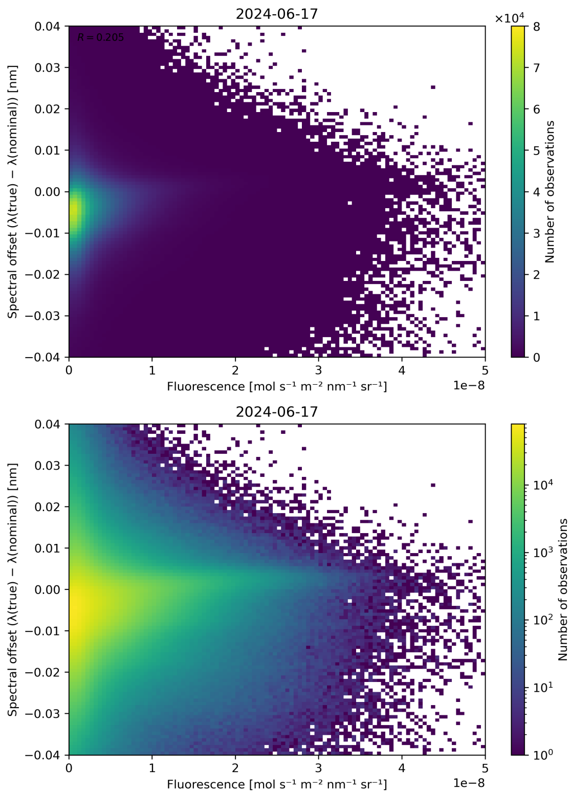
Figure 87: Scatter density plot of “Fluorescence” against “Spectral offset ( \lambda(\text{true}) - \lambda(\text{nominal}) )” for 2024-06-16 to 2024-06-18.
