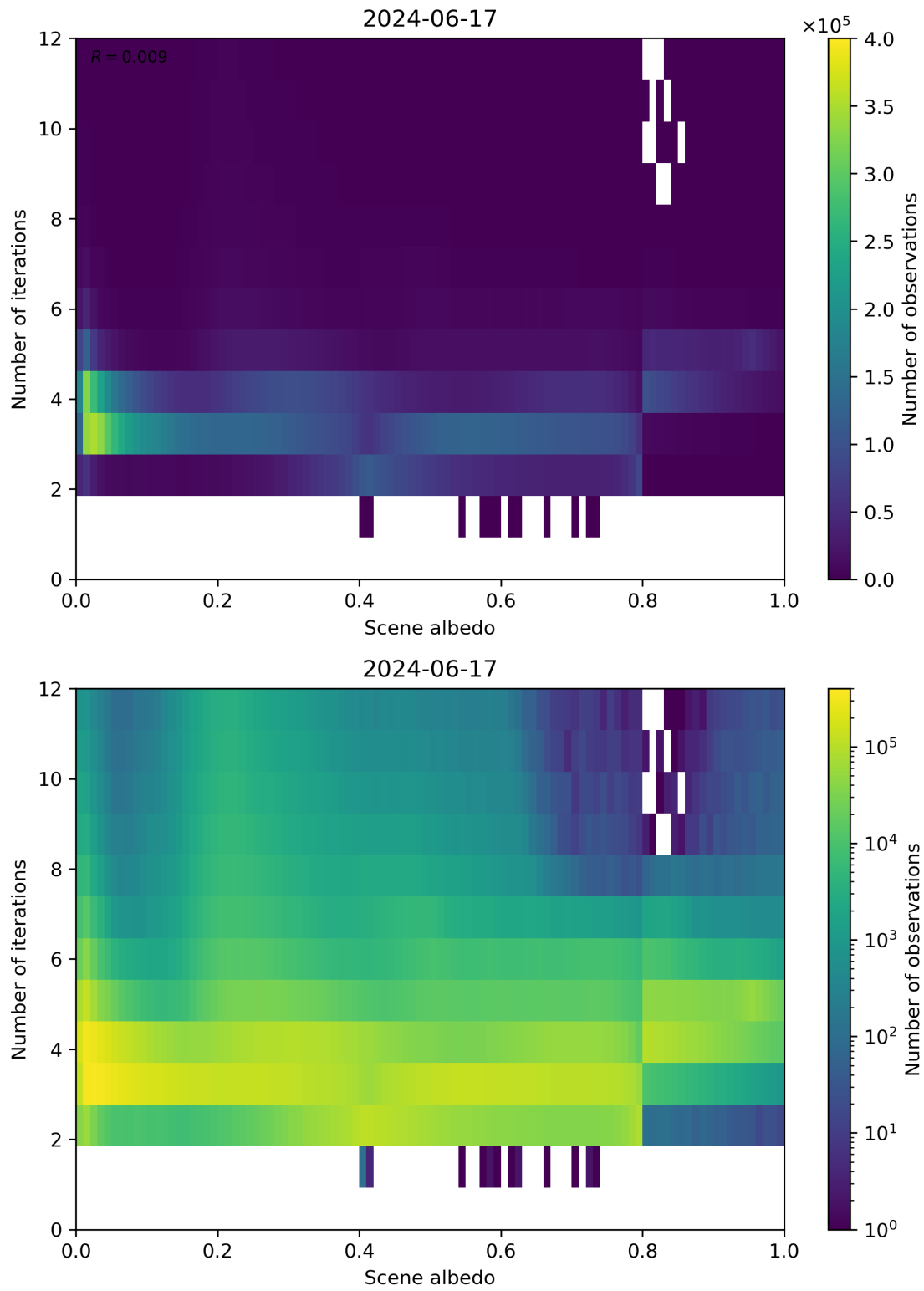
Figure 105: Scatter density plot of “Scene albedo” against “Number of iterations” for 2024-06-16 to 2024-06-18.
