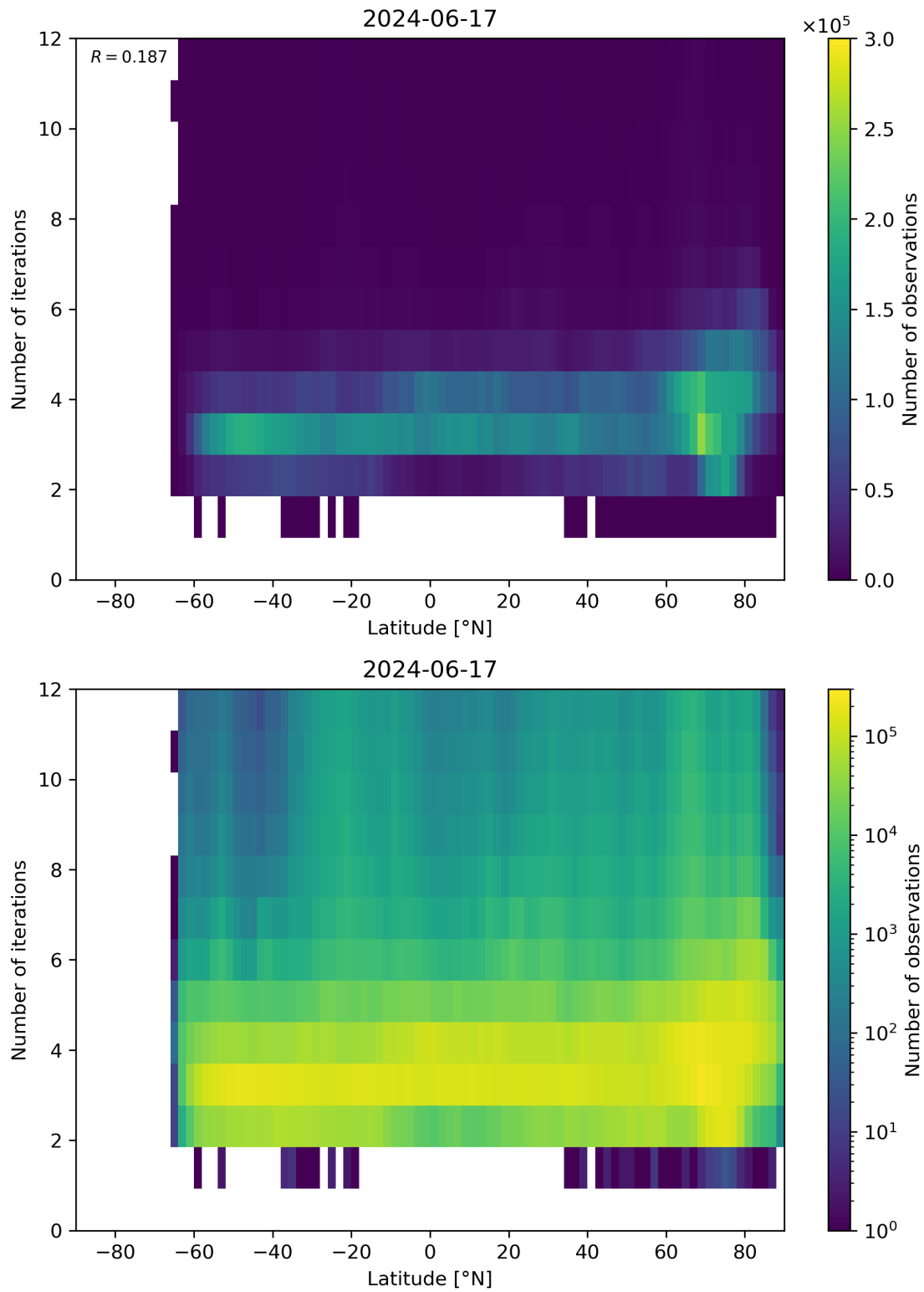
Figure 93: Scatter density plot of “Latitude” against “Number of iterations” for 2024-06-16 to 2024-06-18.
