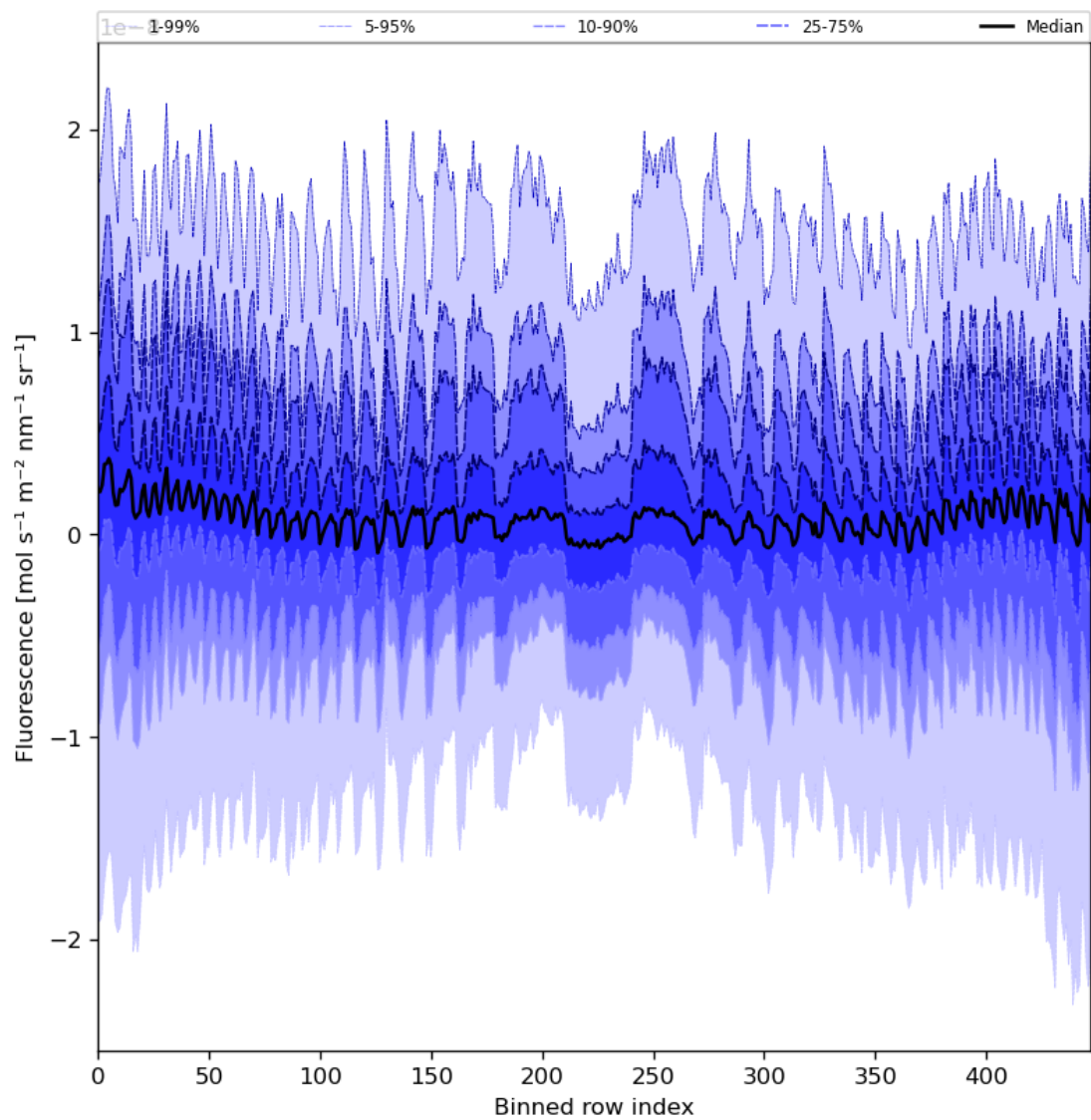
Figure 57: Along track statistics of “Fluorescence” for 2024-06-16 to 2024-06-18
