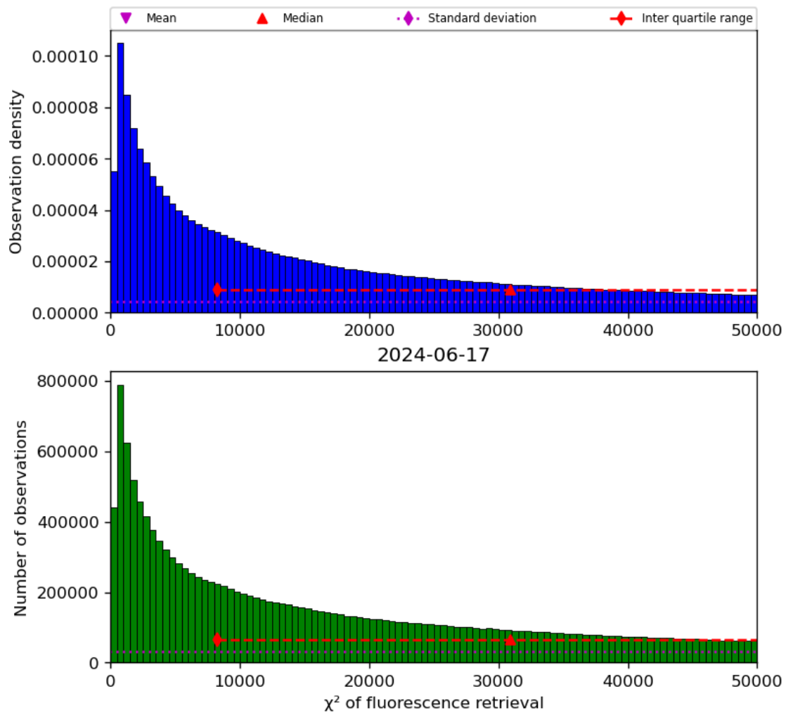
Figure 42: Histogram of “ \chi^2 of fluorescence retrieval” for 2024-06-16 to 2024-06-18
