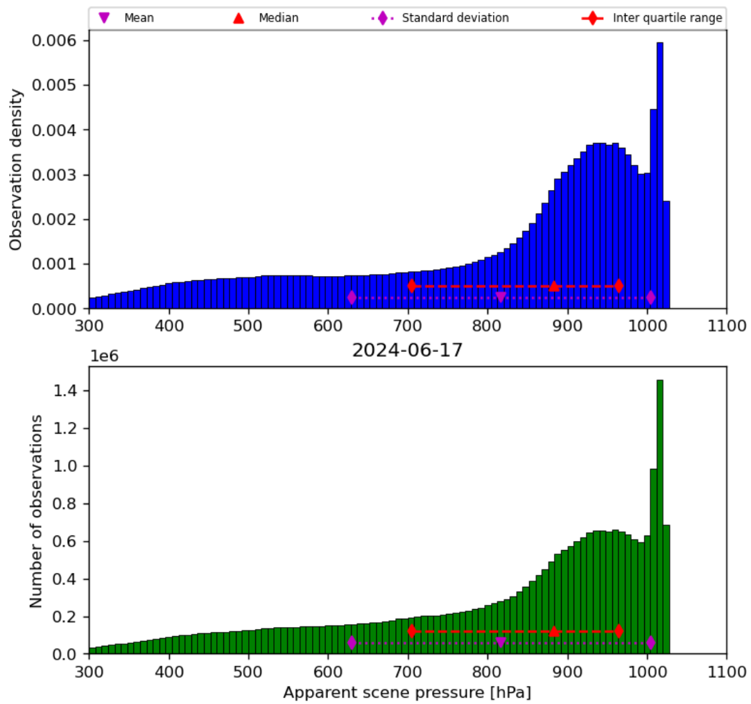
Figure 36: Histogram of “Apparent scene pressure” for 2024-06-16 to 2024-06-18
