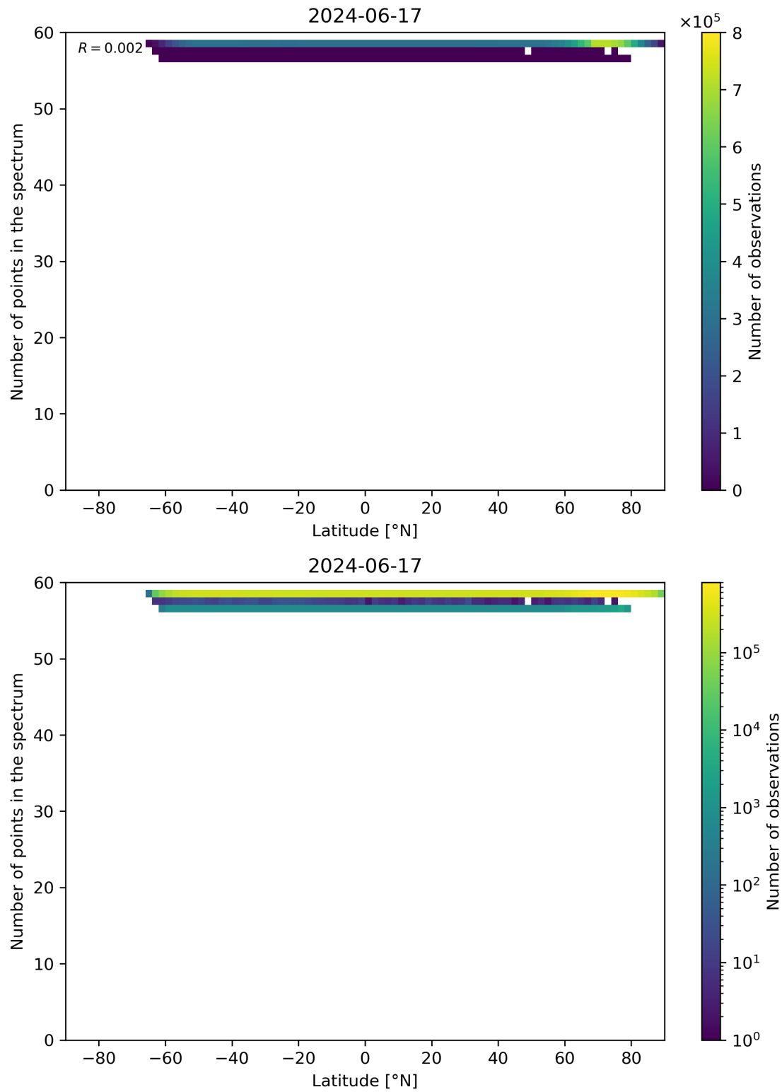
Figure 94: Scatter density plot of “Latitude” against “Number of points in the spectrum” for 2024-06-16 to 2024-06-18.
