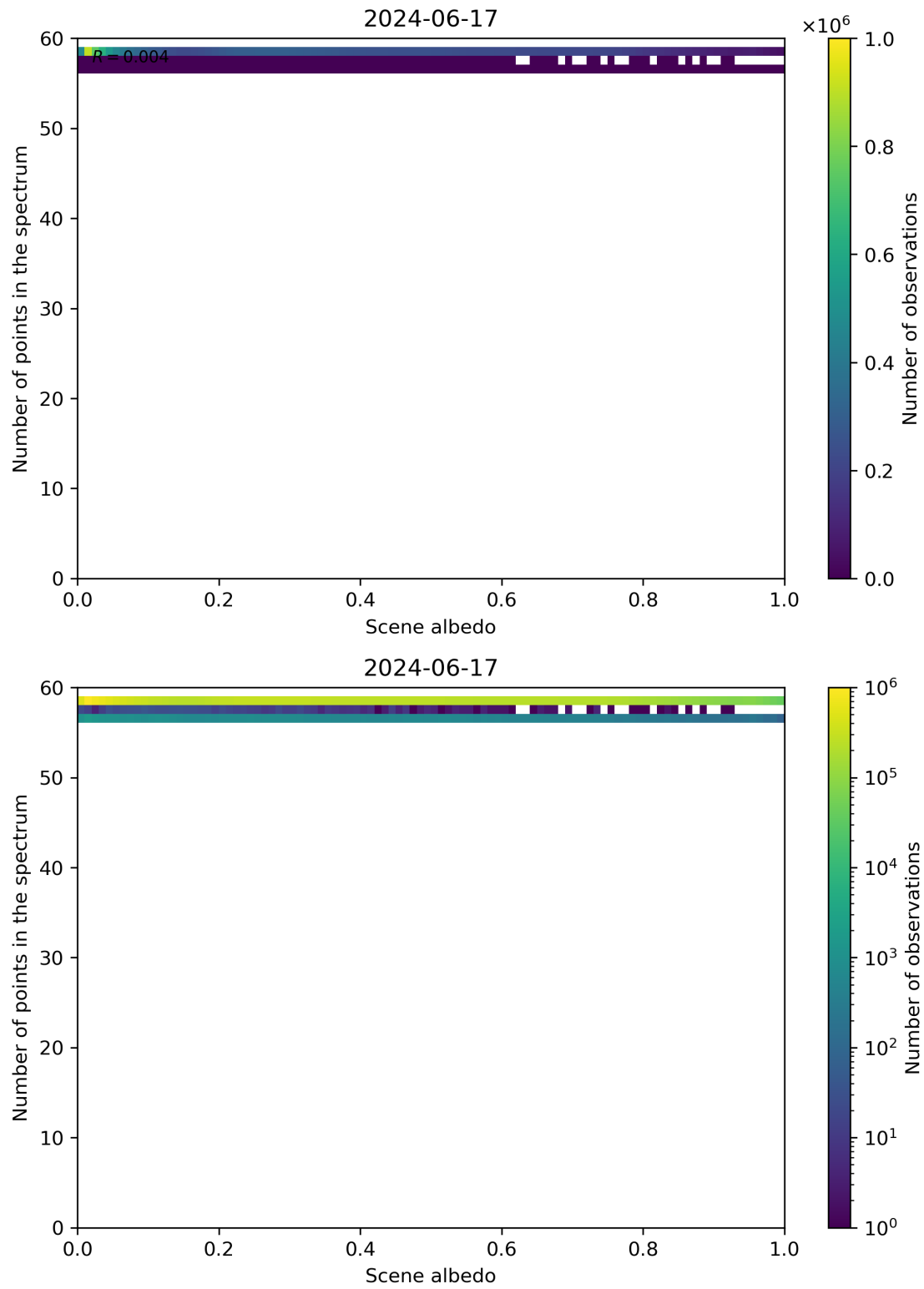
Figure 106: Scatter density plot of “Scene albedo” against “Number of points in the spectrum” for 2024-06-16 to 2024-06-18.
