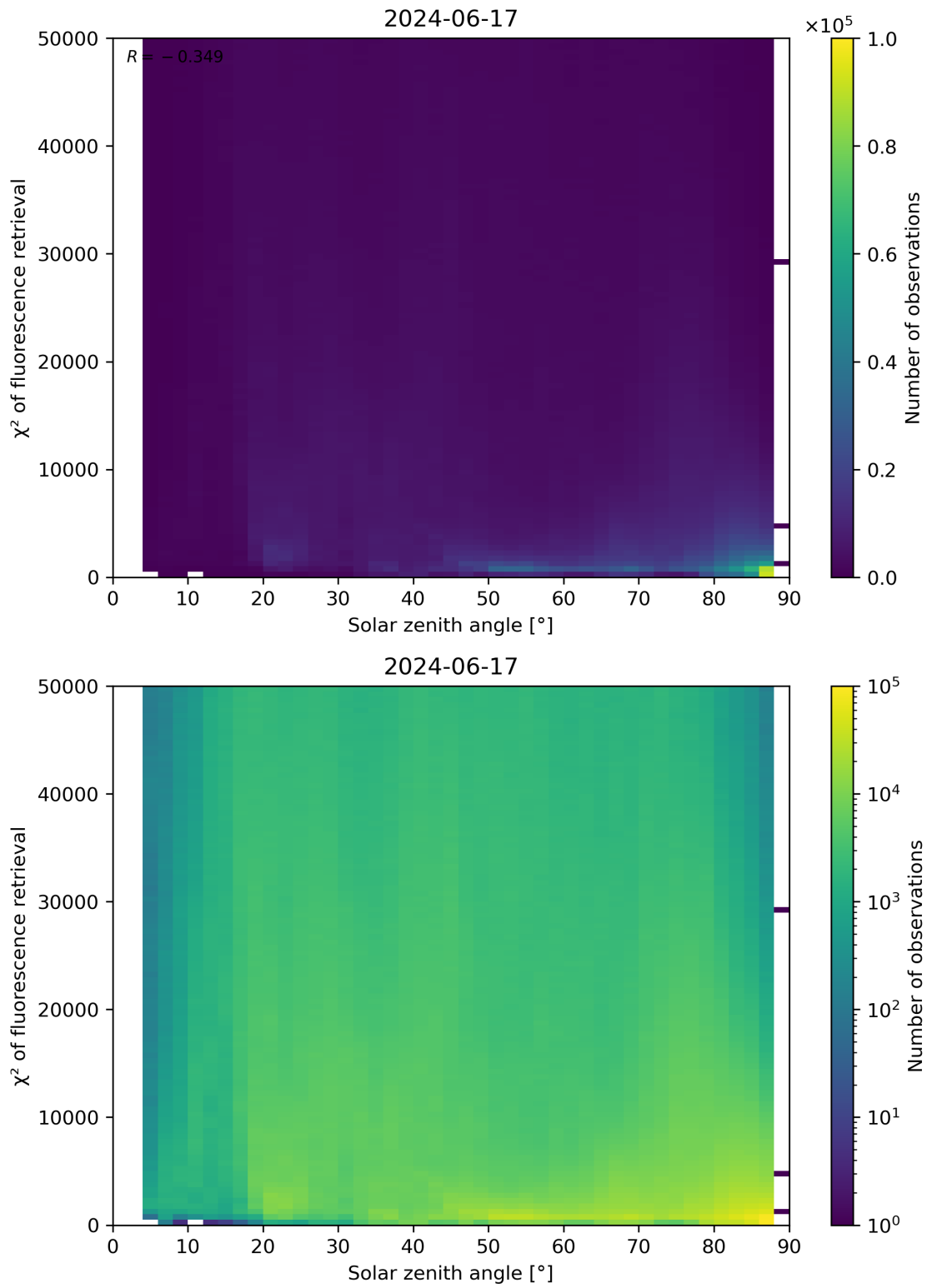
Figure 109: Scatter density plot of “Solar zenith angle” against “ \chi^2 of fluorescence retrieval” for 2024-06-16 to 2024-06-18.
