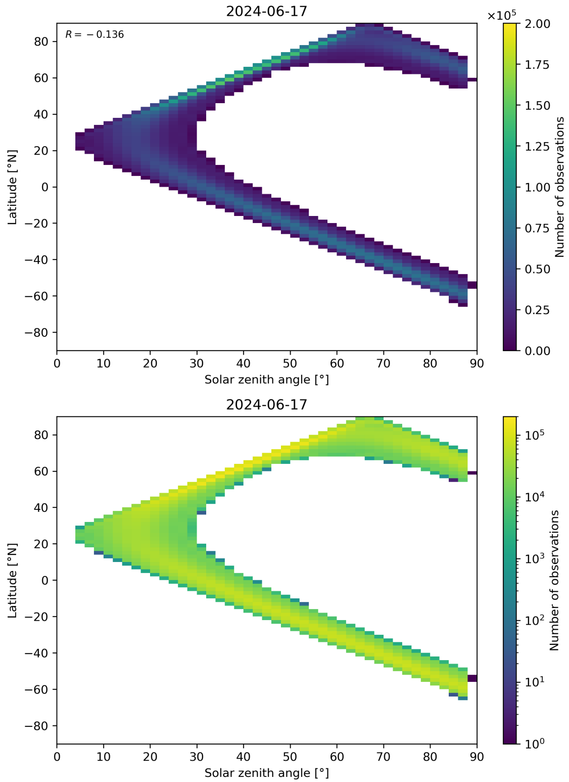
Figure 113: Scatter density plot of “Solar zenith angle” against “Latitude” for 2024-06-16 to 2024-06-18.
