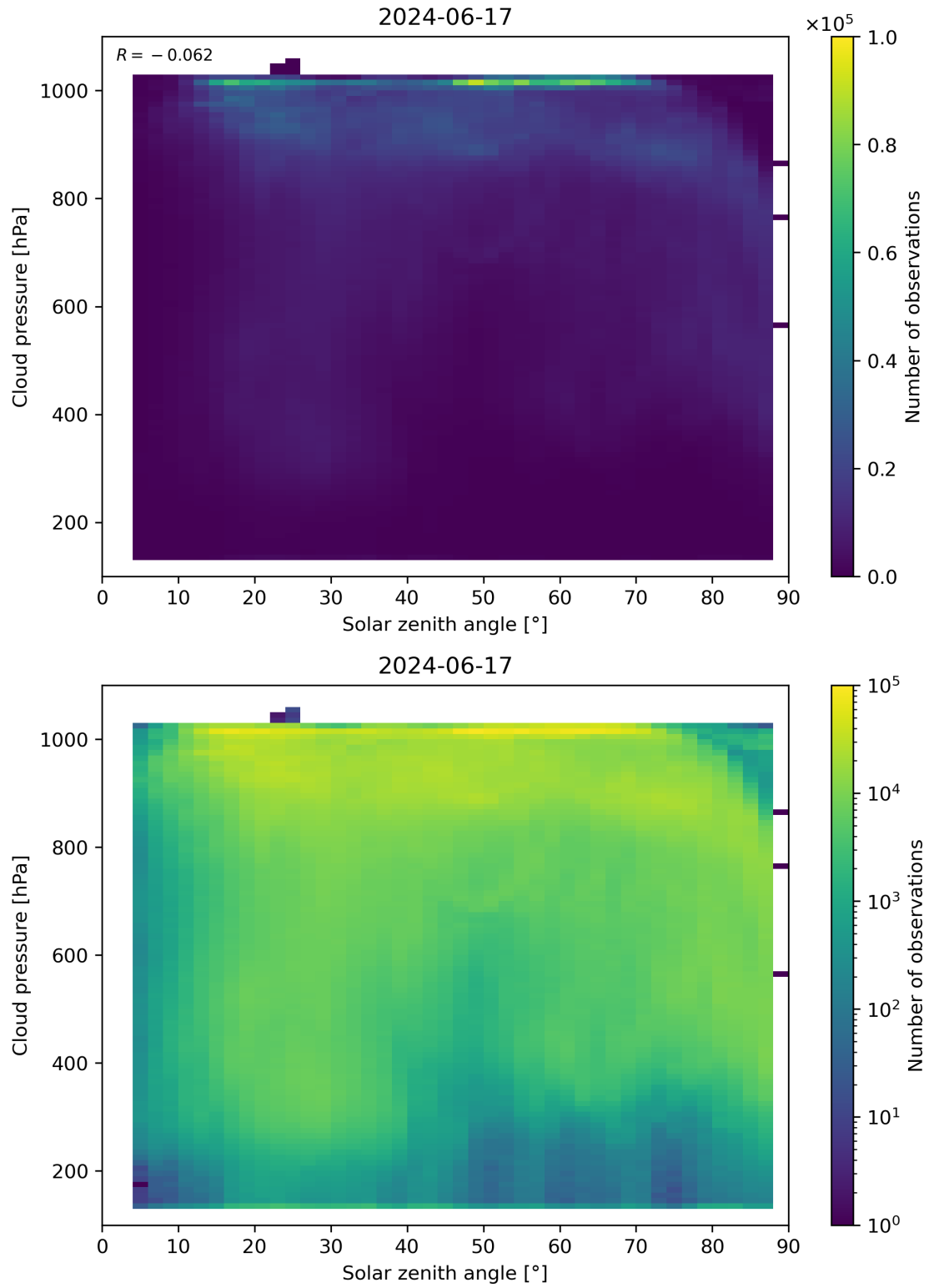
Figure 111: Scatter density plot of “Solar zenith angle” against “Cloud pressure” for 2024-06-16 to 2024-06-18.
