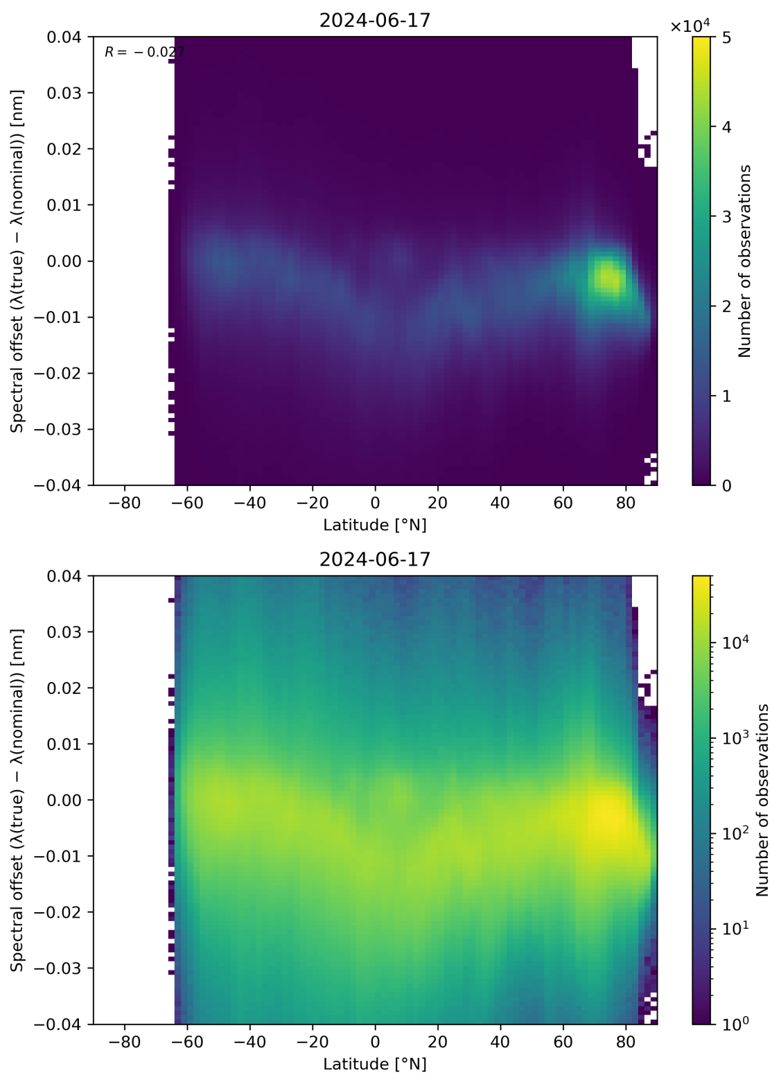
Figure 96: Scatter density plot of “Latitude” against “Spectral offset ( \lambda(\text{true}) - \lambda(\text{nominal}) )” for 2024-06-16 to 2024-06-18.
