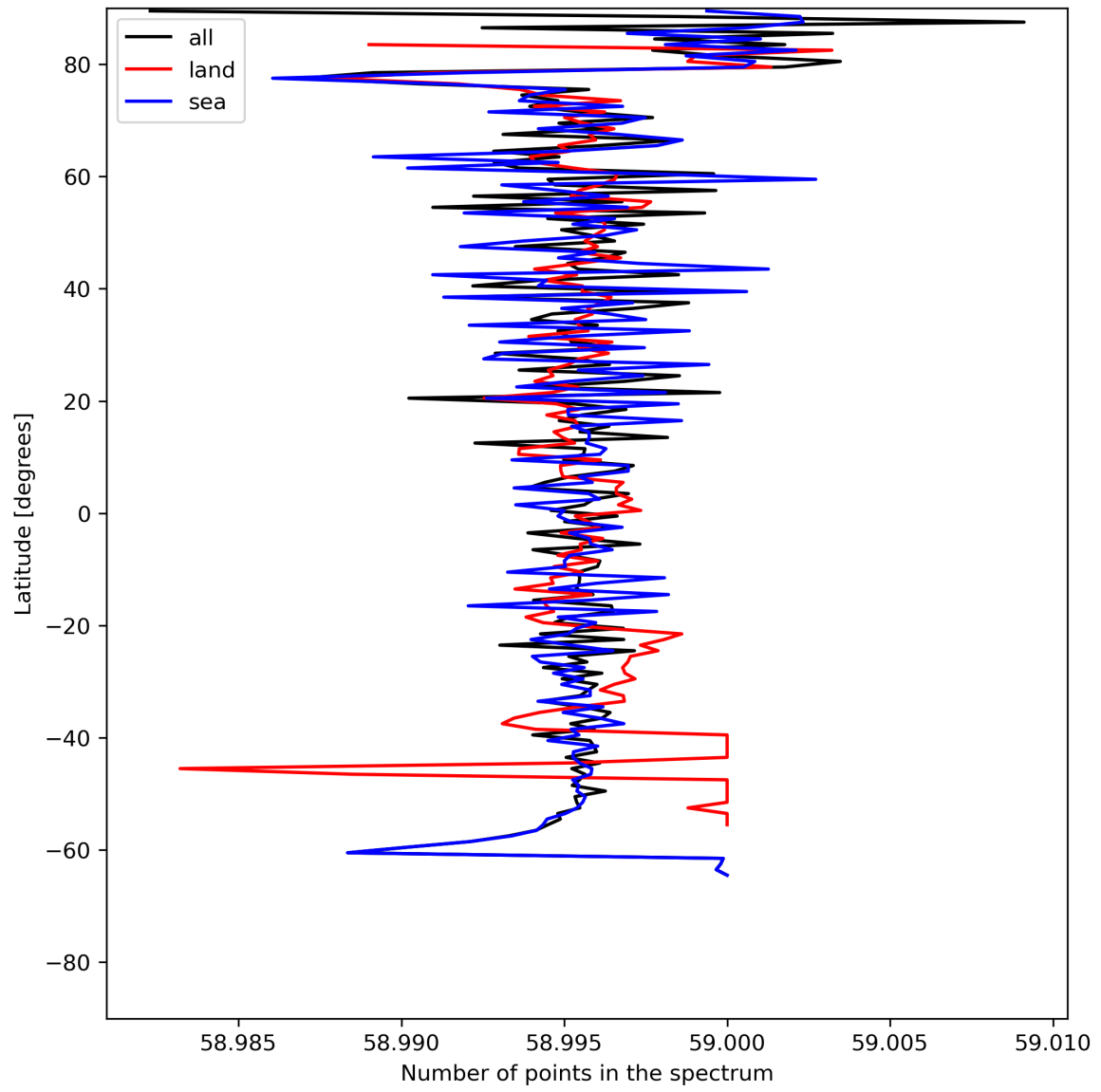
Figure 27: Zonal average of “Number of points in the spectrum” for 2024-06-16 to 2024-06-18.
