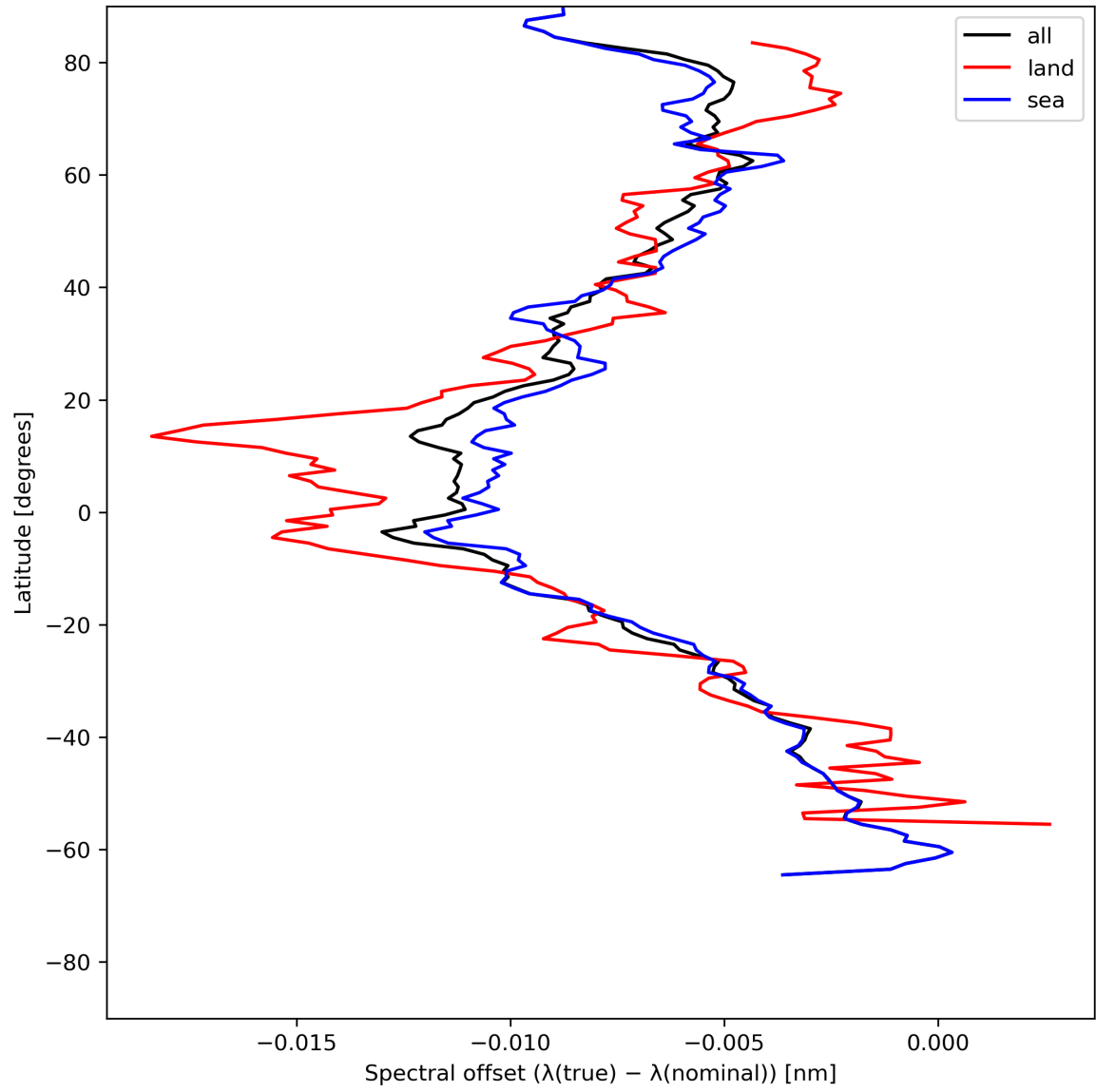
Figure 28: Zonal average of “Spectral offset ( \lambda(\text{true}) - \lambda(\text{nominal}) )” for 2024-06-16 to 2024-06-18.
