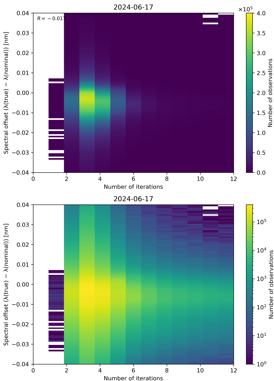
Figure 100: Scatter density plot of “Number of iterations” against “Spectral offset ( \lambda(\text{true}) - \lambda(\text{nominal}) )” for 2024-06-16 to 2024-06-18.
