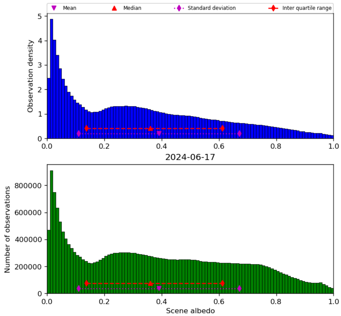
Figure 34: Histogram of “Scene albedo” for 2024-06-16 to 2024-06-18
