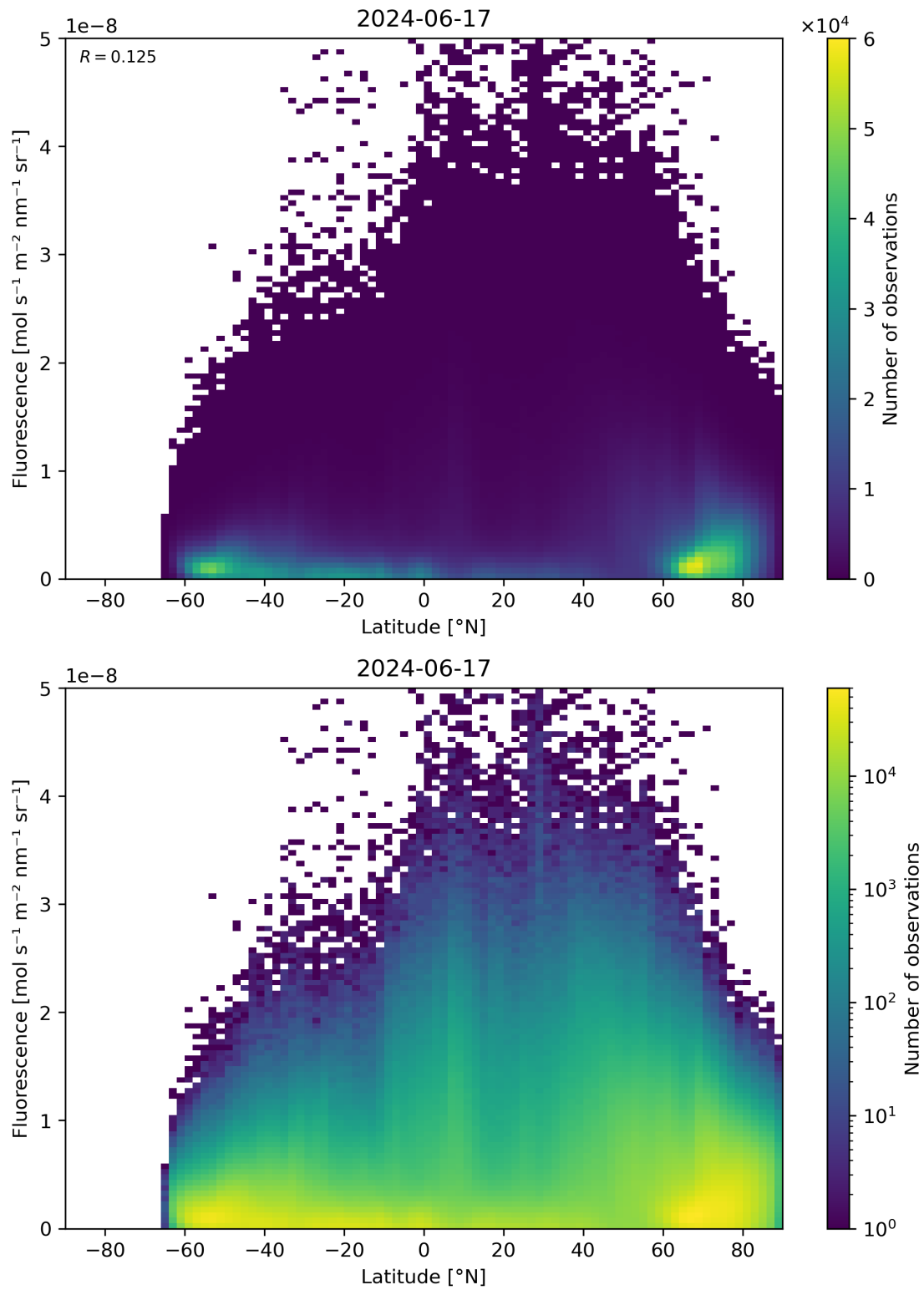
Figure 92: Scatter density plot of “Latitude” against “Fluorescence” for 2024-06-16 to 2024-06-18.
