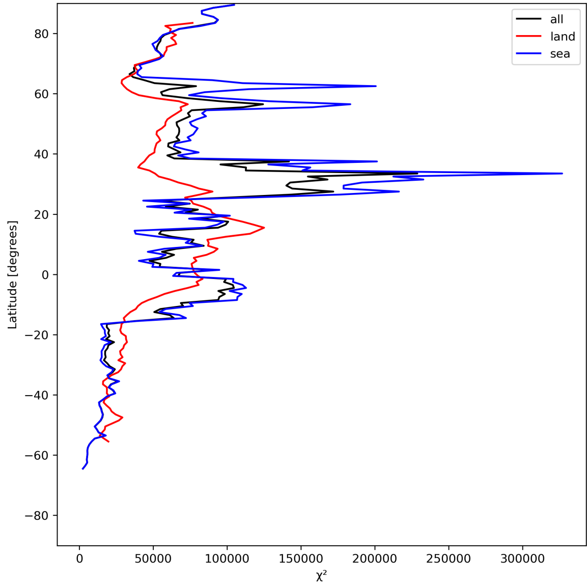
Figure 21: Zonal average of “ \chi^2 ” for 2024-06-16 to 2024-06-18.
