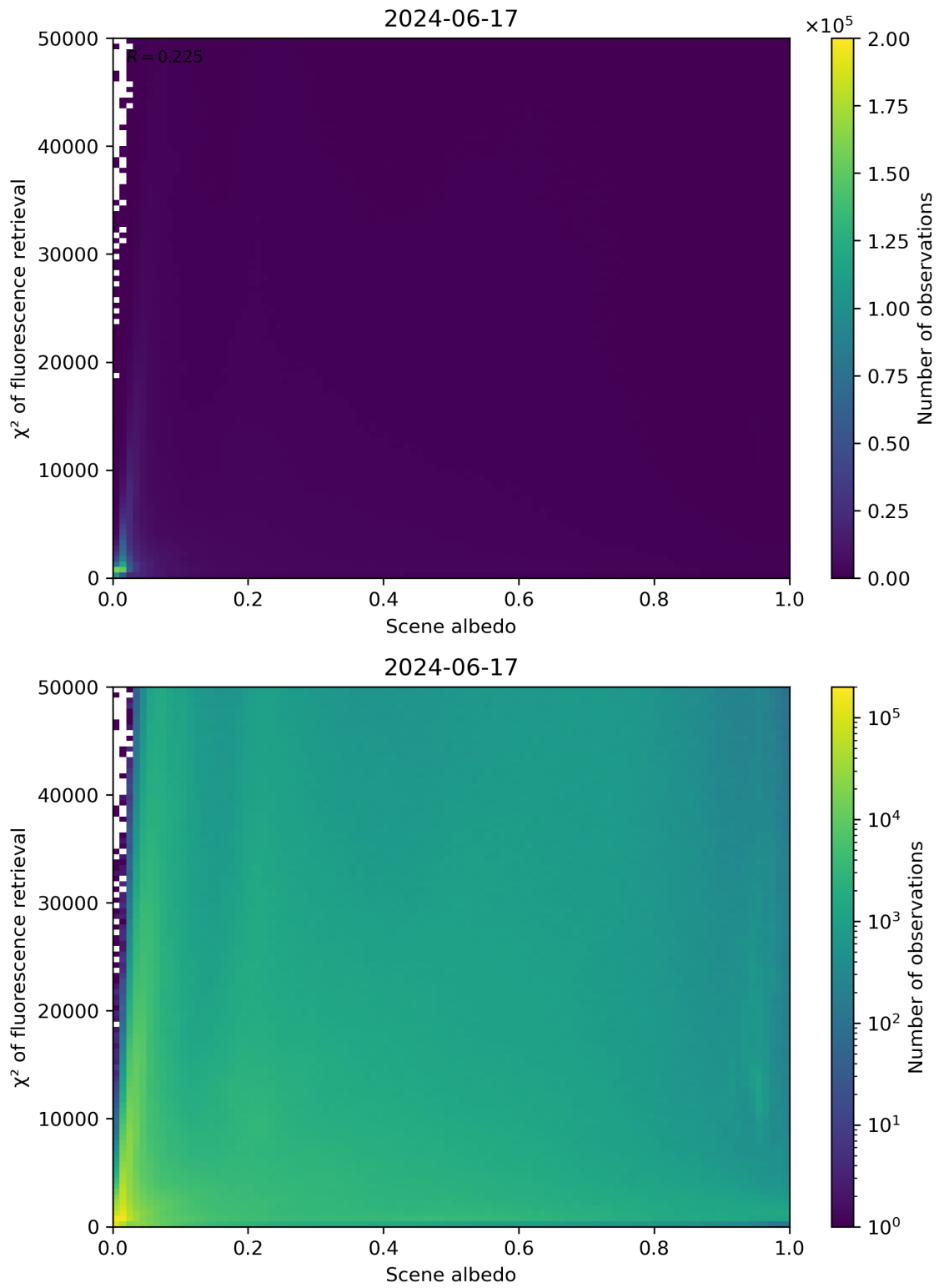
Figure 103: Scatter density plot of “Scene albedo” against “ \chi^2 of fluorescence retrieval” for 2024-06-16 to 2024-06-18.
