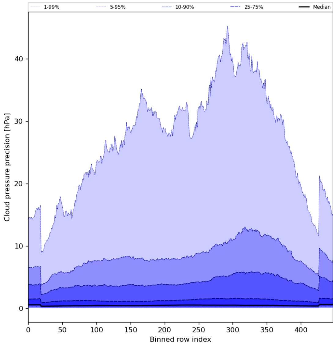
Figure 48: Along track statistics of “Cloud pressure precision” for 2024-06-16 to 2024-06-18
