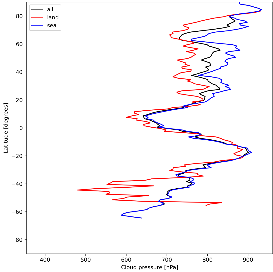
Figure 13: Zonal average of “Cloud pressure” for 2024-06-16 to 2024-06-18.
