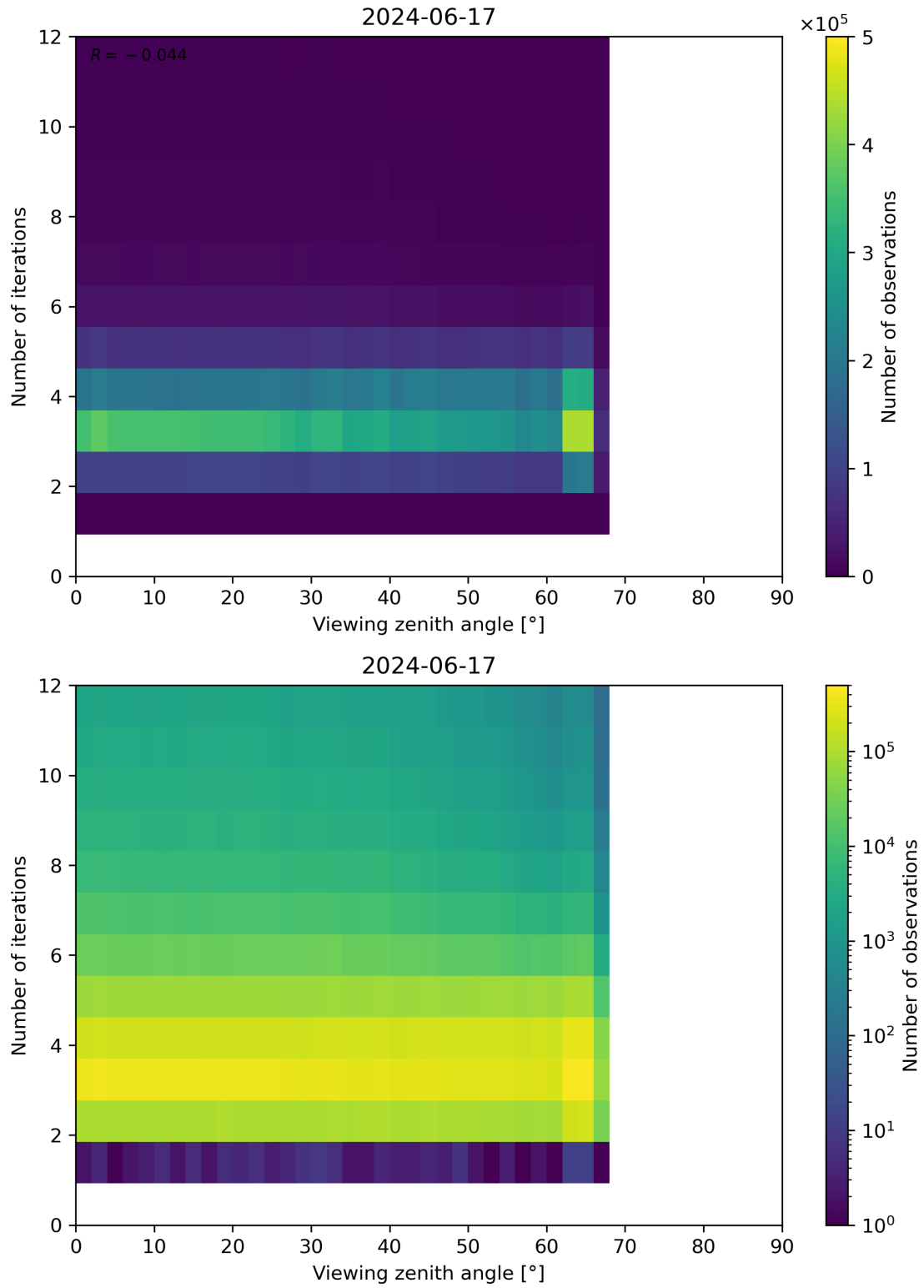
Figure 124: Scatter density plot of “Viewing zenith angle” against “Number of iterations” for 2024-06-16 to 2024-06-18.
