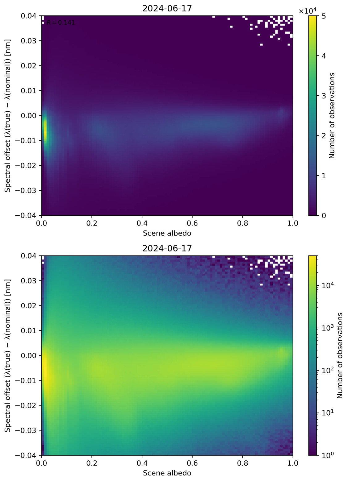
Figure 107: Scatter density plot of “Scene albedo” against “Spectral offset ( \lambda(\text{true}) - \lambda(\text{nominal}) )” for 2024-06-16 to 2024-06-18.
