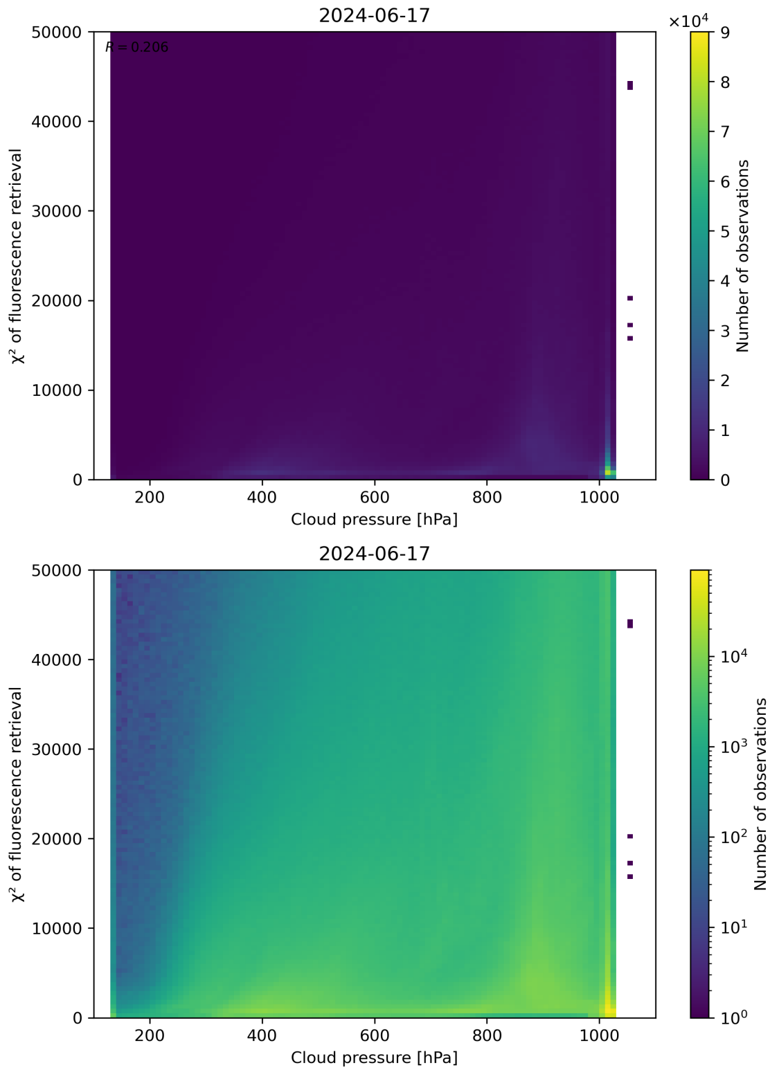
Figure 78: Scatter density plot of “Cloud pressure” against “ \chi^2 of fluorescence retrieval” for 2024-06-16 to 2024-06-18.
