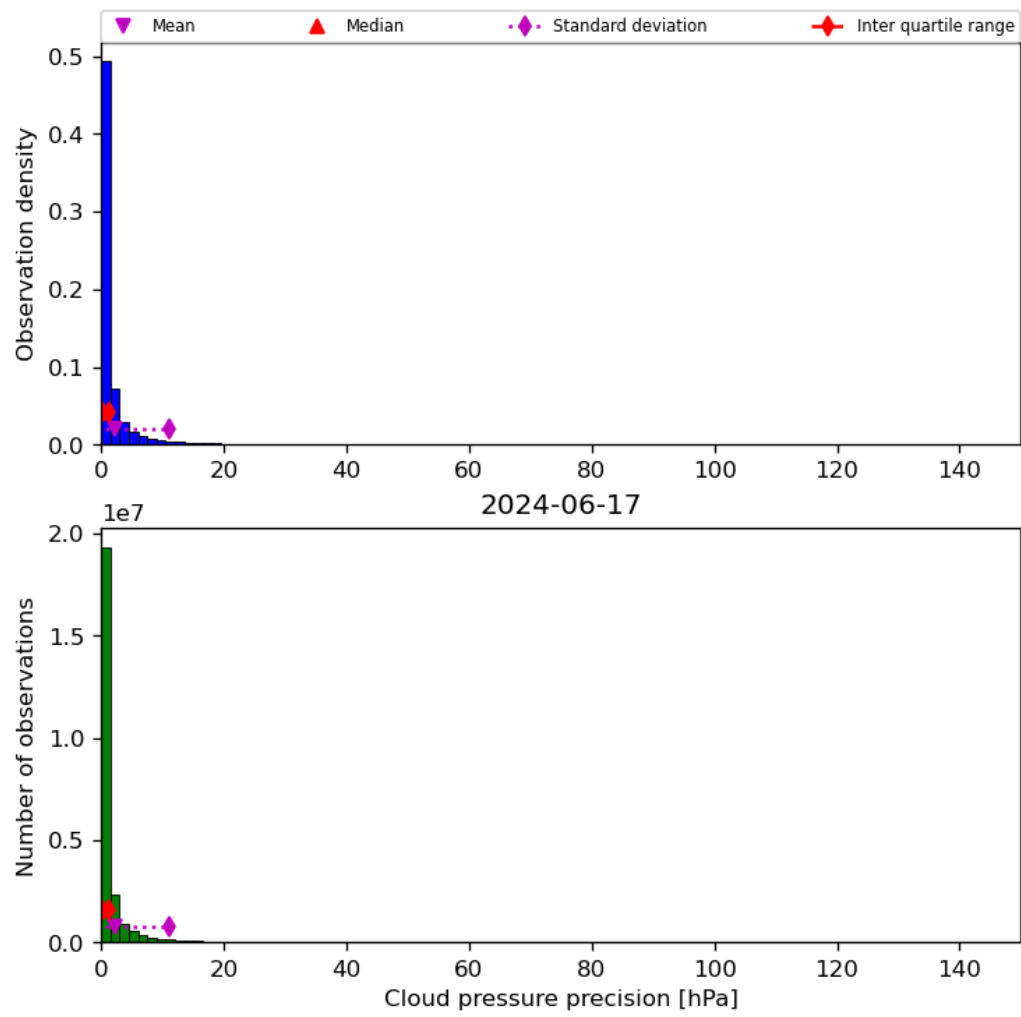
Figure 31: Histogram of “Cloud pressure precision” for 2024-06-16 to 2024-06-18
