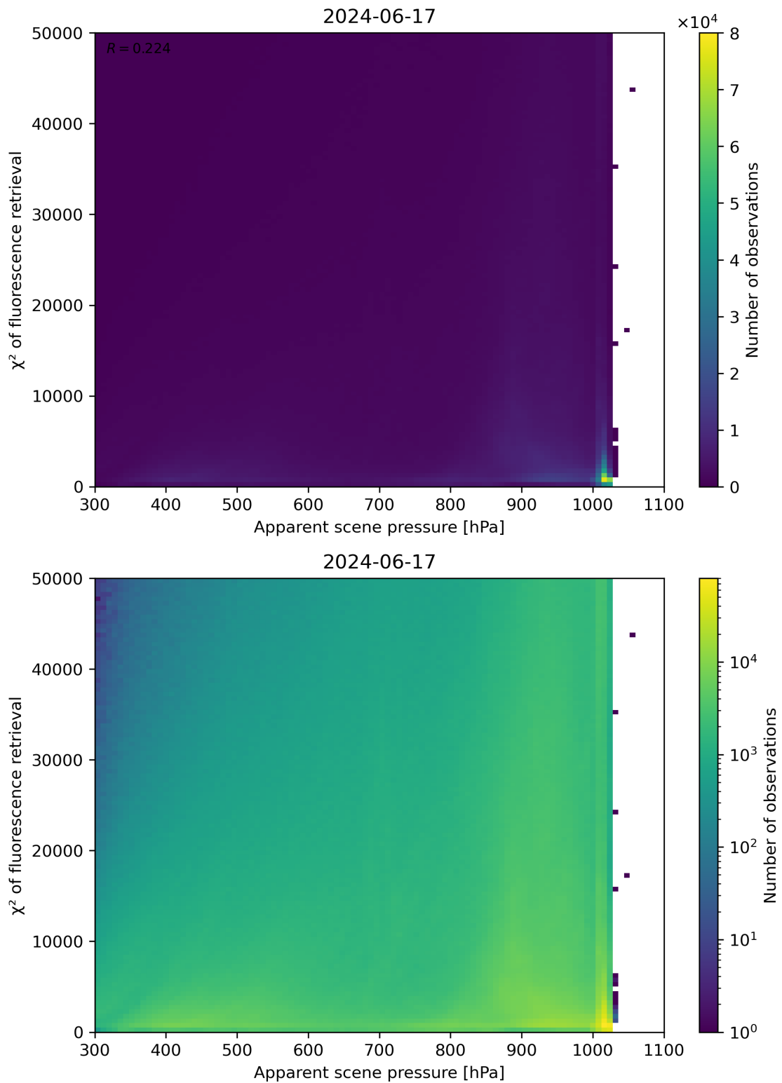
Figure 63: Scatter density plot of “Apparent scene pressure” against “ \chi^2 of fluorescence retrieval” for 2024-06-16 to 2024-06-18.
