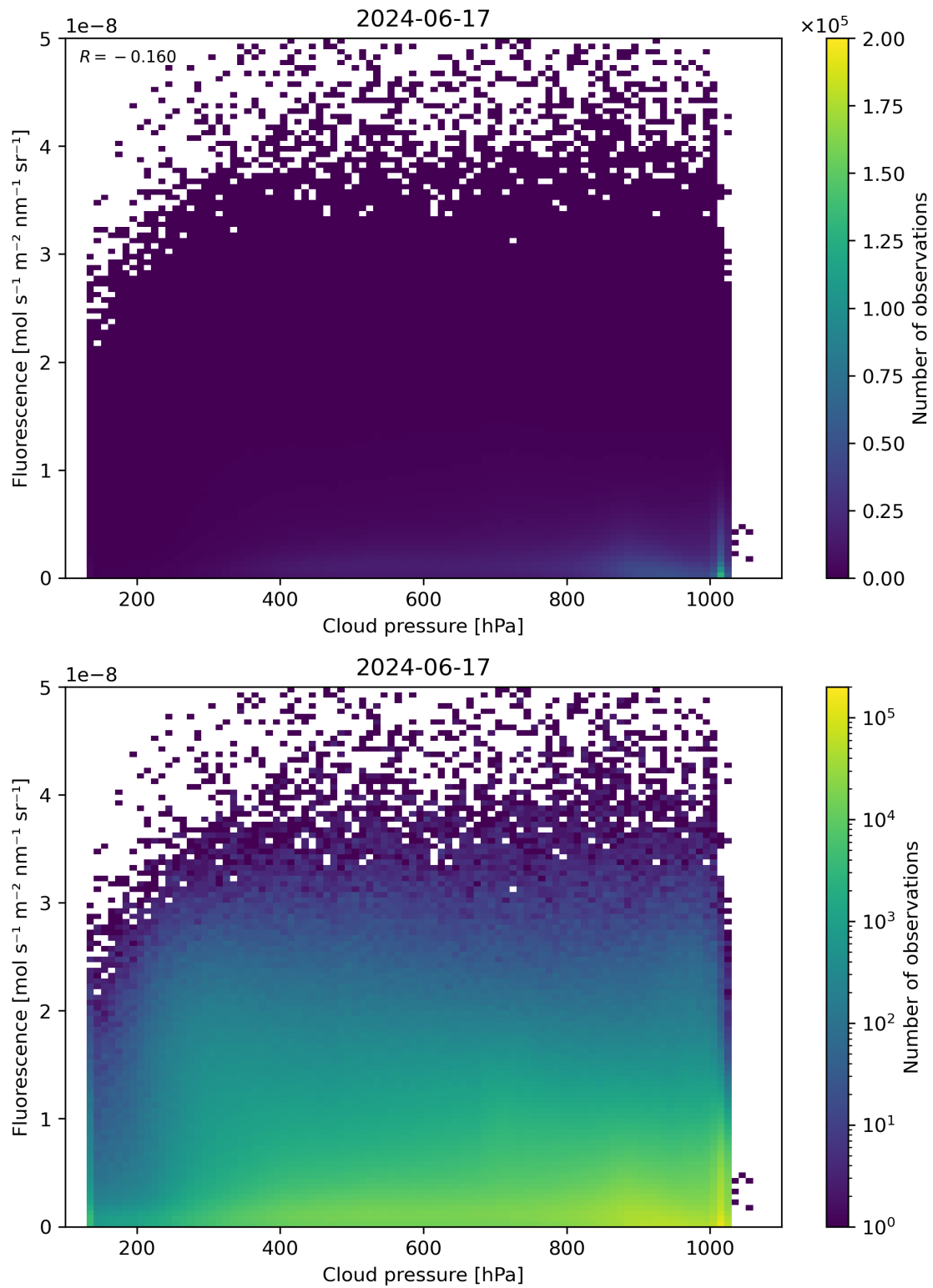
Figure 80: Scatter density plot of “Cloud pressure” against “Fluorescence” for 2024-06-16 to 2024-06-18.
