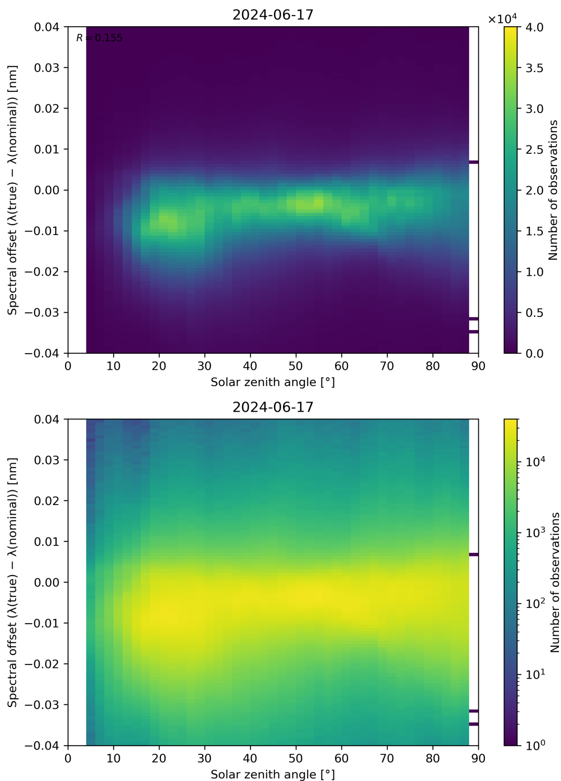
Figure 117: Scatter density plot of “Solar zenith angle” against “Spectral offset ( \lambda(\text{true}) - \lambda(\text{nominal}) )” for 2024-06-16 to 2024-06-18.
