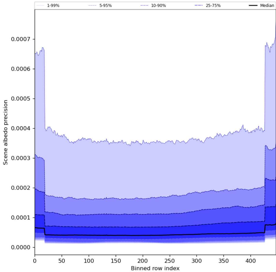
Figure 52: Along track statistics of “Scene albedo precision” for 2024-06-16 to 2024-06-18
