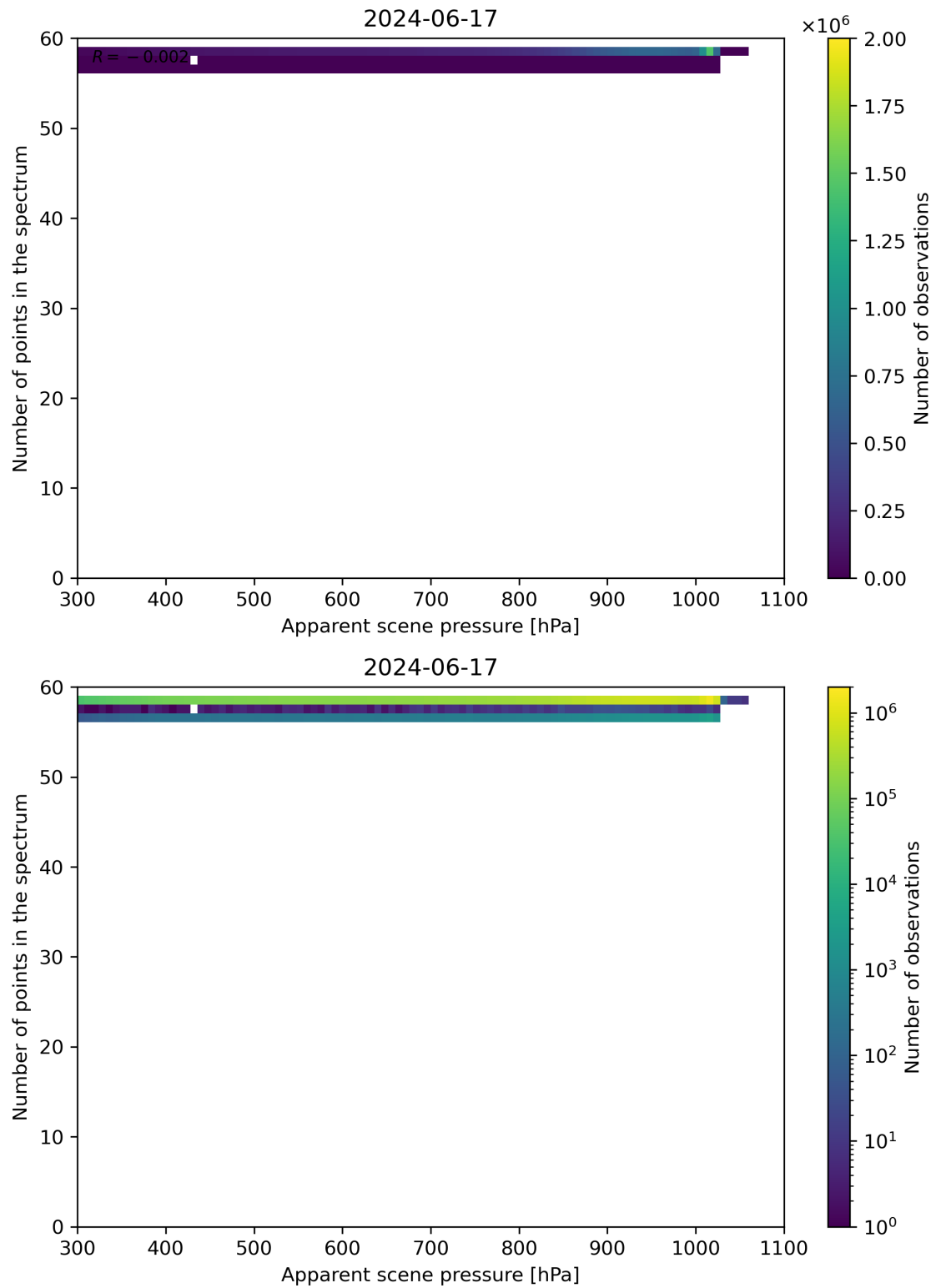
Figure 66: Scatter density plot of “Apparent scene pressure” against “Number of points in the spectrum” for 2024-06-16 to 2024-06-18.
