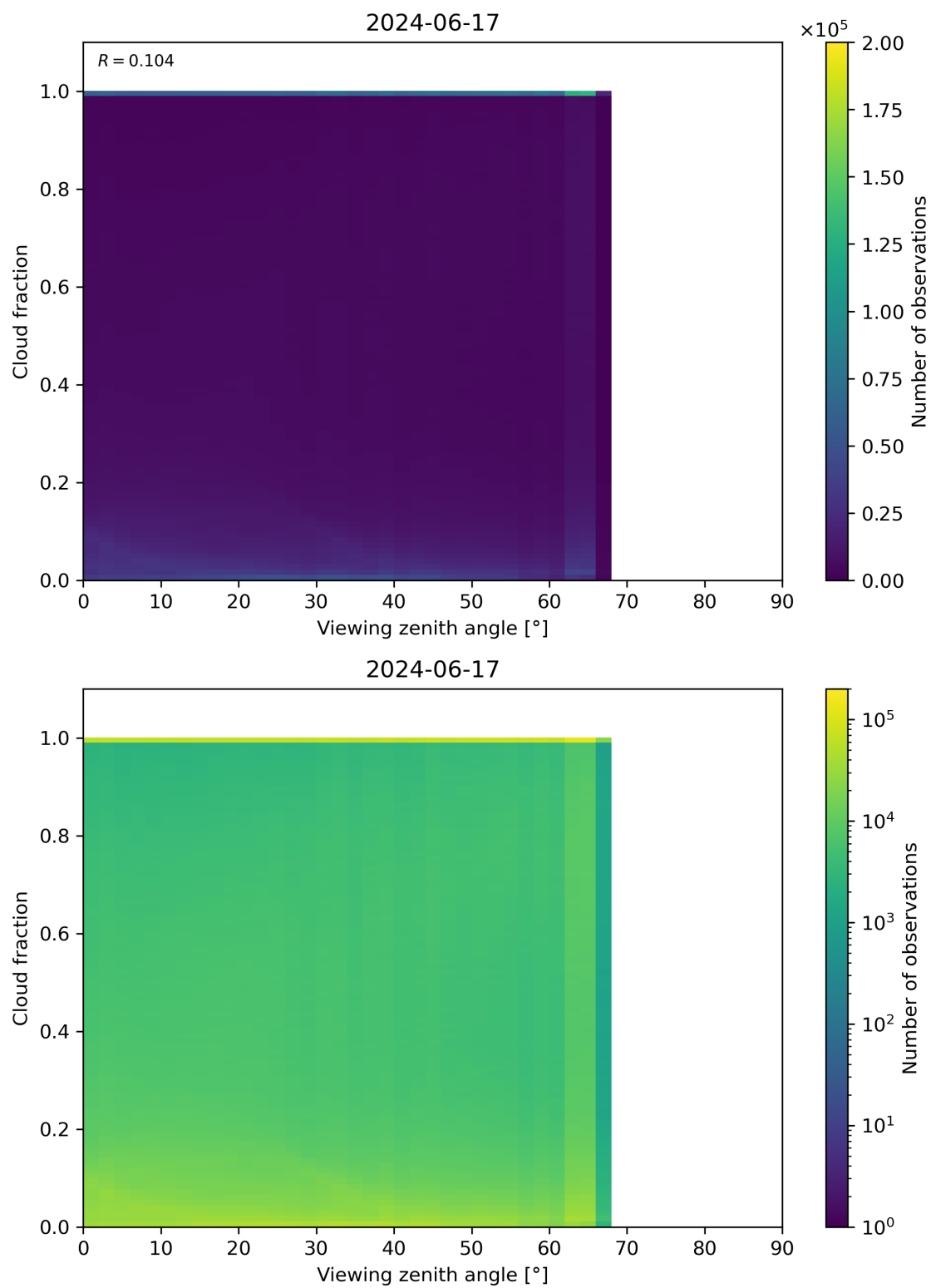
Figure 120: Scatter density plot of “Viewing zenith angle” against “Cloud fraction” for 2024-06-16 to 2024-06-18.
