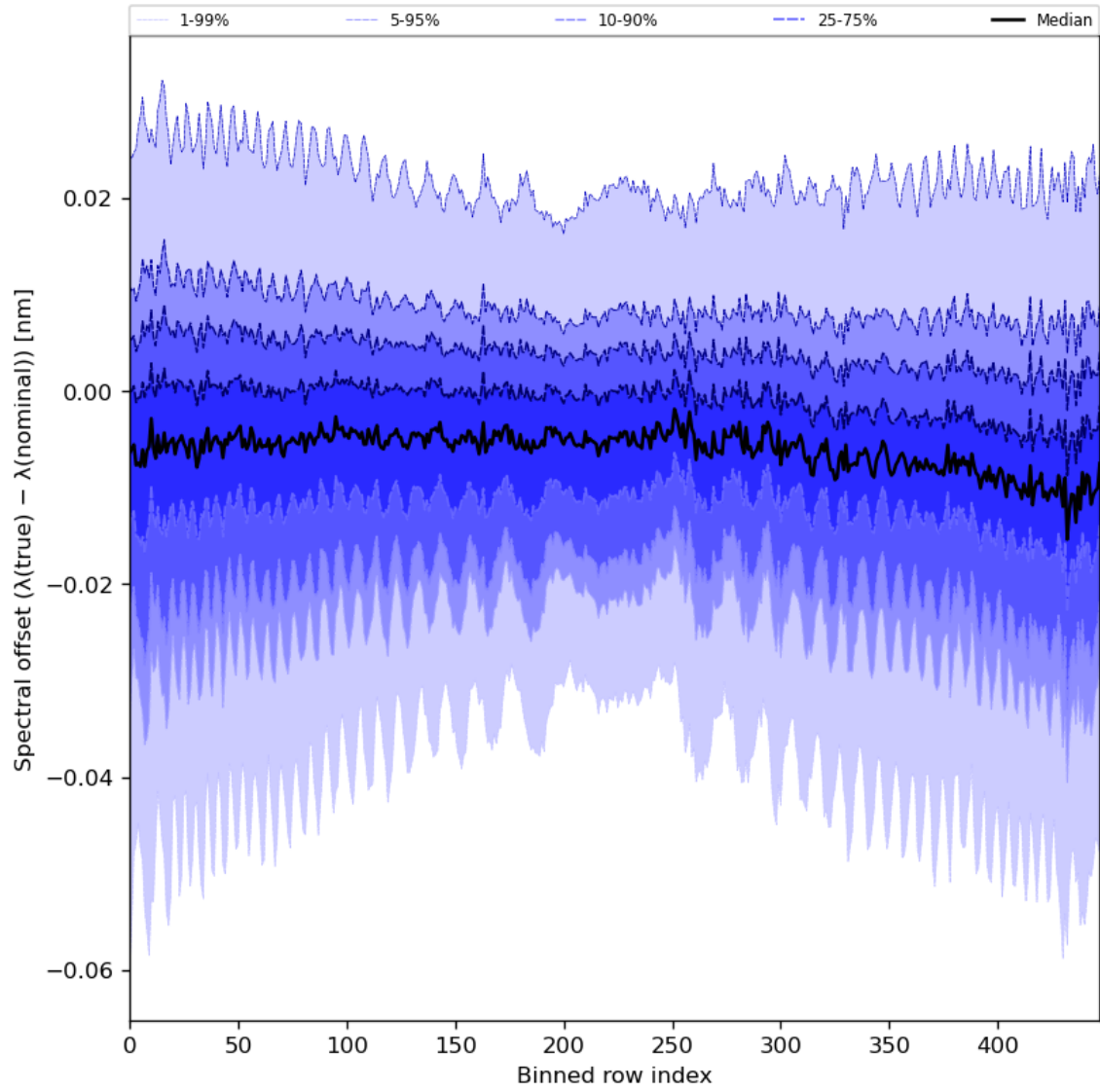
Figure 62: Along track statistics of “Spectral offset ( \lambda(\text{true}) - \lambda(\text{nominal}) )” for 2024-06-17 to 2024-06-19
