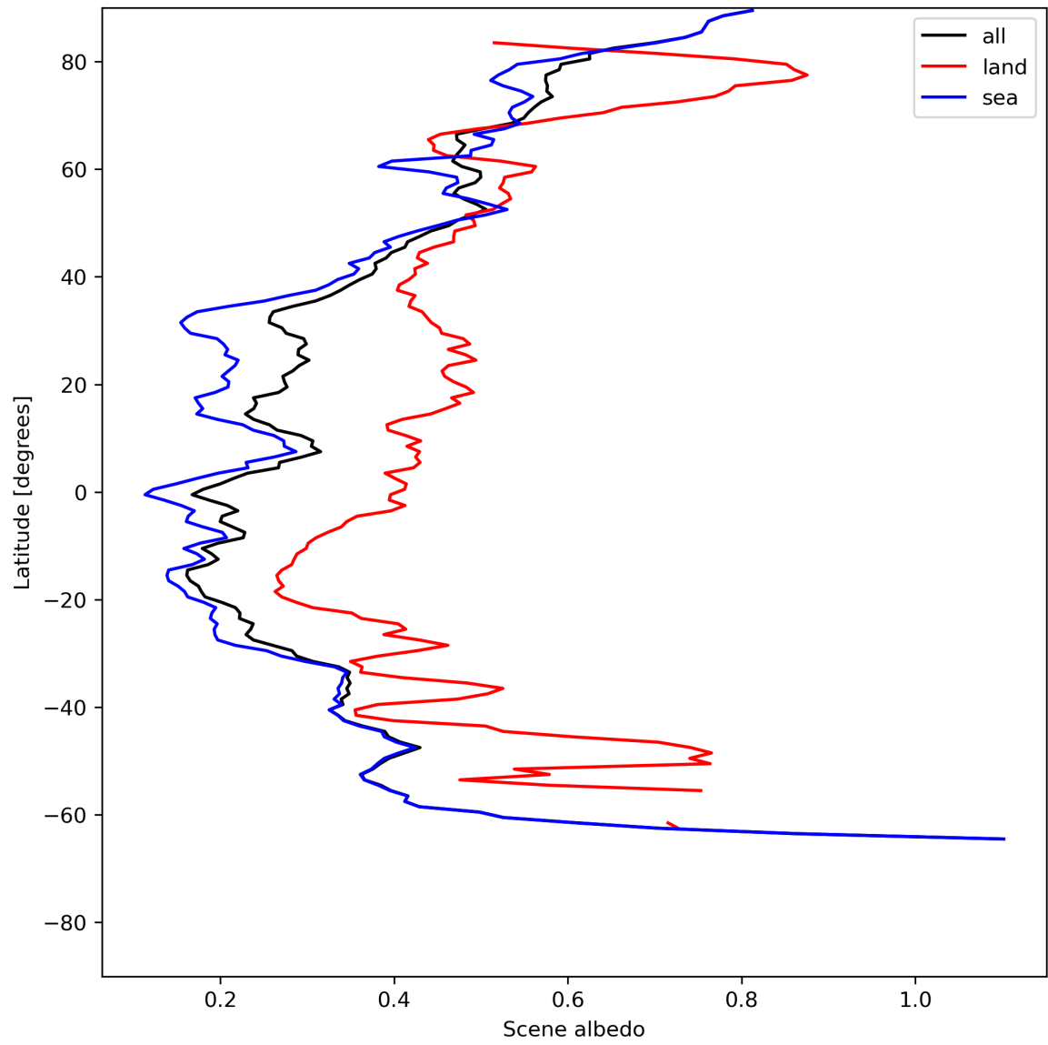
Figure 17: Zonal average of “Scene albedo” for 2024-06-17 to 2024-06-19.
