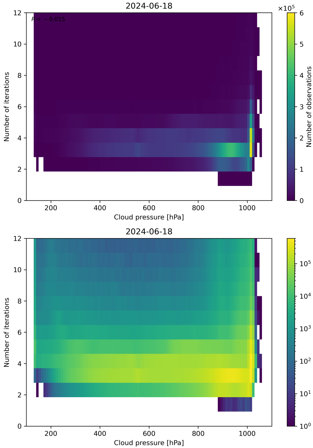
Figure 81: Scatter density plot of “Cloud pressure” against “Number of iterations” for 2024-06-17 to 2024-06-19.
