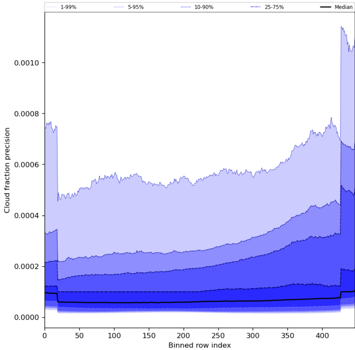
Figure 50: Along track statistics of “Cloud fraction precision” for 2024-06-17 to 2024-06-19
