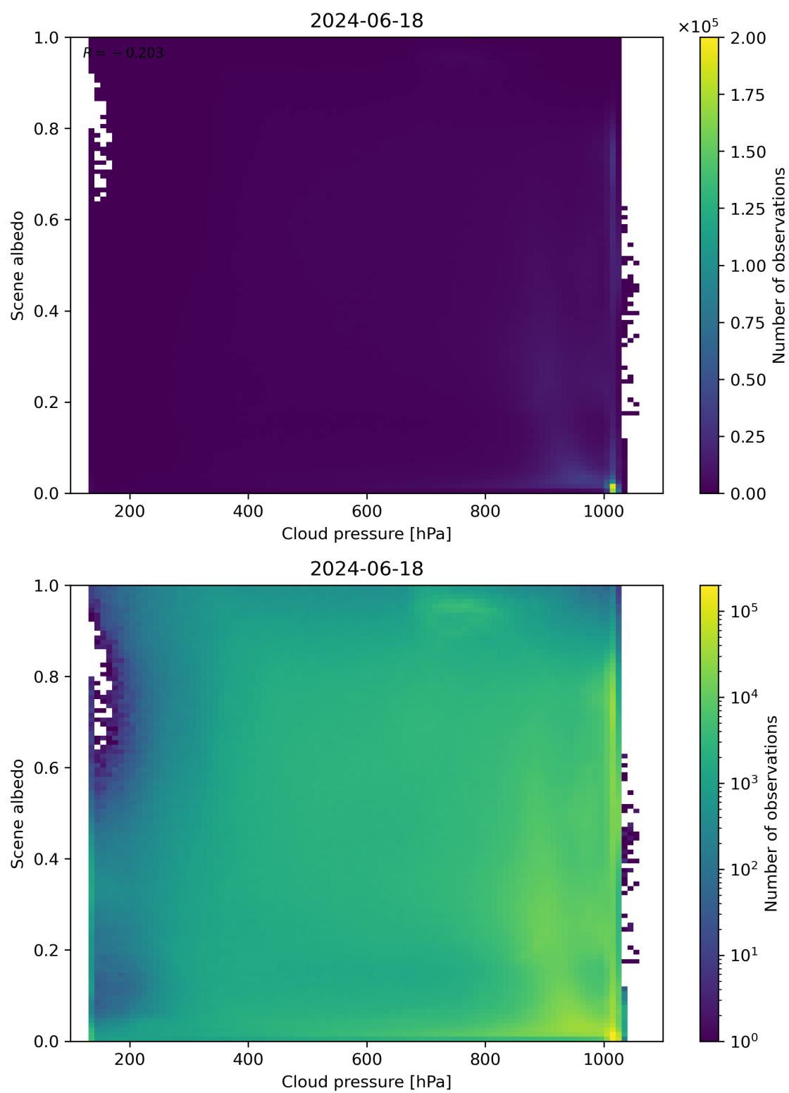
Figure 83: Scatter density plot of “Cloud pressure” against “Scene albedo” for 2024-06-17 to 2024-06-19.
