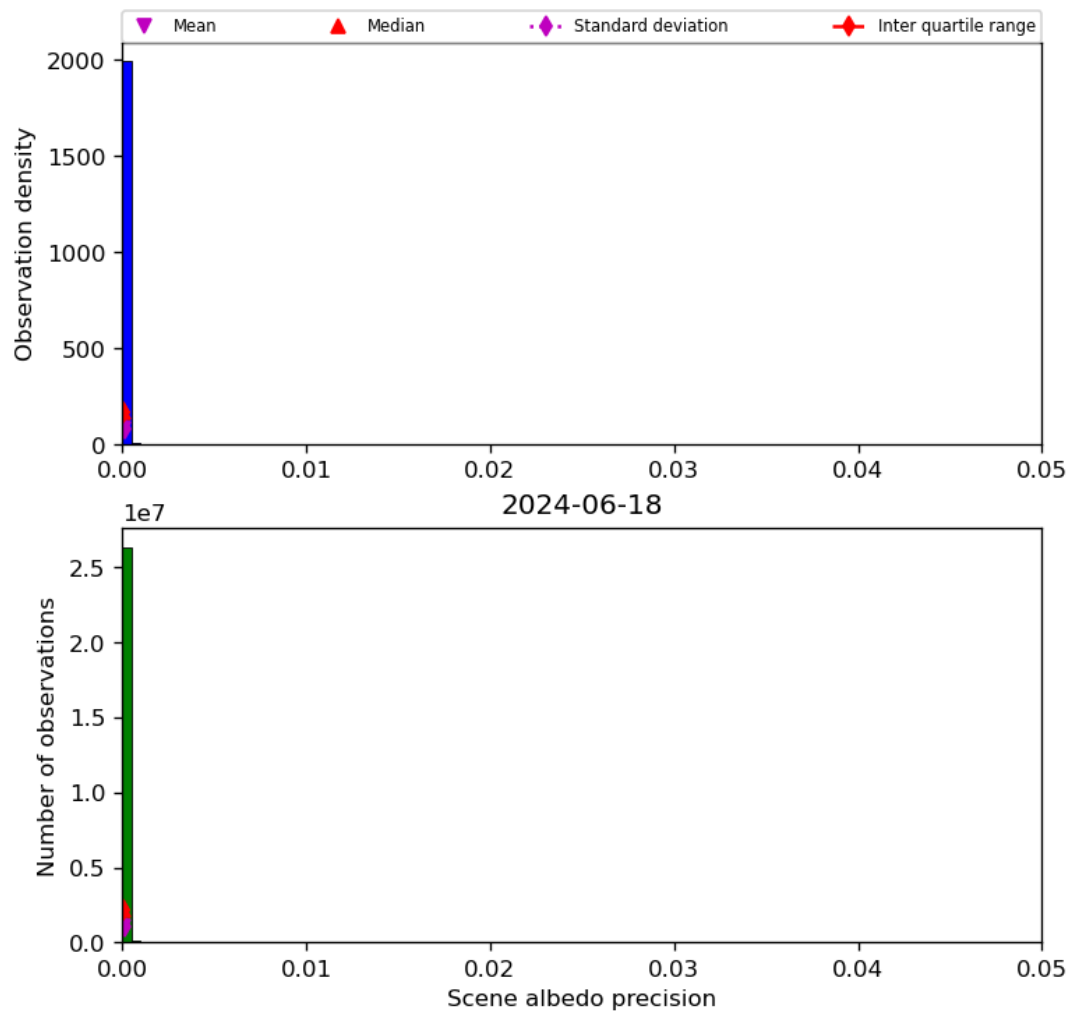
Figure 35: Histogram of “Scene albedo precision” for 2024-06-17 to 2024-06-19
