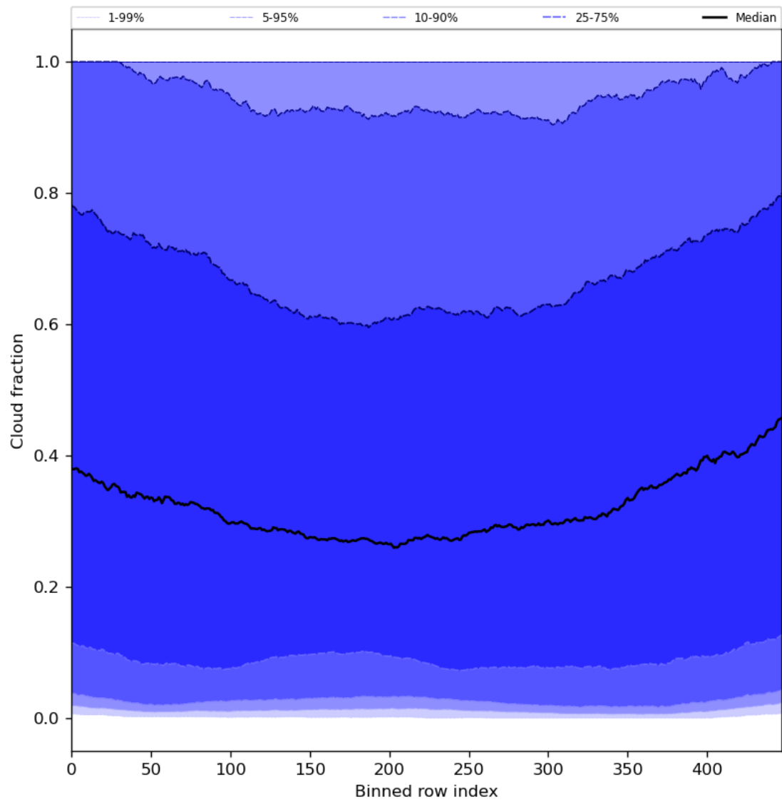
Figure 49: Along track statistics of “Cloud fraction” for 2024-06-17 to 2024-06-19
