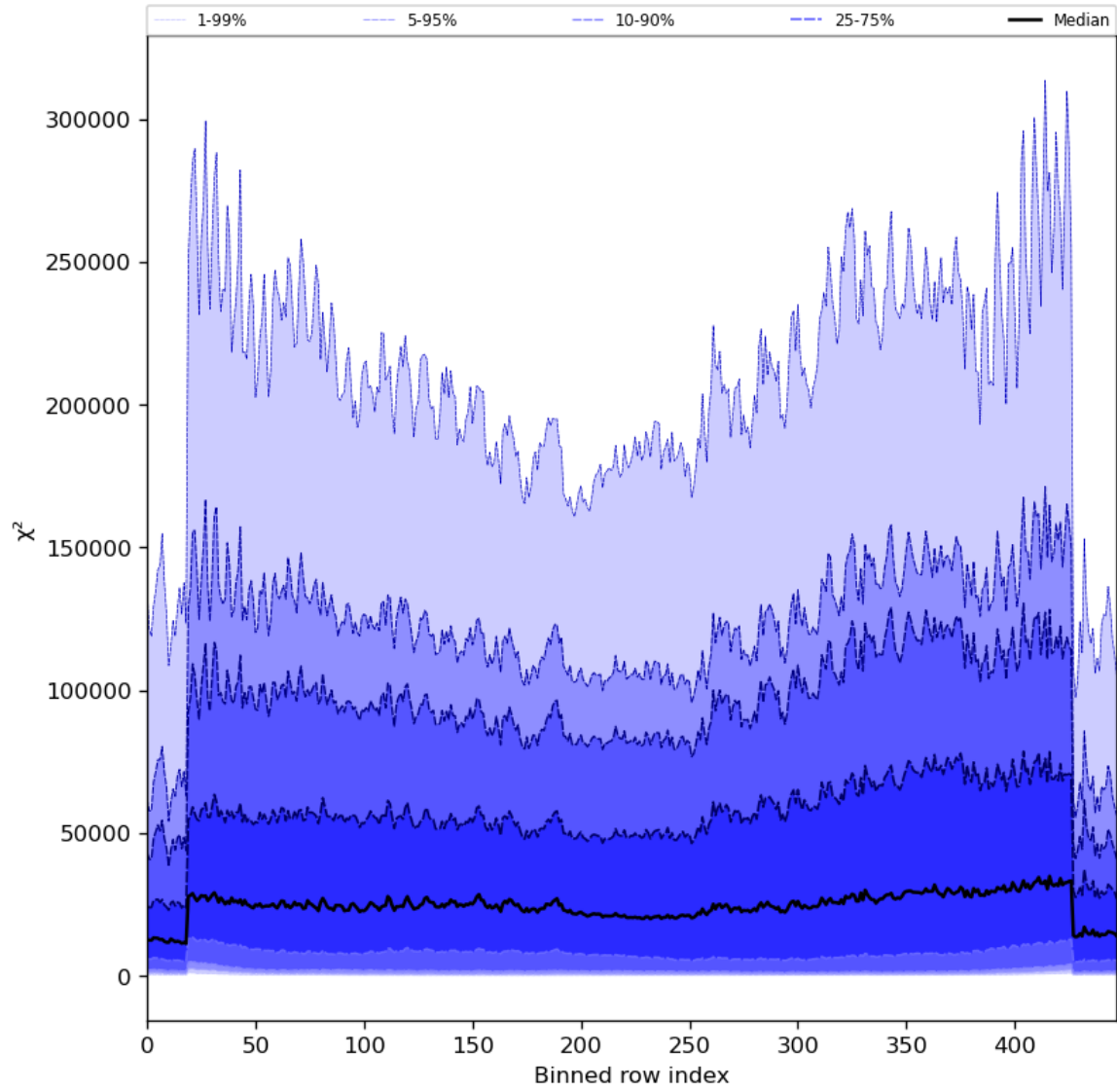
Figure 55: Along track statistics of “ \chi^2 ” for 2024-06-17 to 2024-06-19
