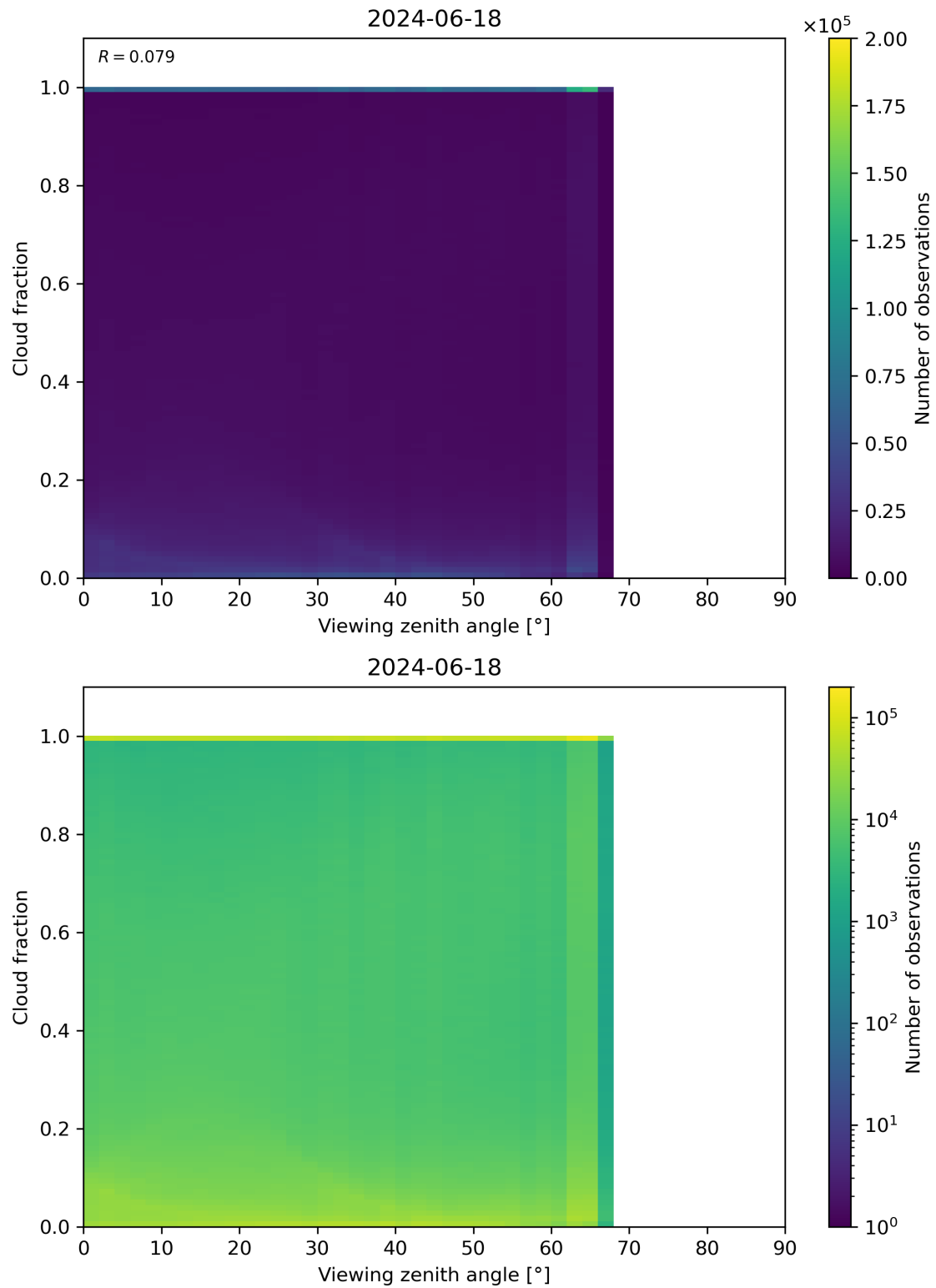
Figure 120: Scatter density plot of “Viewing zenith angle” against “Cloud fraction” for 2024-06-17 to 2024-06-19.
