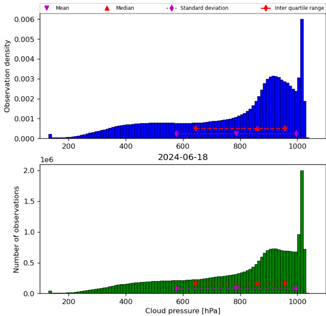
Figure 30: Histogram of “Cloud pressure” for 2024-06-17 to 2024-06-19
