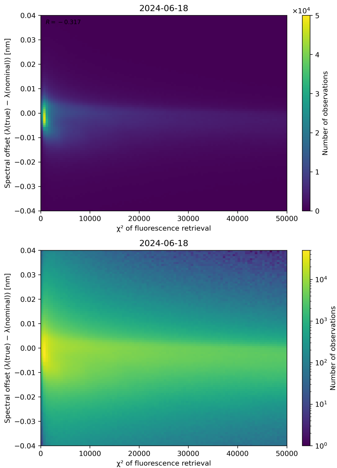
Figure 69: Scatter density plot of “ \chi^2 of fluorescence retrieval” against “Spectral offset ( \lambda(\text{true}) - \lambda(\text{nominal}) )” for 2024-06-17 to 2024-06-19.
