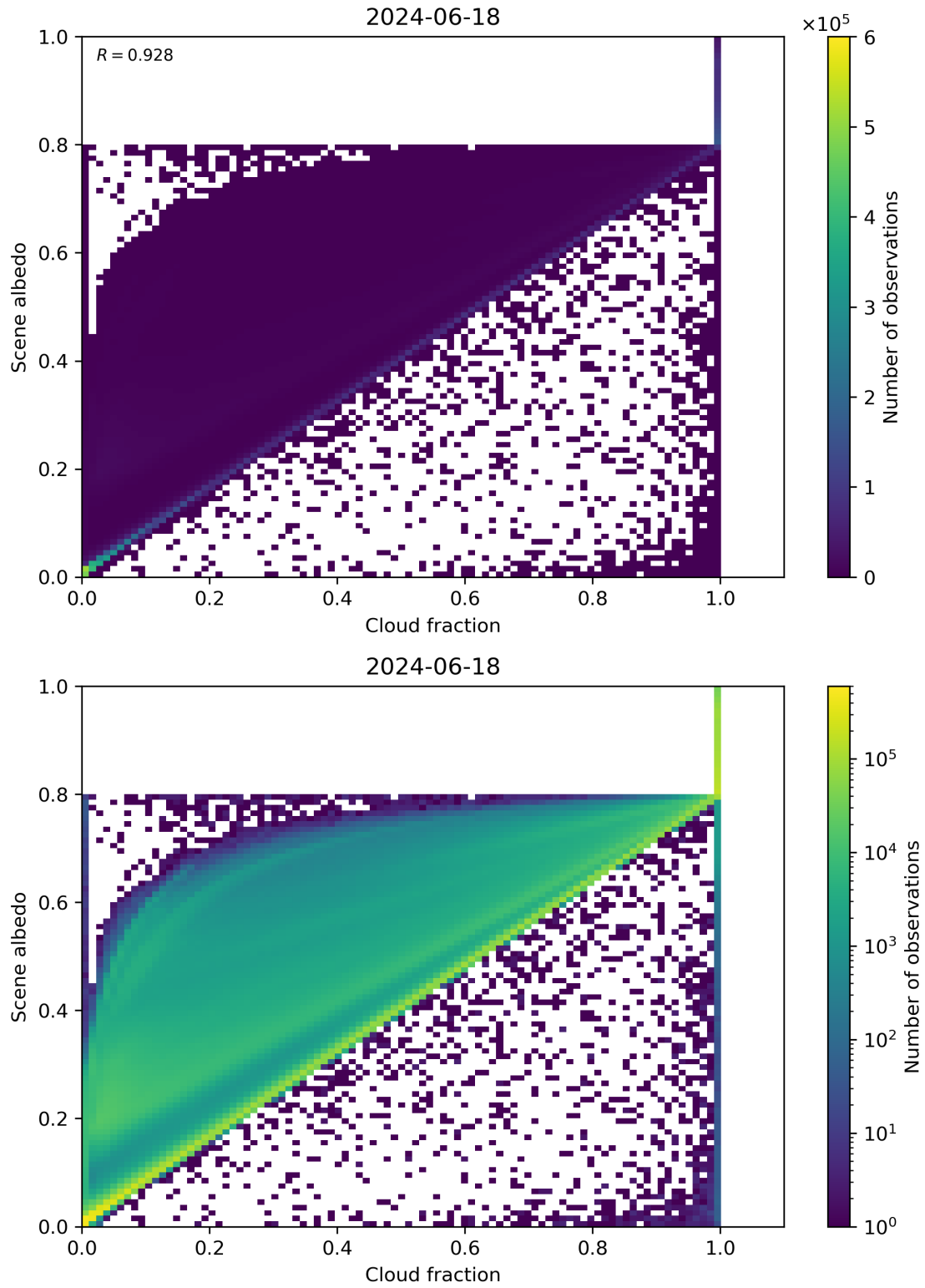
Figure 75: Scatter density plot of “Cloud fraction” against “Scene albedo” for 2024-06-17 to 2024-06-19.
