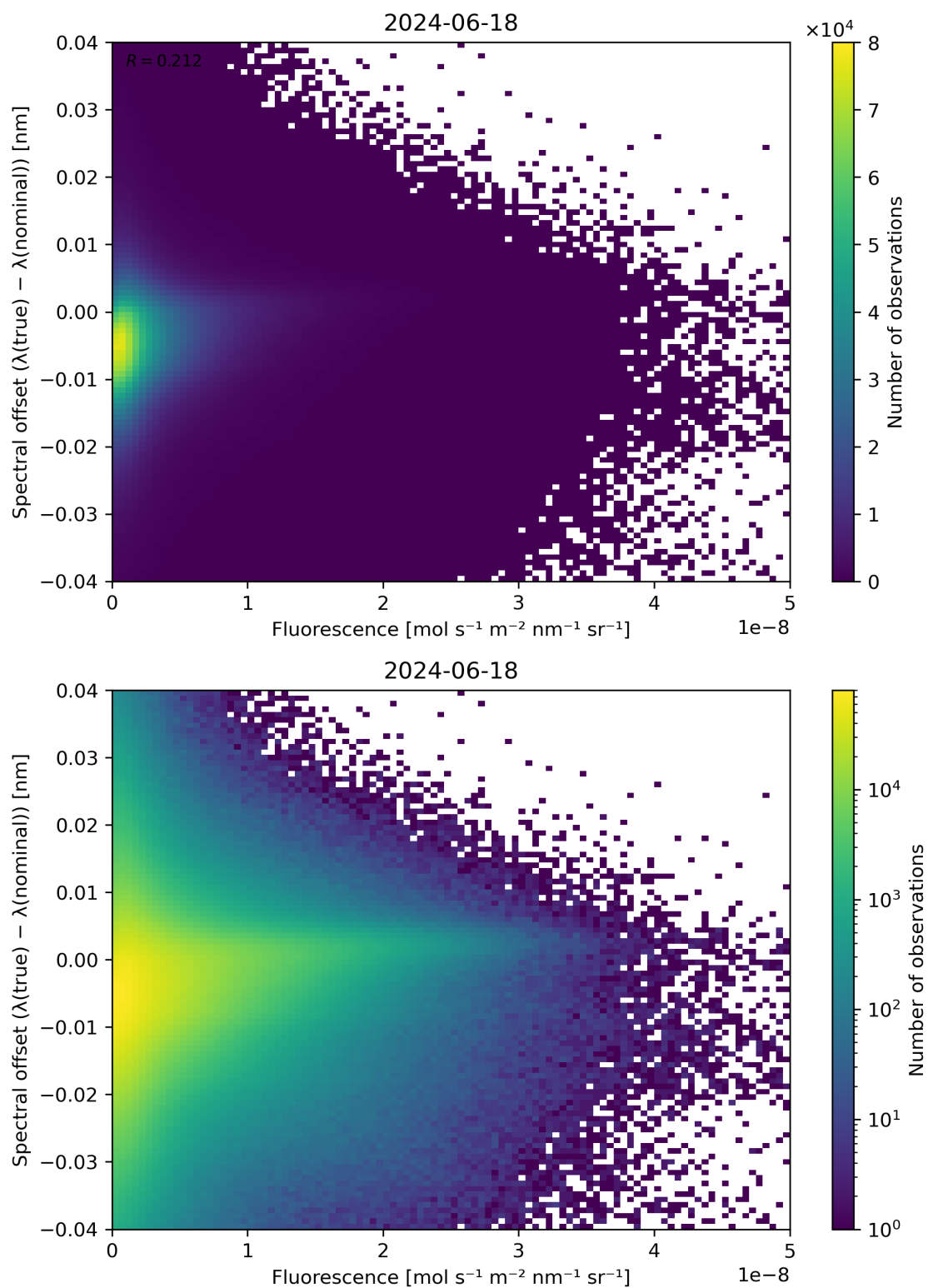
Figure 87: Scatter density plot of “Fluorescence” against “Spectral offset ( \lambda(\text{true}) - \lambda(\text{nominal}) )” for 2024-06-17 to 2024-06-19.
