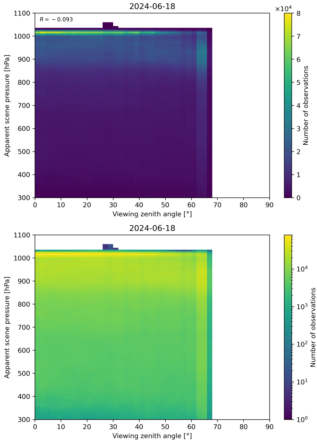
Figure 118: Scatter density plot of “Viewing zenith angle” against “Apparent scene pressure” for 2024-06-17 to 2024-06-19.
