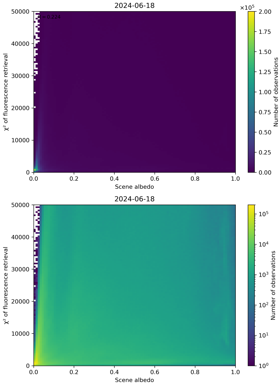
Figure 103: Scatter density plot of “Scene albedo” against “ \chi^2 of fluorescence retrieval” for 2024-06-17 to 2024-06-19.
