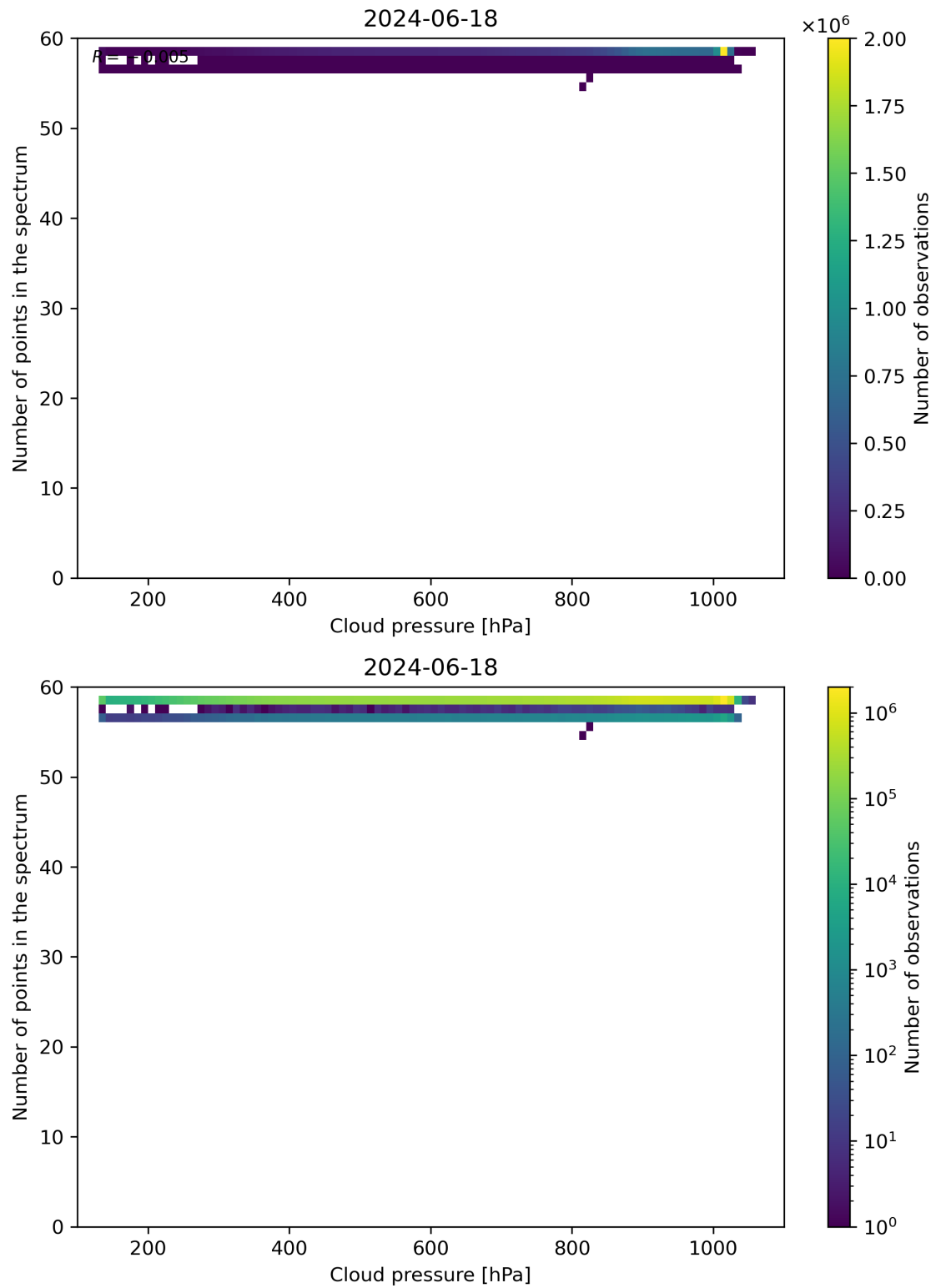
Figure 82: Scatter density plot of “Cloud pressure” against “Number of points in the spectrum” for 2024-06-17 to 2024-06-19.
