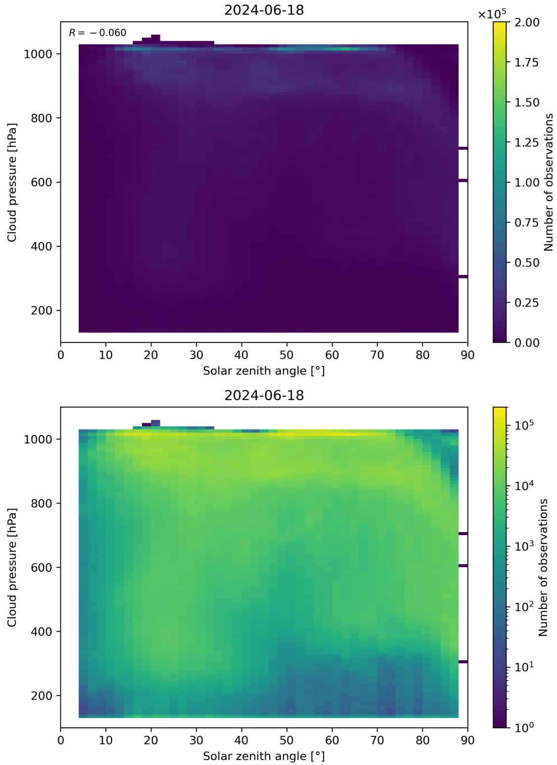
Figure 111: Scatter density plot of “Solar zenith angle” against “Cloud pressure” for 2024-06-17 to 2024-06-19.
