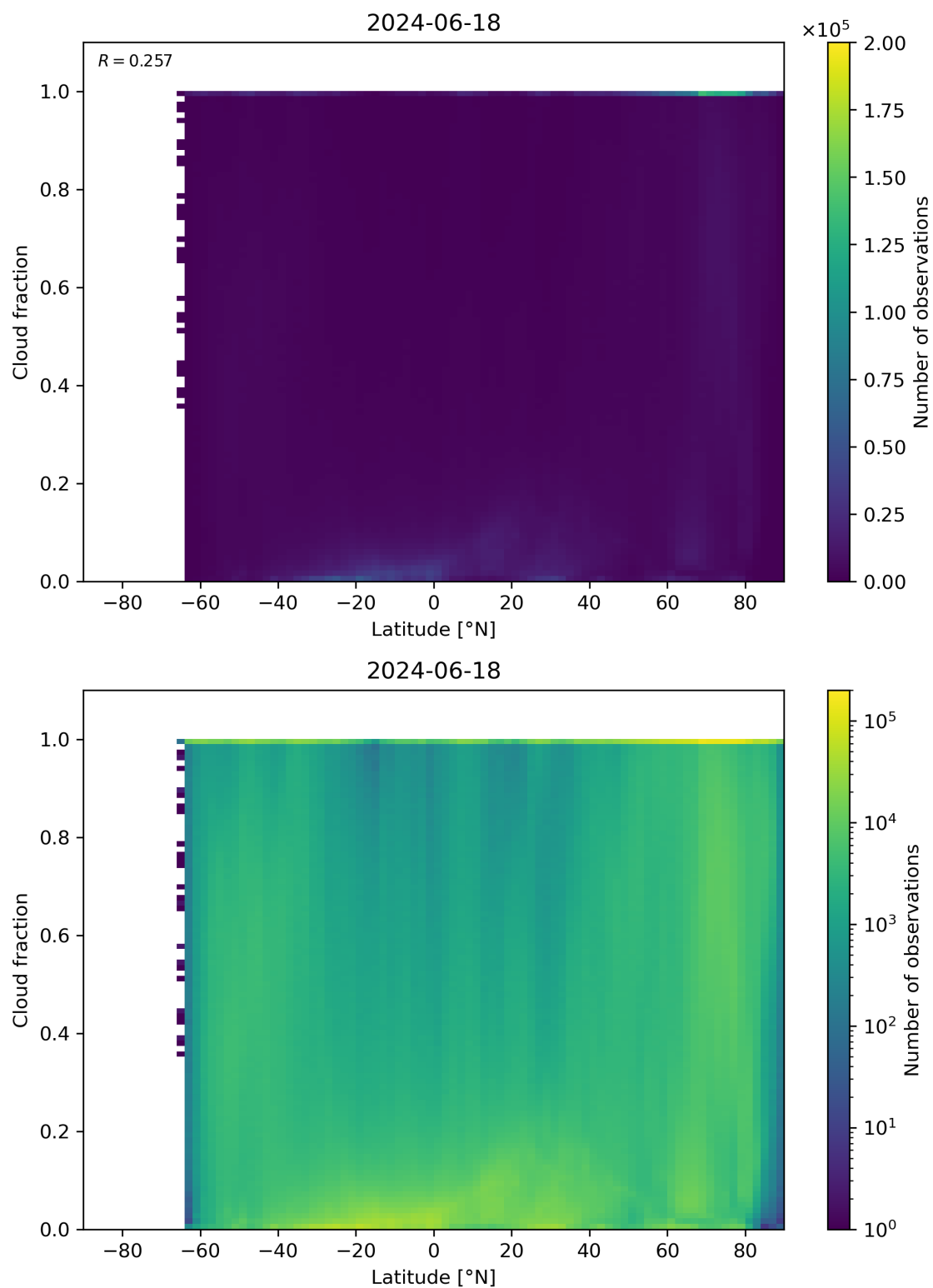
Figure 90: Scatter density plot of “Latitude” against “Cloud fraction” for 2024-06-17 to 2024-06-19.
