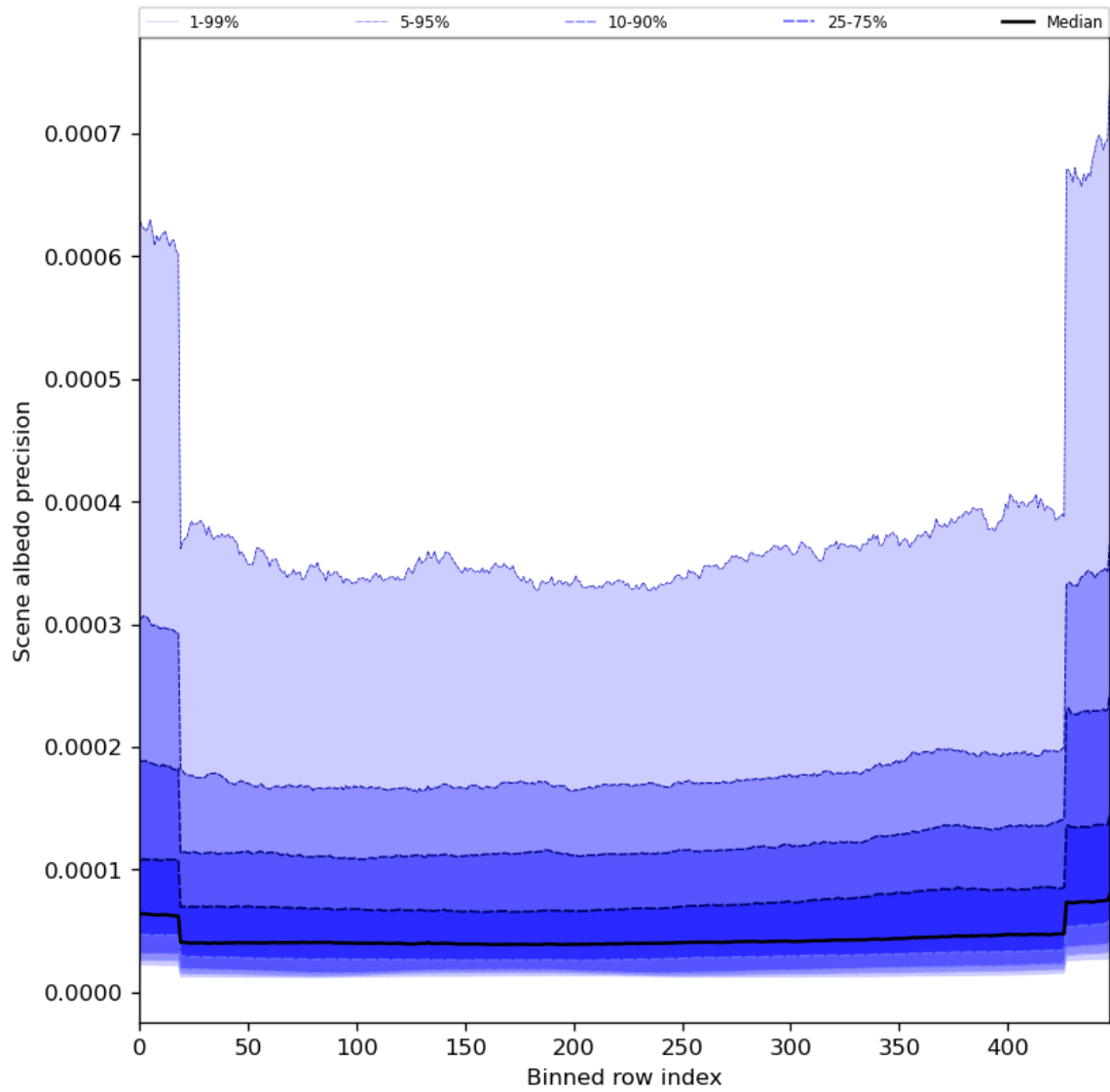
Figure 52: Along track statistics of “Scene albedo precision” for 2024-06-17 to 2024-06-19
