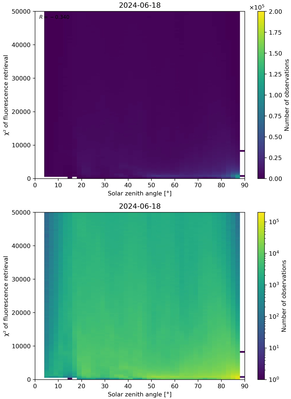
Figure 109: Scatter density plot of “Solar zenith angle” against “ \chi^2 of fluorescence retrieval” for 2024-06-17 to 2024-06-19.
