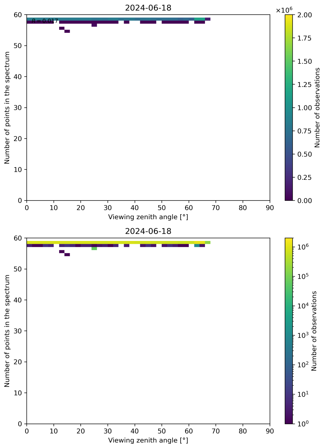
Figure 125: Scatter density plot of “Viewing zenith angle” against “Number of points in the spectrum” for 2024-06-17 to 2024-06-19.
