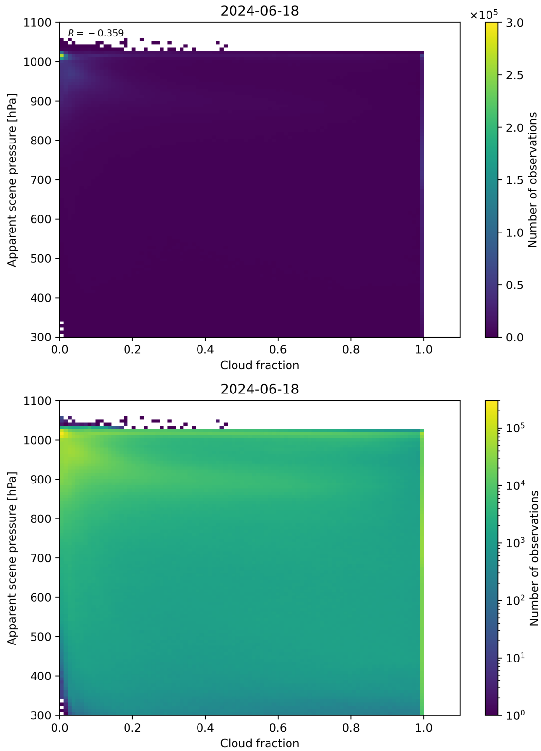
Figure 70: Scatter density plot of “Cloud fraction” against “Apparent scene pressure” for 2024-06-17 to 2024-06-19.
