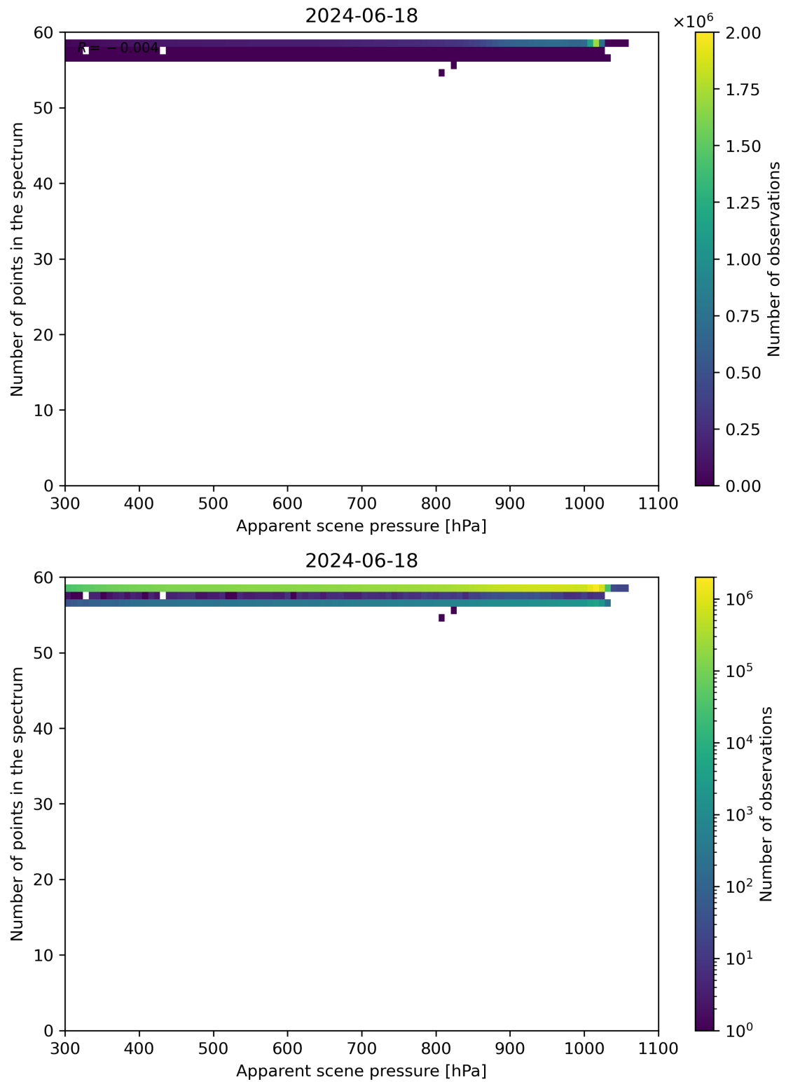
Figure 66: Scatter density plot of “Apparent scene pressure” against “Number of points in the spectrum” for 2024-06-17 to 2024-06-19.
