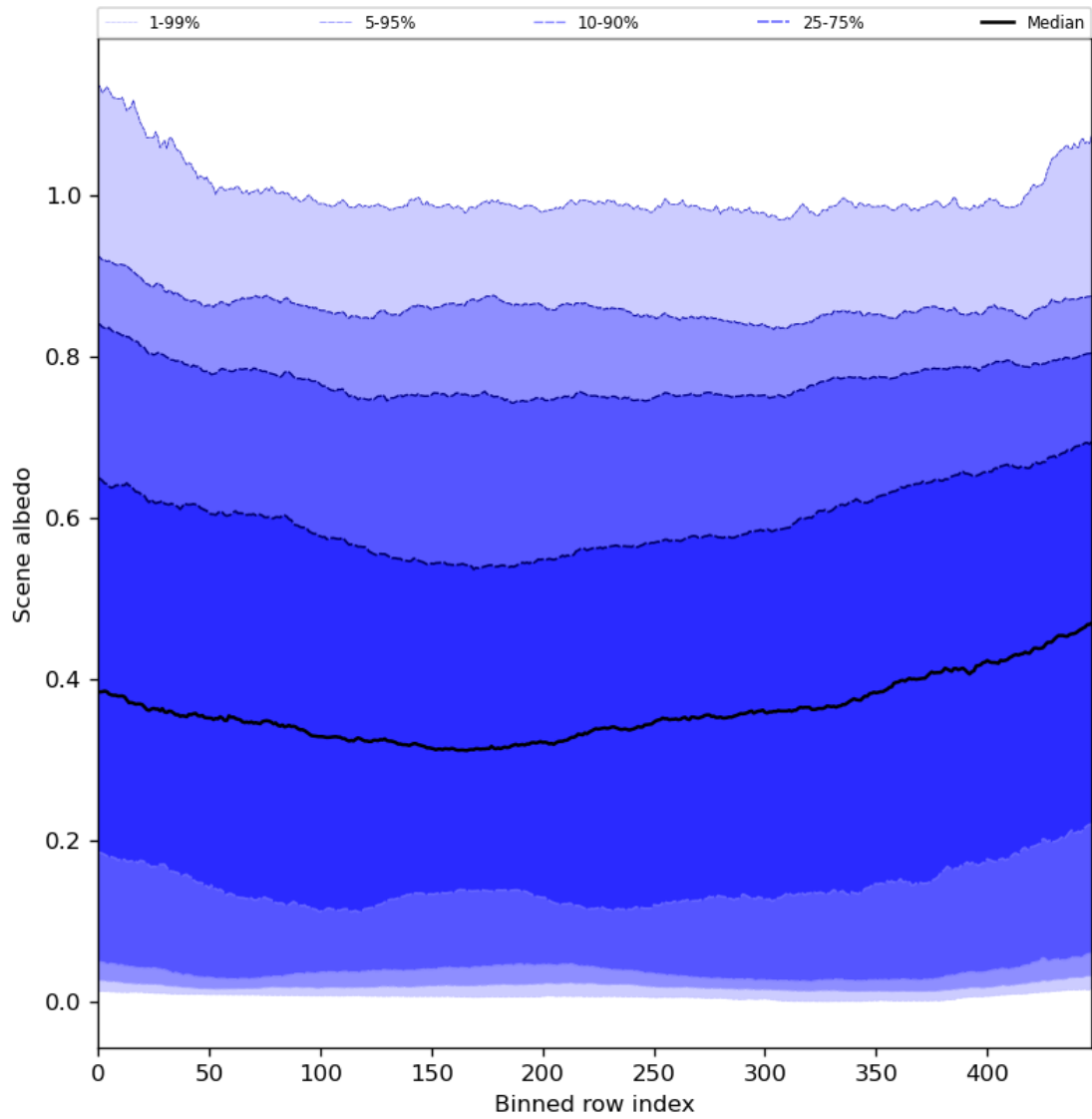
Figure 51: Along track statistics of “Scene albedo” for 2024-06-17 to 2024-06-19
