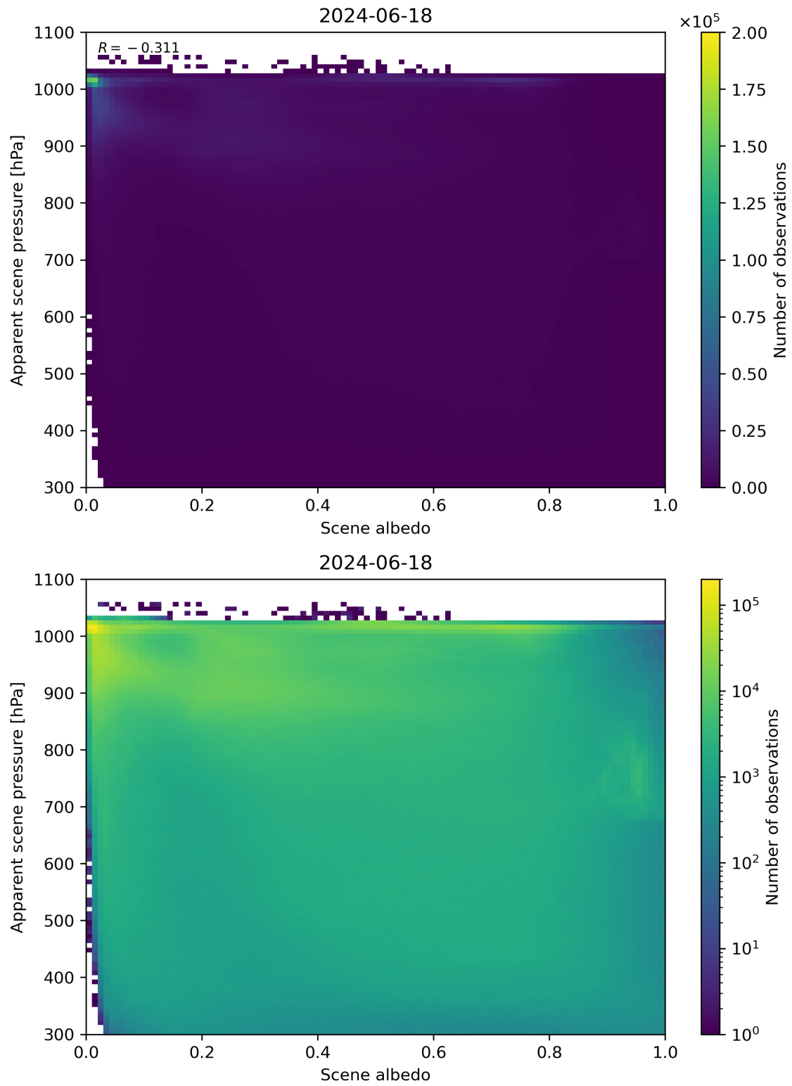
Figure 102: Scatter density plot of “Scene albedo” against “Apparent scene pressure” for 2024-06-17 to 2024-06-19.
