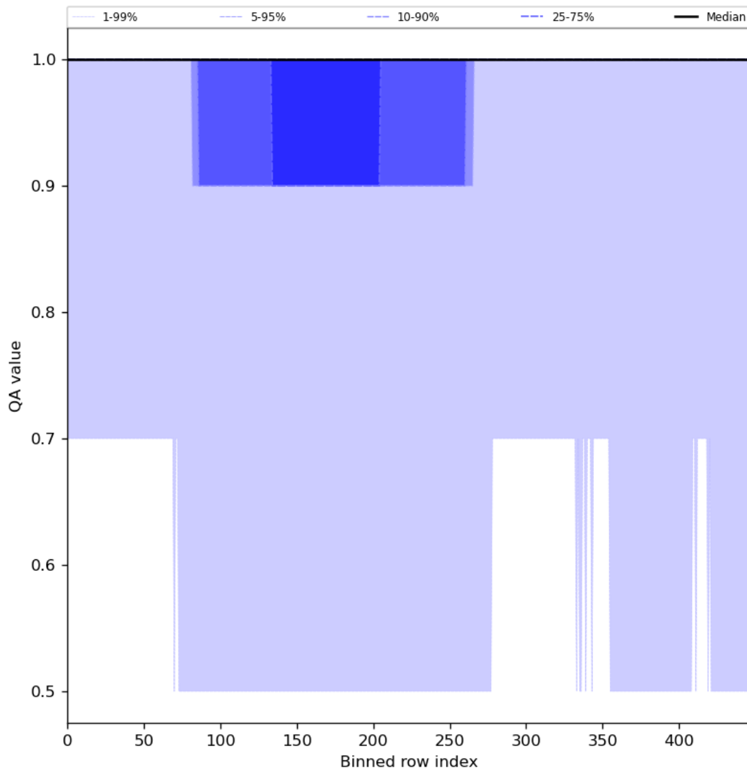
Figure 46: Along track statistics of "QA value" for 2024-06-17 to 2024-06-19
