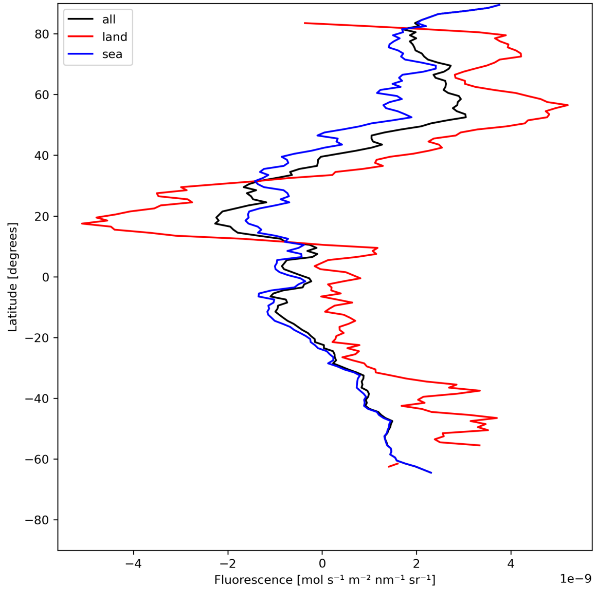
Figure 23: Zonal average of “Fluorescence” for 2024-06-17 to 2024-06-19.
