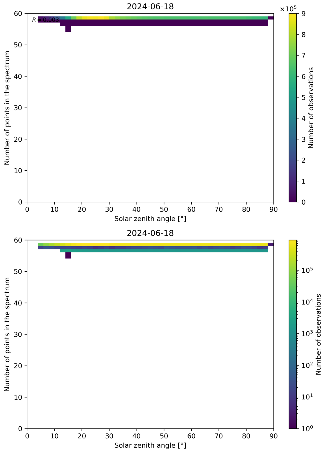
Figure 115: Scatter density plot of “Solar zenith angle” against “Number of points in the spectrum” for 2024-06-17 to 2024-06-19.
