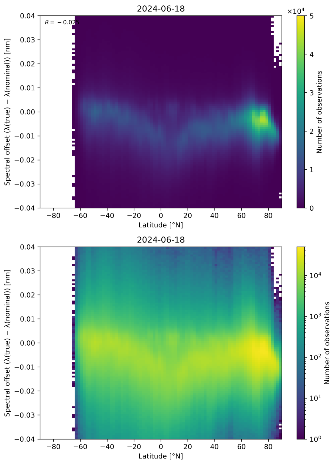
Figure 96: Scatter density plot of “Latitude” against “Spectral offset ( \lambda(\text{true}) - \lambda(\text{nominal}) )” for 2024-06-17 to 2024-06-19.
