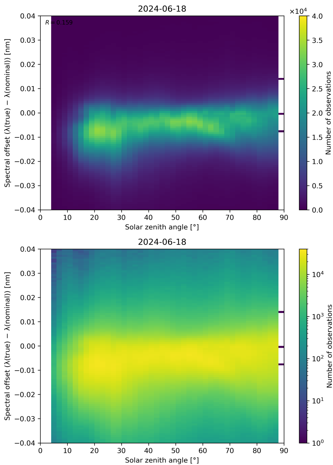
Figure 117: Scatter density plot of “Solar zenith angle” against “Spectral offset ( \lambda(\text{true}) - \lambda(\text{nominal}) )” for 2024-06-17 to 2024-06-19.
