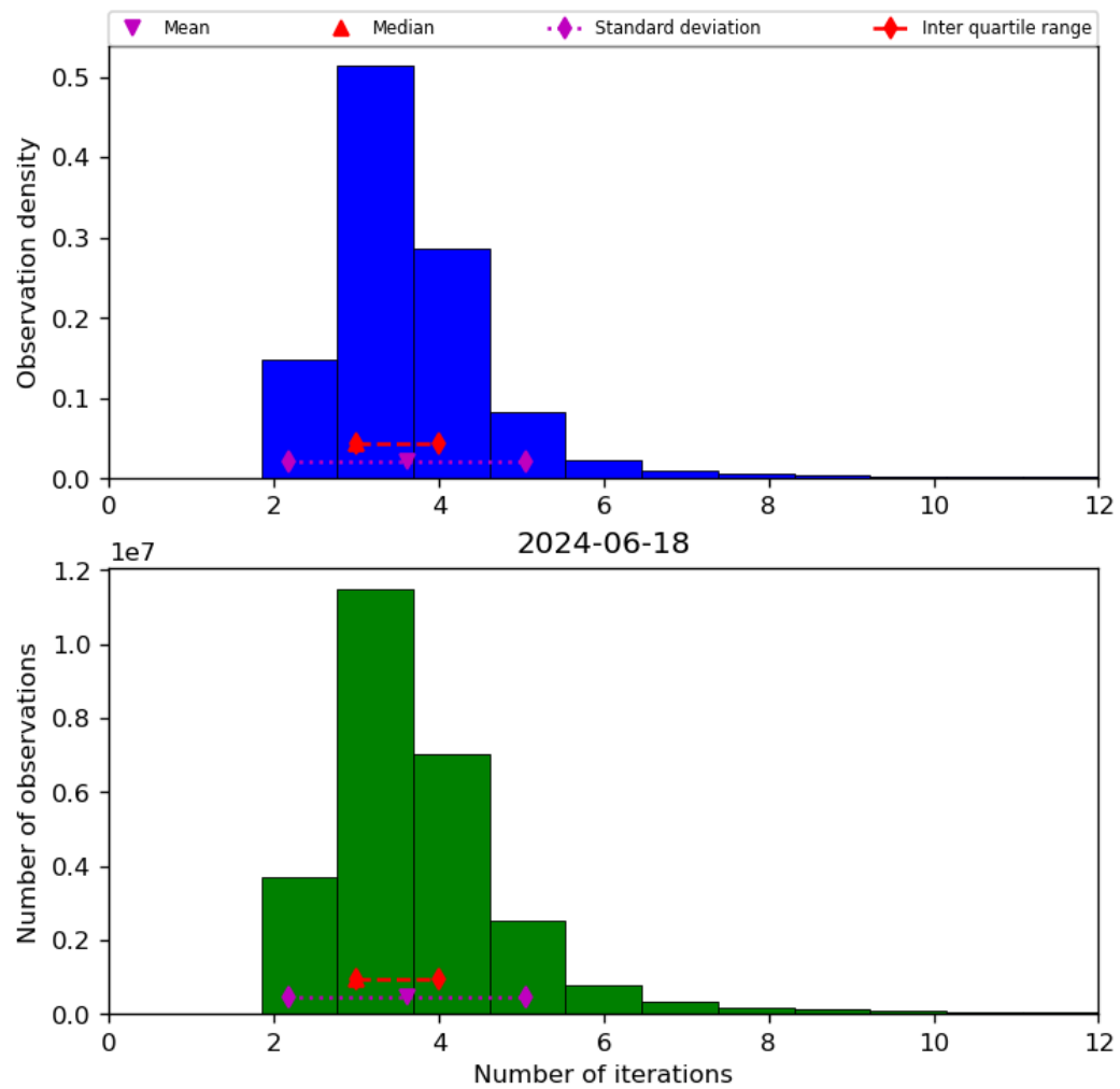
Figure 39: Histogram of “Number of iterations” for 2024-06-17 to 2024-06-19
