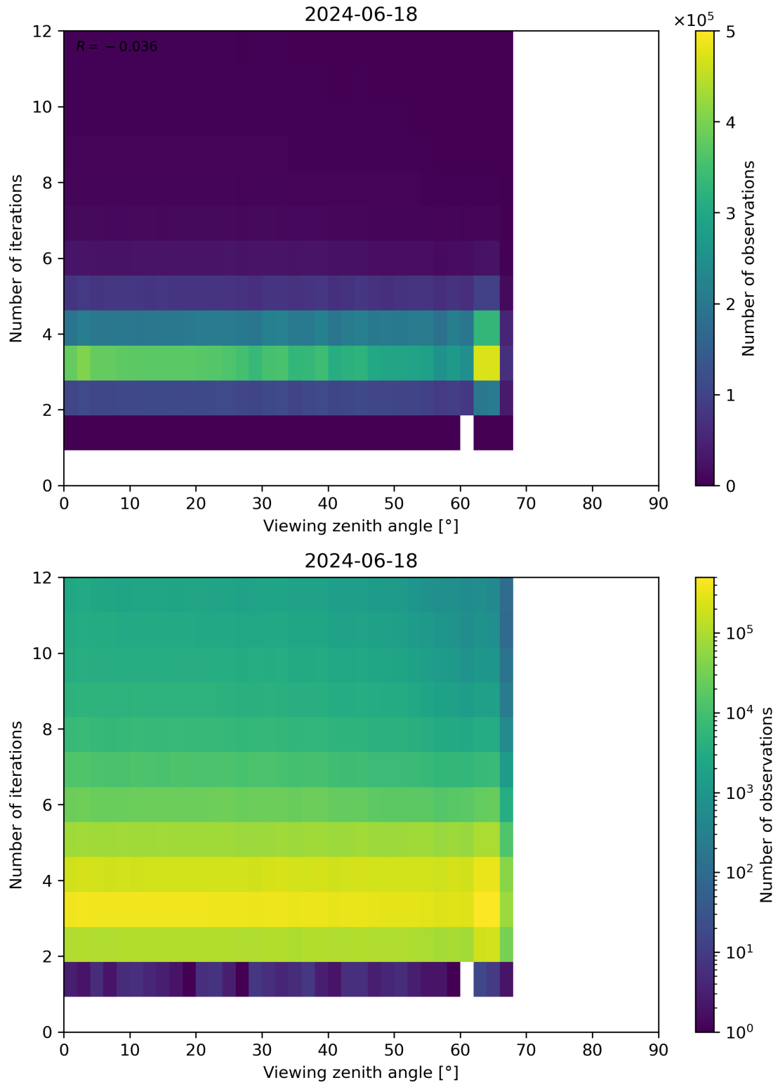
Figure 124: Scatter density plot of “Viewing zenith angle” against “Number of iterations” for 2024-06-17 to 2024-06-19.
