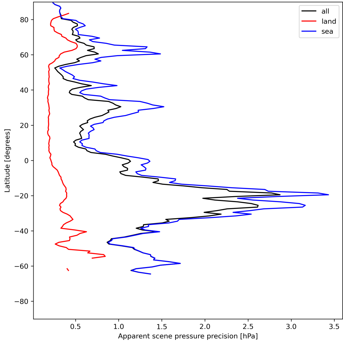
Figure 20: Zonal average of “Apparent scene pressure precision” for 2024-06-17 to 2024-06-19.
