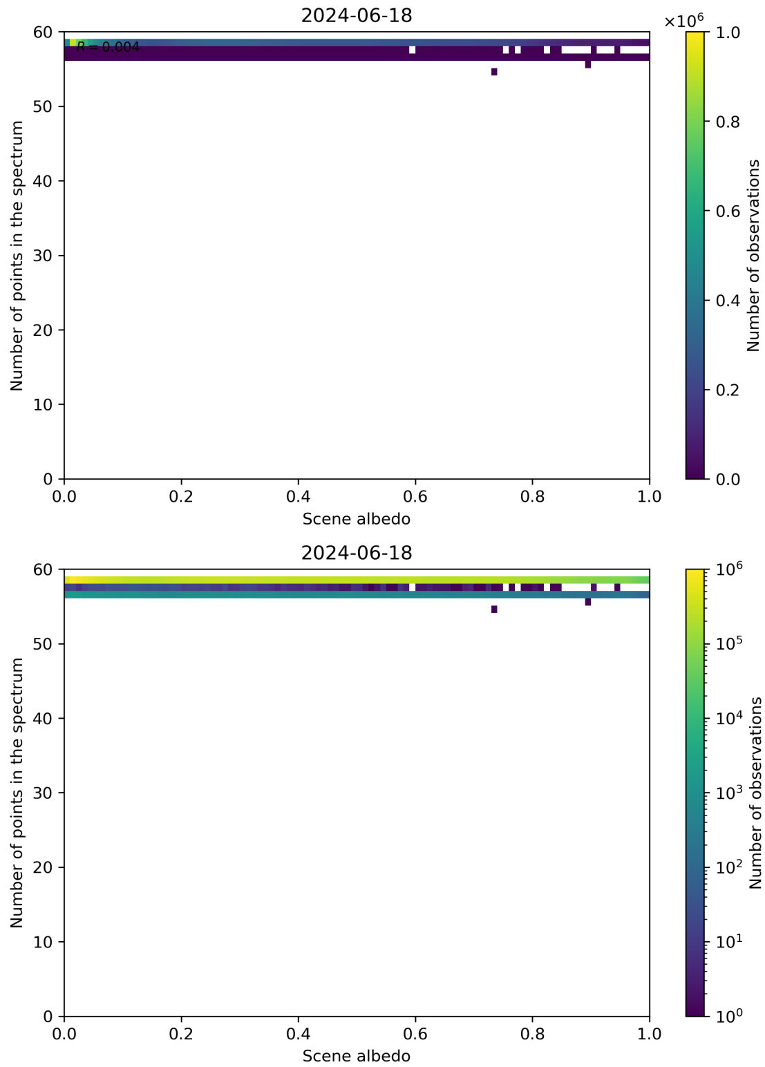
Figure 106: Scatter density plot of “Scene albedo” against “Number of points in the spectrum” for 2024-06-17 to 2024-06-19.
