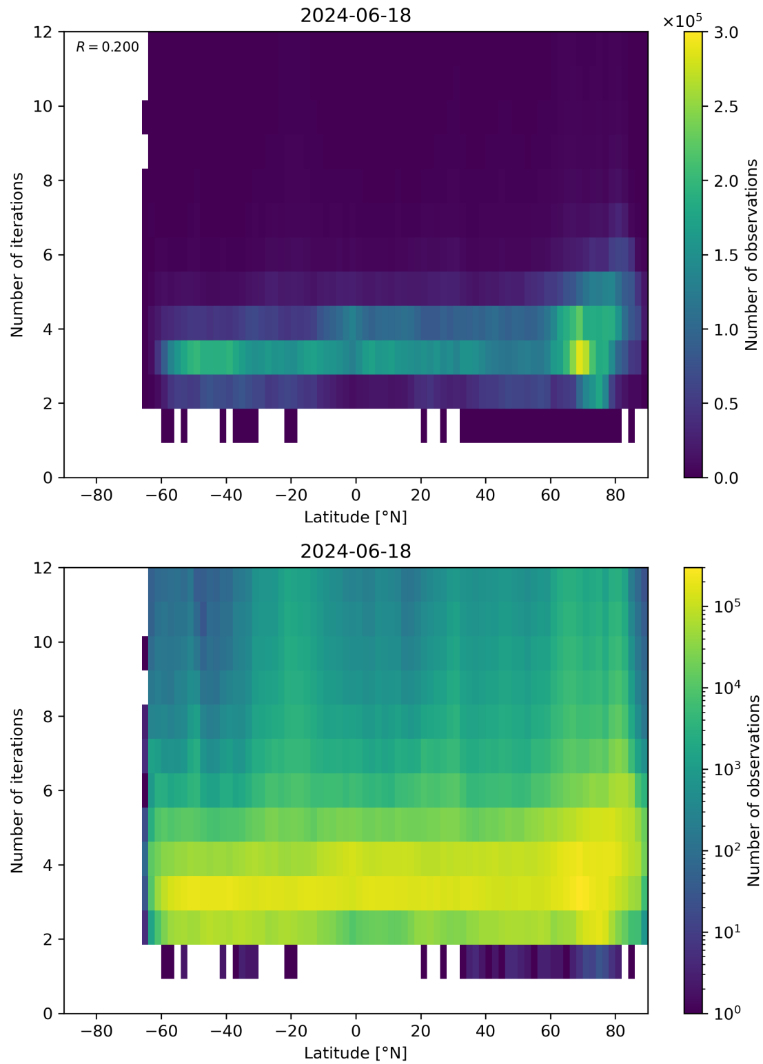
Figure 93: Scatter density plot of “Latitude” against “Number of iterations” for 2024-06-17 to 2024-06-19.
