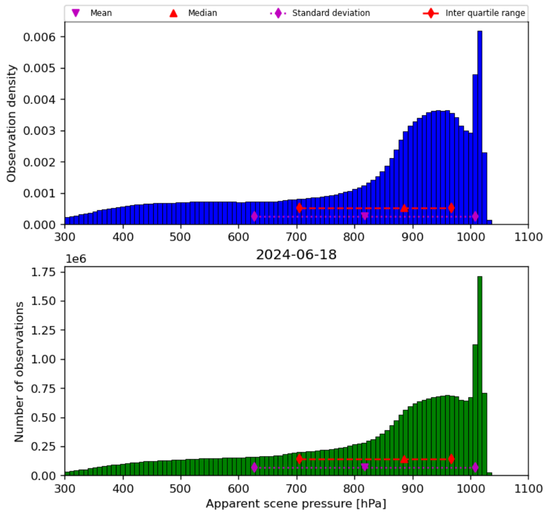
Figure 36: Histogram of “Apparent scene pressure” for 2024-06-17 to 2024-06-19
