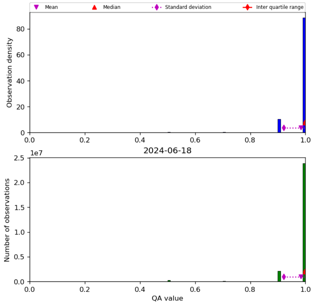
Figure 29: Histogram of “QA value” for 2024-06-17 to 2024-06-19
