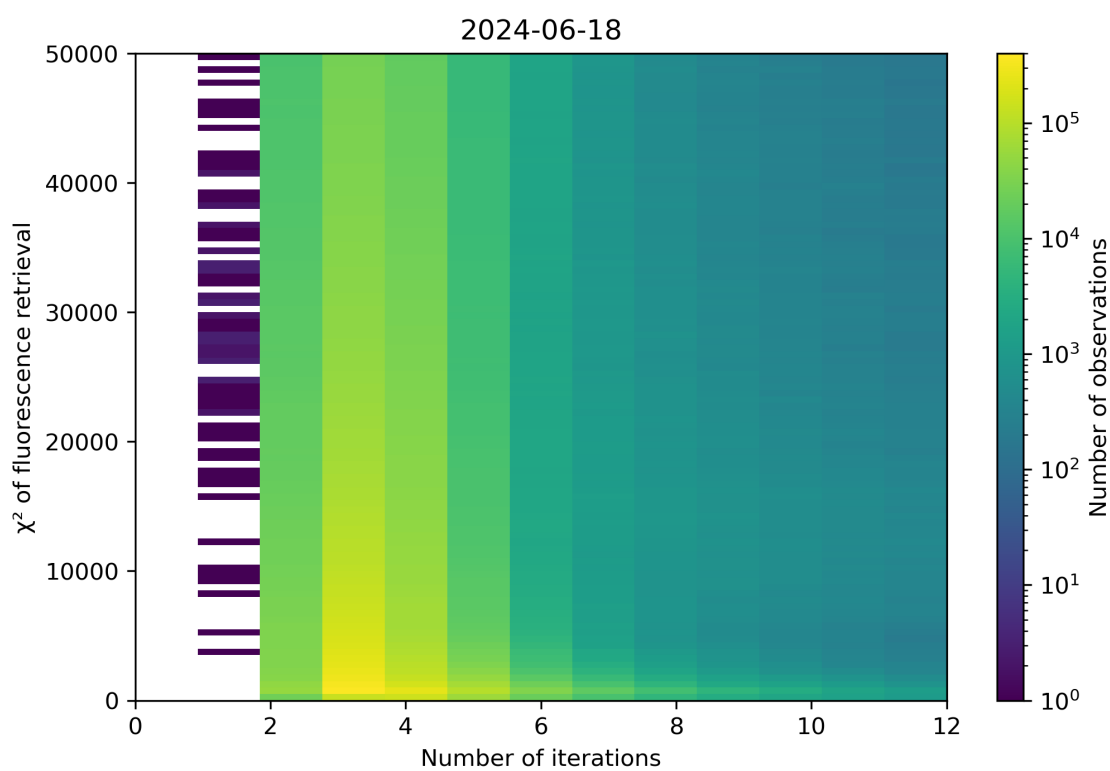
Figure 97: Scatter density plot of “Number of iterations” against “ \chi^2 of fluorescence retrieval” for 2024-06-17 to 2024-06-19.
