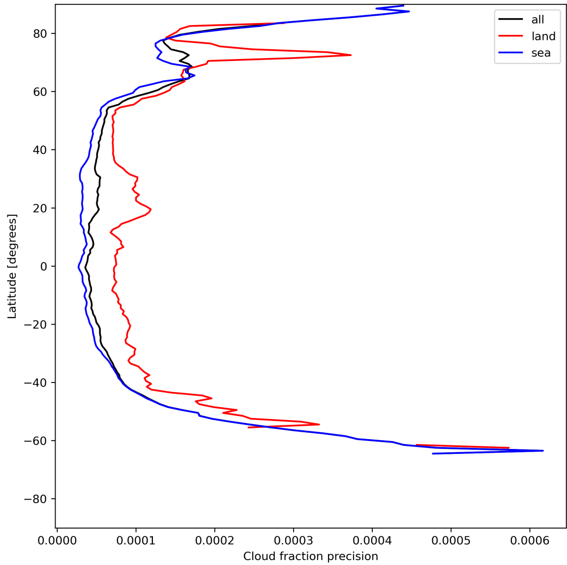
Figure 16: Zonal average of “Cloud fraction precision” for 2024-06-17 to 2024-06-19.
