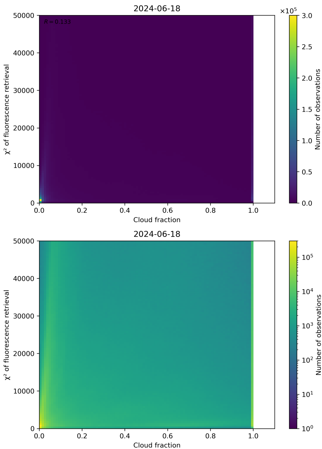
Figure 71: Scatter density plot of “Cloud fraction” against “ \chi^2 of fluorescence retrieval” for 2024-06-17 to 2024-06-19.
