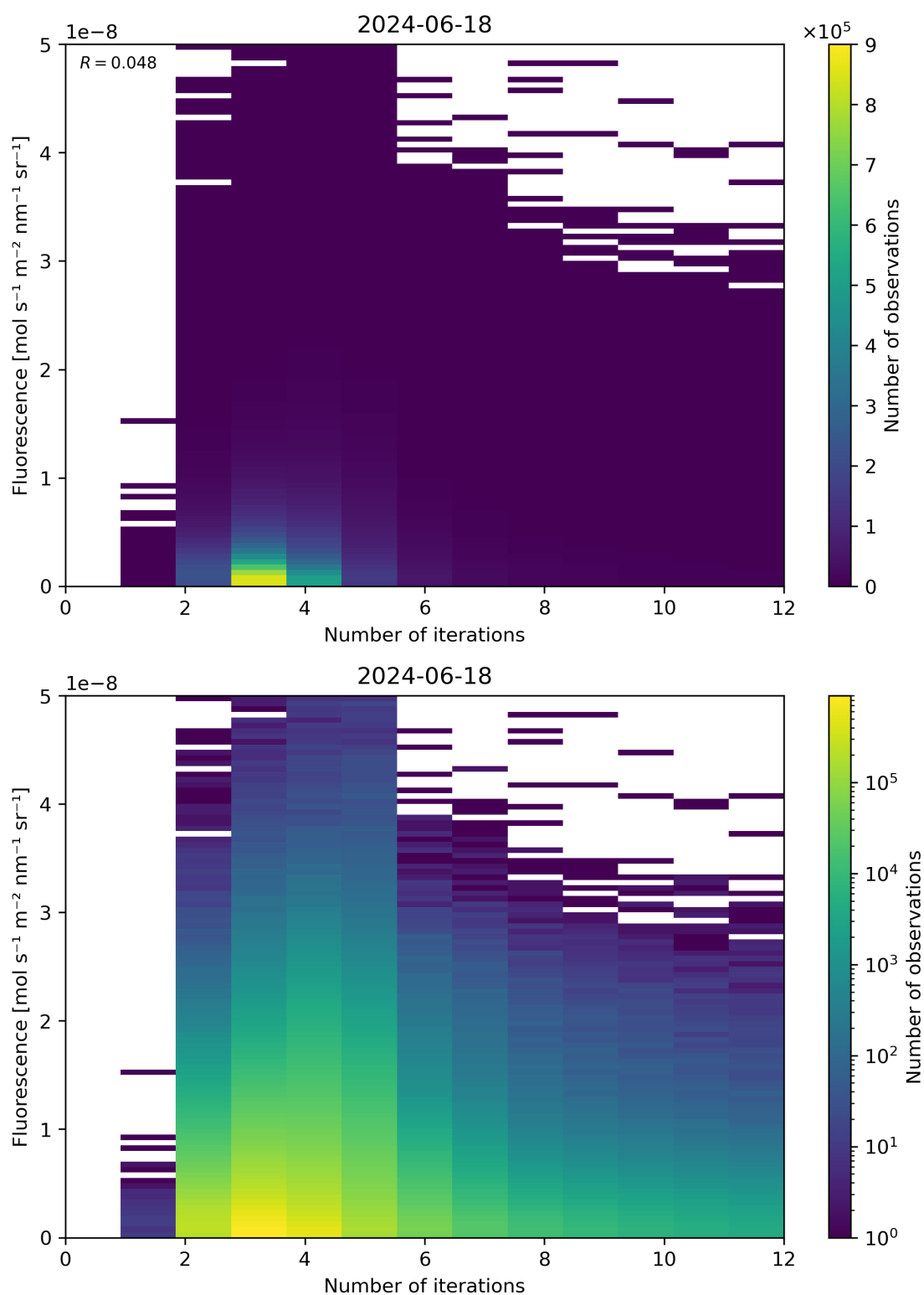
Figure 98: Scatter density plot of “Number of iterations” against “Fluorescence” for 2024-06-17 to 2024-06-19.
