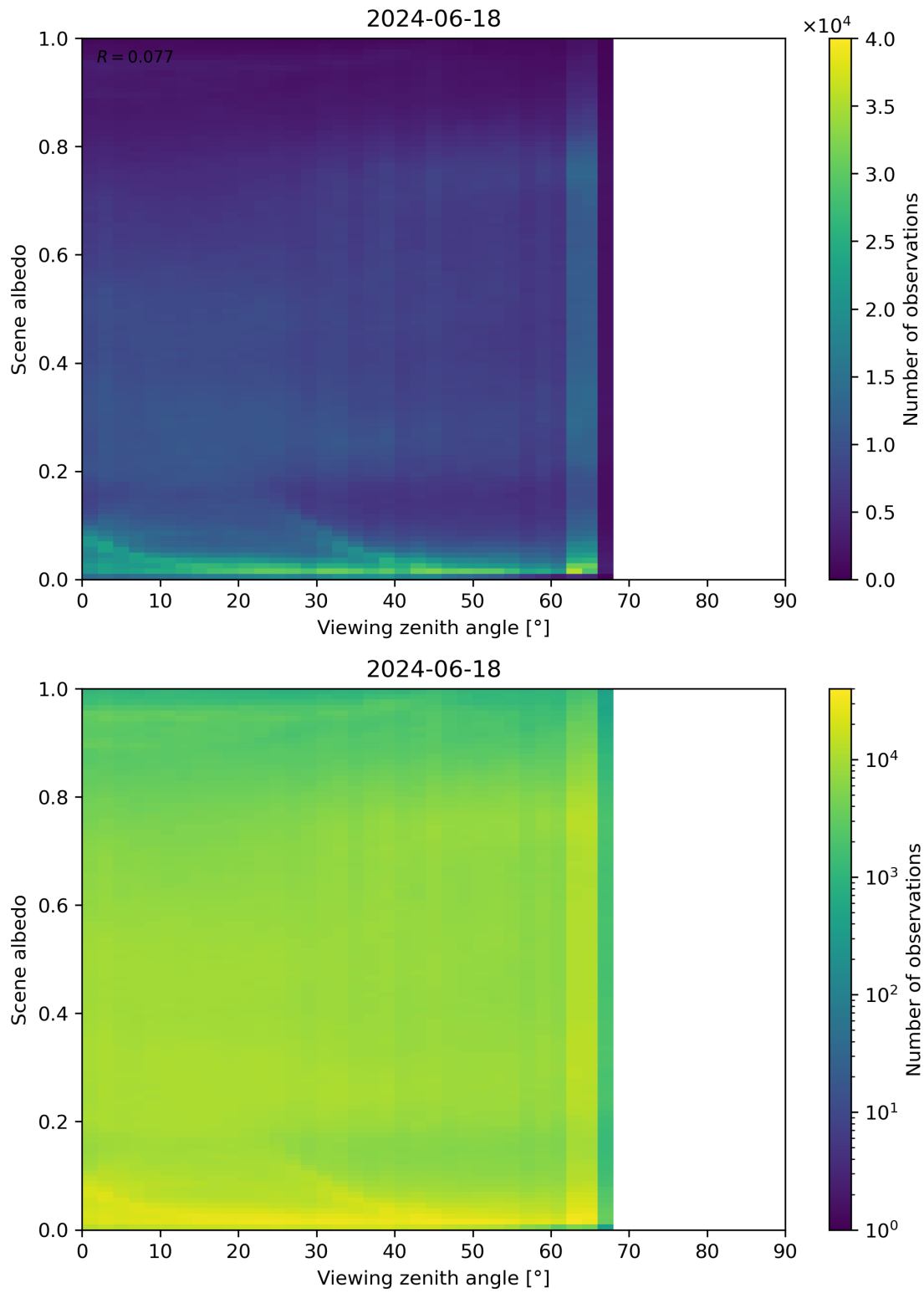
Figure 126: Scatter density plot of “Viewing zenith angle” against “Scene albedo” for 2024-06-17 to 2024-06-19.
