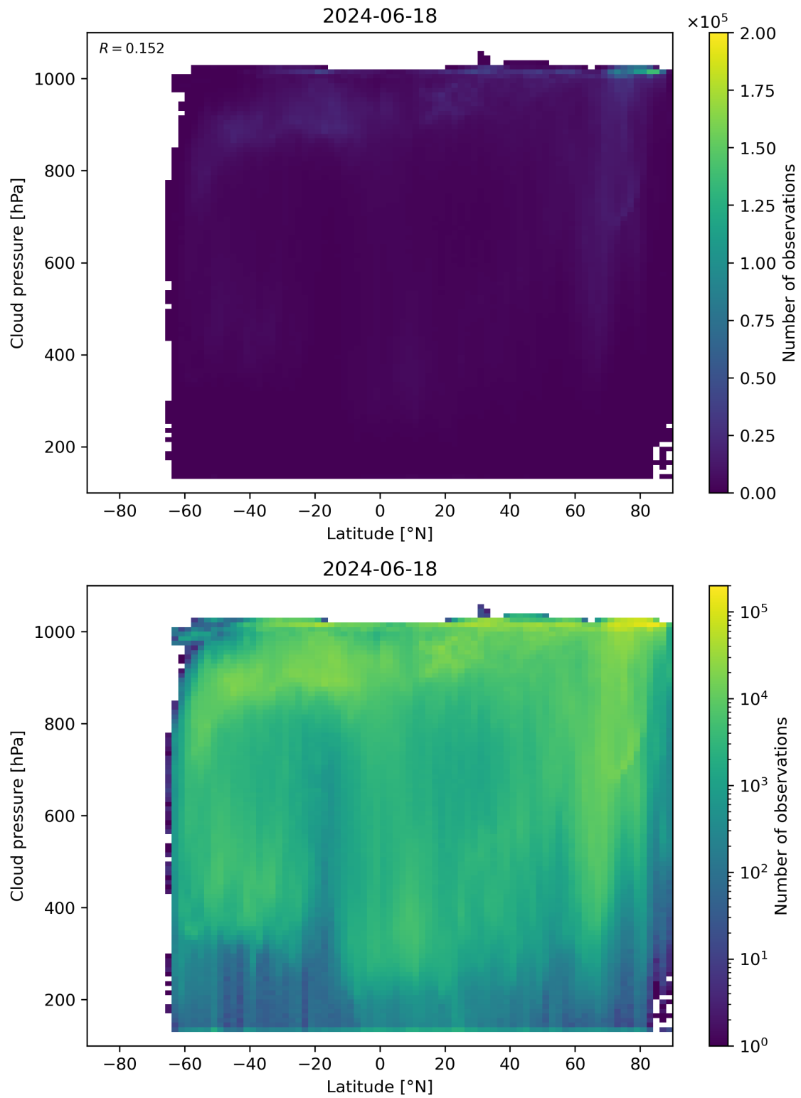
Figure 91: Scatter density plot of “Latitude” against “Cloud pressure” for 2024-06-17 to 2024-06-19.
