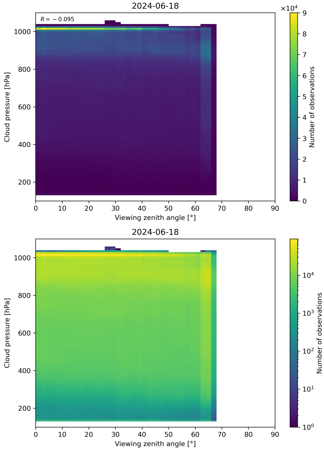
Figure 121: Scatter density plot of “Viewing zenith angle” against “Cloud pressure” for 2024-06-17 to 2024-06-19.
