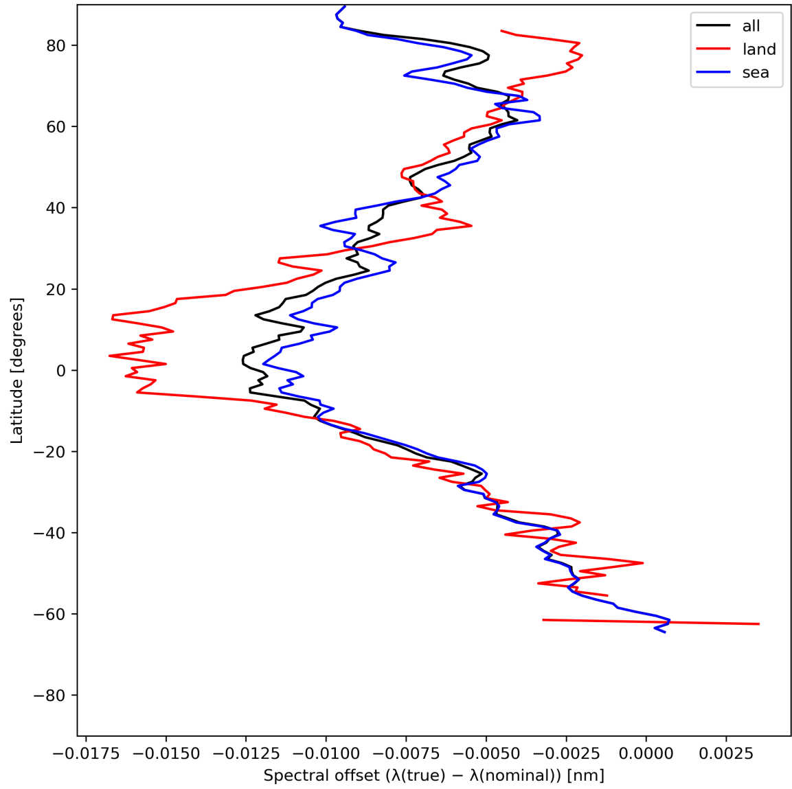
Figure 28: Zonal average of “Spectral offset ( \lambda(\text{true}) - \lambda(\text{nominal}) )” for 2024-06-17 to 2024-06-19.
