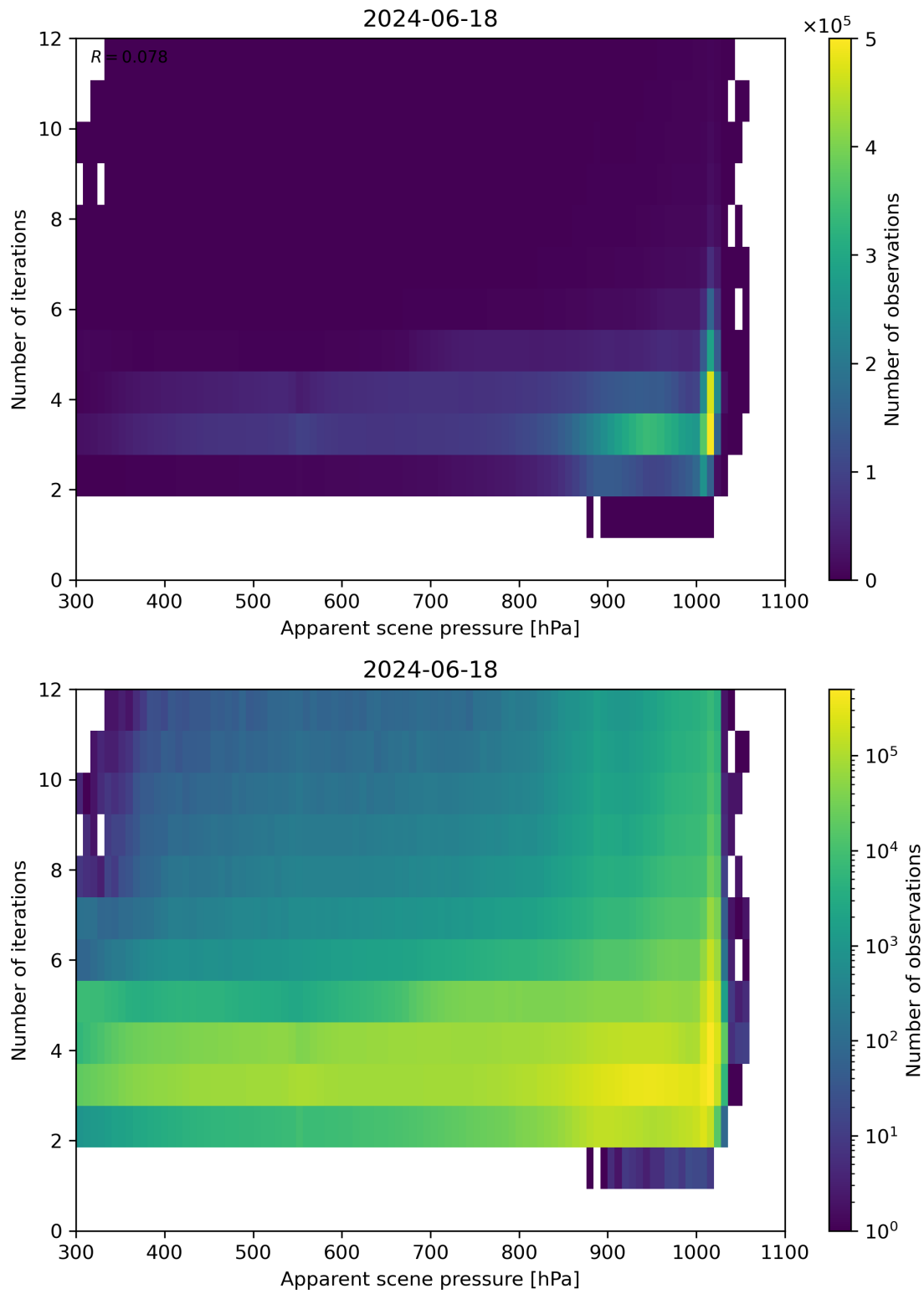
Figure 65: Scatter density plot of “Apparent scene pressure” against “Number of iterations” for 2024-06-17 to 2024-06-19.
