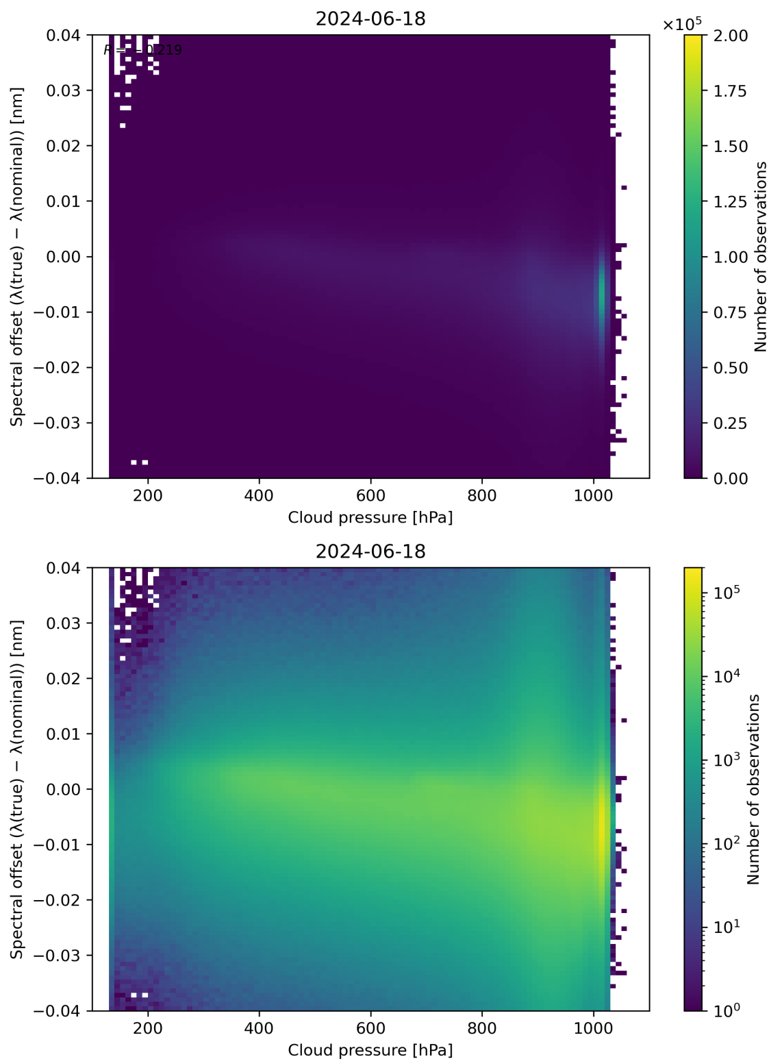
Figure 84: Scatter density plot of “Cloud pressure” against “Spectral offset ( \lambda(\text{true}) - \lambda(\text{nominal}) )” for 2024-06-17 to 2024-06-19.
