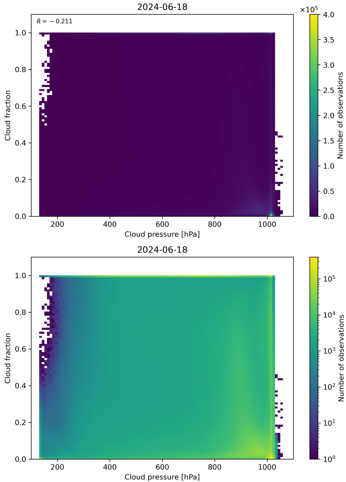
Figure 79: Scatter density plot of “Cloud pressure” against “Cloud fraction” for 2024-06-17 to 2024-06-19.
