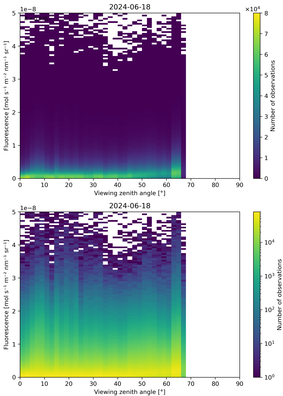
Figure 122: Scatter density plot of “Viewing zenith angle” against “Fluorescence” for 2024-06-17 to 2024-06-19.
