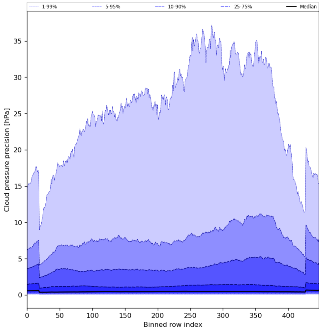
Figure 48: Along track statistics of “Cloud pressure precision” for 2024-06-17 to 2024-06-19
