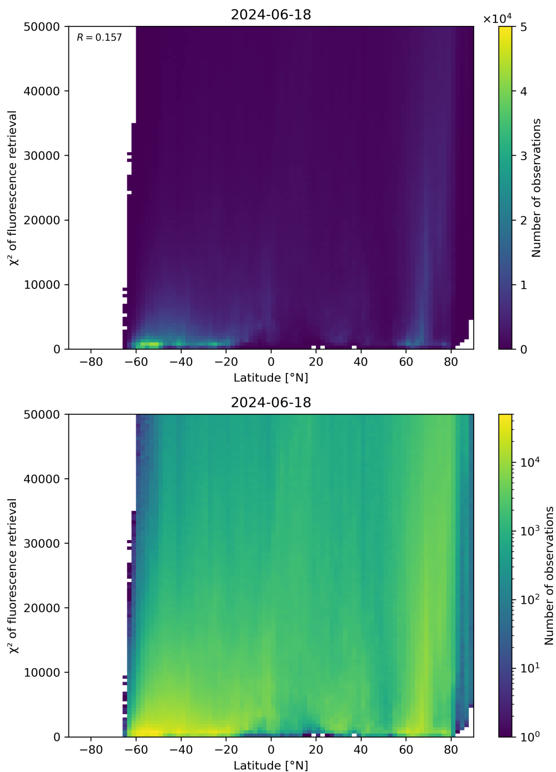
Figure 89: Scatter density plot of “Latitude” against “ \chi^2 of fluorescence retrieval” for 2024-06-17 to 2024-06-19.
