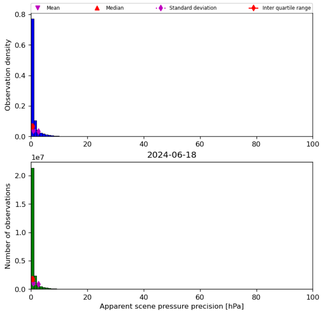
Figure 37: Histogram of “Apparent scene pressure precision” for 2024-06-17 to 2024-06-19
