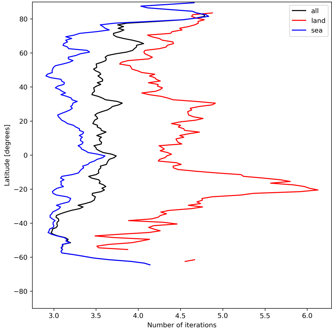
Figure 22: Zonal average of “Number of iterations” for 2024-06-17 to 2024-06-19.
