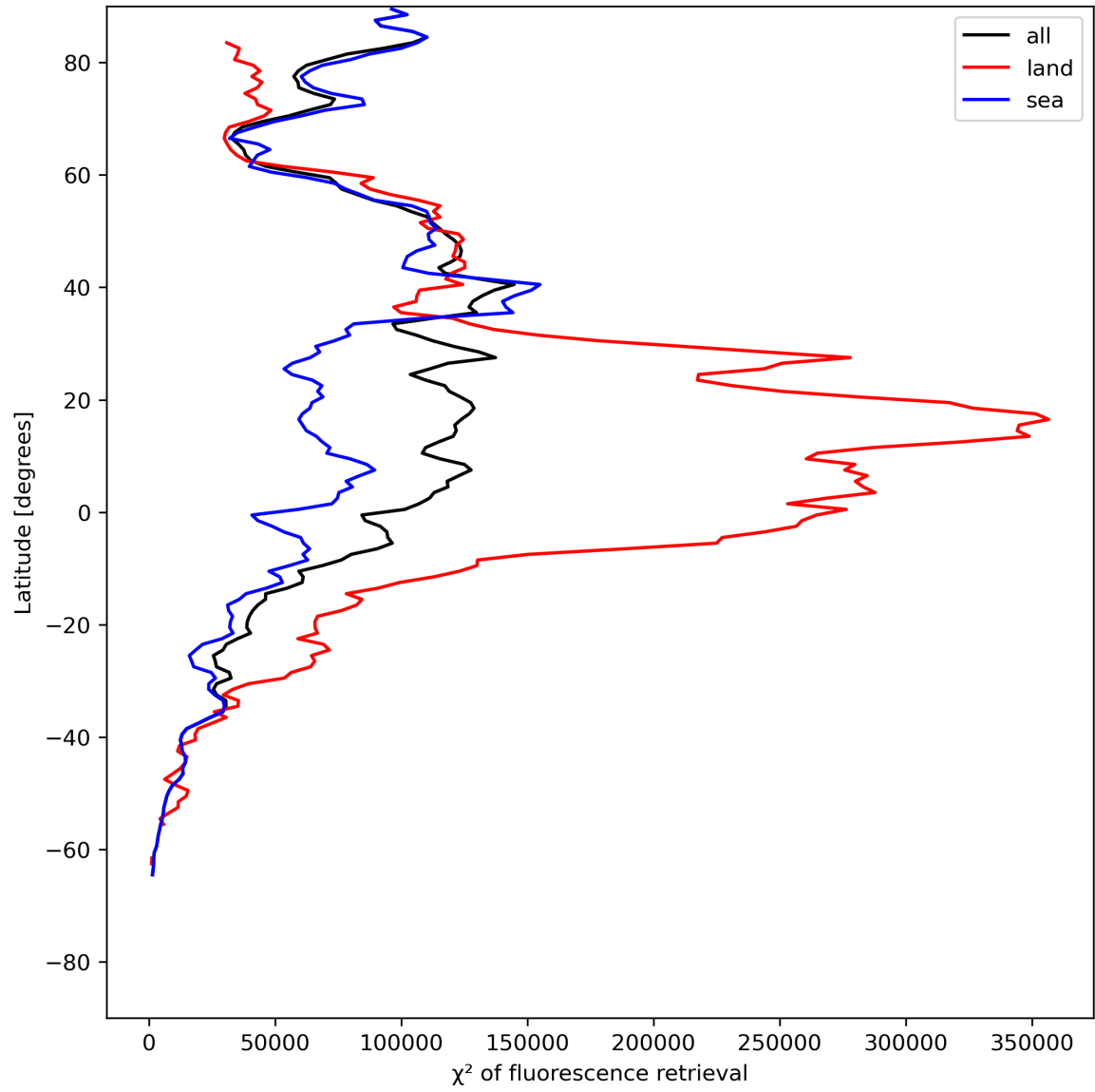
Figure 25: Zonal average of “ \chi^2 of fluorescence retrieval” for 2024-06-17 to 2024-06-19.
