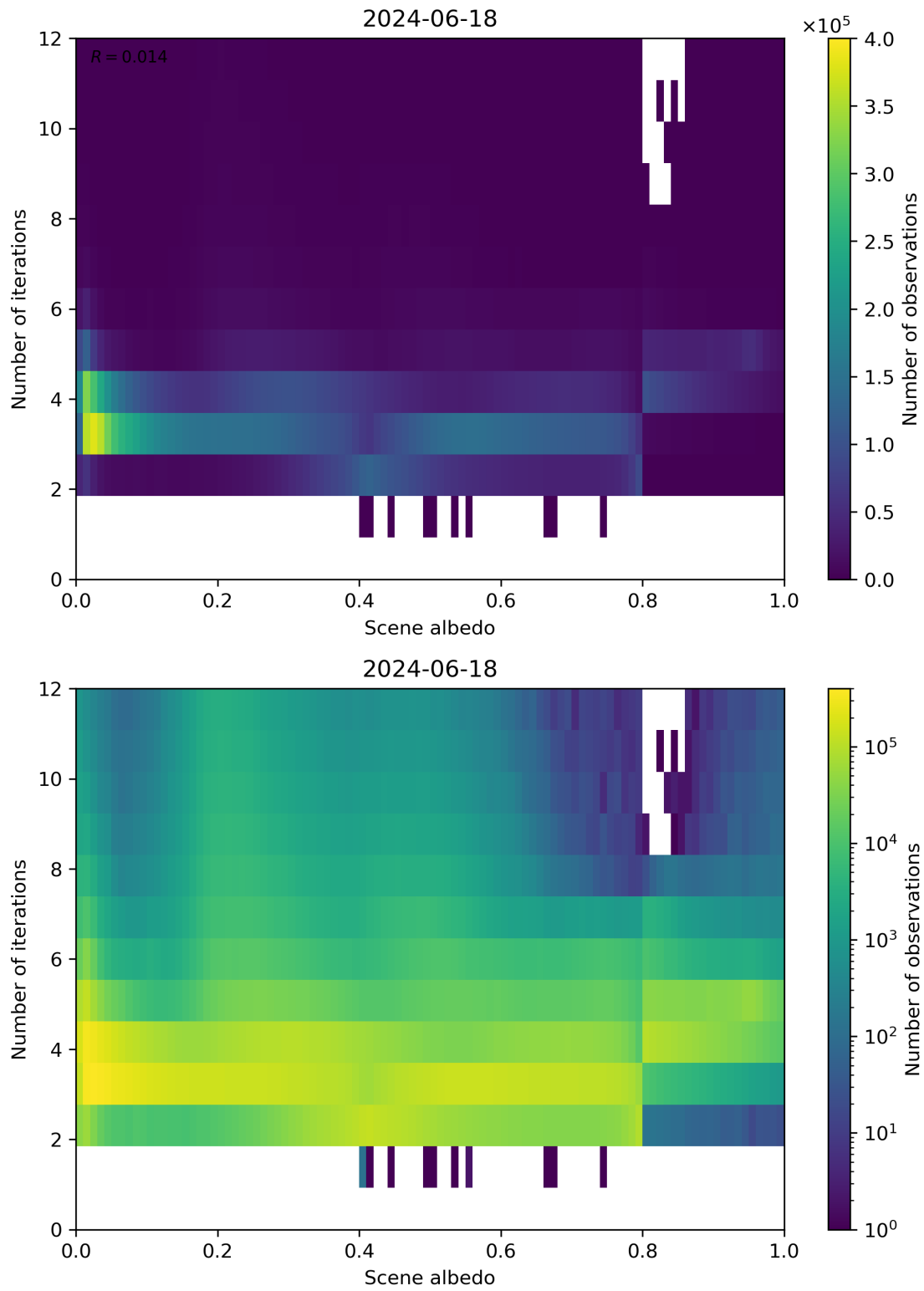
Figure 105: Scatter density plot of “Scene albedo” against “Number of iterations” for 2024-06-17 to 2024-06-19.
