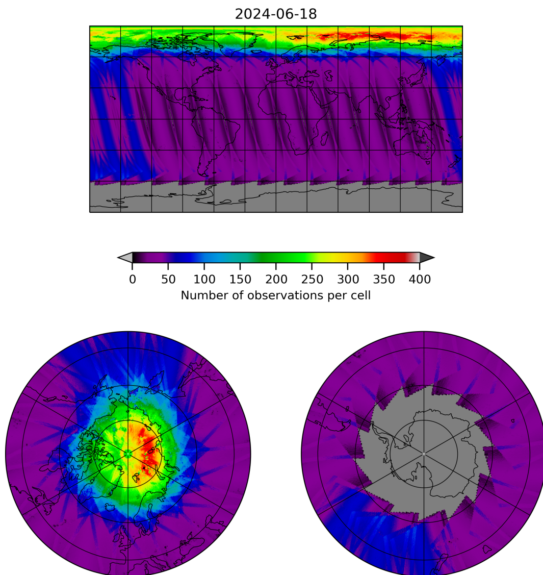
Figure 11: Map of the number of observations for 2024-06-17 to 2024-06-19
