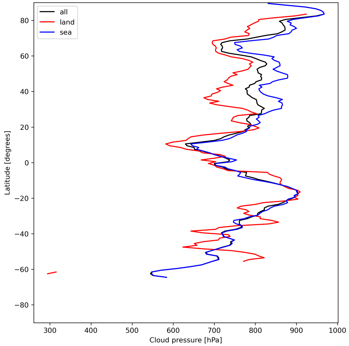
Figure 13: Zonal average of “Cloud pressure” for 2024-06-17 to 2024-06-19.
