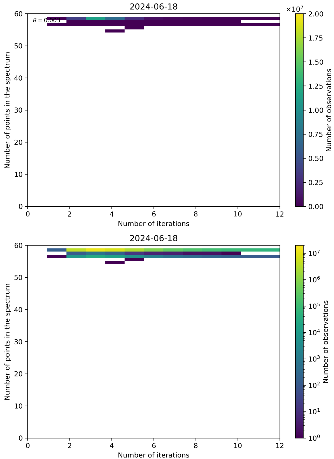
Figure 99: Scatter density plot of “Number of iterations” against “Number of points in the spectrum” for 2024-06-17 to 2024-06-19.
