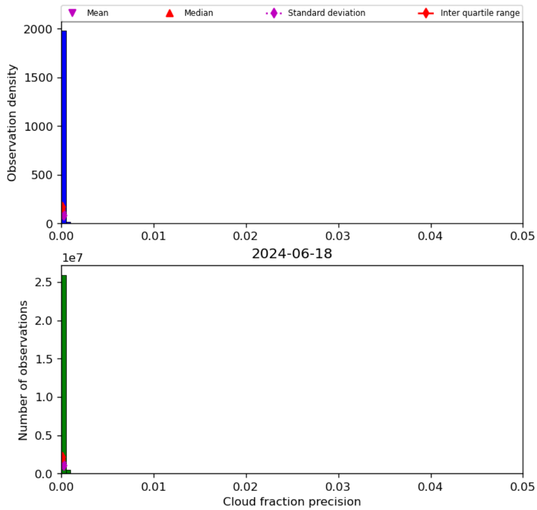
Figure 33: Histogram of “Cloud fraction precision” for 2024-06-17 to 2024-06-19
