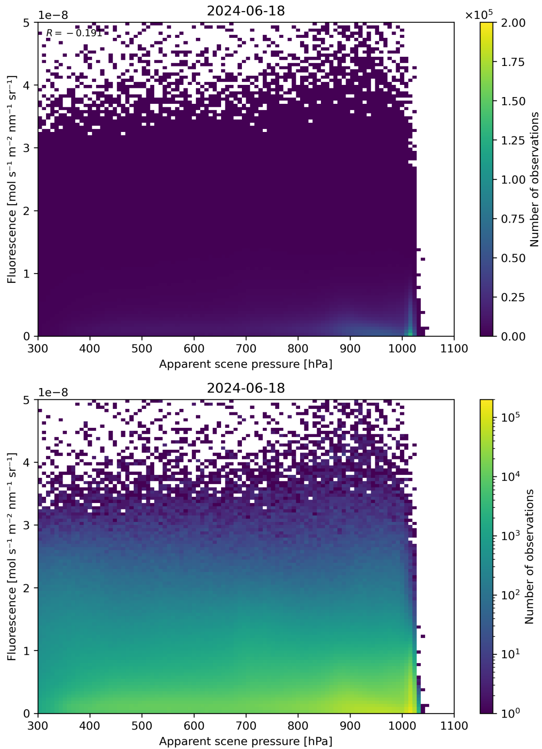
Figure 64: Scatter density plot of “Apparent scene pressure” against “Fluorescence” for 2024-06-17 to 2024-06-19.
