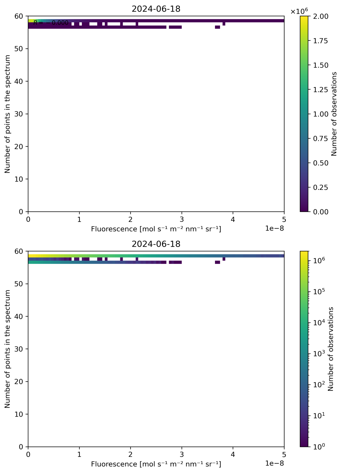
Figure 86: Scatter density plot of “Fluorescence” against “Number of points in the spectrum” for 2024-06-17 to 2024-06-19.
