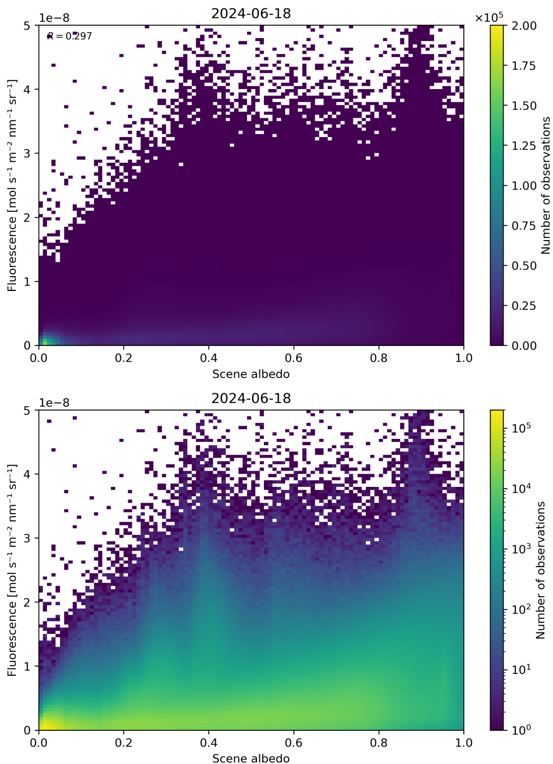
Figure 104: Scatter density plot of “Scene albedo” against “Fluorescence” for 2024-06-17 to 2024-06-19.
