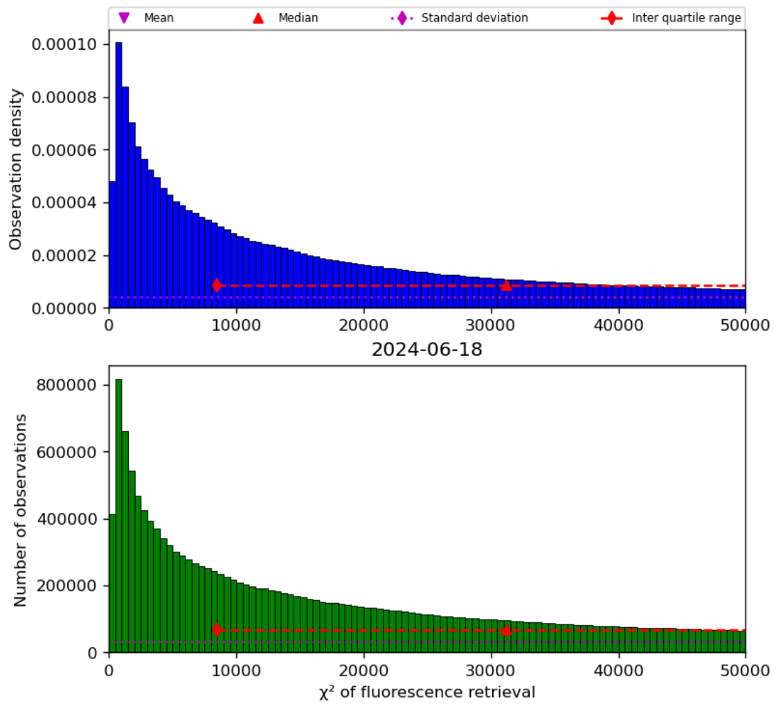
Figure 42: Histogram of “ \chi^2 of fluorescence retrieval” for 2024-06-17 to 2024-06-19
