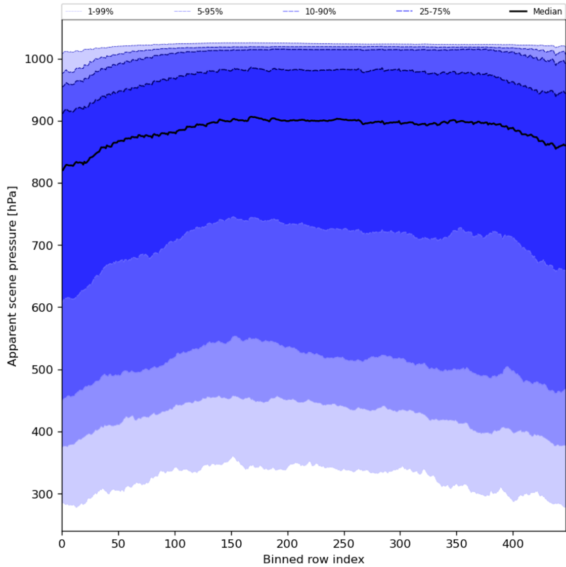
Figure 53: Along track statistics of “Apparent scene pressure” for 2024-06-17 to 2024-06-19
