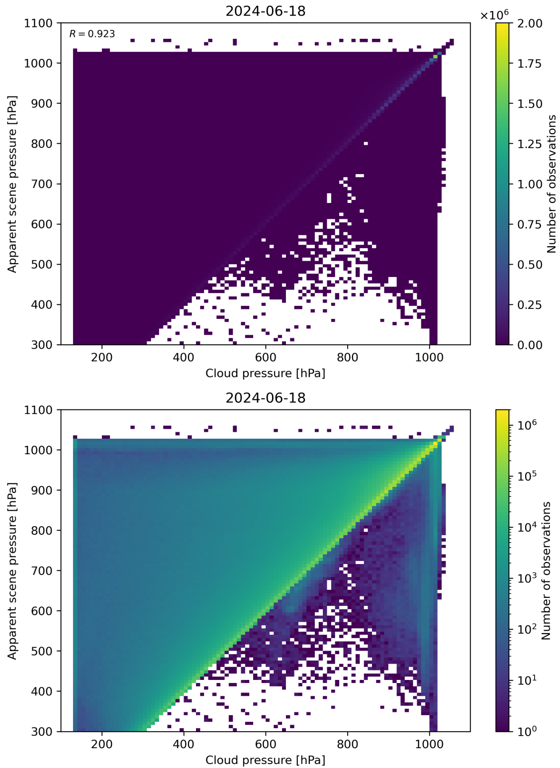
Figure 77: Scatter density plot of “Cloud pressure” against “Apparent scene pressure” for 2024-06-17 to 2024-06-19.
