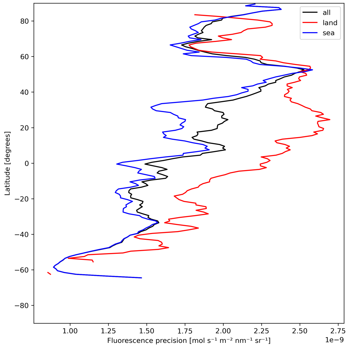
Figure 24: Zonal average of “Fluorescence precision” for 2024-06-17 to 2024-06-19.
