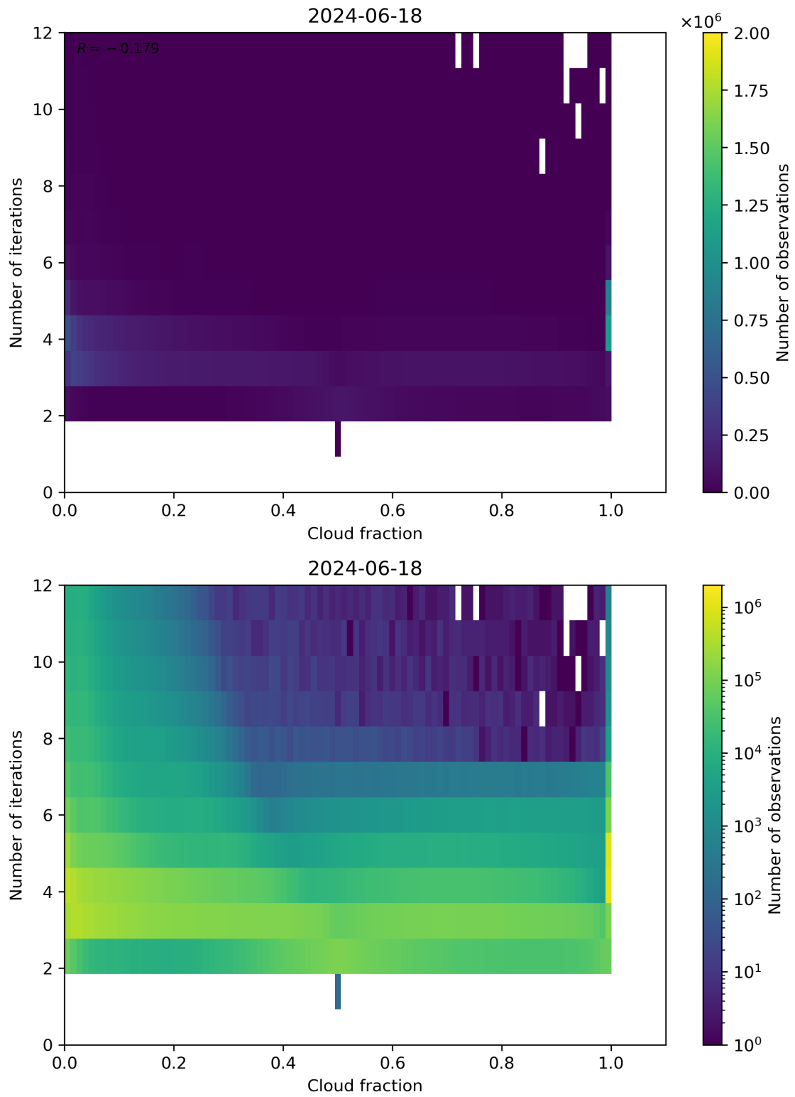
Figure 73: Scatter density plot of “Cloud fraction” against “Number of iterations” for 2024-06-17 to 2024-06-19.
