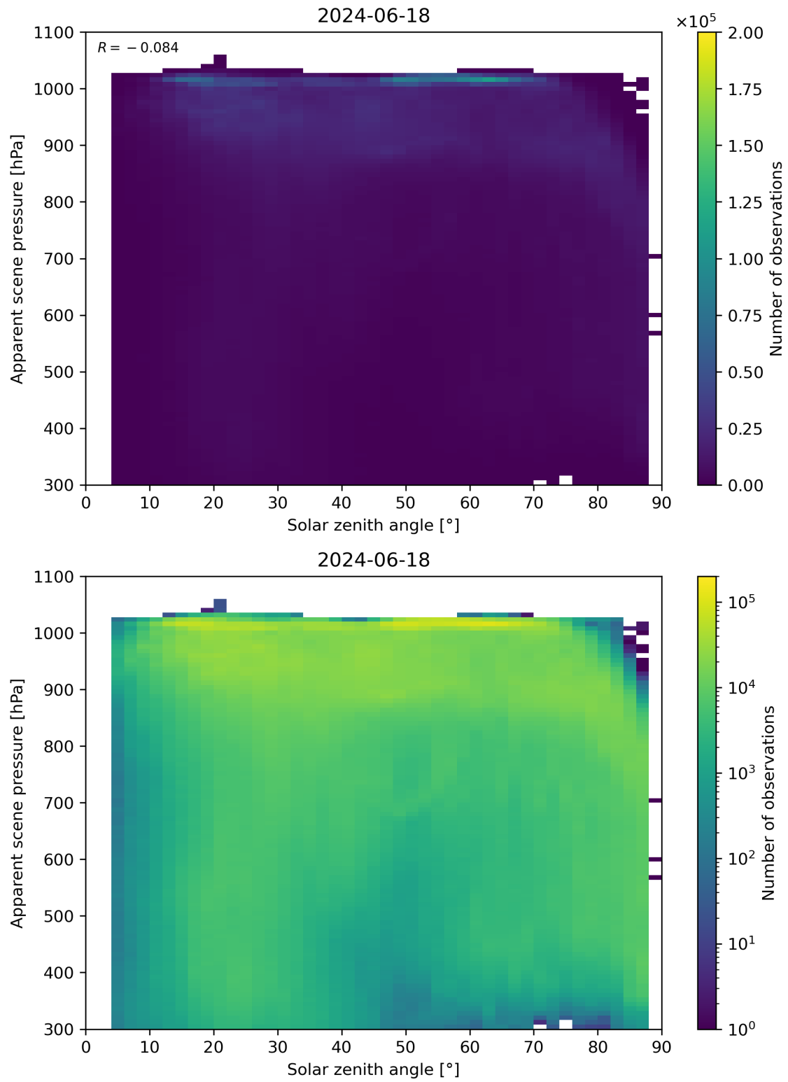
Figure 108: Scatter density plot of “Solar zenith angle” against “Apparent scene pressure” for 2024-06-17 to 2024-06-19.
