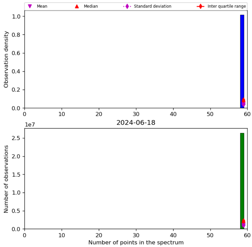
Figure 44: Histogram of “Number of points in the spectrum” for 2024-06-17 to 2024-06-19
