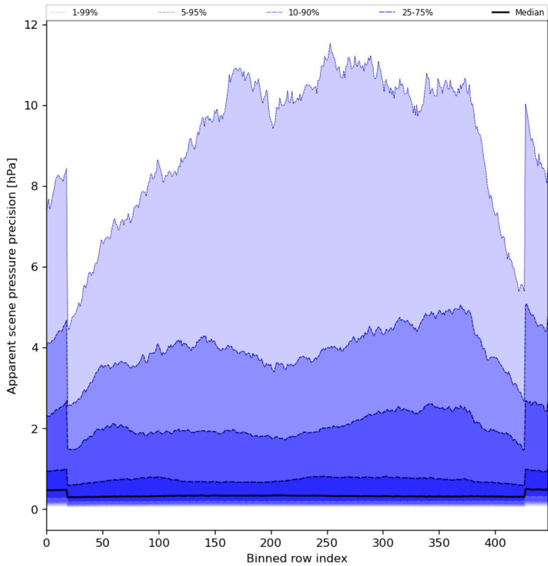
Figure 54: Along track statistics of “Apparent scene pressure precision” for 2024-06-17 to 2024-06-19
