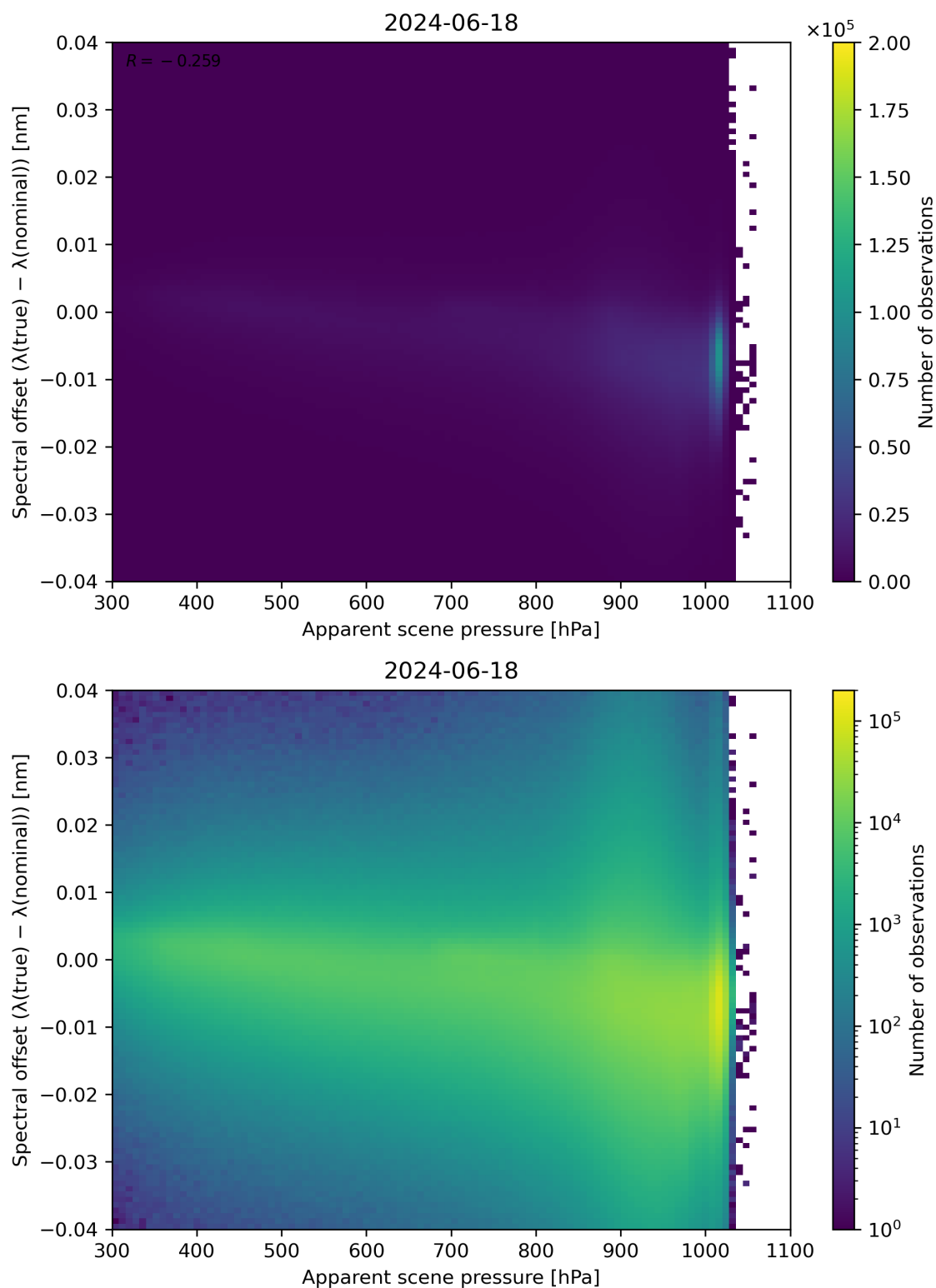
Figure 67: Scatter density plot of “Apparent scene pressure” against “Spectral offset ( \lambda(\text{true}) - \lambda(\text{nominal}) )” for 2024-06-17 to 2024-06-19.
