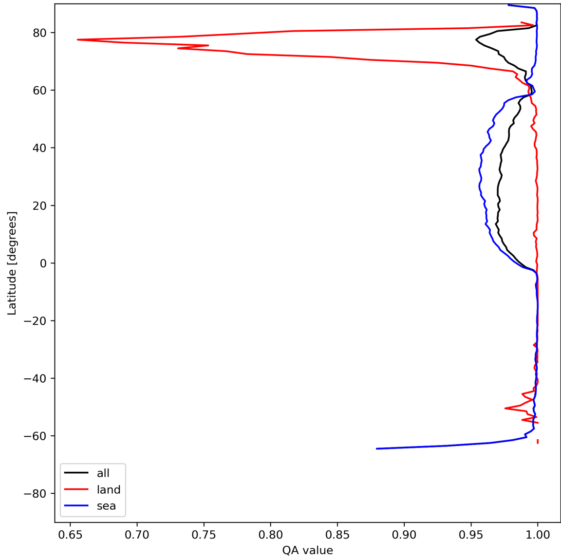
Figure 12: Zonal average of “QA value” for 2024-06-17 to 2024-06-19.
