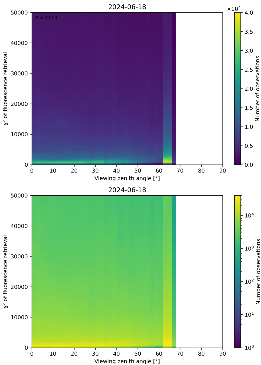
Figure 119: Scatter density plot of “Viewing zenith angle” against “ \chi^2 of fluorescence retrieval” for 2024-06-17 to 2024-06-19.
