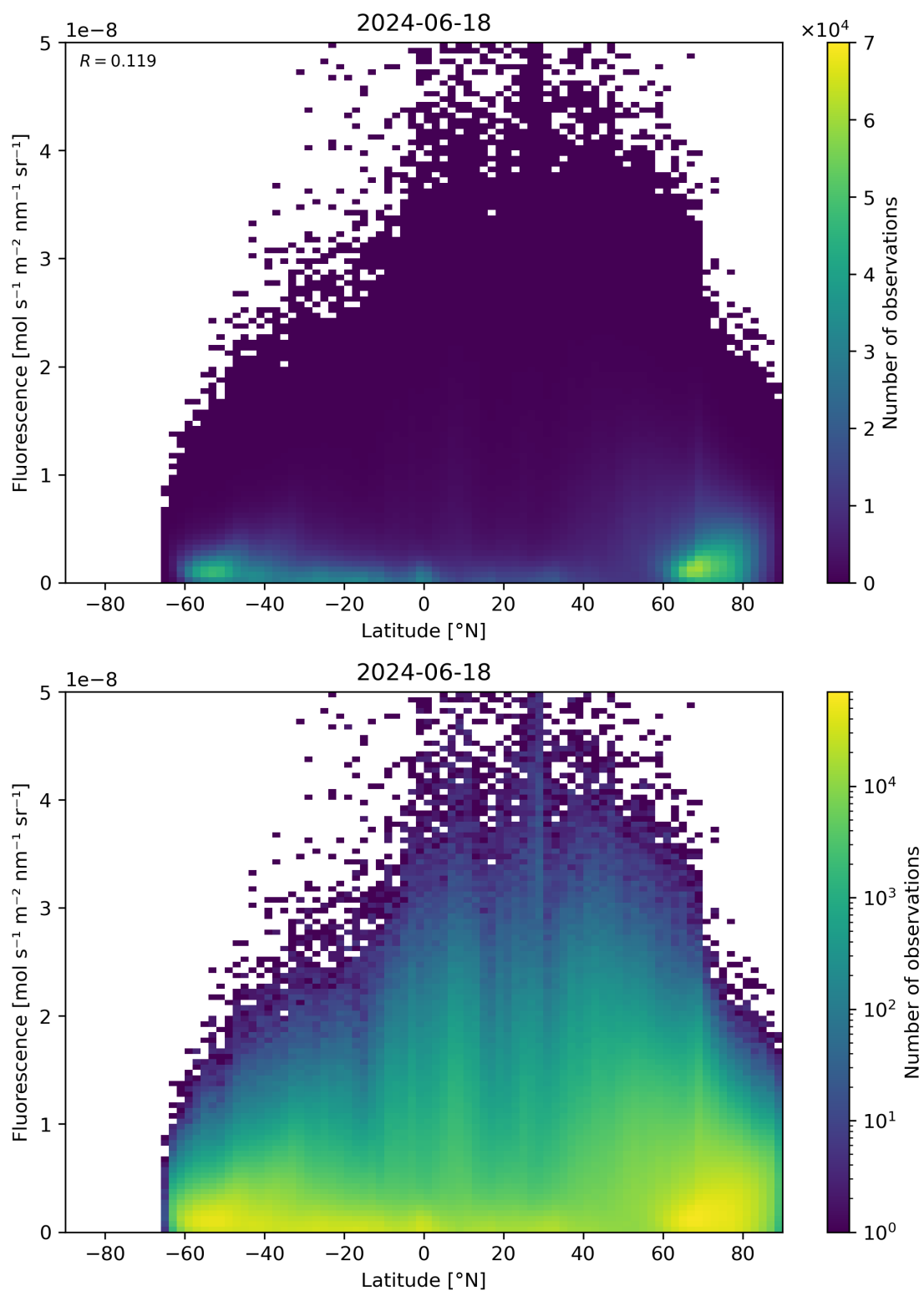
Figure 92: Scatter density plot of “Latitude” against “Fluorescence” for 2024-06-17 to 2024-06-19.
