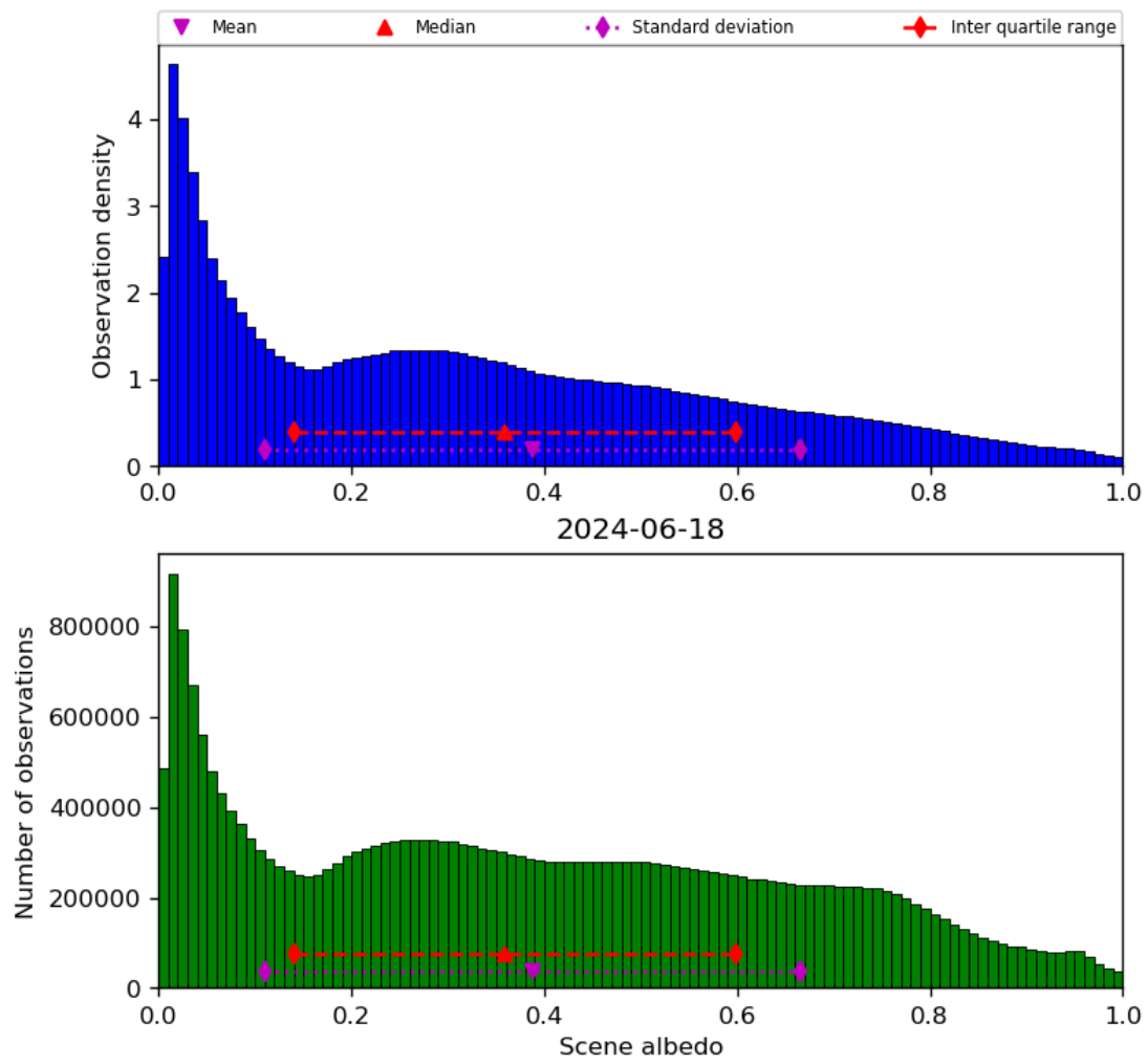
Figure 34: Histogram of “Scene albedo” for 2024-06-17 to 2024-06-19
