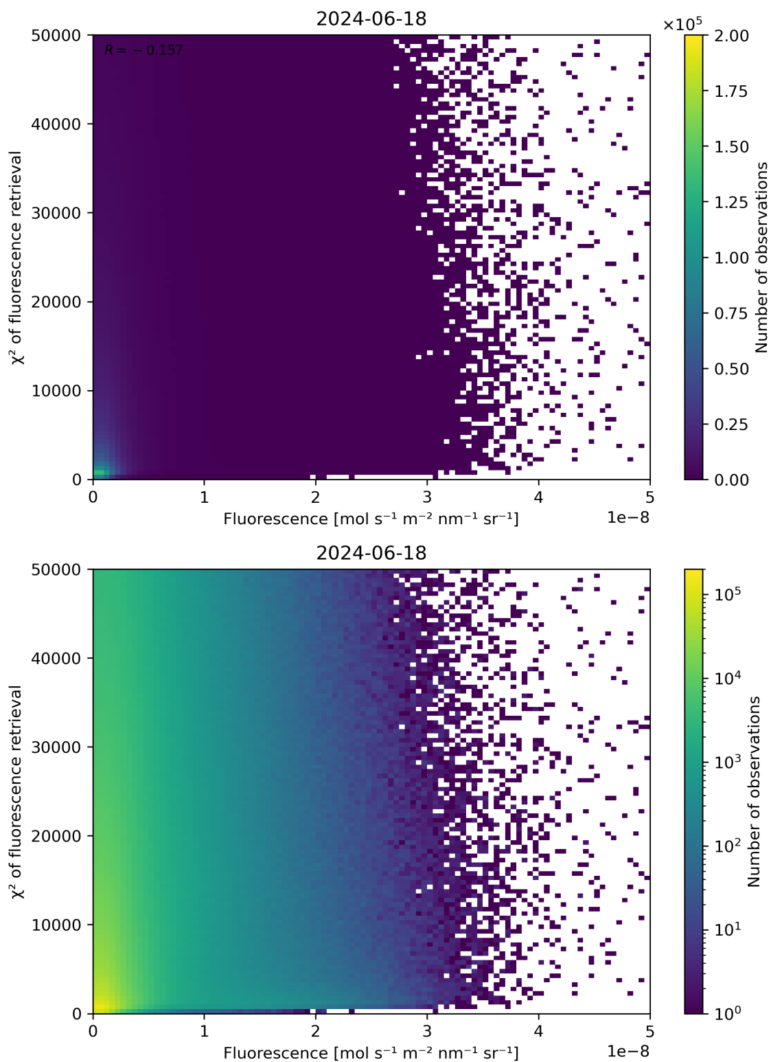
Figure 85: Scatter density plot of “Fluorescence” against “ \chi^2 of fluorescence retrieval” for 2024-06-17 to 2024-06-19.
