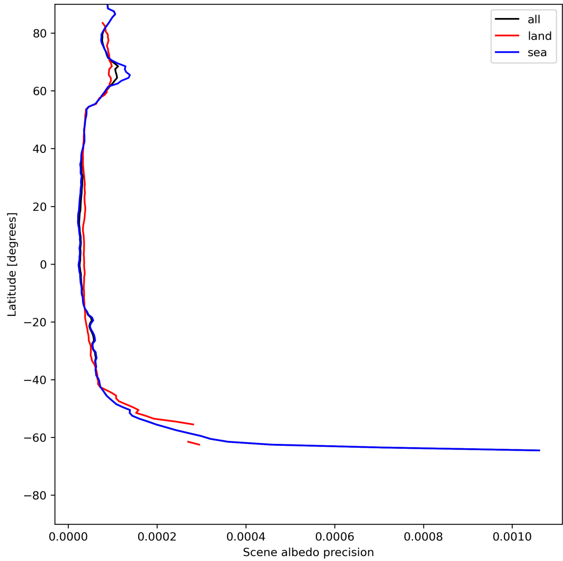
Figure 18: Zonal average of “Scene albedo precision” for 2024-06-17 to 2024-06-19.
