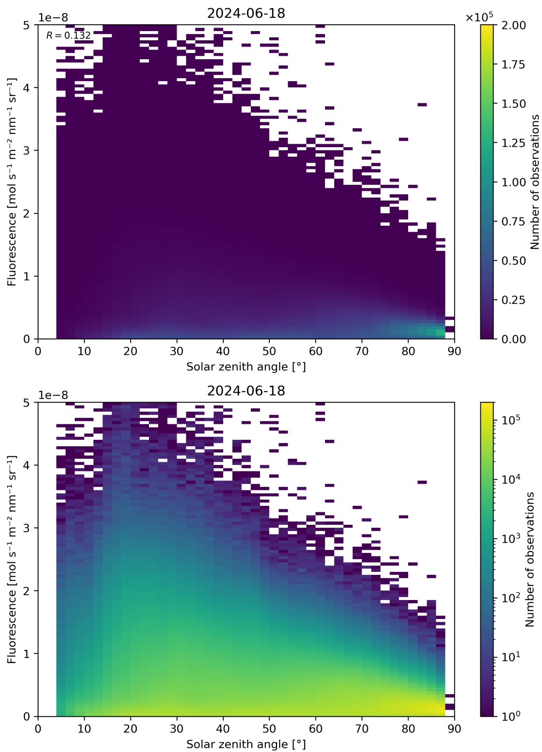
Figure 112: Scatter density plot of “Solar zenith angle” against “Fluorescence” for 2024-06-17 to 2024-06-19.
