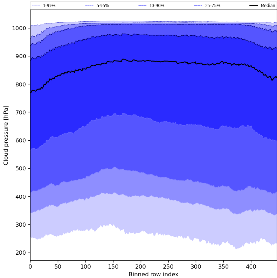
Figure 47: Along track statistics of “Cloud pressure” for 2024-06-17 to 2024-06-19
