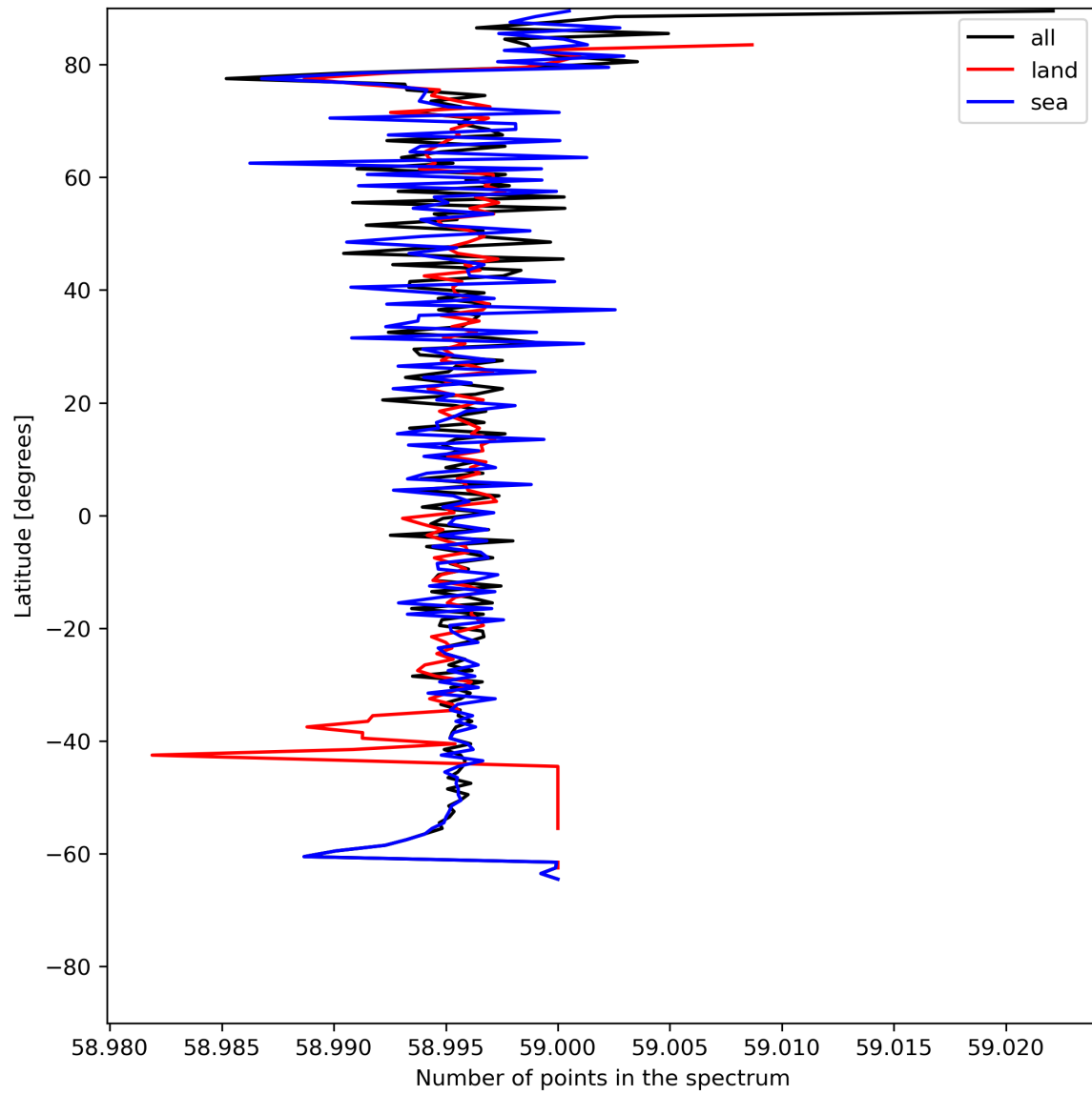
Figure 27: Zonal average of “Number of points in the spectrum” for 2024-06-17 to 2024-06-19.
