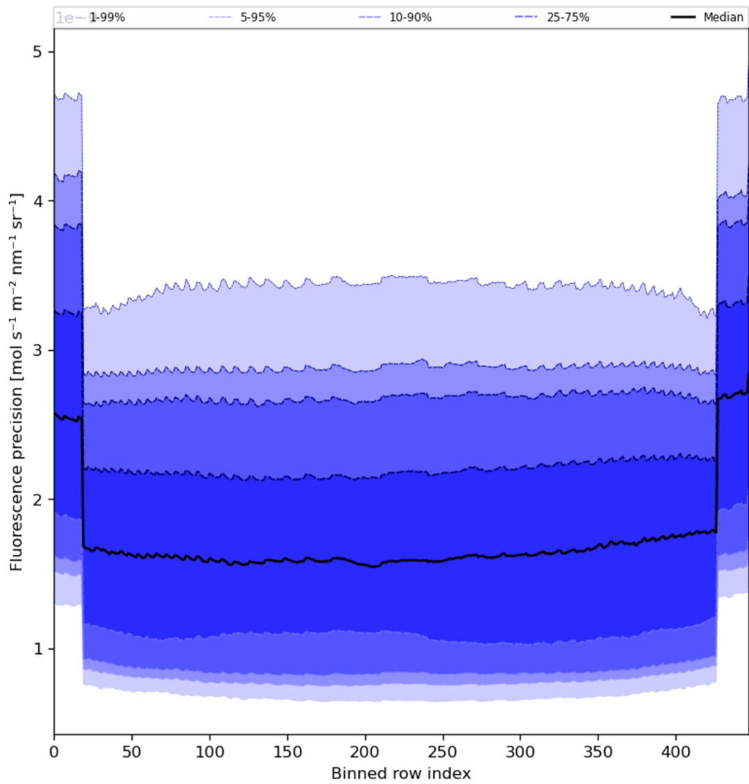
Figure 58: Along track statistics of “Fluorescence precision” for 2024-06-17 to 2024-06-19
