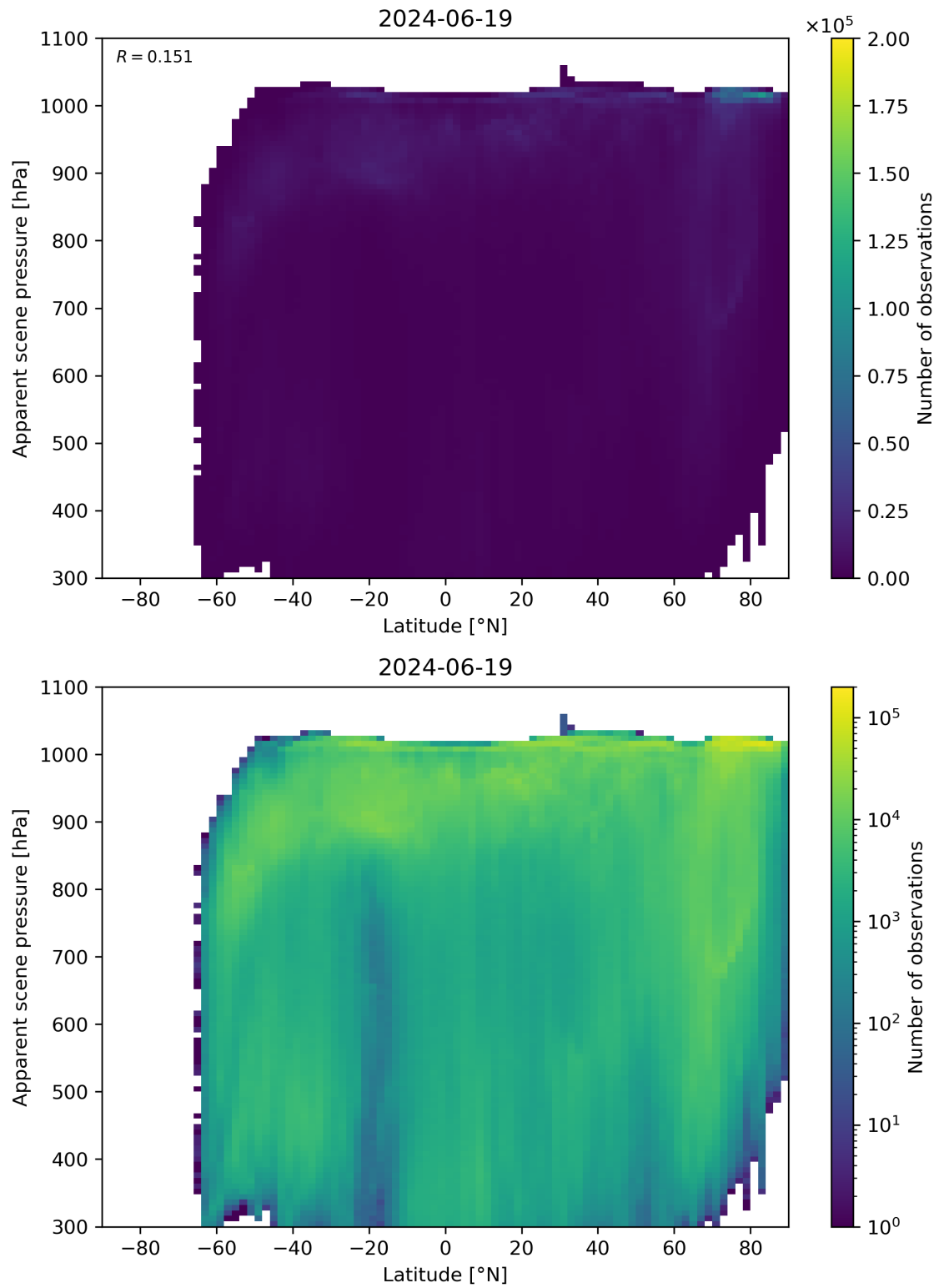
Figure 88: Scatter density plot of “Latitude” against “Apparent scene pressure” for 2024-06-19 to 2024-06-20.
