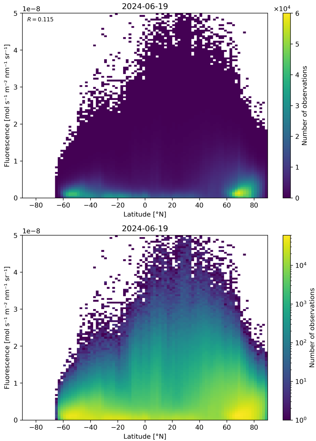
Figure 92: Scatter density plot of “Latitude” against “Fluorescence” for 2024-06-19 to 2024-06-20.
