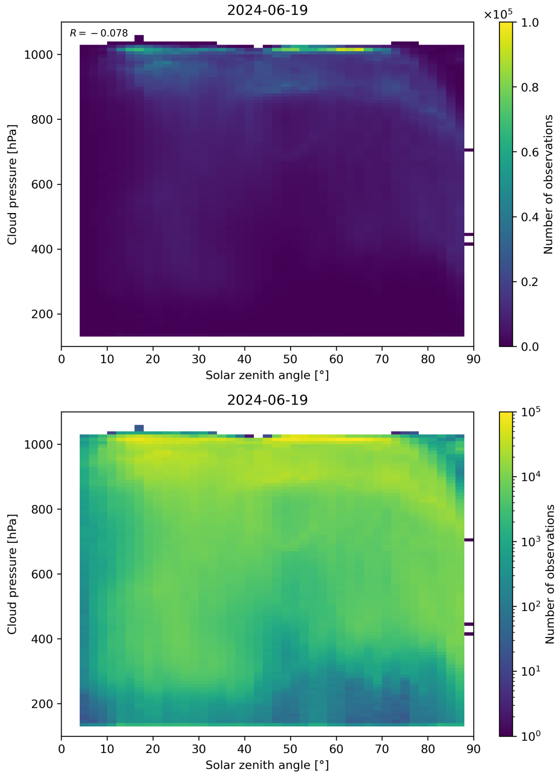
Figure 111: Scatter density plot of “Solar zenith angle” against “Cloud pressure” for 2024-06-19 to 2024-06-20.
