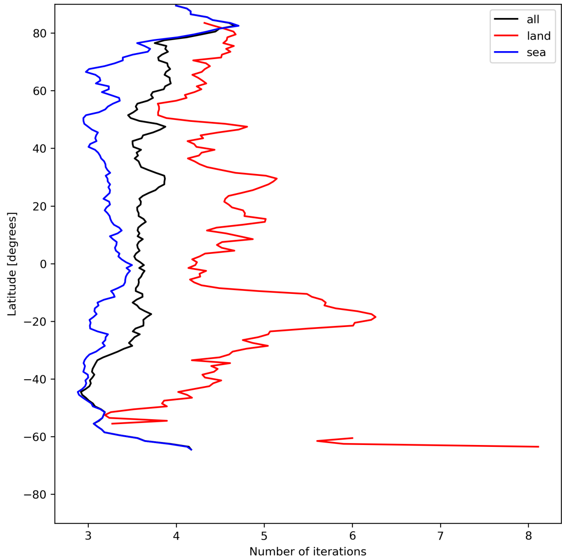
Figure 22: Zonal average of “Number of iterations” for 2024-06-19 to 2024-06-20.
