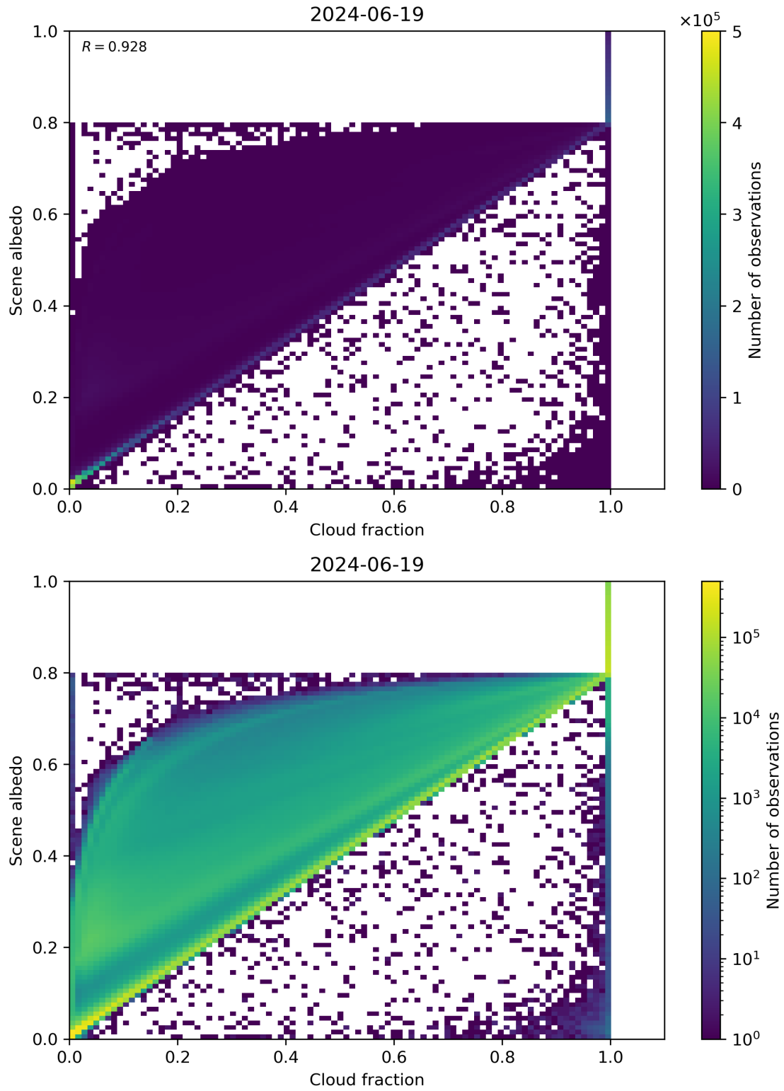
Figure 75: Scatter density plot of “Cloud fraction” against “Scene albedo” for 2024-06-19 to 2024-06-20.
