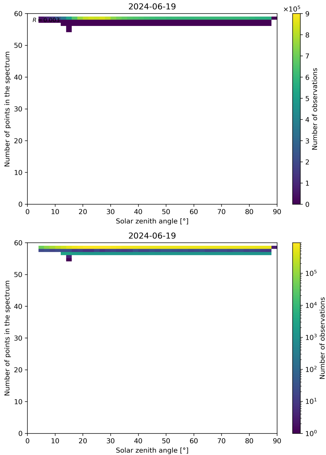
Figure 115: Scatter density plot of “Solar zenith angle” against “Number of points in the spectrum” for 2024-06-19 to 2024-06-20.
