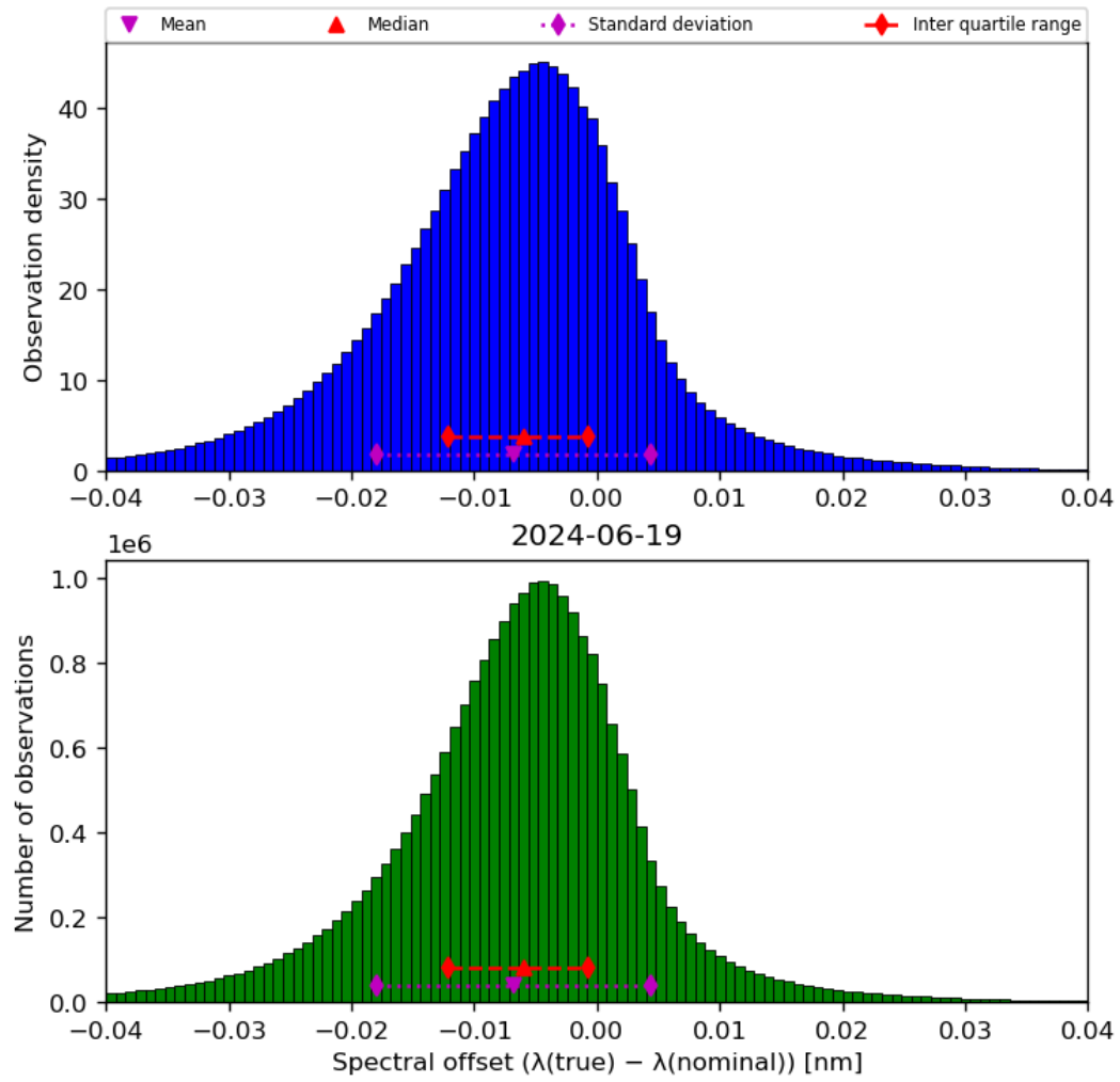
Figure 45: Histogram of “Spectral offset ( \lambda(\text{true}) - \lambda(\text{nominal}) )” for 2024-06-19 to 2024-06-20
