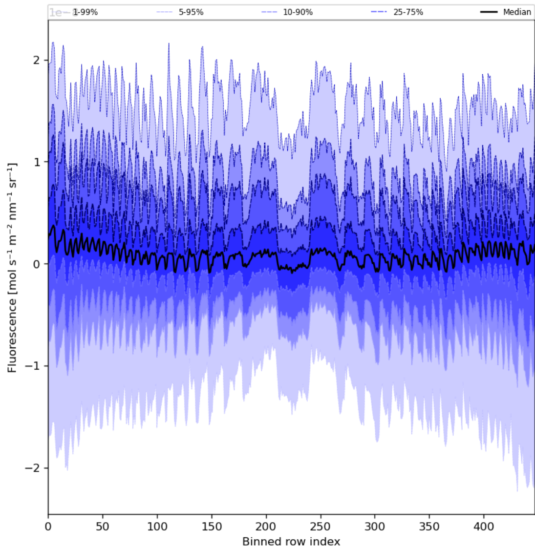
Figure 57: Along track statistics of “Fluorescence” for 2024-06-19 to 2024-06-20
