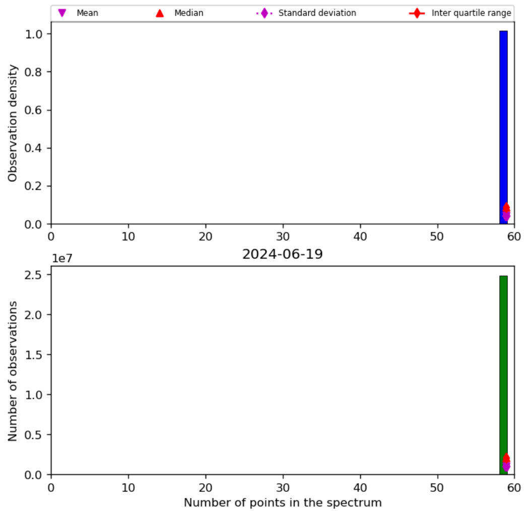
Figure 44: Histogram of “Number of points in the spectrum” for 2024-06-19 to 2024-06-20
