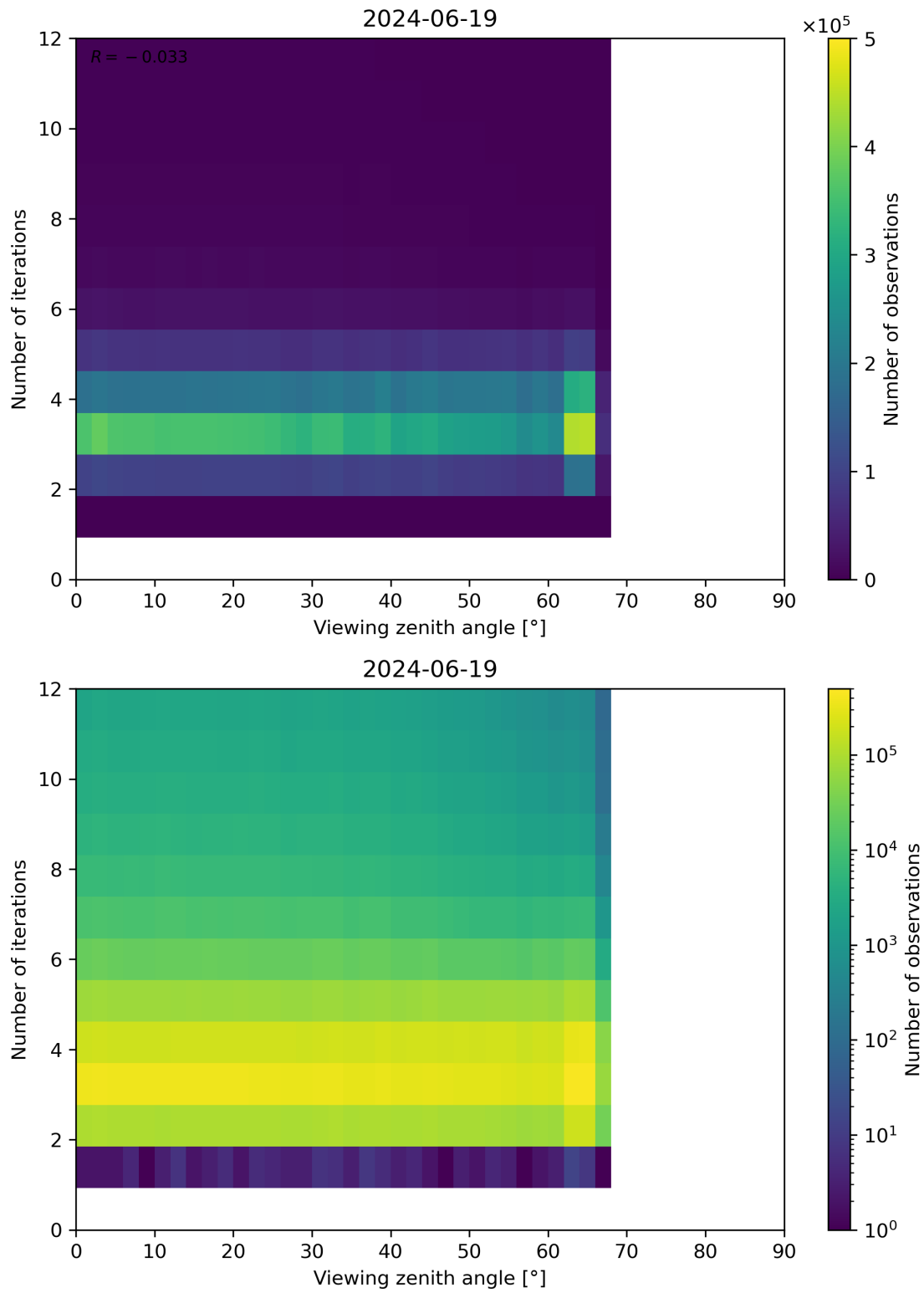
Figure 124: Scatter density plot of “Viewing zenith angle” against “Number of iterations” for 2024-06-19 to 2024-06-20.
