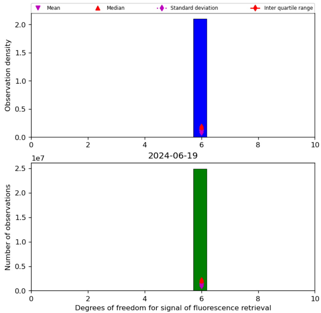
Figure 43: Histogram of “Degrees of freedom for signal of fluorescence retrieval” for 2024-06-19 to 2024-06-20
