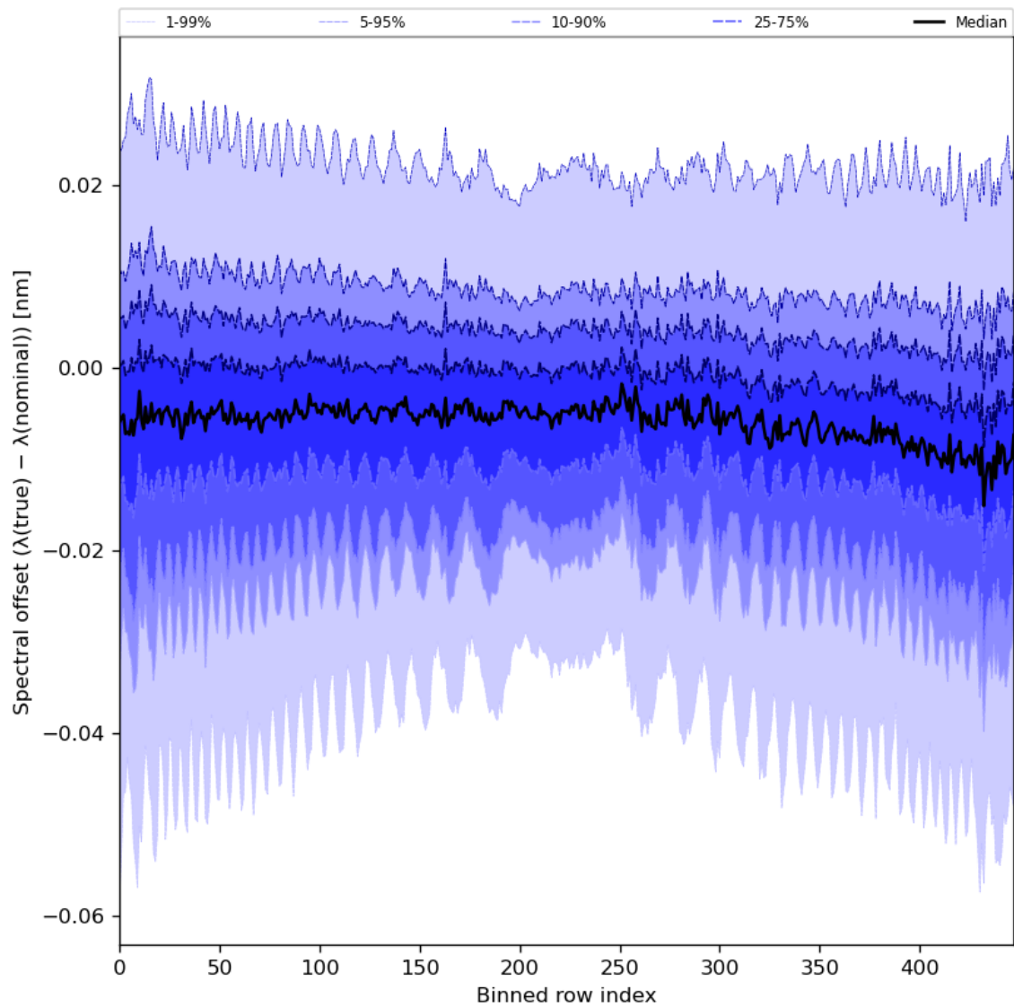
Figure 62: Along track statistics of “Spectral offset ( \lambda(\text{true}) - \lambda(\text{nominal}) )” for 2024-06-19 to 2024-06-20
