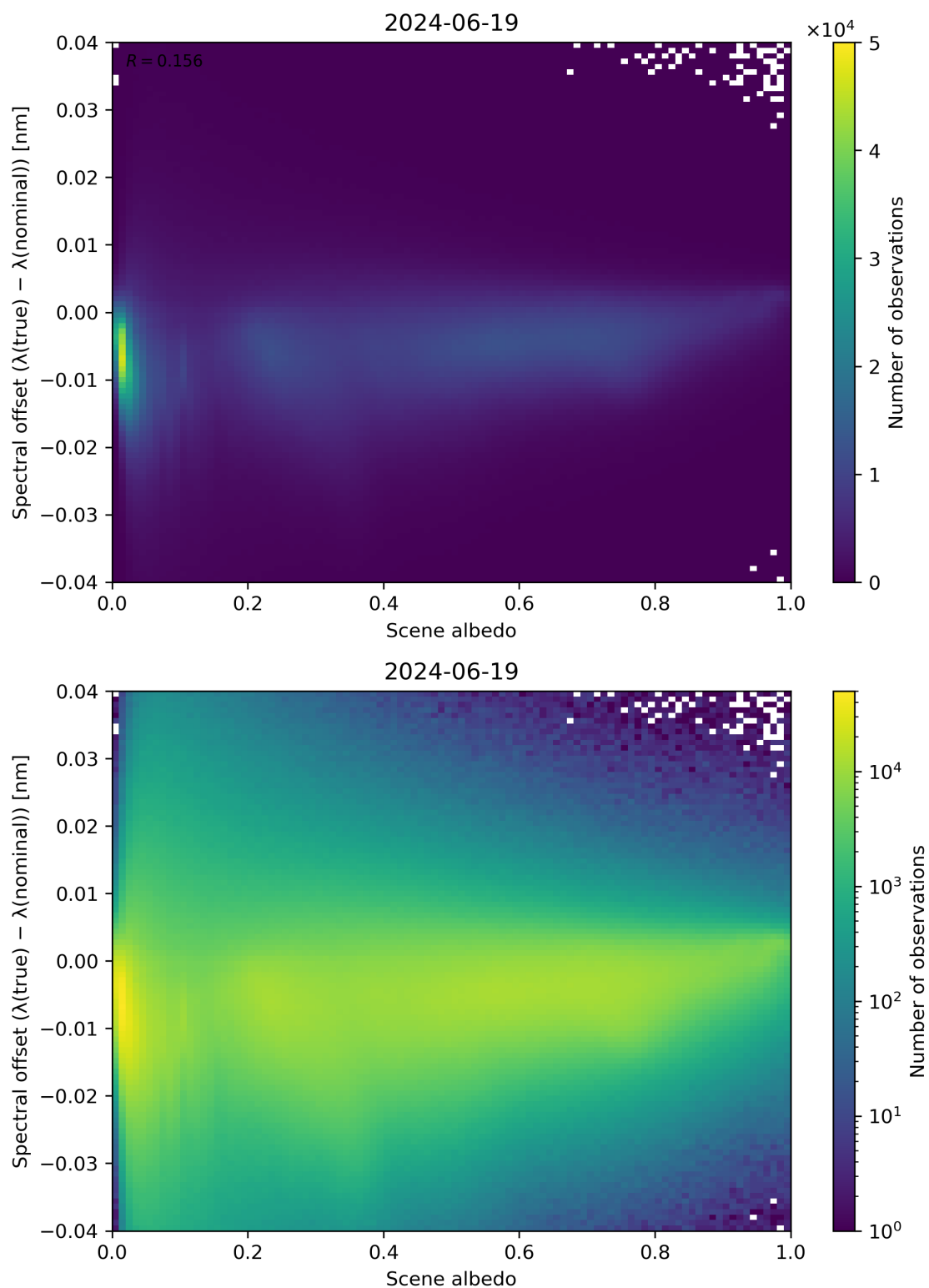
Figure 107: Scatter density plot of “Scene albedo” against “Spectral offset ( \lambda(\text{true}) - \lambda(\text{nominal}) )” for 2024-06-19 to 2024-06-20.
