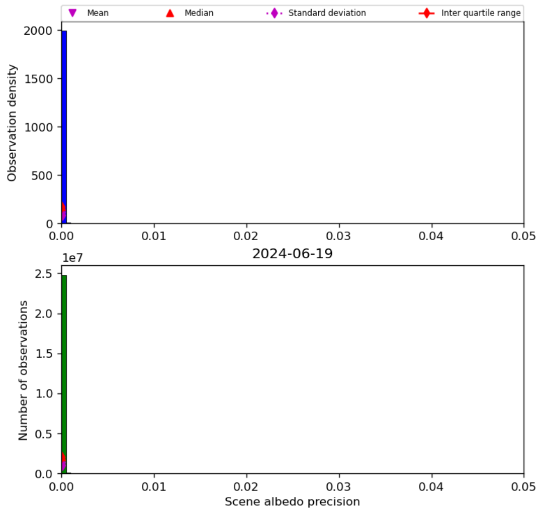
Figure 35: Histogram of “Scene albedo precision” for 2024-06-19 to 2024-06-20
