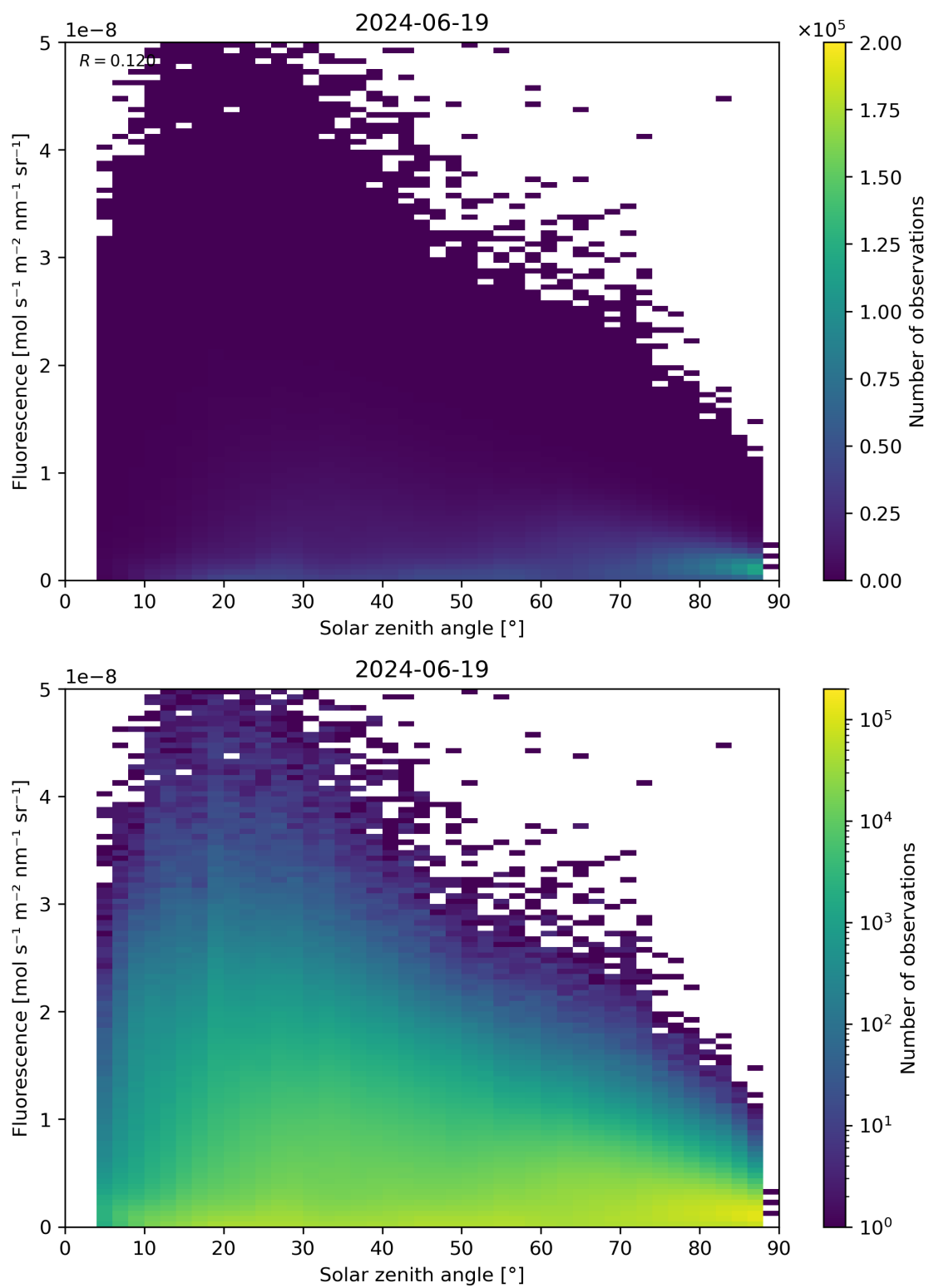
Figure 112: Scatter density plot of “Solar zenith angle” against “Fluorescence” for 2024-06-19 to 2024-06-20.
