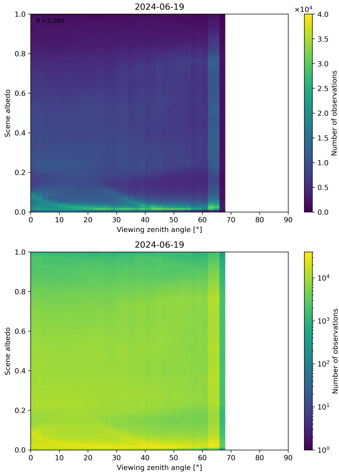
Figure 126: Scatter density plot of “Viewing zenith angle” against “Scene albedo” for 2024-06-19 to 2024-06-20.
