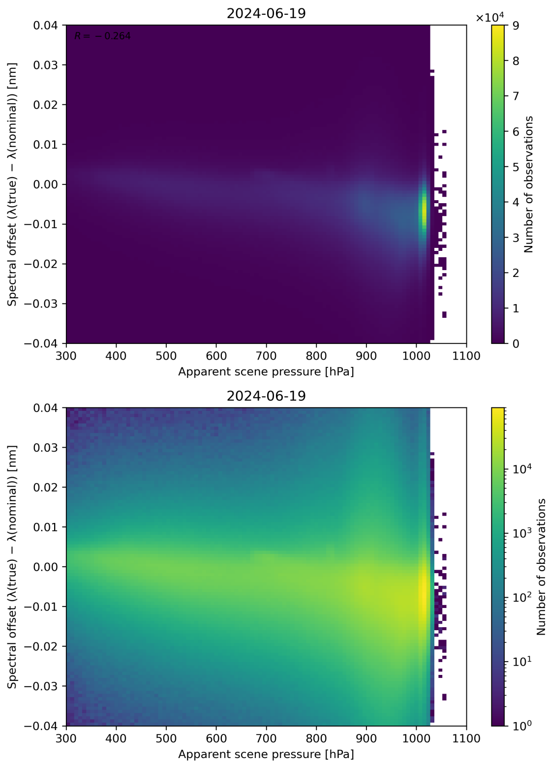
Figure 67: Scatter density plot of “Apparent scene pressure” against “Spectral offset ( \lambda(\text{true}) - \lambda(\text{nominal}) )” for 2024-06-19 to 2024-06-20.
