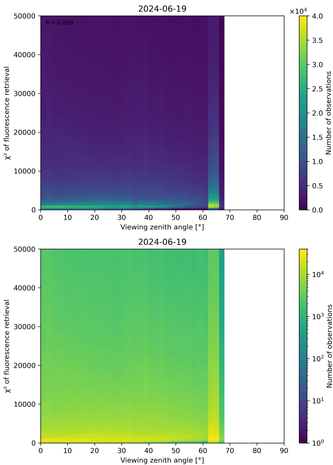
Figure 119: Scatter density plot of “Viewing zenith angle” against “ \chi^2 of fluorescence retrieval” for 2024-06-19 to 2024-06-20.
