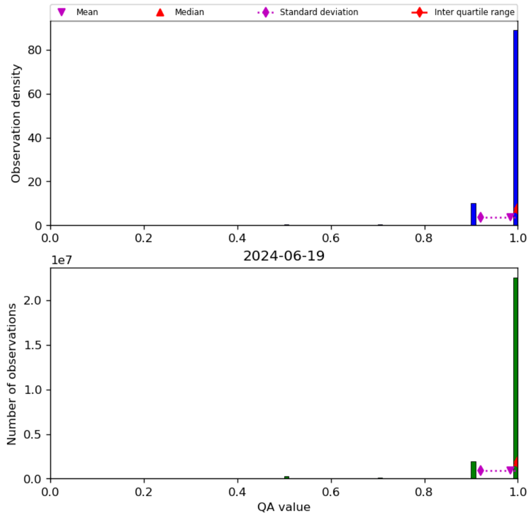
Figure 29: Histogram of “QA value” for 2024-06-19 to 2024-06-20
