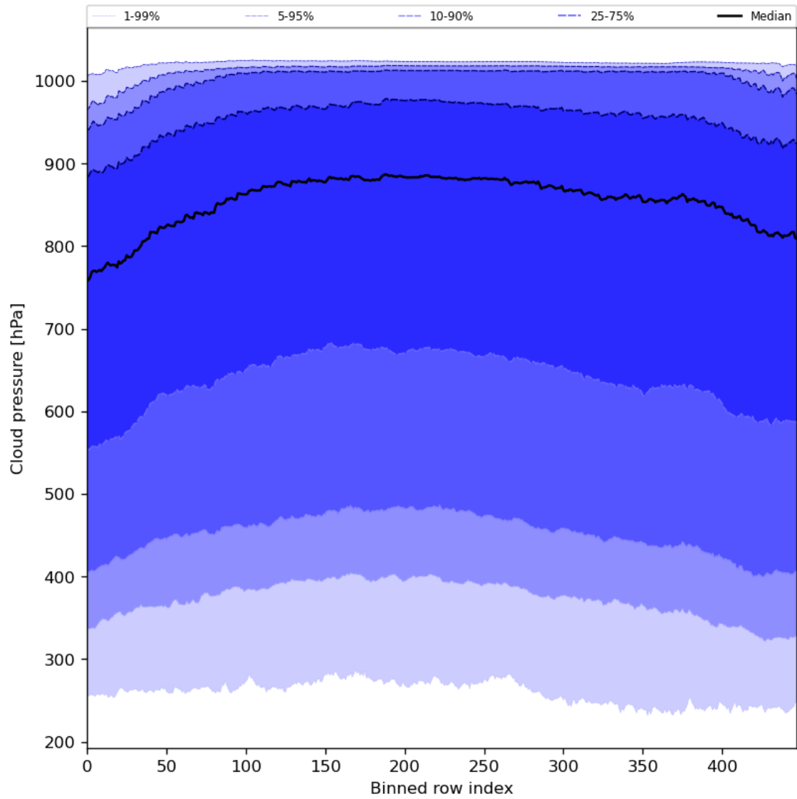
Figure 47: Along track statistics of “Cloud pressure” for 2024-06-19 to 2024-06-20
