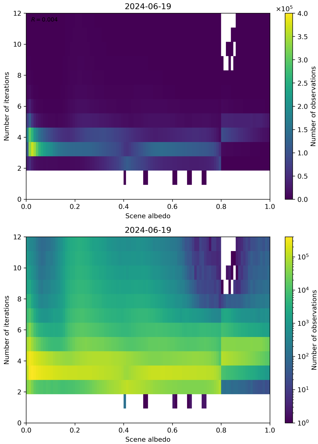
Figure 105: Scatter density plot of “Scene albedo” against “Number of iterations” for 2024-06-19 to 2024-06-20.
