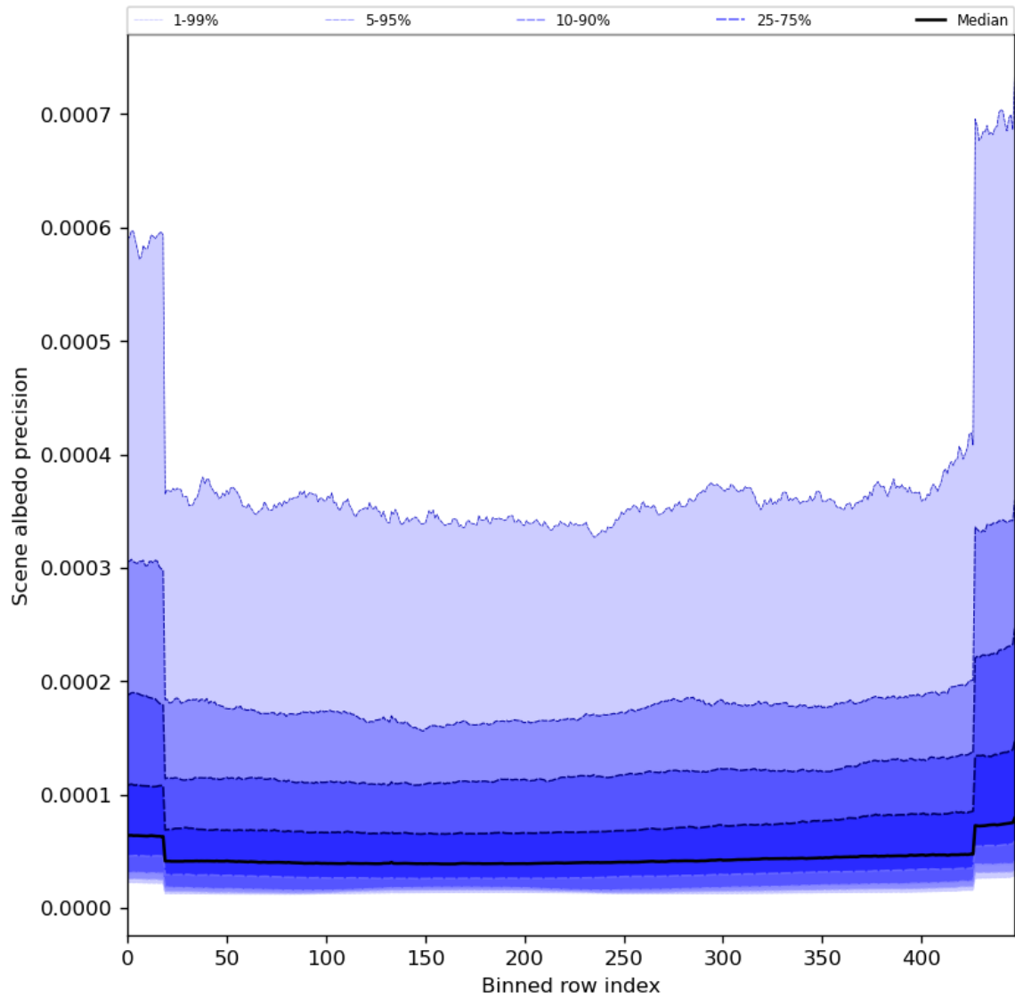
Figure 52: Along track statistics of “Scene albedo precision” for 2024-06-19 to 2024-06-20
