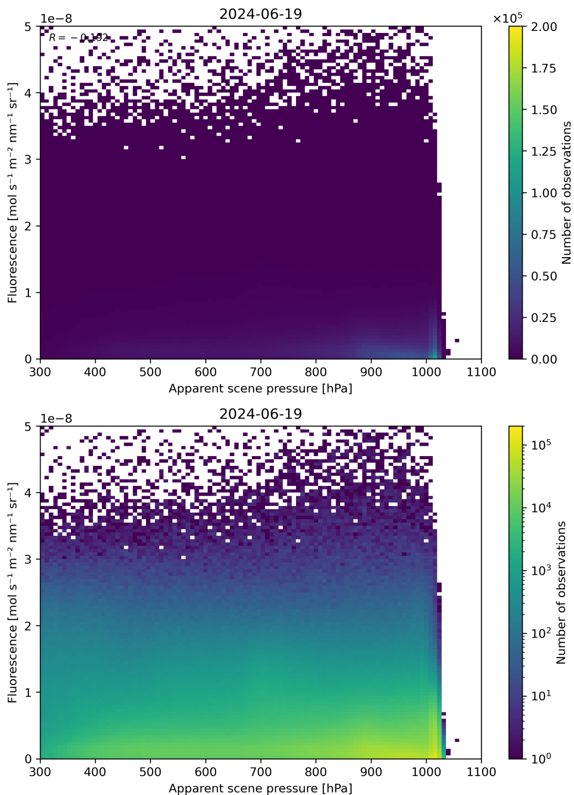
Figure 64: Scatter density plot of “Apparent scene pressure” against “Fluorescence” for 2024-06-19 to 2024-06-20.
