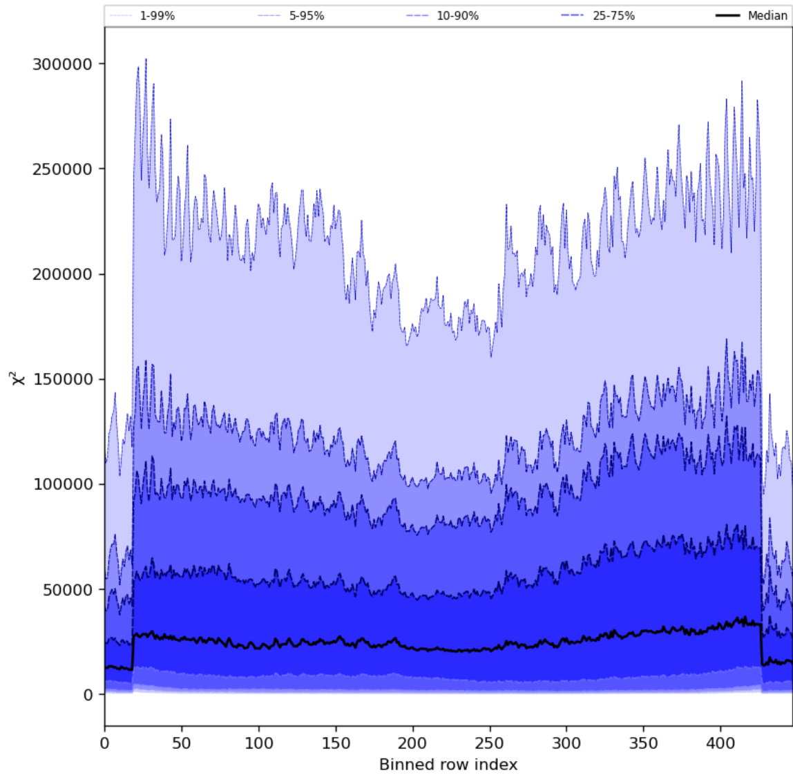
Figure 55: Along track statistics of “ \chi^2 ” for 2024-06-19 to 2024-06-20
