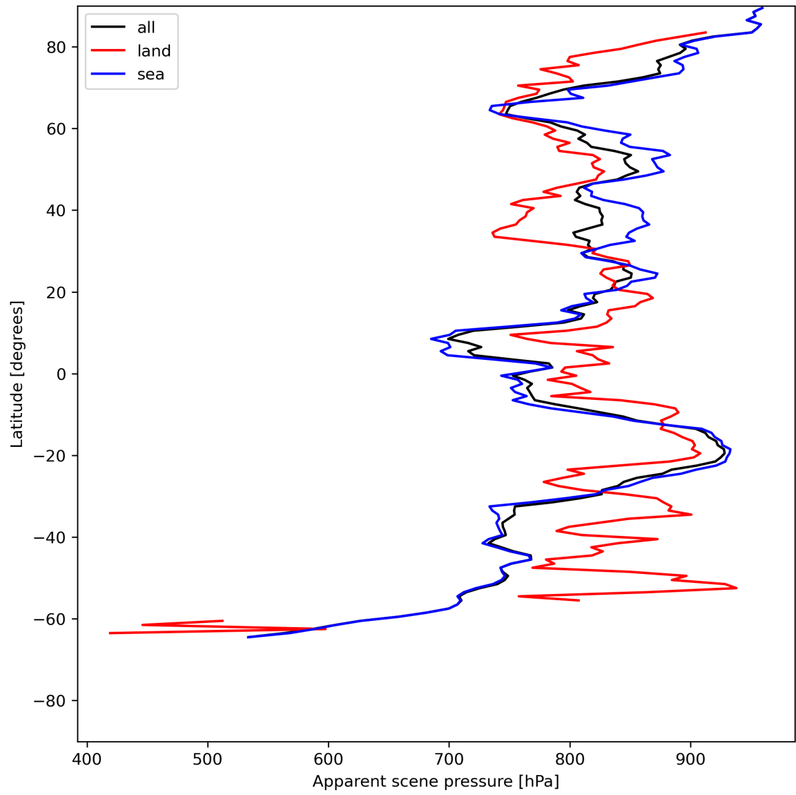
Figure 19: Zonal average of “Apparent scene pressure” for 2024-06-19 to 2024-06-20.
