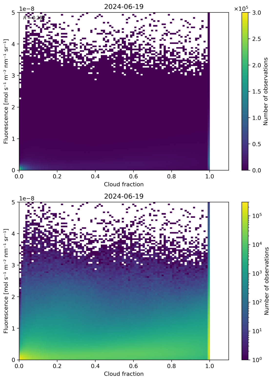
Figure 72: Scatter density plot of “Cloud fraction” against “Fluorescence” for 2024-06-19 to 2024-06-20.
