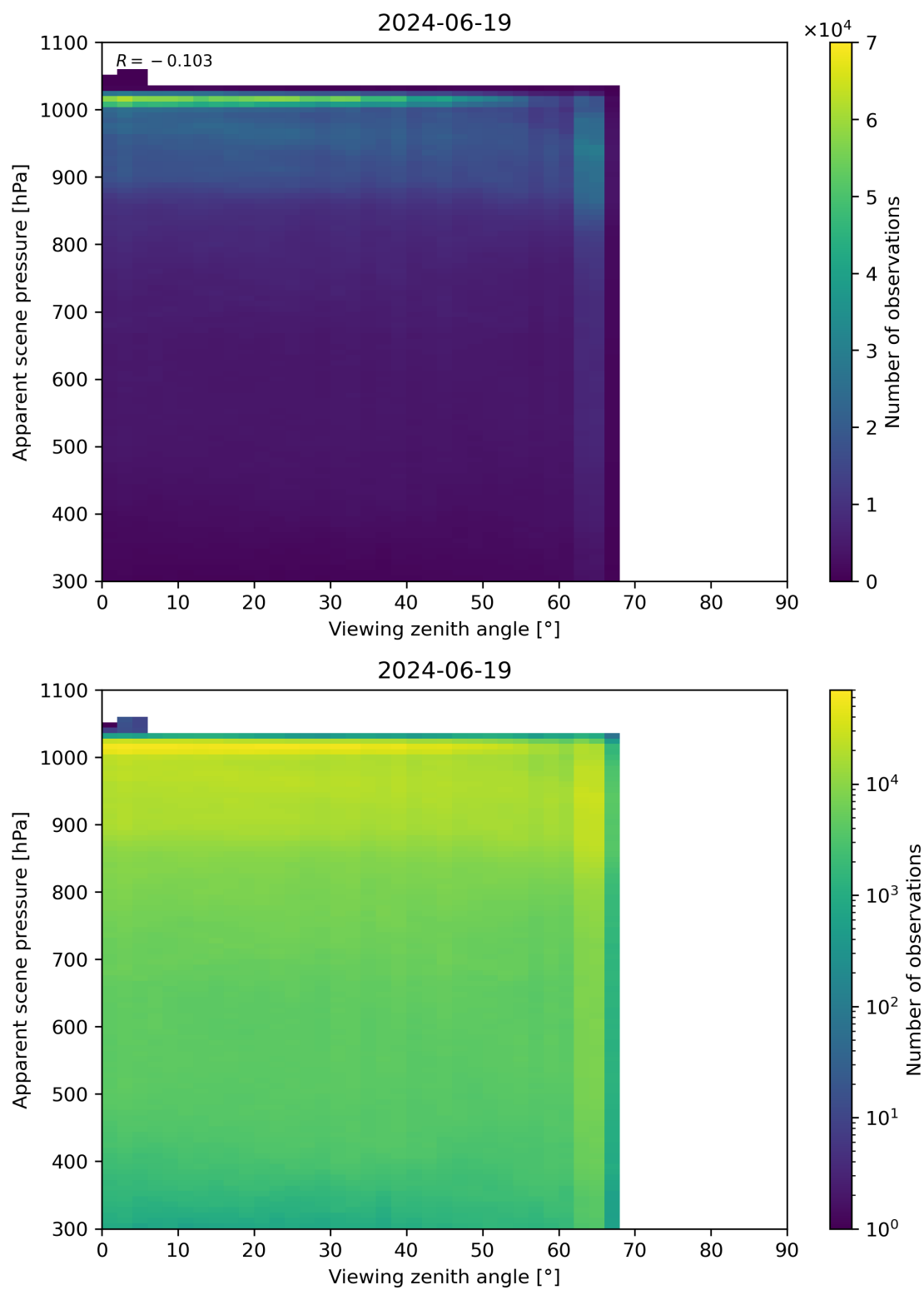
Figure 118: Scatter density plot of “Viewing zenith angle” against “Apparent scene pressure” for 2024-06-19 to 2024-06-20.
