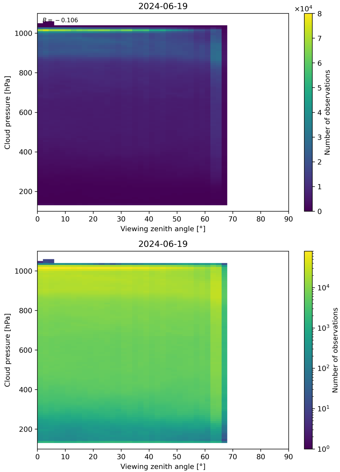
Figure 121: Scatter density plot of “Viewing zenith angle” against “Cloud pressure” for 2024-06-19 to 2024-06-20.
