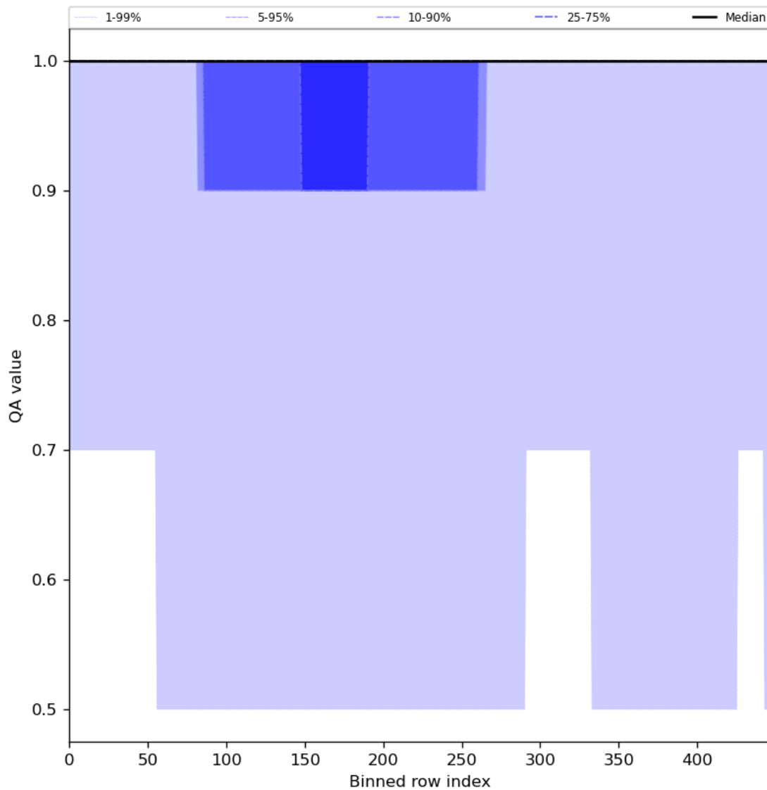
Figure 46: Along track statistics of “QA value” for 2024-06-19 to 2024-06-20
