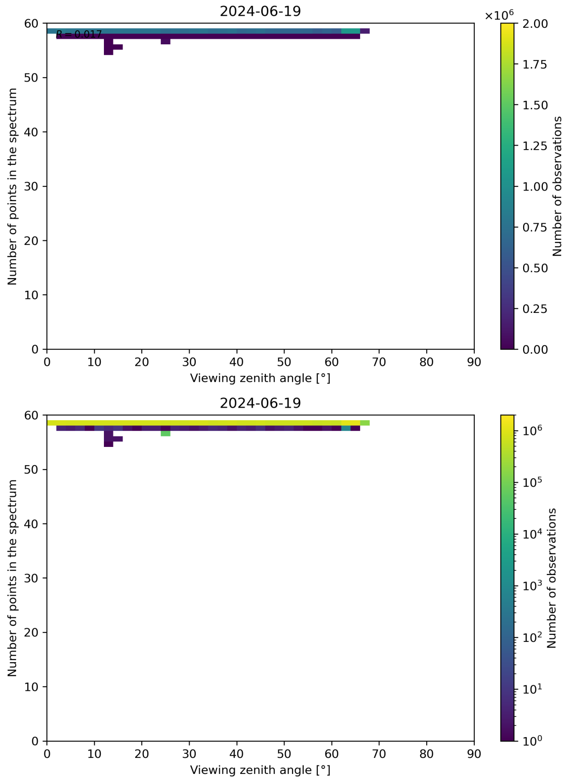
Figure 125: Scatter density plot of “Viewing zenith angle” against “Number of points in the spectrum” for 2024-06-19 to 2024-06-20.
