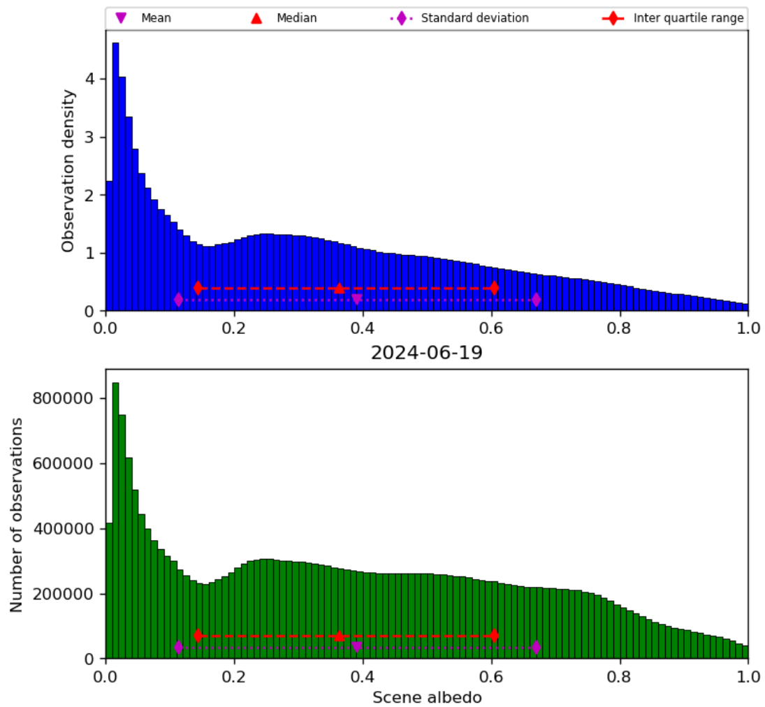
Figure 34: Histogram of “Scene albedo” for 2024-06-19 to 2024-06-20
