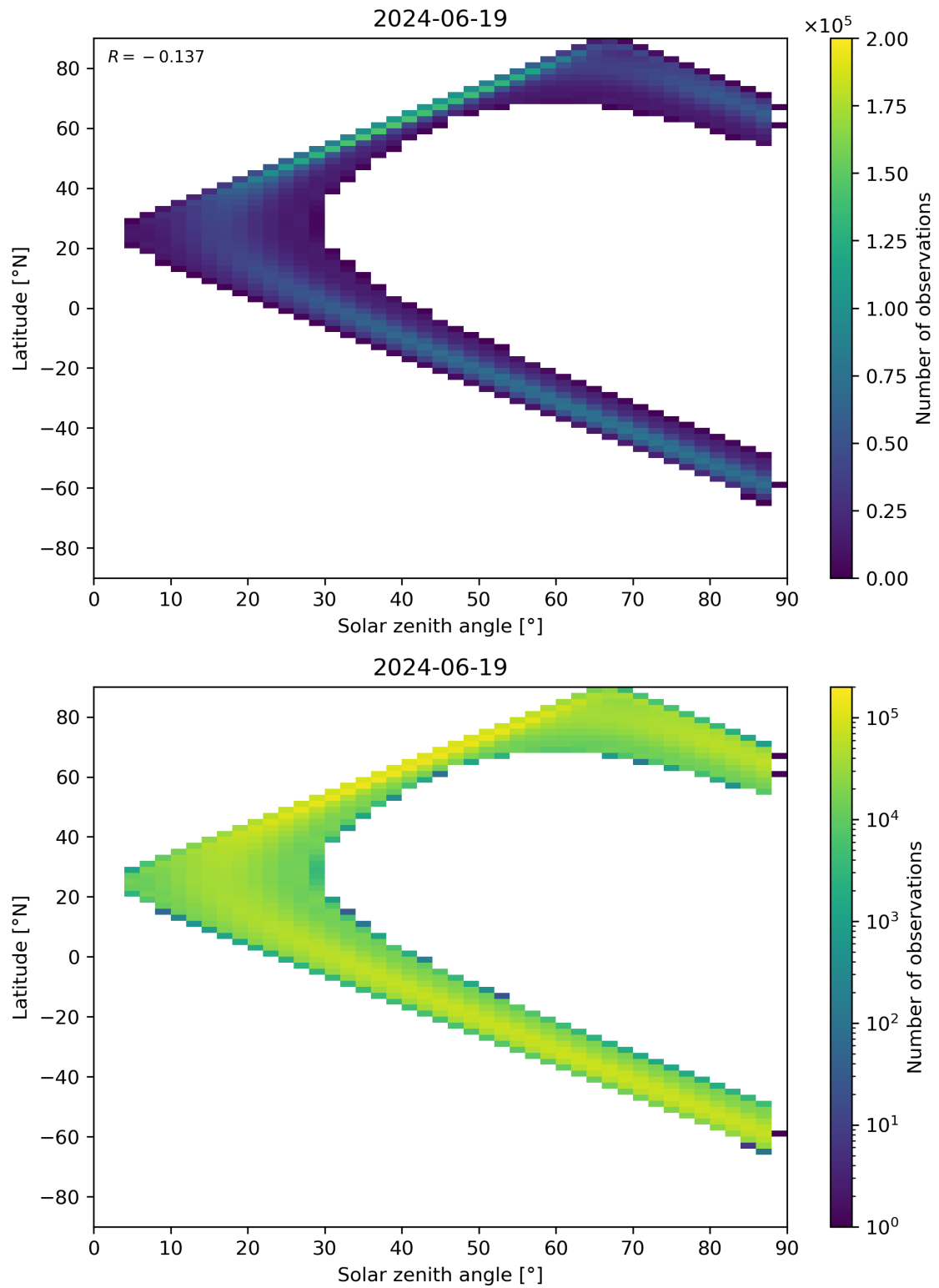
Figure 113: Scatter density plot of “Solar zenith angle” against “Latitude” for 2024-06-19 to 2024-06-20.
