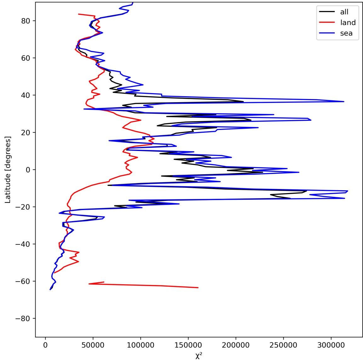
Figure 21: Zonal average of “ \chi^2 ” for 2024-06-19 to 2024-06-20.
