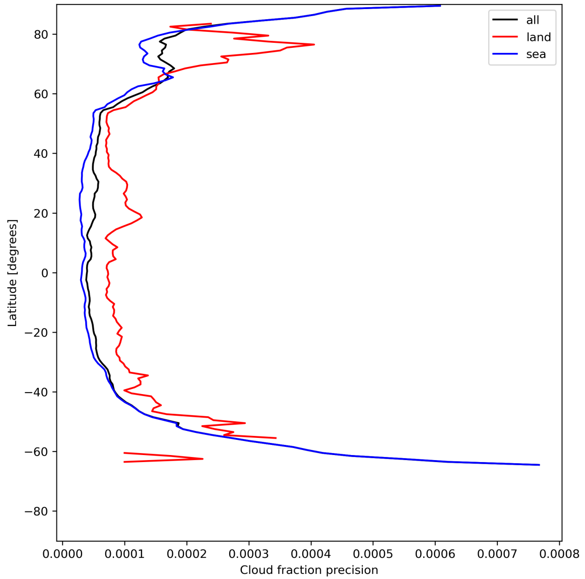
Figure 16: Zonal average of “Cloud fraction precision” for 2024-06-19 to 2024-06-20.
