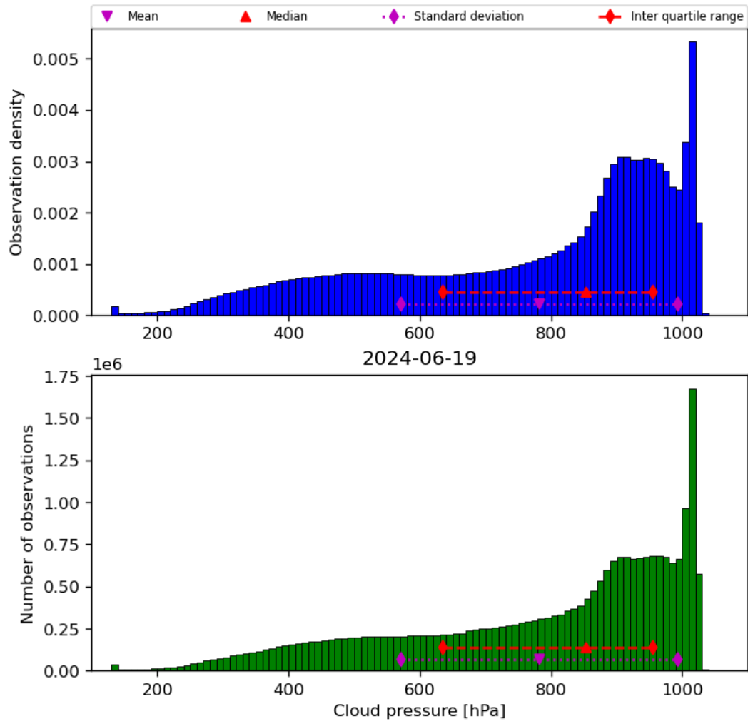
Figure 30: Histogram of “Cloud pressure” for 2024-06-19 to 2024-06-20
