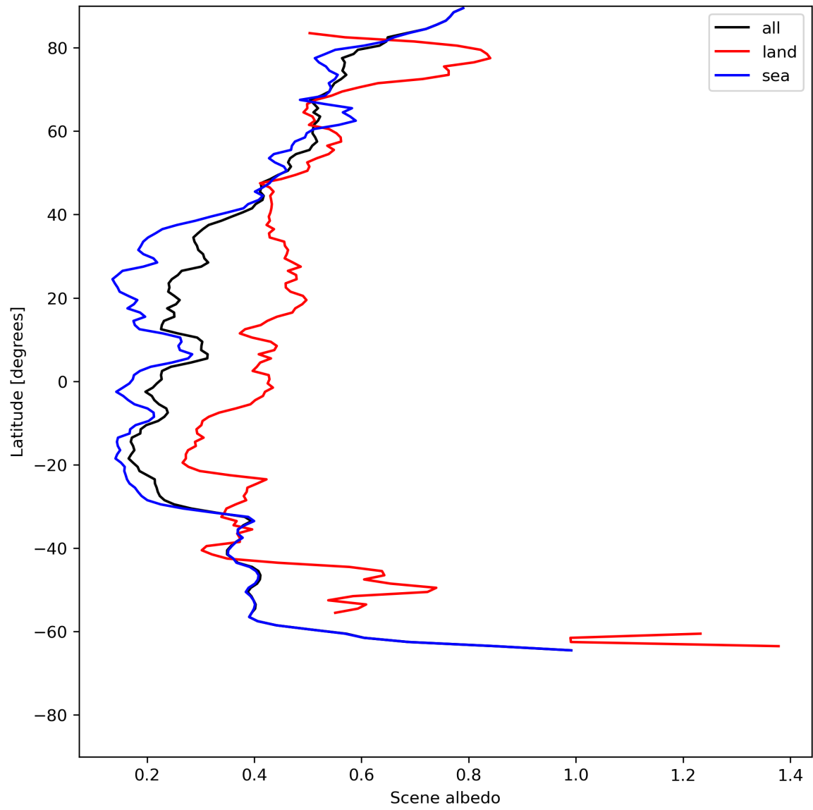
Figure 17: Zonal average of “Scene albedo” for 2024-06-19 to 2024-06-20.
