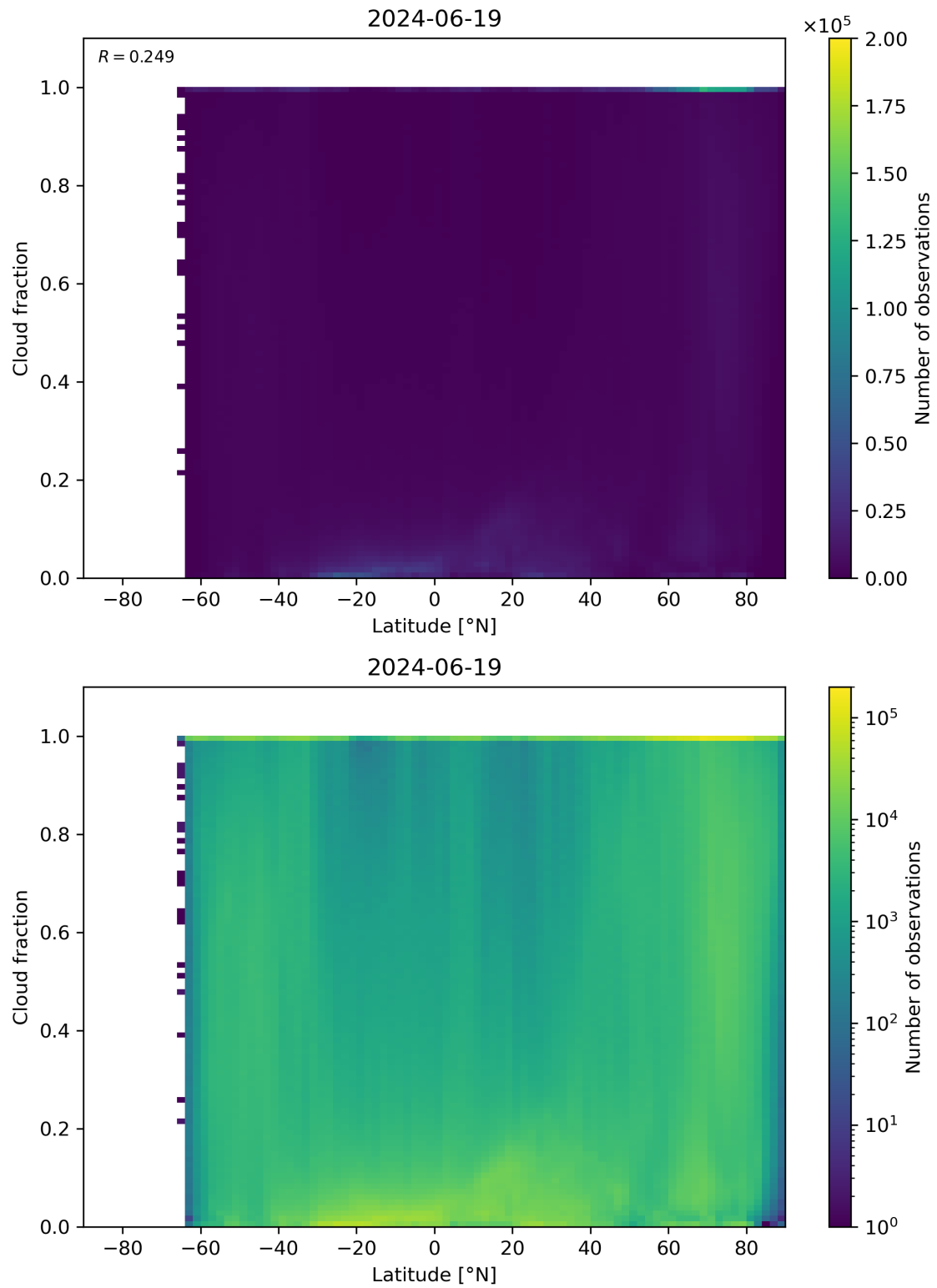
Figure 90: Scatter density plot of “Latitude” against “Cloud fraction” for 2024-06-19 to 2024-06-20.
