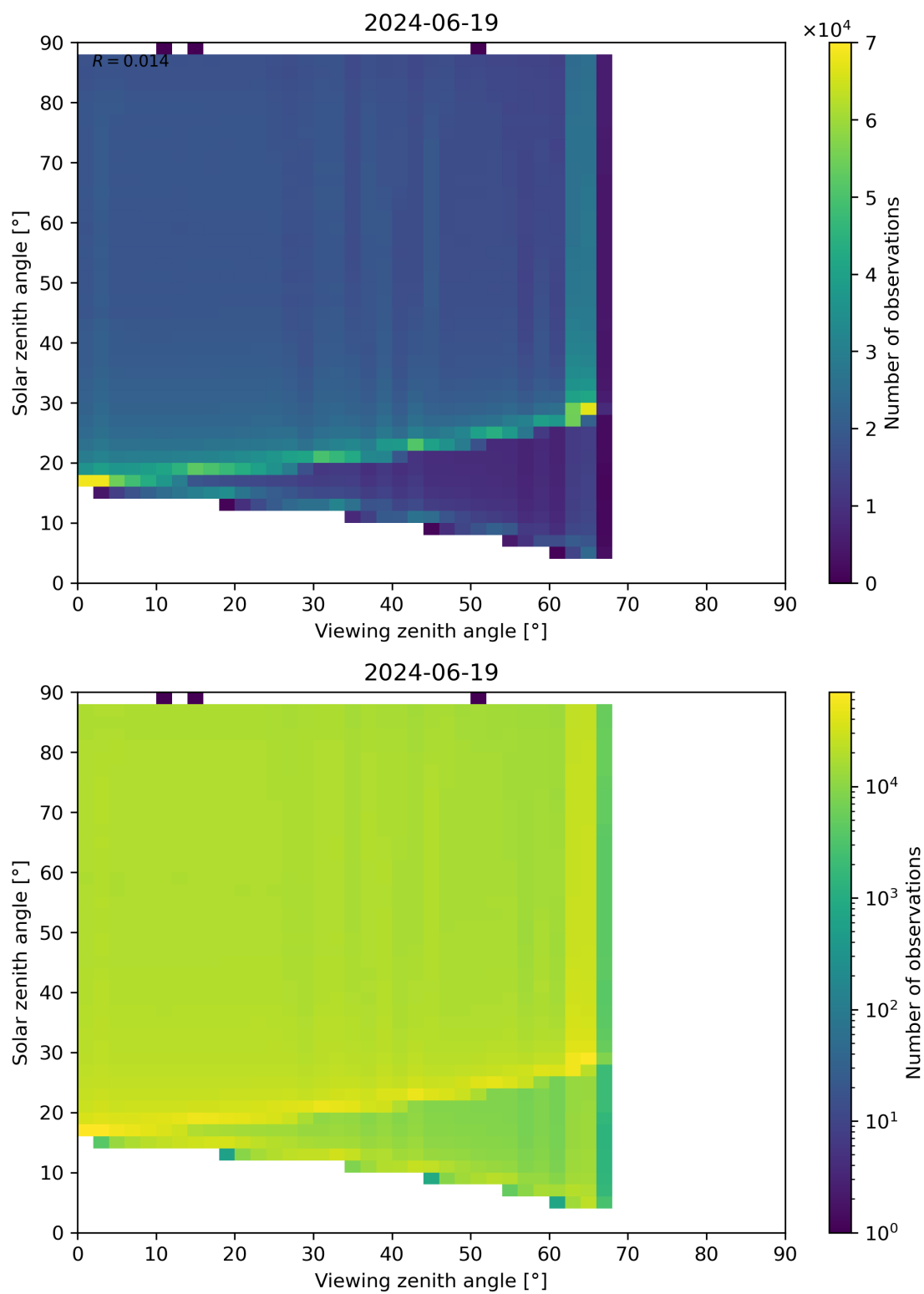
Figure 127: Scatter density plot of “Viewing zenith angle” against “Solar zenith angle” for 2024-06-19 to 2024-06-20.
