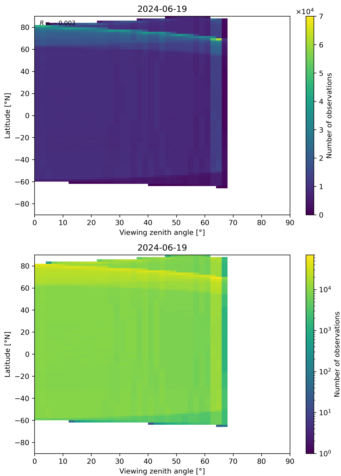
Figure 123: Scatter density plot of “Viewing zenith angle” against “Latitude” for 2024-06-19 to 2024-06-20.
