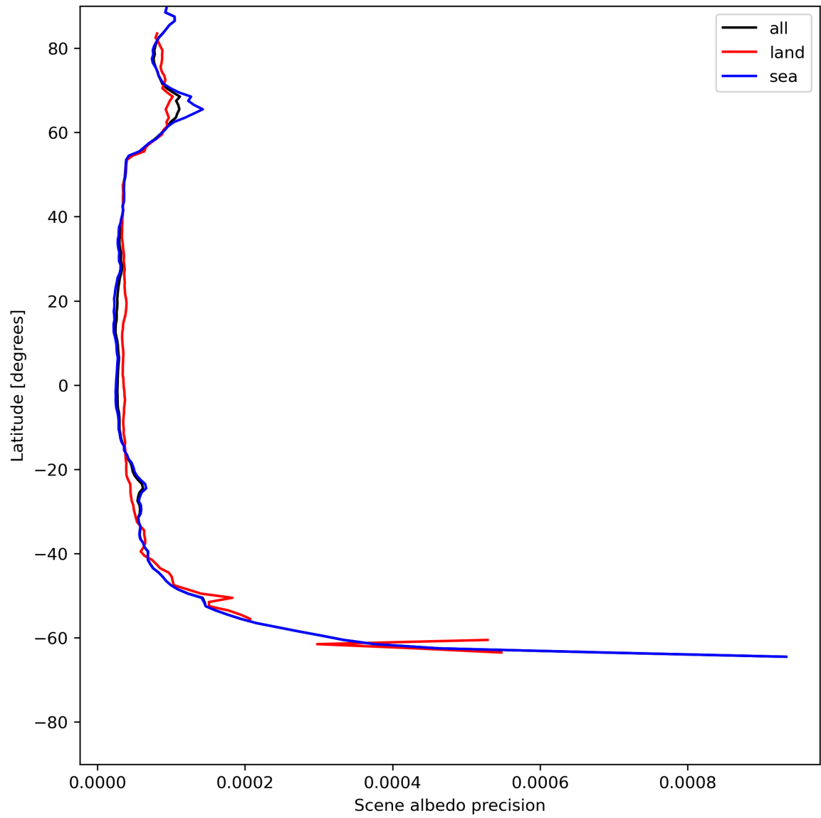
Figure 18: Zonal average of "Scene albedo precision" for 2024-06-19 to 2024-06-20.
