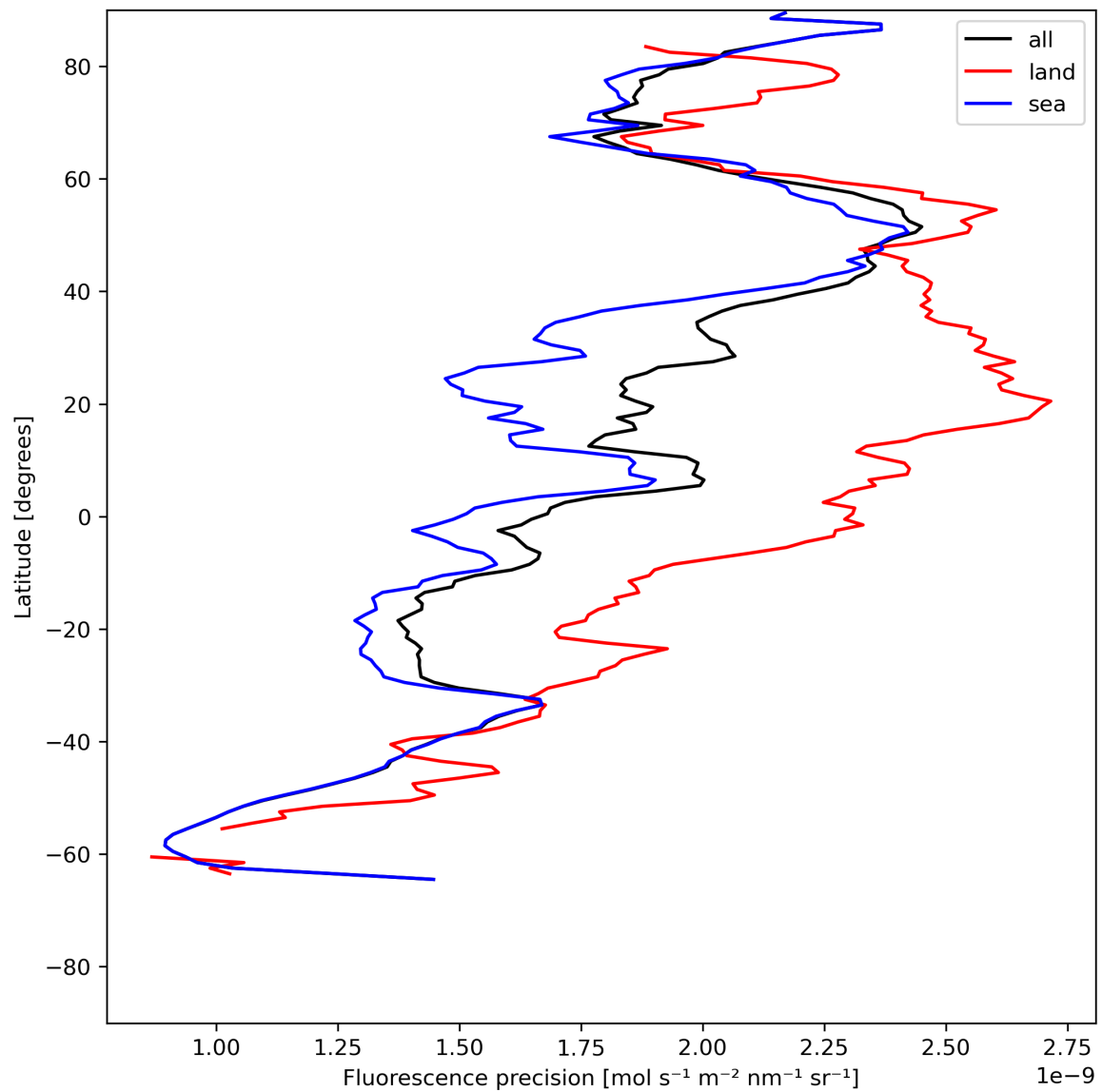
Figure 24: Zonal average of “Fluorescence precision” for 2024-06-19 to 2024-06-20.
