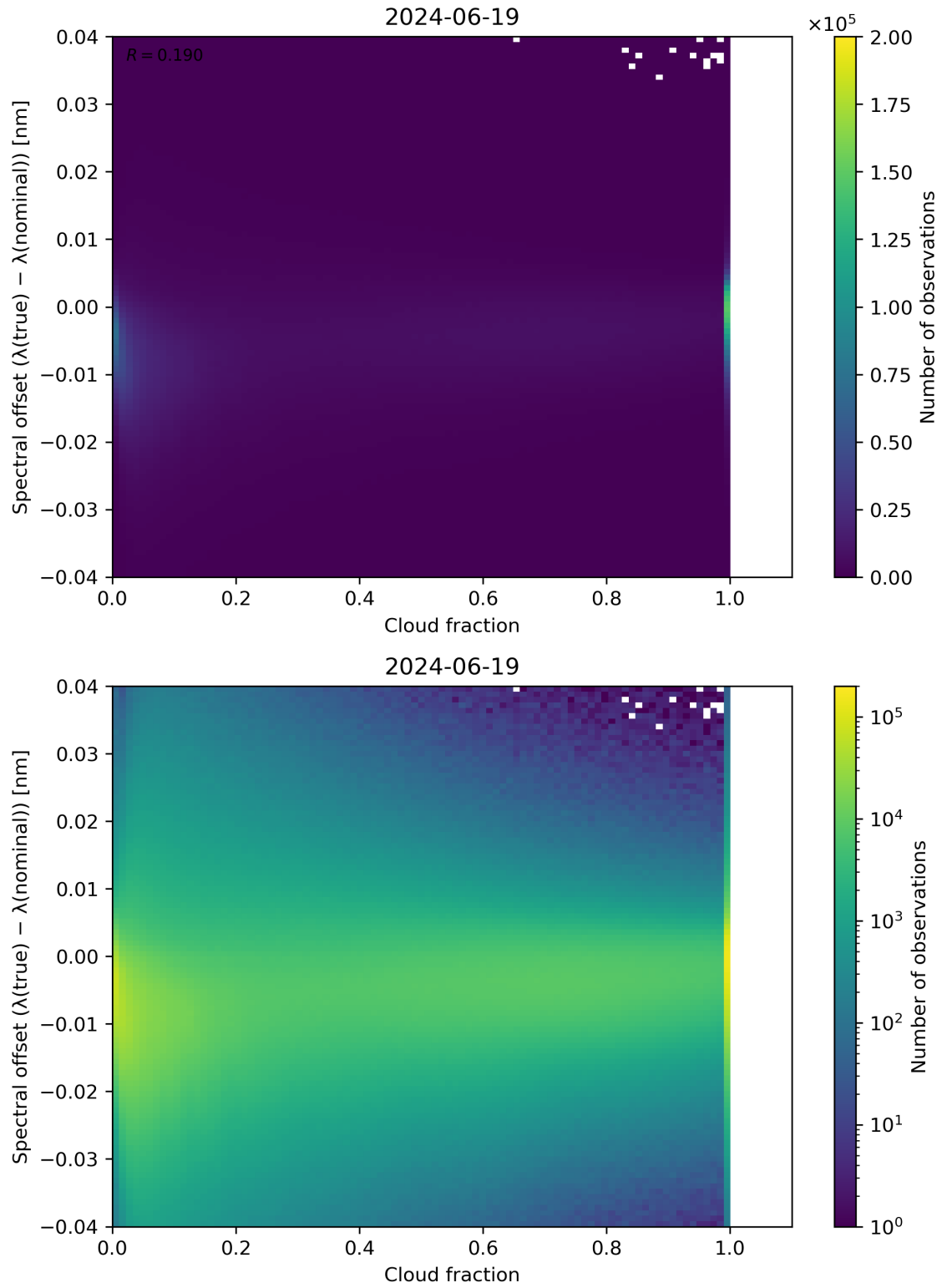
Figure 76: Scatter density plot of “Cloud fraction” against “Spectral offset ( \lambda(\text{true}) - \lambda(\text{nominal}) )” for 2024-06-19 to 2024-06-20.
