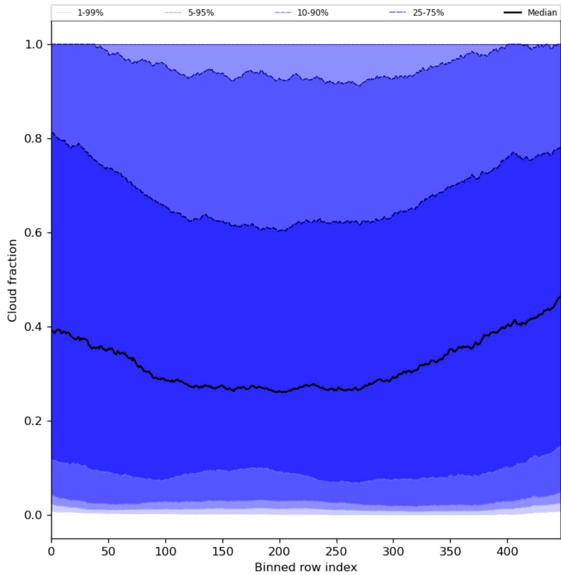
Figure 49: Along track statistics of “Cloud fraction” for 2024-06-19 to 2024-06-20
