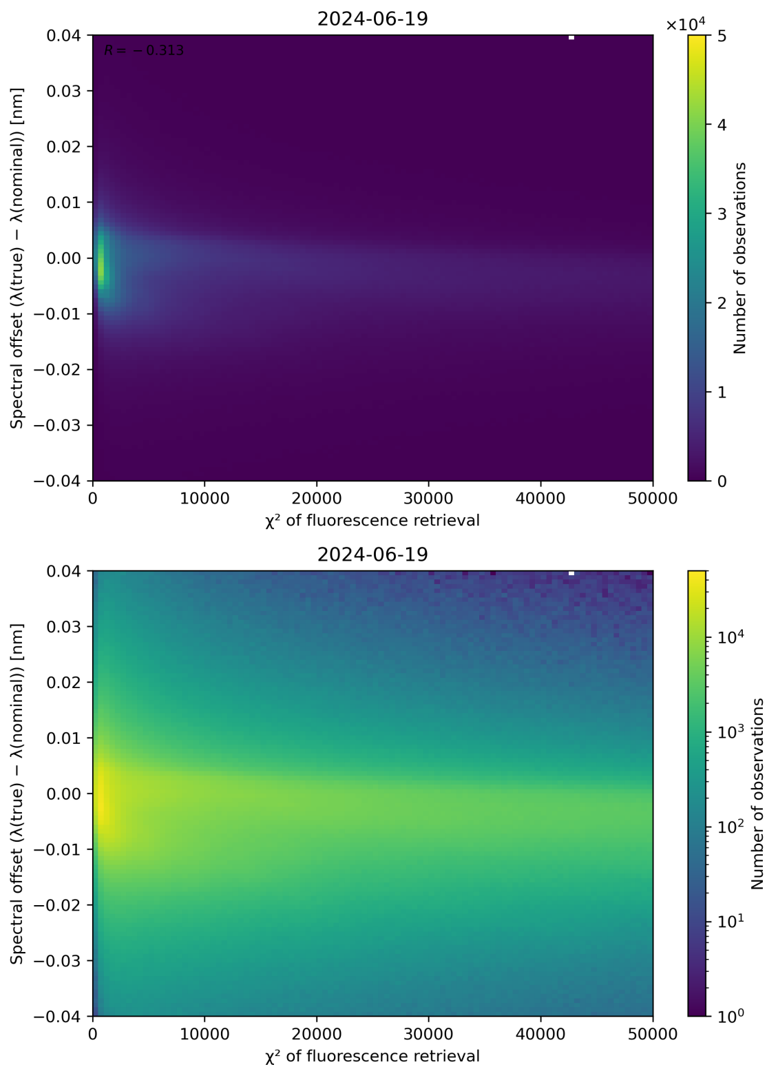
Figure 69: Scatter density plot of " \chi^2 of fluorescence retrieval" against "Spectral offset ( \lambda(\text{true}) - \lambda(\text{nominal})) " for 2024-06-19 to 2024-06-20.
