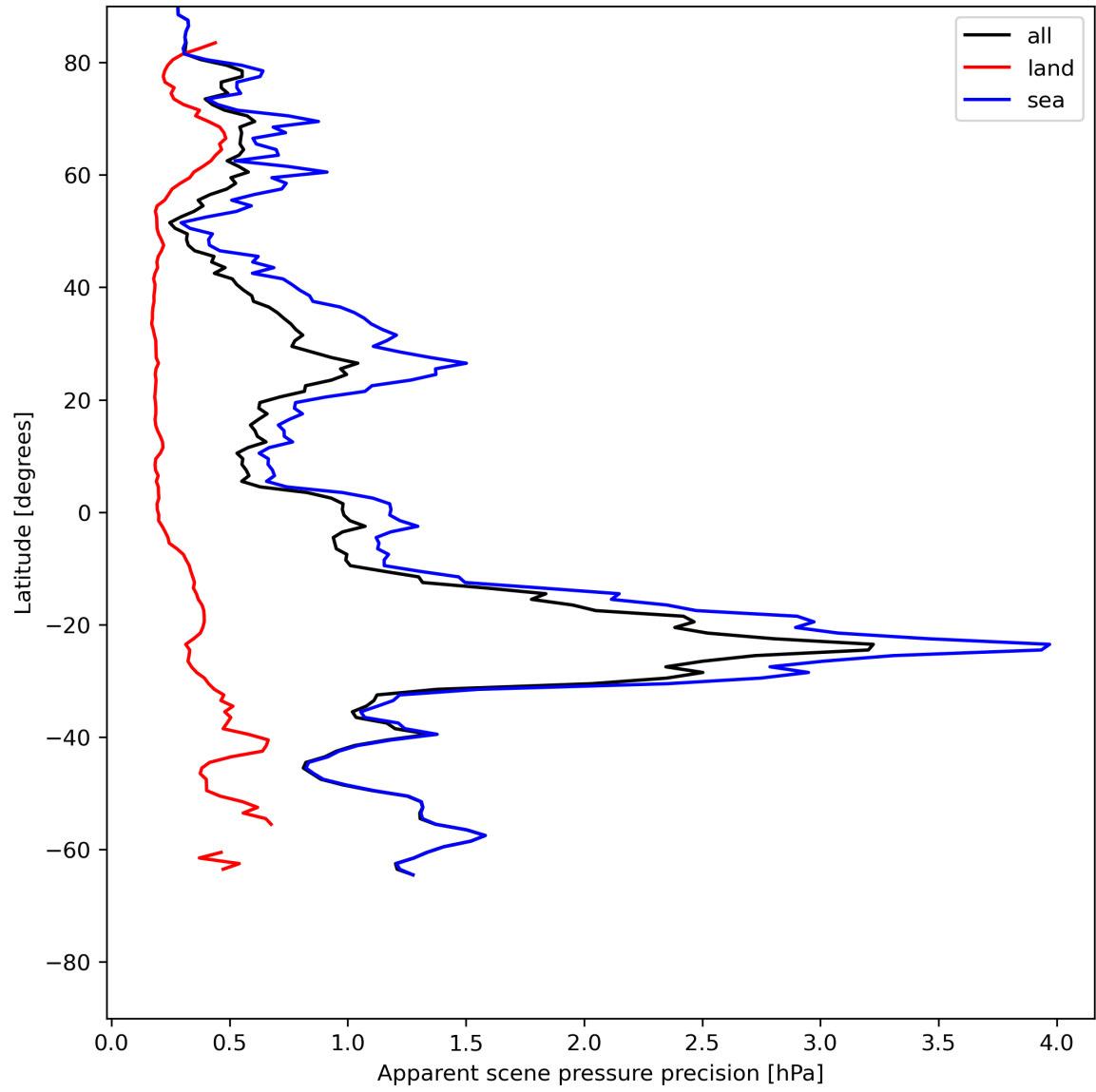
Figure 20: Zonal average of “Apparent scene pressure precision” for 2024-06-19 to 2024-06-20.
