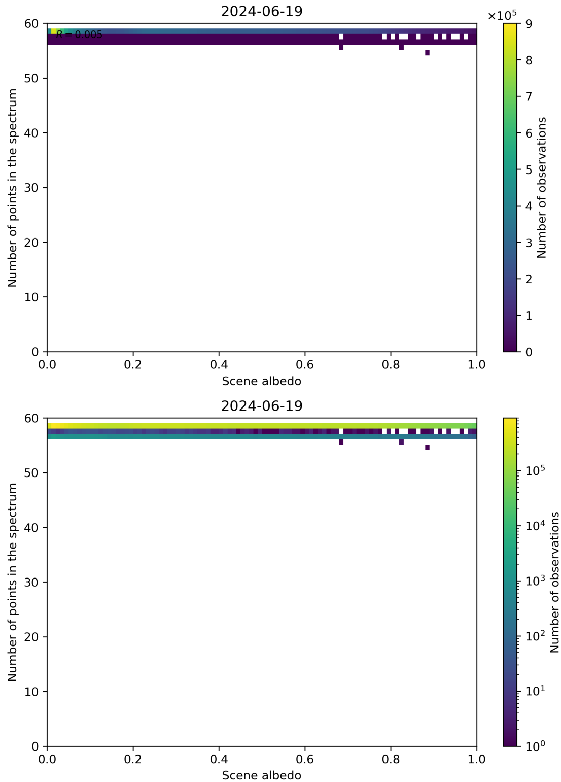
Figure 106: Scatter density plot of “Scene albedo” against “Number of points in the spectrum” for 2024-06-19 to 2024-06-20.
