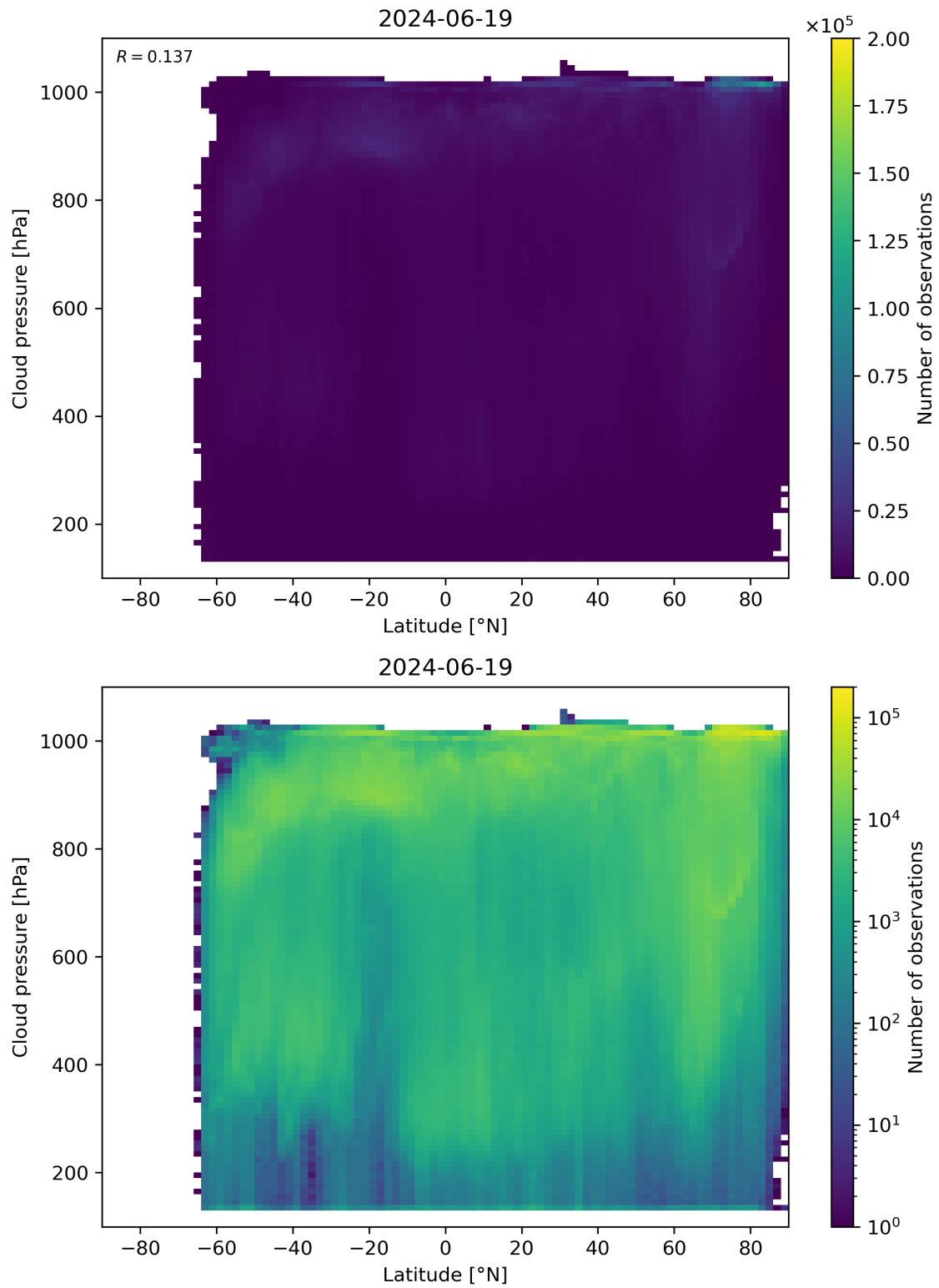
Figure 91: Scatter density plot of “Latitude” against “Cloud pressure” for 2024-06-19 to 2024-06-20.
