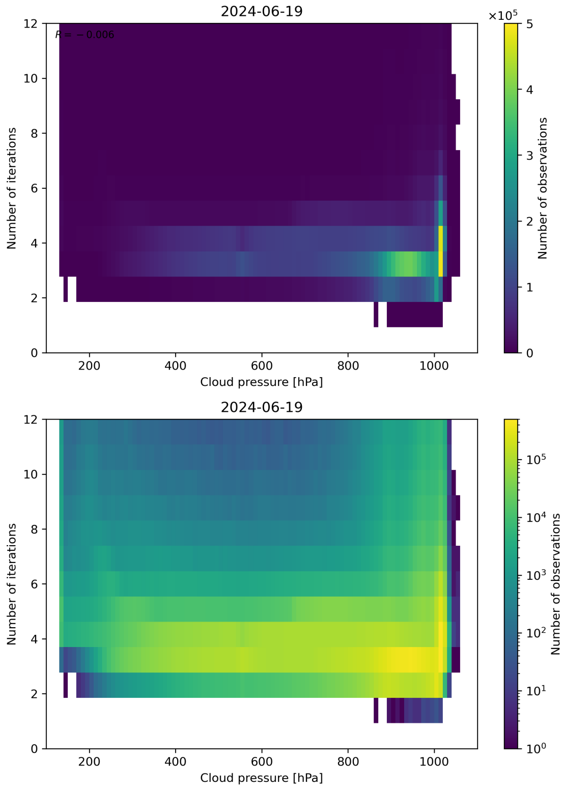
Figure 81: Scatter density plot of “Cloud pressure” against “Number of iterations” for 2024-06-19 to 2024-06-20.
