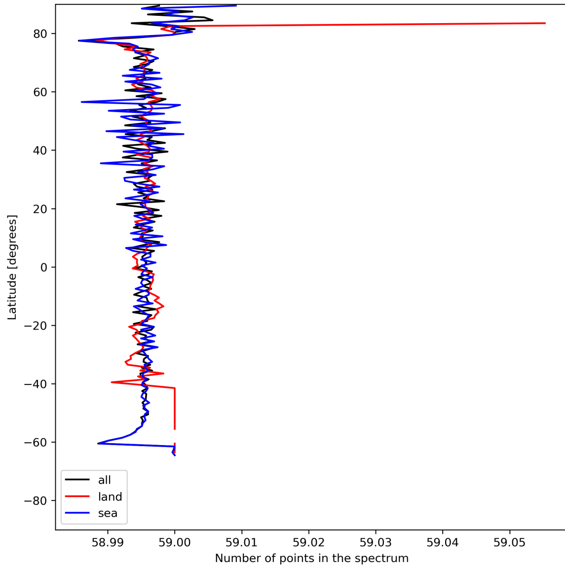
Figure 27: Zonal average of “Number of points in the spectrum” for 2024-06-19 to 2024-06-20.
