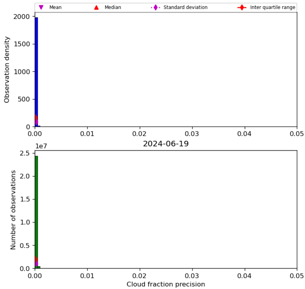
Figure 33: Histogram of “Cloud fraction precision” for 2024-06-19 to 2024-06-20
