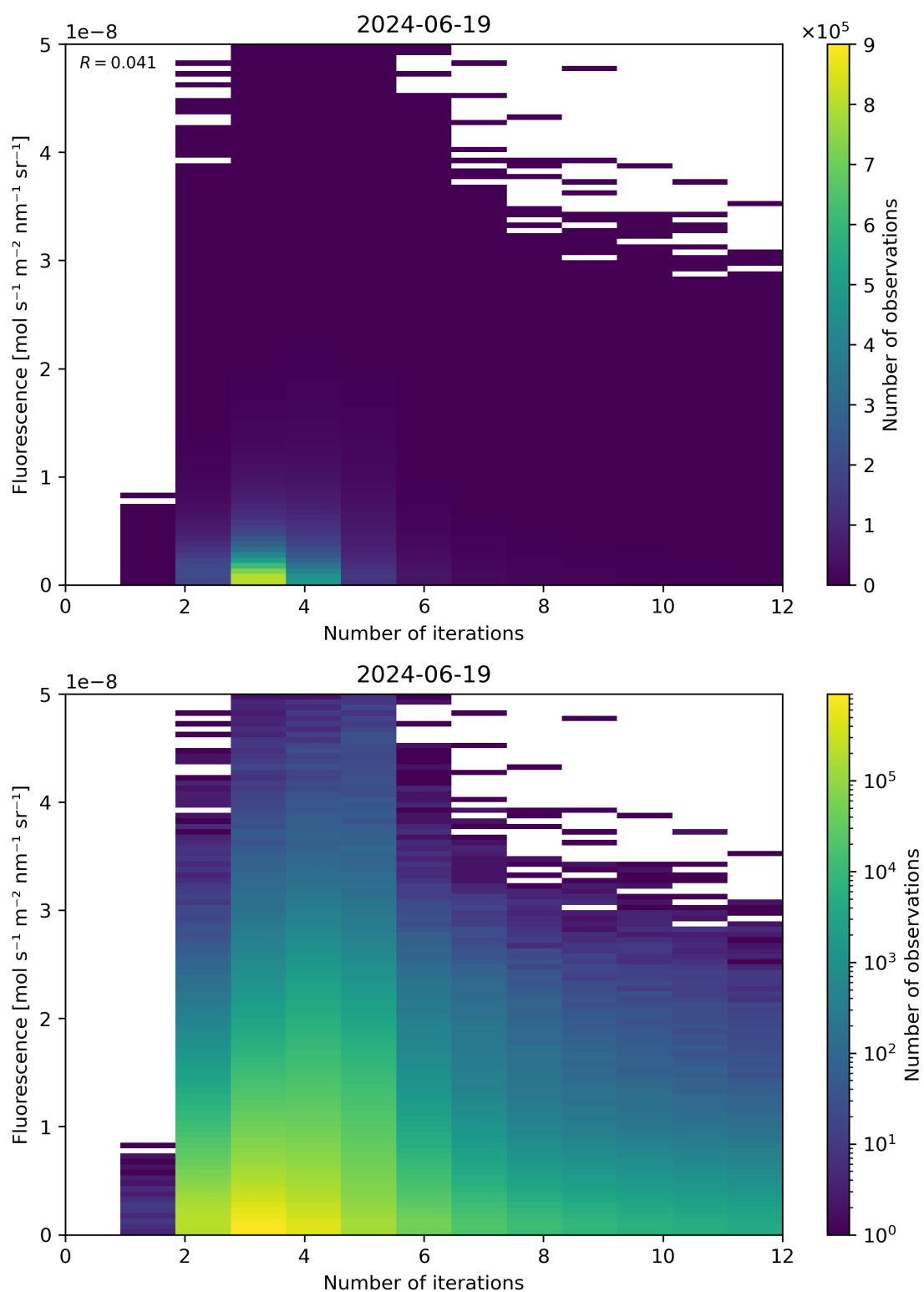
Figure 98: Scatter density plot of “Number of iterations” against “Fluorescence” for 2024-06-19 to 2024-06-20.
