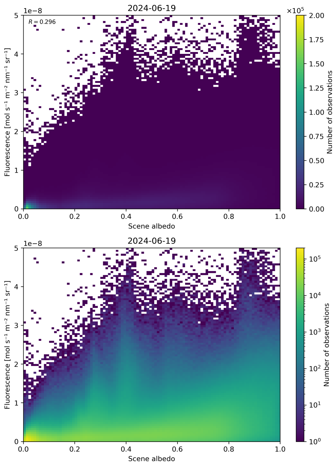
Figure 104: Scatter density plot of “Scene albedo” against “Fluorescence” for 2024-06-19 to 2024-06-20.
