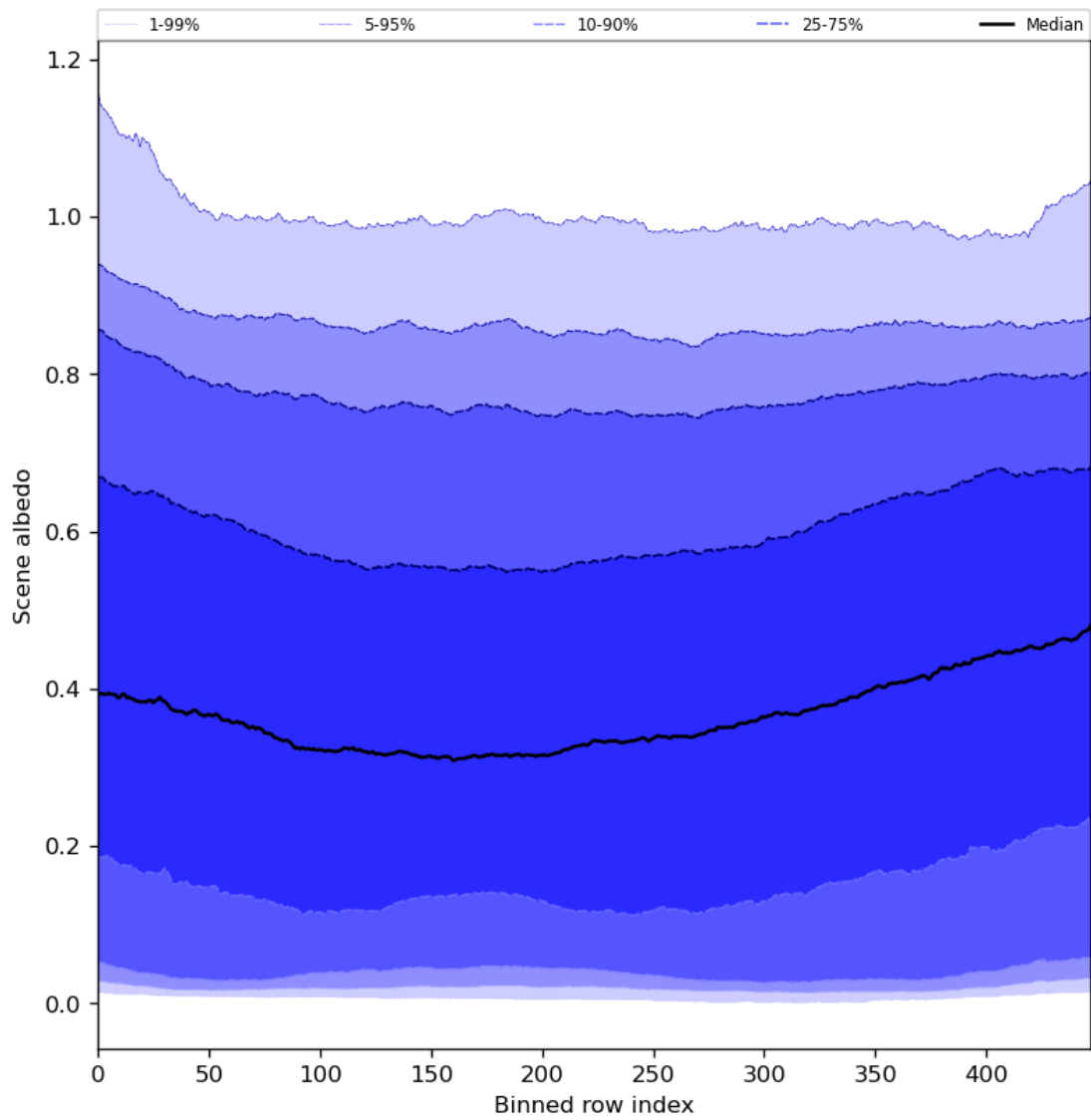
Figure 51: Along track statistics of “Scene albedo” for 2024-06-19 to 2024-06-20
