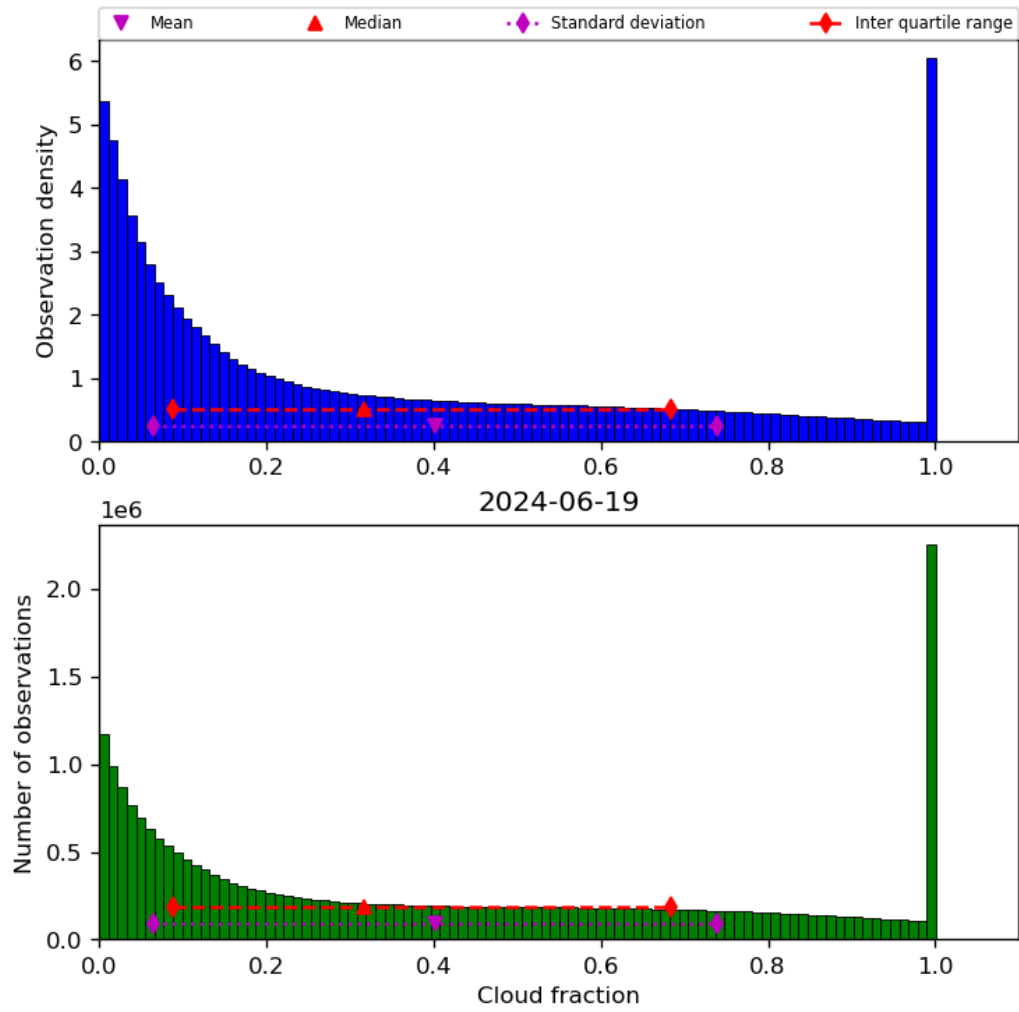
Figure 32: Histogram of “Cloud fraction” for 2024-06-19 to 2024-06-20
