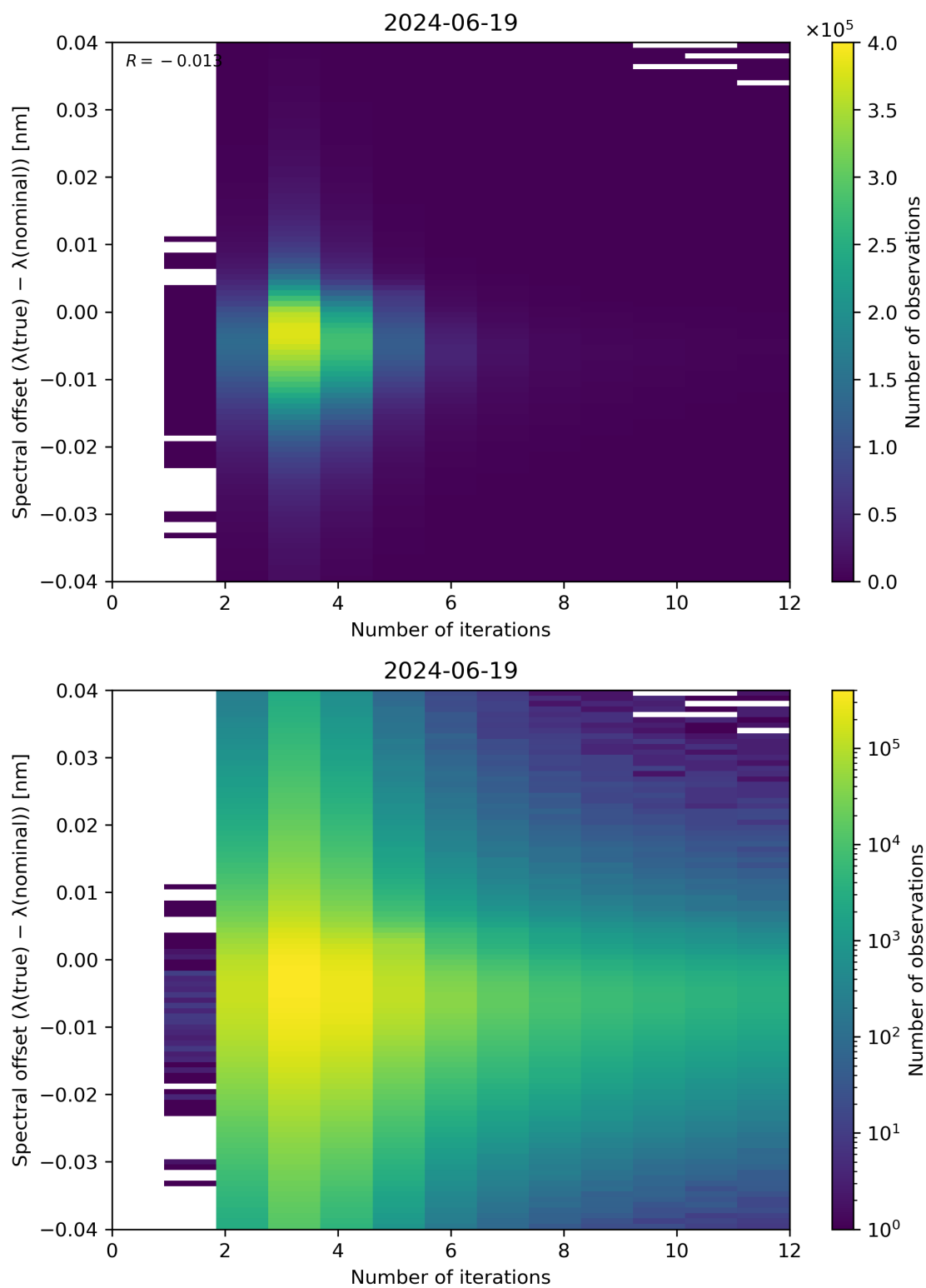
Figure 100: Scatter density plot of “Number of iterations” against “Spectral offset ( \lambda(\text{true}) - \lambda(\text{nominal}) )” for 2024-06-19 to 2024-06-20.
