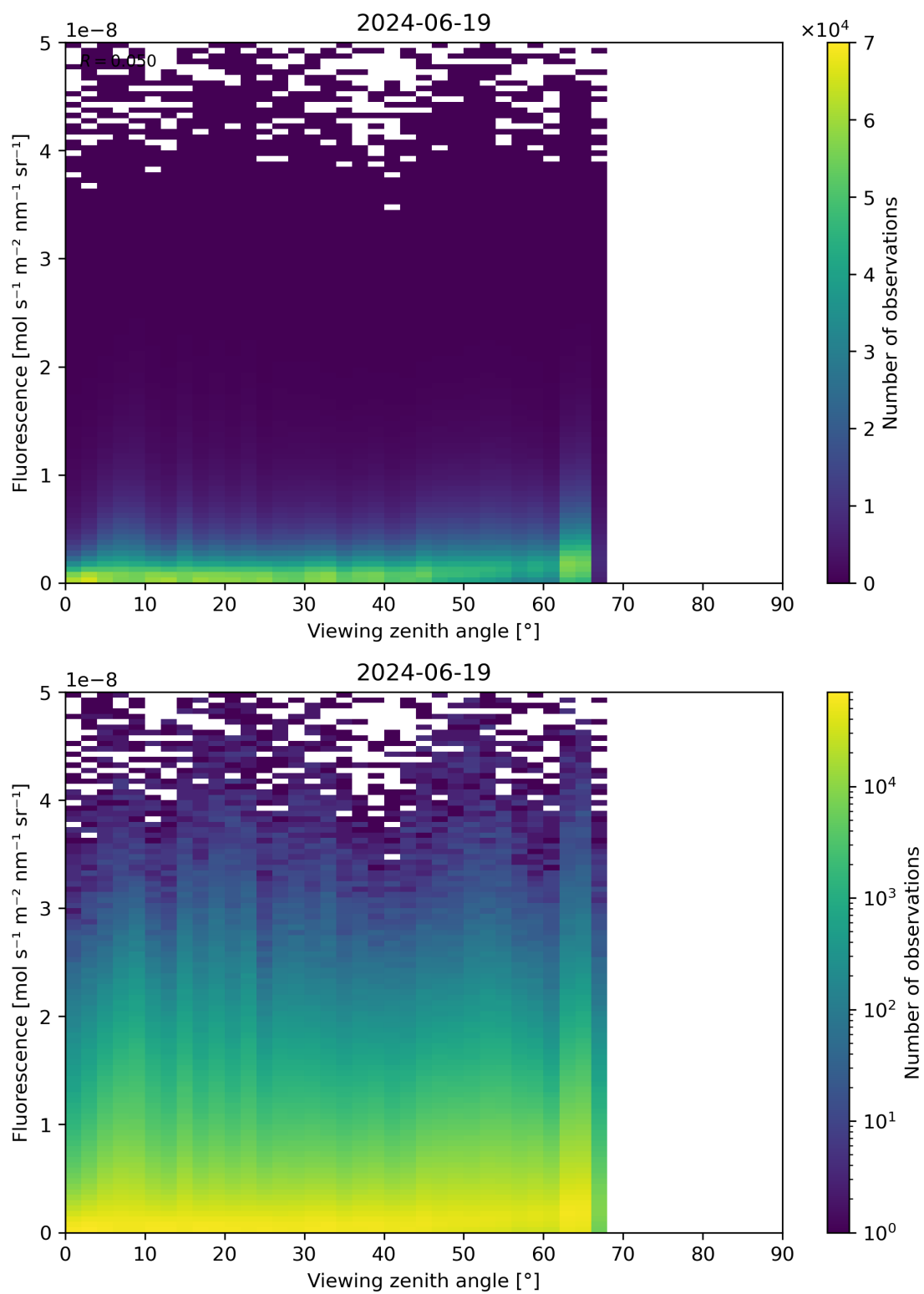
Figure 122: Scatter density plot of “Viewing zenith angle” against “Fluorescence” for 2024-06-19 to 2024-06-20.
