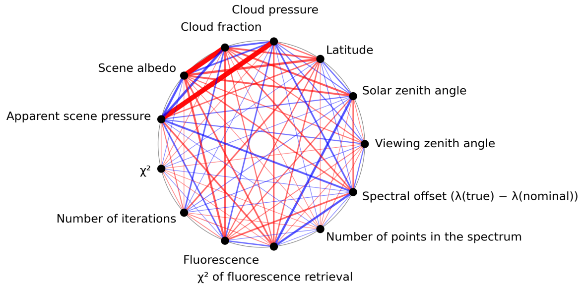
Figure 1: Map of correlation graph for 2024-06-19 to 2024-06-20.
