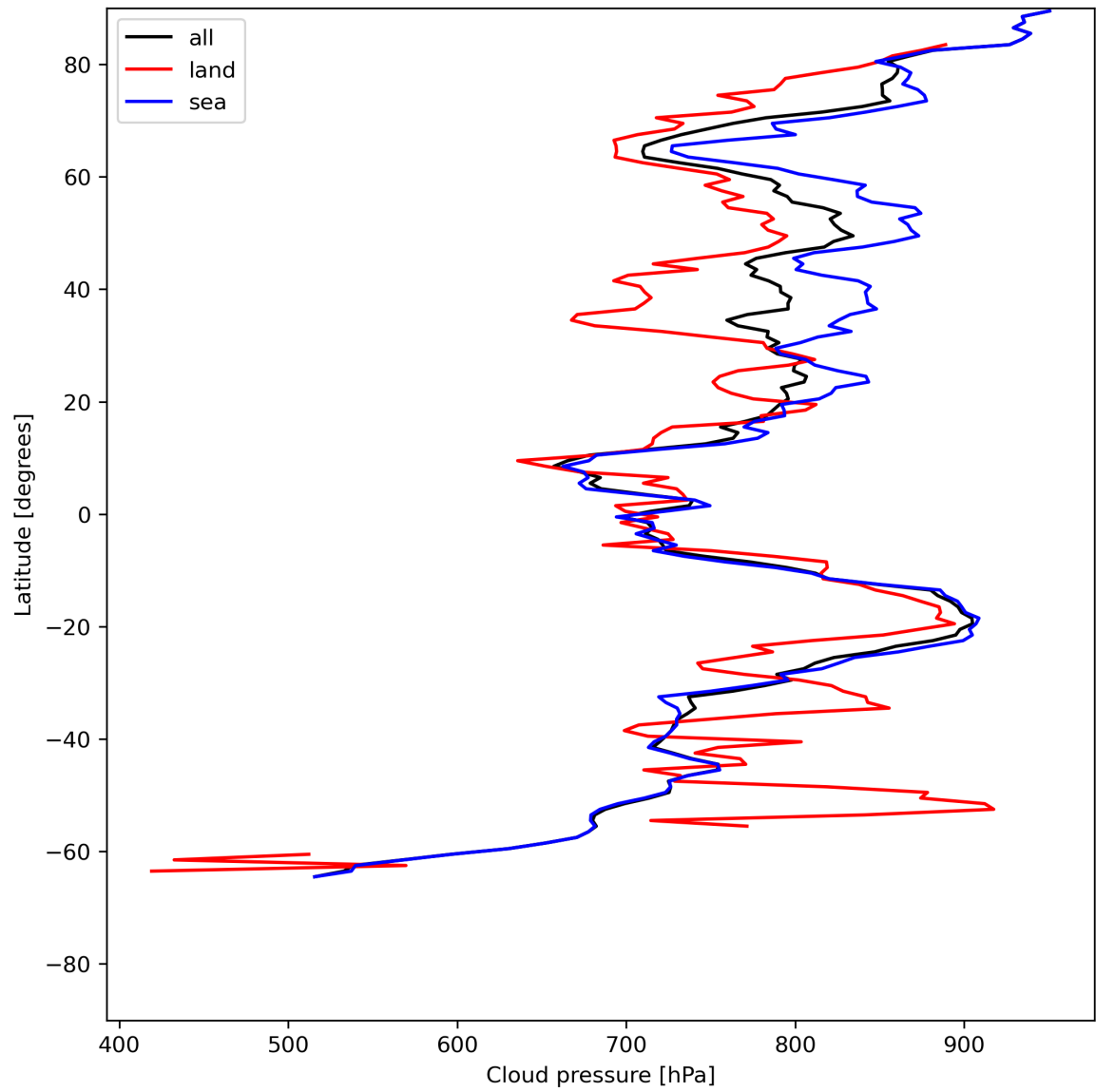
Figure 13: Zonal average of “Cloud pressure” for 2024-06-19 to 2024-06-20.
