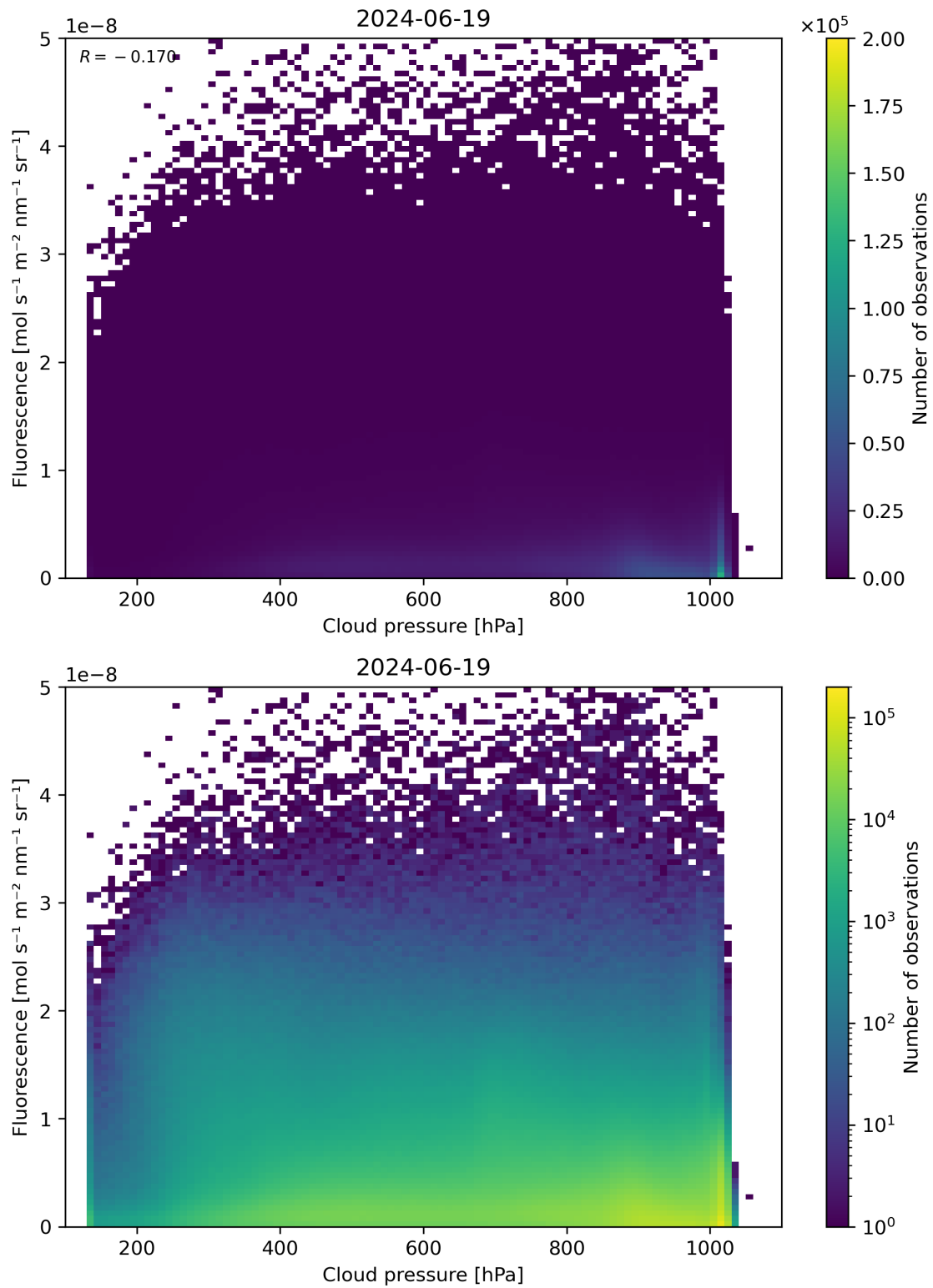
Figure 80: Scatter density plot of “Cloud pressure” against “Fluorescence” for 2024-06-19 to 2024-06-20.
