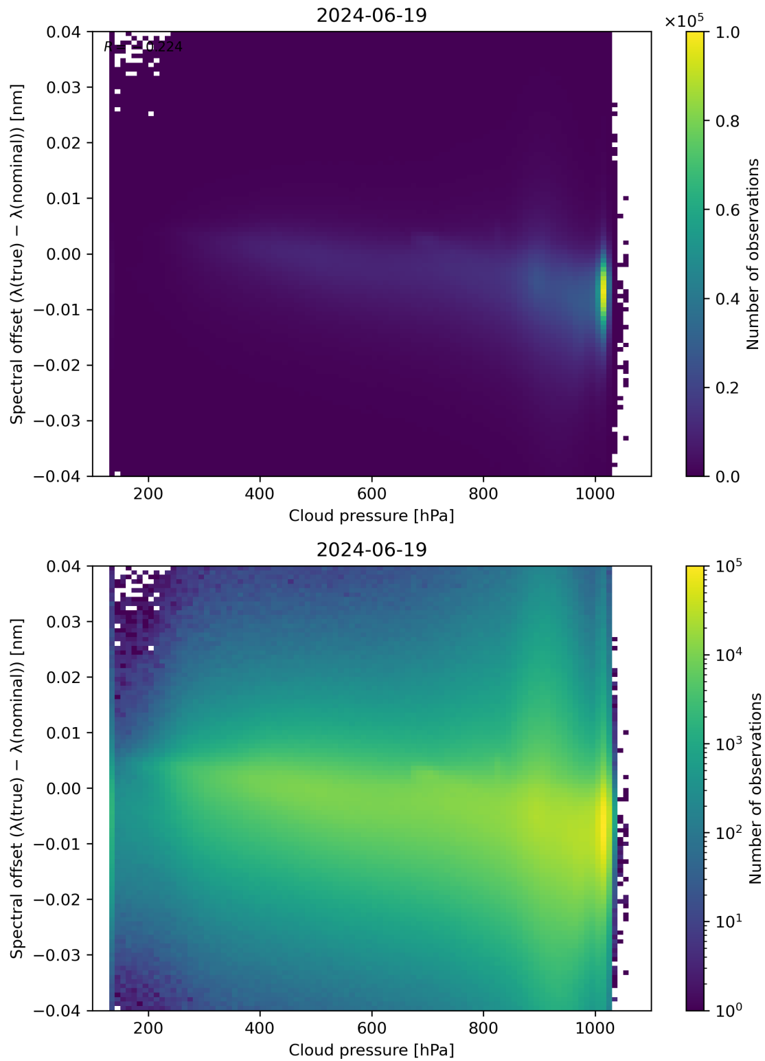
Figure 84: Scatter density plot of “Cloud pressure” against “Spectral offset ( \lambda(\text{true}) - \lambda(\text{nominal}) )” for 2024-06-19 to 2024-06-20.
