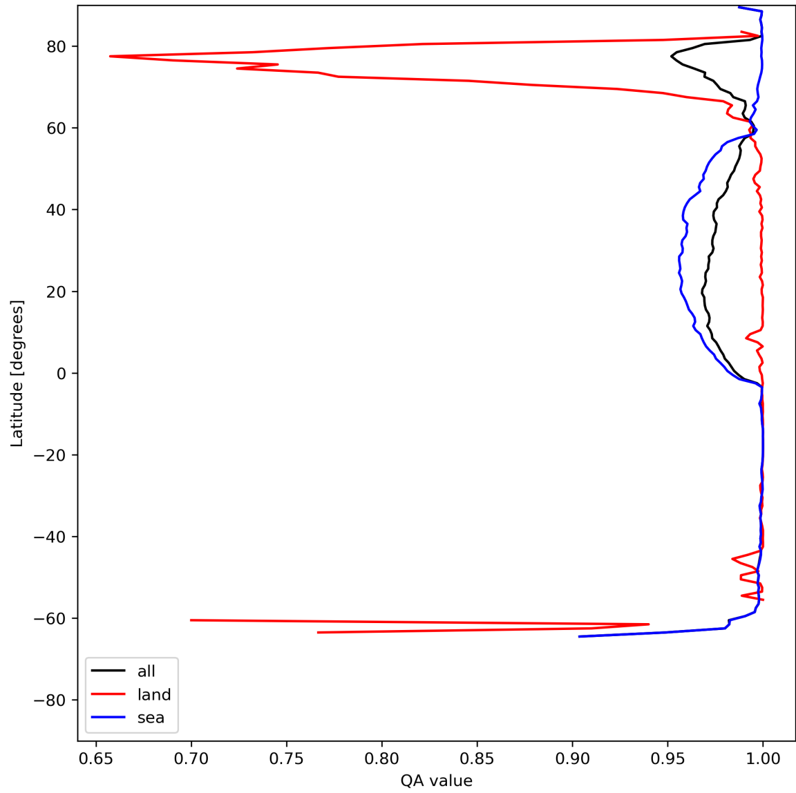
Figure 12: Zonal average of “QA value” for 2024-06-19 to 2024-06-20.
