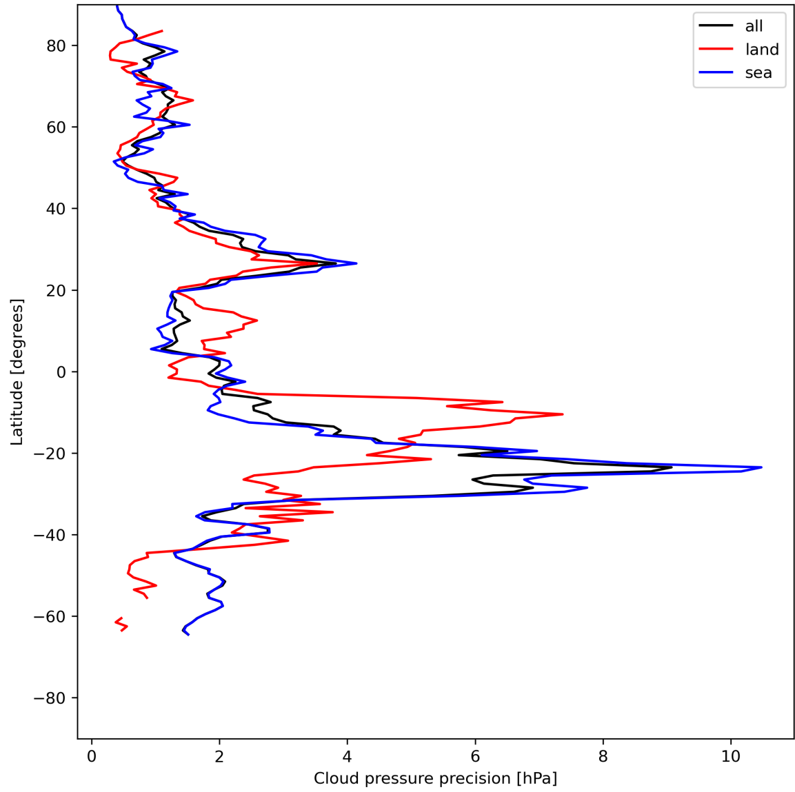
Figure 14: Zonal average of “Cloud pressure precision” for 2024-06-19 to 2024-06-20.
