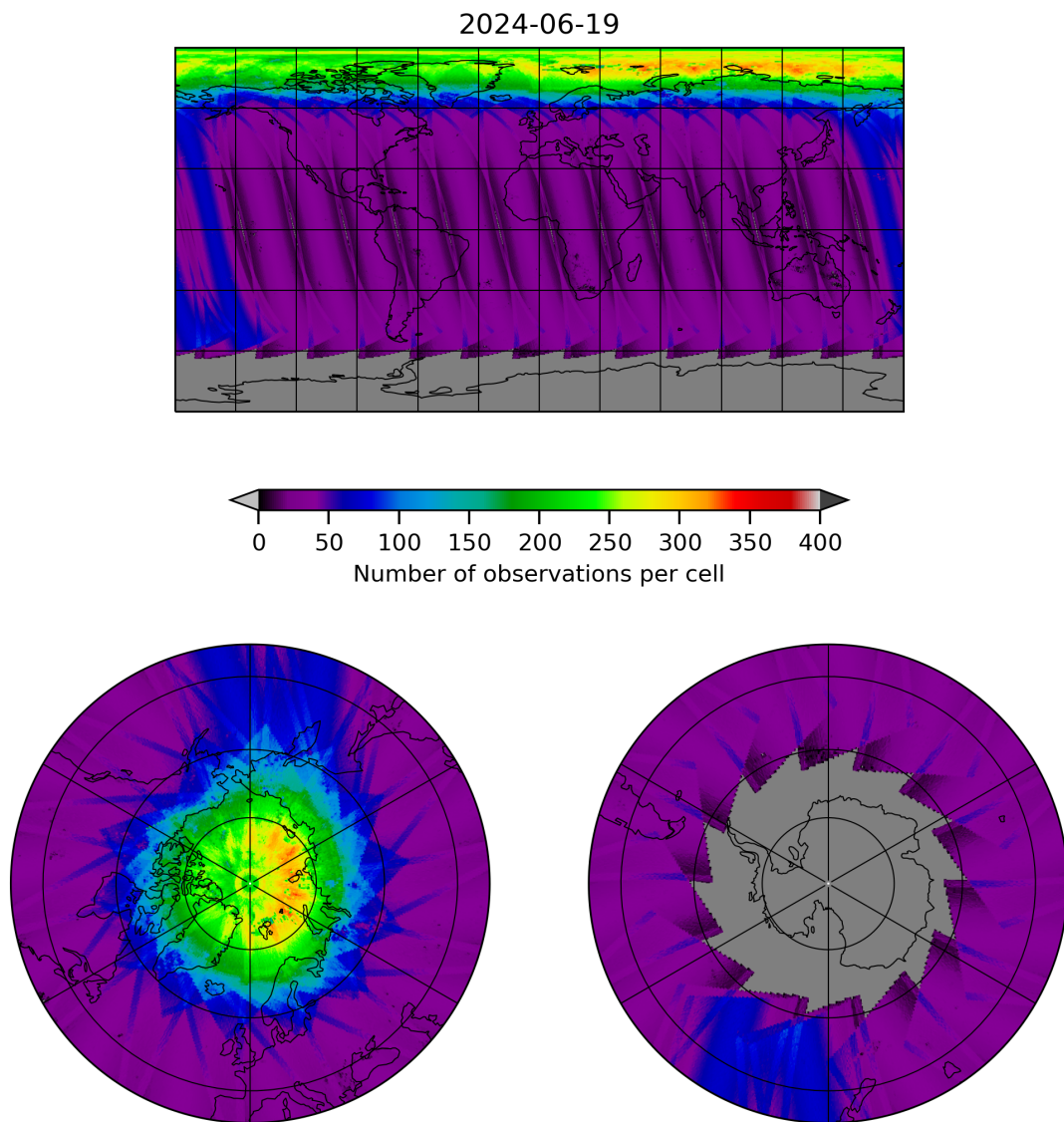
Figure 11: Map of the number of observations for 2024-06-19 to 2024-06-20
