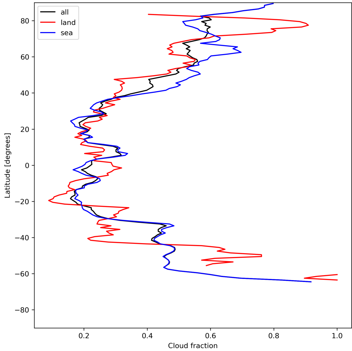
Figure 15: Zonal average of “Cloud fraction” for 2024-06-19 to 2024-06-20.
