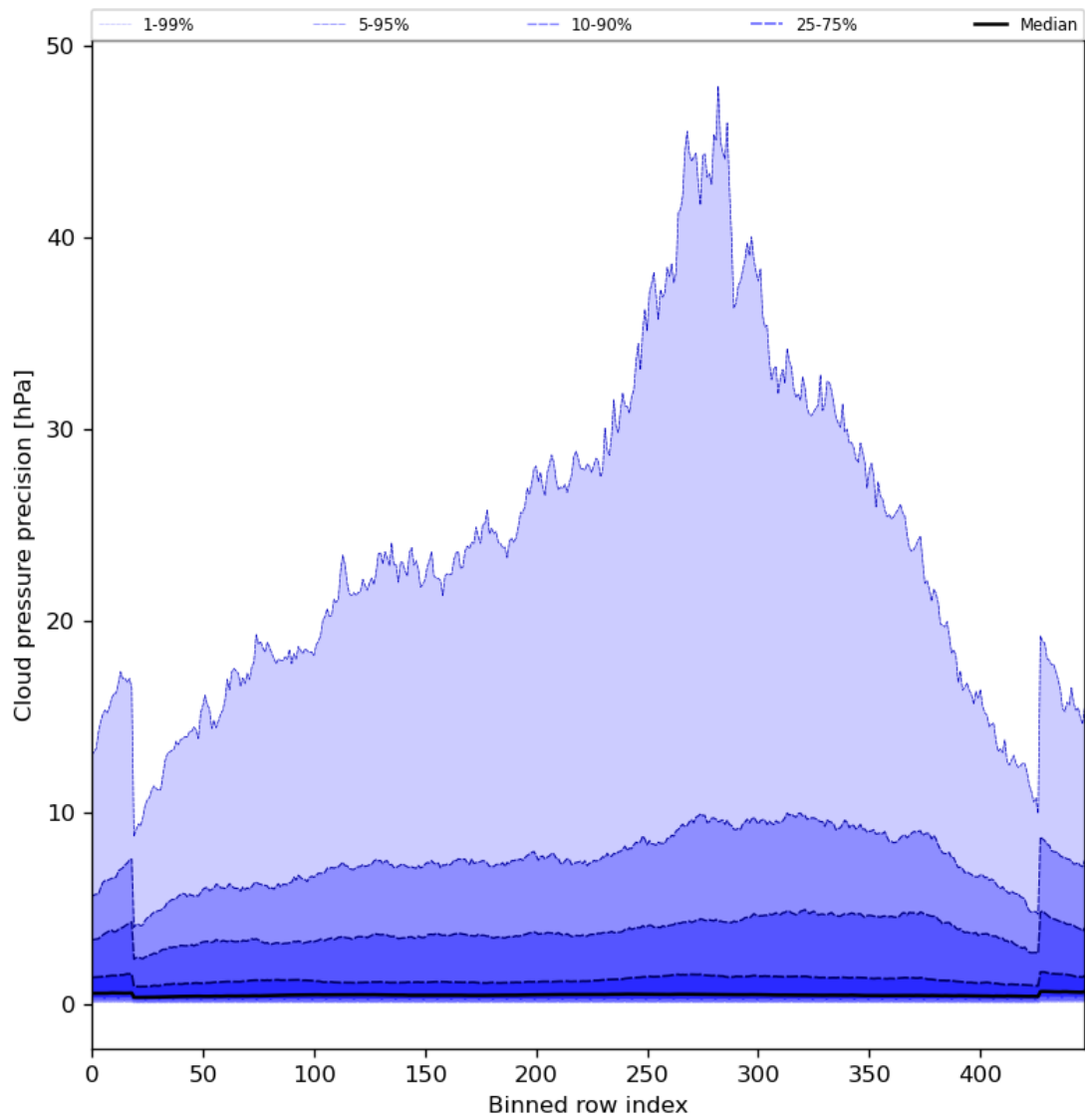
Figure 48: Along track statistics of “Cloud pressure precision” for 2024-06-19 to 2024-06-20
