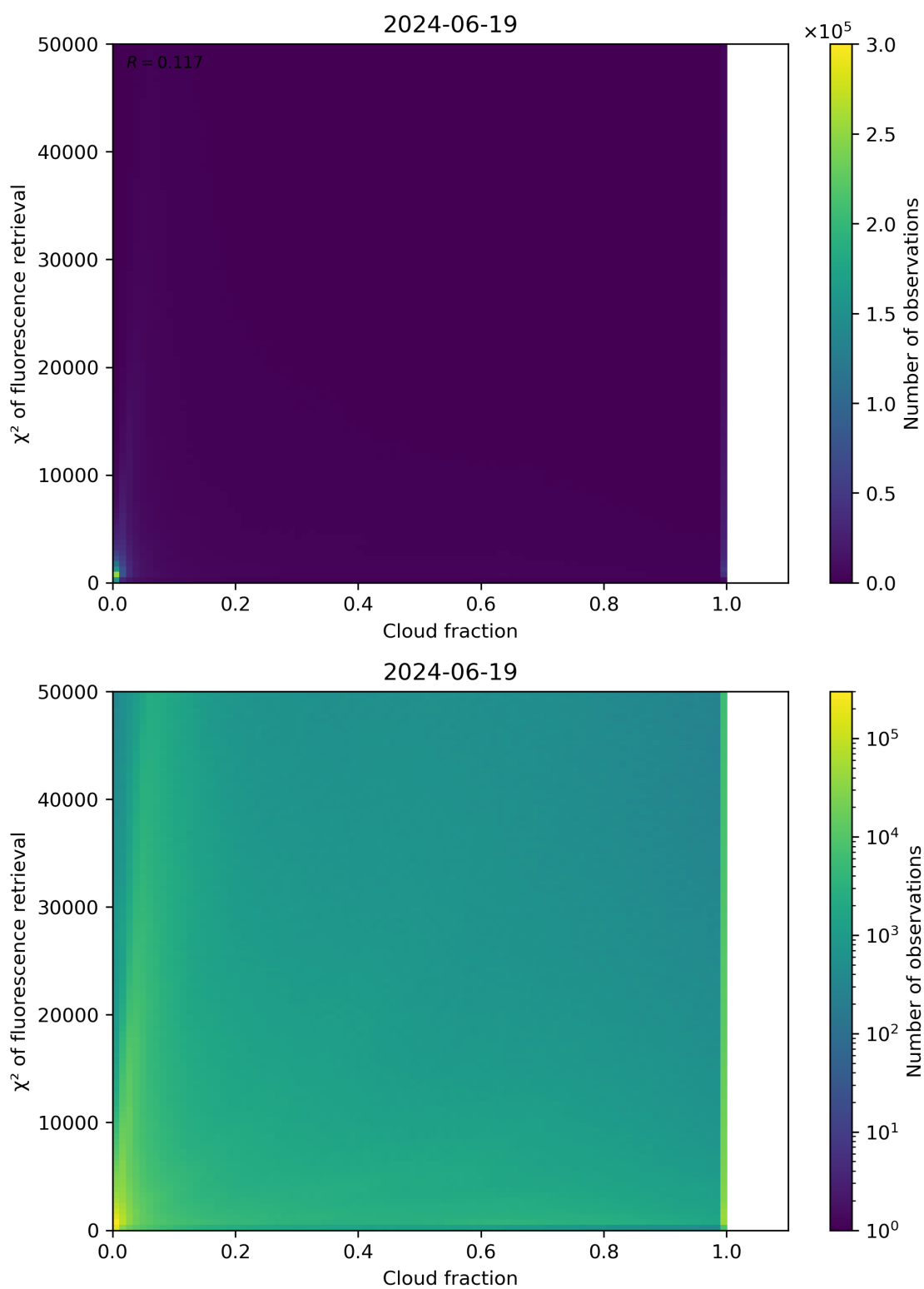
Figure 71: Scatter density plot of “Cloud fraction” against “ \chi^2 of fluorescence retrieval” for 2024-06-19 to 2024-06-20.
