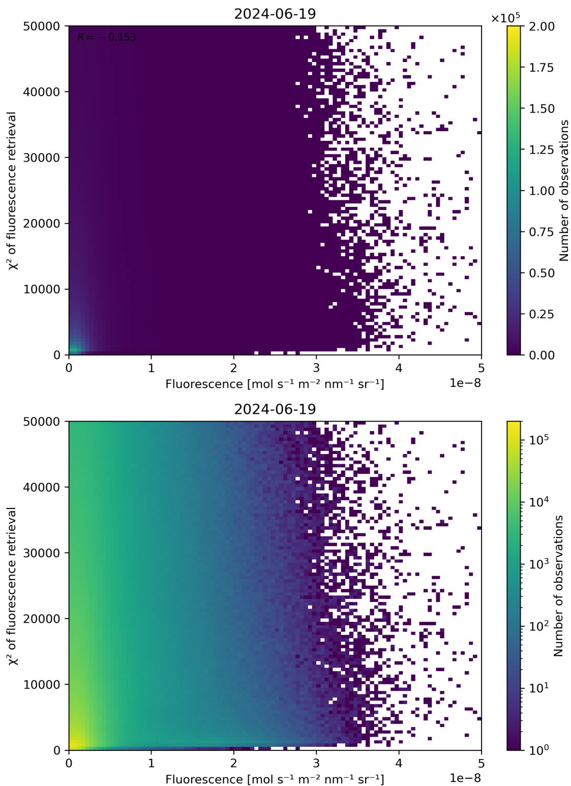
Figure 85: Scatter density plot of “Fluorescence” against “ \chi^2 of fluorescence retrieval” for 2024-06-19 to 2024-06-20.
