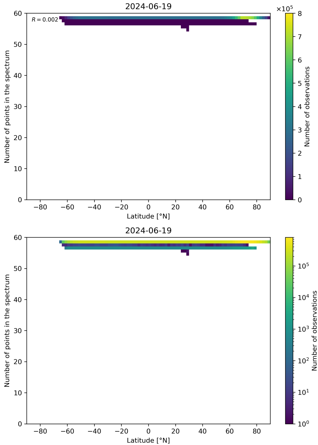
Figure 94: Scatter density plot of “Latitude” against “Number of points in the spectrum” for 2024-06-19 to 2024-06-20.
