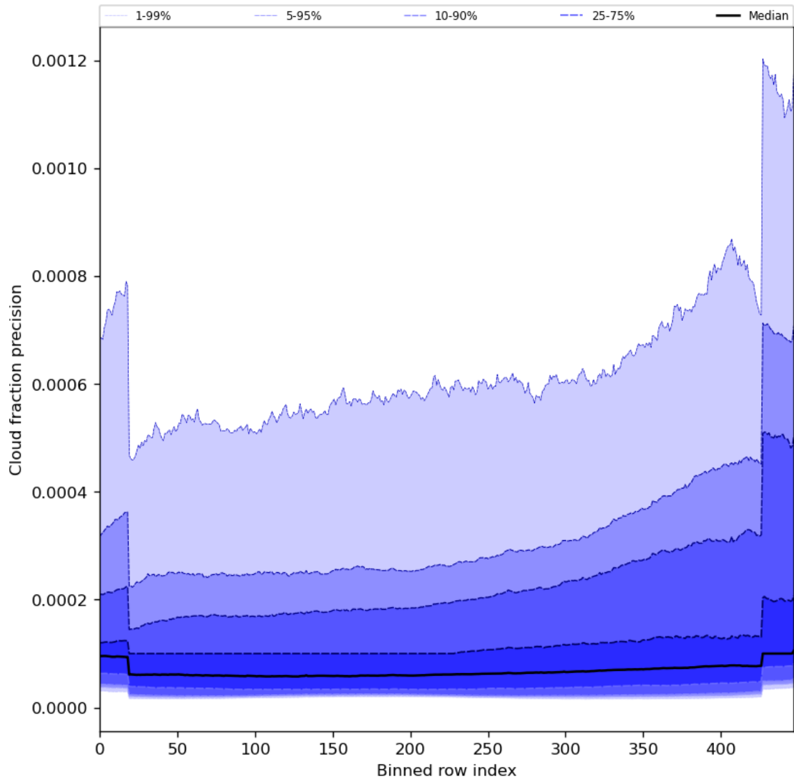
Figure 50: Along track statistics of “Cloud fraction precision” for 2024-06-19 to 2024-06-20
