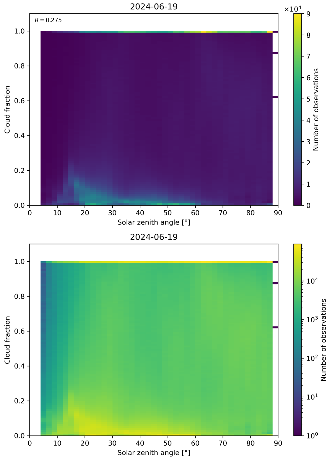
Figure 110: Scatter density plot of “Solar zenith angle” against “Cloud fraction” for 2024-06-19 to 2024-06-20.
