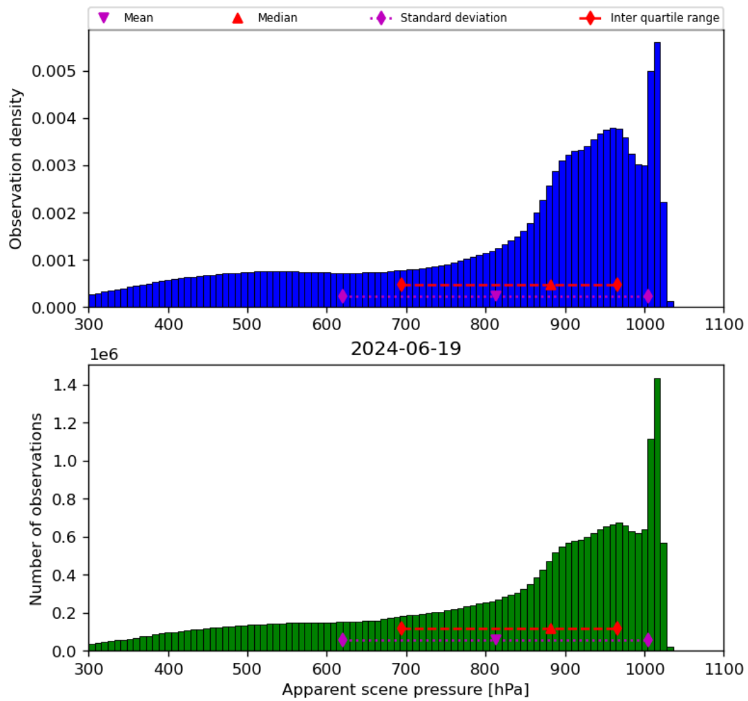
Figure 36: Histogram of “Apparent scene pressure” for 2024-06-19 to 2024-06-20
