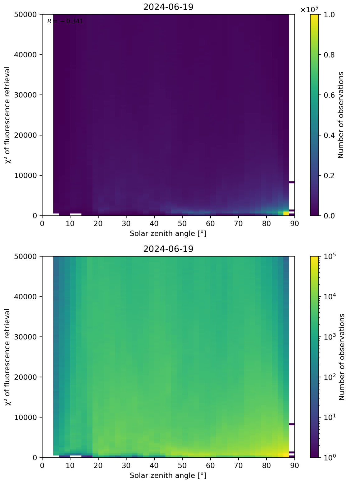
Figure 109: Scatter density plot of “Solar zenith angle” against “ \chi^2 of fluorescence retrieval” for 2024-06-19 to 2024-06-20.
