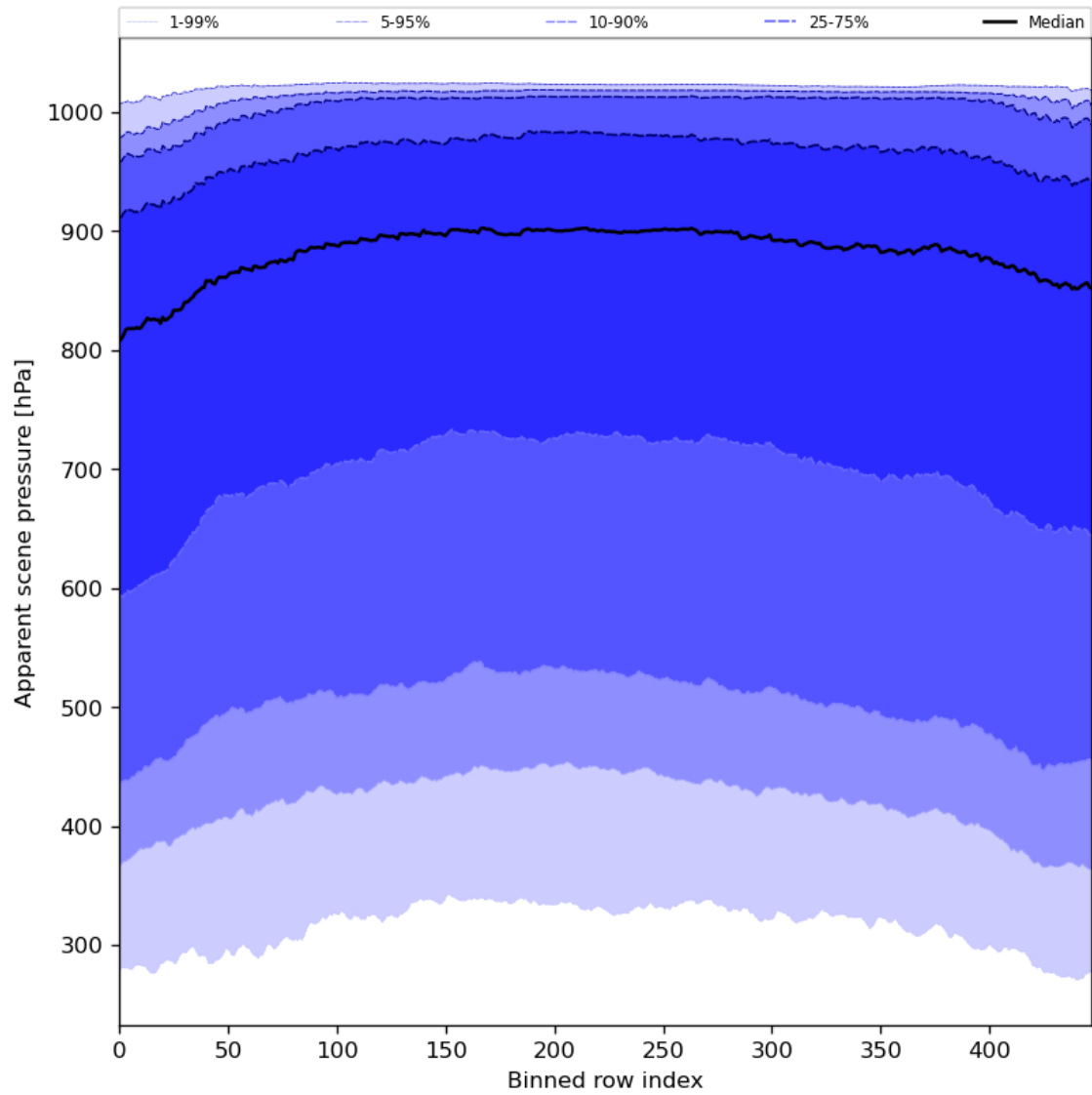
Figure 53: Along track statistics of “Apparent scene pressure” for 2024-06-19 to 2024-06-20
