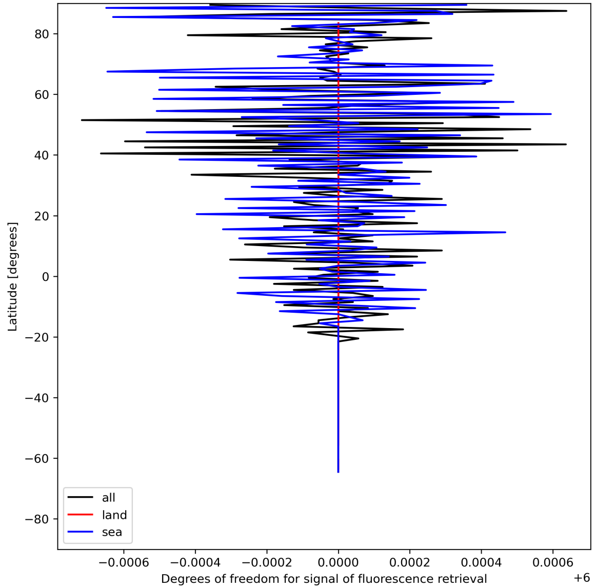
Figure 26: Zonal average of “Degrees of freedom for signal of fluorescence retrieval” for 2024-06-19 to 2024-06-20.
