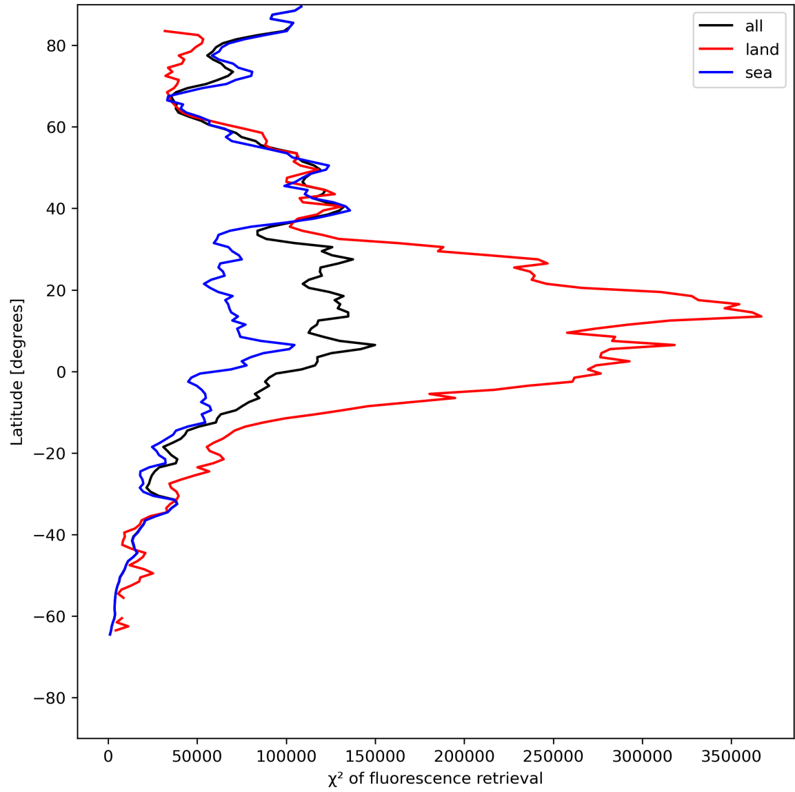
Figure 25: Zonal average of “ \chi^2 of fluorescence retrieval” for 2024-06-19 to 2024-06-20.
