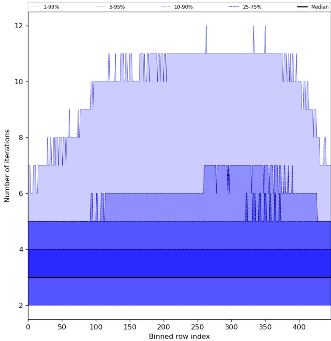
Figure 56: Along track statistics of “Number of iterations” for 2024-06-19 to 2024-06-20
