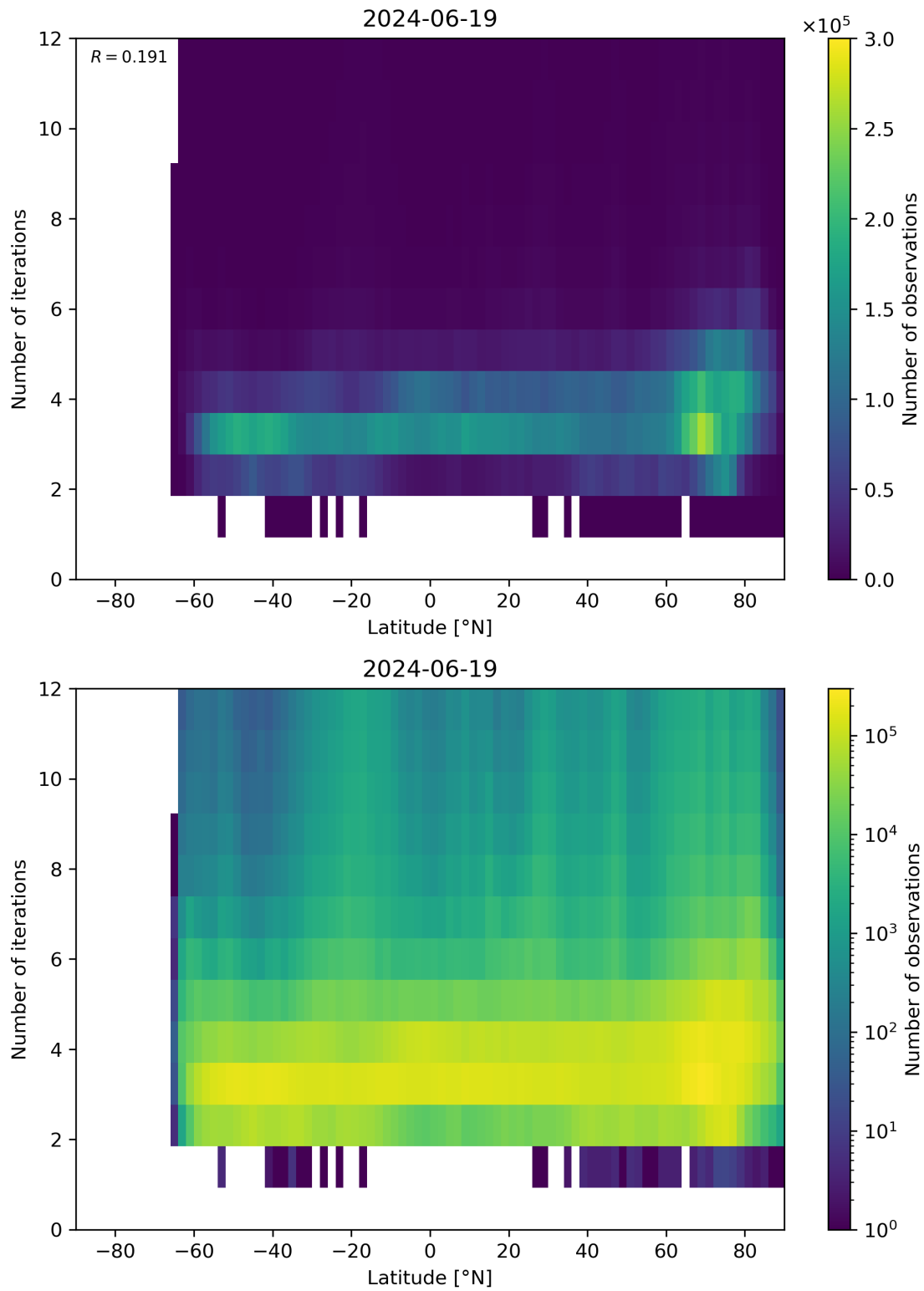
Figure 93: Scatter density plot of “Latitude” against “Number of iterations” for 2024-06-19 to 2024-06-20.
