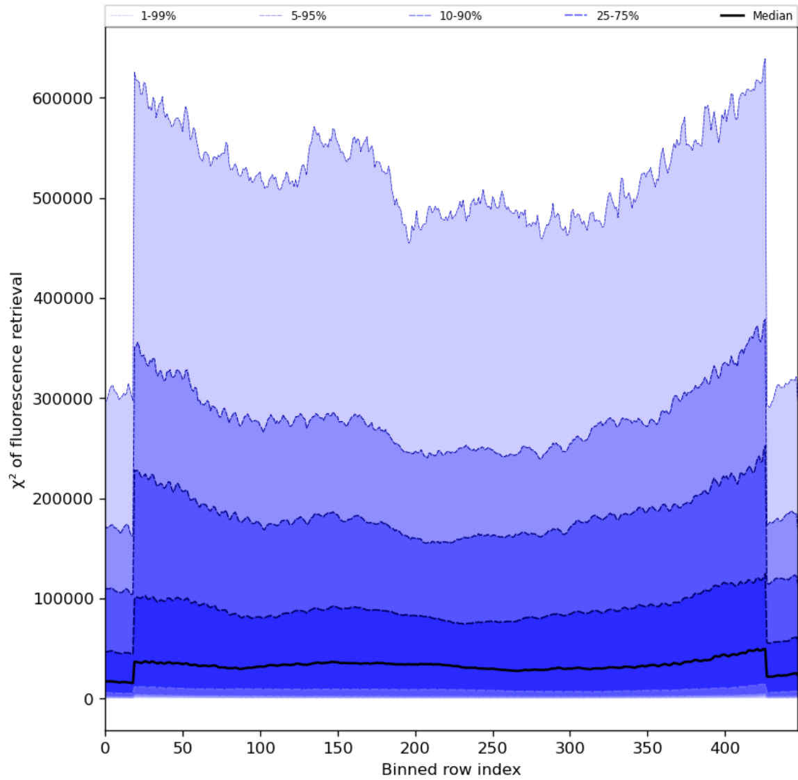
Figure 59: Along track statistics of “ \chi^2 of fluorescence retrieval” for 2024-06-19 to 2024-06-20
