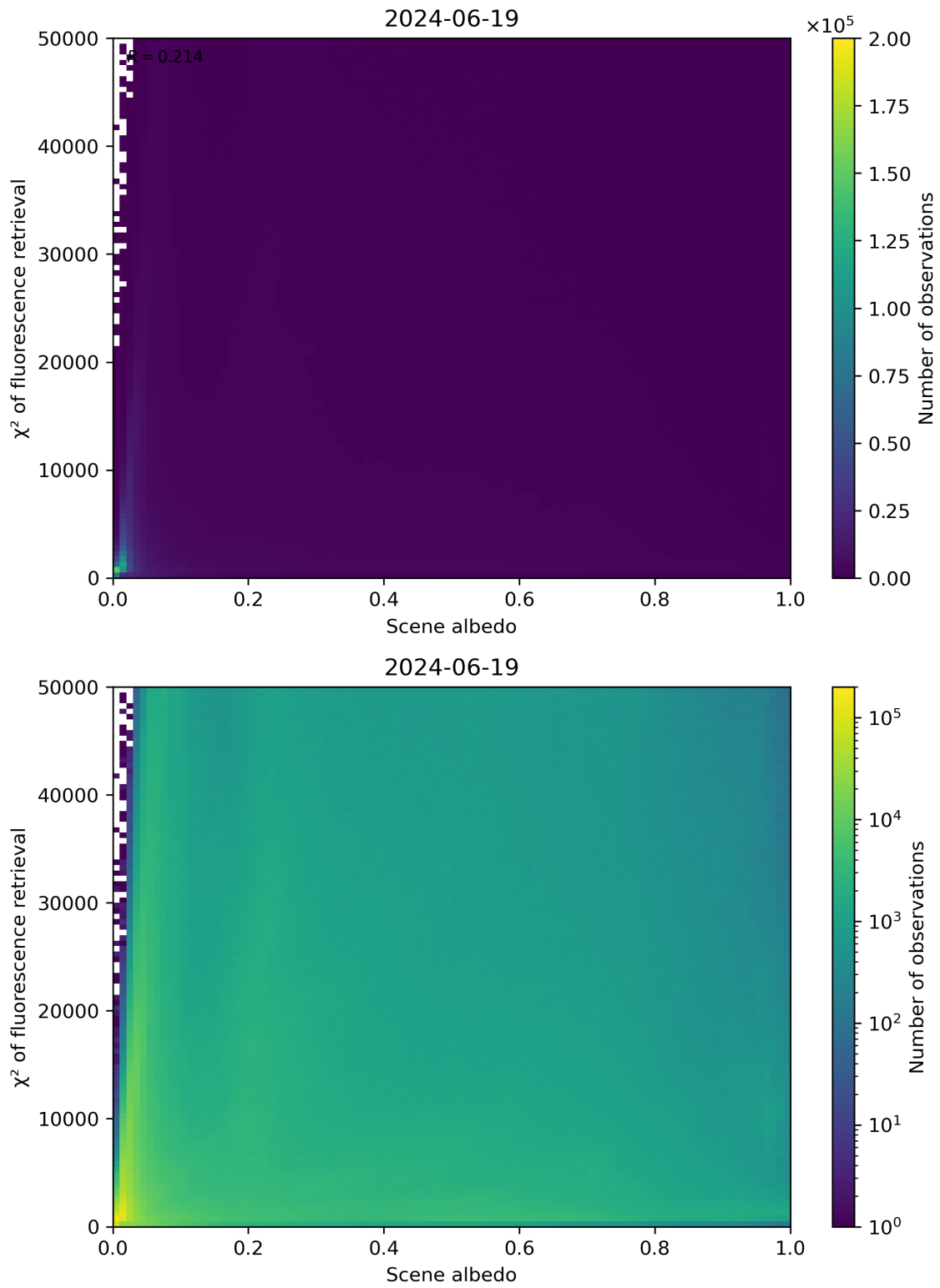
Figure 103: Scatter density plot of “Scene albedo” against “ \chi^2 of fluorescence retrieval” for 2024-06-19 to 2024-06-20.
