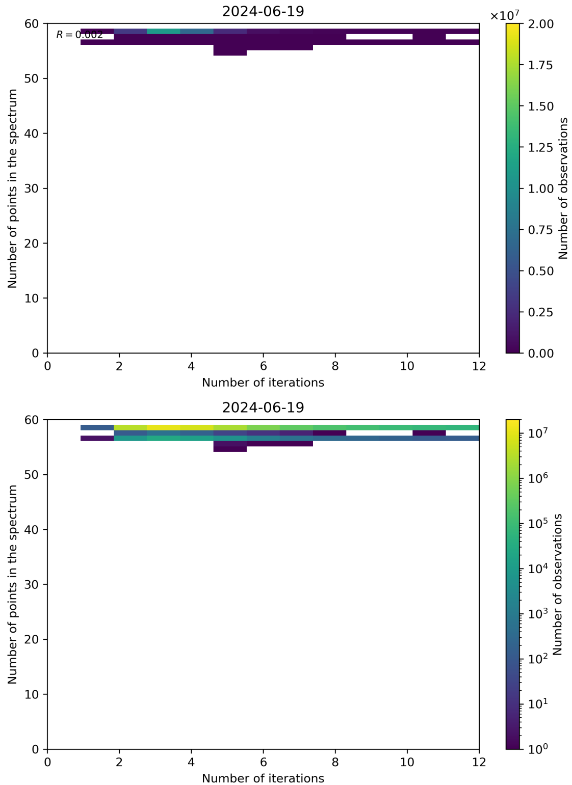
Figure 99: Scatter density plot of “Number of iterations” against “Number of points in the spectrum” for 2024-06-19 to 2024-06-20.
