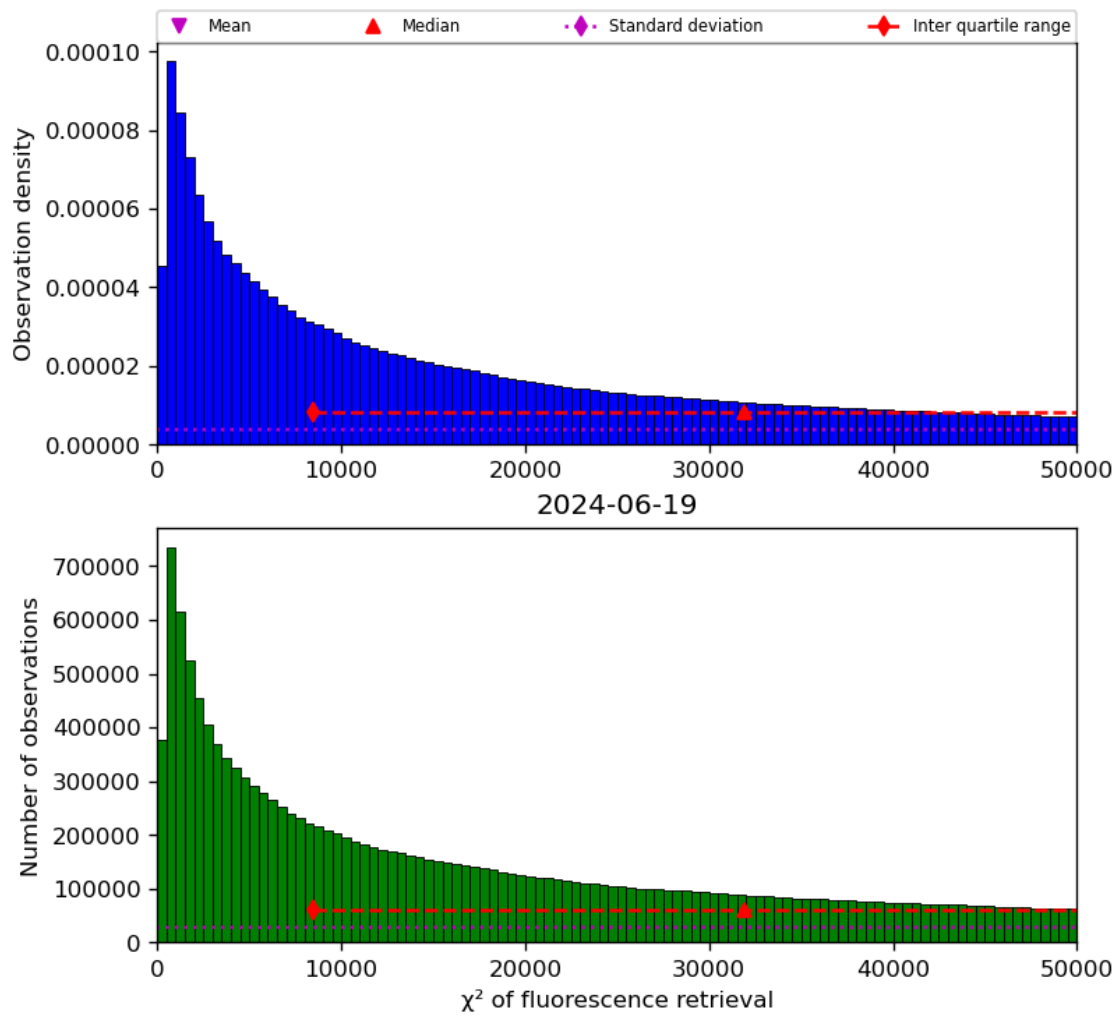
Figure 42: Histogram of “ \chi^2 of fluorescence retrieval” for 2024-06-19 to 2024-06-20
