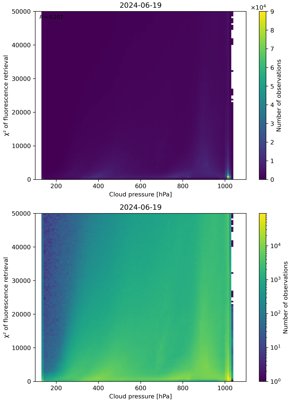
Figure 78: Scatter density plot of “Cloud pressure” against “ \chi^2 of fluorescence retrieval” for 2024-06-19 to 2024-06-20.
