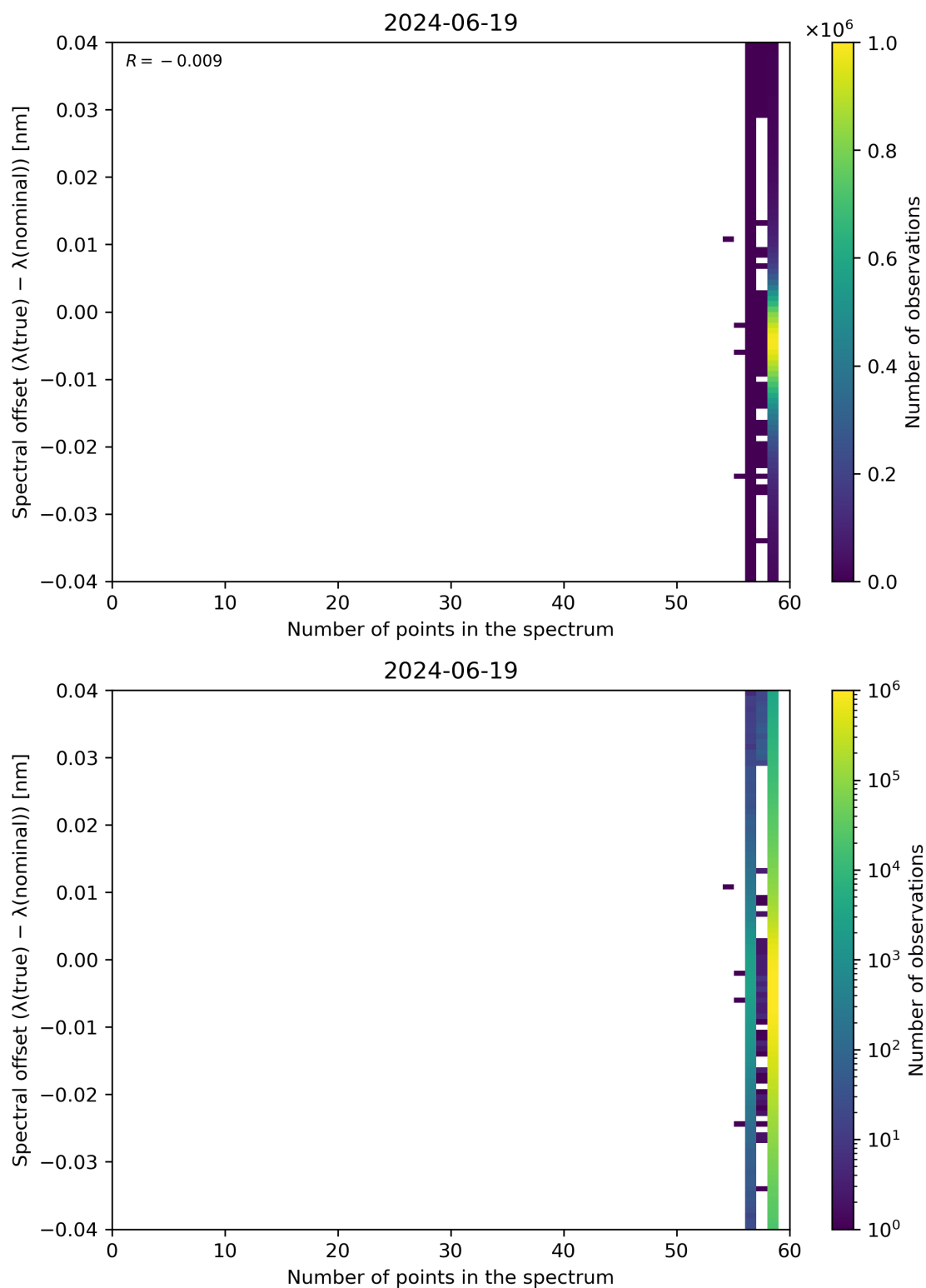
Figure 101: Scatter density plot of “Number of points in the spectrum” against “Spectral offset ( \lambda(\text{true}) - \lambda(\text{nominal}) )” for 2024-06-19 to 2024-06-20.
