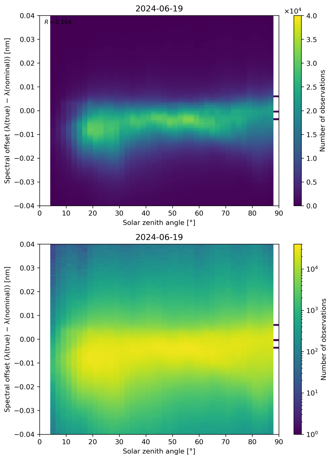
Figure 117: Scatter density plot of “Solar zenith angle” against “Spectral offset ( \lambda(\text{true}) - \lambda(\text{nominal}) )” for 2024-06-19 to 2024-06-20.
