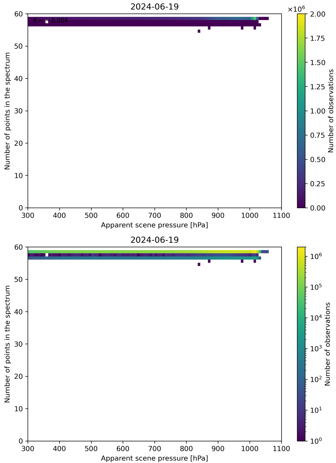
Figure 66: Scatter density plot of “Apparent scene pressure” against “Number of points in the spectrum” for 2024-06-19 to 2024-06-20.
