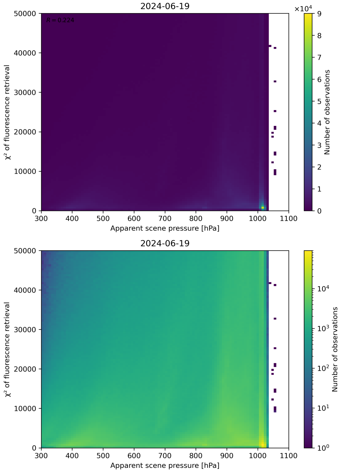
Figure 63: Scatter density plot of “Apparent scene pressure” against “ \chi^2 of fluorescence retrieval” for 2024-06-19 to 2024-06-20.
