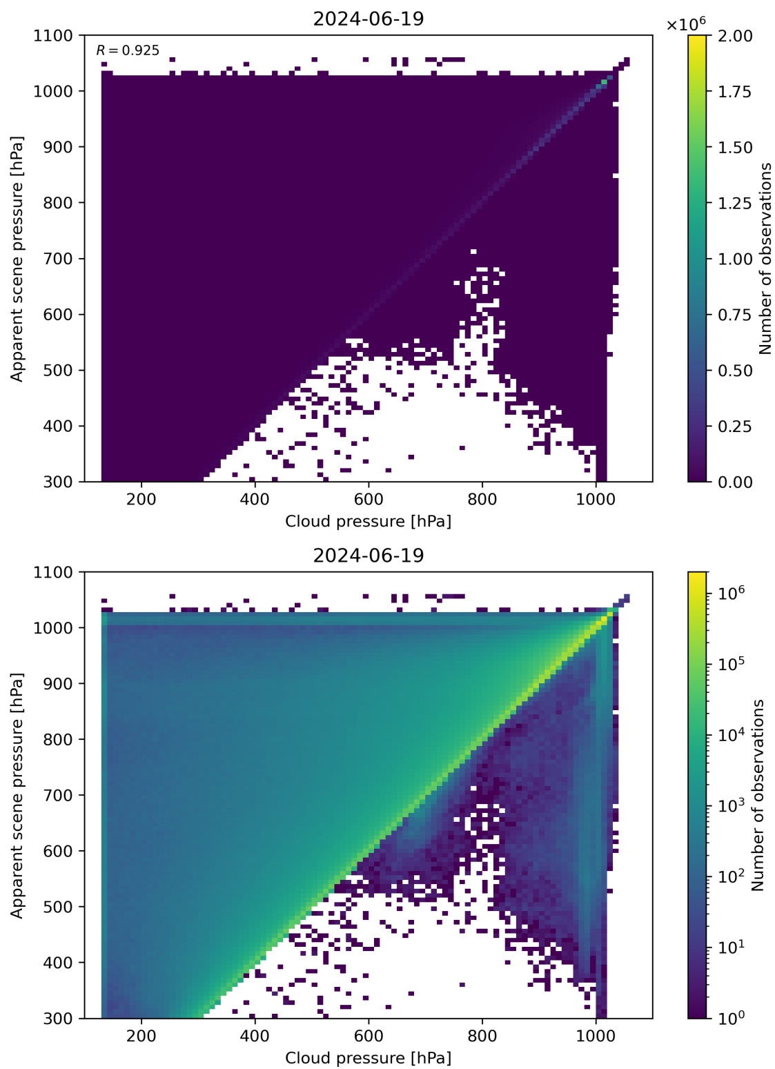
Figure 77: Scatter density plot of “Cloud pressure” against “Apparent scene pressure” for 2024-06-19 to 2024-06-20.
