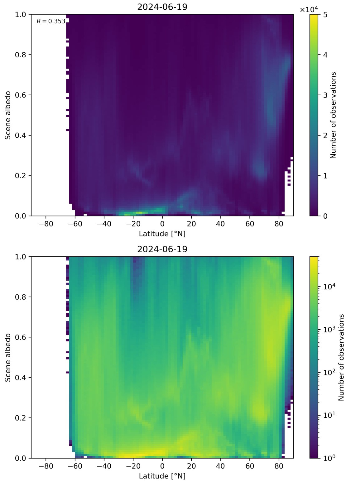
Figure 95: Scatter density plot of “Latitude” against “Scene albedo” for 2024-06-19 to 2024-06-20.
