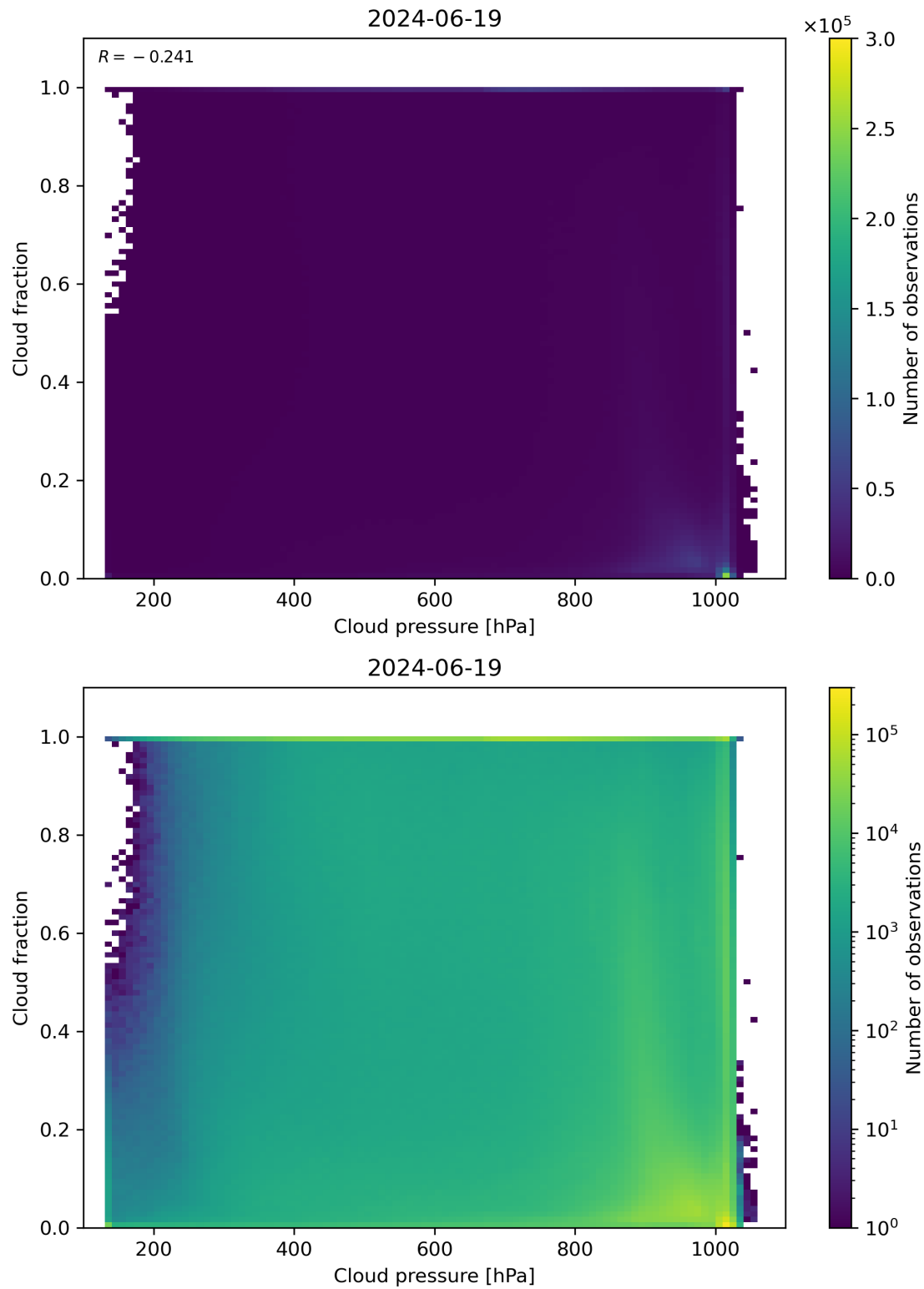
Figure 79: Scatter density plot of “Cloud pressure” against “Cloud fraction” for 2024-06-19 to 2024-06-20.
