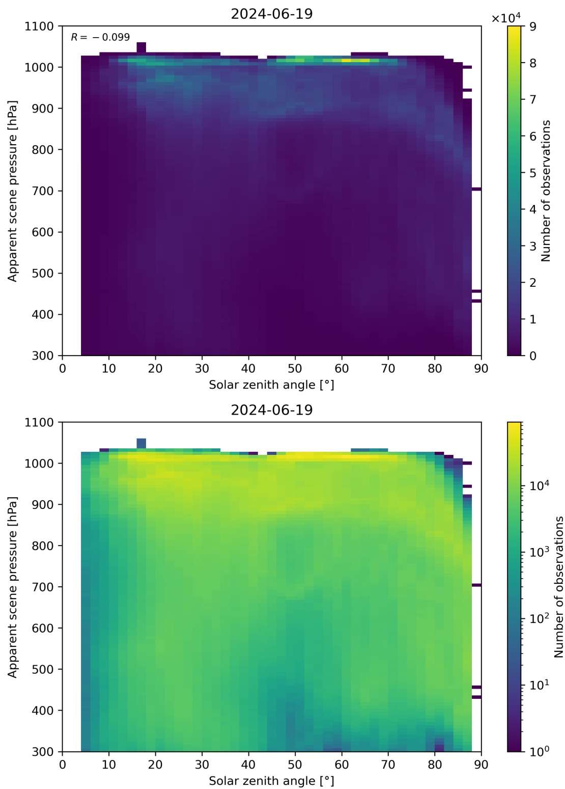
Figure 108: Scatter density plot of “Solar zenith angle” against “Apparent scene pressure” for 2024-06-19 to 2024-06-20.
