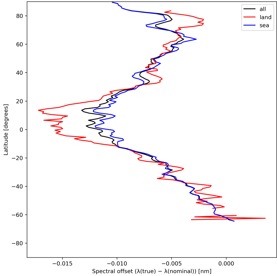
Figure 28: Zonal average of “Spectral offset ( \lambda(\text{true}) - \lambda(\text{nominal}) )” for 2024-06-19 to 2024-06-20.
