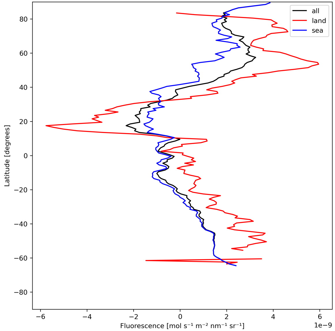
Figure 23: Zonal average of “Fluorescence” for 2024-06-19 to 2024-06-20.
