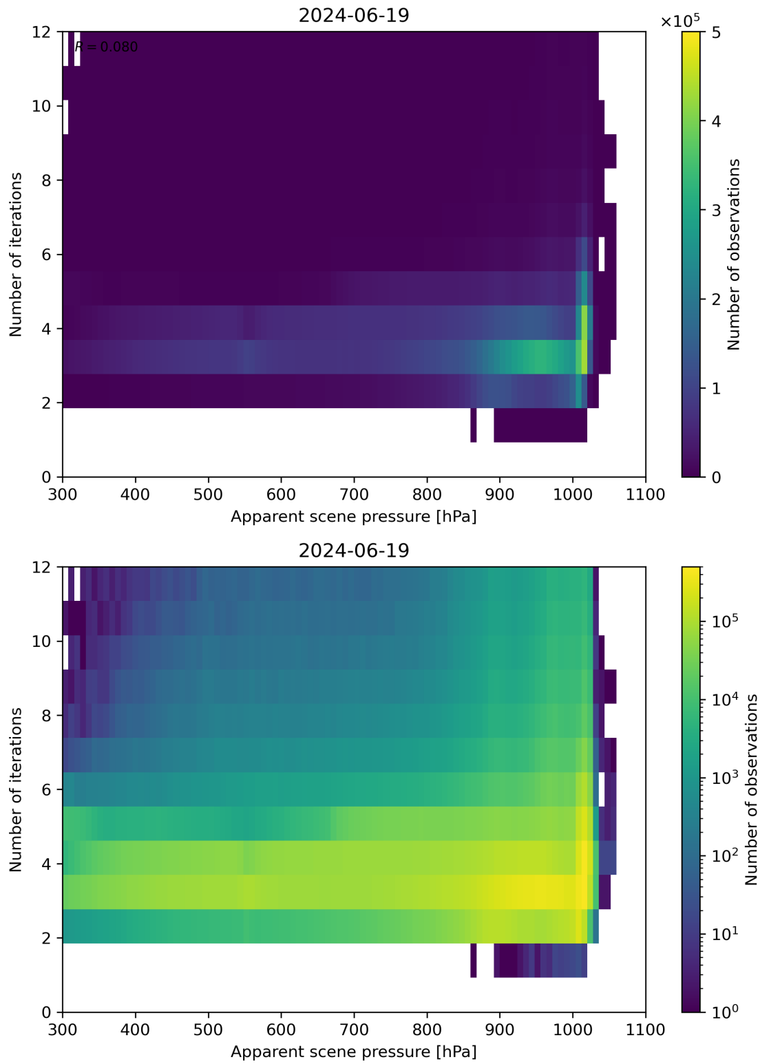
Figure 65: Scatter density plot of “Apparent scene pressure” against “Number of iterations” for 2024-06-19 to 2024-06-20.
