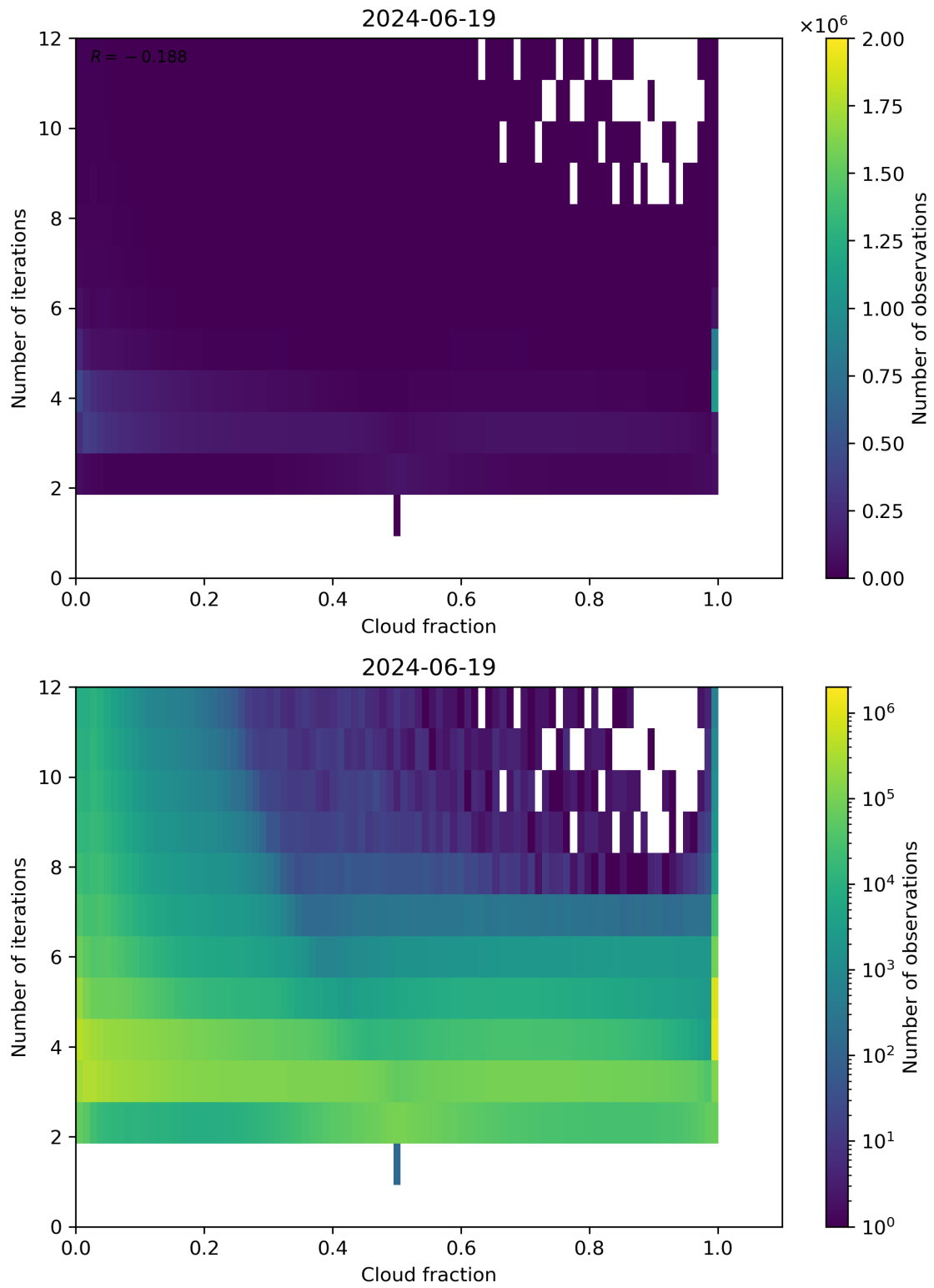
Figure 73: Scatter density plot of “Cloud fraction” against “Number of iterations” for 2024-06-19 to 2024-06-20.
