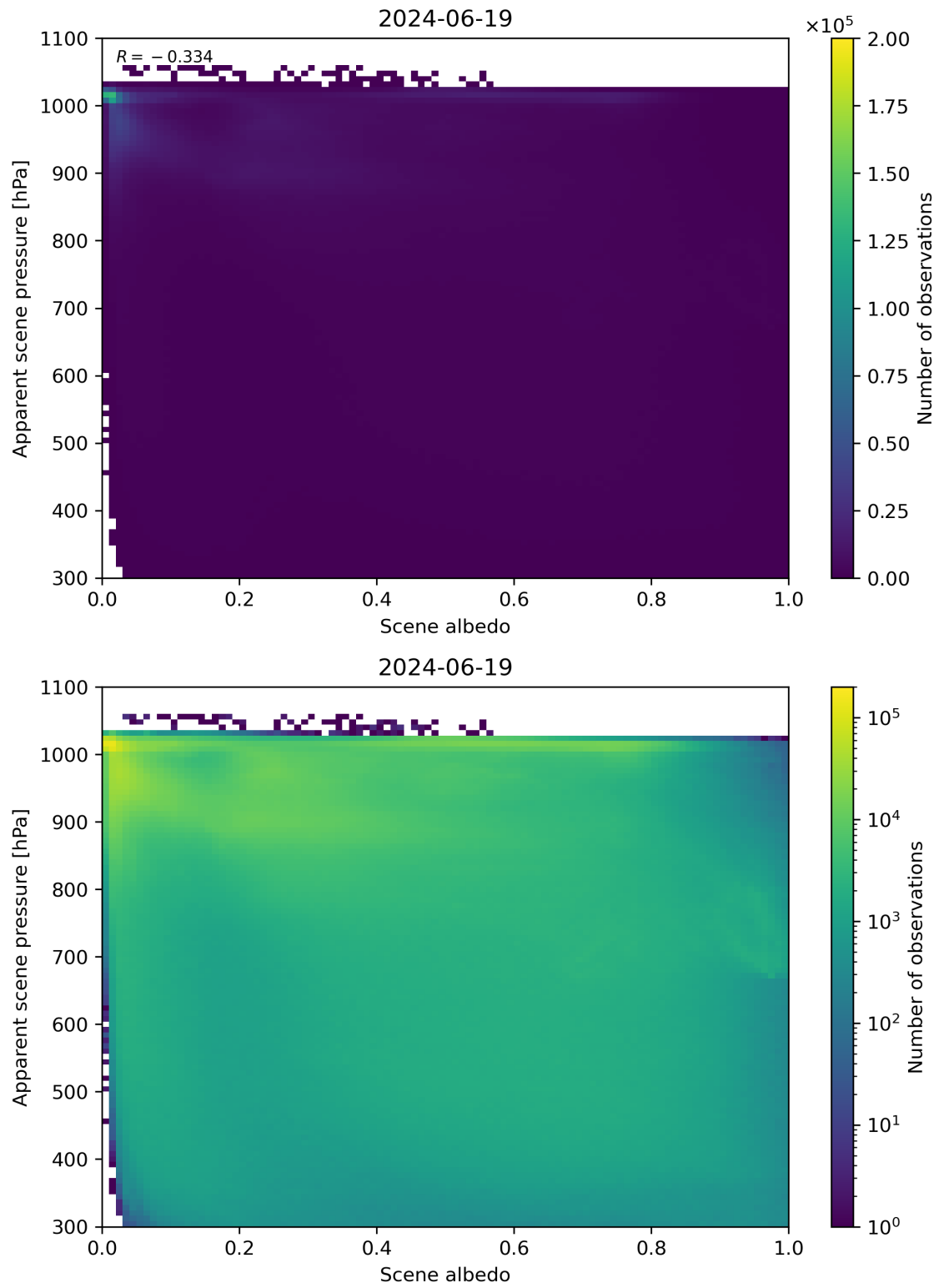
Figure 102: Scatter density plot of “Scene albedo” against “Apparent scene pressure” for 2024-06-19 to 2024-06-20.
