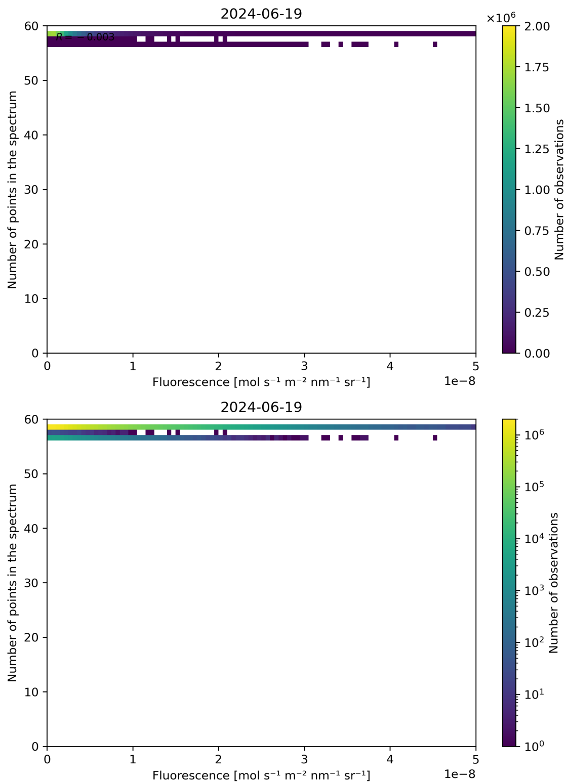
Figure 86: Scatter density plot of “Fluorescence” against “Number of points in the spectrum” for 2024-06-19 to 2024-06-20.
