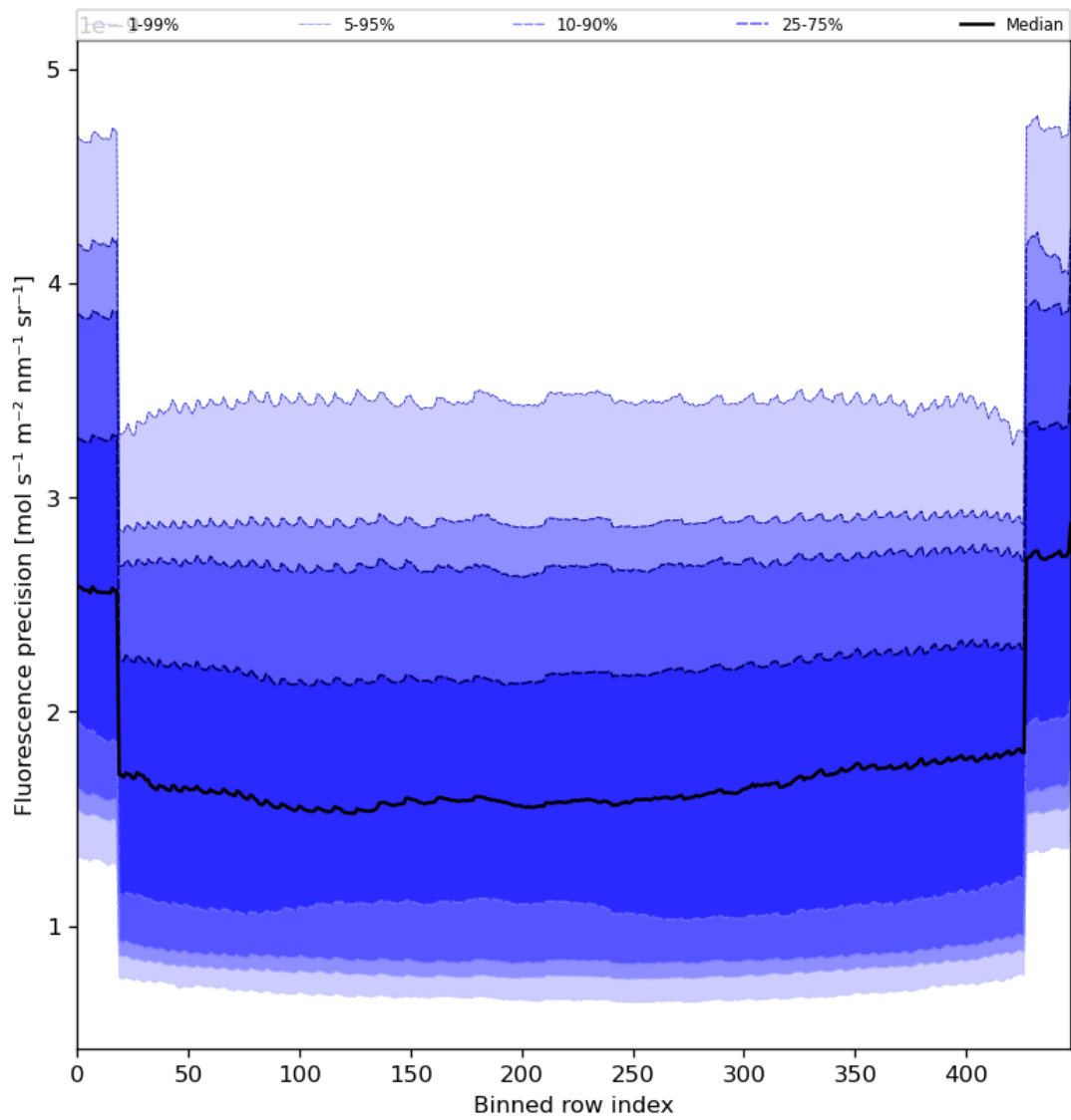
Figure 58: Along track statistics of “Fluorescence precision” for 2024-06-19 to 2024-06-20
