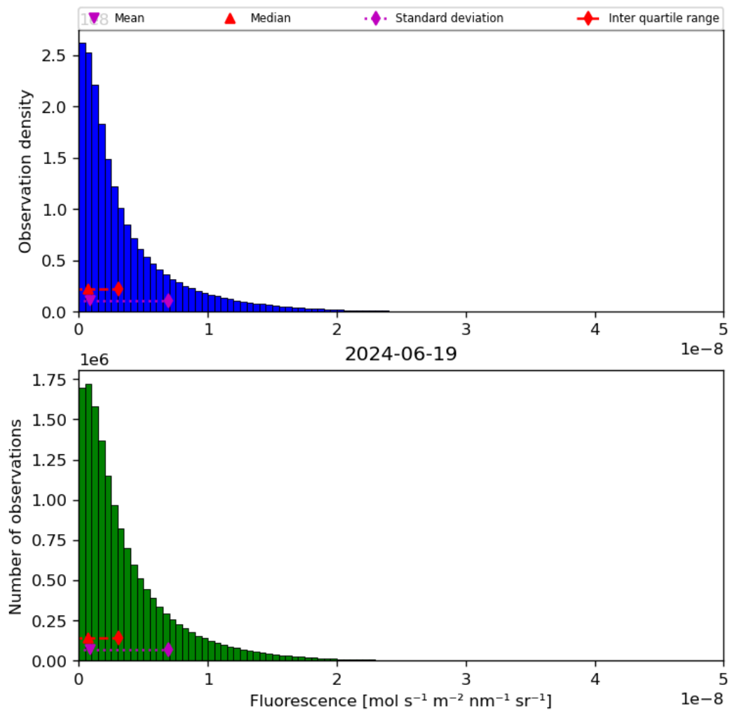
Figure 40: Histogram of “Fluorescence” for 2024-06-19 to 2024-06-20
