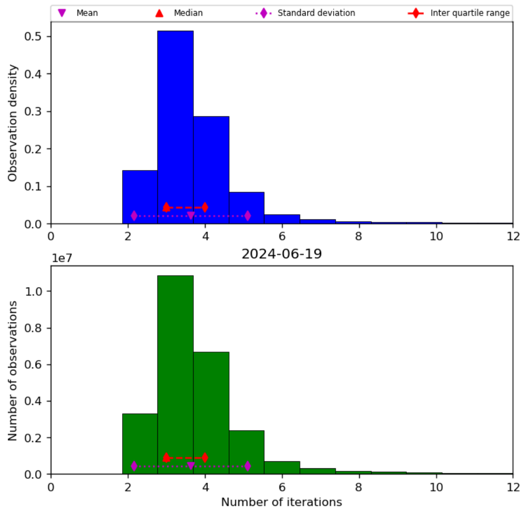
Figure 39: Histogram of “Number of iterations” for 2024-06-19 to 2024-06-20
