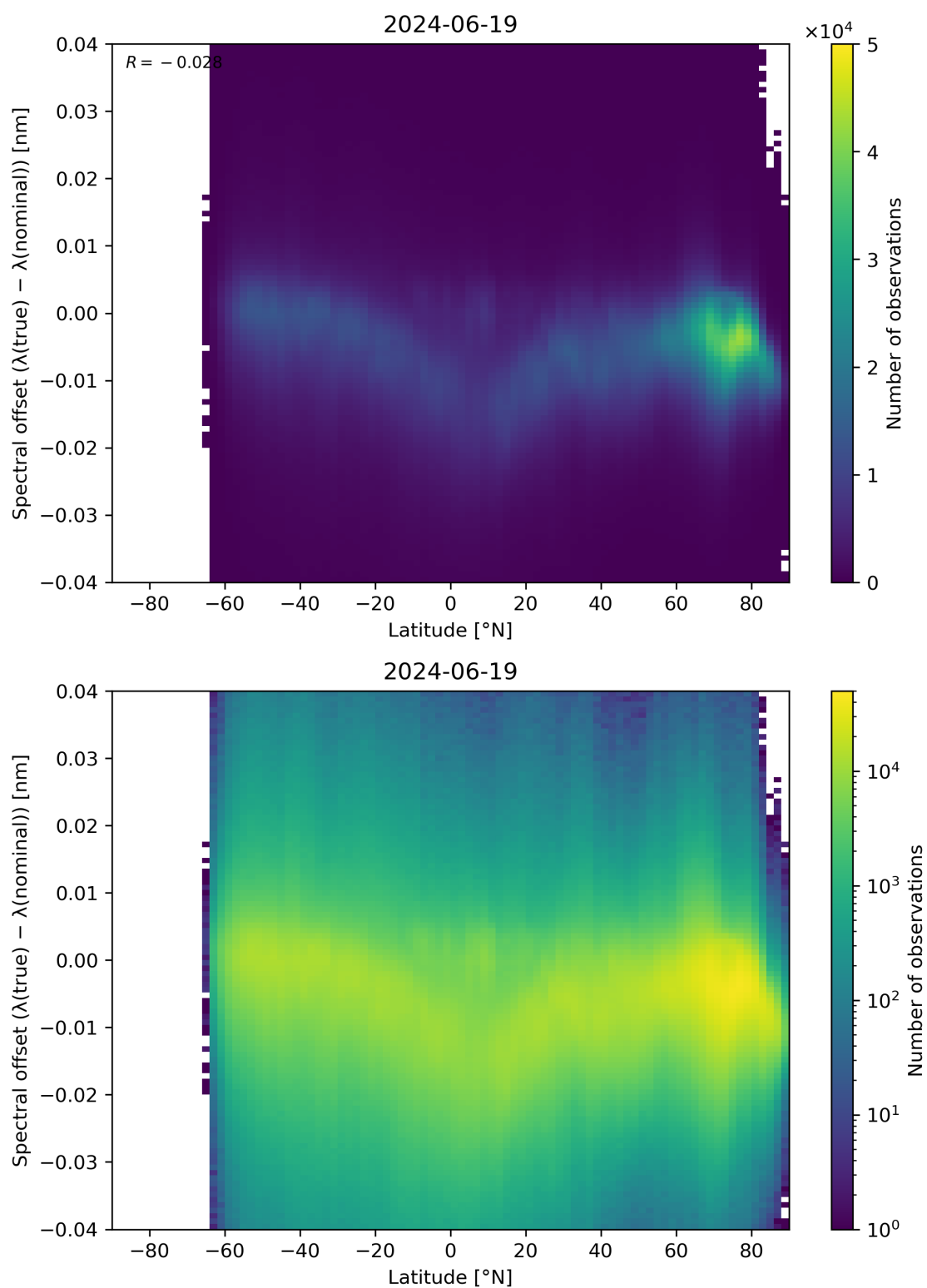
Figure 96: Scatter density plot of “Latitude” against “Spectral offset ( \lambda(\text{true}) - \lambda(\text{nominal}) )” for 2024-06-19 to 2024-06-20.
