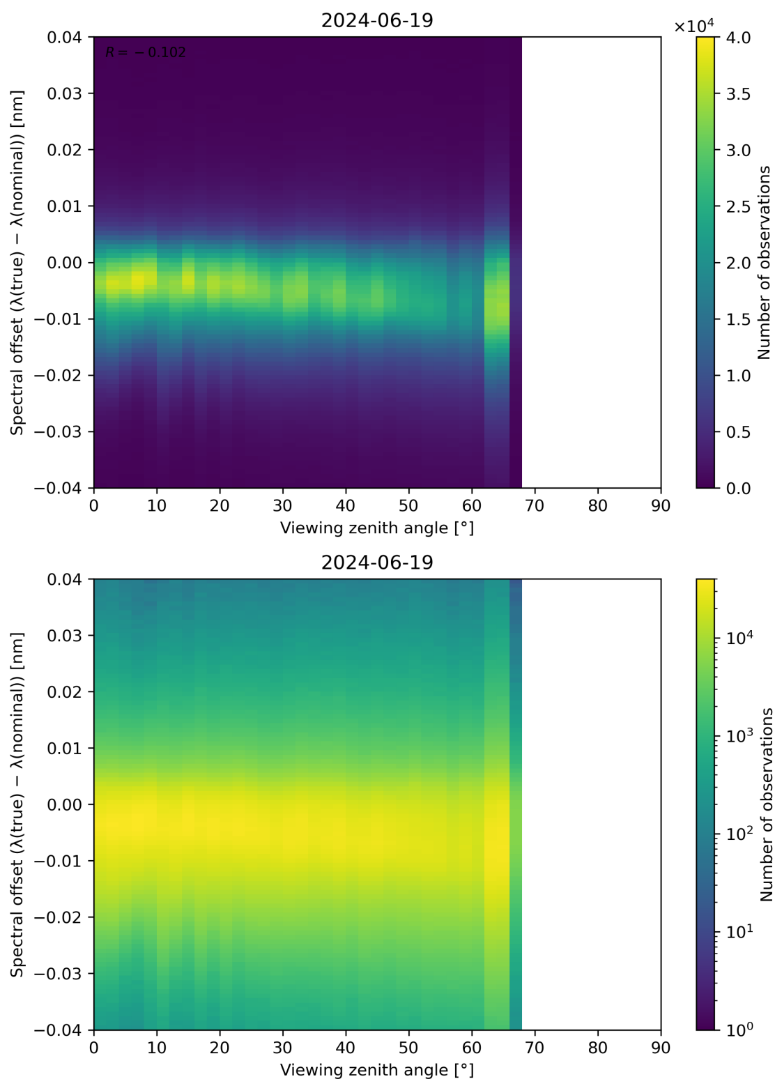
Figure 128: Scatter density plot of “Viewing zenith angle” against “Spectral offset ( \lambda(\text{true}) - \lambda(\text{nominal}) )” for 2024-06-19 to 2024-06-20.
