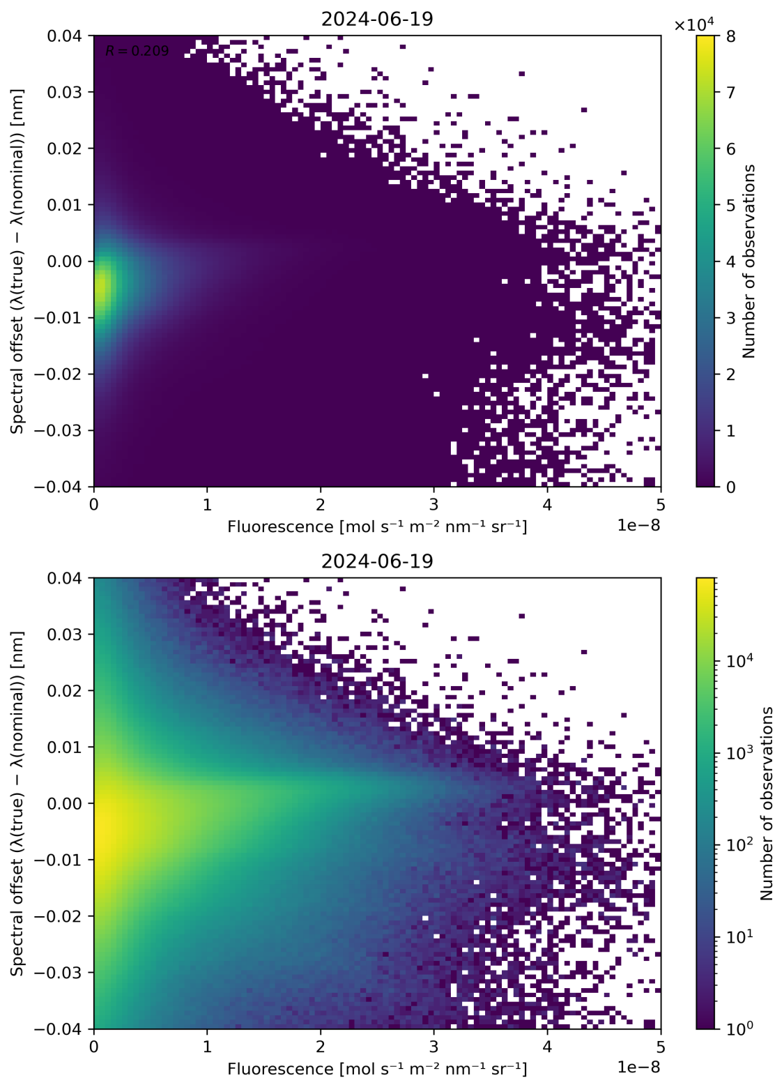
Figure 87: Scatter density plot of “Fluorescence” against “Spectral offset ( \lambda(\text{true}) - \lambda(\text{nominal}) )” for 2024-06-19 to 2024-06-20.
