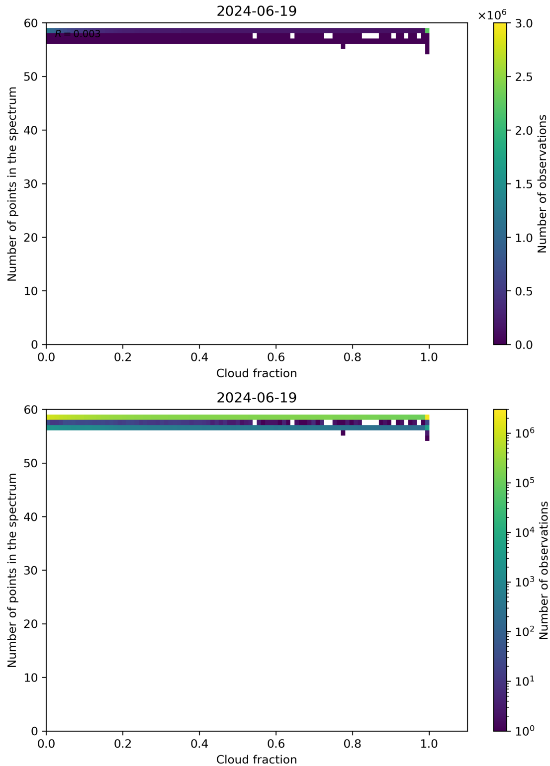
Figure 74: Scatter density plot of “Cloud fraction” against “Number of points in the spectrum” for 2024-06-19 to 2024-06-20.
