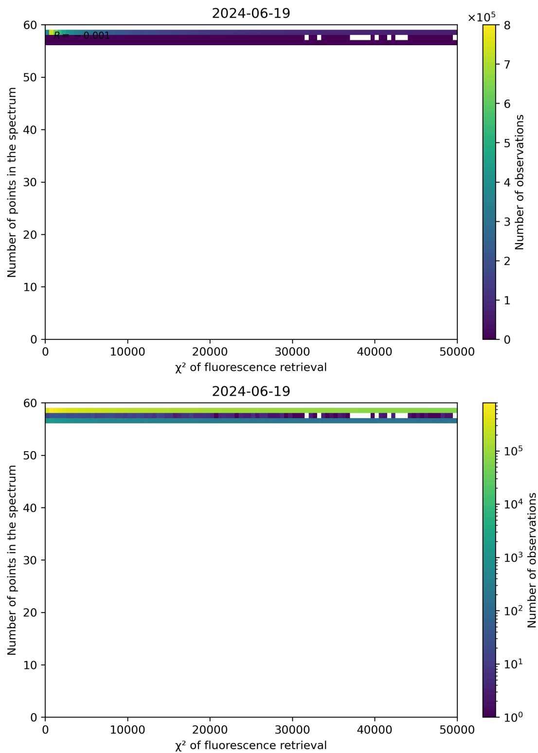
Figure 68: Scatter density plot of " \chi^2 of fluorescence retrieval" against "Number of points in the spectrum" for 2024-06-19 to 2024-06-20.
