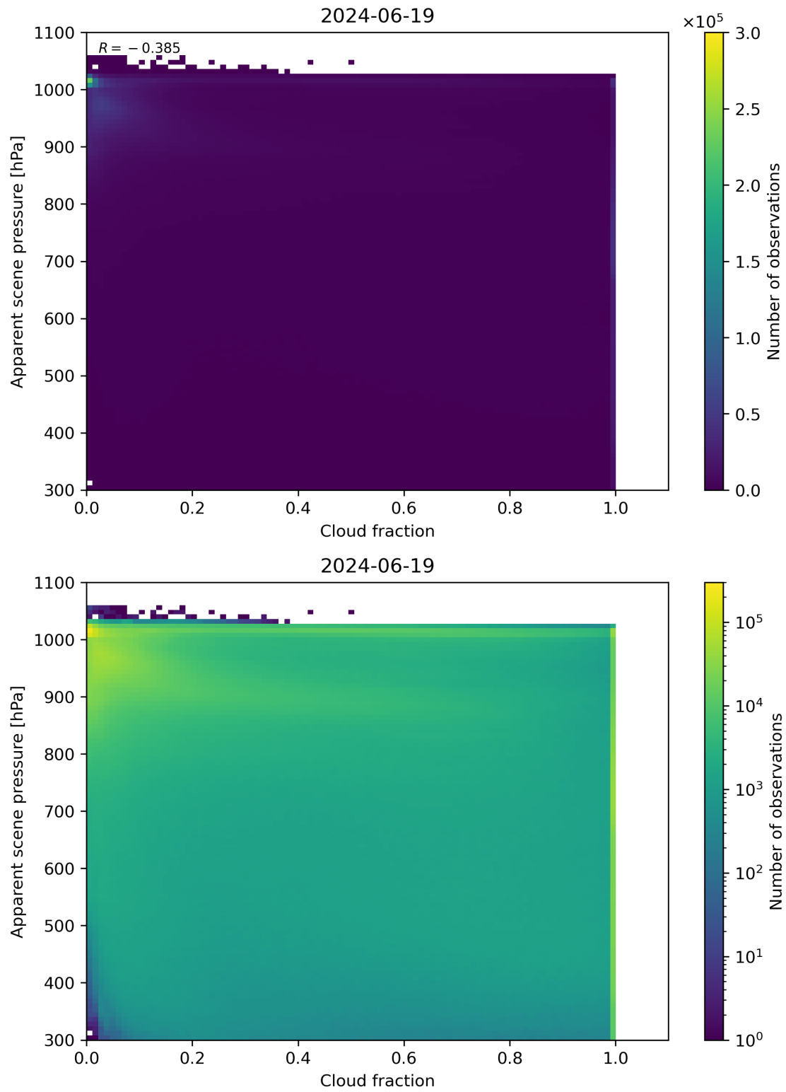
Figure 70: Scatter density plot of “Cloud fraction” against “Apparent scene pressure” for 2024-06-19 to 2024-06-20.
