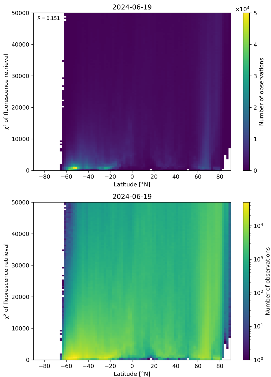
Figure 89: Scatter density plot of “Latitude” against “ \chi^2 of fluorescence retrieval” for 2024-06-19 to 2024-06-20.
