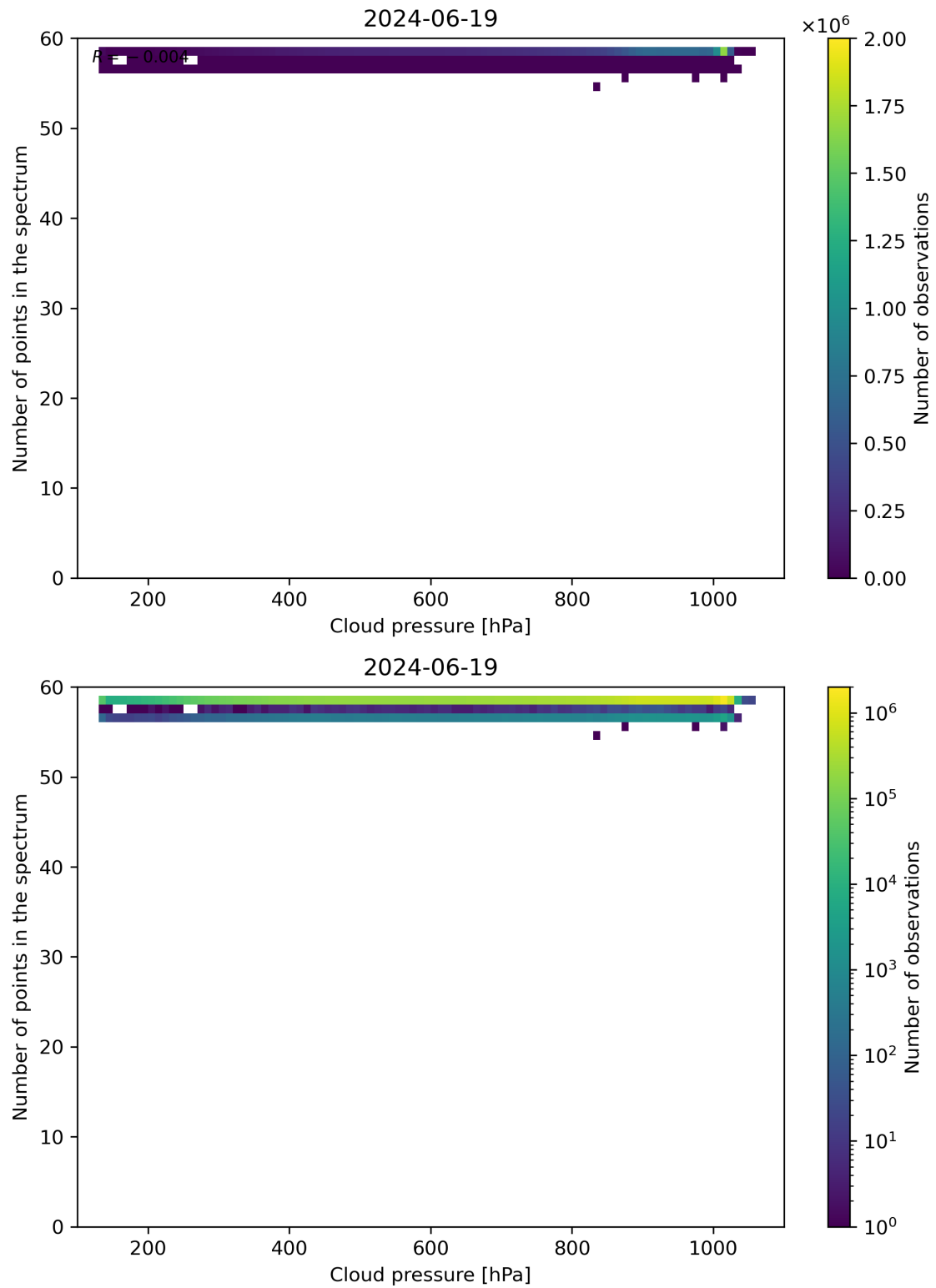
Figure 82: Scatter density plot of “Cloud pressure” against “Number of points in the spectrum” for 2024-06-19 to 2024-06-20.
