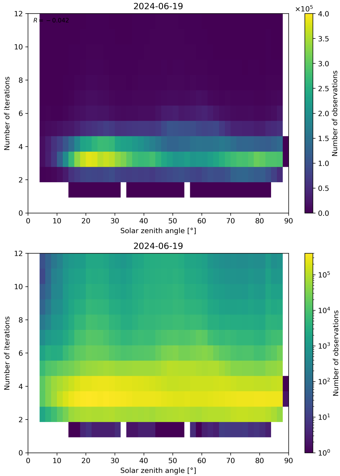
Figure 114: Scatter density plot of “Solar zenith angle” against “Number of iterations” for 2024-06-19 to 2024-06-20.
