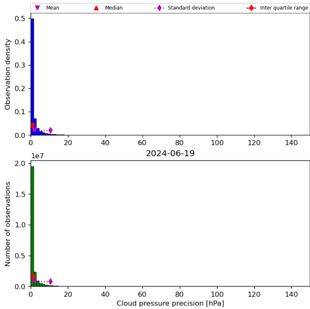
Figure 31: Histogram of “Cloud pressure precision” for 2024-06-19 to 2024-06-20
