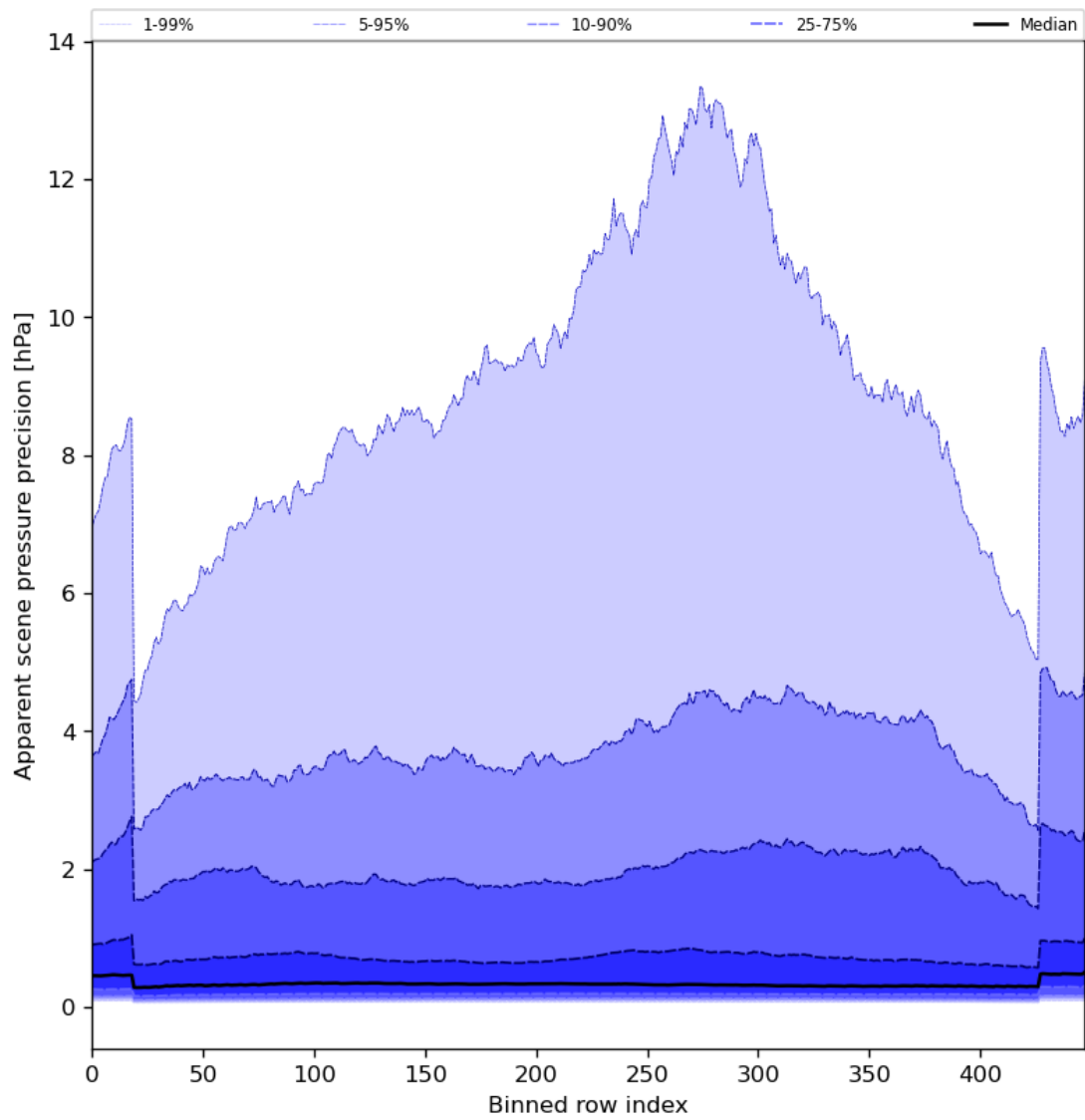
Figure 54: Along track statistics of “Apparent scene pressure precision” for 2024-06-19 to 2024-06-20
