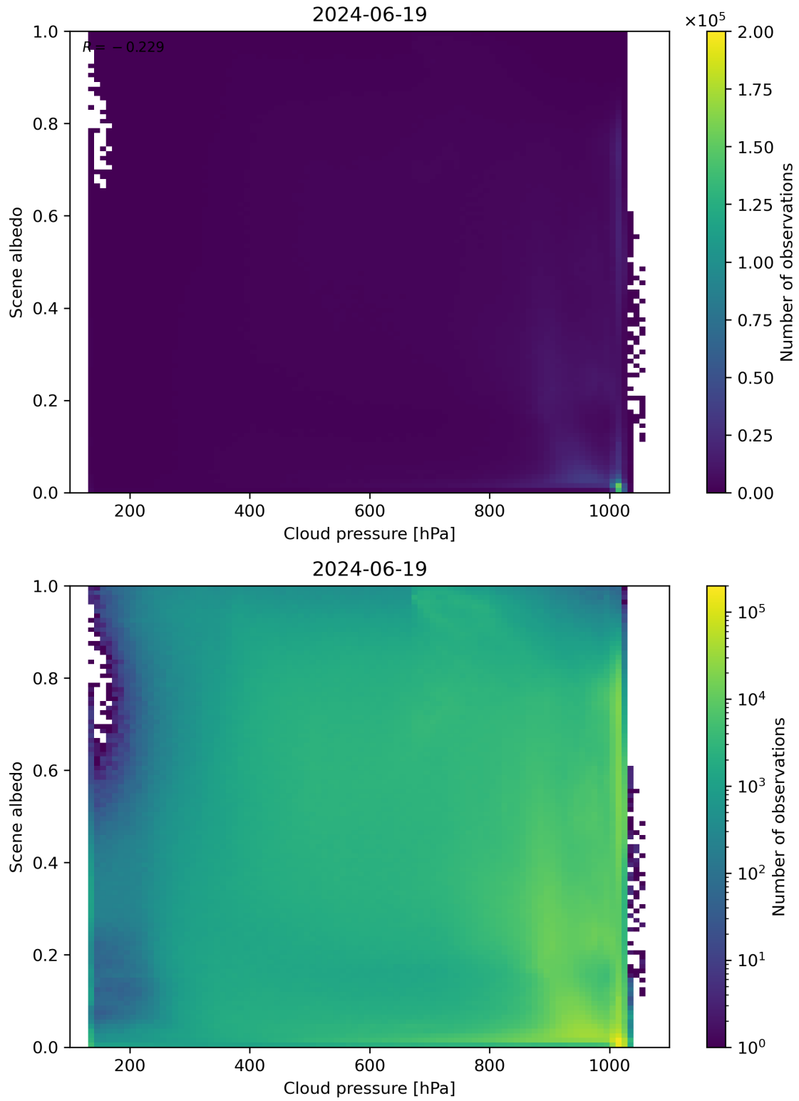
Figure 83: Scatter density plot of “Cloud pressure” against “Scene albedo” for 2024-06-19 to 2024-06-20.
