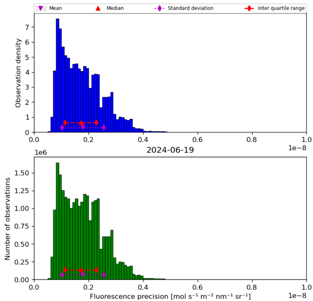
Figure 41: Histogram of “Fluorescence precision” for 2024-06-19 to 2024-06-20
