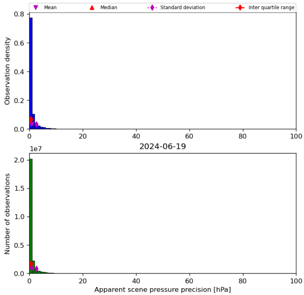
Figure 37: Histogram of “Apparent scene pressure precision” for 2024-06-19 to 2024-06-20
