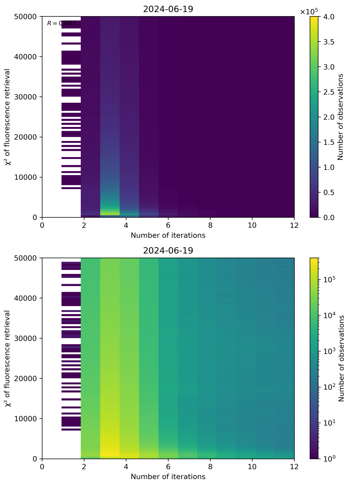
Figure 97: Scatter density plot of “Number of iterations” against “ \chi^2 of fluorescence retrieval” for 2024-06-19 to 2024-06-20.
