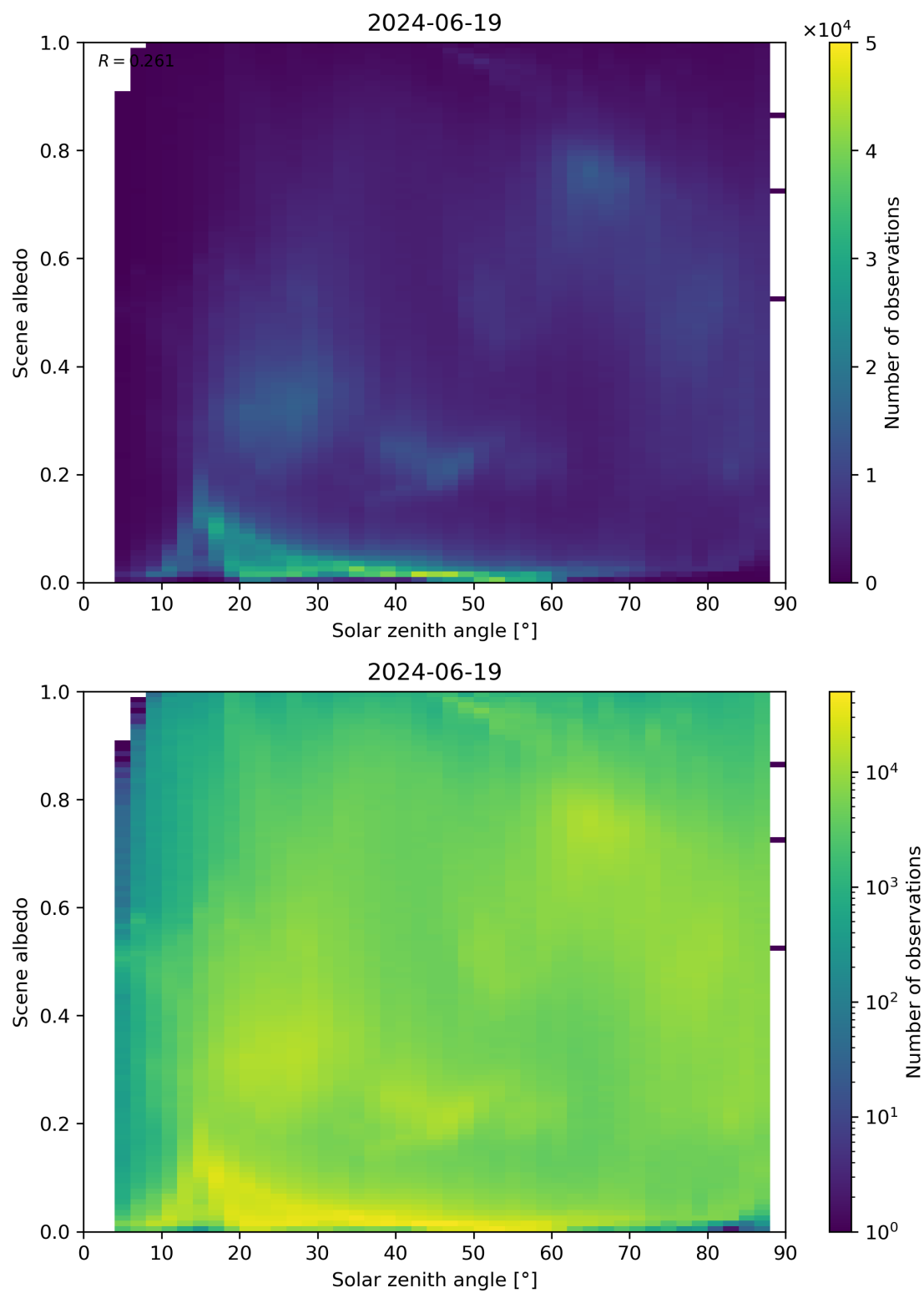
Figure 116: Scatter density plot of “Solar zenith angle” against “Scene albedo” for 2024-06-19 to 2024-06-20.
