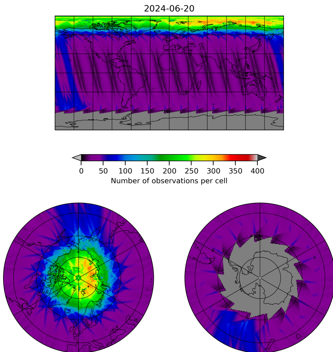
Figure 11: Map of the number of observations for 2024-06-19 to 2024-06-21
