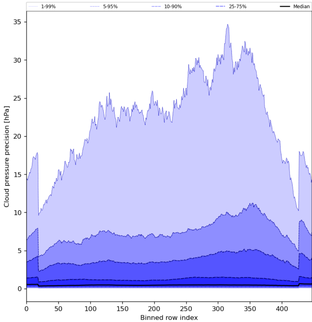
Figure 48: Along track statistics of “Cloud pressure precision” for 2024-06-19 to 2024-06-21
