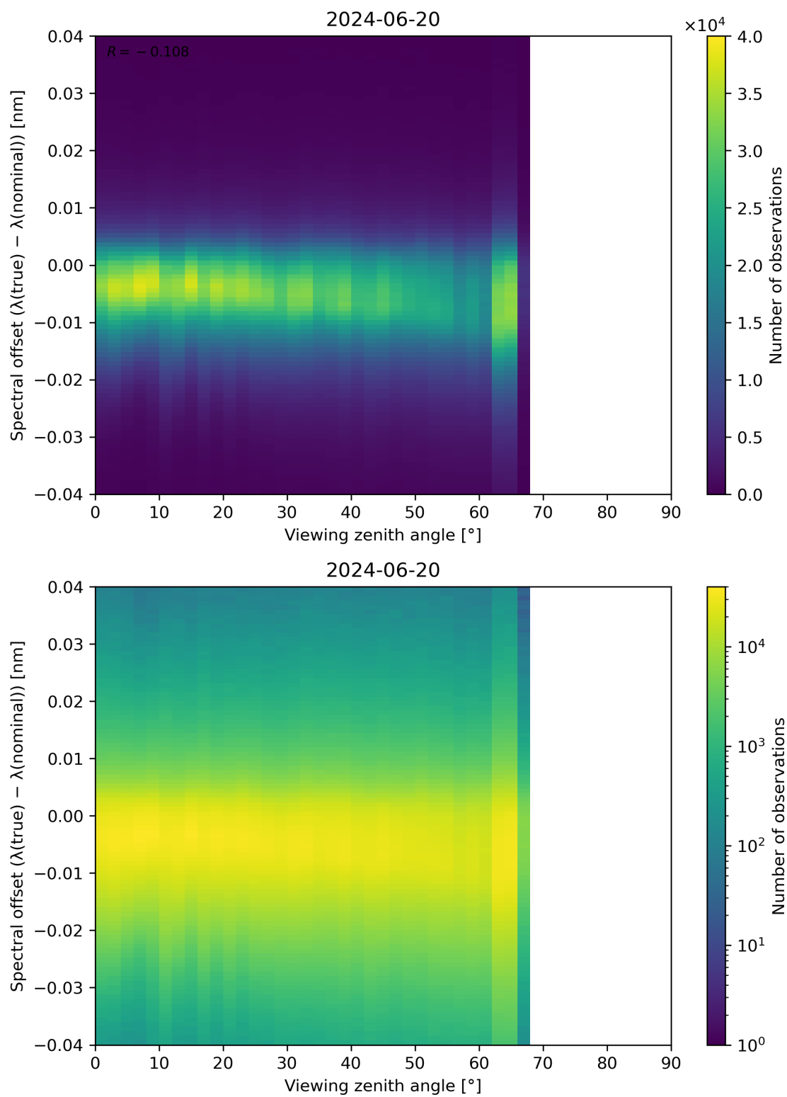
Figure 128: Scatter density plot of “Viewing zenith angle” against “Spectral offset ( \lambda(\text{true}) - \lambda(\text{nominal}) )” for 2024-06-19 to 2024-06-21.
