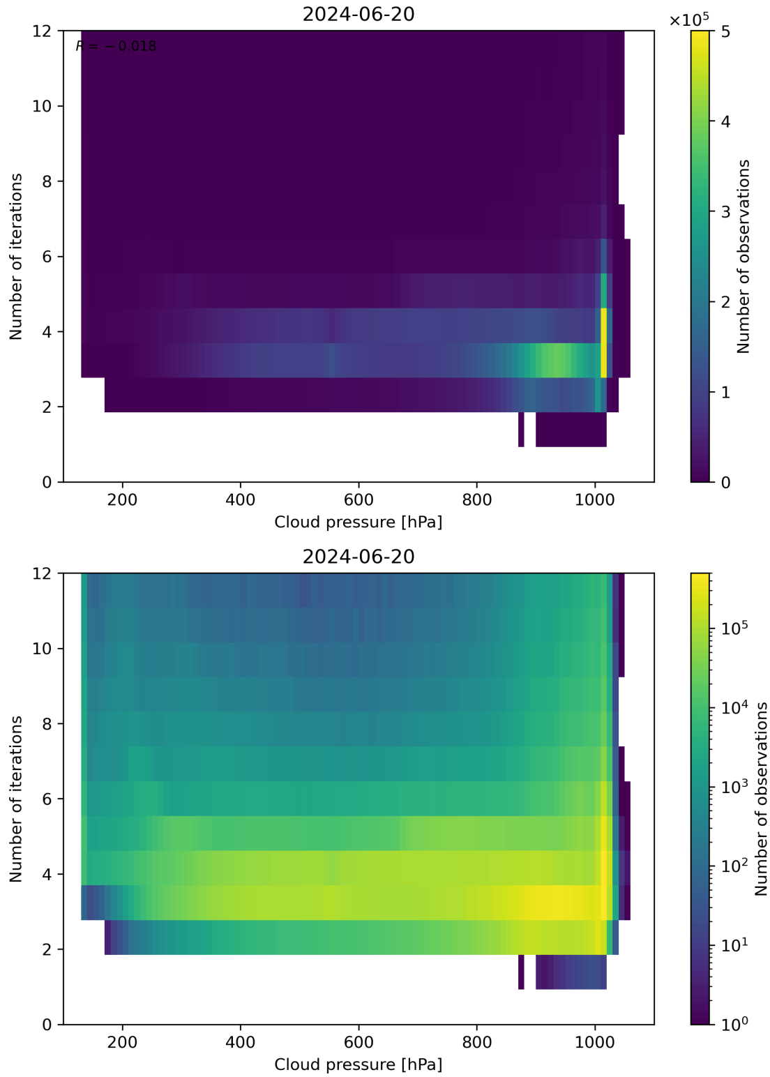
Figure 81: Scatter density plot of “Cloud pressure” against “Number of iterations” for 2024-06-19 to 2024-06-21.
