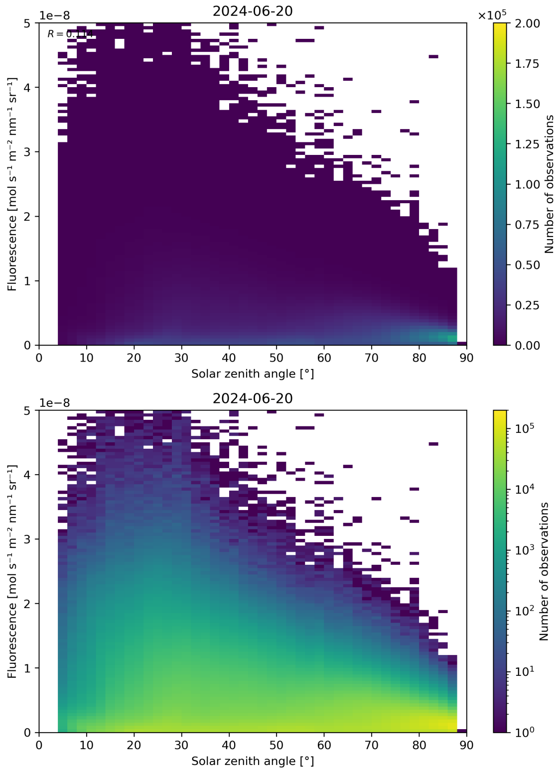
Figure 112: Scatter density plot of “Solar zenith angle” against “Fluorescence” for 2024-06-19 to 2024-06-21.
