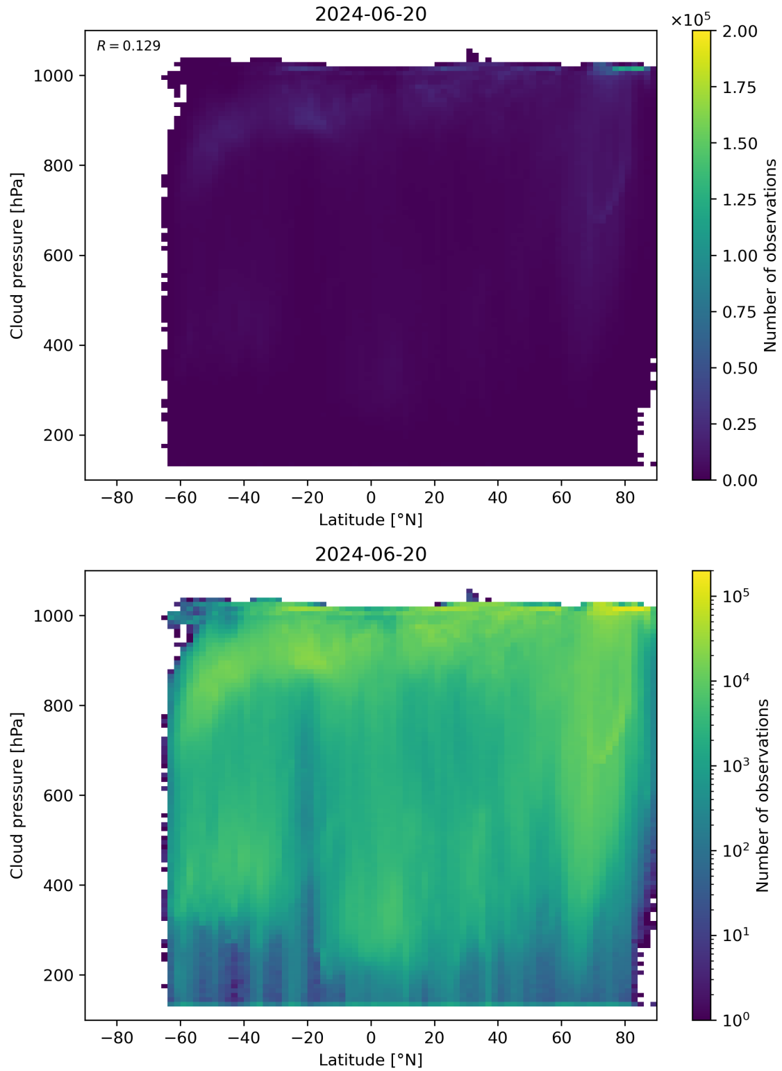
Figure 91: Scatter density plot of “Latitude” against “Cloud pressure” for 2024-06-19 to 2024-06-21.
