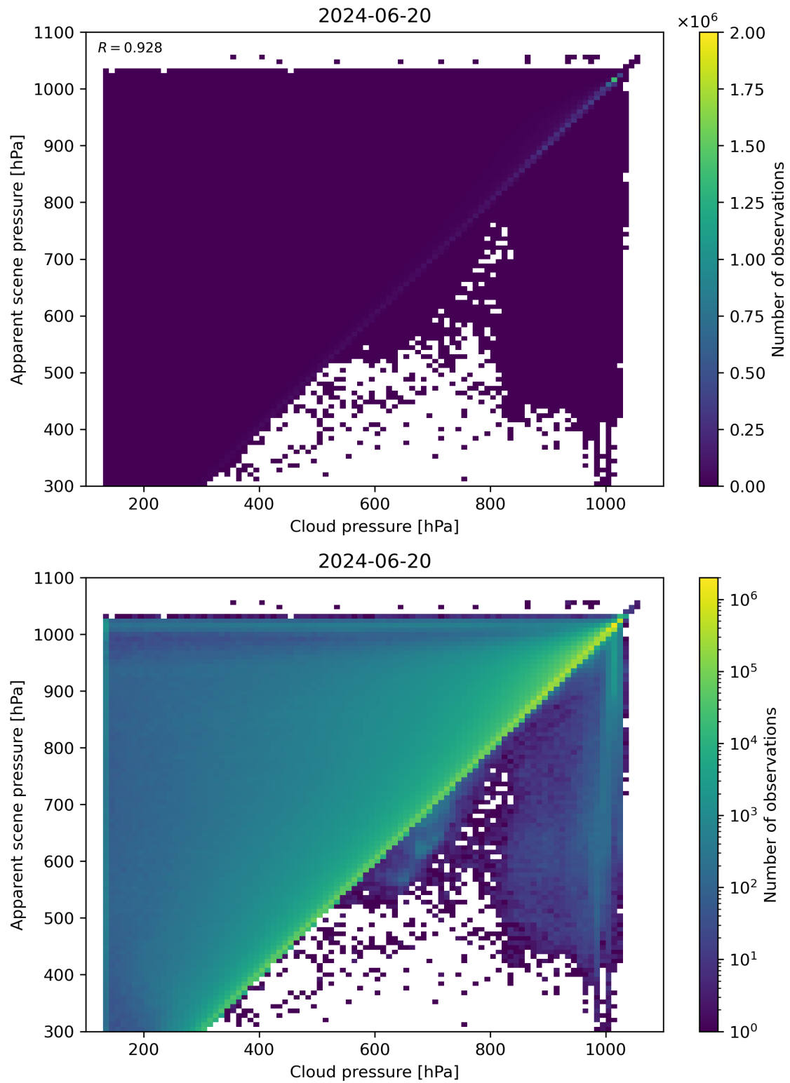
Figure 77: Scatter density plot of “Cloud pressure” against “Apparent scene pressure” for 2024-06-19 to 2024-06-21.
