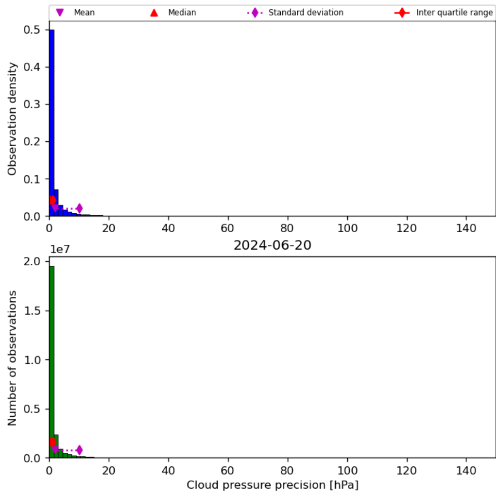
Figure 31: Histogram of “Cloud pressure precision” for 2024-06-19 to 2024-06-21
