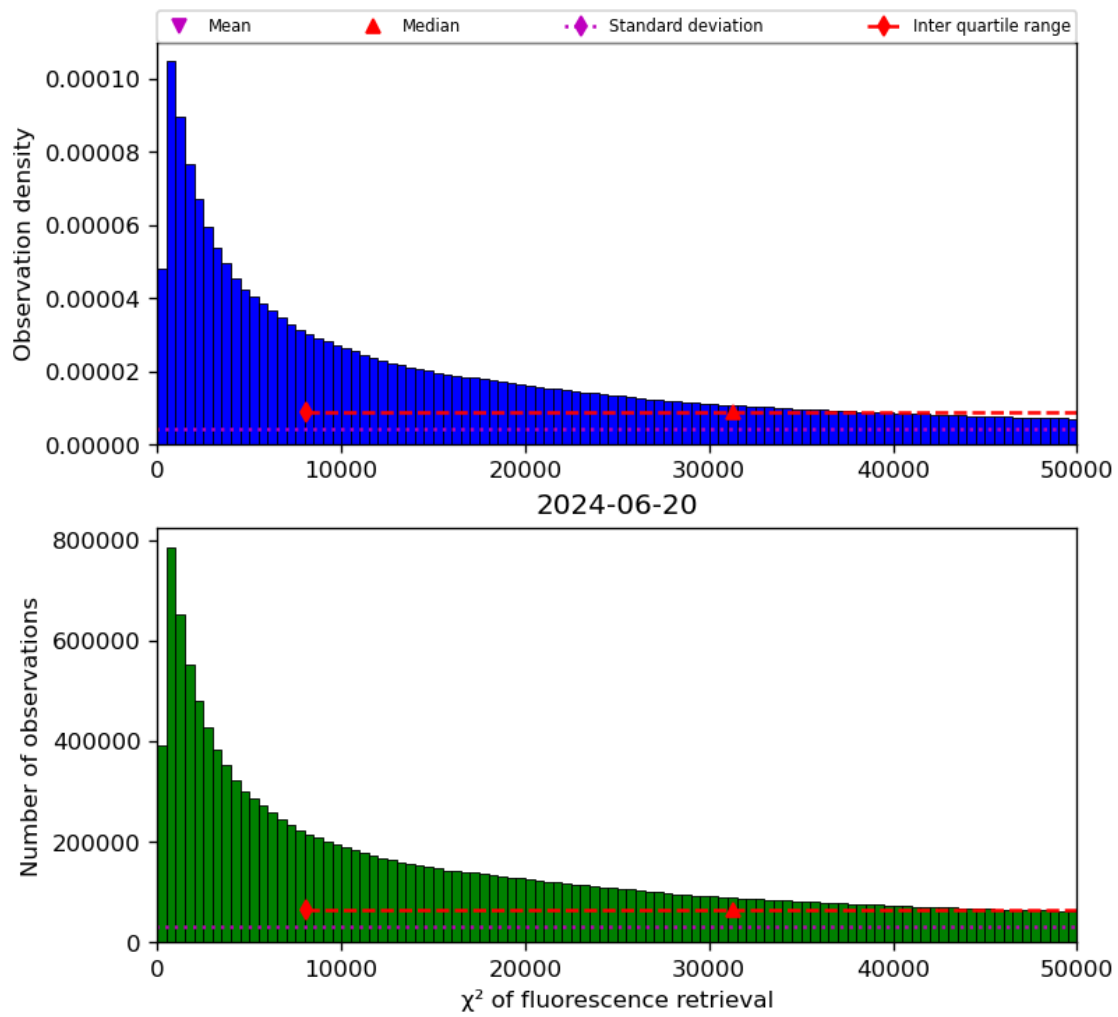
Figure 42: Histogram of “ \chi^2 of fluorescence retrieval” for 2024-06-19 to 2024-06-21
