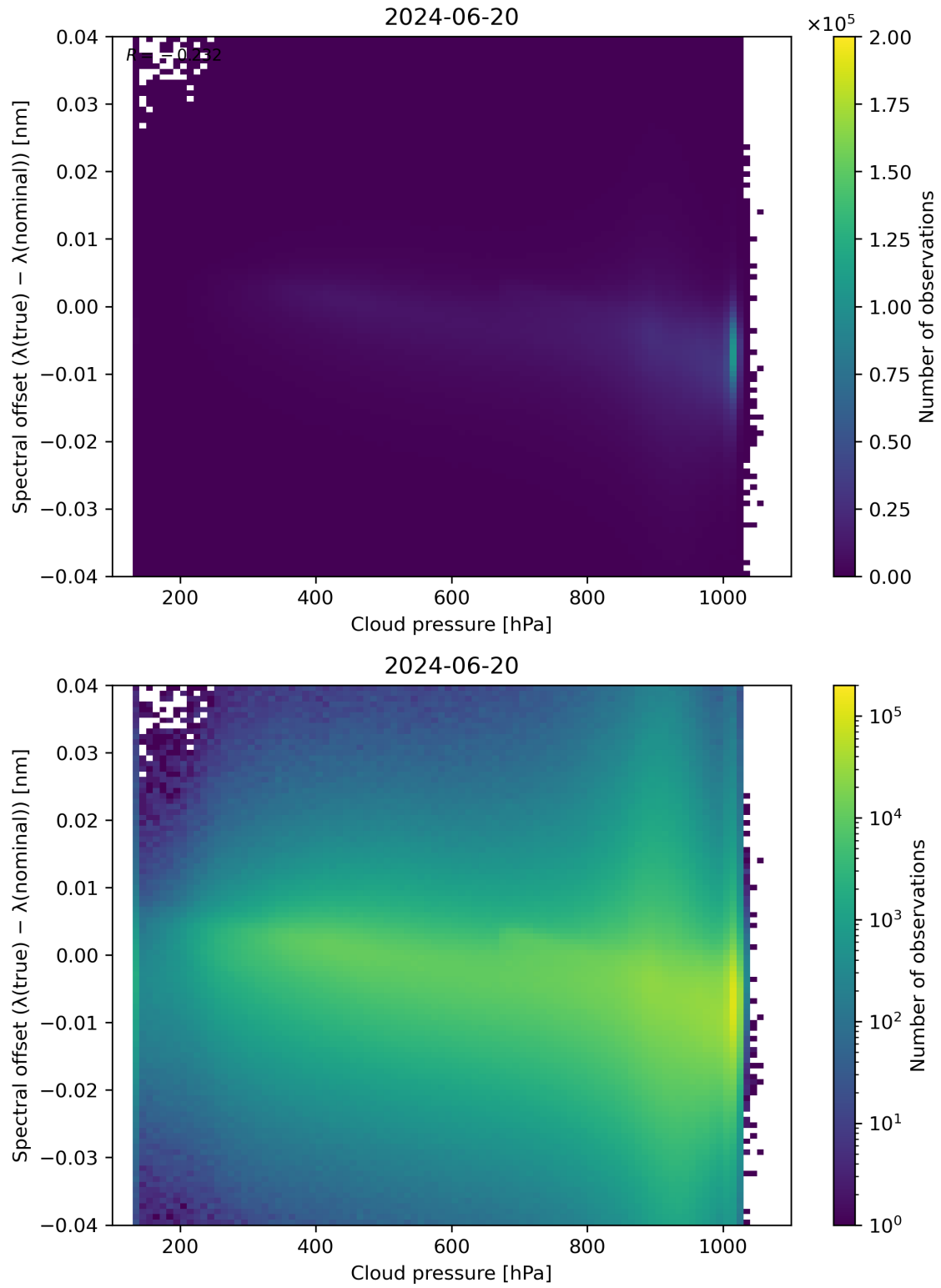
Figure 84: Scatter density plot of “Cloud pressure” against “Spectral offset ( \lambda(\text{true}) - \lambda(\text{nominal}) )” for 2024-06-19 to 2024-06-21.
