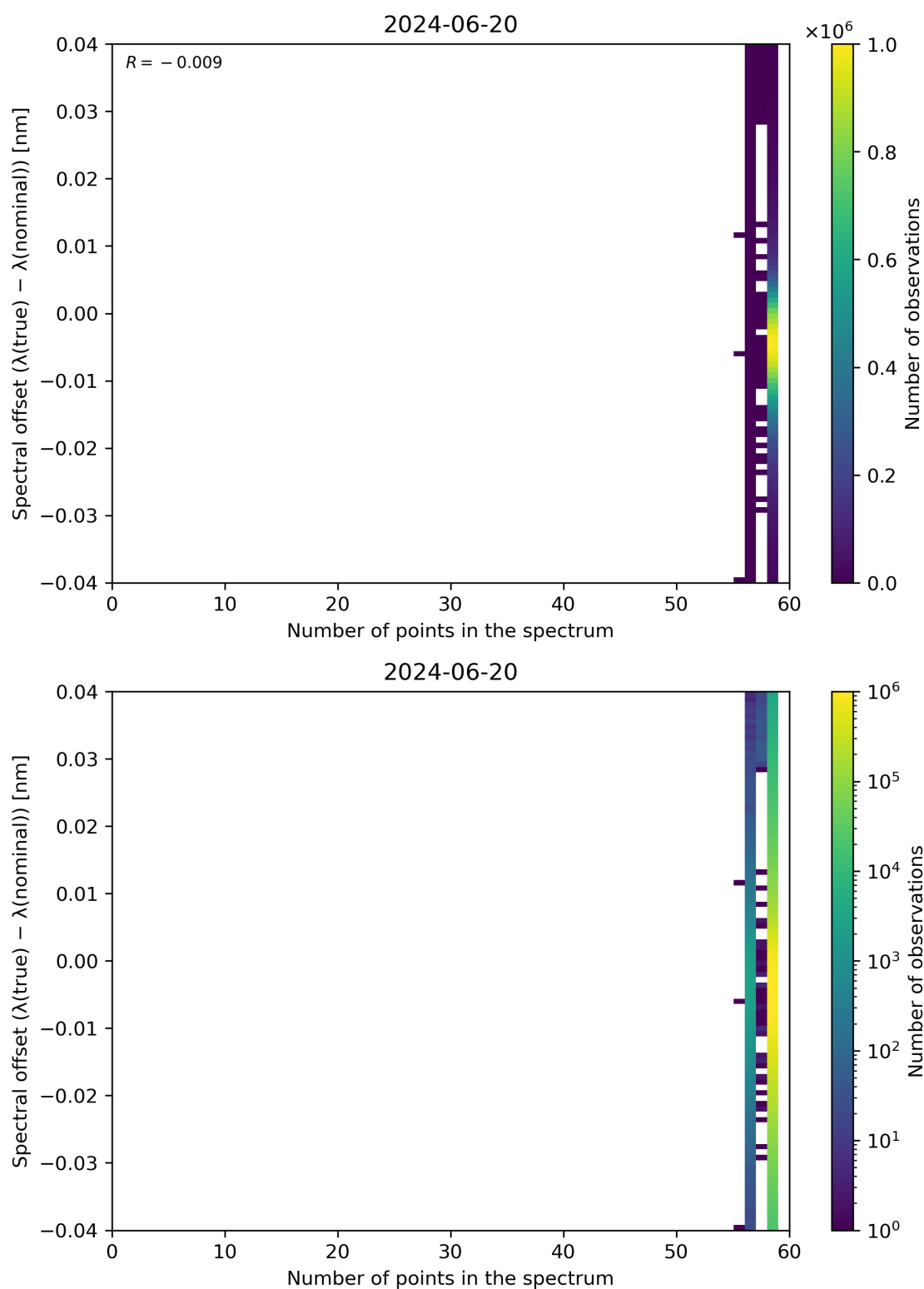
Figure 101: Scatter density plot of “Number of points in the spectrum” against “Spectral offset ( \lambda(\text{true}) - \lambda(\text{nominal}) )” for 2024-06-19 to 2024-06-21.
