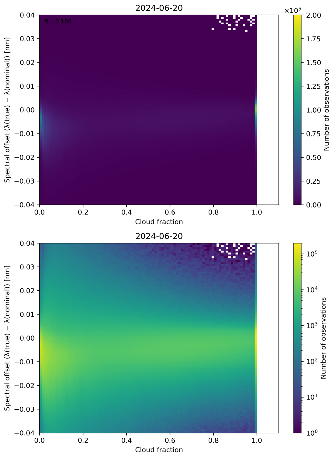
Figure 76: Scatter density plot of “Cloud fraction” against “Spectral offset ( \lambda(\text{true}) - \lambda(\text{nominal}) )” for 2024-06-19 to 2024-06-21.
