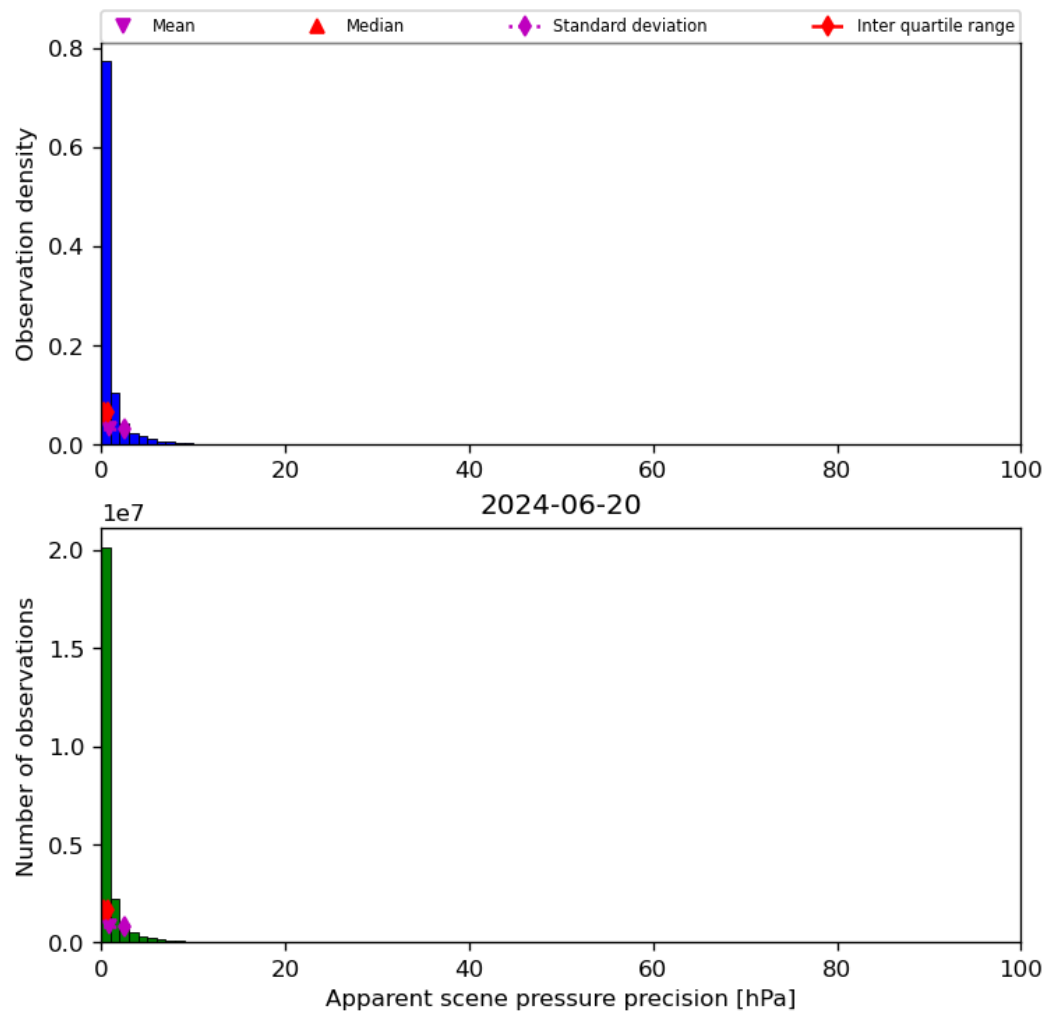
Figure 37: Histogram of “Apparent scene pressure precision” for 2024-06-19 to 2024-06-21
