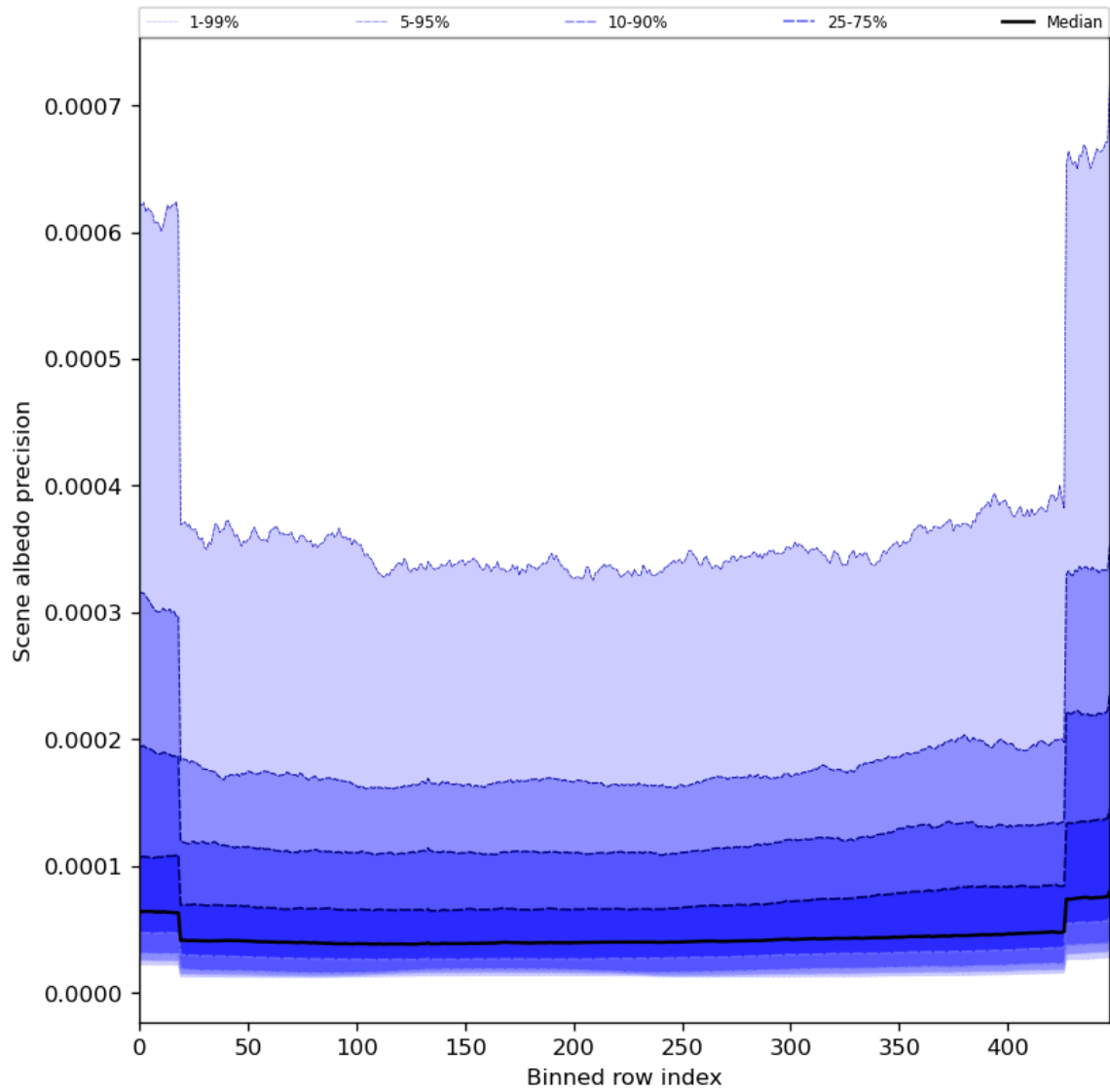
Figure 52: Along track statistics of “Scene albedo precision” for 2024-06-19 to 2024-06-21
