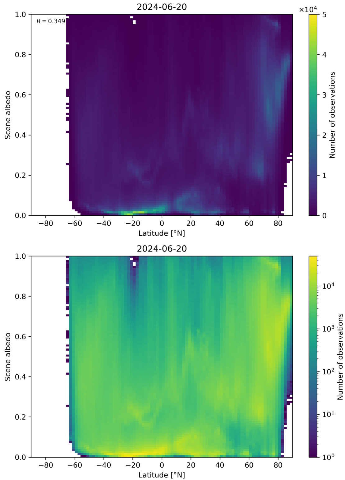
Figure 95: Scatter density plot of “Latitude” against “Scene albedo” for 2024-06-19 to 2024-06-21.
