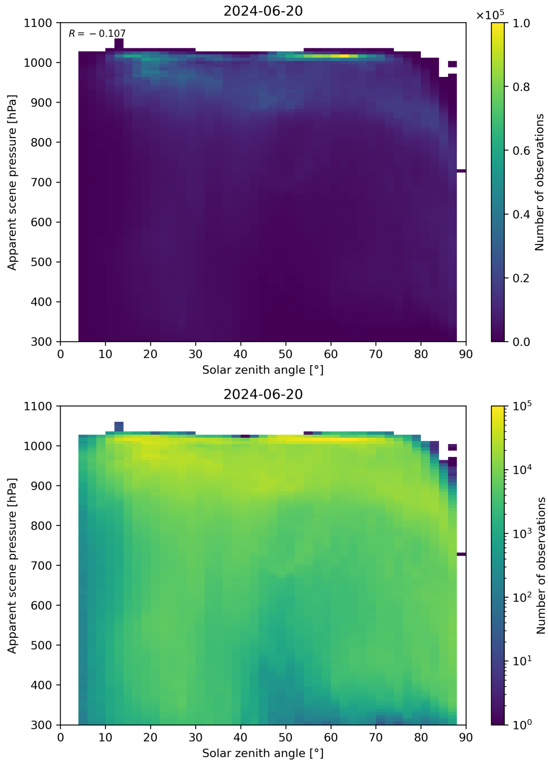
Figure 108: Scatter density plot of “Solar zenith angle” against “Apparent scene pressure” for 2024-06-19 to 2024-06-21.
