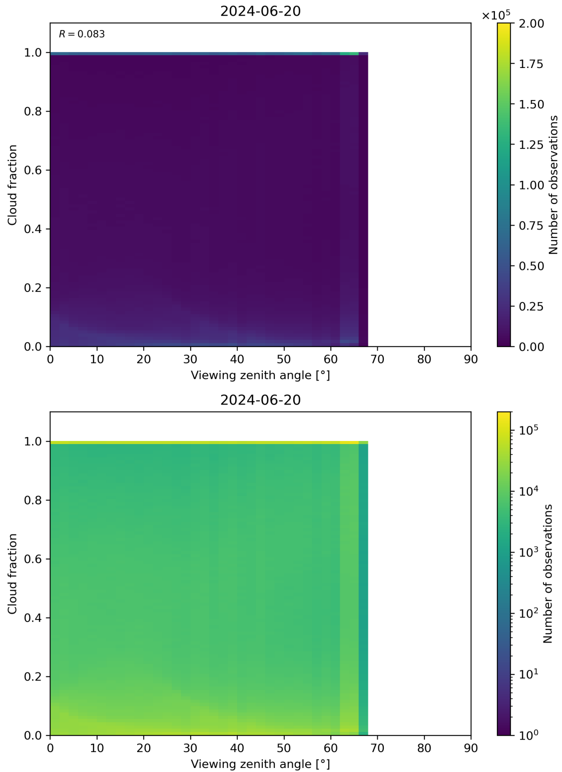
Figure 120: Scatter density plot of “Viewing zenith angle” against “Cloud fraction” for 2024-06-19 to 2024-06-21.
