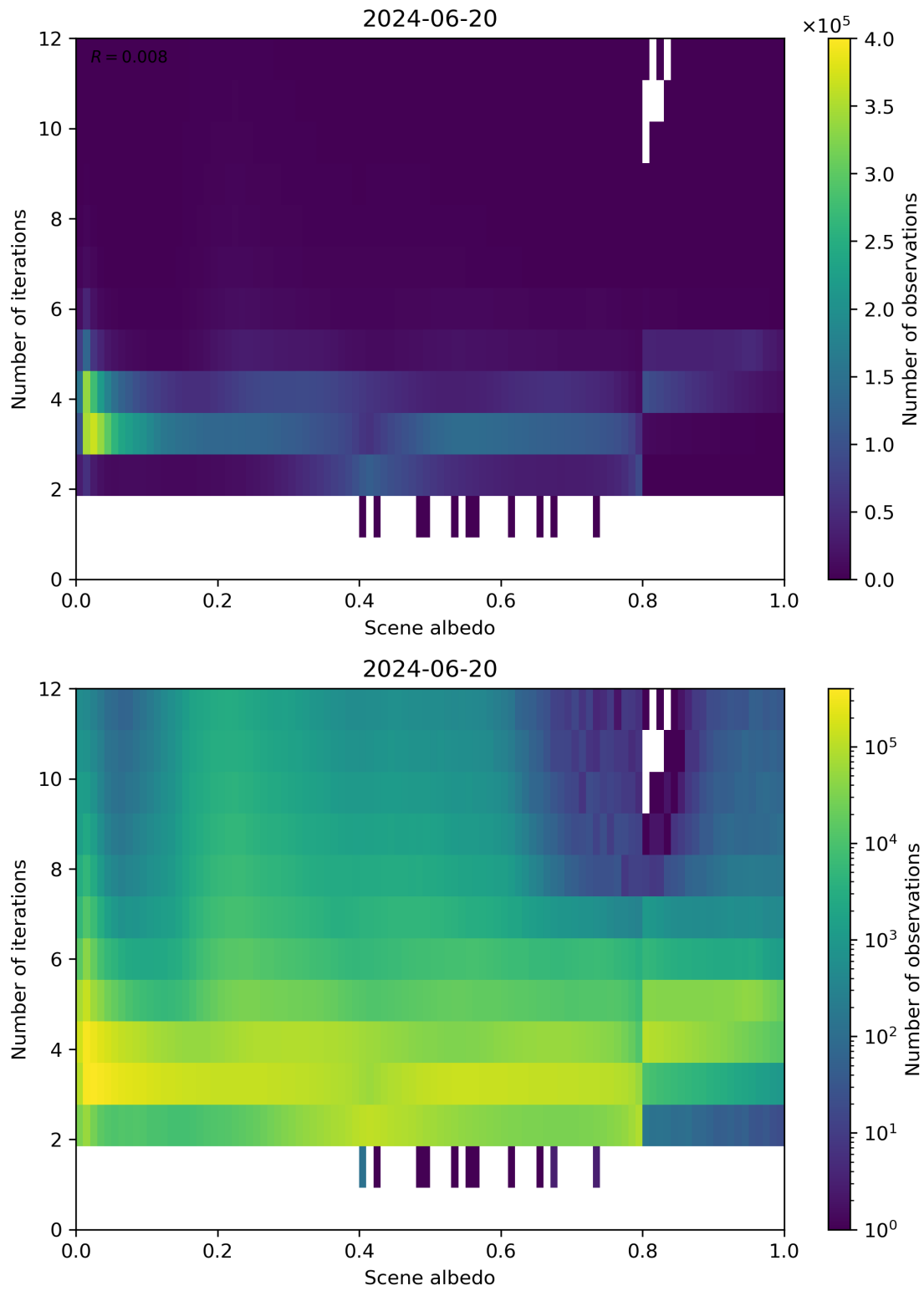
Figure 105: Scatter density plot of “Scene albedo” against “Number of iterations” for 2024-06-19 to 2024-06-21.
