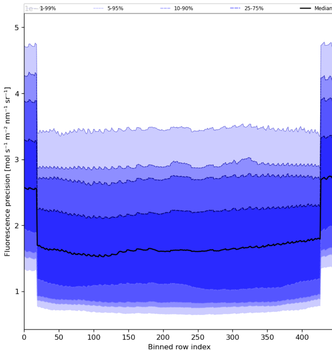
Figure 58: Along track statistics of “Fluorescence precision” for 2024-06-19 to 2024-06-21
