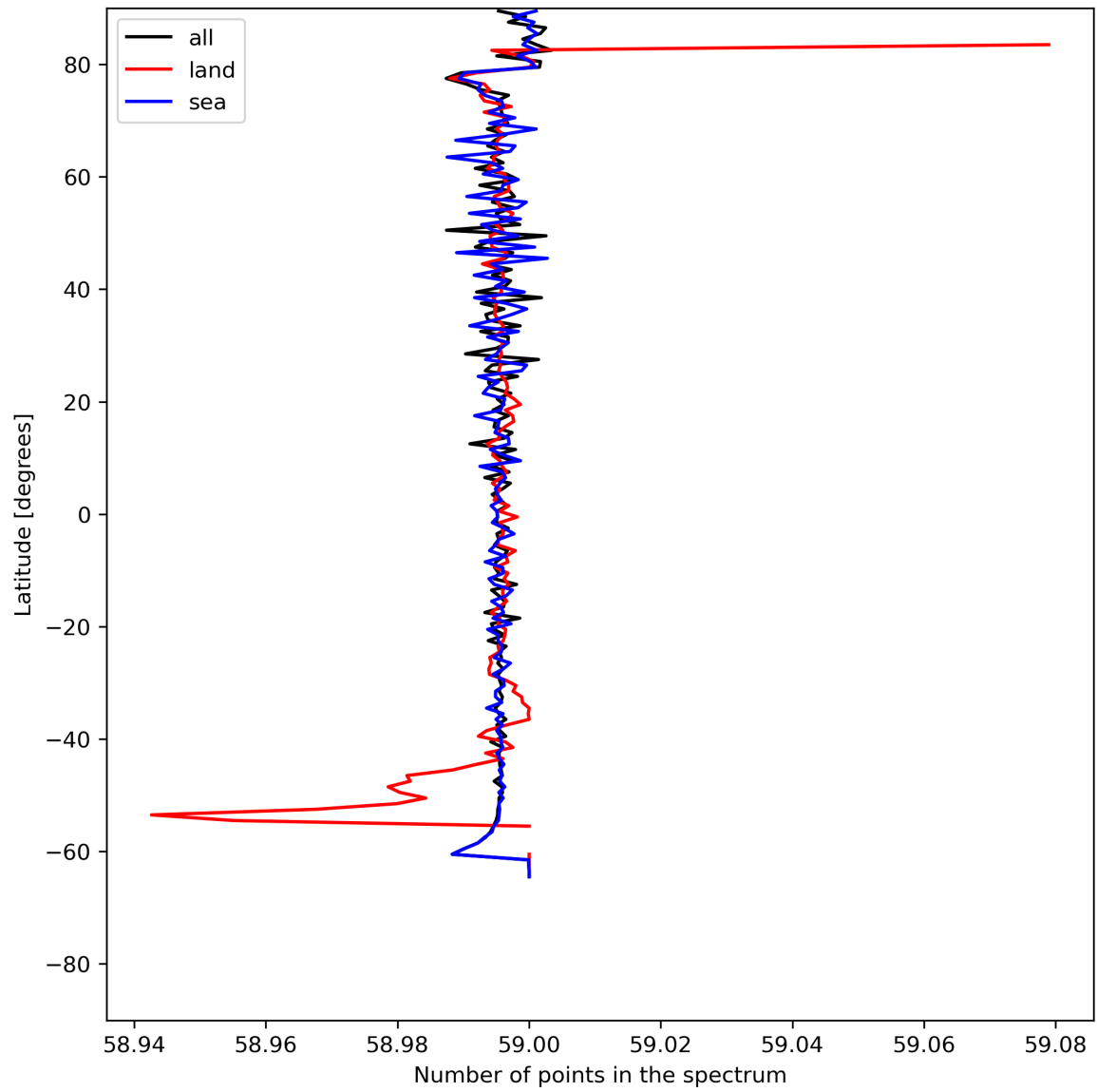
Figure 27: Zonal average of “Number of points in the spectrum” for 2024-06-19 to 2024-06-21.
