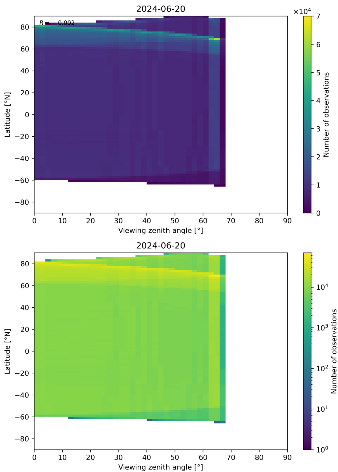
Figure 123: Scatter density plot of “Viewing zenith angle” against “Latitude” for 2024-06-19 to 2024-06-21.
