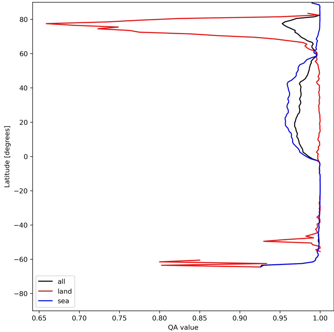
Figure 12: Zonal average of “QA value” for 2024-06-19 to 2024-06-21.
