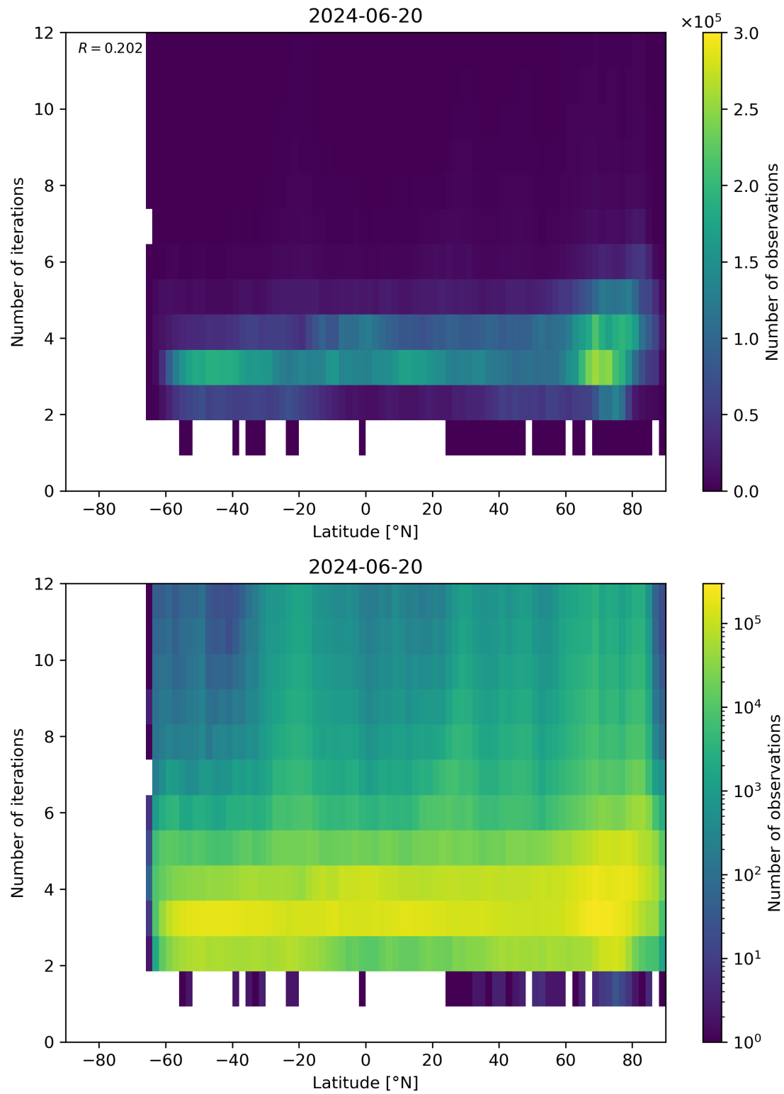
Figure 93: Scatter density plot of “Latitude” against “Number of iterations” for 2024-06-19 to 2024-06-21.
