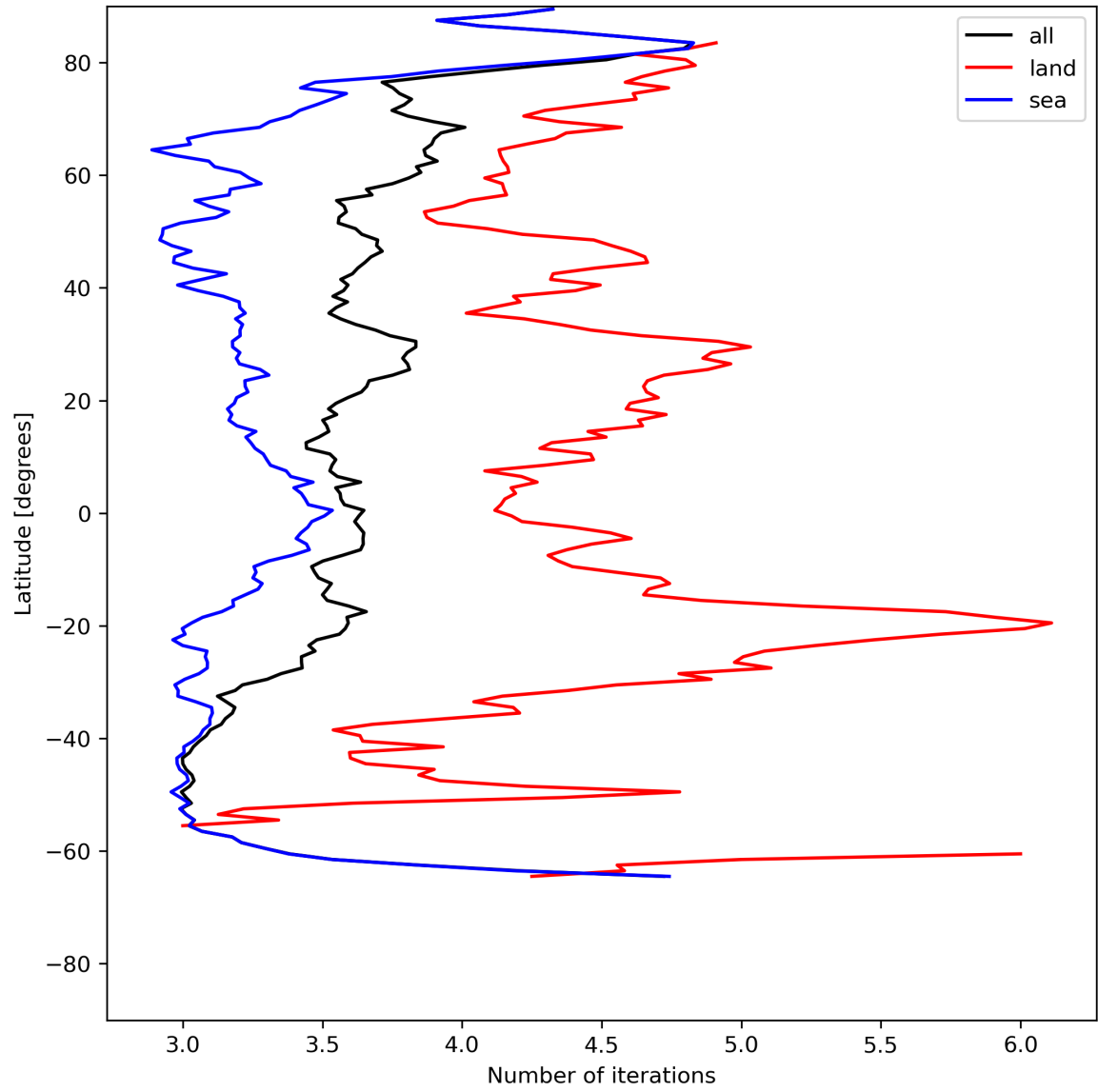
Figure 22: Zonal average of “Number of iterations” for 2024-06-19 to 2024-06-21.
