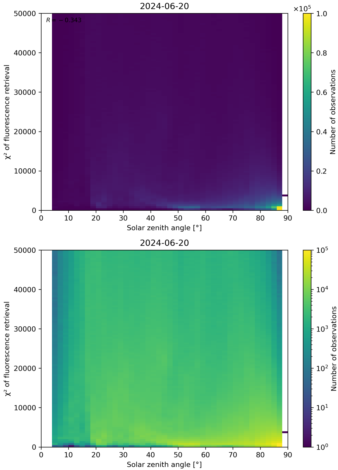
Figure 109: Scatter density plot of “Solar zenith angle” against “ \chi^2 of fluorescence retrieval” for 2024-06-19 to 2024-06-21.
