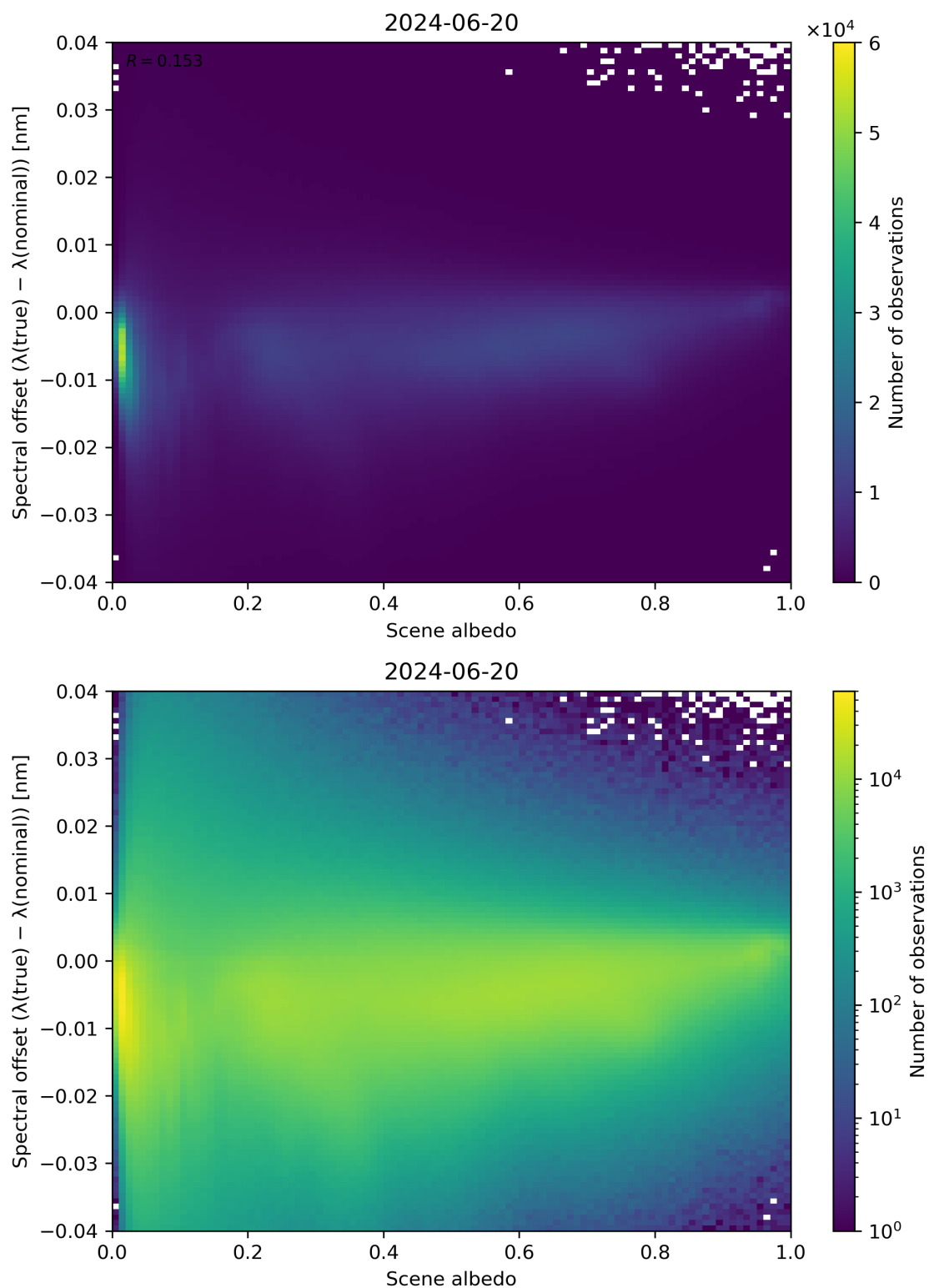
Figure 107: Scatter density plot of “Scene albedo” against “Spectral offset ( \lambda(\text{true}) - \lambda(\text{nominal}) )” for 2024-06-19 to 2024-06-21.
