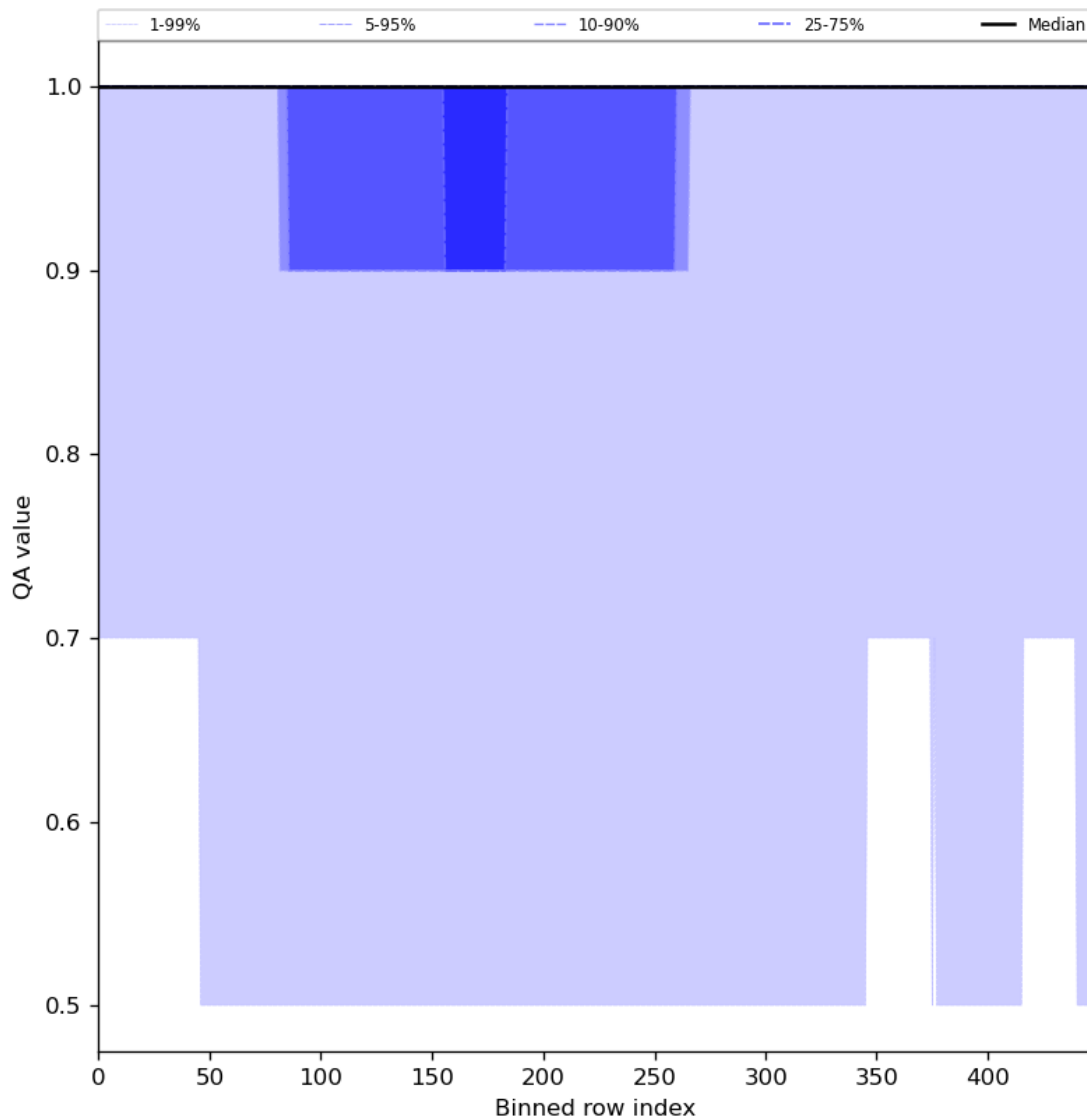
Figure 46: Along track statistics of “QA value” for 2024-06-19 to 2024-06-21
