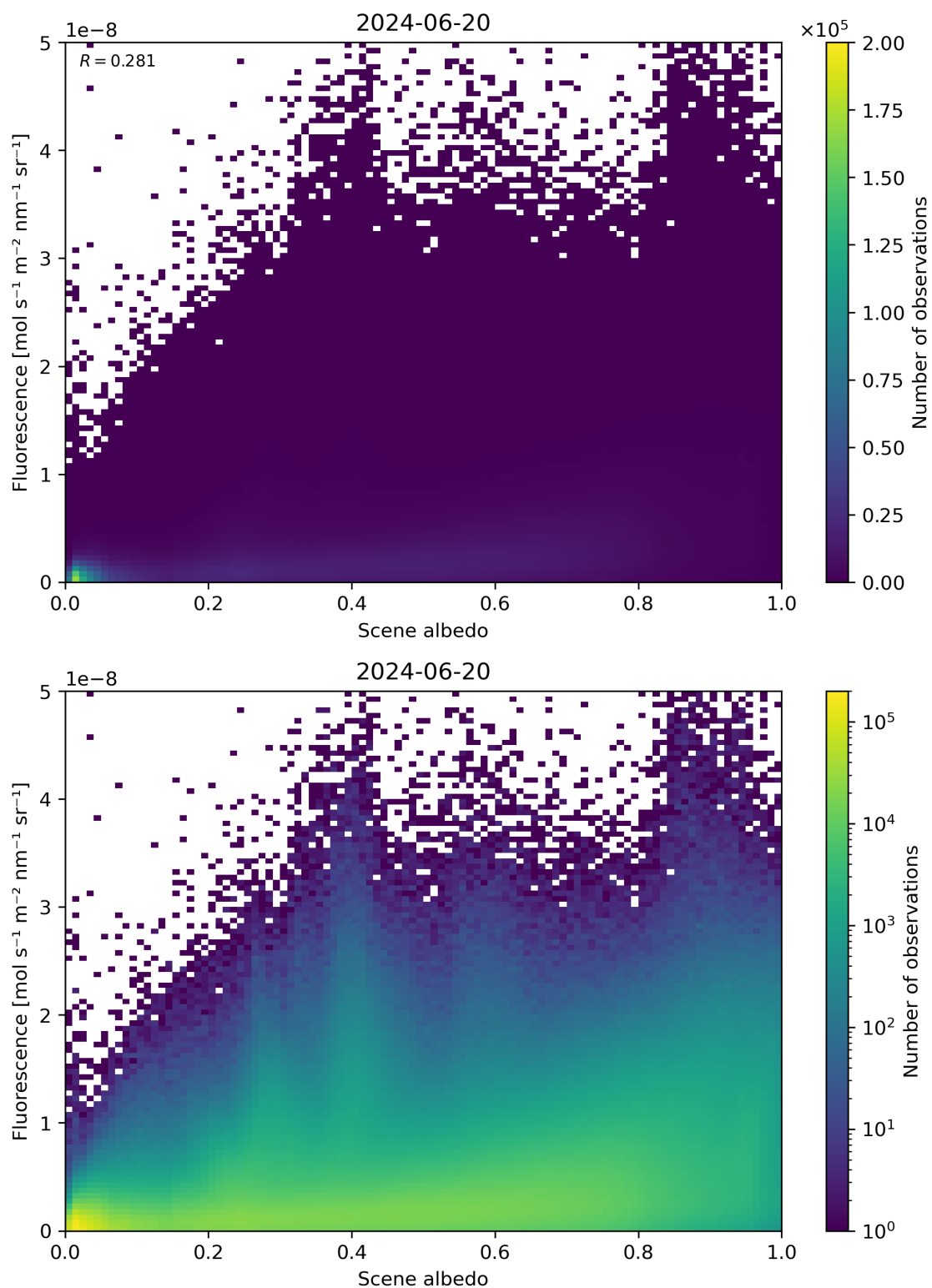
Figure 104: Scatter density plot of “Scene albedo” against “Fluorescence” for 2024-06-19 to 2024-06-21.
