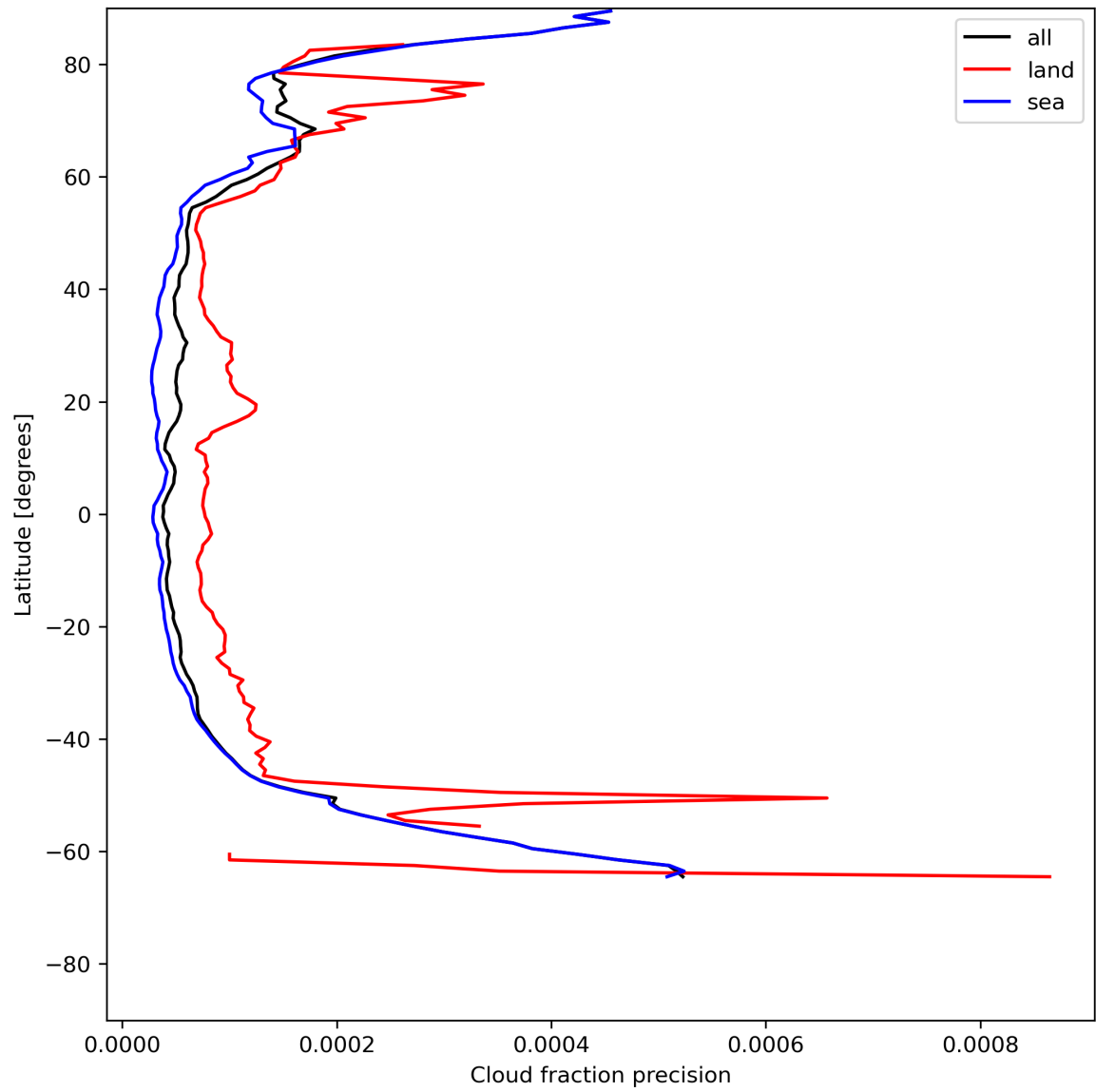
Figure 16: Zonal average of “Cloud fraction precision” for 2024-06-19 to 2024-06-21.
