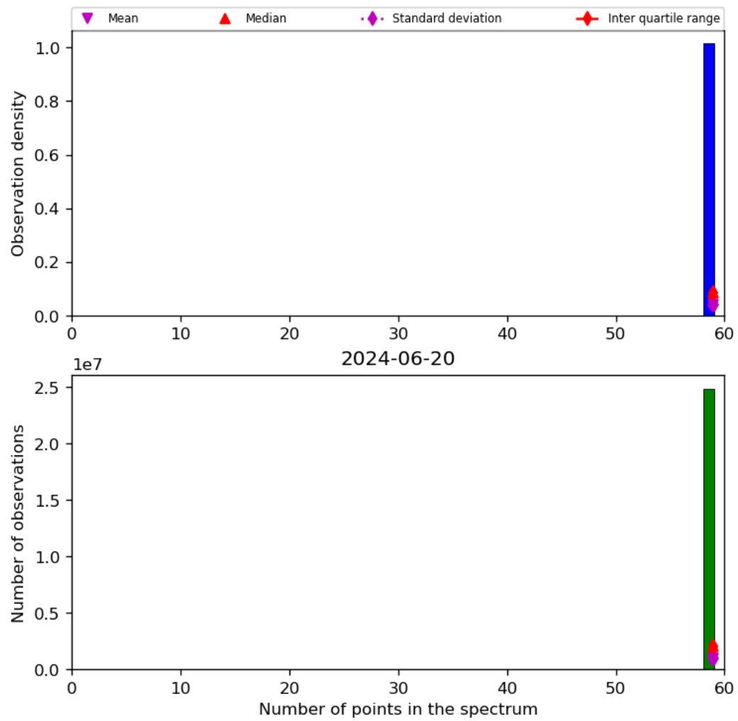
Figure 44: Histogram of “Number of points in the spectrum” for 2024-06-19 to 2024-06-21
