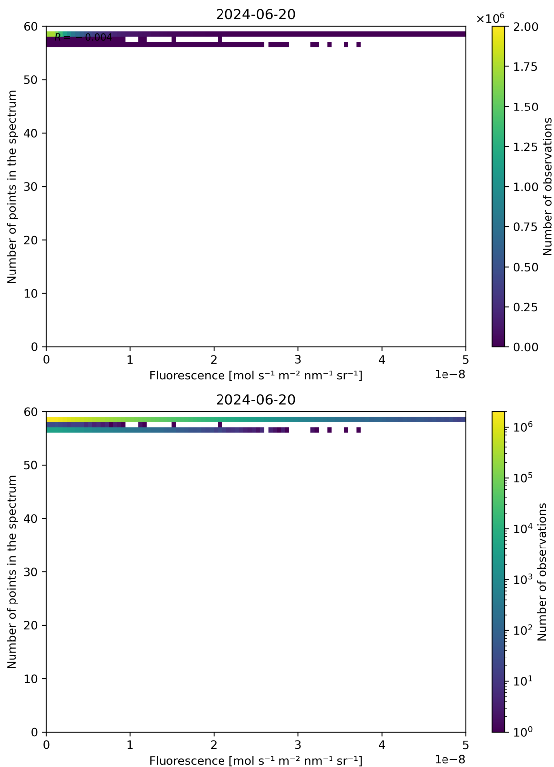
Figure 86: Scatter density plot of “Fluorescence” against “Number of points in the spectrum” for 2024-06-19 to 2024-06-21.
