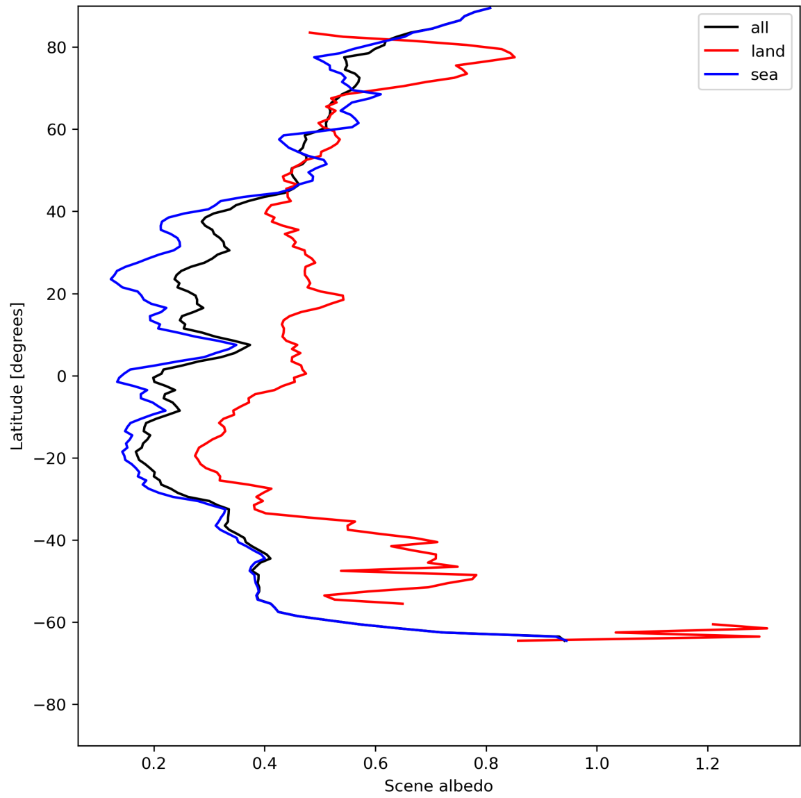
Figure 17: Zonal average of “Scene albedo” for 2024-06-19 to 2024-06-21.
