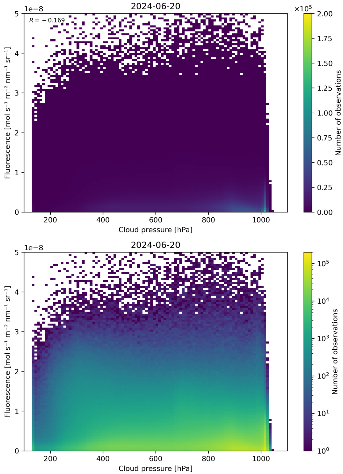
Figure 80: Scatter density plot of “Cloud pressure” against “Fluorescence” for 2024-06-19 to 2024-06-21.
