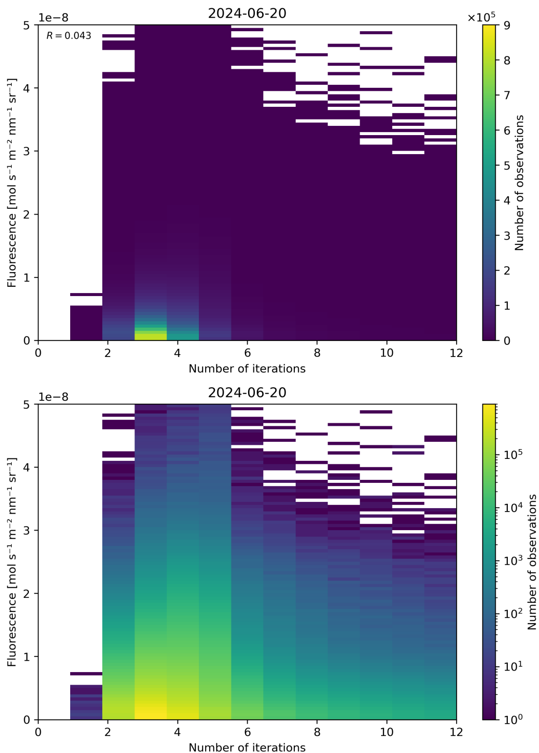
Figure 98: Scatter density plot of “Number of iterations” against “Fluorescence” for 2024-06-19 to 2024-06-21.
