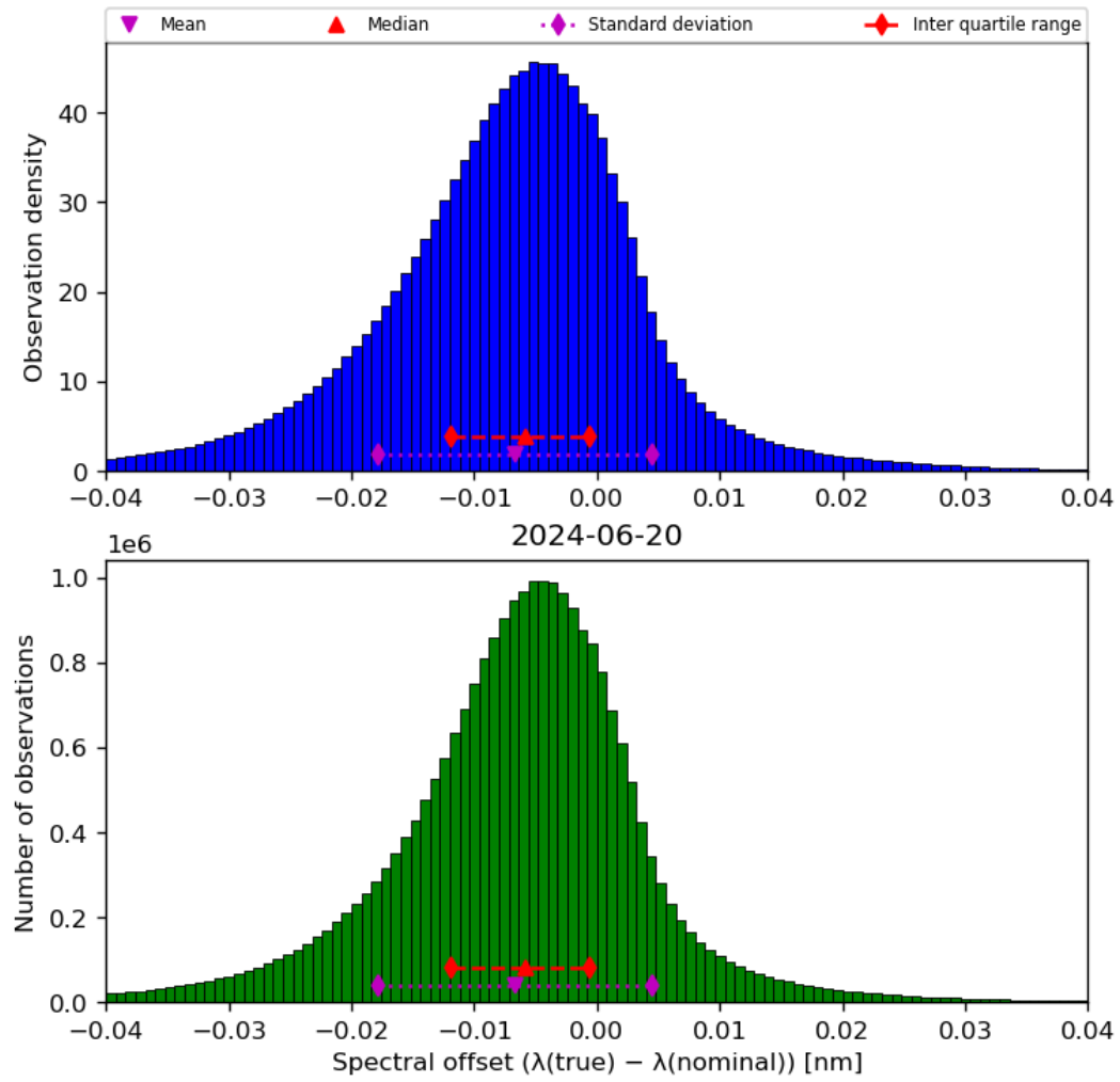
Figure 45: Histogram of “Spectral offset ( \lambda(\text{true}) - \lambda(\text{nominal}) )” for 2024-06-19 to 2024-06-21
