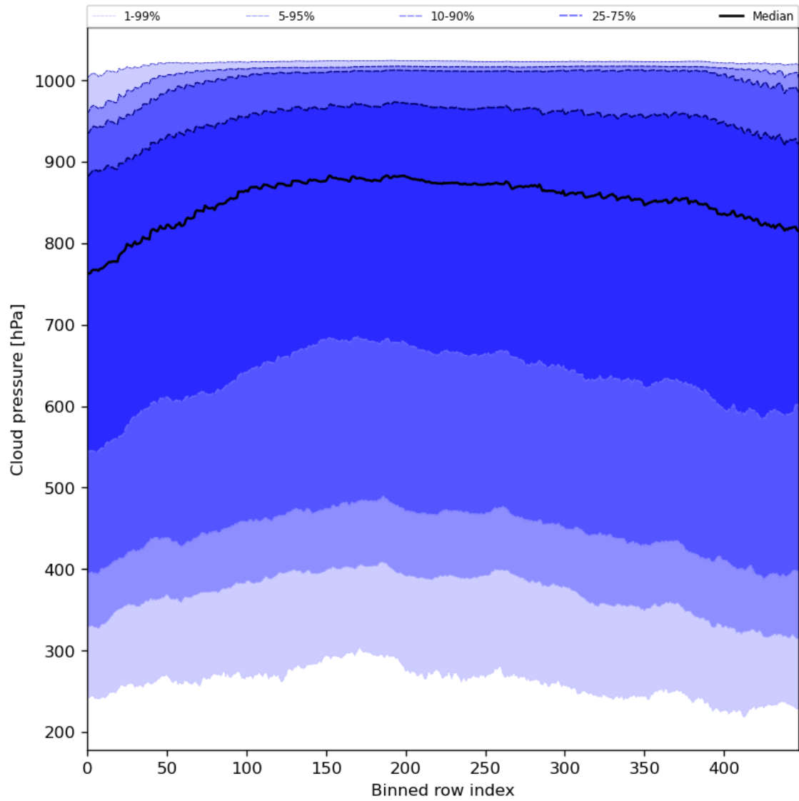
Figure 47: Along track statistics of “Cloud pressure” for 2024-06-19 to 2024-06-21
