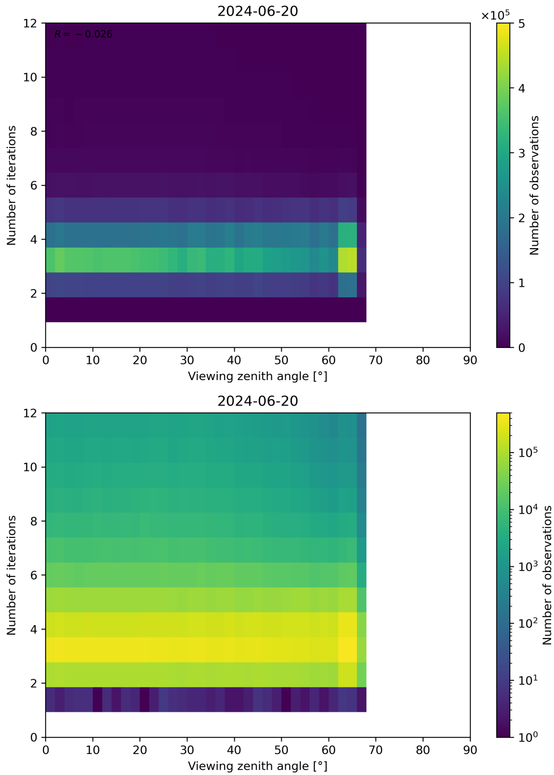
Figure 124: Scatter density plot of “Viewing zenith angle” against “Number of iterations” for 2024-06-19 to 2024-06-21.
