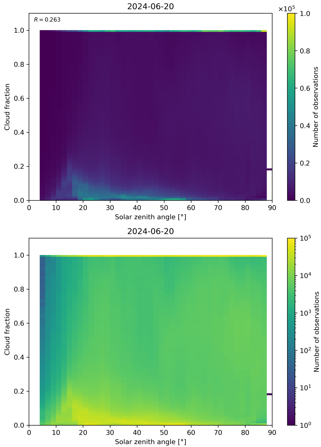
Figure 110: Scatter density plot of “Solar zenith angle” against “Cloud fraction” for 2024-06-19 to 2024-06-21.
