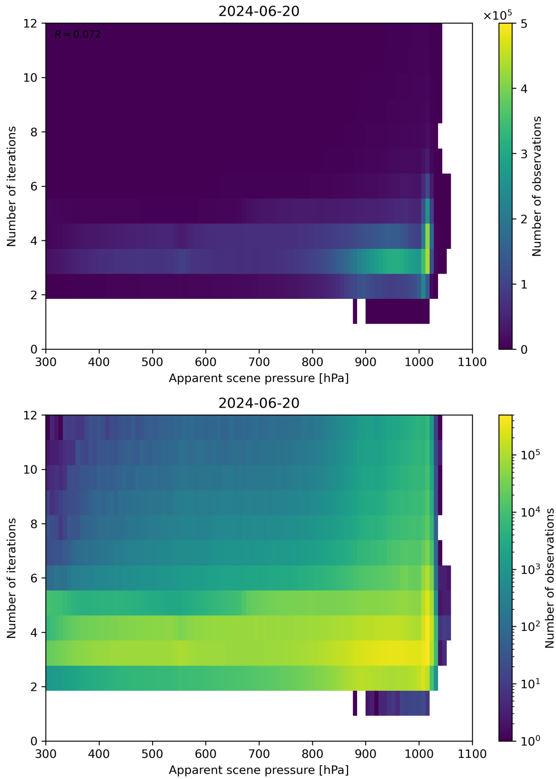
Figure 65: Scatter density plot of “Apparent scene pressure” against “Number of iterations” for 2024-06-19 to 2024-06-21.
