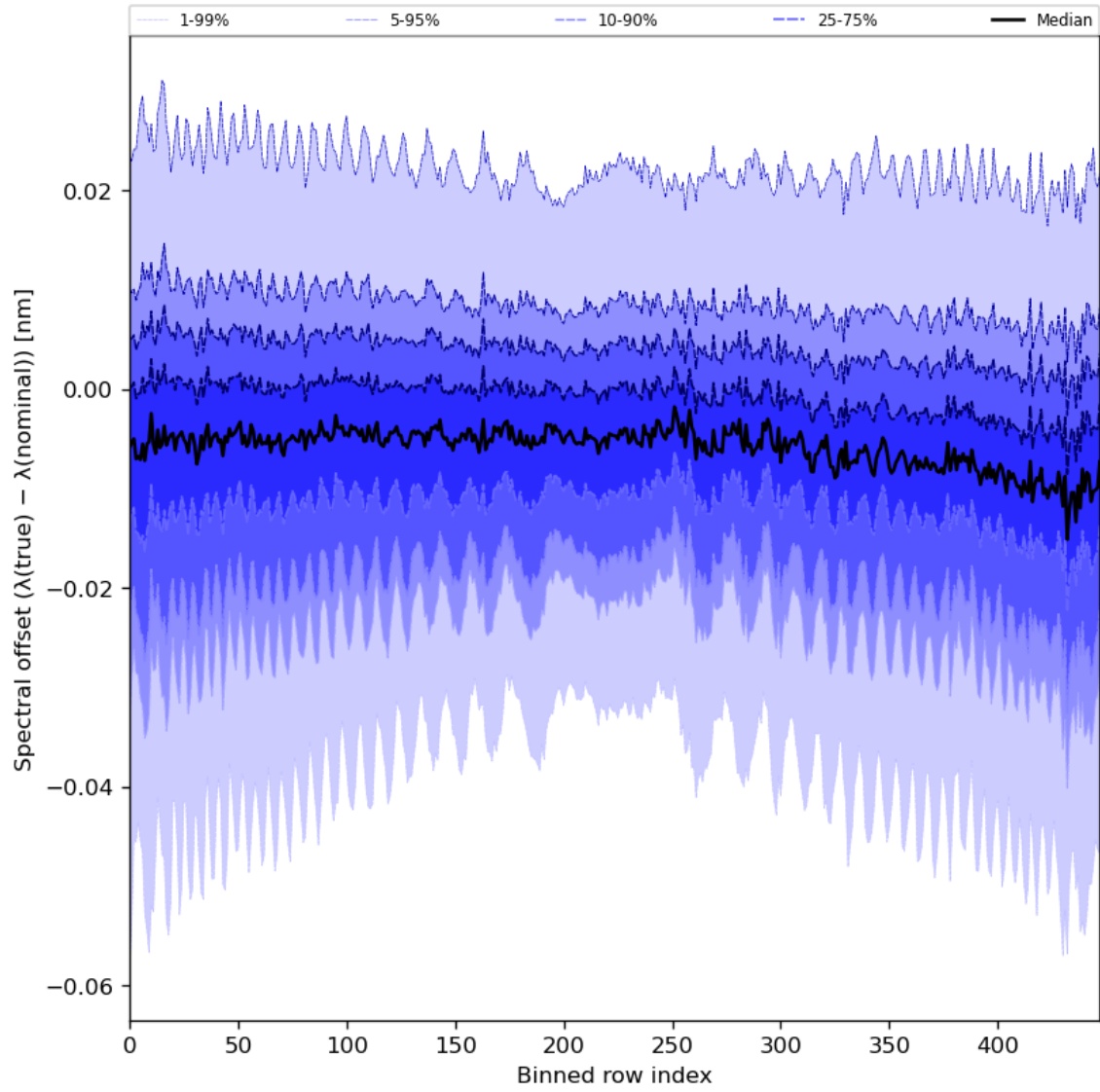
Figure 62: Along track statistics of “Spectral offset ( \lambda(\text{true}) - \lambda(\text{nominal}) )” for 2024-06-19 to 2024-06-21
