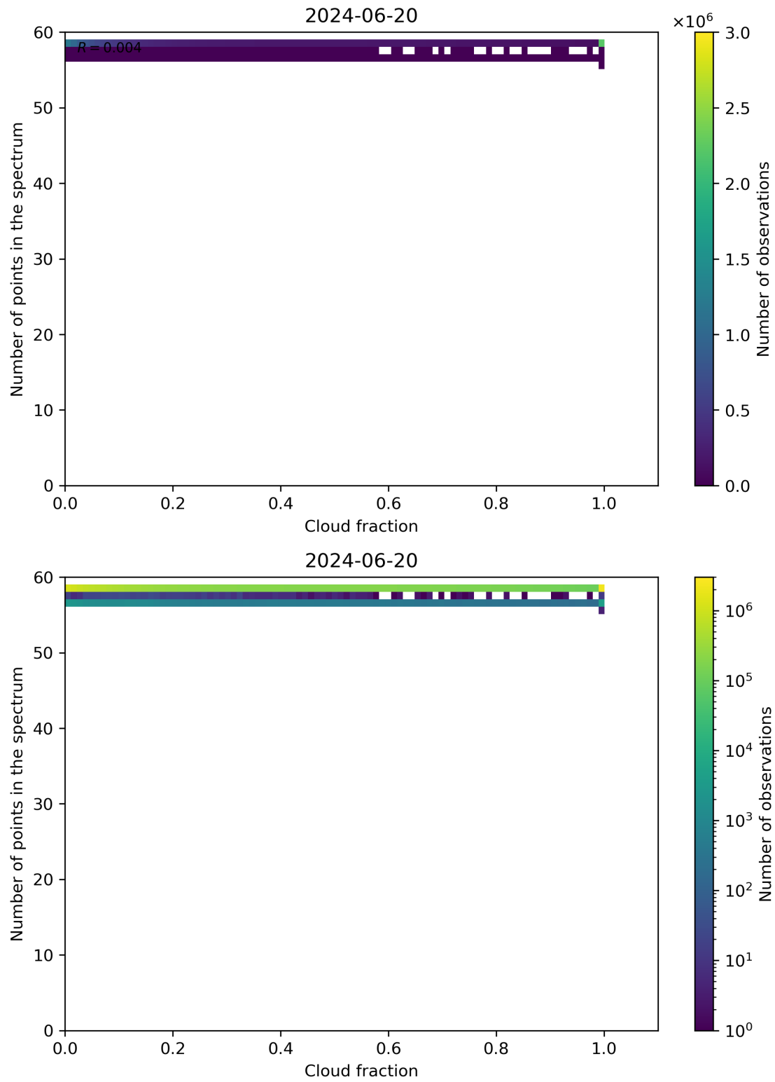
Figure 74: Scatter density plot of “Cloud fraction” against “Number of points in the spectrum” for 2024-06-19 to 2024-06-21.
