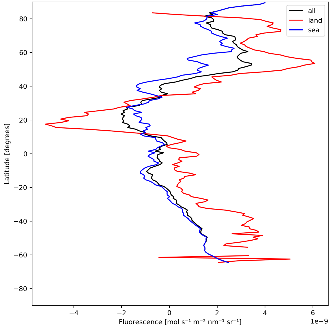
Figure 23: Zonal average of “Fluorescence” for 2024-06-19 to 2024-06-21.
