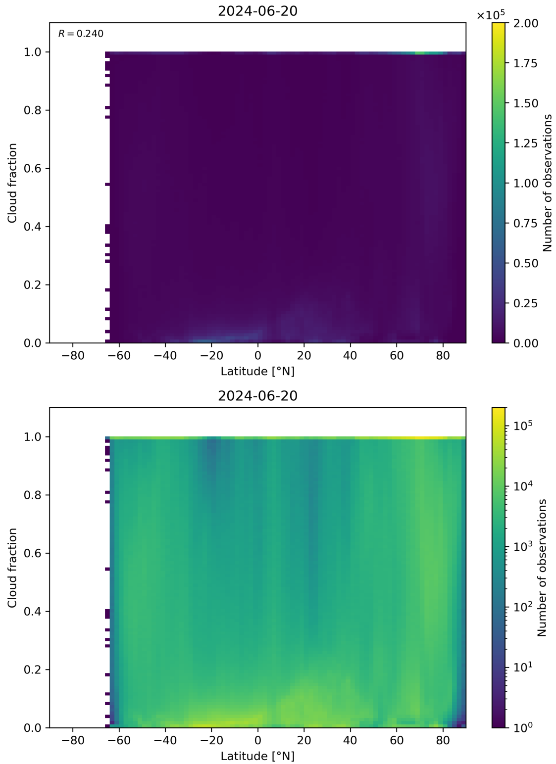
Figure 90: Scatter density plot of “Latitude” against “Cloud fraction” for 2024-06-19 to 2024-06-21.
