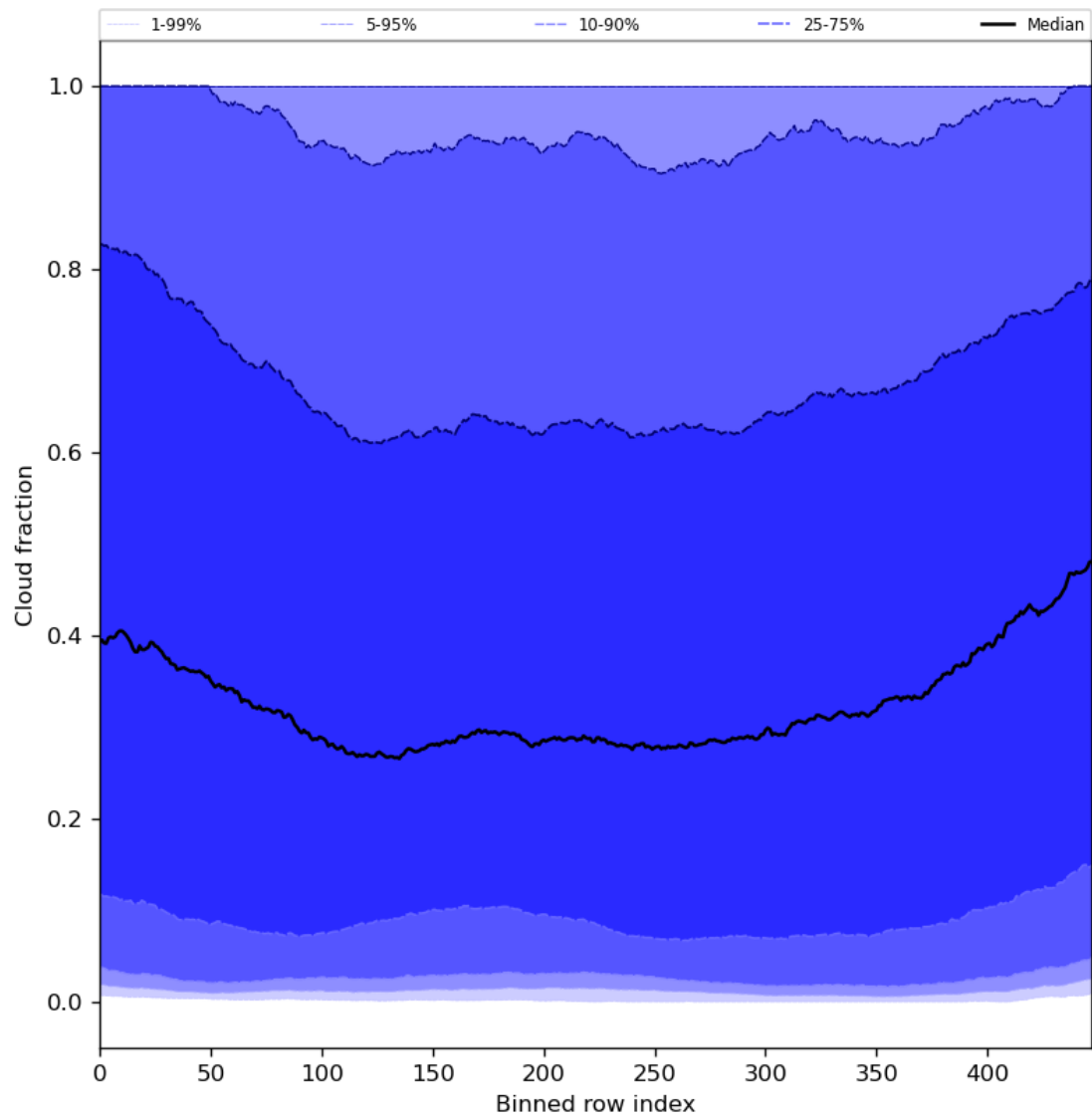
Figure 49: Along track statistics of “Cloud fraction” for 2024-06-19 to 2024-06-21
