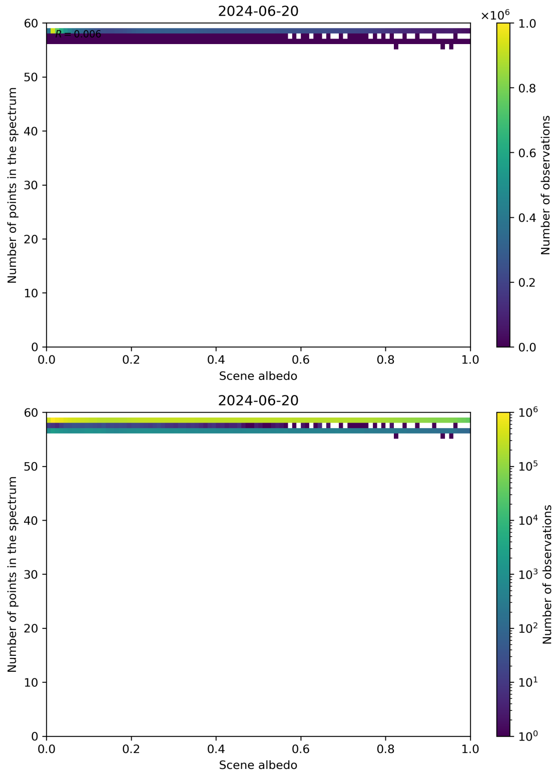
Figure 106: Scatter density plot of “Scene albedo” against “Number of points in the spectrum” for 2024-06-19 to 2024-06-21.
