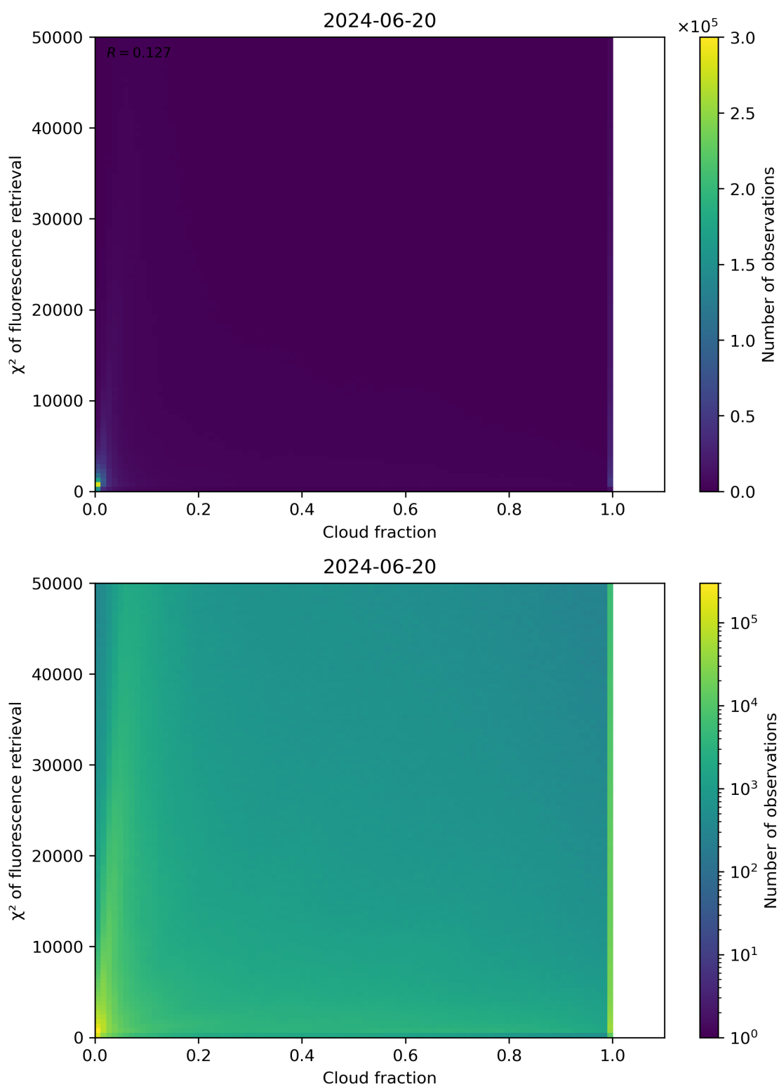
Figure 71: Scatter density plot of “Cloud fraction” against “ \chi^2 of fluorescence retrieval” for 2024-06-19 to 2024-06-21.
