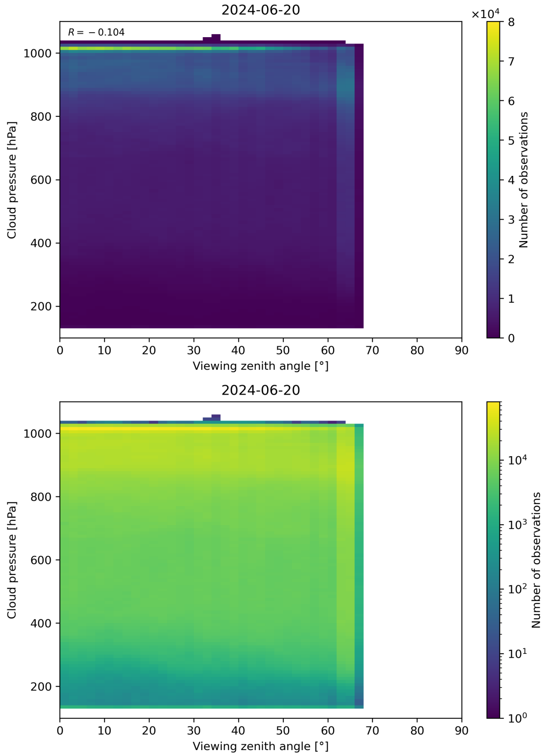
Figure 121: Scatter density plot of “Viewing zenith angle” against “Cloud pressure” for 2024-06-19 to 2024-06-21.
