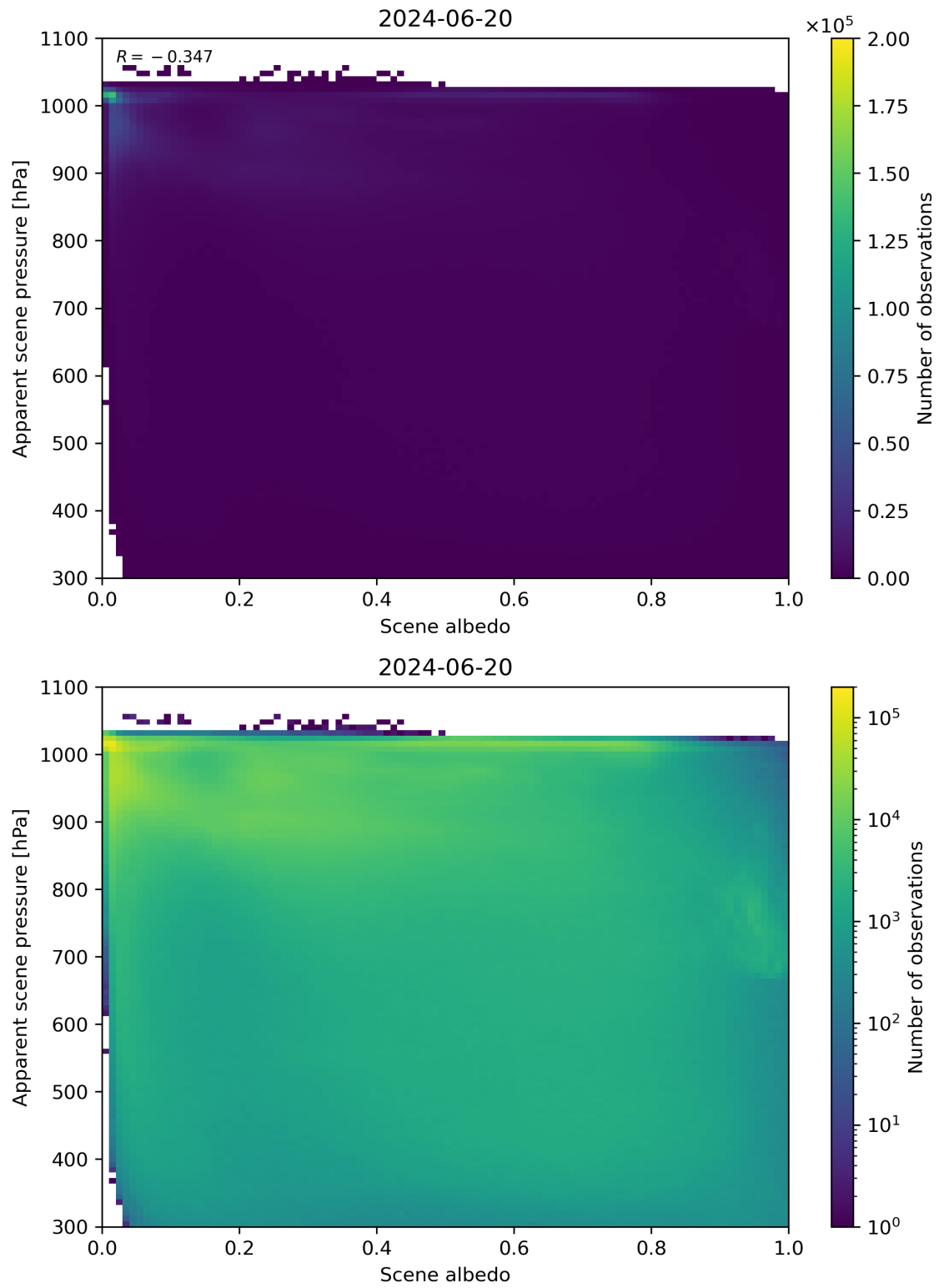
Figure 102: Scatter density plot of “Scene albedo” against “Apparent scene pressure” for 2024-06-19 to 2024-06-21.
