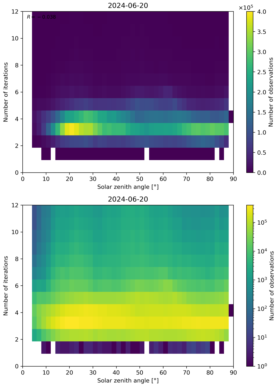
Figure 114: Scatter density plot of “Solar zenith angle” against “Number of iterations” for 2024-06-19 to 2024-06-21.
