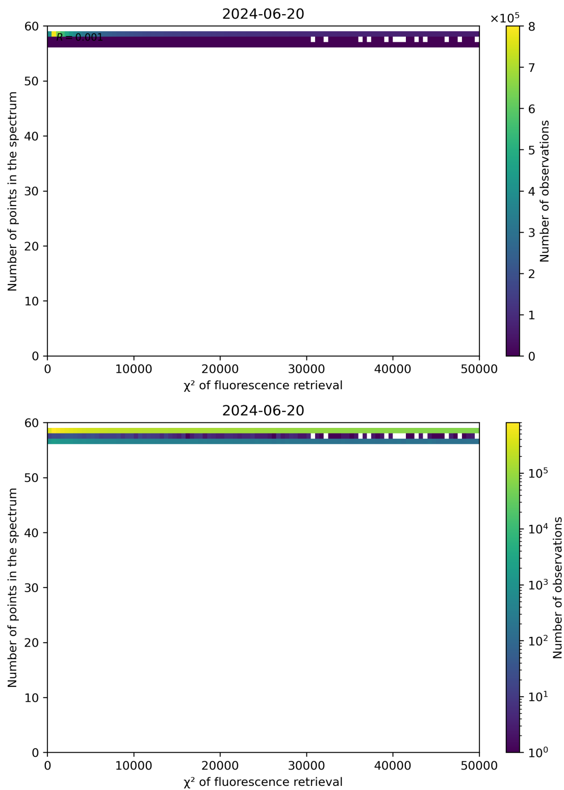
Figure 68: Scatter density plot of " \chi^2 of fluorescence retrieval" against "Number of points in the spectrum" for 2024-06-19 to 2024-06-21.
