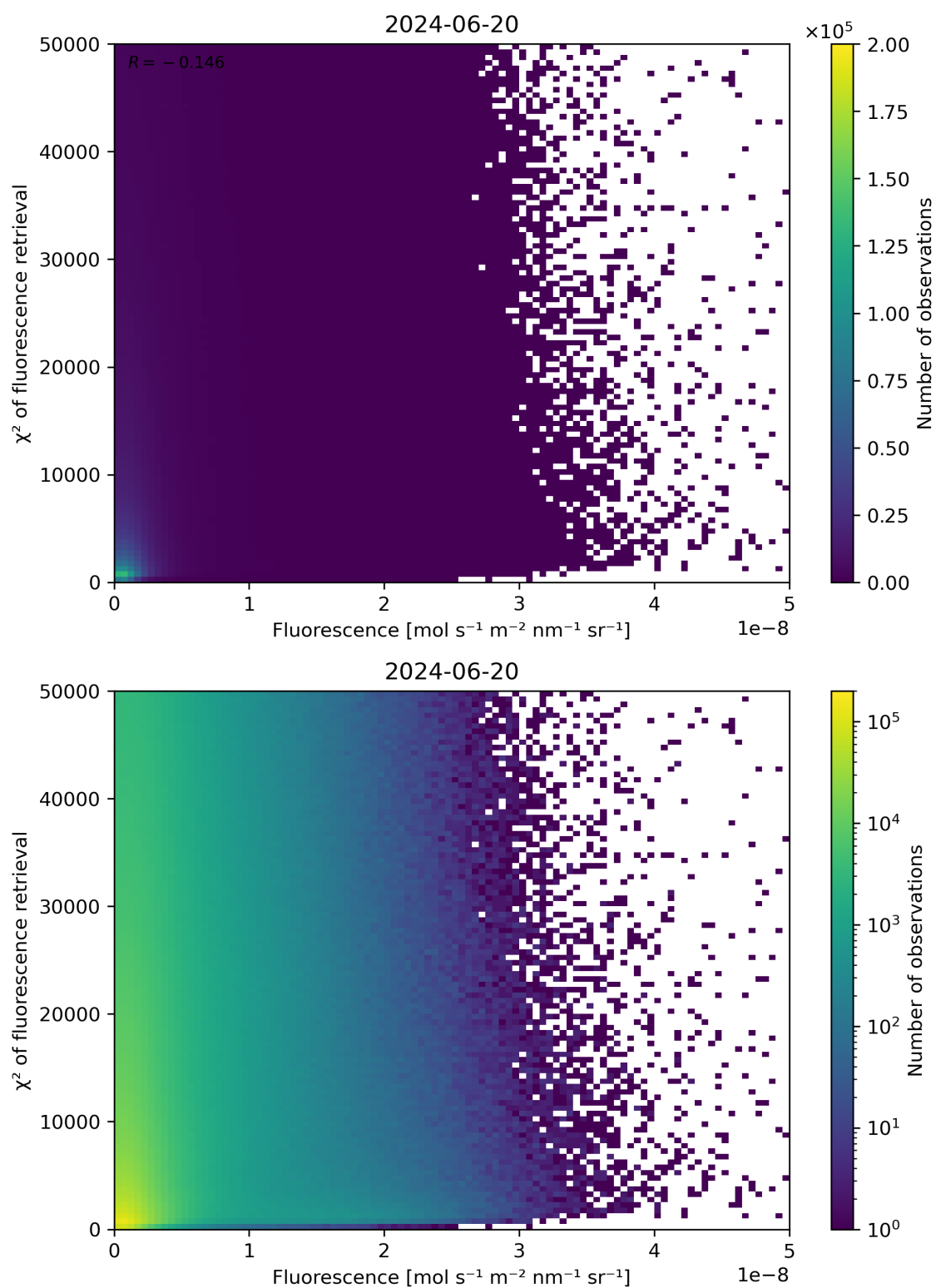
Figure 85: Scatter density plot of “Fluorescence” against “ \chi^2 of fluorescence retrieval” for 2024-06-19 to 2024-06-21.
