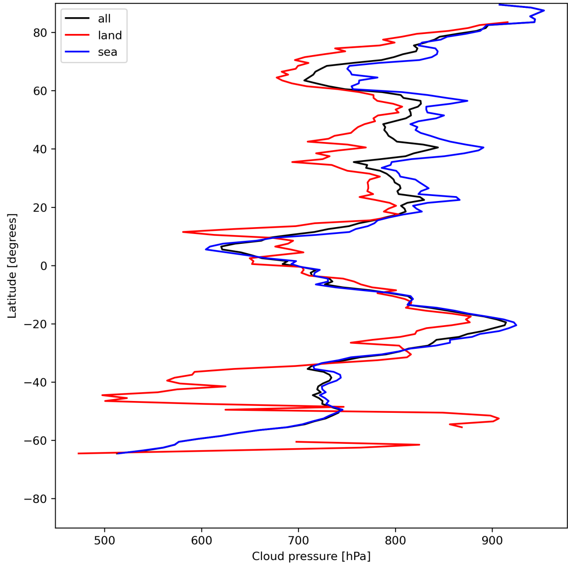
Figure 13: Zonal average of “Cloud pressure” for 2024-06-19 to 2024-06-21.
