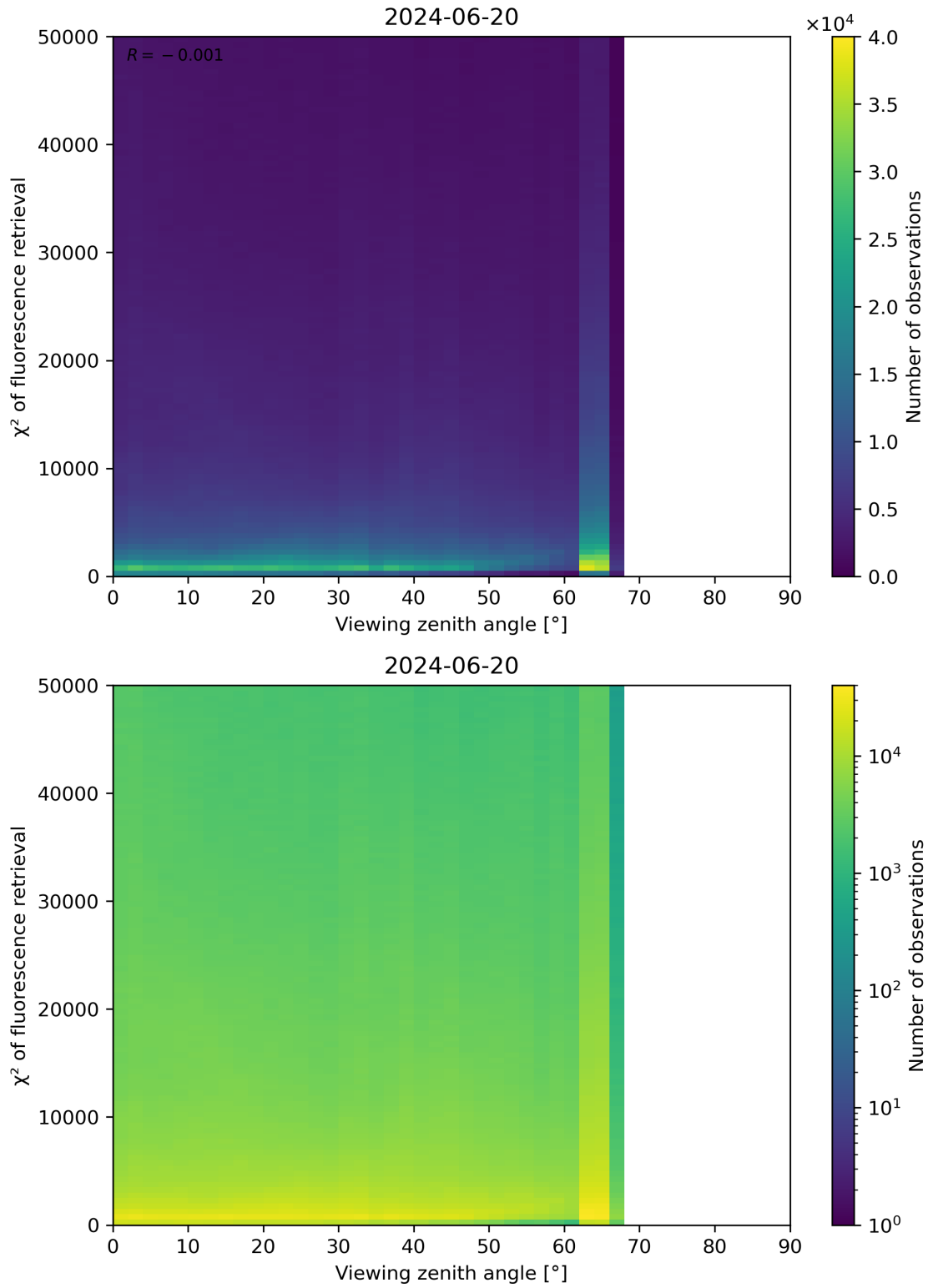
Figure 119: Scatter density plot of “Viewing zenith angle” against “ \chi^2 of fluorescence retrieval” for 2024-06-19 to 2024-06-21.
