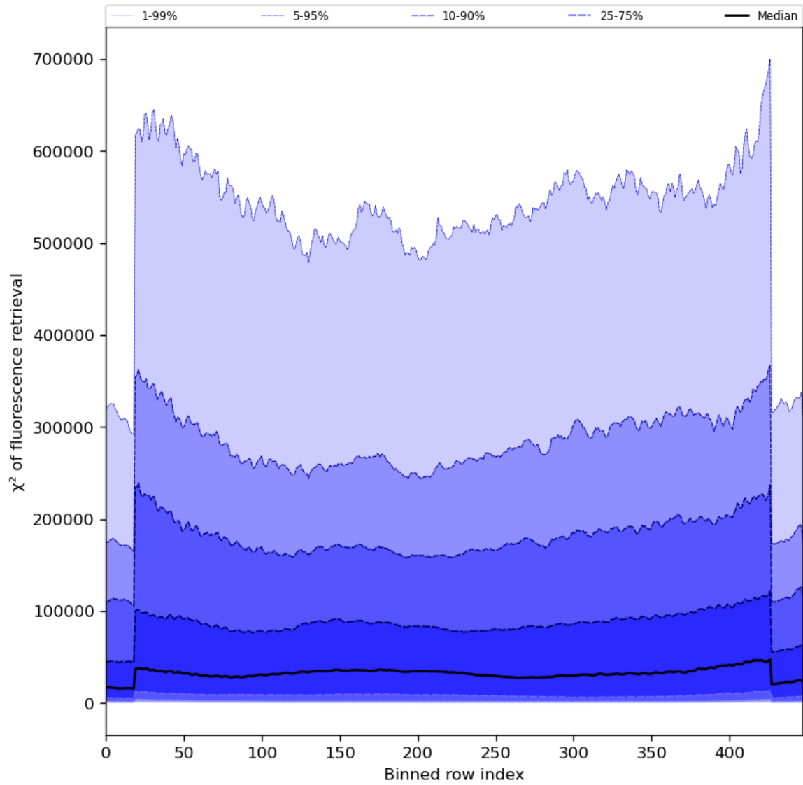
Figure 59: Along track statistics of “ \chi^2 of fluorescence retrieval” for 2024-06-19 to 2024-06-21
