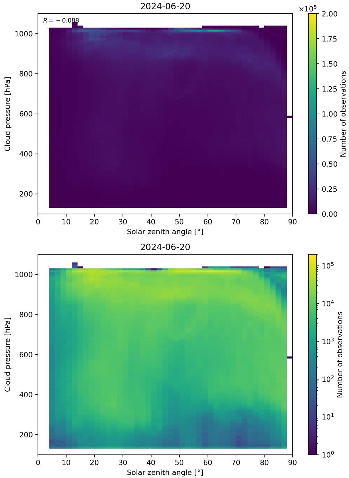
Figure 111: Scatter density plot of “Solar zenith angle” against “Cloud pressure” for 2024-06-19 to 2024-06-21.
