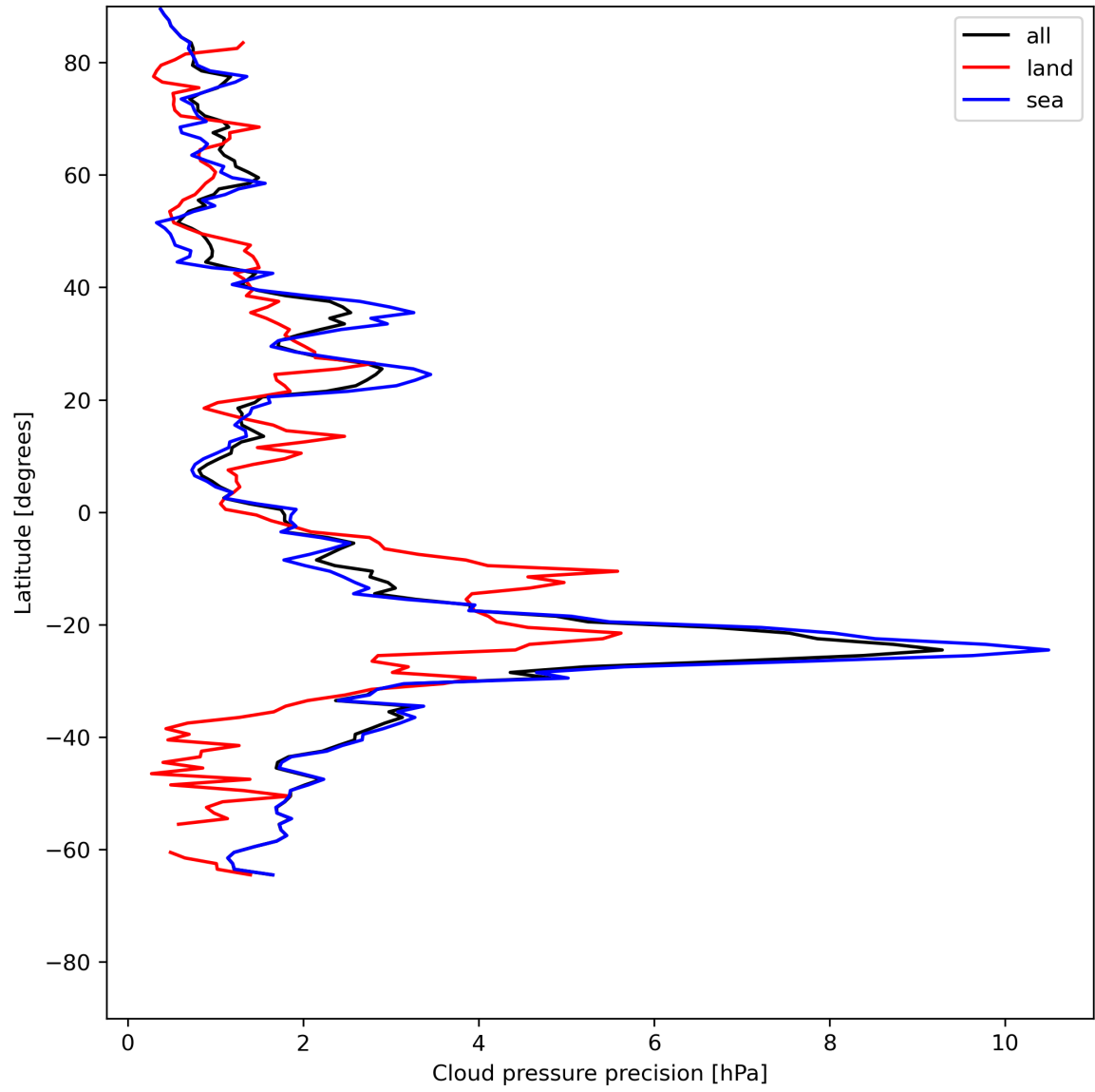
Figure 14: Zonal average of “Cloud pressure precision” for 2024-06-19 to 2024-06-21.
