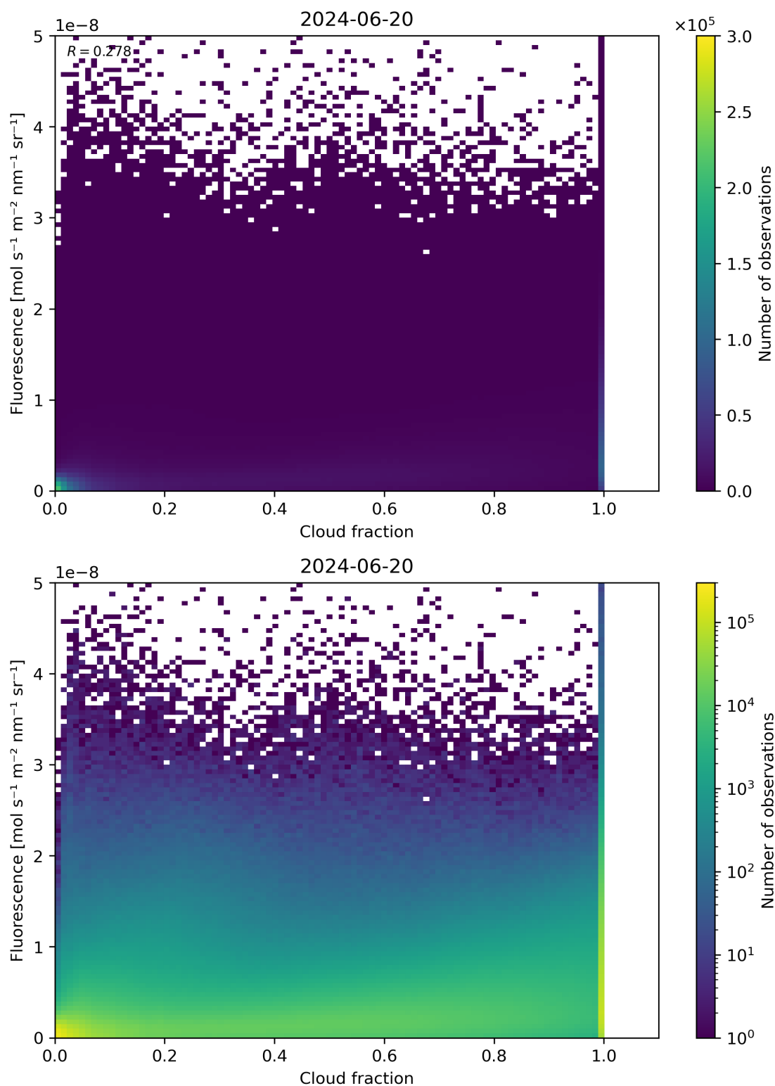
Figure 72: Scatter density plot of “Cloud fraction” against “Fluorescence” for 2024-06-19 to 2024-06-21.
