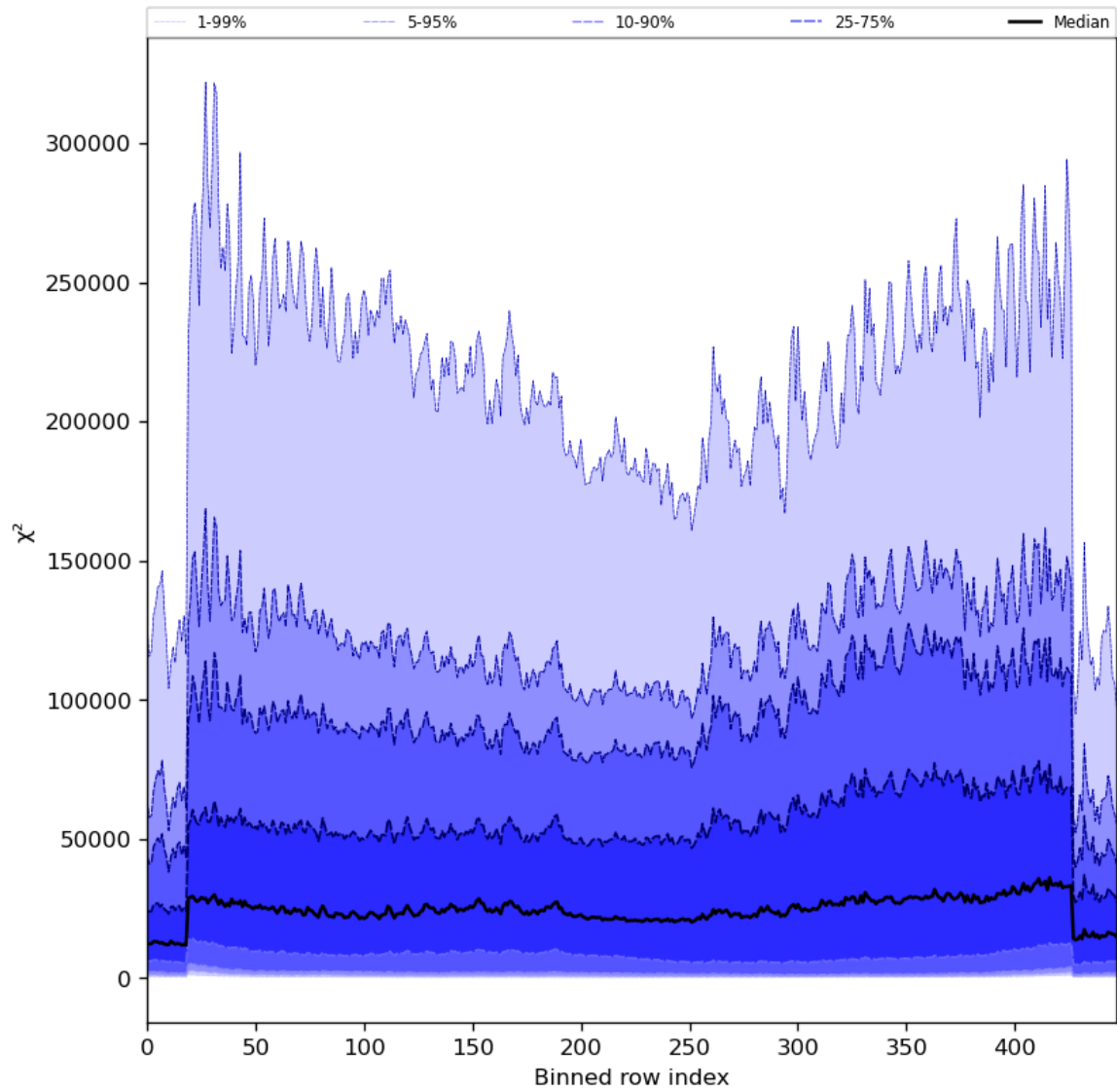
Figure 55: Along track statistics of “ \chi^2 ” for 2024-06-19 to 2024-06-21
