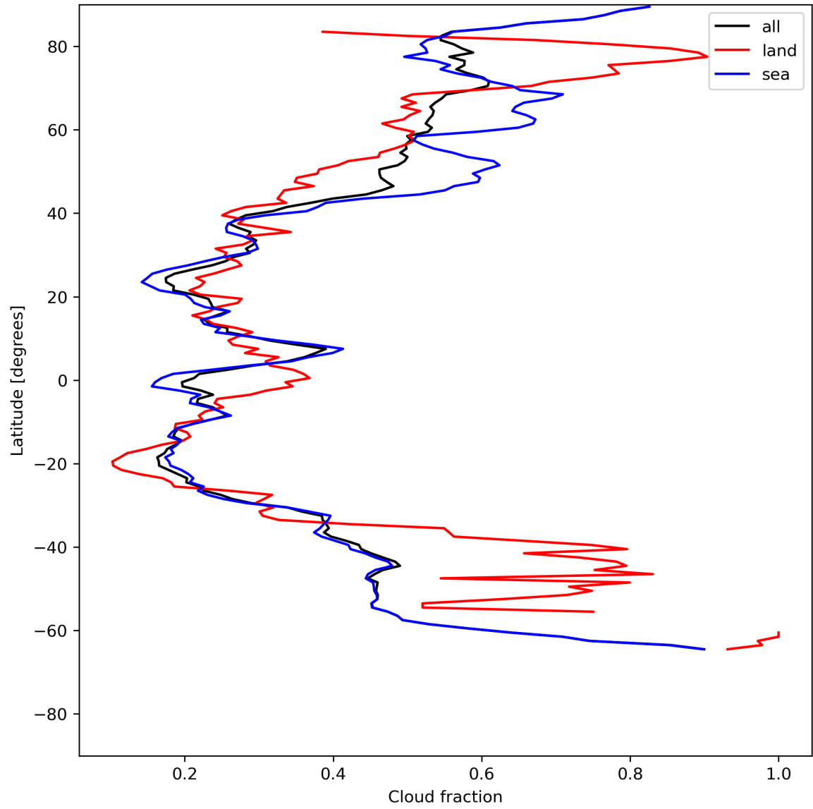
Figure 15: Zonal average of “Cloud fraction” for 2024-06-19 to 2024-06-21.
