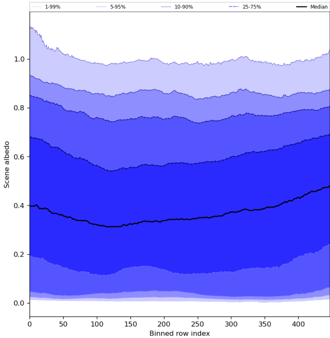
Figure 51: Along track statistics of “Scene albedo” for 2024-06-19 to 2024-06-21
