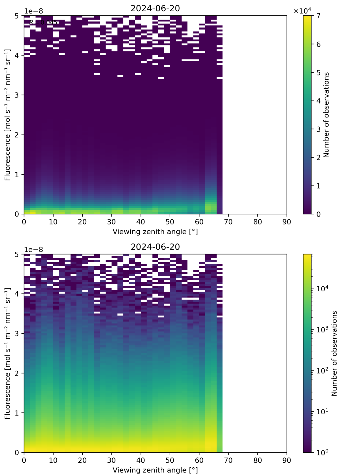
Figure 122: Scatter density plot of “Viewing zenith angle” against “Fluorescence” for 2024-06-19 to 2024-06-21.
