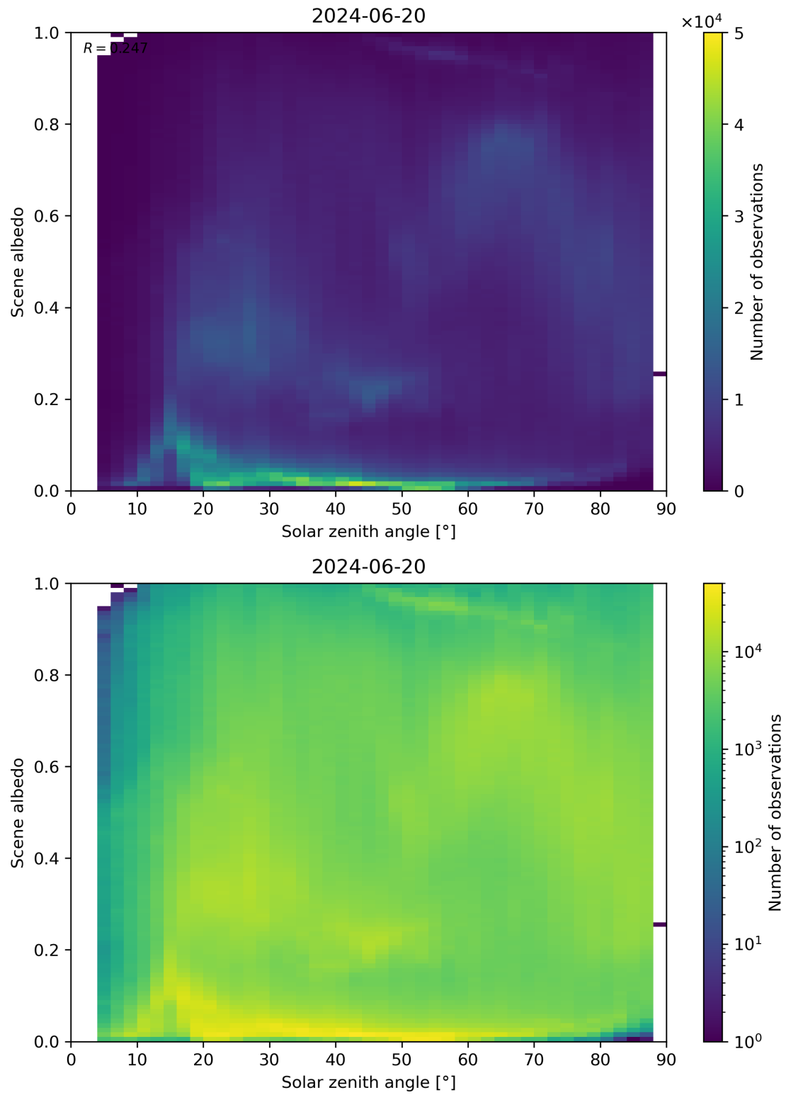
Figure 116: Scatter density plot of “Solar zenith angle” against “Scene albedo” for 2024-06-19 to 2024-06-21.
