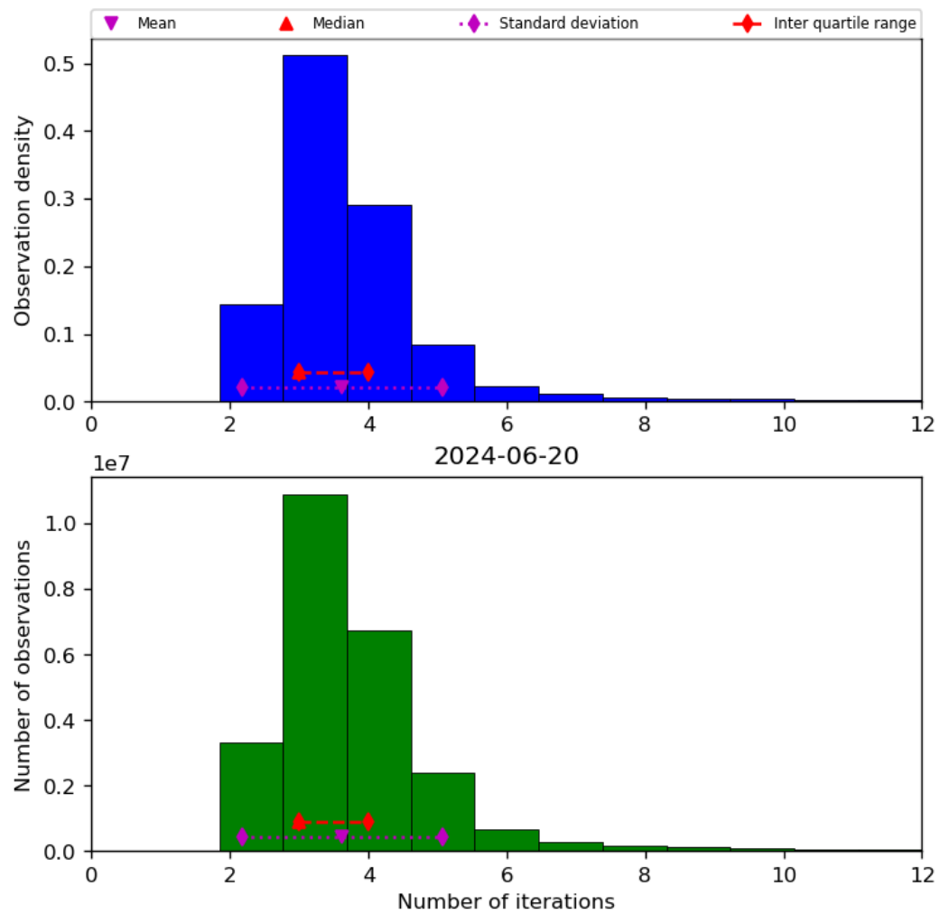
Figure 39: Histogram of “Number of iterations” for 2024-06-19 to 2024-06-21
