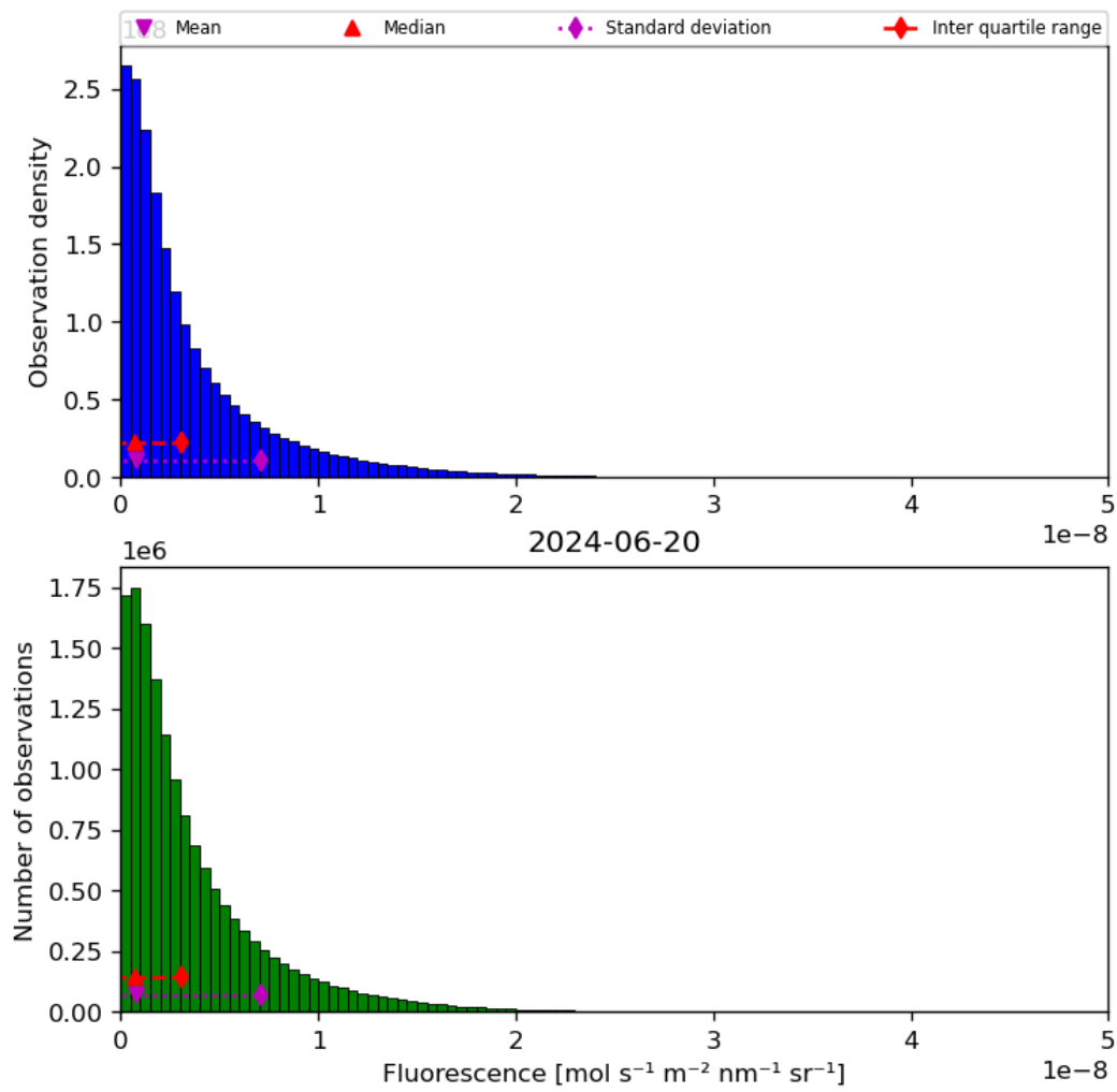
Figure 40: Histogram of “Fluorescence” for 2024-06-19 to 2024-06-21
