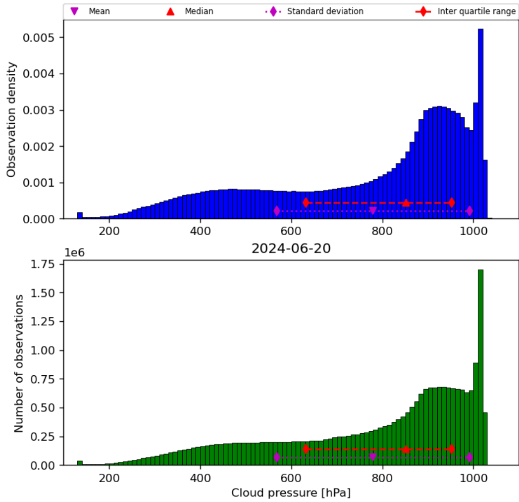
Figure 30: Histogram of “Cloud pressure” for 2024-06-19 to 2024-06-21
