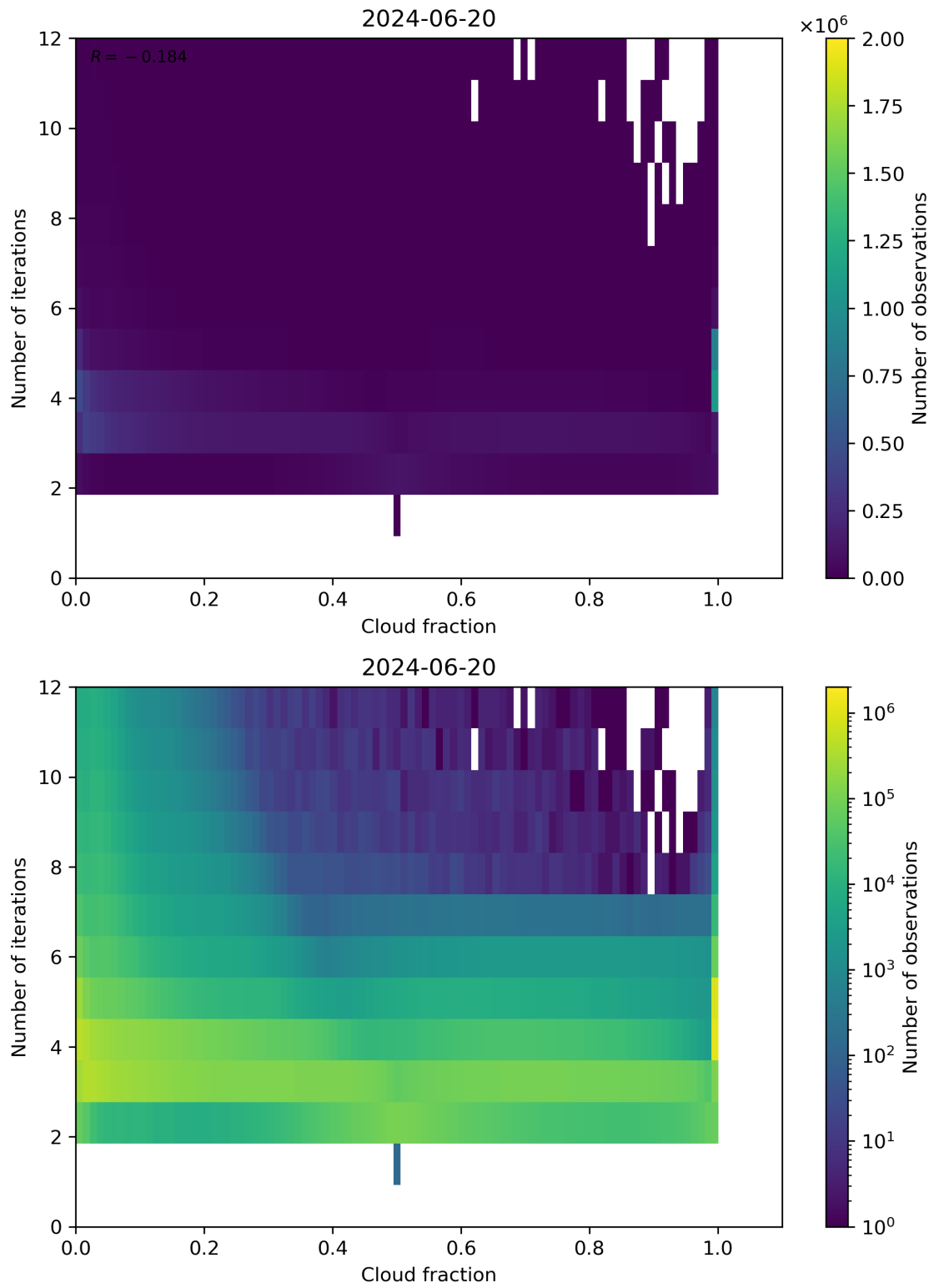
Figure 73: Scatter density plot of “Cloud fraction” against “Number of iterations” for 2024-06-19 to 2024-06-21.
