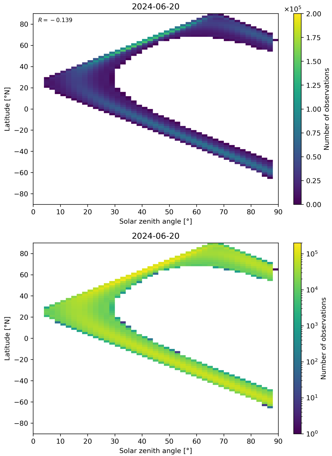
Figure 113: Scatter density plot of “Solar zenith angle” against “Latitude” for 2024-06-19 to 2024-06-21.
