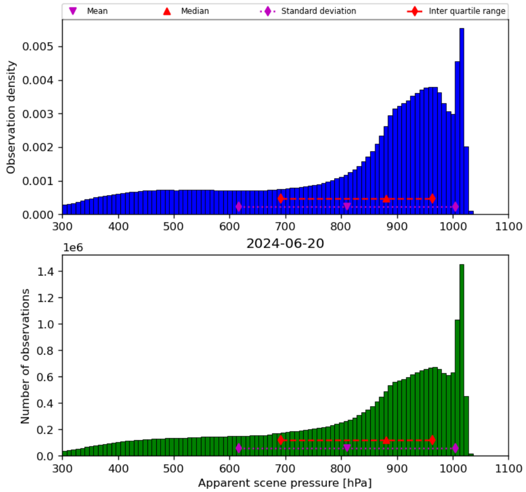
Figure 36: Histogram of “Apparent scene pressure” for 2024-06-19 to 2024-06-21
