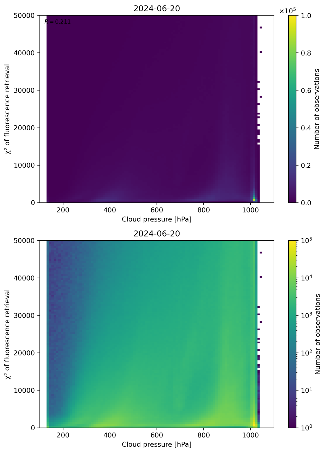
Figure 78: Scatter density plot of “Cloud pressure” against “ \chi^2 of fluorescence retrieval” for 2024-06-19 to 2024-06-21.
