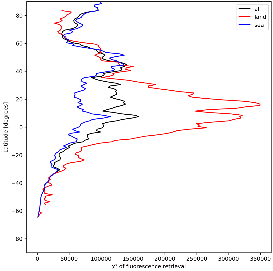
Figure 25: Zonal average of “ \chi^2 of fluorescence retrieval” for 2024-06-19 to 2024-06-21.
