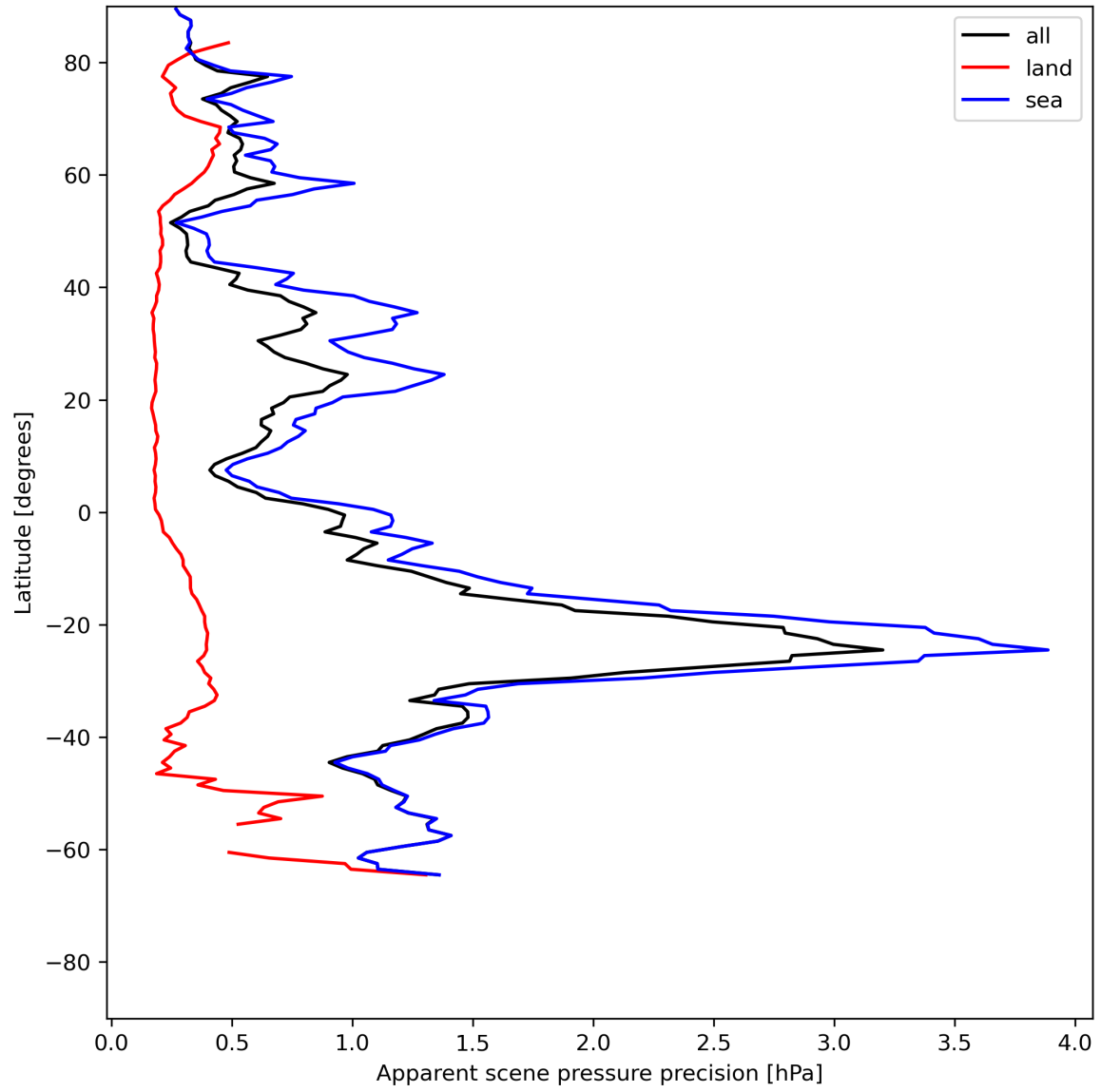
Figure 20: Zonal average of “Apparent scene pressure precision” for 2024-06-19 to 2024-06-21.
