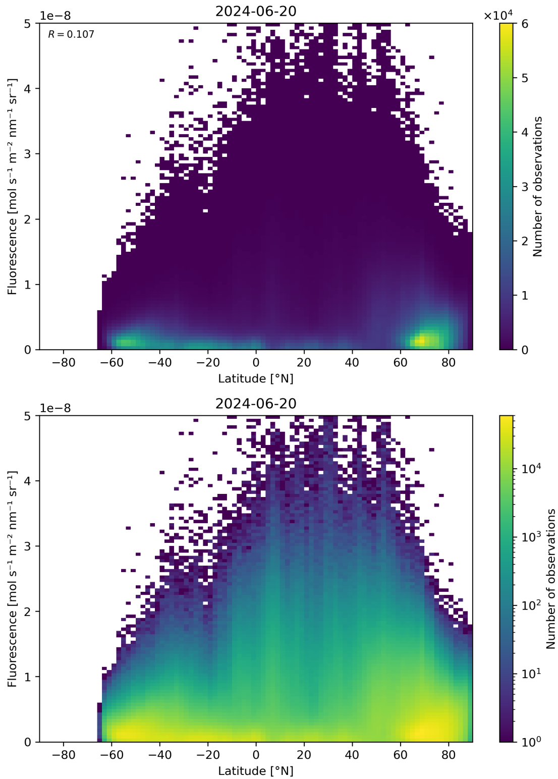
Figure 92: Scatter density plot of “Latitude” against “Fluorescence” for 2024-06-19 to 2024-06-21.
