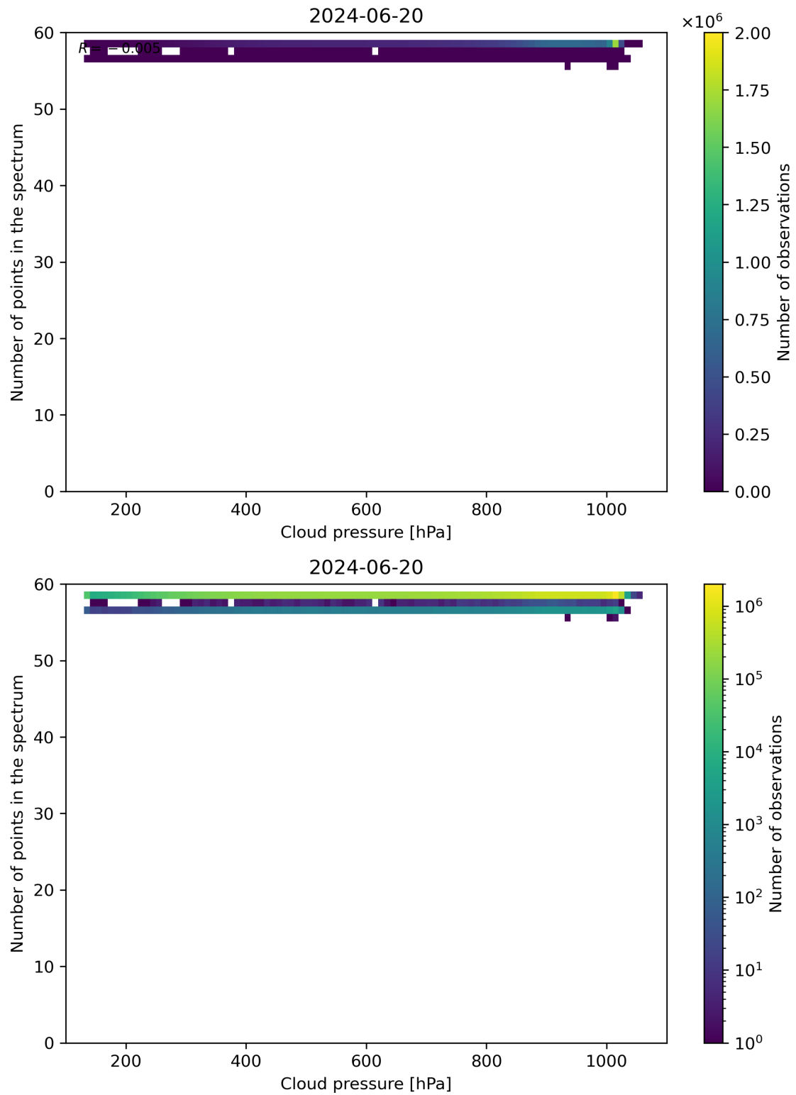
Figure 82: Scatter density plot of “Cloud pressure” against “Number of points in the spectrum” for 2024-06-19 to 2024-06-21.
