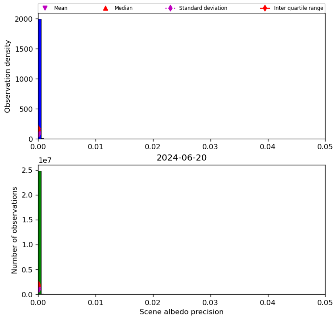
Figure 35: Histogram of “Scene albedo precision” for 2024-06-19 to 2024-06-21
