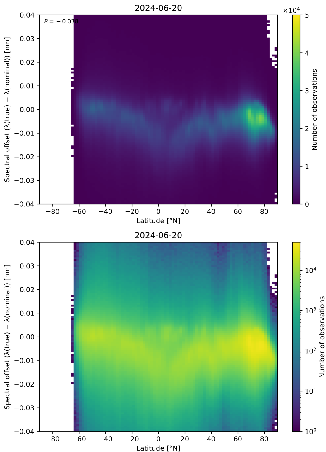
Figure 96: Scatter density plot of “Latitude” against “Spectral offset ( \lambda(\text{true}) - \lambda(\text{nominal}) )” for 2024-06-19 to 2024-06-21.
