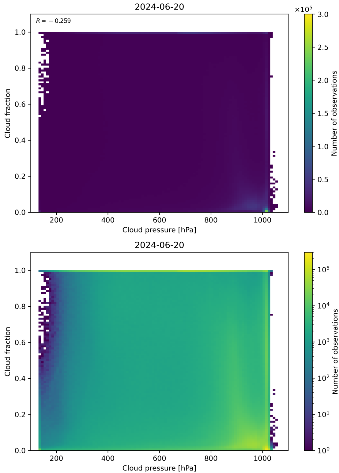
Figure 79: Scatter density plot of “Cloud pressure” against “Cloud fraction” for 2024-06-19 to 2024-06-21.
