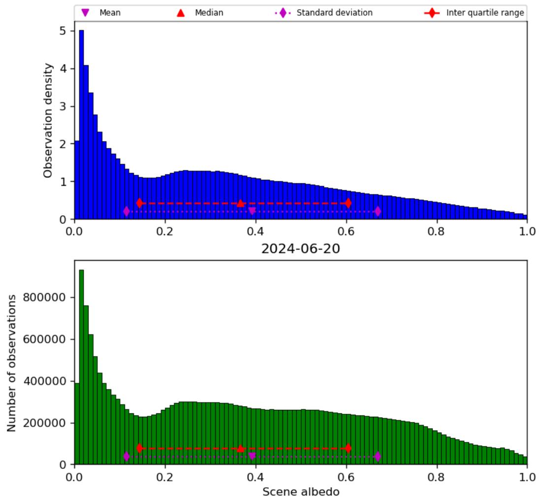
Figure 34: Histogram of “Scene albedo” for 2024-06-19 to 2024-06-21
