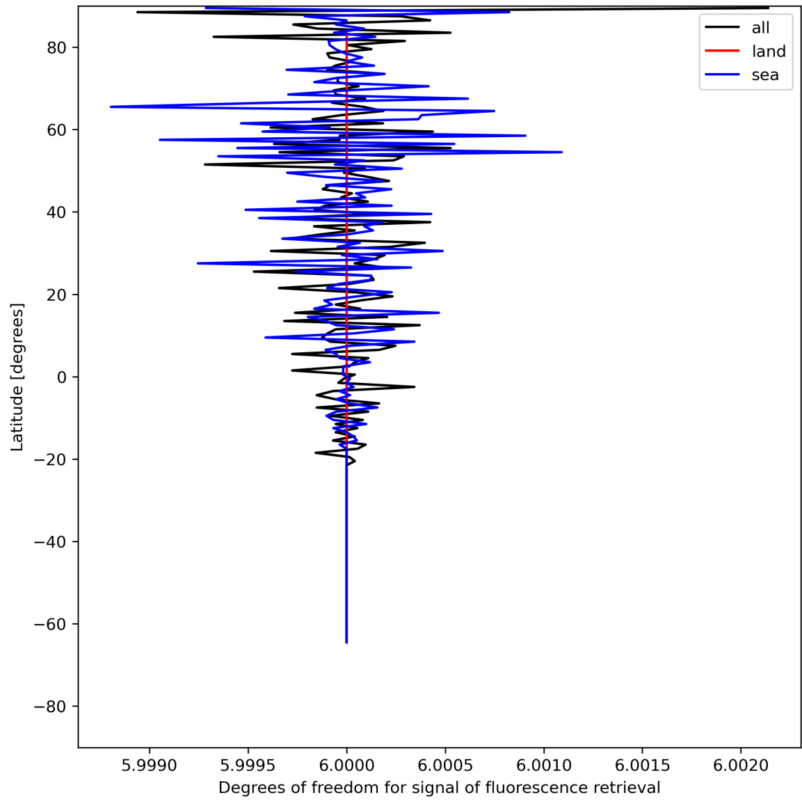
Figure 26: Zonal average of “Degrees of freedom for signal of fluorescence retrieval” for 2024-06-19 to 2024-06-21.
