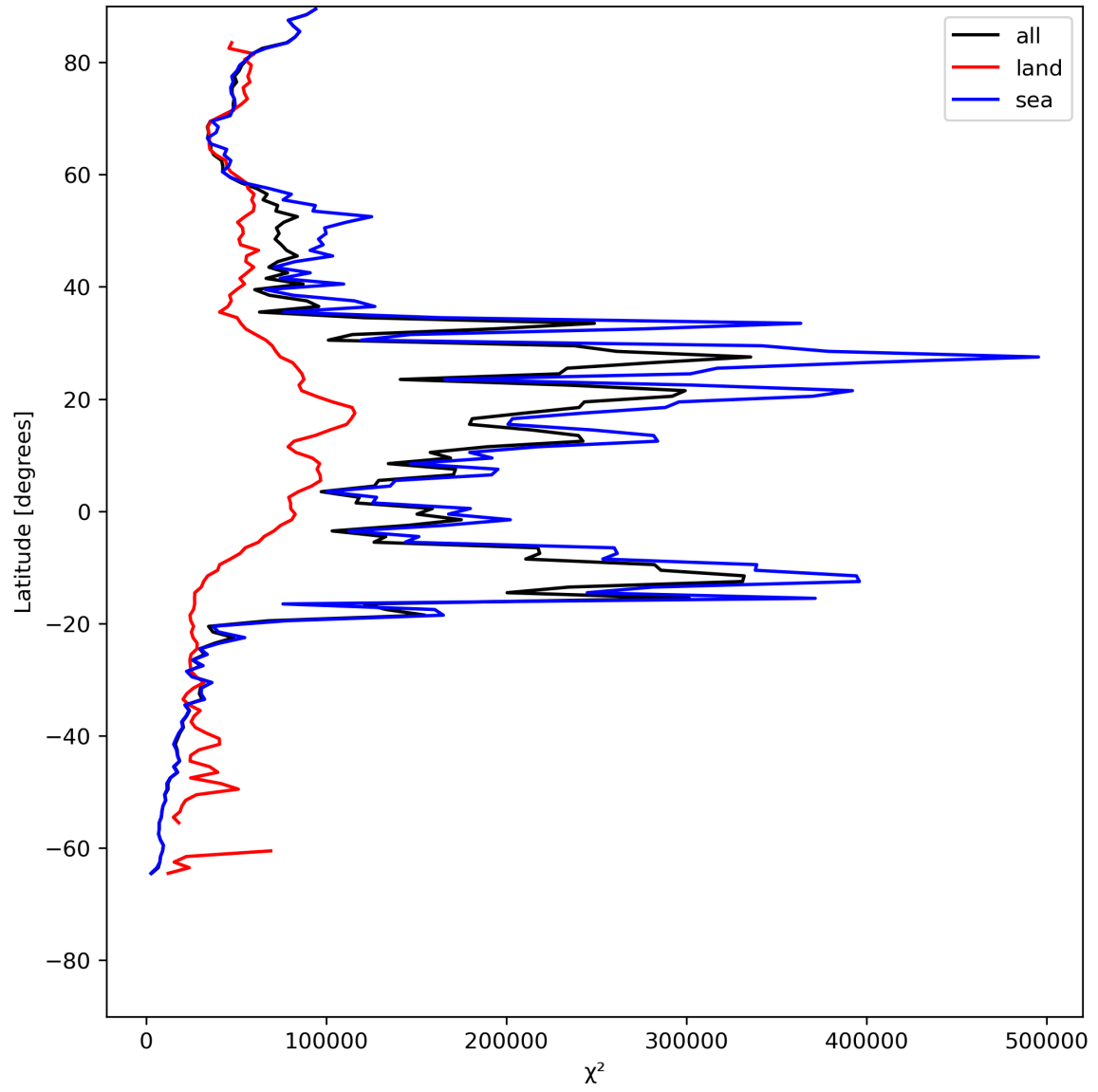
Figure 21: Zonal average of “ \chi^2 ” for 2024-06-19 to 2024-06-21.
