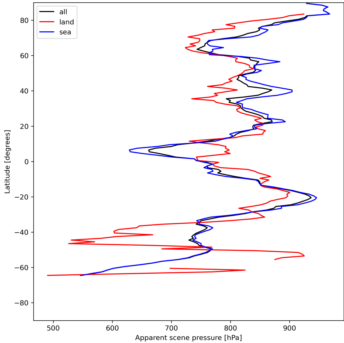
Figure 19: Zonal average of “Apparent scene pressure” for 2024-06-19 to 2024-06-21.
