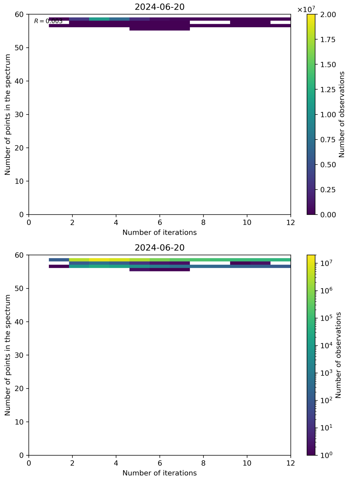
Figure 99: Scatter density plot of “Number of iterations” against “Number of points in the spectrum” for 2024-06-19 to 2024-06-21.
