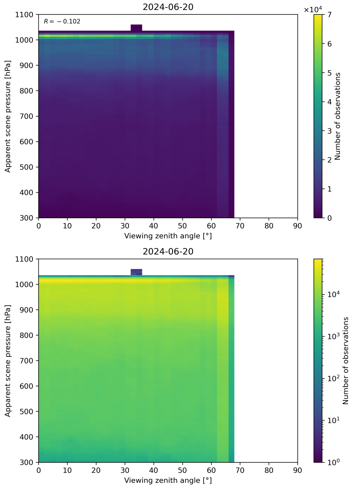
Figure 118: Scatter density plot of “Viewing zenith angle” against “Apparent scene pressure” for 2024-06-19 to 2024-06-21.
