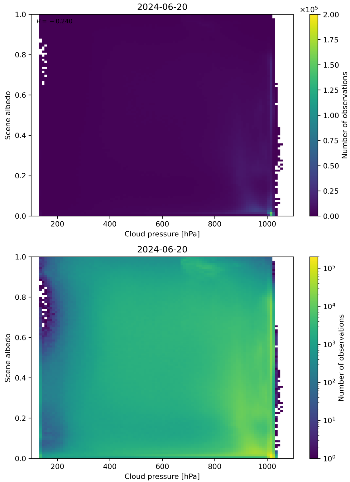
Figure 83: Scatter density plot of “Cloud pressure” against “Scene albedo” for 2024-06-19 to 2024-06-21.
