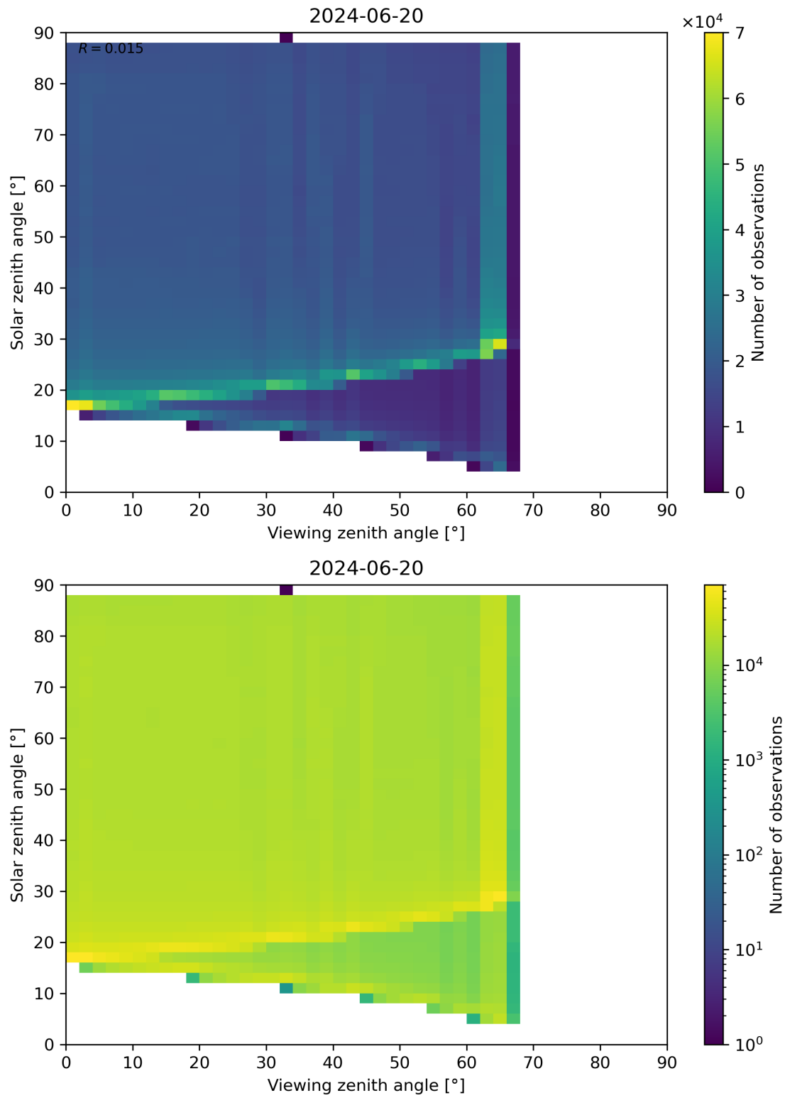
Figure 127: Scatter density plot of “Viewing zenith angle” against “Solar zenith angle” for 2024-06-19 to 2024-06-21.
