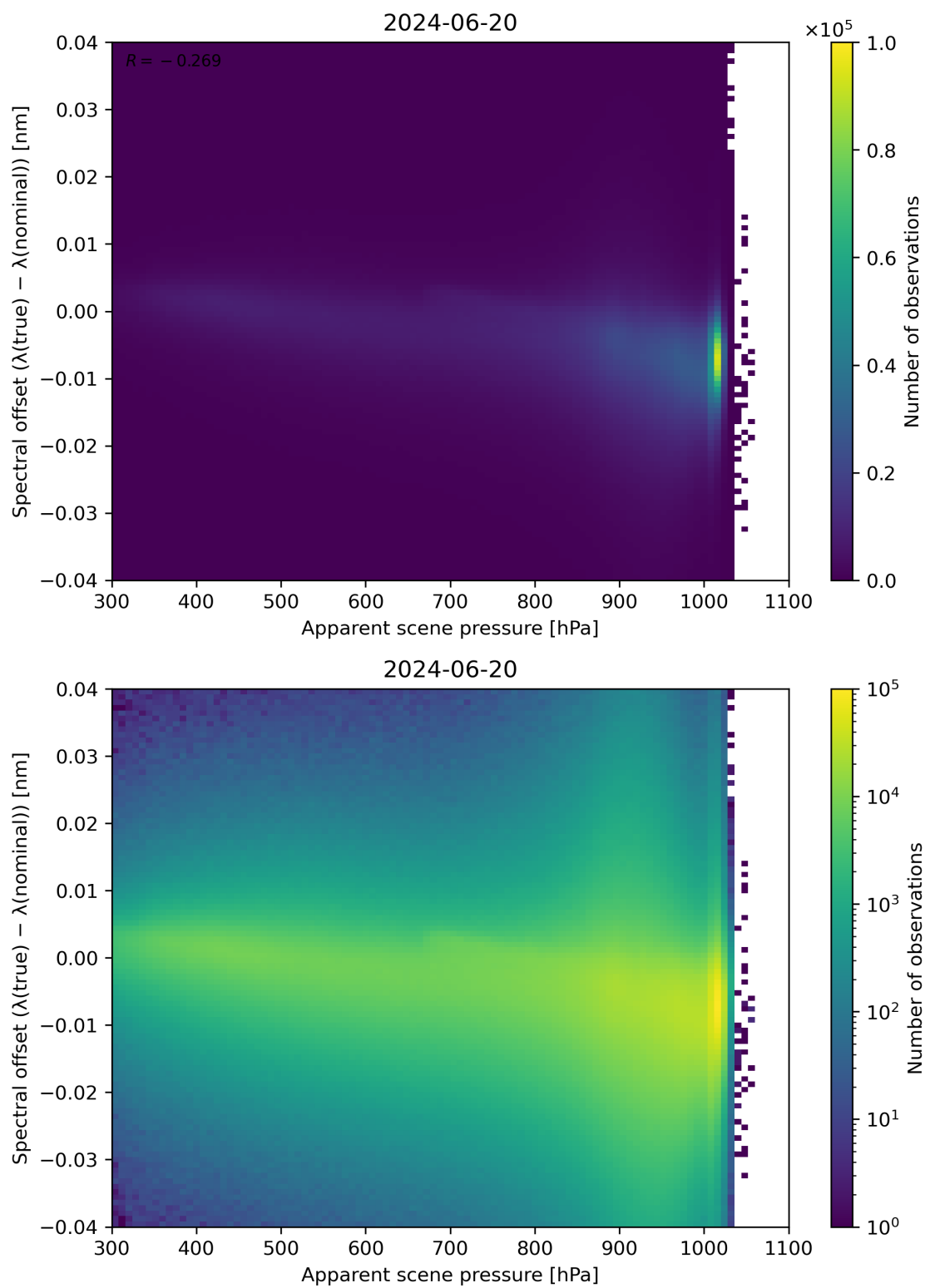
Figure 67: Scatter density plot of “Apparent scene pressure” against “Spectral offset ( \lambda(\text{true}) - \lambda(\text{nominal}) )” for 2024-06-19 to 2024-06-21.
