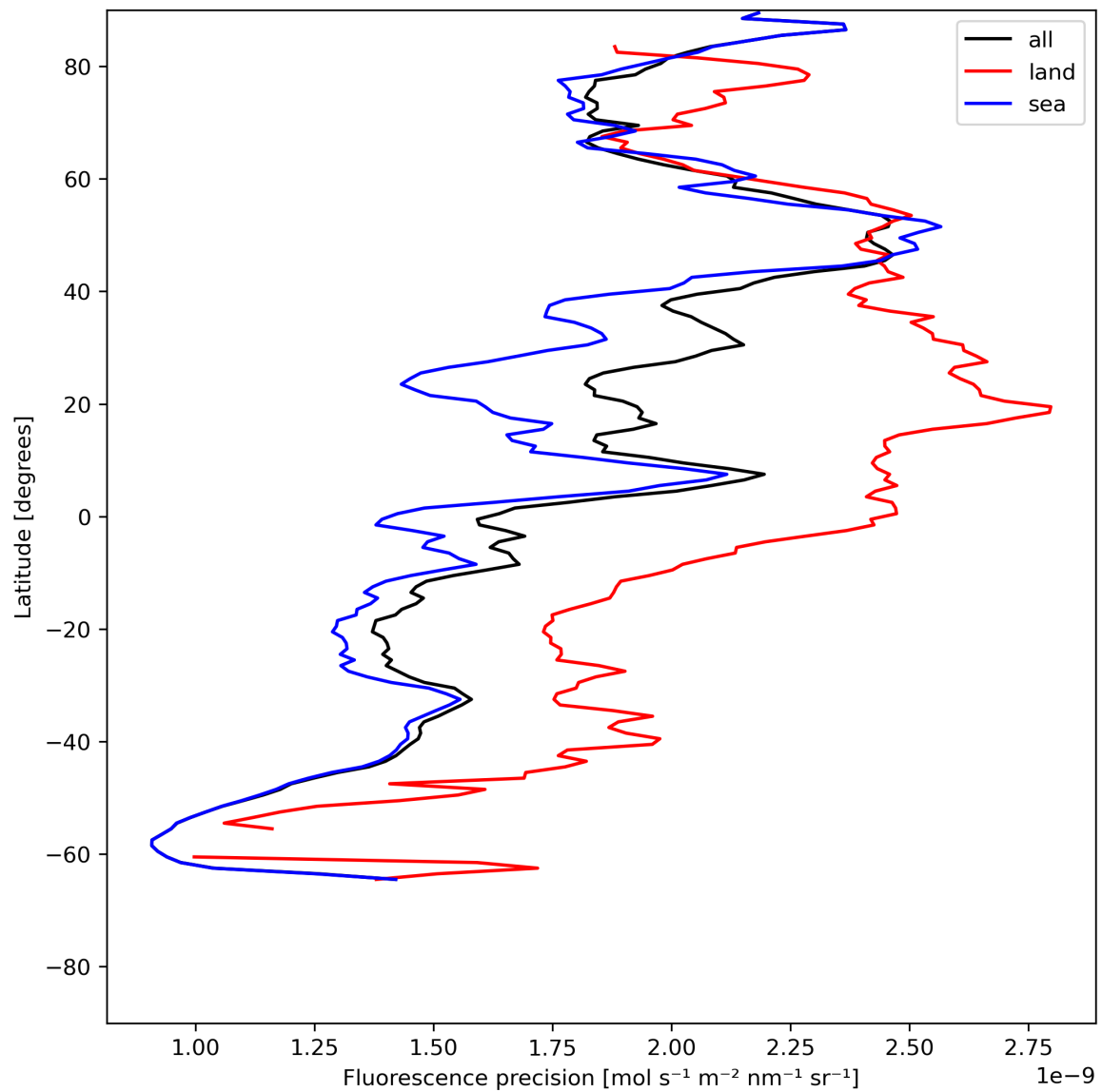
Figure 24: Zonal average of “Fluorescence precision” for 2024-06-19 to 2024-06-21.
