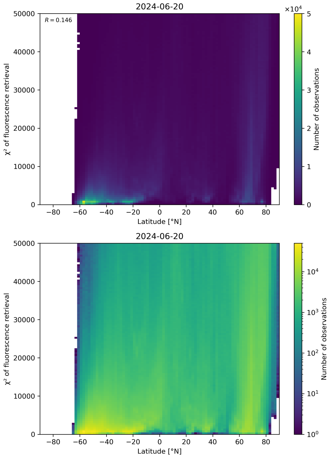
Figure 89: Scatter density plot of “Latitude” against “ \chi^2 of fluorescence retrieval” for 2024-06-19 to 2024-06-21.
