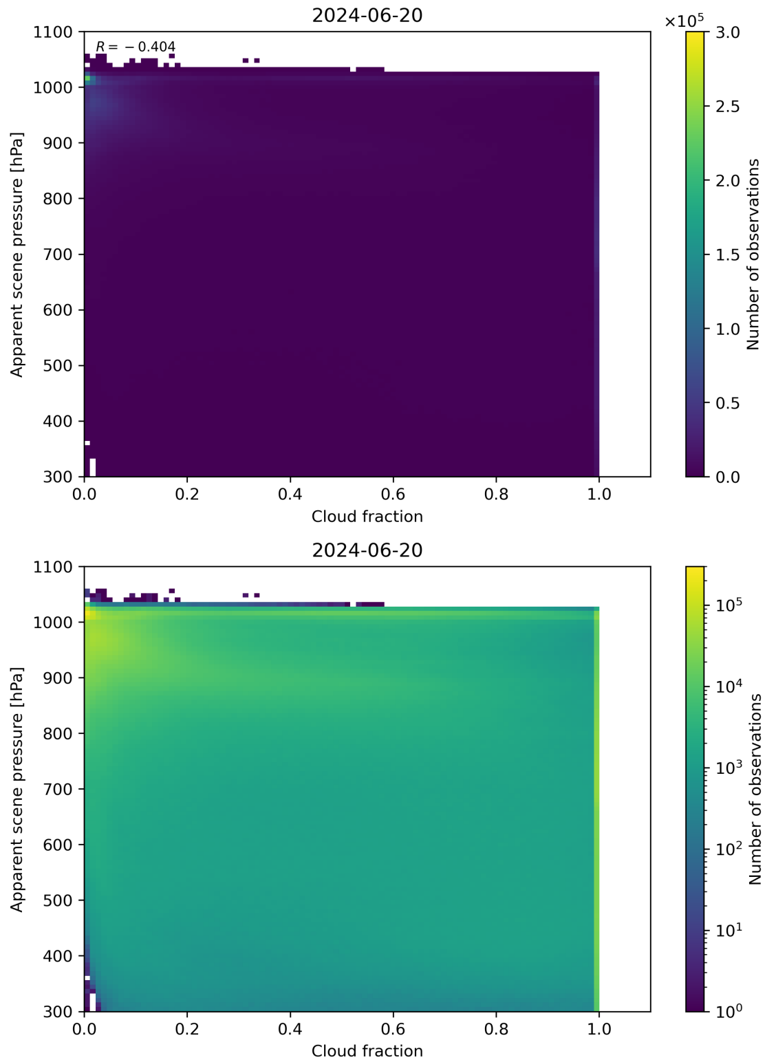
Figure 70: Scatter density plot of “Cloud fraction” against “Apparent scene pressure” for 2024-06-19 to 2024-06-21.
