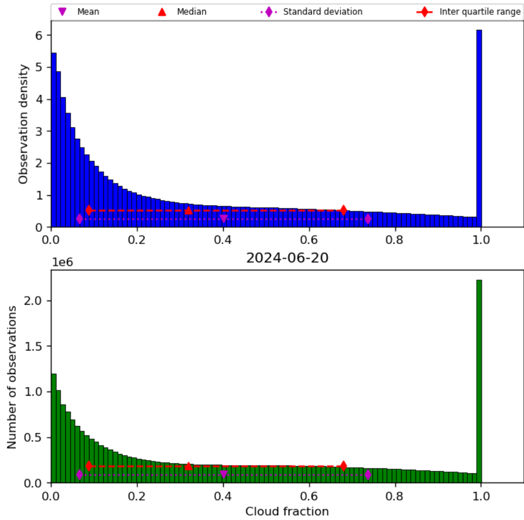
Figure 32: Histogram of “Cloud fraction” for 2024-06-19 to 2024-06-21
