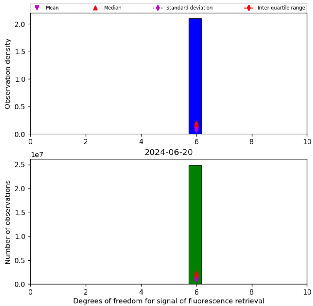
Figure 43: Histogram of “Degrees of freedom for signal of fluorescence retrieval” for 2024-06-19 to 2024-06-21
