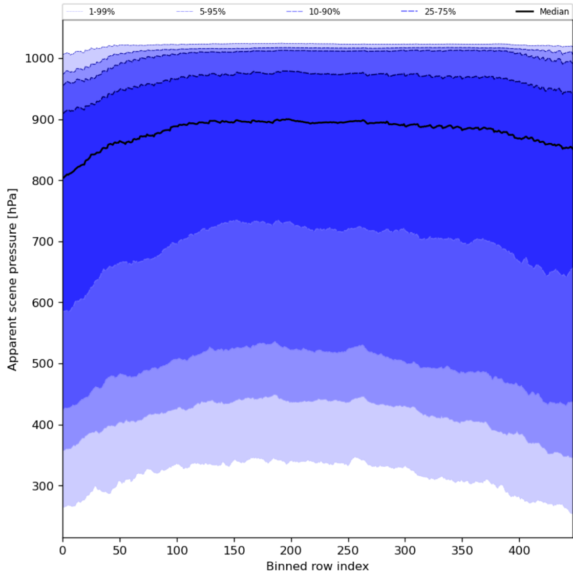
Figure 53: Along track statistics of “Apparent scene pressure” for 2024-06-19 to 2024-06-21
