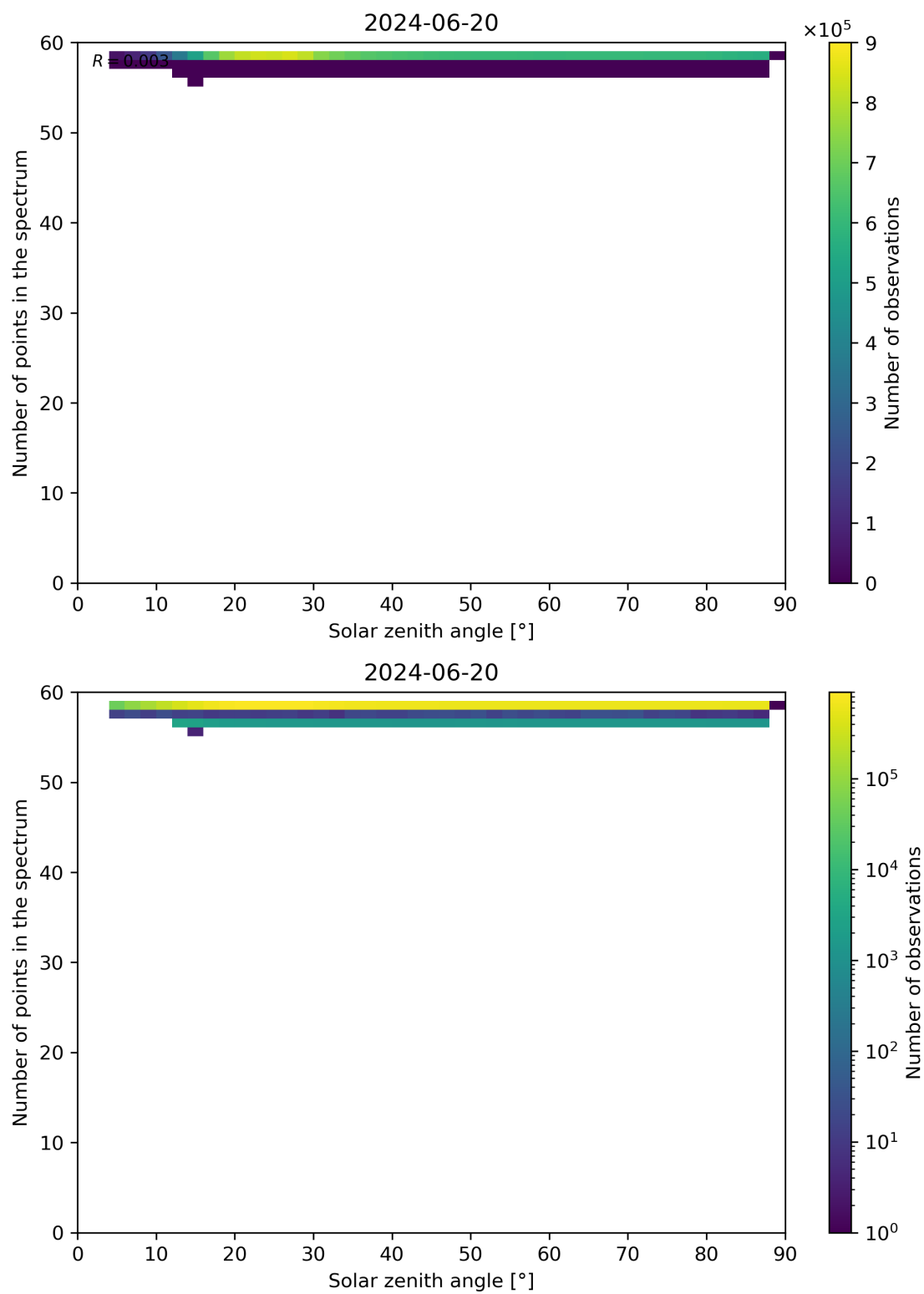
Figure 115: Scatter density plot of “Solar zenith angle” against “Number of points in the spectrum” for 2024-06-19 to 2024-06-21.
