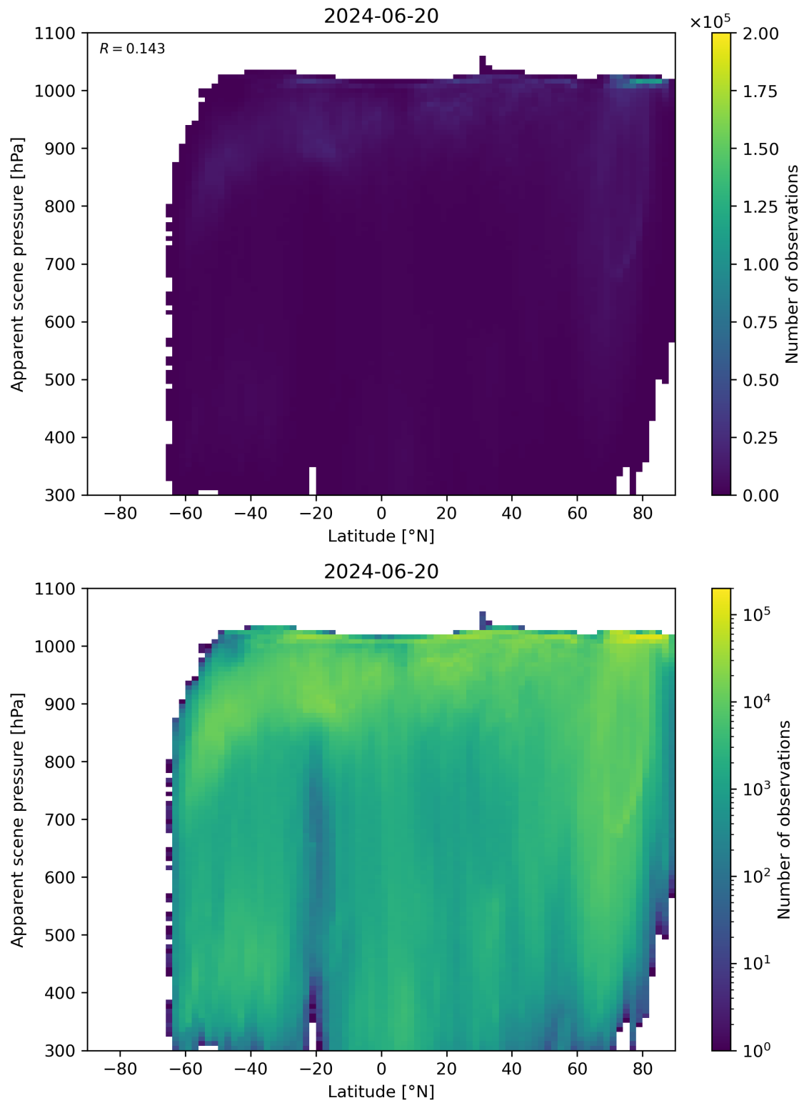
Figure 88: Scatter density plot of “Latitude” against “Apparent scene pressure” for 2024-06-19 to 2024-06-21.
