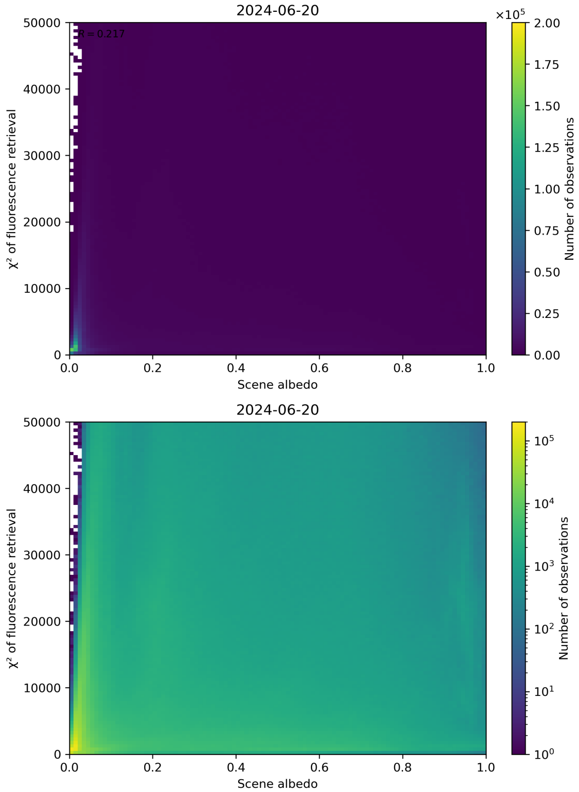
Figure 103: Scatter density plot of “Scene albedo” against “ \chi^2 of fluorescence retrieval” for 2024-06-19 to 2024-06-21.
