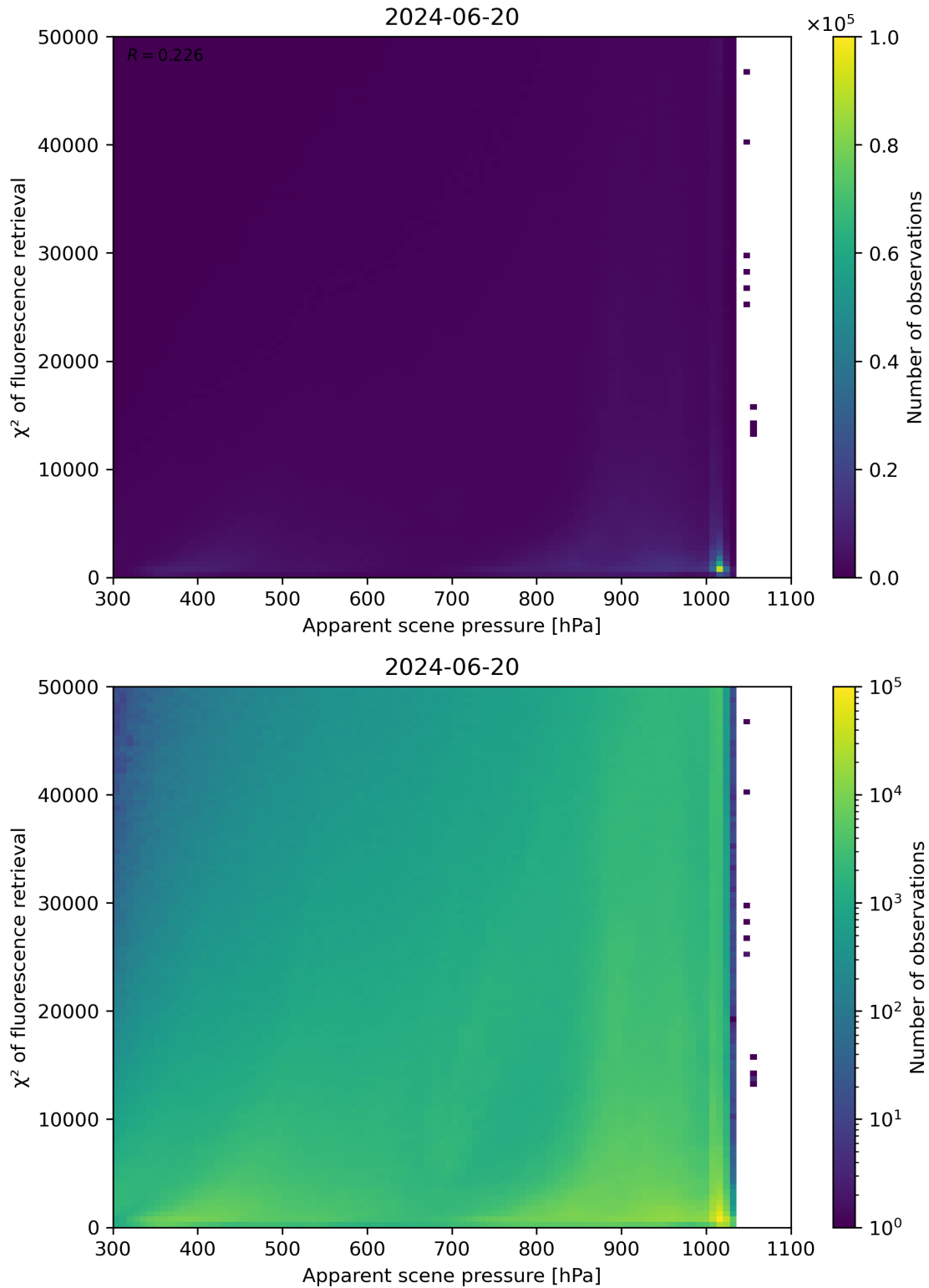
Figure 63: Scatter density plot of “Apparent scene pressure” against “ \chi^2 of fluorescence retrieval” for 2024-06-19 to 2024-06-21.
