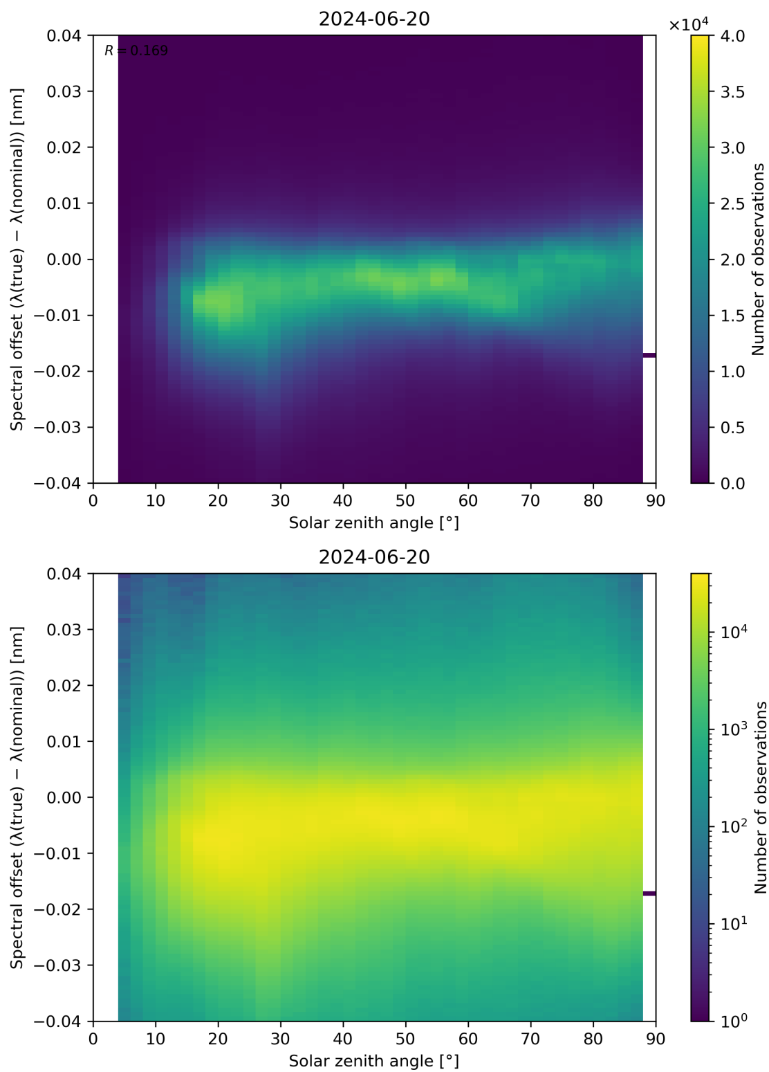
Figure 117: Scatter density plot of “Solar zenith angle” against “Spectral offset ( \lambda(\text{true}) - \lambda(\text{nominal}) )” for 2024-06-19 to 2024-06-21.
