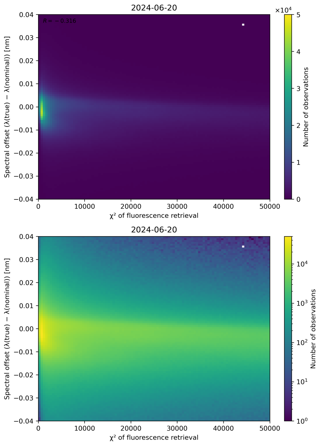
Figure 69: Scatter density plot of “ \chi^2 of fluorescence retrieval” against “Spectral offset ( \lambda(\text{true}) - \lambda(\text{nominal}) )” for 2024-06-19 to 2024-06-21.
