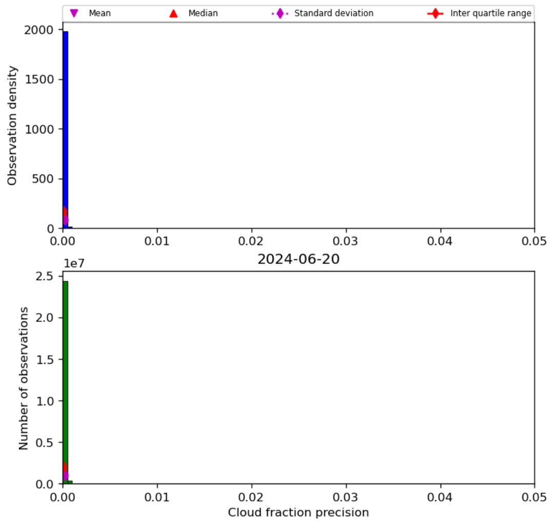
Figure 33: Histogram of “Cloud fraction precision” for 2024-06-19 to 2024-06-21
