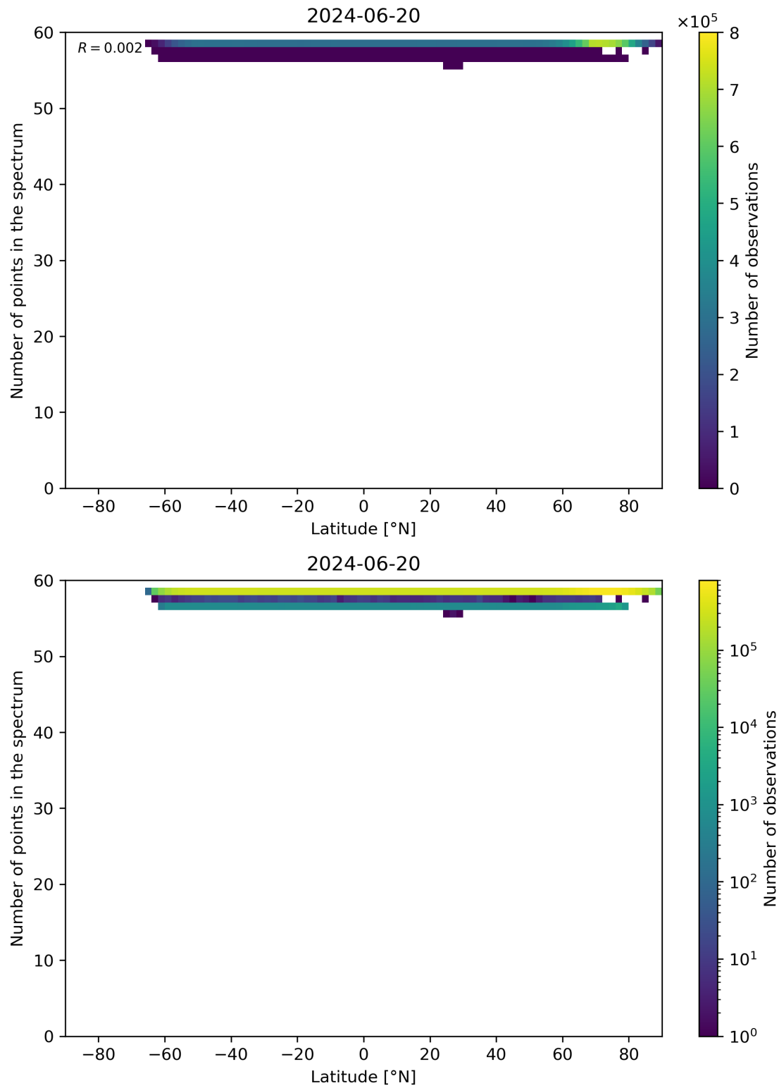
Figure 94: Scatter density plot of “Latitude” against “Number of points in the spectrum” for 2024-06-19 to 2024-06-21.
