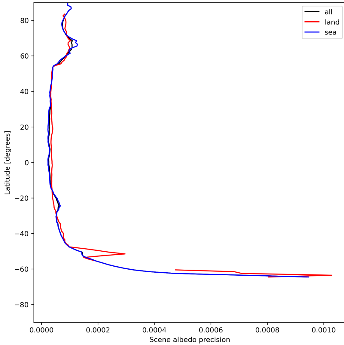
Figure 18: Zonal average of “Scene albedo precision” for 2024-06-19 to 2024-06-21.
