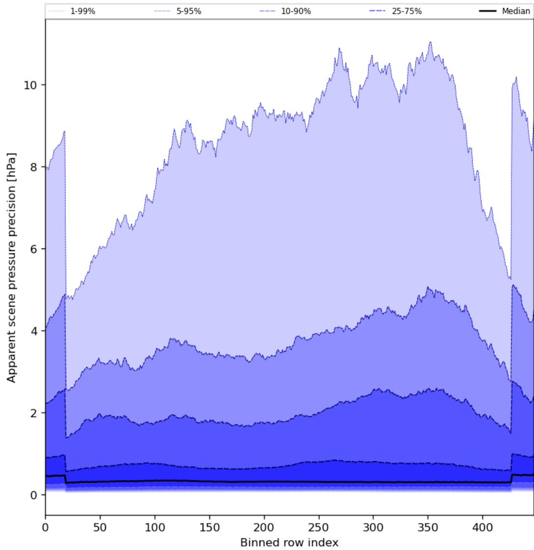
Figure 54: Along track statistics of “Apparent scene pressure precision” for 2024-06-19 to 2024-06-21
