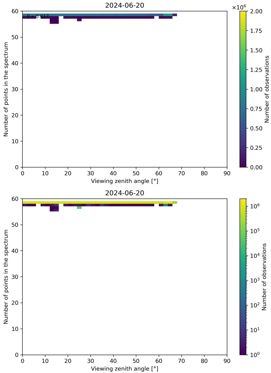
Figure 125: Scatter density plot of “Viewing zenith angle” against “Number of points in the spectrum” for 2024-06-19 to 2024-06-21.
