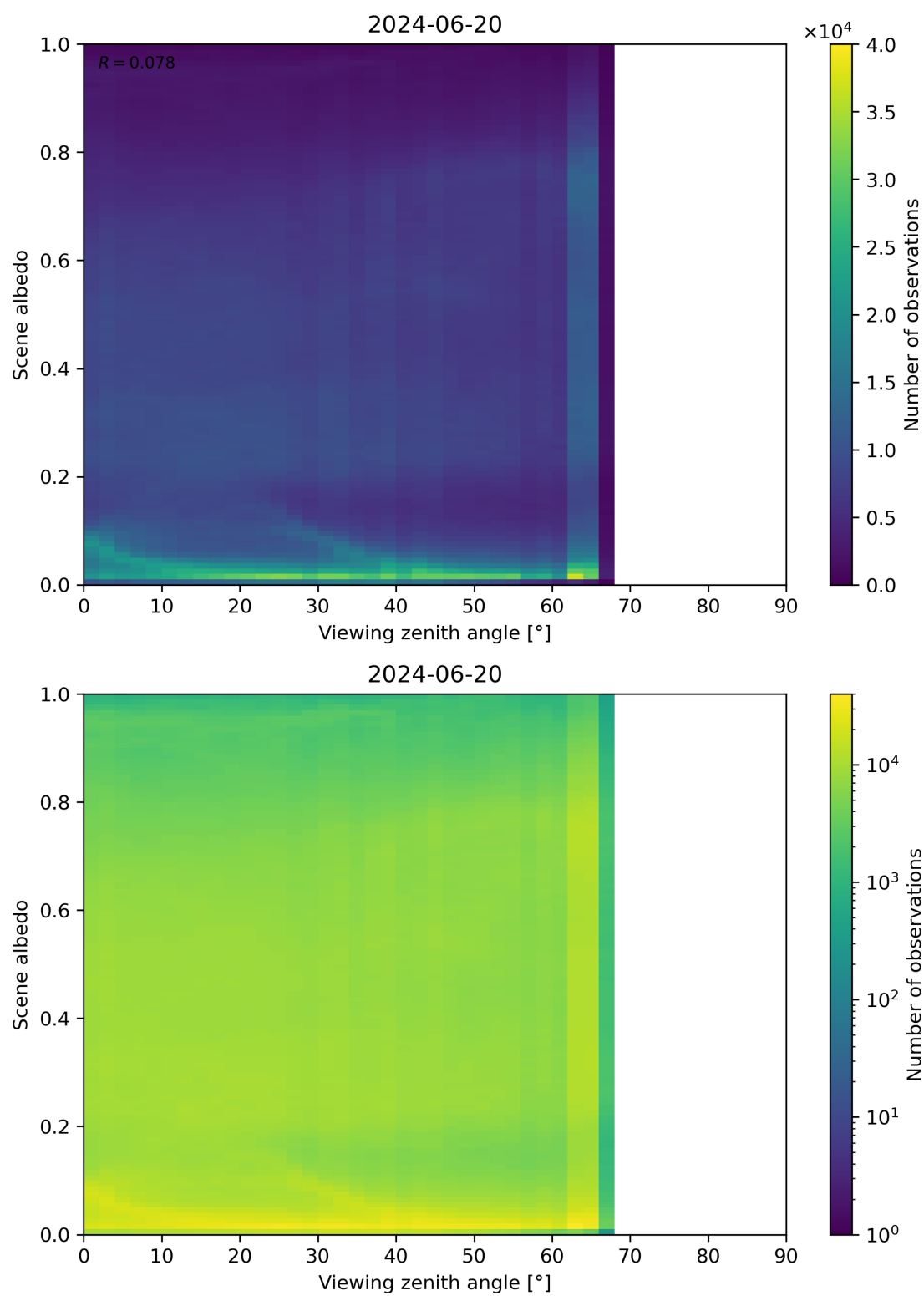
Figure 126: Scatter density plot of “Viewing zenith angle” against “Scene albedo” for 2024-06-19 to 2024-06-21.
