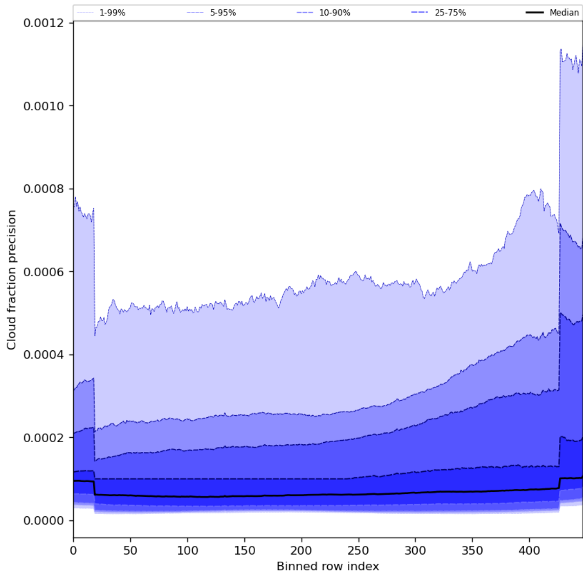
Figure 50: Along track statistics of “Cloud fraction precision” for 2024-06-19 to 2024-06-21
