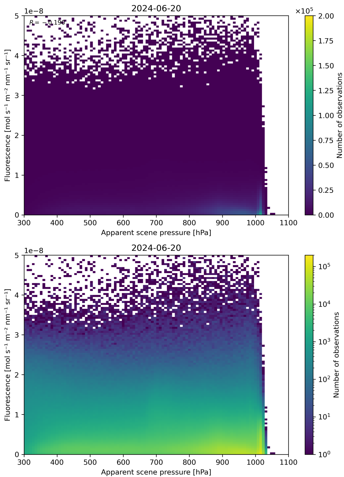
Figure 64: Scatter density plot of “Apparent scene pressure” against “Fluorescence” for 2024-06-19 to 2024-06-21.
