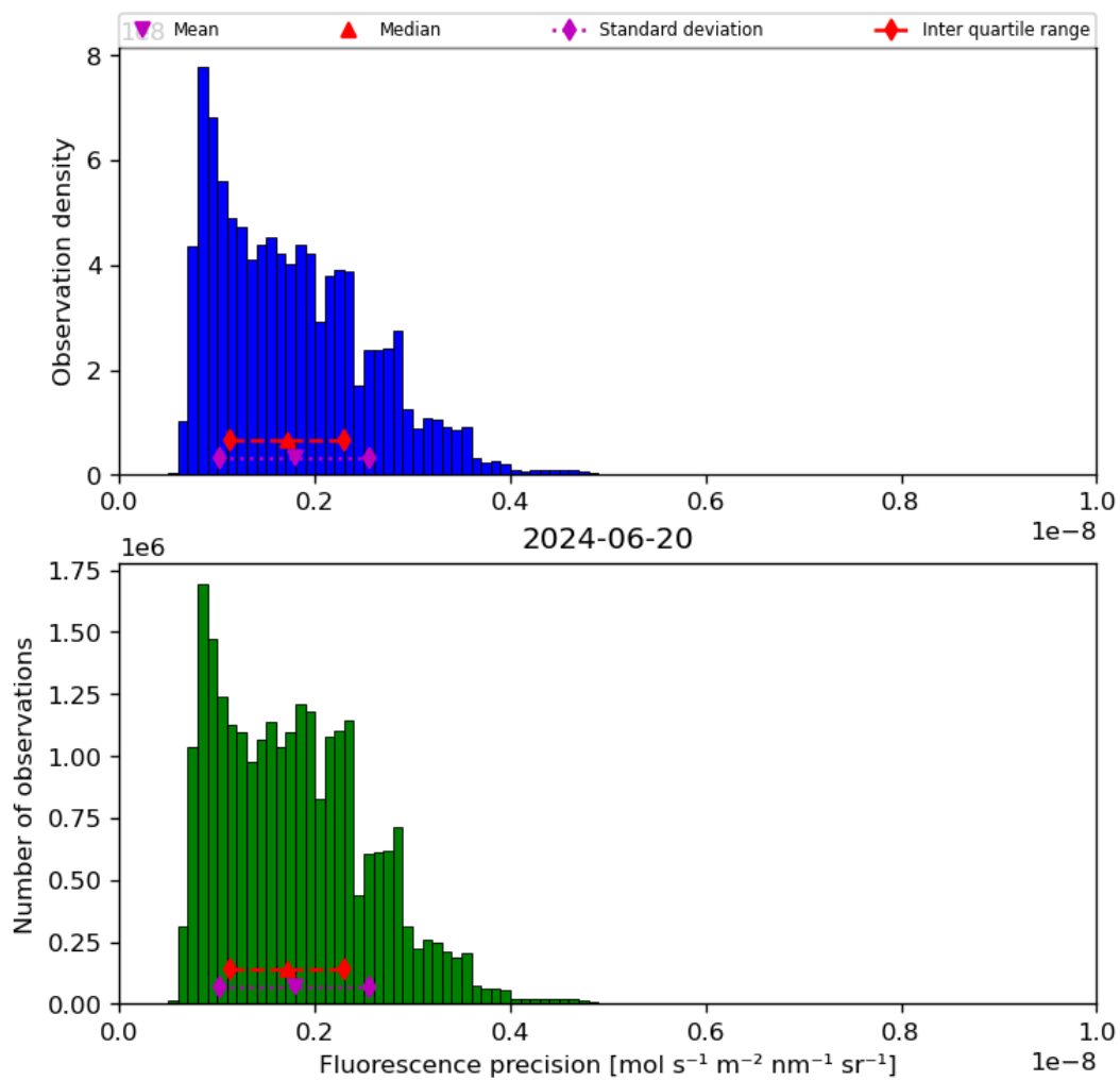
Figure 41: Histogram of “Fluorescence precision” for 2024-06-19 to 2024-06-21
