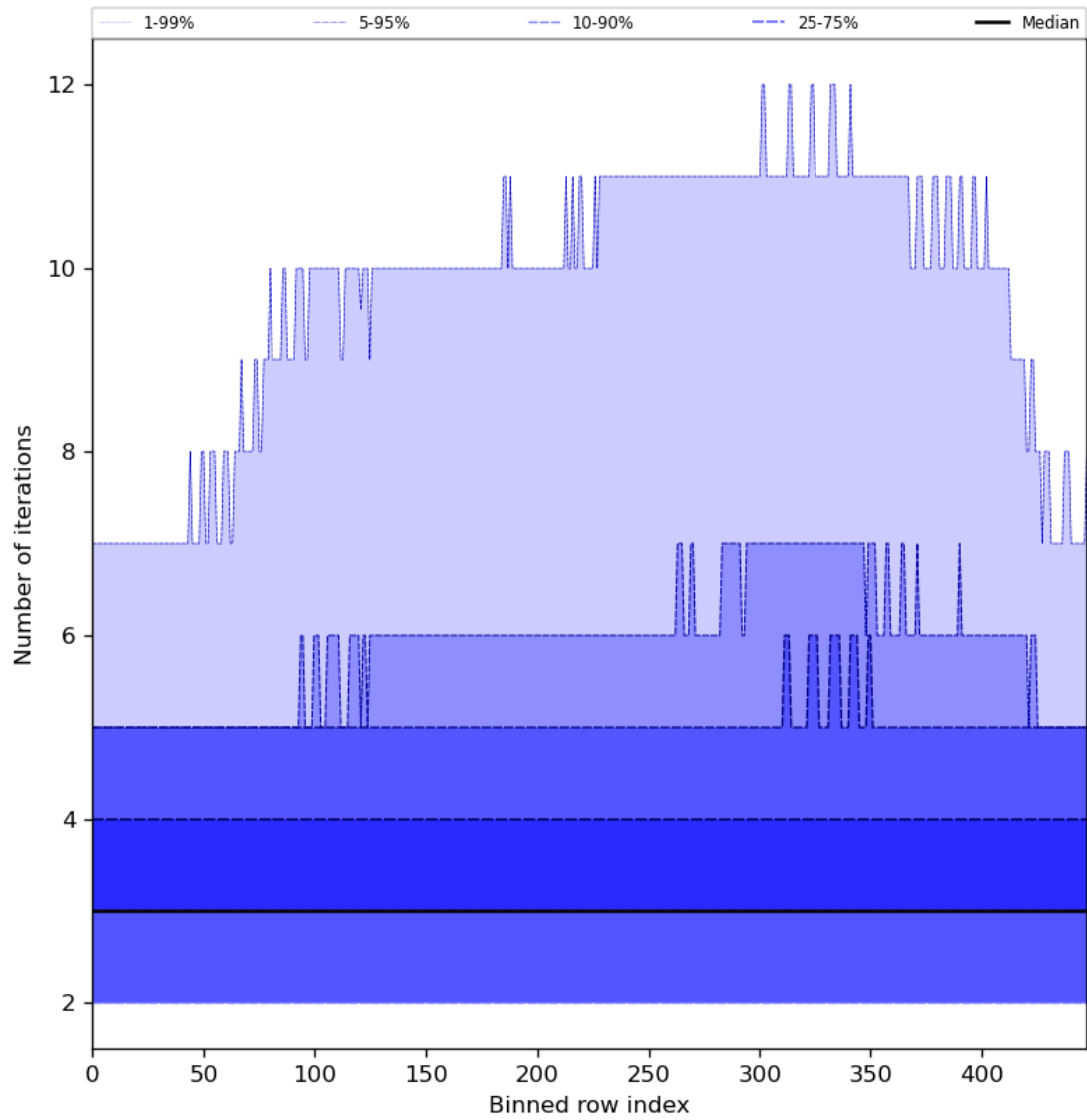
Figure 56: Along track statistics of “Number of iterations” for 2024-06-19 to 2024-06-21
