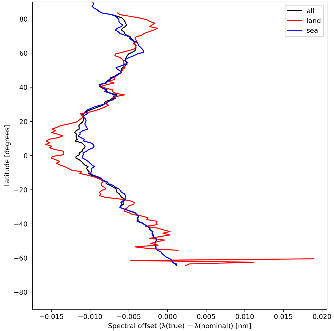
Figure 28: Zonal average of “Spectral offset ( \lambda(\text{true}) - \lambda(\text{nominal}) )” for 2024-06-19 to 2024-06-21.
