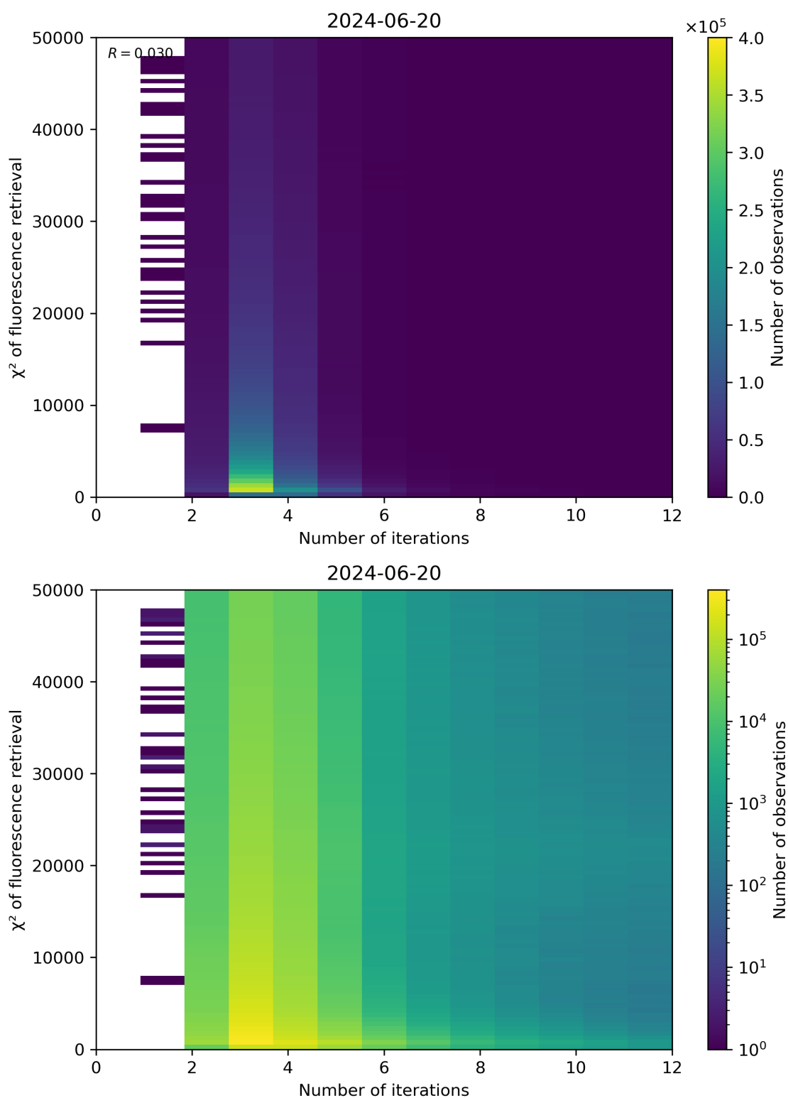
Figure 97: Scatter density plot of “Number of iterations” against “ \chi^2 of fluorescence retrieval” for 2024-06-19 to 2024-06-21.
