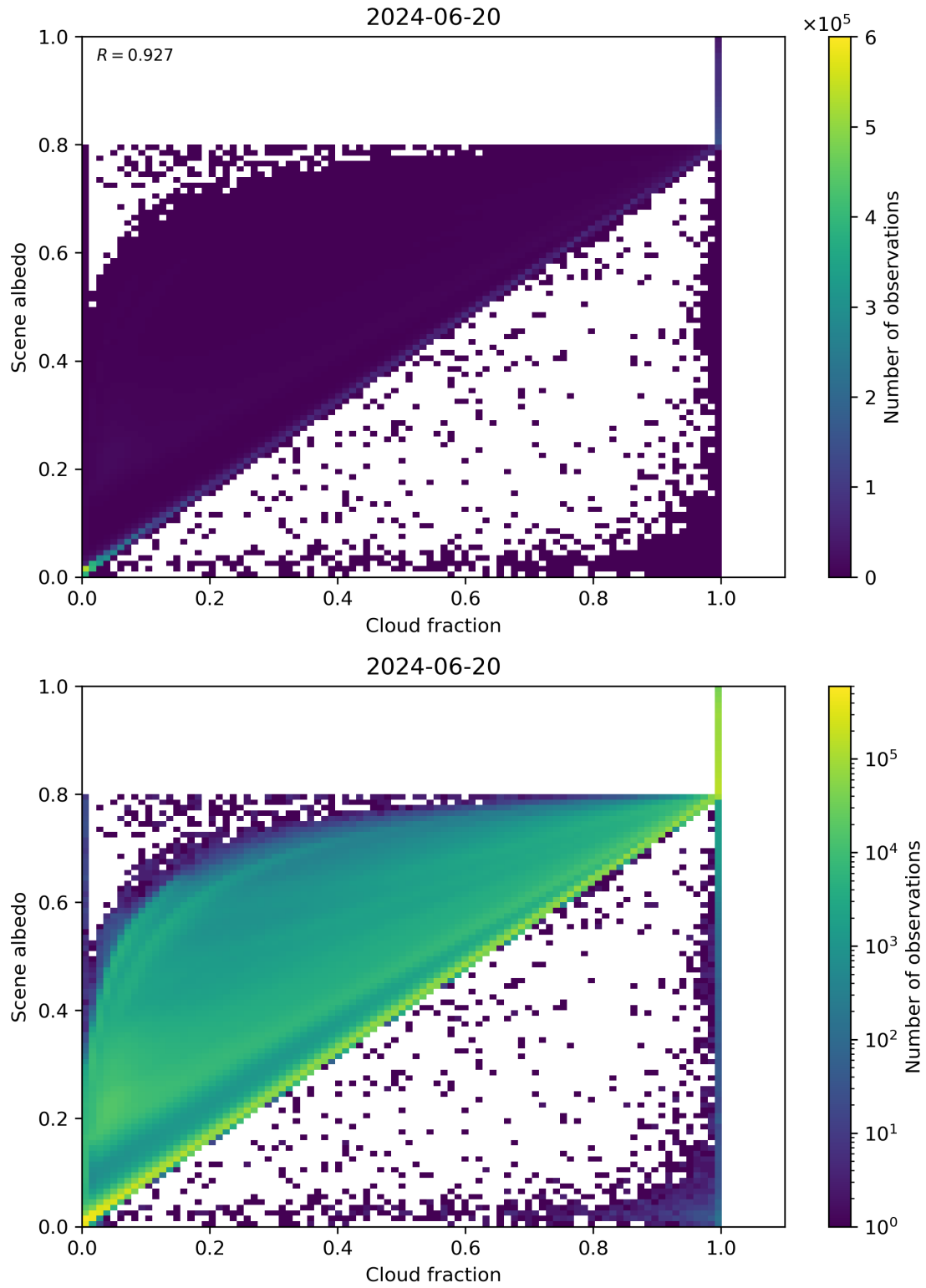
Figure 75: Scatter density plot of “Cloud fraction” against “Scene albedo” for 2024-06-19 to 2024-06-21.
