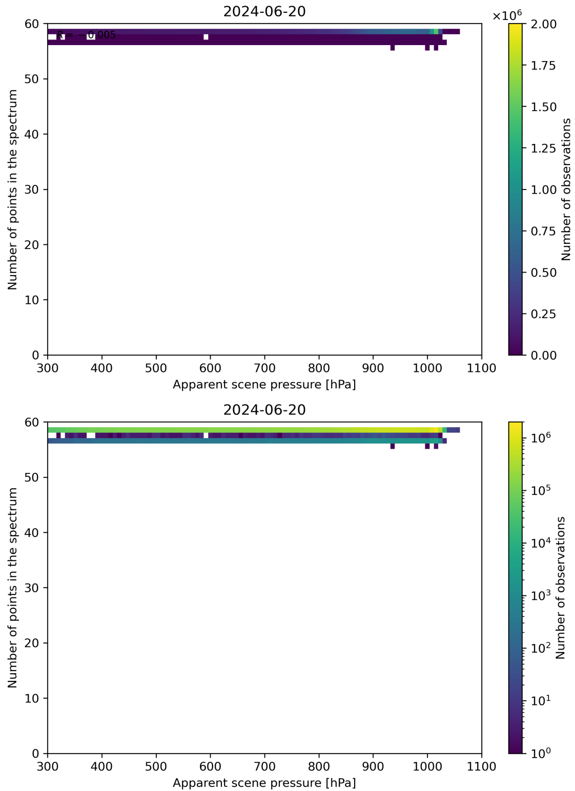
Figure 66: Scatter density plot of “Apparent scene pressure” against “Number of points in the spectrum” for 2024-06-19 to 2024-06-21.
