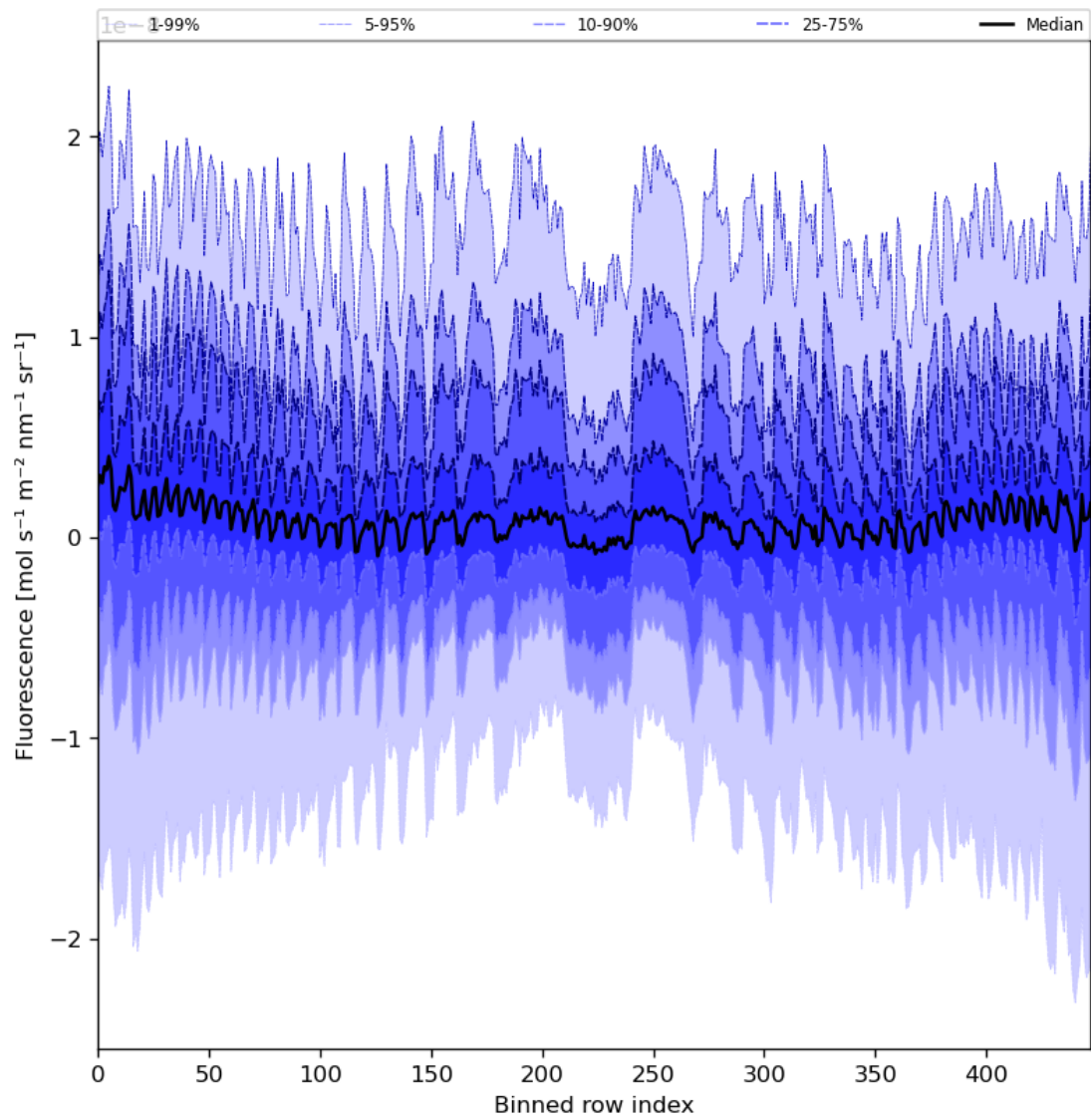
Figure 57: Along track statistics of “Fluorescence” for 2024-06-19 to 2024-06-21
