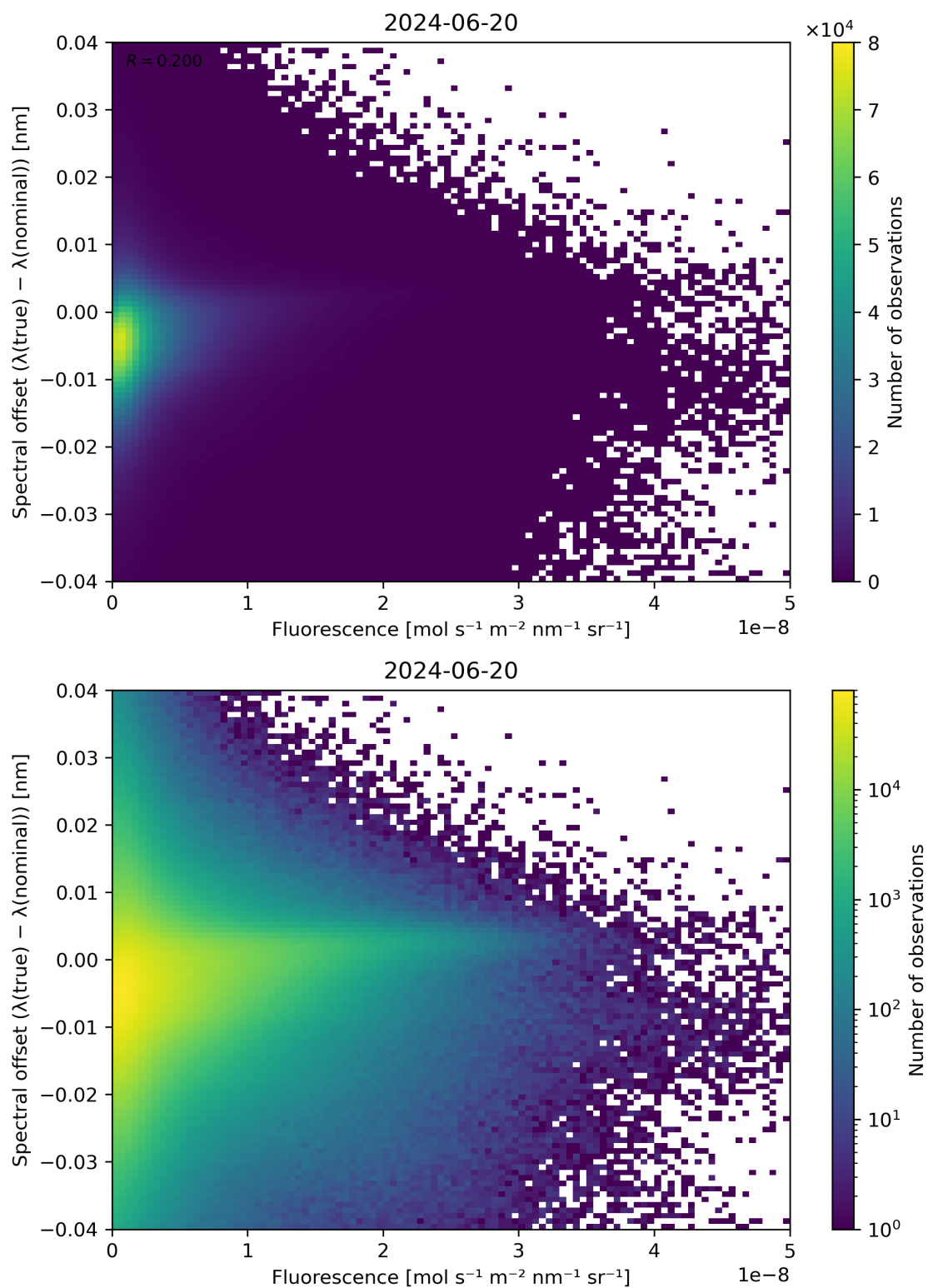
Figure 87: Scatter density plot of “Fluorescence” against “Spectral offset ( \lambda(\text{true}) - \lambda(\text{nominal}) )” for 2024-06-19 to 2024-06-21.
