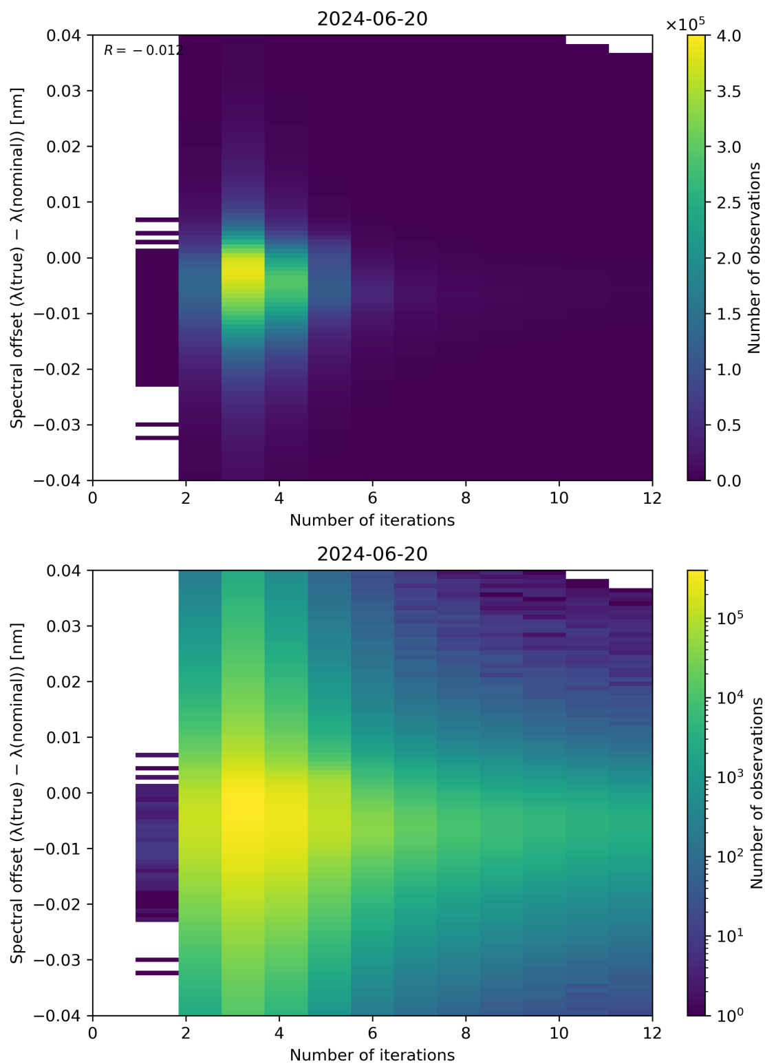
Figure 100: Scatter density plot of “Number of iterations” against “Spectral offset ( \lambda(\text{true}) - \lambda(\text{nominal}) )” for 2024-06-19 to 2024-06-21.
