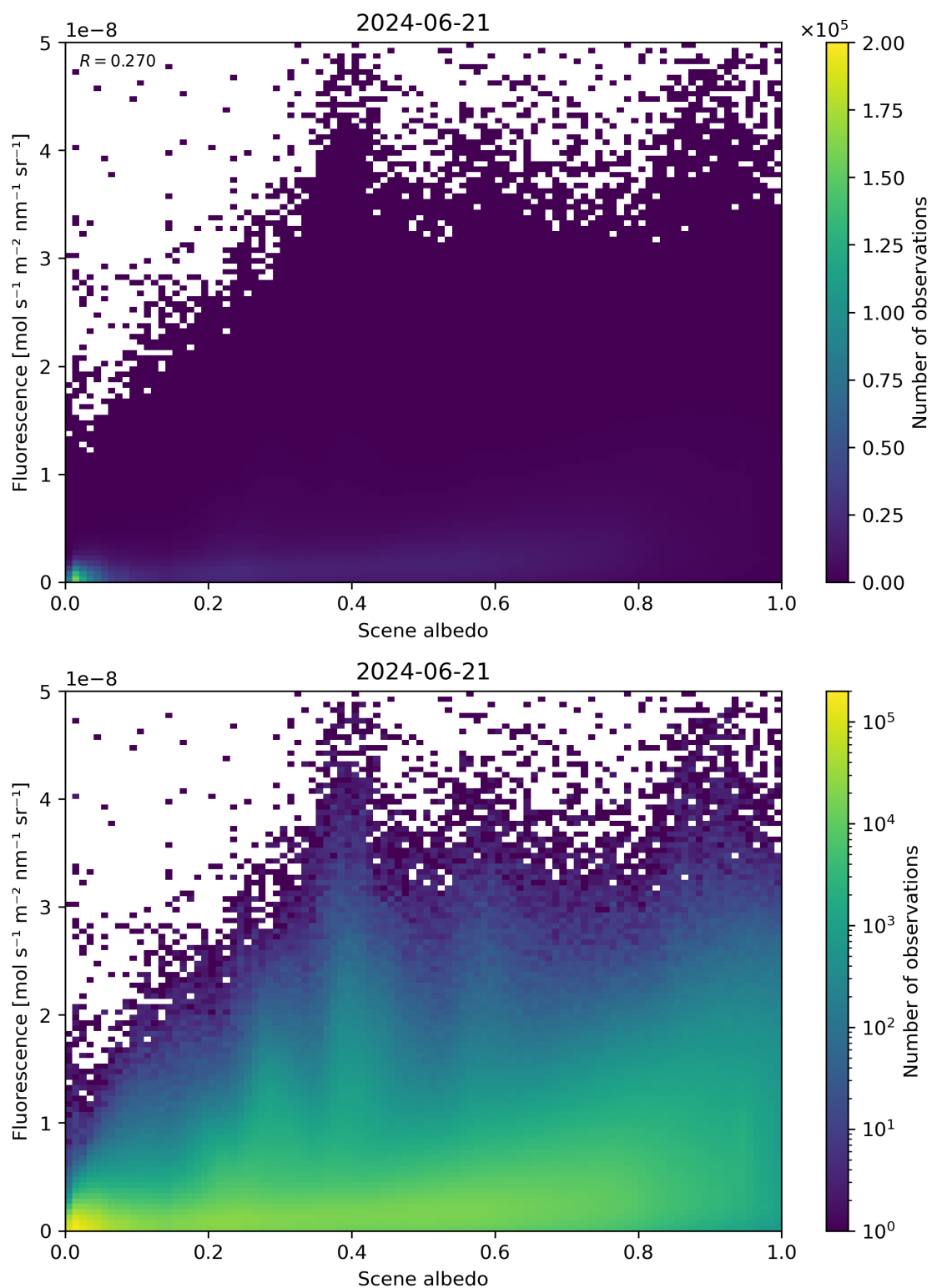
Figure 104: Scatter density plot of “Scene albedo” against “Fluorescence” for 2024-06-20 to 2024-06-22.
