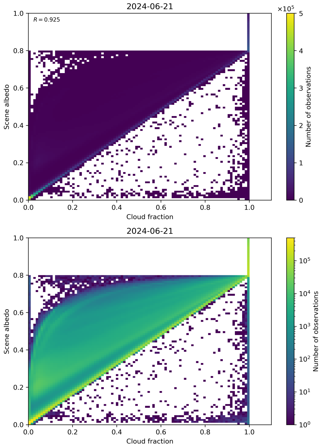
Figure 75: Scatter density plot of “Cloud fraction” against “Scene albedo” for 2024-06-20 to 2024-06-22.
