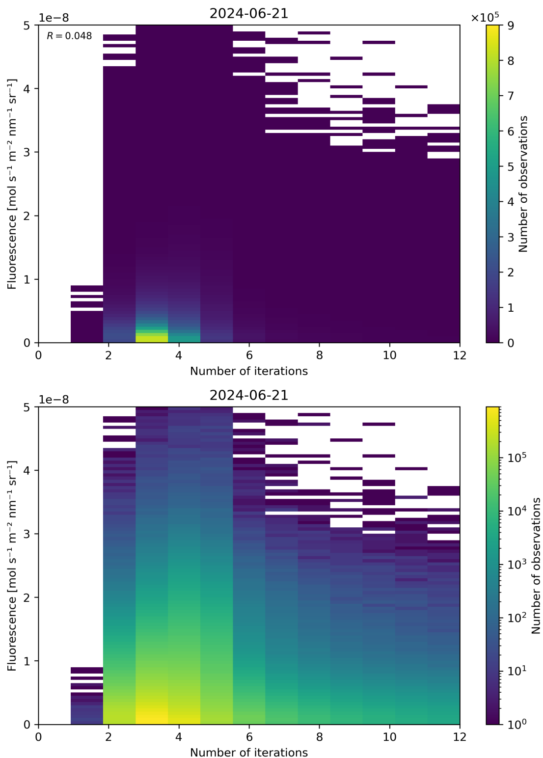
Figure 98: Scatter density plot of “Number of iterations” against “Fluorescence” for 2024-06-20 to 2024-06-22.
