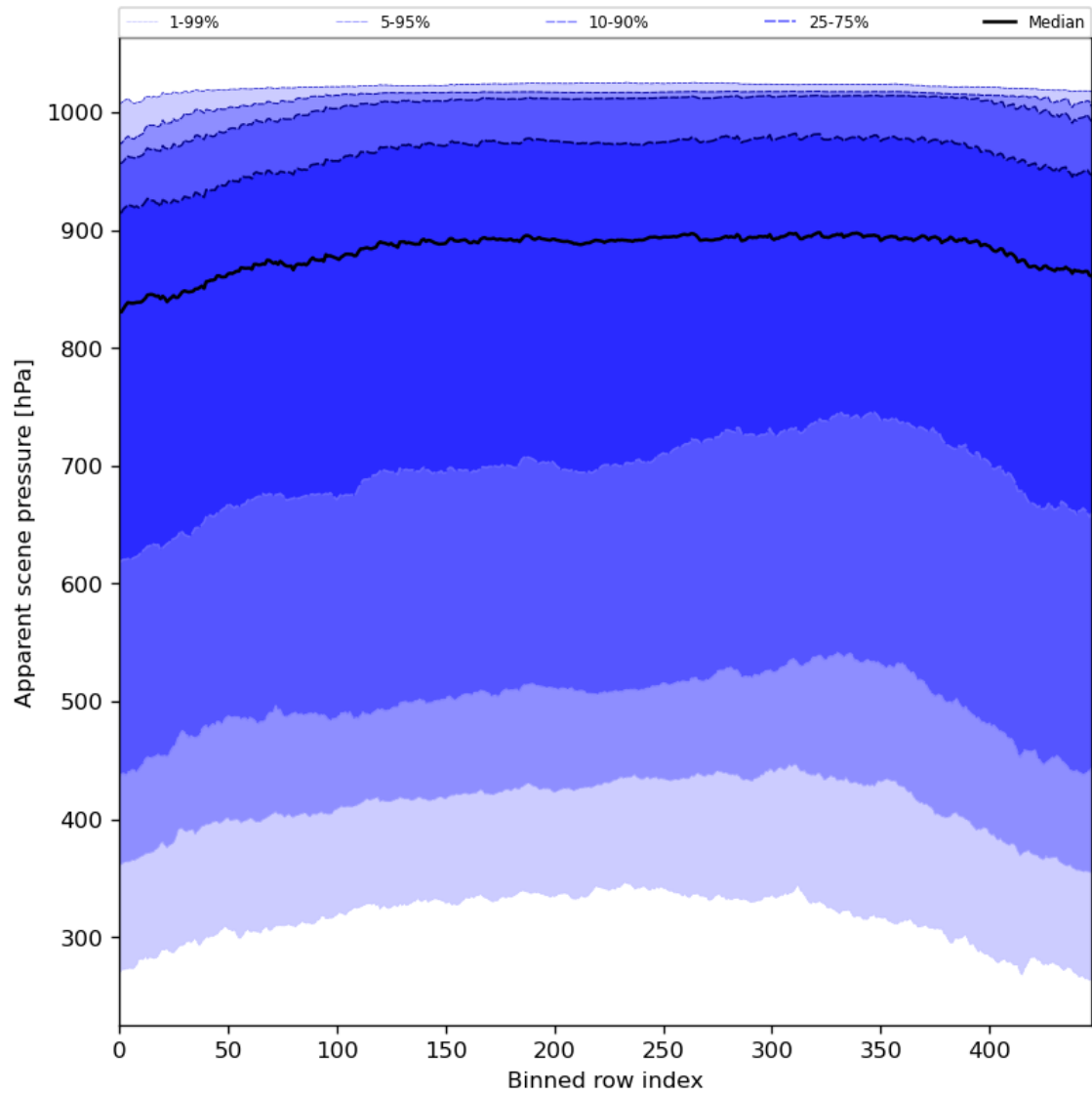
Figure 53: Along track statistics of “Apparent scene pressure” for 2024-06-20 to 2024-06-22
