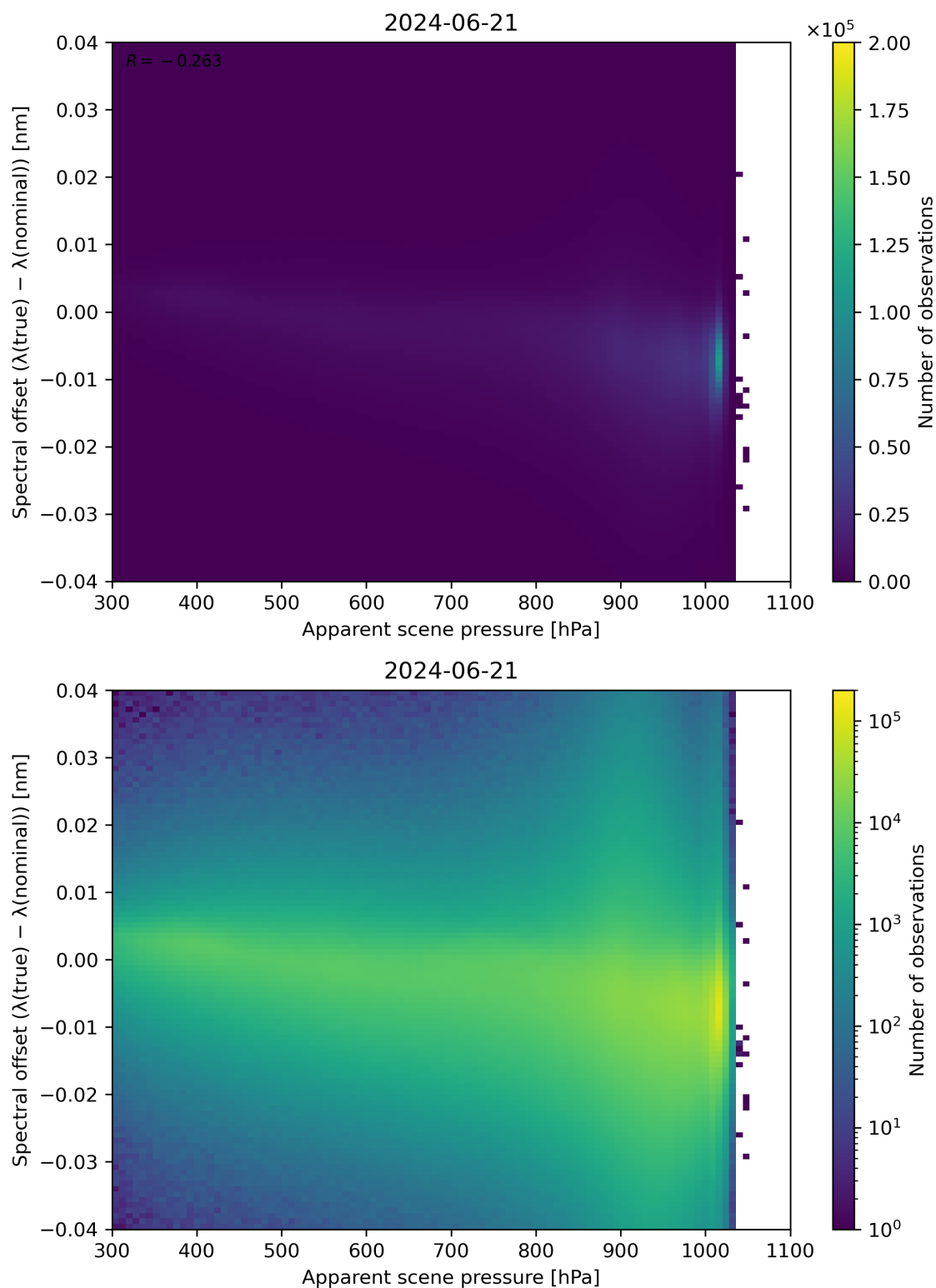
Figure 67: Scatter density plot of “Apparent scene pressure” against “Spectral offset ( \lambda(\text{true}) - \lambda(\text{nominal}) )” for 2024-06-20 to 2024-06-22.
