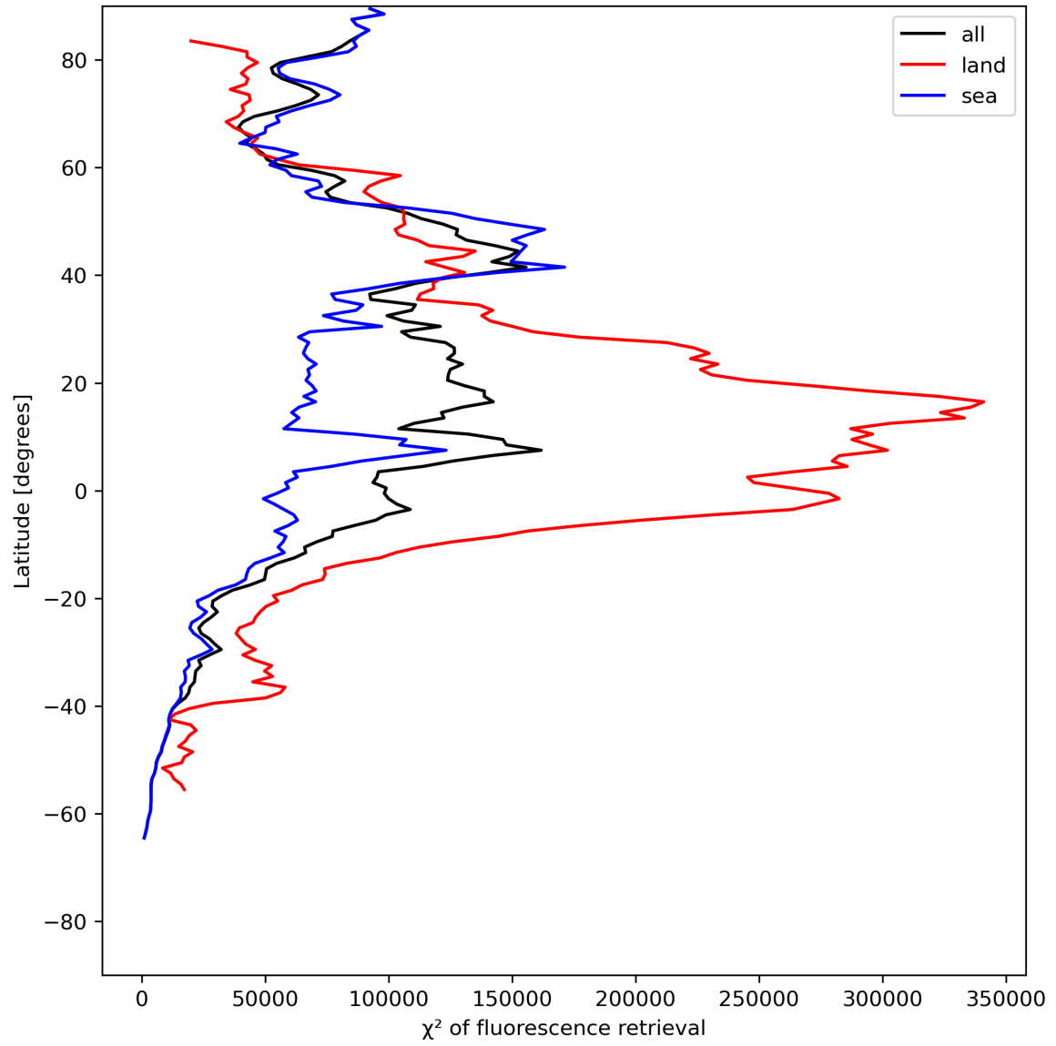
Figure 25: Zonal average of “ \chi^2 of fluorescence retrieval” for 2024-06-20 to 2024-06-22.
