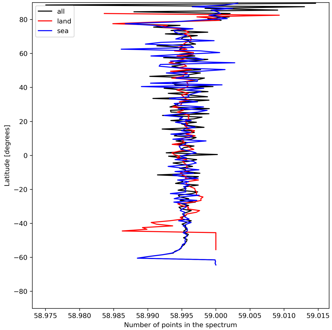
Figure 27: Zonal average of “Number of points in the spectrum” for 2024-06-20 to 2024-06-22.
