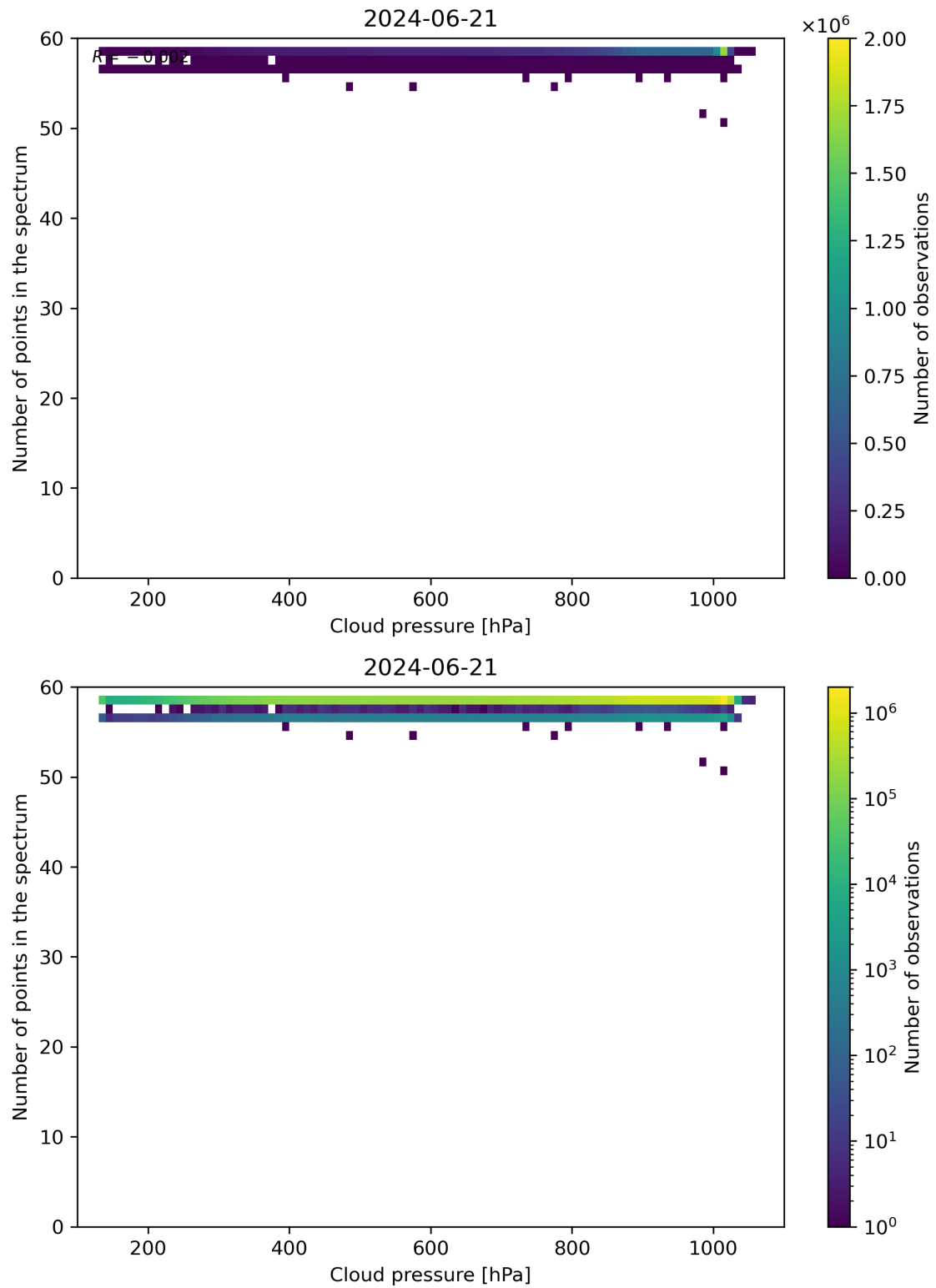
Figure 82: Scatter density plot of “Cloud pressure” against “Number of points in the spectrum” for 2024-06-20 to 2024-06-22.
