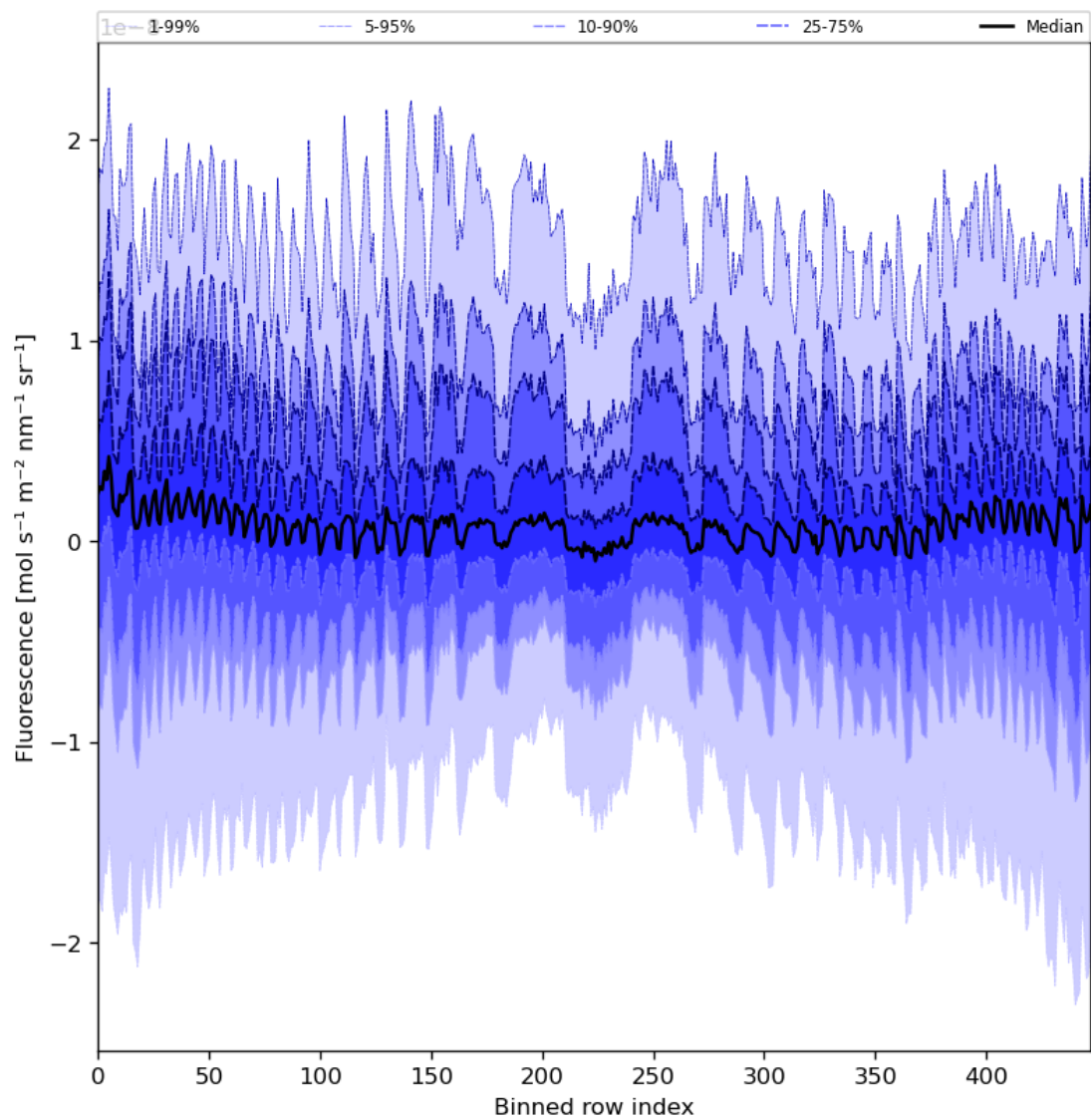
Figure 57: Along track statistics of “Fluorescence” for 2024-06-20 to 2024-06-22
