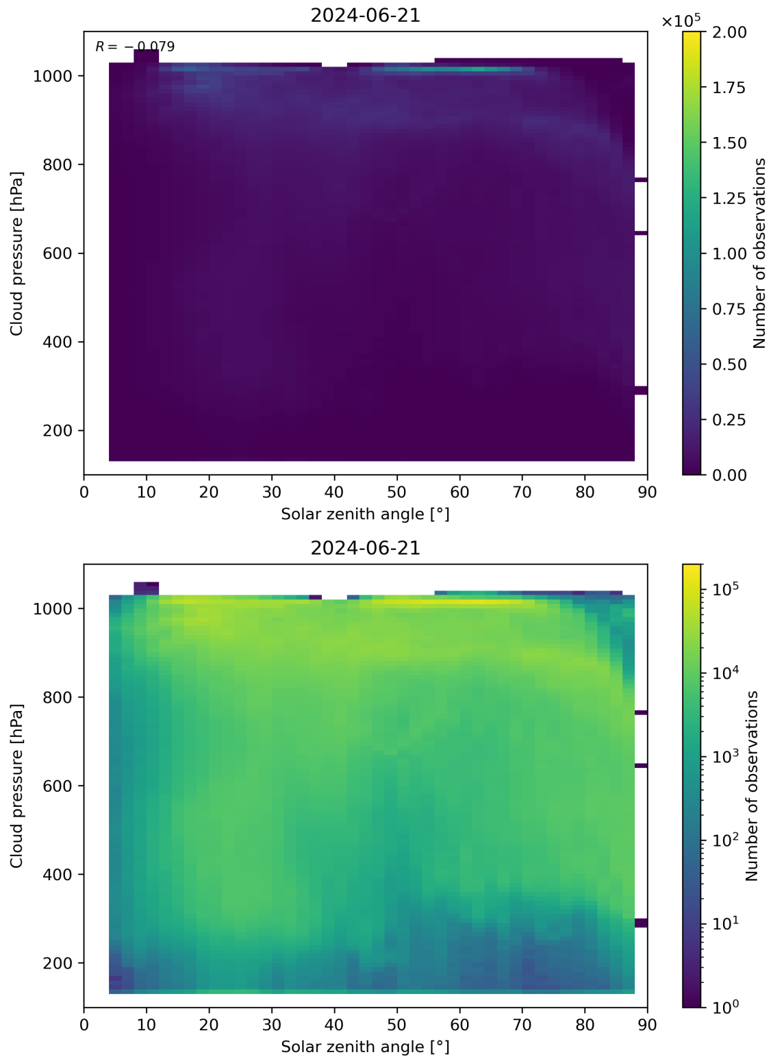
Figure 111: Scatter density plot of “Solar zenith angle” against “Cloud pressure” for 2024-06-20 to 2024-06-22.
