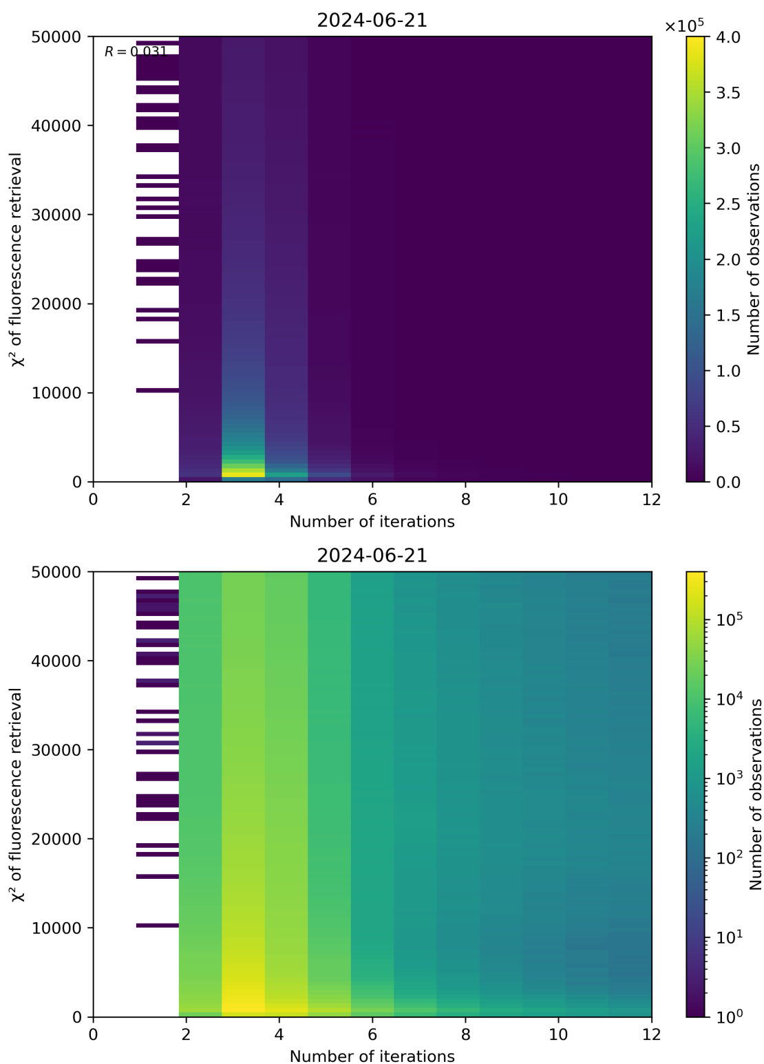
Figure 97: Scatter density plot of “Number of iterations” against “ \chi^2 of fluorescence retrieval” for 2024-06-20 to 2024-06-22.
