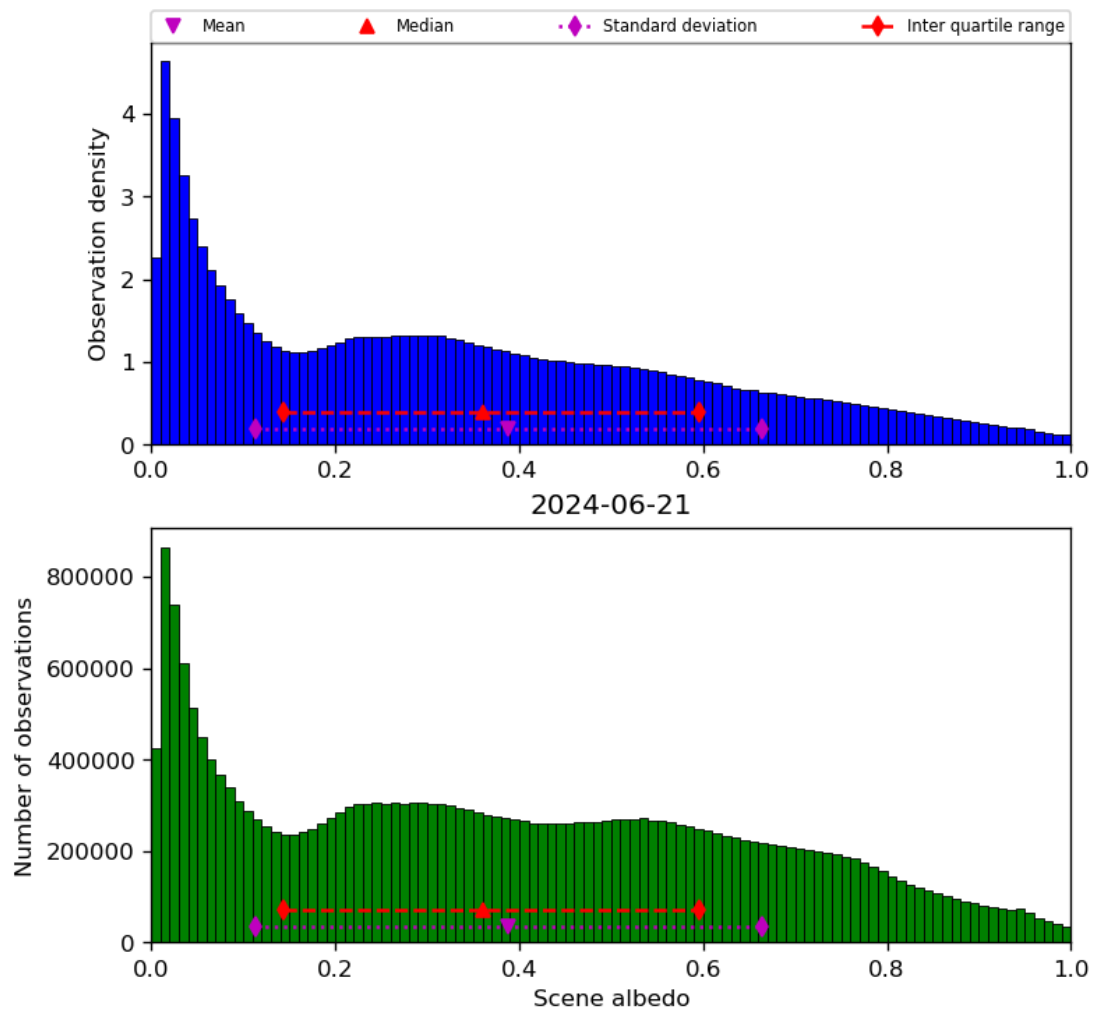
Figure 34: Histogram of “Scene albedo” for 2024-06-20 to 2024-06-22
