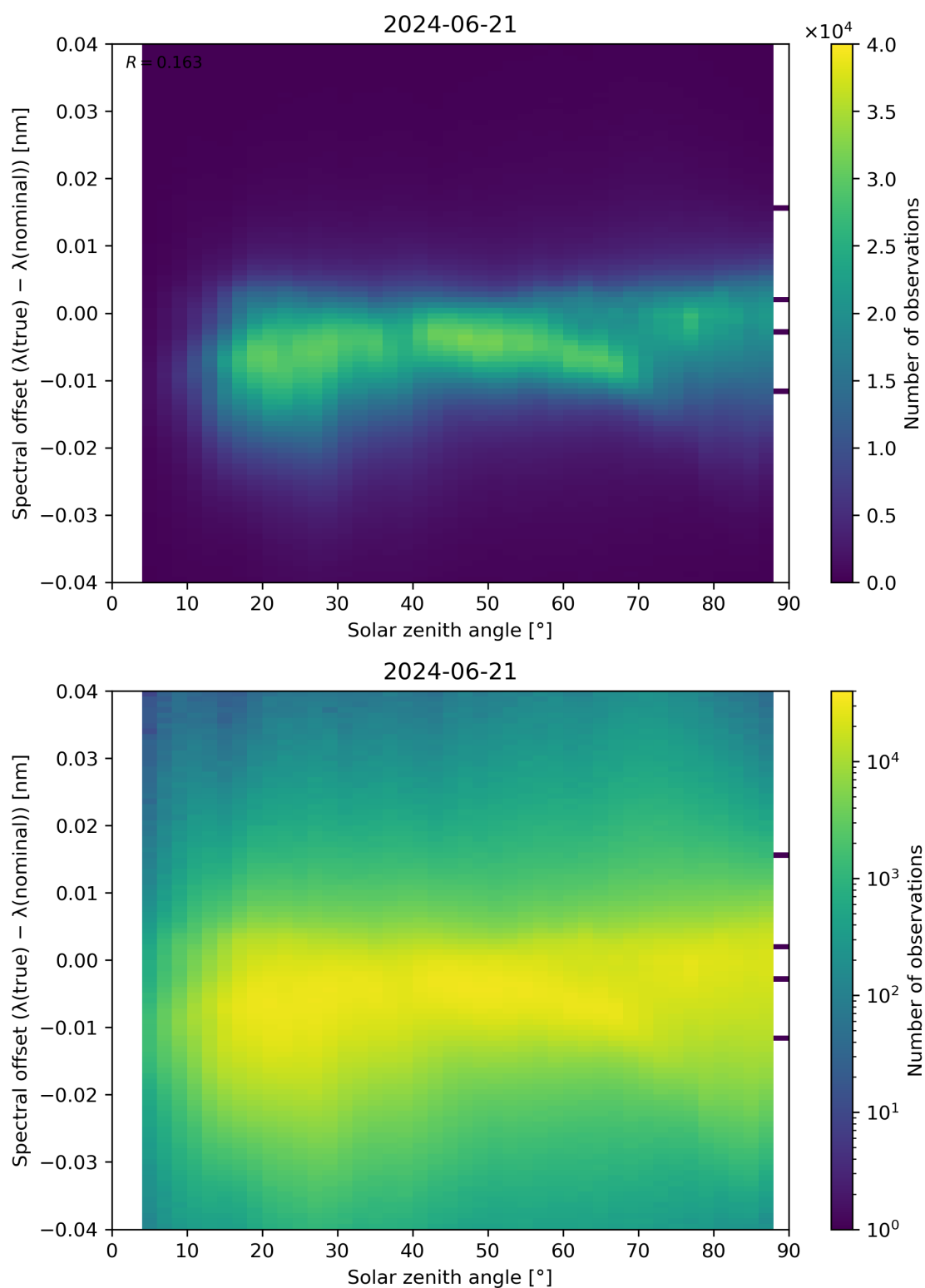
Figure 117: Scatter density plot of “Solar zenith angle” against “Spectral offset ( \lambda(\text{true}) - \lambda(\text{nominal}) )” for 2024-06-20 to 2024-06-22.
