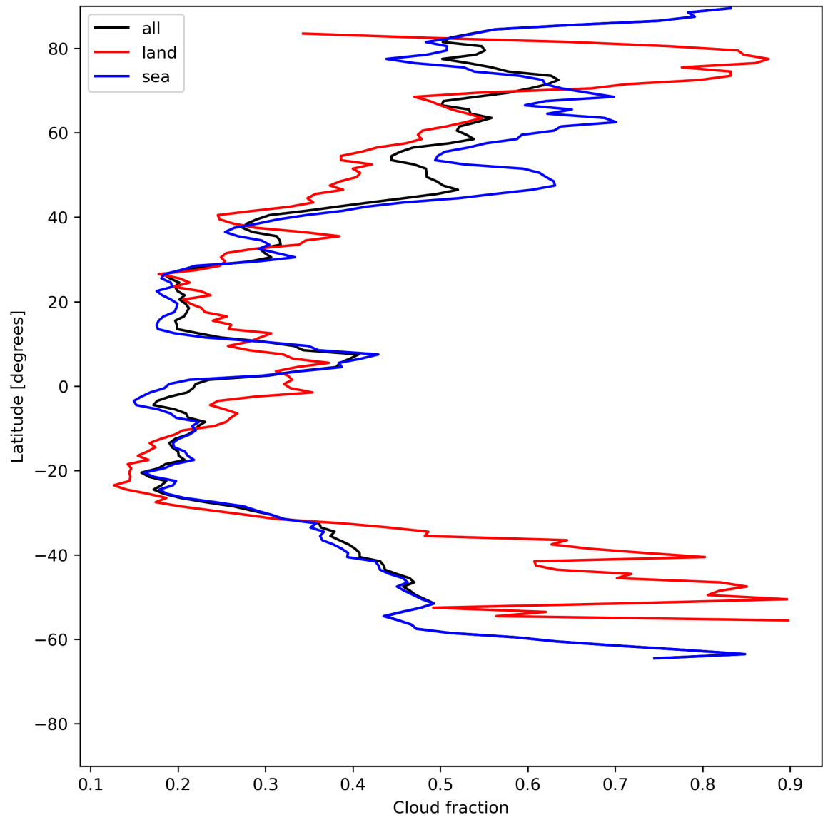
Figure 15: Zonal average of “Cloud fraction” for 2024-06-20 to 2024-06-22.
