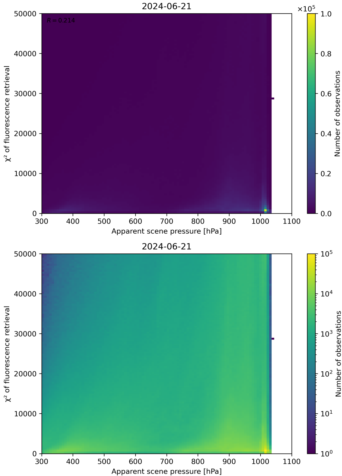
Figure 63: Scatter density plot of “Apparent scene pressure” against “ \chi^2 of fluorescence retrieval” for 2024-06-20 to 2024-06-22.
