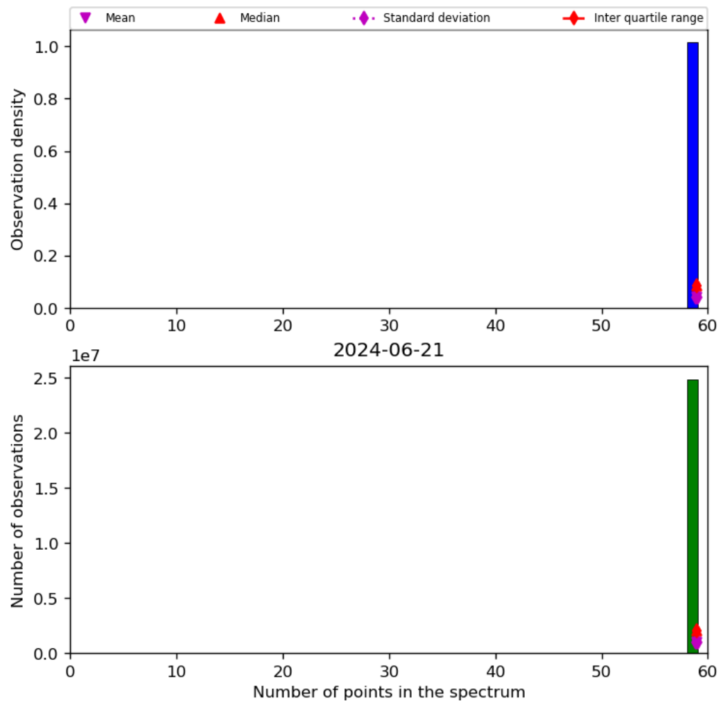
Figure 44: Histogram of “Number of points in the spectrum” for 2024-06-20 to 2024-06-22
