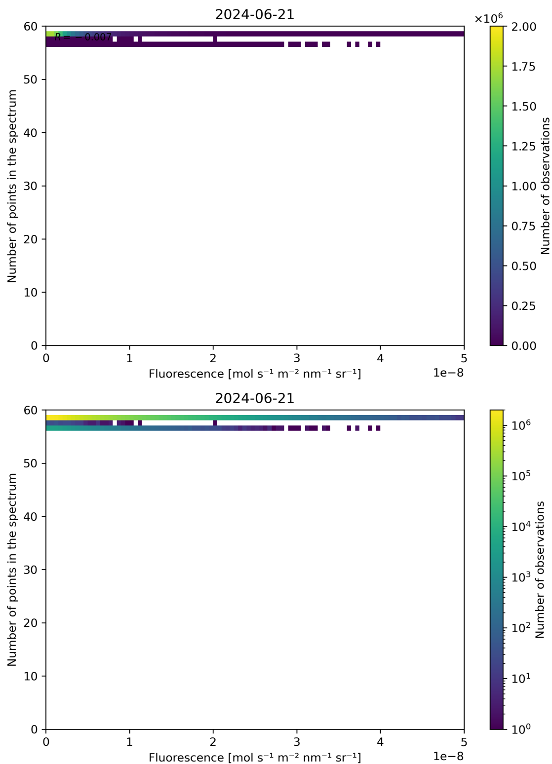
Figure 86: Scatter density plot of “Fluorescence” against “Number of points in the spectrum” for 2024-06-20 to 2024-06-22.
