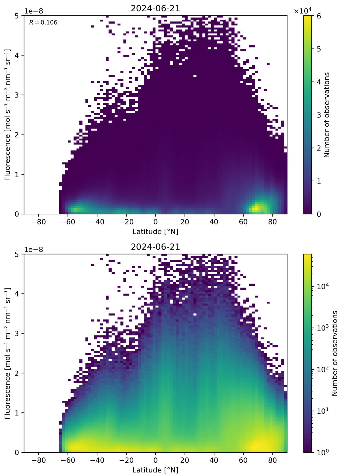
Figure 92: Scatter density plot of “Latitude” against “Fluorescence” for 2024-06-20 to 2024-06-22.
