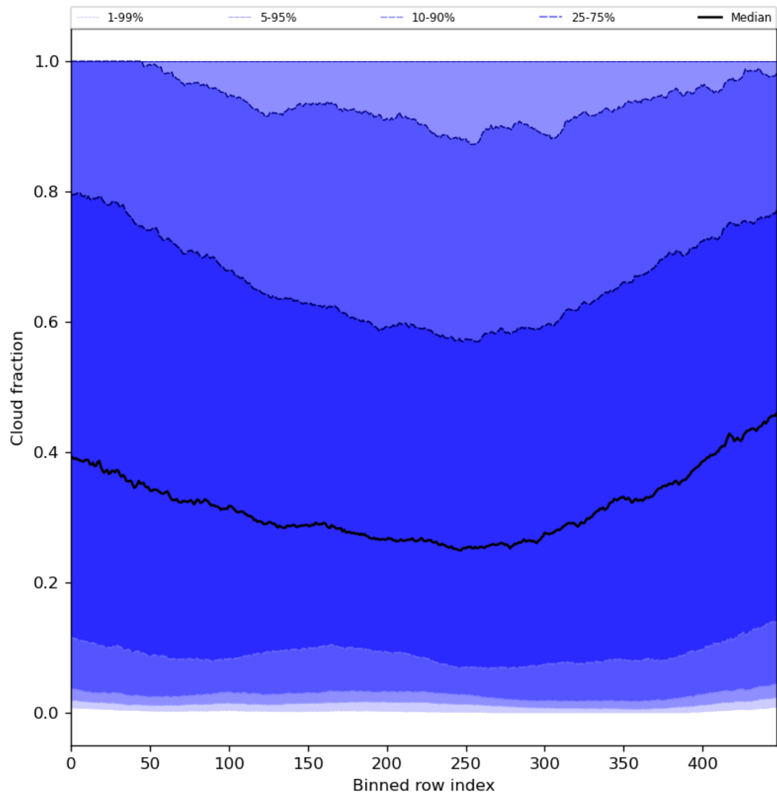
Figure 49: Along track statistics of “Cloud fraction” for 2024-06-20 to 2024-06-22
