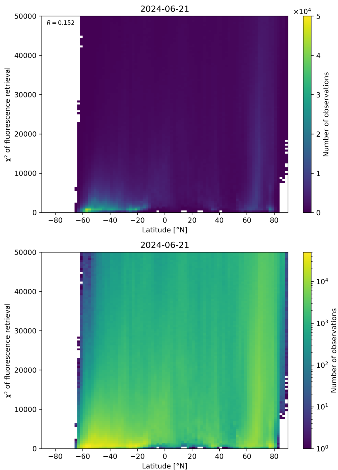
Figure 89: Scatter density plot of “Latitude” against “ \chi^2 of fluorescence retrieval” for 2024-06-20 to 2024-06-22.
