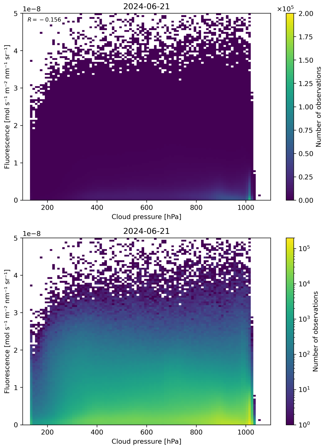
Figure 80: Scatter density plot of “Cloud pressure” against “Fluorescence” for 2024-06-20 to 2024-06-22.
