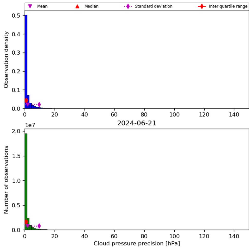
Figure 31: Histogram of “Cloud pressure precision” for 2024-06-20 to 2024-06-22
