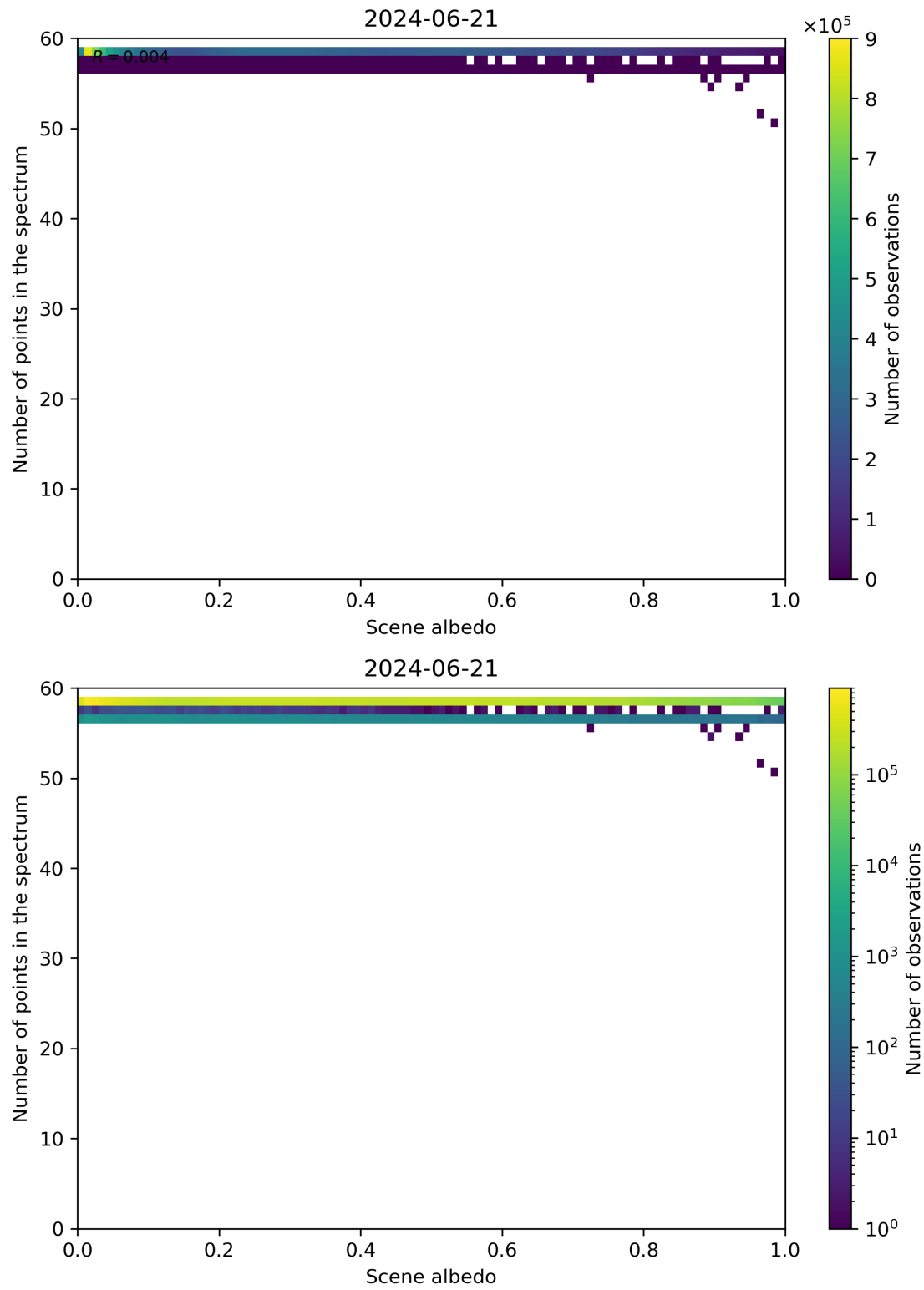
Figure 106: Scatter density plot of “Scene albedo” against “Number of points in the spectrum” for 2024-06-20 to 2024-06-22.
