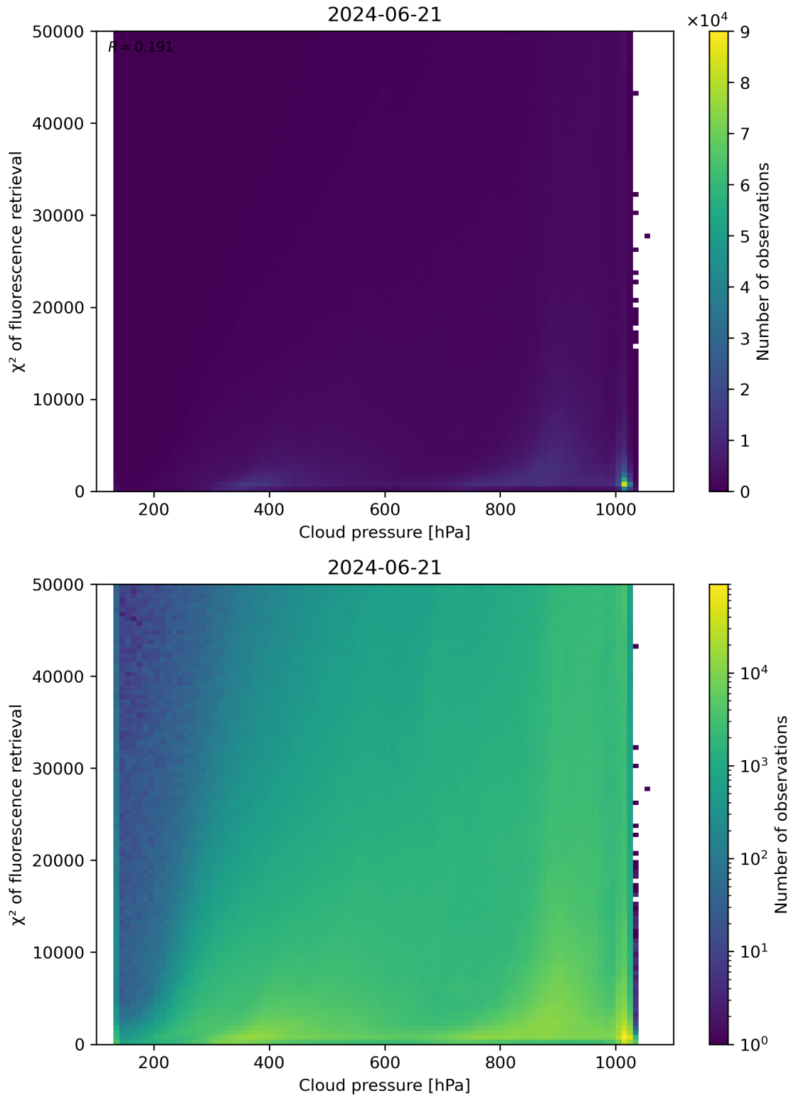
Figure 78: Scatter density plot of “Cloud pressure” against “ \chi^2 of fluorescence retrieval” for 2024-06-20 to 2024-06-22.
