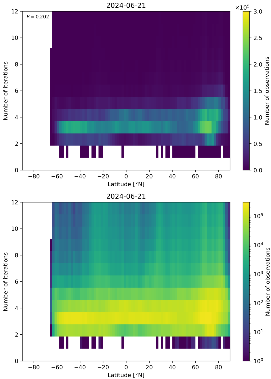
Figure 93: Scatter density plot of “Latitude” against “Number of iterations” for 2024-06-20 to 2024-06-22.
