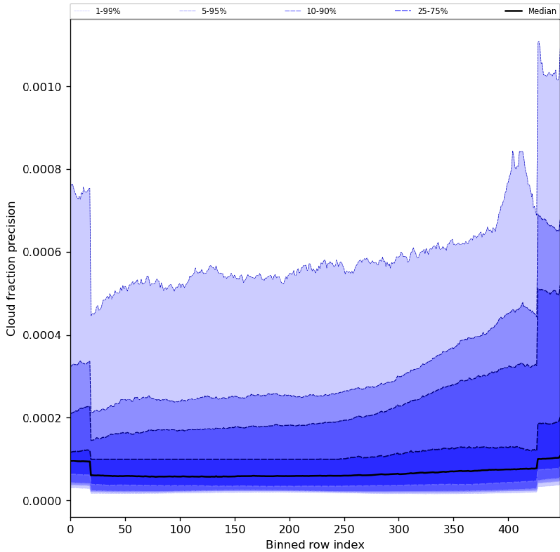
Figure 50: Along track statistics of “Cloud fraction precision” for 2024-06-20 to 2024-06-22
