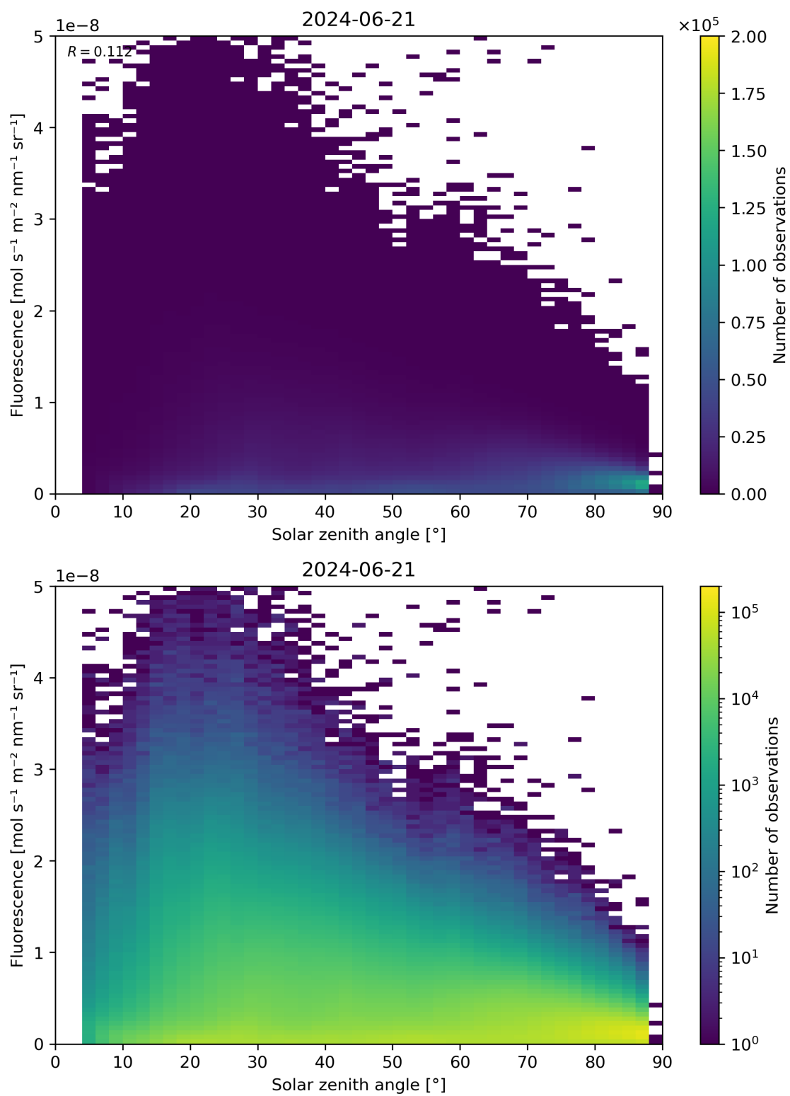
Figure 112: Scatter density plot of “Solar zenith angle” against “Fluorescence” for 2024-06-20 to 2024-06-22.
