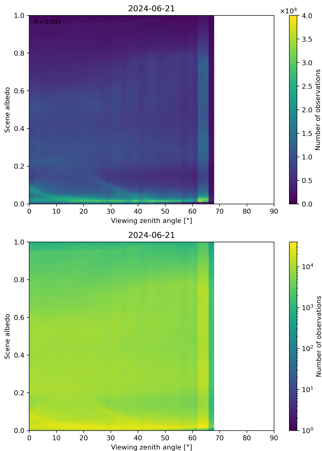
Figure 126: Scatter density plot of “Viewing zenith angle” against “Scene albedo” for 2024-06-20 to 2024-06-22.
