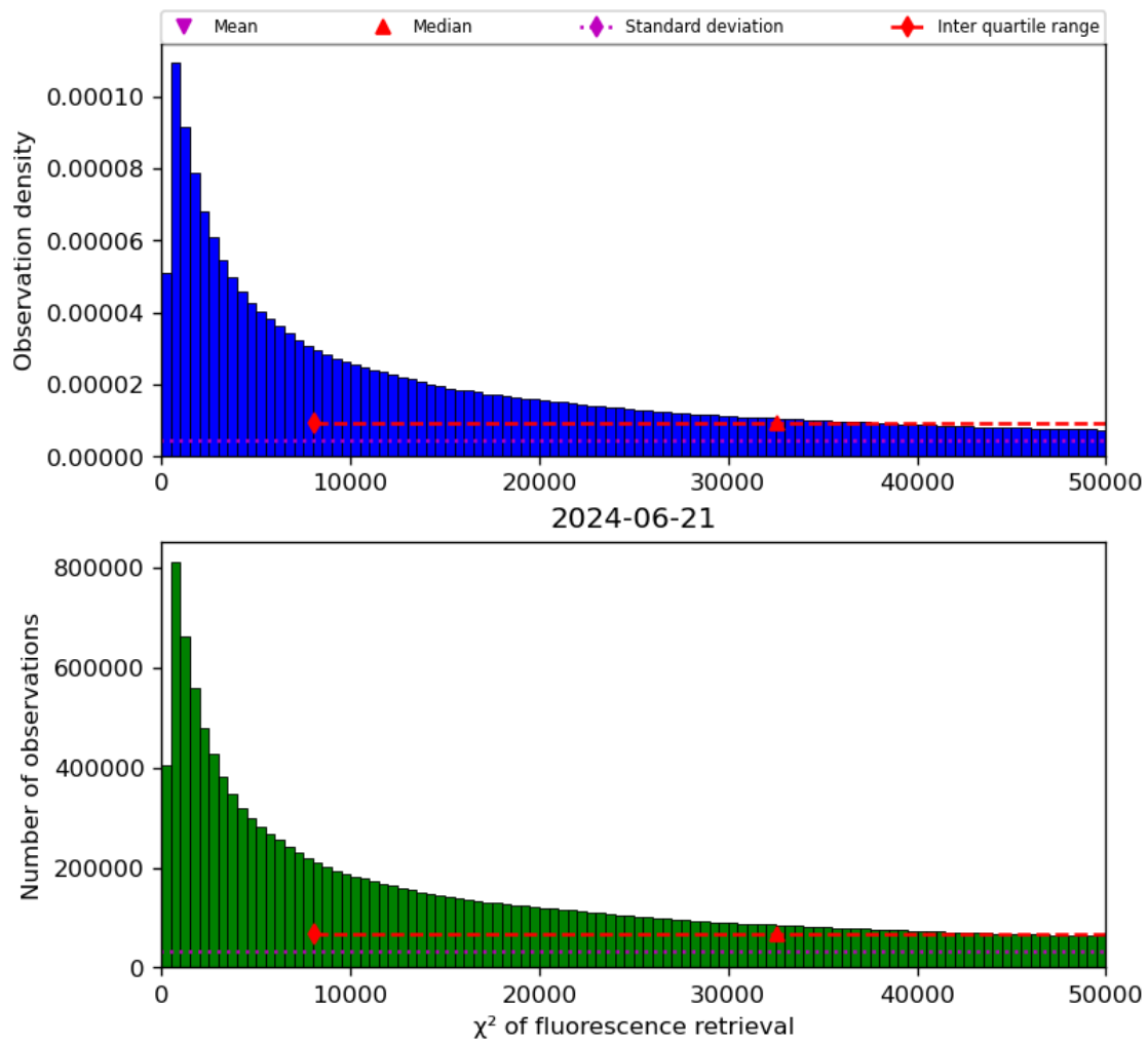
Figure 42: Histogram of “ \chi^2 of fluorescence retrieval” for 2024-06-20 to 2024-06-22
