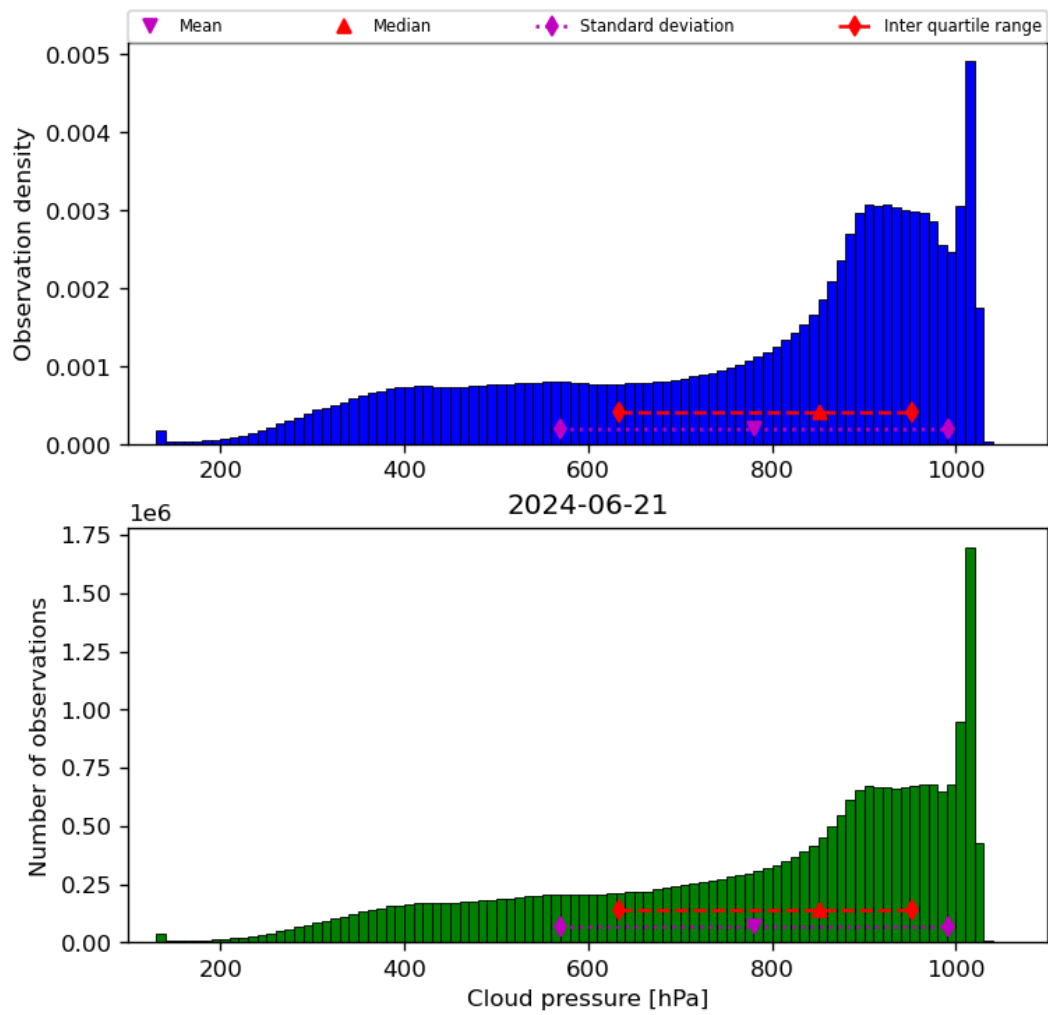
Figure 30: Histogram of “Cloud pressure” for 2024-06-20 to 2024-06-22
