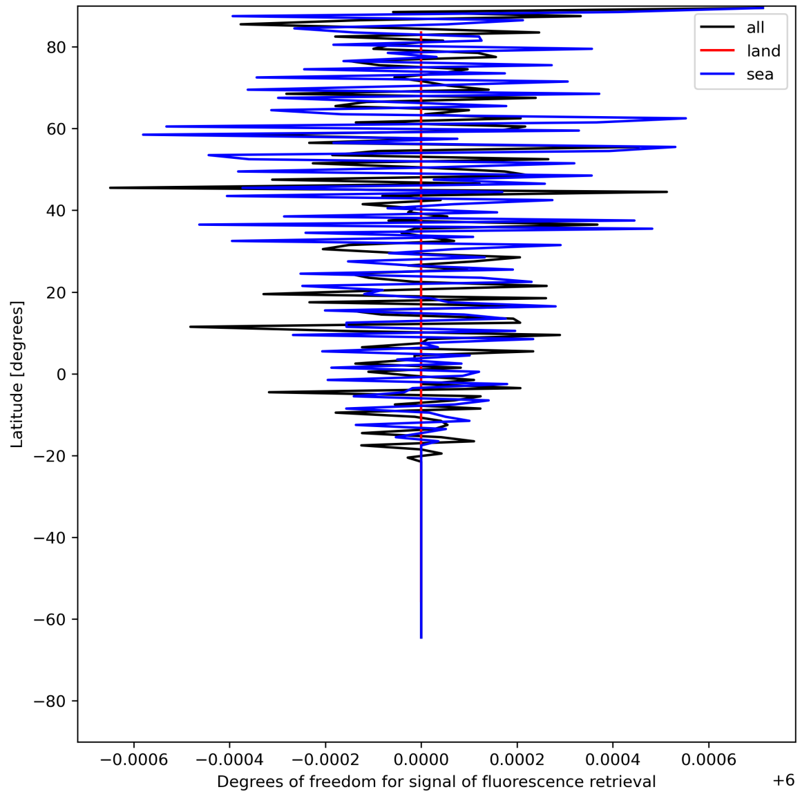
Figure 26: Zonal average of “Degrees of freedom for signal of fluorescence retrieval” for 2024-06-20 to 2024-06-22.
