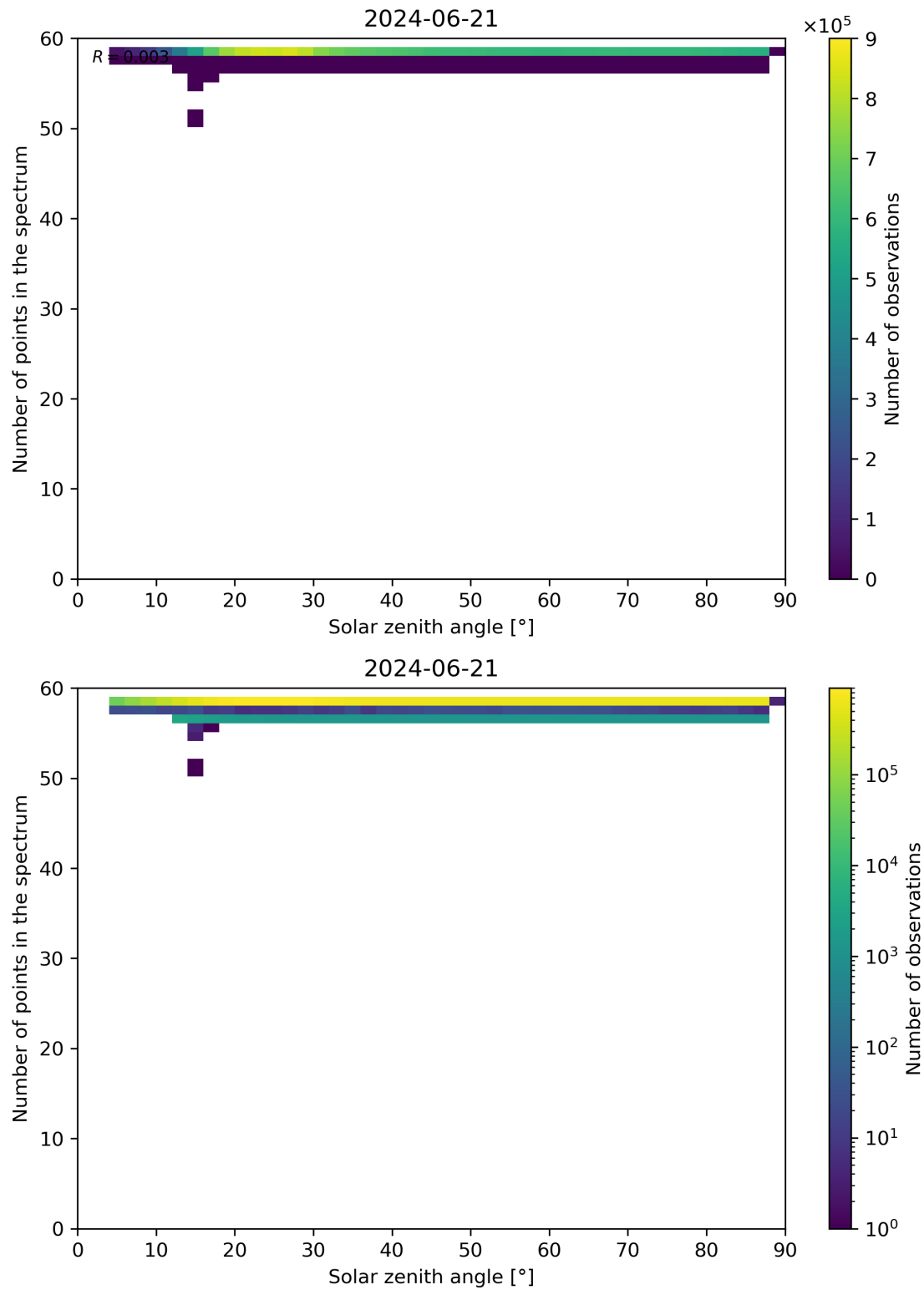
Figure 115: Scatter density plot of “Solar zenith angle” against “Number of points in the spectrum” for 2024-06-20 to 2024-06-22.
