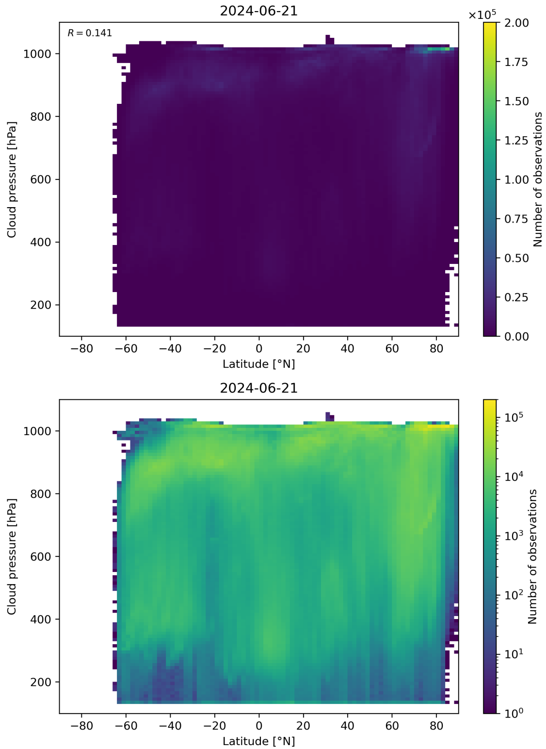
Figure 91: Scatter density plot of “Latitude” against “Cloud pressure” for 2024-06-20 to 2024-06-22.
