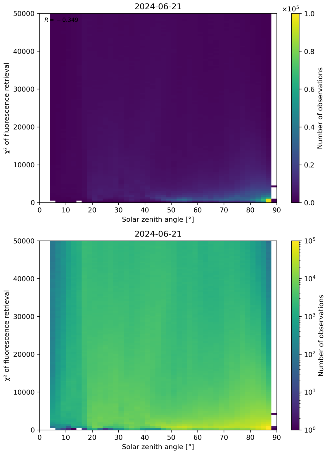
Figure 109: Scatter density plot of “Solar zenith angle” against “ \chi^2 of fluorescence retrieval” for 2024-06-20 to 2024-06-22.
