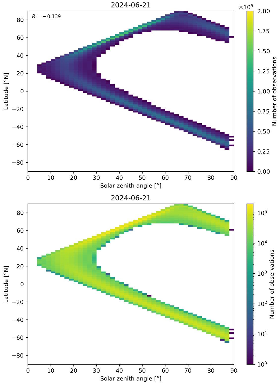
Figure 113: Scatter density plot of “Solar zenith angle” against “Latitude” for 2024-06-20 to 2024-06-22.
