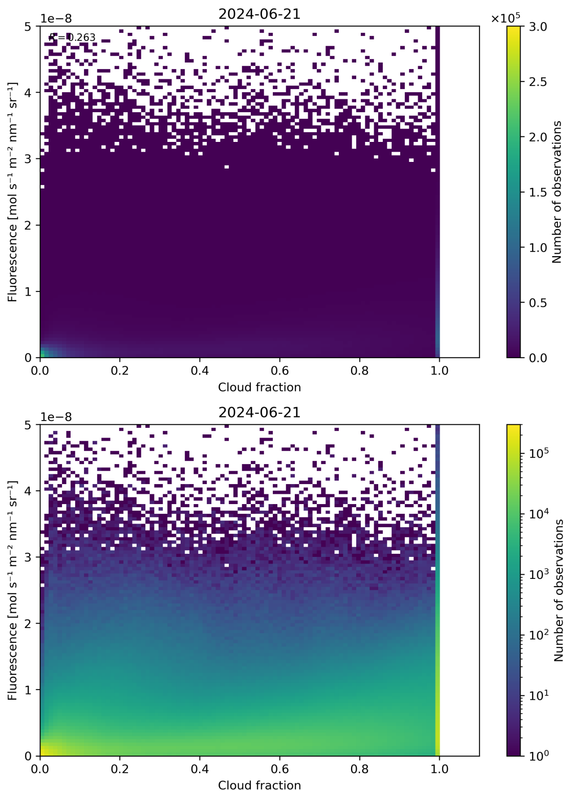
Figure 72: Scatter density plot of “Cloud fraction” against “Fluorescence” for 2024-06-20 to 2024-06-22.
