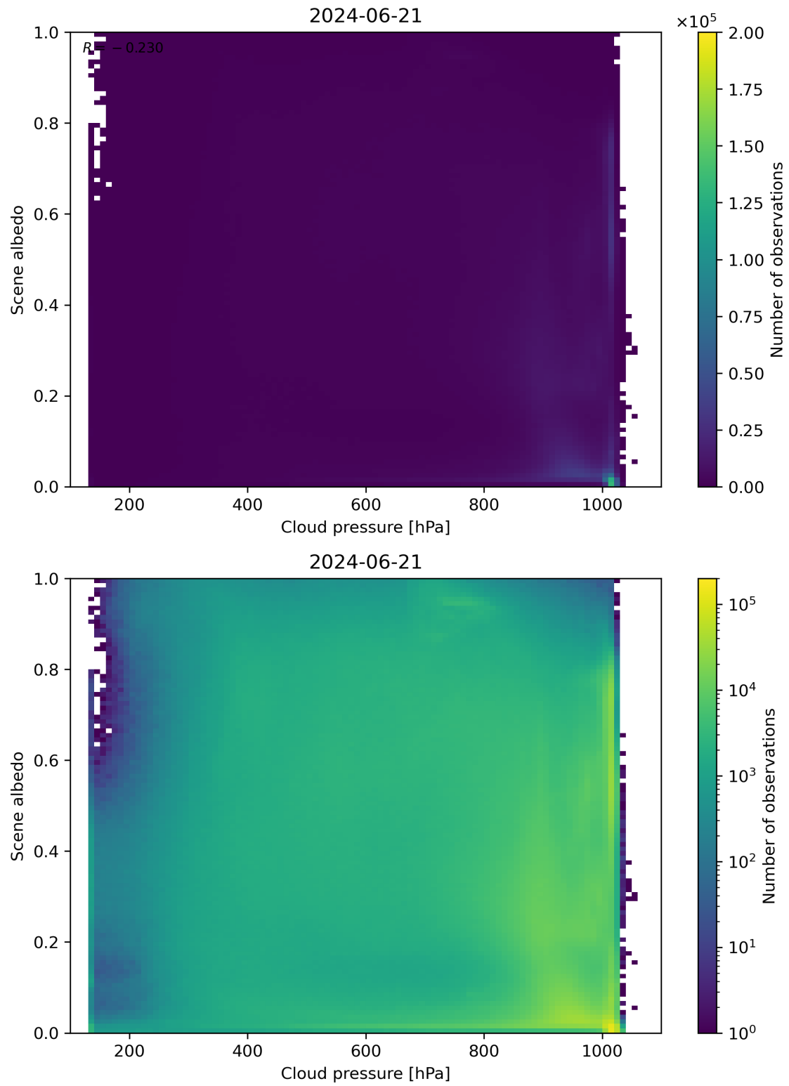
Figure 83: Scatter density plot of “Cloud pressure” against “Scene albedo” for 2024-06-20 to 2024-06-22.
