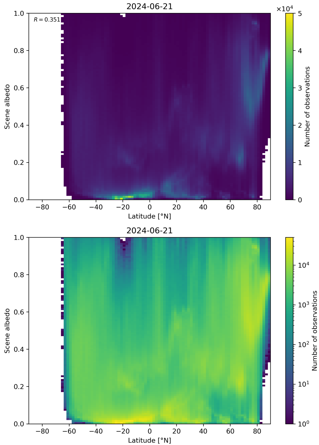
Figure 95: Scatter density plot of “Latitude” against “Scene albedo” for 2024-06-20 to 2024-06-22.
