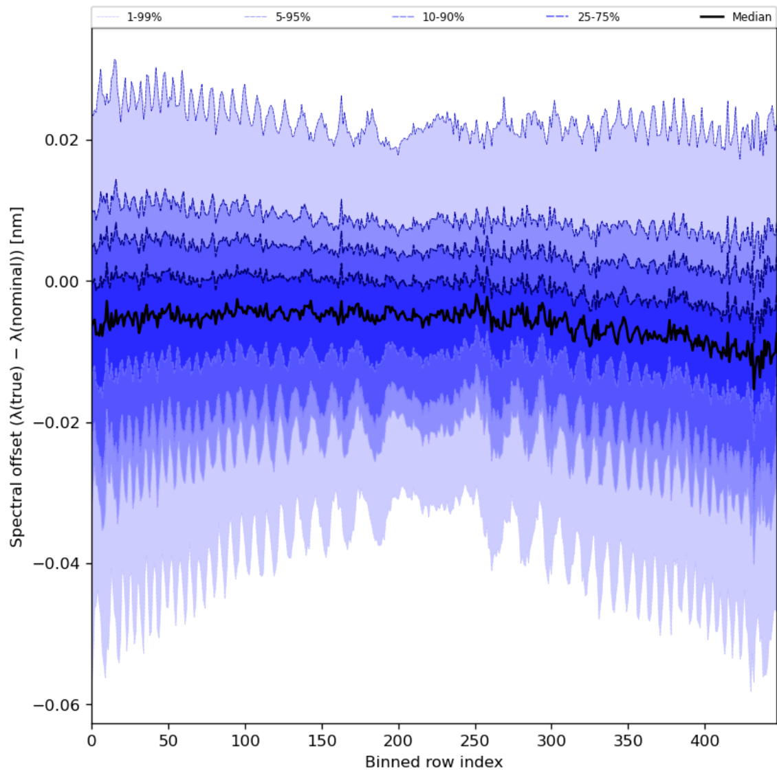
Figure 62: Along track statistics of “Spectral offset ( \lambda(\text{true}) - \lambda(\text{nominal}) )” for 2024-06-20 to 2024-06-22
