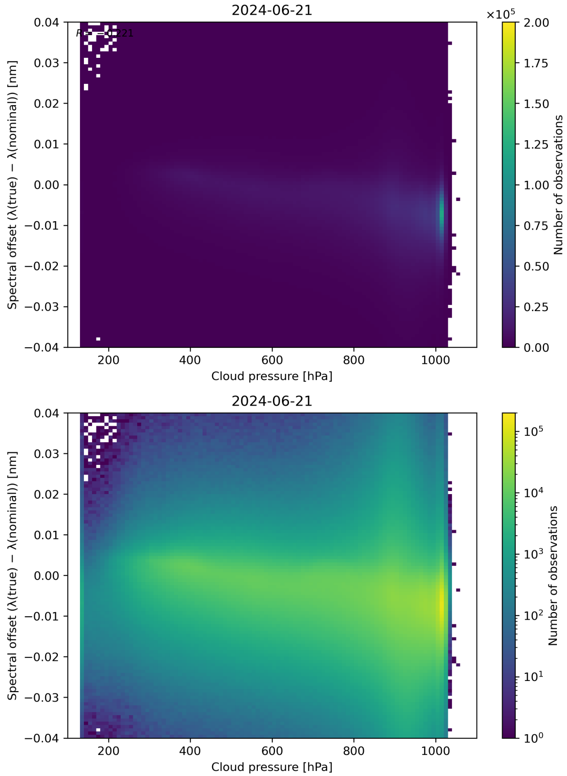
Figure 84: Scatter density plot of “Cloud pressure” against “Spectral offset ( \lambda(\text{true}) - \lambda(\text{nominal}) )” for 2024-06-20 to 2024-06-22.
