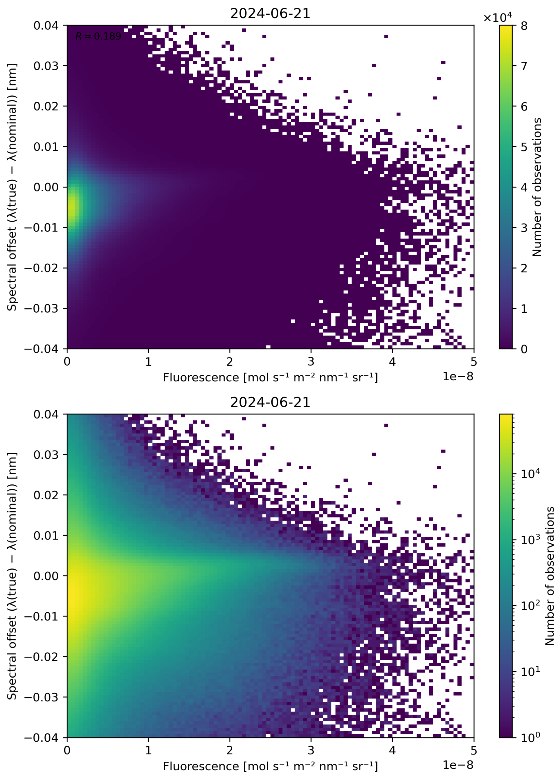
Figure 87: Scatter density plot of “Fluorescence” against “Spectral offset ( \lambda(\text{true}) - \lambda(\text{nominal}) )” for 2024-06-20 to 2024-06-22.
