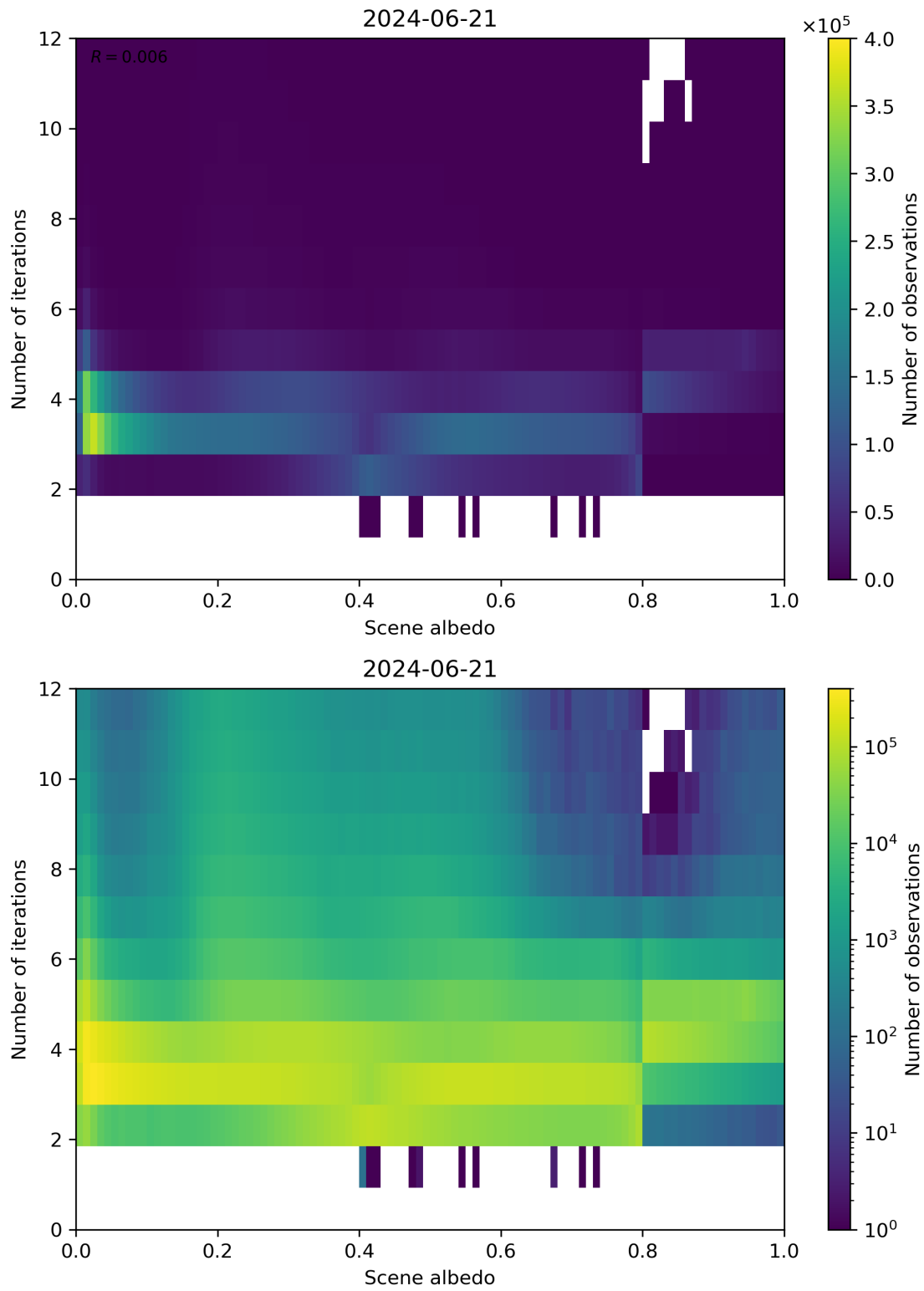
Figure 105: Scatter density plot of “Scene albedo” against “Number of iterations” for 2024-06-20 to 2024-06-22.
