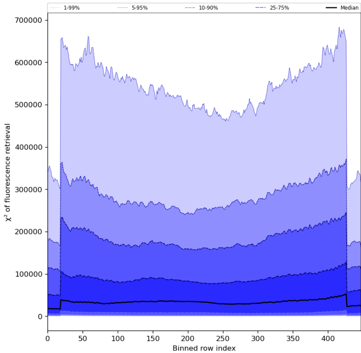
Figure 59: Along track statistics of “ \chi^2 of fluorescence retrieval” for 2024-06-20 to 2024-06-22
