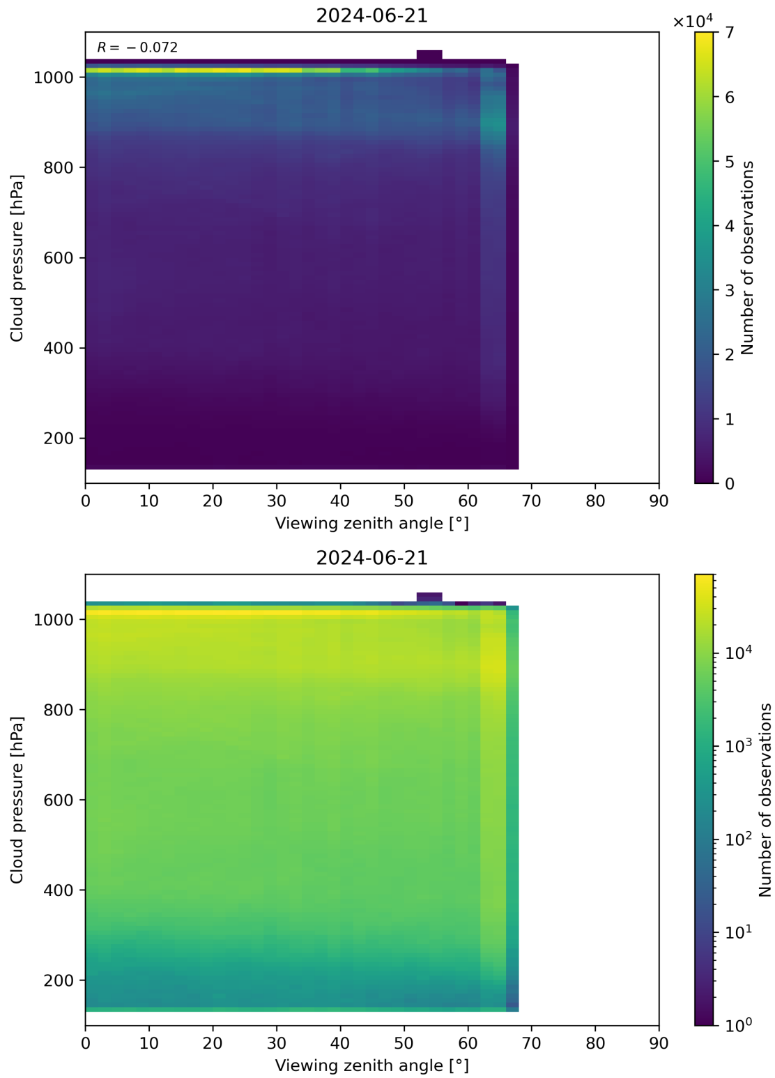
Figure 121: Scatter density plot of “Viewing zenith angle” against “Cloud pressure” for 2024-06-20 to 2024-06-22.
