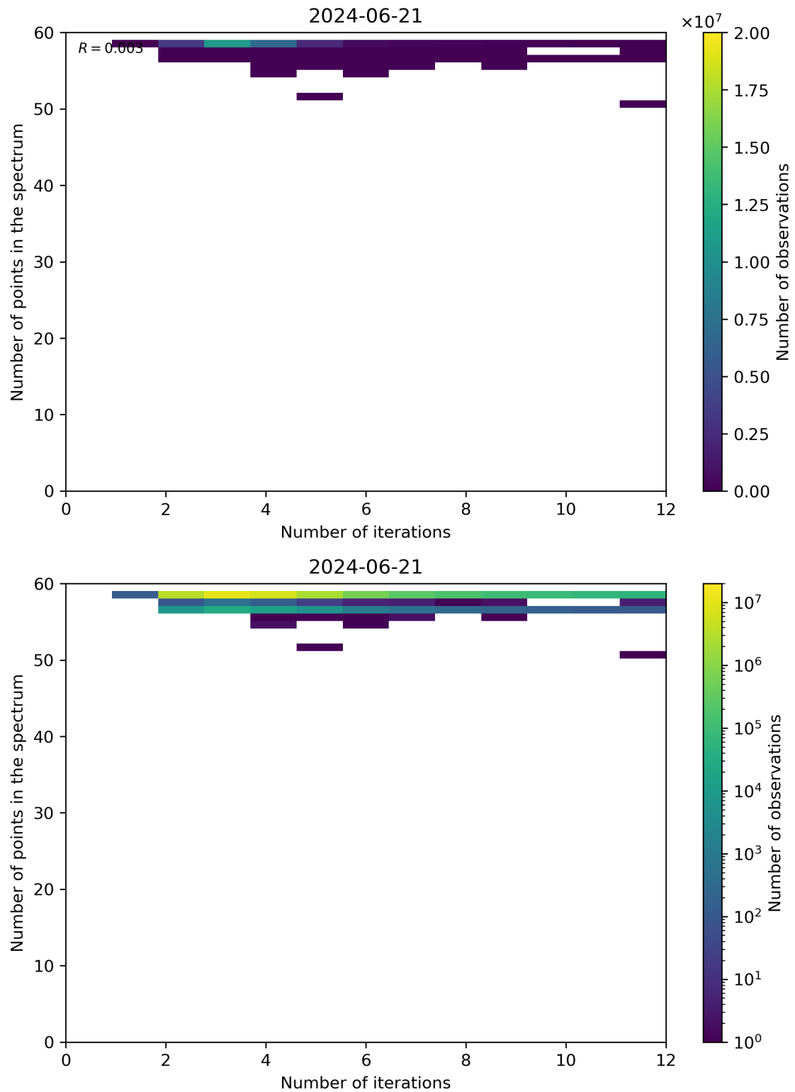
Figure 99: Scatter density plot of “Number of iterations” against “Number of points in the spectrum” for 2024-06-20 to 2024-06-22.
