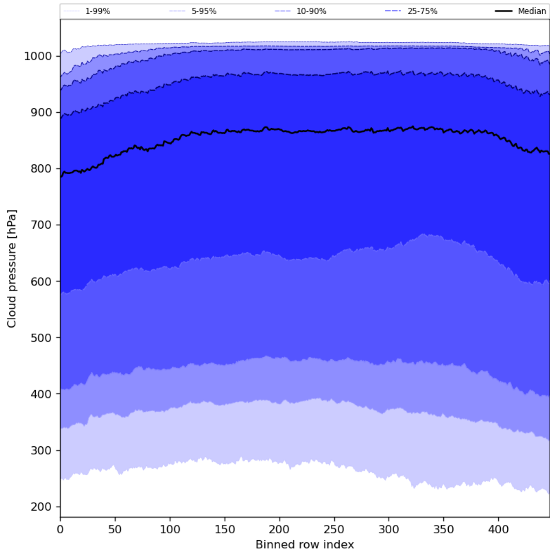
Figure 47: Along track statistics of “Cloud pressure” for 2024-06-20 to 2024-06-22
