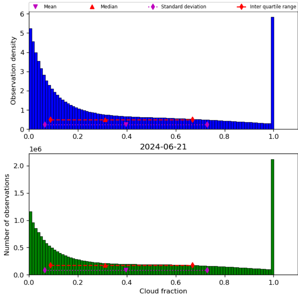
Figure 32: Histogram of “Cloud fraction” for 2024-06-20 to 2024-06-22
