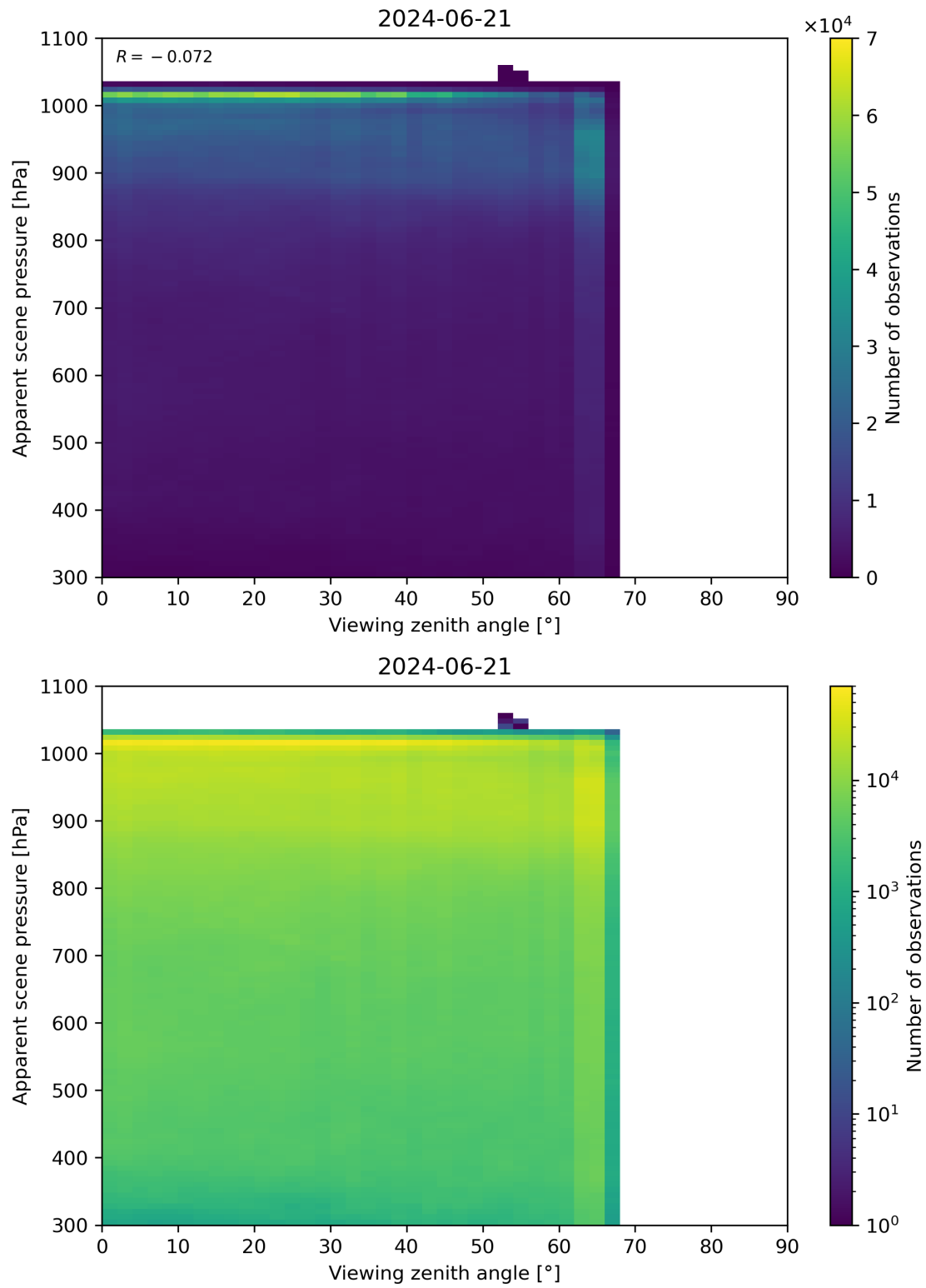
Figure 118: Scatter density plot of “Viewing zenith angle” against “Apparent scene pressure” for 2024-06-20 to 2024-06-22.
