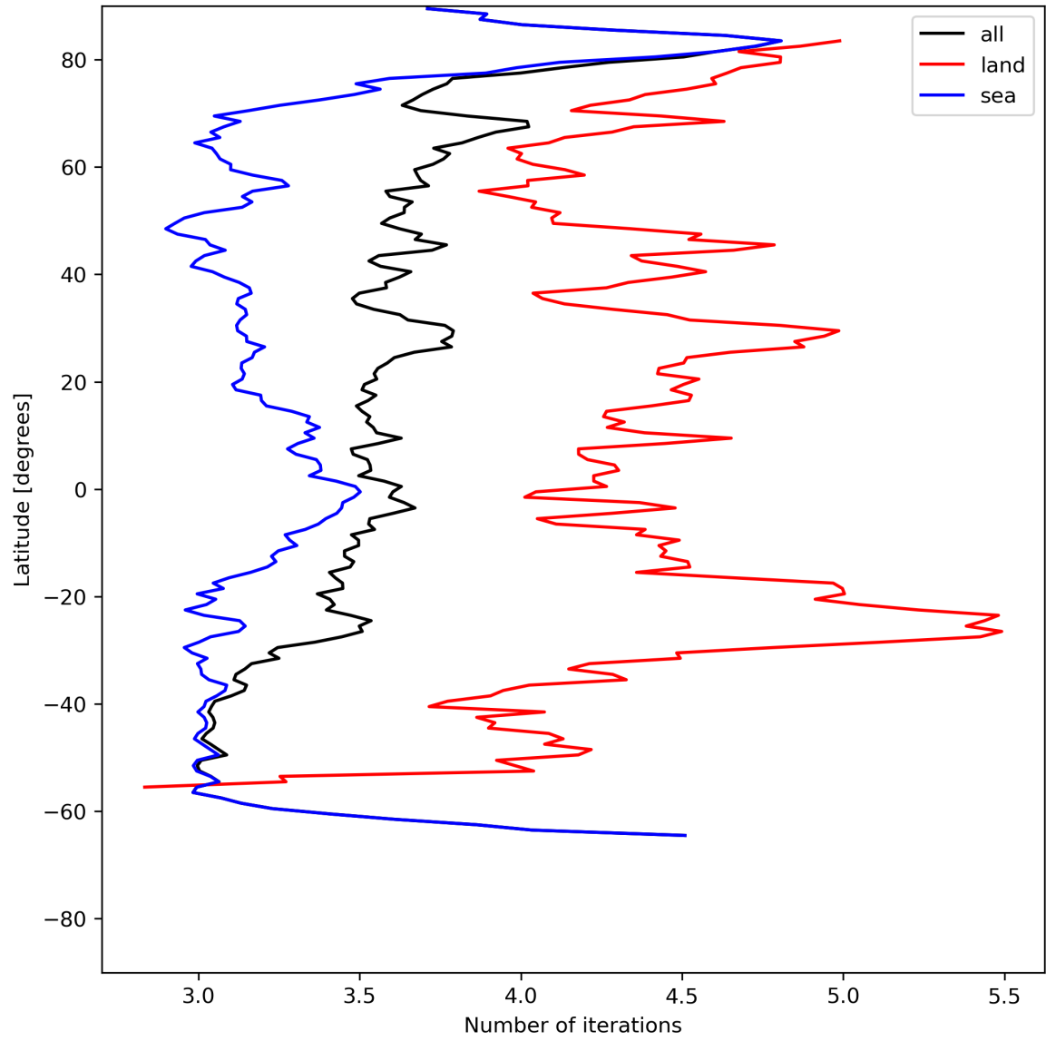
Figure 22: Zonal average of “Number of iterations” for 2024-06-20 to 2024-06-22.
