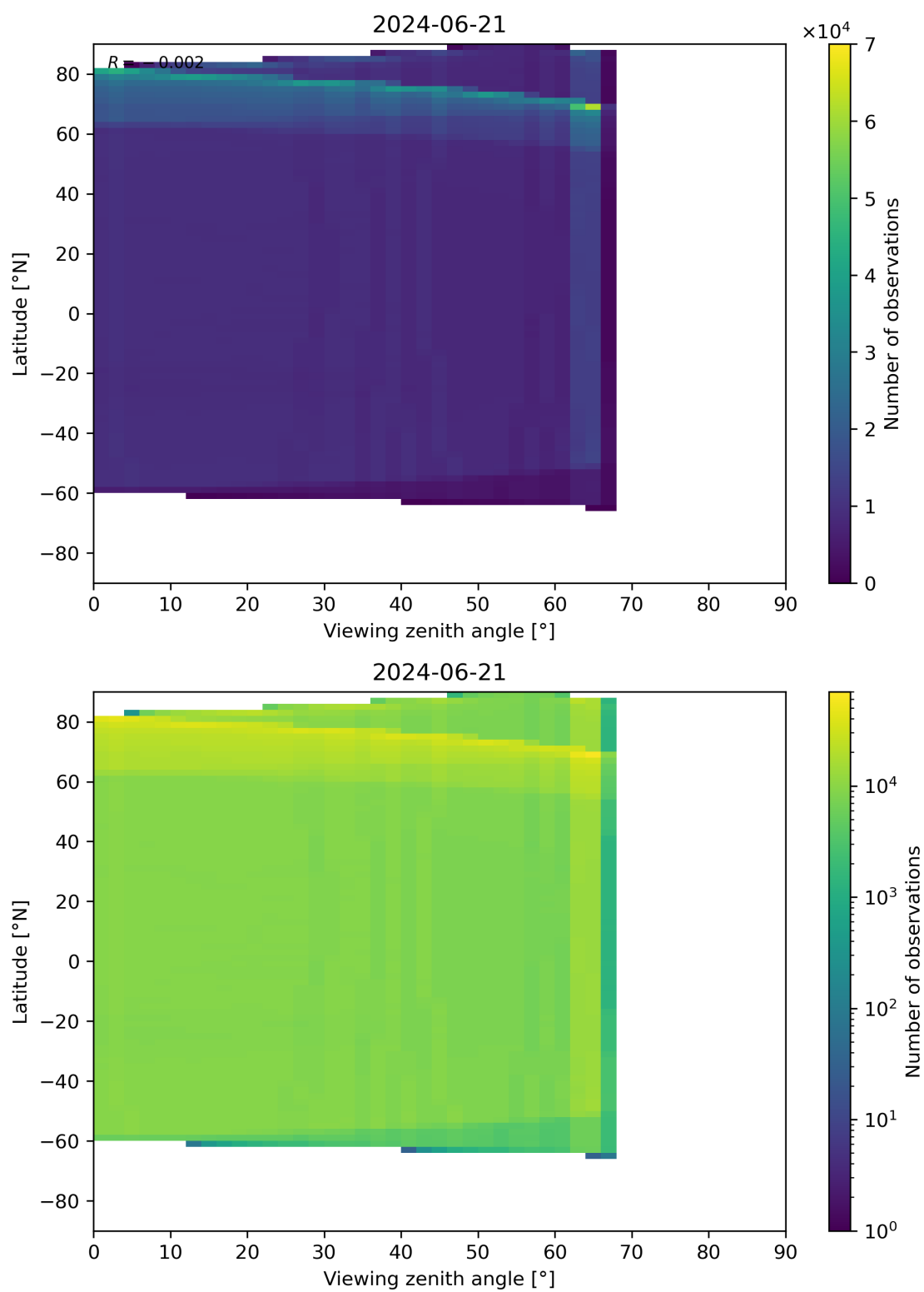
Figure 123: Scatter density plot of “Viewing zenith angle” against “Latitude” for 2024-06-20 to 2024-06-22.
