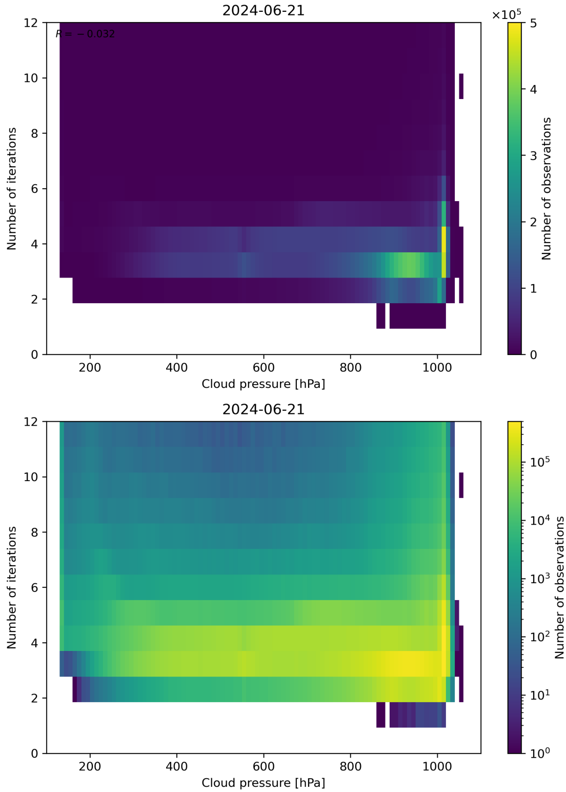
Figure 81: Scatter density plot of “Cloud pressure” against “Number of iterations” for 2024-06-20 to 2024-06-22.
