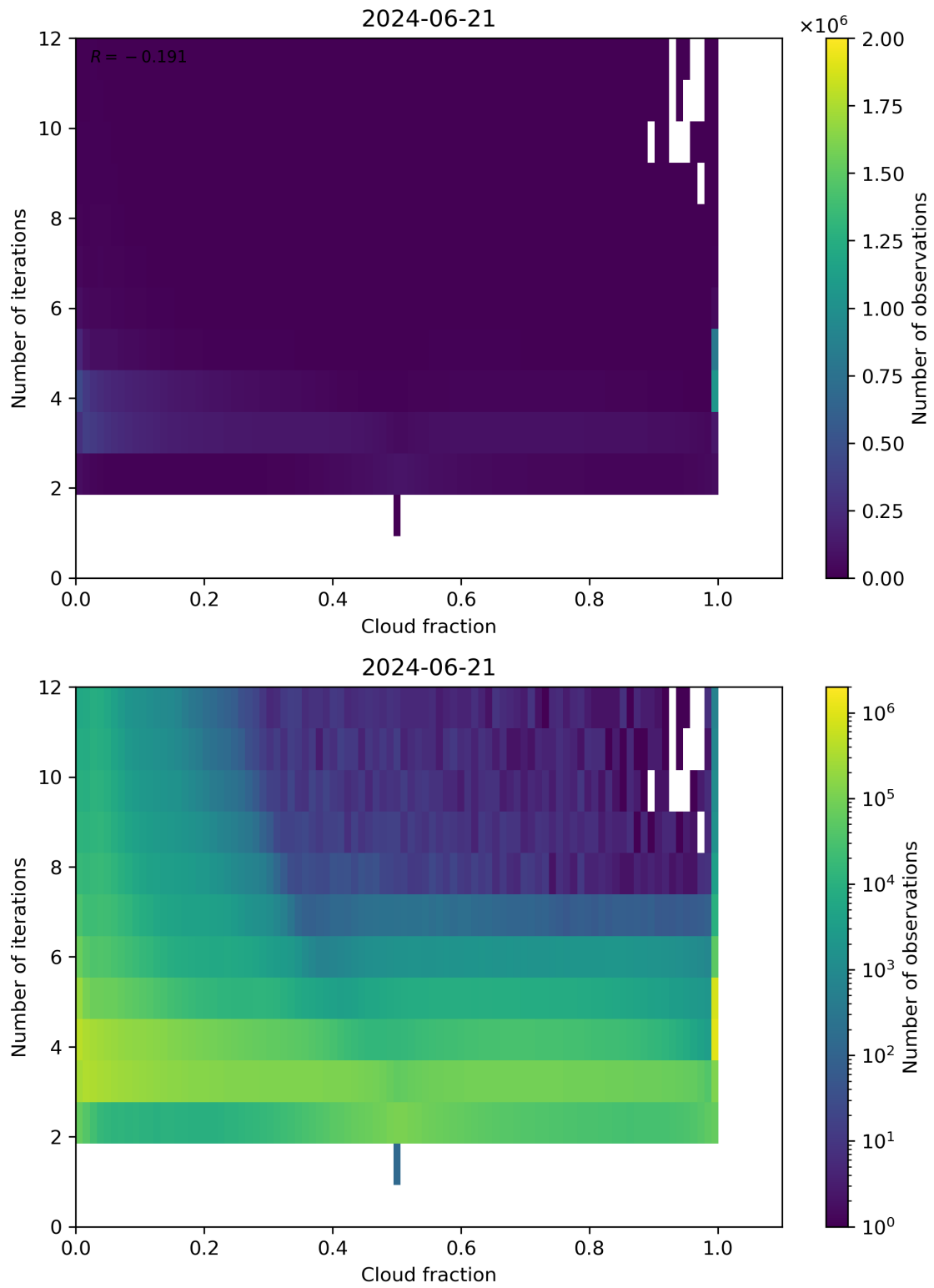
Figure 73: Scatter density plot of “Cloud fraction” against “Number of iterations” for 2024-06-20 to 2024-06-22.
