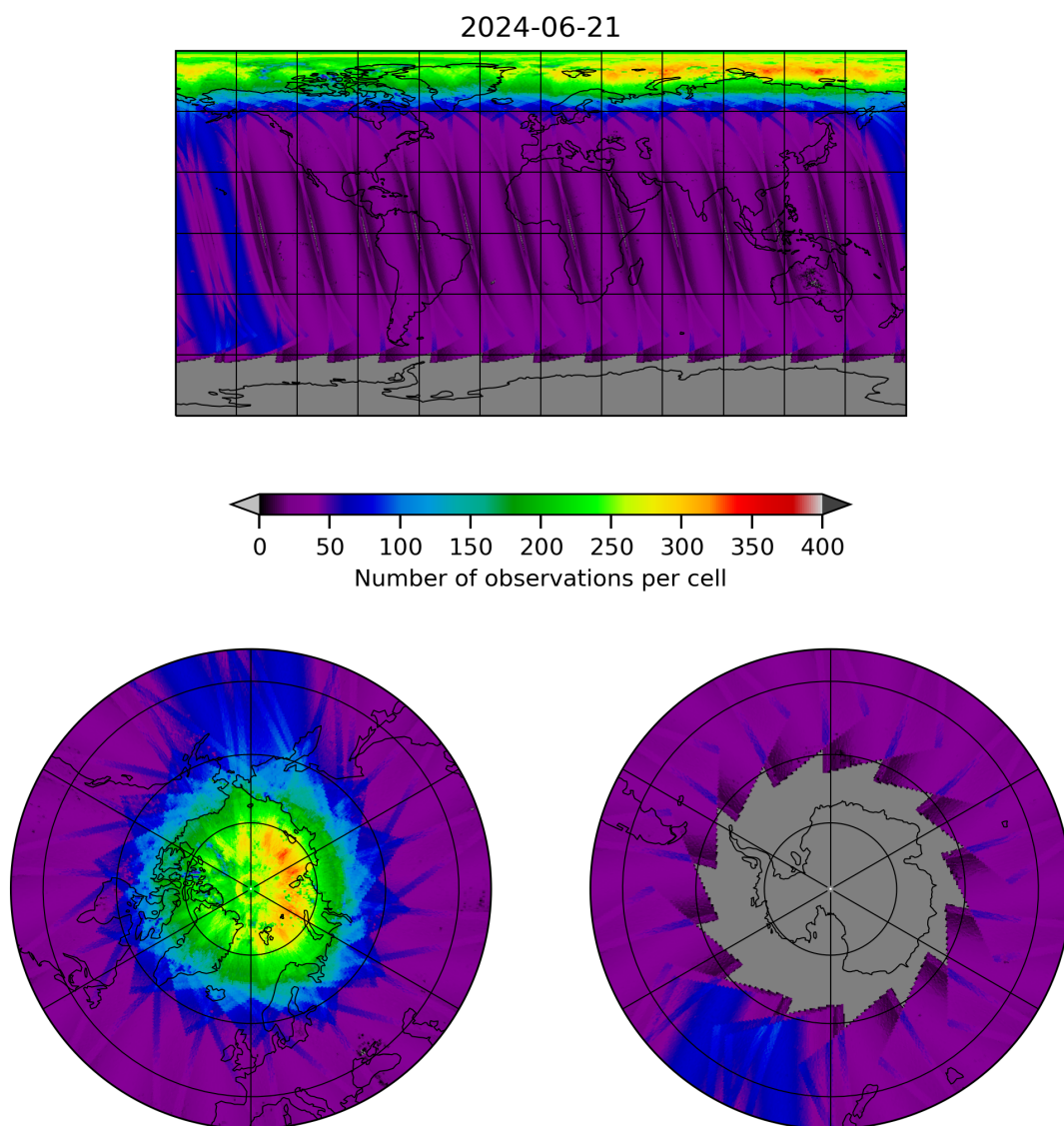
Figure 11: Map of the number of observations for 2024-06-20 to 2024-06-22
