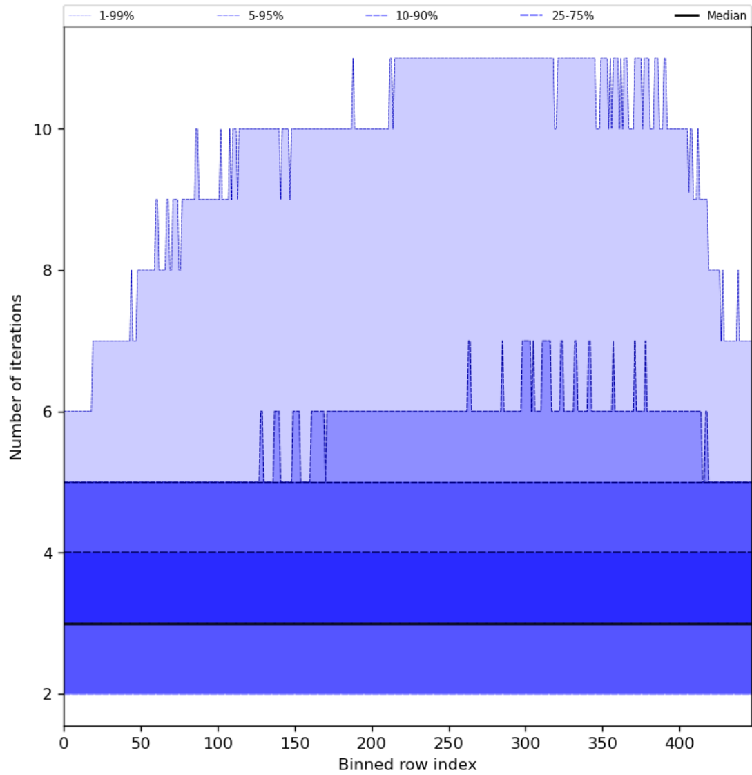
Figure 56: Along track statistics of “Number of iterations” for 2024-06-20 to 2024-06-22
