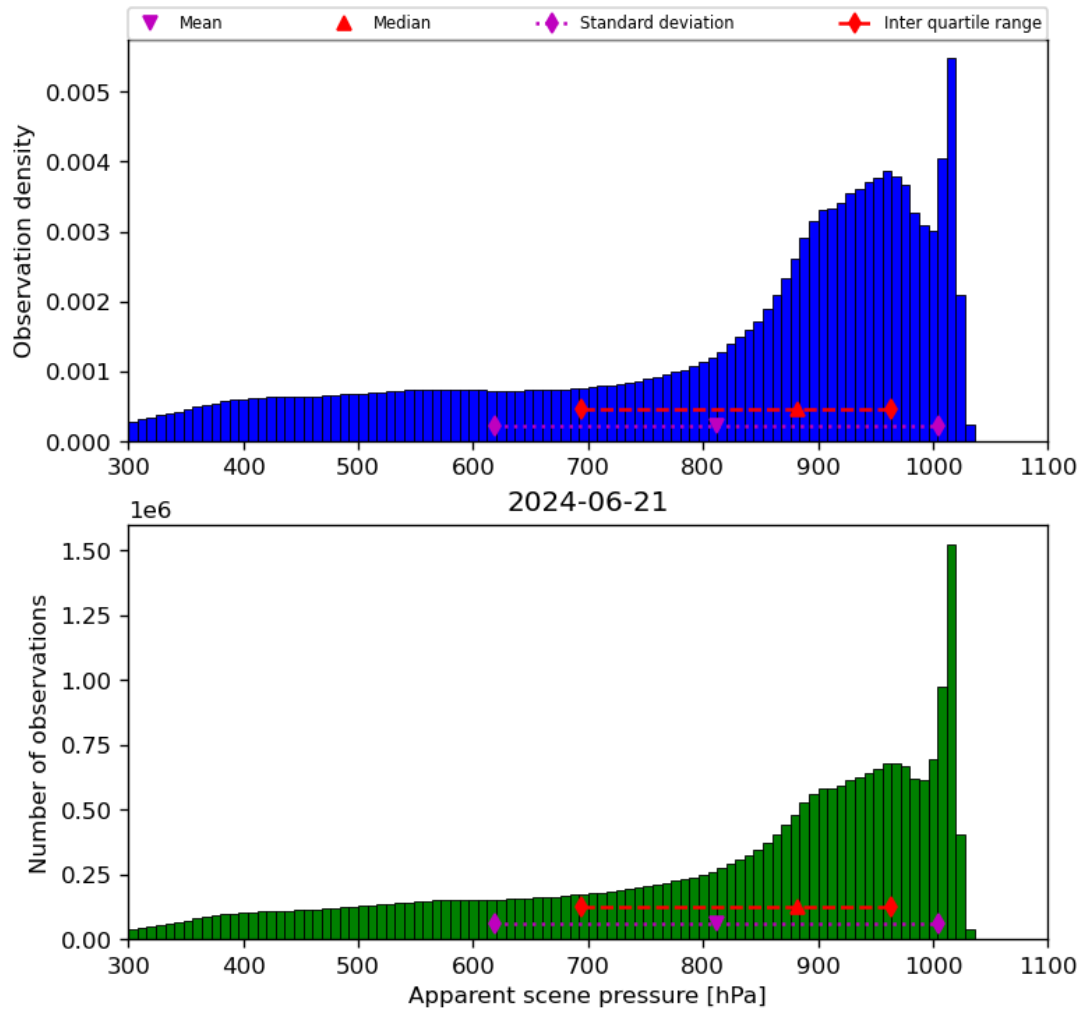
Figure 36: Histogram of “Apparent scene pressure” for 2024-06-20 to 2024-06-22
