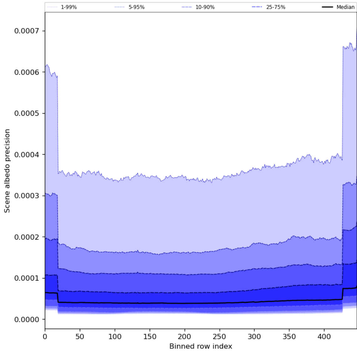
Figure 52: Along track statistics of “Scene albedo precision” for 2024-06-20 to 2024-06-22
