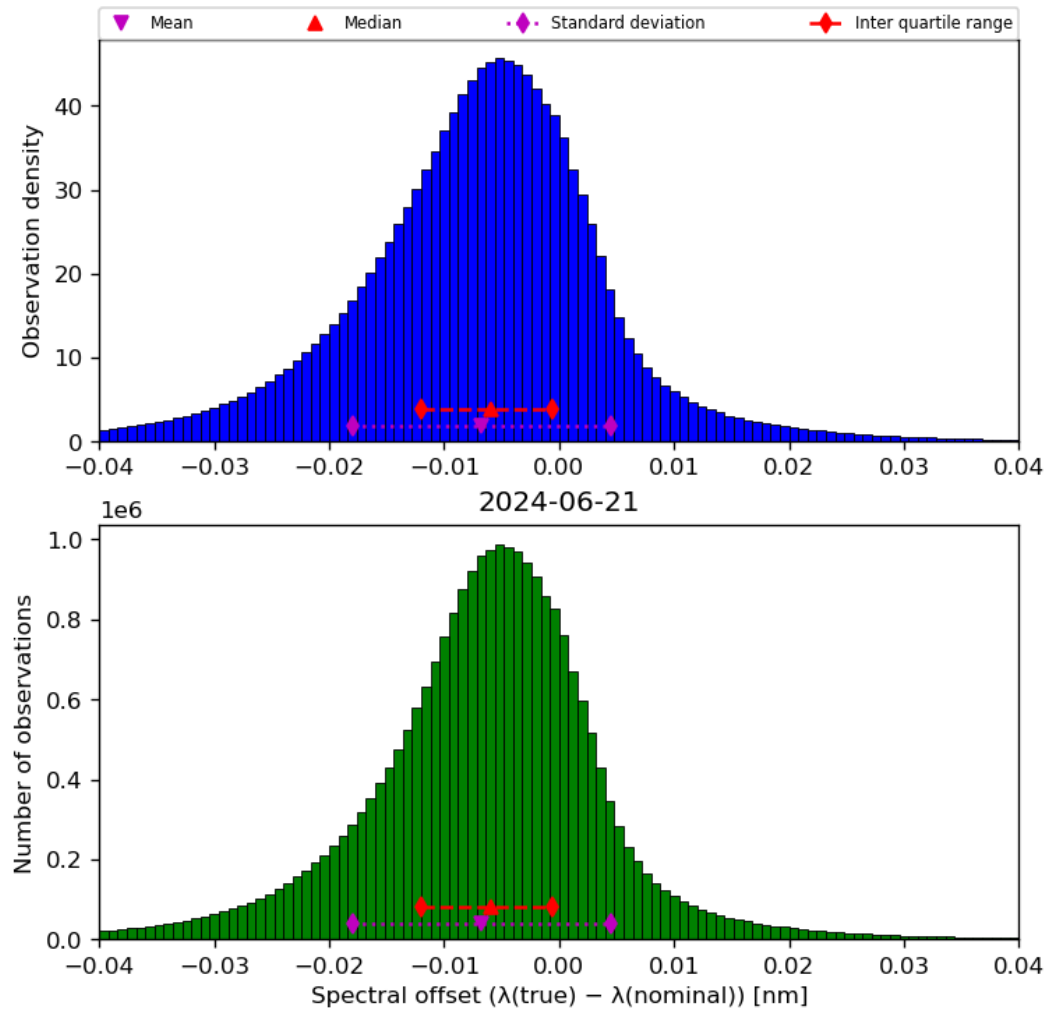
Figure 45: Histogram of “Spectral offset ( \lambda(\text{true}) - \lambda(\text{nominal}) )” for 2024-06-20 to 2024-06-22
