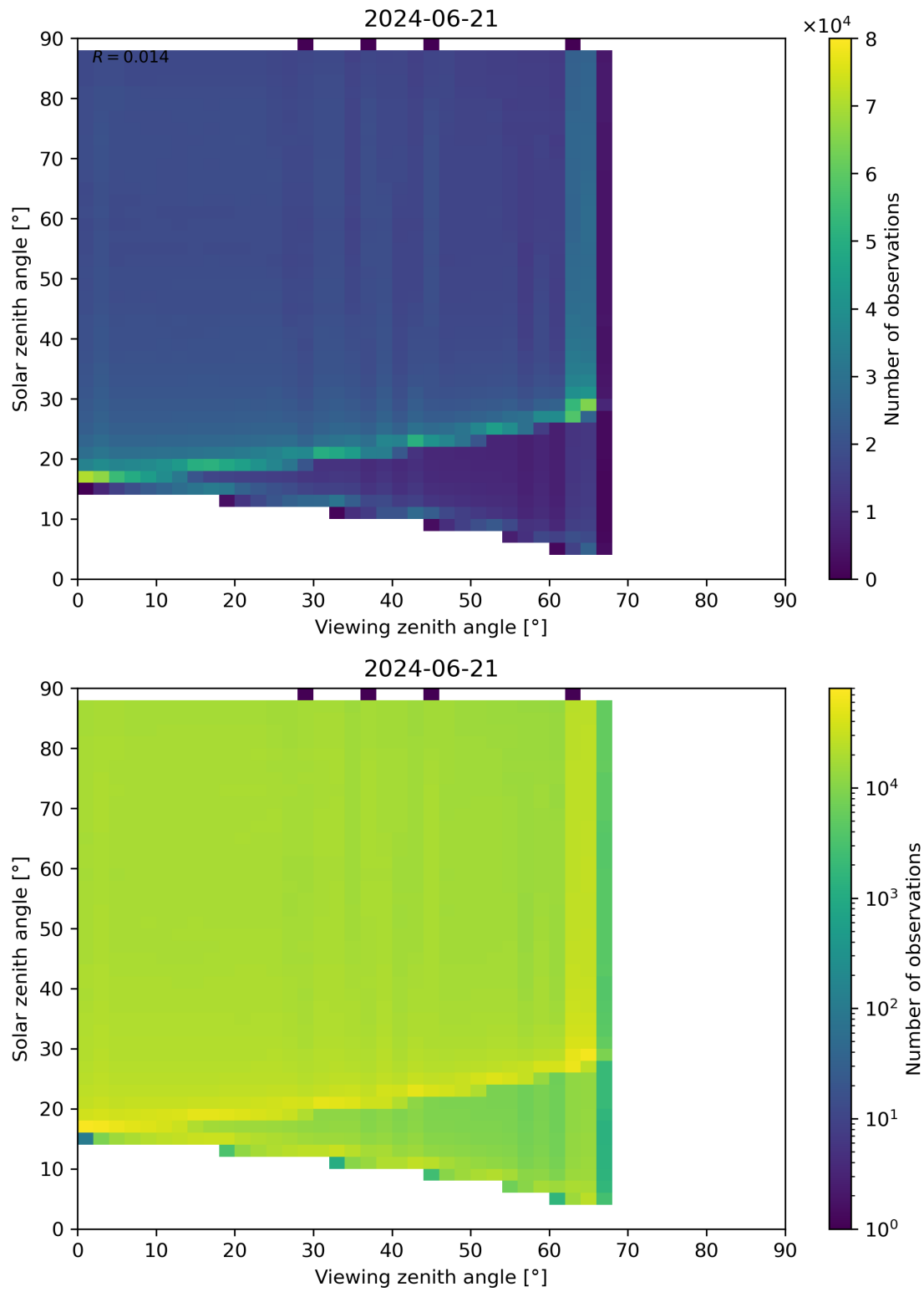
Figure 127: Scatter density plot of “Viewing zenith angle” against “Solar zenith angle” for 2024-06-20 to 2024-06-22.
