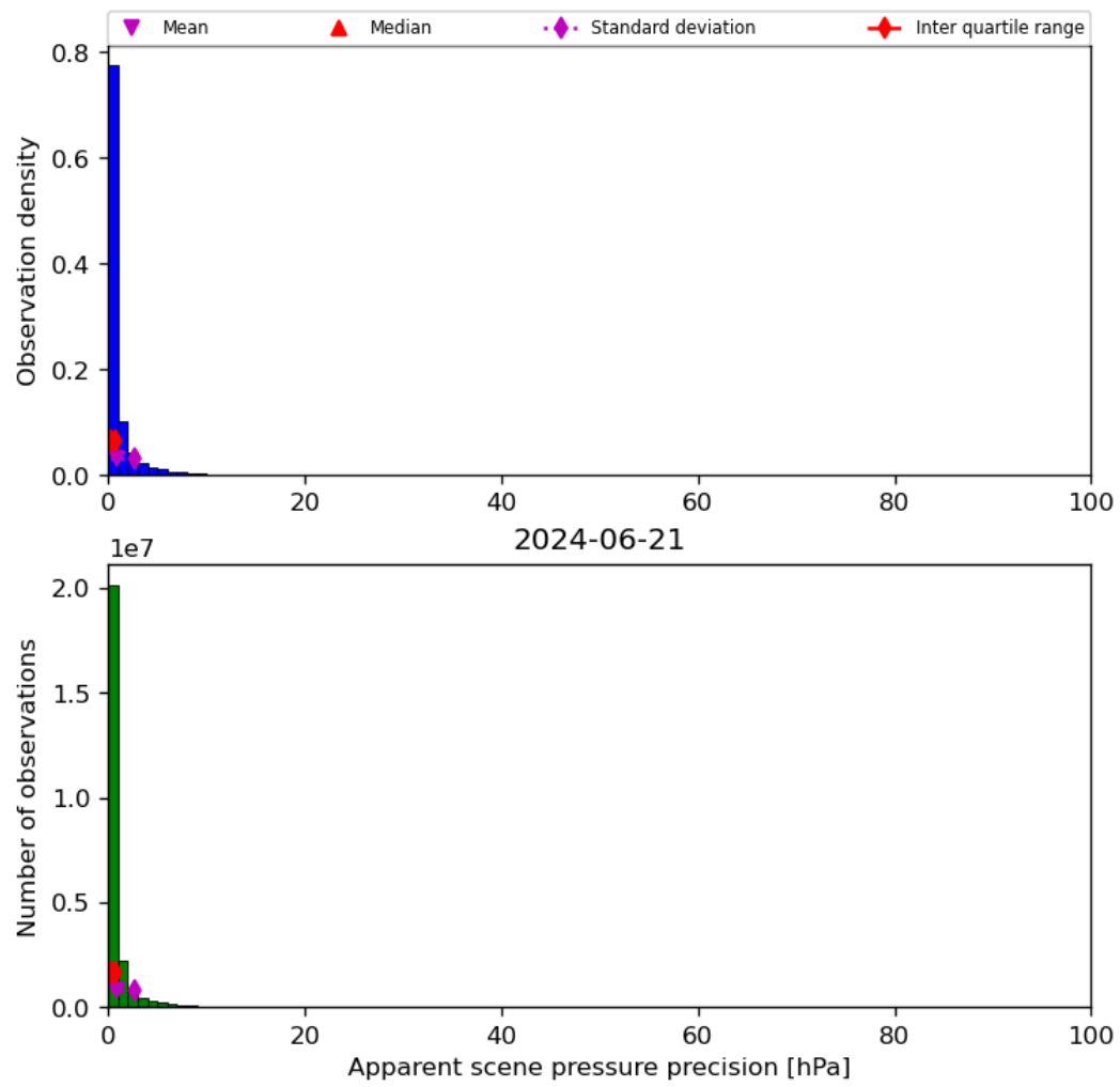
Figure 37: Histogram of “Apparent scene pressure precision” for 2024-06-20 to 2024-06-22
