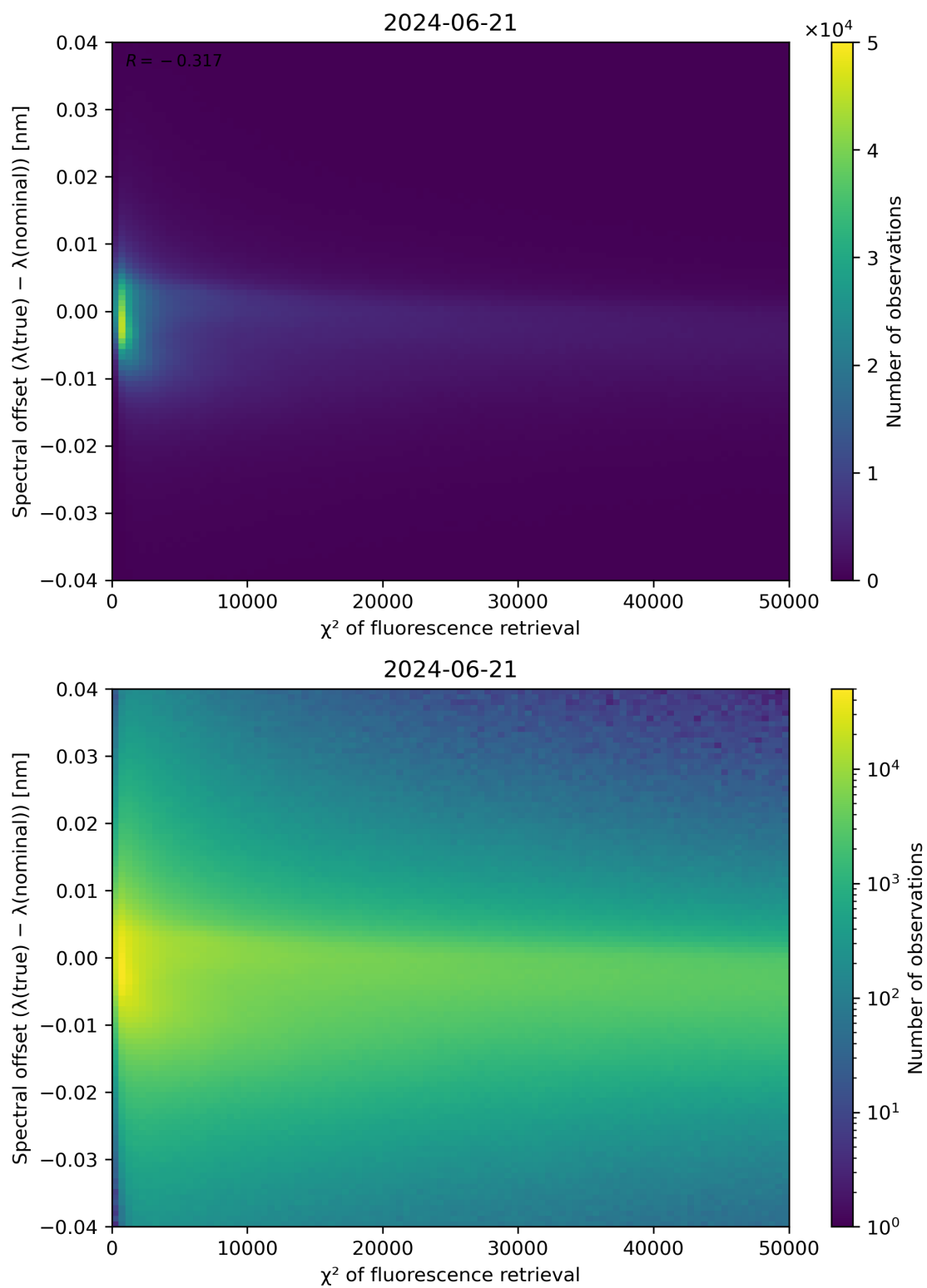
Figure 69: Scatter density plot of " \chi^2 of fluorescence retrieval" against "Spectral offset ( \lambda(\text{true}) - \lambda(\text{nominal})) " for 2024-06-20 to 2024-06-22.
