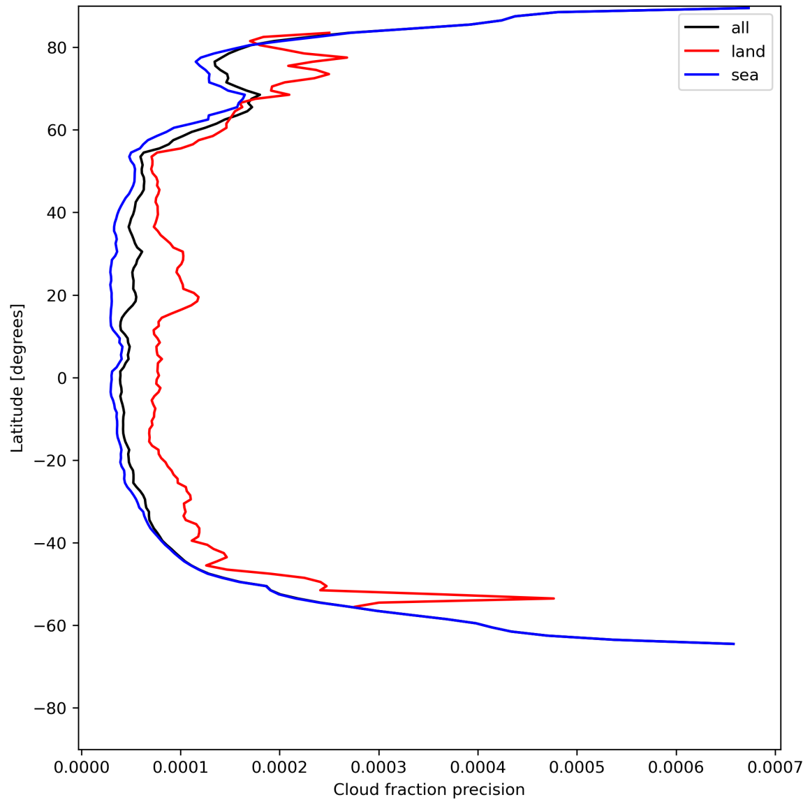
Figure 16: Zonal average of “Cloud fraction precision” for 2024-06-20 to 2024-06-22.
