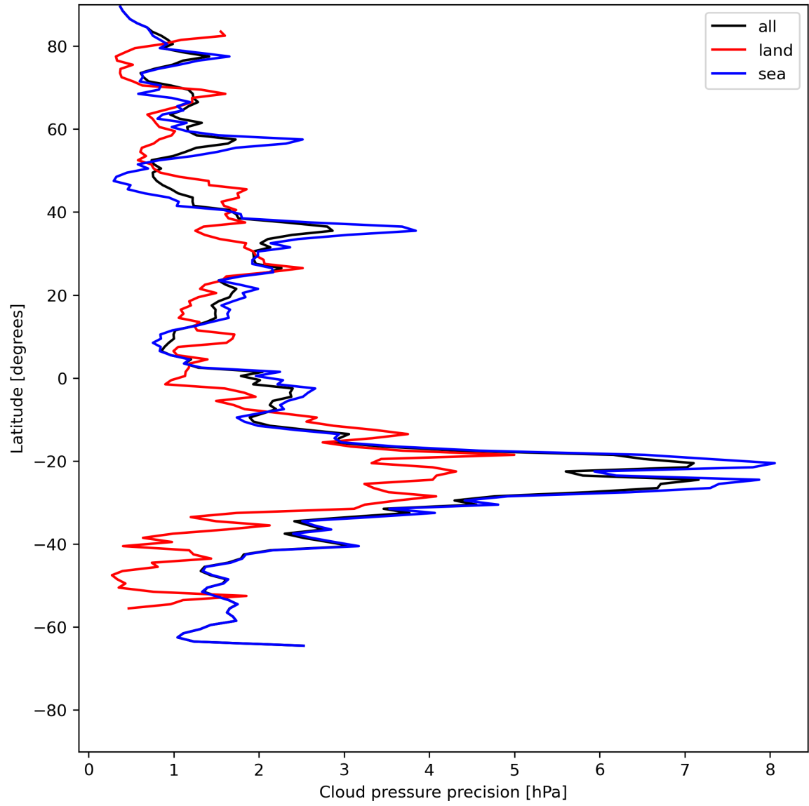
Figure 14: Zonal average of "Cloud pressure precision" for 2024-06-20 to 2024-06-22.
