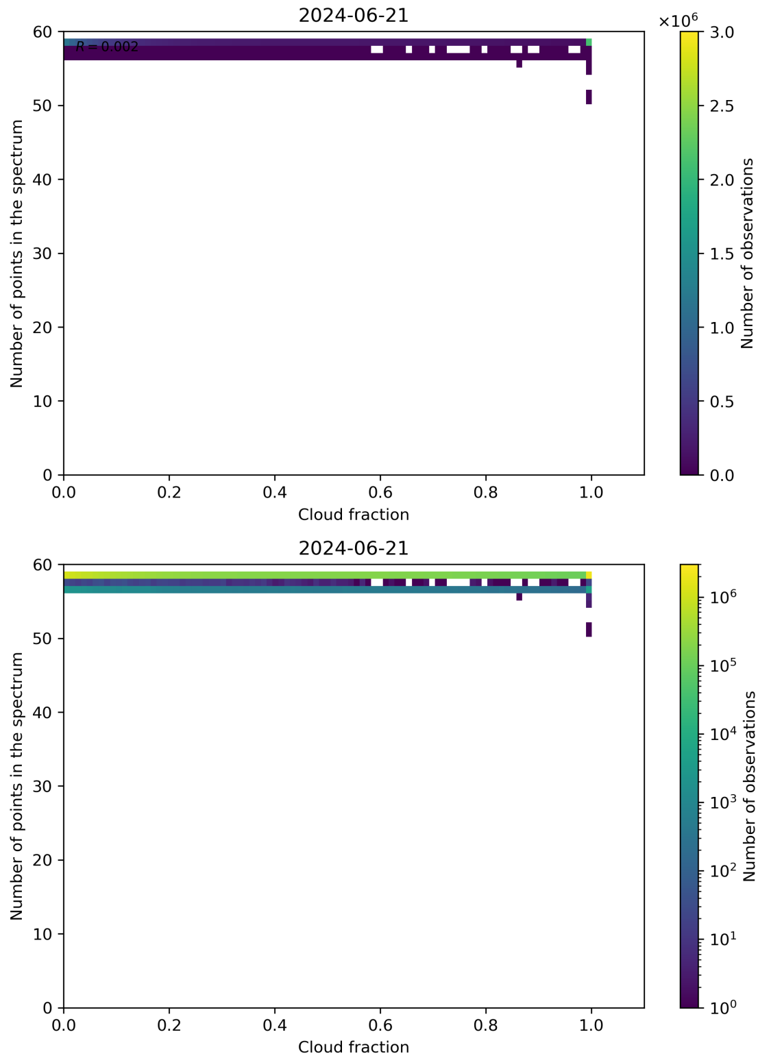
Figure 74: Scatter density plot of “Cloud fraction” against “Number of points in the spectrum” for 2024-06-20 to 2024-06-22.
