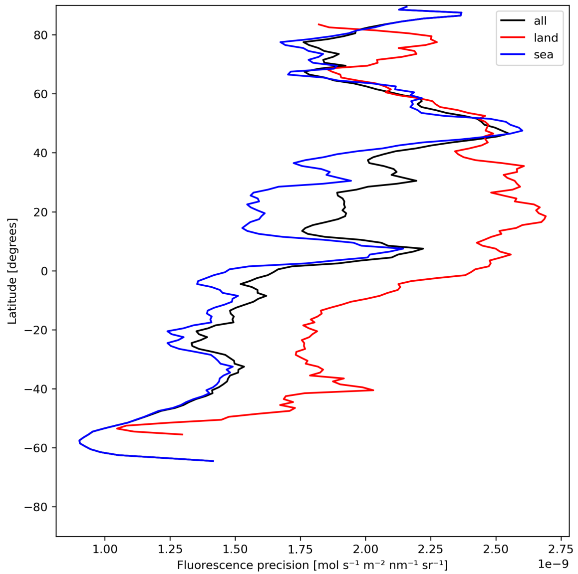
Figure 24: Zonal average of “Fluorescence precision” for 2024-06-20 to 2024-06-22.
