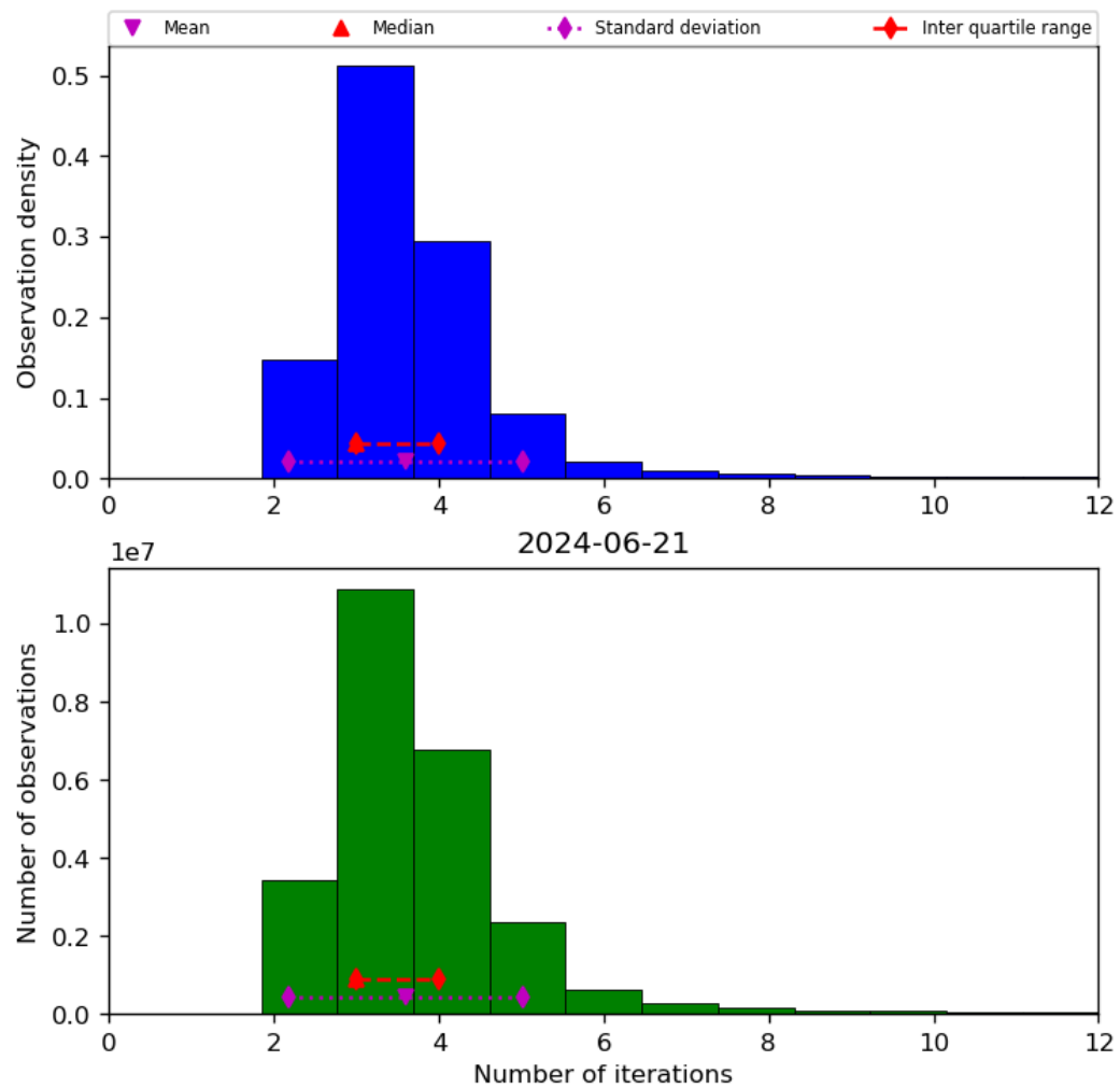
Figure 39: Histogram of “Number of iterations” for 2024-06-20 to 2024-06-22
