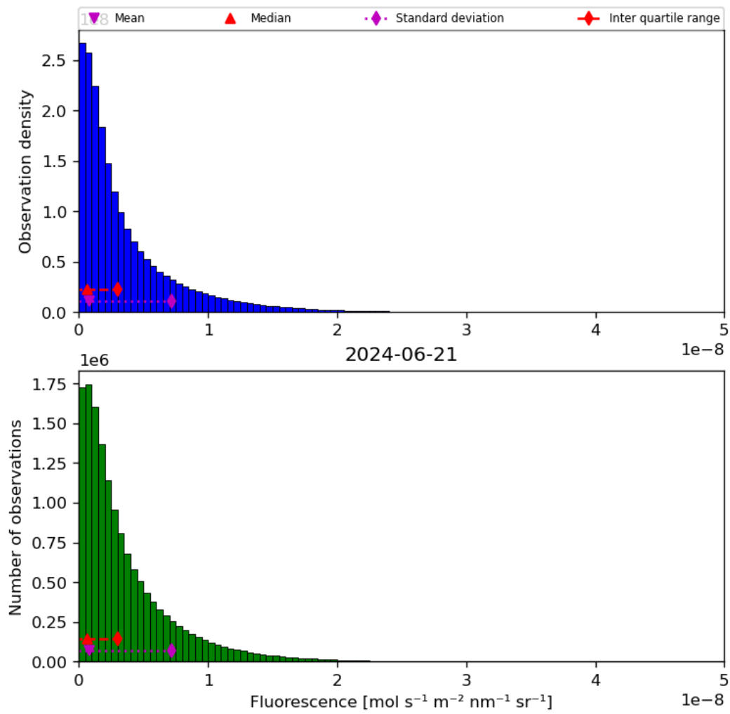
Figure 40: Histogram of “Fluorescence” for 2024-06-20 to 2024-06-22
