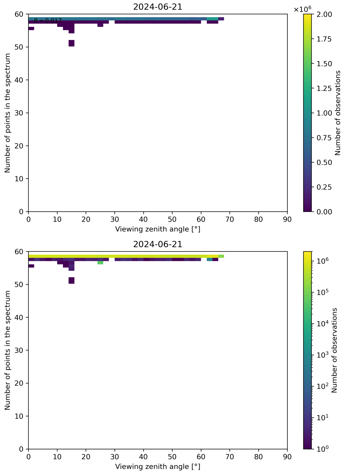
Figure 125: Scatter density plot of “Viewing zenith angle” against “Number of points in the spectrum” for 2024-06-20 to 2024-06-22.
