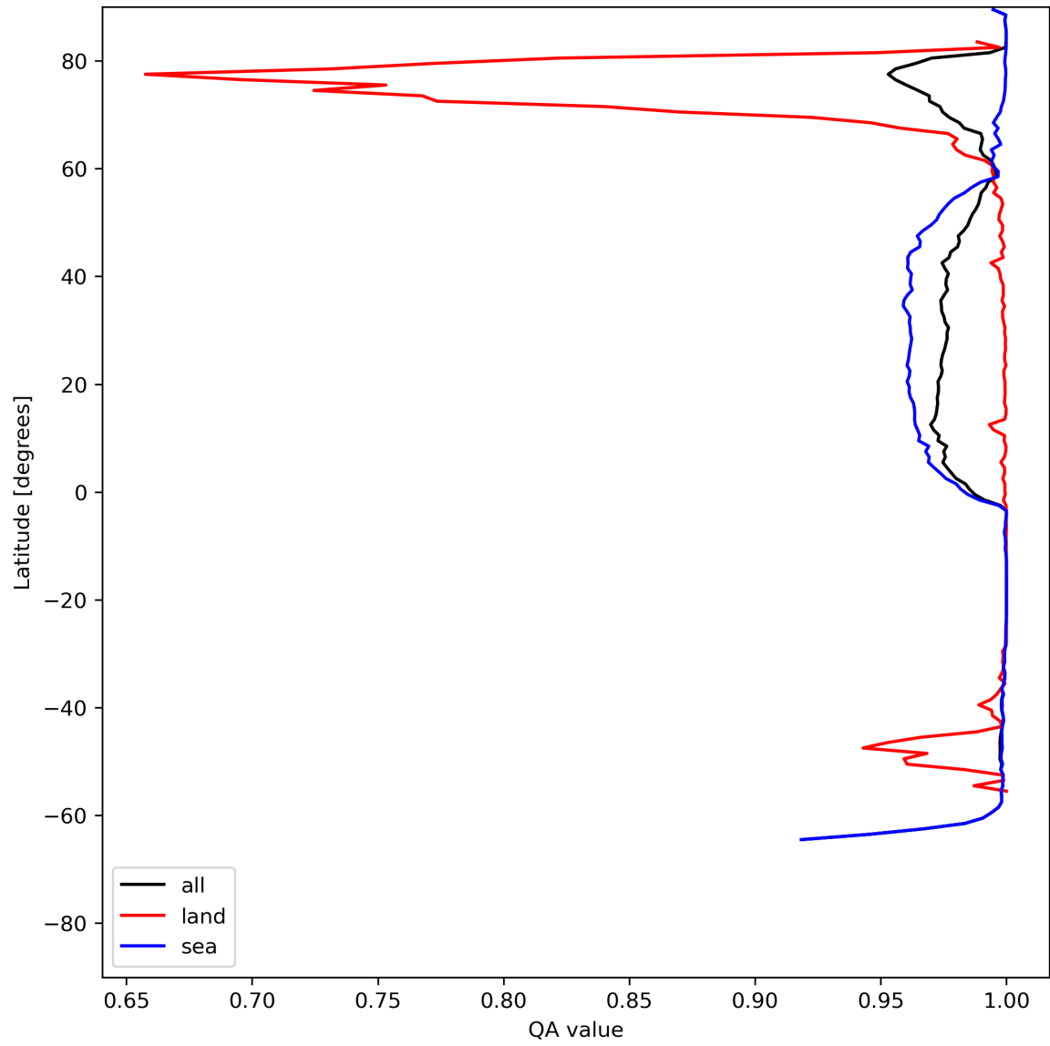
Figure 12: Zonal average of “QA value” for 2024-06-20 to 2024-06-22.
