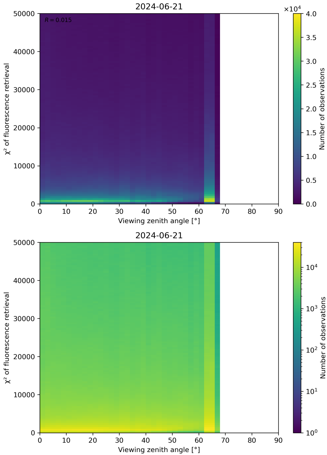
Figure 119: Scatter density plot of “Viewing zenith angle” against “ \chi^2 of fluorescence retrieval” for 2024-06-20 to 2024-06-22.
