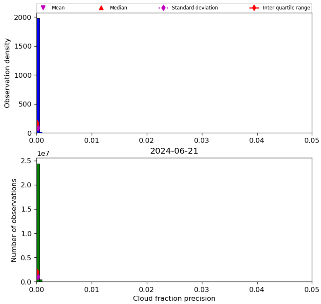
Figure 33: Histogram of “Cloud fraction precision” for 2024-06-20 to 2024-06-22
