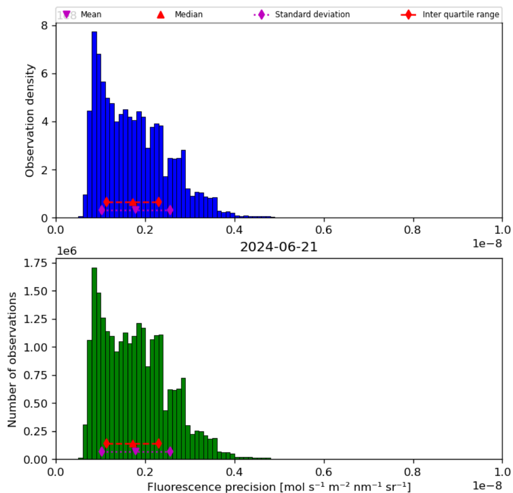
Figure 41: Histogram of “Fluorescence precision” for 2024-06-20 to 2024-06-22
