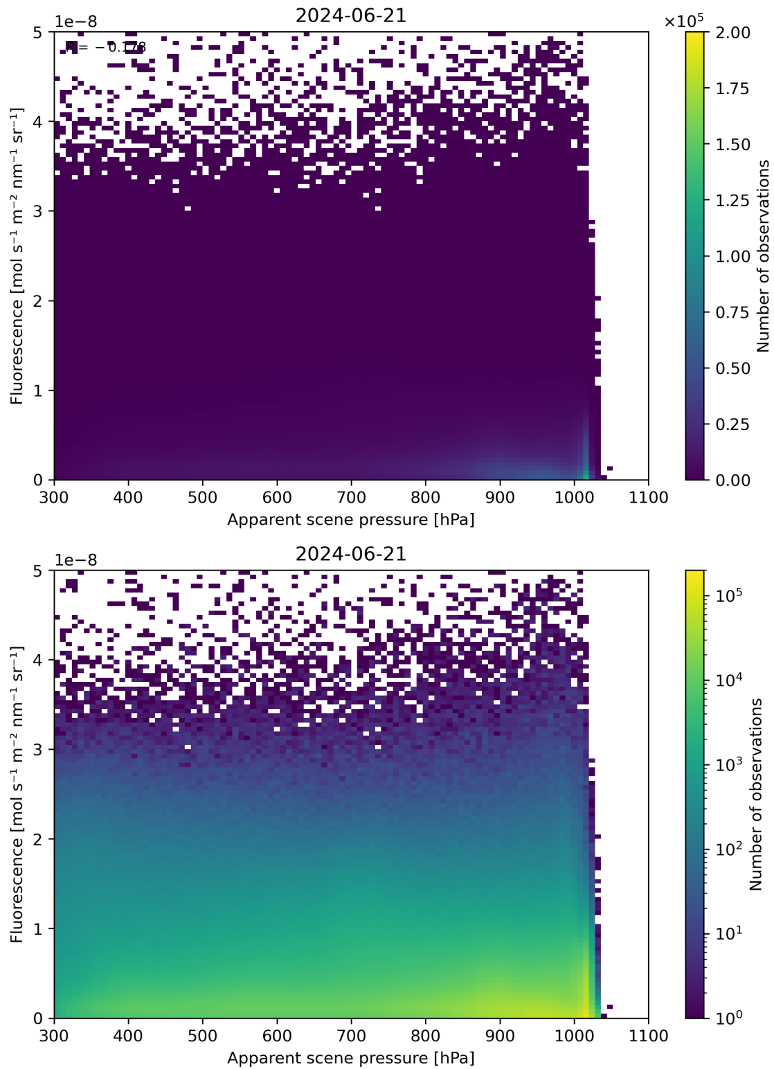
Figure 64: Scatter density plot of “Apparent scene pressure” against “Fluorescence” for 2024-06-20 to 2024-06-22.
