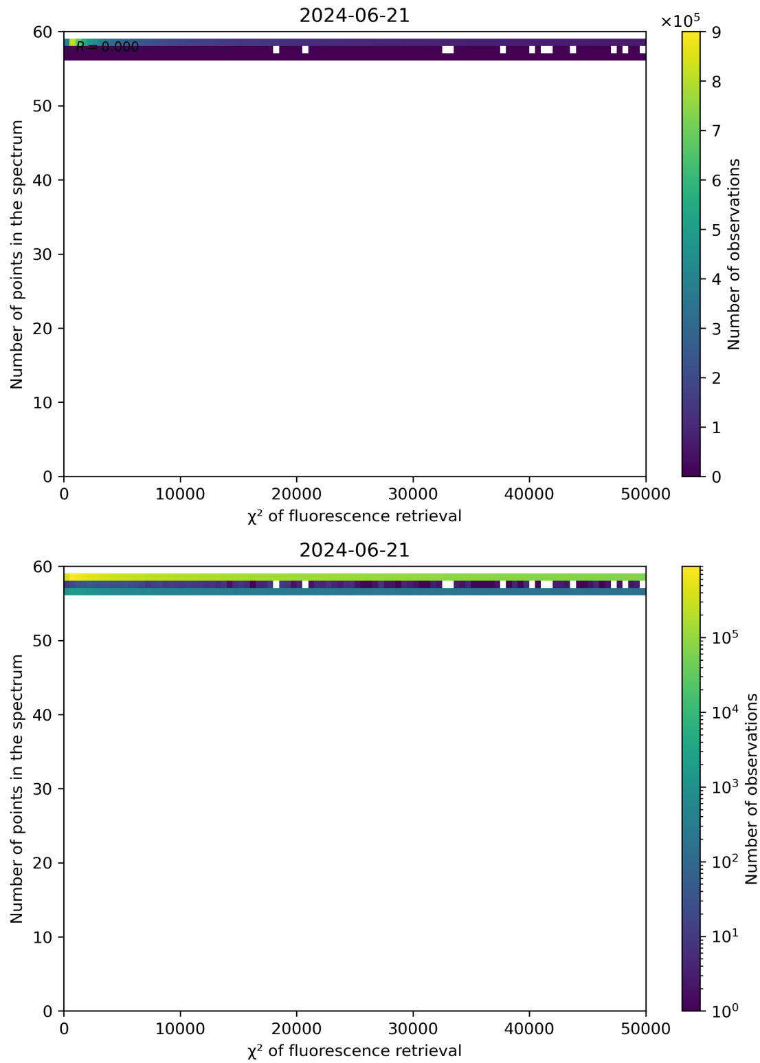
Figure 68: Scatter density plot of " \chi^2 of fluorescence retrieval" against "Number of points in the spectrum" for 2024-06-20 to 2024-06-22.
