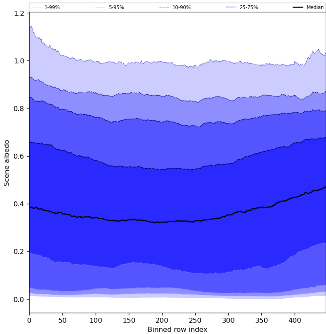
Figure 51: Along track statistics of “Scene albedo” for 2024-06-20 to 2024-06-22
