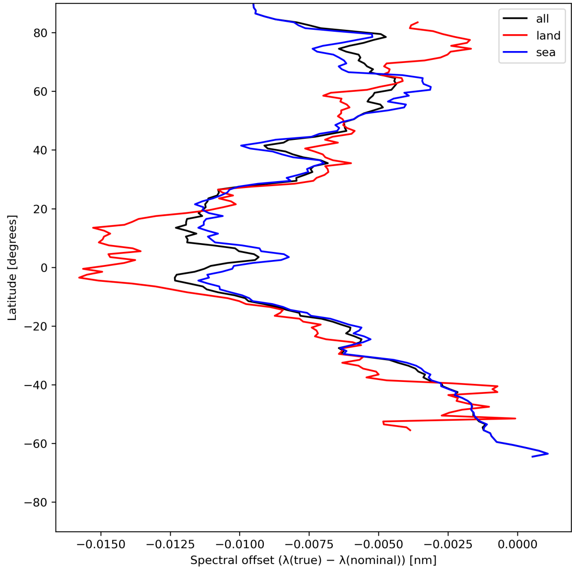
Figure 28: Zonal average of “Spectral offset ( \lambda(\text{true}) - \lambda(\text{nominal}) )” for 2024-06-20 to 2024-06-22.
