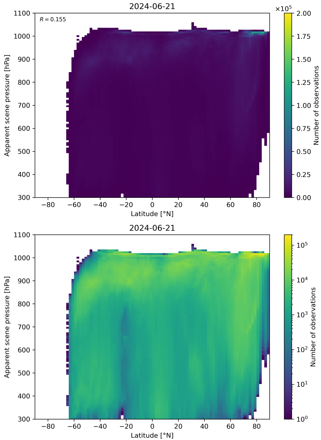
Figure 88: Scatter density plot of “Latitude” against “Apparent scene pressure” for 2024-06-20 to 2024-06-22.
