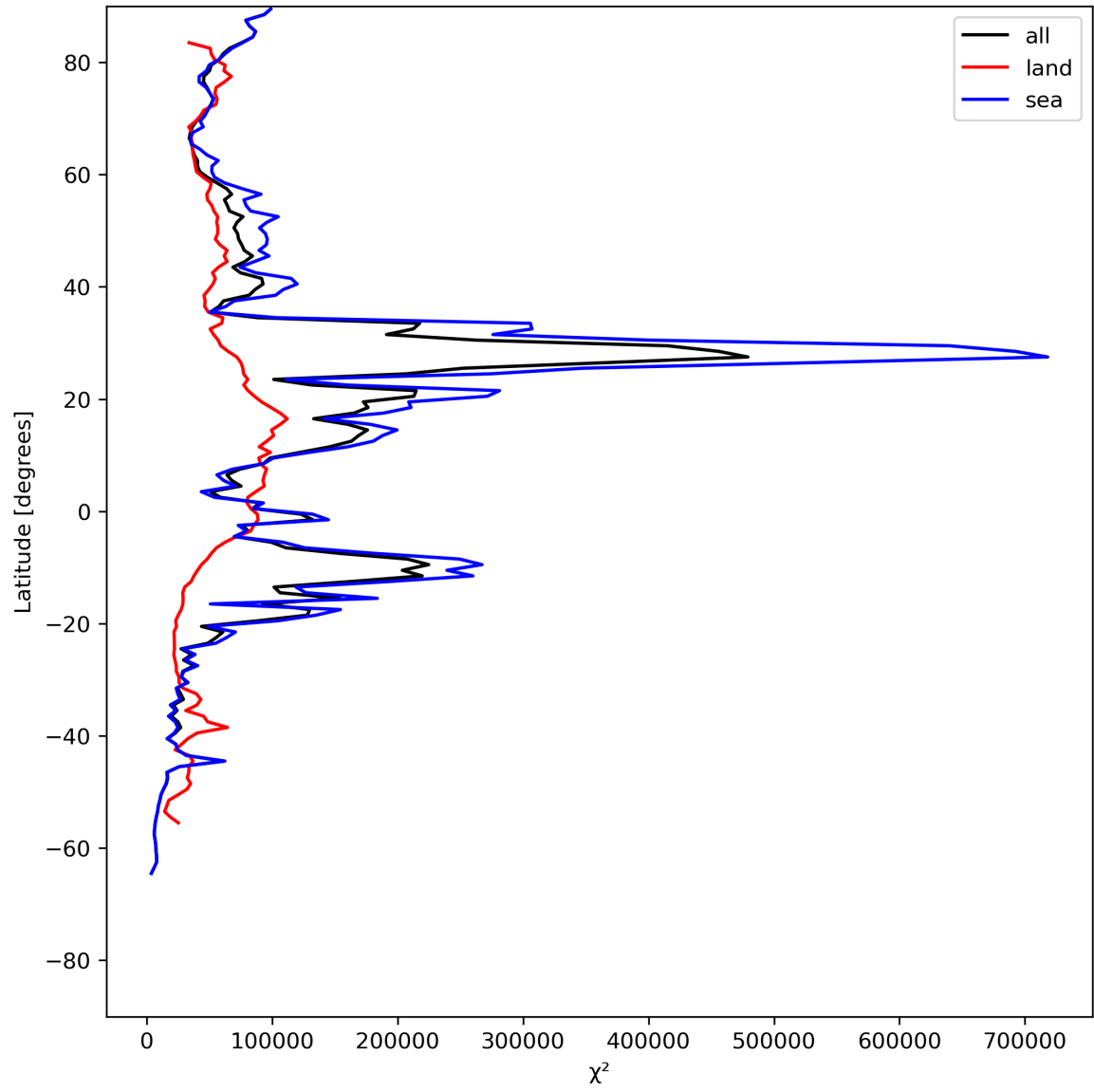
Figure 21: Zonal average of “ \chi^2 ” for 2024-06-20 to 2024-06-22.
