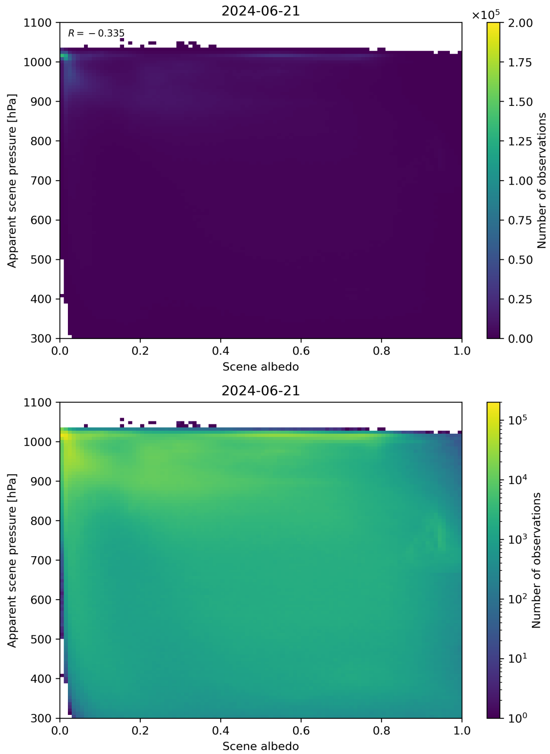
Figure 102: Scatter density plot of “Scene albedo” against “Apparent scene pressure” for 2024-06-20 to 2024-06-22.
