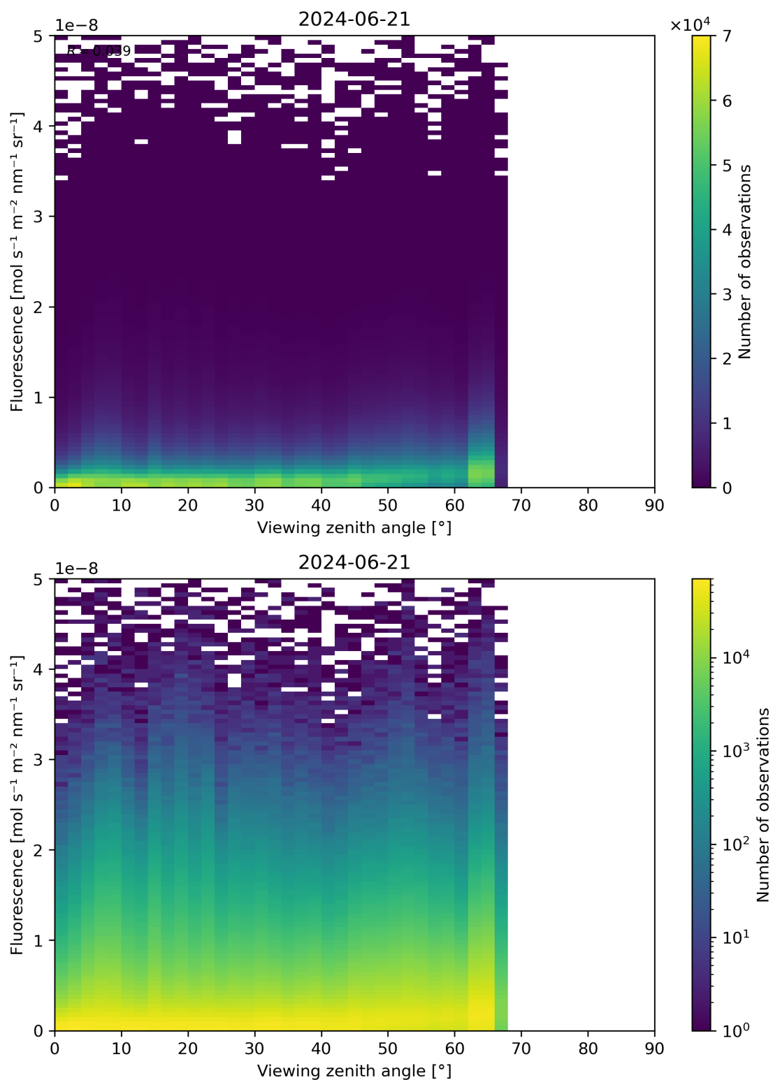
Figure 122: Scatter density plot of “Viewing zenith angle” against “Fluorescence” for 2024-06-20 to 2024-06-22.
