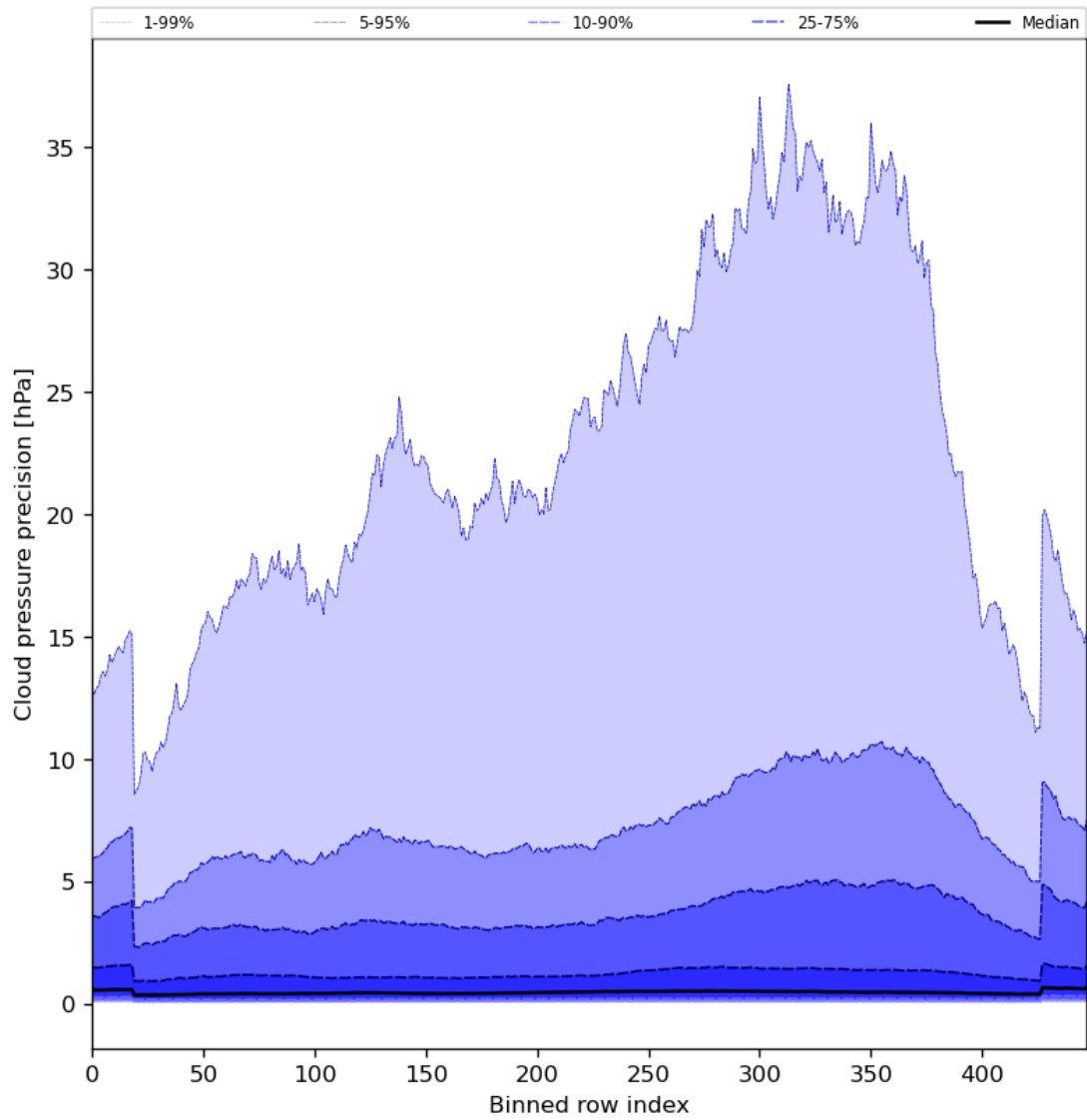
Figure 48: Along track statistics of “Cloud pressure precision” for 2024-06-20 to 2024-06-22
