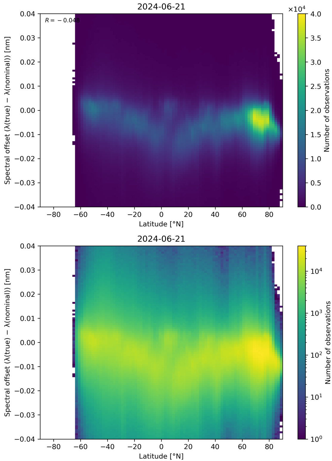
Figure 96: Scatter density plot of “Latitude” against “Spectral offset ( \lambda(\text{true}) - \lambda(\text{nominal}) )” for 2024-06-20 to 2024-06-22.
