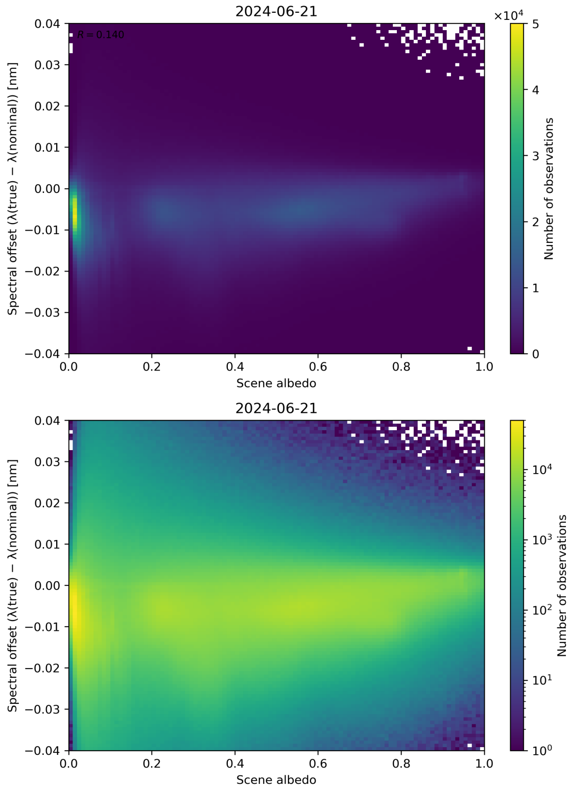
Figure 107: Scatter density plot of “Scene albedo” against “Spectral offset ( \lambda(\text{true}) - \lambda(\text{nominal}) )” for 2024-06-20 to 2024-06-22.
