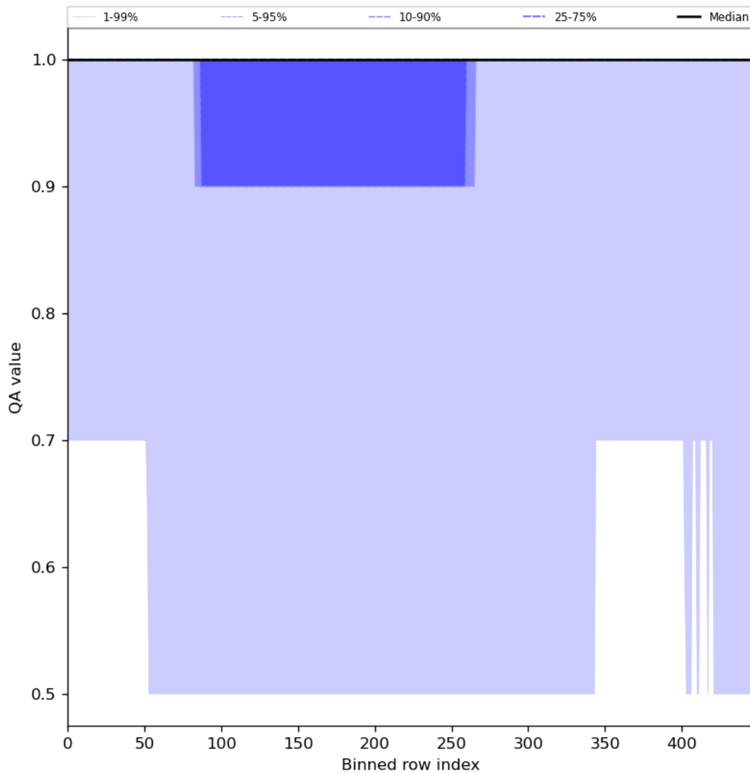
Figure 46: Along track statistics of “QA value” for 2024-06-20 to 2024-06-22
