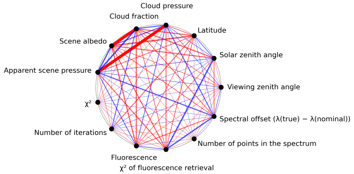
Figure 1: Map of correlation graph for 2024-06-20 to 2024-06-22.
