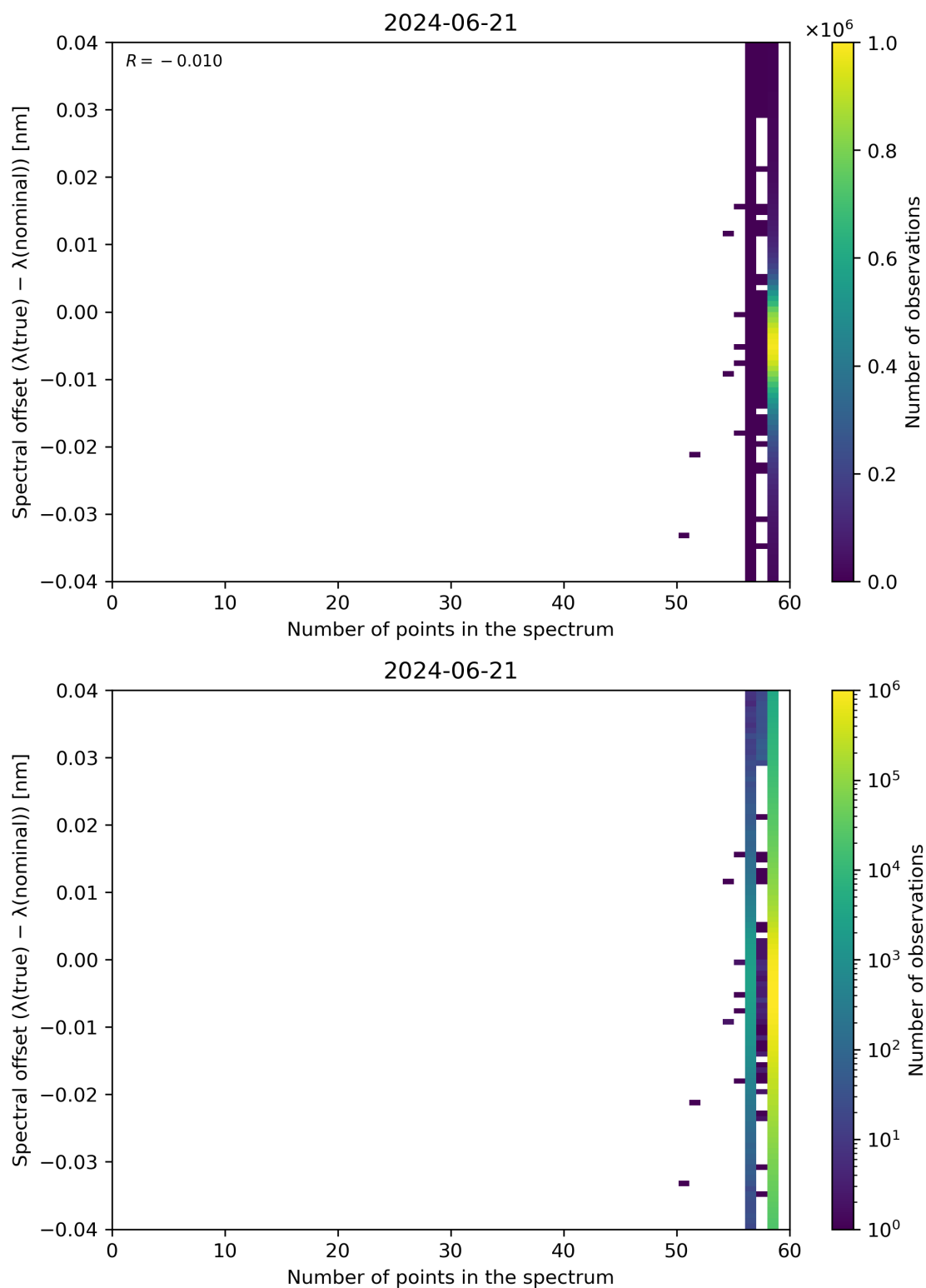
Figure 101: Scatter density plot of “Number of points in the spectrum” against “Spectral offset ( \lambda(\text{true}) - \lambda(\text{nominal}) )” for 2024-06-20 to 2024-06-22.
