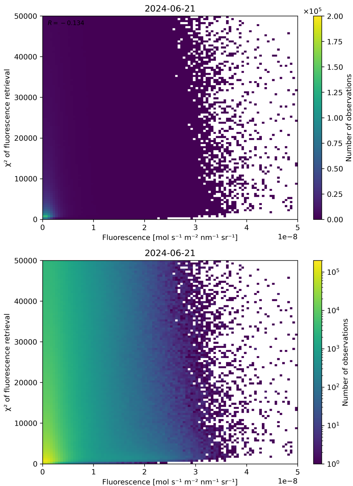
Figure 85: Scatter density plot of “Fluorescence” against “ \chi^2 of fluorescence retrieval” for 2024-06-20 to 2024-06-22.
