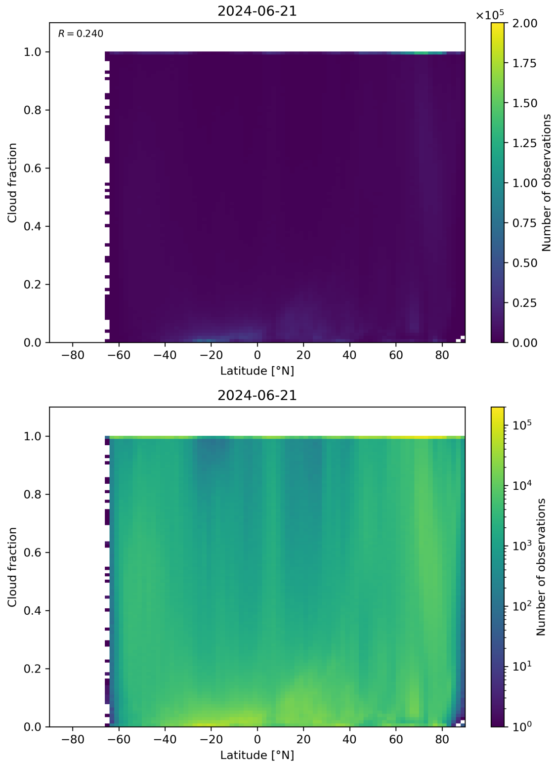
Figure 90: Scatter density plot of “Latitude” against “Cloud fraction” for 2024-06-20 to 2024-06-22.
