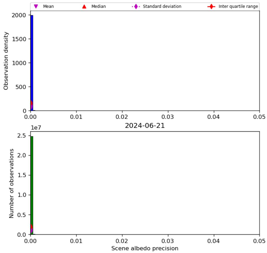
Figure 35: Histogram of “Scene albedo precision” for 2024-06-20 to 2024-06-22
