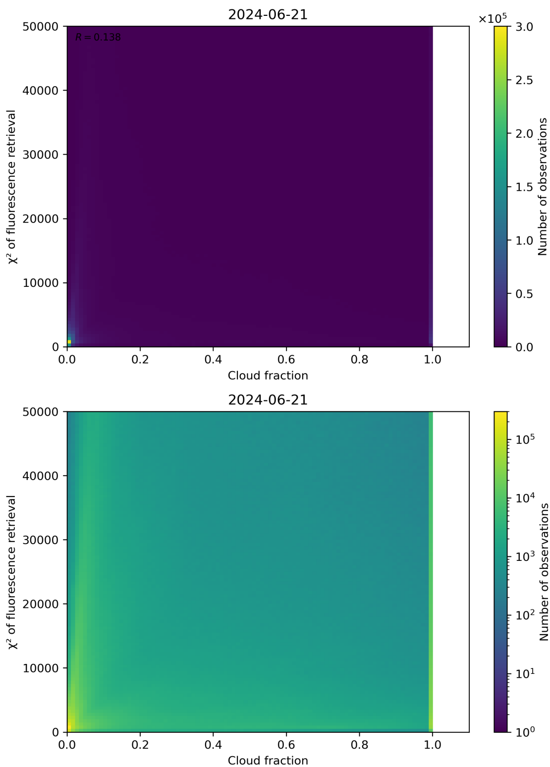
Figure 71: Scatter density plot of “Cloud fraction” against “ \chi^2 of fluorescence retrieval” for 2024-06-20 to 2024-06-22.
