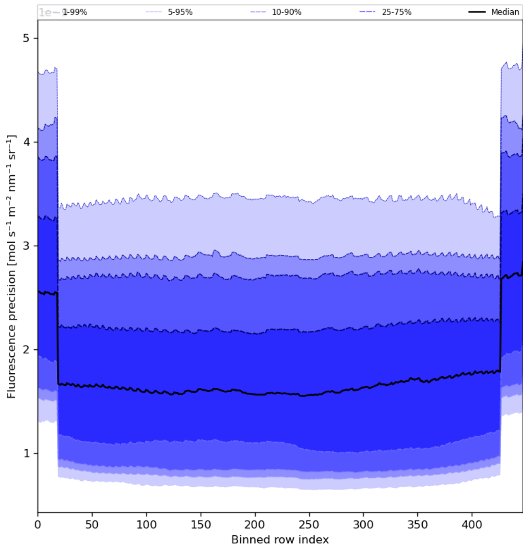
Figure 58: Along track statistics of “Fluorescence precision” for 2024-06-20 to 2024-06-22
