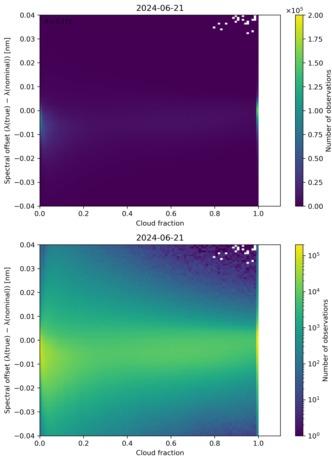
Figure 76: Scatter density plot of “Cloud fraction” against “Spectral offset ( \lambda(\text{true}) - \lambda(\text{nominal}) )” for 2024-06-20 to 2024-06-22.
