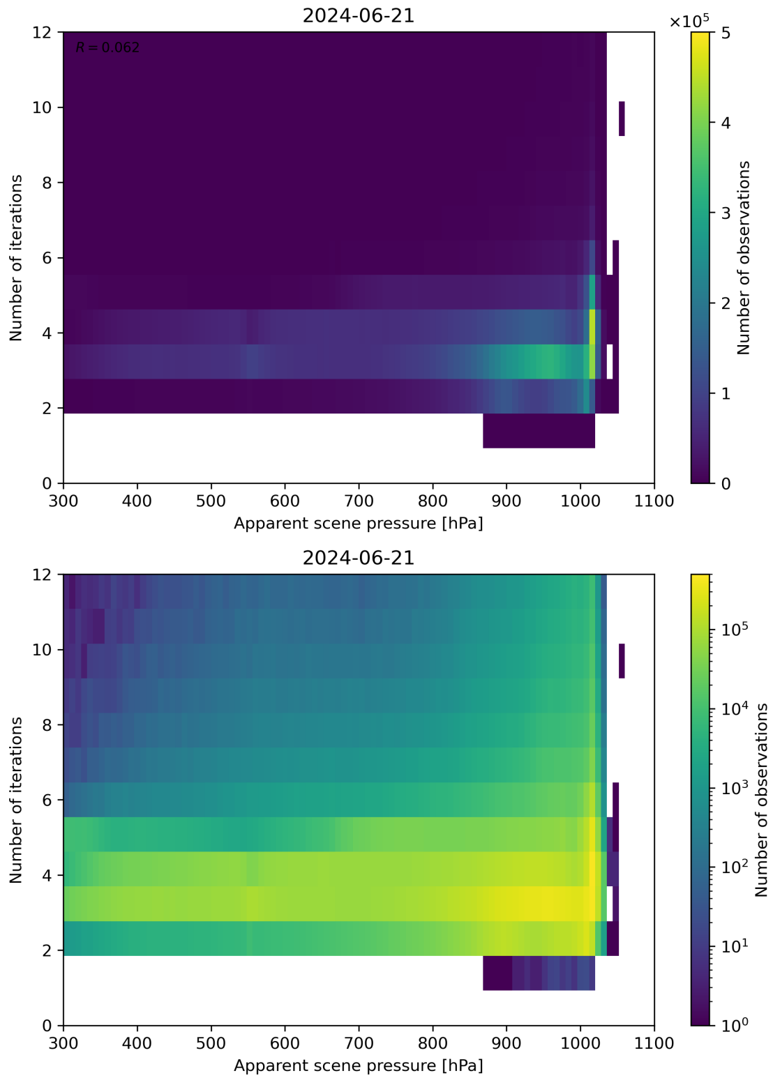
Figure 65: Scatter density plot of “Apparent scene pressure” against “Number of iterations” for 2024-06-20 to 2024-06-22.
