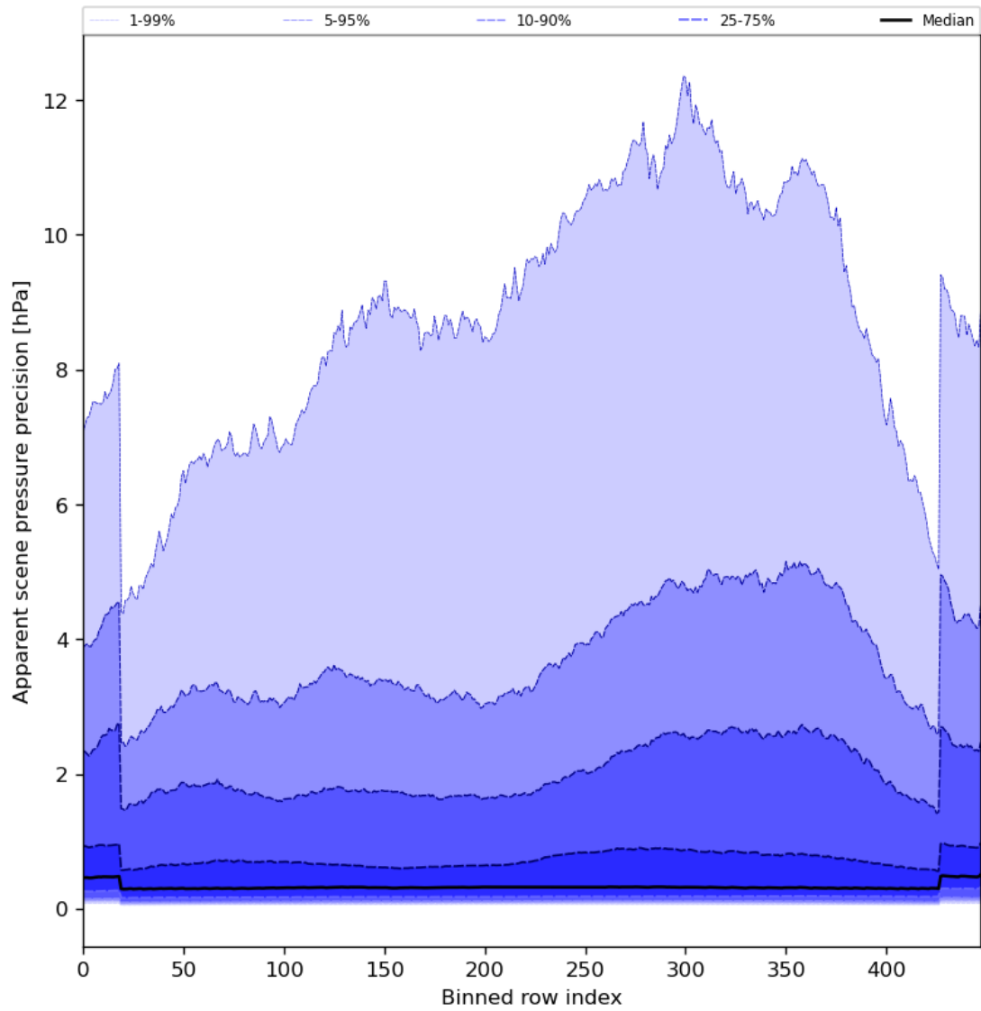
Figure 54: Along track statistics of “Apparent scene pressure precision” for 2024-06-20 to 2024-06-22
