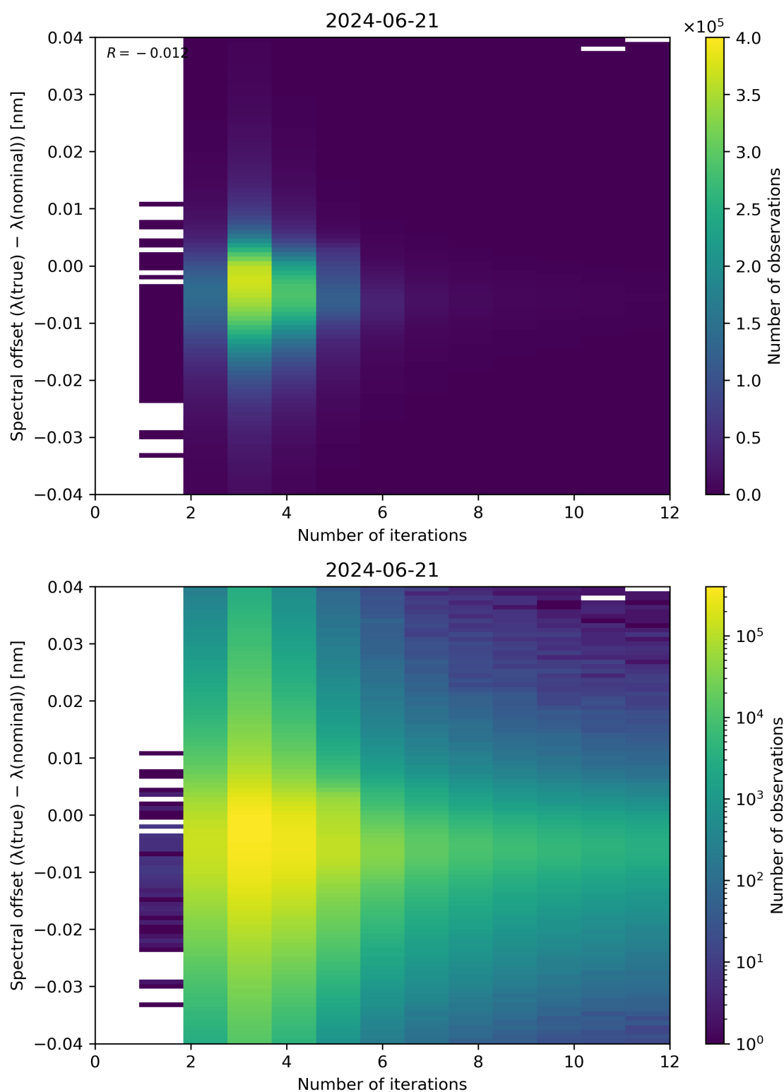
Figure 100: Scatter density plot of “Number of iterations” against “Spectral offset ( \lambda(\text{true}) - \lambda(\text{nominal}) )” for 2024-06-20 to 2024-06-22.
