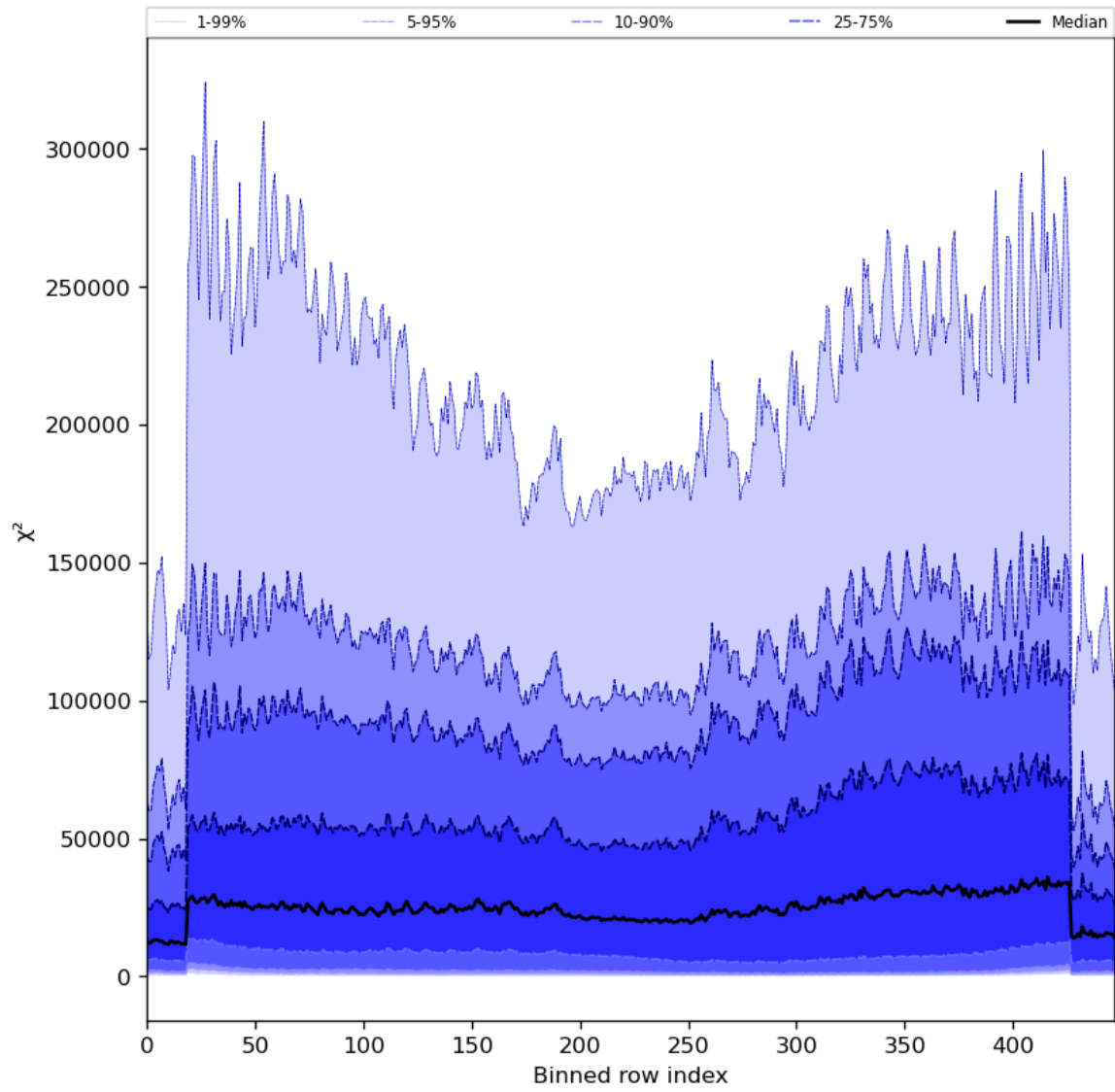
Figure 55: Along track statistics of “ \chi^2 ” for 2024-06-20 to 2024-06-22
