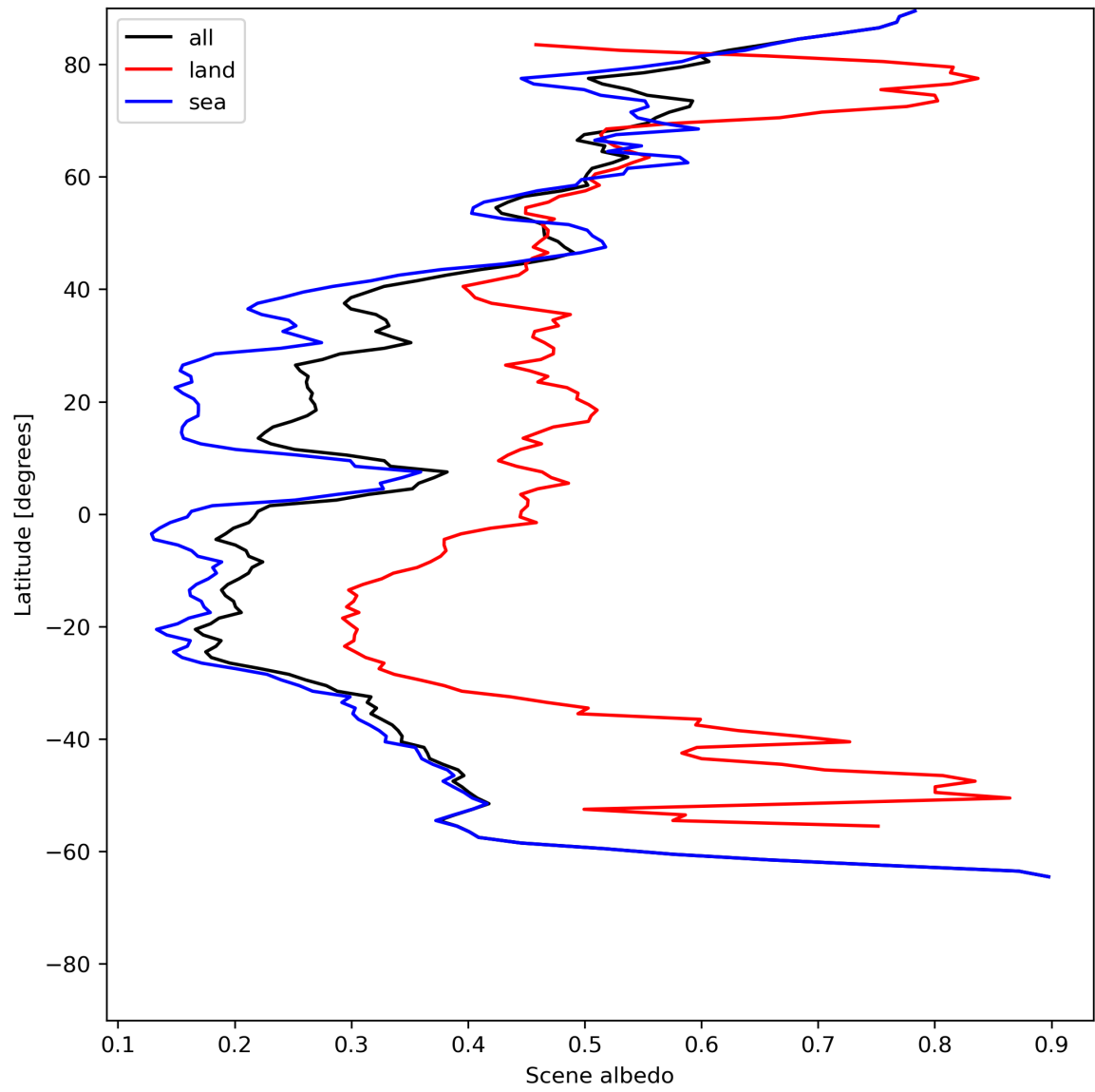
Figure 17: Zonal average of “Scene albedo” for 2024-06-20 to 2024-06-22.
