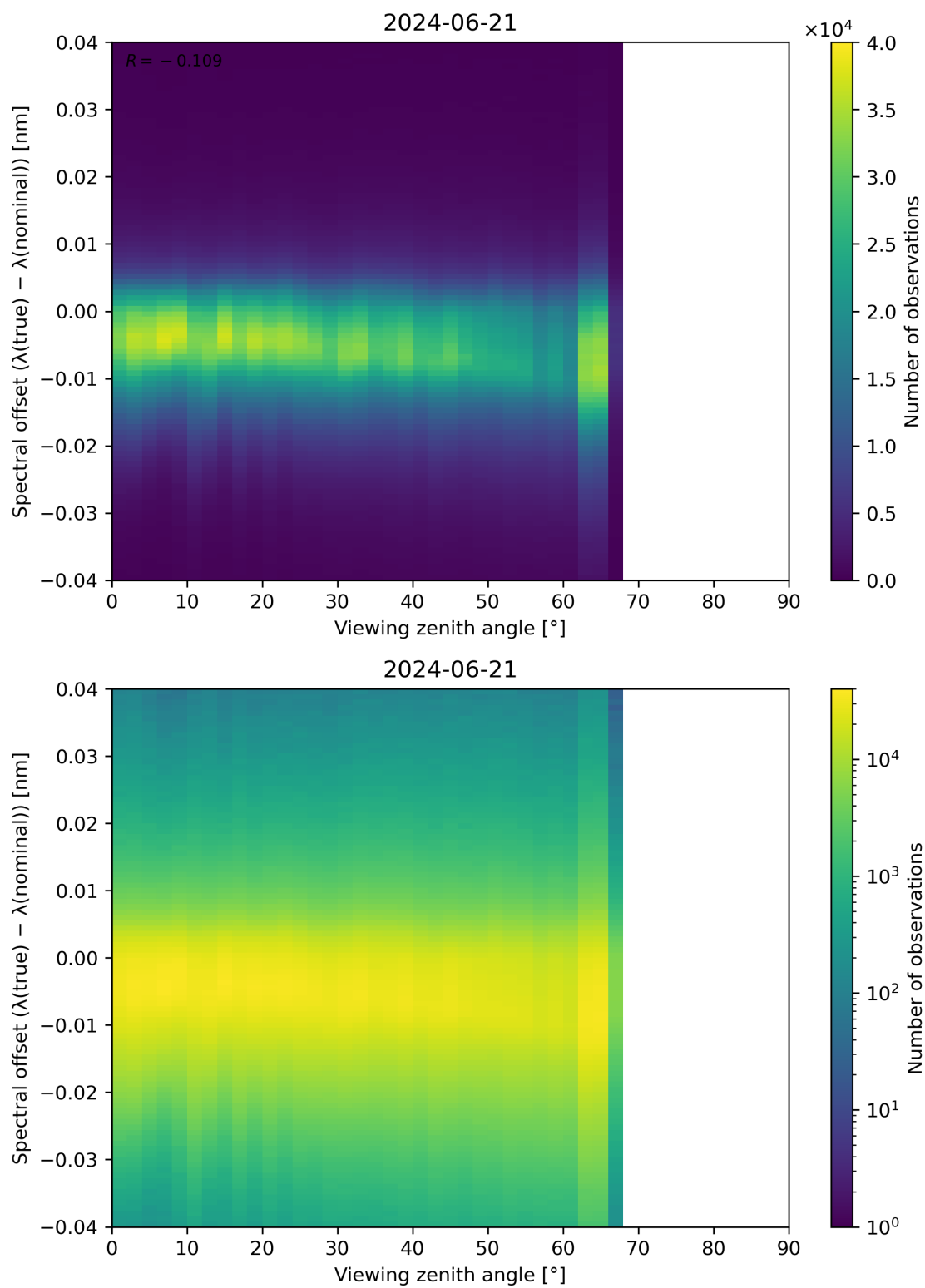
Figure 128: Scatter density plot of “Viewing zenith angle” against “Spectral offset ( \lambda(\text{true}) - \lambda(\text{nominal}) )” for 2024-06-20 to 2024-06-22.
