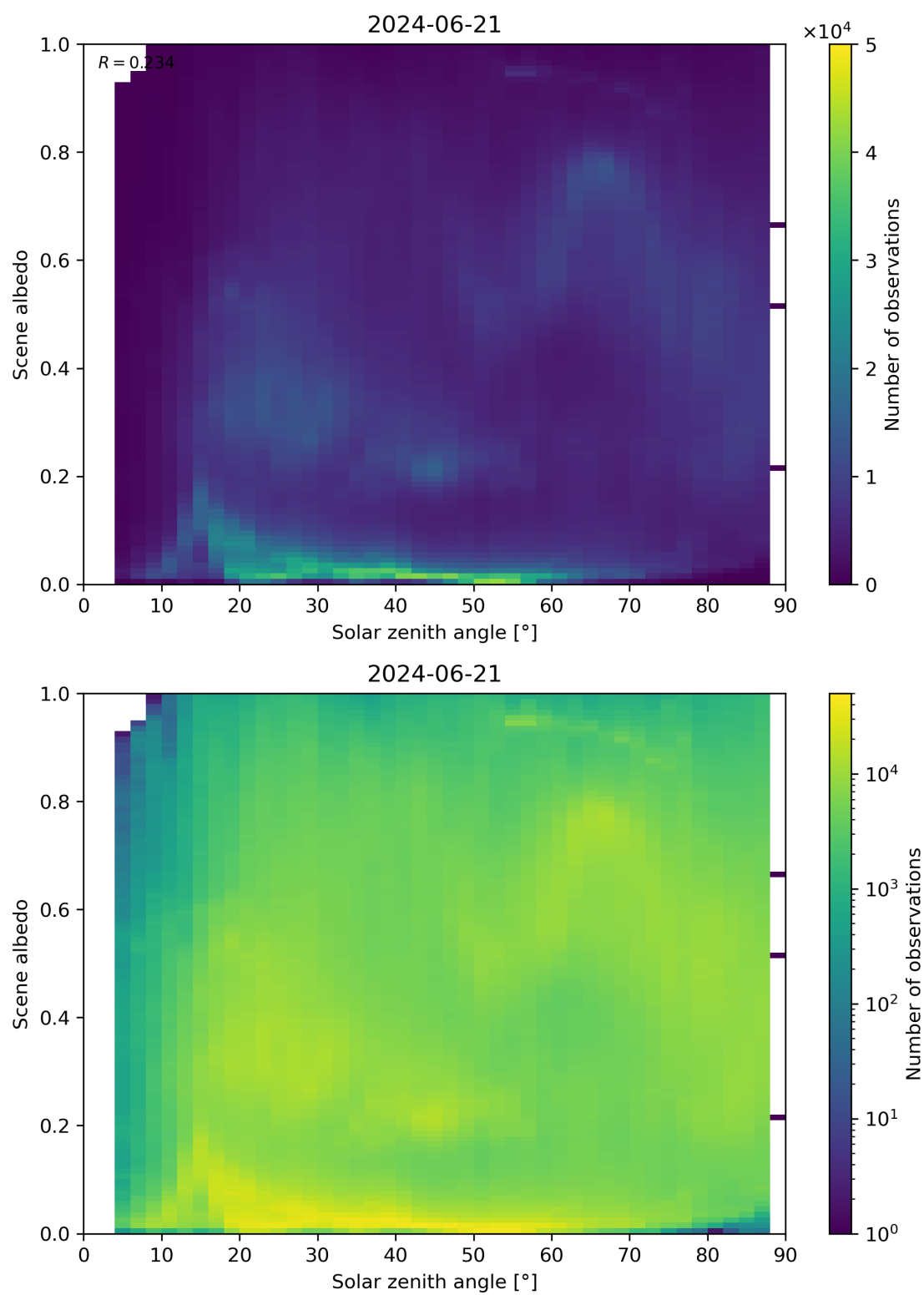
Figure 116: Scatter density plot of “Solar zenith angle” against “Scene albedo” for 2024-06-20 to 2024-06-22.
