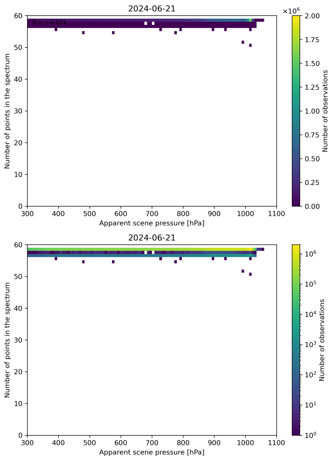
Figure 66: Scatter density plot of “Apparent scene pressure” against “Number of points in the spectrum” for 2024-06-20 to 2024-06-22.
