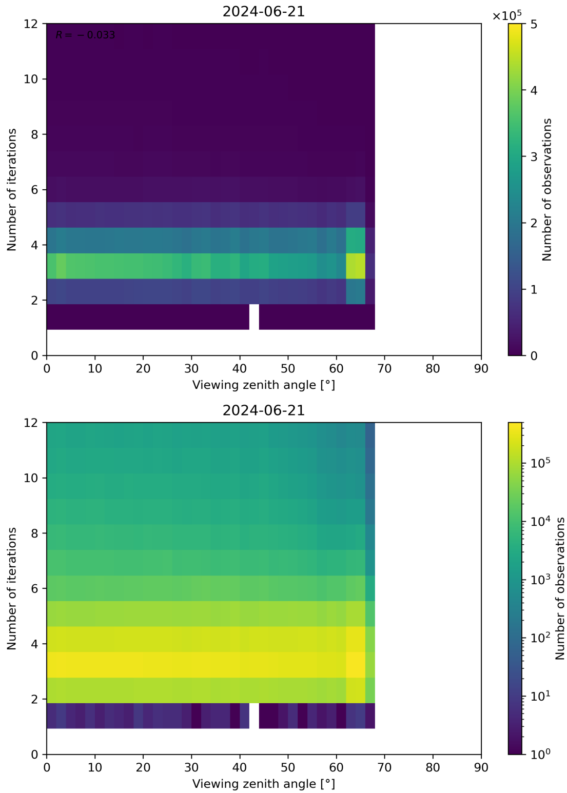
Figure 124: Scatter density plot of “Viewing zenith angle” against “Number of iterations” for 2024-06-20 to 2024-06-22.
