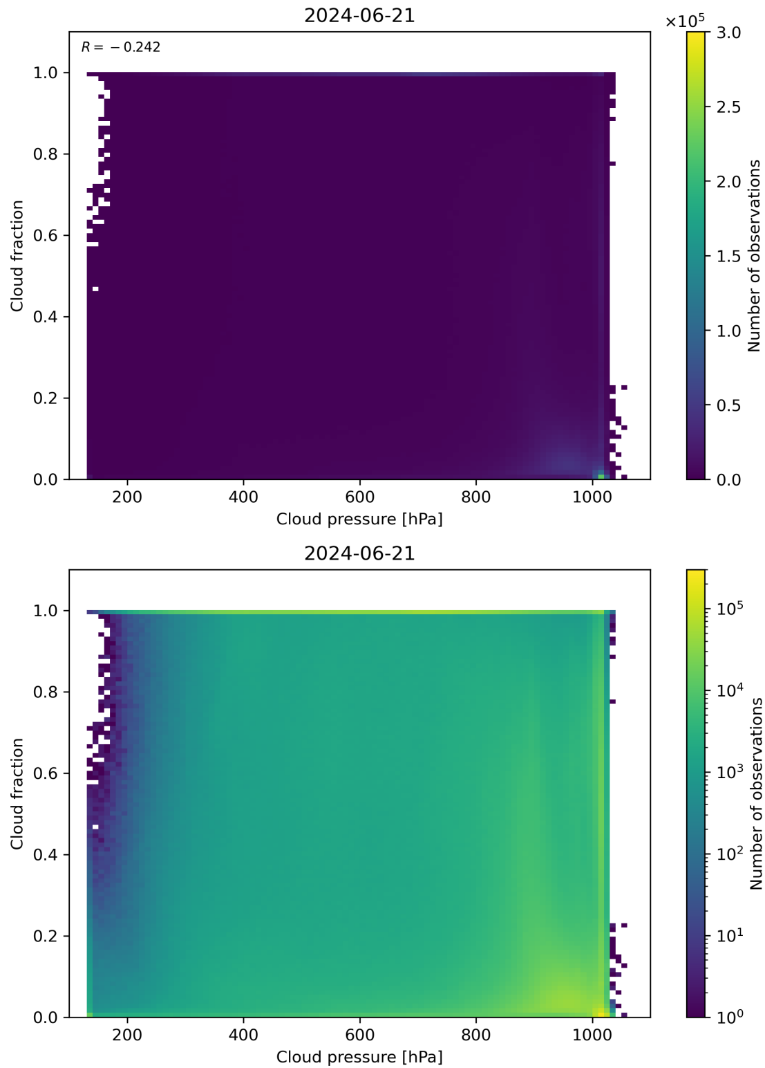
Figure 79: Scatter density plot of “Cloud pressure” against “Cloud fraction” for 2024-06-20 to 2024-06-22.
