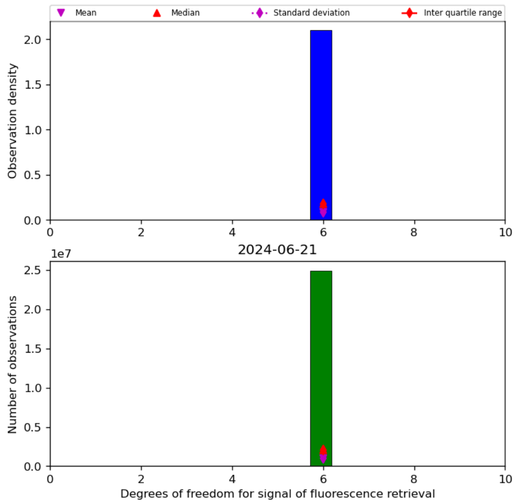
Figure 43: Histogram of “Degrees of freedom for signal of fluorescence retrieval” for 2024-06-20 to 2024-06-22
