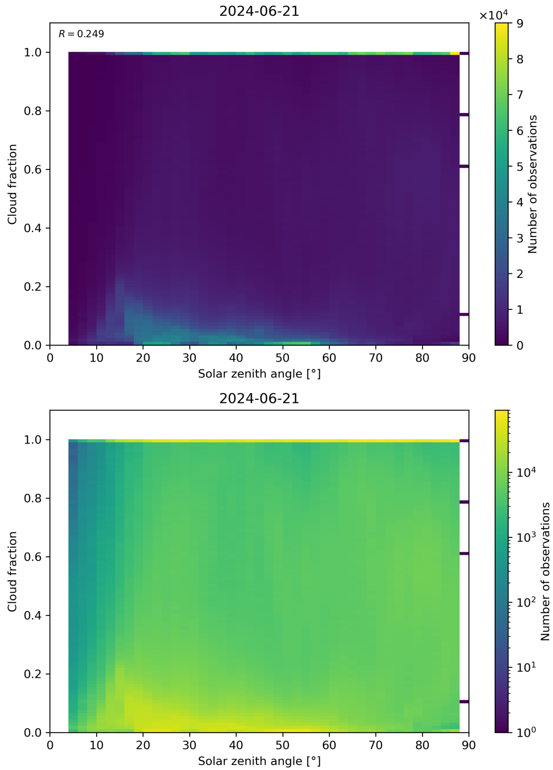
Figure 110: Scatter density plot of “Solar zenith angle” against “Cloud fraction” for 2024-06-20 to 2024-06-22.
