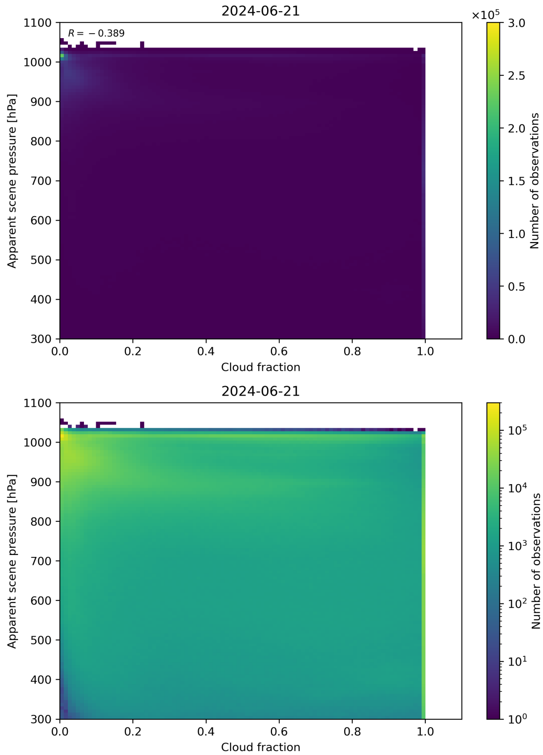
Figure 70: Scatter density plot of “Cloud fraction” against “Apparent scene pressure” for 2024-06-20 to 2024-06-22.
