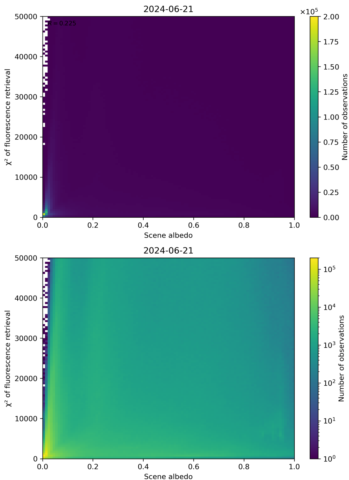
Figure 103: Scatter density plot of “Scene albedo” against “ \chi^2 of fluorescence retrieval” for 2024-06-20 to 2024-06-22.
