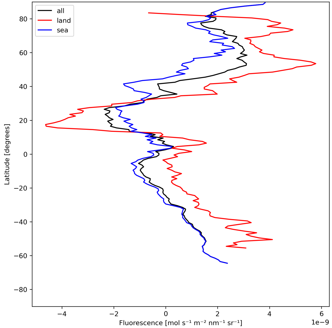
Figure 23: Zonal average of “Fluorescence” for 2024-06-20 to 2024-06-22.
