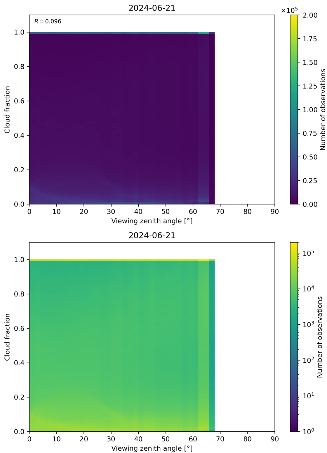
Figure 120: Scatter density plot of “Viewing zenith angle” against “Cloud fraction” for 2024-06-20 to 2024-06-22.
