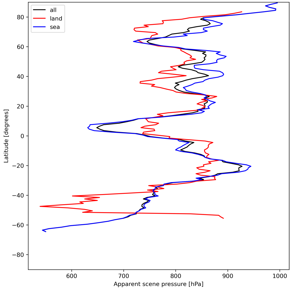
Figure 19: Zonal average of “Apparent scene pressure” for 2024-06-20 to 2024-06-22.
