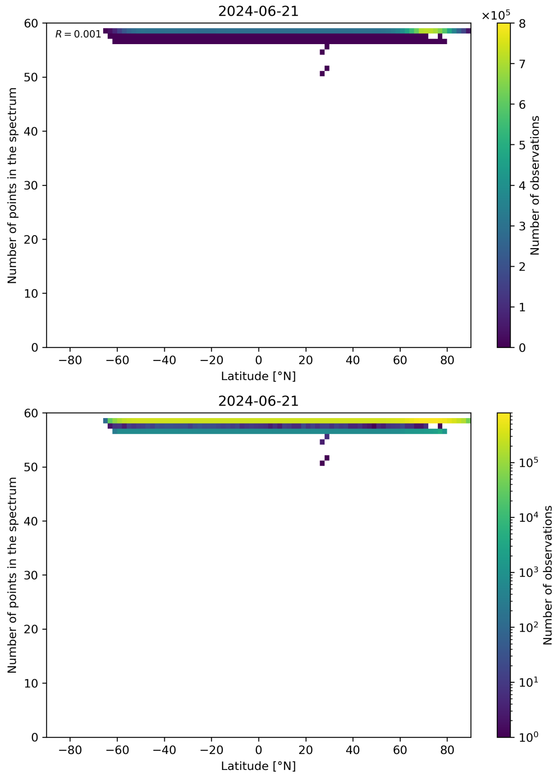
Figure 94: Scatter density plot of “Latitude” against “Number of points in the spectrum” for 2024-06-20 to 2024-06-22.
