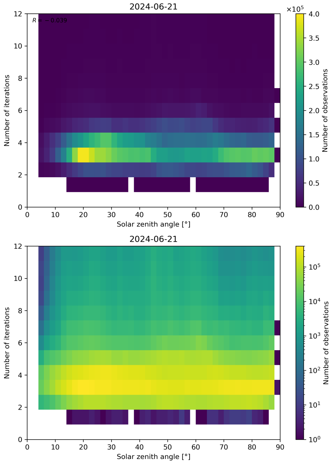
Figure 114: Scatter density plot of “Solar zenith angle” against “Number of iterations” for 2024-06-20 to 2024-06-22.
