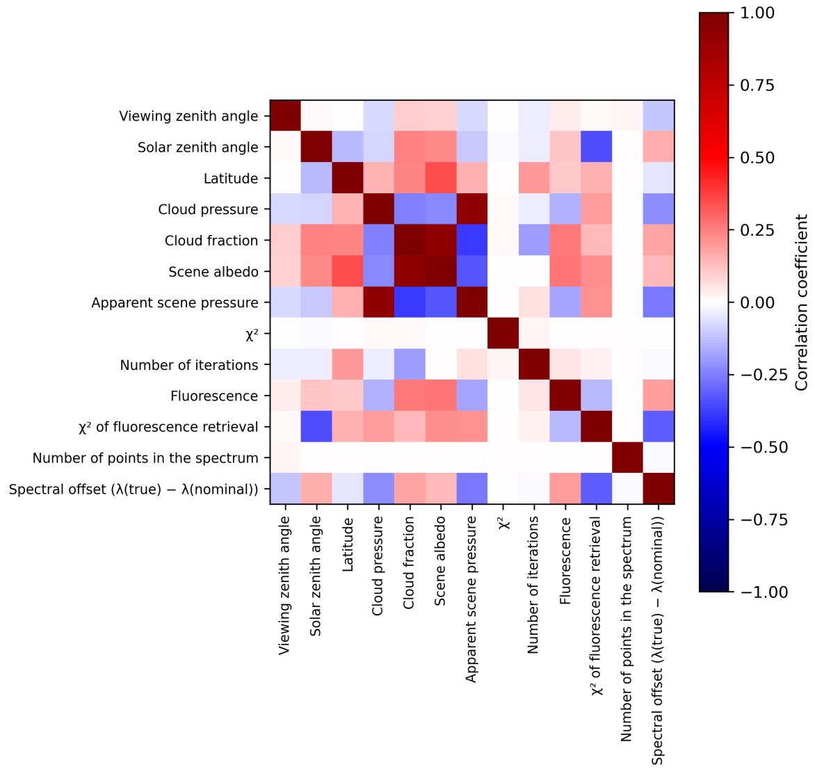
Figure 2: Map of correlation matrix for 2024-06-20 to 2024-06-22.
