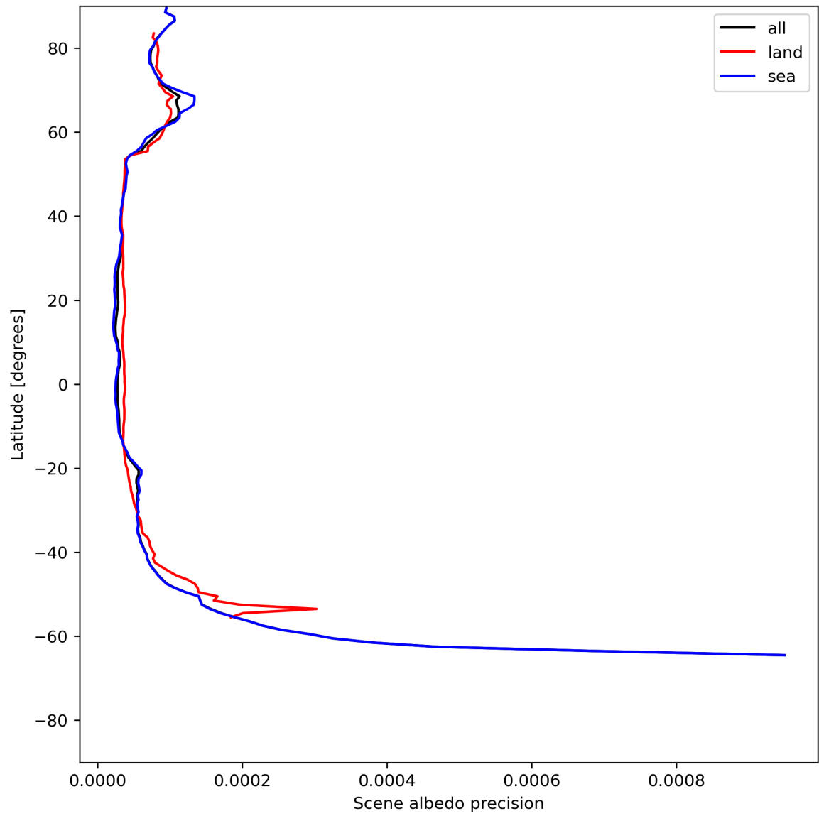
Figure 18: Zonal average of “Scene albedo precision” for 2024-06-20 to 2024-06-22.
