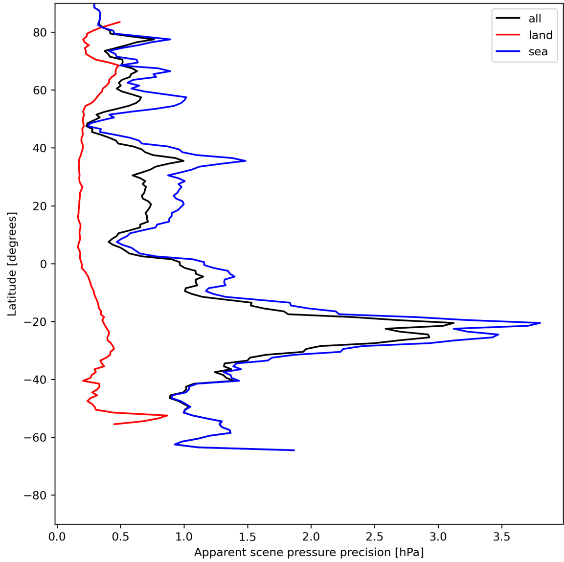
Figure 20: Zonal average of “Apparent scene pressure precision” for 2024-06-20 to 2024-06-22.
