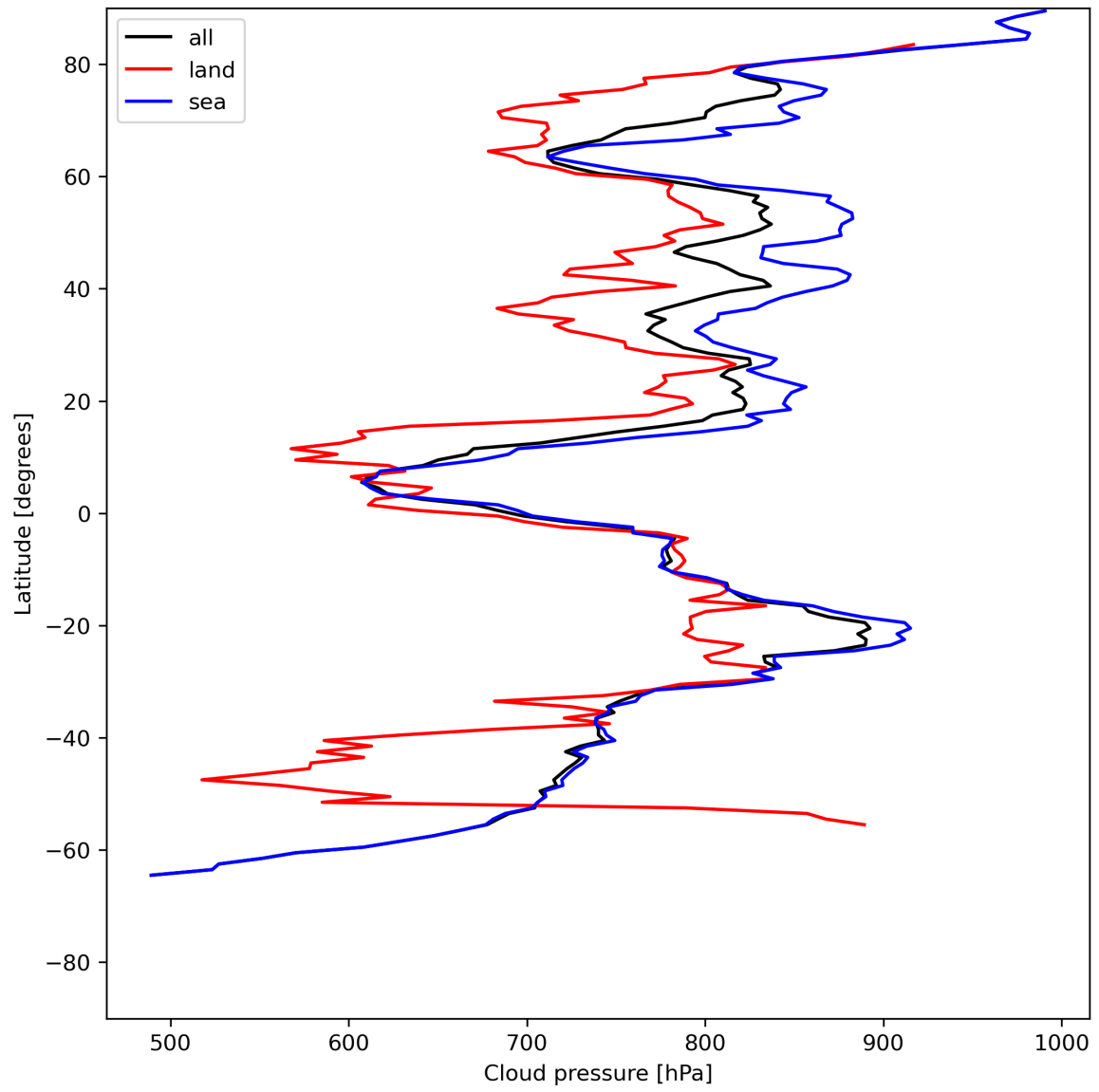
Figure 13: Zonal average of “Cloud pressure” for 2024-06-20 to 2024-06-22.
