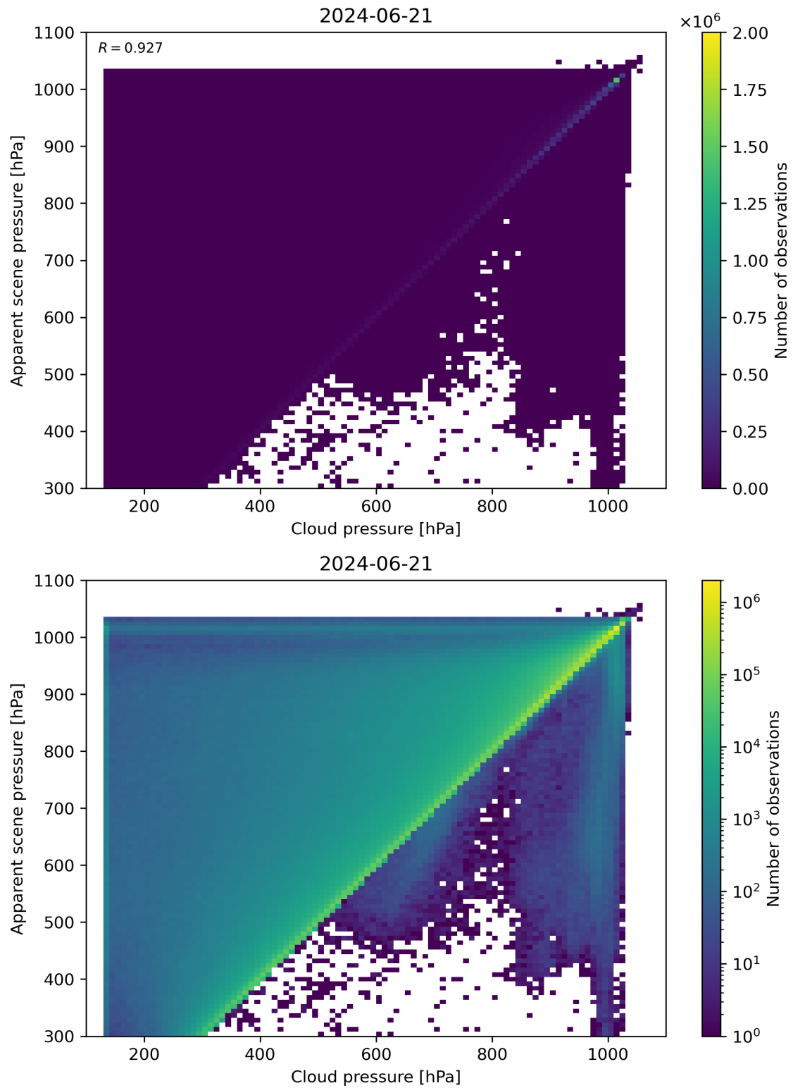
Figure 77: Scatter density plot of “Cloud pressure” against “Apparent scene pressure” for 2024-06-20 to 2024-06-22.
