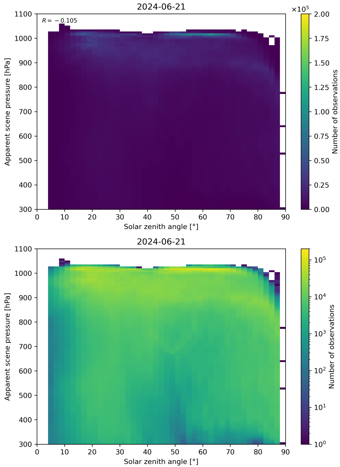
Figure 108: Scatter density plot of “Solar zenith angle” against “Apparent scene pressure” for 2024-06-20 to 2024-06-22.
