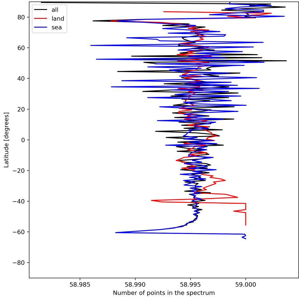
Figure 27: Zonal average of “Number of points in the spectrum” for 2024-06-21 to 2024-06-23.
