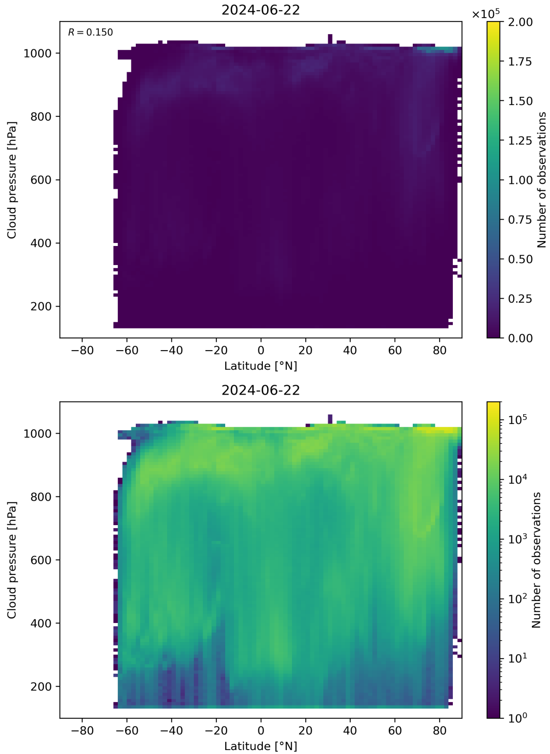
Figure 91: Scatter density plot of “Latitude” against “Cloud pressure” for 2024-06-21 to 2024-06-23.
