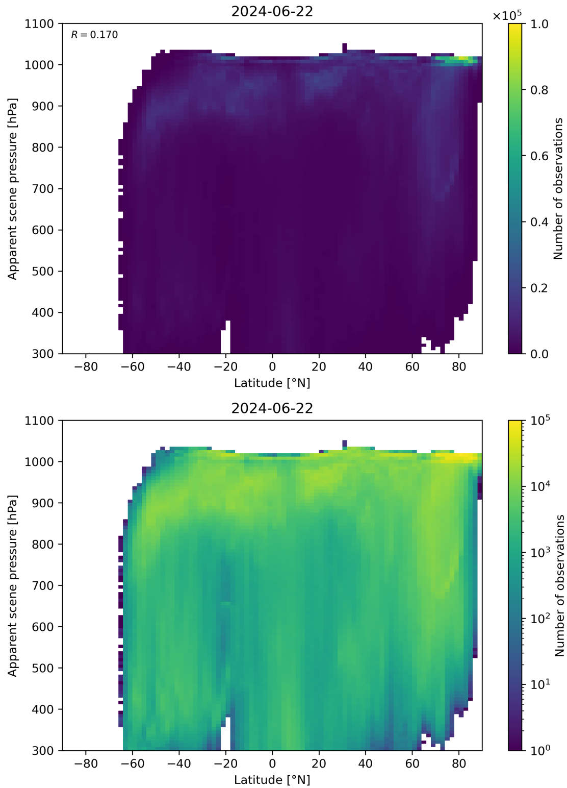
Figure 88: Scatter density plot of “Latitude” against “Apparent scene pressure” for 2024-06-21 to 2024-06-23.
