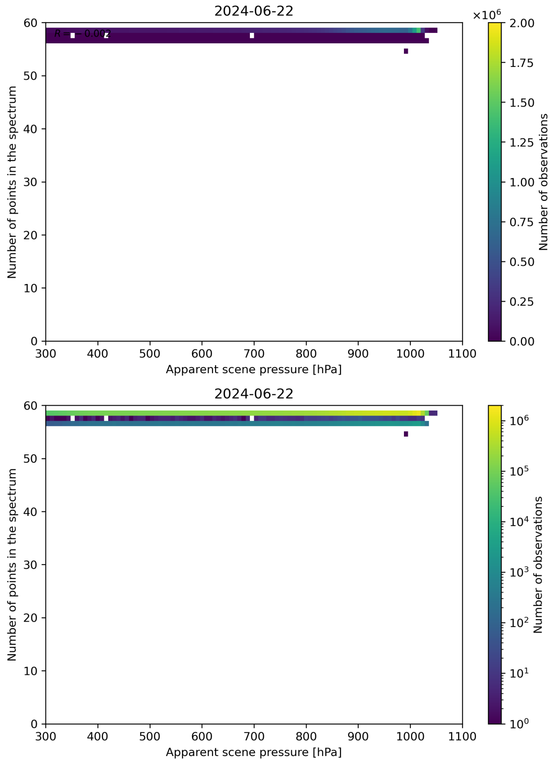
Figure 66: Scatter density plot of “Apparent scene pressure” against “Number of points in the spectrum” for 2024-06-21 to 2024-06-23.
