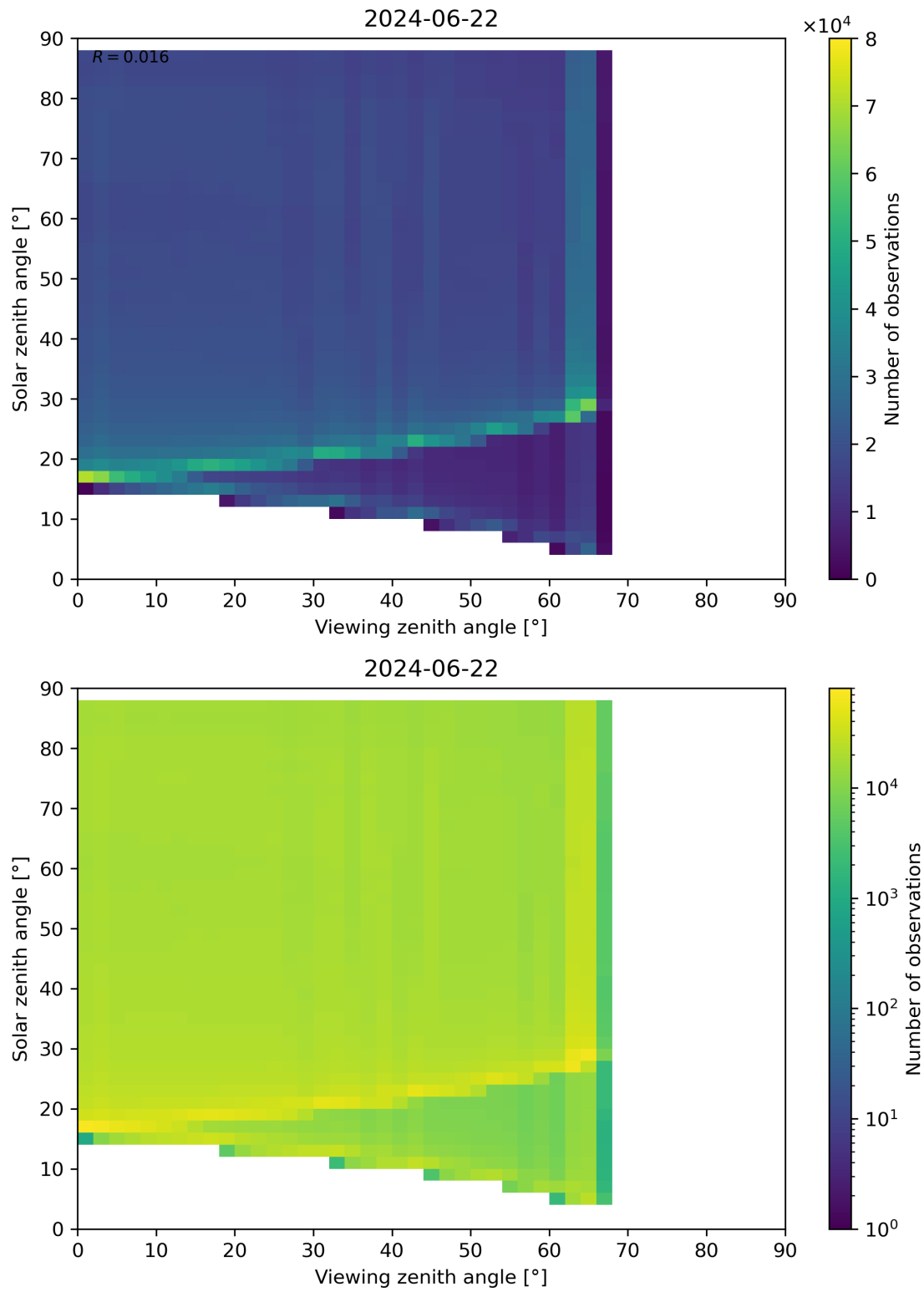
Figure 127: Scatter density plot of “Viewing zenith angle” against “Solar zenith angle” for 2024-06-21 to 2024-06-23.
