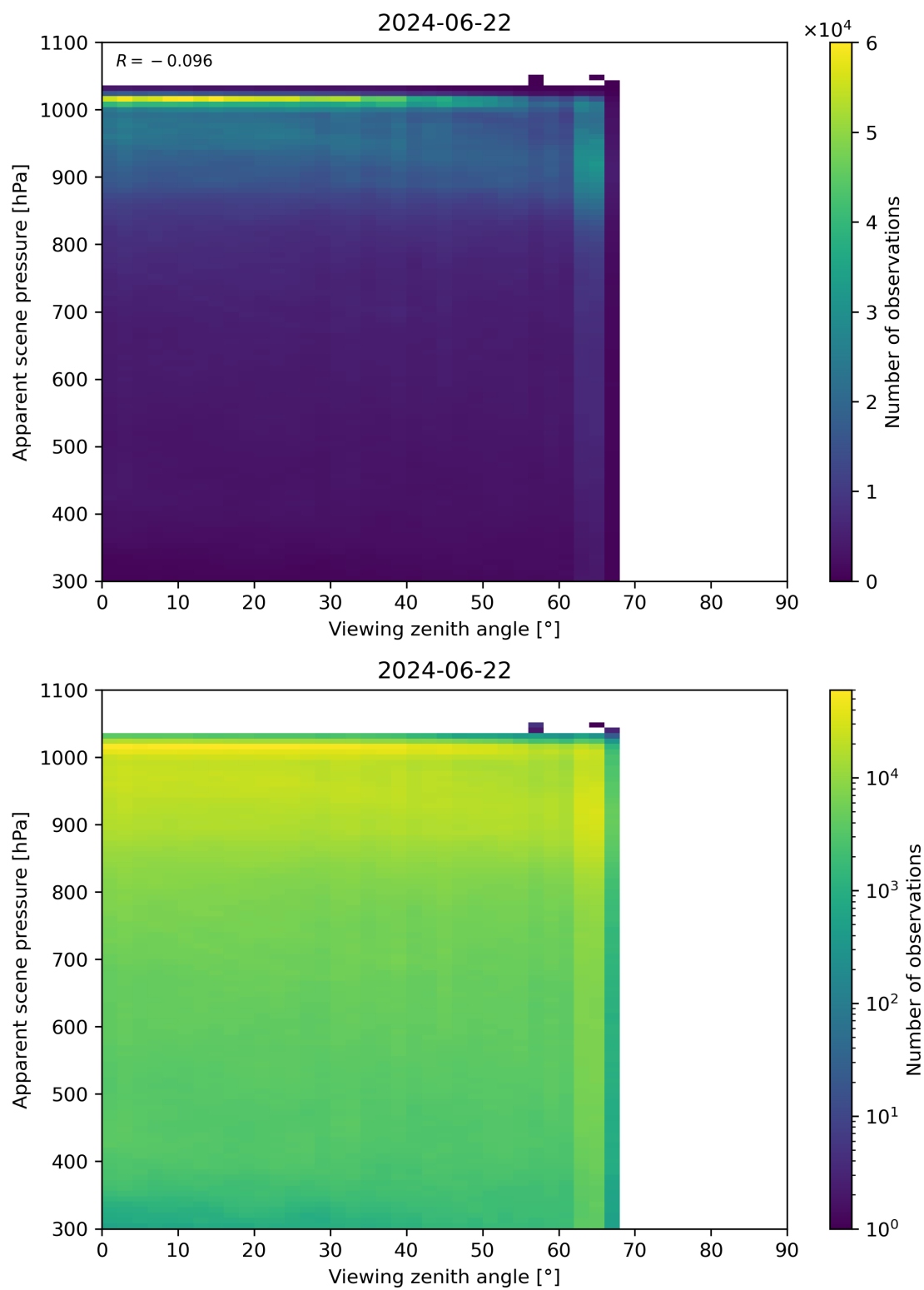
Figure 118: Scatter density plot of “Viewing zenith angle” against “Apparent scene pressure” for 2024-06-21 to 2024-06-23.
