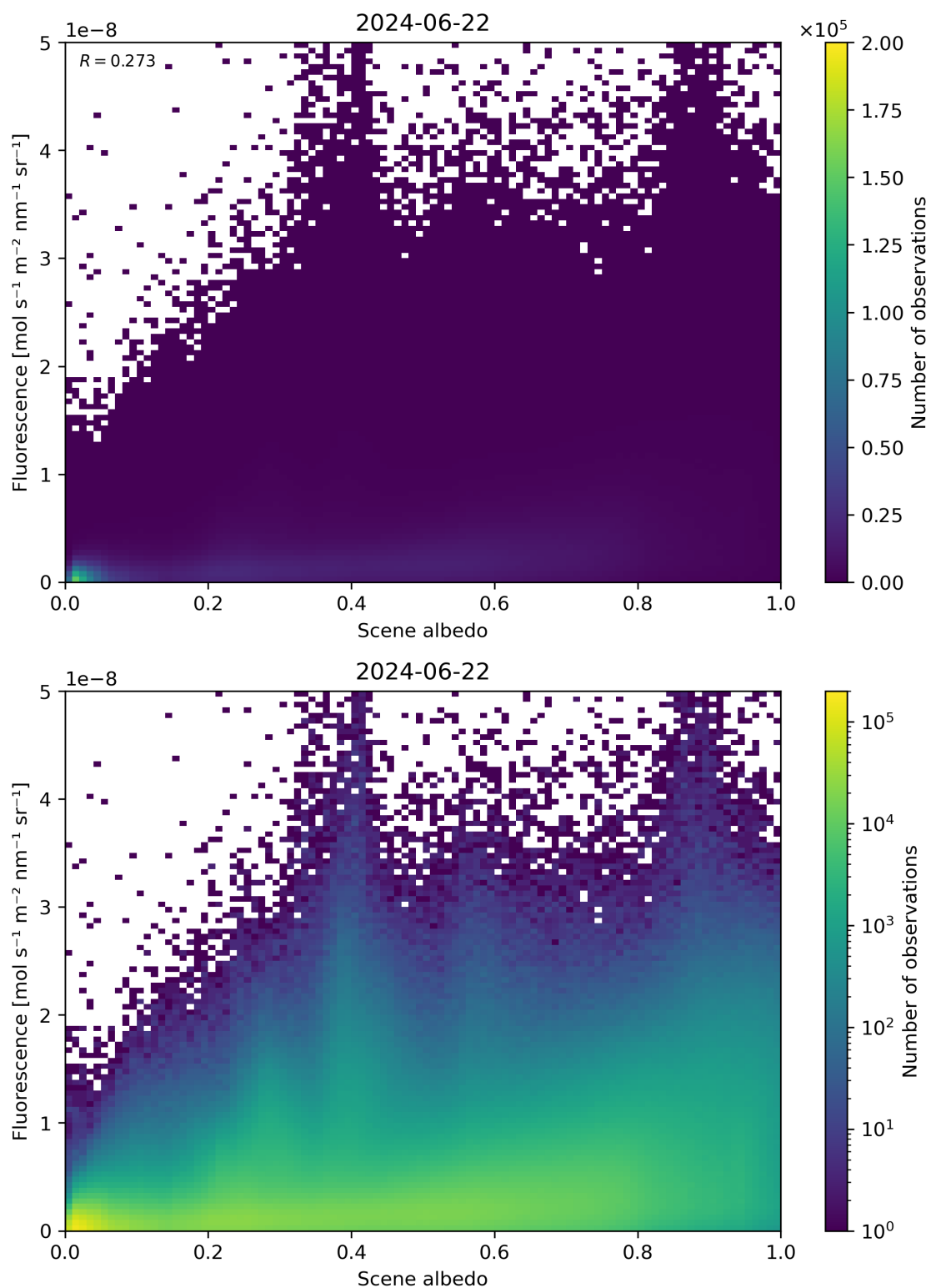
Figure 104: Scatter density plot of “Scene albedo” against “Fluorescence” for 2024-06-21 to 2024-06-23.
