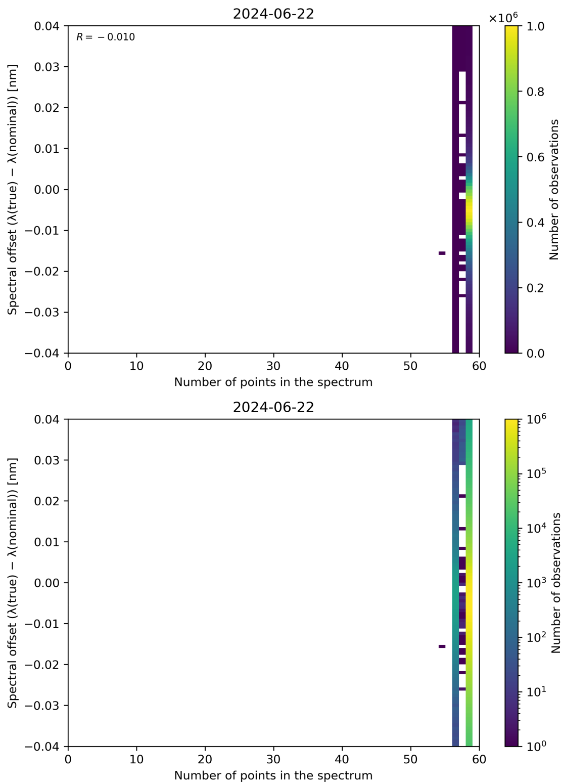
Figure 101: Scatter density plot of “Number of points in the spectrum” against “Spectral offset ( \lambda(\text{true}) - \lambda(\text{nominal}) )” for 2024-06-21 to 2024-06-23.
