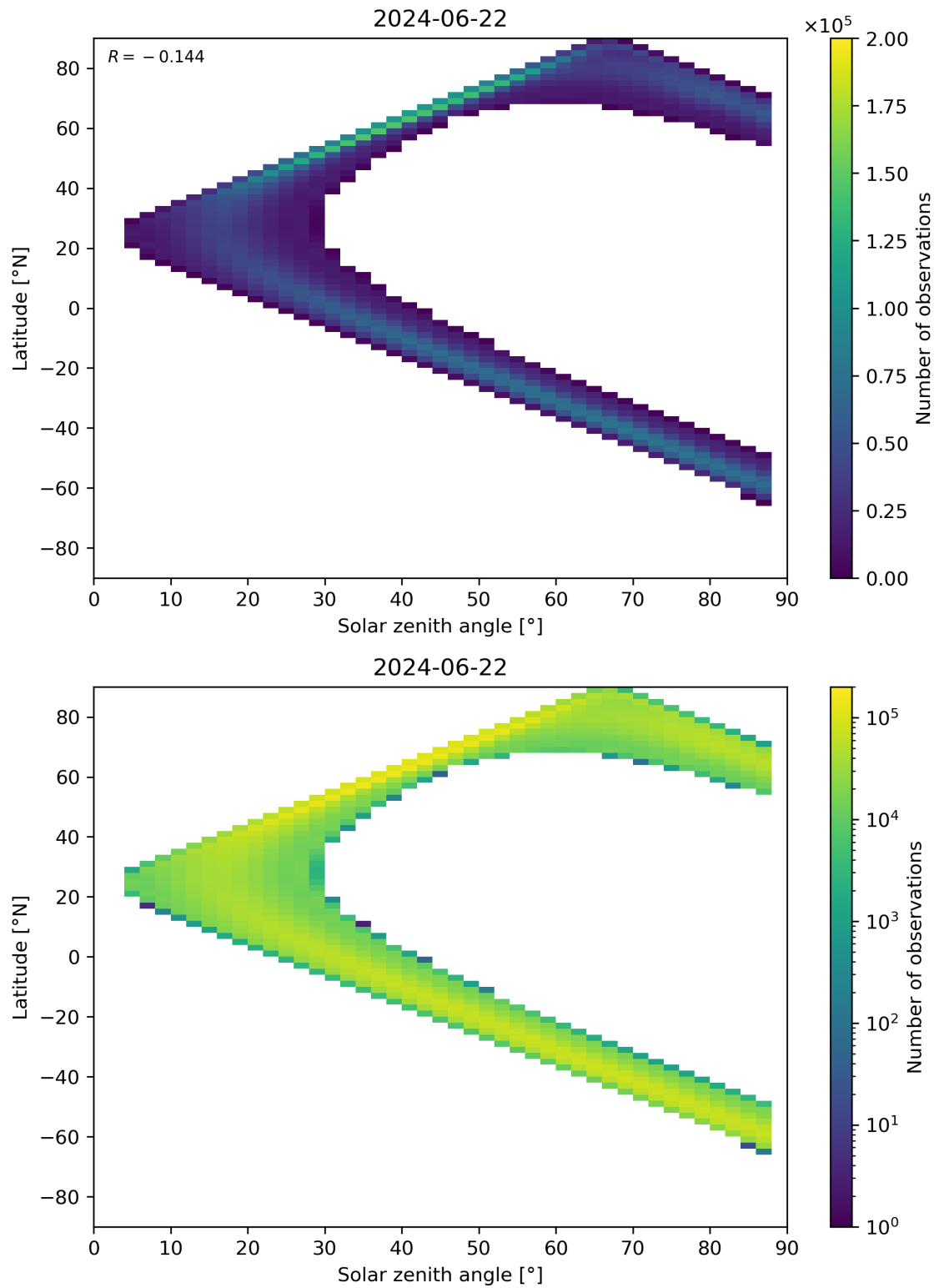
Figure 113: Scatter density plot of “Solar zenith angle” against “Latitude” for 2024-06-21 to 2024-06-23.
