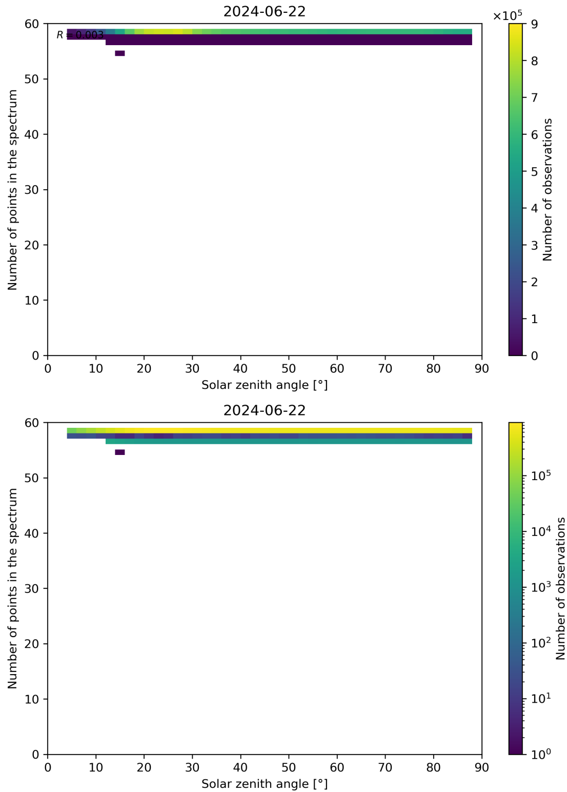
Figure 115: Scatter density plot of “Solar zenith angle” against “Number of points in the spectrum” for 2024-06-21 to 2024-06-23.
