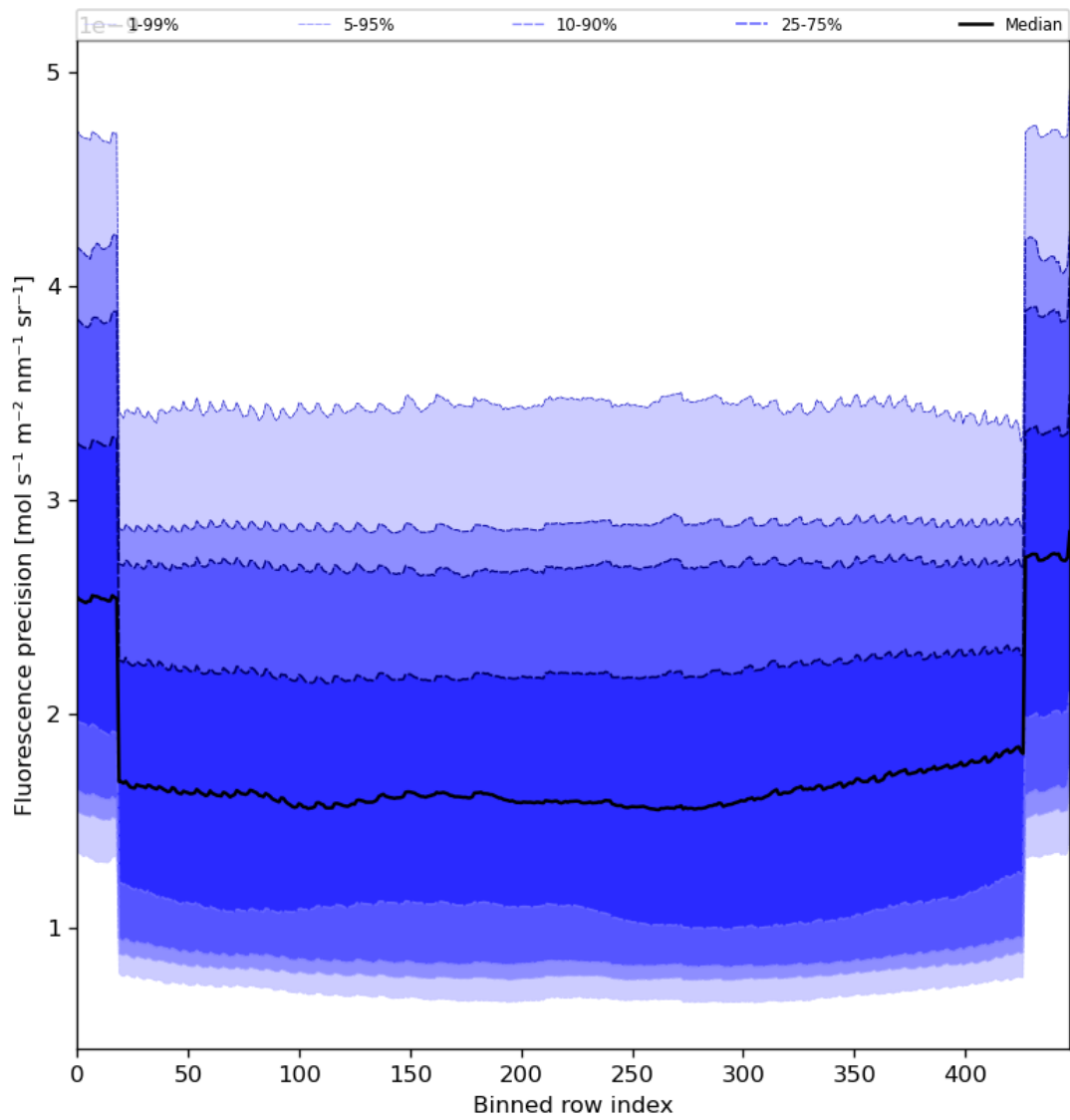
Figure 58: Along track statistics of “Fluorescence precision” for 2024-06-21 to 2024-06-23
