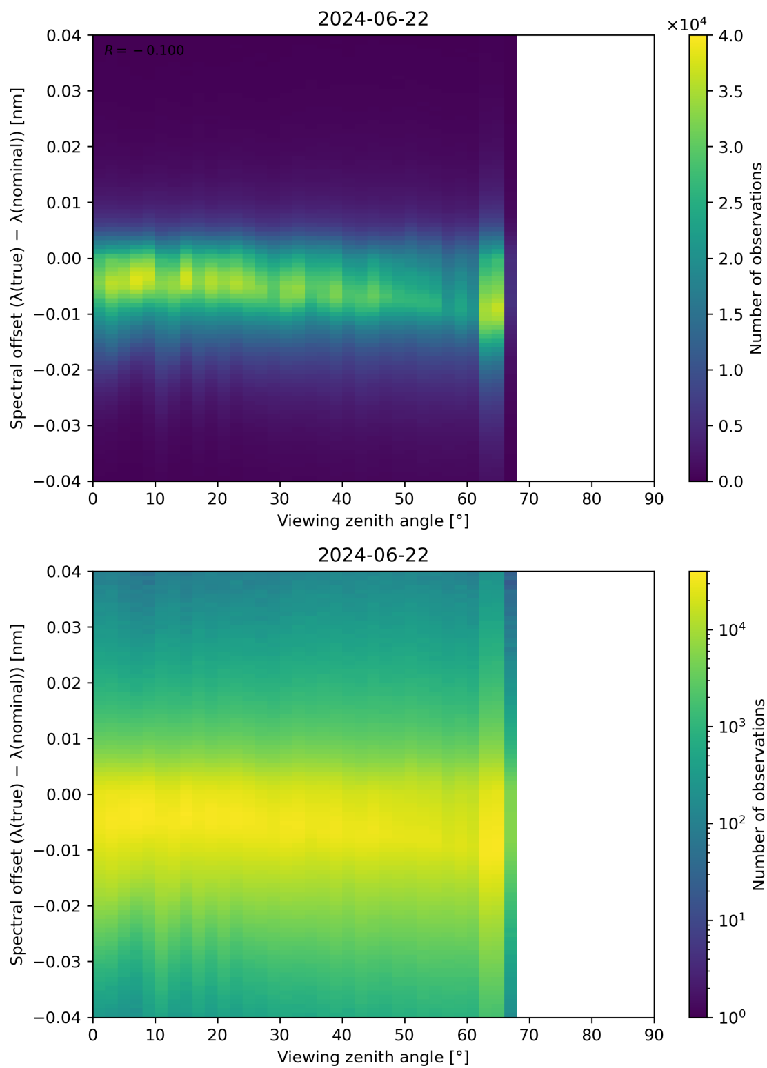
Figure 128: Scatter density plot of “Viewing zenith angle” against “Spectral offset ( \lambda(\text{true}) - \lambda(\text{nominal}) )” for 2024-06-21 to 2024-06-23.
