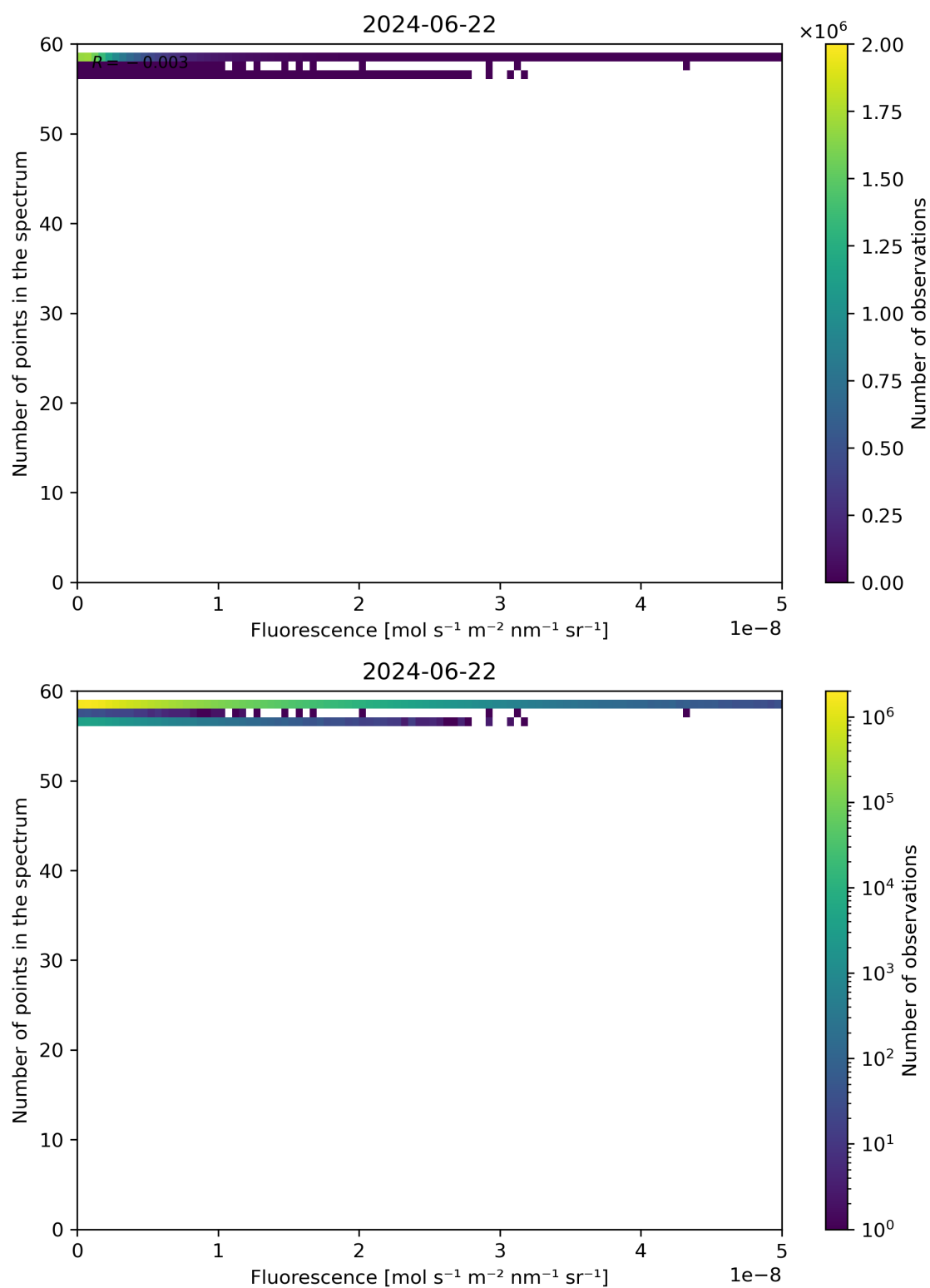
Figure 86: Scatter density plot of “Fluorescence” against “Number of points in the spectrum” for 2024-06-21 to 2024-06-23.
