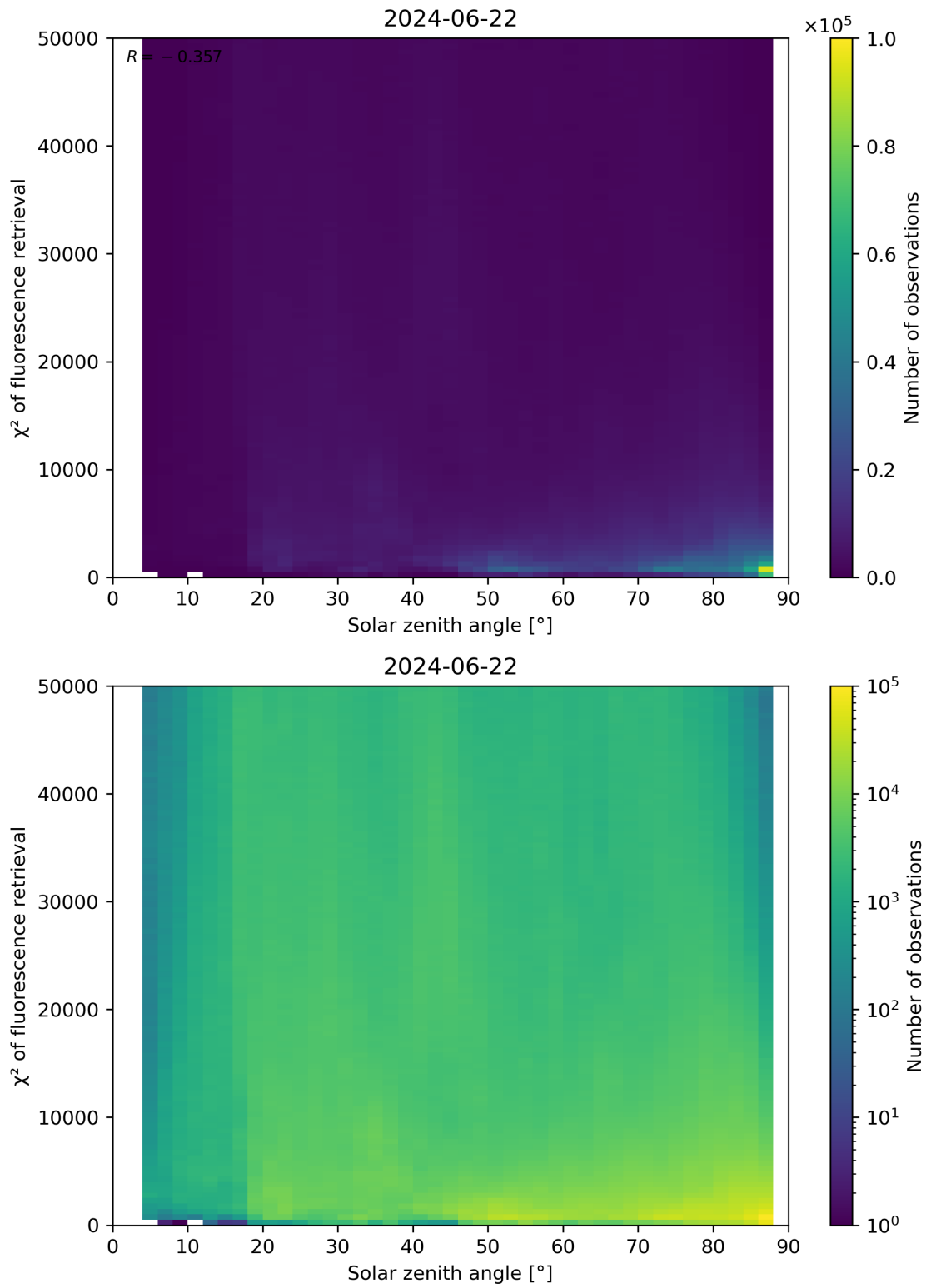
Figure 109: Scatter density plot of “Solar zenith angle” against “ \chi^2 of fluorescence retrieval” for 2024-06-21 to 2024-06-23.
