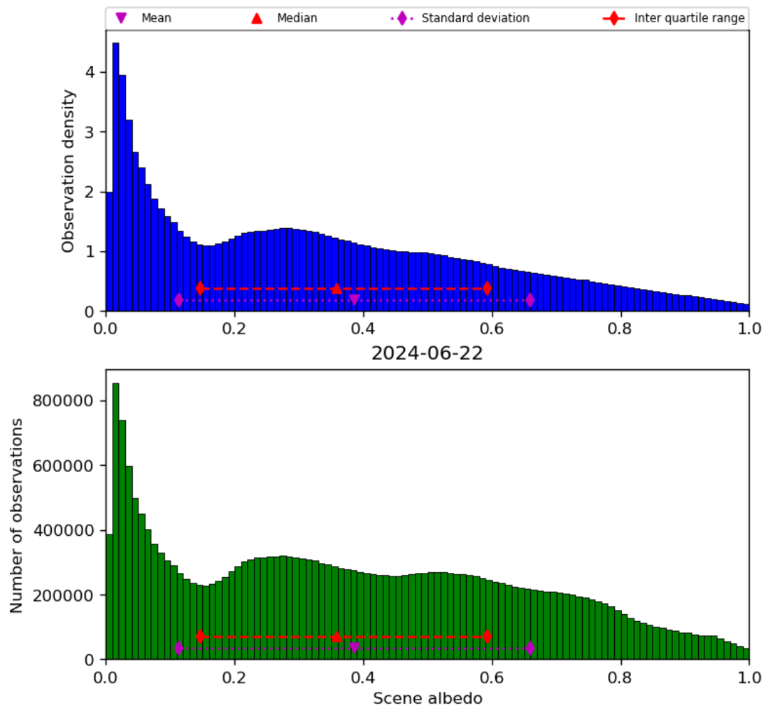
Figure 34: Histogram of “Scene albedo” for 2024-06-21 to 2024-06-23
