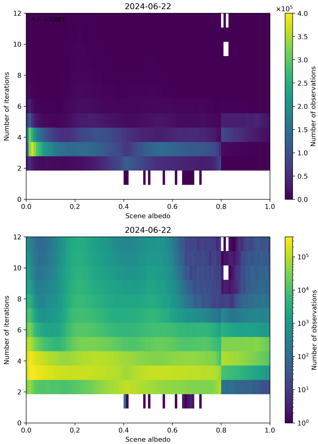
Figure 105: Scatter density plot of “Scene albedo” against “Number of iterations” for 2024-06-21 to 2024-06-23.
