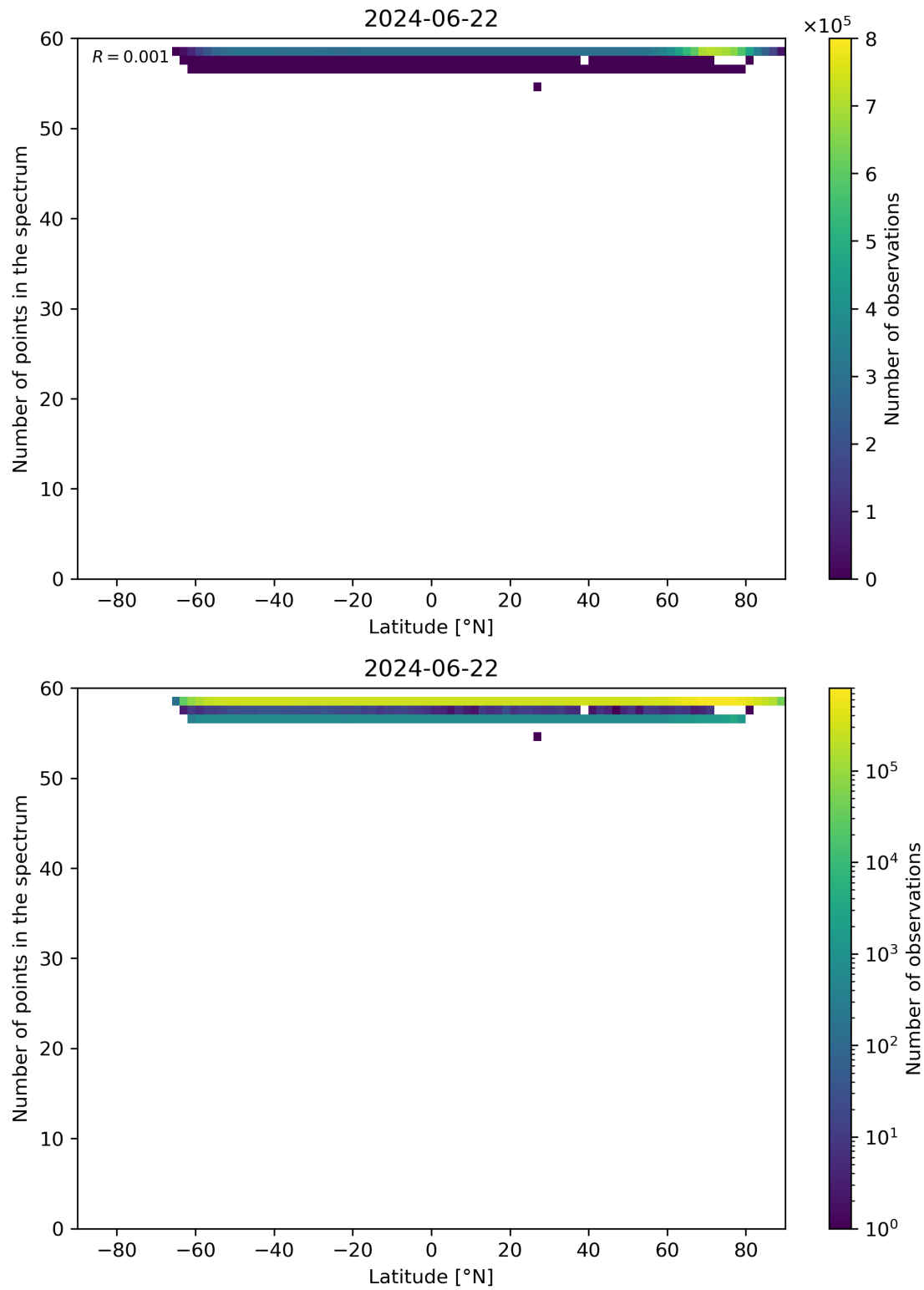
Figure 94: Scatter density plot of “Latitude” against “Number of points in the spectrum” for 2024-06-21 to 2024-06-23.
