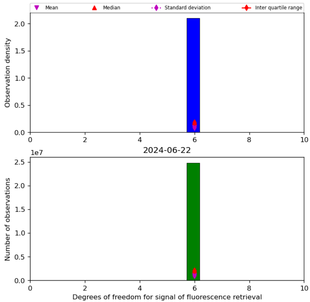
Figure 43: Histogram of “Degrees of freedom for signal of fluorescence retrieval” for 2024-06-21 to 2024-06-23
