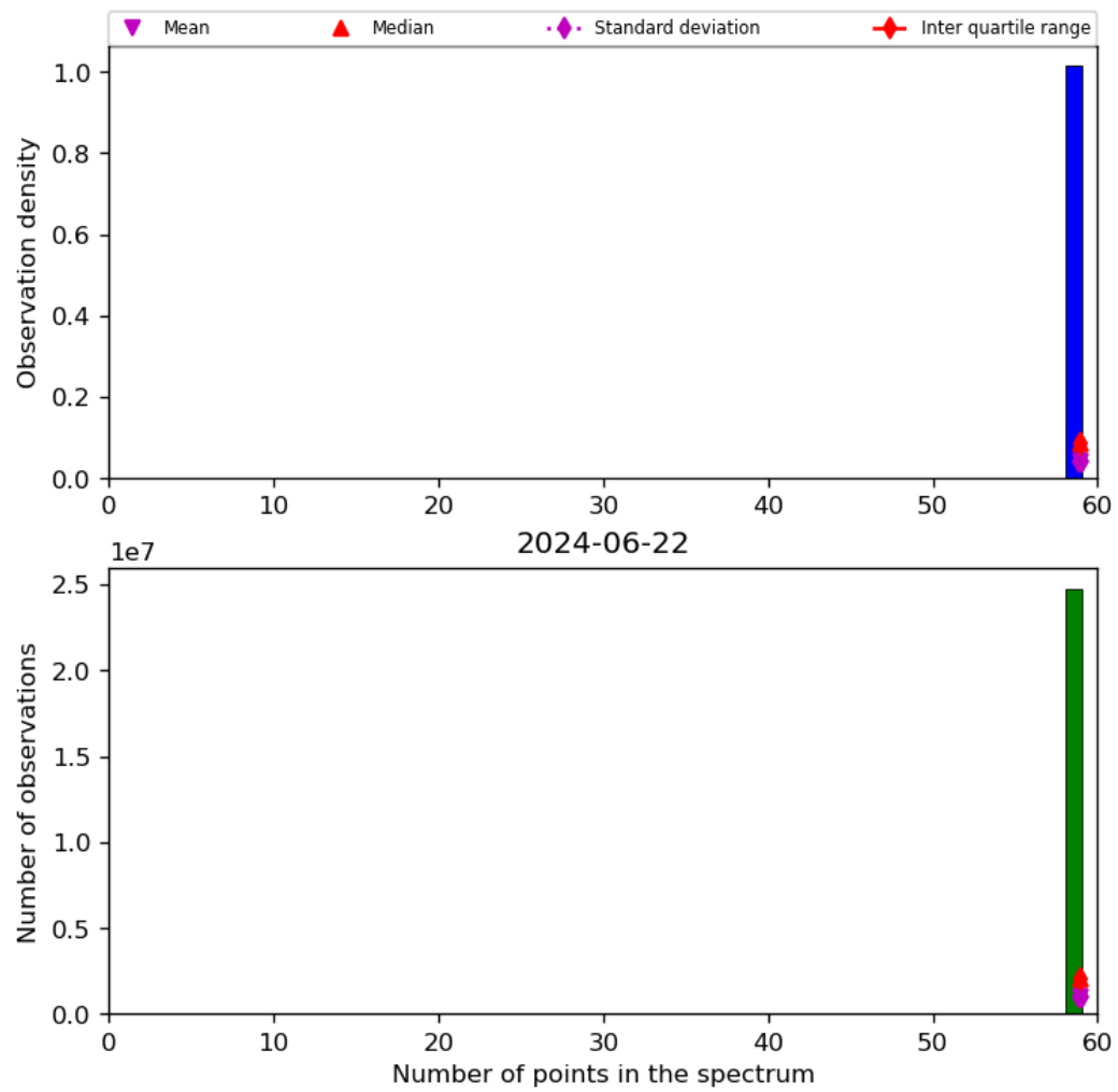
Figure 44: Histogram of “Number of points in the spectrum” for 2024-06-21 to 2024-06-23
