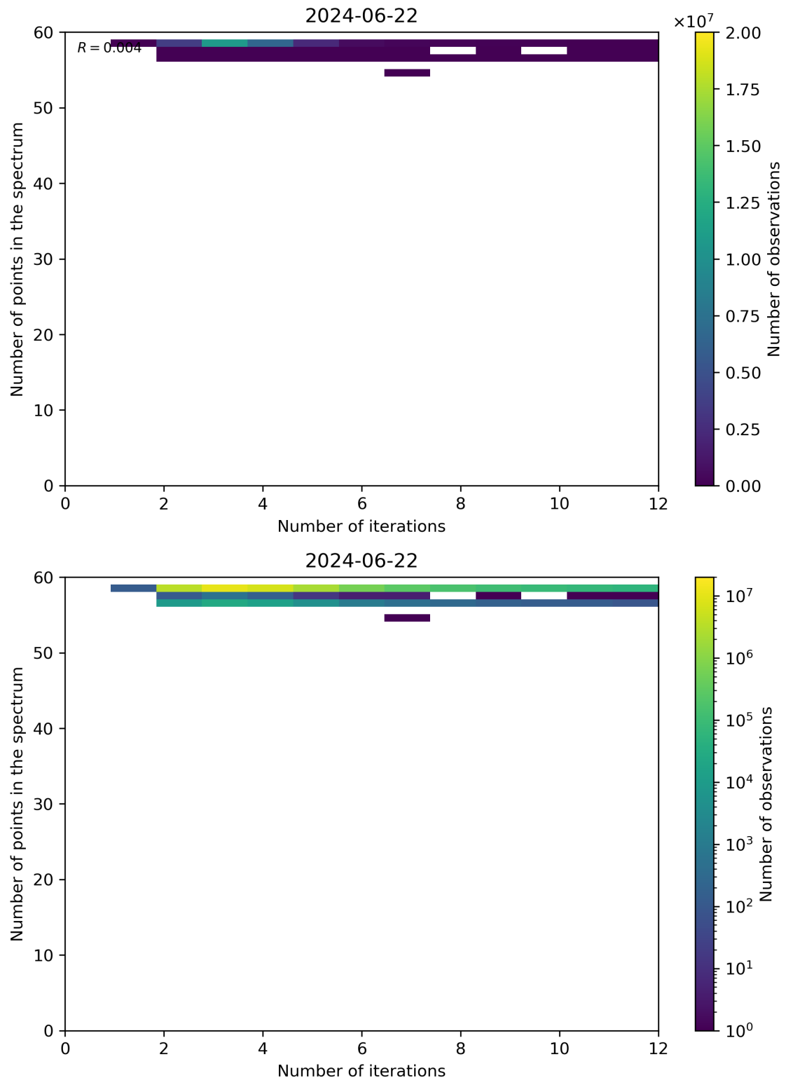
Figure 99: Scatter density plot of “Number of iterations” against “Number of points in the spectrum” for 2024-06-21 to 2024-06-23.
