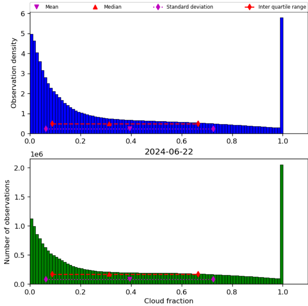
Figure 32: Histogram of “Cloud fraction” for 2024-06-21 to 2024-06-23
