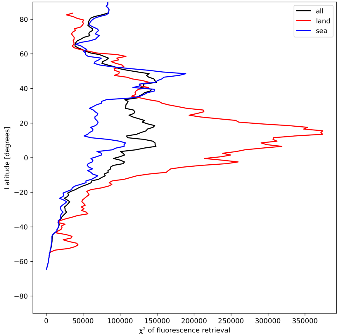
Figure 25: Zonal average of “ \chi^2 of fluorescence retrieval” for 2024-06-21 to 2024-06-23.
