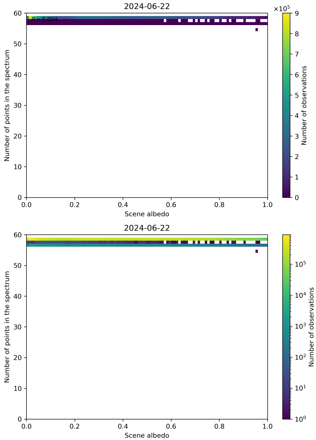
Figure 106: Scatter density plot of “Scene albedo” against “Number of points in the spectrum” for 2024-06-21 to 2024-06-23.
