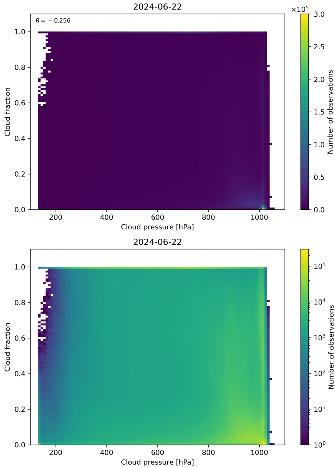
Figure 79: Scatter density plot of “Cloud pressure” against “Cloud fraction” for 2024-06-21 to 2024-06-23.
