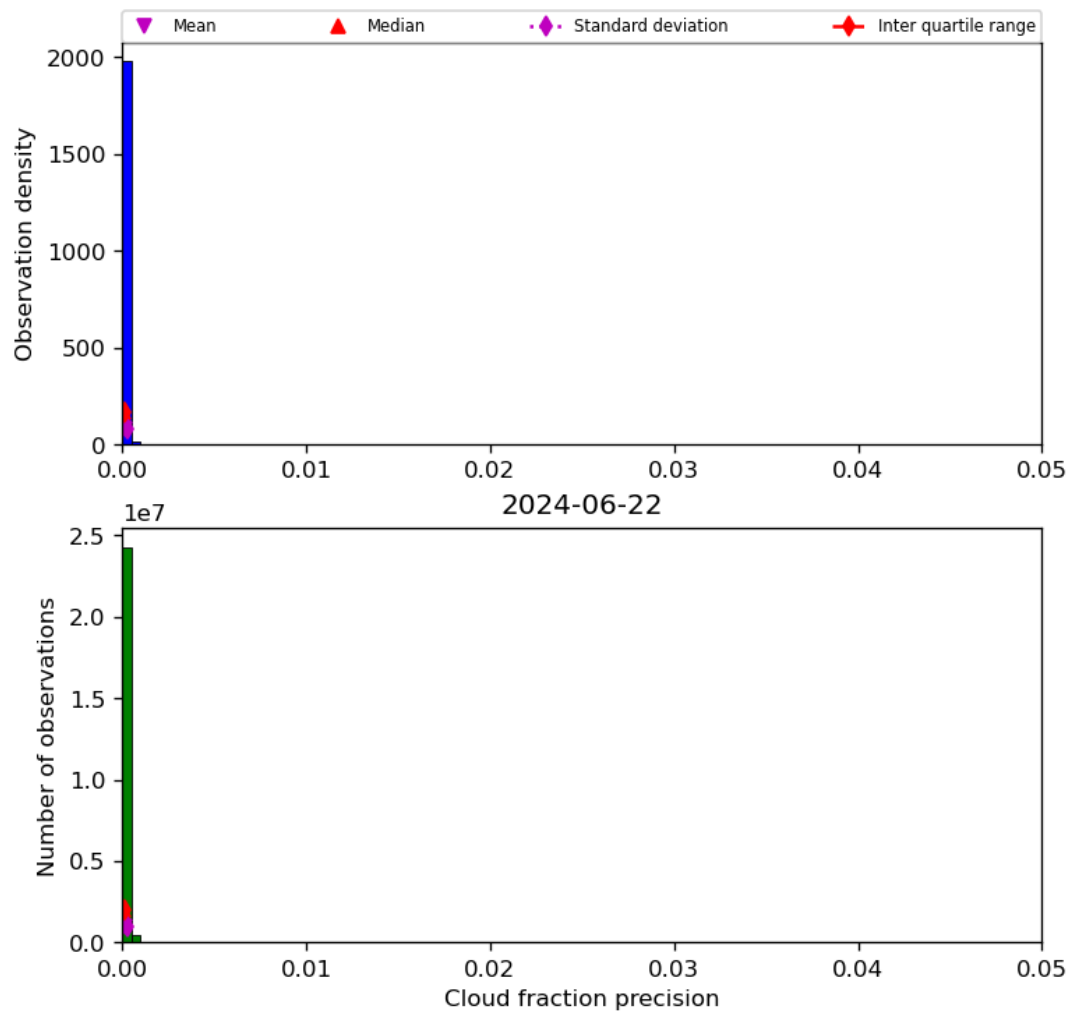
Figure 33: Histogram of “Cloud fraction precision” for 2024-06-21 to 2024-06-23
