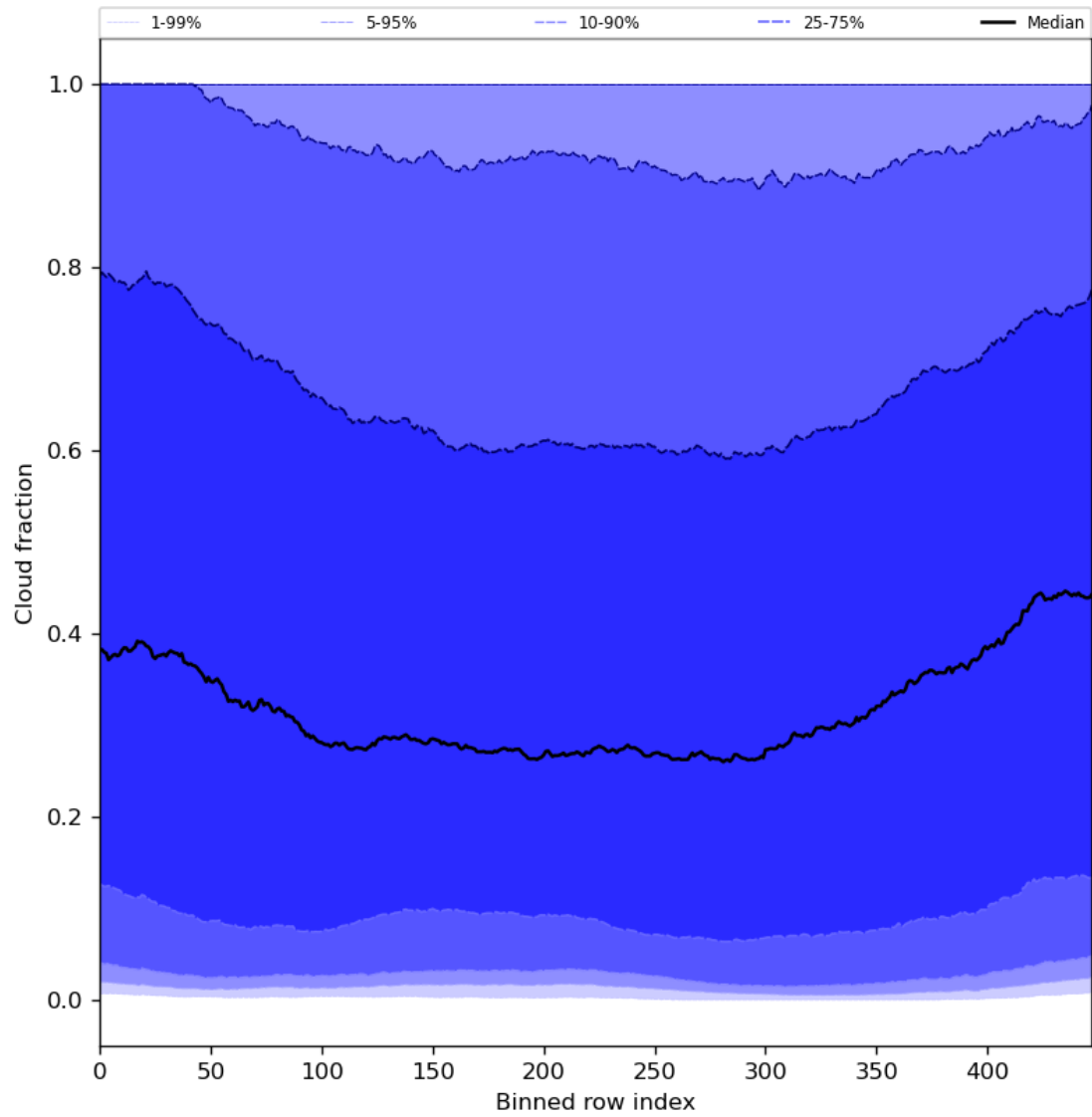
Figure 49: Along track statistics of “Cloud fraction” for 2024-06-21 to 2024-06-23
