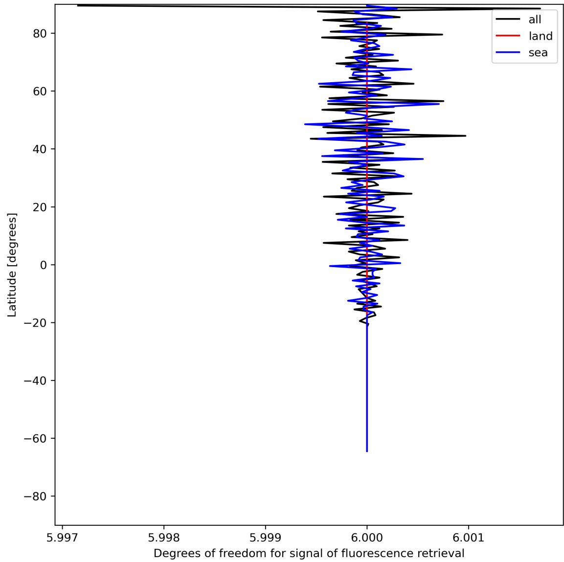
Figure 26: Zonal average of “Degrees of freedom for signal of fluorescence retrieval” for 2024-06-21 to 2024-06-23.
