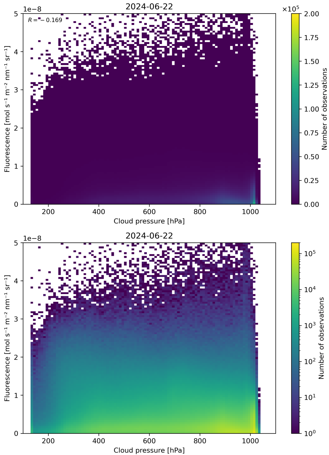
Figure 80: Scatter density plot of “Cloud pressure” against “Fluorescence” for 2024-06-21 to 2024-06-23.
