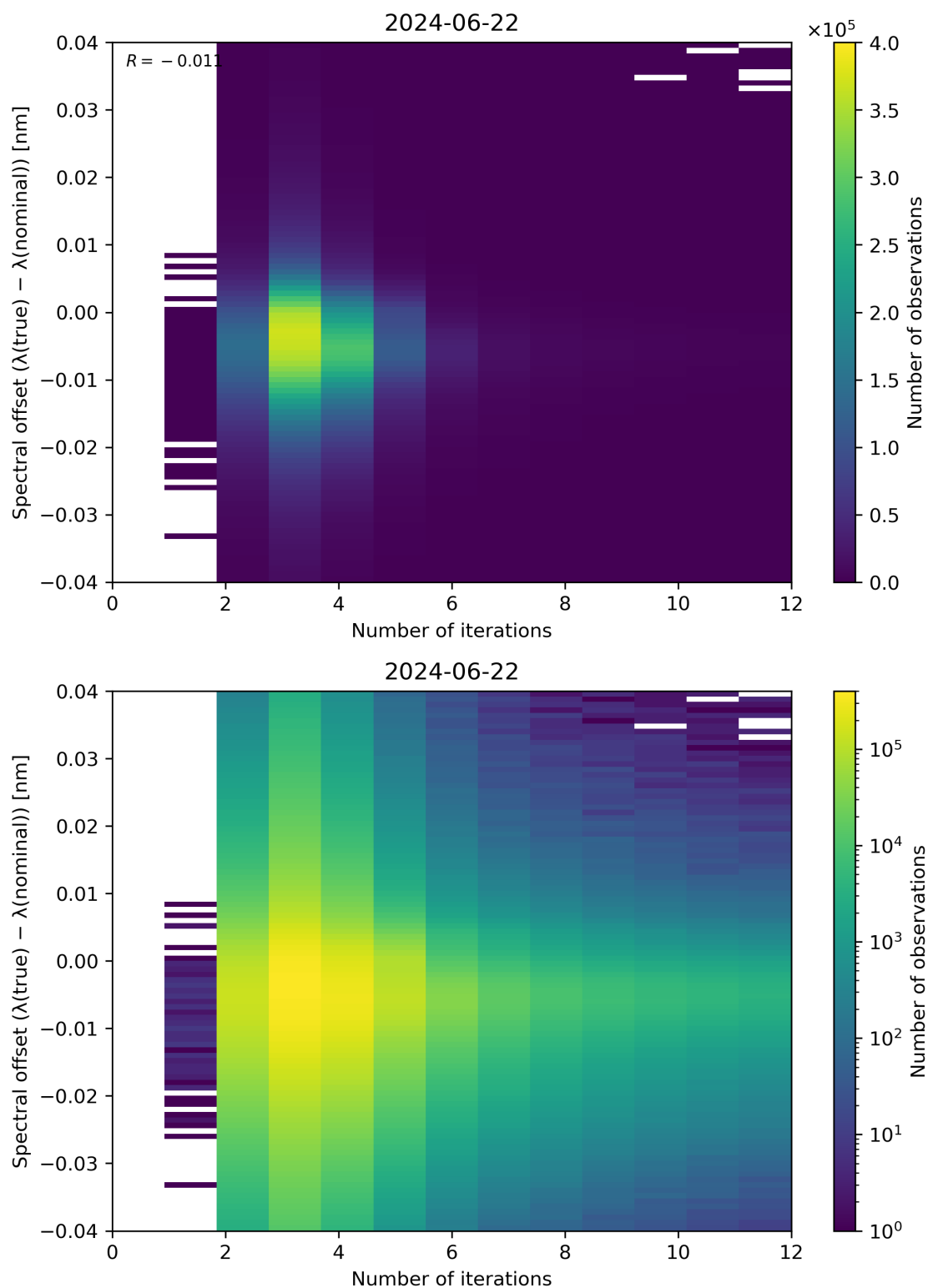
Figure 100: Scatter density plot of “Number of iterations” against “Spectral offset ( \lambda(\text{true}) - \lambda(\text{nominal}) )” for 2024-06-21 to 2024-06-23.
