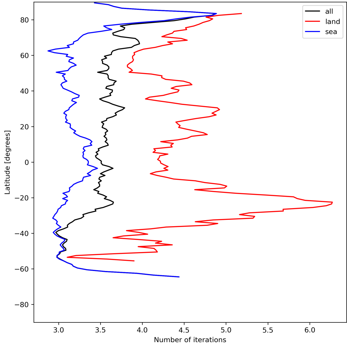
Figure 22: Zonal average of “Number of iterations” for 2024-06-21 to 2024-06-23.
