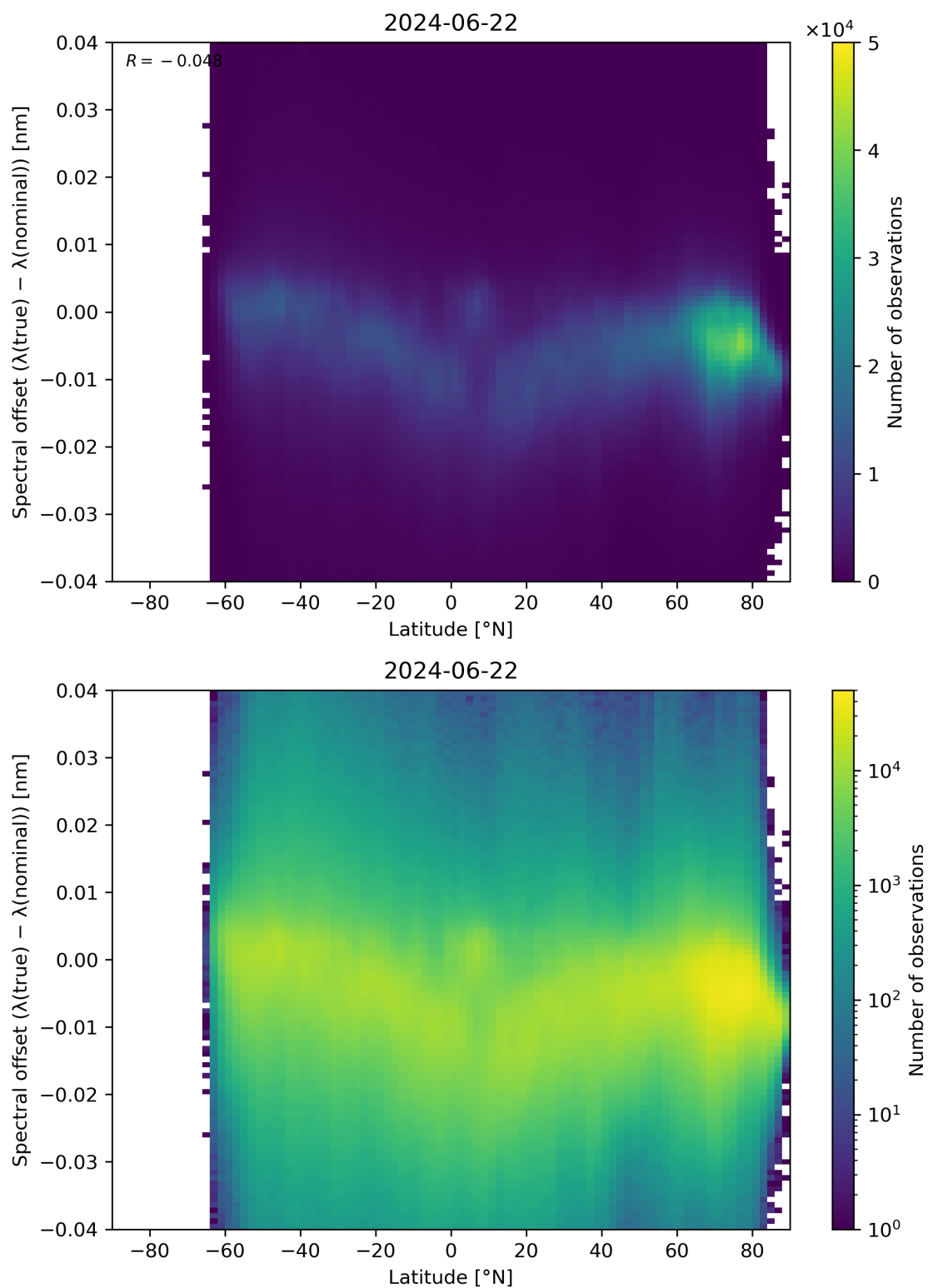
Figure 96: Scatter density plot of “Latitude” against “Spectral offset ( \lambda(\text{true}) - \lambda(\text{nominal}) )” for 2024-06-21 to 2024-06-23.
