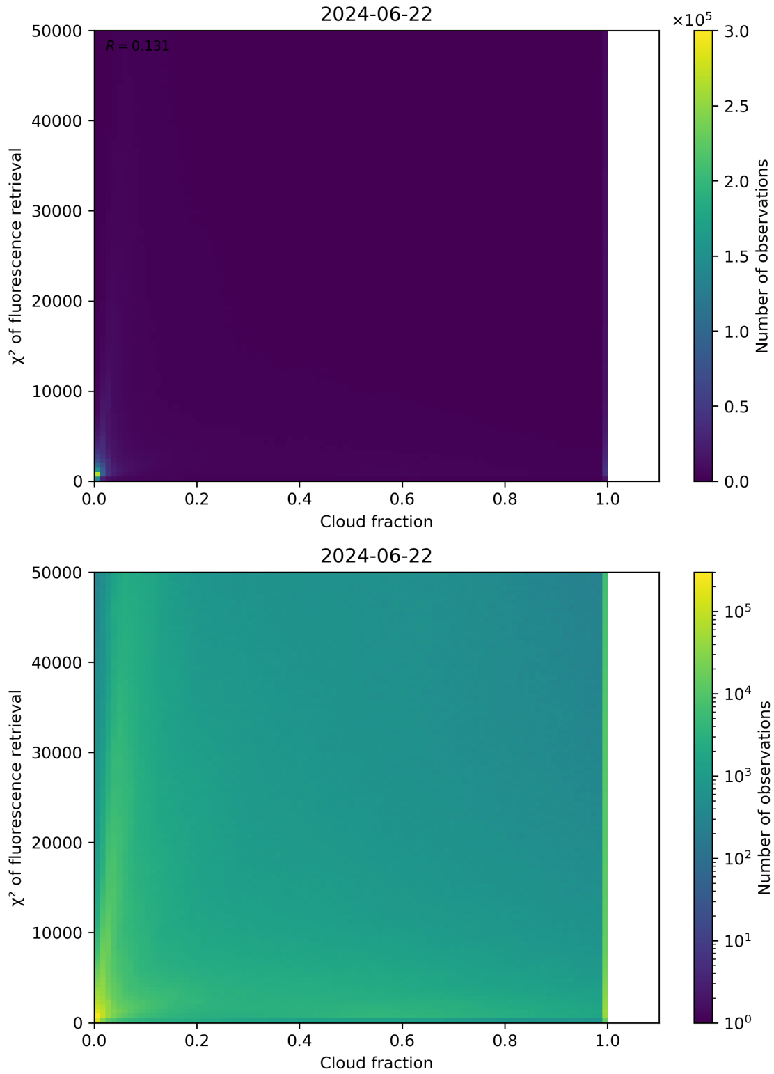
Figure 71: Scatter density plot of “Cloud fraction” against “ \chi^2 of fluorescence retrieval” for 2024-06-21 to 2024-06-23.
