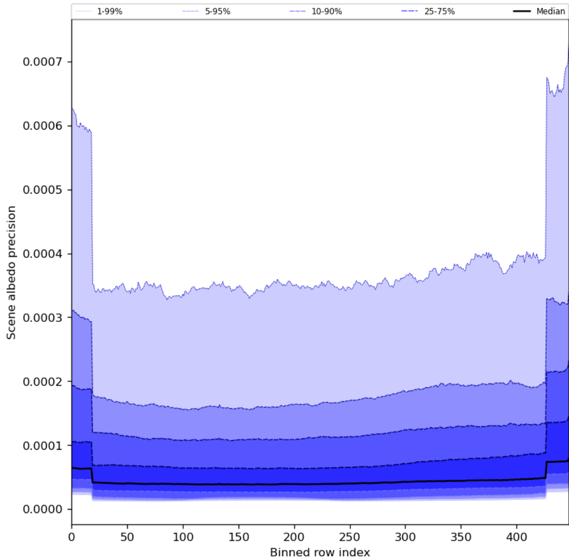
Figure 52: Along track statistics of “Scene albedo precision” for 2024-06-21 to 2024-06-23
