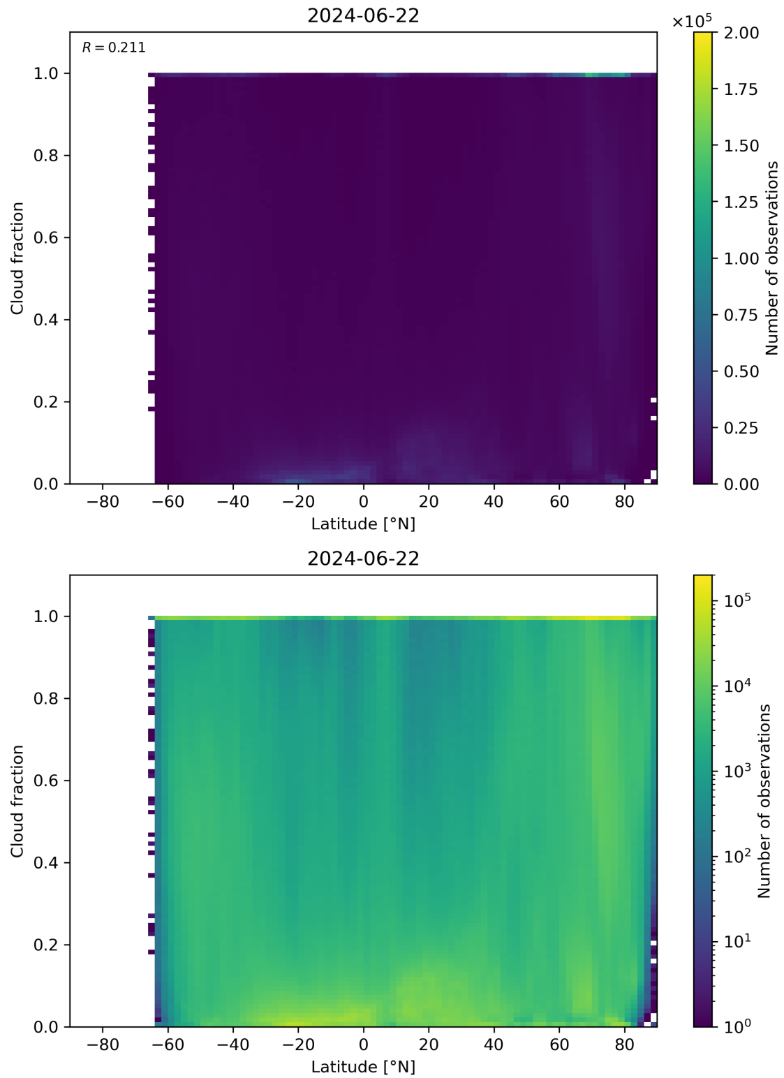
Figure 90: Scatter density plot of “Latitude” against “Cloud fraction” for 2024-06-21 to 2024-06-23.
