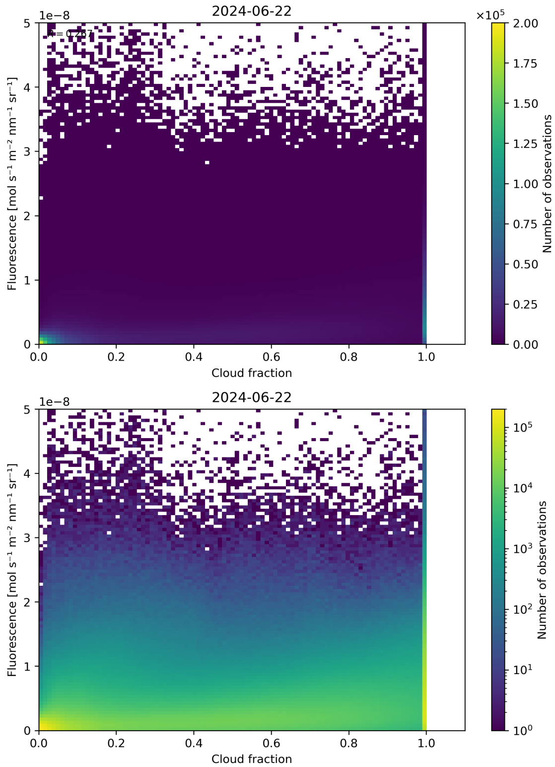
Figure 72: Scatter density plot of “Cloud fraction” against “Fluorescence” for 2024-06-21 to 2024-06-23.
