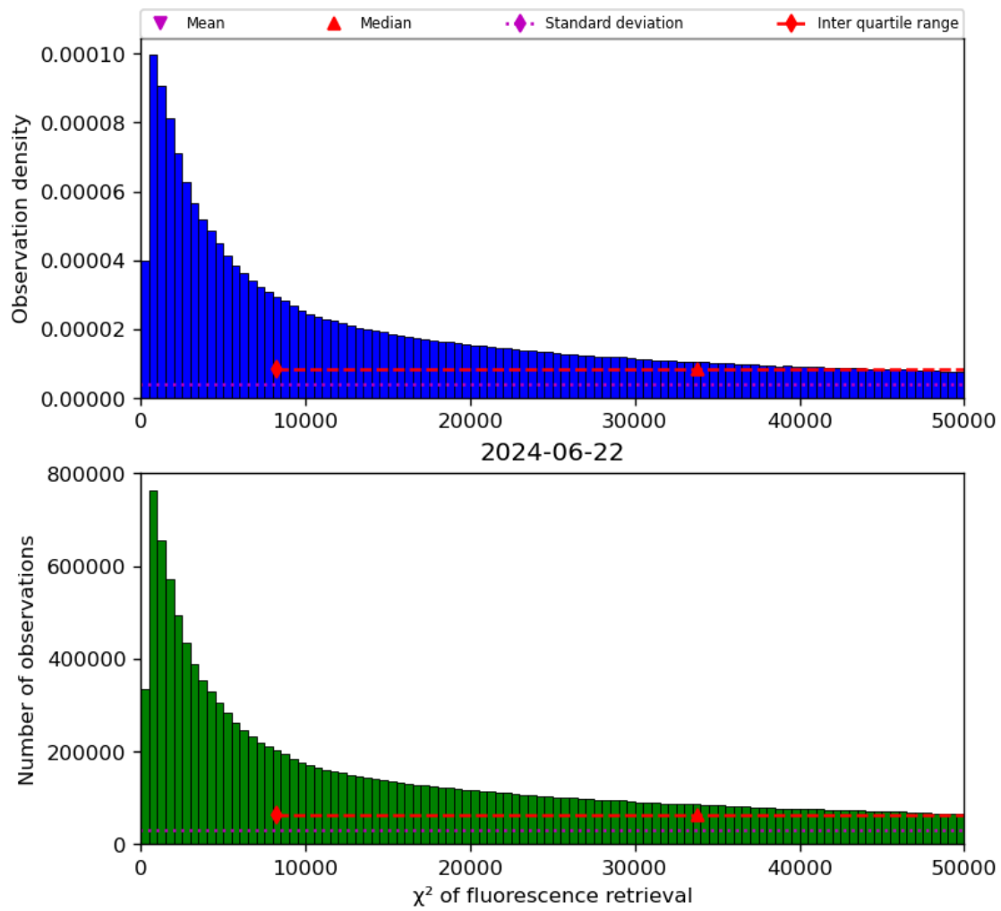
Figure 42: Histogram of “ \chi^2 of fluorescence retrieval” for 2024-06-21 to 2024-06-23
