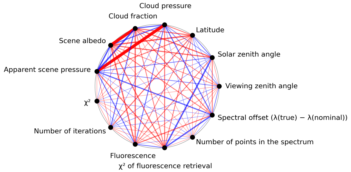
Figure 1: Map of correlation graph for 2024-06-21 to 2024-06-23.
