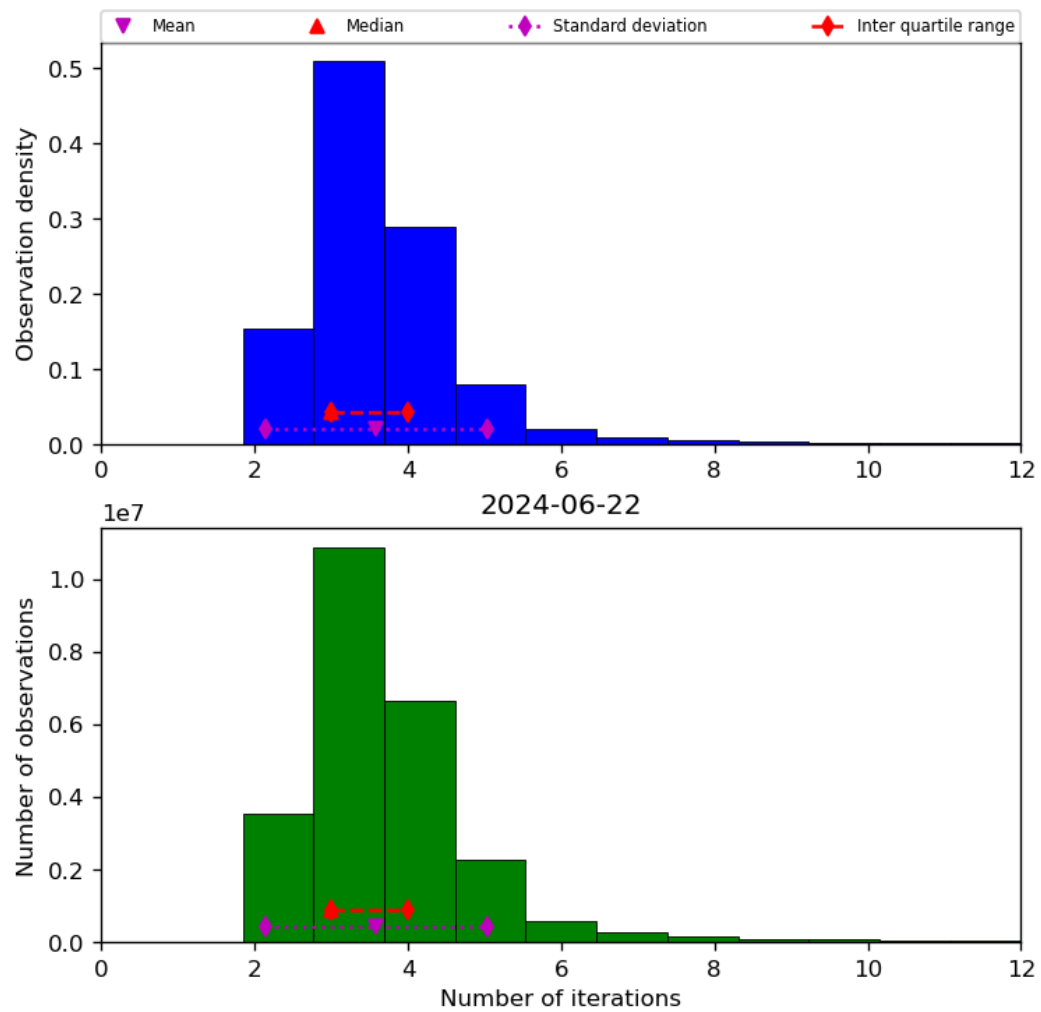
Figure 39: Histogram of “Number of iterations” for 2024-06-21 to 2024-06-23
