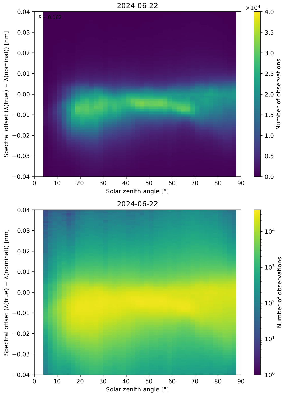
Figure 117: Scatter density plot of “Solar zenith angle” against “Spectral offset ( \lambda(\text{true}) - \lambda(\text{nominal}) )” for 2024-06-21 to 2024-06-23.
