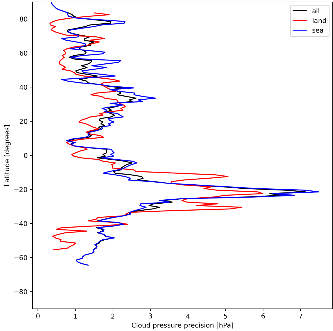
Figure 14: Zonal average of “Cloud pressure precision” for 2024-06-21 to 2024-06-23.
