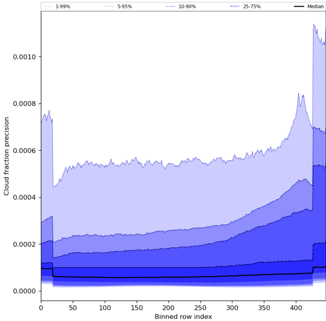
Figure 50: Along track statistics of “Cloud fraction precision” for 2024-06-21 to 2024-06-23
