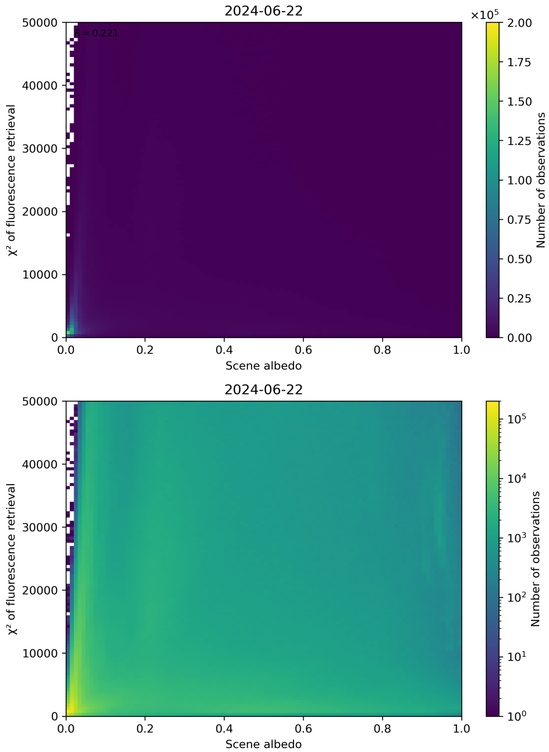
Figure 103: Scatter density plot of “Scene albedo” against “ \chi^2 of fluorescence retrieval” for 2024-06-21 to 2024-06-23.
