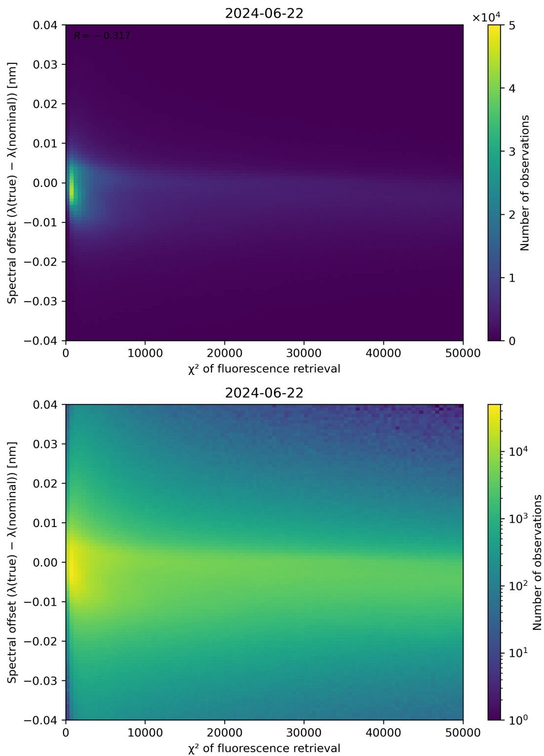
Figure 69: Scatter density plot of “ \chi^2 of fluorescence retrieval” against “Spectral offset ( \lambda(\text{true}) - \lambda(\text{nominal}) )” for 2024-06-21 to 2024-06-23.
