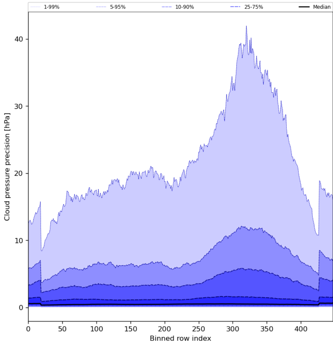
Figure 48: Along track statistics of “Cloud pressure precision” for 2024-06-21 to 2024-06-23
