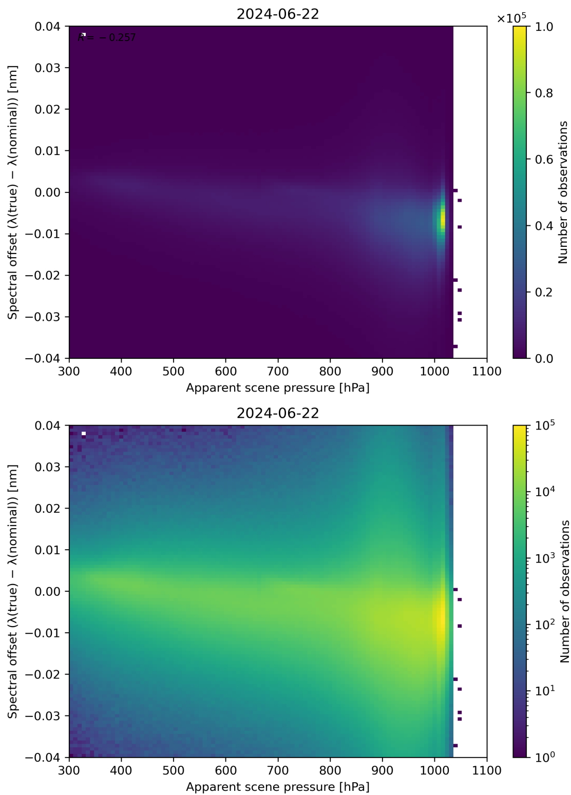
Figure 67: Scatter density plot of “Apparent scene pressure” against “Spectral offset ( \lambda(\text{true}) - \lambda(\text{nominal}) )” for 2024-06-21 to 2024-06-23.
