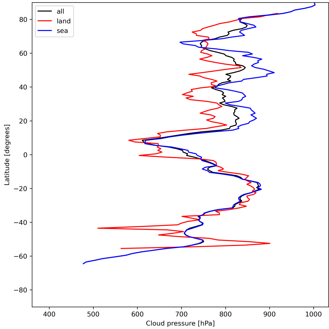
Figure 13: Zonal average of “Cloud pressure” for 2024-06-21 to 2024-06-23.
