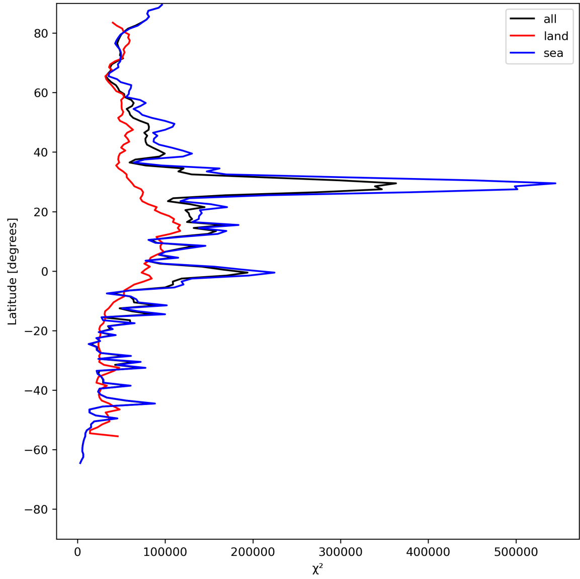
Figure 21: Zonal average of “ \chi^2 ” for 2024-06-21 to 2024-06-23.
