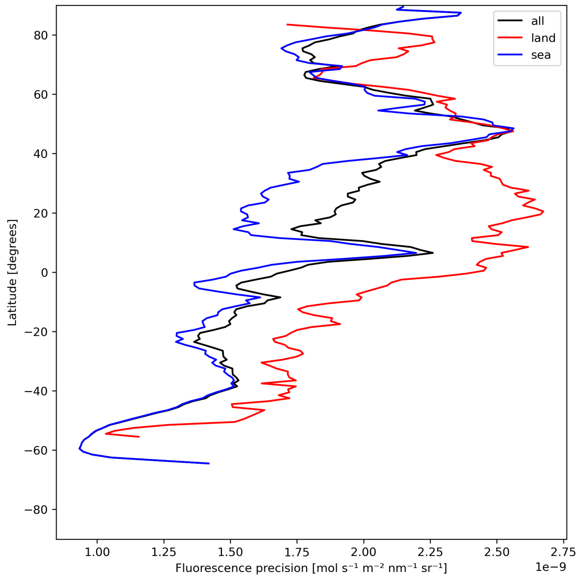
Figure 24: Zonal average of “Fluorescence precision” for 2024-06-21 to 2024-06-23.
