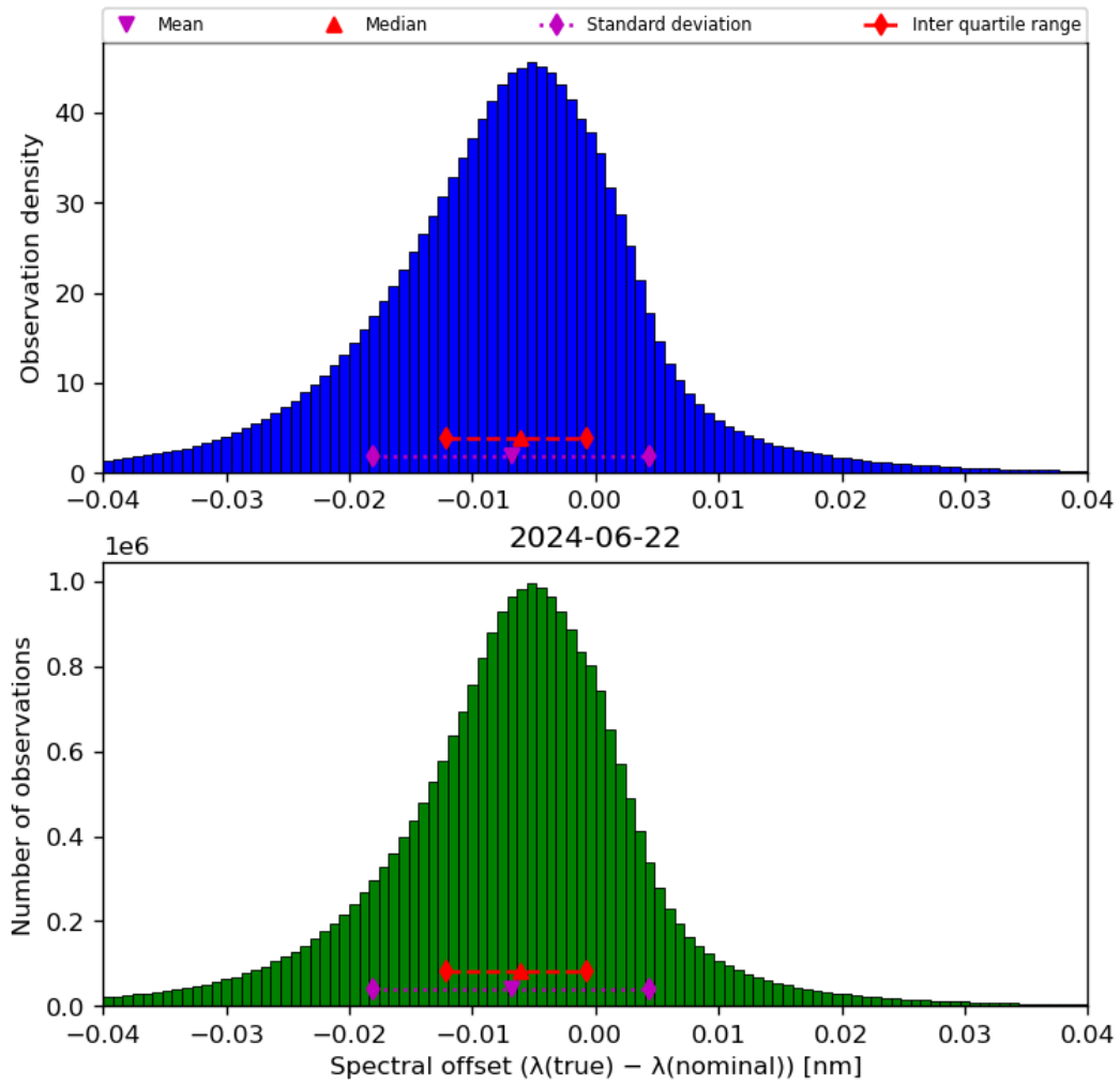
Figure 45: Histogram of “Spectral offset ( \lambda(\text{true}) - \lambda(\text{nominal}) )” for 2024-06-21 to 2024-06-23
