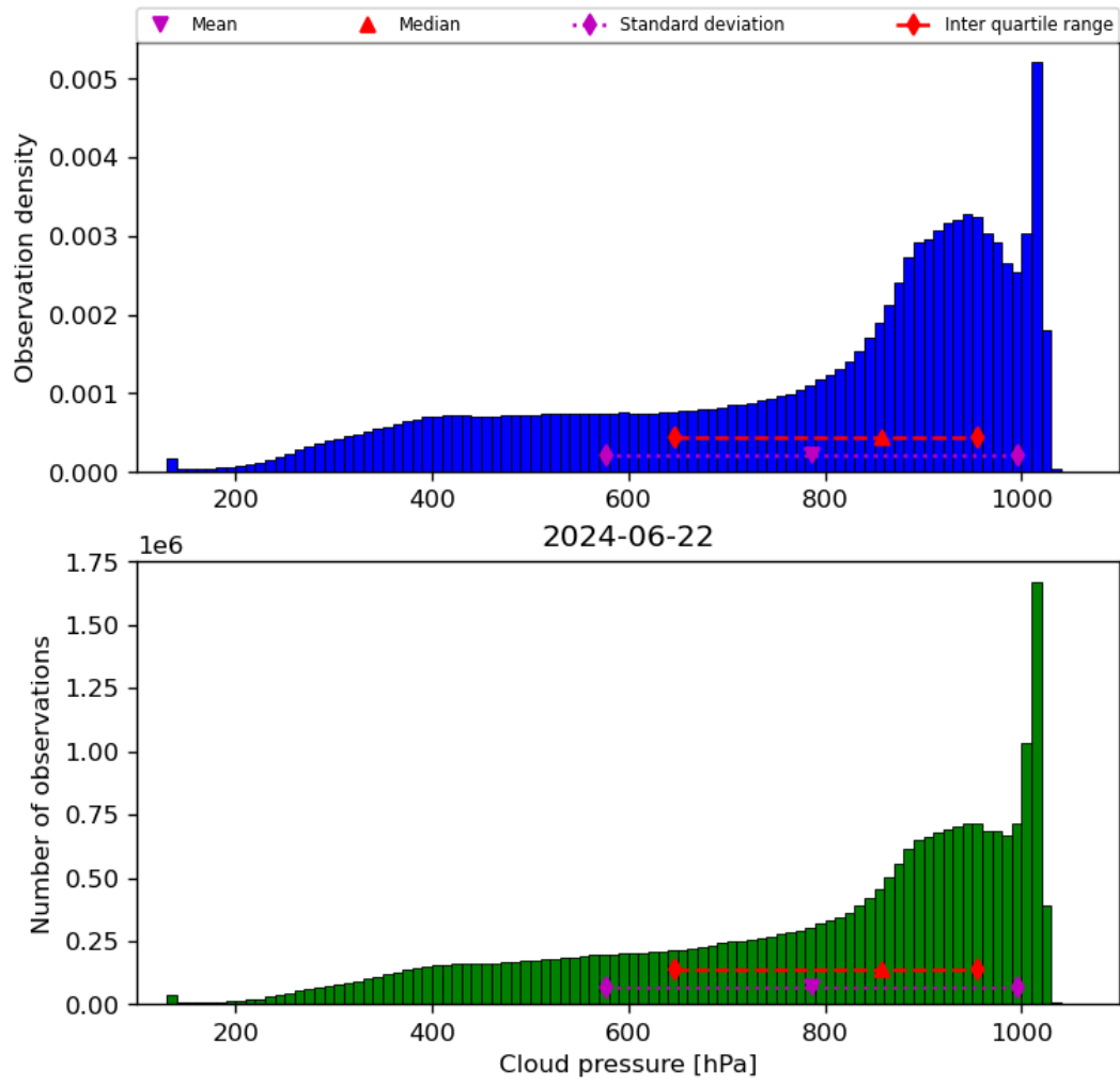
Figure 30: Histogram of “Cloud pressure” for 2024-06-21 to 2024-06-23
