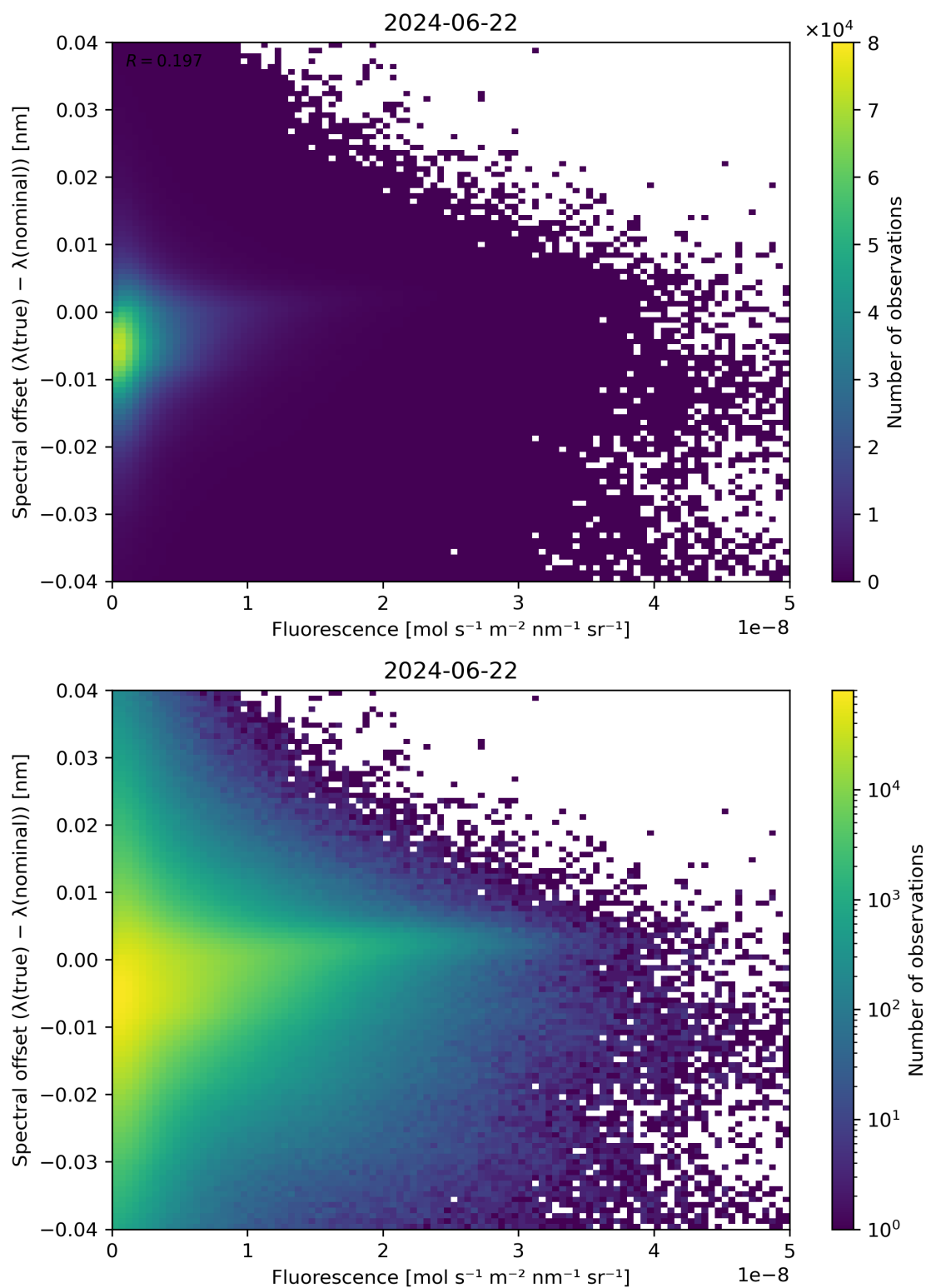
Figure 87: Scatter density plot of “Fluorescence” against “Spectral offset ( \lambda(\text{true}) - \lambda(\text{nominal}) )” for 2024-06-21 to 2024-06-23.
