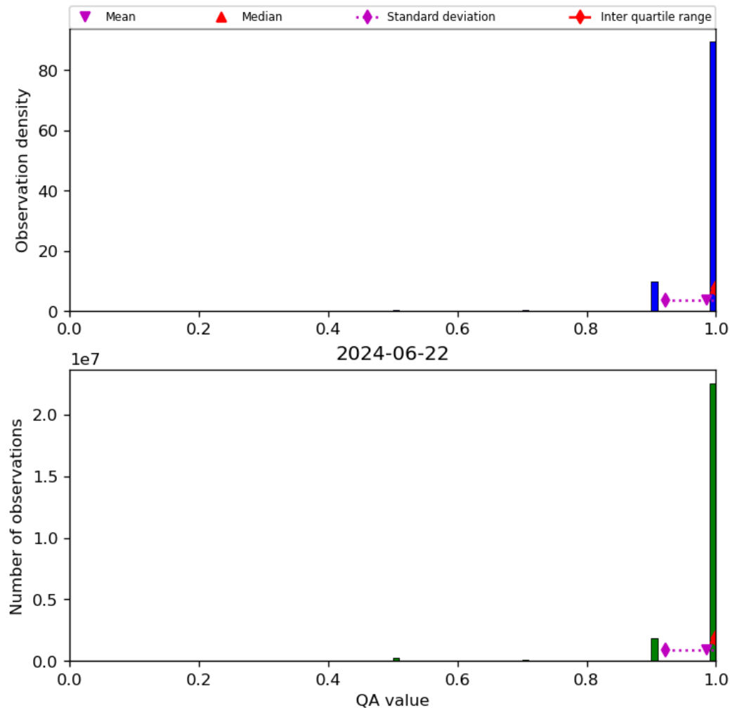
Figure 29: Histogram of “QA value” for 2024-06-21 to 2024-06-23
