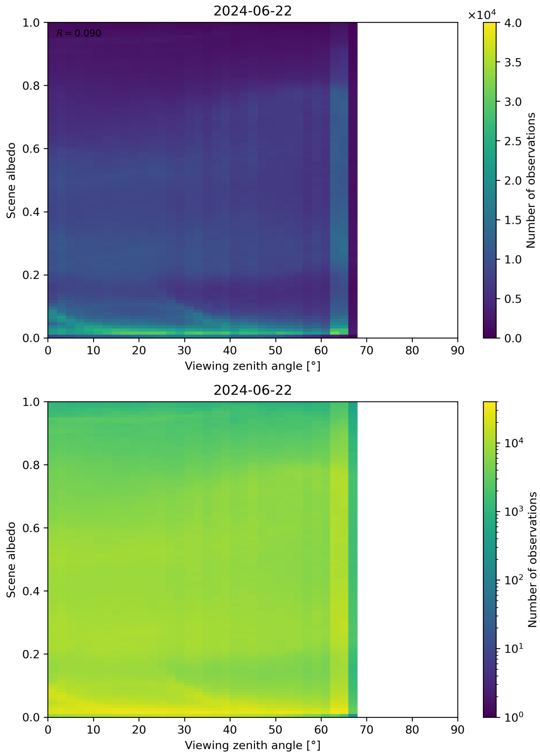
Figure 126: Scatter density plot of “Viewing zenith angle” against “Scene albedo” for 2024-06-21 to 2024-06-23.
