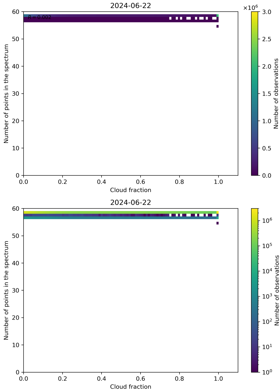
Figure 74: Scatter density plot of “Cloud fraction” against “Number of points in the spectrum” for 2024-06-21 to 2024-06-23.
