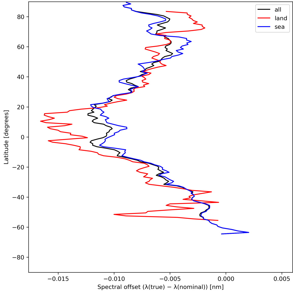
Figure 28: Zonal average of “Spectral offset ( \lambda(\text{true}) - \lambda(\text{nominal}) )” for 2024-06-21 to 2024-06-23.
