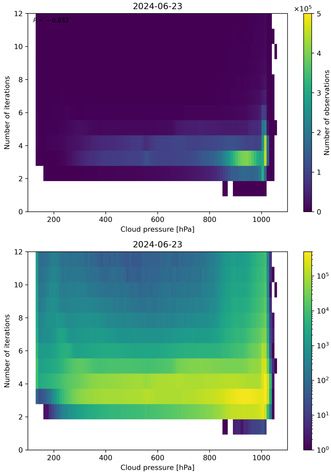
Figure 81: Scatter density plot of “Cloud pressure” against “Number of iterations” for 2024-06-22 to 2024-06-24.
