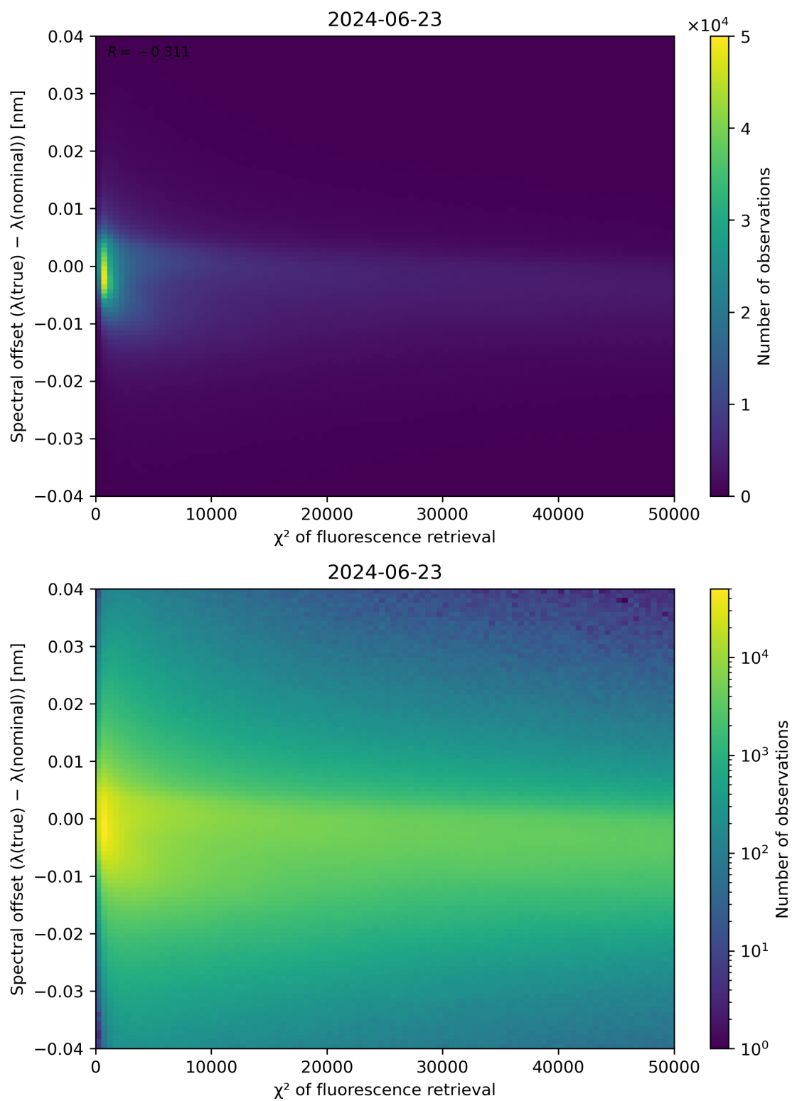
Figure 69: Scatter density plot of “ \chi^2 of fluorescence retrieval” against “Spectral offset ( \lambda(\text{true}) - \lambda(\text{nominal}) )” for 2024-06-22 to 2024-06-24.
