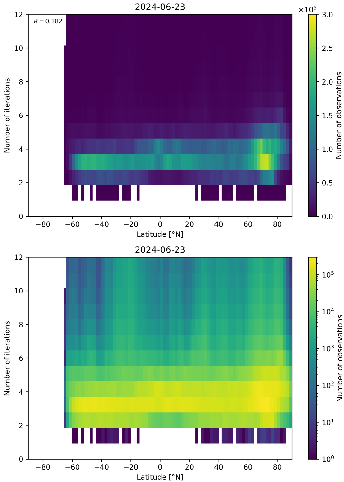
Figure 93: Scatter density plot of “Latitude” against “Number of iterations” for 2024-06-22 to 2024-06-24.
