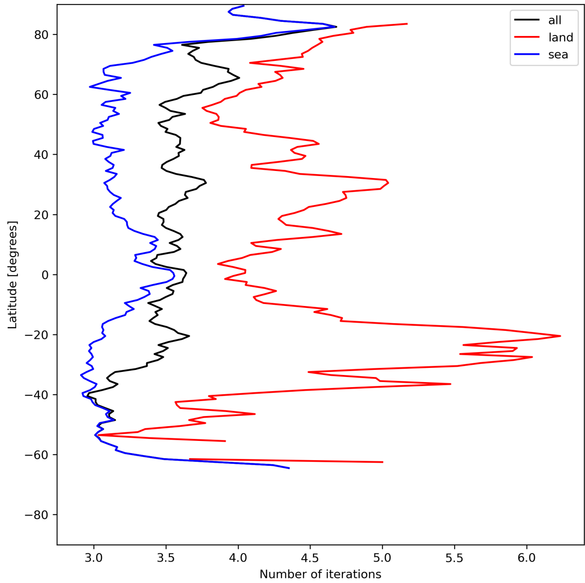
Figure 22: Zonal average of “Number of iterations” for 2024-06-22 to 2024-06-24.
