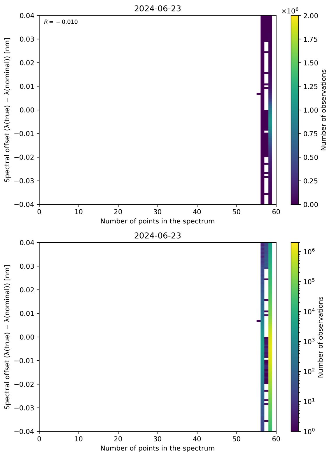
Figure 101: Scatter density plot of “Number of points in the spectrum” against “Spectral offset ( \lambda(\text{true}) - \lambda(\text{nominal}) )” for 2024-06-22 to 2024-06-24.
