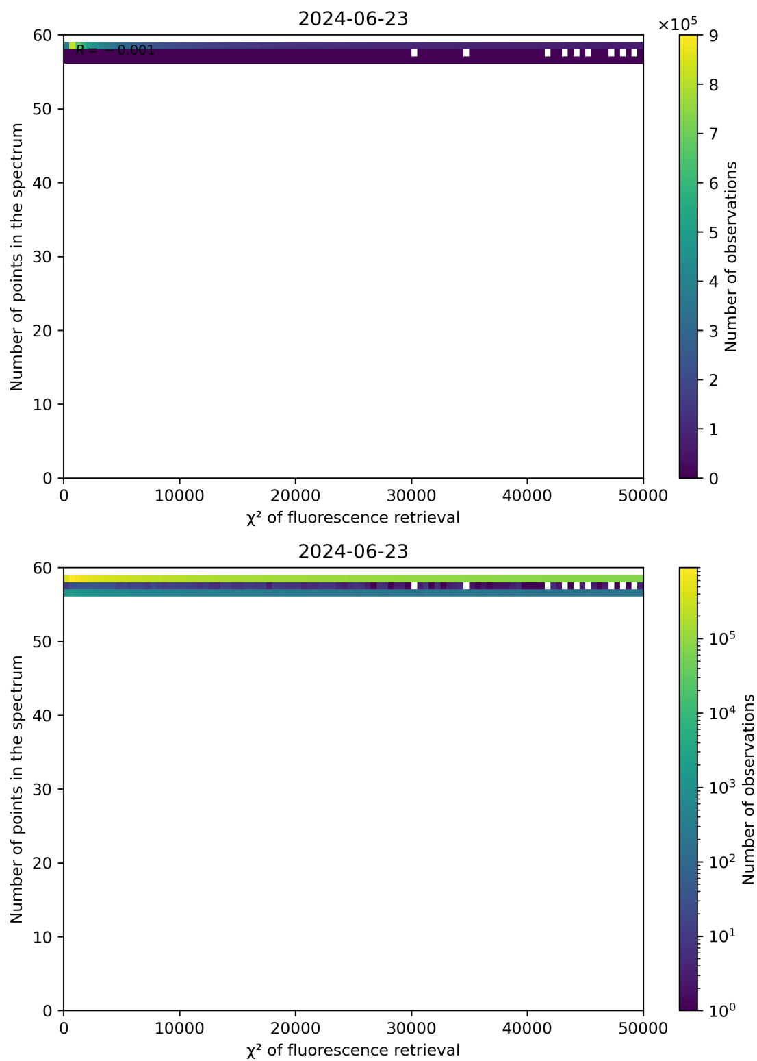
Figure 68: Scatter density plot of " \chi^2 of fluorescence retrieval" against "Number of points in the spectrum" for 2024-06-22 to 2024-06-24.
