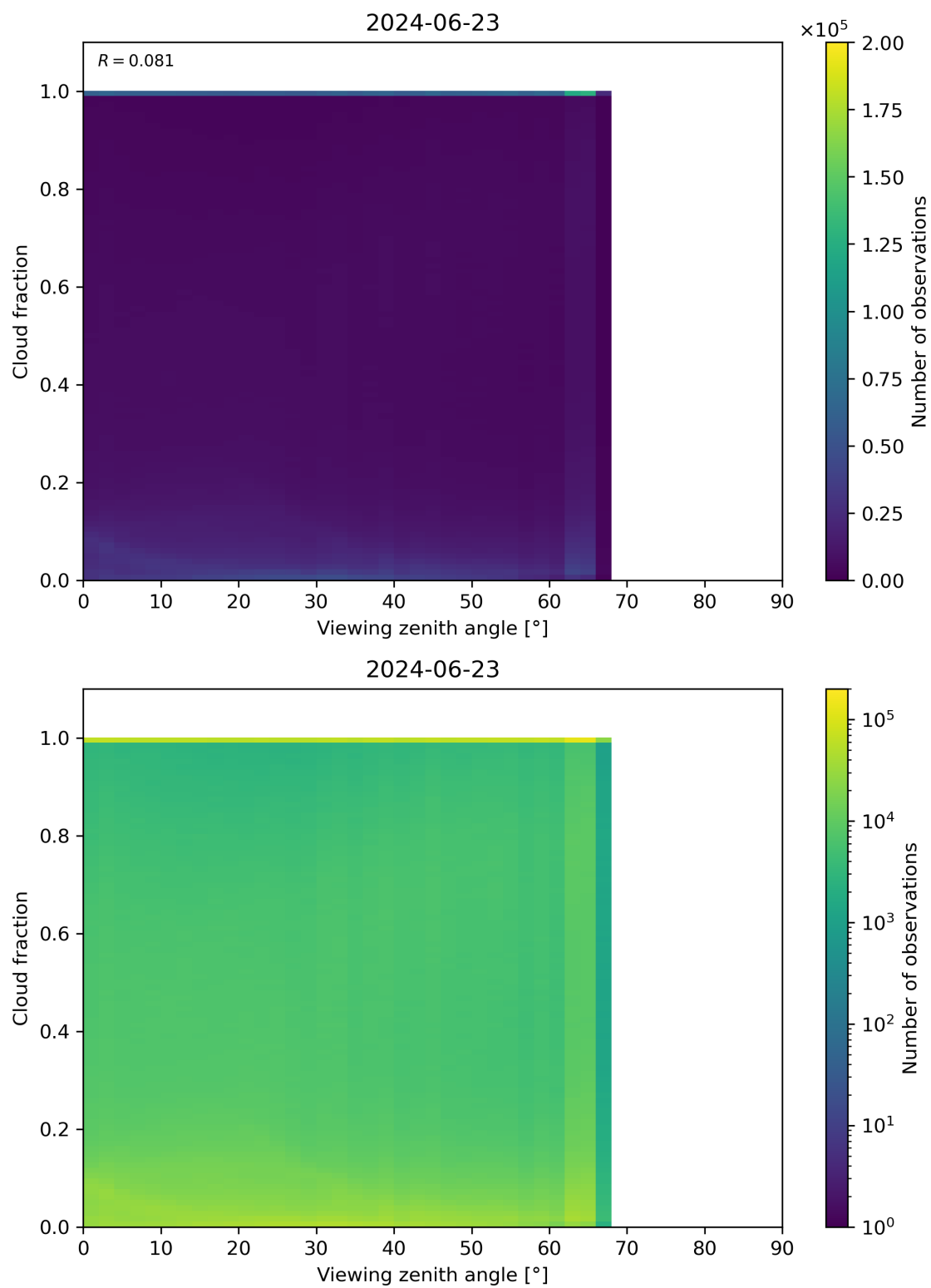
Figure 120: Scatter density plot of “Viewing zenith angle” against “Cloud fraction” for 2024-06-22 to 2024-06-24.
