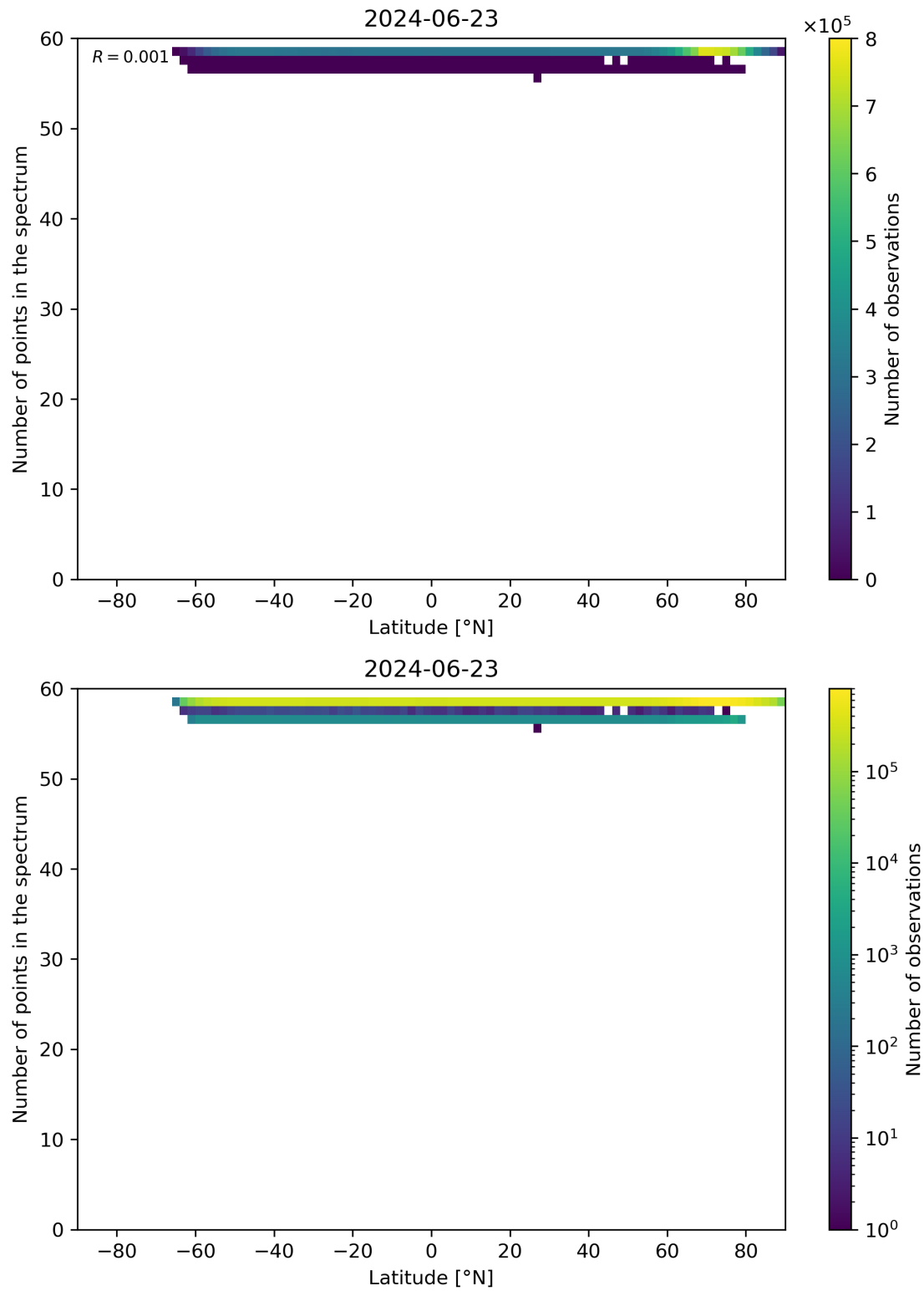
Figure 94: Scatter density plot of “Latitude” against “Number of points in the spectrum” for 2024-06-22 to 2024-06-24.
