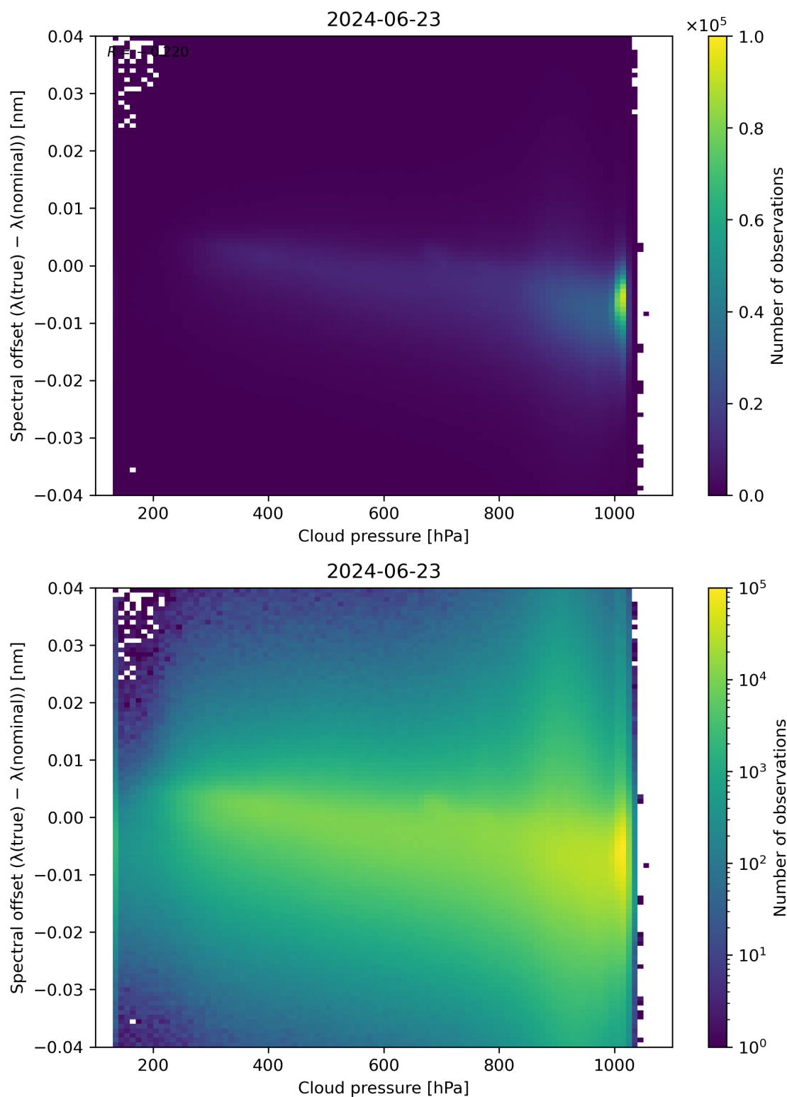
Figure 84: Scatter density plot of “Cloud pressure” against “Spectral offset ( \lambda(\text{true}) - \lambda(\text{nominal}) )” for 2024-06-22 to 2024-06-24.
