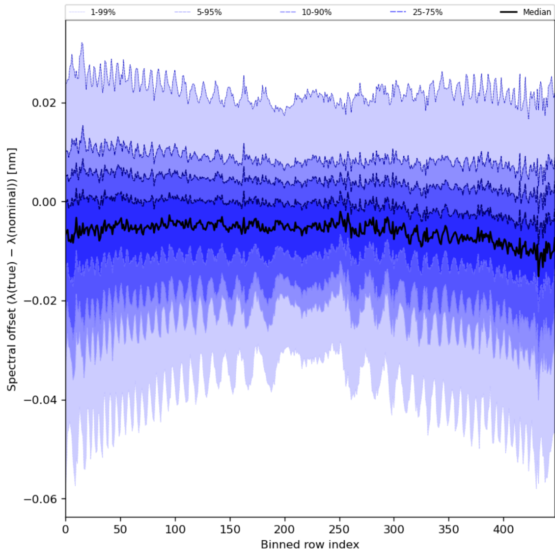
Figure 62: Along track statistics of “Spectral offset ( \lambda(\text{true}) - \lambda(\text{nominal}) )” for 2024-06-22 to 2024-06-24
