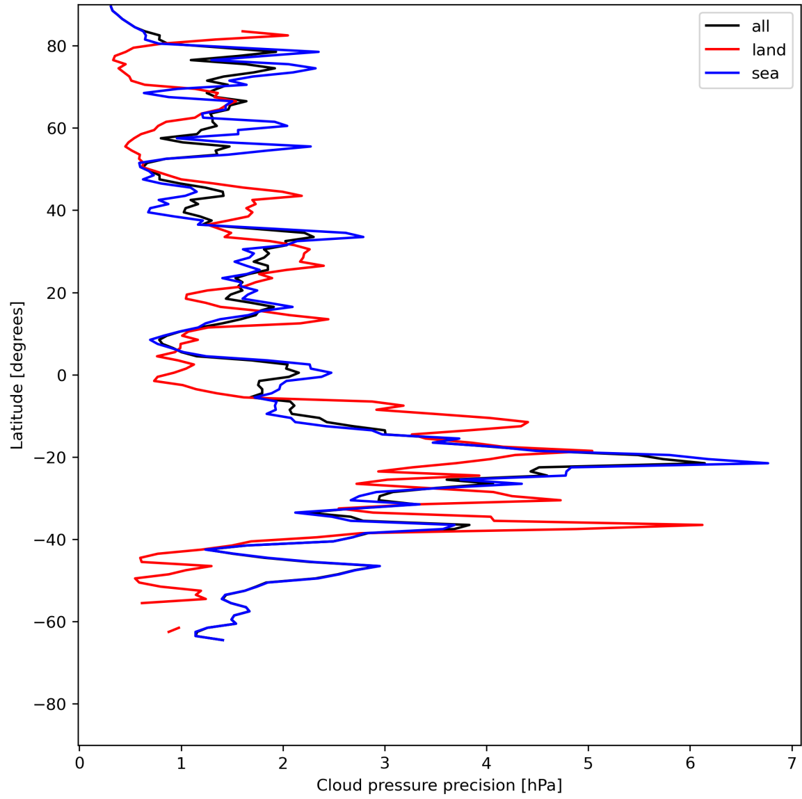
Figure 14: Zonal average of “Cloud pressure precision” for 2024-06-22 to 2024-06-24.
