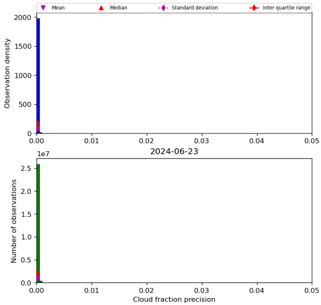
Figure 33: Histogram of “Cloud fraction precision” for 2024-06-22 to 2024-06-24
