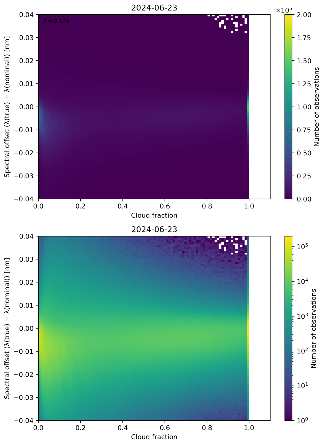
Figure 76: Scatter density plot of “Cloud fraction” against “Spectral offset ( \lambda(\text{true}) - \lambda(\text{nominal}) )” for 2024-06-22 to 2024-06-24.
