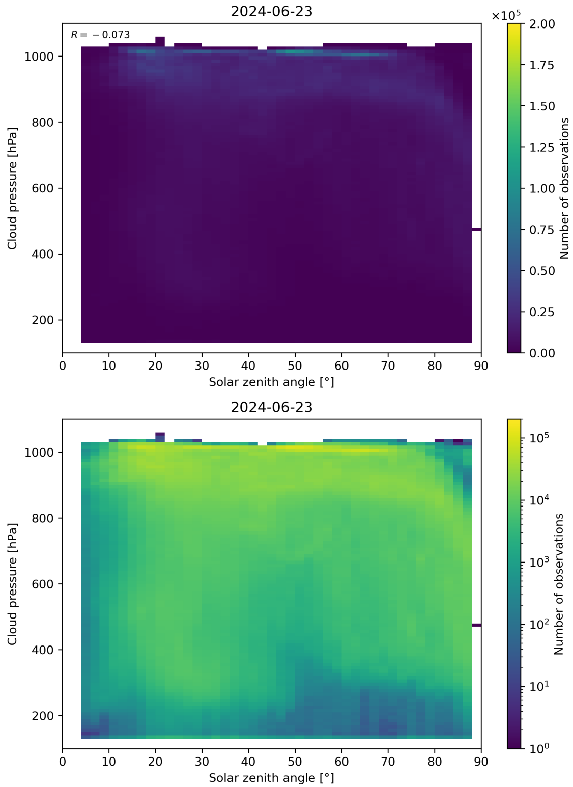
Figure 111: Scatter density plot of “Solar zenith angle” against “Cloud pressure” for 2024-06-22 to 2024-06-24.
