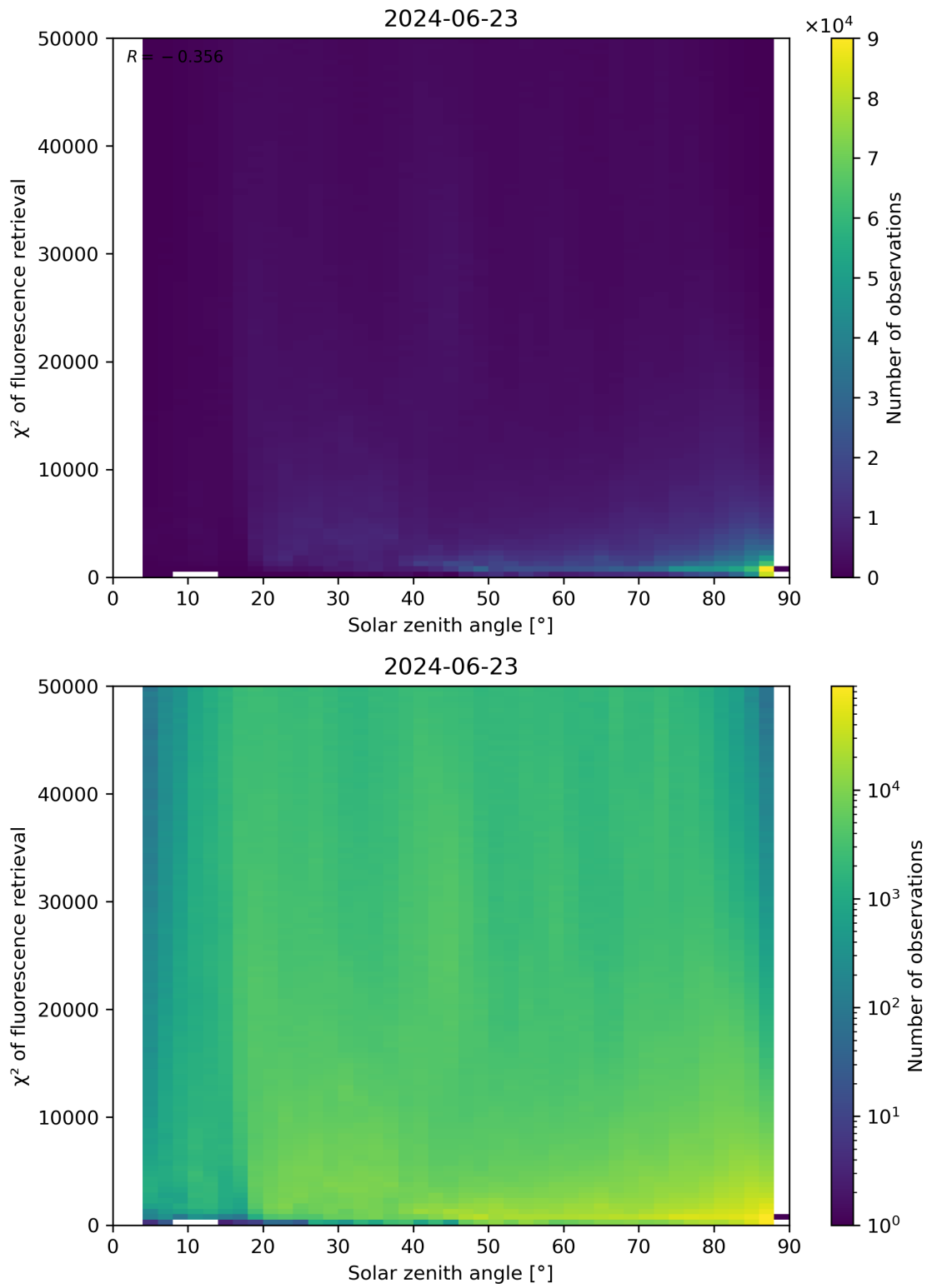
Figure 109: Scatter density plot of “Solar zenith angle” against “ \chi^2 of fluorescence retrieval” for 2024-06-22 to 2024-06-24.
