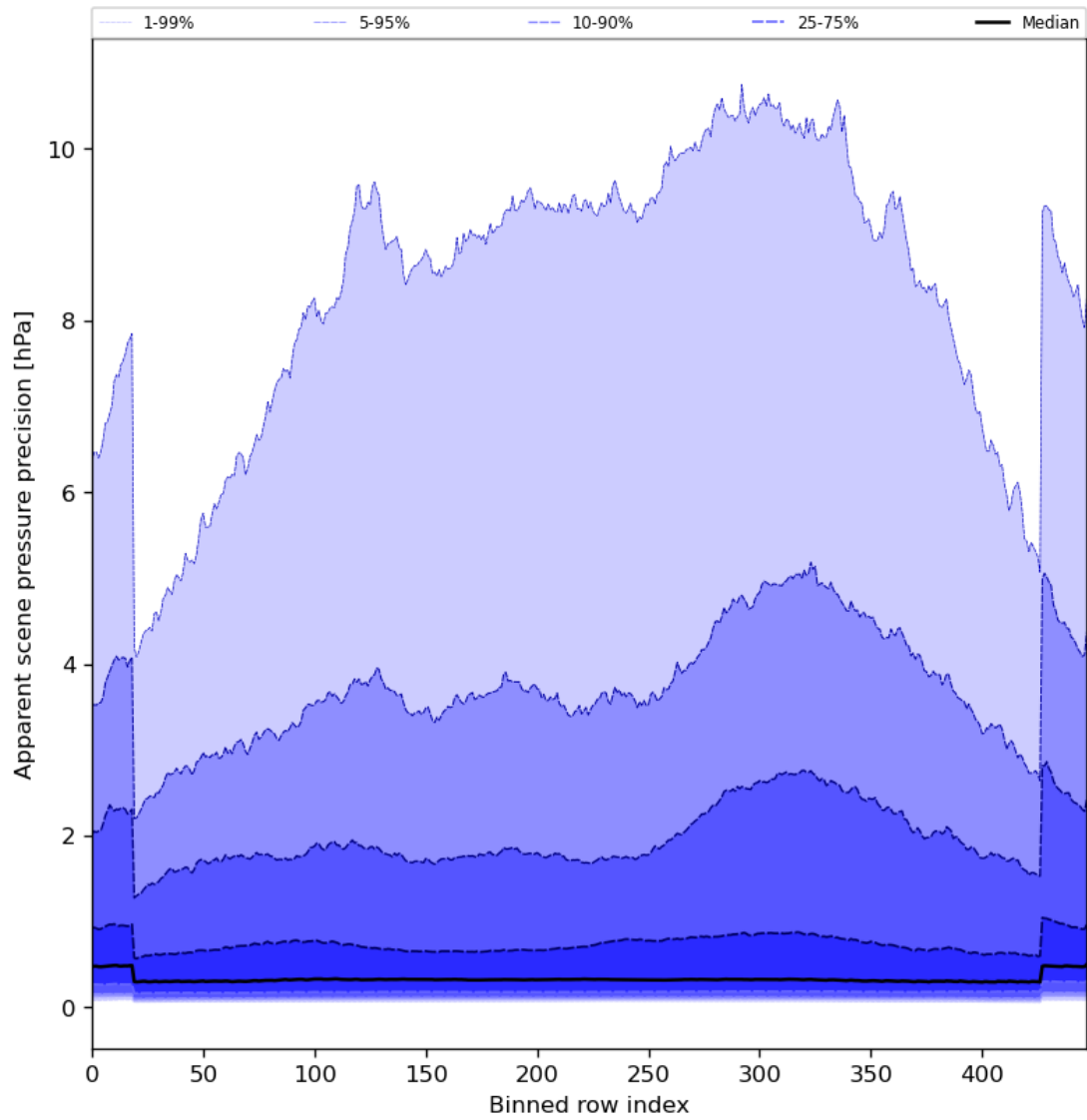
Figure 54: Along track statistics of “Apparent scene pressure precision” for 2024-06-22 to 2024-06-24
