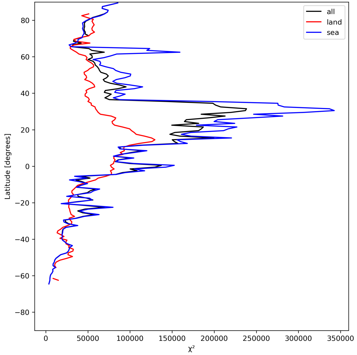
Figure 21: Zonal average of “ \chi^2 ” for 2024-06-22 to 2024-06-24.
