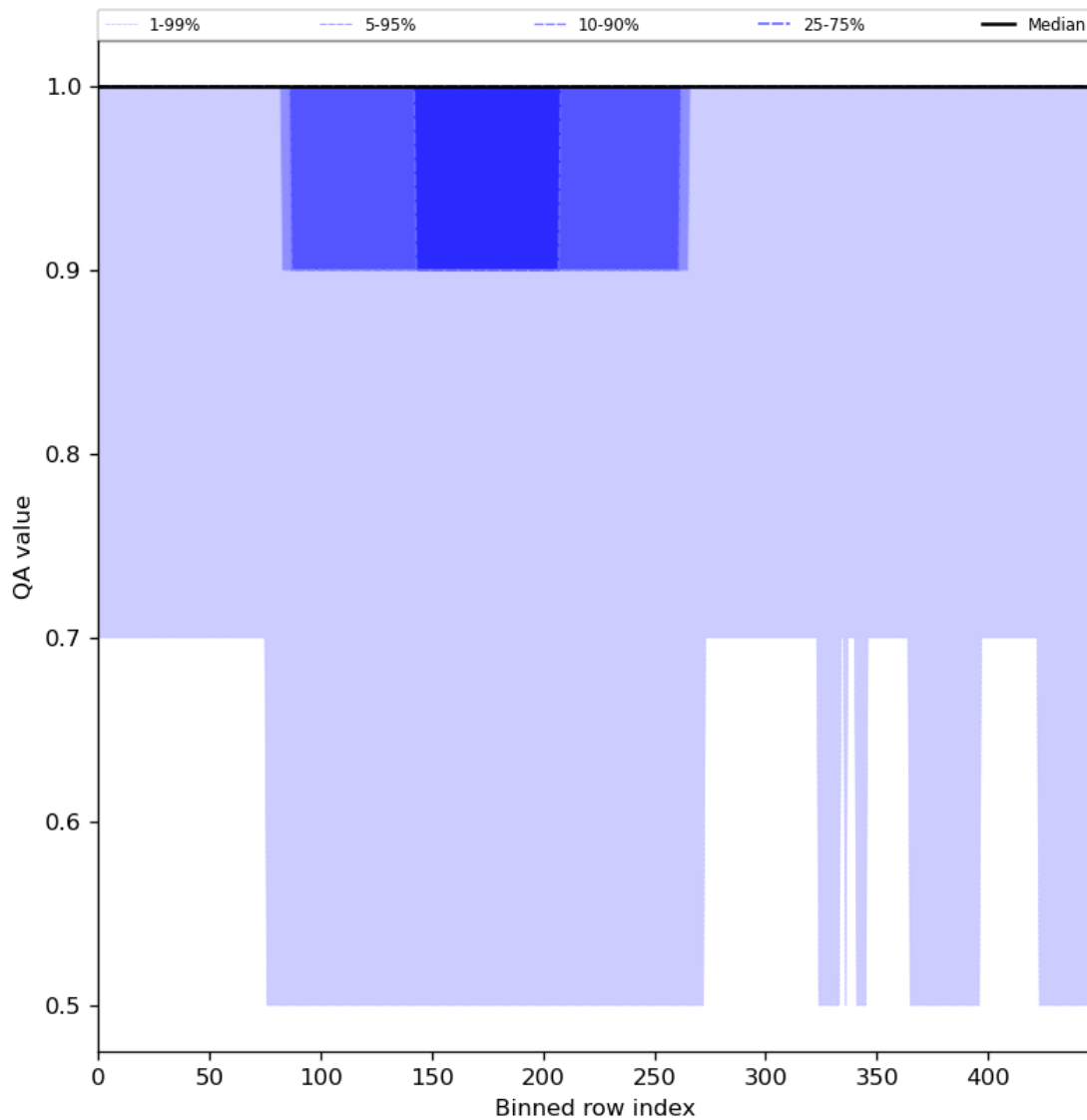
Figure 46: Along track statistics of “QA value” for 2024-06-22 to 2024-06-24
