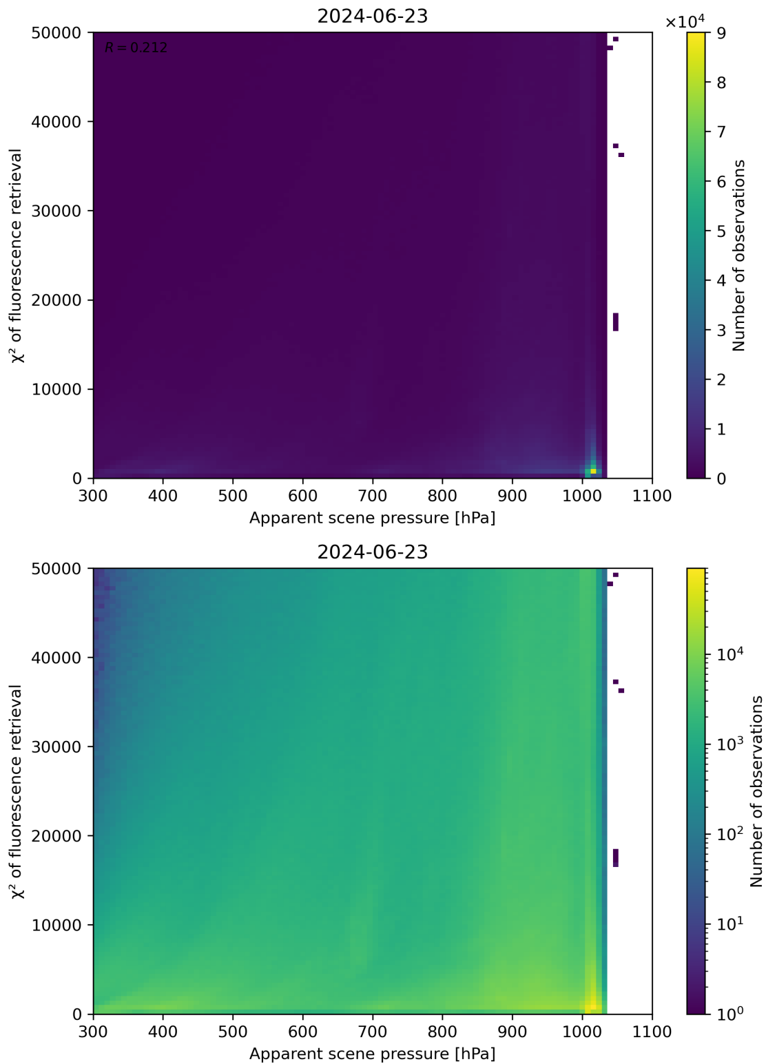
Figure 63: Scatter density plot of “Apparent scene pressure” against “ \chi^2 of fluorescence retrieval” for 2024-06-22 to 2024-06-24.
