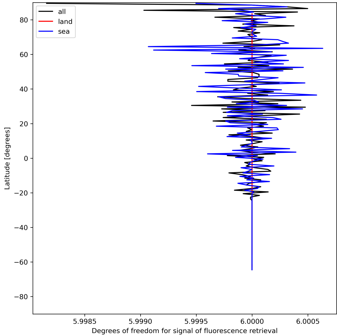
Figure 26: Zonal average of “Degrees of freedom for signal of fluorescence retrieval” for 2024-06-22 to 2024-06-24.
