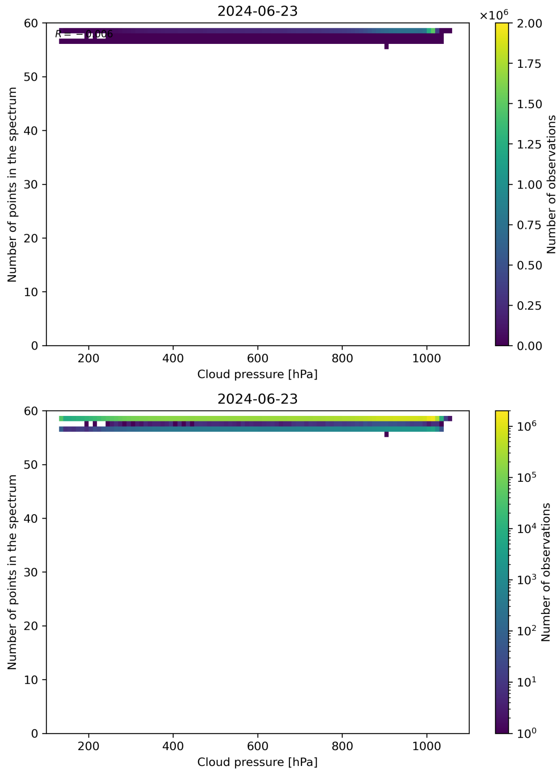
Figure 82: Scatter density plot of “Cloud pressure” against “Number of points in the spectrum” for 2024-06-22 to 2024-06-24.
