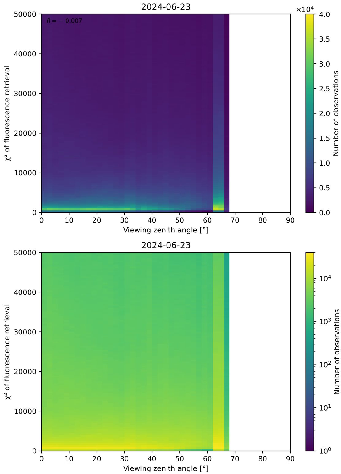
Figure 119: Scatter density plot of “Viewing zenith angle” against “ \chi^2 of fluorescence retrieval” for 2024-06-22 to 2024-06-24.
