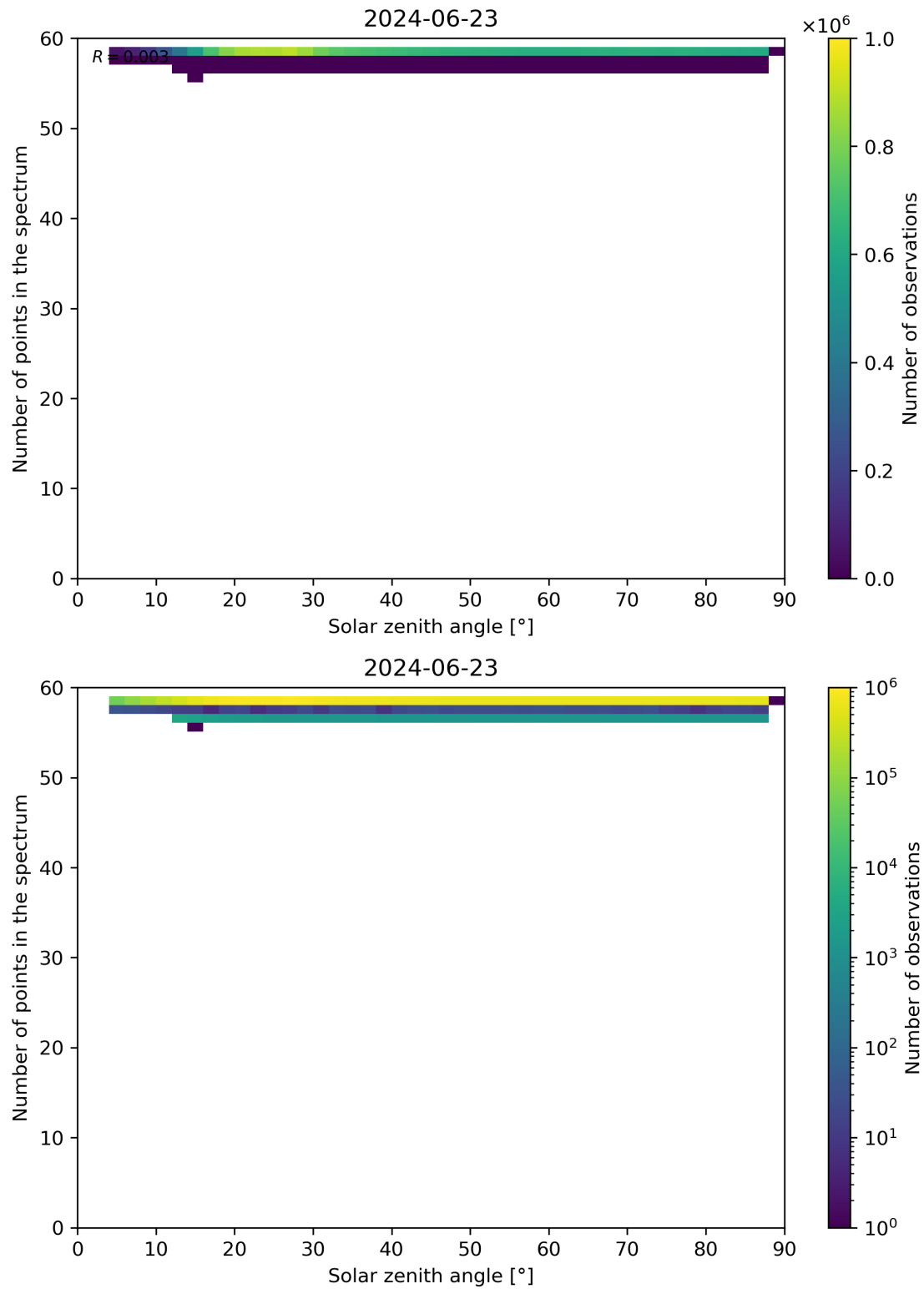
Figure 115: Scatter density plot of “Solar zenith angle” against “Number of points in the spectrum” for 2024-06-22 to 2024-06-24.
