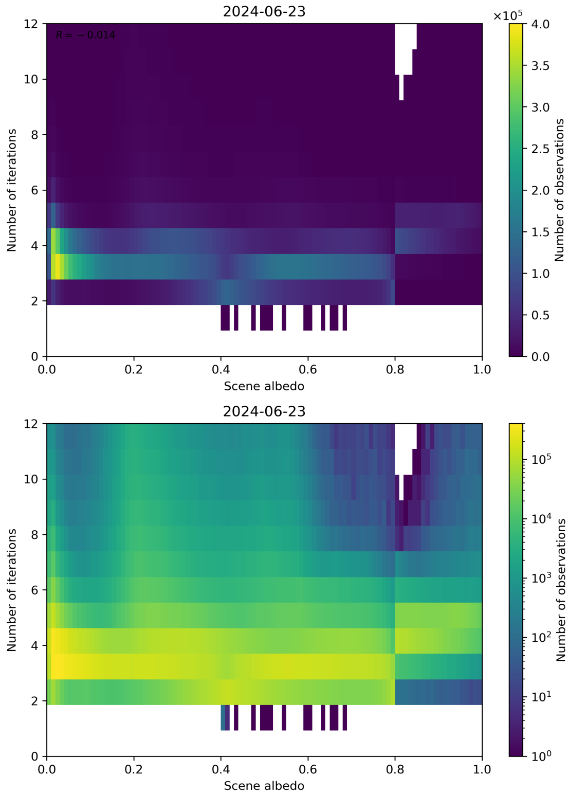
Figure 105: Scatter density plot of “Scene albedo” against “Number of iterations” for 2024-06-22 to 2024-06-24.
