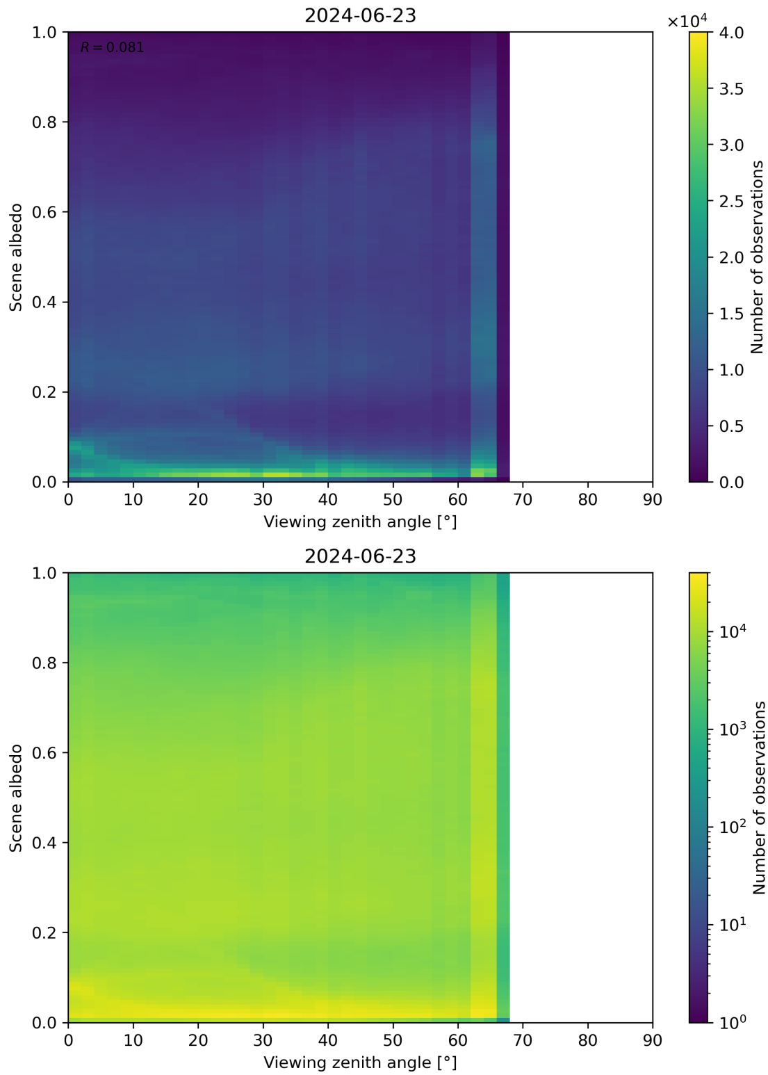
Figure 126: Scatter density plot of “Viewing zenith angle” against “Scene albedo” for 2024-06-22 to 2024-06-24.
