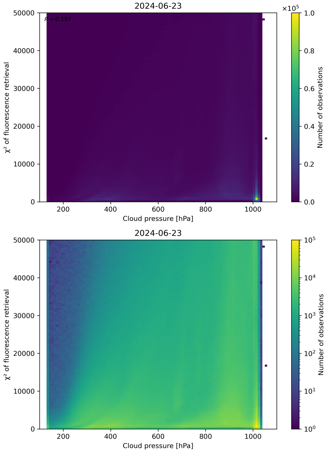
Figure 78: Scatter density plot of “Cloud pressure” against “ \chi^2 of fluorescence retrieval” for 2024-06-22 to 2024-06-24.
