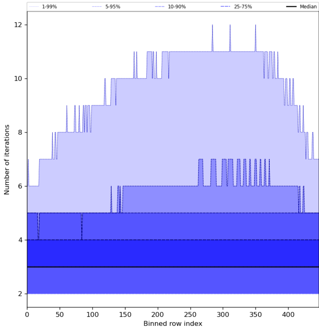
Figure 56: Along track statistics of “Number of iterations” for 2024-06-22 to 2024-06-24
