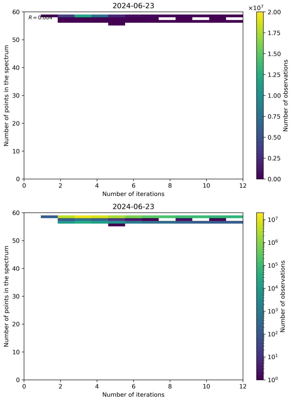
Figure 99: Scatter density plot of “Number of iterations” against “Number of points in the spectrum” for 2024-06-22 to 2024-06-24.
