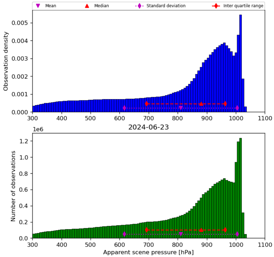
Figure 36: Histogram of “Apparent scene pressure” for 2024-06-22 to 2024-06-24
