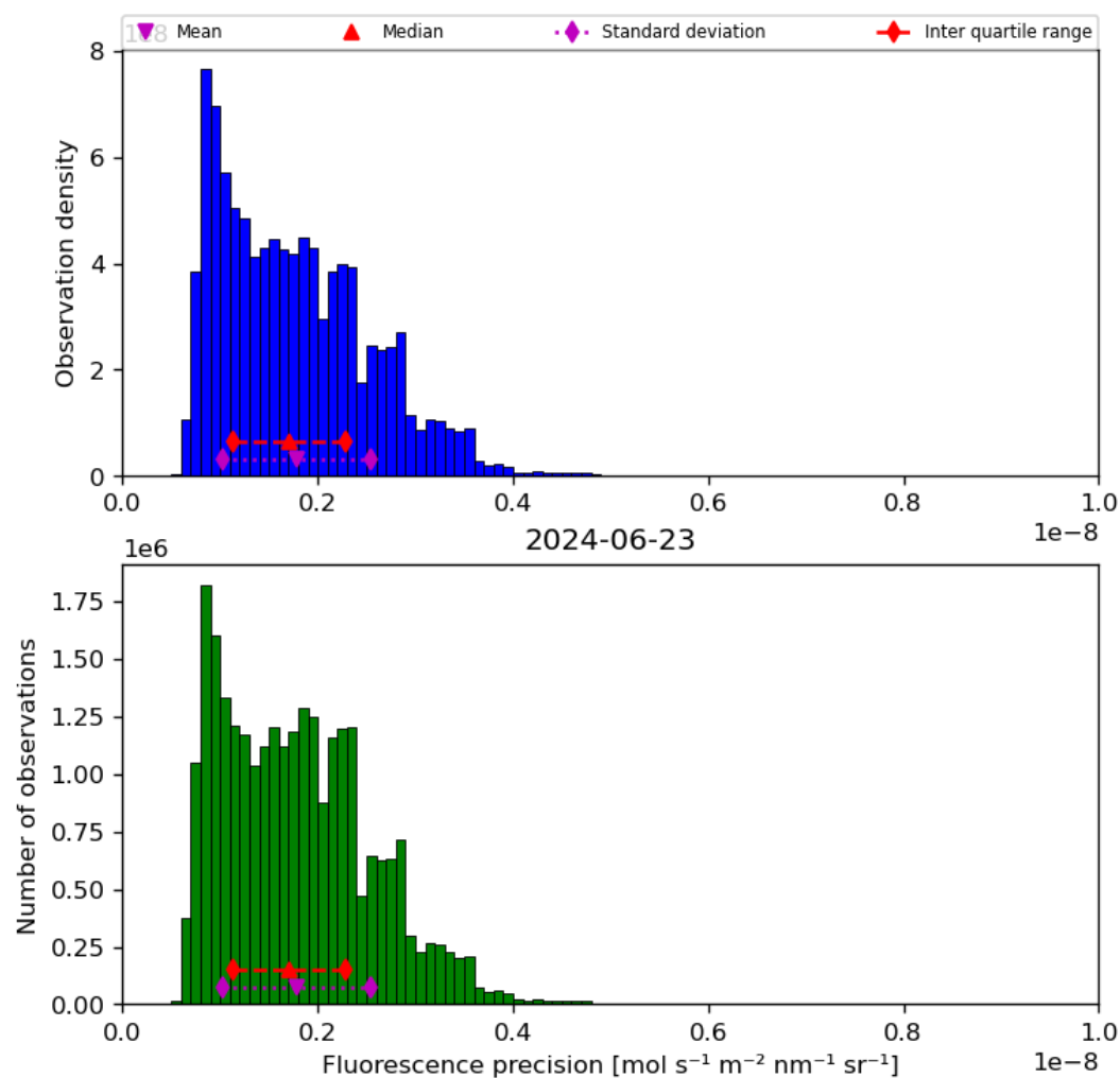
Figure 41: Histogram of “Fluorescence precision” for 2024-06-22 to 2024-06-24
