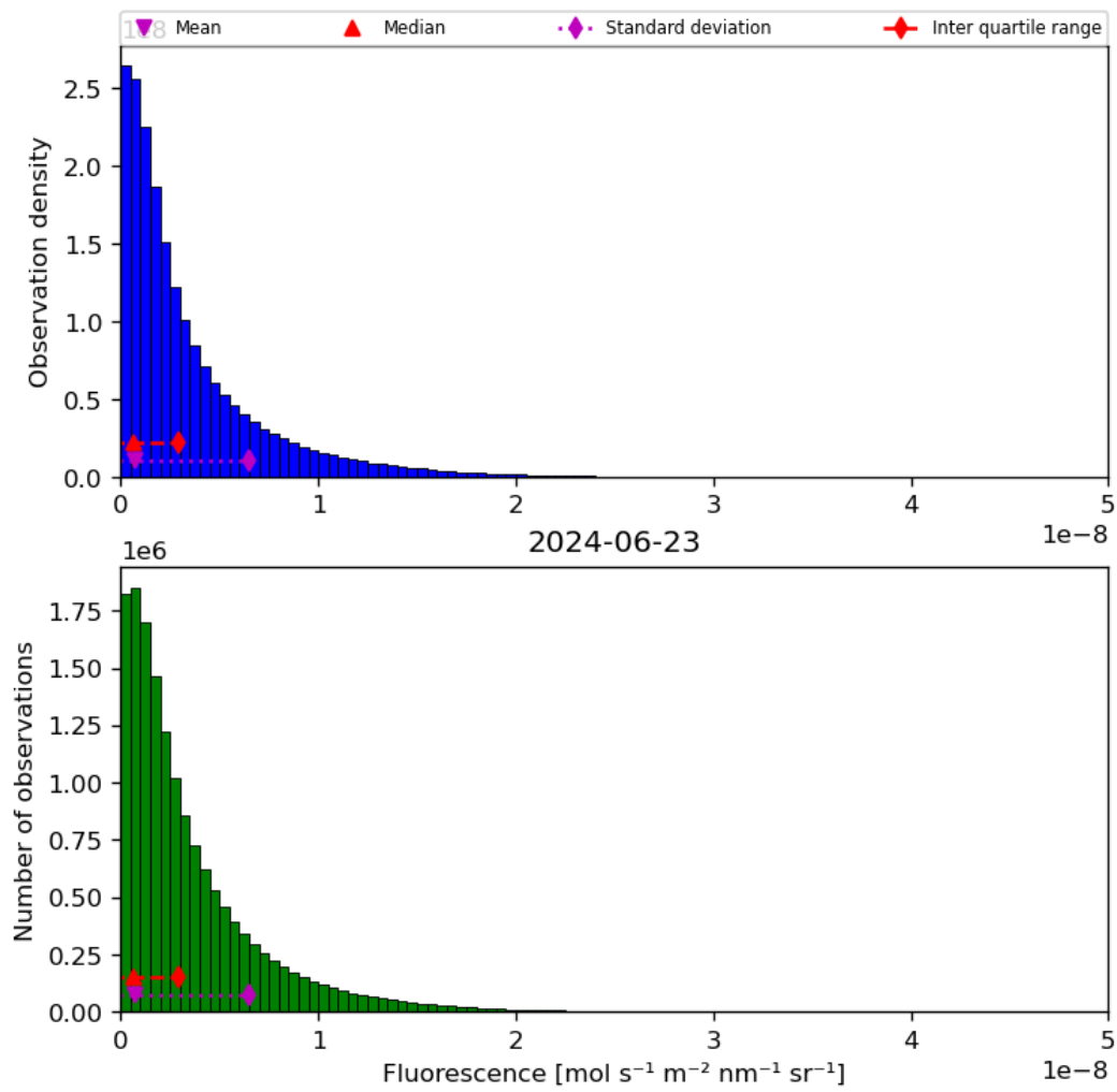
Figure 40: Histogram of “Fluorescence” for 2024-06-22 to 2024-06-24
