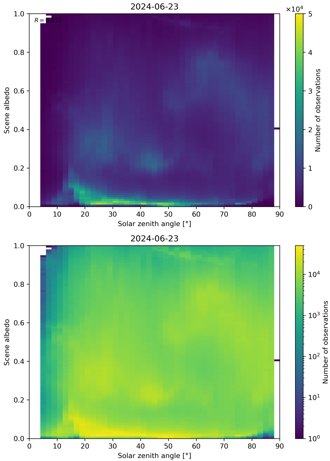
Figure 116: Scatter density plot of “Solar zenith angle” against “Scene albedo” for 2024-06-22 to 2024-06-24.
