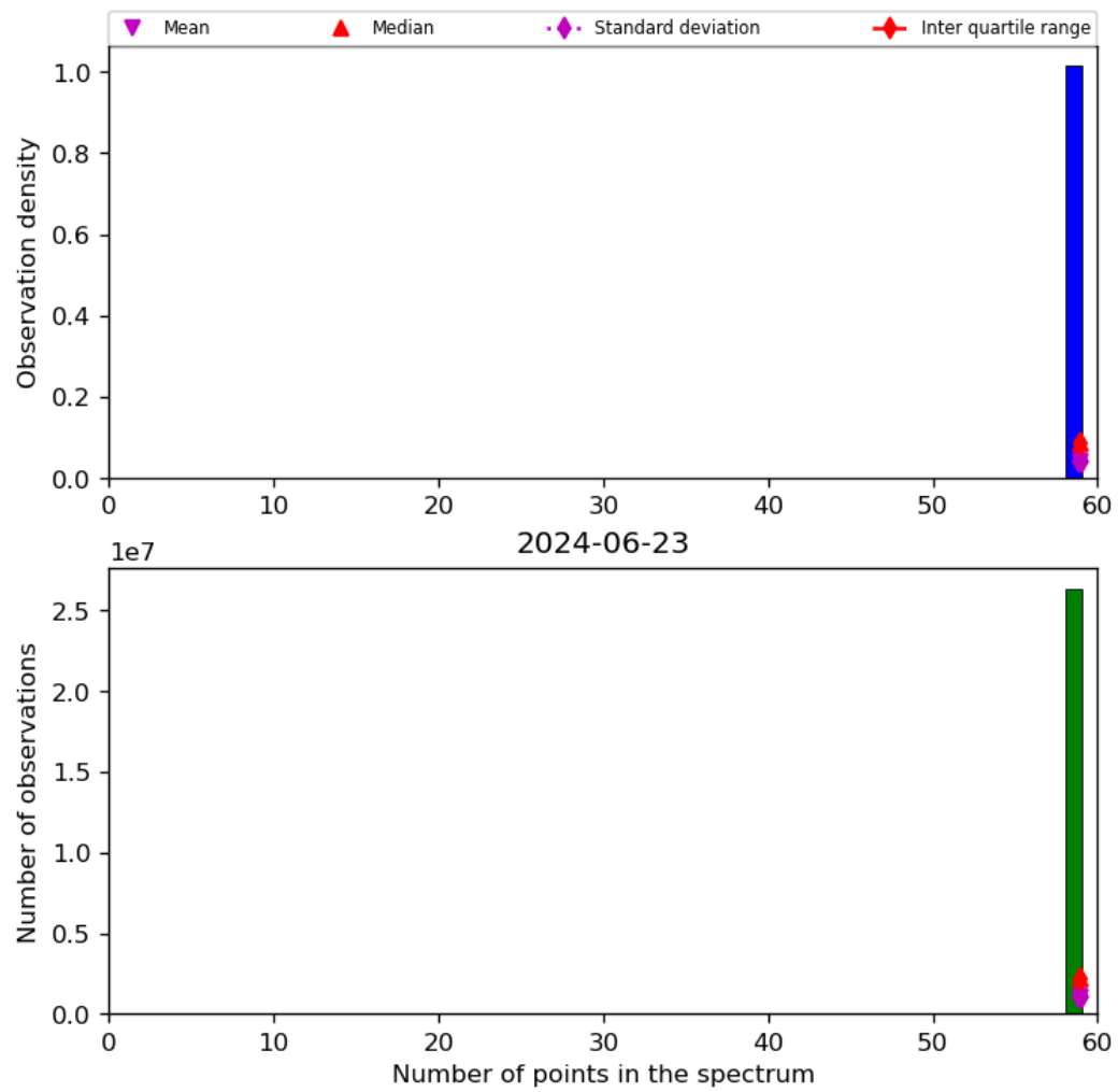
Figure 44: Histogram of “Number of points in the spectrum” for 2024-06-22 to 2024-06-24
