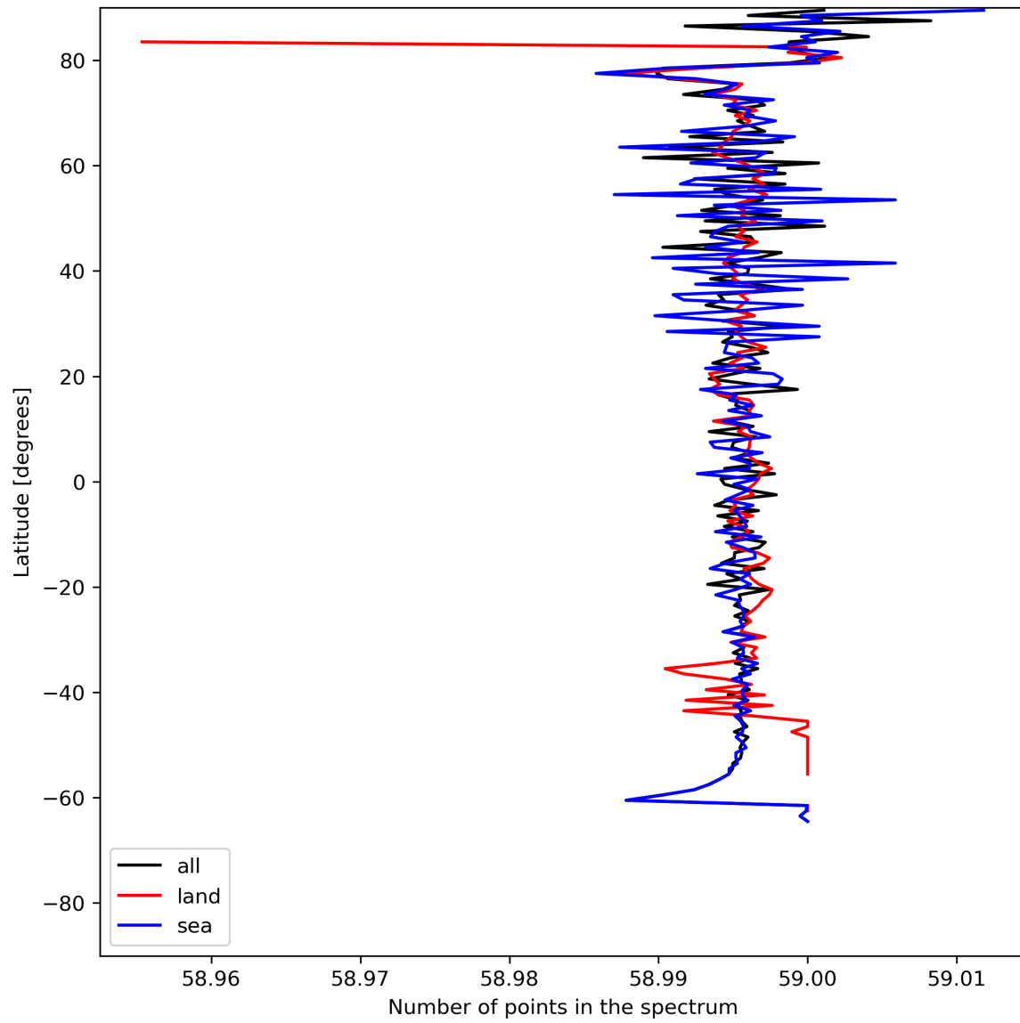
Figure 27: Zonal average of “Number of points in the spectrum” for 2024-06-22 to 2024-06-24.
