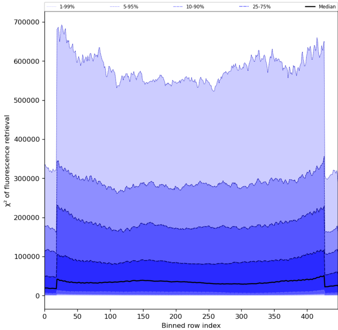
Figure 59: Along track statistics of “ \chi^2 of fluorescence retrieval” for 2024-06-22 to 2024-06-24
