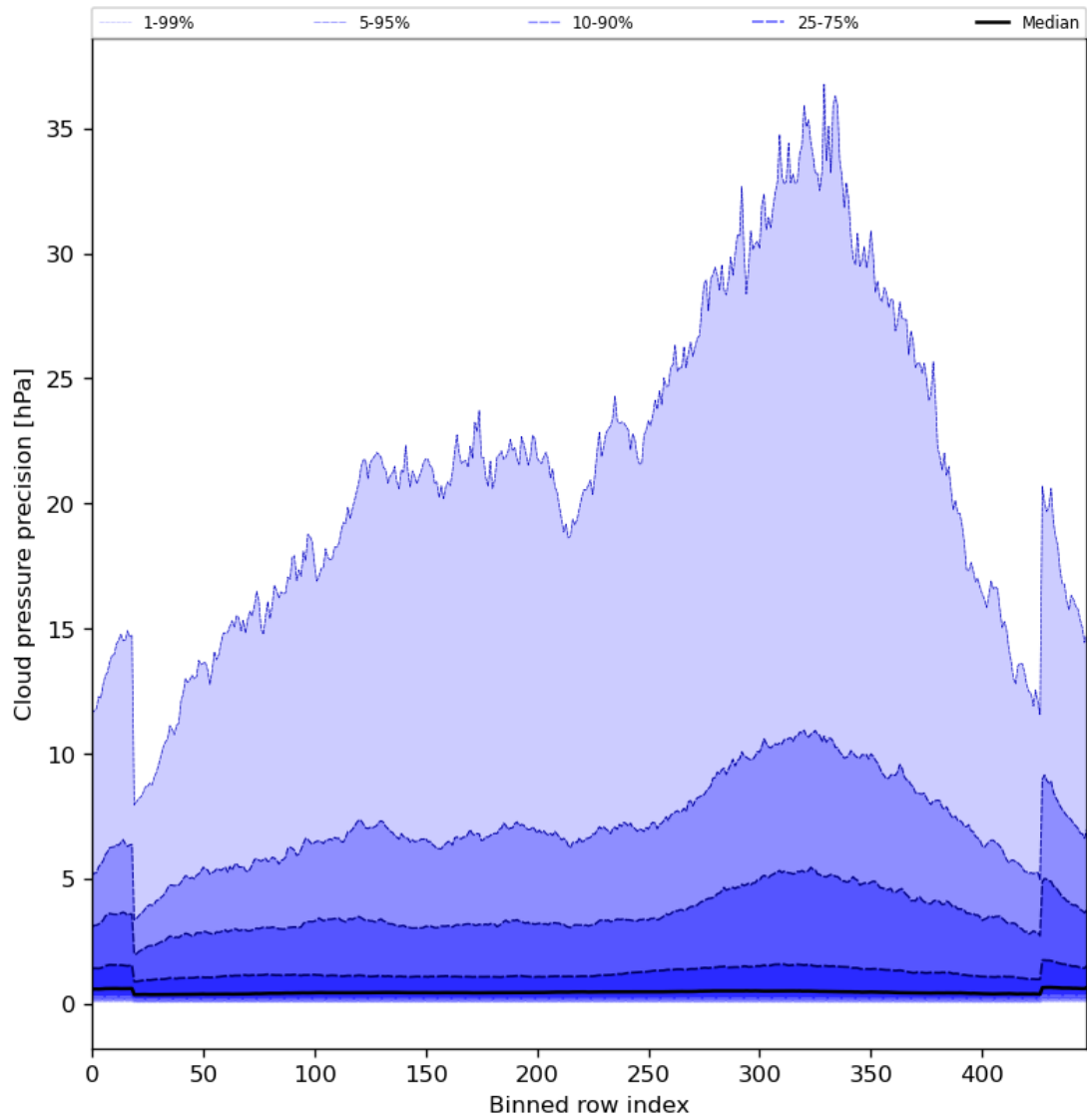
Figure 48: Along track statistics of “Cloud pressure precision” for 2024-06-22 to 2024-06-24
