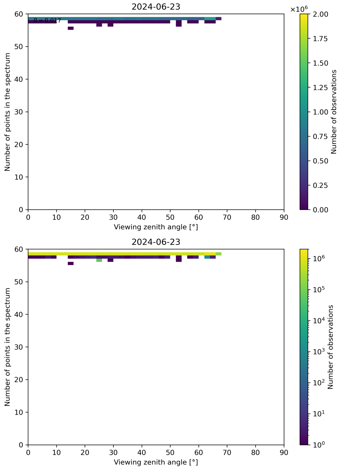
Figure 125: Scatter density plot of “Viewing zenith angle” against “Number of points in the spectrum” for 2024-06-22 to 2024-06-24.
