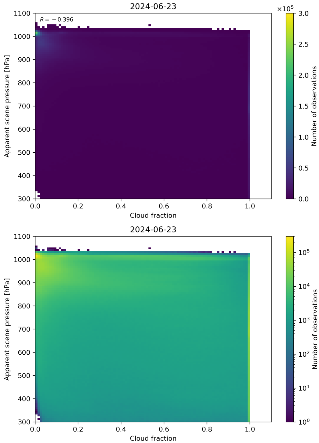
Figure 70: Scatter density plot of “Cloud fraction” against “Apparent scene pressure” for 2024-06-22 to 2024-06-24.
