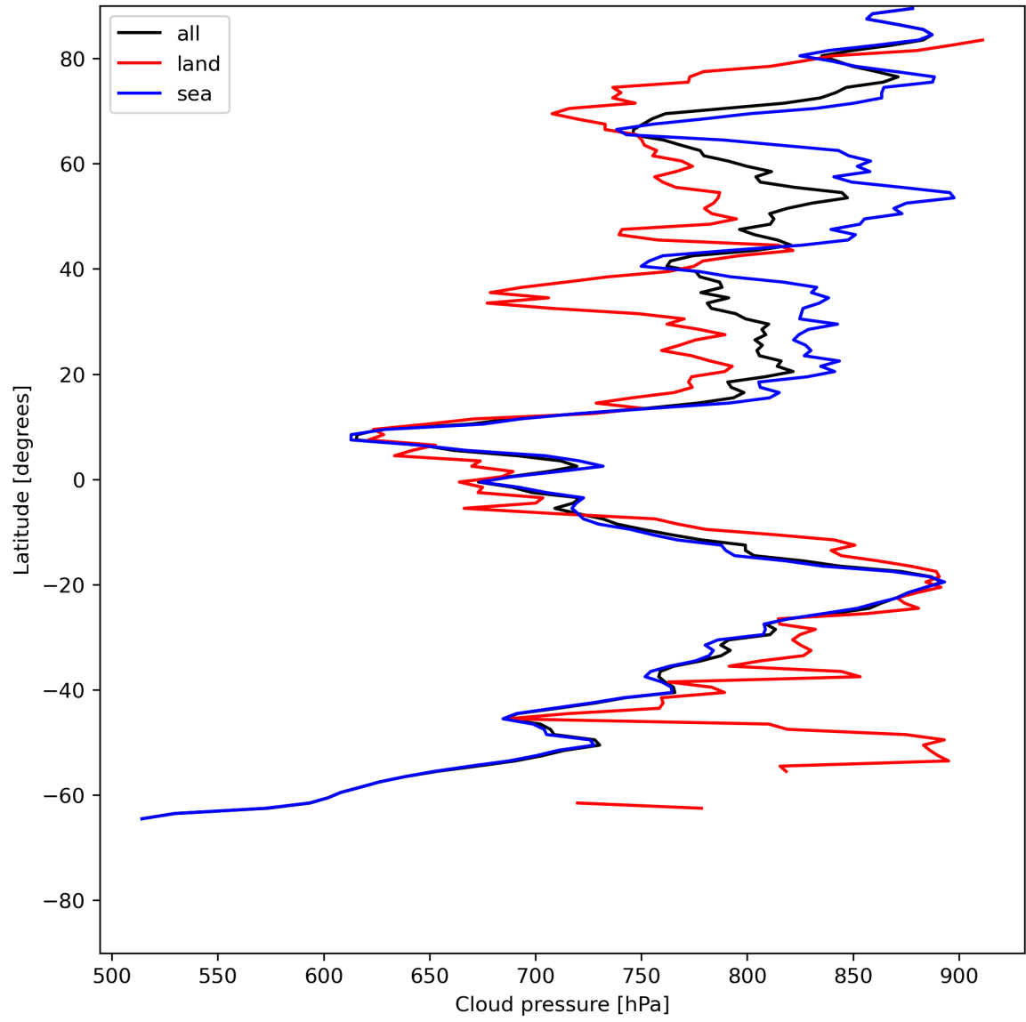
Figure 13: Zonal average of “Cloud pressure” for 2024-06-22 to 2024-06-24.
