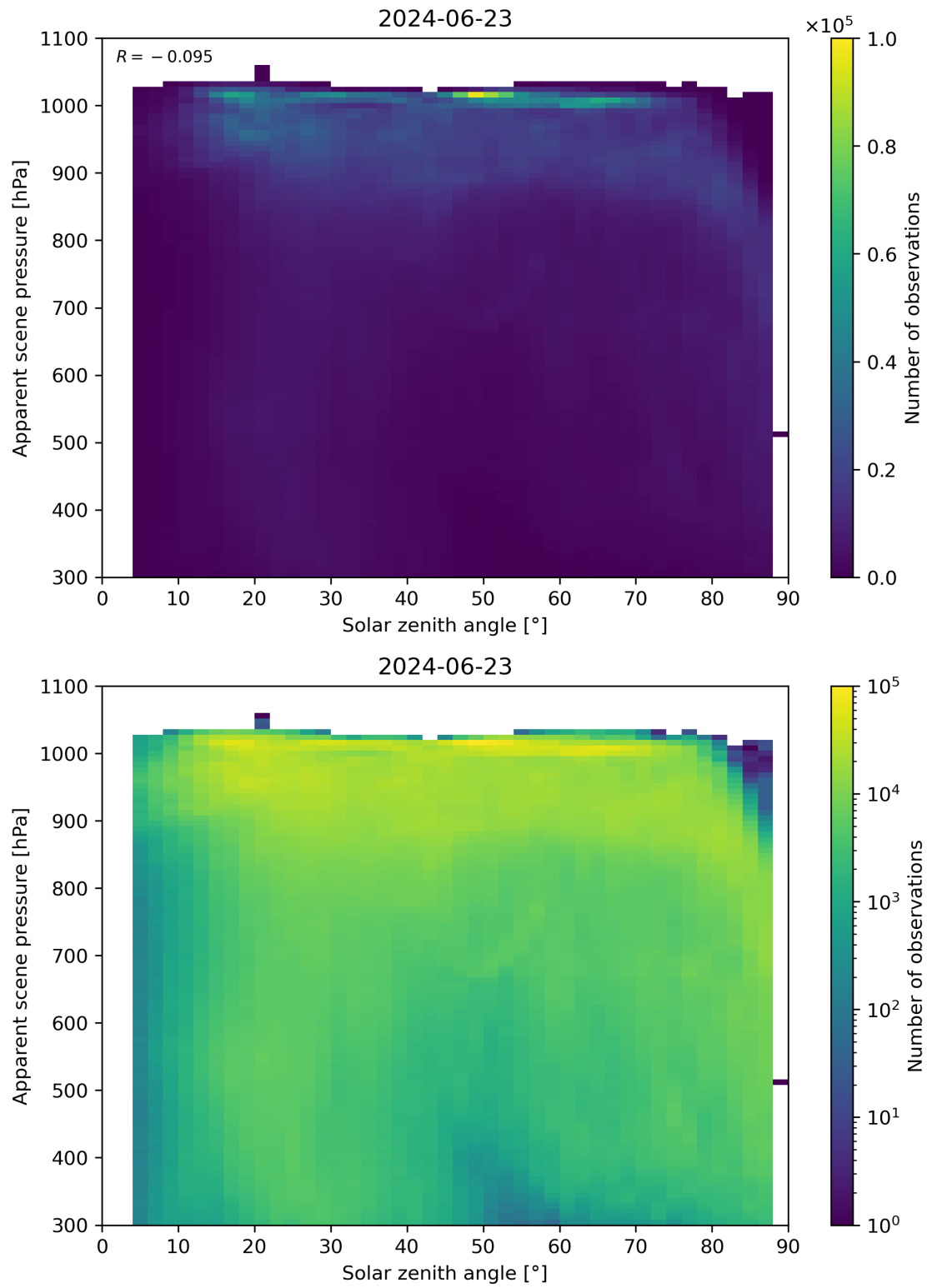
Figure 108: Scatter density plot of “Solar zenith angle” against “Apparent scene pressure” for 2024-06-22 to 2024-06-24.
