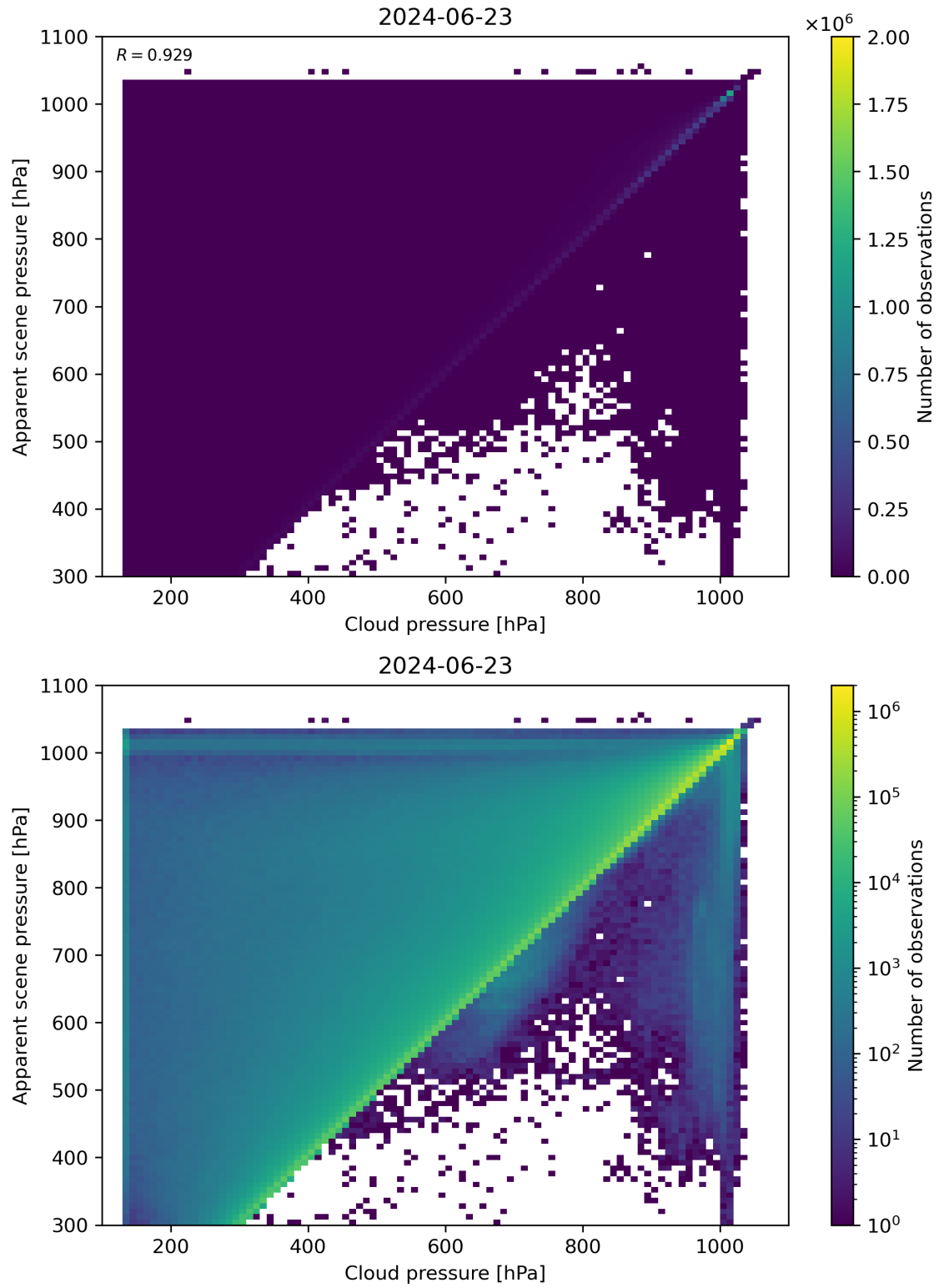
Figure 77: Scatter density plot of “Cloud pressure” against “Apparent scene pressure” for 2024-06-22 to 2024-06-24.
