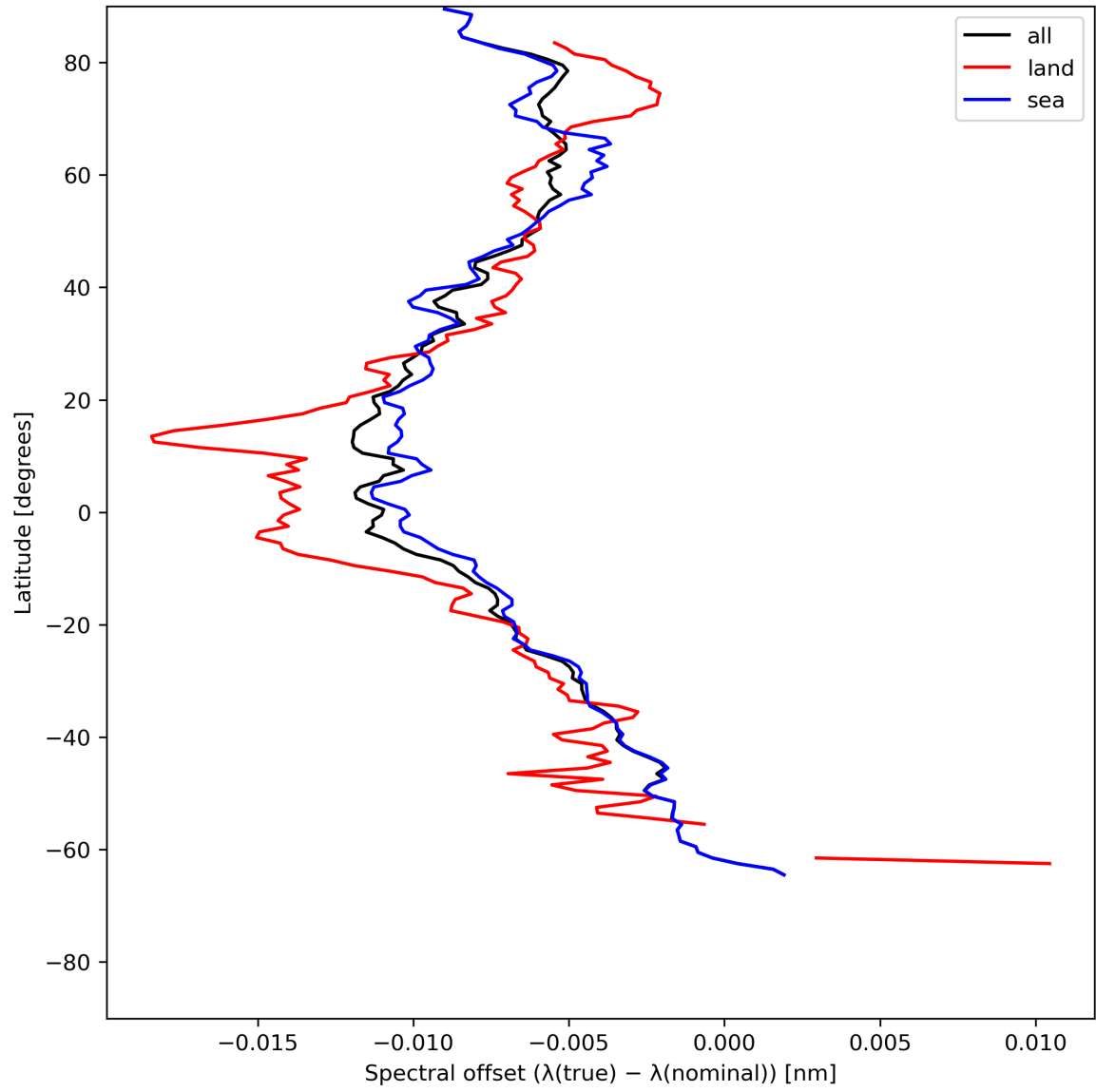
Figure 28: Zonal average of “Spectral offset ( \lambda(\text{true}) - \lambda(\text{nominal}) )” for 2024-06-22 to 2024-06-24.
