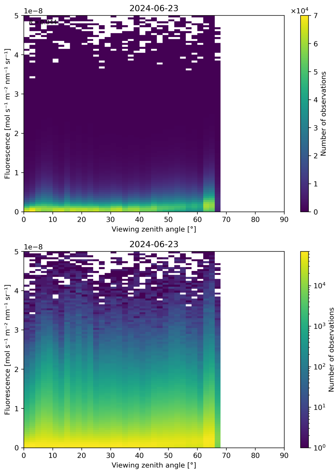
Figure 122: Scatter density plot of “Viewing zenith angle” against “Fluorescence” for 2024-06-22 to 2024-06-24.
