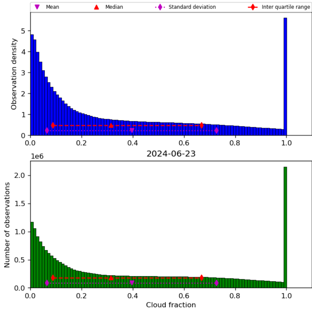
Figure 32: Histogram of “Cloud fraction” for 2024-06-22 to 2024-06-24
