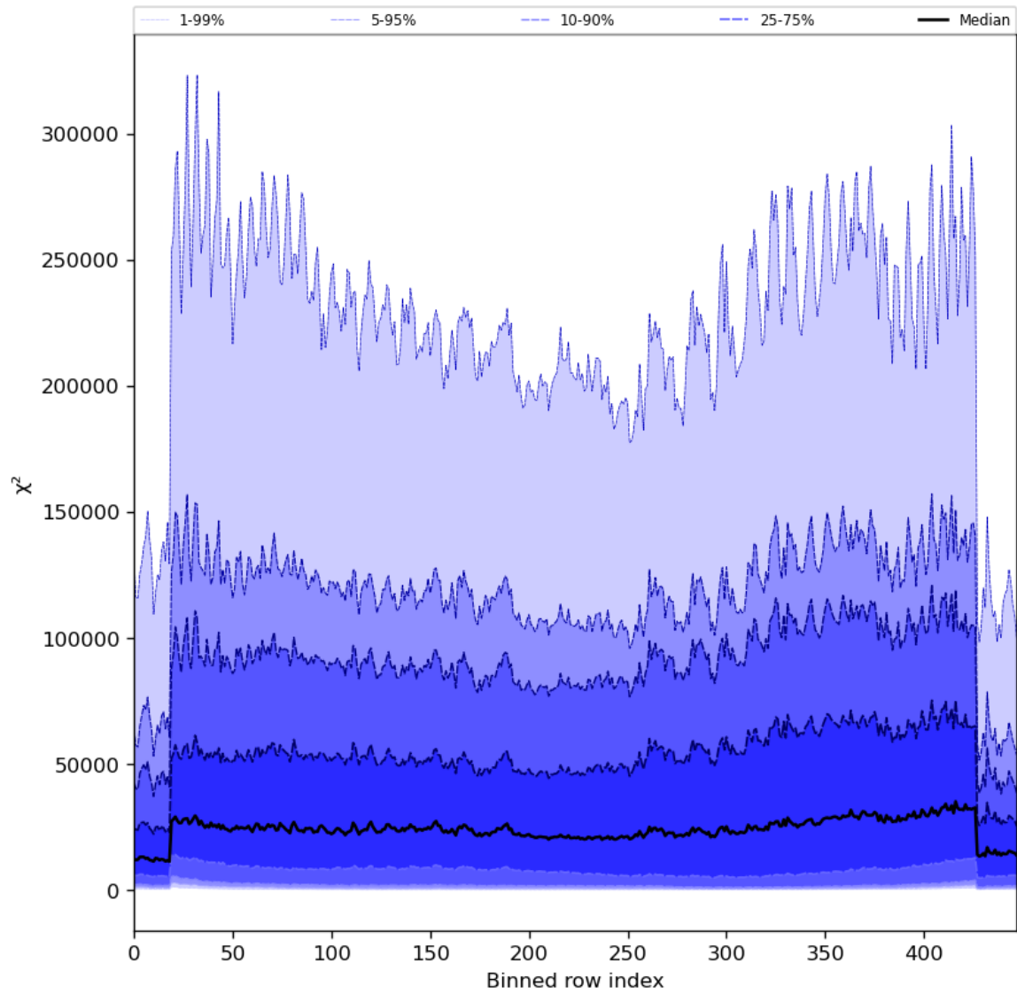
Figure 55: Along track statistics of “ \chi^2 ” for 2024-06-22 to 2024-06-24
