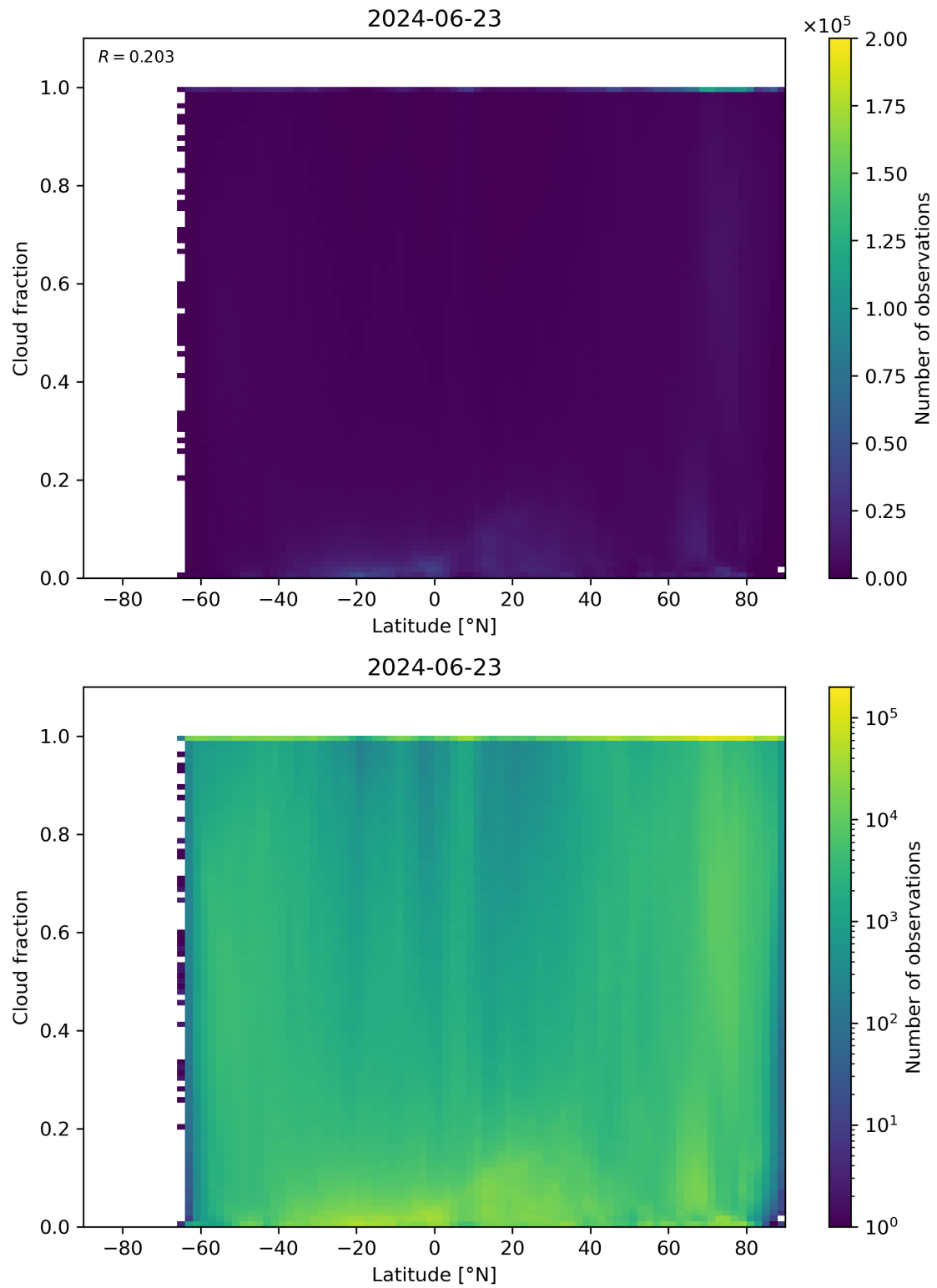
Figure 90: Scatter density plot of “Latitude” against “Cloud fraction” for 2024-06-22 to 2024-06-24.
