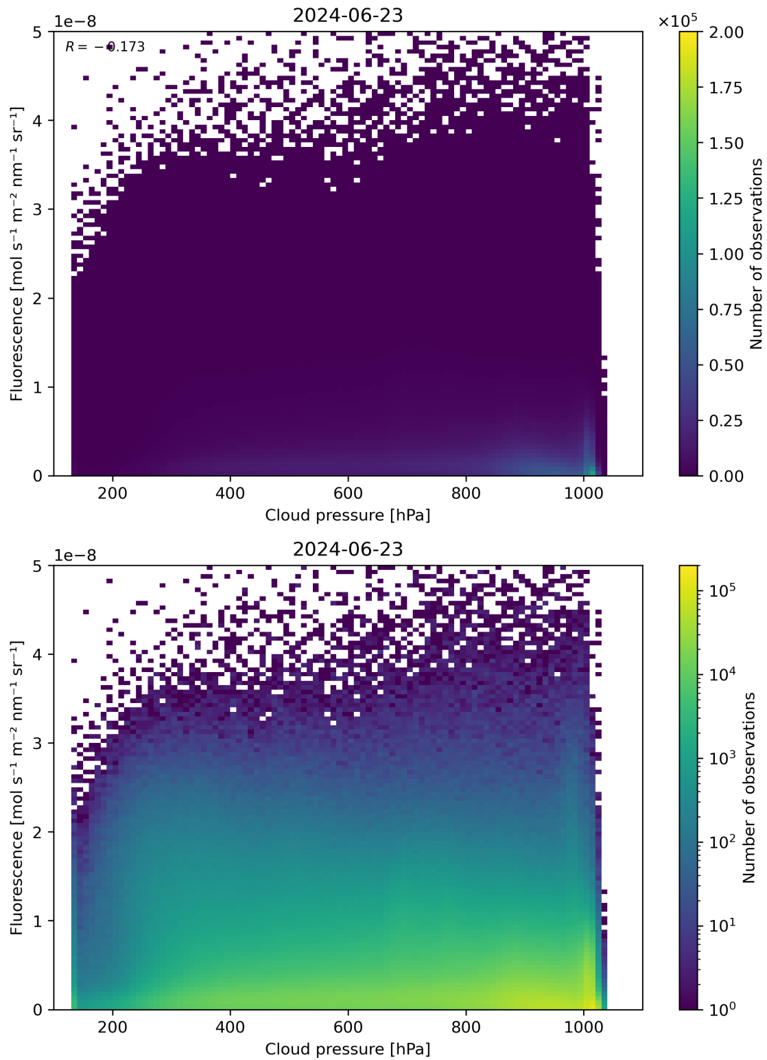
Figure 80: Scatter density plot of “Cloud pressure” against “Fluorescence” for 2024-06-22 to 2024-06-24.
