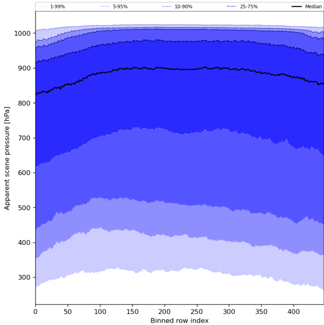
Figure 53: Along track statistics of “Apparent scene pressure” for 2024-06-22 to 2024-06-24
