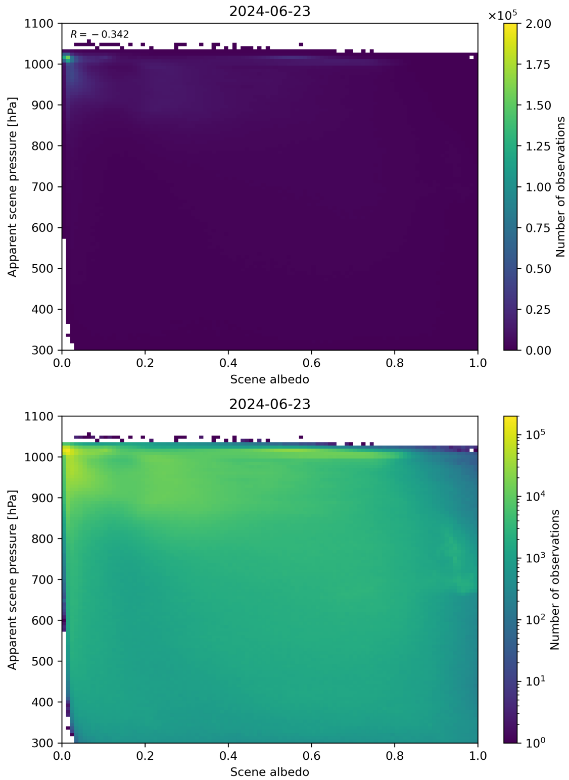
Figure 102: Scatter density plot of “Scene albedo” against “Apparent scene pressure” for 2024-06-22 to 2024-06-24.
