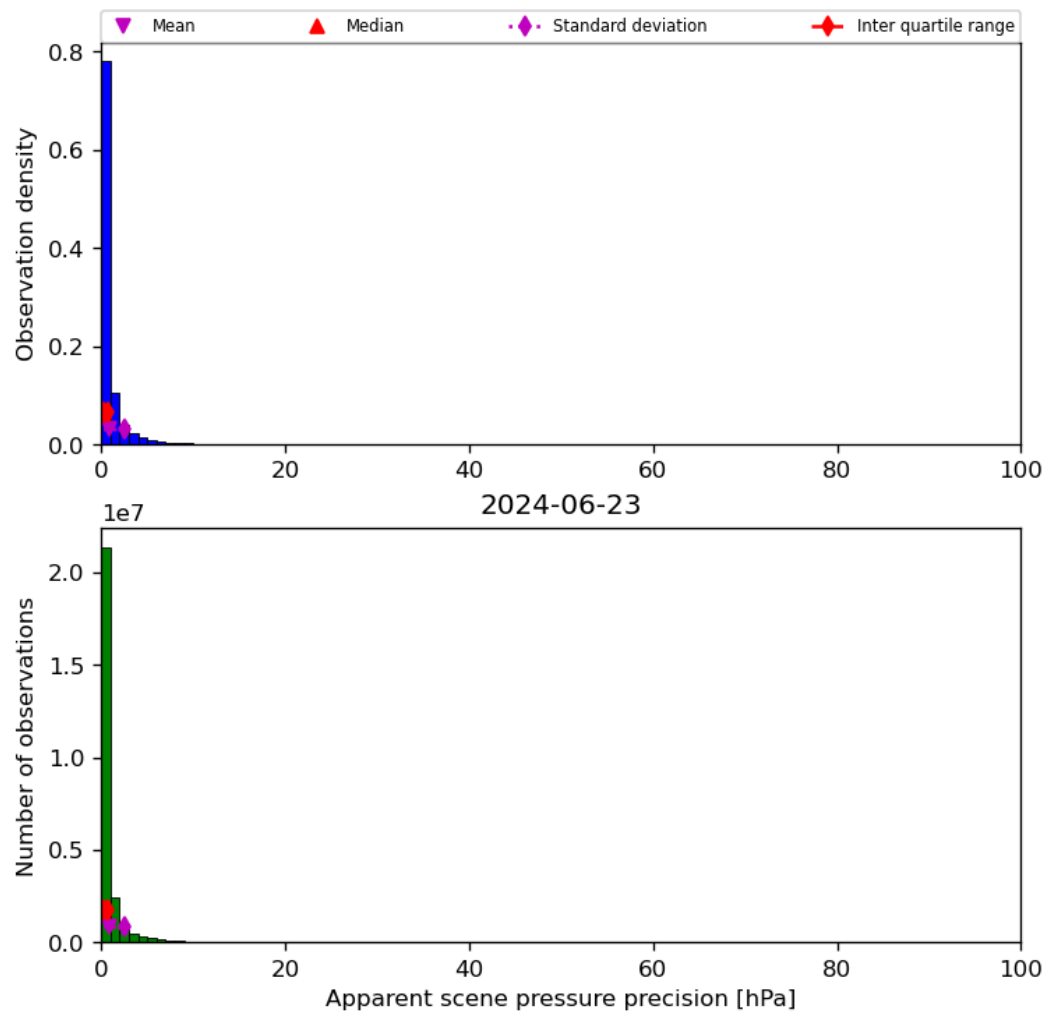
Figure 37: Histogram of “Apparent scene pressure precision” for 2024-06-22 to 2024-06-24
