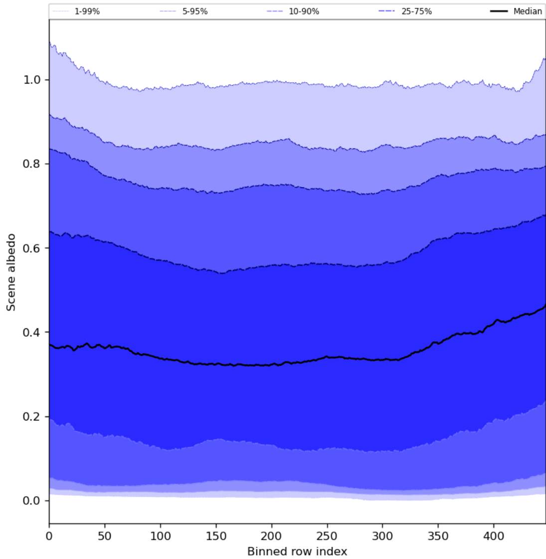
Figure 51: Along track statistics of “Scene albedo” for 2024-06-22 to 2024-06-24
