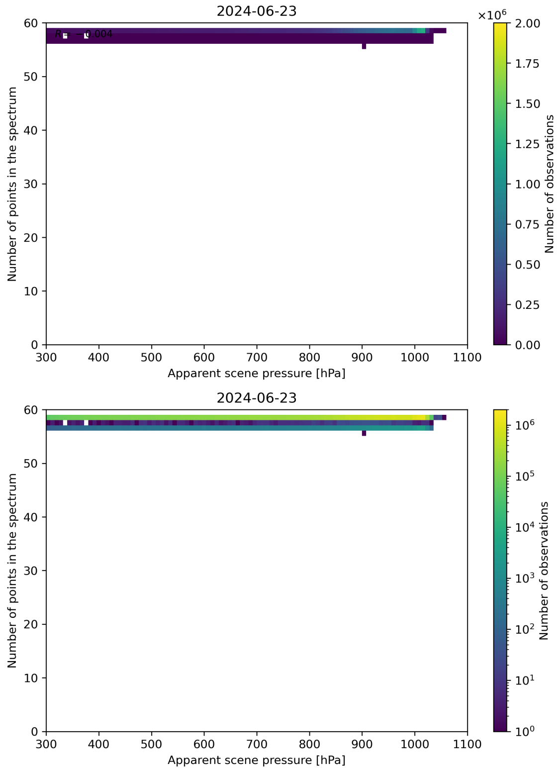
Figure 66: Scatter density plot of “Apparent scene pressure” against “Number of points in the spectrum” for 2024-06-22 to 2024-06-24.
