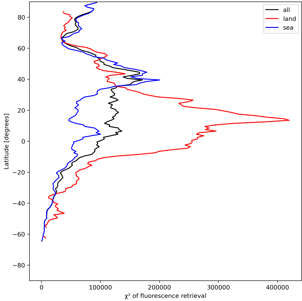
Figure 25: Zonal average of “ \chi^2 of fluorescence retrieval” for 2024-06-22 to 2024-06-24.
