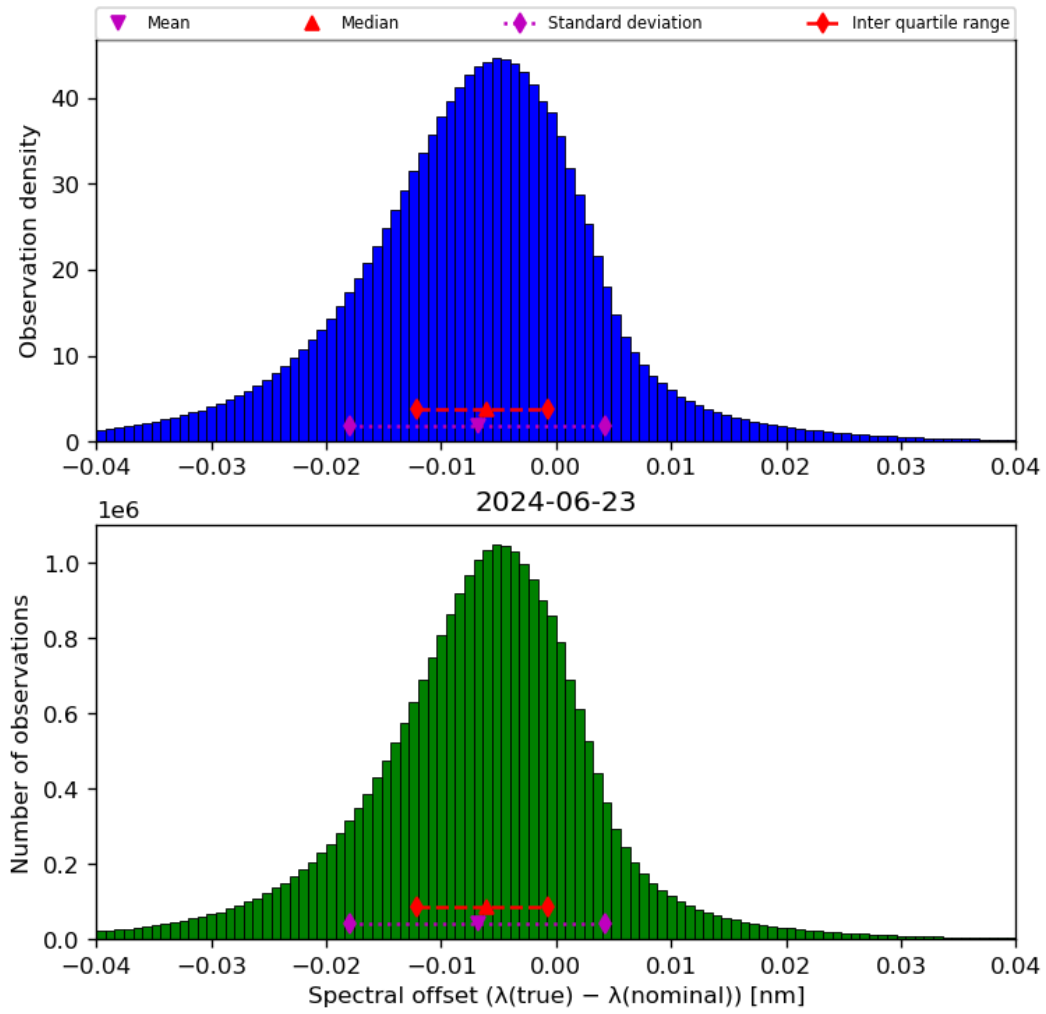
Figure 45: Histogram of “Spectral offset ( \lambda(\text{true}) - \lambda(\text{nominal}) )” for 2024-06-22 to 2024-06-24
