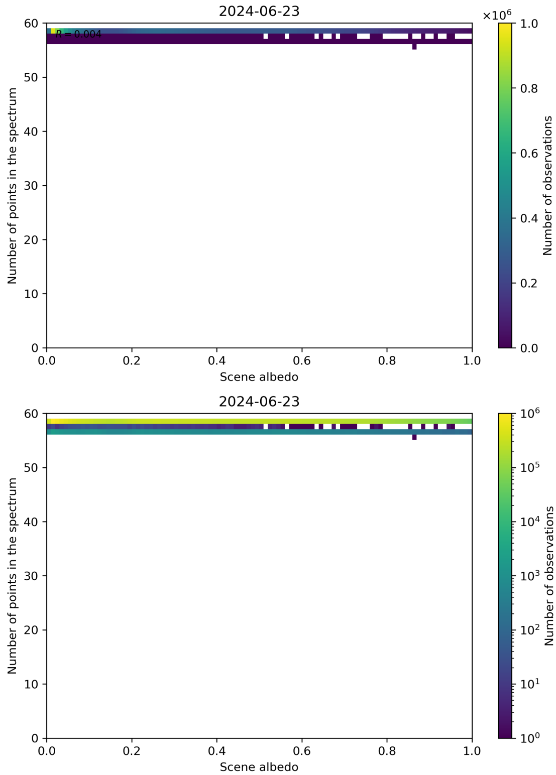
Figure 106: Scatter density plot of “Scene albedo” against “Number of points in the spectrum” for 2024-06-22 to 2024-06-24.
