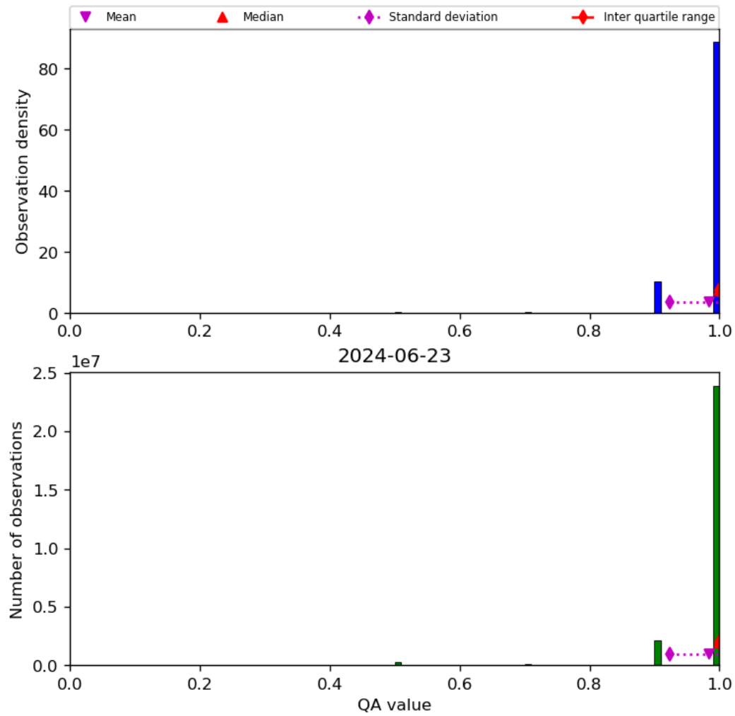
Figure 29: Histogram of “QA value” for 2024-06-22 to 2024-06-24
