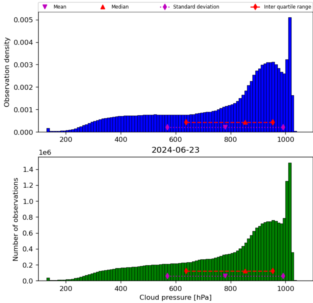
Figure 30: Histogram of “Cloud pressure” for 2024-06-22 to 2024-06-24
