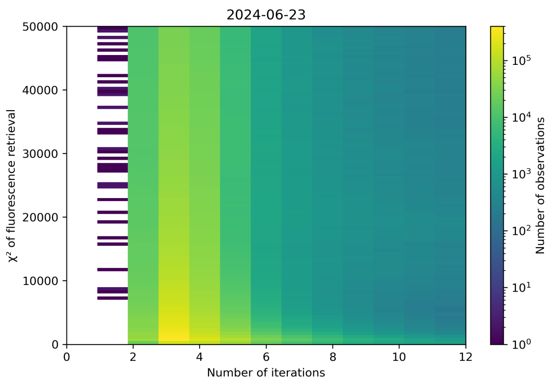
Figure 97: Scatter density plot of “Number of iterations” against “ \chi^2 of fluorescence retrieval” for 2024-06-22 to 2024-06-24.
