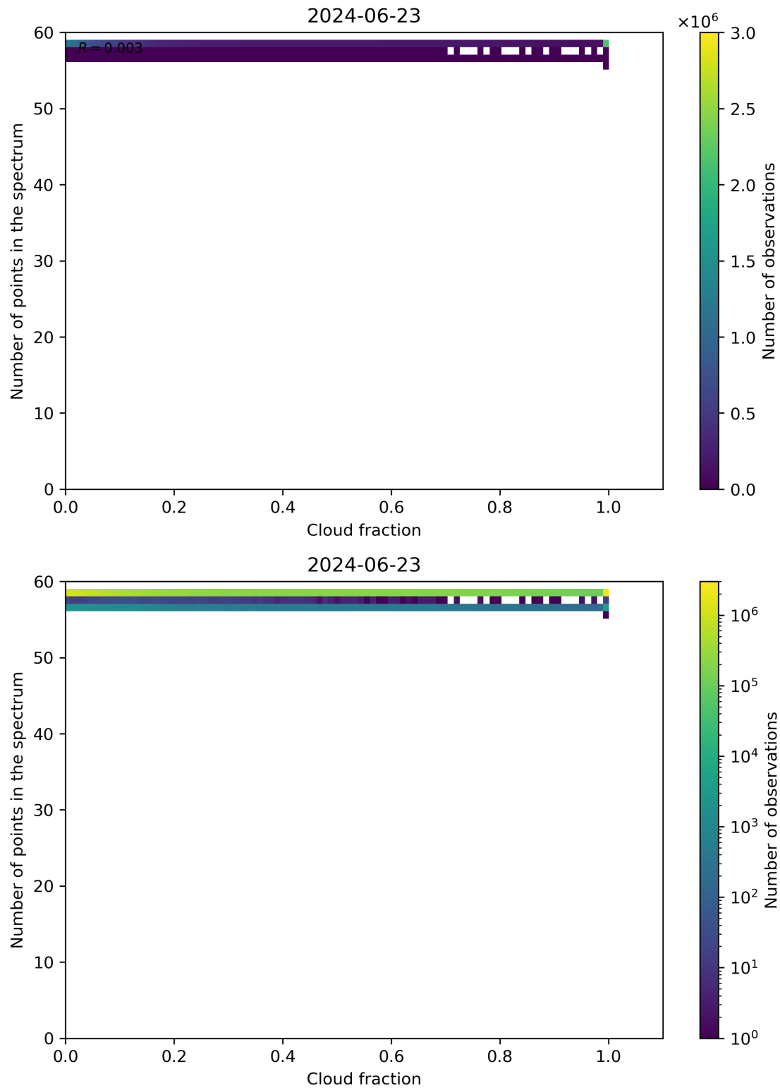
Figure 74: Scatter density plot of “Cloud fraction” against “Number of points in the spectrum” for 2024-06-22 to 2024-06-24.
