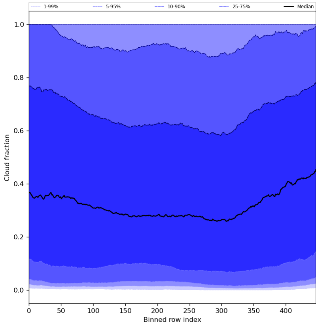
Figure 49: Along track statistics of “Cloud fraction” for 2024-06-22 to 2024-06-24
