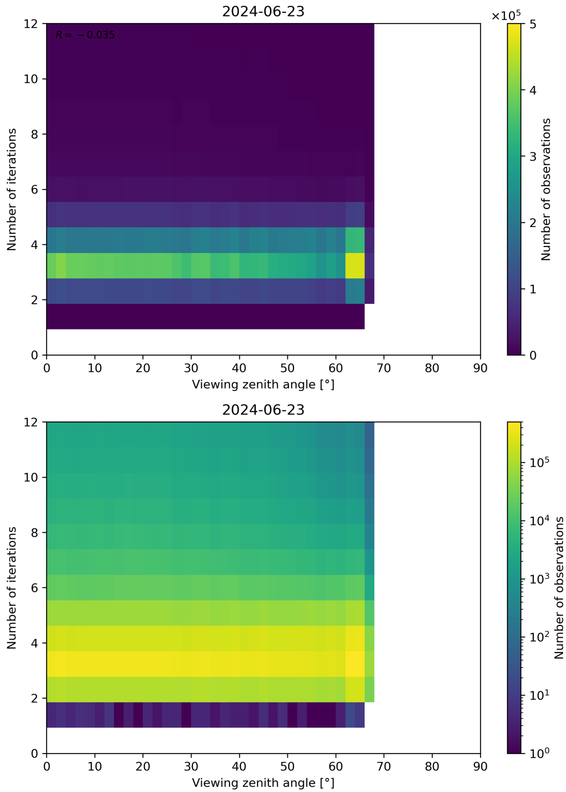
Figure 124: Scatter density plot of “Viewing zenith angle” against “Number of iterations” for 2024-06-22 to 2024-06-24.
