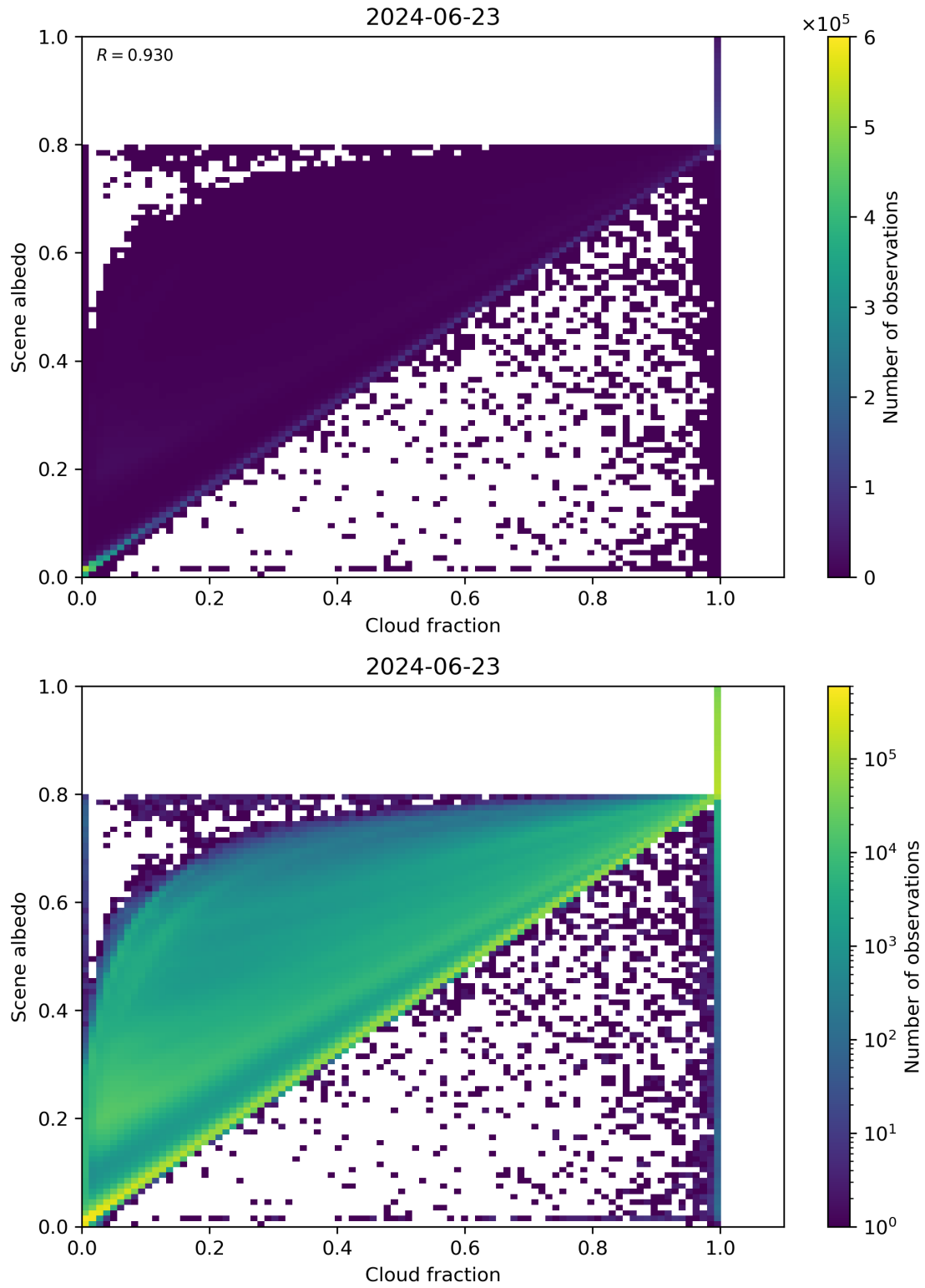
Figure 75: Scatter density plot of “Cloud fraction” against “Scene albedo” for 2024-06-22 to 2024-06-24.
