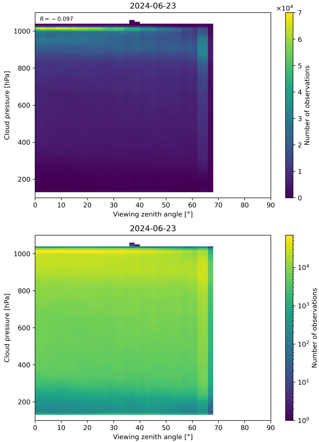
Figure 121: Scatter density plot of “Viewing zenith angle” against “Cloud pressure” for 2024-06-22 to 2024-06-24.
