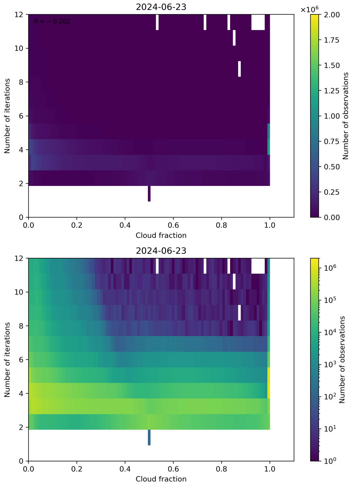
Figure 73: Scatter density plot of “Cloud fraction” against “Number of iterations” for 2024-06-22 to 2024-06-24.
