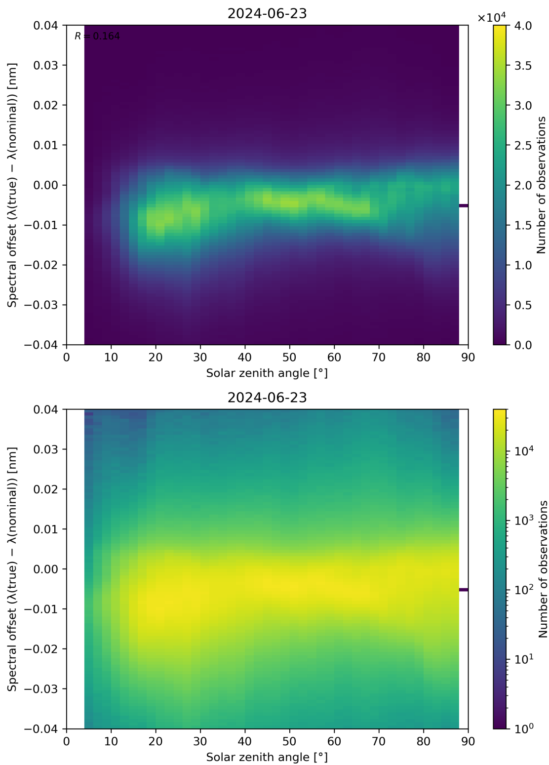
Figure 117: Scatter density plot of “Solar zenith angle” against “Spectral offset ( \lambda(\text{true}) - \lambda(\text{nominal}) )” for 2024-06-22 to 2024-06-24.
