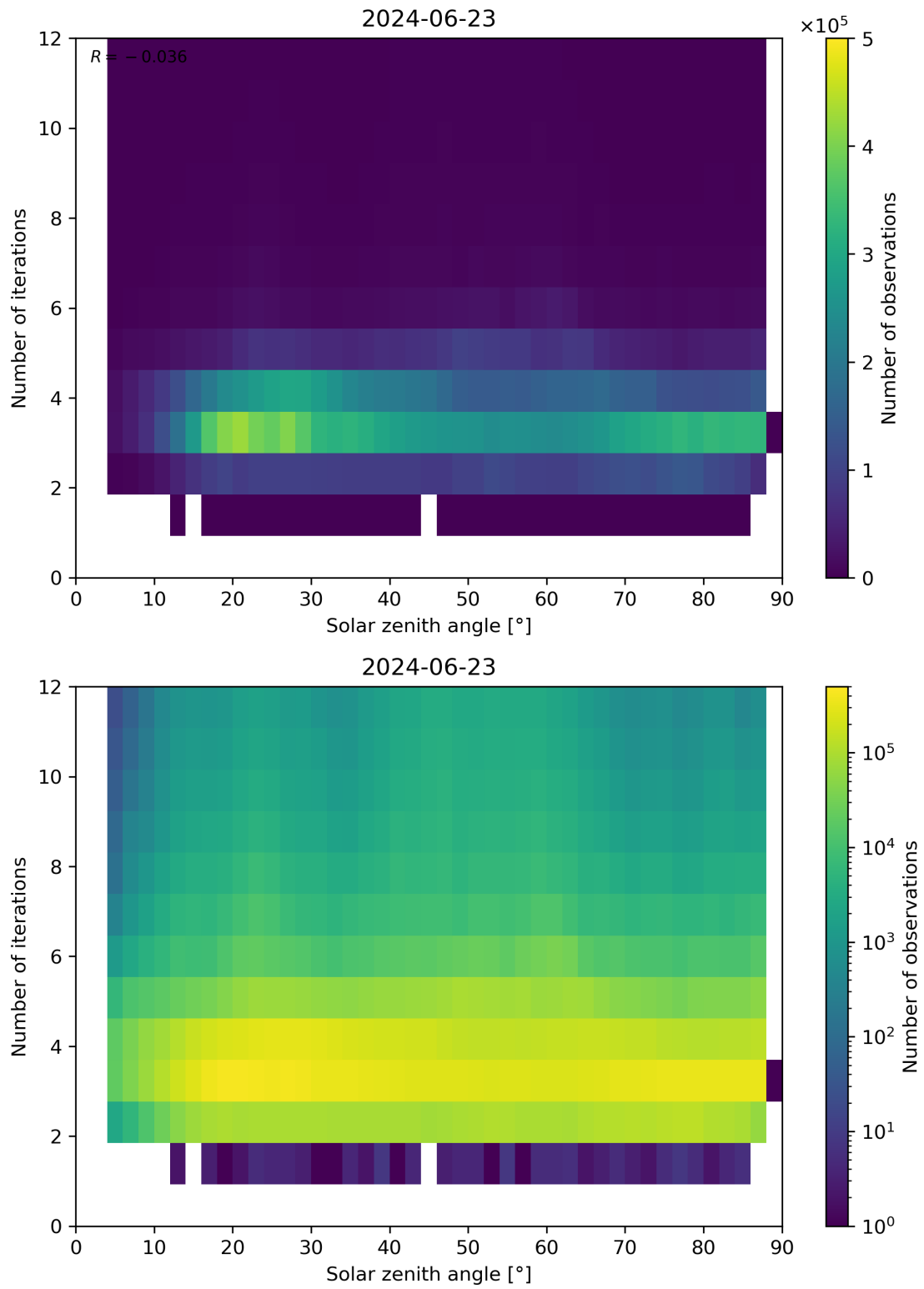
Figure 114: Scatter density plot of “Solar zenith angle” against “Number of iterations” for 2024-06-22 to 2024-06-24.
