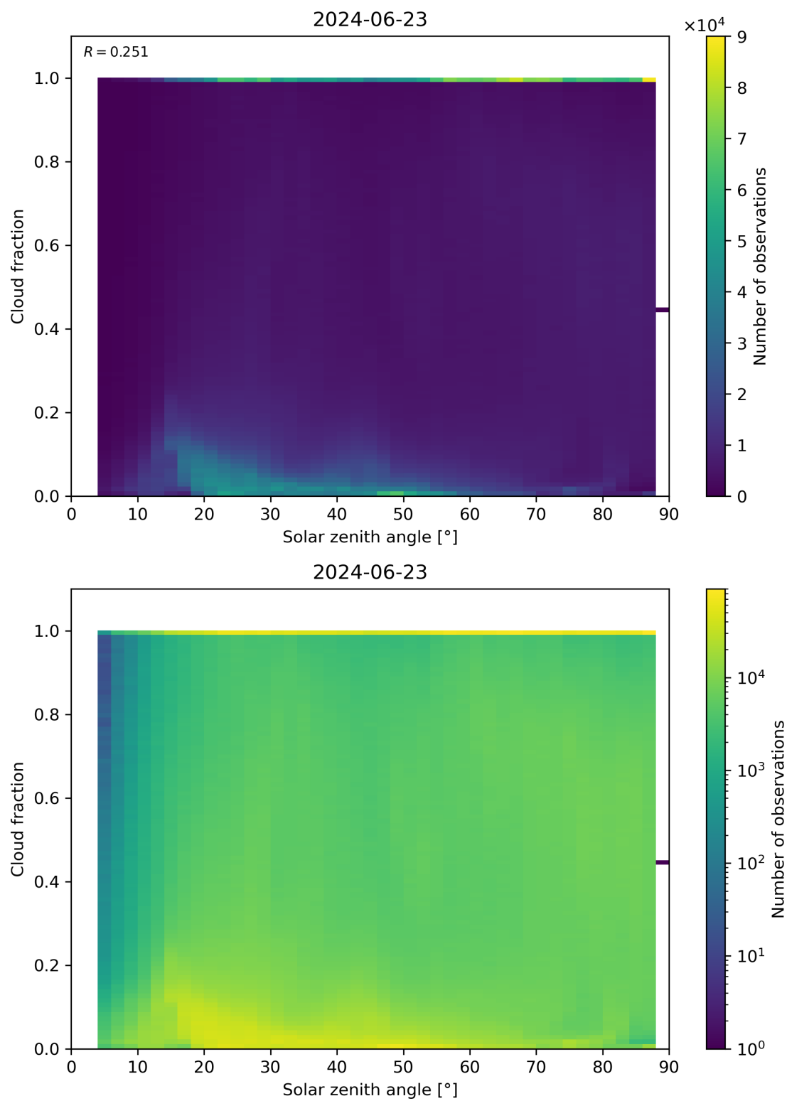
Figure 110: Scatter density plot of “Solar zenith angle” against “Cloud fraction” for 2024-06-22 to 2024-06-24.
