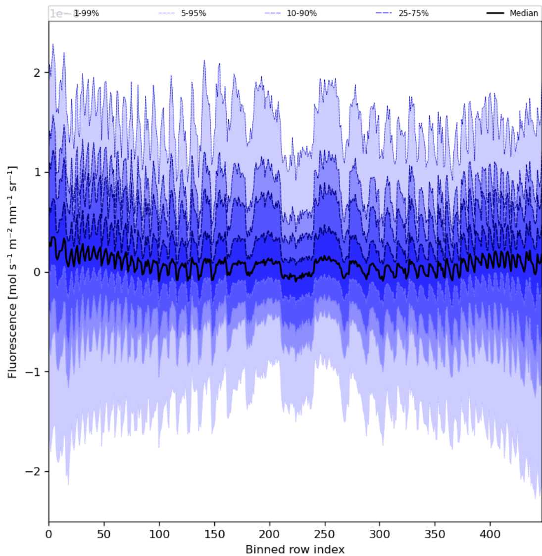
Figure 57: Along track statistics of “Fluorescence” for 2024-06-22 to 2024-06-24
