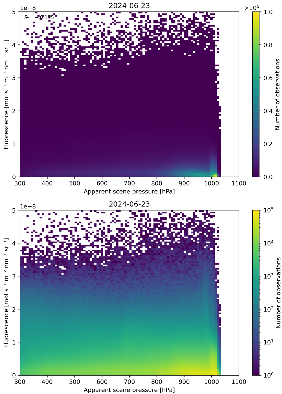
Figure 64: Scatter density plot of “Apparent scene pressure” against “Fluorescence” for 2024-06-22 to 2024-06-24.
