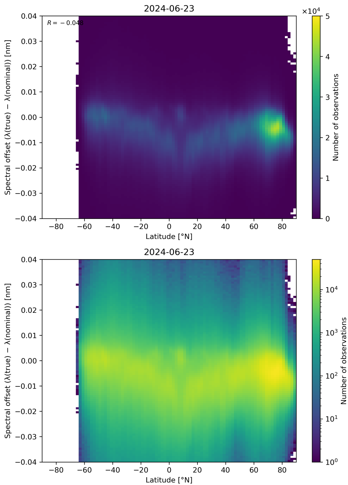
Figure 96: Scatter density plot of “Latitude” against “Spectral offset ( \lambda(\text{true}) - \lambda(\text{nominal}) )” for 2024-06-22 to 2024-06-24.
