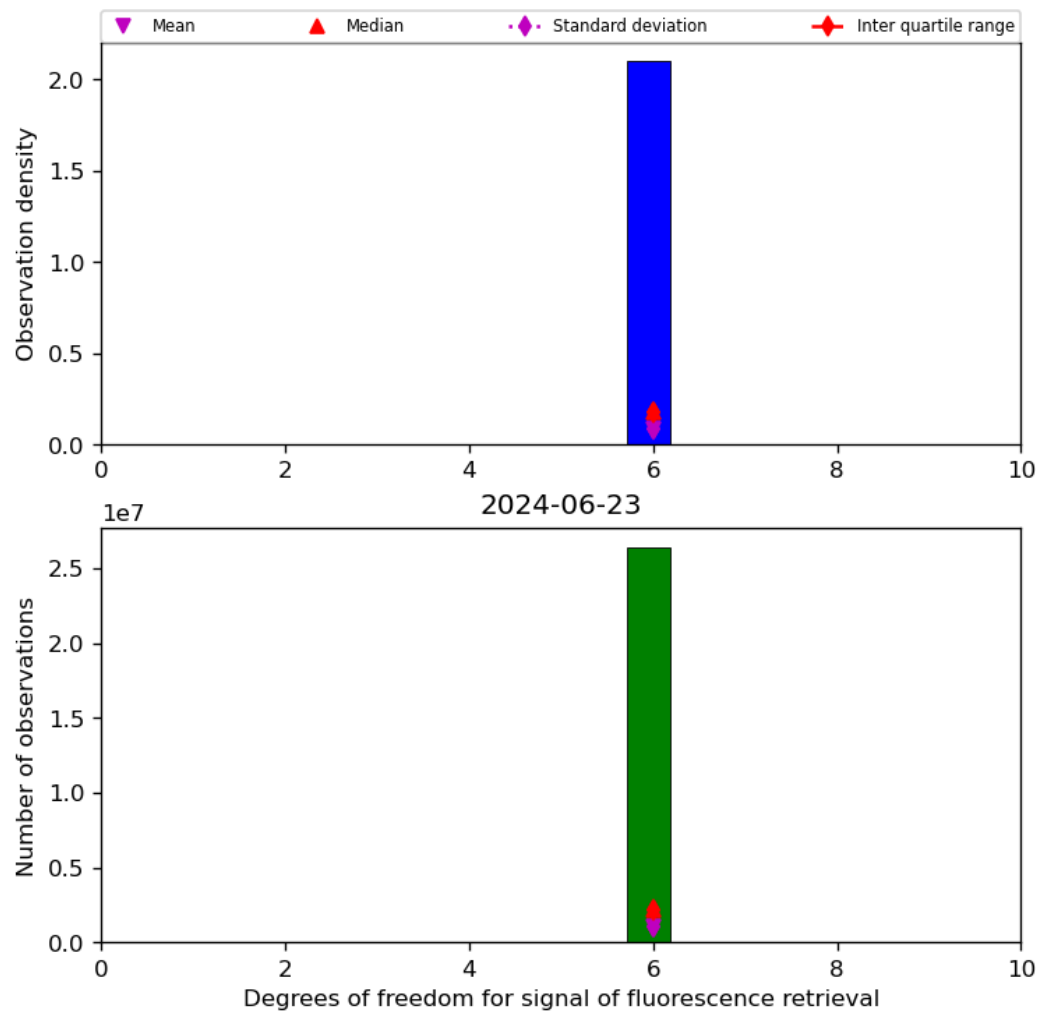
Figure 43: Histogram of “Degrees of freedom for signal of fluorescence retrieval” for 2024-06-22 to 2024-06-24
