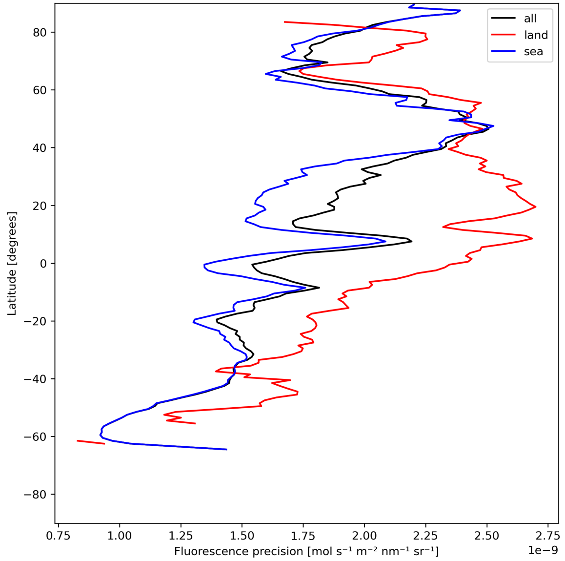
Figure 24: Zonal average of “Fluorescence precision” for 2024-06-22 to 2024-06-24.
