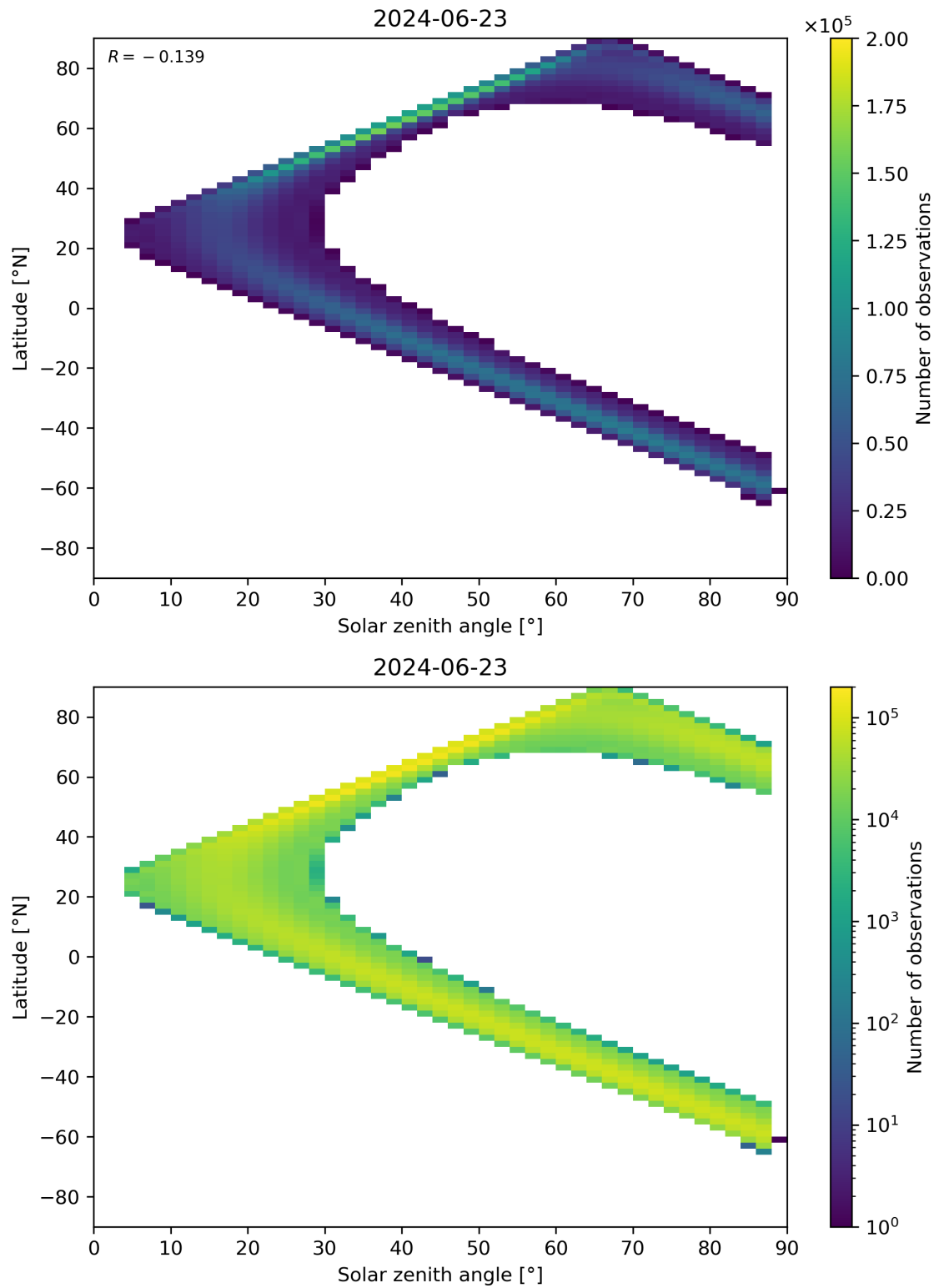
Figure 113: Scatter density plot of “Solar zenith angle” against “Latitude” for 2024-06-22 to 2024-06-24.
