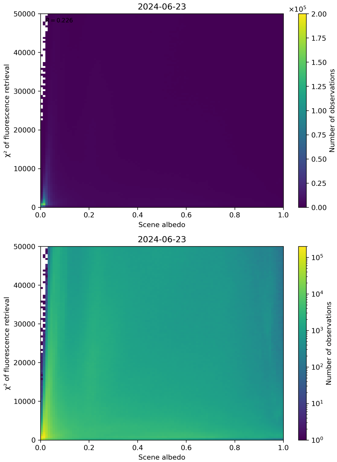
Figure 103: Scatter density plot of “Scene albedo” against “ \chi^2 of fluorescence retrieval” for 2024-06-22 to 2024-06-24.
