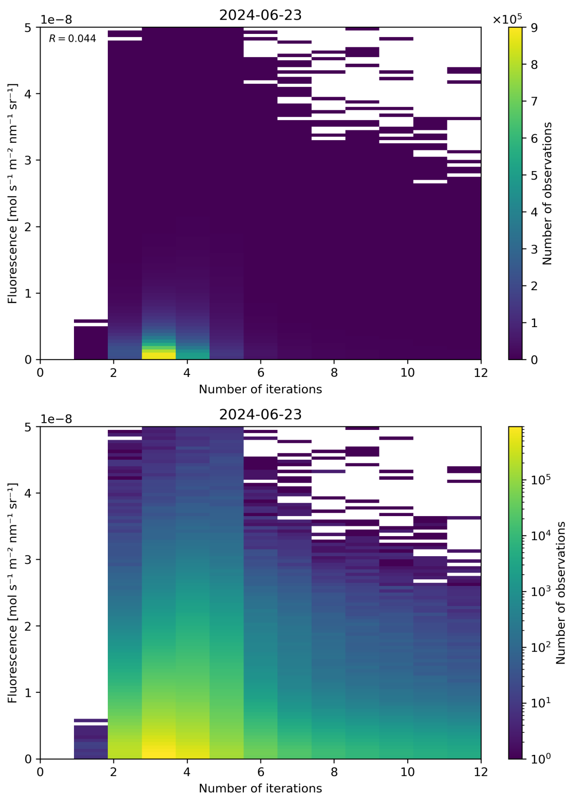
Figure 98: Scatter density plot of “Number of iterations” against “Fluorescence” for 2024-06-22 to 2024-06-24.
