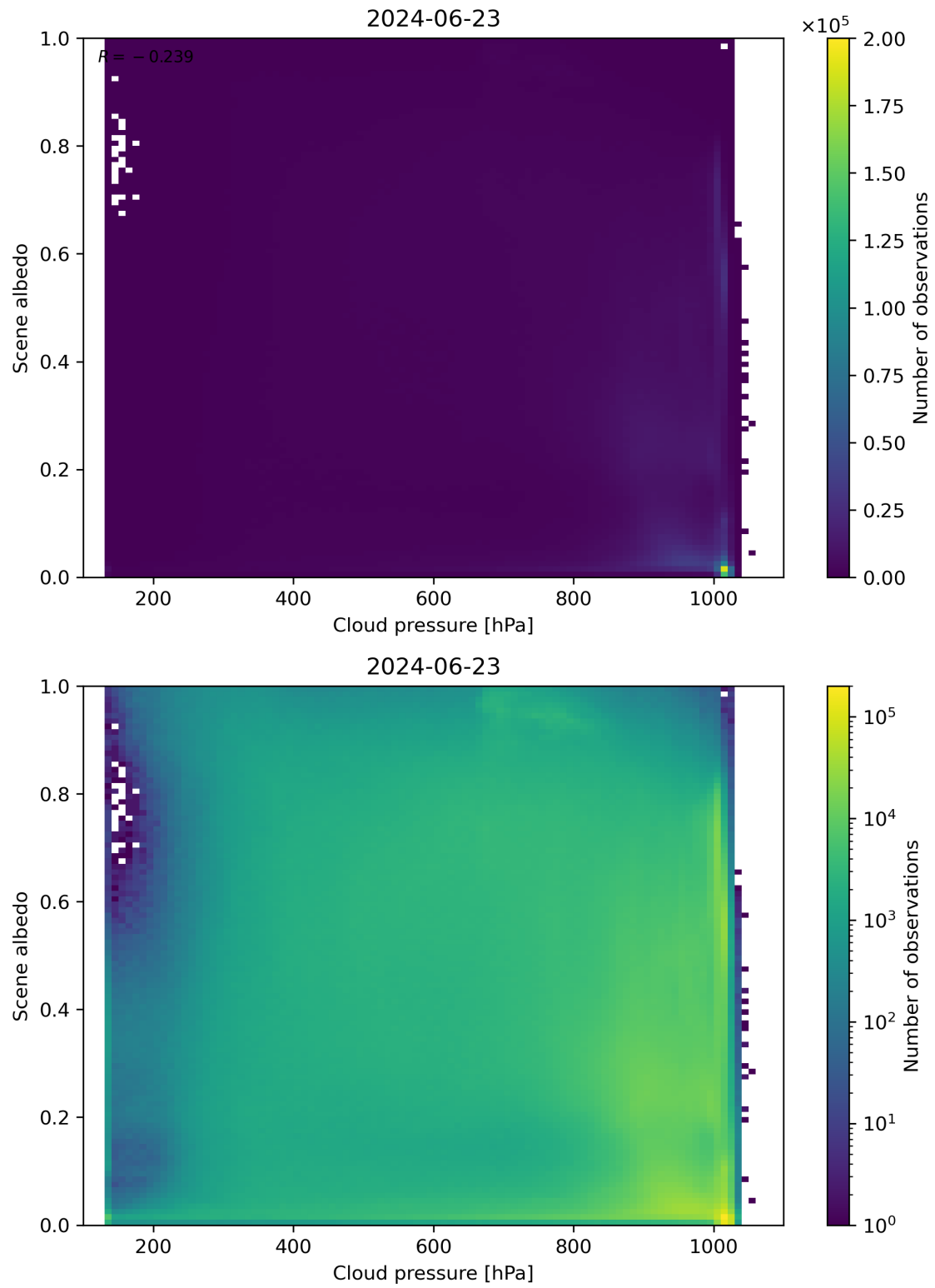
Figure 83: Scatter density plot of “Cloud pressure” against “Scene albedo” for 2024-06-22 to 2024-06-24.
