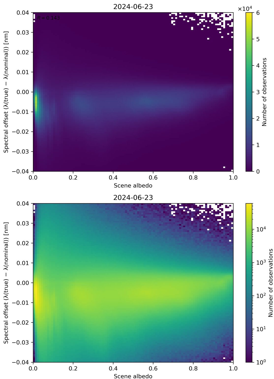
Figure 107: Scatter density plot of “Scene albedo” against “Spectral offset ( \lambda(\text{true}) - \lambda(\text{nominal}) )” for 2024-06-22 to 2024-06-24.
