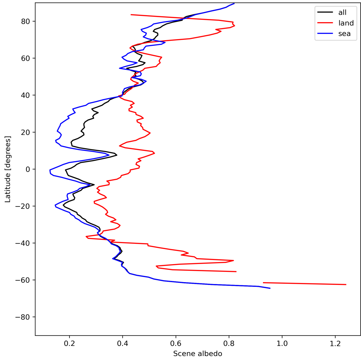
Figure 17: Zonal average of “Scene albedo” for 2024-06-22 to 2024-06-24.
