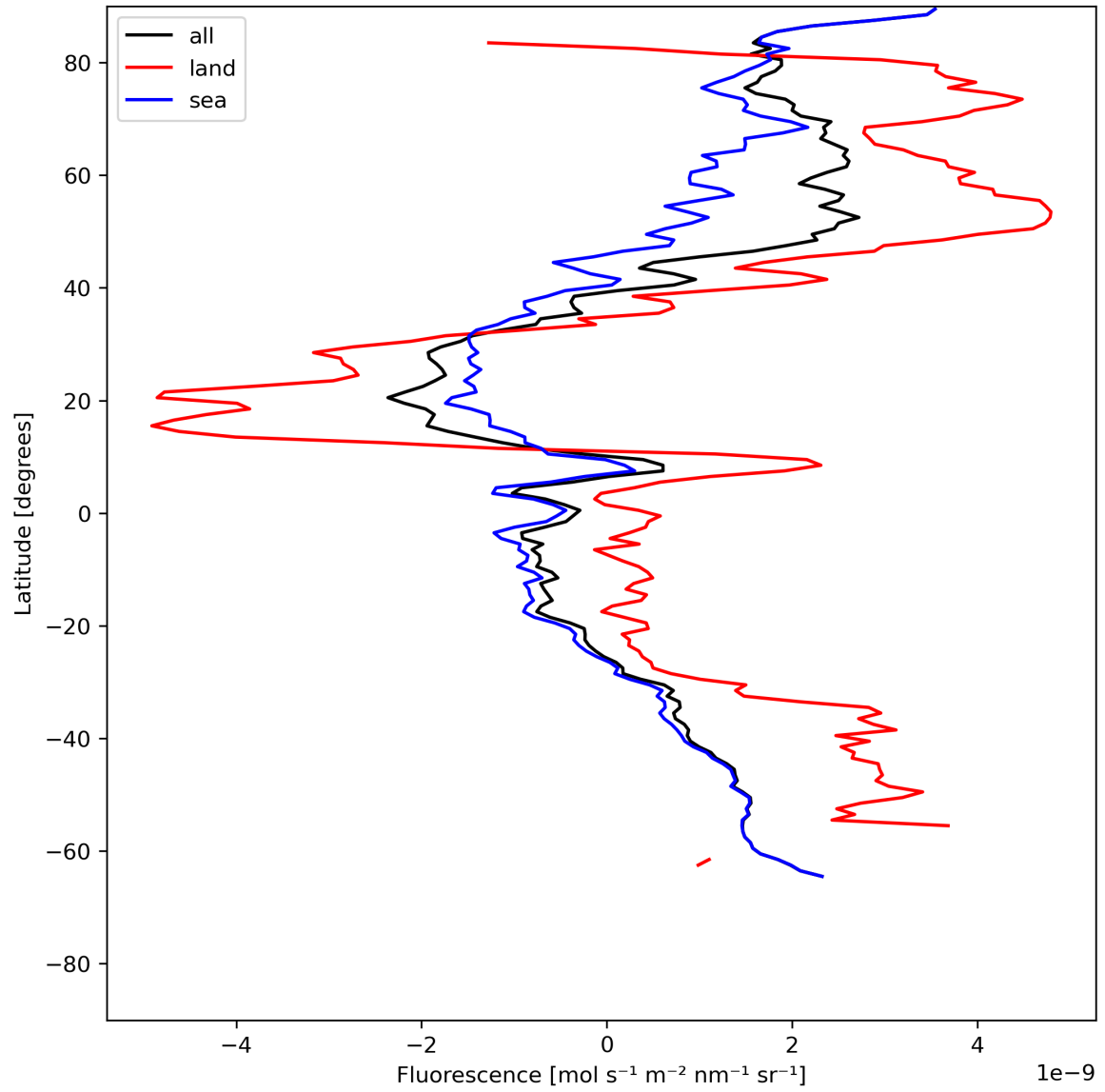
Figure 23: Zonal average of “Fluorescence” for 2024-06-22 to 2024-06-24.
