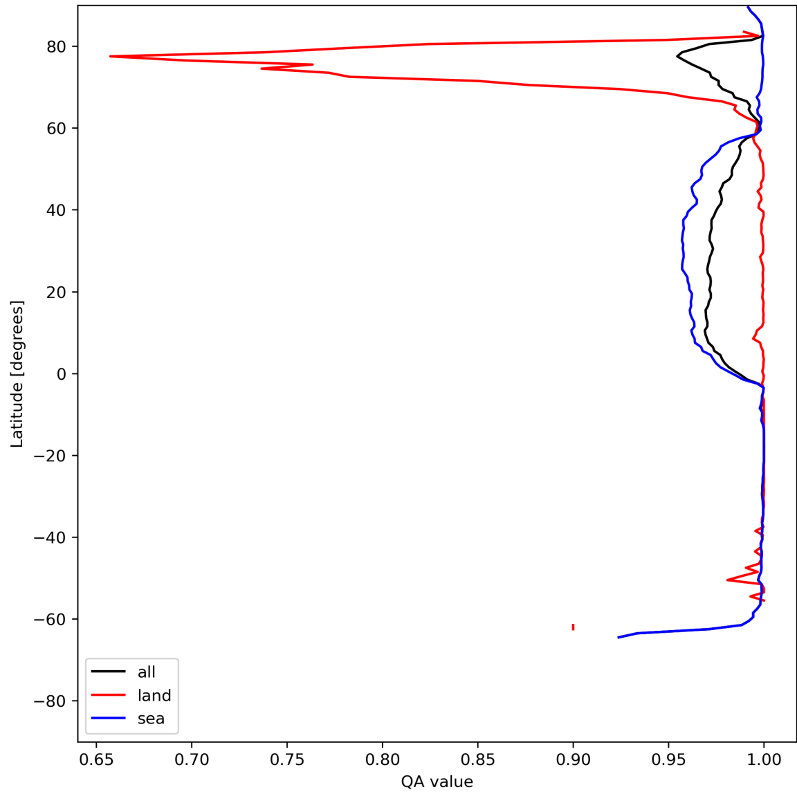
Figure 12: Zonal average of “QA value” for 2024-06-22 to 2024-06-24.
