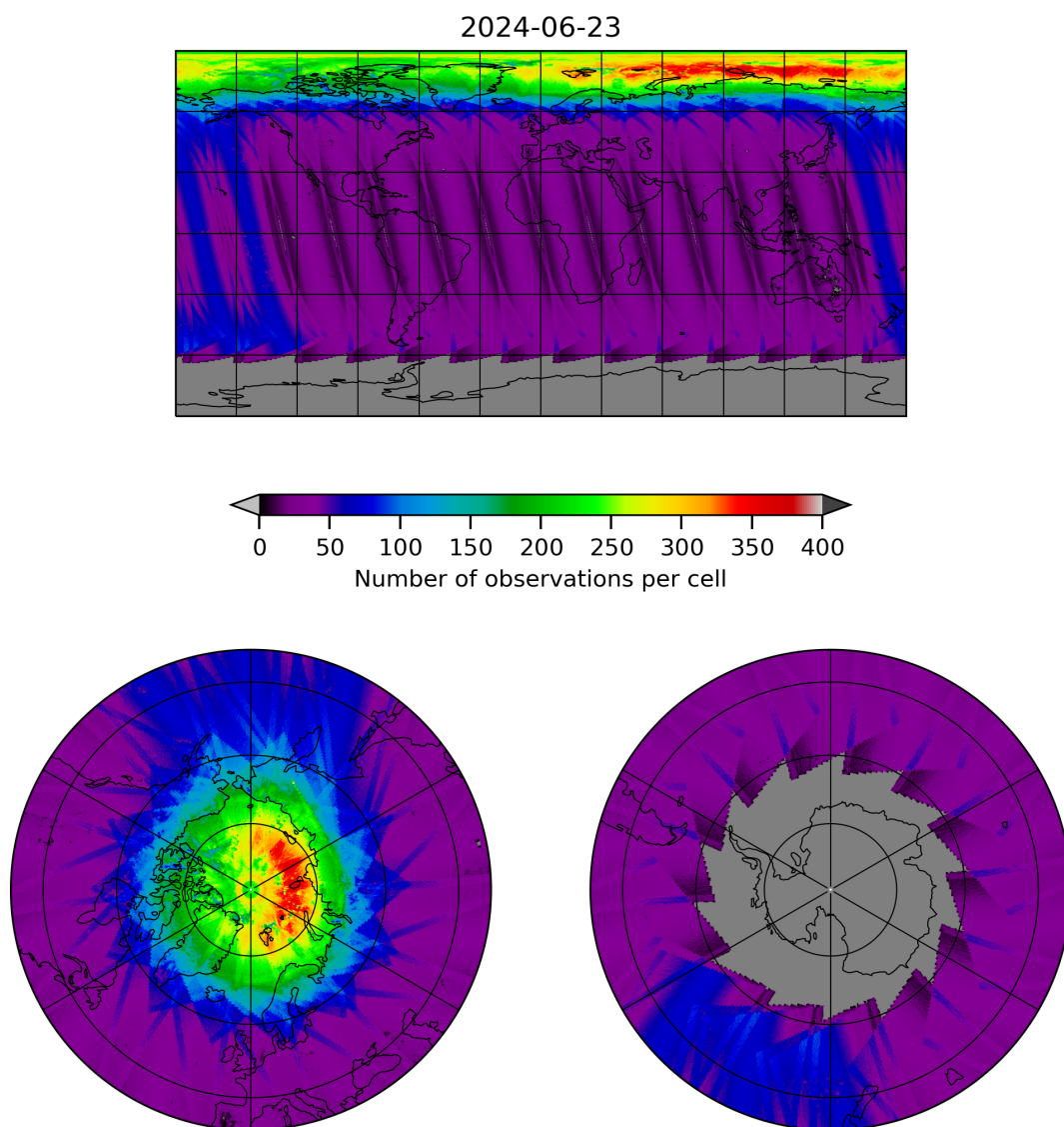
Figure 11: Map of the number of observations for 2024-06-22 to 2024-06-24
