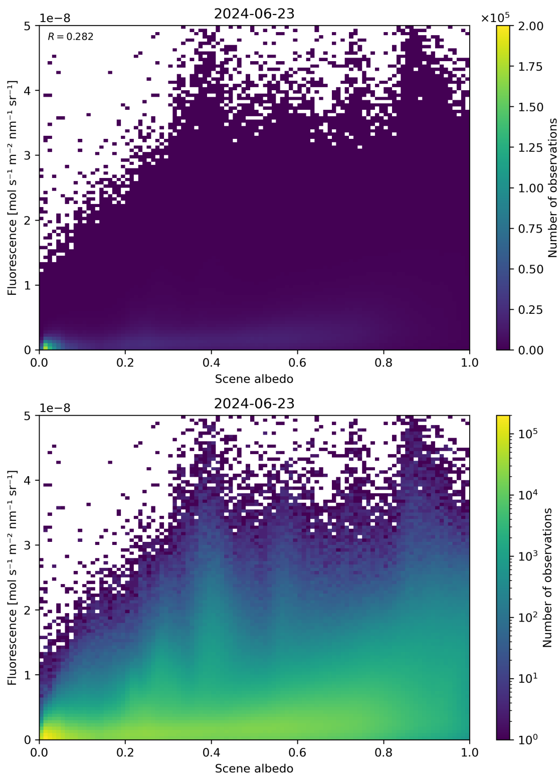
Figure 104: Scatter density plot of “Scene albedo” against “Fluorescence” for 2024-06-22 to 2024-06-24.
