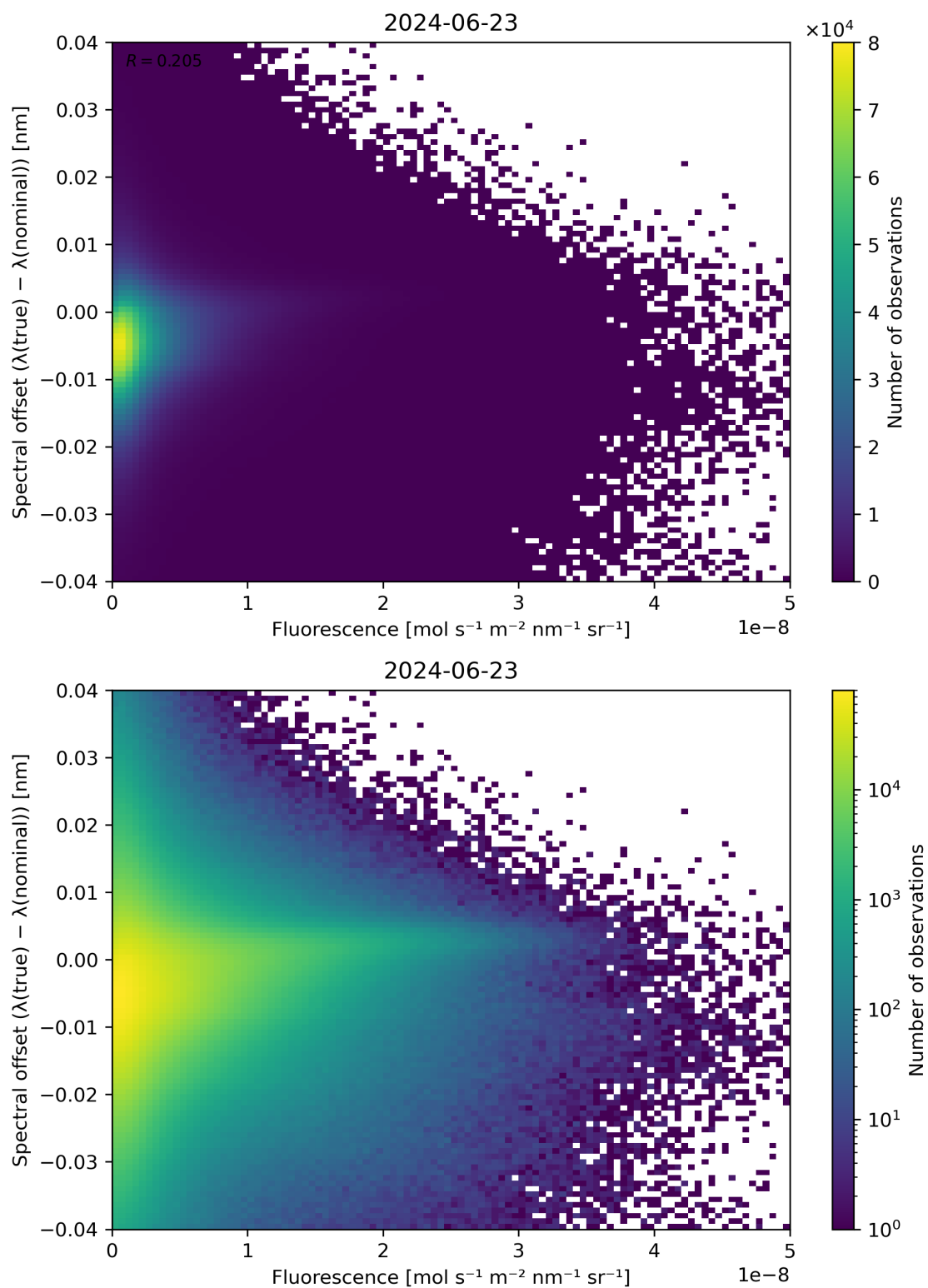
Figure 87: Scatter density plot of “Fluorescence” against “Spectral offset ( \lambda(\text{true}) - \lambda(\text{nominal}) )” for 2024-06-22 to 2024-06-24.
