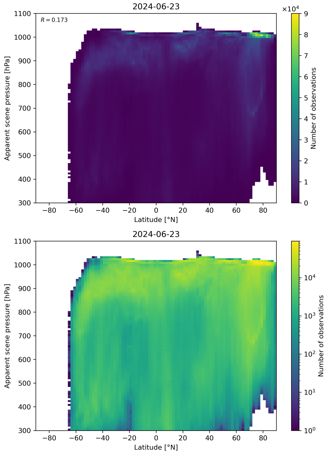
Figure 88: Scatter density plot of “Latitude” against “Apparent scene pressure” for 2024-06-22 to 2024-06-24.
