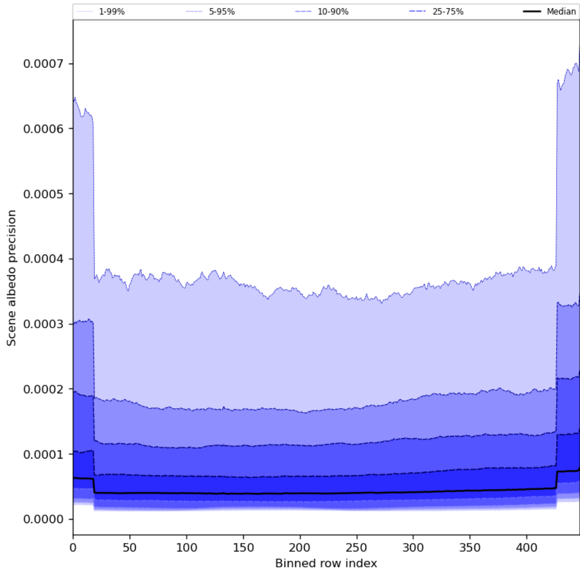
Figure 52: Along track statistics of “Scene albedo precision” for 2024-06-22 to 2024-06-24
