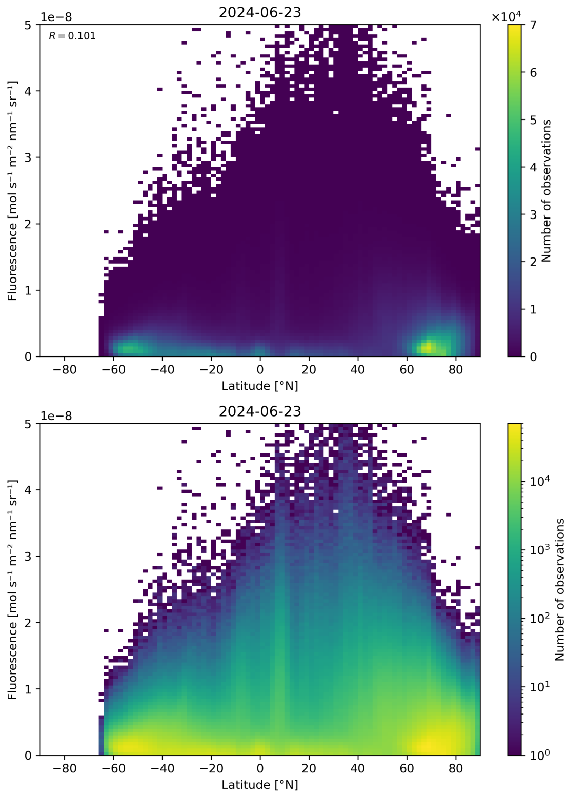
Figure 92: Scatter density plot of “Latitude” against “Fluorescence” for 2024-06-22 to 2024-06-24.
