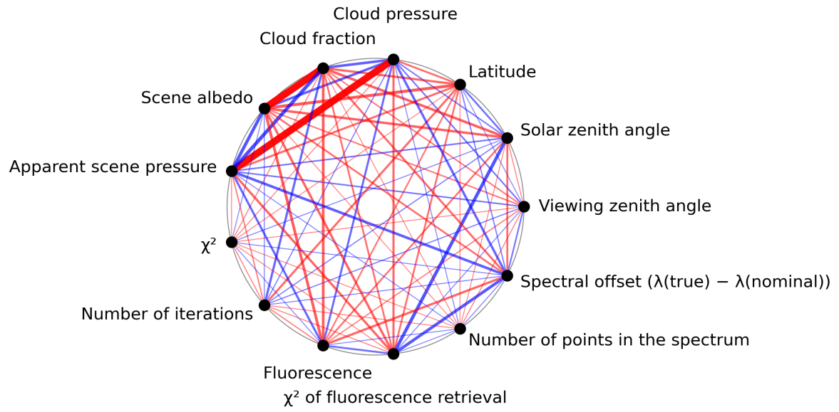
Figure 1: Map of correlation graph for 2024-06-22 to 2024-06-24.
