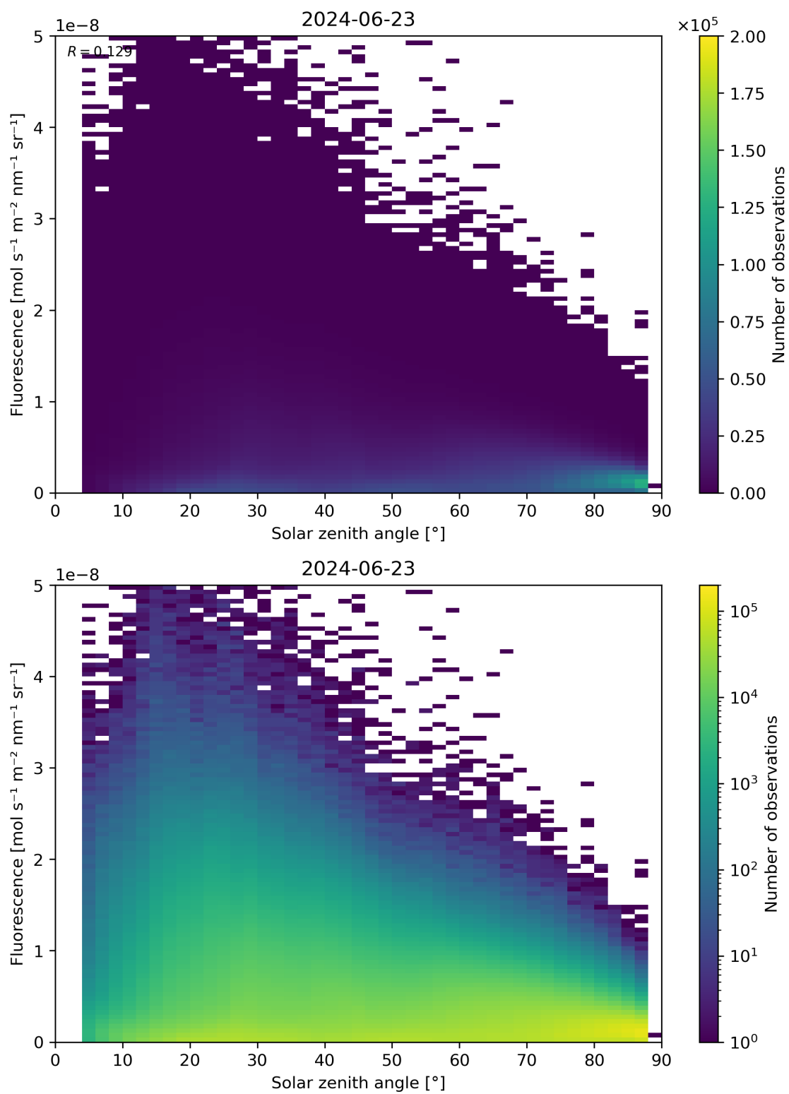
Figure 112: Scatter density plot of “Solar zenith angle” against “Fluorescence” for 2024-06-22 to 2024-06-24.
