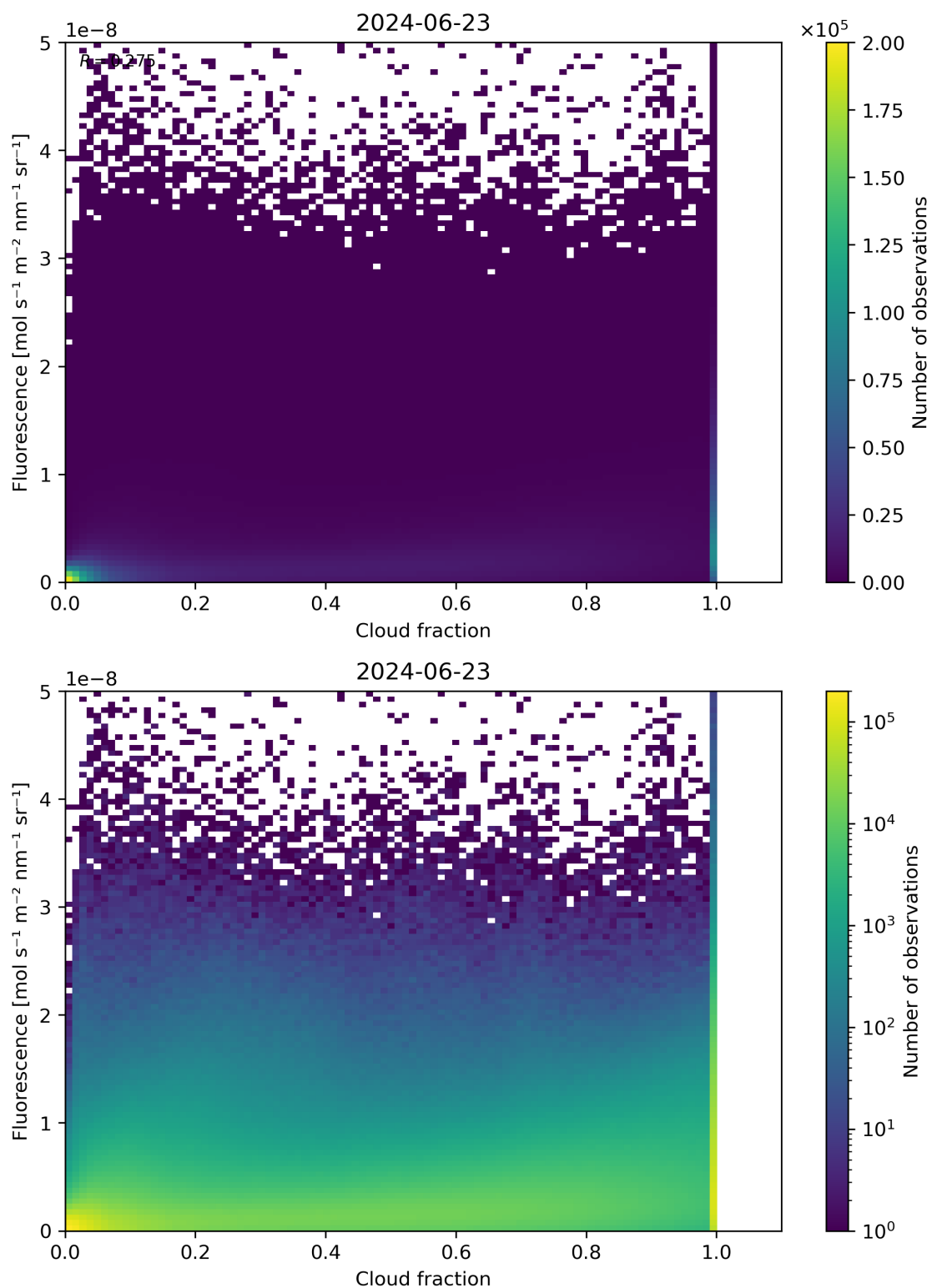
Figure 72: Scatter density plot of “Cloud fraction” against “Fluorescence” for 2024-06-22 to 2024-06-24.
