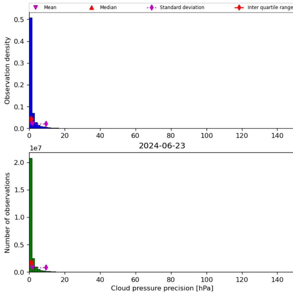
Figure 31: Histogram of “Cloud pressure precision” for 2024-06-22 to 2024-06-24
