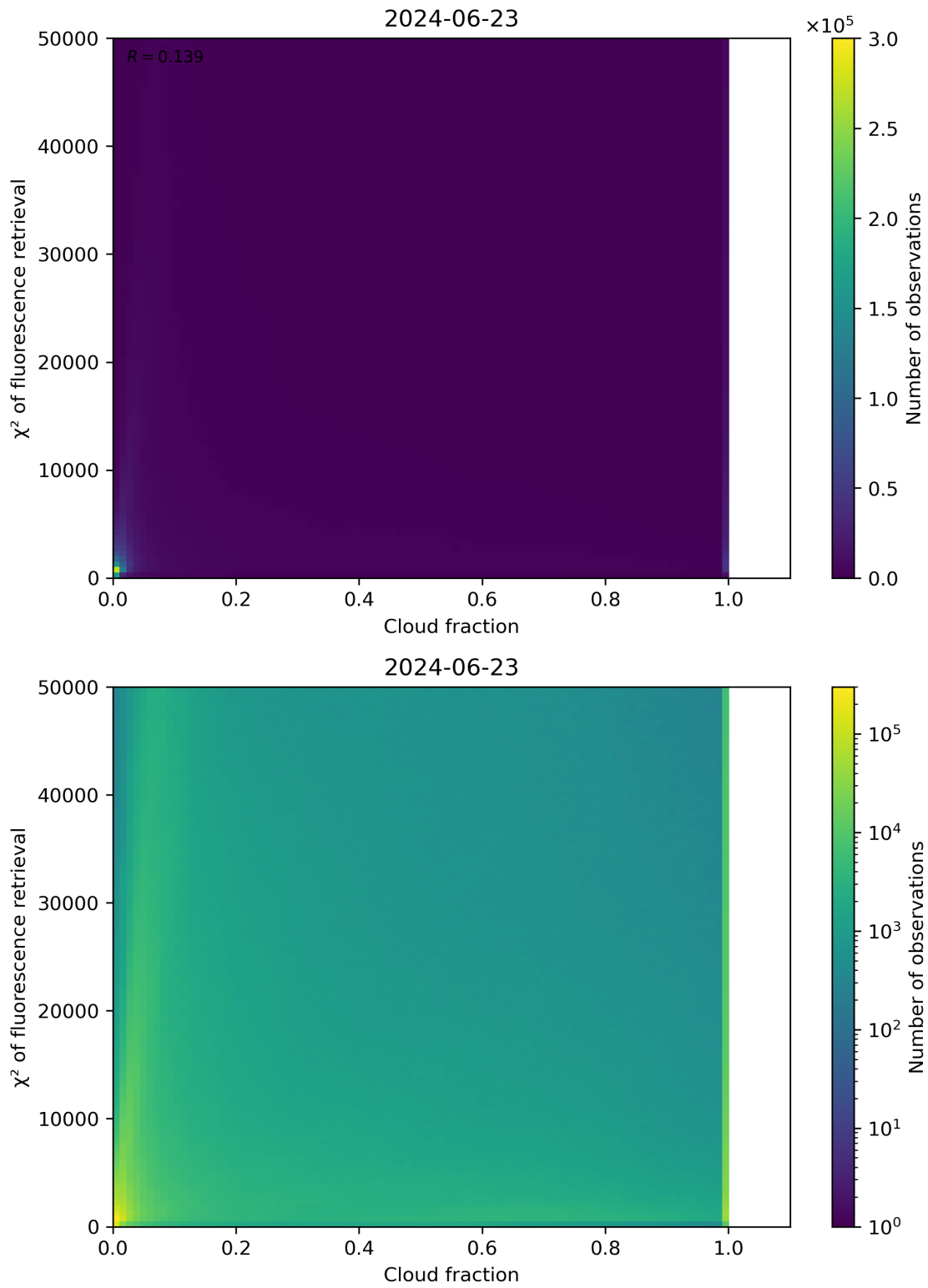
Figure 71: Scatter density plot of “Cloud fraction” against “ \chi^2 of fluorescence retrieval” for 2024-06-22 to 2024-06-24.
