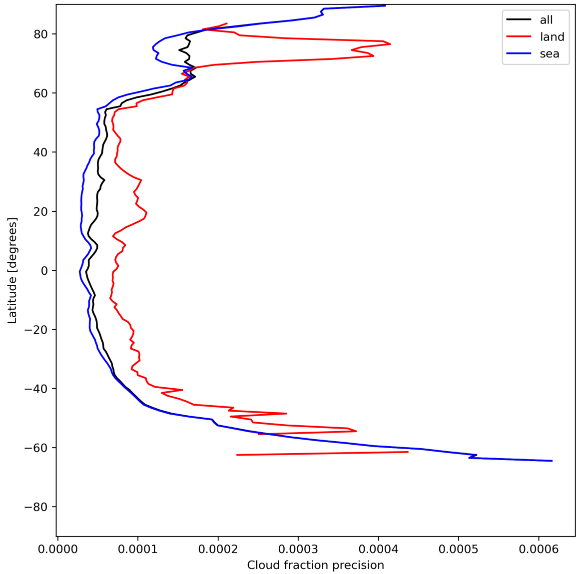
Figure 16: Zonal average of “Cloud fraction precision” for 2024-06-22 to 2024-06-24.
