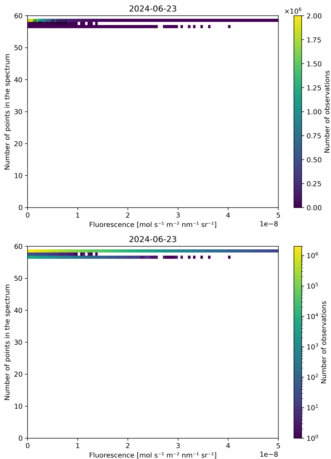
Figure 86: Scatter density plot of “Fluorescence” against “Number of points in the spectrum” for 2024-06-22 to 2024-06-24.
