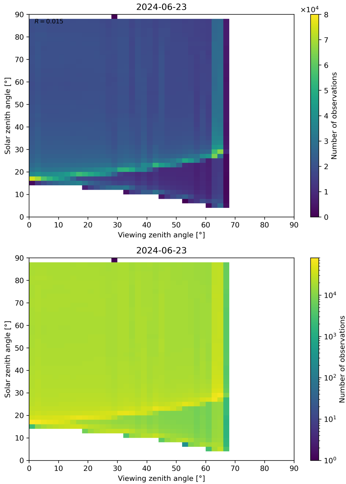
Figure 127: Scatter density plot of “Viewing zenith angle” against “Solar zenith angle” for 2024-06-22 to 2024-06-24.
