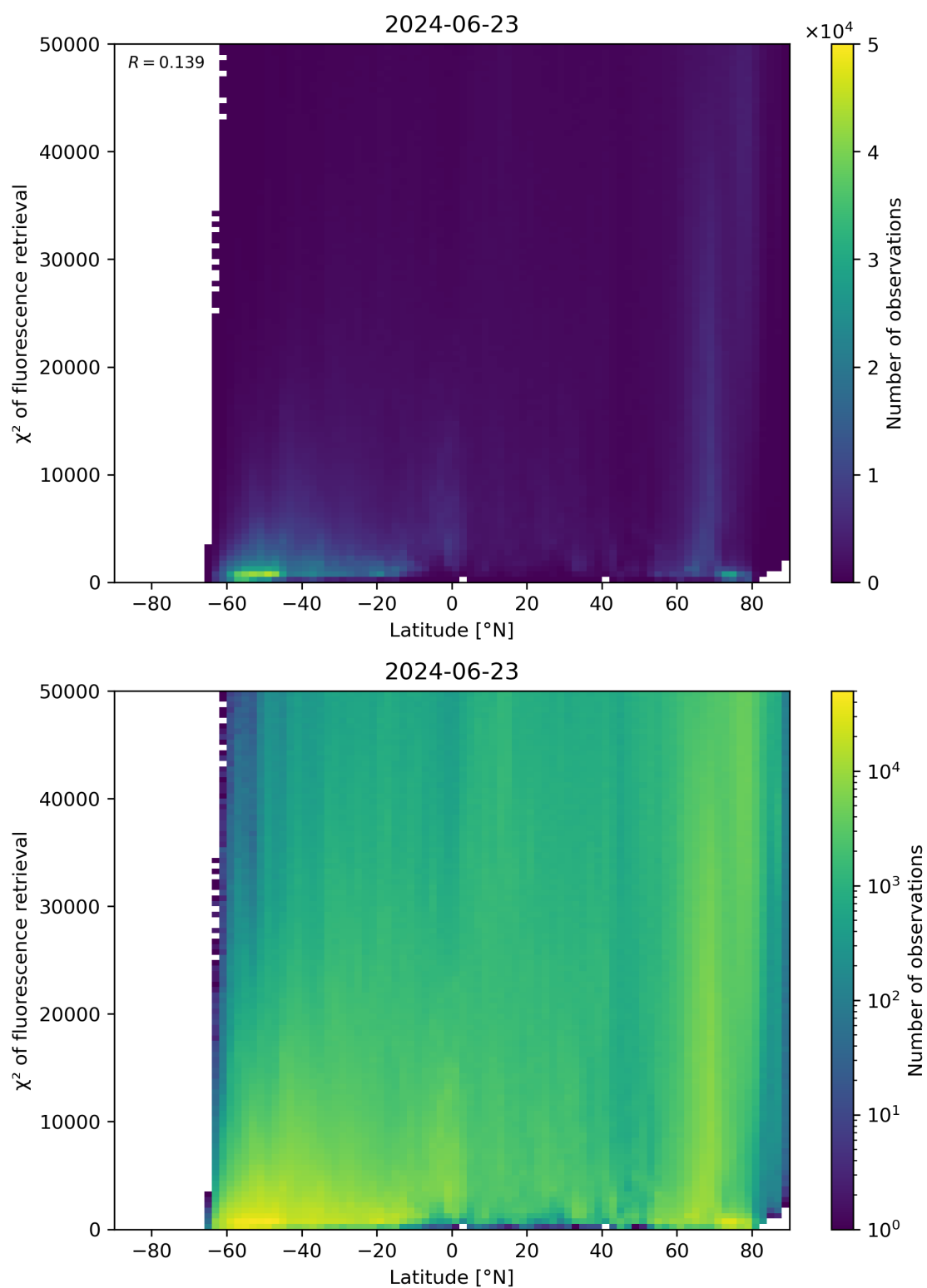
Figure 89: Scatter density plot of “Latitude” against “ \chi^2 of fluorescence retrieval” for 2024-06-22 to 2024-06-24.
