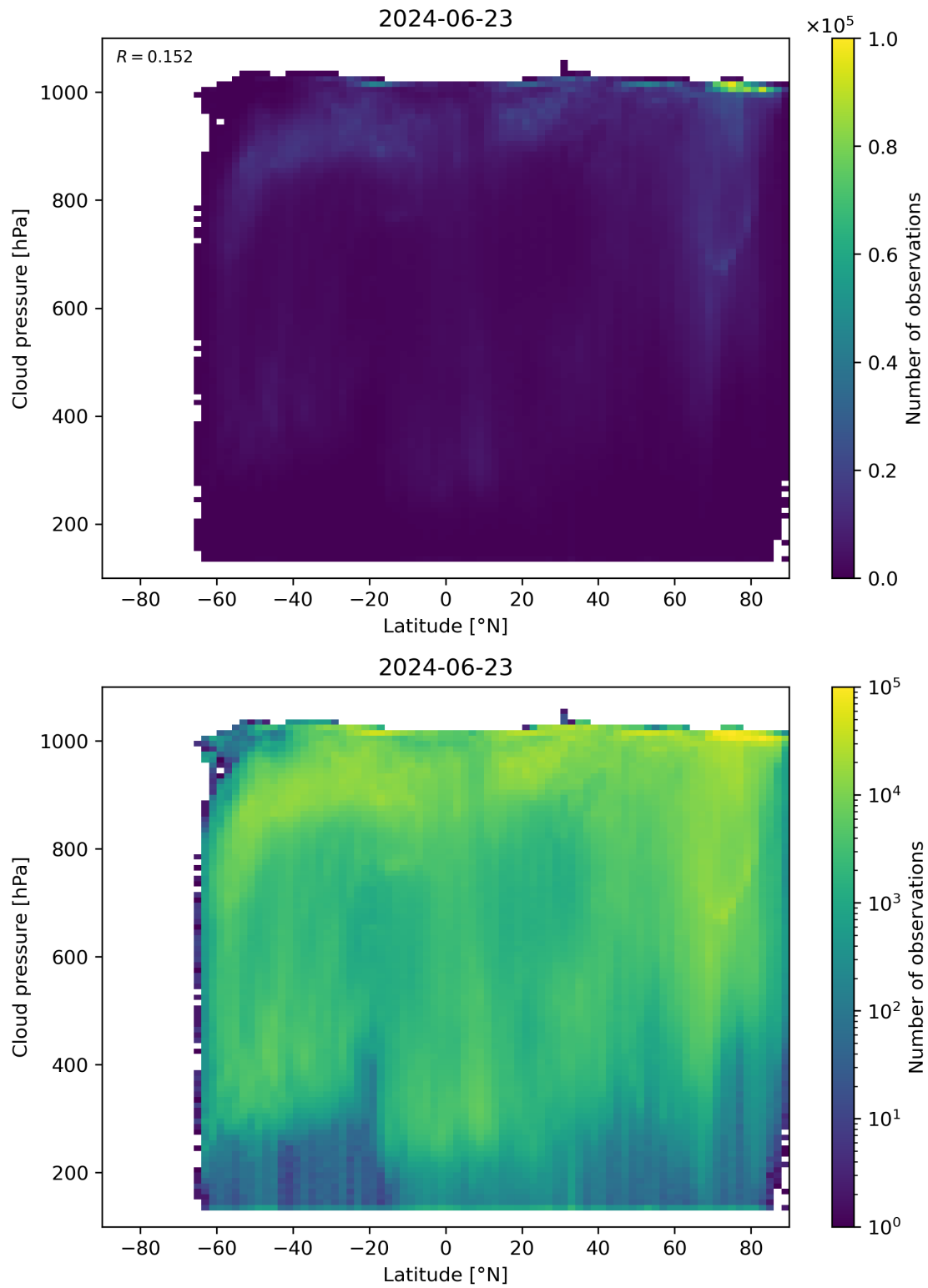
Figure 91: Scatter density plot of “Latitude” against “Cloud pressure” for 2024-06-22 to 2024-06-24.
