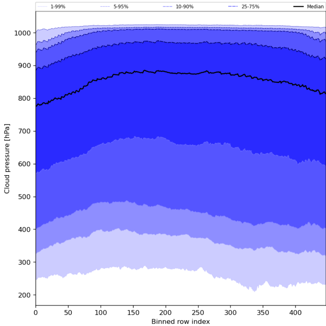
Figure 47: Along track statistics of “Cloud pressure” for 2024-06-22 to 2024-06-24
