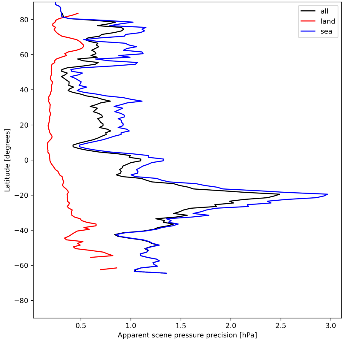
Figure 20: Zonal average of “Apparent scene pressure precision” for 2024-06-22 to 2024-06-24.
