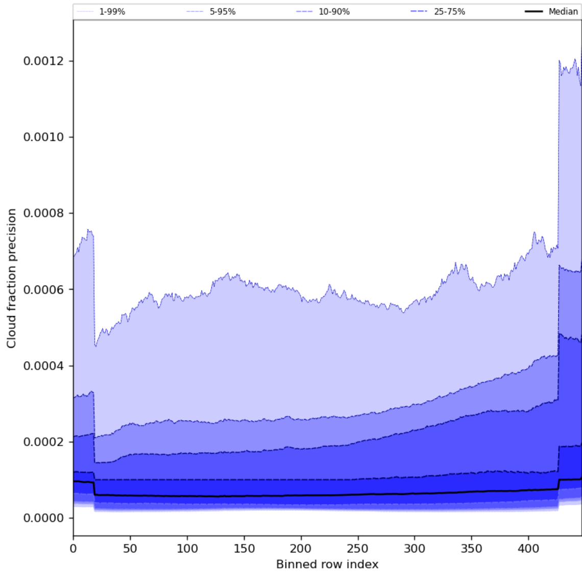
Figure 50: Along track statistics of “Cloud fraction precision” for 2024-06-22 to 2024-06-24
