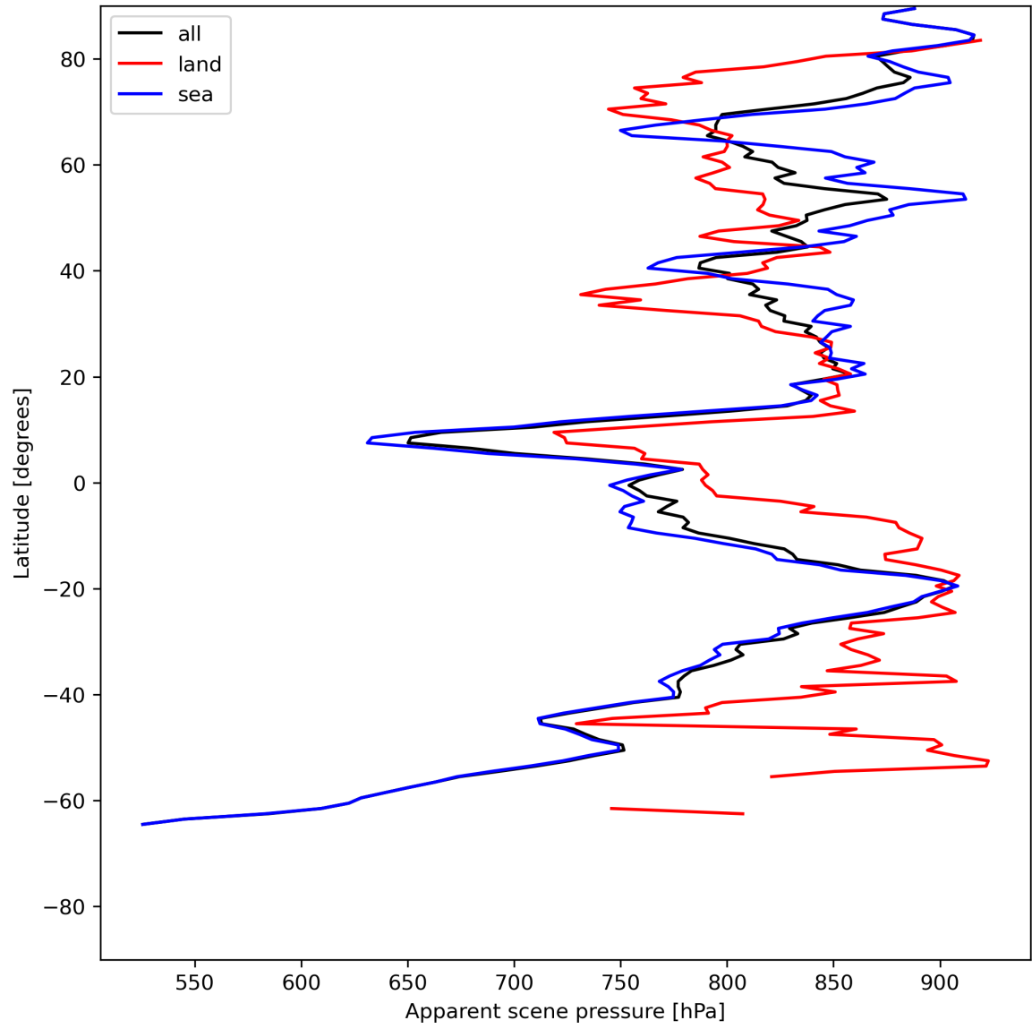
Figure 19: Zonal average of “Apparent scene pressure” for 2024-06-22 to 2024-06-24.
