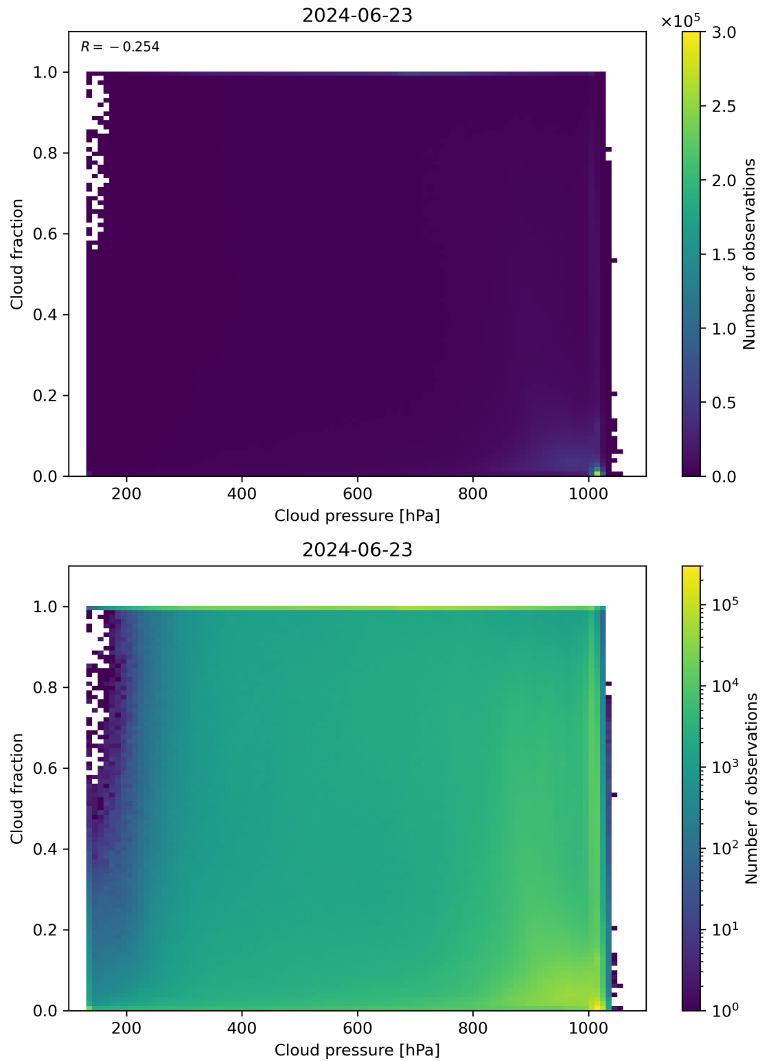
Figure 79: Scatter density plot of “Cloud pressure” against “Cloud fraction” for 2024-06-22 to 2024-06-24.
