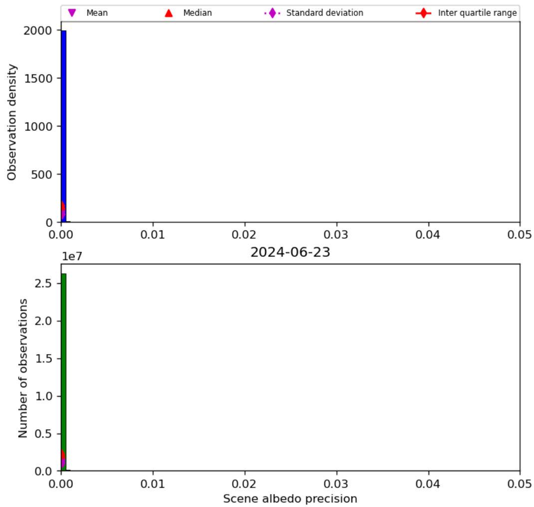
Figure 35: Histogram of “Scene albedo precision” for 2024-06-22 to 2024-06-24
