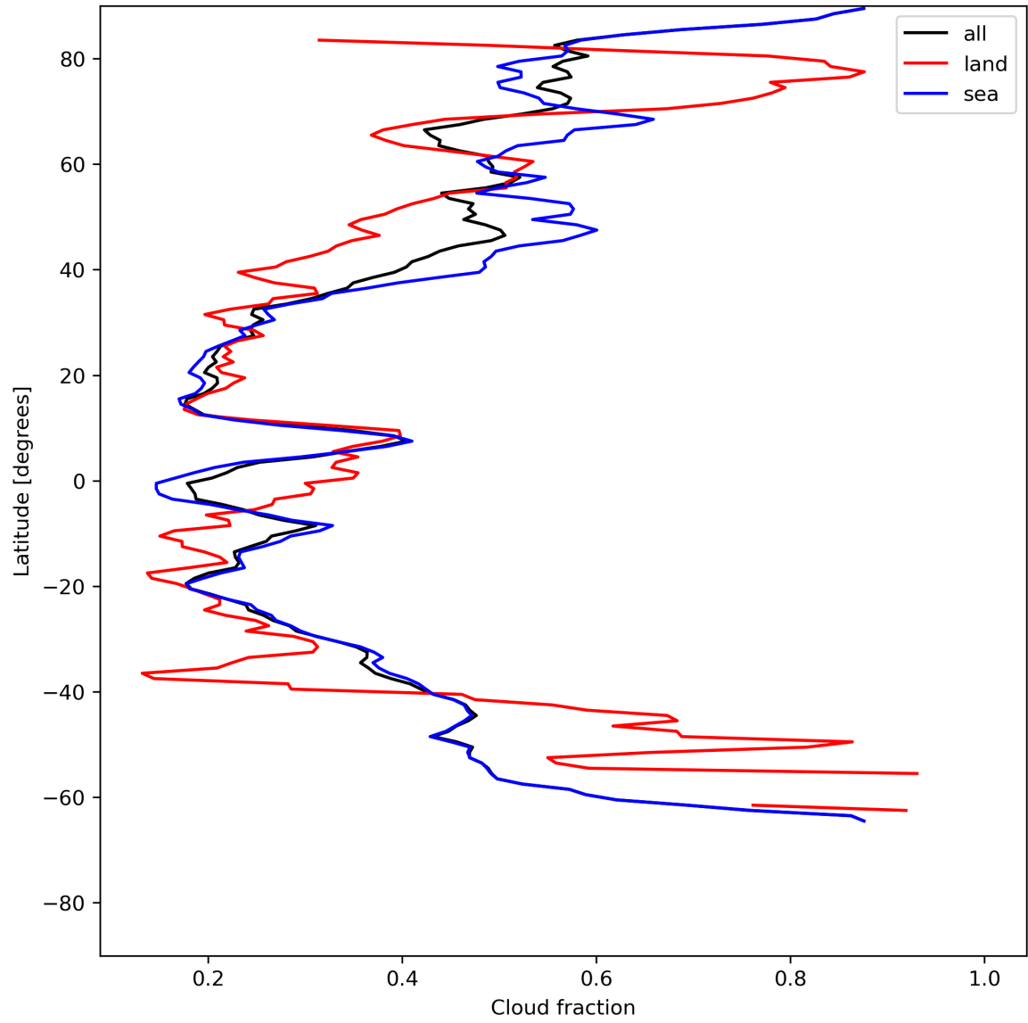
Figure 15: Zonal average of “Cloud fraction” for 2024-06-22 to 2024-06-24.
