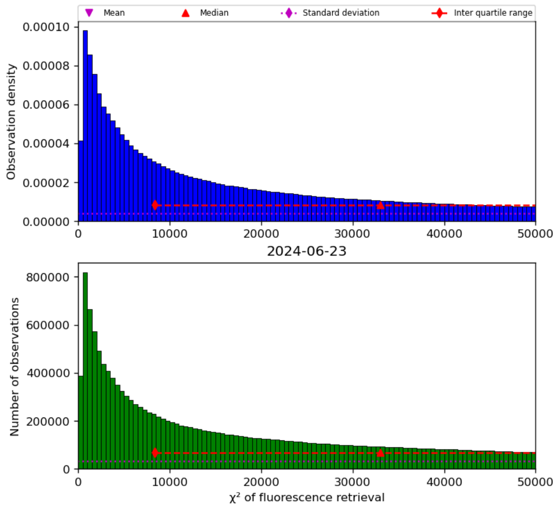
Figure 42: Histogram of “ \chi^2 of fluorescence retrieval” for 2024-06-22 to 2024-06-24
