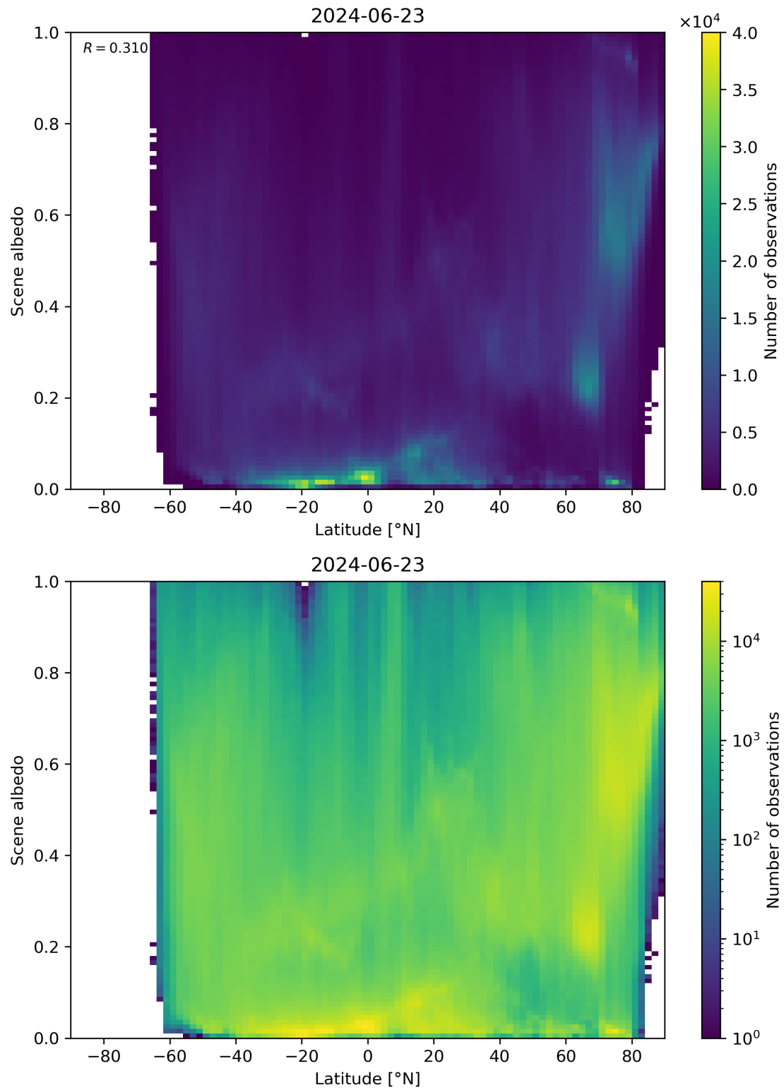
Figure 95: Scatter density plot of “Latitude” against “Scene albedo” for 2024-06-22 to 2024-06-24.
