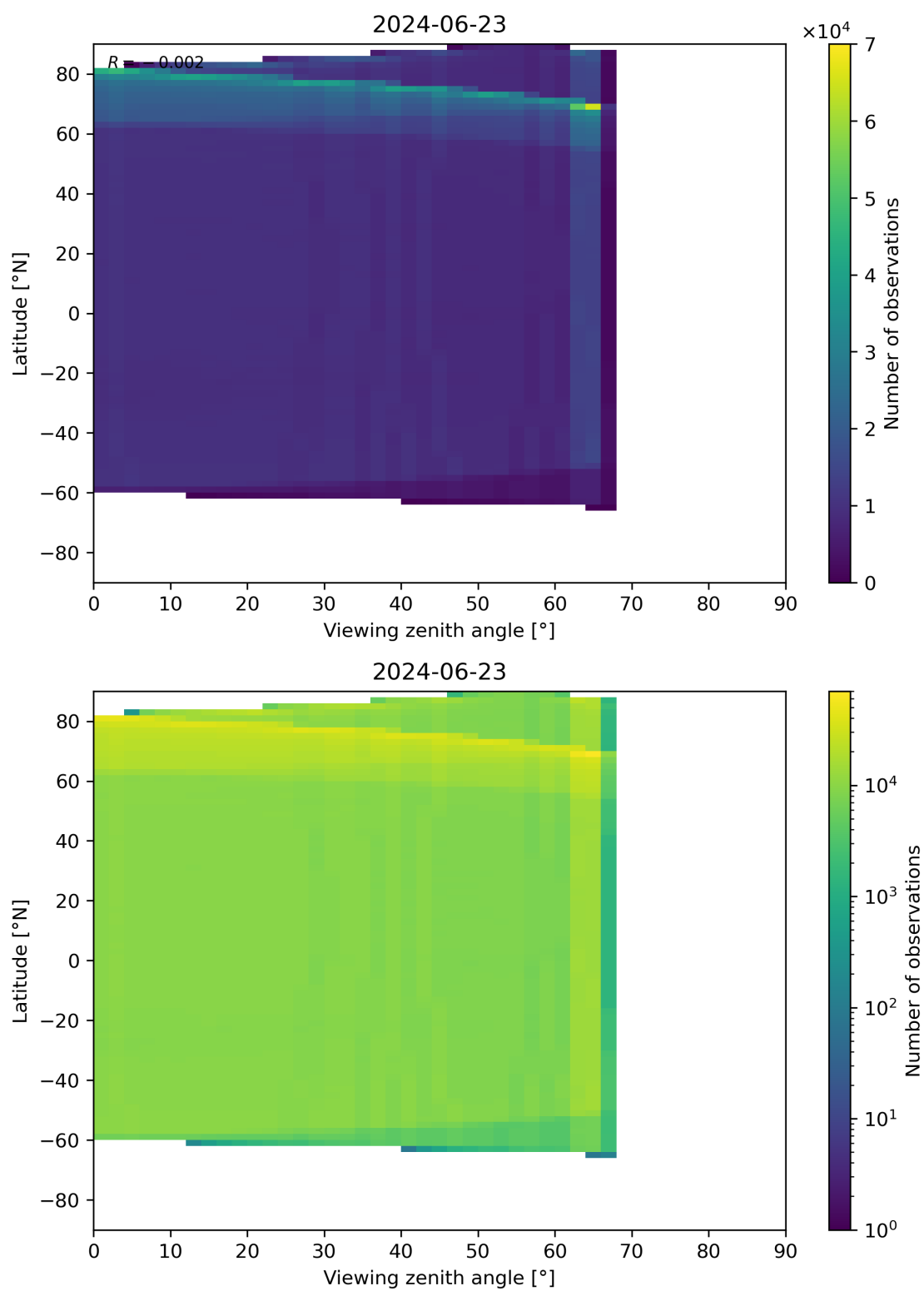
Figure 123: Scatter density plot of “Viewing zenith angle” against “Latitude” for 2024-06-22 to 2024-06-24.
