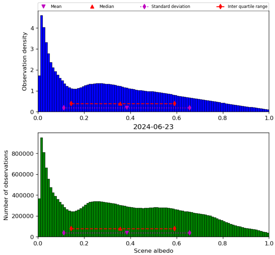
Figure 34: Histogram of “Scene albedo” for 2024-06-22 to 2024-06-24
