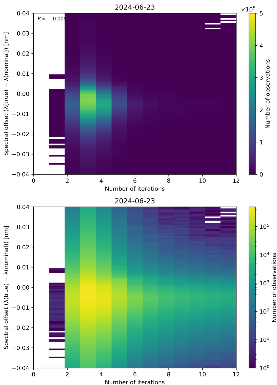
Figure 100: Scatter density plot of “Number of iterations” against “Spectral offset ( \lambda(\text{true}) - \lambda(\text{nominal}) )” for 2024-06-22 to 2024-06-24.
