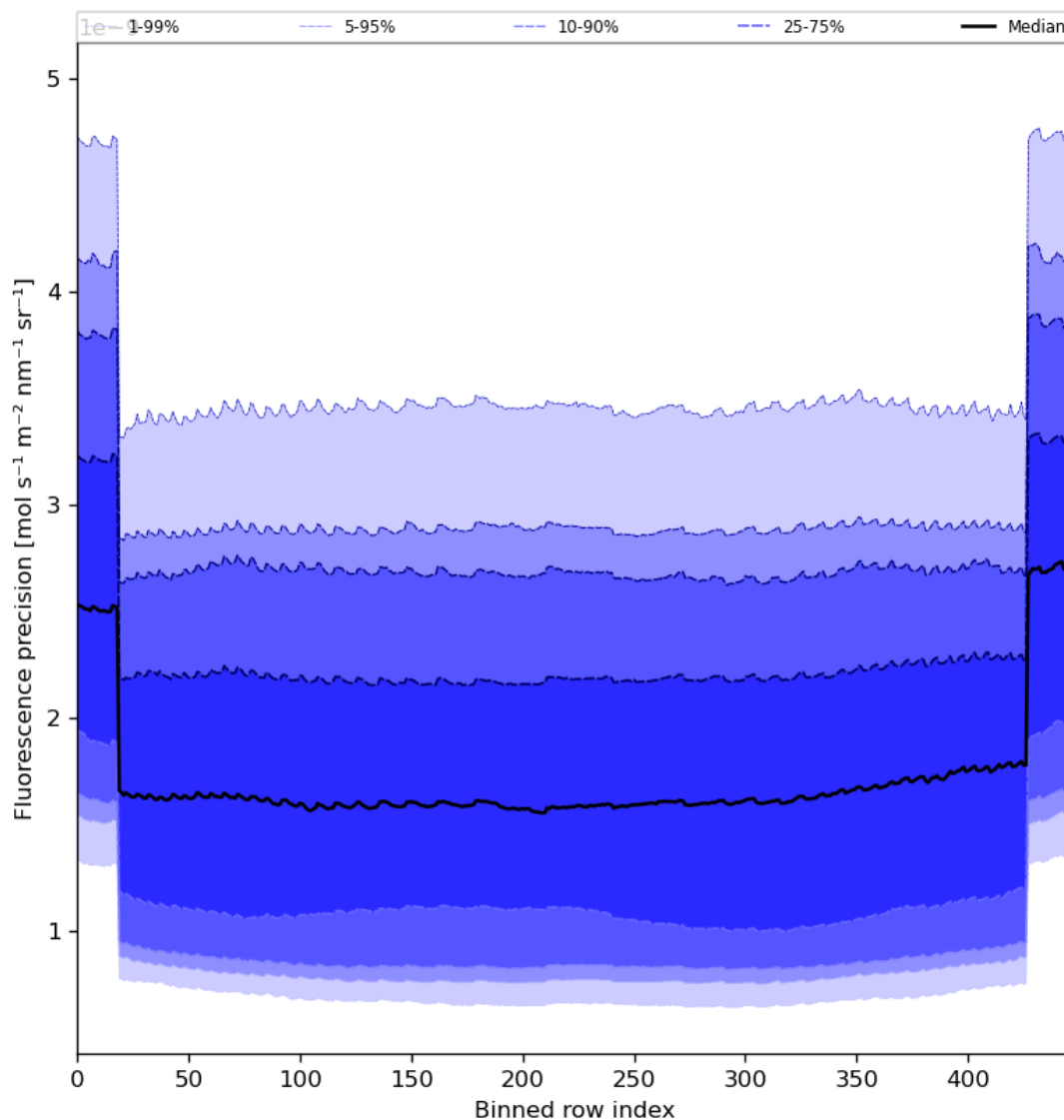
Figure 58: Along track statistics of “Fluorescence precision” for 2024-06-22 to 2024-06-24
