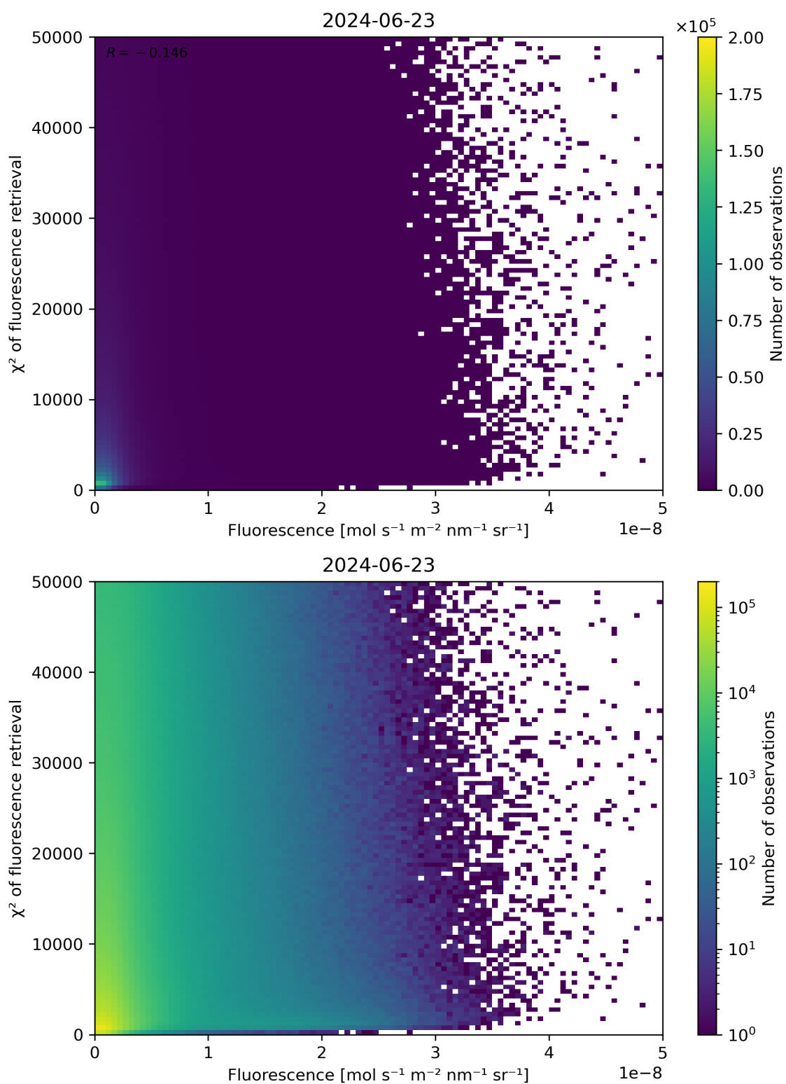
Figure 85: Scatter density plot of “Fluorescence” against “ \chi^2 of fluorescence retrieval” for 2024-06-22 to 2024-06-24.
