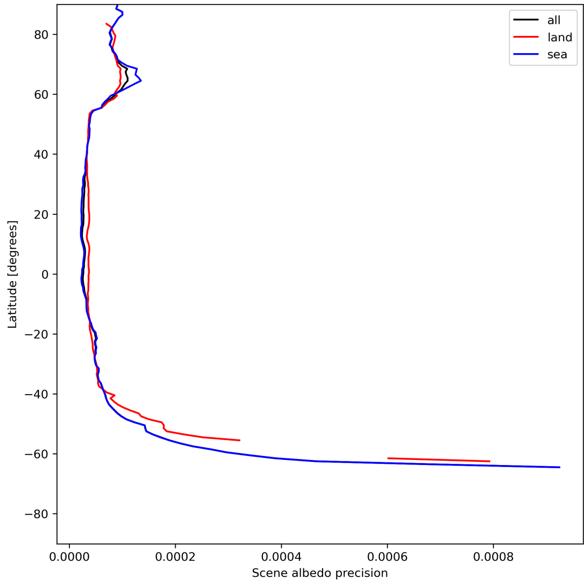
Figure 18: Zonal average of “Scene albedo precision” for 2024-06-22 to 2024-06-24.
