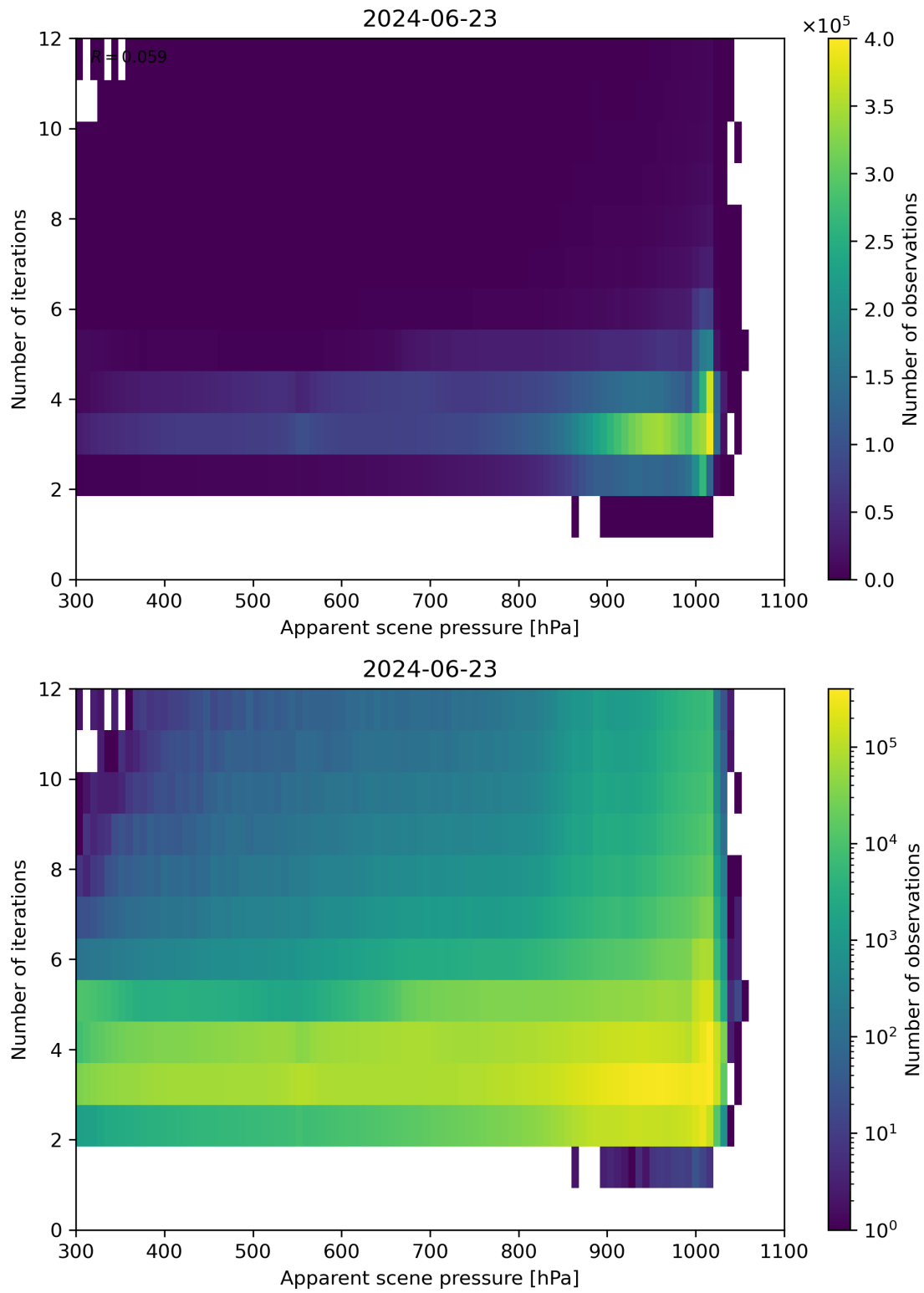
Figure 65: Scatter density plot of “Apparent scene pressure” against “Number of iterations” for 2024-06-22 to 2024-06-24.
