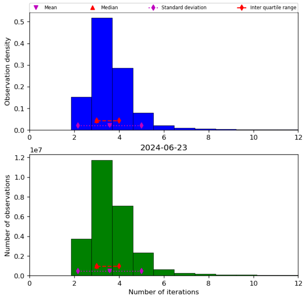
Figure 39: Histogram of “Number of iterations” for 2024-06-22 to 2024-06-24
