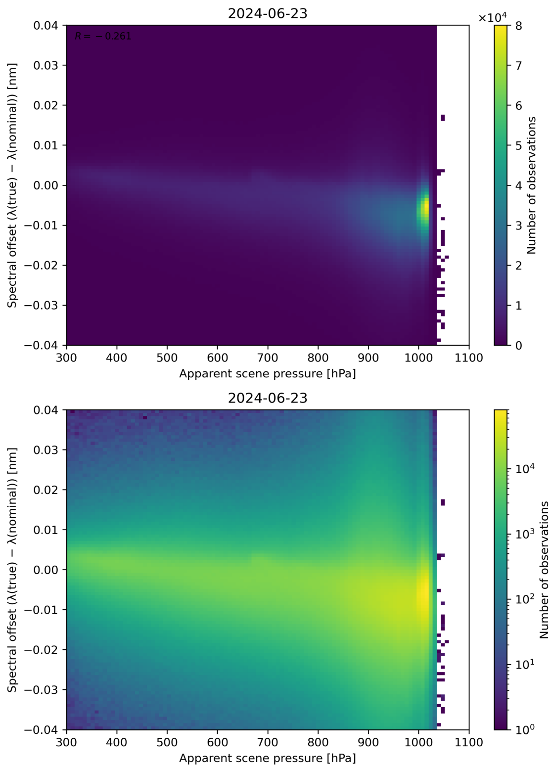
Figure 67: Scatter density plot of “Apparent scene pressure” against “Spectral offset ( \lambda(\text{true}) - \lambda(\text{nominal}) )” for 2024-06-22 to 2024-06-24.
