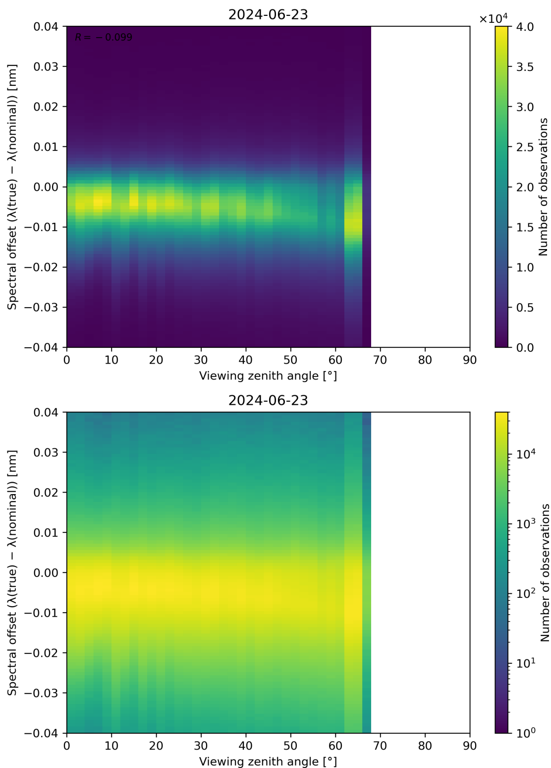
Figure 128: Scatter density plot of “Viewing zenith angle” against “Spectral offset ( \lambda(\text{true}) - \lambda(\text{nominal}) )” for 2024-06-22 to 2024-06-24.
