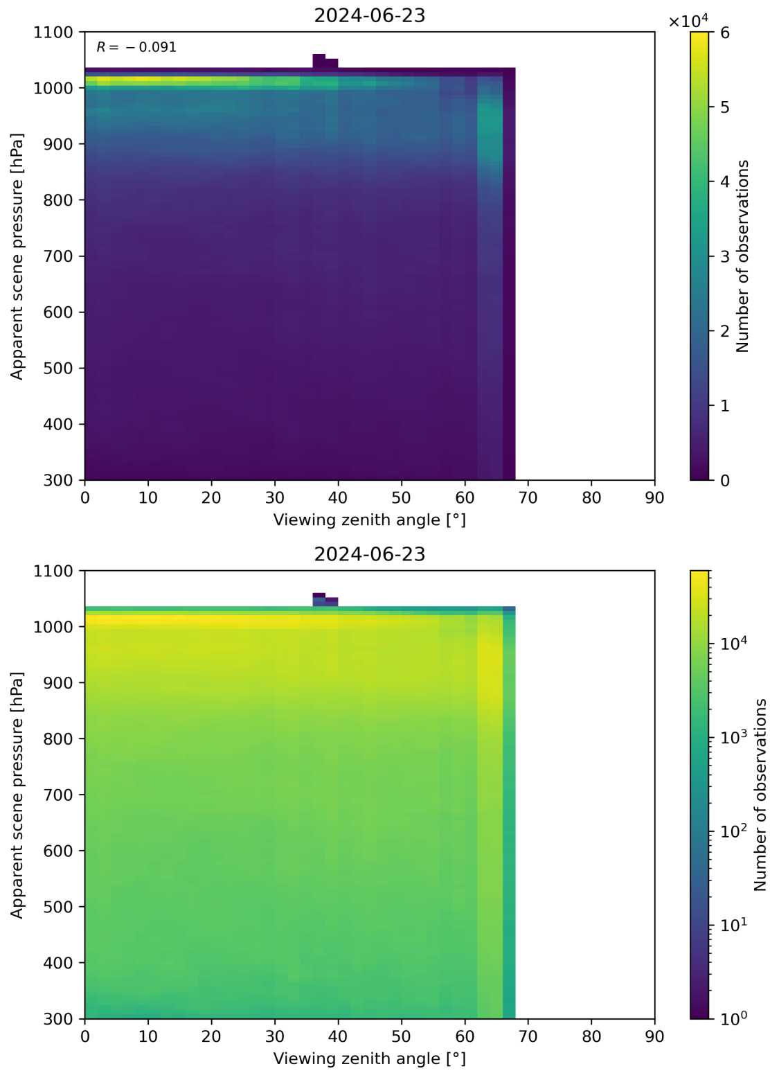
Figure 118: Scatter density plot of “Viewing zenith angle” against “Apparent scene pressure” for 2024-06-22 to 2024-06-24.
