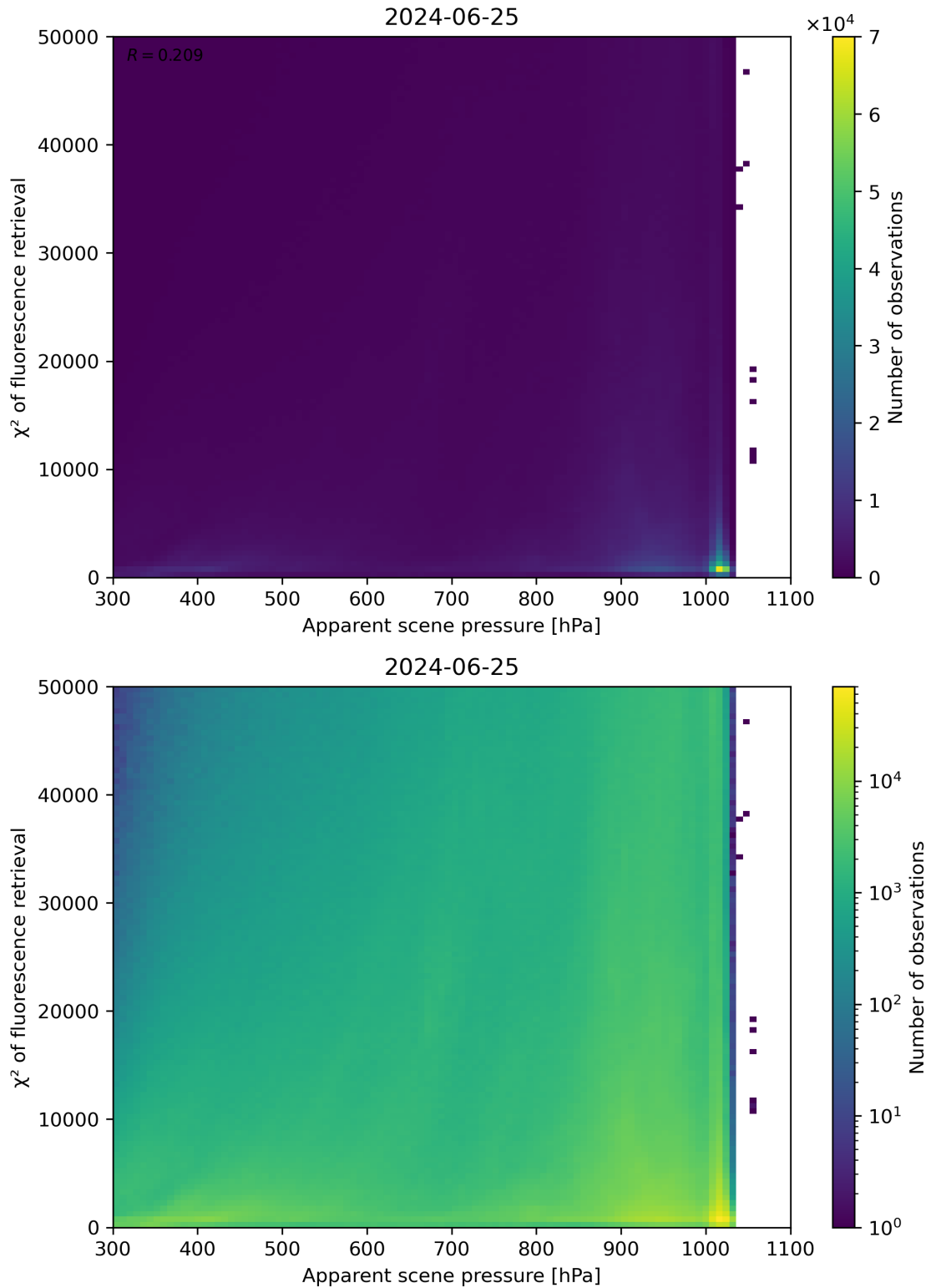
Figure 63: Scatter density plot of “Apparent scene pressure” against “ \chi^2 of fluorescence retrieval” for 2024-06-24 to 2024-06-26.
