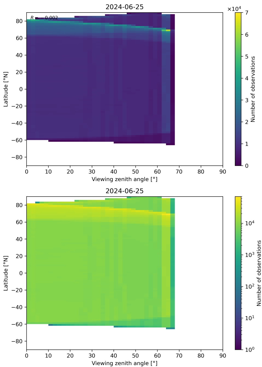
Figure 123: Scatter density plot of “Viewing zenith angle” against “Latitude” for 2024-06-24 to 2024-06-26.
