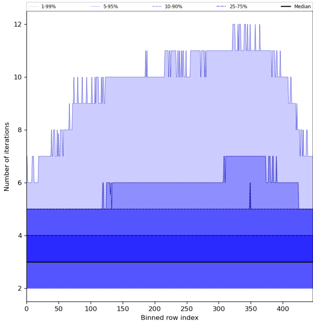
Figure 56: Along track statistics of “Number of iterations” for 2024-06-24 to 2024-06-26
