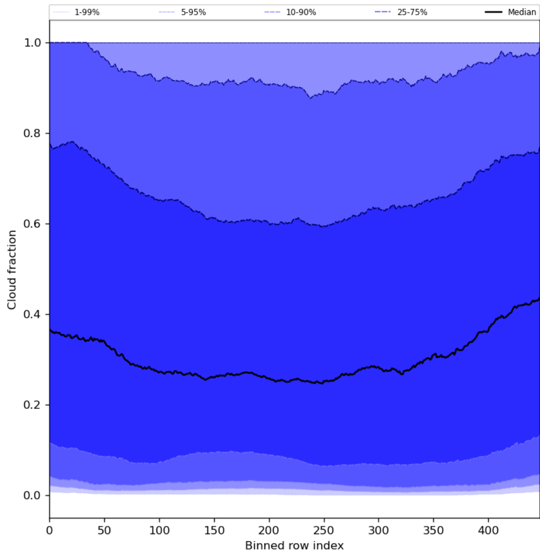
Figure 49: Along track statistics of “Cloud fraction” for 2024-06-24 to 2024-06-26
