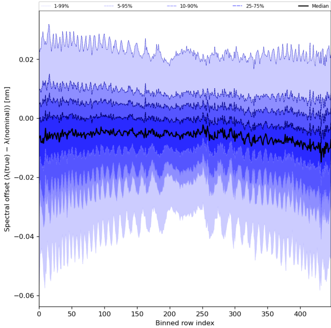
Figure 62: Along track statistics of “Spectral offset ( \lambda(\text{true}) - \lambda(\text{nominal}) )” for 2024-06-24 to 2024-06-26
