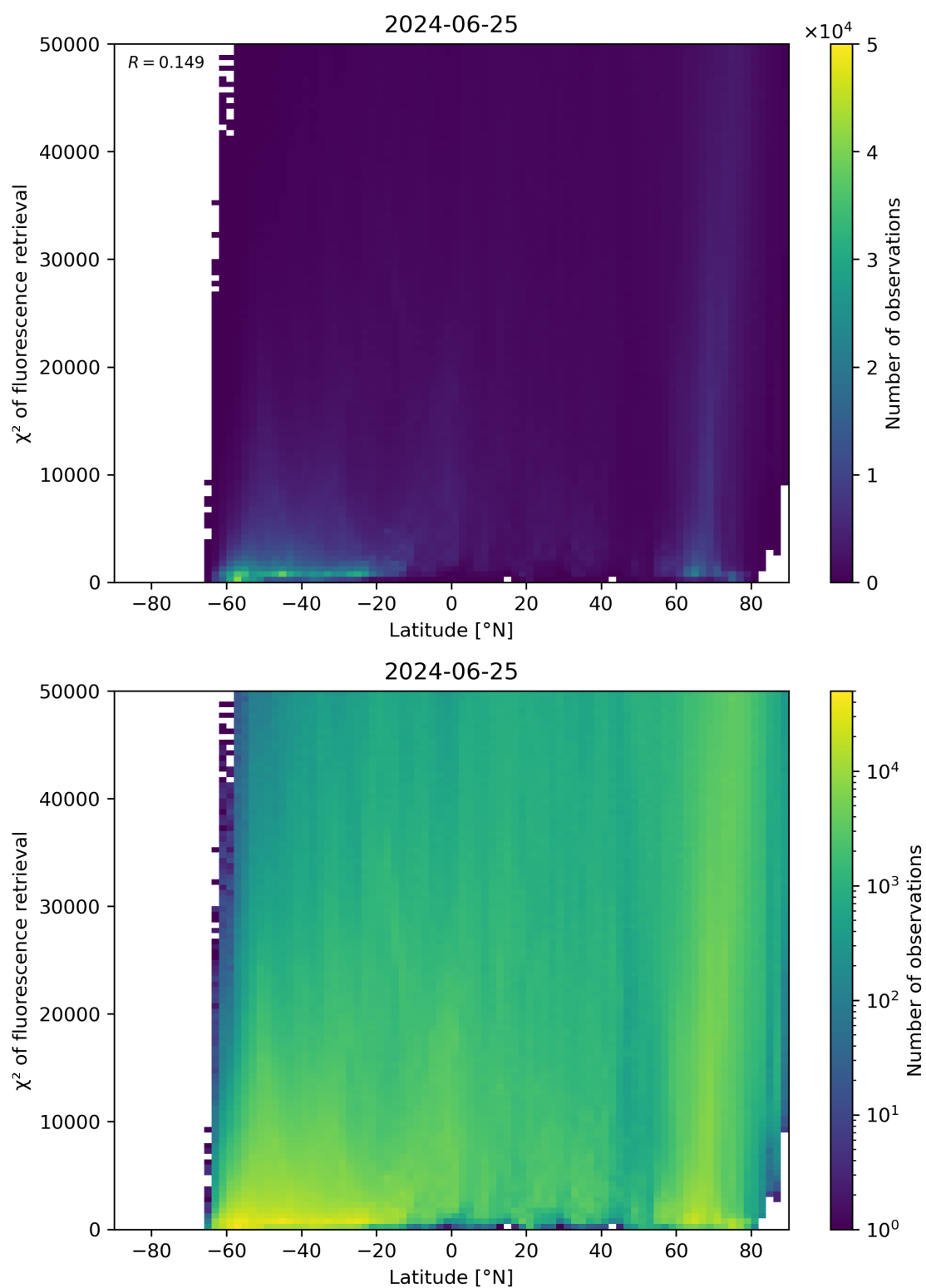
Figure 89: Scatter density plot of “Latitude” against “ \chi^2 of fluorescence retrieval” for 2024-06-24 to 2024-06-26.
