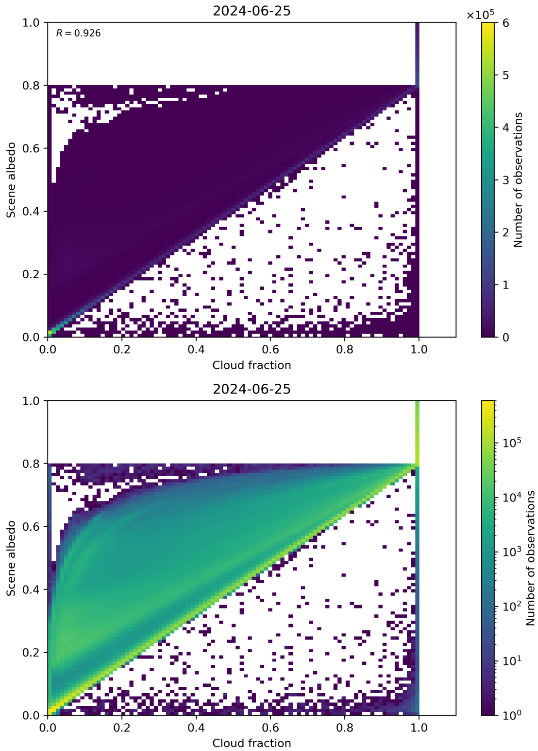
Figure 75: Scatter density plot of “Cloud fraction” against “Scene albedo” for 2024-06-24 to 2024-06-26.
