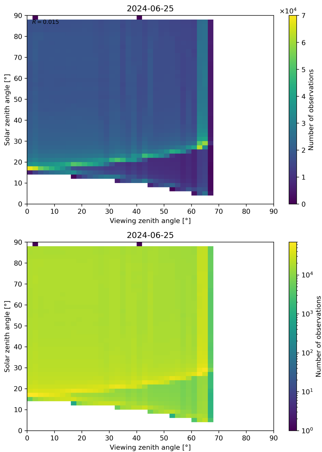
Figure 127: Scatter density plot of “Viewing zenith angle” against “Solar zenith angle” for 2024-06-24 to 2024-06-26.
