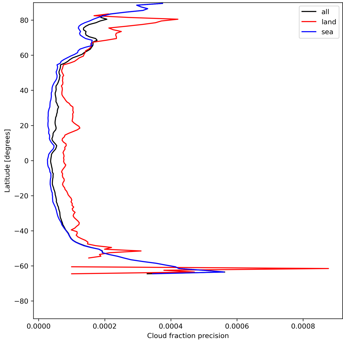
Figure 16: Zonal average of “Cloud fraction precision” for 2024-06-24 to 2024-06-26.
