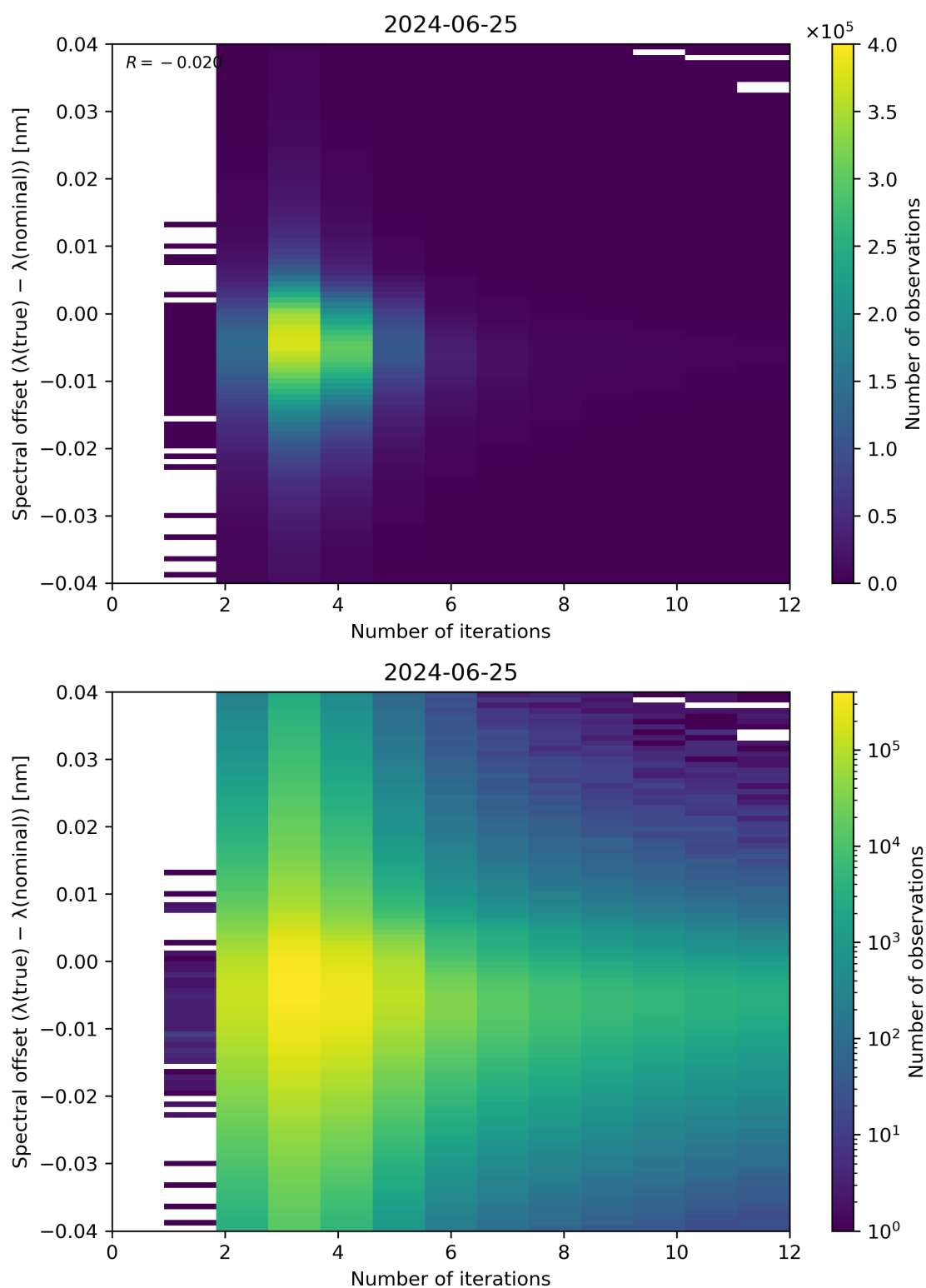
Figure 100: Scatter density plot of “Number of iterations” against “Spectral offset ( \lambda(\text{true}) - \lambda(\text{nominal}) )” for 2024-06-24 to 2024-06-26.
