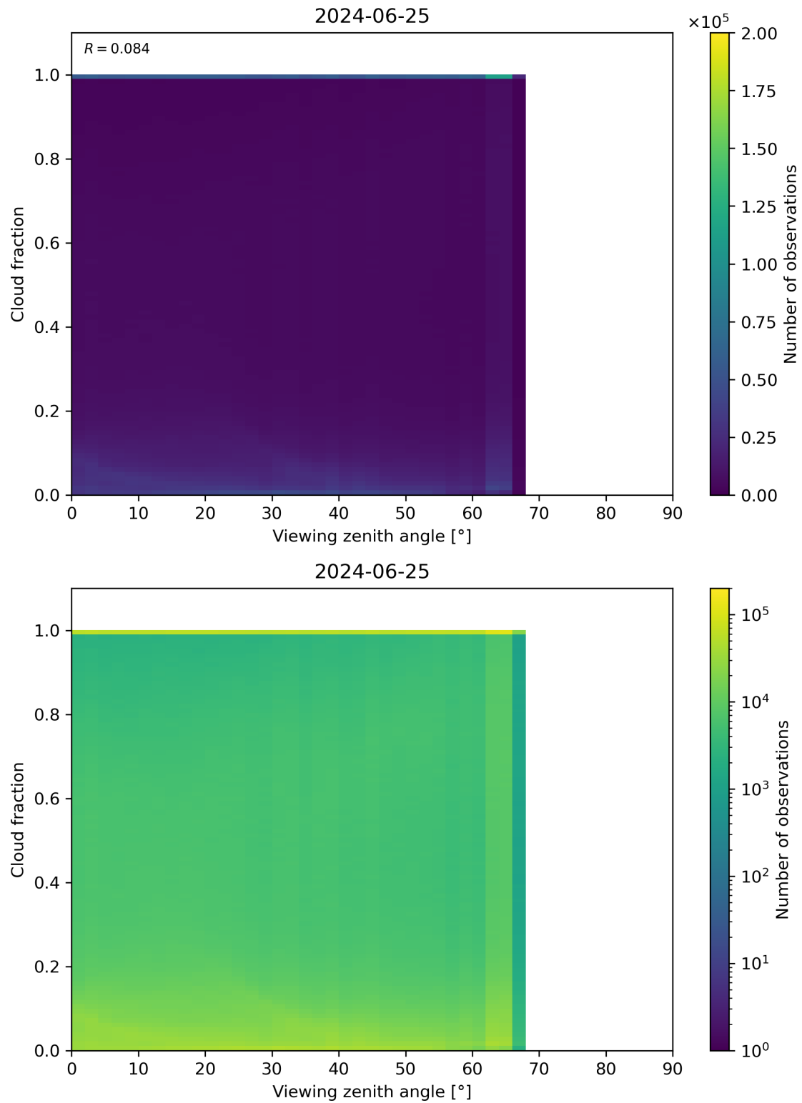
Figure 120: Scatter density plot of “Viewing zenith angle” against “Cloud fraction” for 2024-06-24 to 2024-06-26.
