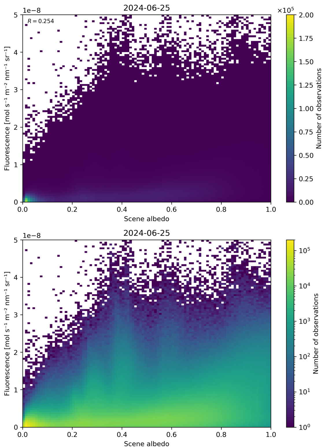
Figure 104: Scatter density plot of “Scene albedo” against “Fluorescence” for 2024-06-24 to 2024-06-26.
