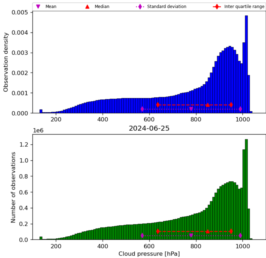
Figure 30: Histogram of “Cloud pressure” for 2024-06-24 to 2024-06-26
