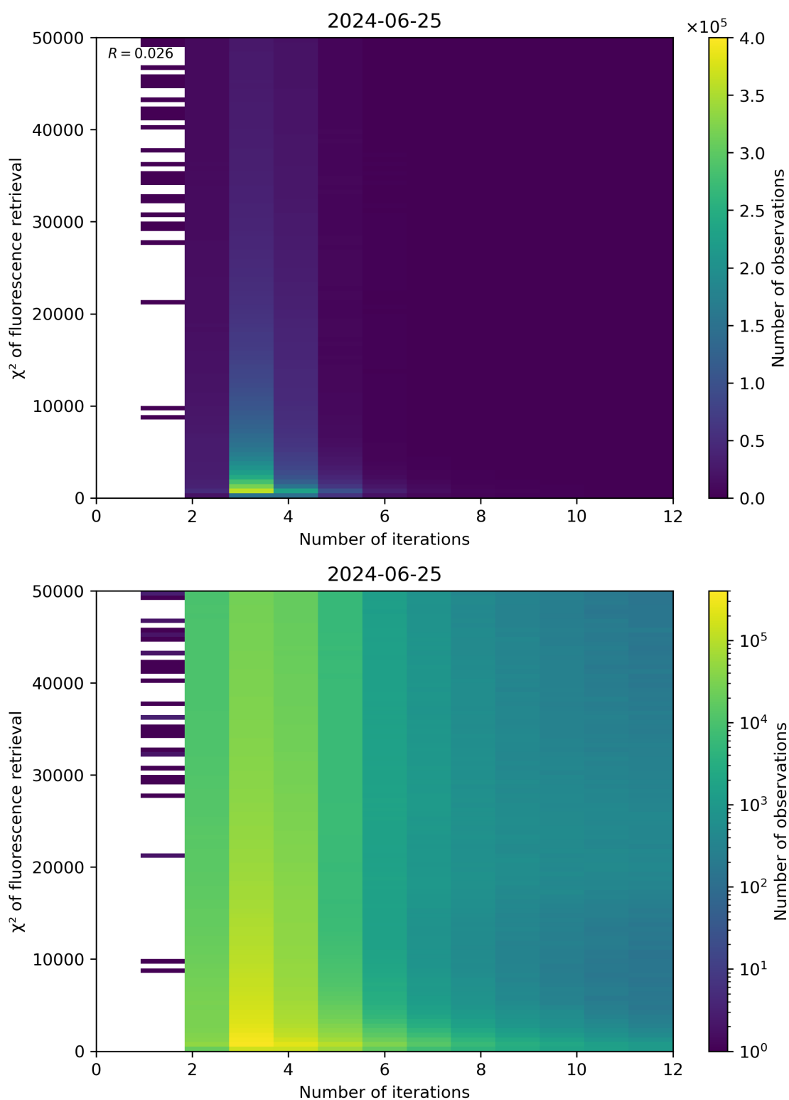
Figure 97: Scatter density plot of “Number of iterations” against “ \chi^2 of fluorescence retrieval” for 2024-06-24 to 2024-06-26.
