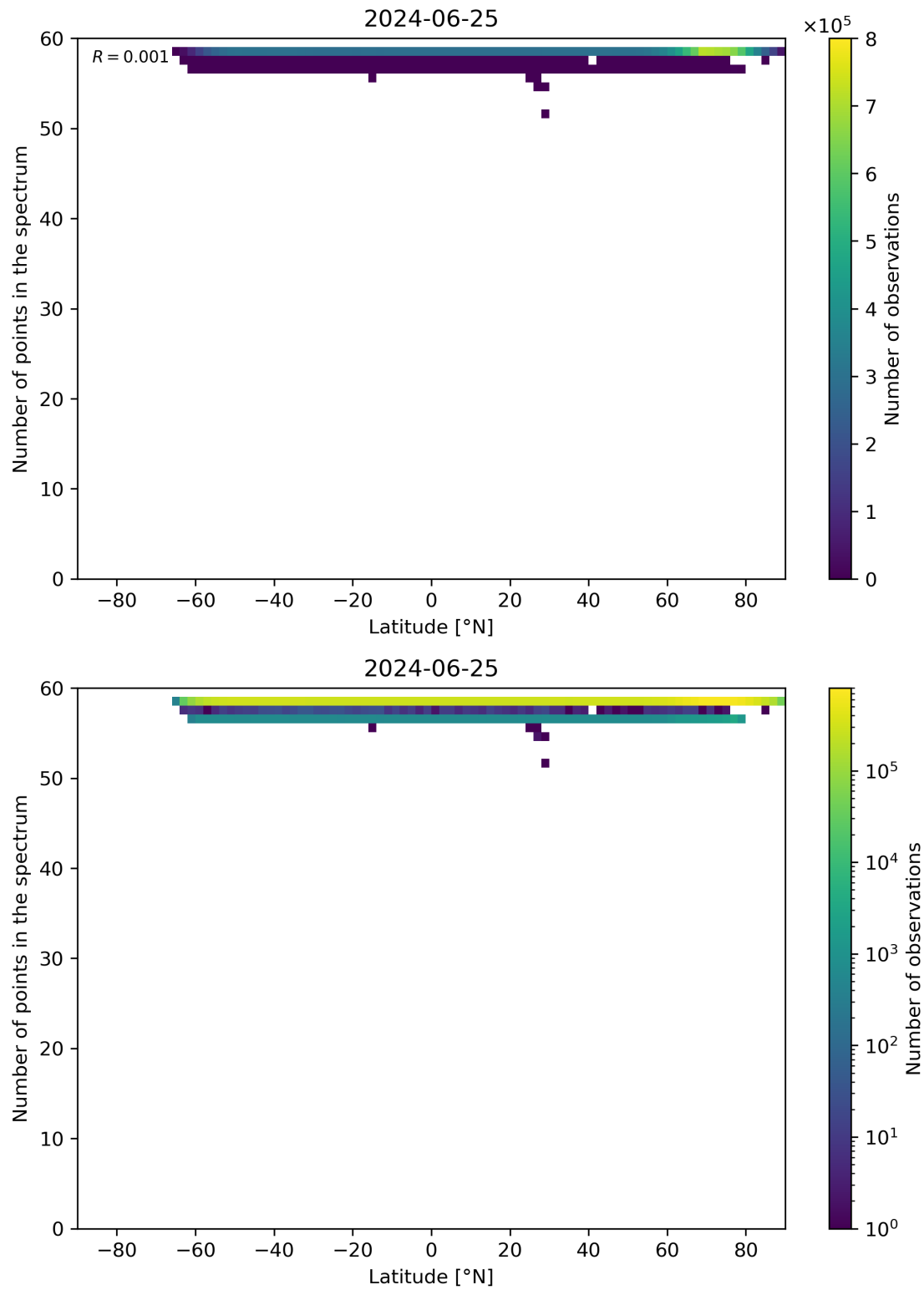
Figure 94: Scatter density plot of “Latitude” against “Number of points in the spectrum” for 2024-06-24 to 2024-06-26.
