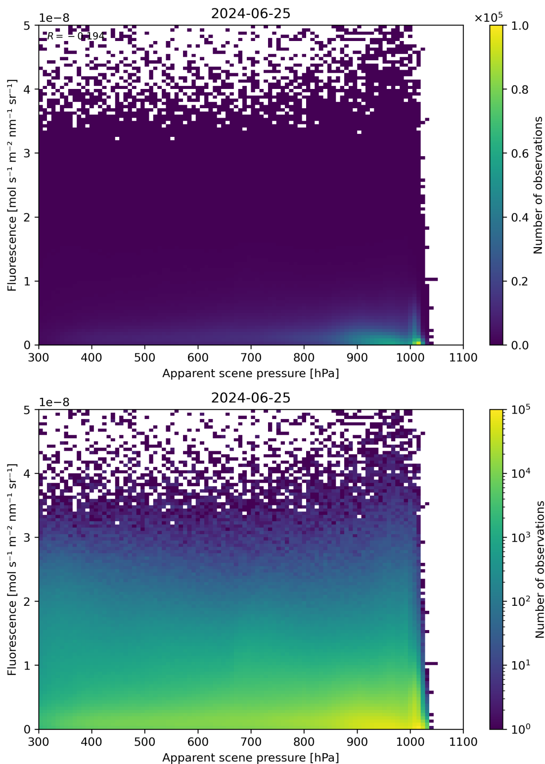
Figure 64: Scatter density plot of “Apparent scene pressure” against “Fluorescence” for 2024-06-24 to 2024-06-26.
