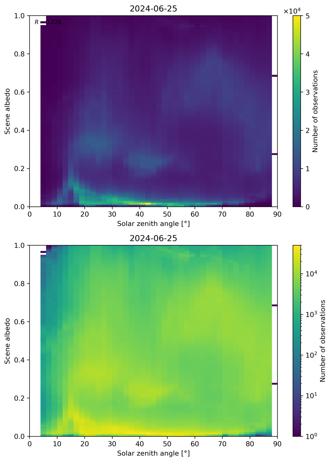
Figure 116: Scatter density plot of “Solar zenith angle” against “Scene albedo” for 2024-06-24 to 2024-06-26.
