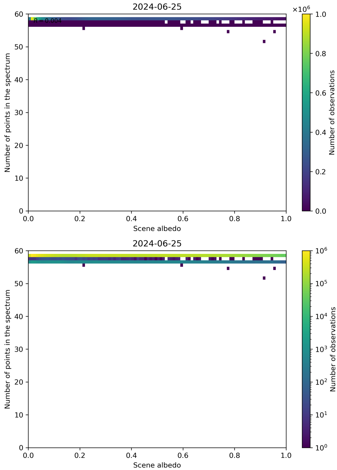
Figure 106: Scatter density plot of “Scene albedo” against “Number of points in the spectrum” for 2024-06-24 to 2024-06-26.
