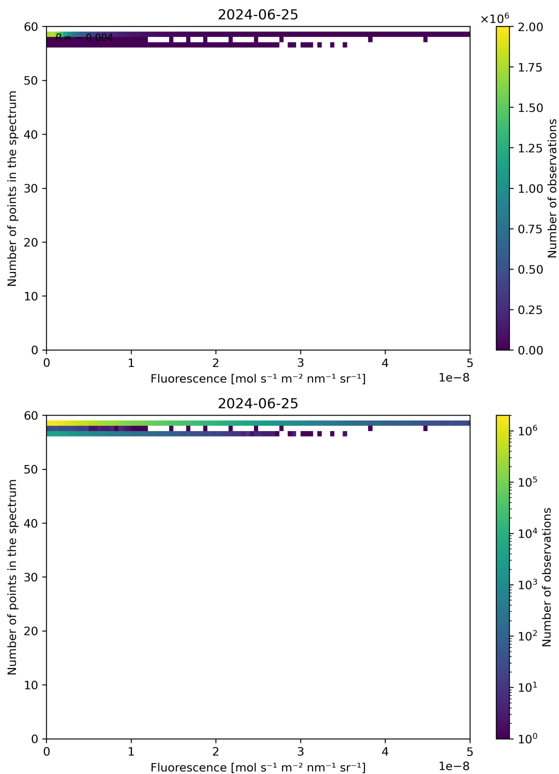
Figure 86: Scatter density plot of “Fluorescence” against “Number of points in the spectrum” for 2024-06-24 to 2024-06-26.
