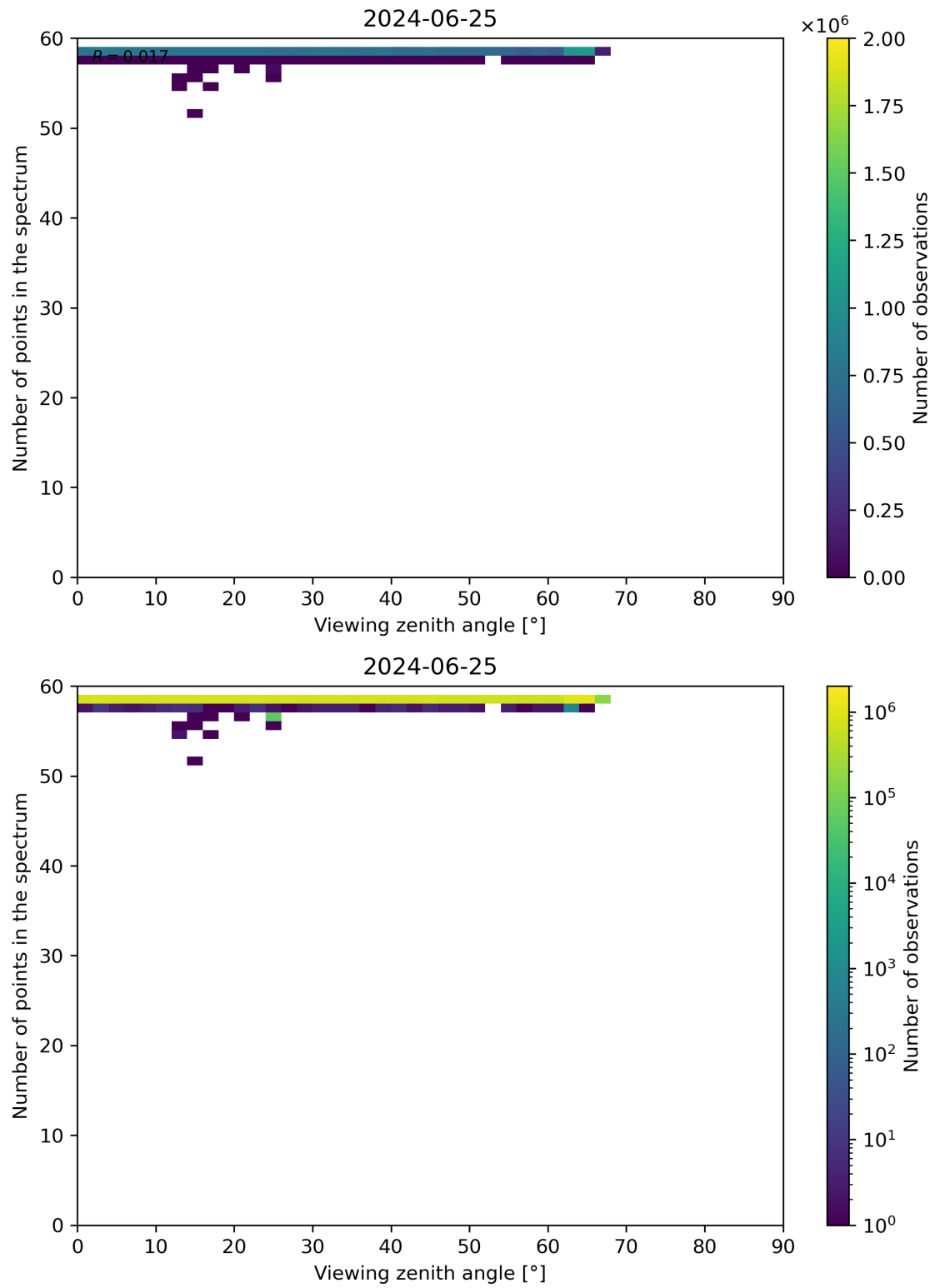
Figure 125: Scatter density plot of “Viewing zenith angle” against “Number of points in the spectrum” for 2024-06-24 to 2024-06-26.
