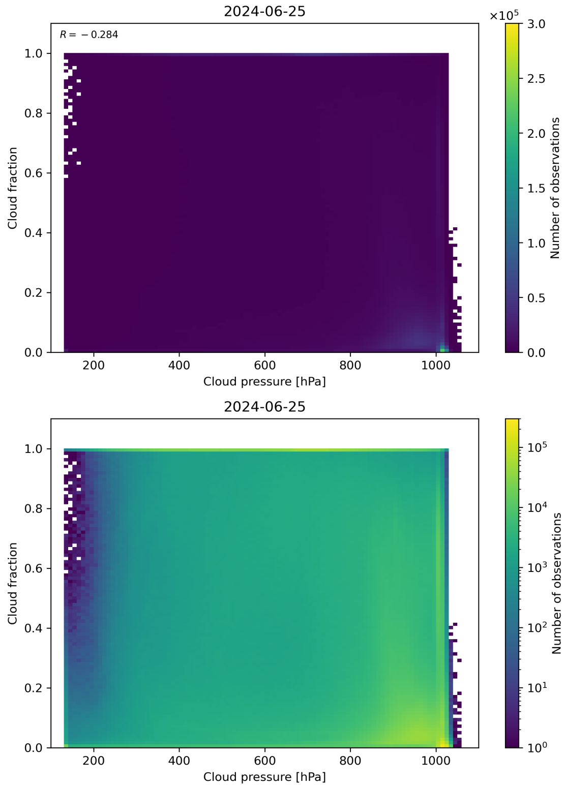
Figure 79: Scatter density plot of “Cloud pressure” against “Cloud fraction” for 2024-06-24 to 2024-06-26.
