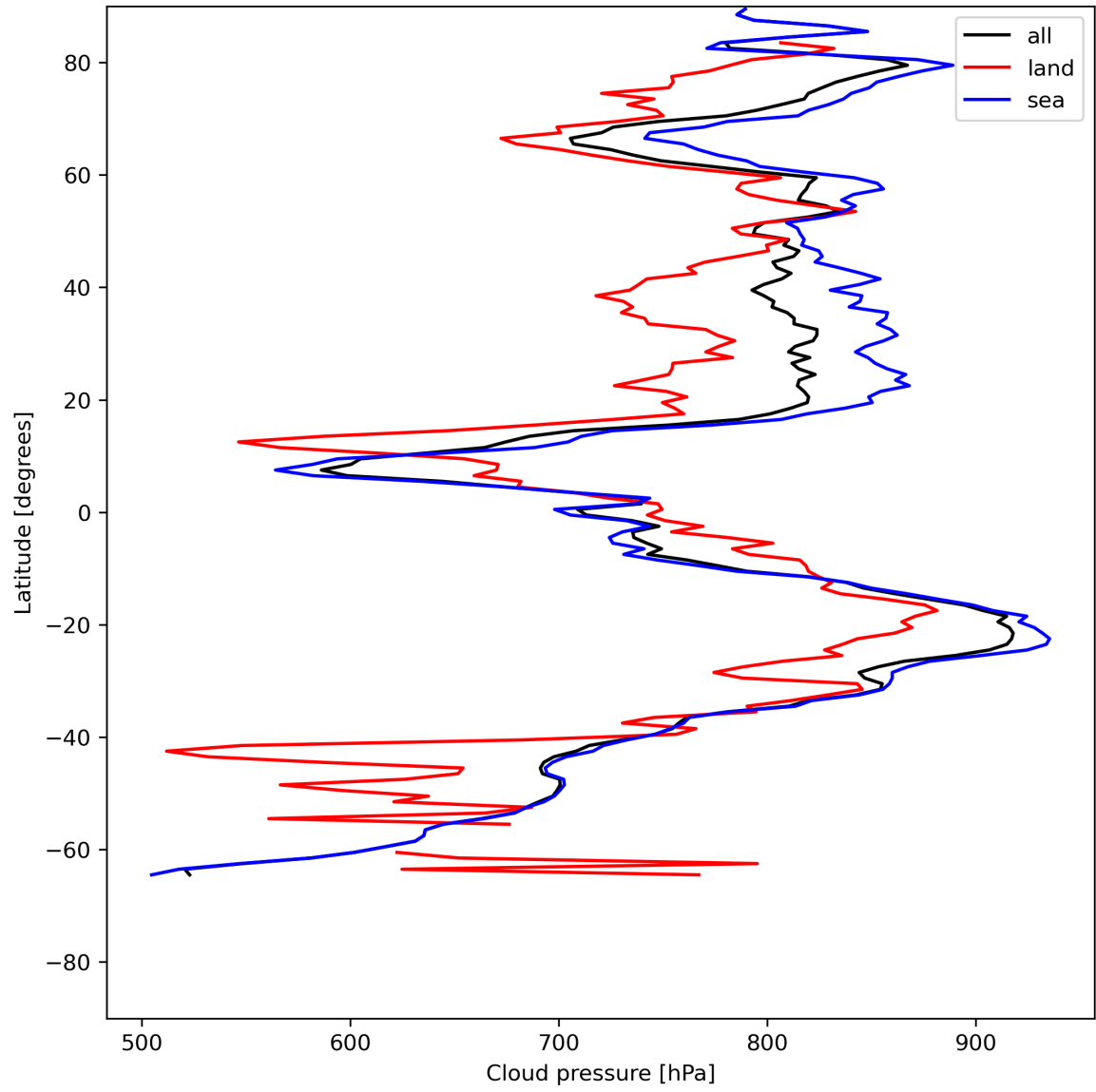
Figure 13: Zonal average of “Cloud pressure” for 2024-06-24 to 2024-06-26.
