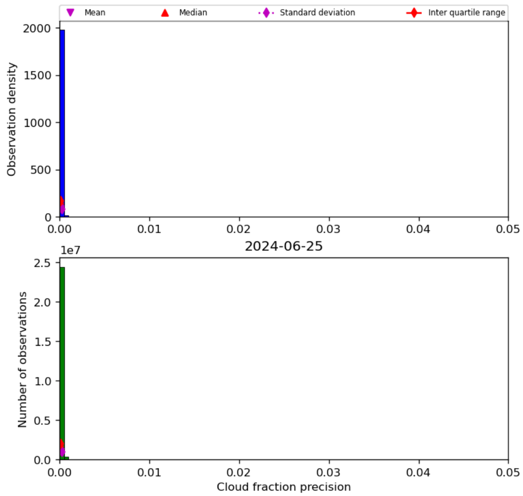
Figure 33: Histogram of “Cloud fraction precision” for 2024-06-24 to 2024-06-26
