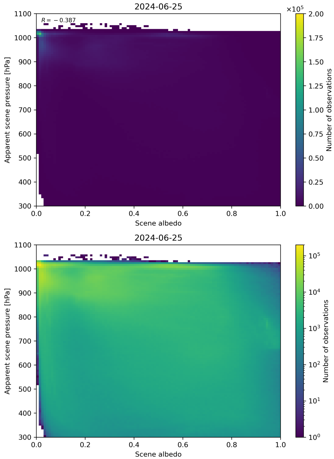
Figure 102: Scatter density plot of “Scene albedo” against “Apparent scene pressure” for 2024-06-24 to 2024-06-26.
