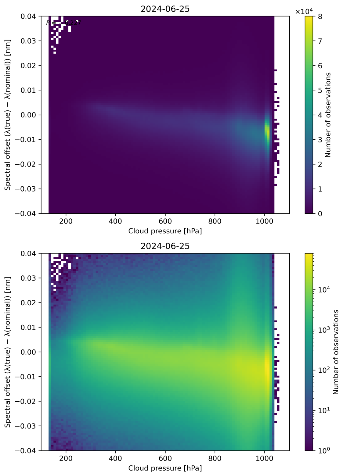
Figure 84: Scatter density plot of “Cloud pressure” against “Spectral offset ( \lambda(\text{true}) - \lambda(\text{nominal}) )” for 2024-06-24 to 2024-06-26.
