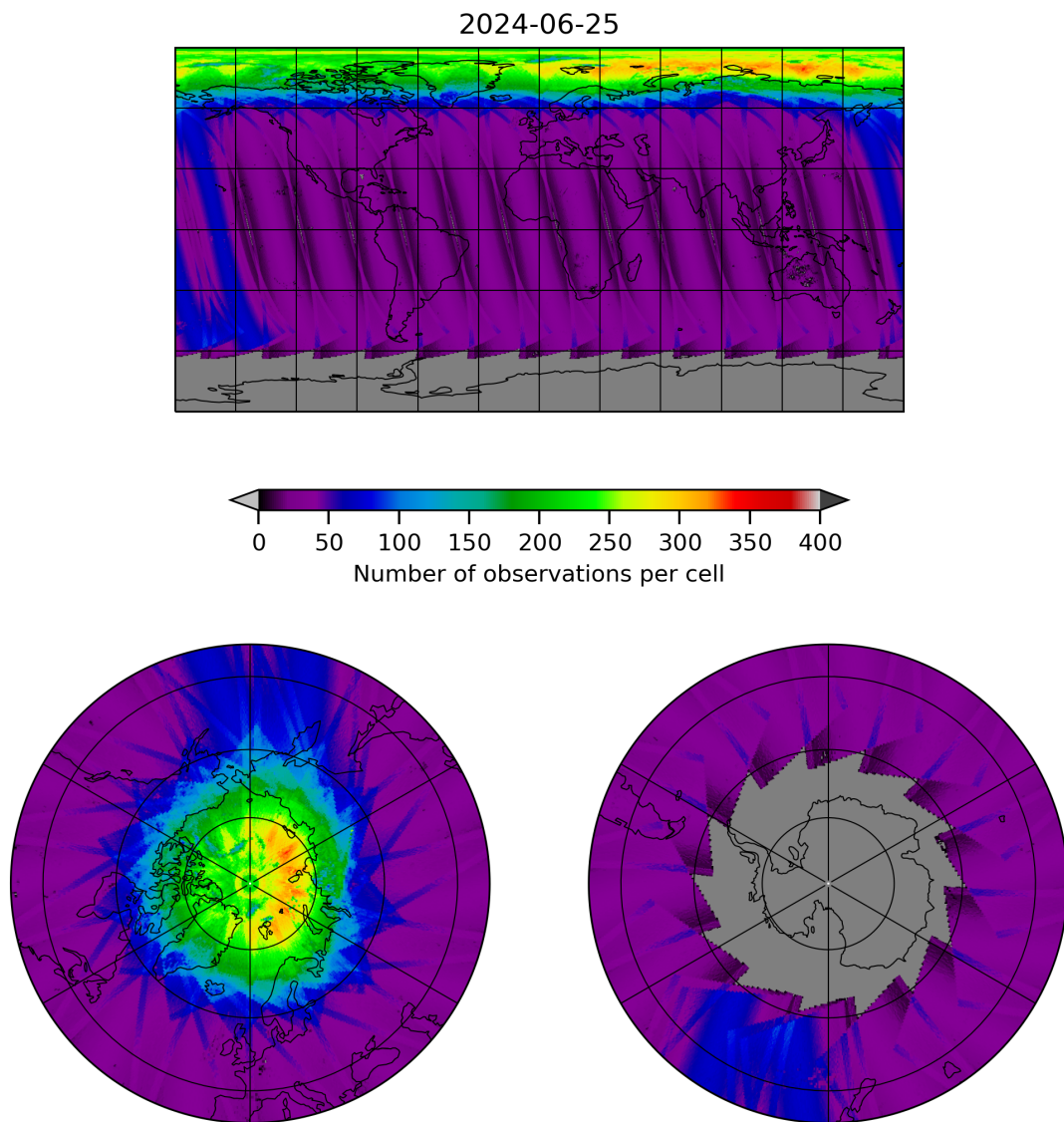
Figure 11: Map of the number of observations for 2024-06-24 to 2024-06-26
