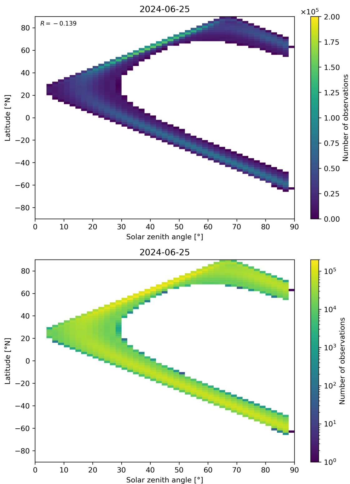
Figure 113: Scatter density plot of “Solar zenith angle” against “Latitude” for 2024-06-24 to 2024-06-26.
