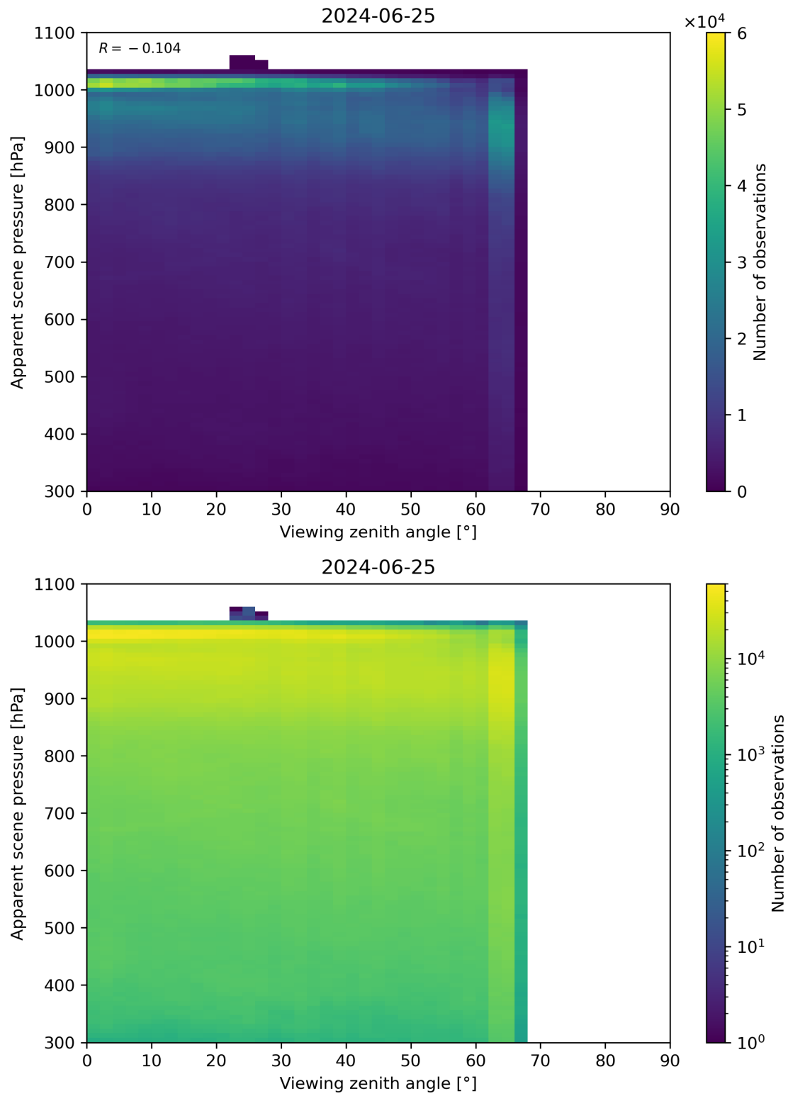
Figure 118: Scatter density plot of “Viewing zenith angle” against “Apparent scene pressure” for 2024-06-24 to 2024-06-26.
