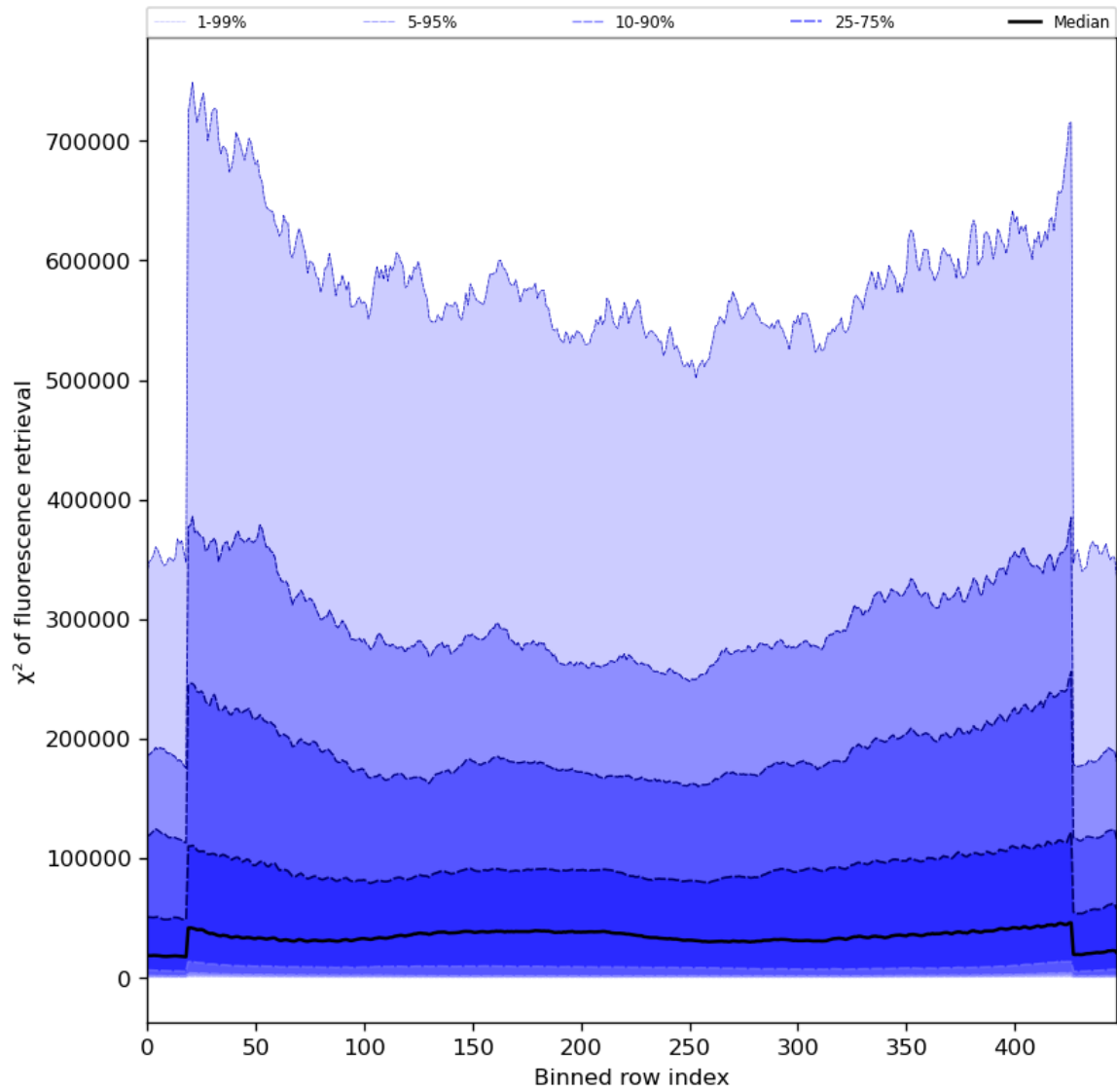
Figure 59: Along track statistics of “ \chi^2 of fluorescence retrieval” for 2024-06-24 to 2024-06-26
