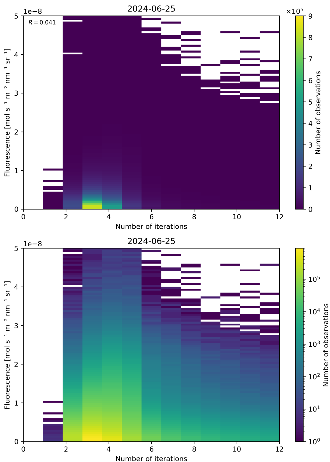
Figure 98: Scatter density plot of “Number of iterations” against “Fluorescence” for 2024-06-24 to 2024-06-26.
