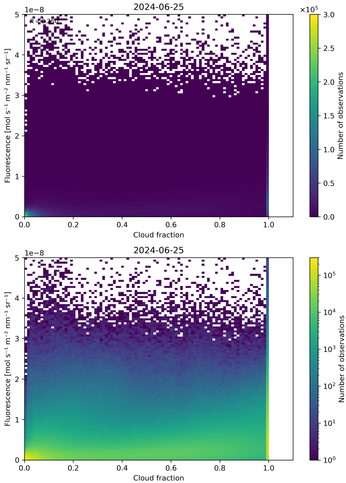
Figure 72: Scatter density plot of “Cloud fraction” against “Fluorescence” for 2024-06-24 to 2024-06-26.
