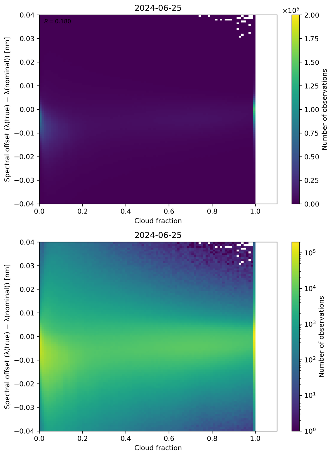
Figure 76: Scatter density plot of “Cloud fraction” against “Spectral offset ( \lambda(\text{true}) - \lambda(\text{nominal}) )” for 2024-06-24 to 2024-06-26.
