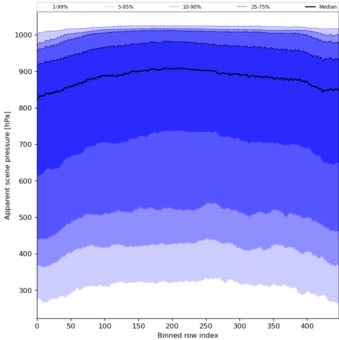
Figure 53: Along track statistics of “Apparent scene pressure” for 2024-06-24 to 2024-06-26
