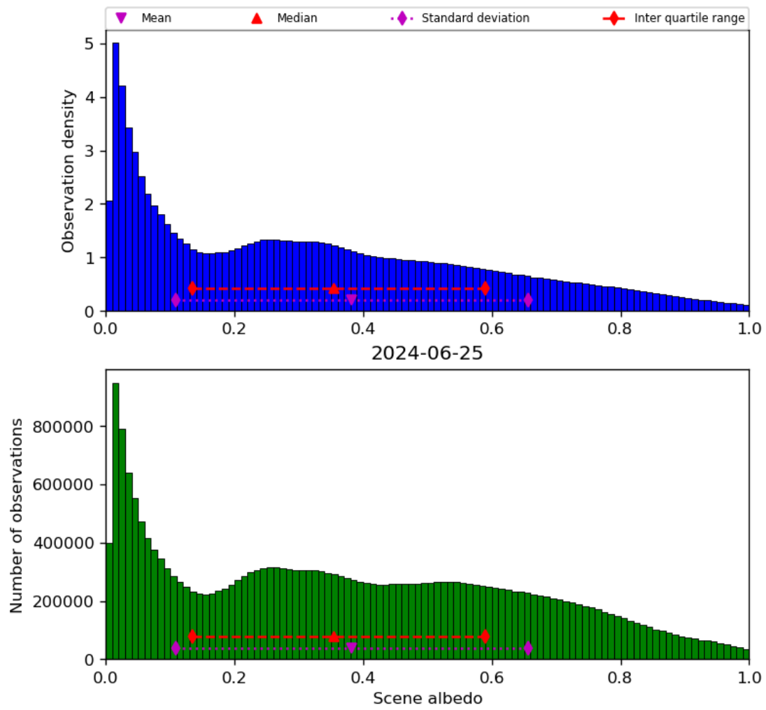
Figure 34: Histogram of “Scene albedo” for 2024-06-24 to 2024-06-26
