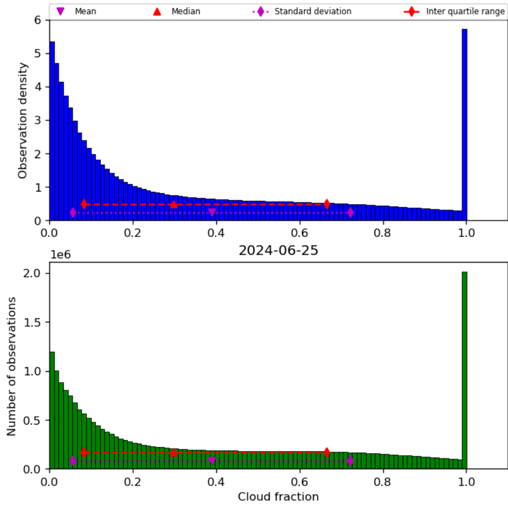
Figure 32: Histogram of “Cloud fraction” for 2024-06-24 to 2024-06-26
