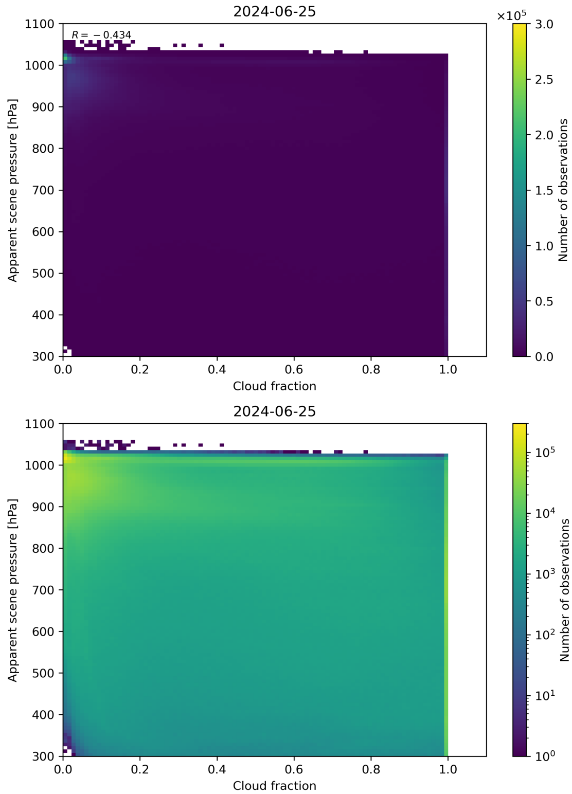
Figure 70: Scatter density plot of “Cloud fraction” against “Apparent scene pressure” for 2024-06-24 to 2024-06-26.
