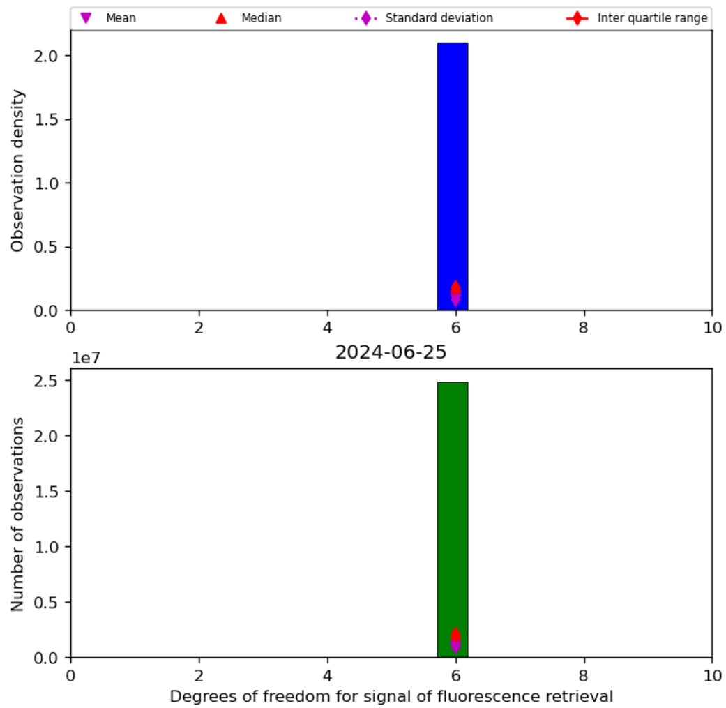
Figure 43: Histogram of “Degrees of freedom for signal of fluorescence retrieval” for 2024-06-24 to 2024-06-26
