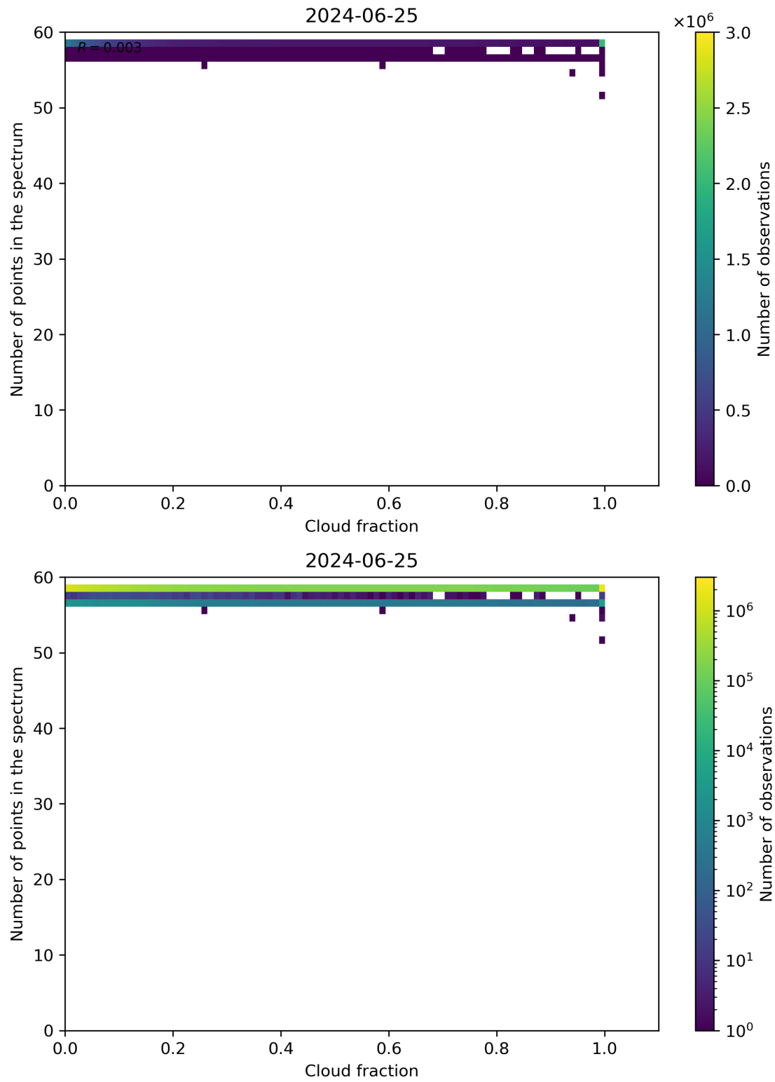
Figure 74: Scatter density plot of “Cloud fraction” against “Number of points in the spectrum” for 2024-06-24 to 2024-06-26.
