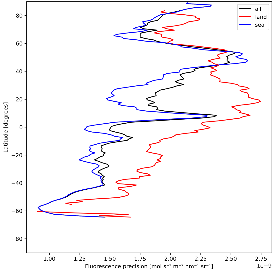
Figure 24: Zonal average of “Fluorescence precision” for 2024-06-24 to 2024-06-26.
