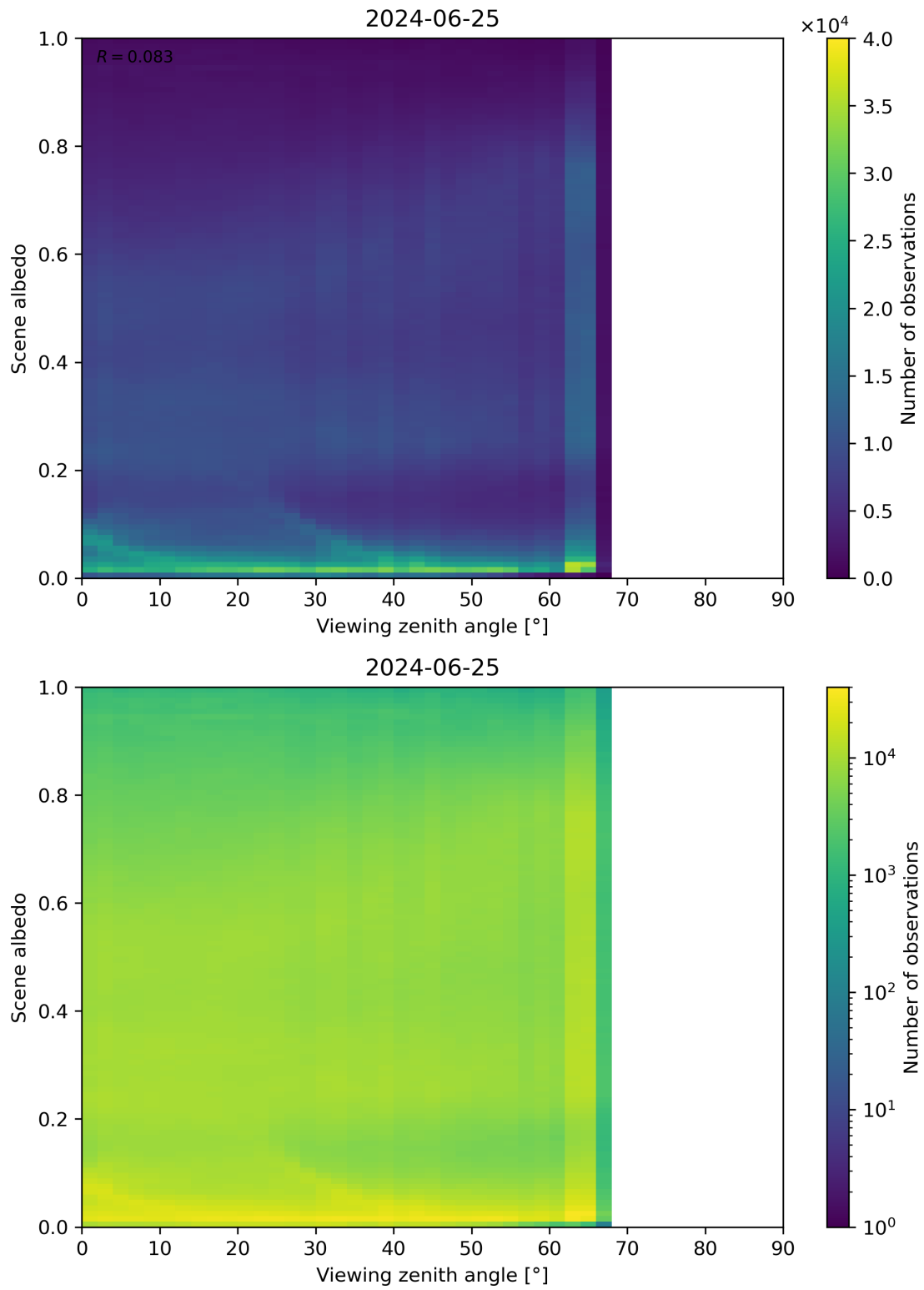
Figure 126: Scatter density plot of “Viewing zenith angle” against “Scene albedo” for 2024-06-24 to 2024-06-26.
