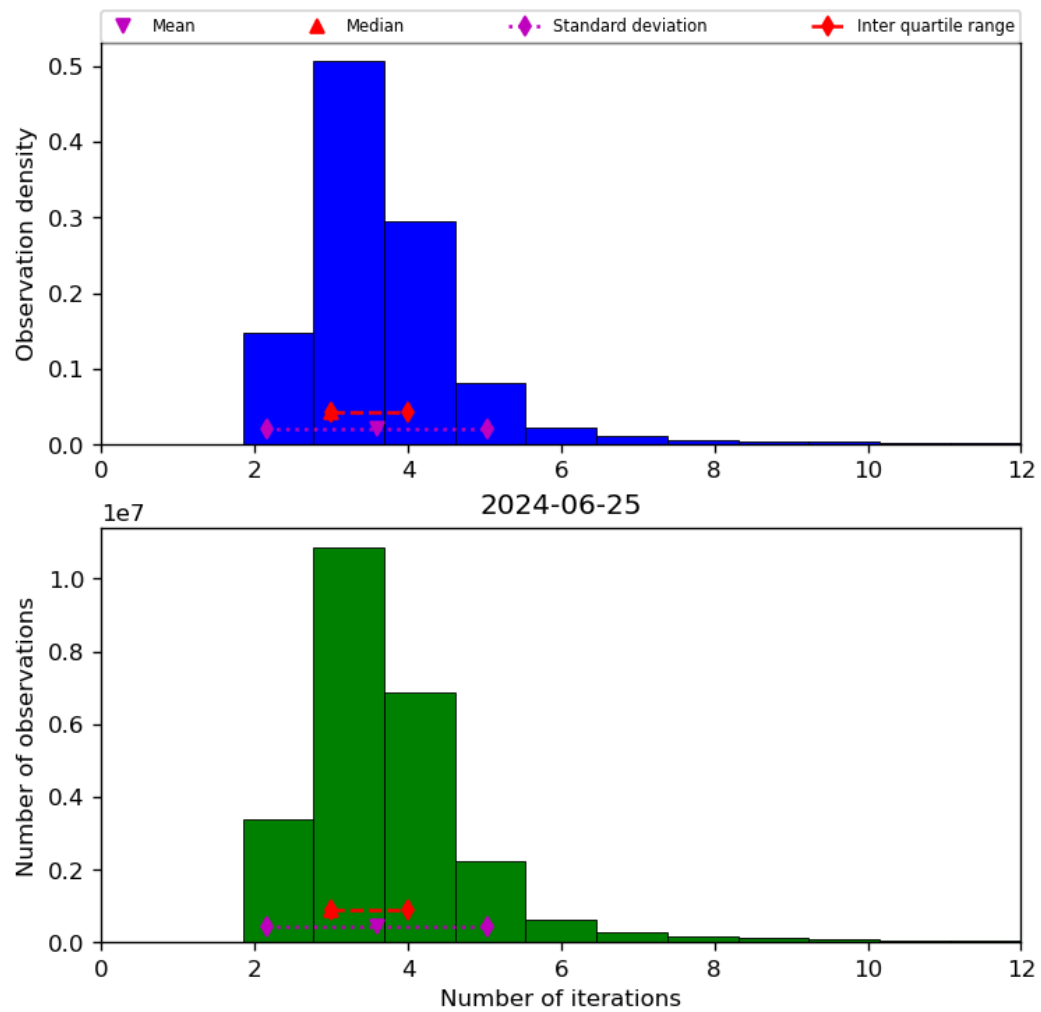
Figure 39: Histogram of “Number of iterations” for 2024-06-24 to 2024-06-26
