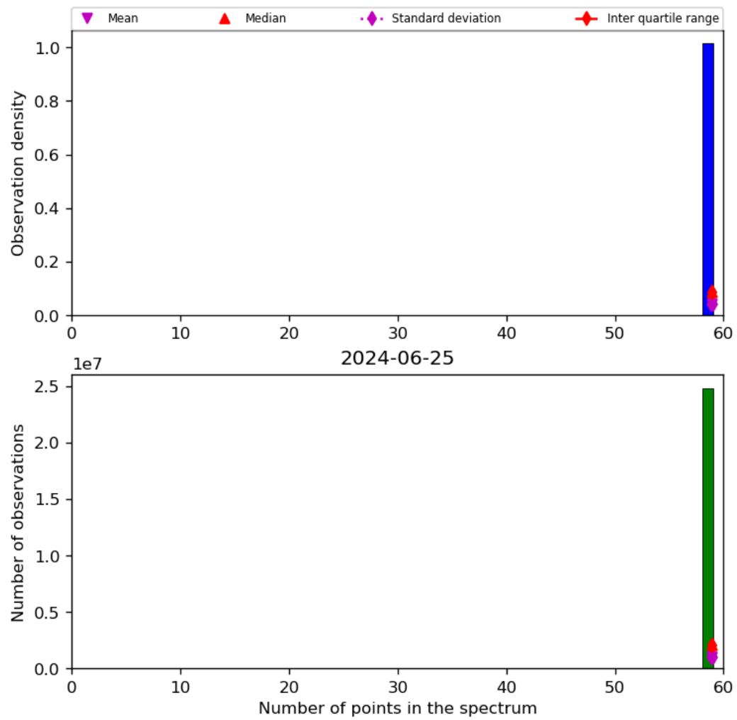
Figure 44: Histogram of “Number of points in the spectrum” for 2024-06-24 to 2024-06-26
