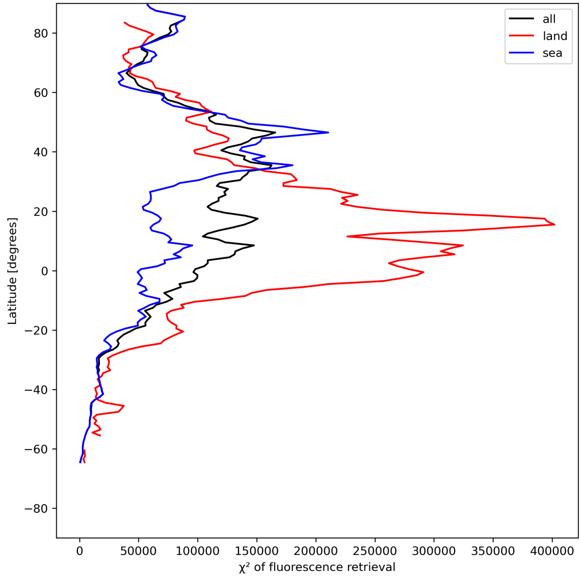
Figure 25: Zonal average of “ \chi^2 of fluorescence retrieval” for 2024-06-24 to 2024-06-26.
