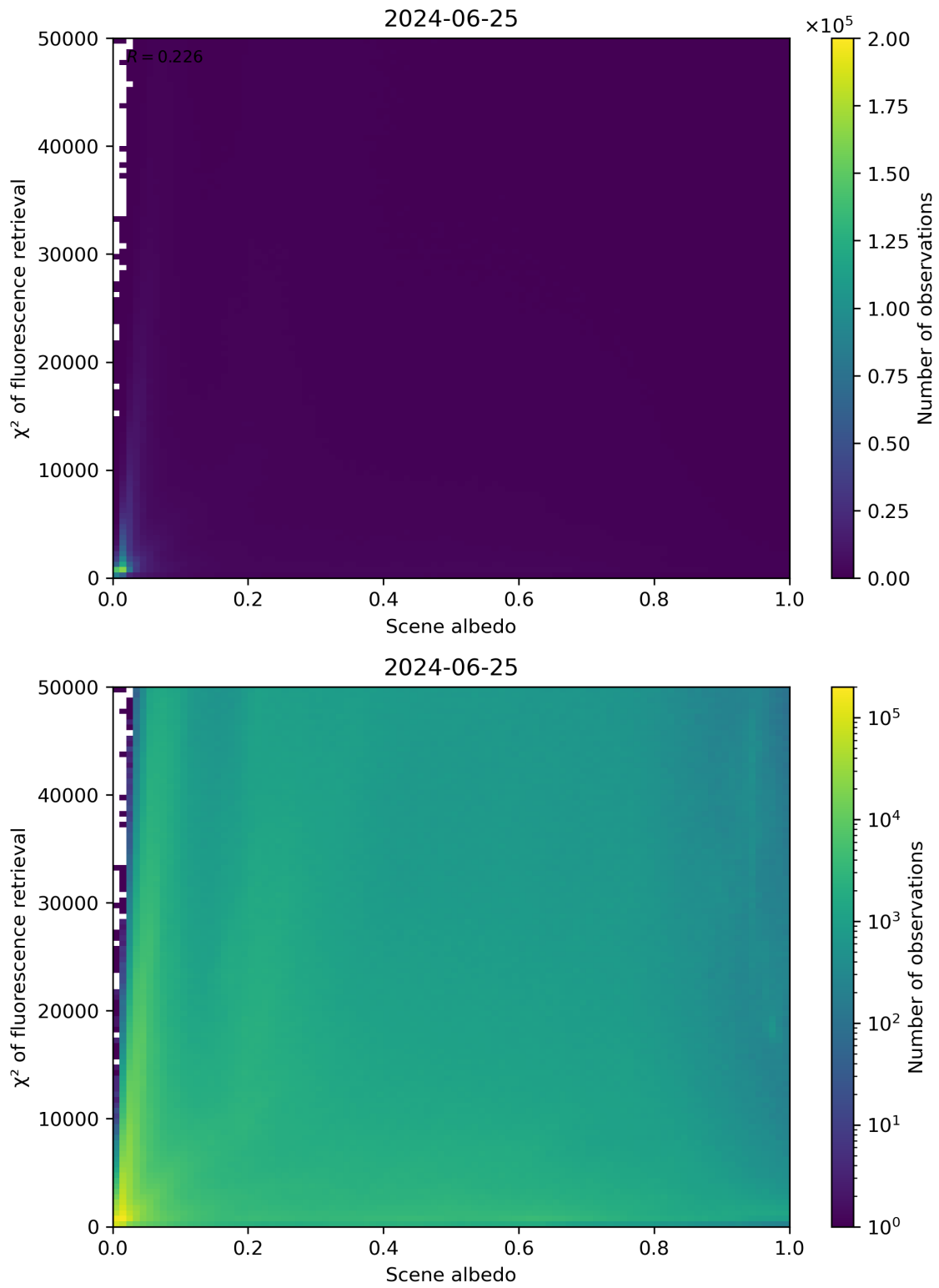
Figure 103: Scatter density plot of “Scene albedo” against “ \chi^2 of fluorescence retrieval” for 2024-06-24 to 2024-06-26.
