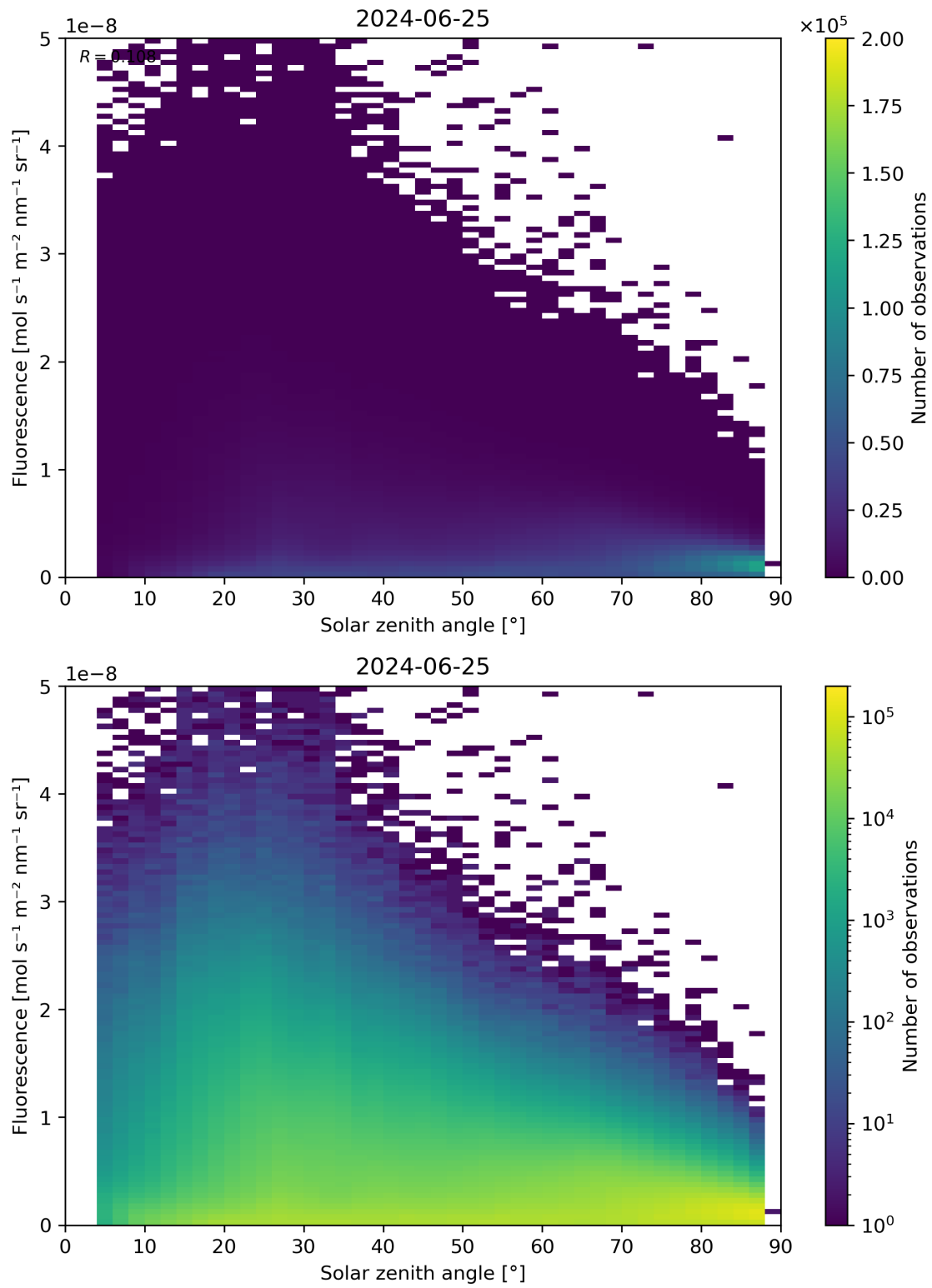
Figure 112: Scatter density plot of “Solar zenith angle” against “Fluorescence” for 2024-06-24 to 2024-06-26.
