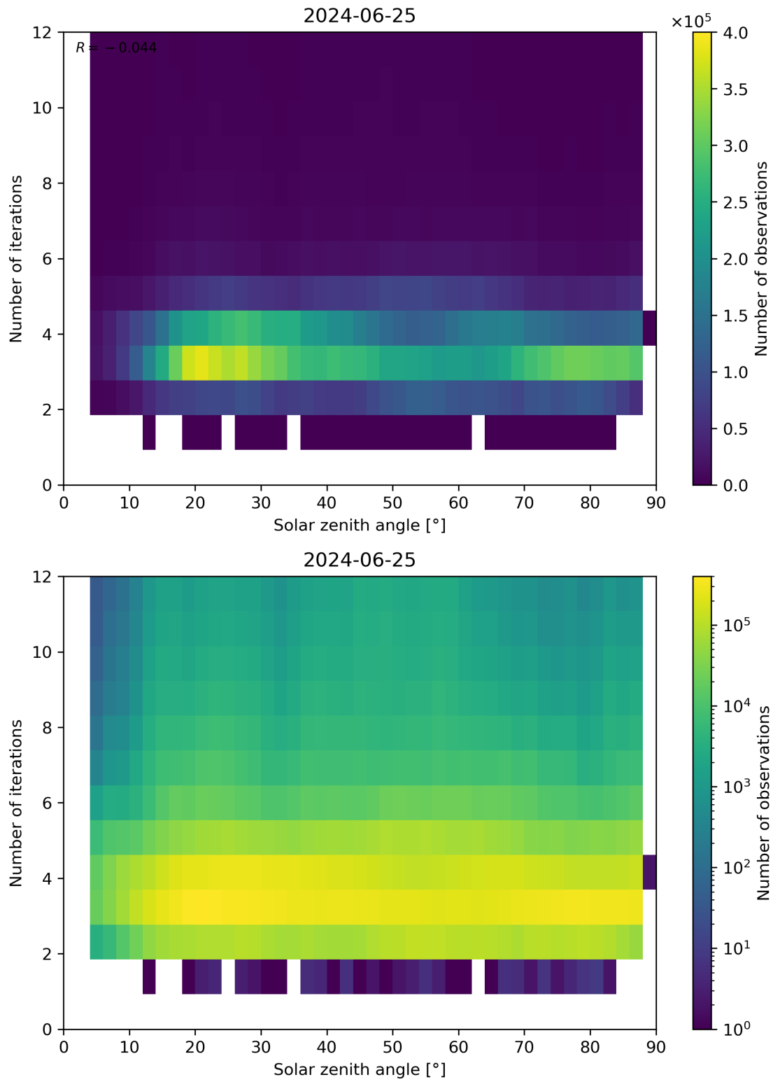
Figure 114: Scatter density plot of “Solar zenith angle” against “Number of iterations” for 2024-06-24 to 2024-06-26.
