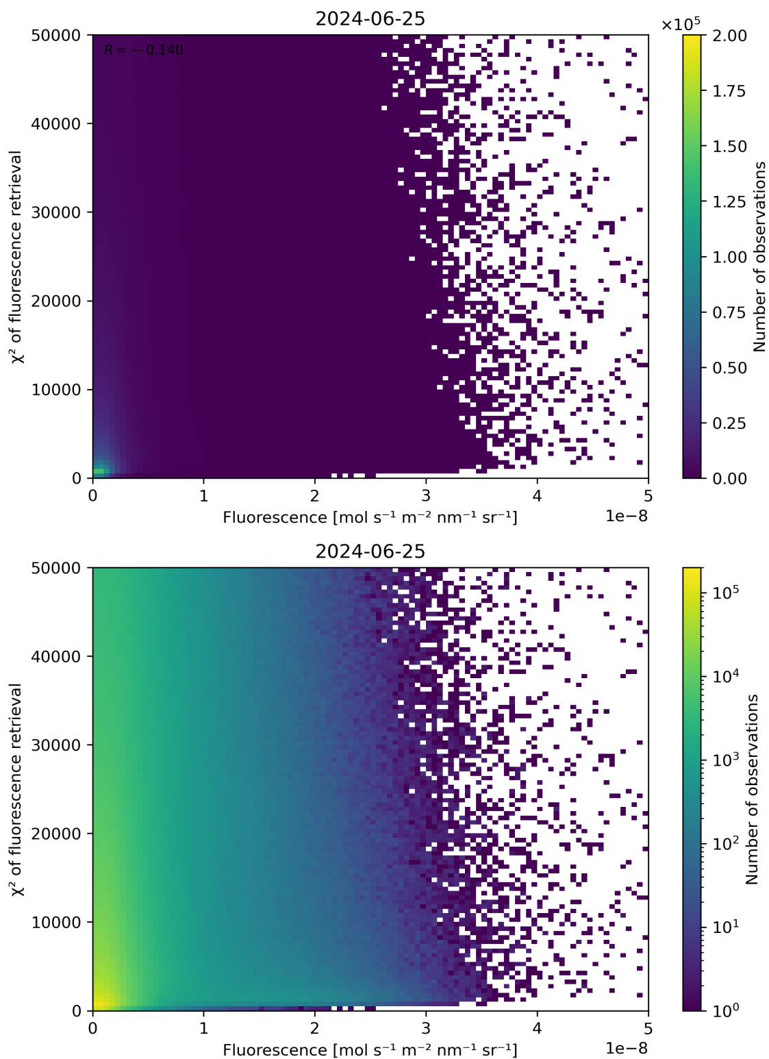
Figure 85: Scatter density plot of “Fluorescence” against “ \chi^2 of fluorescence retrieval” for 2024-06-24 to 2024-06-26.
