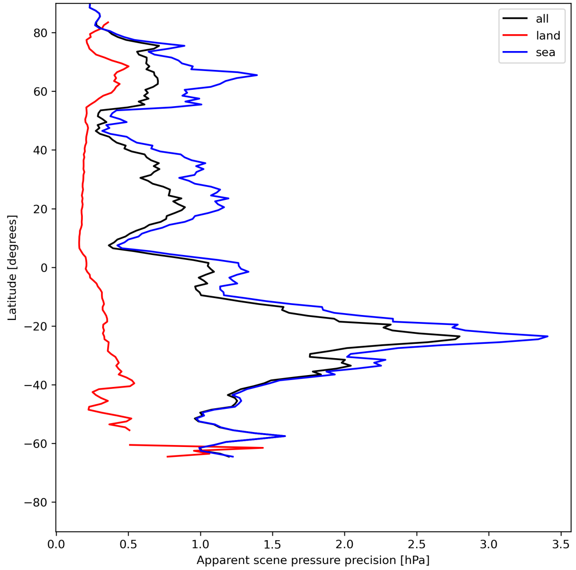
Figure 20: Zonal average of “Apparent scene pressure precision” for 2024-06-24 to 2024-06-26.
