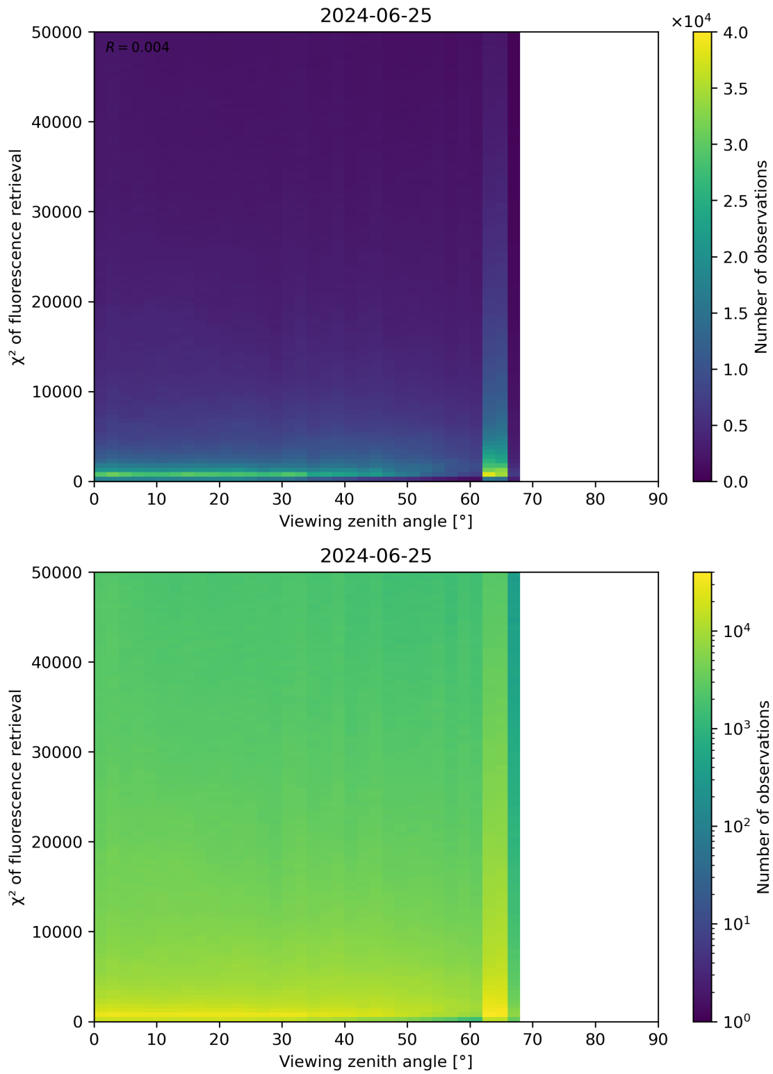
Figure 119: Scatter density plot of “Viewing zenith angle” against “ \chi^2 of fluorescence retrieval” for 2024-06-24 to 2024-06-26.
