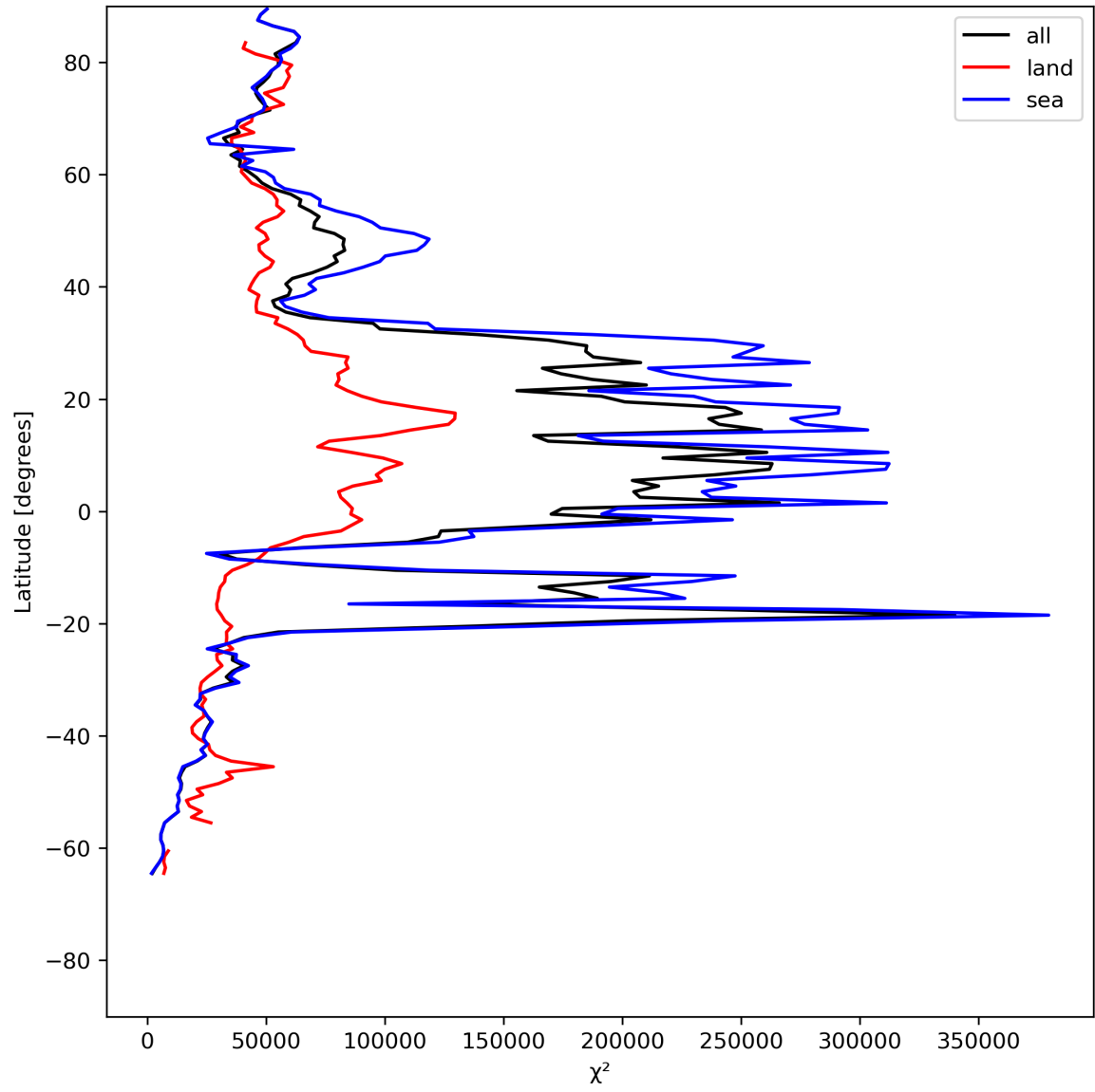
Figure 21: Zonal average of “ \chi^2 ” for 2024-06-24 to 2024-06-26.
