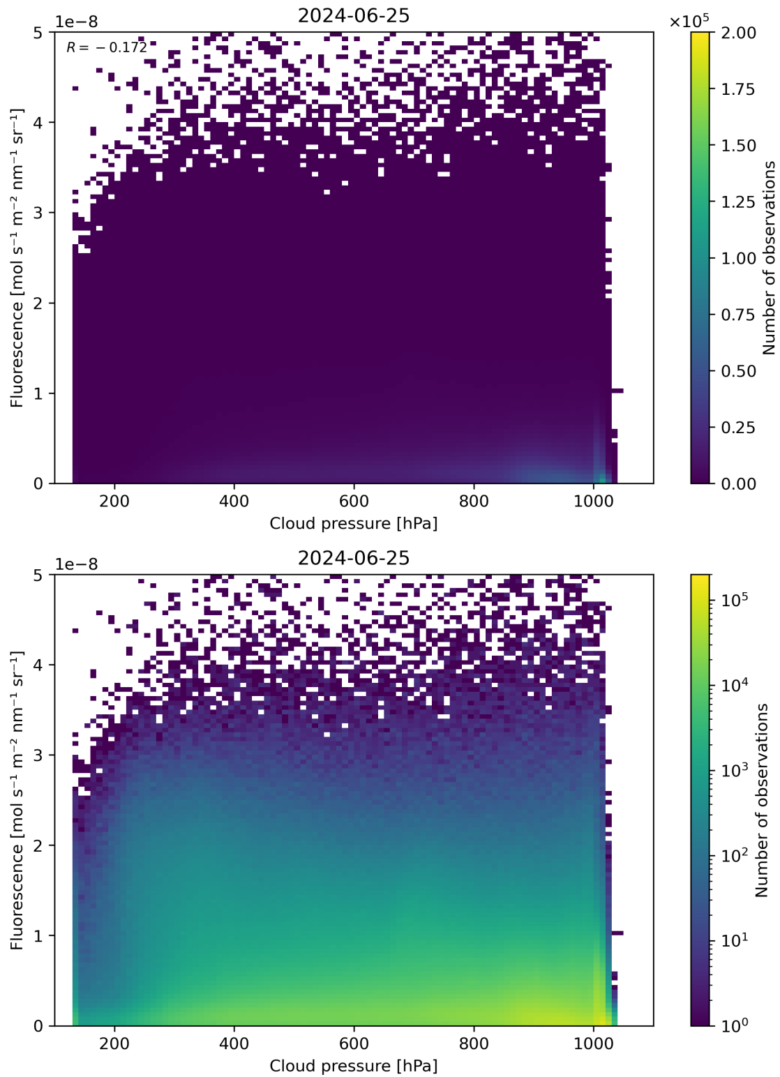
Figure 80: Scatter density plot of “Cloud pressure” against “Fluorescence” for 2024-06-24 to 2024-06-26.
