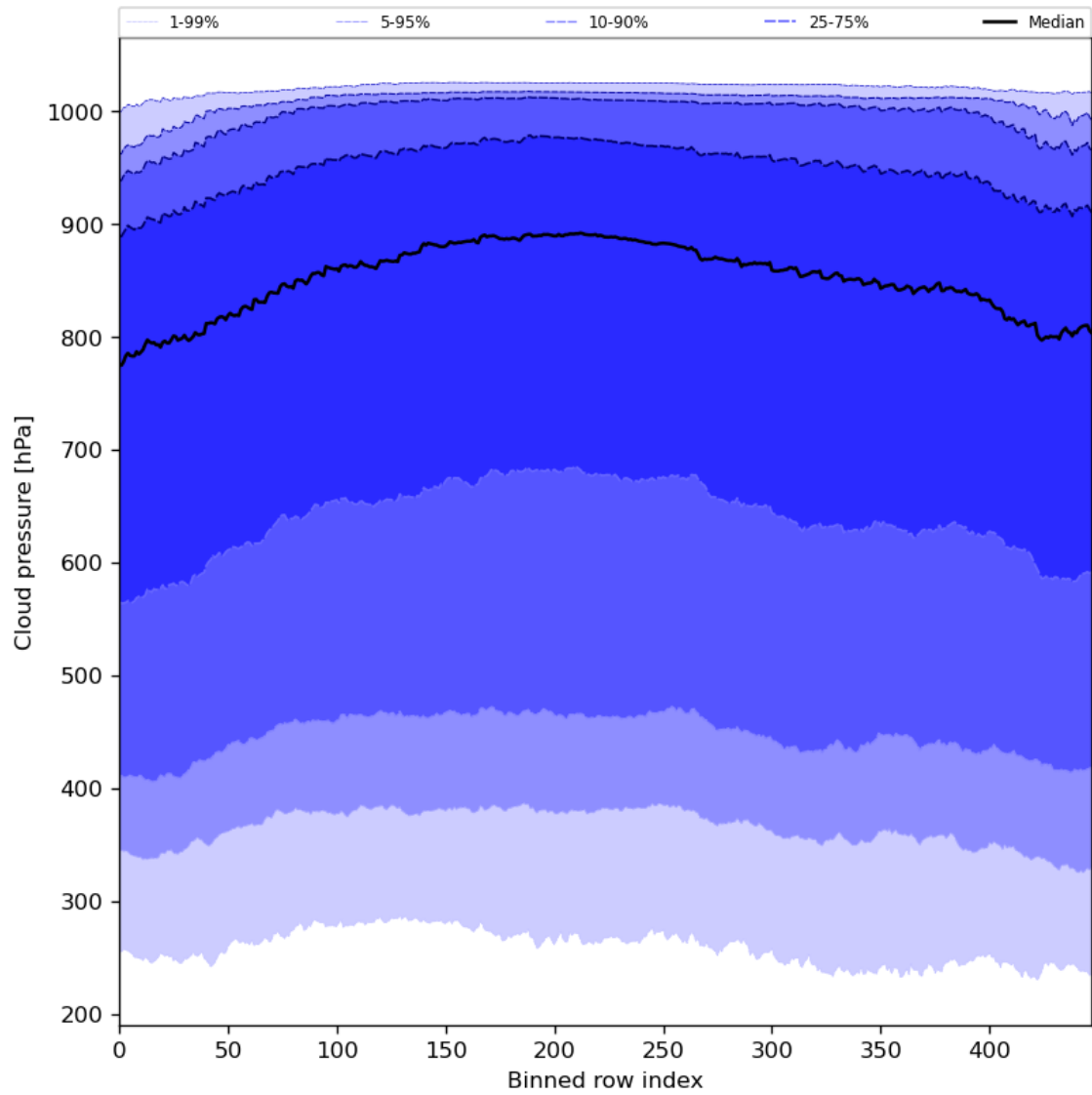
Figure 47: Along track statistics of “Cloud pressure” for 2024-06-24 to 2024-06-26
