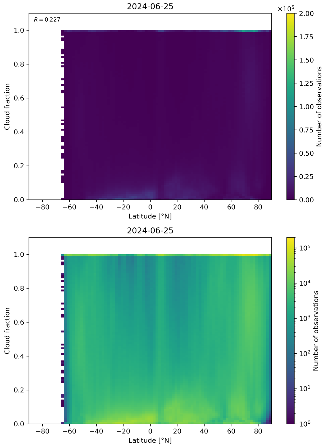
Figure 90: Scatter density plot of “Latitude” against “Cloud fraction” for 2024-06-24 to 2024-06-26.
