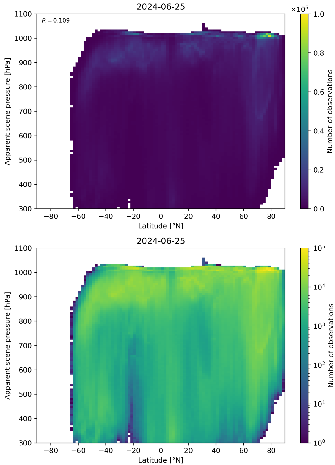
Figure 88: Scatter density plot of “Latitude” against “Apparent scene pressure” for 2024-06-24 to 2024-06-26.
