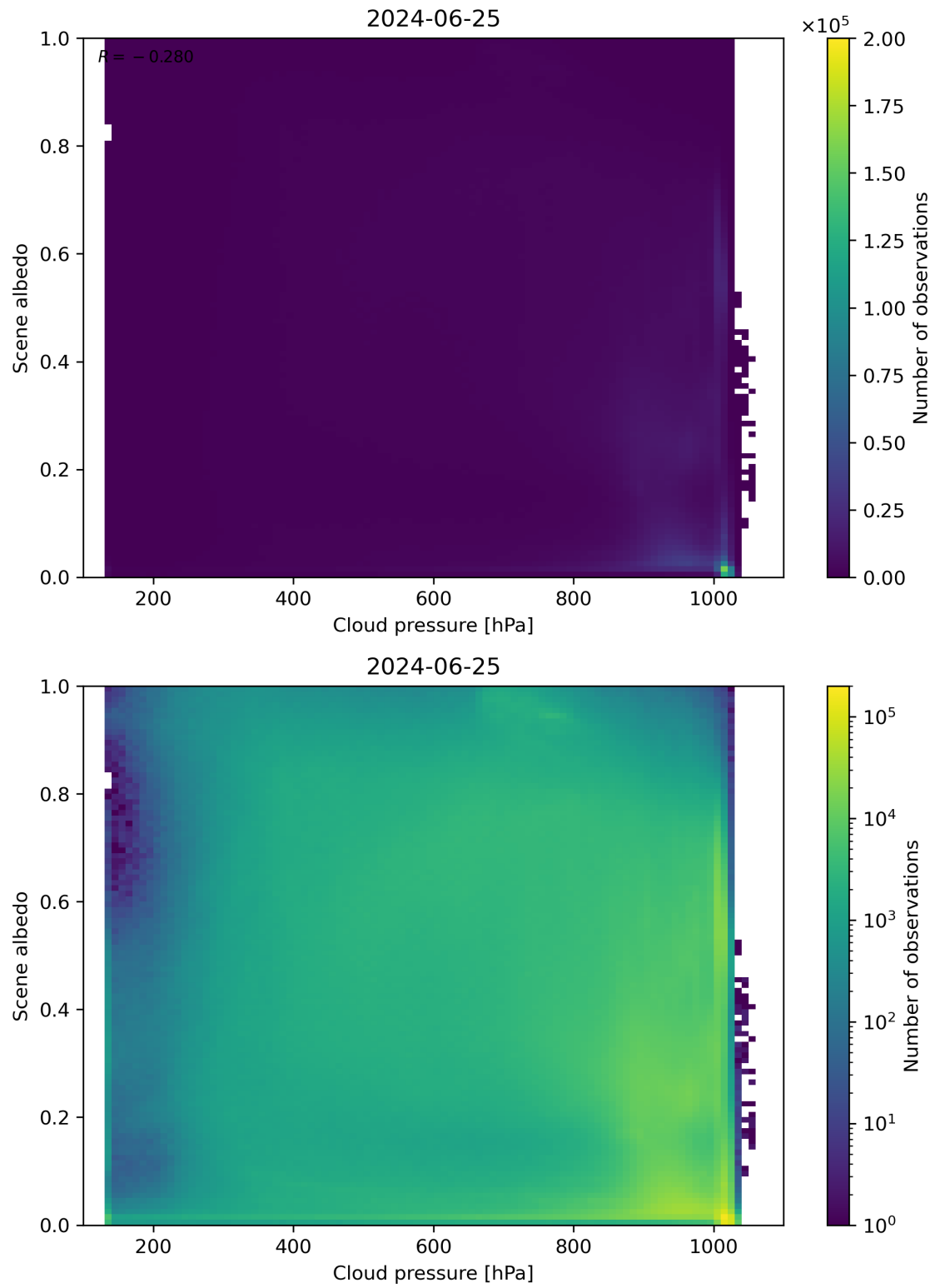
Figure 83: Scatter density plot of “Cloud pressure” against “Scene albedo” for 2024-06-24 to 2024-06-26.
