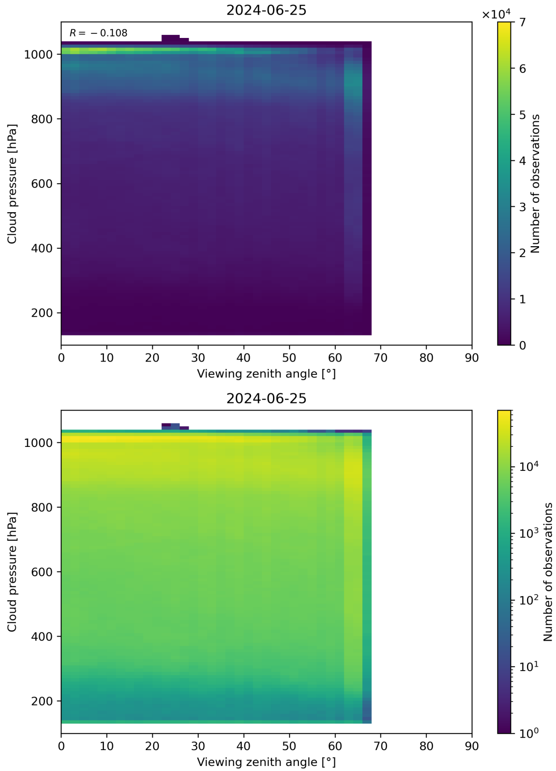
Figure 121: Scatter density plot of “Viewing zenith angle” against “Cloud pressure” for 2024-06-24 to 2024-06-26.
