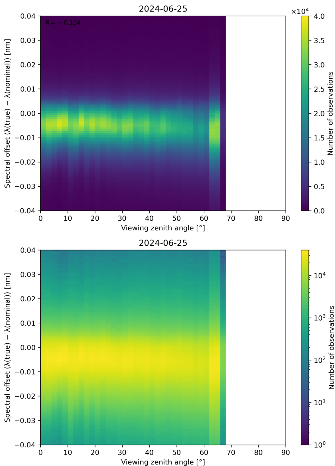
Figure 128: Scatter density plot of “Viewing zenith angle” against “Spectral offset ( \lambda(\text{true}) - \lambda(\text{nominal}) )” for 2024-06-24 to 2024-06-26.
