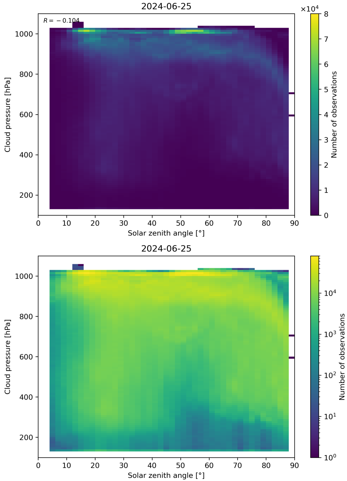
Figure 111: Scatter density plot of “Solar zenith angle” against “Cloud pressure” for 2024-06-24 to 2024-06-26.
