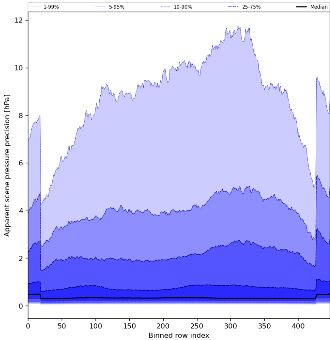
Figure 54: Along track statistics of “Apparent scene pressure precision” for 2024-06-24 to 2024-06-26
