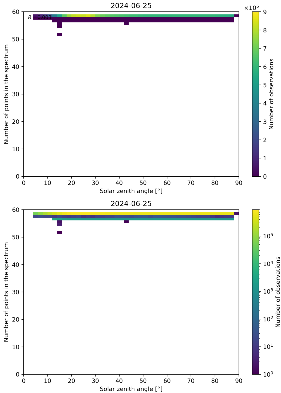
Figure 115: Scatter density plot of “Solar zenith angle” against “Number of points in the spectrum” for 2024-06-24 to 2024-06-26.
