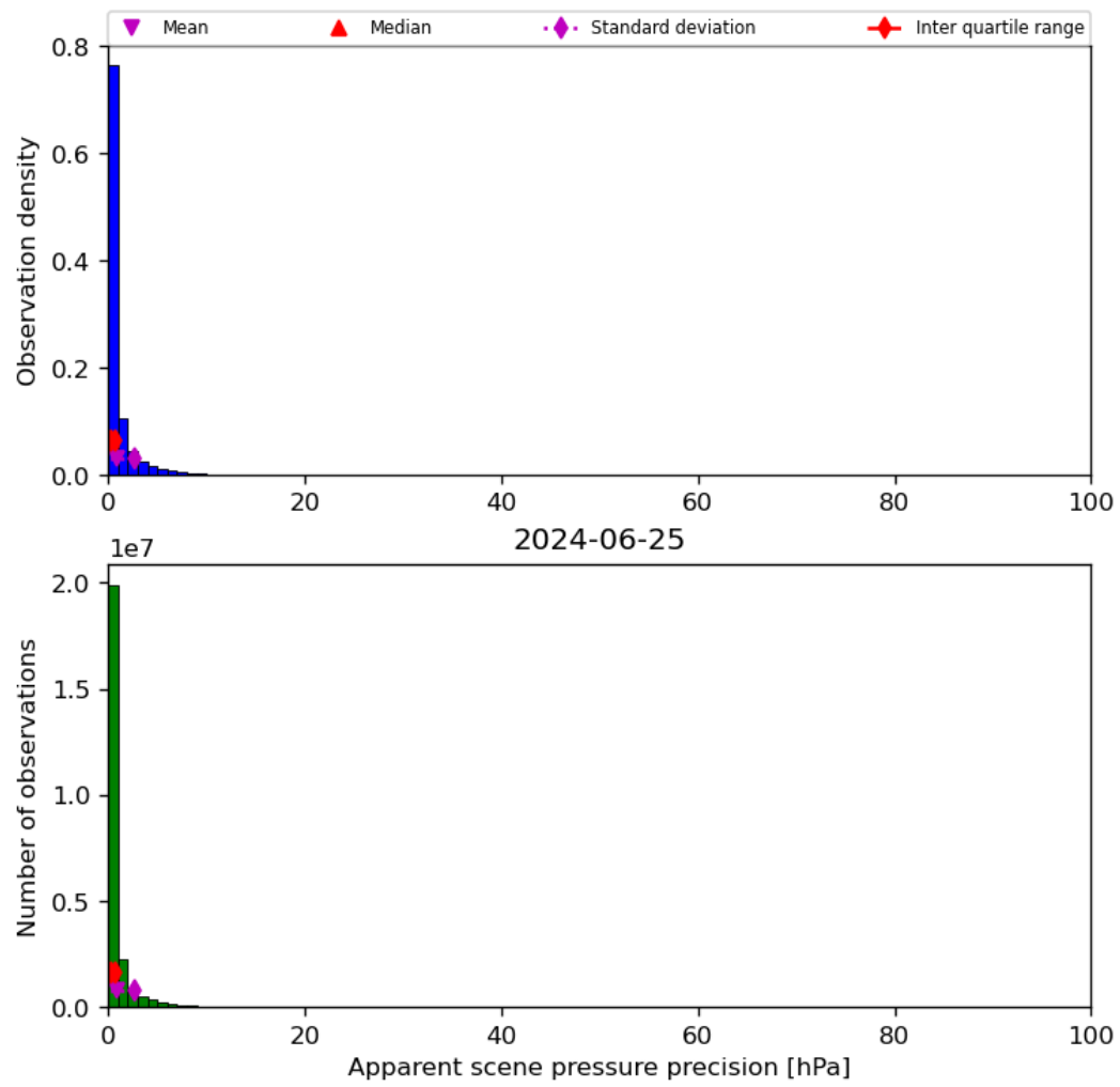
Figure 37: Histogram of “Apparent scene pressure precision” for 2024-06-24 to 2024-06-26
