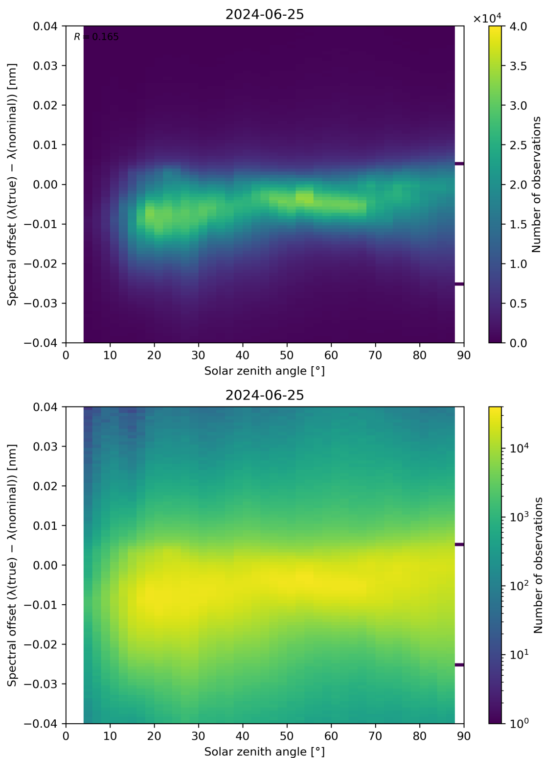
Figure 117: Scatter density plot of “Solar zenith angle” against “Spectral offset ( \lambda(\text{true}) - \lambda(\text{nominal}) )” for 2024-06-24 to 2024-06-26.
