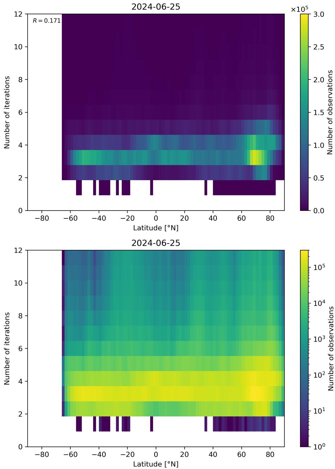
Figure 93: Scatter density plot of “Latitude” against “Number of iterations” for 2024-06-24 to 2024-06-26.
