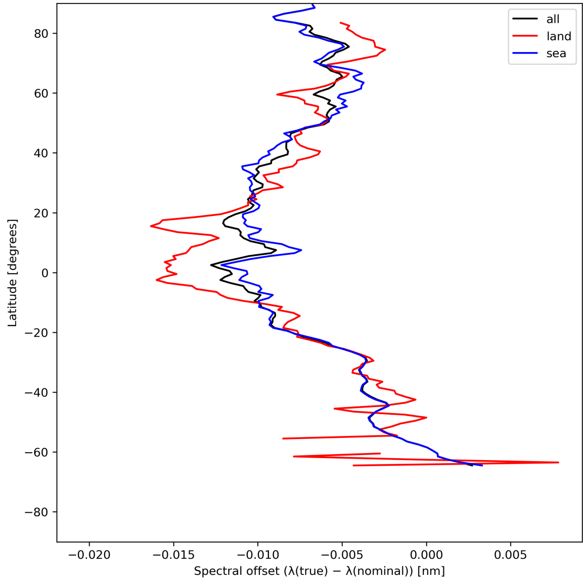
Figure 28: Zonal average of “Spectral offset ( \lambda(\text{true}) - \lambda(\text{nominal}) )” for 2024-06-24 to 2024-06-26.
