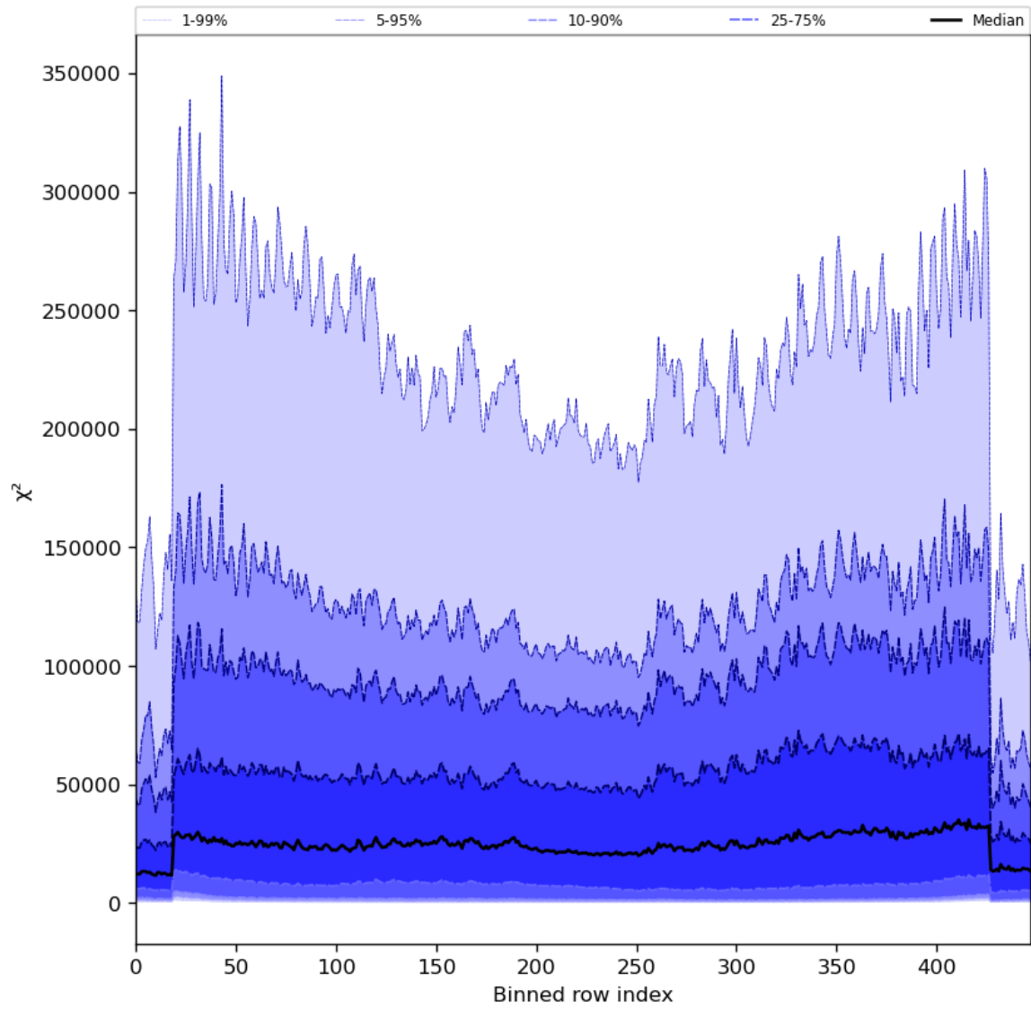
Figure 55: Along track statistics of “ \chi^2 ” for 2024-06-24 to 2024-06-26
