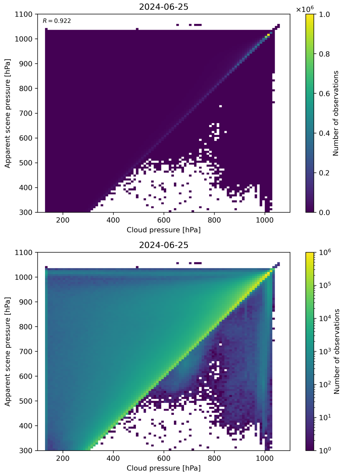
Figure 77: Scatter density plot of “Cloud pressure” against “Apparent scene pressure” for 2024-06-24 to 2024-06-26.
