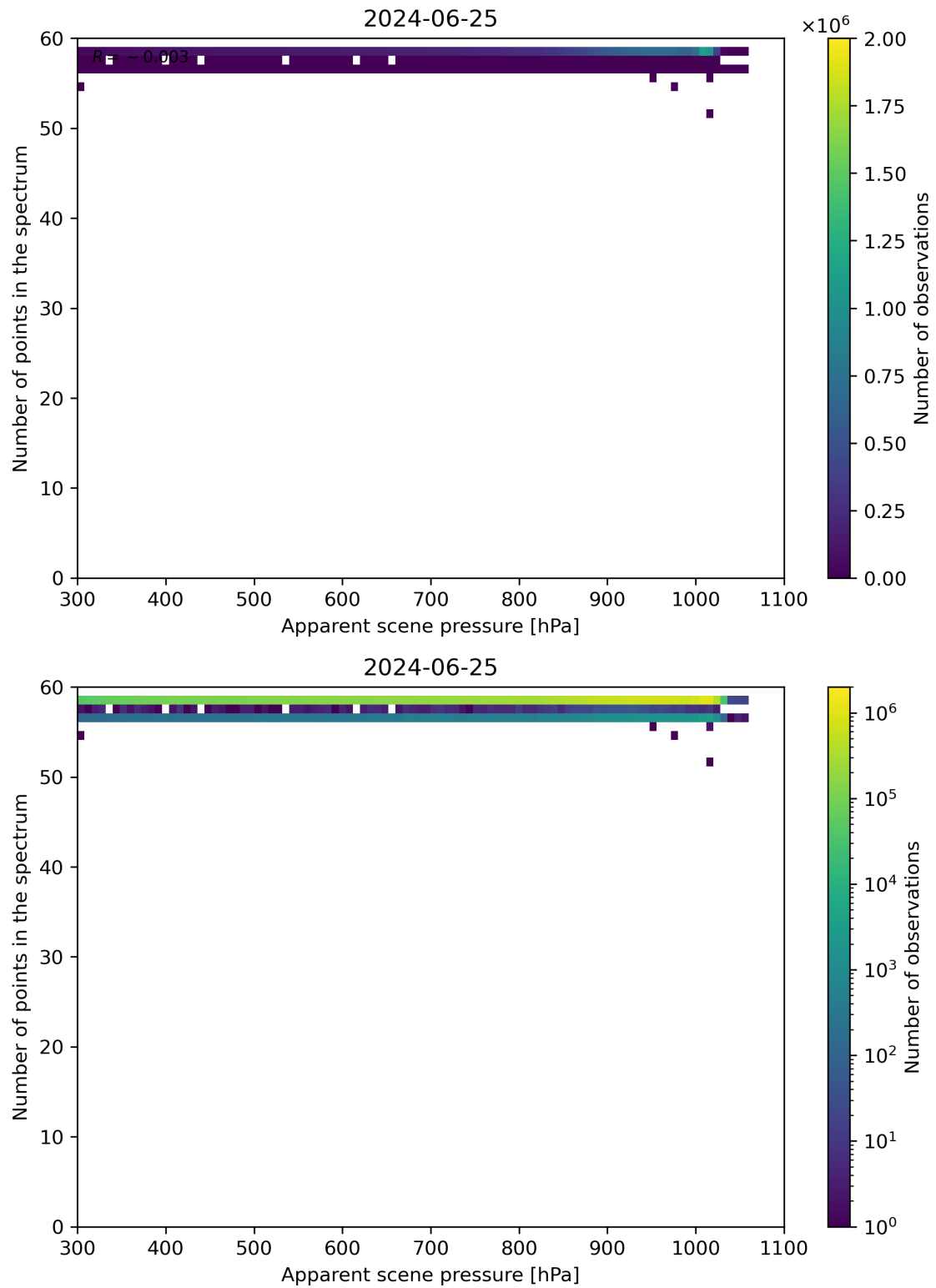
Figure 66: Scatter density plot of “Apparent scene pressure” against “Number of points in the spectrum” for 2024-06-24 to 2024-06-26.
