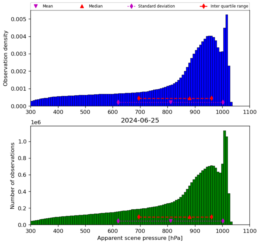
Figure 36: Histogram of “Apparent scene pressure” for 2024-06-24 to 2024-06-26
