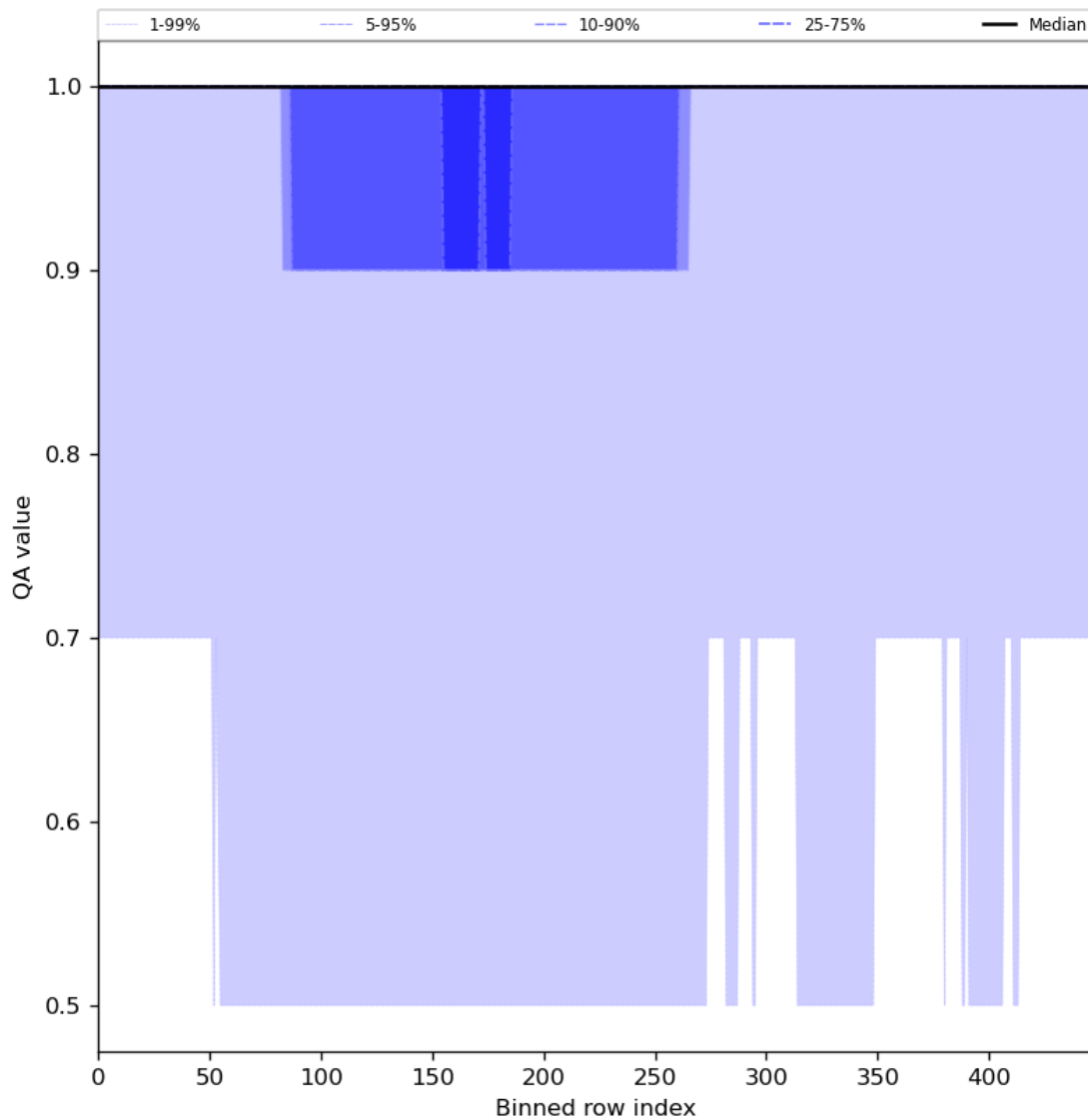
Figure 46: Along track statistics of “QA value” for 2024-06-24 to 2024-06-26
