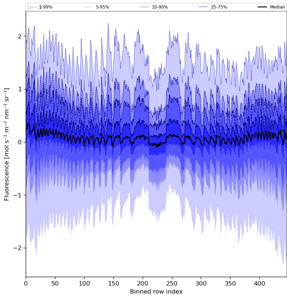
Figure 57: Along track statistics of “Fluorescence” for 2024-06-24 to 2024-06-26
