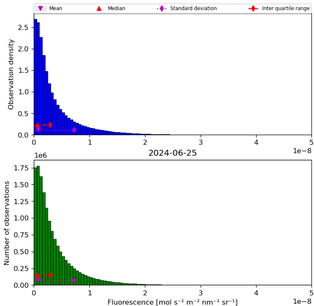
Figure 40: Histogram of “Fluorescence” for 2024-06-24 to 2024-06-26
