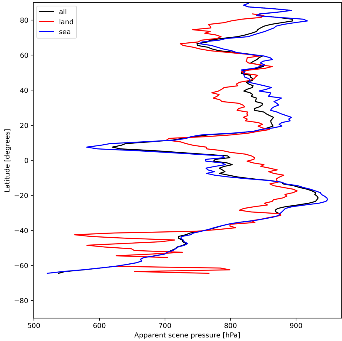
Figure 19: Zonal average of “Apparent scene pressure” for 2024-06-24 to 2024-06-26.
