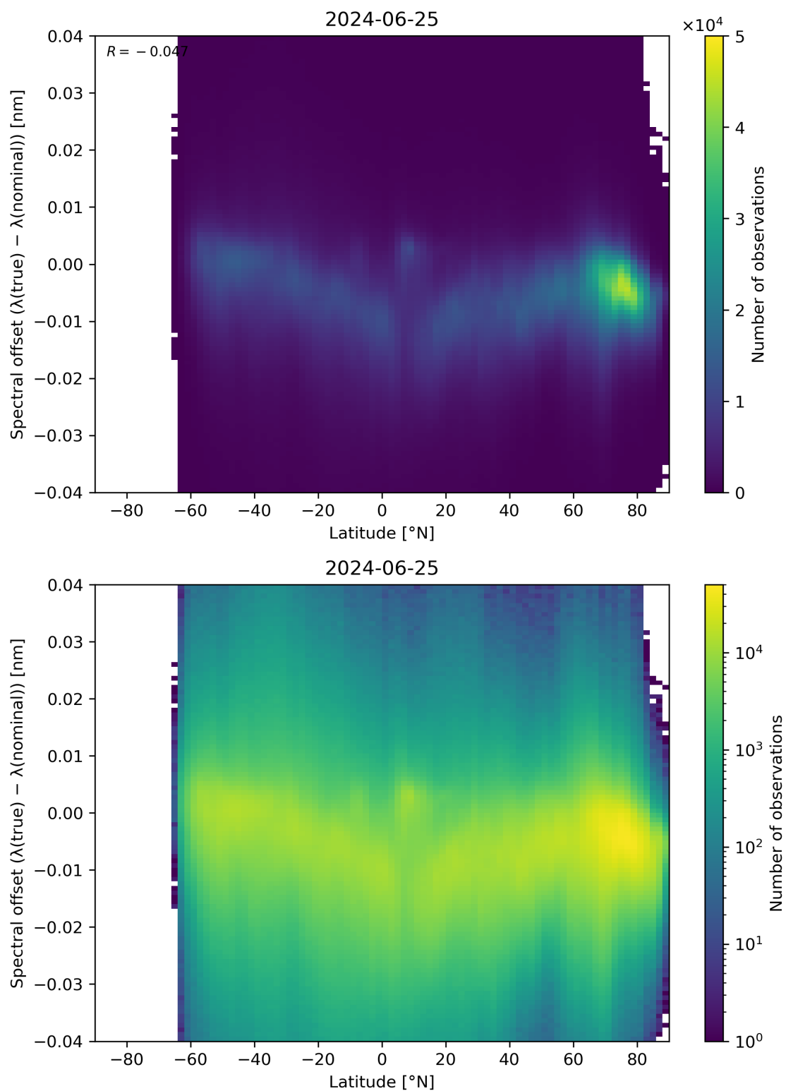
Figure 96: Scatter density plot of “Latitude” against “Spectral offset ( \lambda(\text{true}) - \lambda(\text{nominal}) )” for 2024-06-24 to 2024-06-26.
