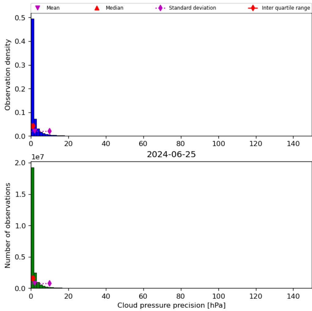
Figure 31: Histogram of “Cloud pressure precision” for 2024-06-24 to 2024-06-26
