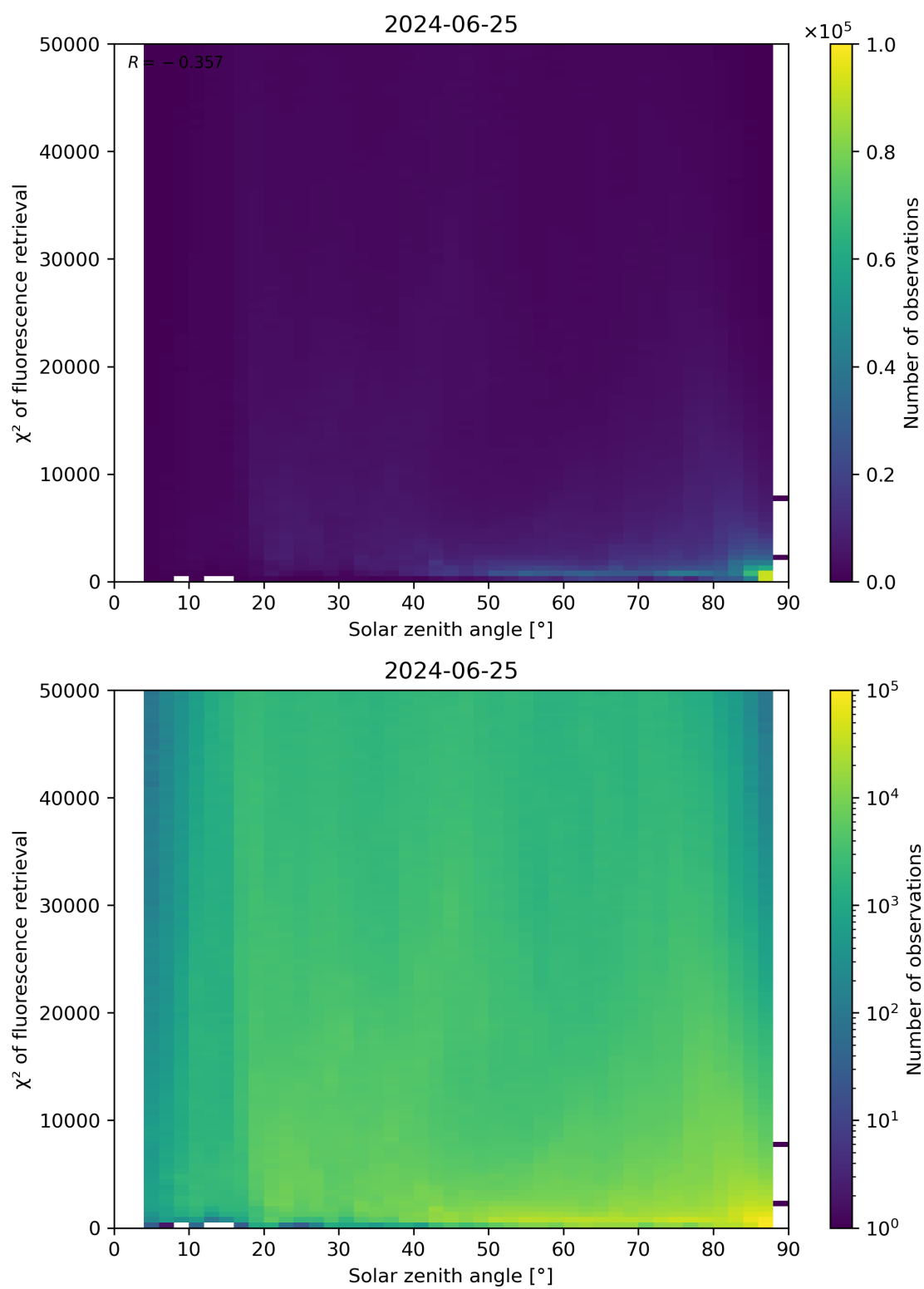
Figure 109: Scatter density plot of “Solar zenith angle” against “ \chi^2 of fluorescence retrieval” for 2024-06-24 to 2024-06-26.
