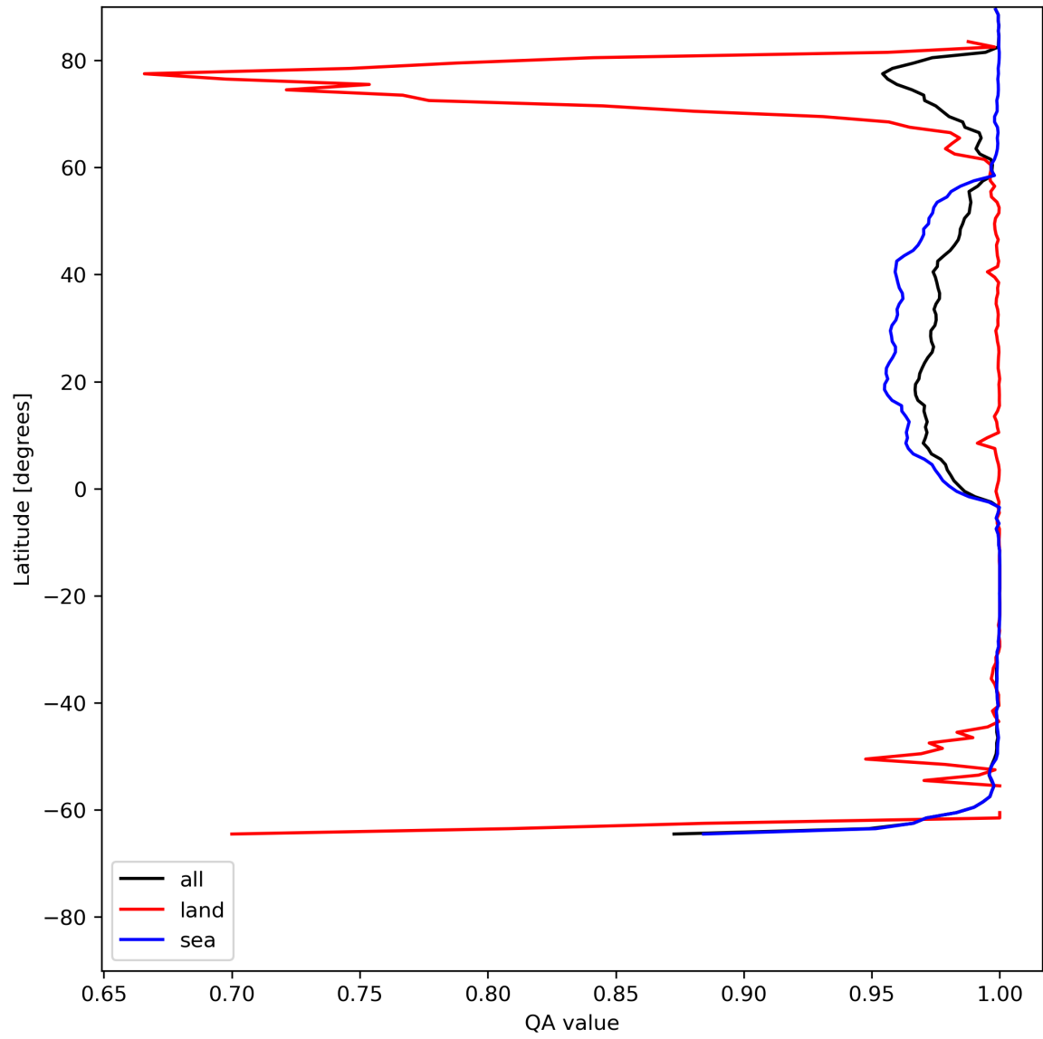
Figure 12: Zonal average of “QA value” for 2024-06-24 to 2024-06-26.
