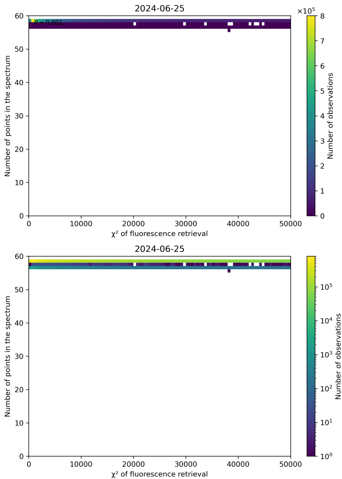
Figure 68: Scatter density plot of " \chi^2 of fluorescence retrieval" against "Number of points in the spectrum" for 2024-06-24 to 2024-06-26.
