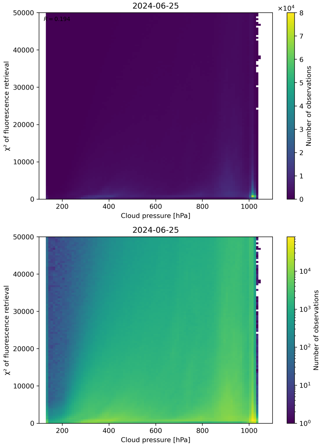
Figure 78: Scatter density plot of “Cloud pressure” against “ \chi^2 of fluorescence retrieval” for 2024-06-24 to 2024-06-26.
