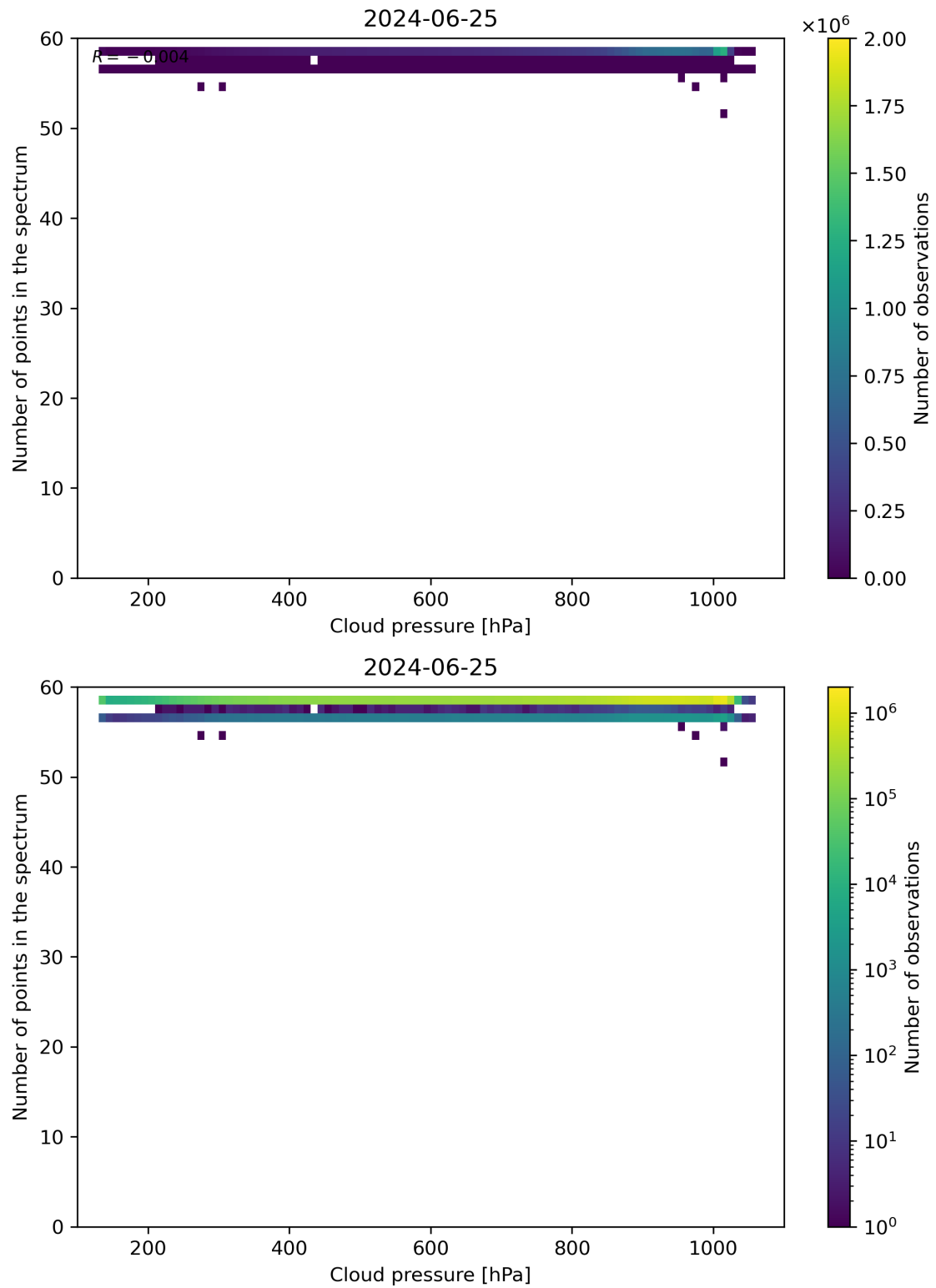
Figure 82: Scatter density plot of “Cloud pressure” against “Number of points in the spectrum” for 2024-06-24 to 2024-06-26.
