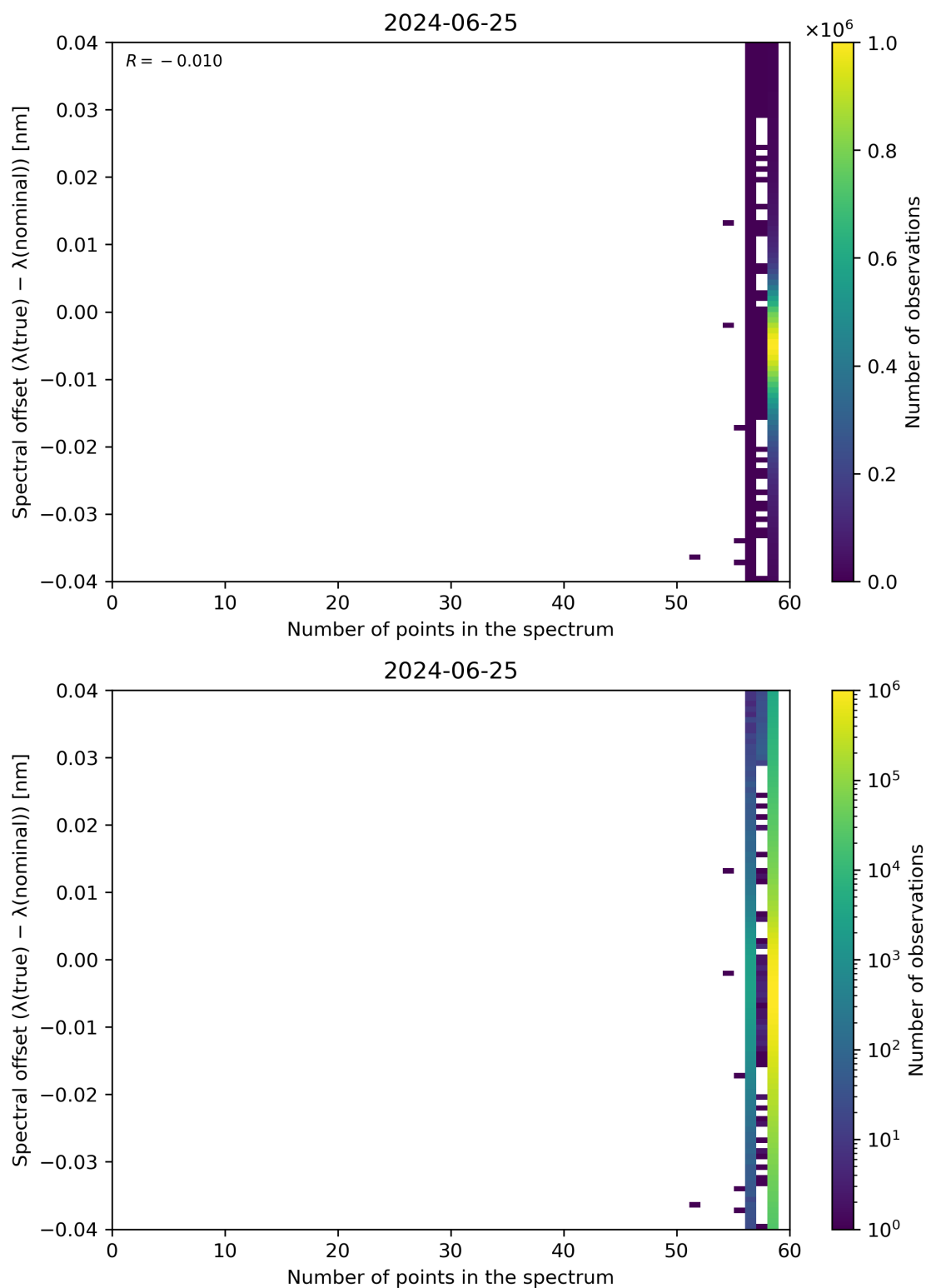
Figure 101: Scatter density plot of “Number of points in the spectrum” against “Spectral offset ( \lambda(\text{true}) - \lambda(\text{nominal}) )” for 2024-06-24 to 2024-06-26.
