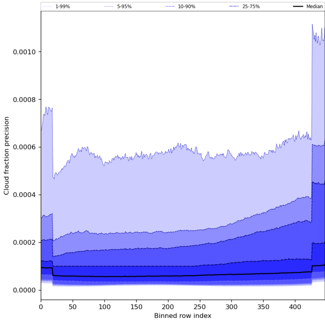
Figure 50: Along track statistics of “Cloud fraction precision” for 2024-06-24 to 2024-06-26
