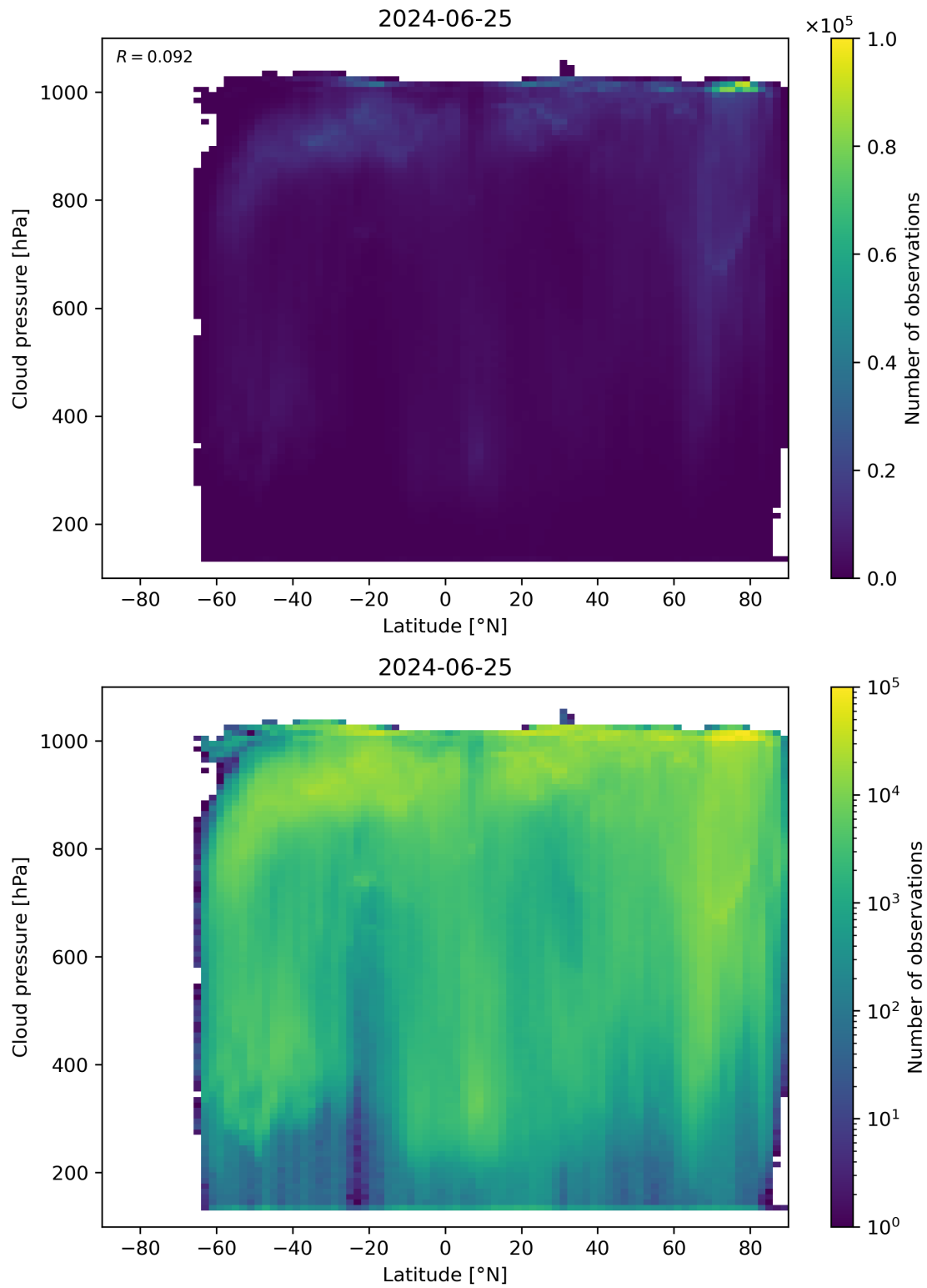
Figure 91: Scatter density plot of “Latitude” against “Cloud pressure” for 2024-06-24 to 2024-06-26.
