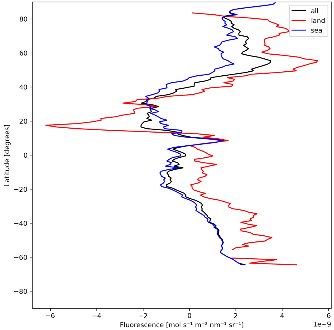
Figure 23: Zonal average of “Fluorescence” for 2024-06-24 to 2024-06-26.
