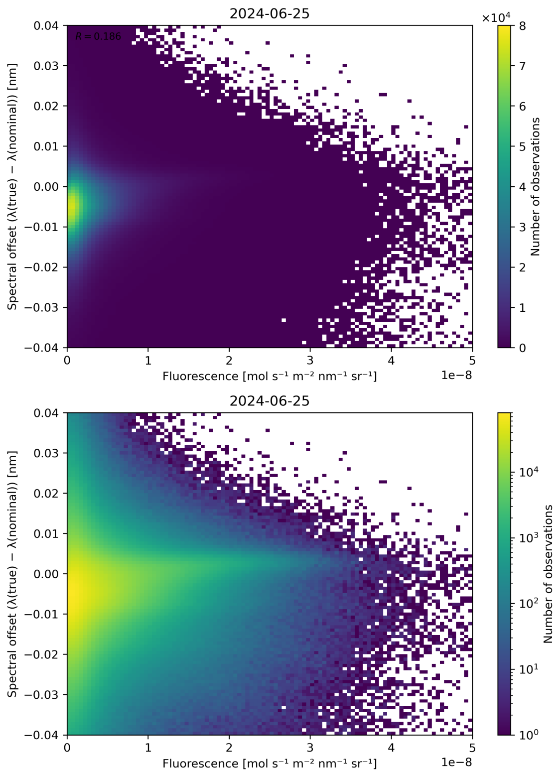
Figure 87: Scatter density plot of “Fluorescence” against “Spectral offset ( \lambda(\text{true}) - \lambda(\text{nominal}) )” for 2024-06-24 to 2024-06-26.
