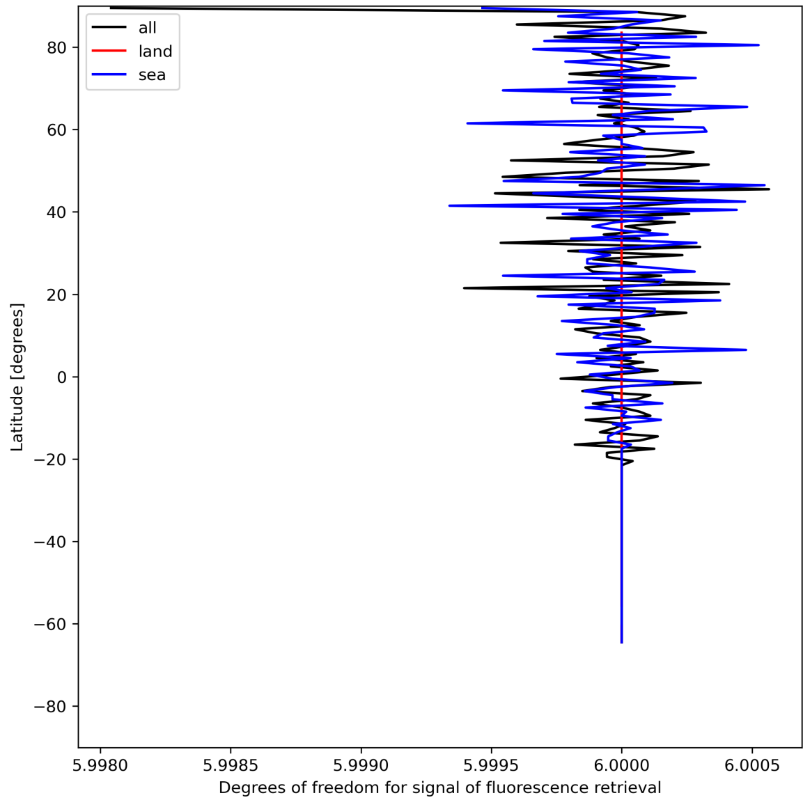
Figure 26: Zonal average of “Degrees of freedom for signal of fluorescence retrieval” for 2024-06-24 to 2024-06-26.
