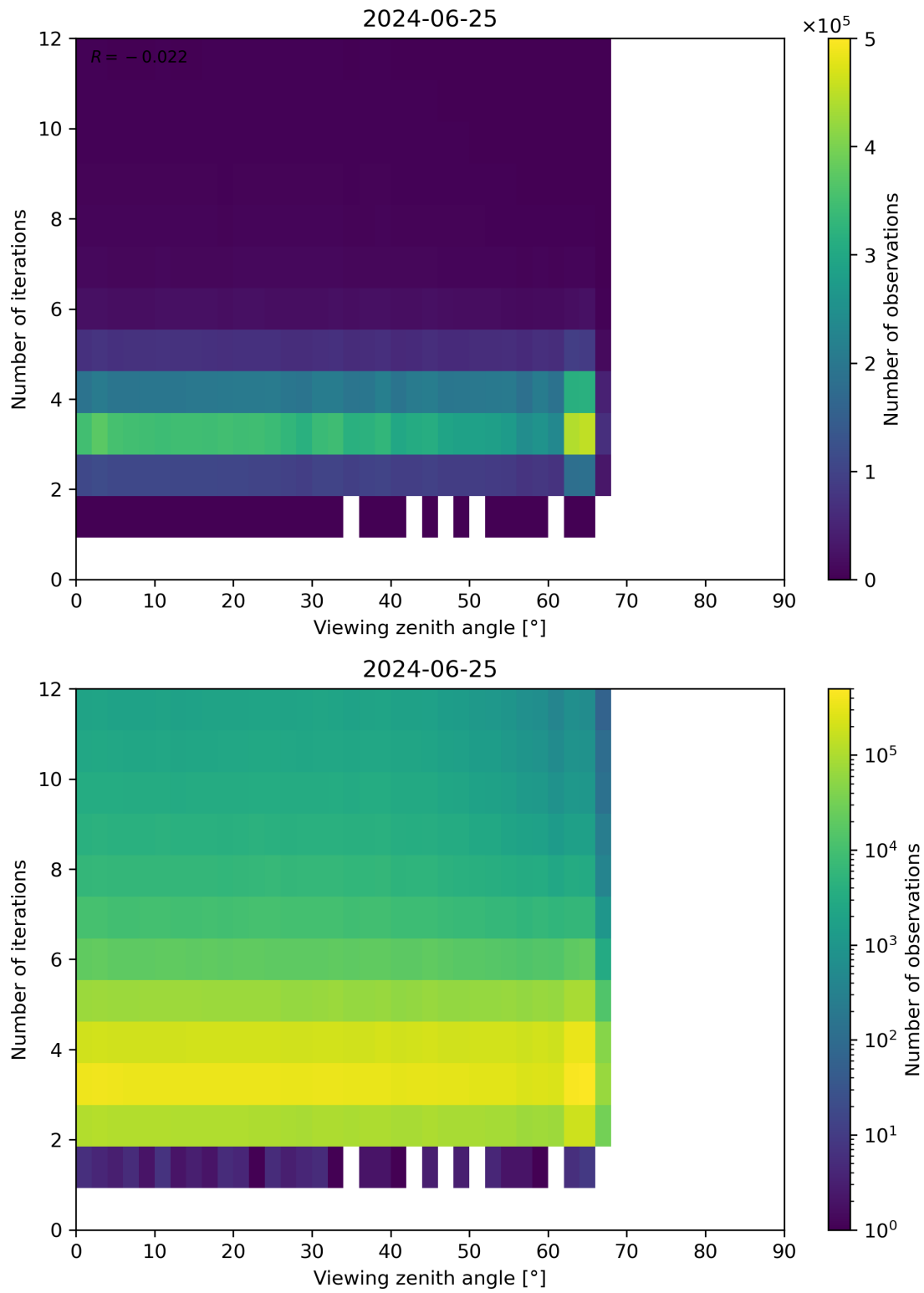
Figure 124: Scatter density plot of “Viewing zenith angle” against “Number of iterations” for 2024-06-24 to 2024-06-26.
