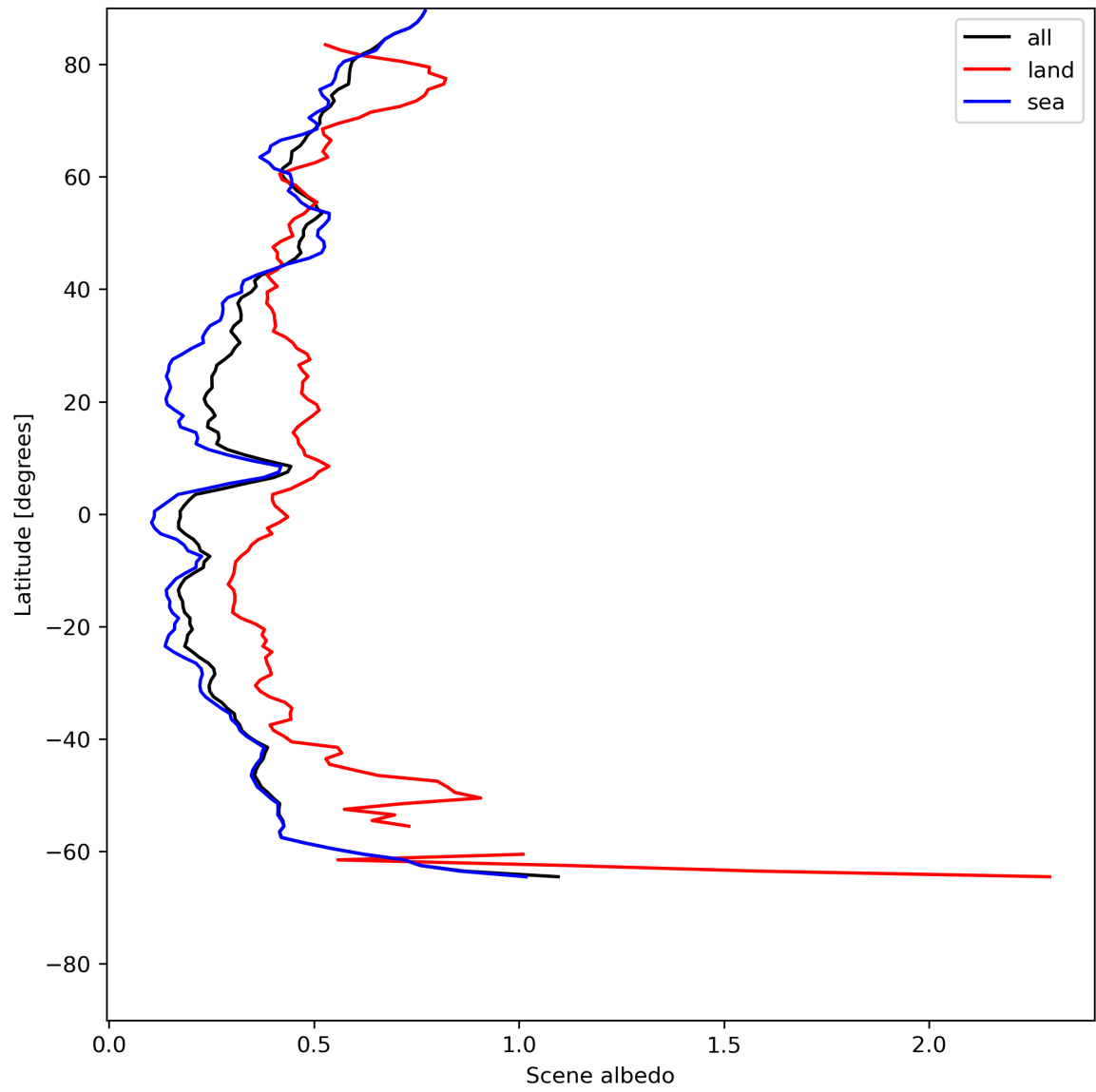
Figure 17: Zonal average of “Scene albedo” for 2024-06-24 to 2024-06-26.
