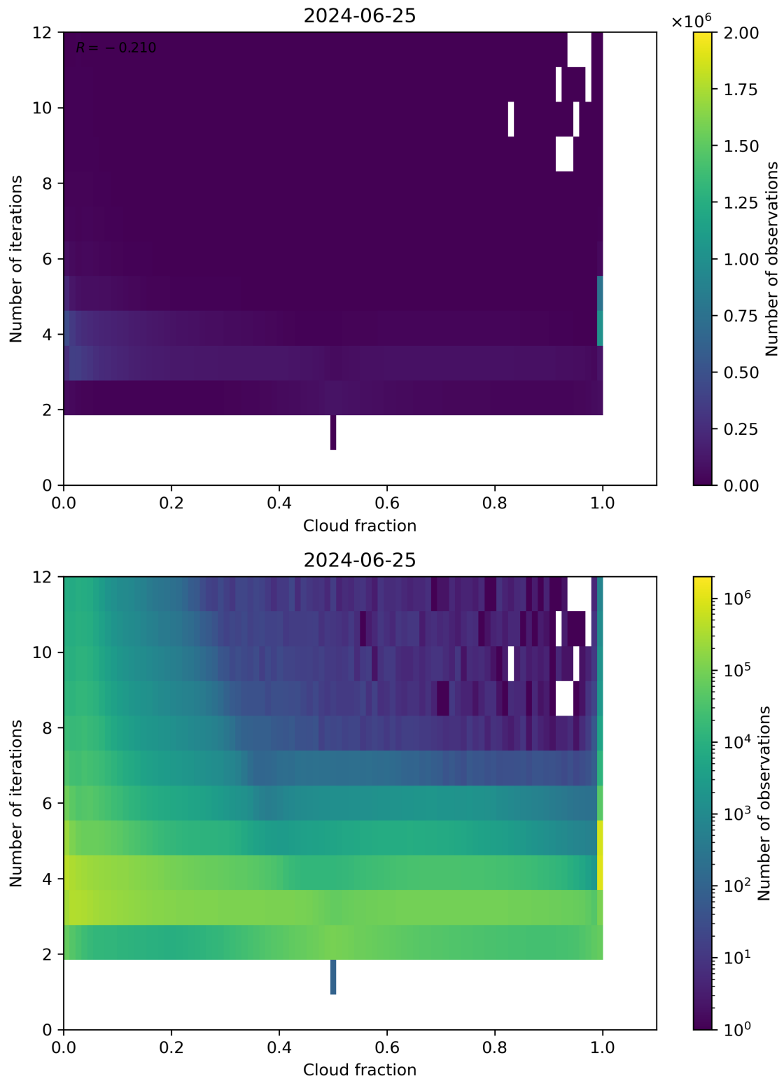
Figure 73: Scatter density plot of “Cloud fraction” against “Number of iterations” for 2024-06-24 to 2024-06-26.
