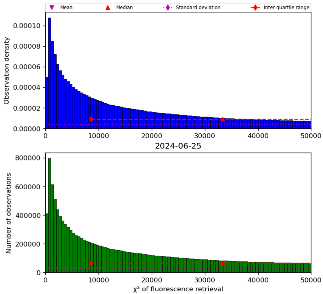
Figure 42: Histogram of “ \chi^2 of fluorescence retrieval” for 2024-06-24 to 2024-06-26
