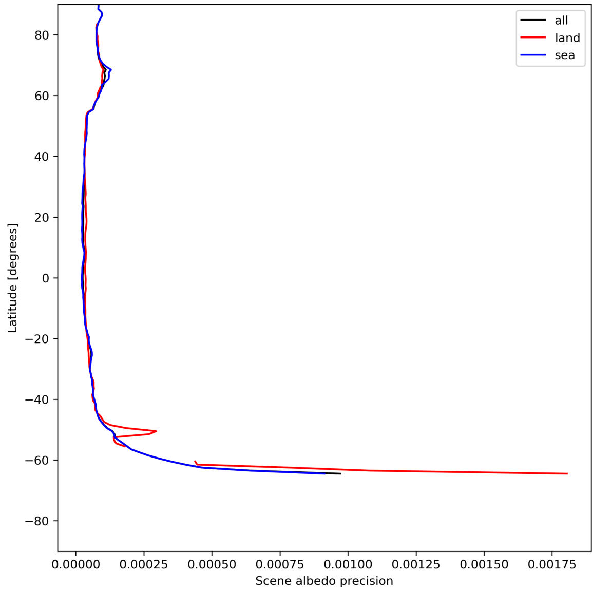
Figure 18: Zonal average of “Scene albedo precision” for 2024-06-24 to 2024-06-26.
