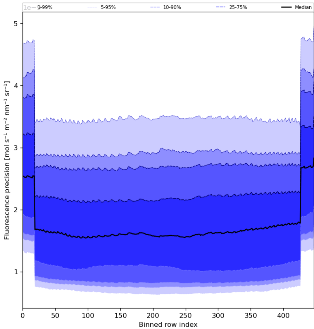
Figure 58: Along track statistics of “Fluorescence precision” for 2024-06-24 to 2024-06-26
