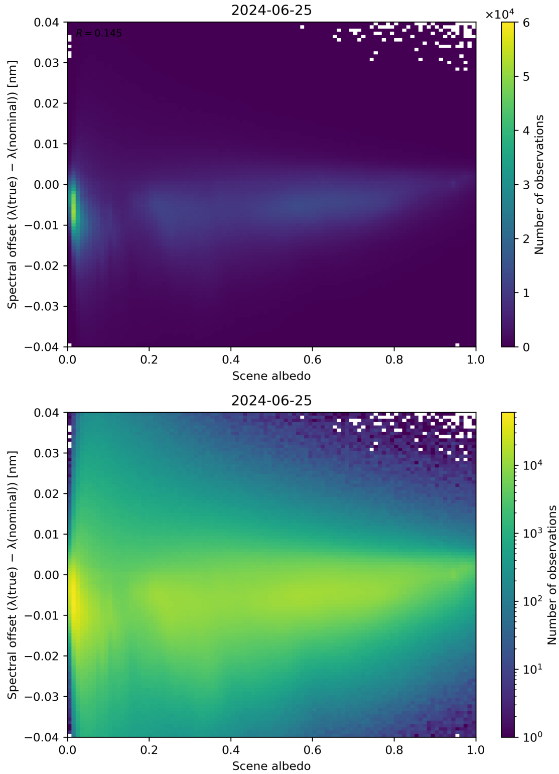
Figure 107: Scatter density plot of “Scene albedo” against “Spectral offset ( \lambda(\text{true}) - \lambda(\text{nominal}) )” for 2024-06-24 to 2024-06-26.
