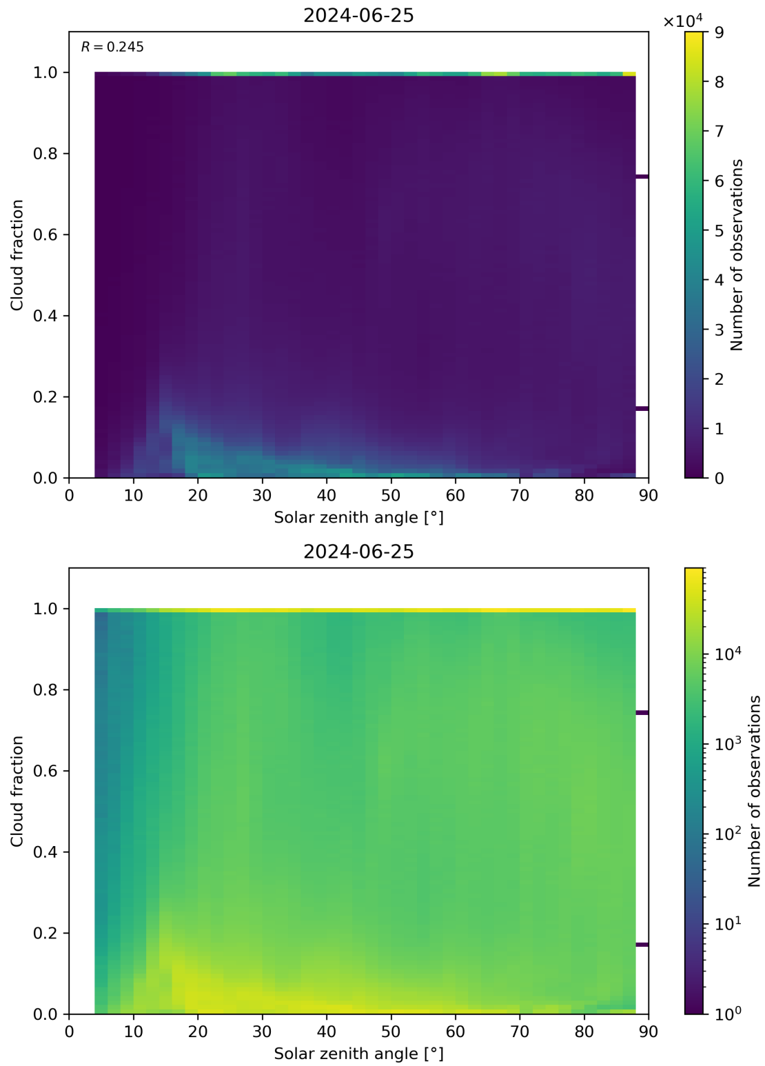
Figure 110: Scatter density plot of “Solar zenith angle” against “Cloud fraction” for 2024-06-24 to 2024-06-26.
