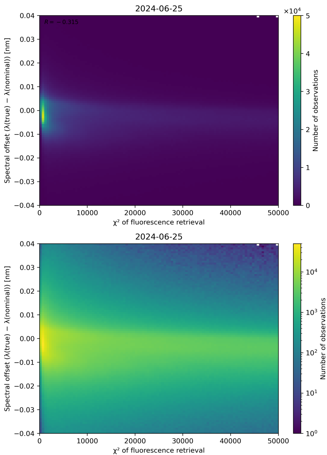
Figure 69: Scatter density plot of “ \chi^2 of fluorescence retrieval” against “Spectral offset ( \lambda(\text{true}) - \lambda(\text{nominal}) )” for 2024-06-24 to 2024-06-26.
