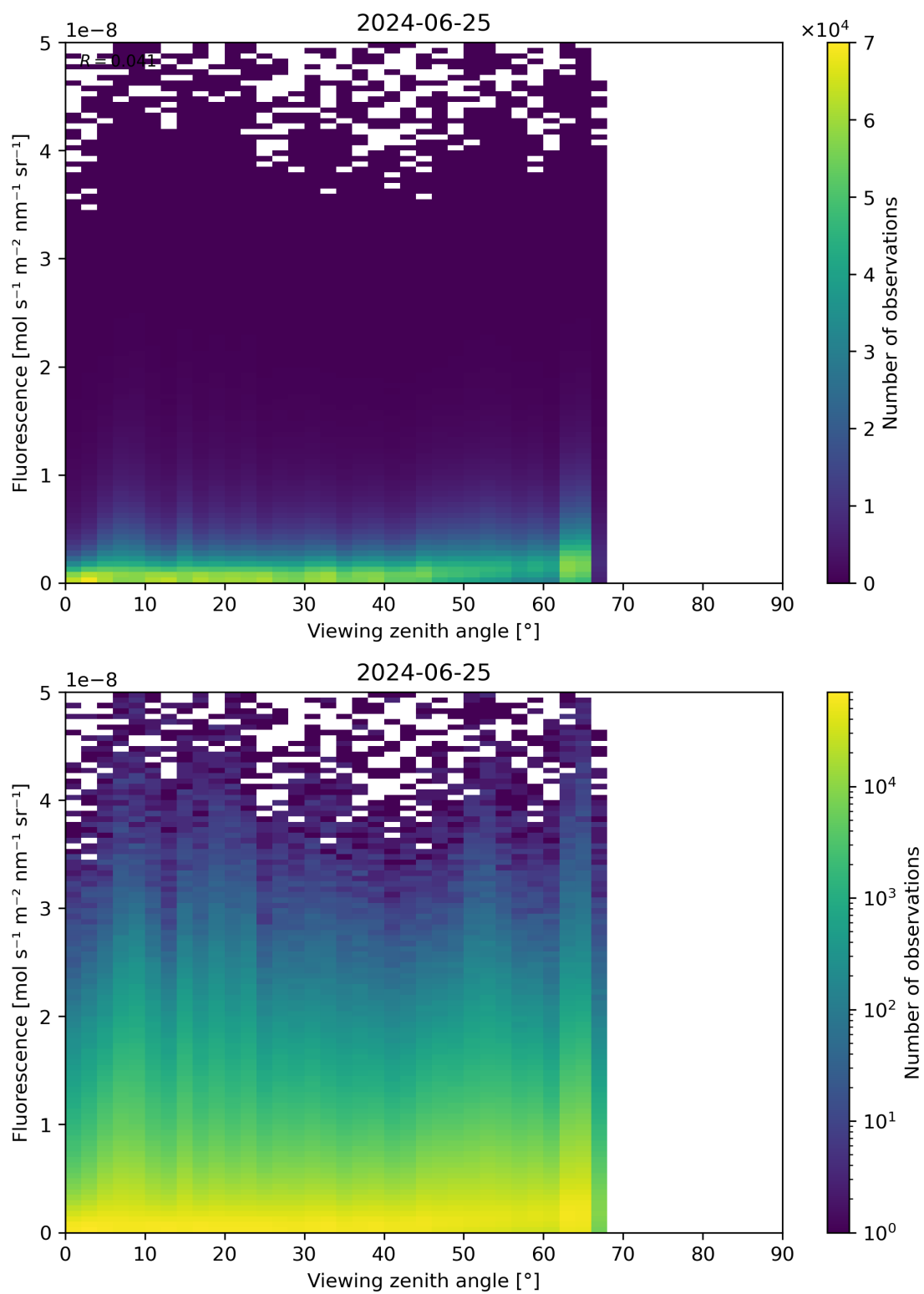
Figure 122: Scatter density plot of “Viewing zenith angle” against “Fluorescence” for 2024-06-24 to 2024-06-26.
