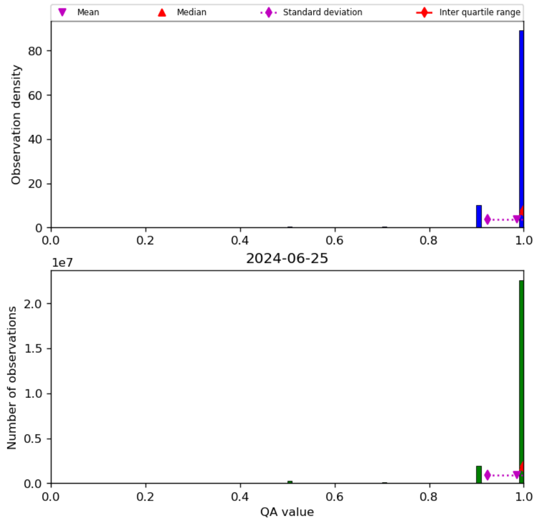
Figure 29: Histogram of “QA value” for 2024-06-24 to 2024-06-26
