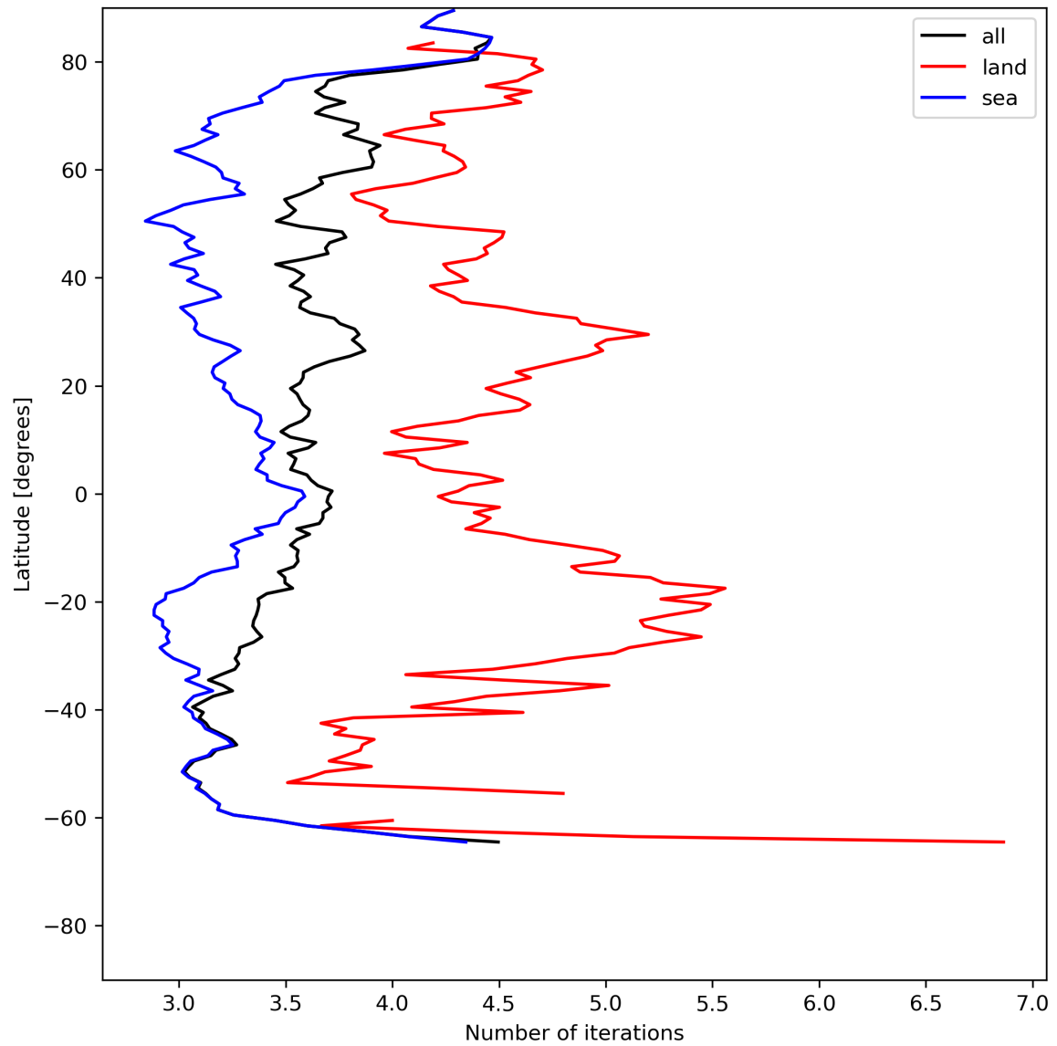
Figure 22: Zonal average of “Number of iterations” for 2024-06-24 to 2024-06-26.
