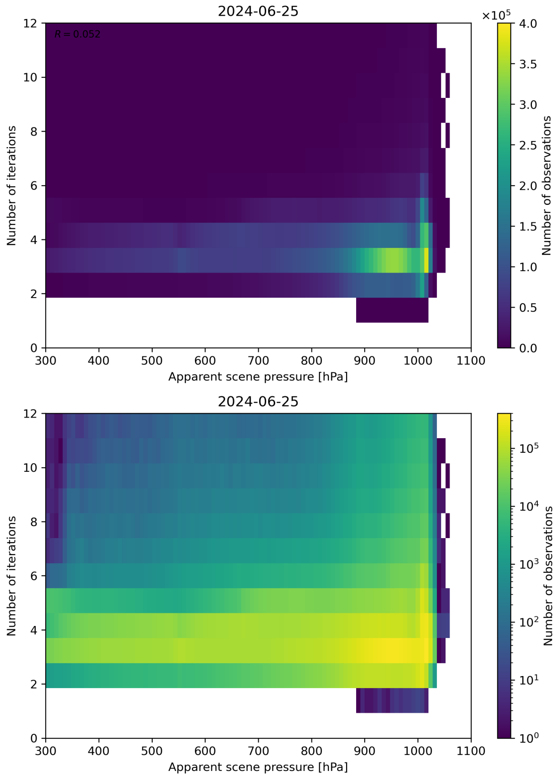
Figure 65: Scatter density plot of “Apparent scene pressure” against “Number of iterations” for 2024-06-24 to 2024-06-26.
