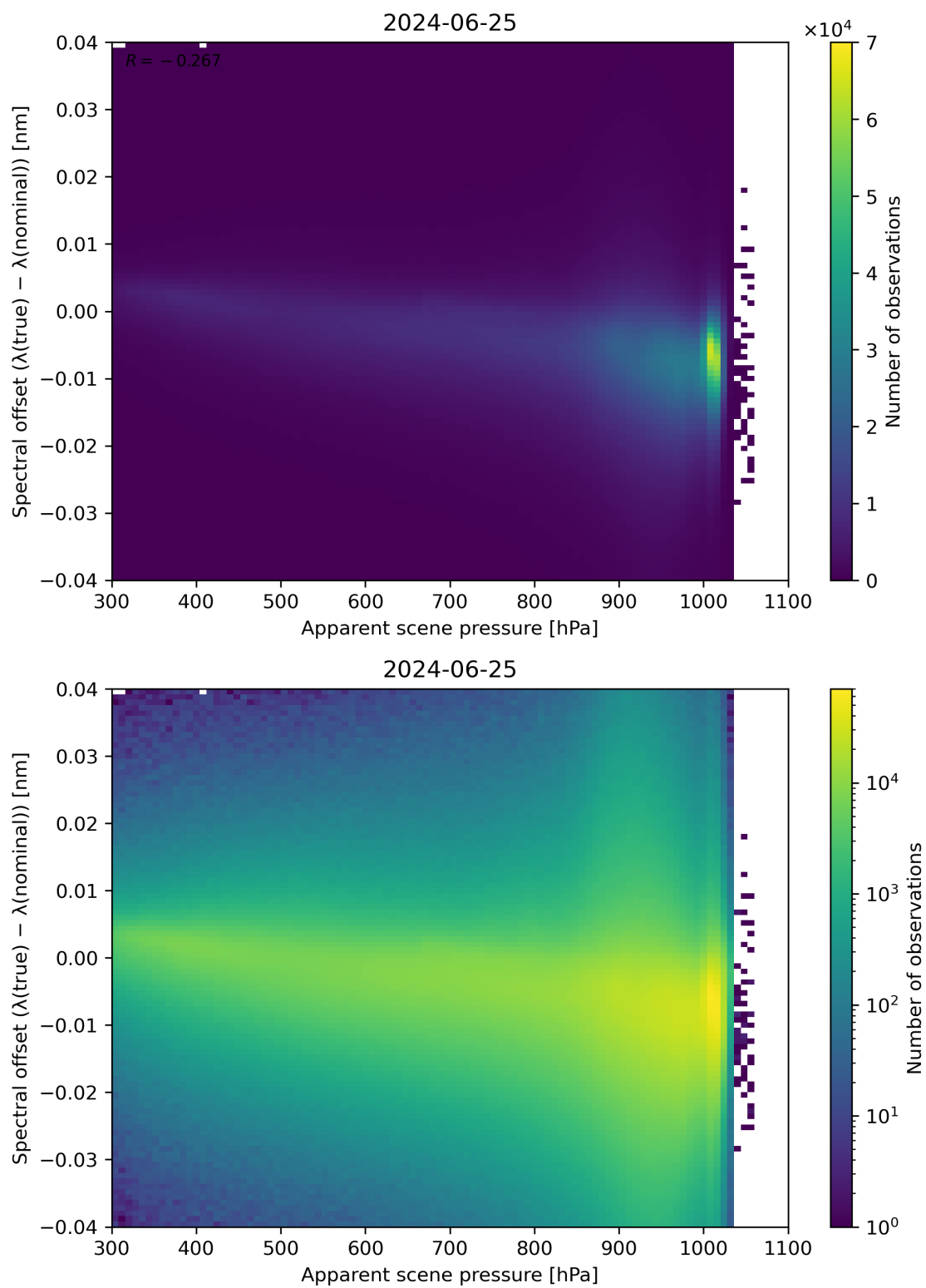
Figure 67: Scatter density plot of “Apparent scene pressure” against “Spectral offset ( \lambda(\text{true}) - \lambda(\text{nominal}) )” for 2024-06-24 to 2024-06-26.
