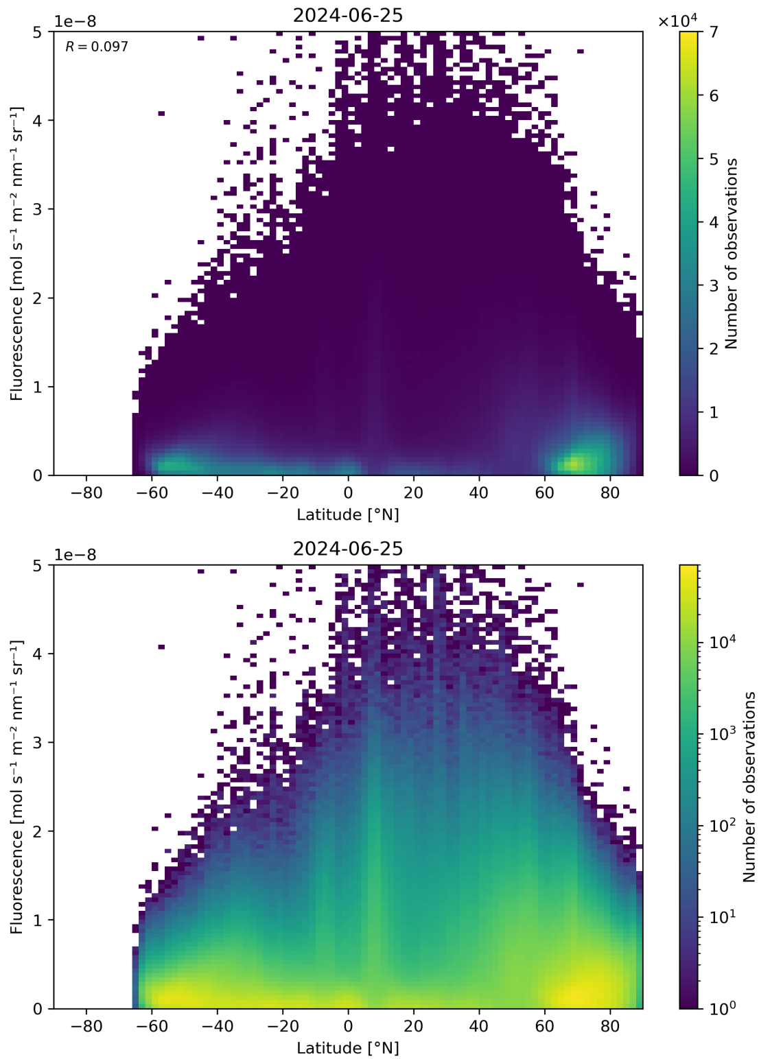
Figure 92: Scatter density plot of “Latitude” against “Fluorescence” for 2024-06-24 to 2024-06-26.
