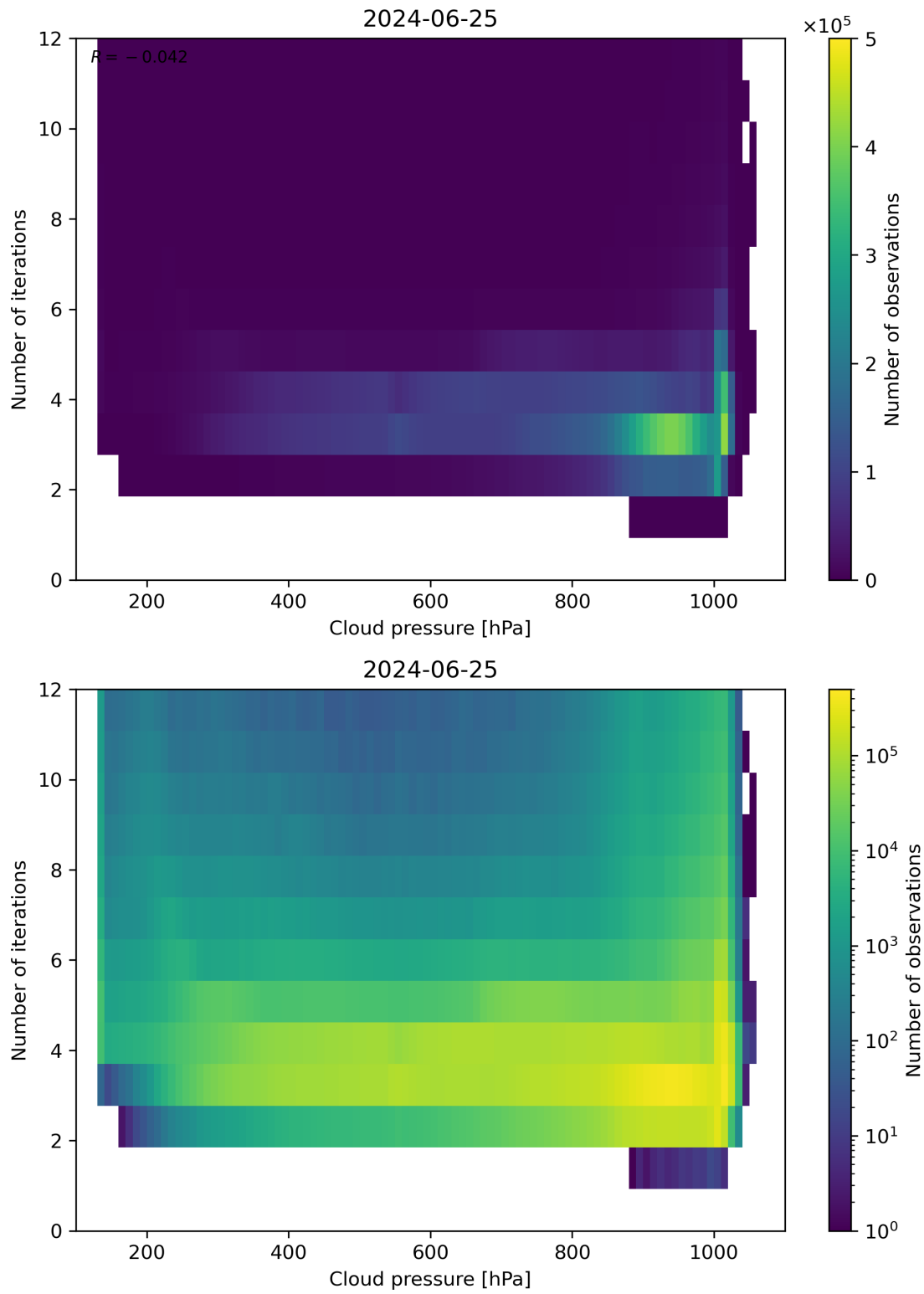
Figure 81: Scatter density plot of “Cloud pressure” against “Number of iterations” for 2024-06-24 to 2024-06-26.
