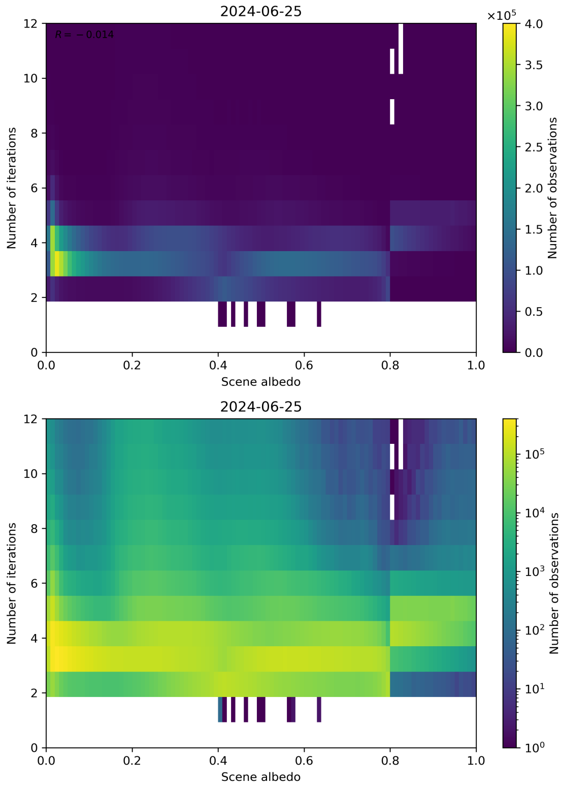
Figure 105: Scatter density plot of “Scene albedo” against “Number of iterations” for 2024-06-24 to 2024-06-26.
