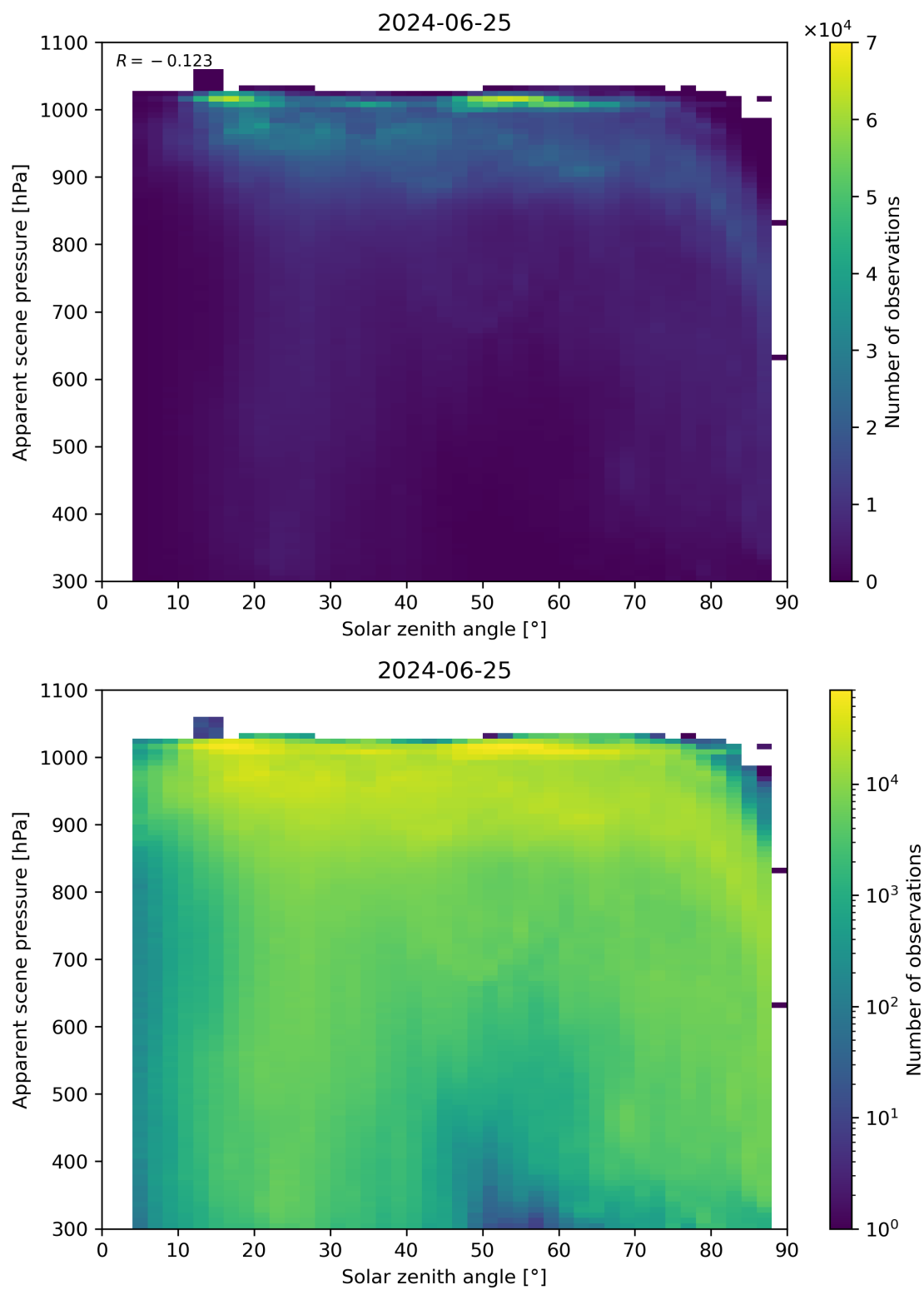
Figure 108: Scatter density plot of “Solar zenith angle” against “Apparent scene pressure” for 2024-06-24 to 2024-06-26.
