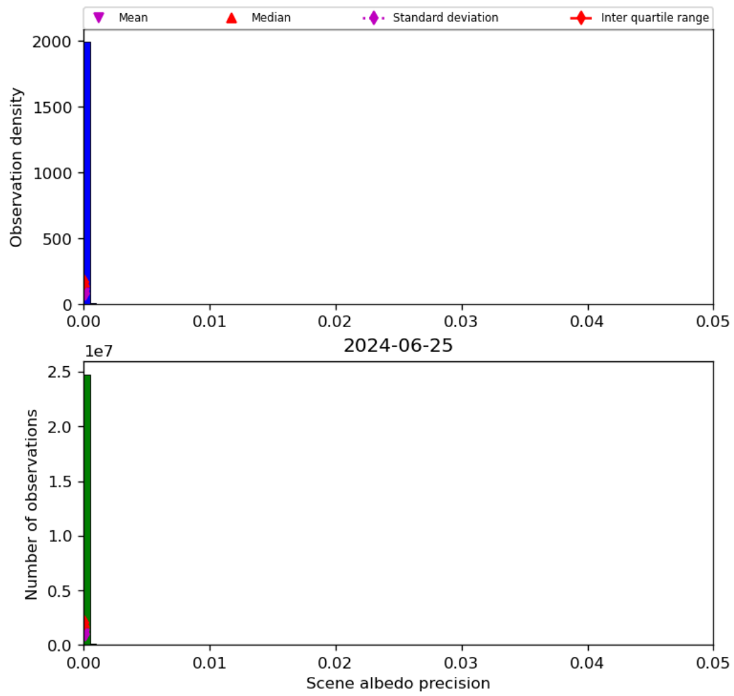
Figure 35: Histogram of “Scene albedo precision” for 2024-06-24 to 2024-06-26
