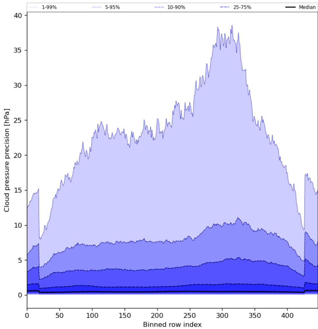
Figure 48: Along track statistics of “Cloud pressure precision” for 2024-06-24 to 2024-06-26
