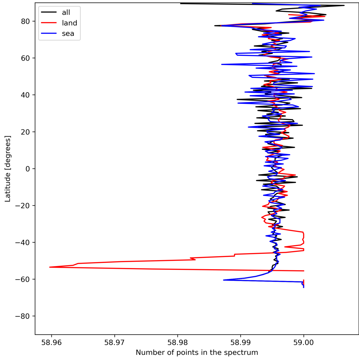
Figure 27: Zonal average of “Number of points in the spectrum” for 2024-06-24 to 2024-06-26.
