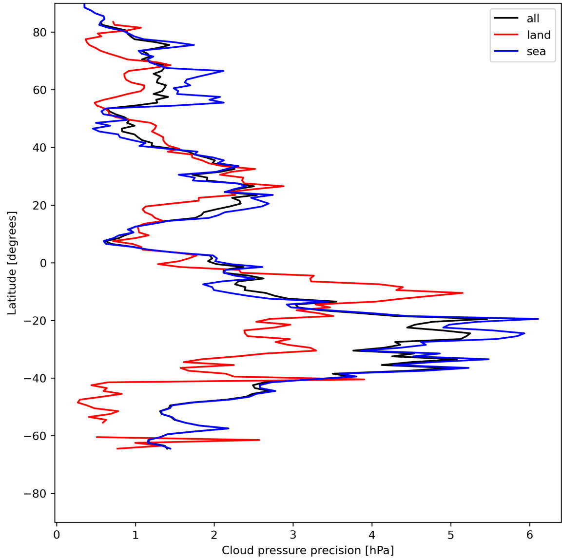
Figure 14: Zonal average of “Cloud pressure precision” for 2024-06-24 to 2024-06-26.
