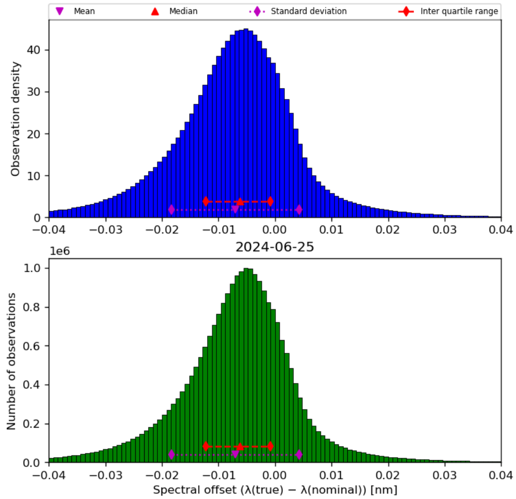
Figure 45: Histogram of “Spectral offset ( \lambda(\text{true}) - \lambda(\text{nominal}) )” for 2024-06-24 to 2024-06-26
