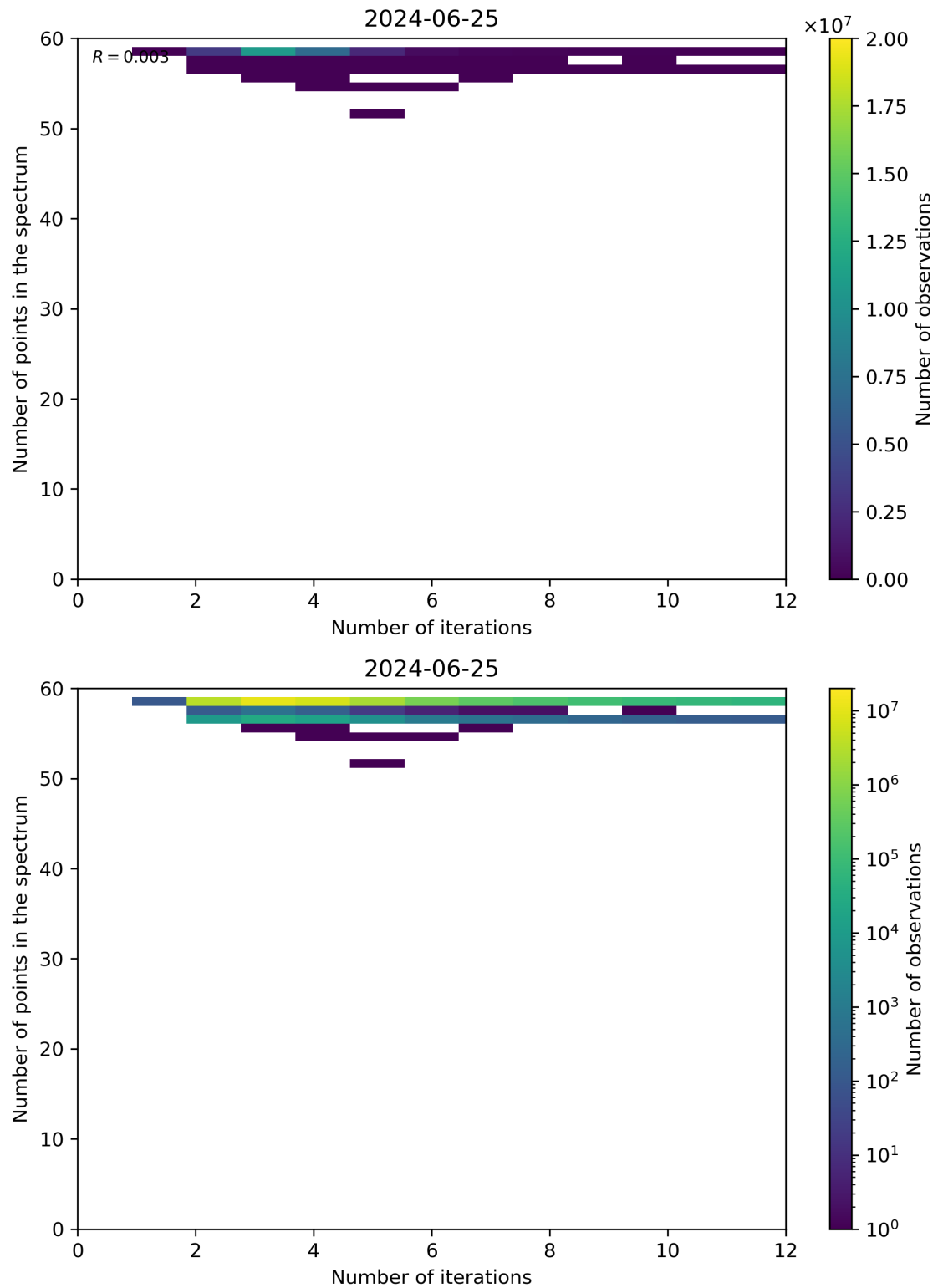
Figure 99: Scatter density plot of “Number of iterations” against “Number of points in the spectrum” for 2024-06-24 to 2024-06-26.
