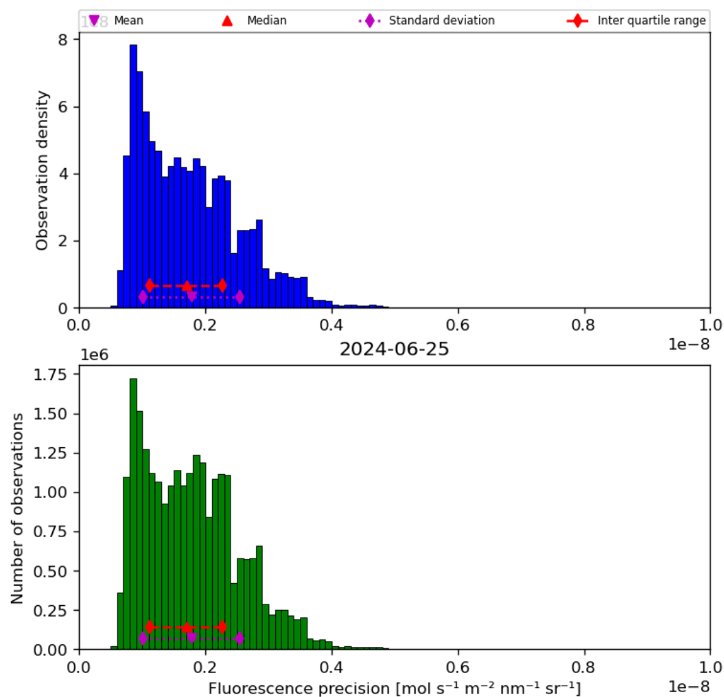
Figure 41: Histogram of “Fluorescence precision” for 2024-06-24 to 2024-06-26
