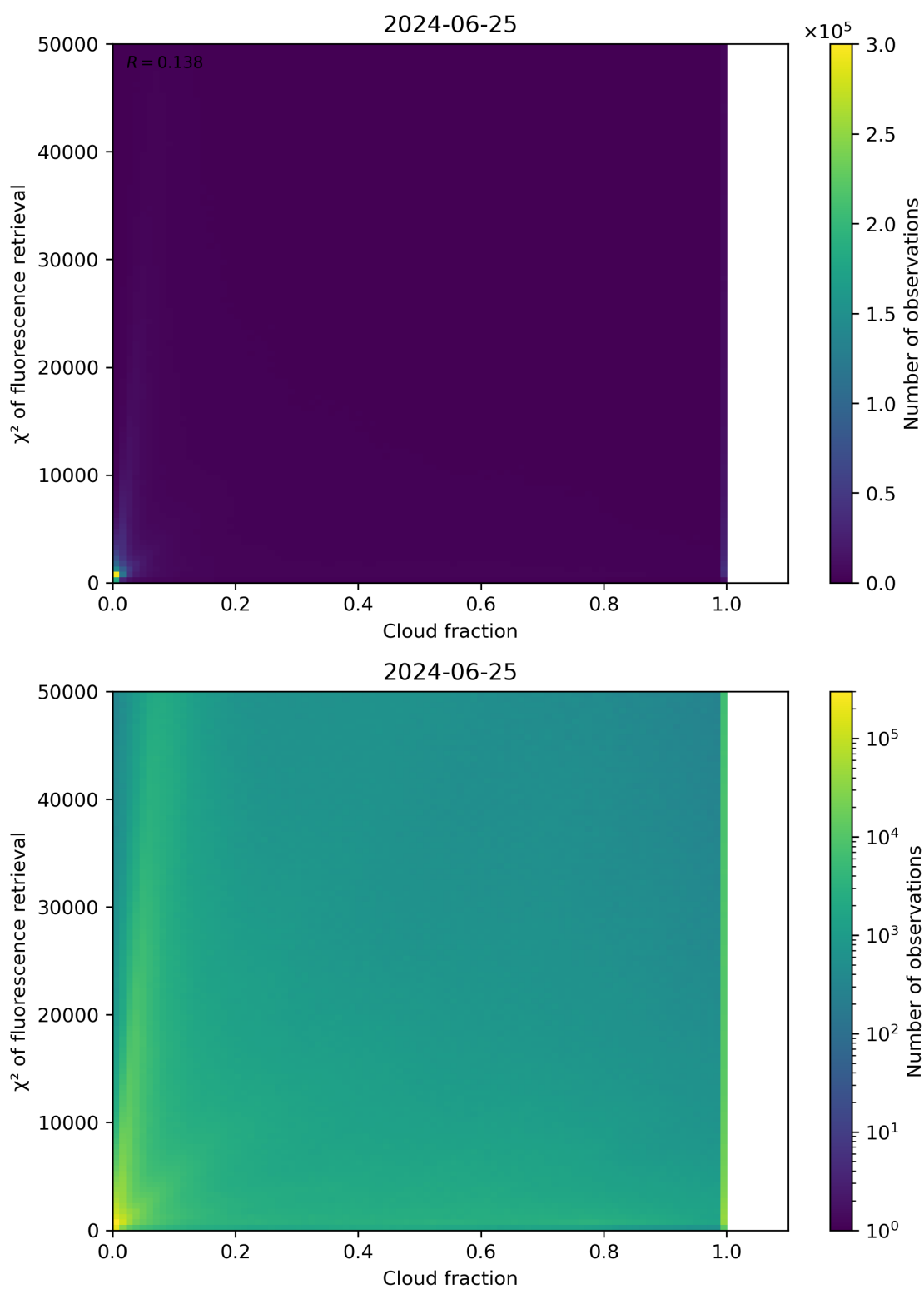
Figure 71: Scatter density plot of “Cloud fraction” against “ \chi^2 of fluorescence retrieval” for 2024-06-24 to 2024-06-26.
