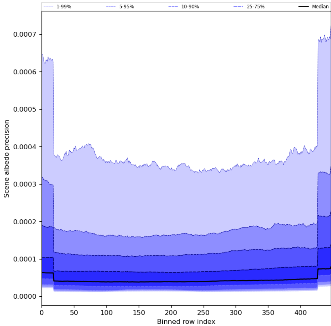
Figure 52: Along track statistics of “Scene albedo precision” for 2024-06-24 to 2024-06-26
