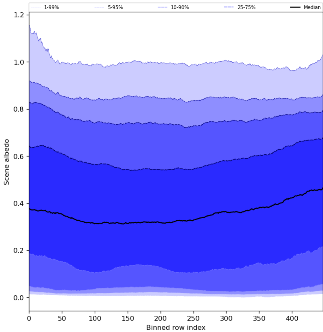
Figure 51: Along track statistics of “Scene albedo” for 2024-06-24 to 2024-06-26
