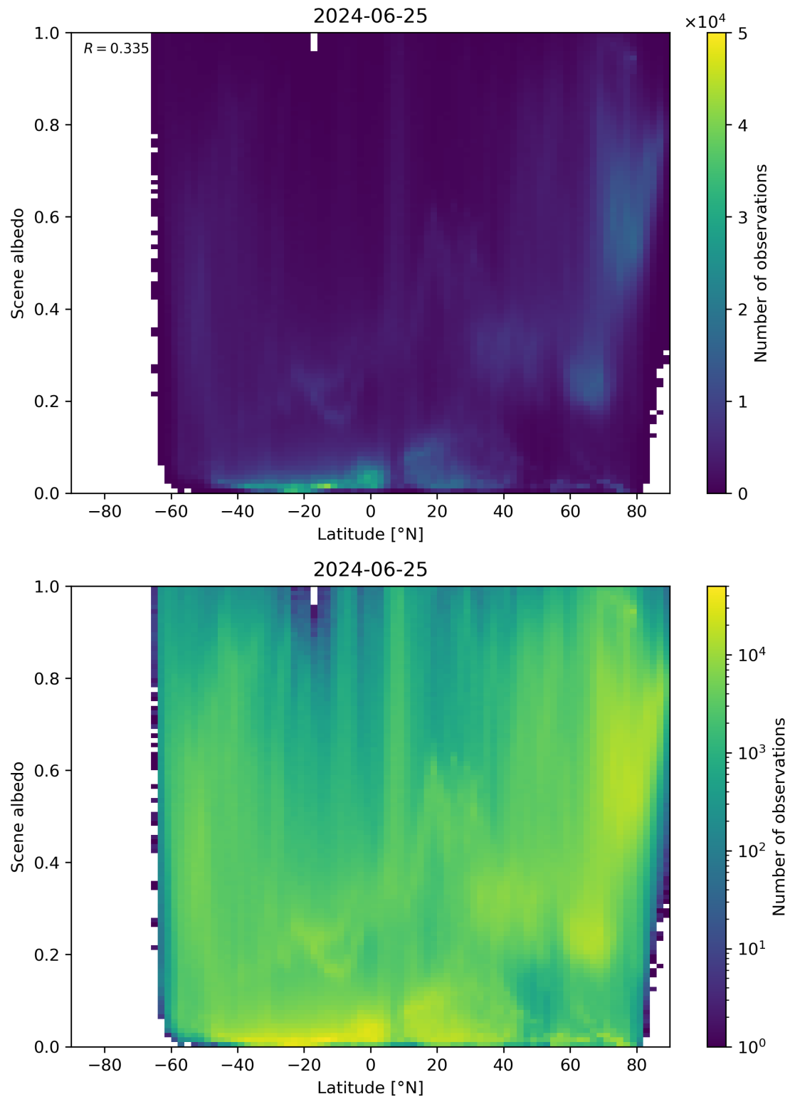
Figure 95: Scatter density plot of “Latitude” against “Scene albedo” for 2024-06-24 to 2024-06-26.
