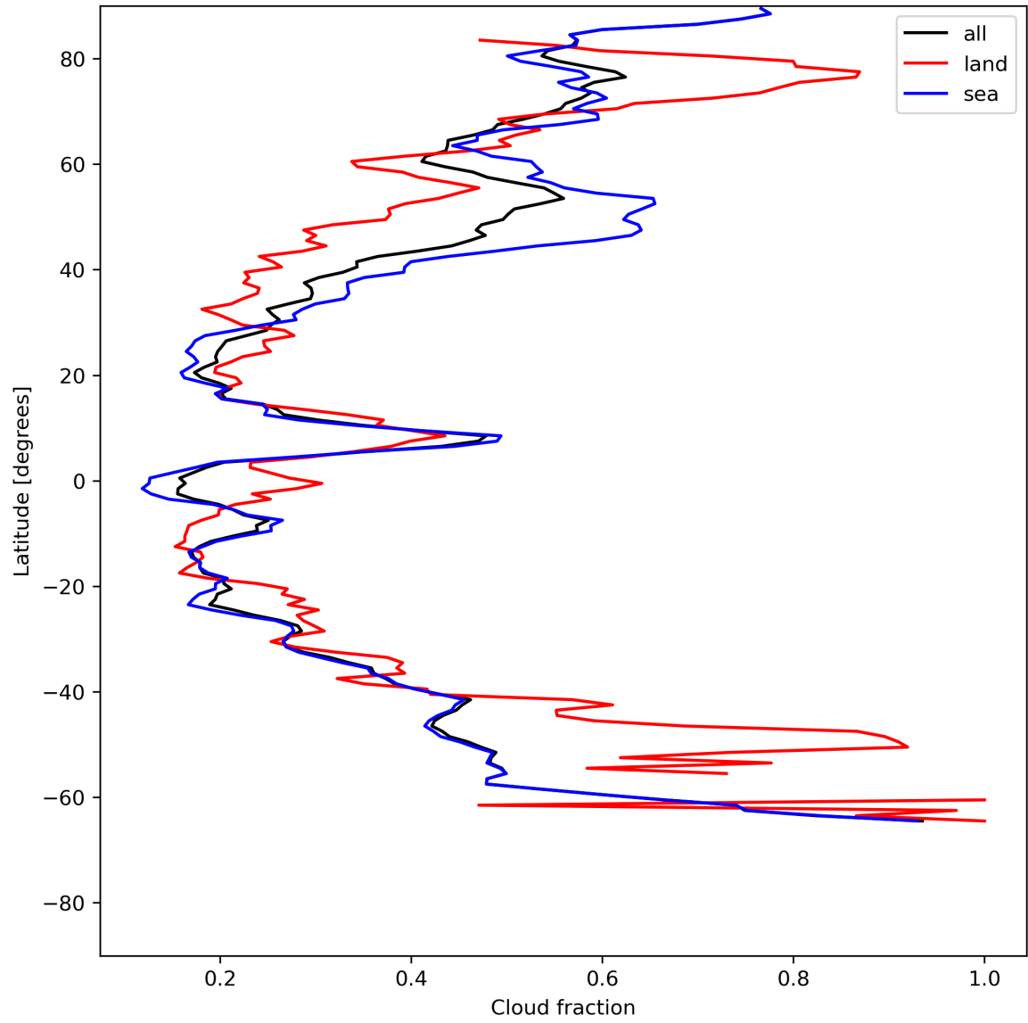
Figure 15: Zonal average of “Cloud fraction” for 2024-06-24 to 2024-06-26.
