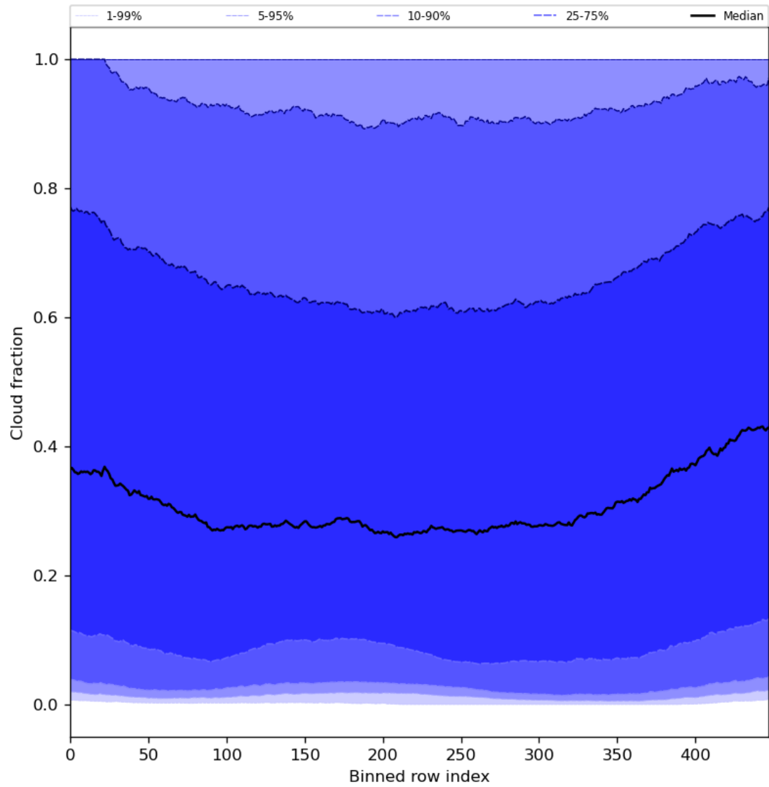
Figure 49: Along track statistics of “Cloud fraction” for 2024-06-25 to 2024-06-27
