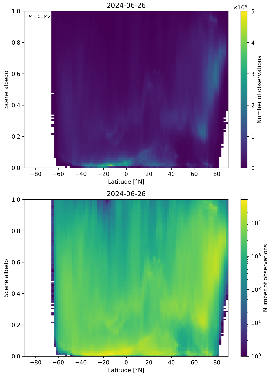
Figure 95: Scatter density plot of “Latitude” against “Scene albedo” for 2024-06-25 to 2024-06-27.
