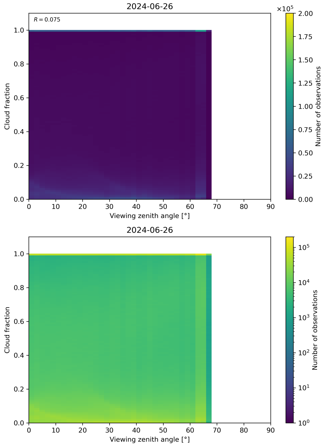
Figure 120: Scatter density plot of “Viewing zenith angle” against “Cloud fraction” for 2024-06-25 to 2024-06-27.
