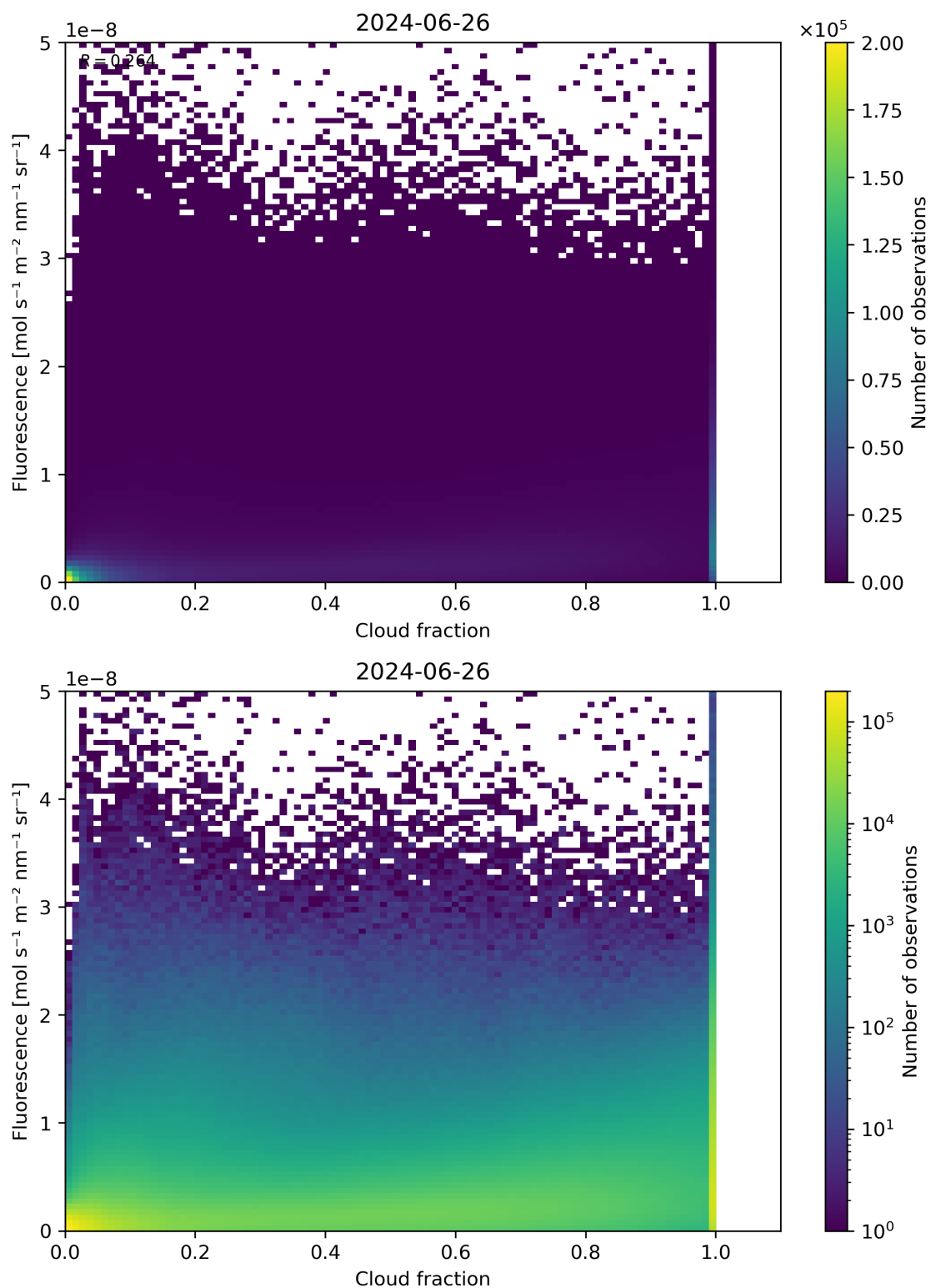
Figure 72: Scatter density plot of “Cloud fraction” against “Fluorescence” for 2024-06-25 to 2024-06-27.
