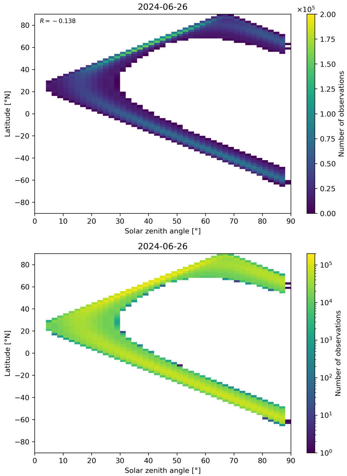
Figure 113: Scatter density plot of “Solar zenith angle” against “Latitude” for 2024-06-25 to 2024-06-27.
