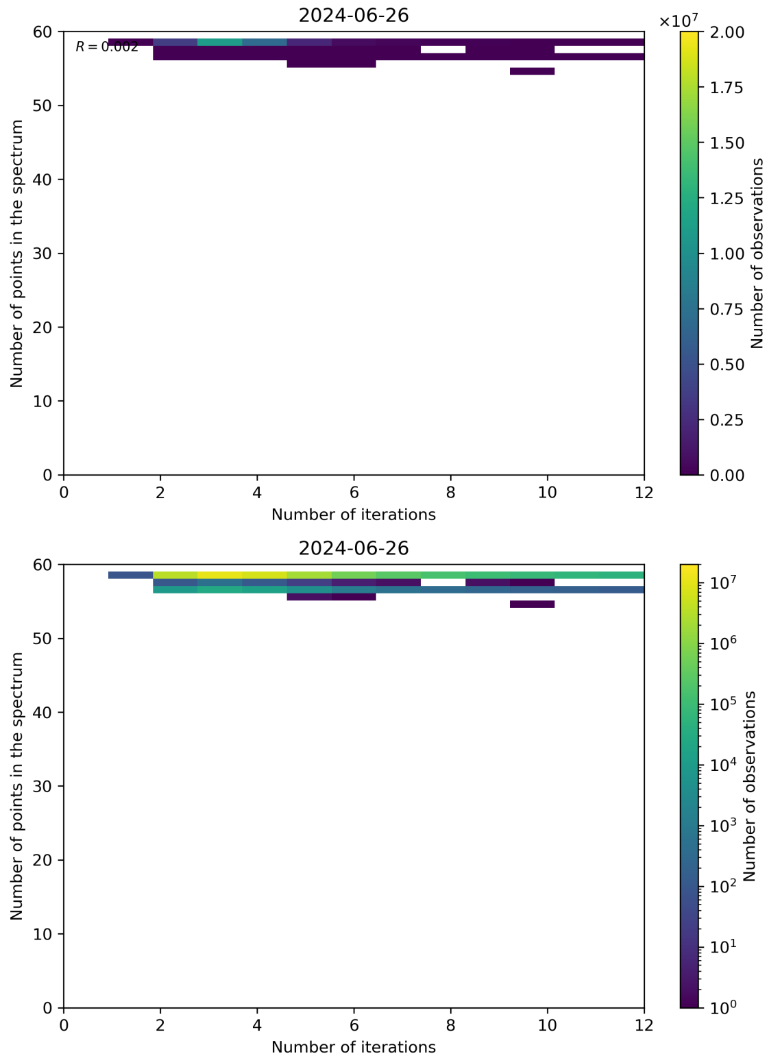
Figure 99: Scatter density plot of “Number of iterations” against “Number of points in the spectrum” for 2024-06-25 to 2024-06-27.
