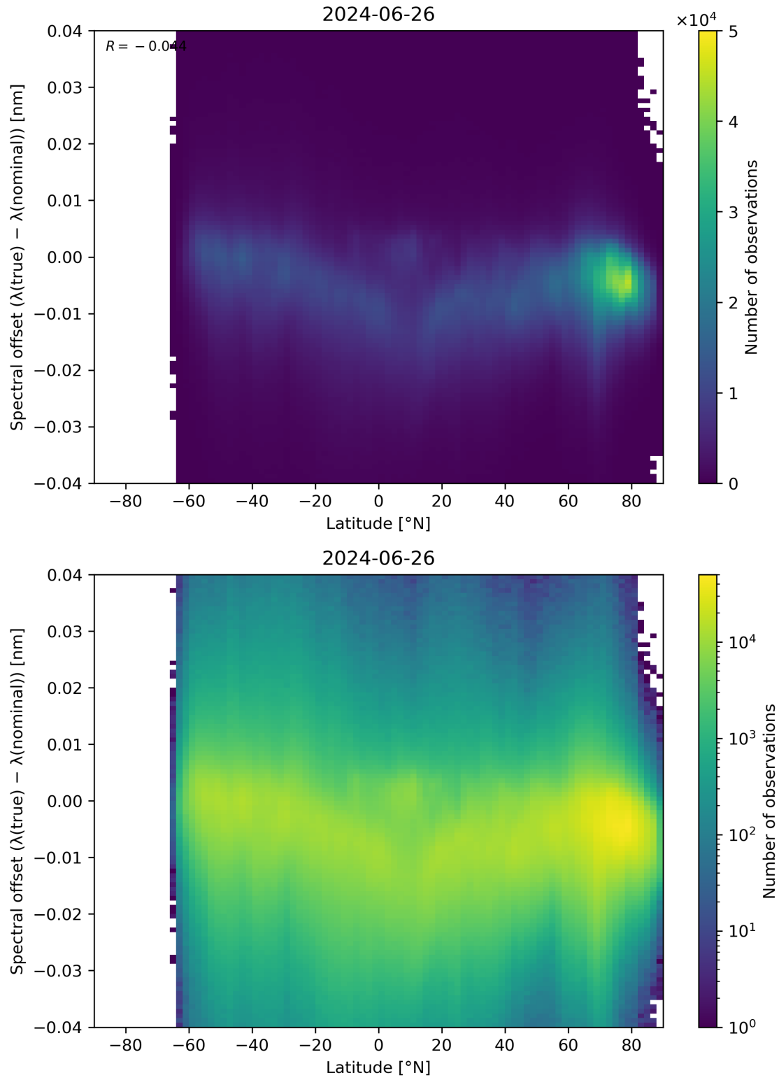
Figure 96: Scatter density plot of “Latitude” against “Spectral offset ( \lambda(\text{true}) - \lambda(\text{nominal}) )” for 2024-06-25 to 2024-06-27.
