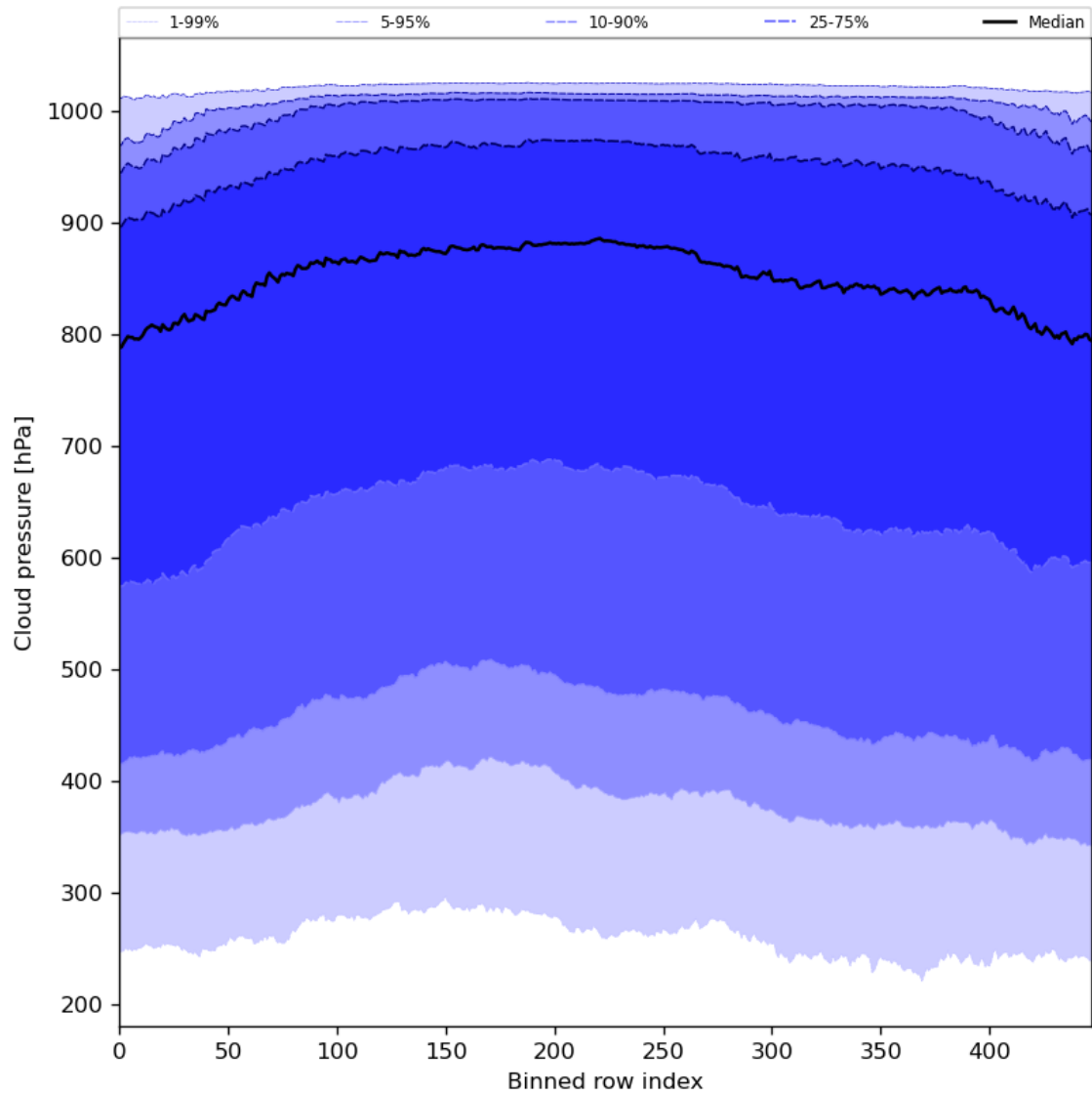
Figure 47: Along track statistics of “Cloud pressure” for 2024-06-25 to 2024-06-27
