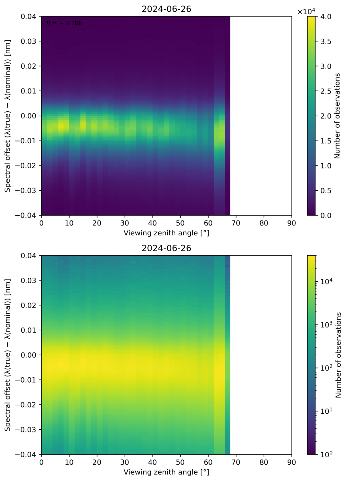
Figure 128: Scatter density plot of “Viewing zenith angle” against “Spectral offset ( \lambda(\text{true}) - \lambda(\text{nominal}) )” for 2024-06-25 to 2024-06-27.
