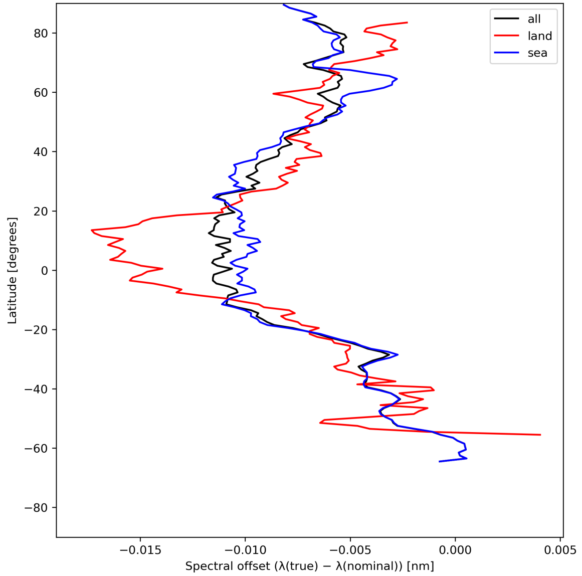
Figure 28: Zonal average of “Spectral offset ( \lambda(\text{true}) - \lambda(\text{nominal}) )” for 2024-06-25 to 2024-06-27.
