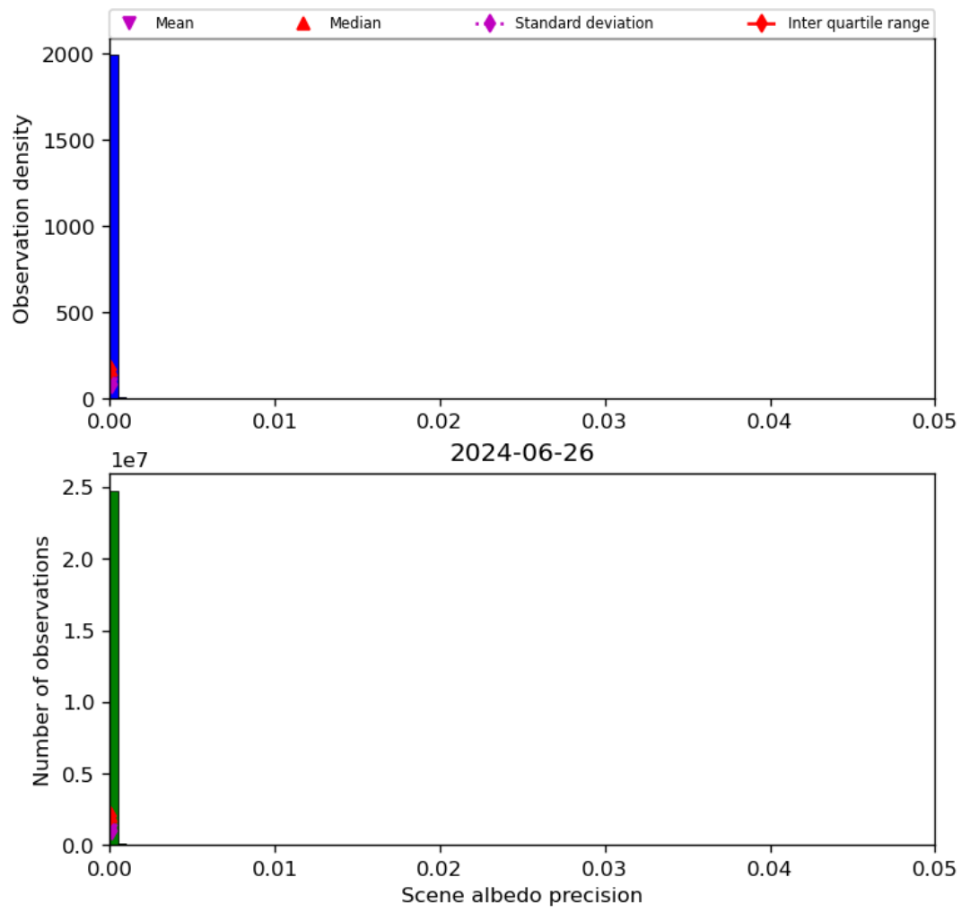
Figure 35: Histogram of “Scene albedo precision” for 2024-06-25 to 2024-06-27
