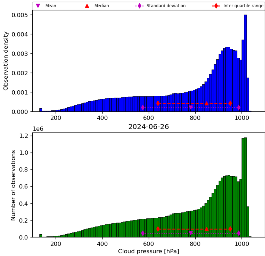
Figure 30: Histogram of “Cloud pressure” for 2024-06-25 to 2024-06-27
