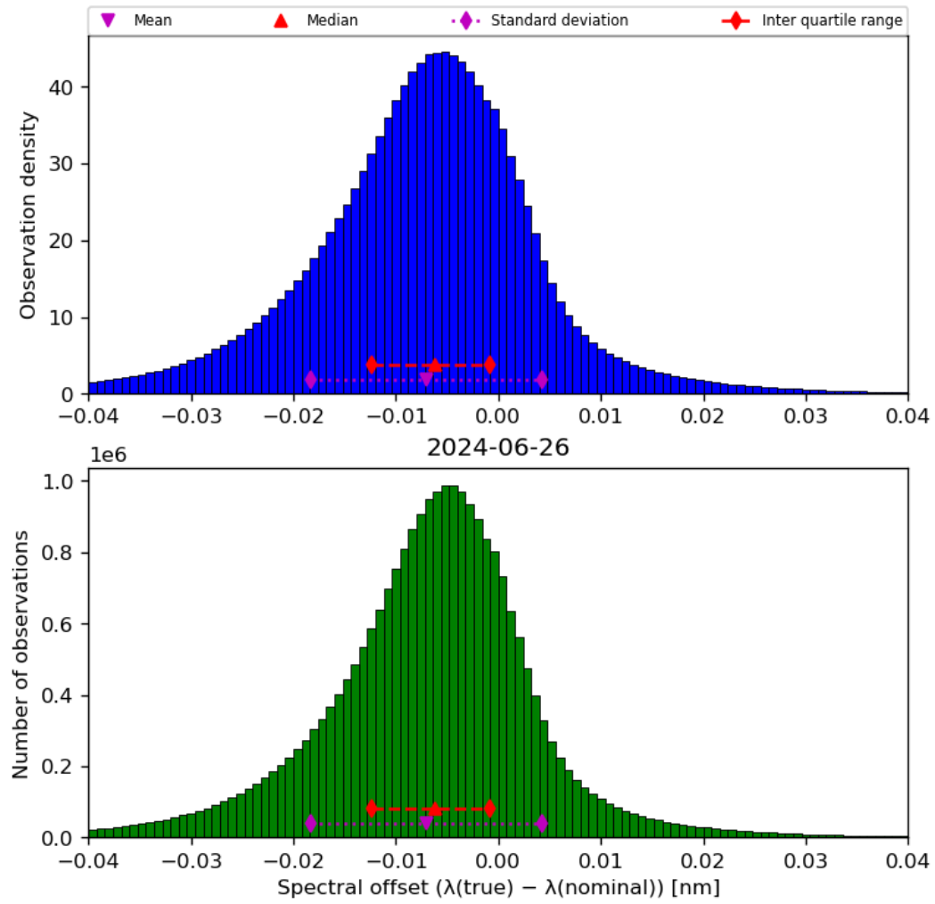
Figure 45: Histogram of “Spectral offset ( \lambda(\text{true}) - \lambda(\text{nominal}) )” for 2024-06-25 to 2024-06-27
