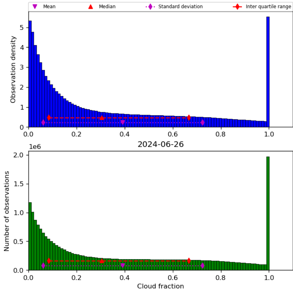
Figure 32: Histogram of “Cloud fraction” for 2024-06-25 to 2024-06-27
