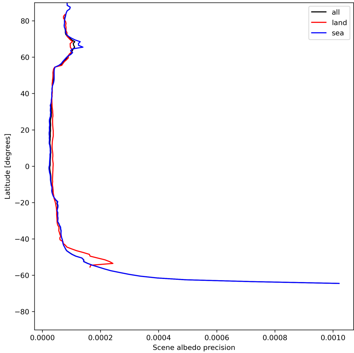
Figure 18: Zonal average of “Scene albedo precision” for 2024-06-25 to 2024-06-27.
