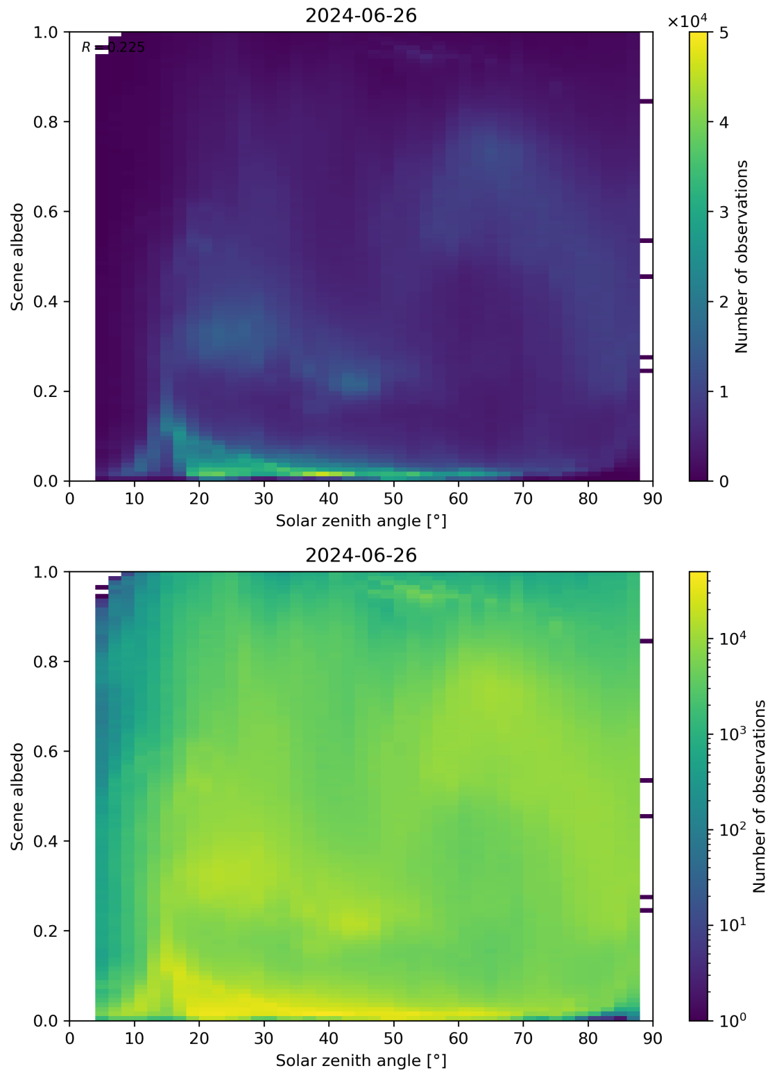
Figure 116: Scatter density plot of “Solar zenith angle” against “Scene albedo” for 2024-06-25 to 2024-06-27.
