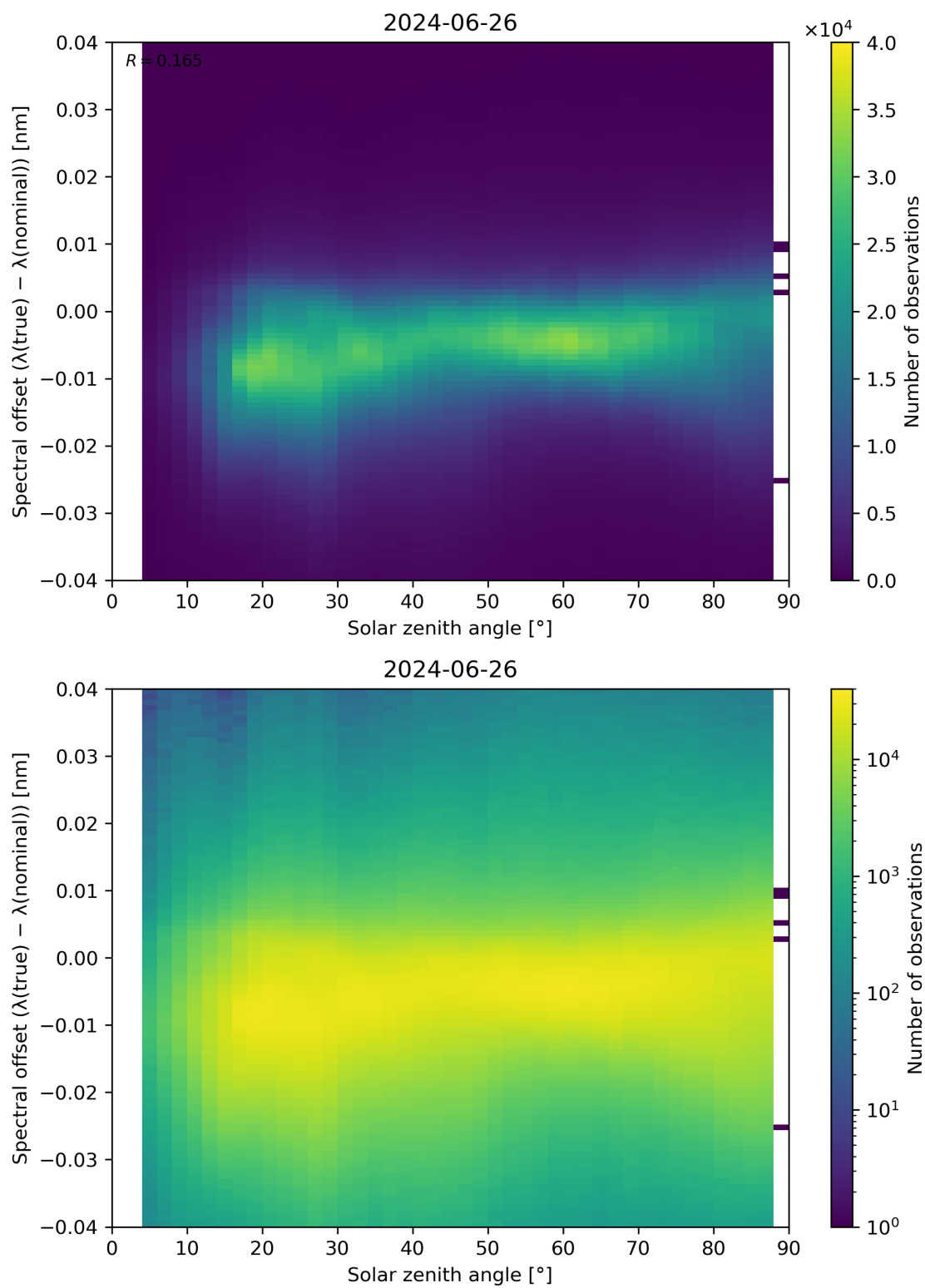
Figure 117: Scatter density plot of “Solar zenith angle” against “Spectral offset ( \lambda(\text{true}) - \lambda(\text{nominal}) )” for 2024-06-25 to 2024-06-27.
