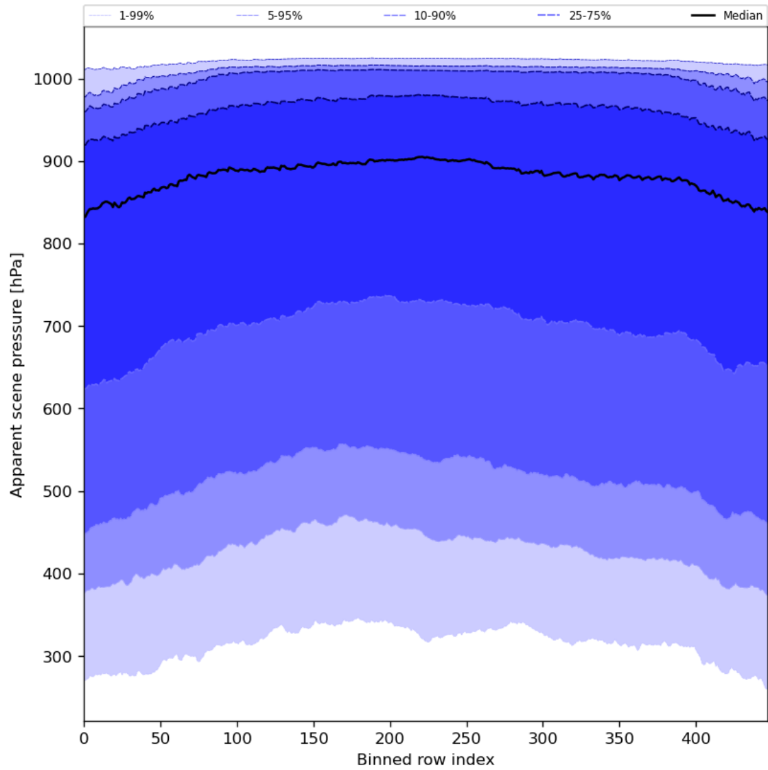
Figure 53: Along track statistics of “Apparent scene pressure” for 2024-06-25 to 2024-06-27
