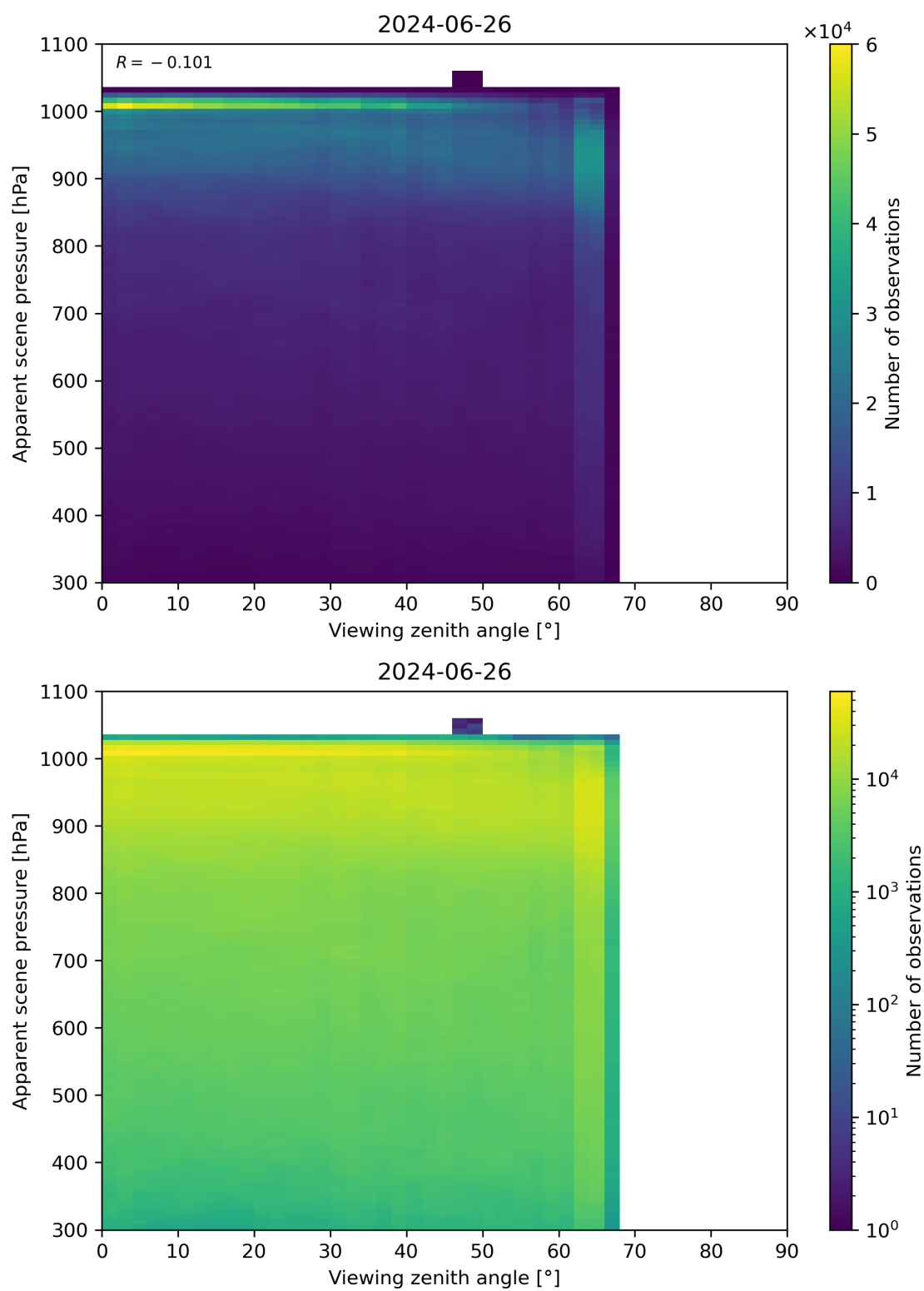
Figure 118: Scatter density plot of “Viewing zenith angle” against “Apparent scene pressure” for 2024-06-25 to 2024-06-27.
