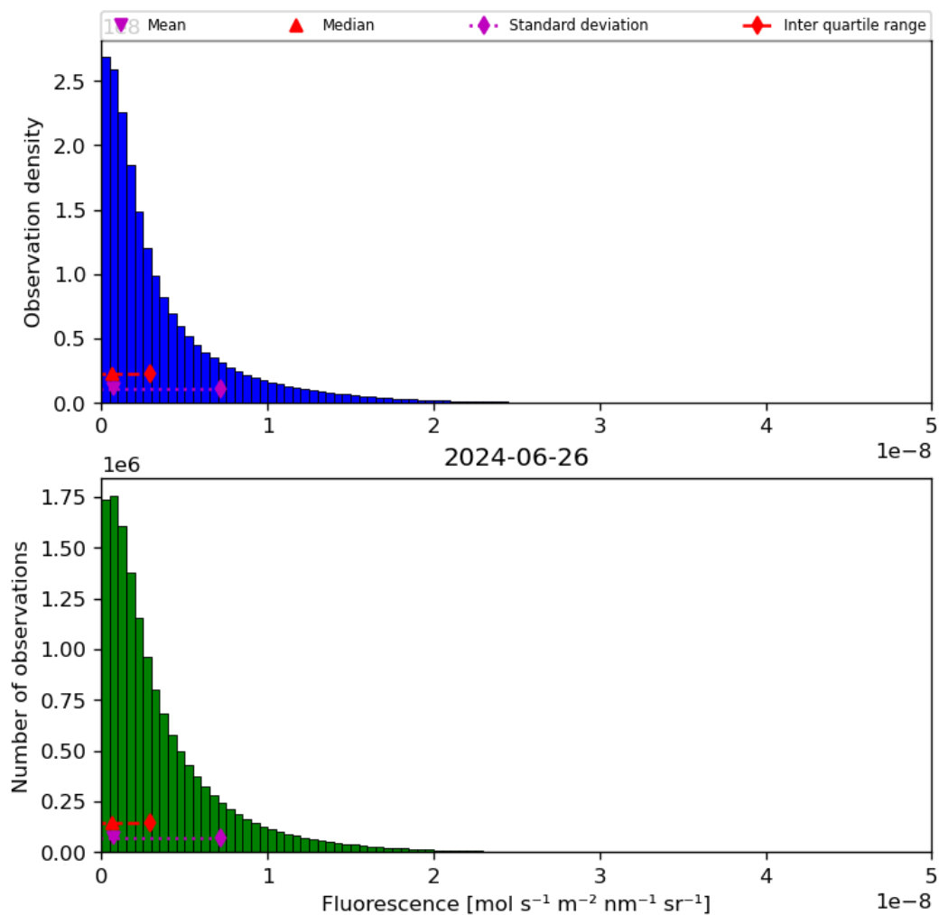
Figure 40: Histogram of “Fluorescence” for 2024-06-25 to 2024-06-27
