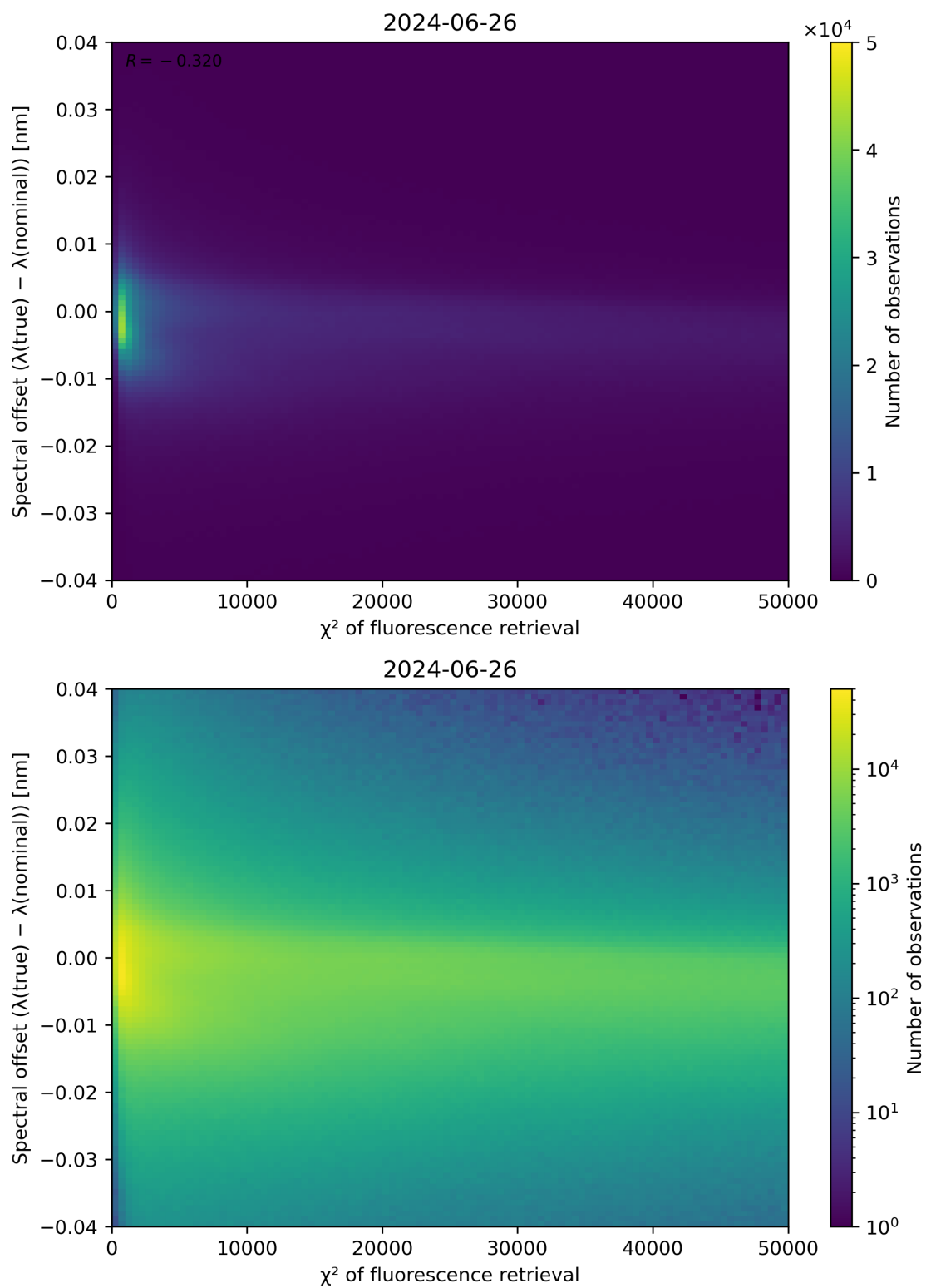
Figure 69: Scatter density plot of " \chi^2 of fluorescence retrieval" against "Spectral offset ( \lambda(\text{true}) - \lambda(\text{nominal}) )" for 2024-06-25 to 2024-06-27.
