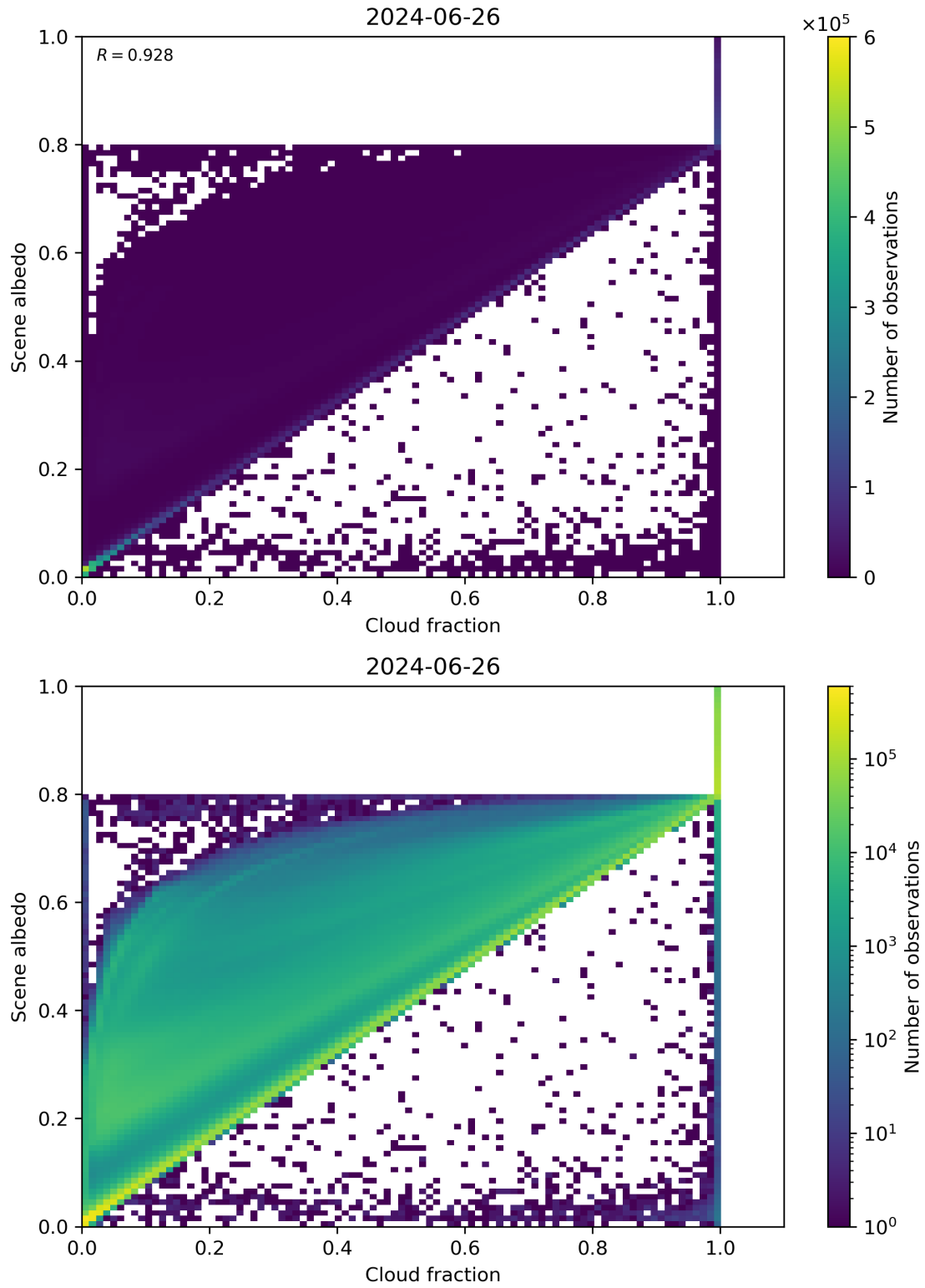
Figure 75: Scatter density plot of “Cloud fraction” against “Scene albedo” for 2024-06-25 to 2024-06-27.
