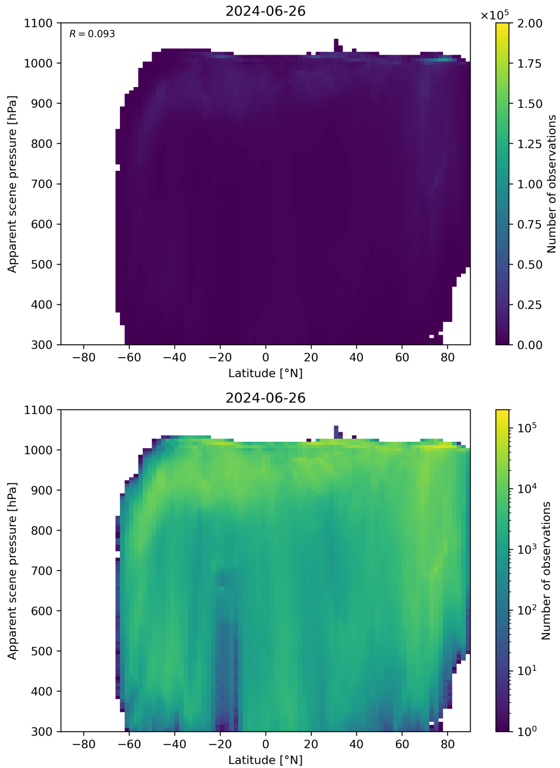
Figure 88: Scatter density plot of “Latitude” against “Apparent scene pressure” for 2024-06-25 to 2024-06-27.
