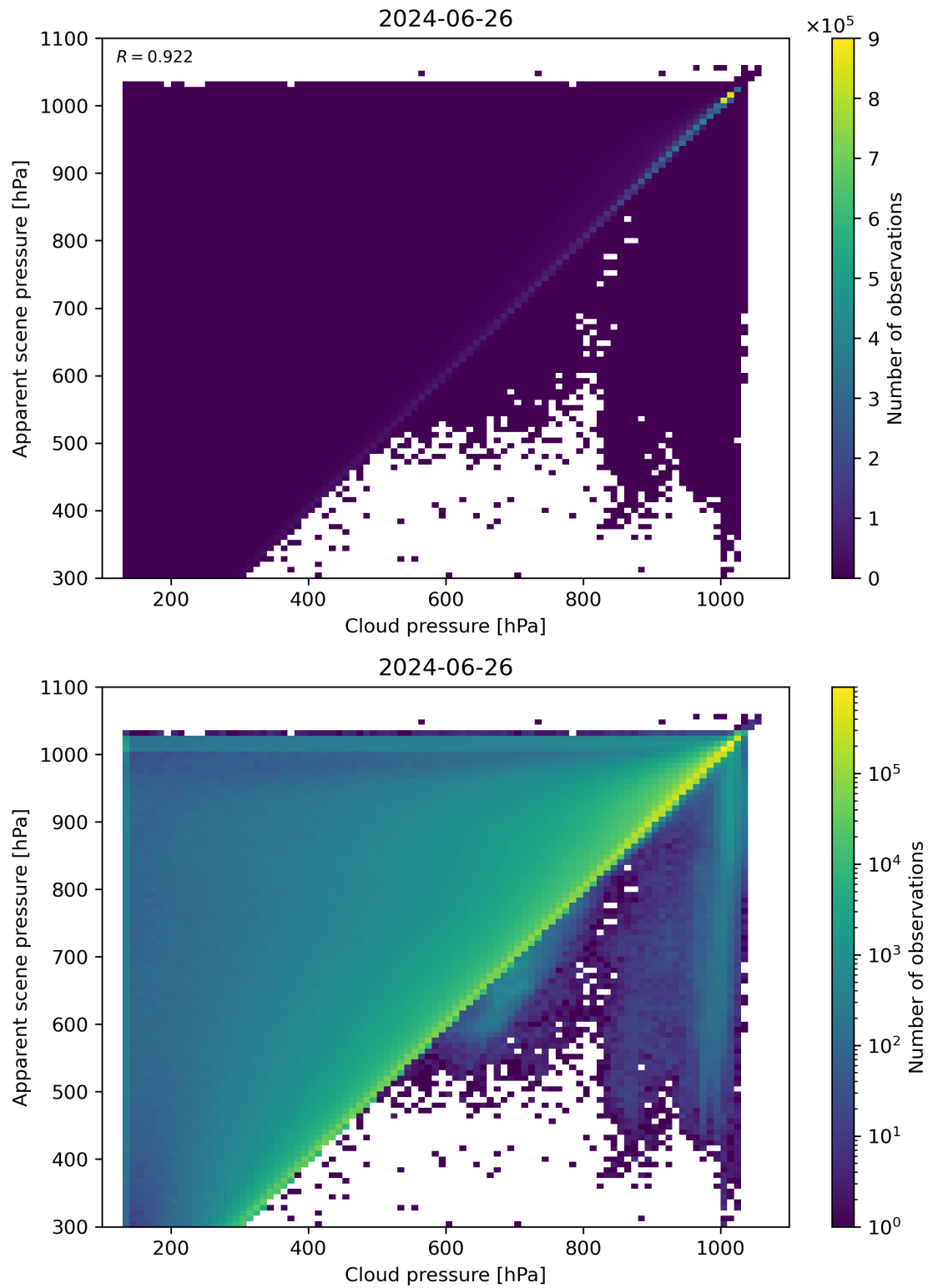
Figure 77: Scatter density plot of “Cloud pressure” against “Apparent scene pressure” for 2024-06-25 to 2024-06-27.
