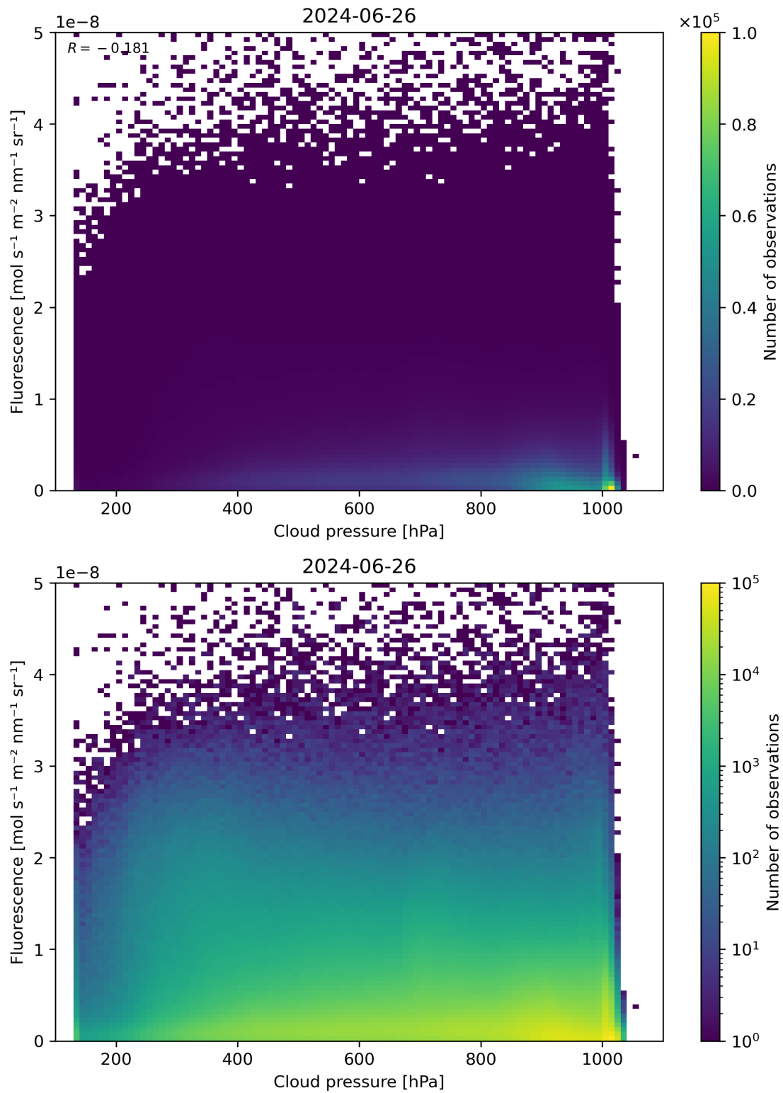
Figure 80: Scatter density plot of “Cloud pressure” against “Fluorescence” for 2024-06-25 to 2024-06-27.
