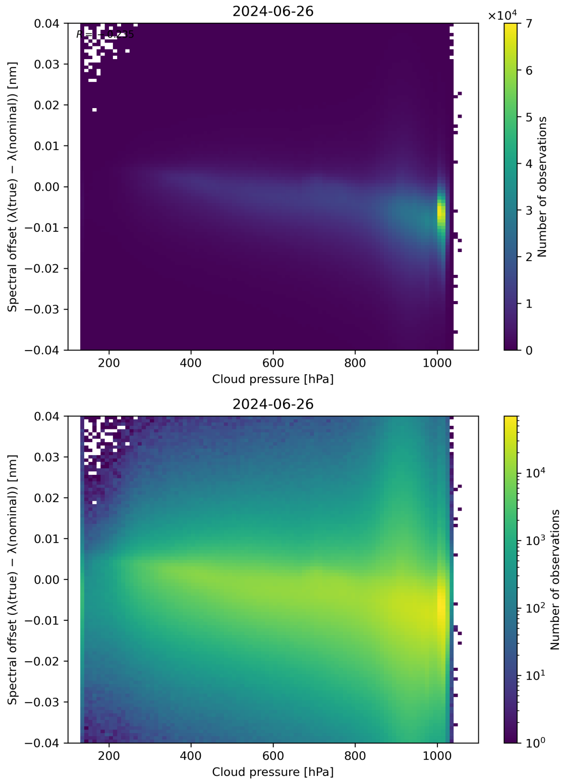
Figure 84: Scatter density plot of “Cloud pressure” against “Spectral offset ( \lambda(\text{true}) - \lambda(\text{nominal}) )” for 2024-06-25 to 2024-06-27.
