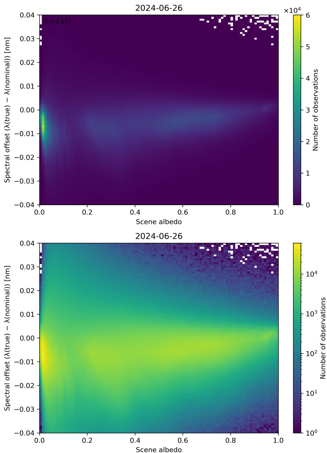
Figure 107: Scatter density plot of “Scene albedo” against “Spectral offset ( \lambda(\text{true}) - \lambda(\text{nominal}) )” for 2024-06-25 to 2024-06-27.
