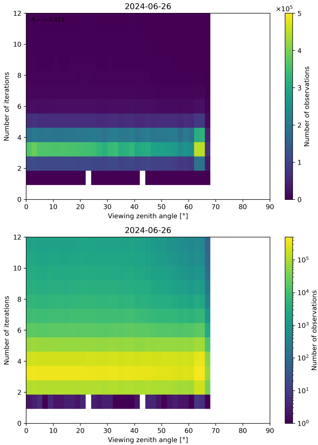
Figure 124: Scatter density plot of “Viewing zenith angle” against “Number of iterations” for 2024-06-25 to 2024-06-27.
