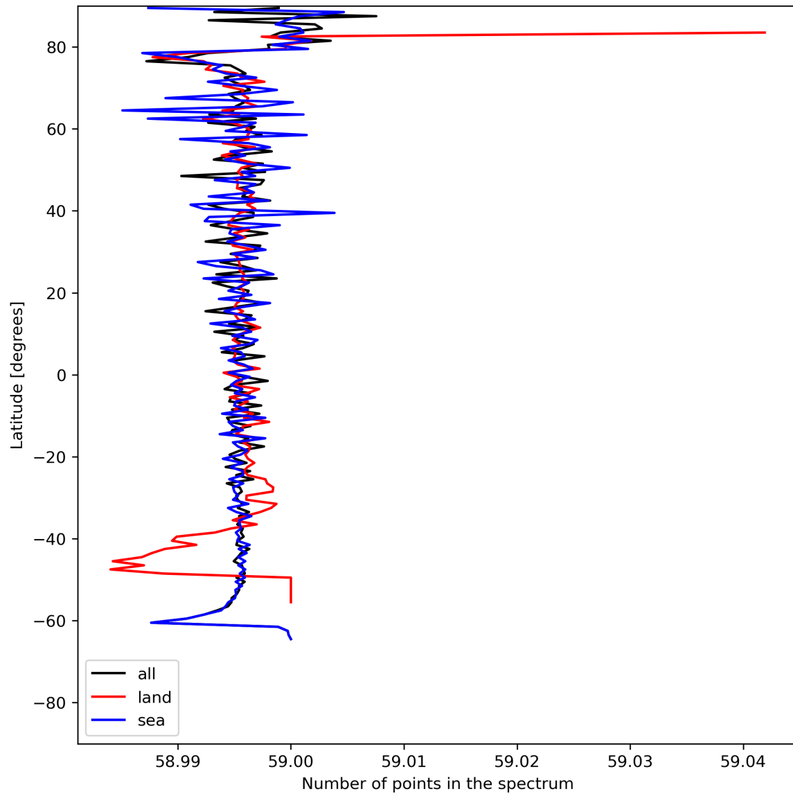
Figure 27: Zonal average of “Number of points in the spectrum” for 2024-06-25 to 2024-06-27.
