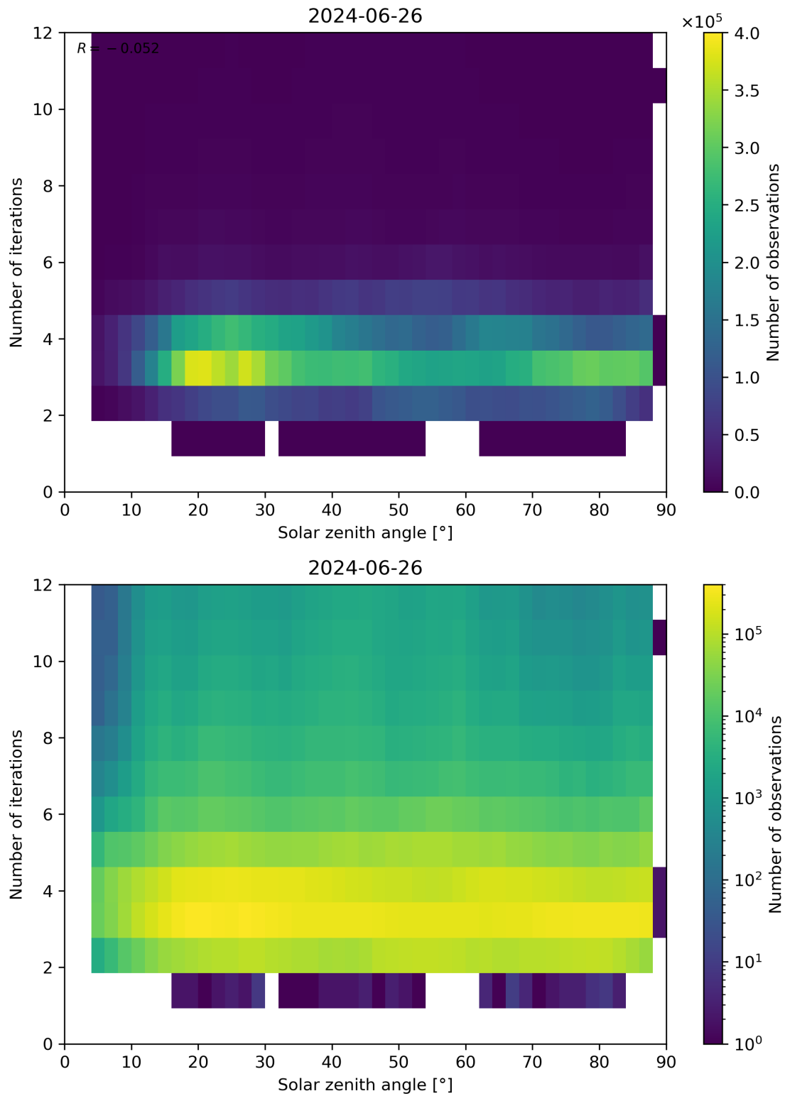
Figure 114: Scatter density plot of “Solar zenith angle” against “Number of iterations” for 2024-06-25 to 2024-06-27.
