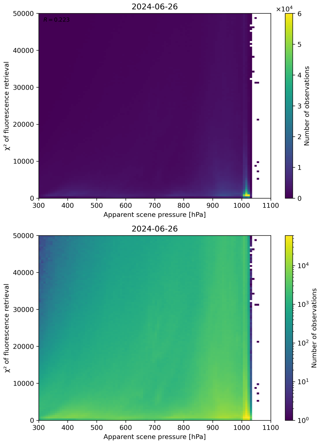
Figure 63: Scatter density plot of “Apparent scene pressure” against “ \chi^2 of fluorescence retrieval” for 2024-06-25 to 2024-06-27.
