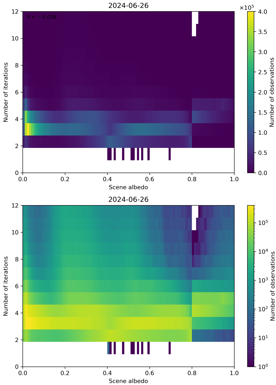
Figure 105: Scatter density plot of “Scene albedo” against “Number of iterations” for 2024-06-25 to 2024-06-27.
