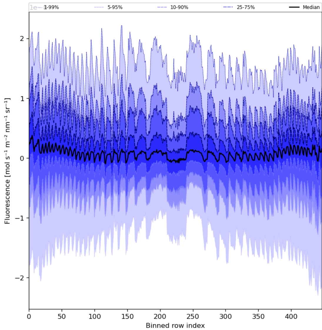
Figure 57: Along track statistics of “Fluorescence” for 2024-06-25 to 2024-06-27
