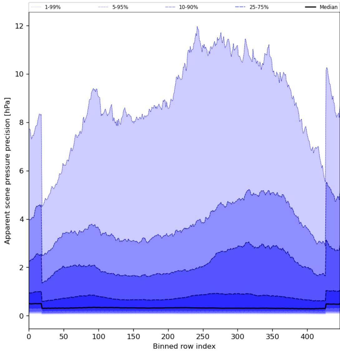
Figure 54: Along track statistics of “Apparent scene pressure precision” for 2024-06-25 to 2024-06-27
