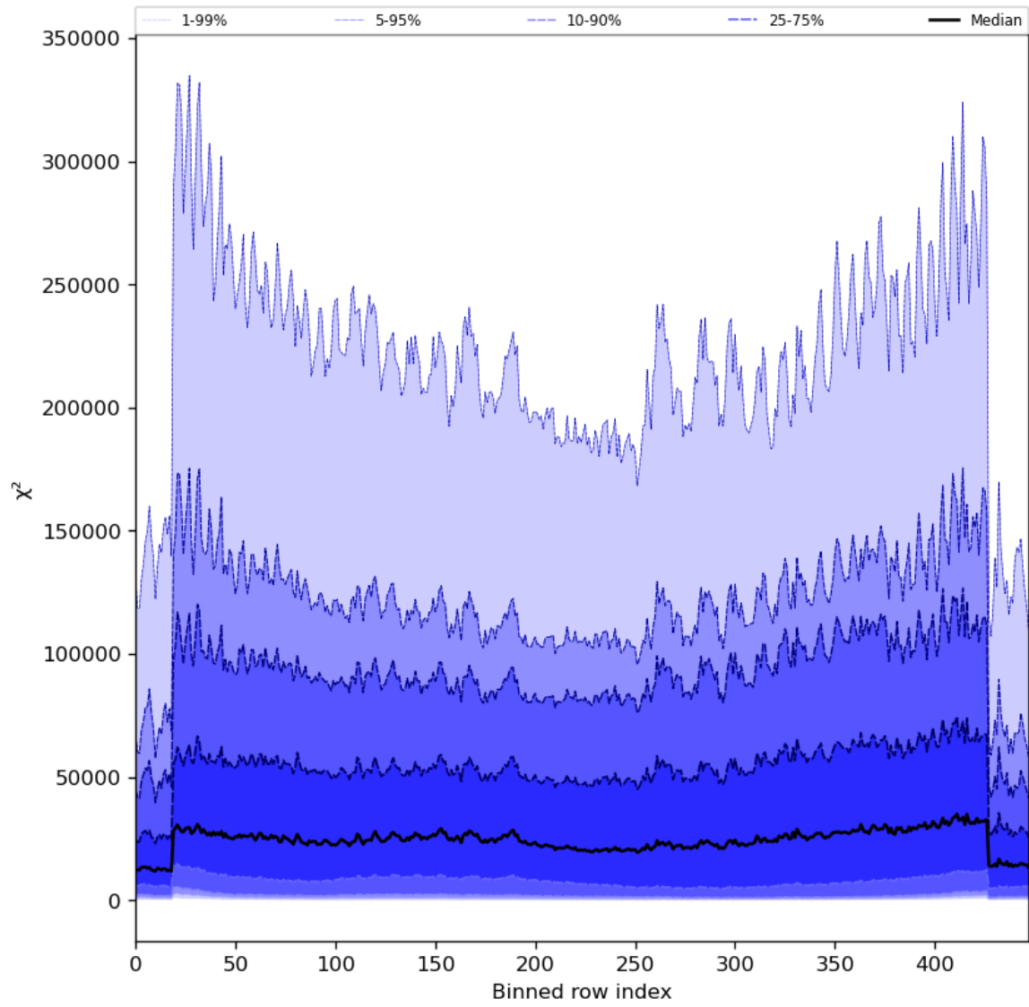
Figure 55: Along track statistics of “ \chi^2 ” for 2024-06-25 to 2024-06-27
