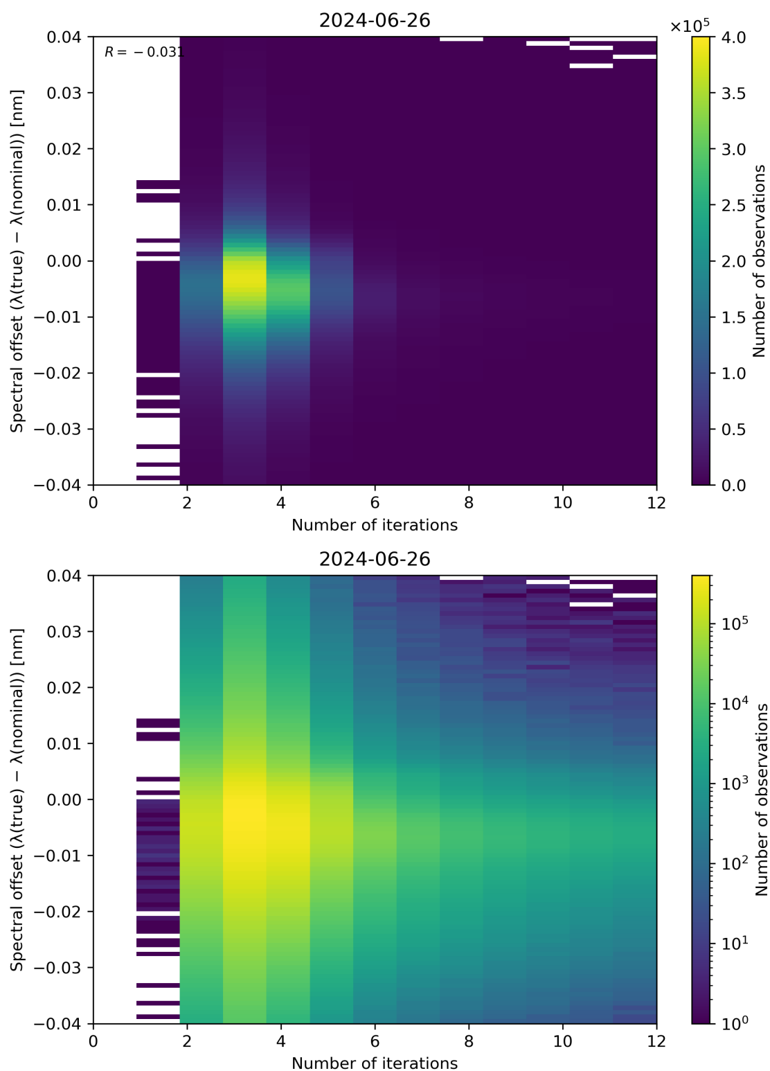
Figure 100: Scatter density plot of “Number of iterations” against “Spectral offset ( \lambda(\text{true}) - \lambda(\text{nominal}) )” for 2024-06-25 to 2024-06-27.
