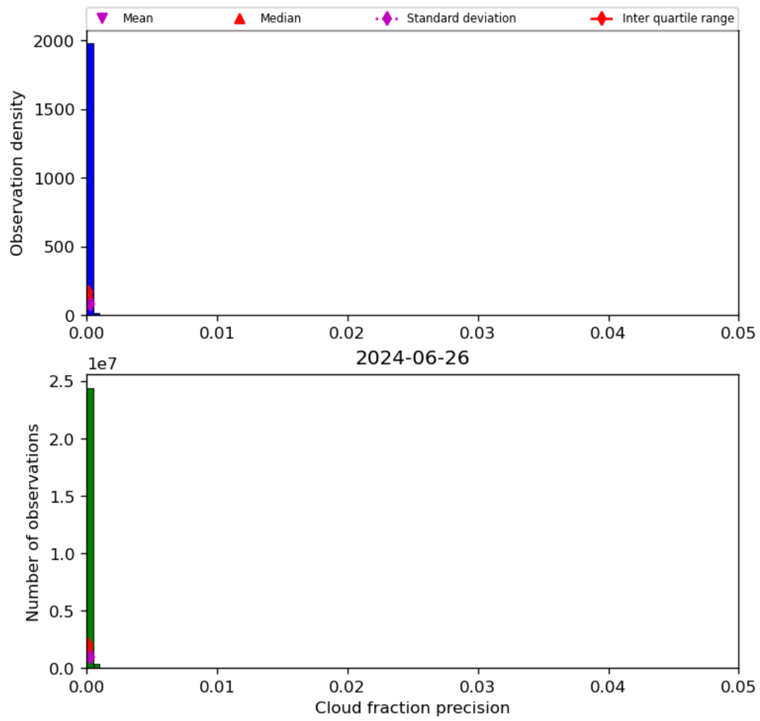
Figure 33: Histogram of “Cloud fraction precision” for 2024-06-25 to 2024-06-27
