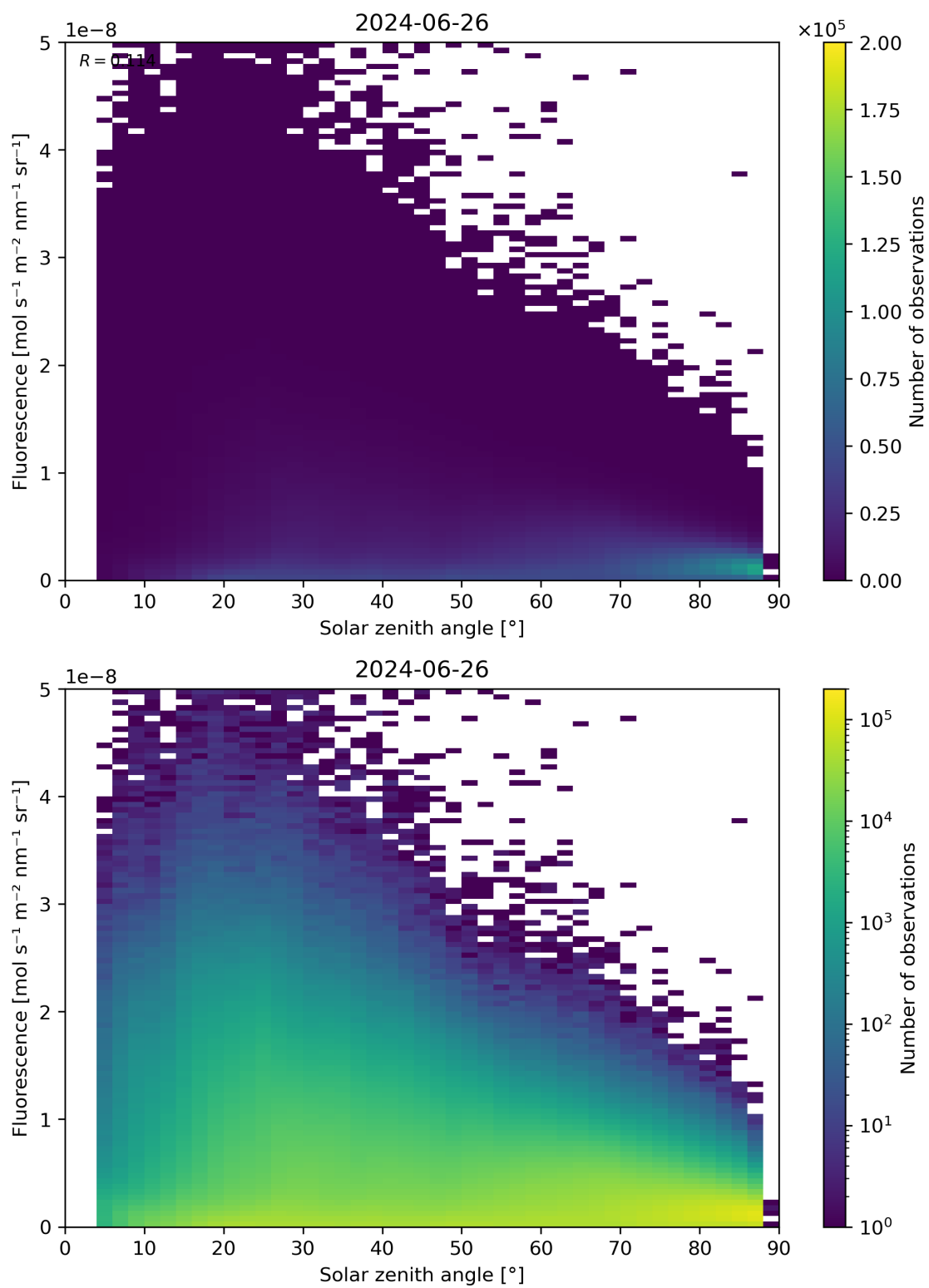
Figure 112: Scatter density plot of “Solar zenith angle” against “Fluorescence” for 2024-06-25 to 2024-06-27.
