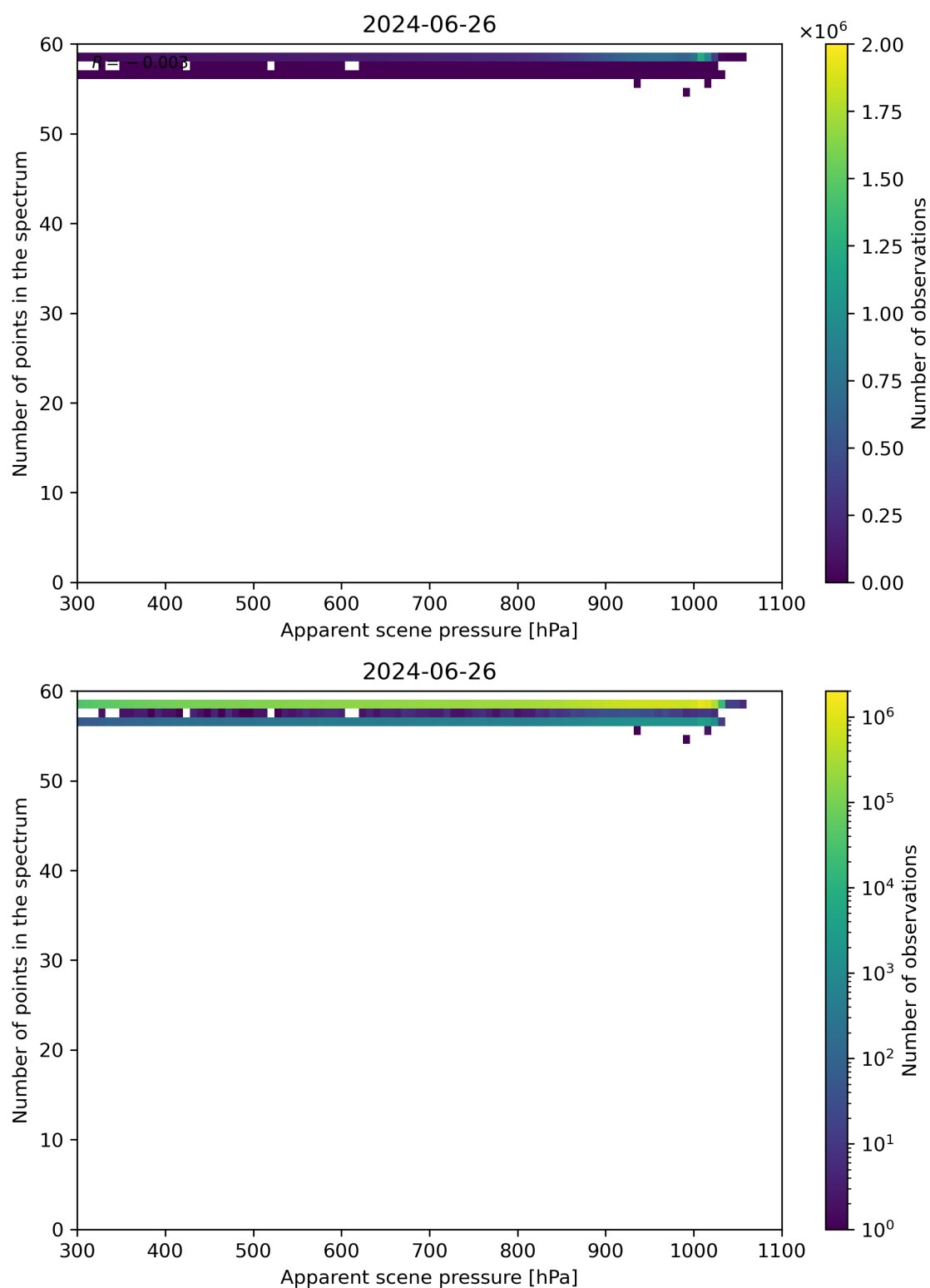
Figure 66: Scatter density plot of “Apparent scene pressure” against “Number of points in the spectrum” for 2024-06-25 to 2024-06-27.
