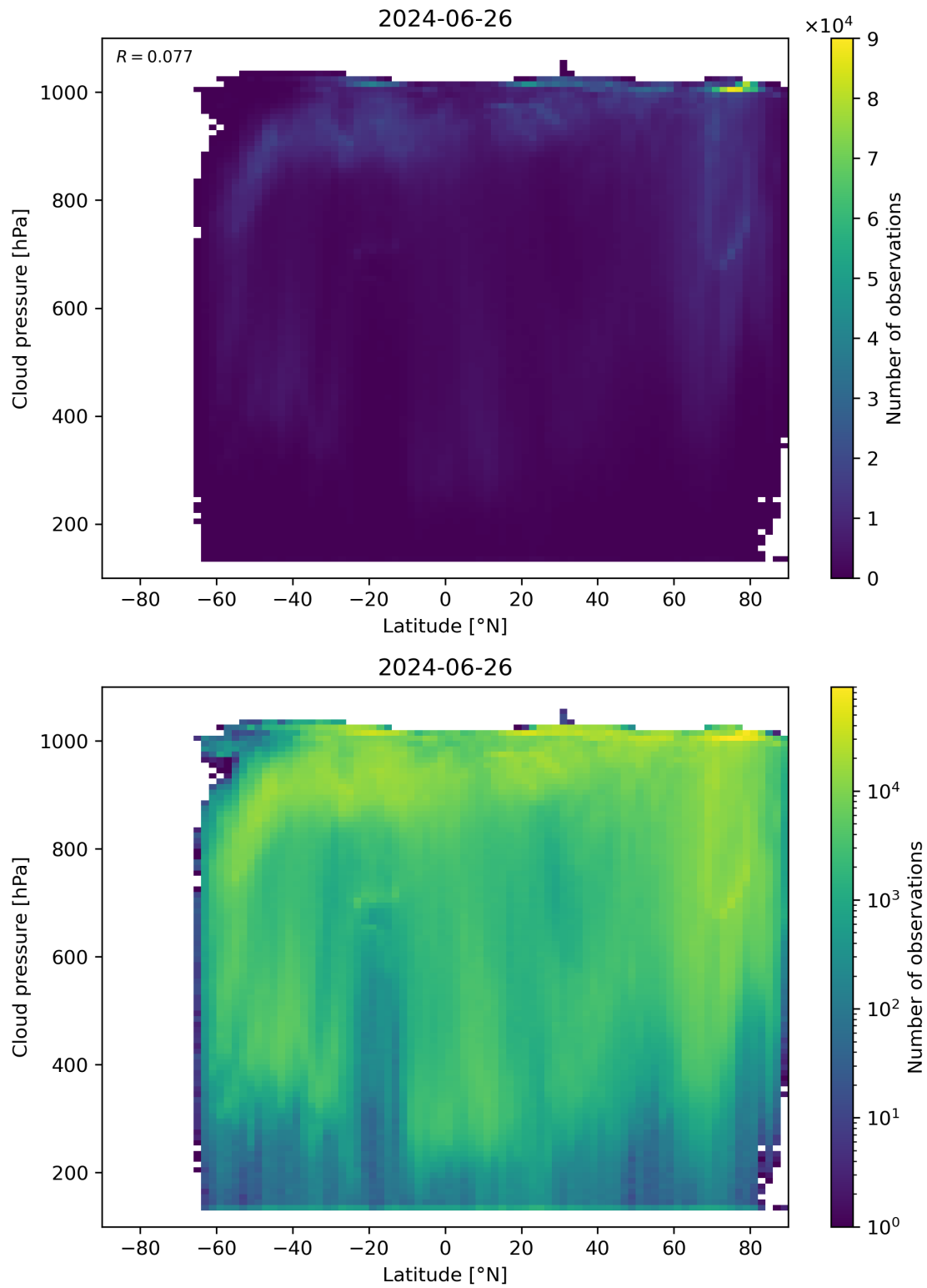
Figure 91: Scatter density plot of “Latitude” against “Cloud pressure” for 2024-06-25 to 2024-06-27.
