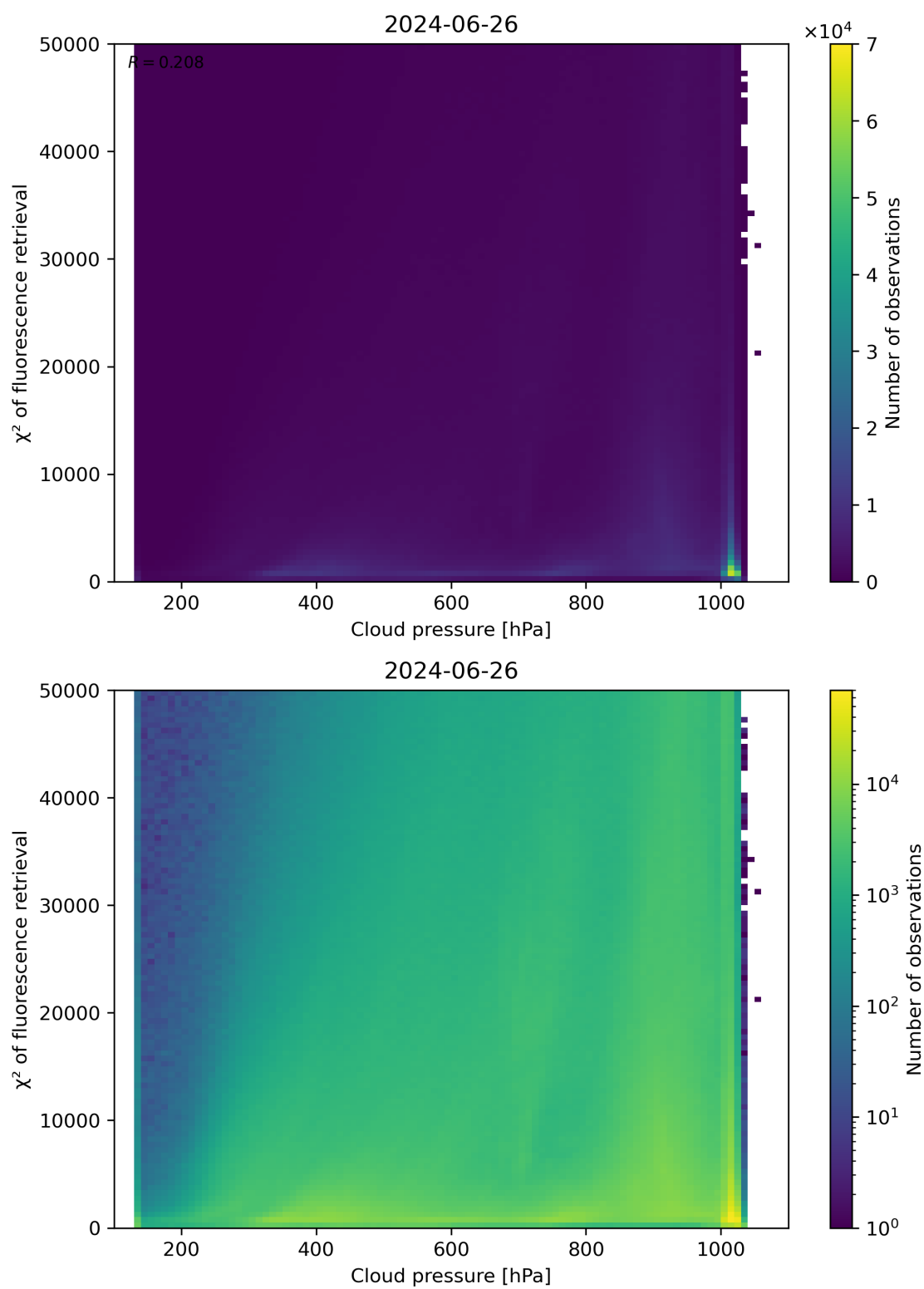
Figure 78: Scatter density plot of “Cloud pressure” against “ \chi^2 of fluorescence retrieval” for 2024-06-25 to 2024-06-27.
