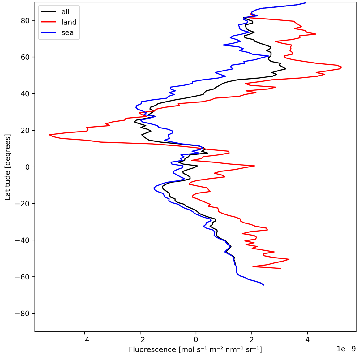
Figure 23: Zonal average of “Fluorescence” for 2024-06-25 to 2024-06-27.
