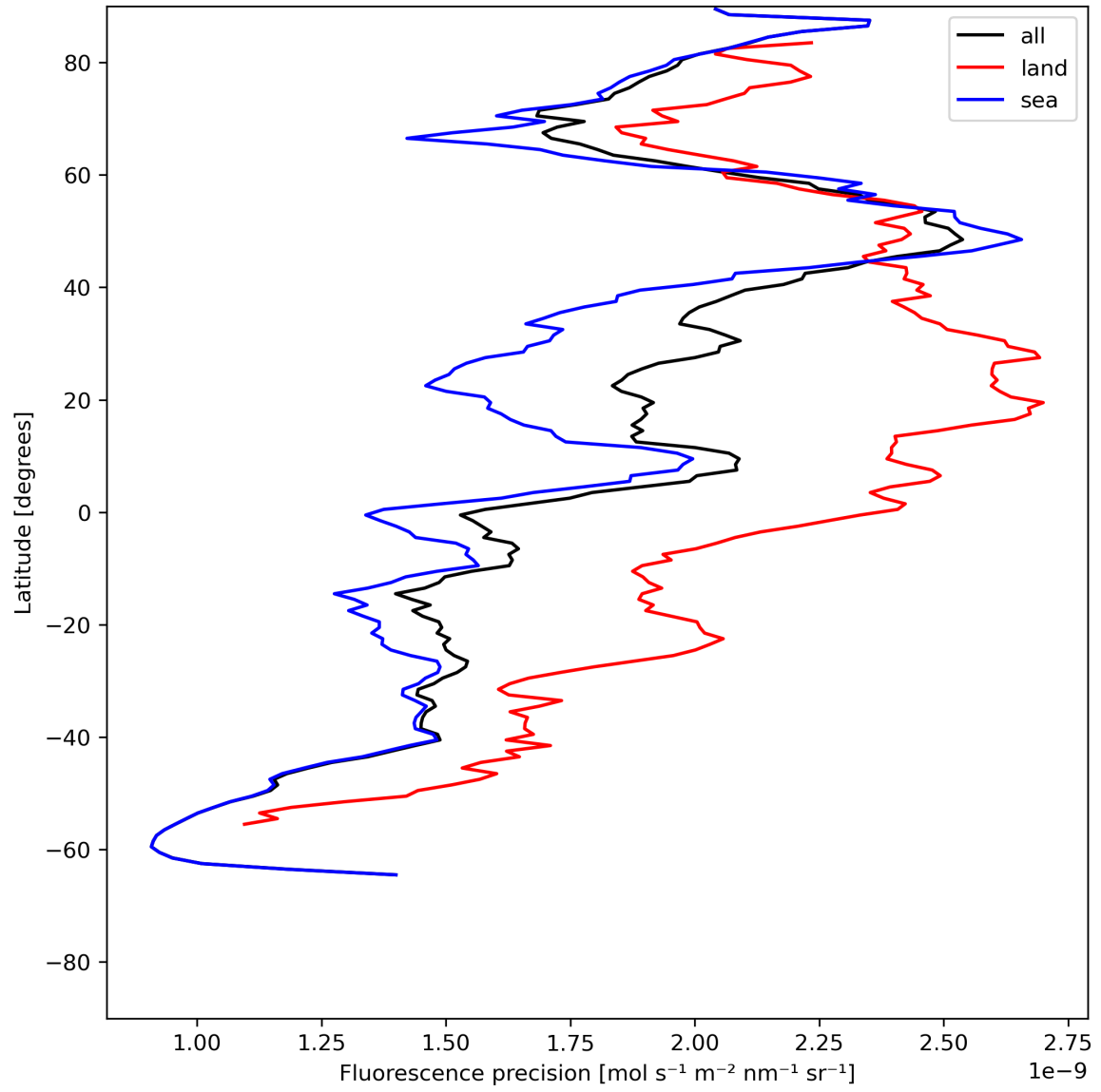
Figure 24: Zonal average of “Fluorescence precision” for 2024-06-25 to 2024-06-27.
