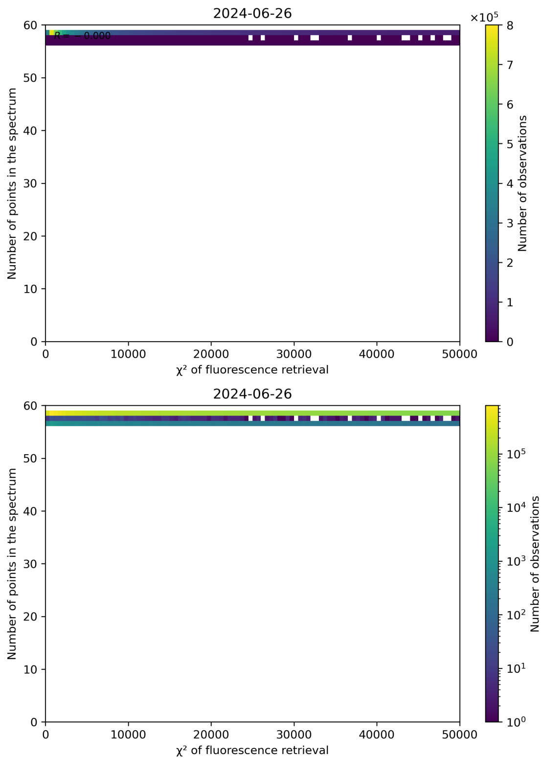
Figure 68: Scatter density plot of " \chi^2 of fluorescence retrieval" against "Number of points in the spectrum" for 2024-06-25 to 2024-06-27.
