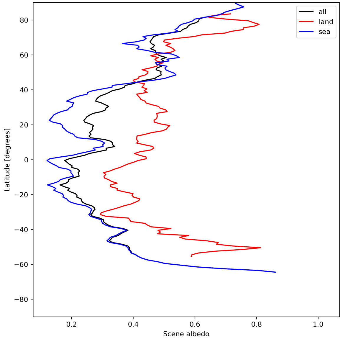
Figure 17: Zonal average of “Scene albedo” for 2024-06-25 to 2024-06-27.
