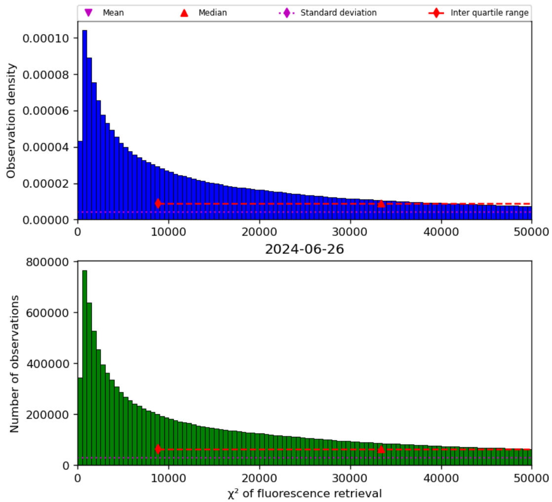
Figure 42: Histogram of “ \chi^2 of fluorescence retrieval” for 2024-06-25 to 2024-06-27
