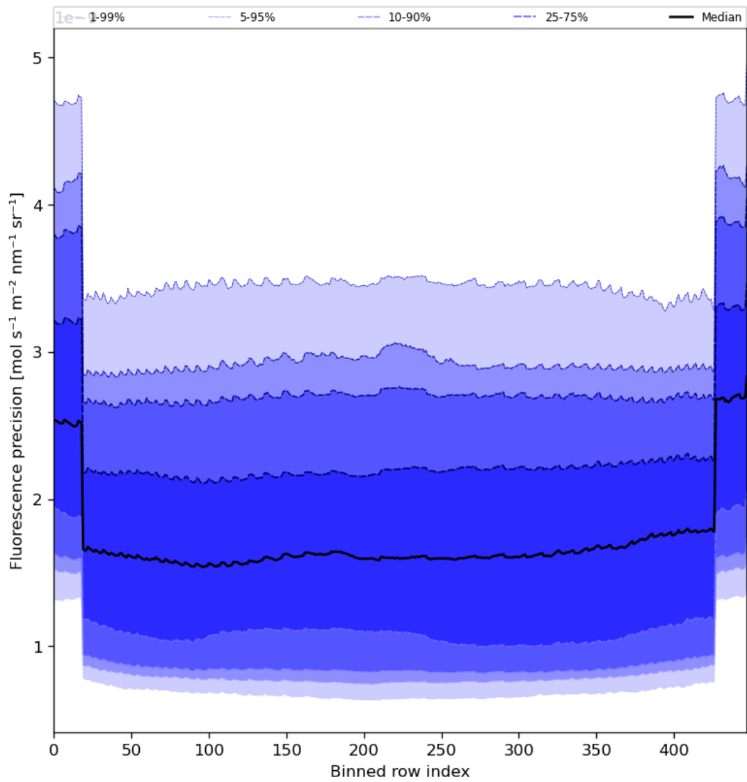
Figure 58: Along track statistics of “Fluorescence precision” for 2024-06-25 to 2024-06-27
