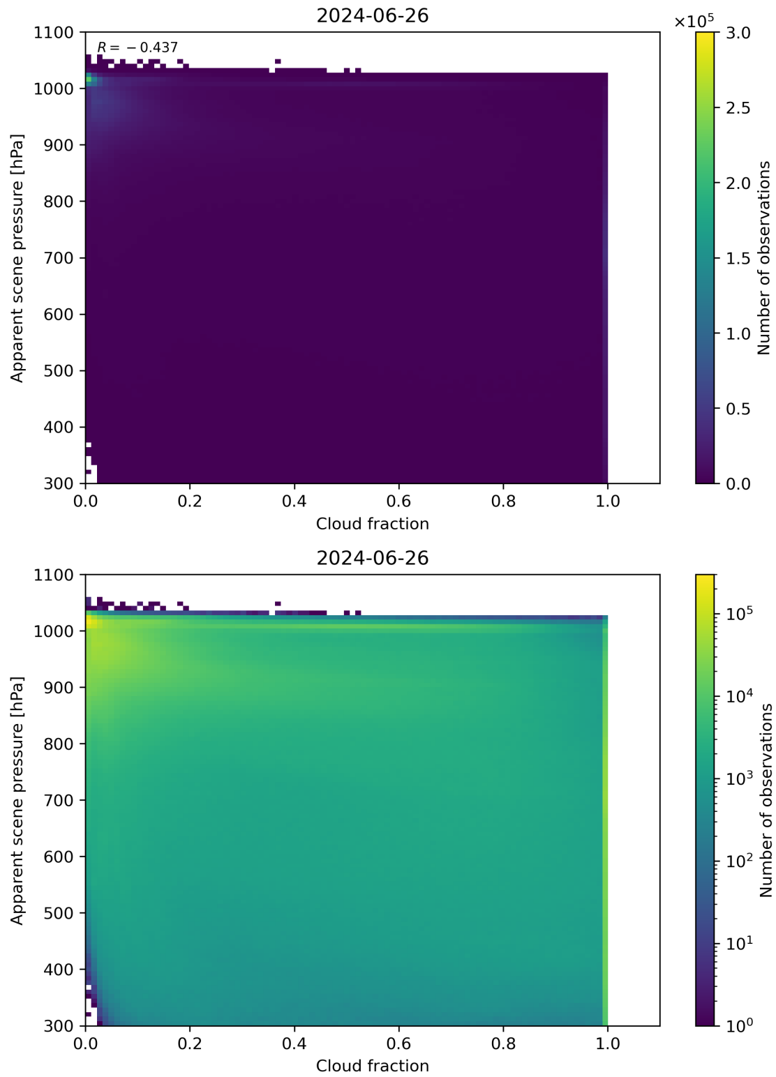
Figure 70: Scatter density plot of “Cloud fraction” against “Apparent scene pressure” for 2024-06-25 to 2024-06-27.
