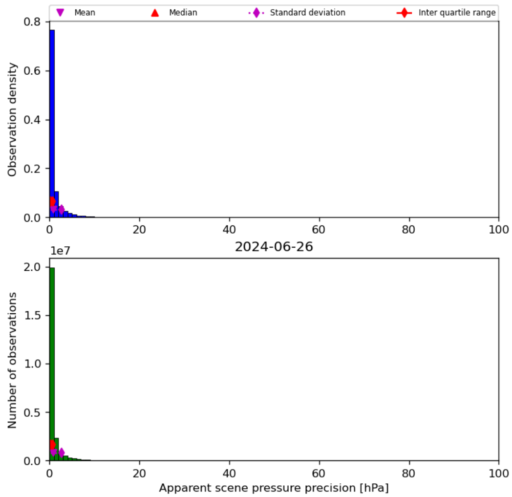
Figure 37: Histogram of “Apparent scene pressure precision” for 2024-06-25 to 2024-06-27
