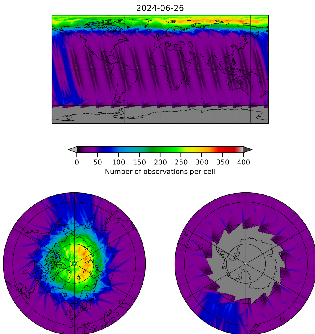
Figure 11: Map of the number of observations for 2024-06-25 to 2024-06-27
