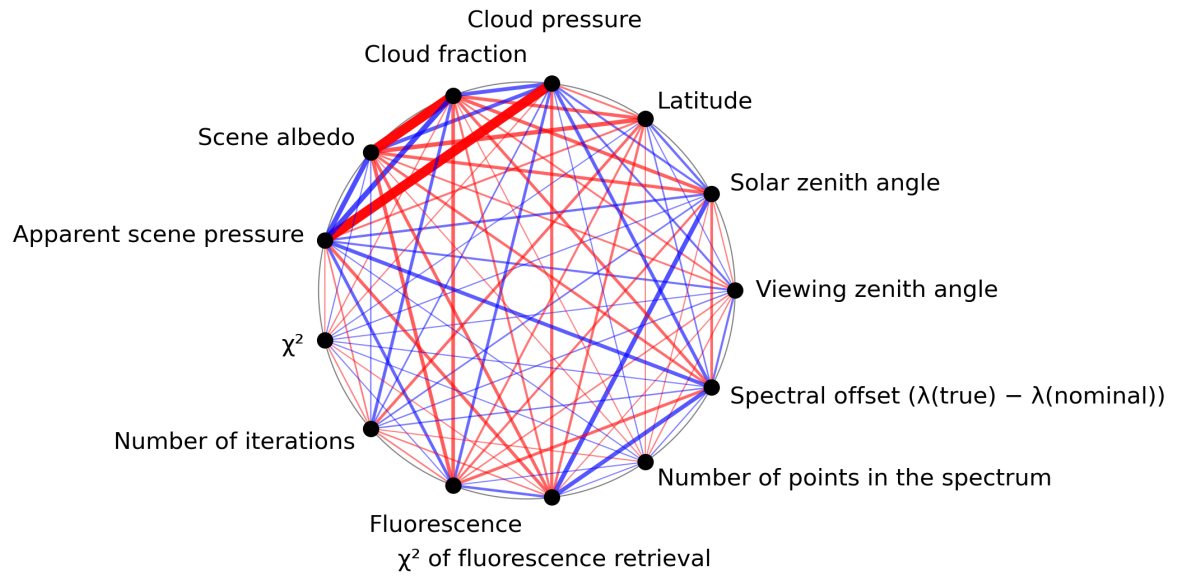
Figure 1: Map of correlation graph for 2024-06-25 to 2024-06-27.
