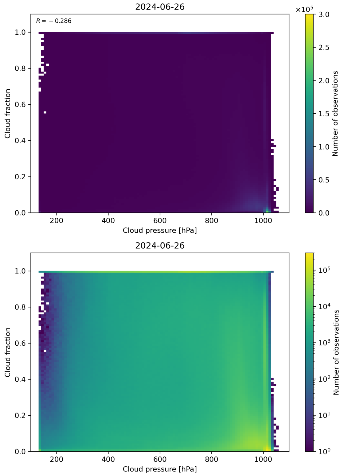
Figure 79: Scatter density plot of “Cloud pressure” against “Cloud fraction” for 2024-06-25 to 2024-06-27.
