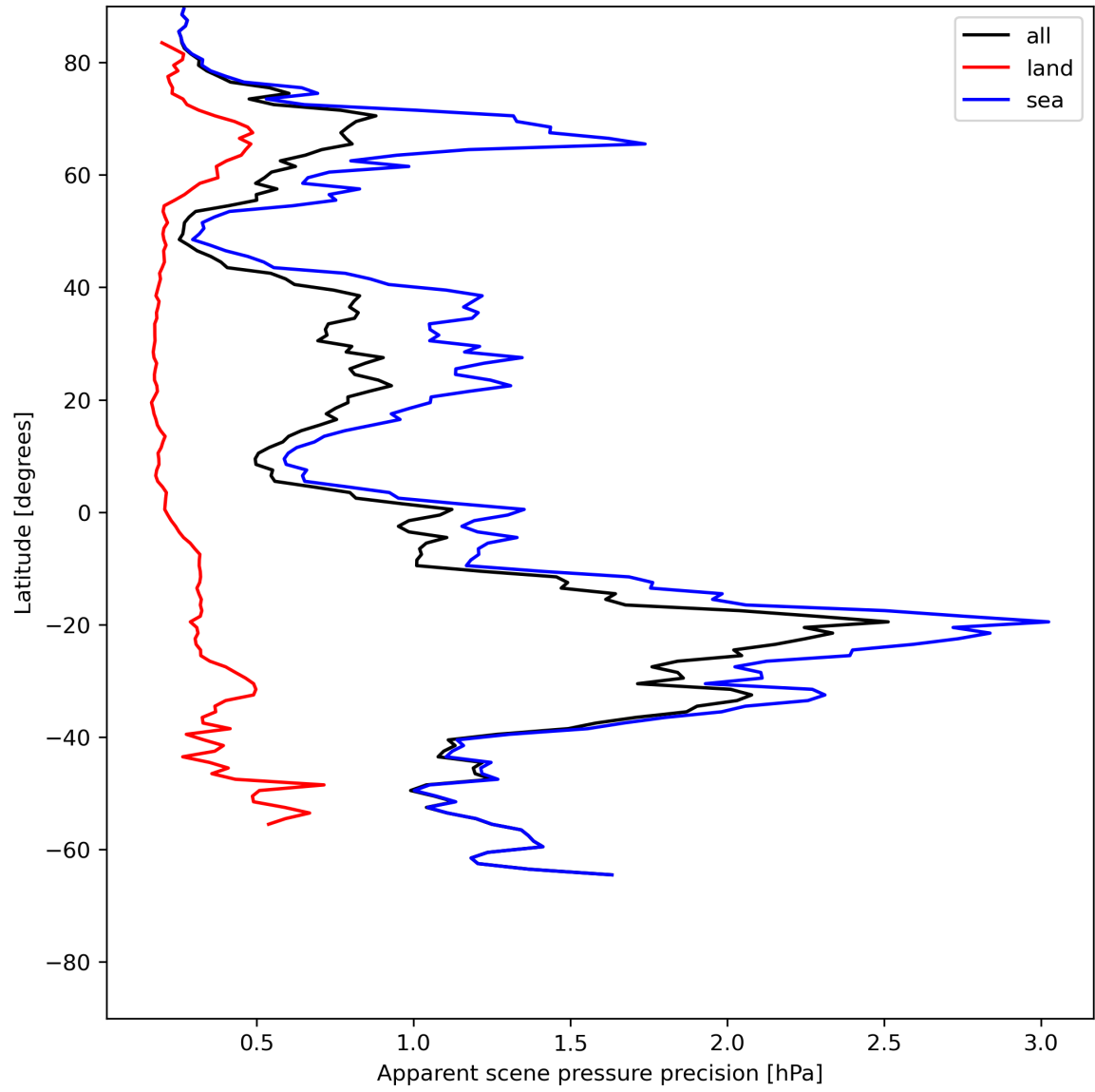
Figure 20: Zonal average of “Apparent scene pressure precision” for 2024-06-25 to 2024-06-27.
