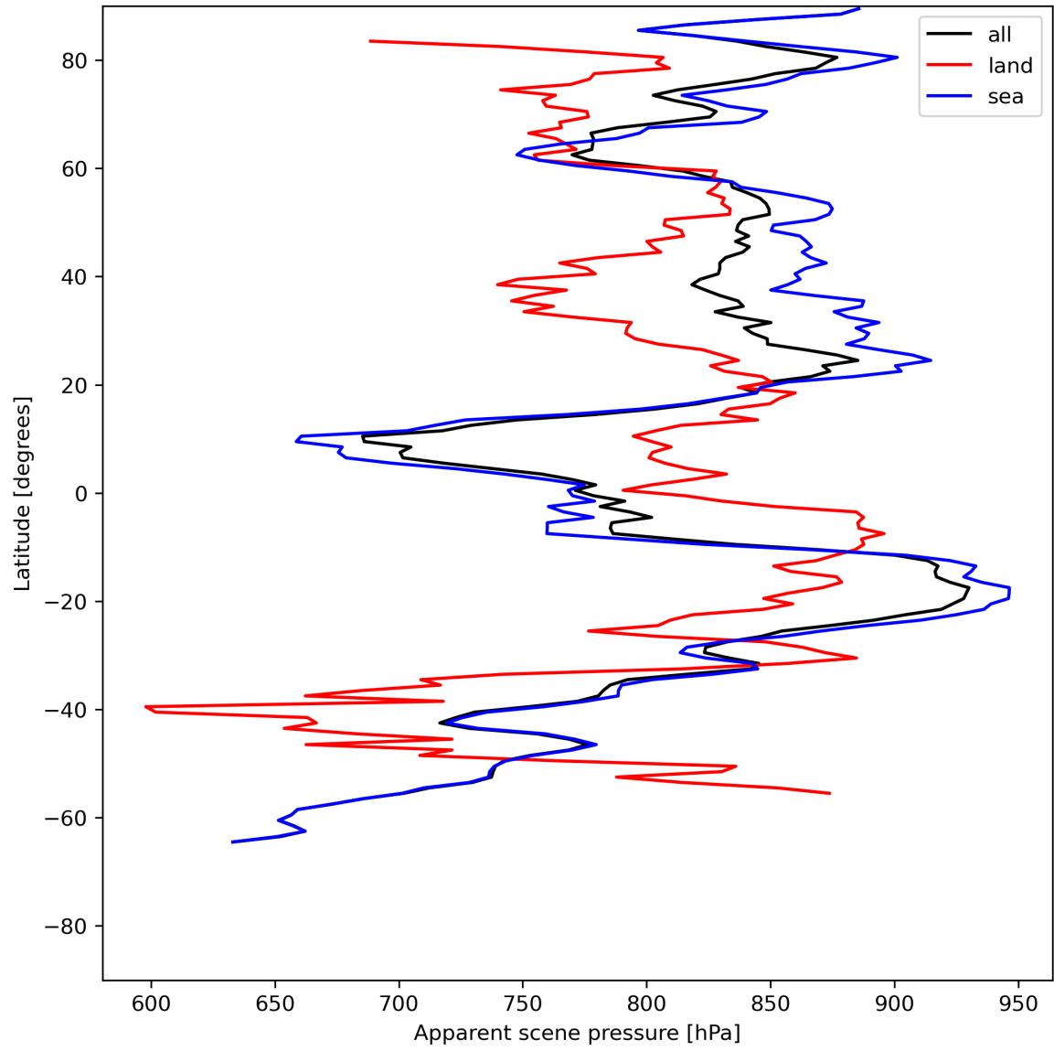
Figure 19: Zonal average of “Apparent scene pressure” for 2024-06-25 to 2024-06-27.
