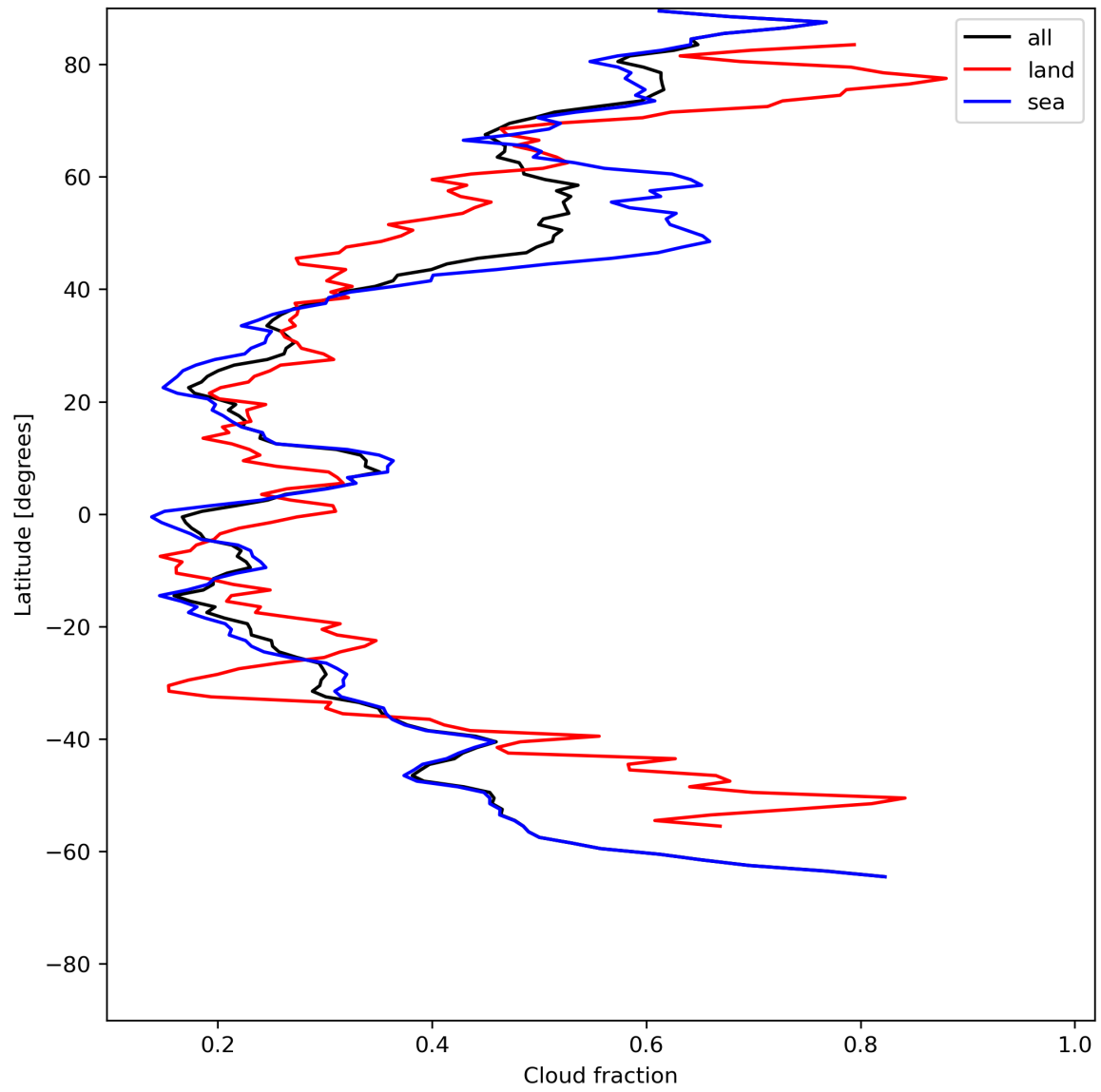
Figure 15: Zonal average of “Cloud fraction” for 2024-06-25 to 2024-06-27.
