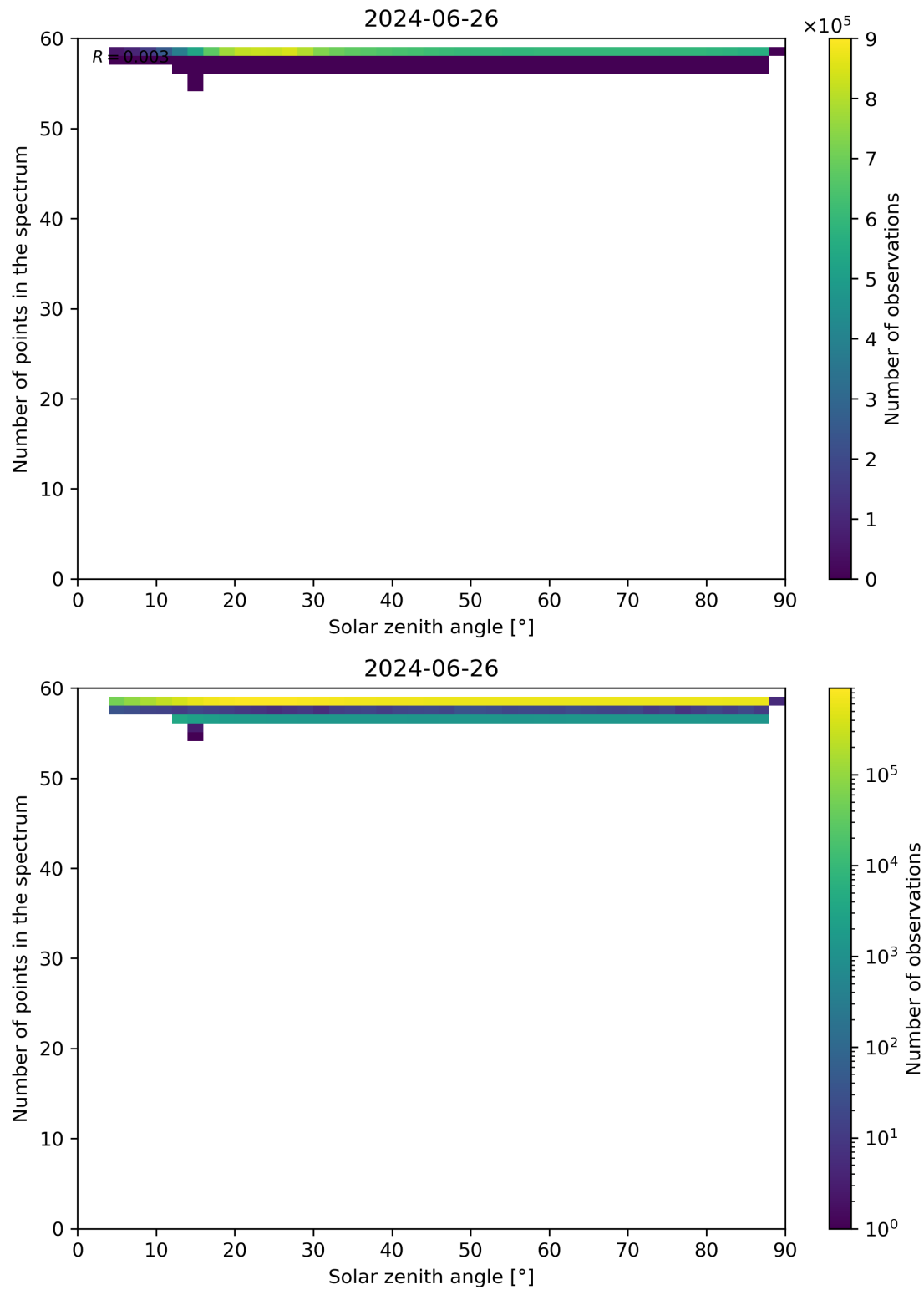
Figure 115: Scatter density plot of “Solar zenith angle” against “Number of points in the spectrum” for 2024-06-25 to 2024-06-27.
