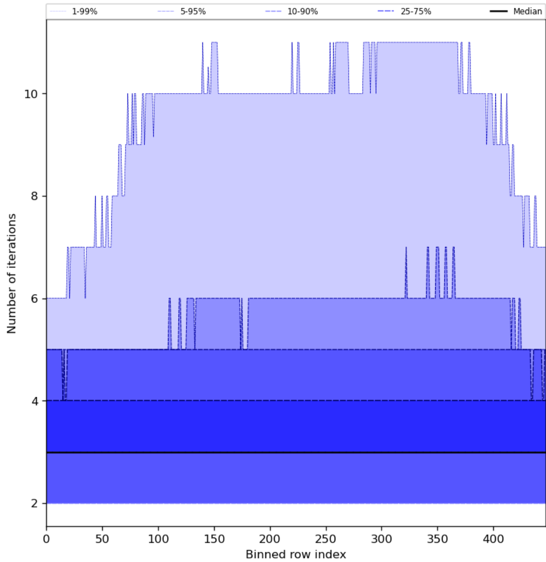
Figure 56: Along track statistics of “Number of iterations” for 2024-06-25 to 2024-06-27
