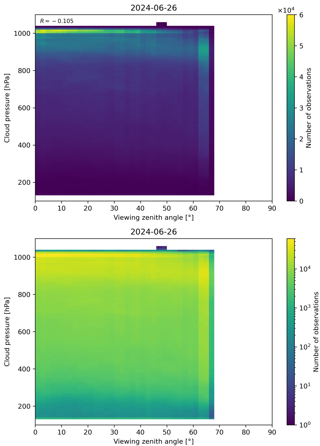
Figure 121: Scatter density plot of “Viewing zenith angle” against “Cloud pressure” for 2024-06-25 to 2024-06-27.
