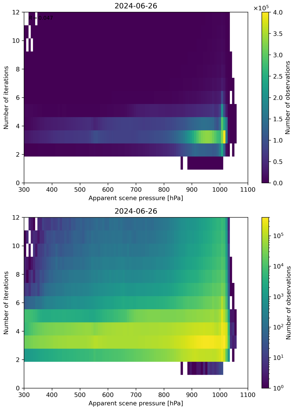
Figure 65: Scatter density plot of “Apparent scene pressure” against “Number of iterations” for 2024-06-25 to 2024-06-27.
