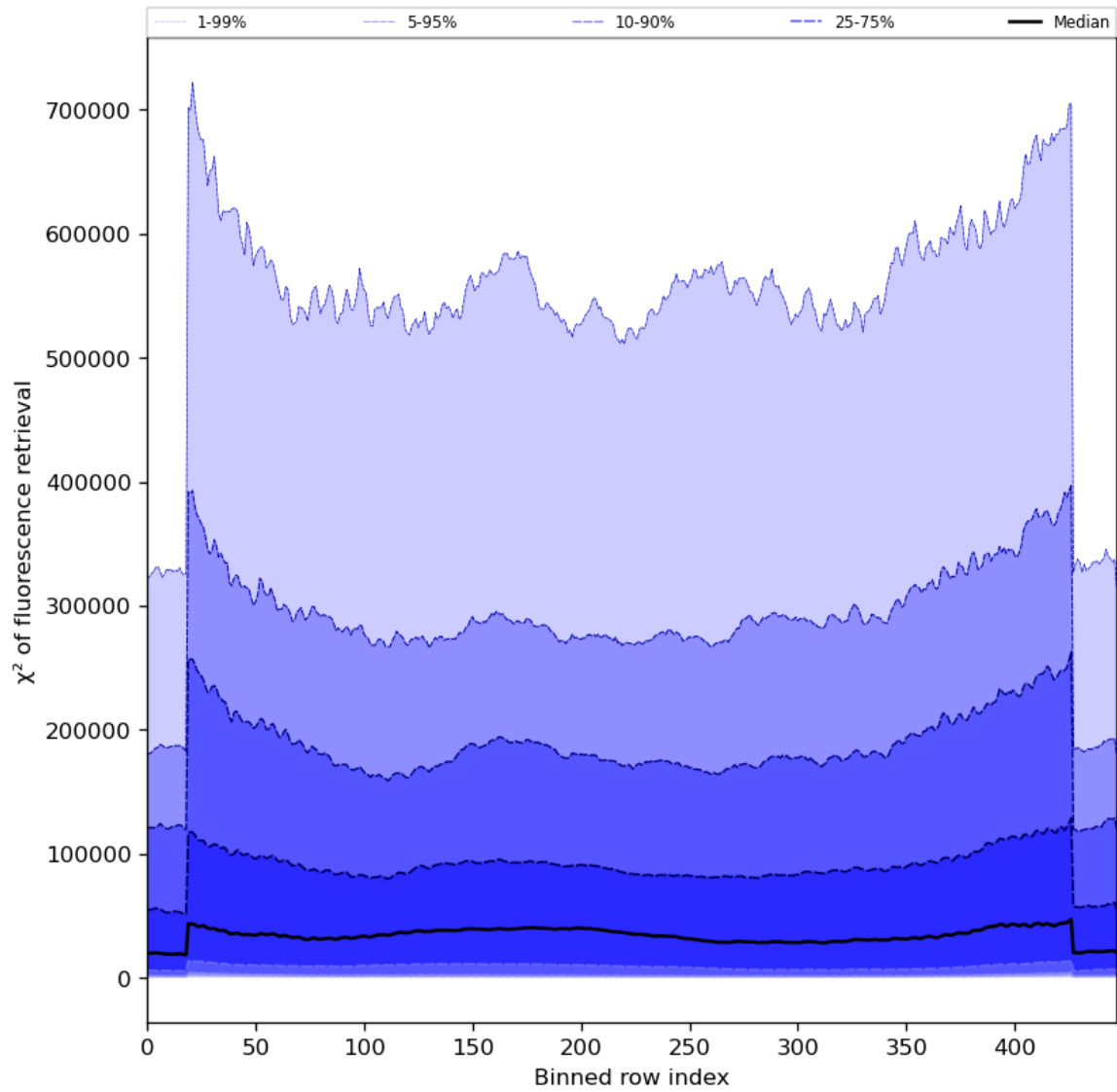
Figure 59: Along track statistics of “ \chi^2 of fluorescence retrieval” for 2024-06-25 to 2024-06-27
