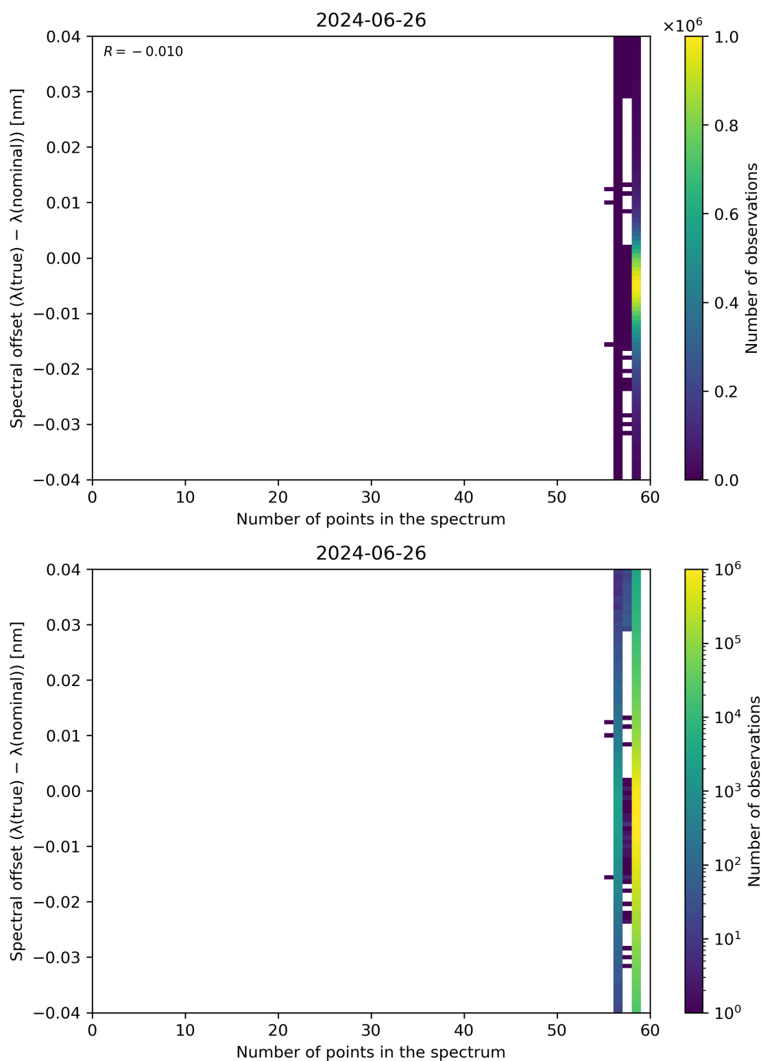
Figure 101: Scatter density plot of “Number of points in the spectrum” against “Spectral offset ( \lambda(\text{true}) - \lambda(\text{nominal}) )” for 2024-06-25 to 2024-06-27.
