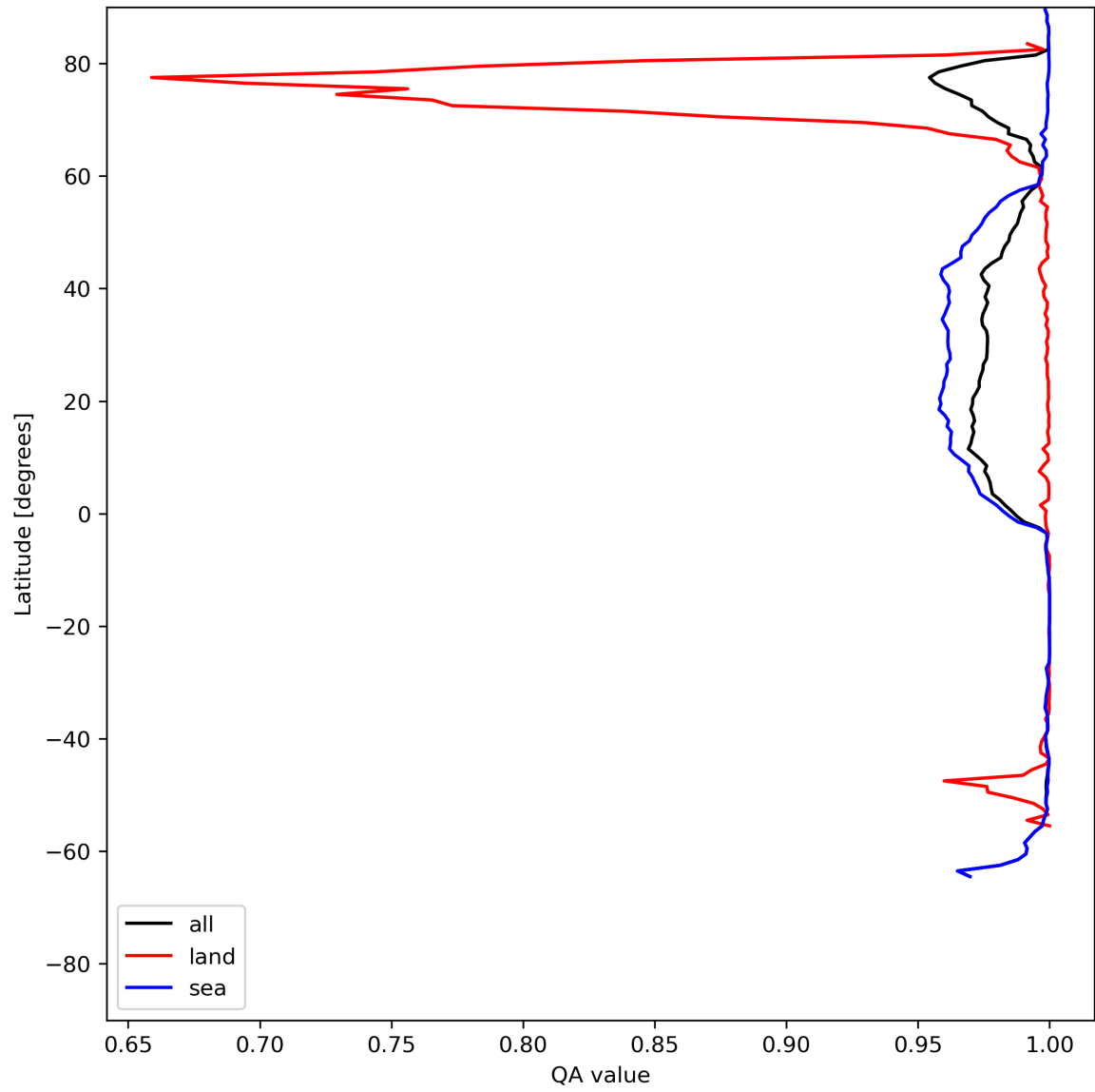
Figure 12: Zonal average of “QA value” for 2024-06-25 to 2024-06-27.
