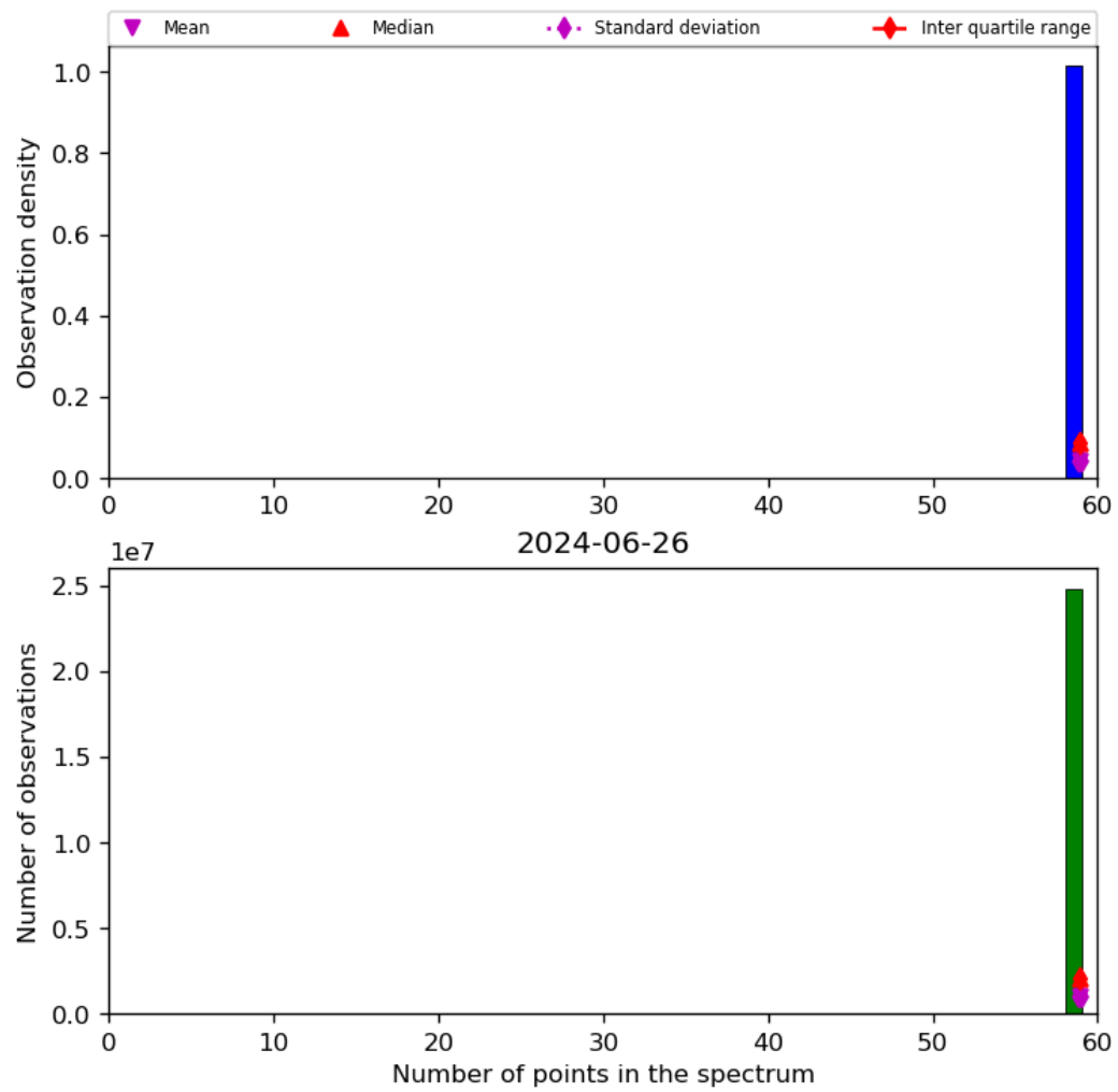
Figure 44: Histogram of “Number of points in the spectrum” for 2024-06-25 to 2024-06-27
