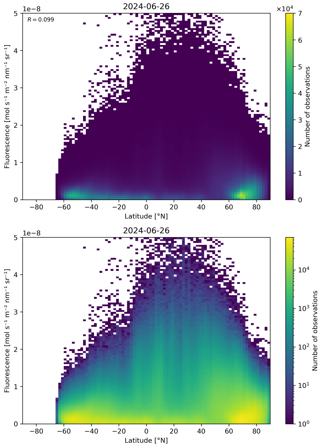
Figure 92: Scatter density plot of “Latitude” against “Fluorescence” for 2024-06-25 to 2024-06-27.
