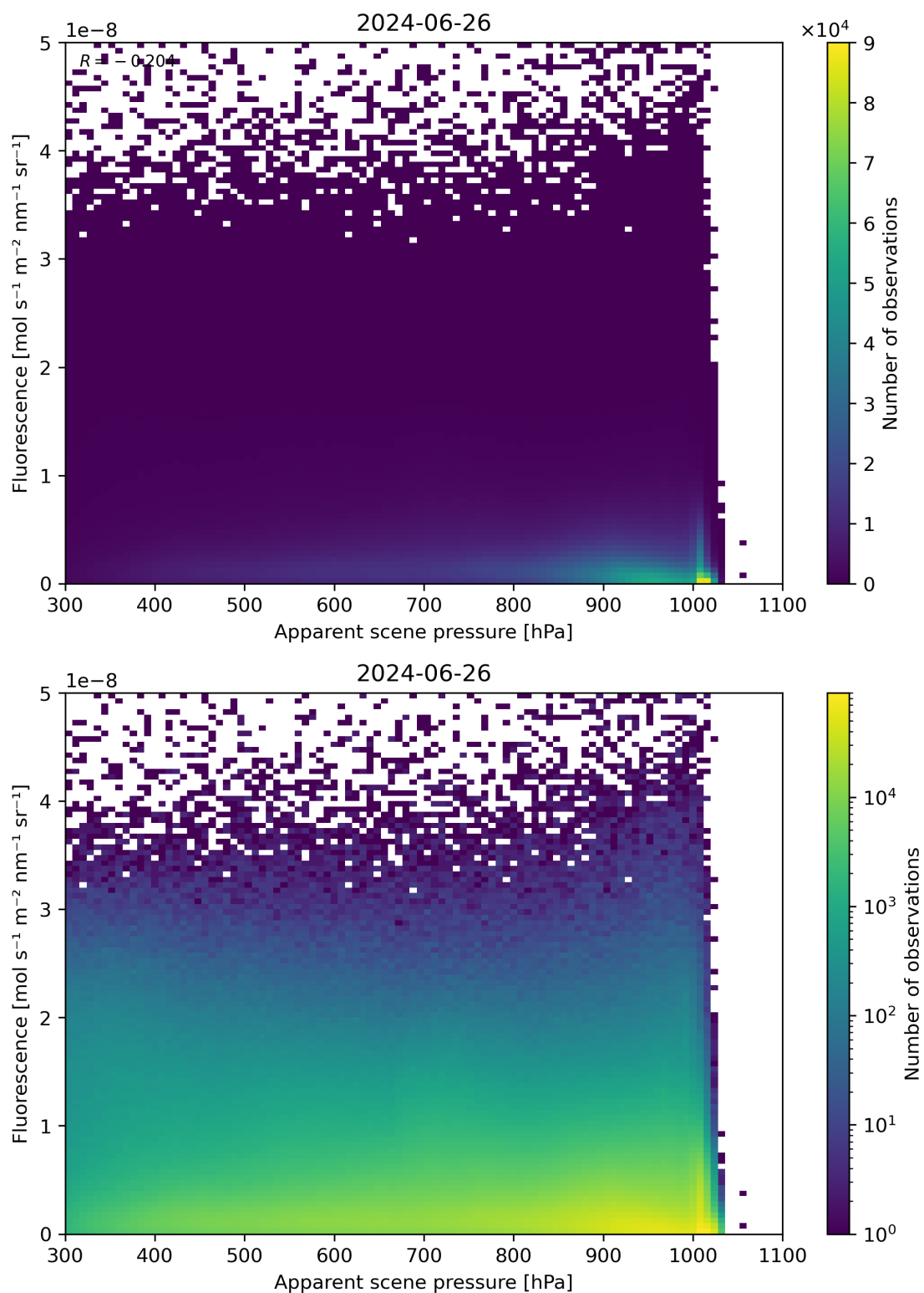
Figure 64: Scatter density plot of “Apparent scene pressure” against “Fluorescence” for 2024-06-25 to 2024-06-27.
