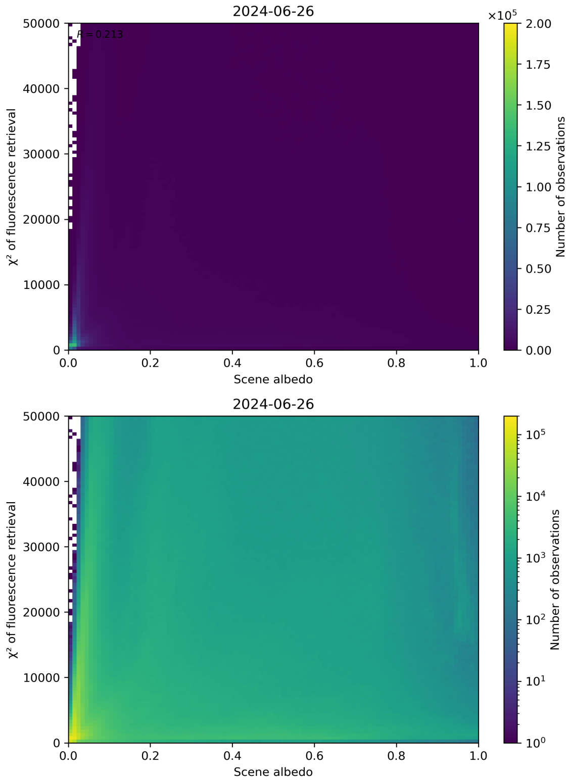
Figure 103: Scatter density plot of “Scene albedo” against “ \chi^2 of fluorescence retrieval” for 2024-06-25 to 2024-06-27.
