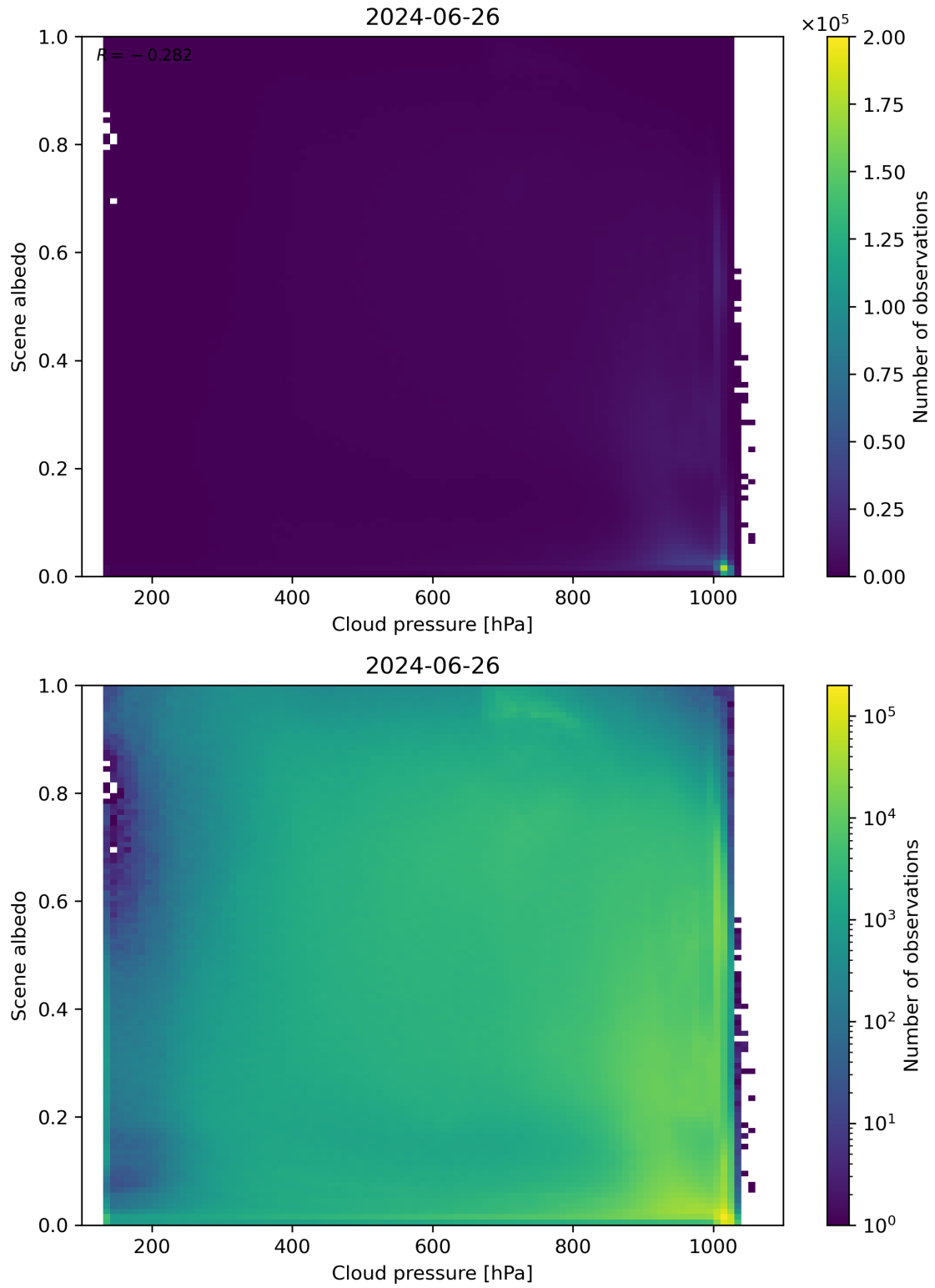
Figure 83: Scatter density plot of “Cloud pressure” against “Scene albedo” for 2024-06-25 to 2024-06-27.
