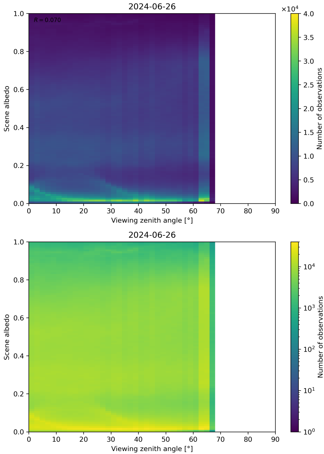
Figure 126: Scatter density plot of “Viewing zenith angle” against “Scene albedo” for 2024-06-25 to 2024-06-27.
