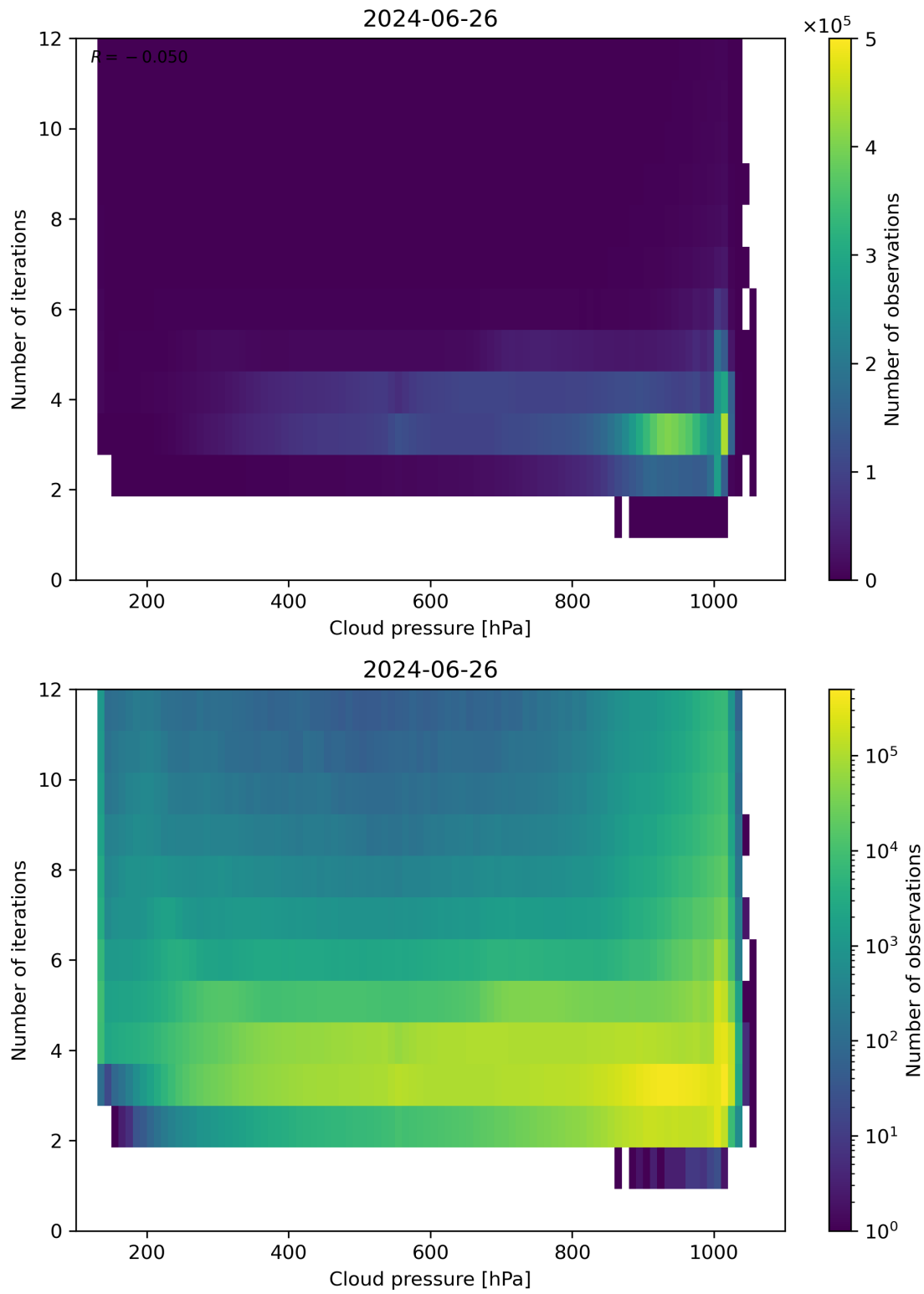
Figure 81: Scatter density plot of “Cloud pressure” against “Number of iterations” for 2024-06-25 to 2024-06-27.
