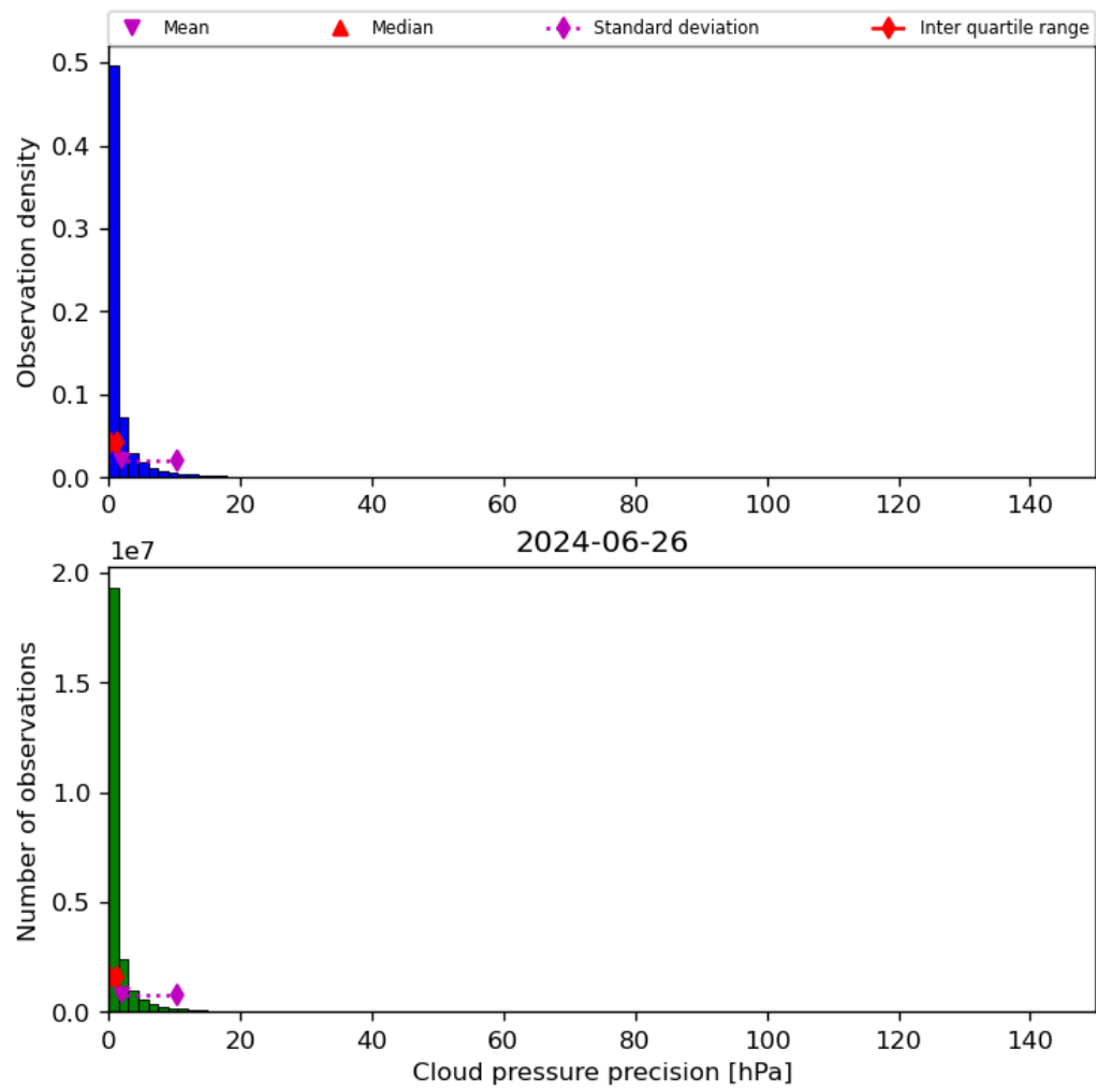
Figure 31: Histogram of “Cloud pressure precision” for 2024-06-25 to 2024-06-27
