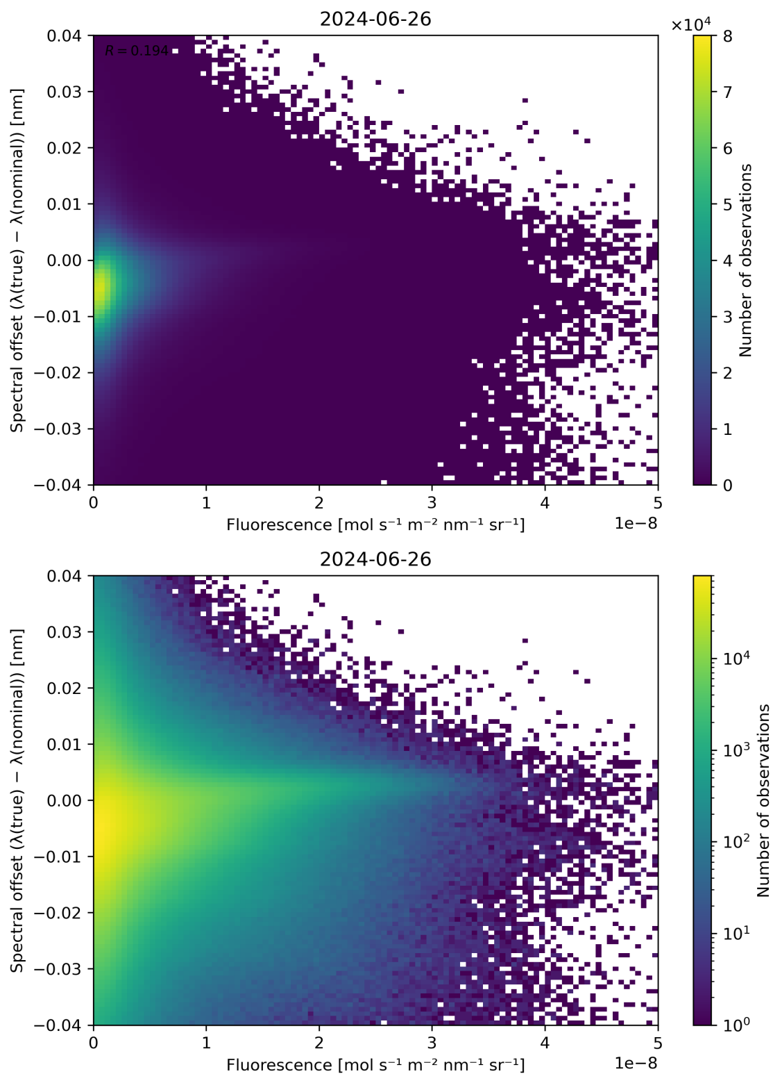
Figure 87: Scatter density plot of “Fluorescence” against “Spectral offset ( \lambda(\text{true}) - \lambda(\text{nominal}) )” for 2024-06-25 to 2024-06-27.
