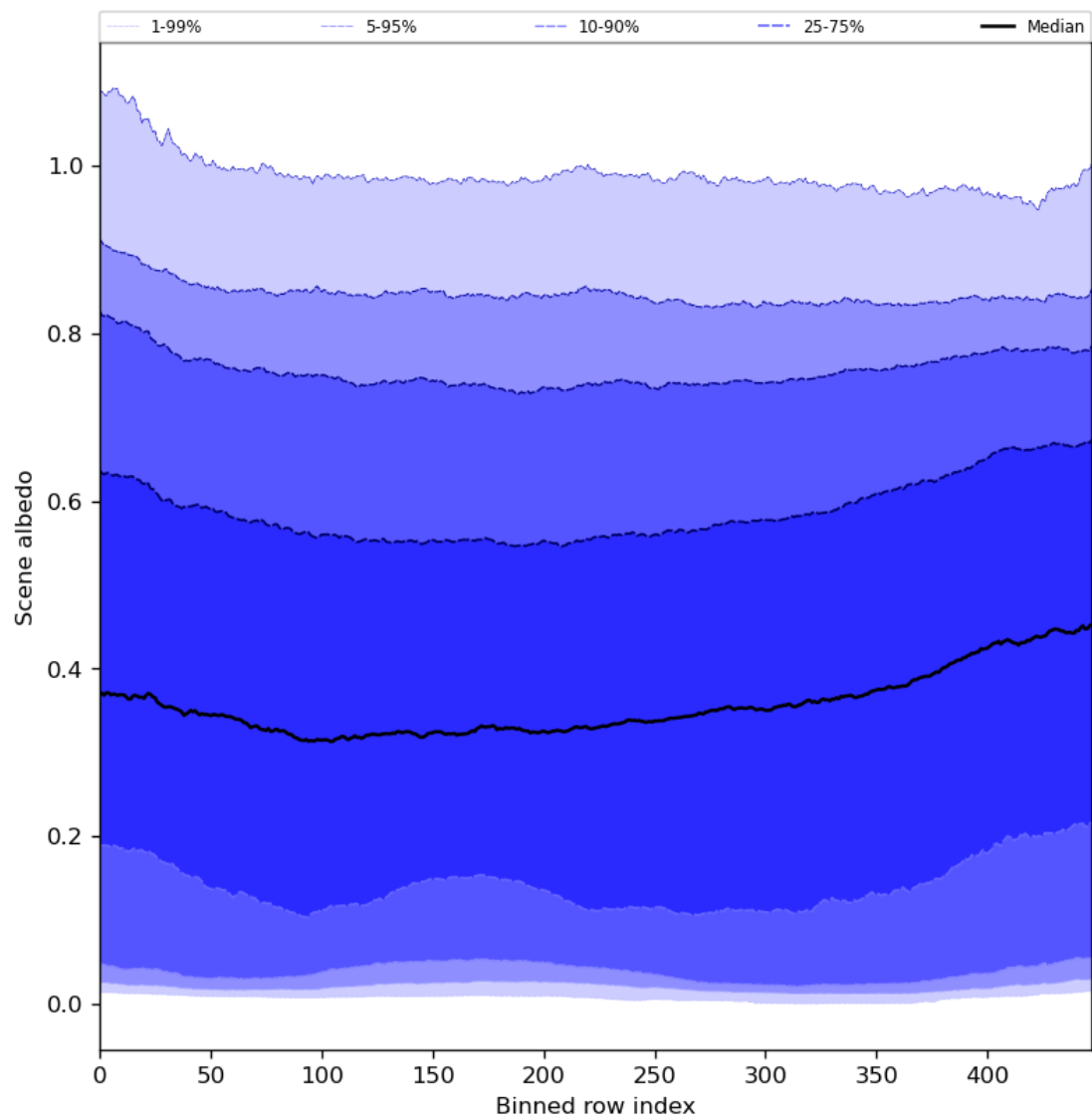
Figure 51: Along track statistics of “Scene albedo” for 2024-06-25 to 2024-06-27
