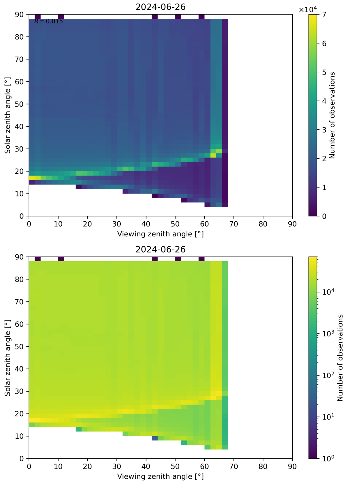
Figure 127: Scatter density plot of “Viewing zenith angle” against “Solar zenith angle” for 2024-06-25 to 2024-06-27.
