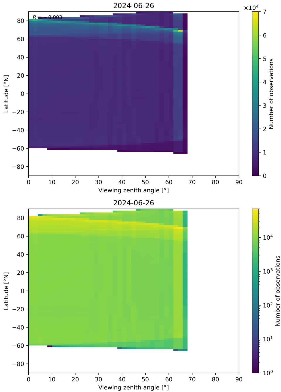
Figure 123: Scatter density plot of “Viewing zenith angle” against “Latitude” for 2024-06-25 to 2024-06-27.
