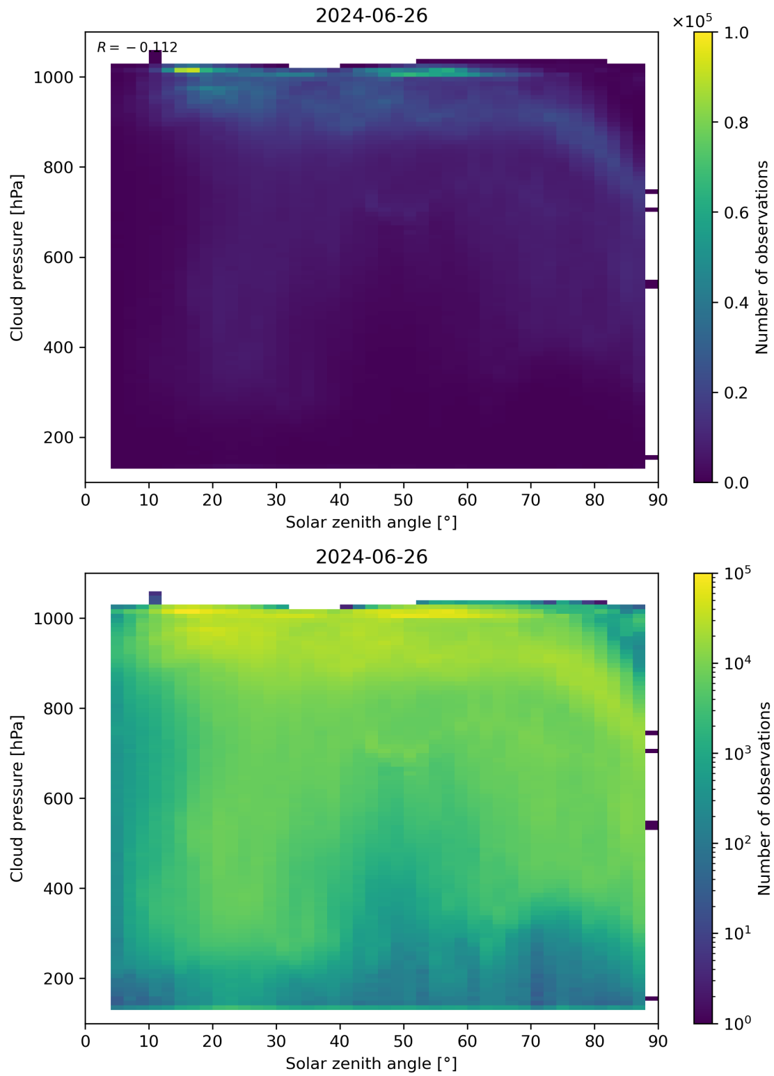
Figure 111: Scatter density plot of “Solar zenith angle” against “Cloud pressure” for 2024-06-25 to 2024-06-27.
