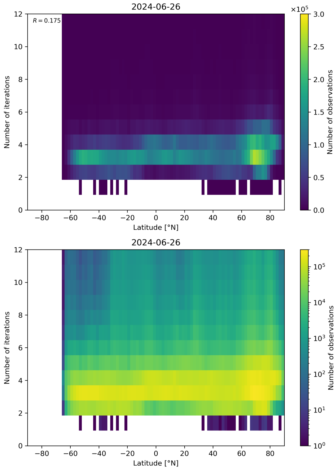
Figure 93: Scatter density plot of “Latitude” against “Number of iterations” for 2024-06-25 to 2024-06-27.
