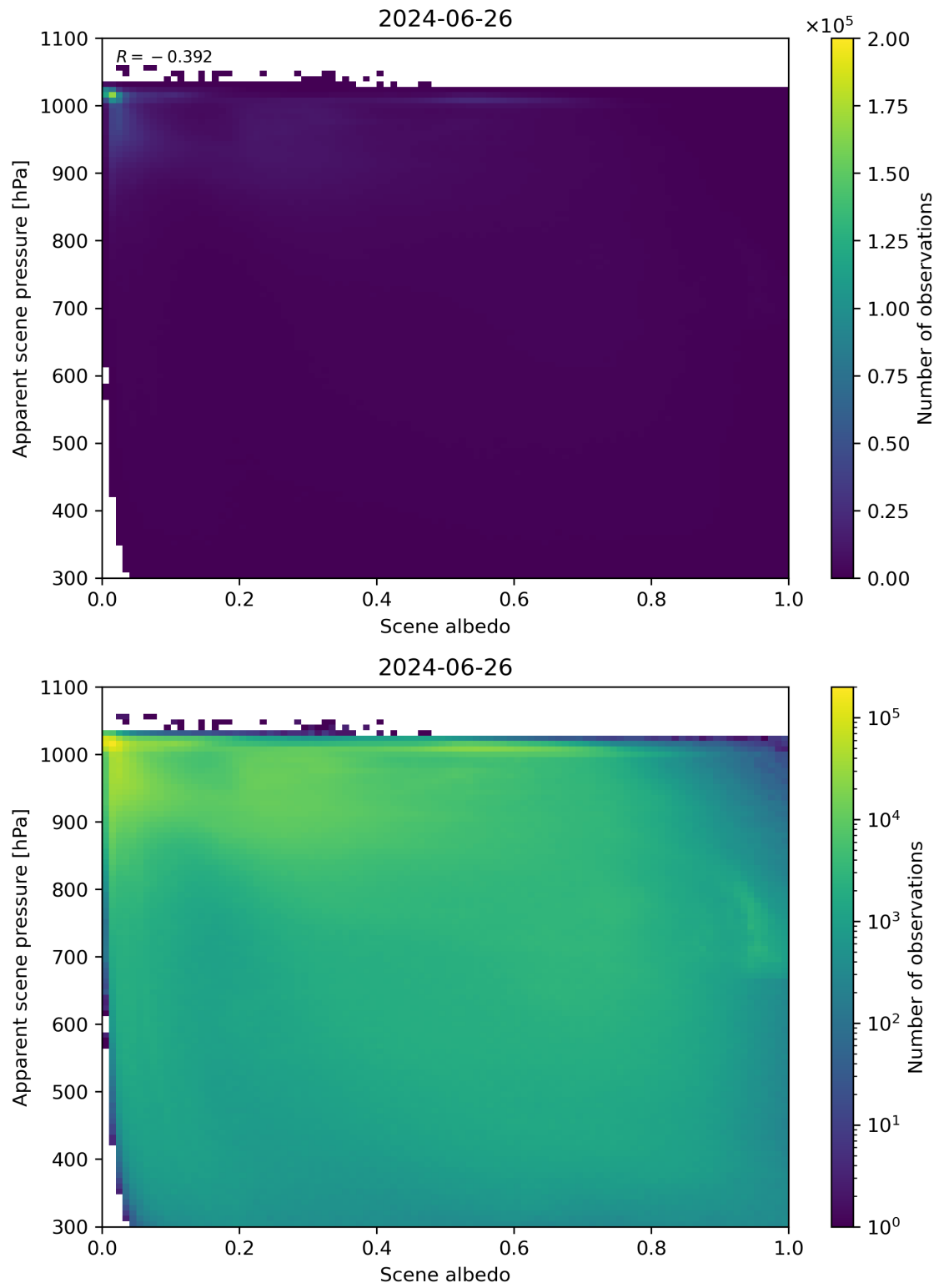
Figure 102: Scatter density plot of “Scene albedo” against “Apparent scene pressure” for 2024-06-25 to 2024-06-27.
