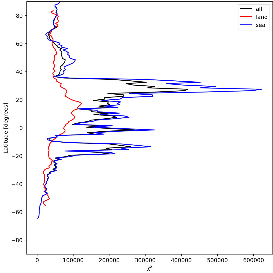
Figure 21: Zonal average of “ \chi^2 ” for 2024-06-25 to 2024-06-27.
