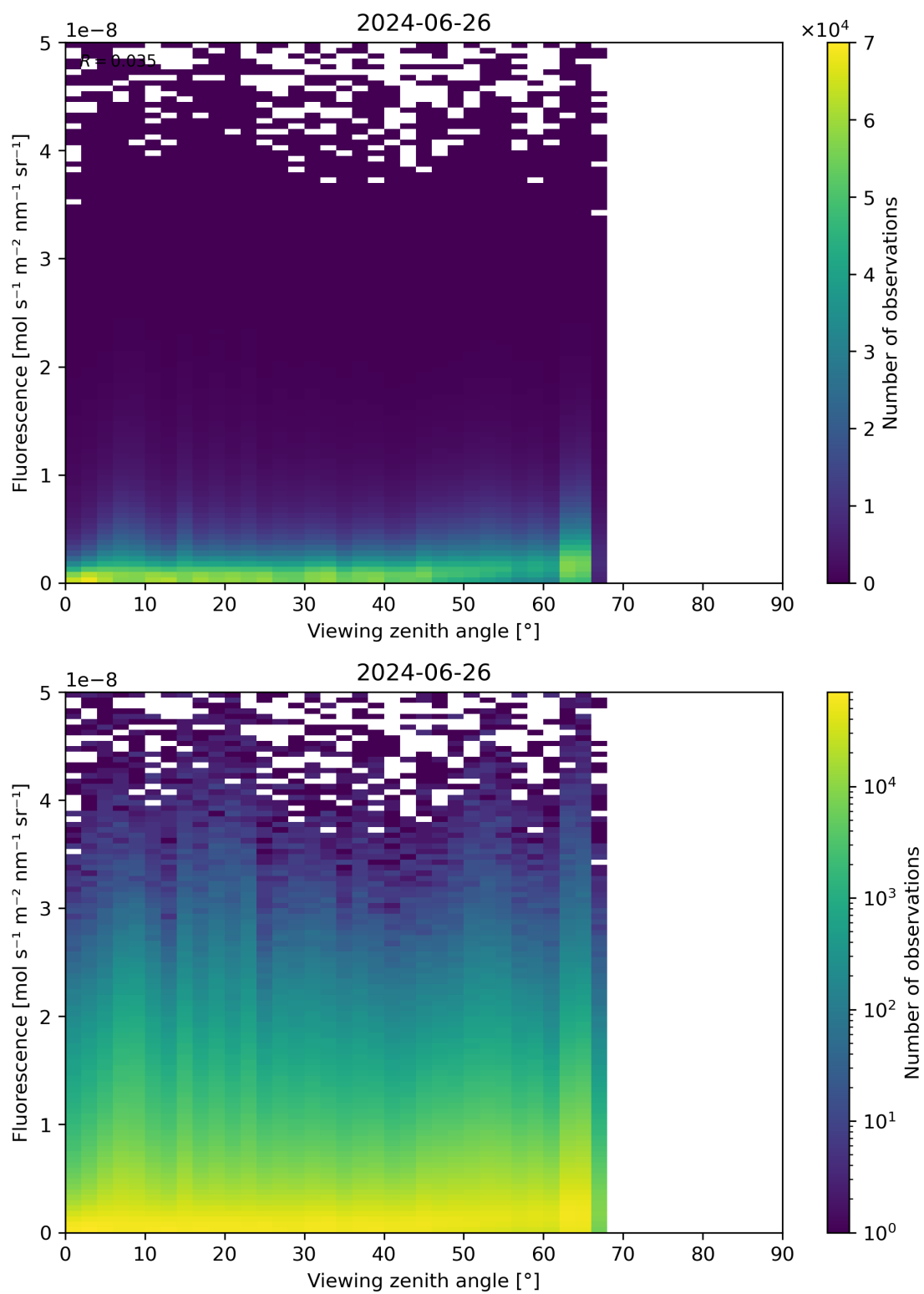
Figure 122: Scatter density plot of “Viewing zenith angle” against “Fluorescence” for 2024-06-25 to 2024-06-27.
