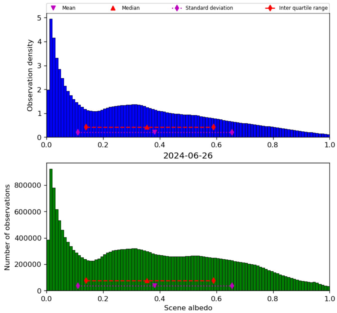
Figure 34: Histogram of “Scene albedo” for 2024-06-25 to 2024-06-27
