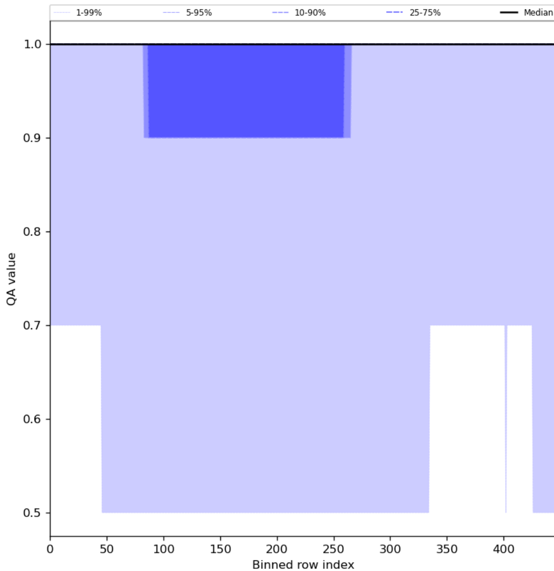
Figure 46: Along track statistics of “QA value” for 2024-06-25 to 2024-06-27
