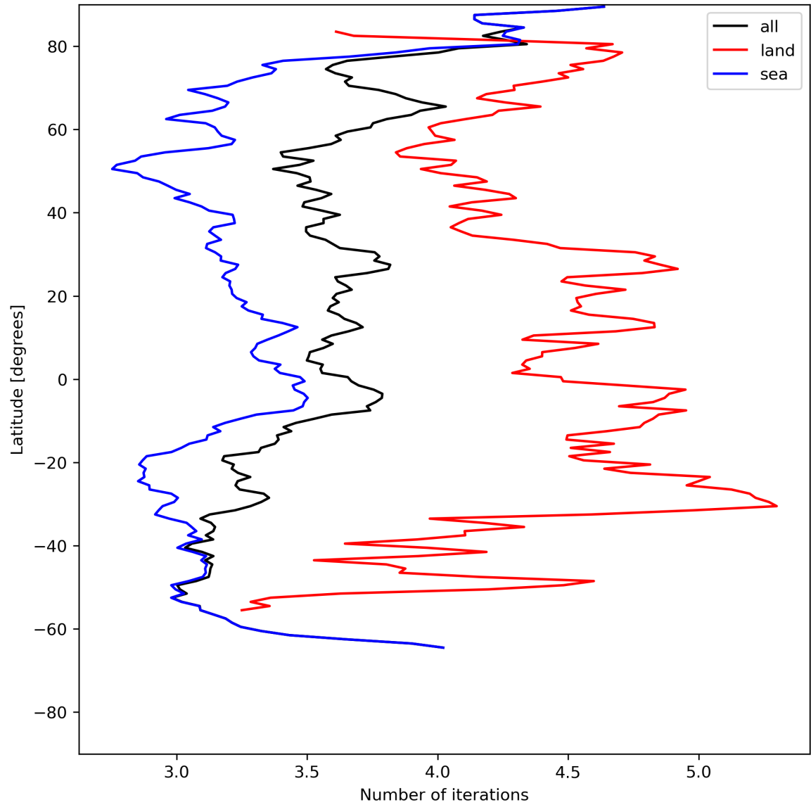
Figure 22: Zonal average of “Number of iterations” for 2024-06-25 to 2024-06-27.
