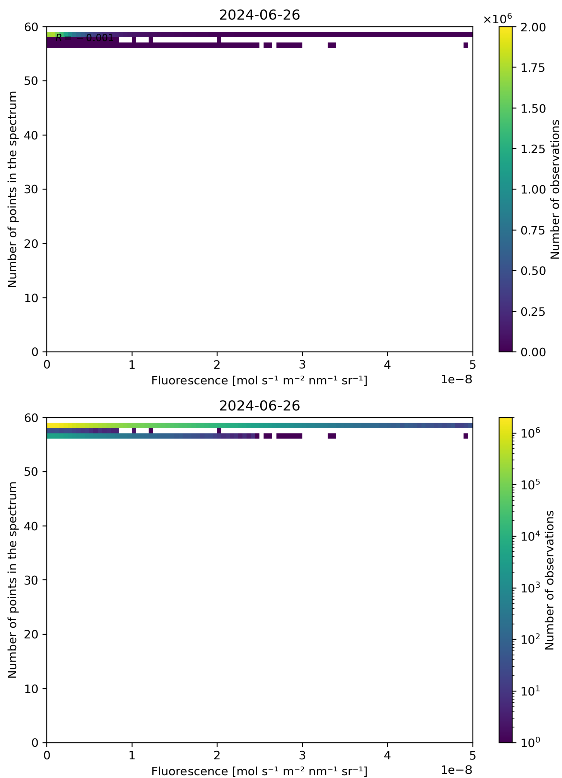
Figure 86: Scatter density plot of “Fluorescence” against “Number of points in the spectrum” for 2024-06-25 to 2024-06-27.
