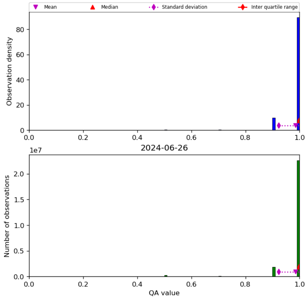
Figure 29: Histogram of “QA value” for 2024-06-25 to 2024-06-27
