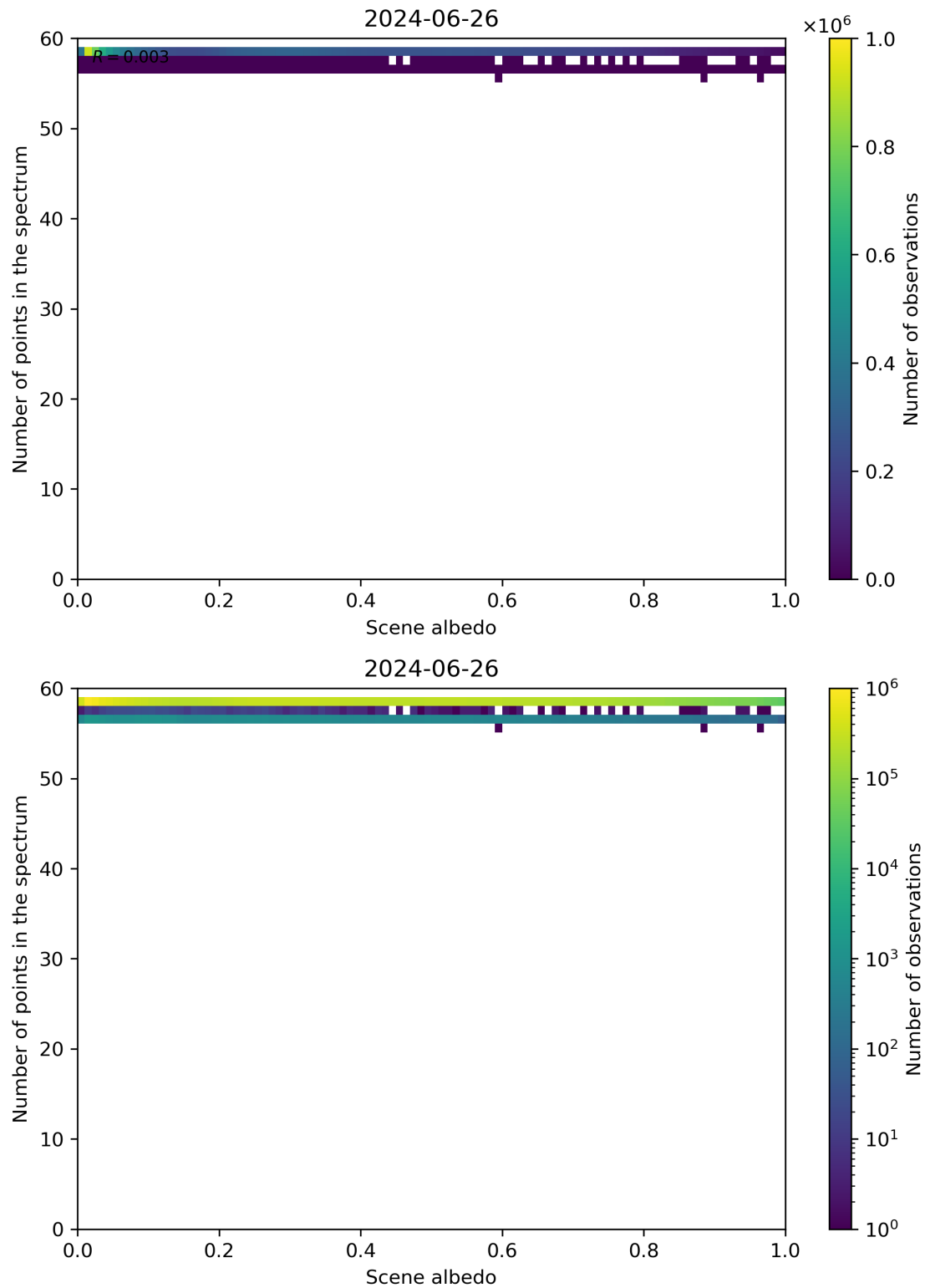
Figure 106: Scatter density plot of “Scene albedo” against “Number of points in the spectrum” for 2024-06-25 to 2024-06-27.
