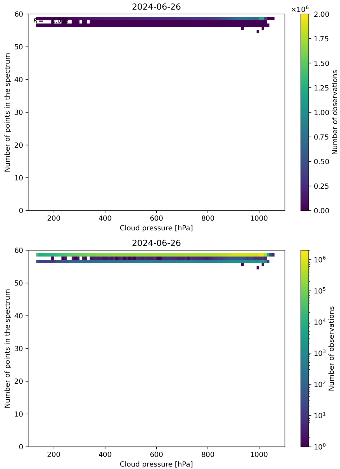
Figure 82: Scatter density plot of “Cloud pressure” against “Number of points in the spectrum” for 2024-06-25 to 2024-06-27.
