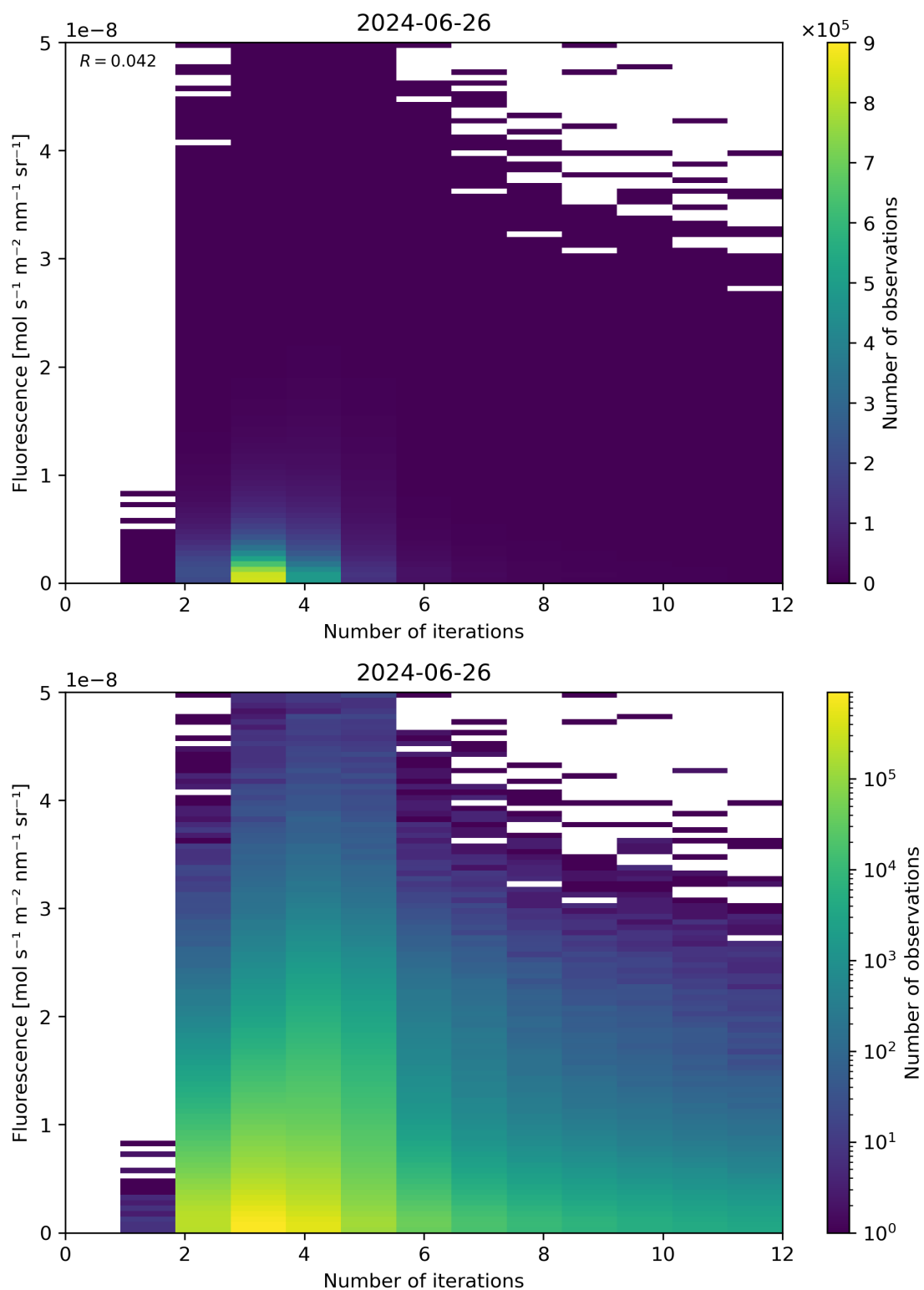
Figure 98: Scatter density plot of “Number of iterations” against “Fluorescence” for 2024-06-25 to 2024-06-27.
