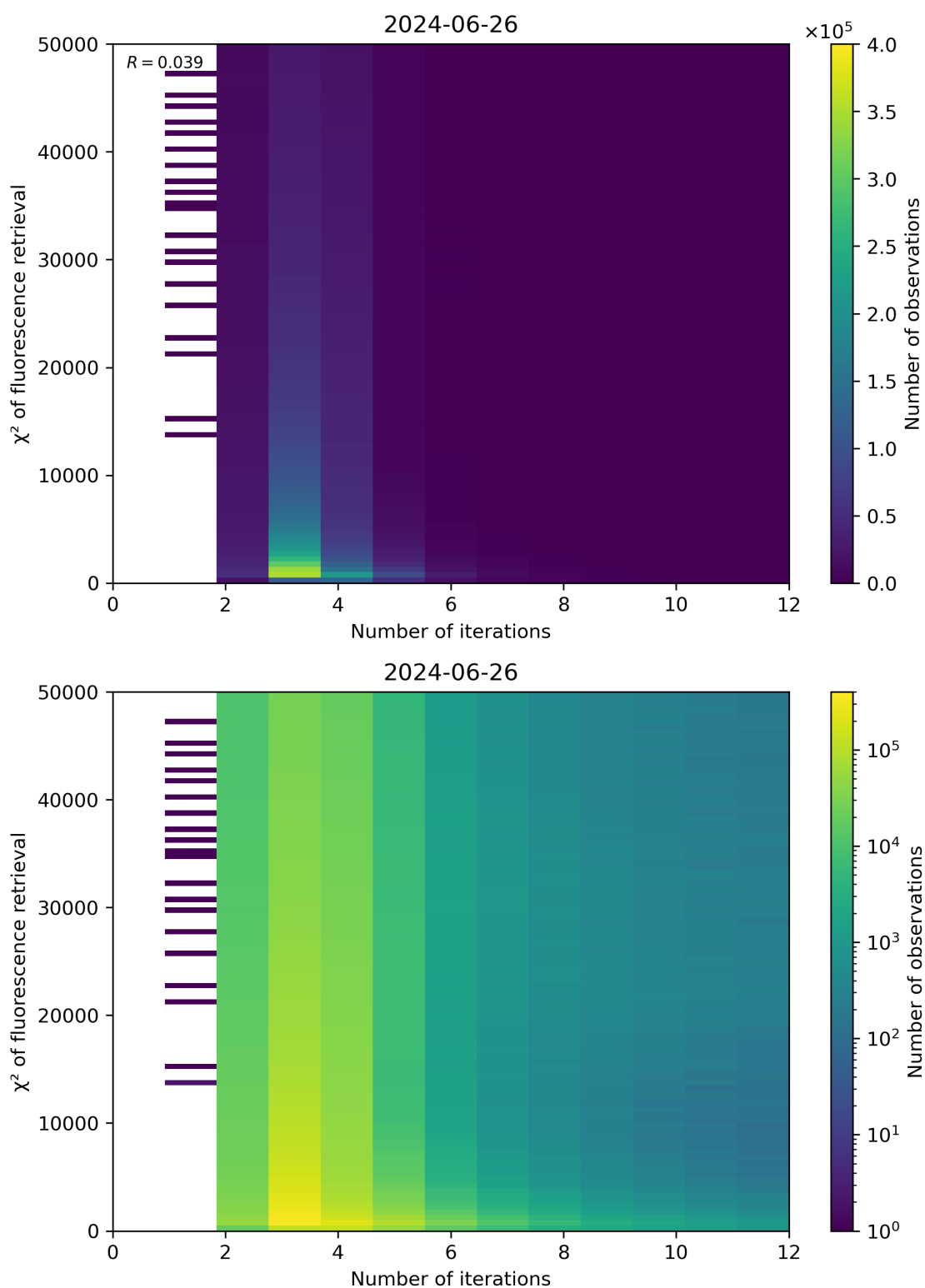
Figure 97: Scatter density plot of “Number of iterations” against “ \chi^2 of fluorescence retrieval” for 2024-06-25 to 2024-06-27.
