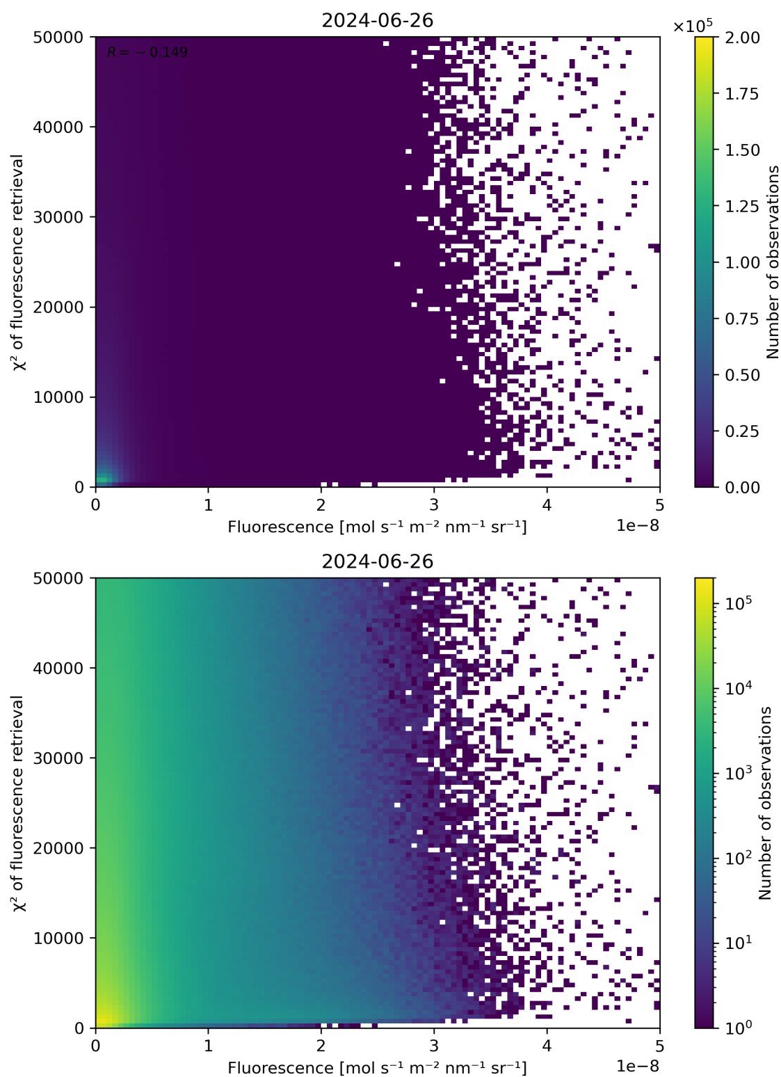
Figure 85: Scatter density plot of “Fluorescence” against “ \chi^2 of fluorescence retrieval” for 2024-06-25 to 2024-06-27.
