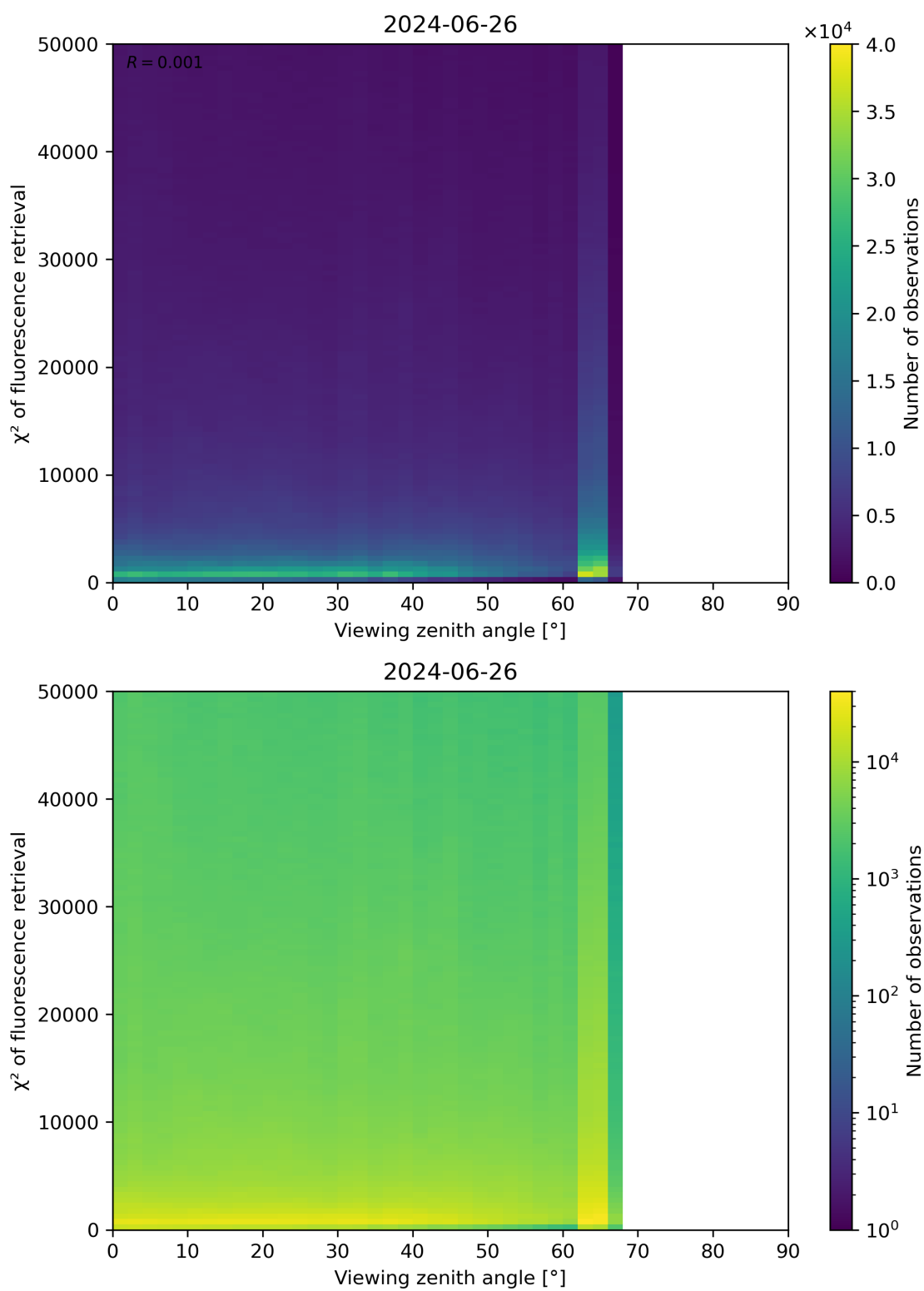
Figure 119: Scatter density plot of “Viewing zenith angle” against “ \chi^2 of fluorescence retrieval” for 2024-06-25 to 2024-06-27.
