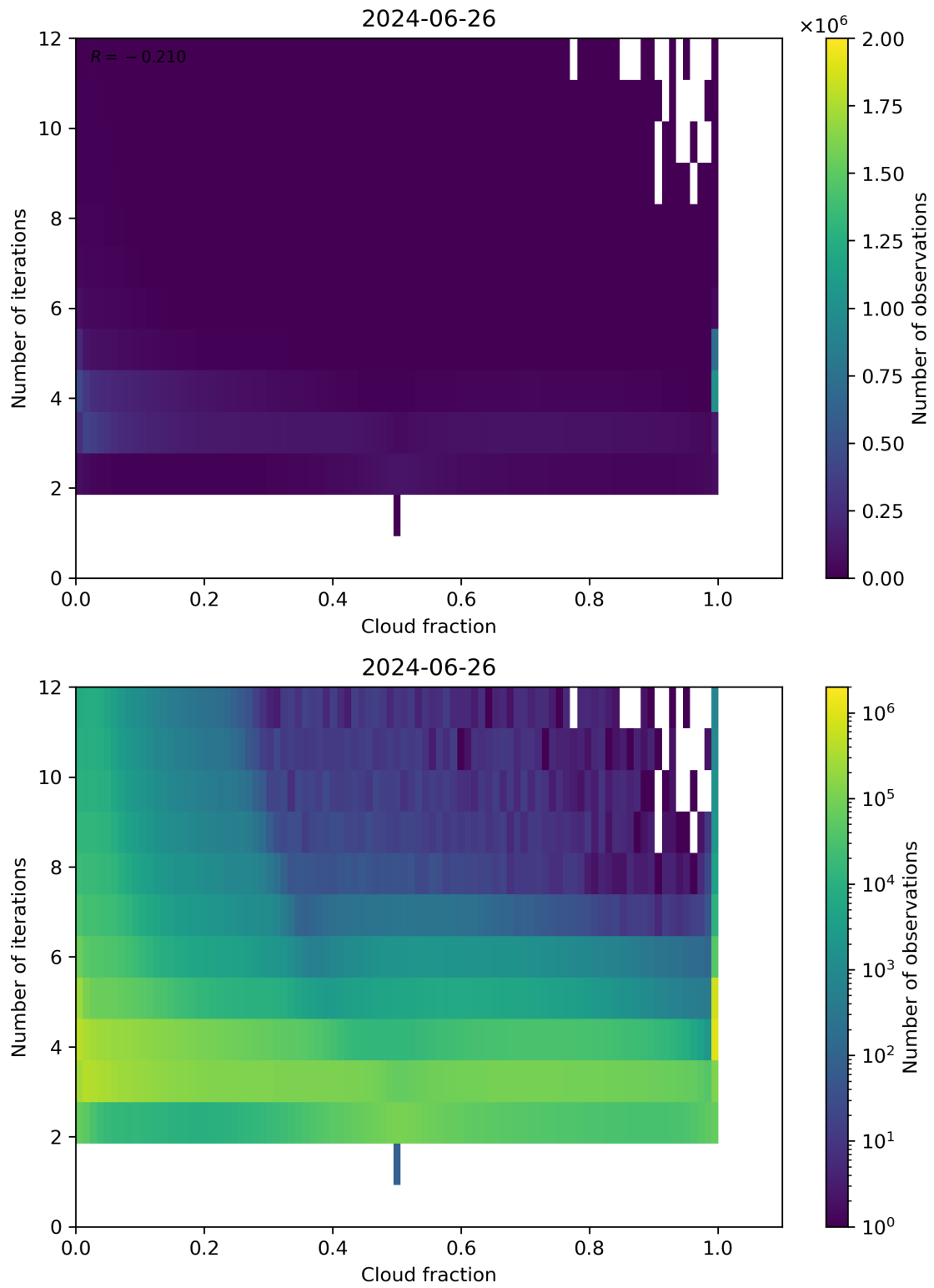
Figure 73: Scatter density plot of “Cloud fraction” against “Number of iterations” for 2024-06-25 to 2024-06-27.
