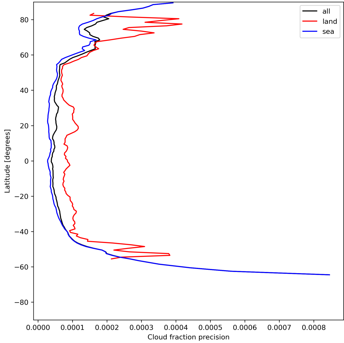
Figure 16: Zonal average of “Cloud fraction precision” for 2024-06-25 to 2024-06-27.
