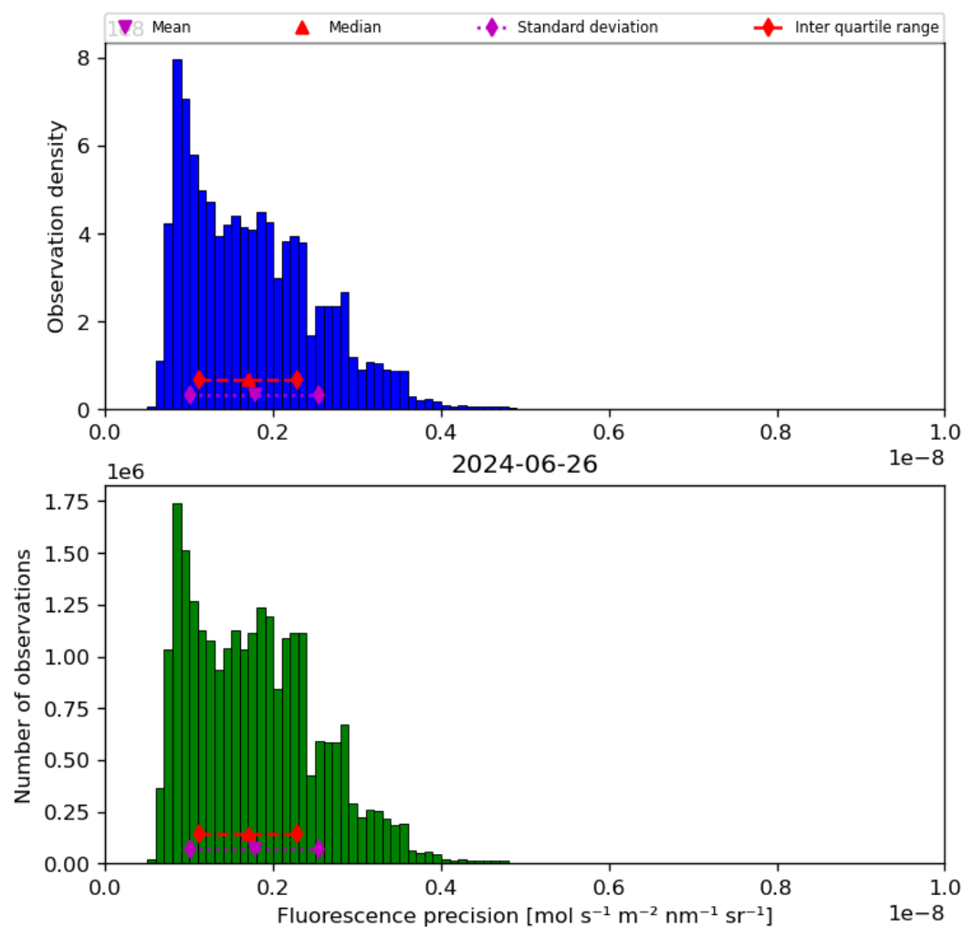
Figure 41: Histogram of “Fluorescence precision” for 2024-06-25 to 2024-06-27
