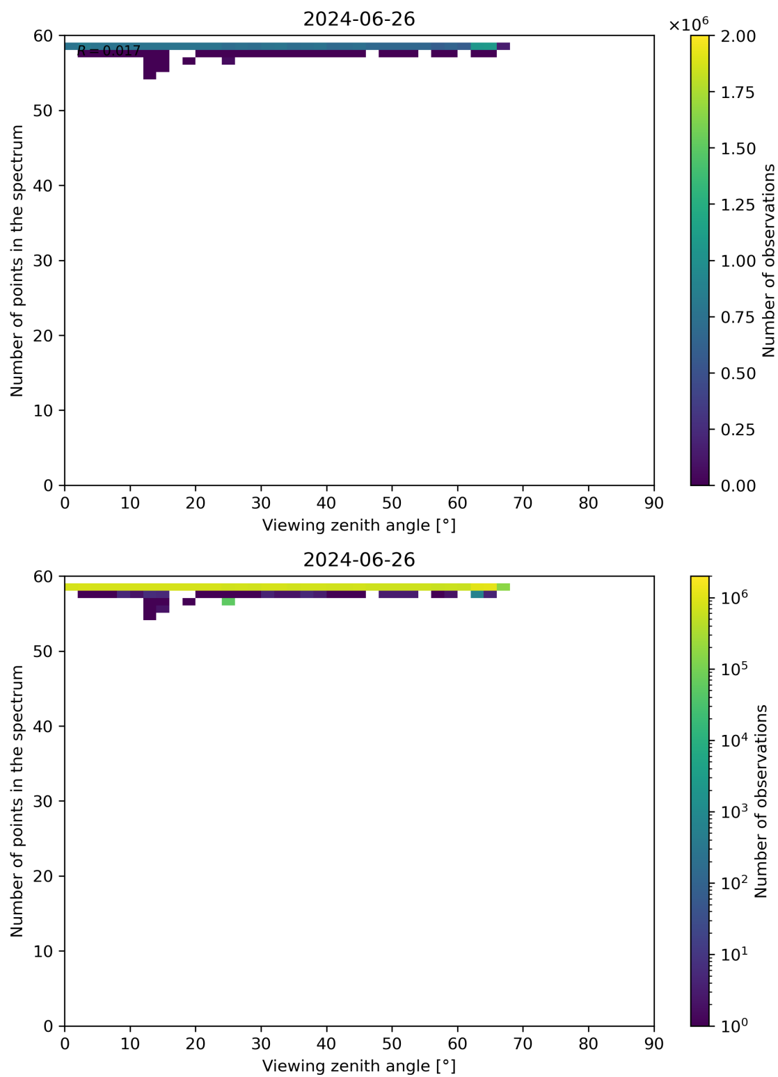
Figure 125: Scatter density plot of “Viewing zenith angle” against “Number of points in the spectrum” for 2024-06-25 to 2024-06-27.
