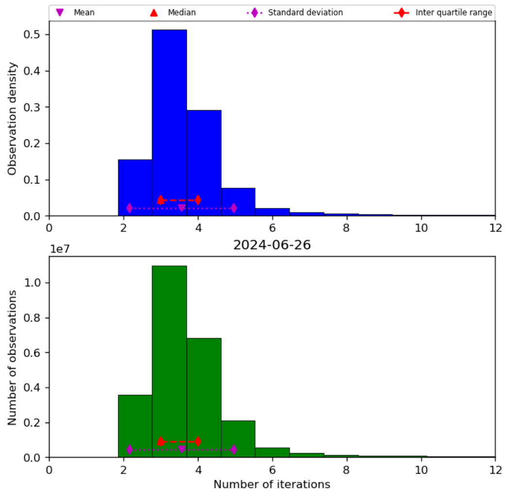
Figure 39: Histogram of “Number of iterations” for 2024-06-25 to 2024-06-27
