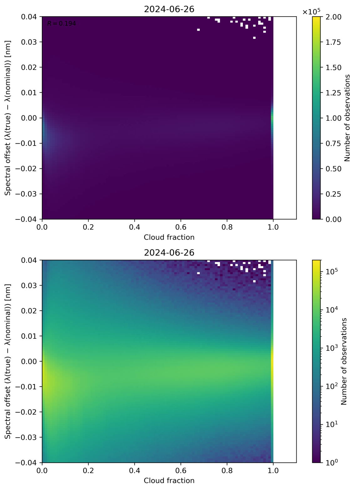
Figure 76: Scatter density plot of “Cloud fraction” against “Spectral offset ( \lambda(\text{true}) - \lambda(\text{nominal}) )” for 2024-06-25 to 2024-06-27.
