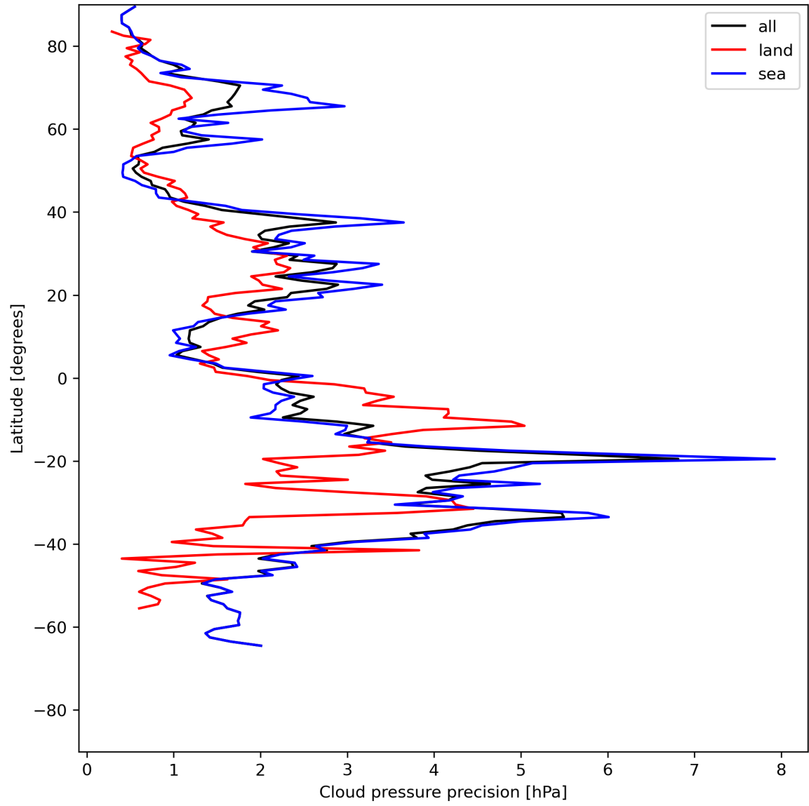
Figure 14: Zonal average of “Cloud pressure precision” for 2024-06-25 to 2024-06-27.
