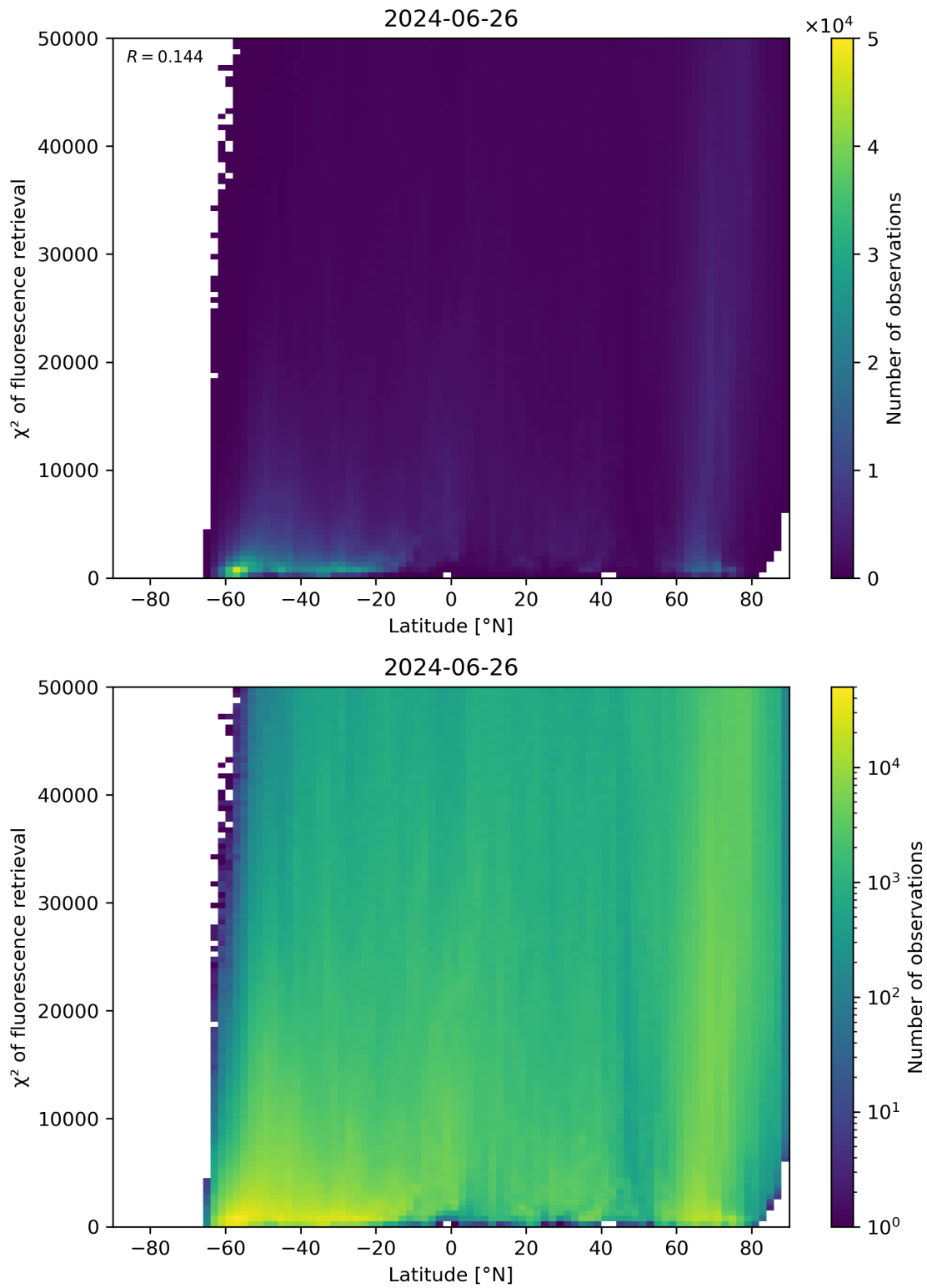
Figure 89: Scatter density plot of “Latitude” against “ \chi^2 of fluorescence retrieval” for 2024-06-25 to 2024-06-27.
