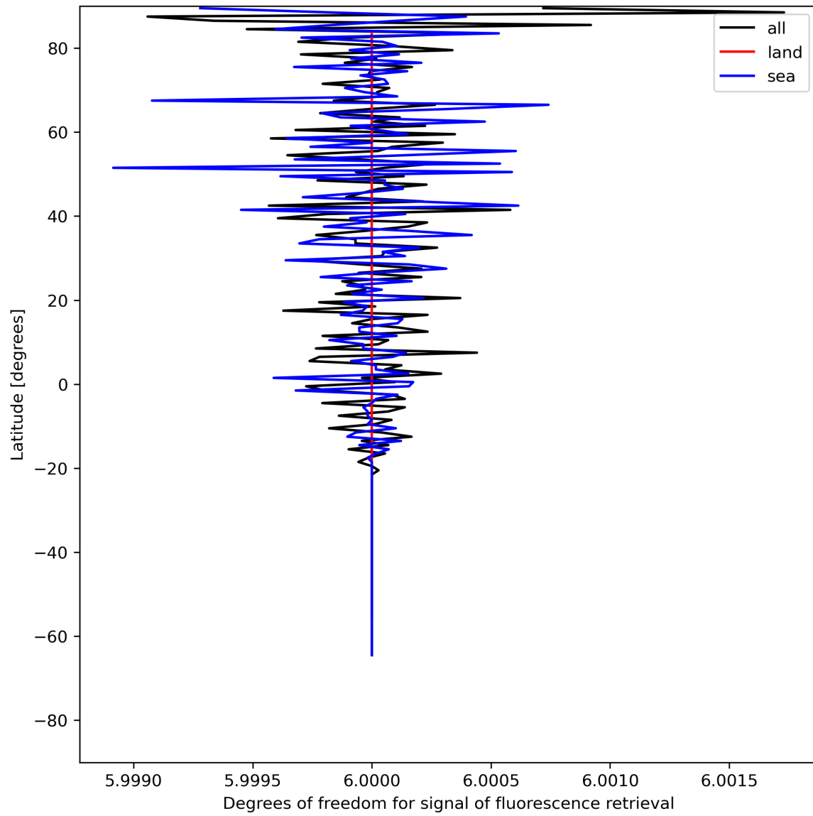
Figure 26: Zonal average of “Degrees of freedom for signal of fluorescence retrieval” for 2024-06-25 to 2024-06-27.
