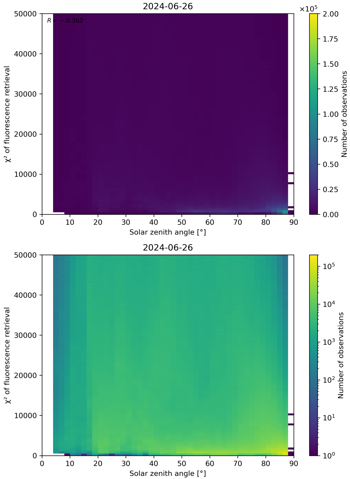
Figure 109: Scatter density plot of “Solar zenith angle” against “ \chi^2 of fluorescence retrieval” for 2024-06-25 to 2024-06-27.
