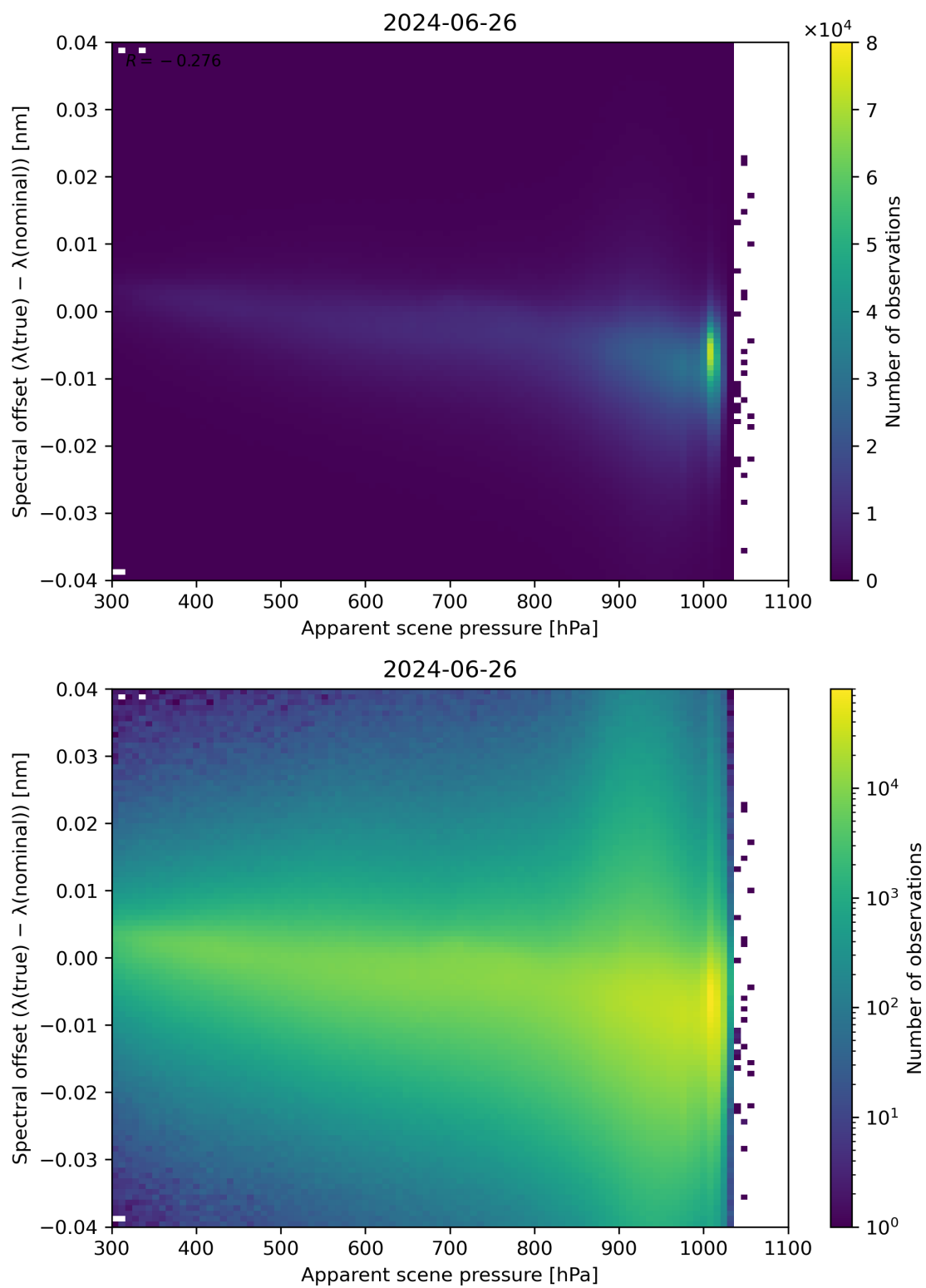
Figure 67: Scatter density plot of “Apparent scene pressure” against “Spectral offset ( \lambda(\text{true}) - \lambda(\text{nominal}) )” for 2024-06-25 to 2024-06-27.
