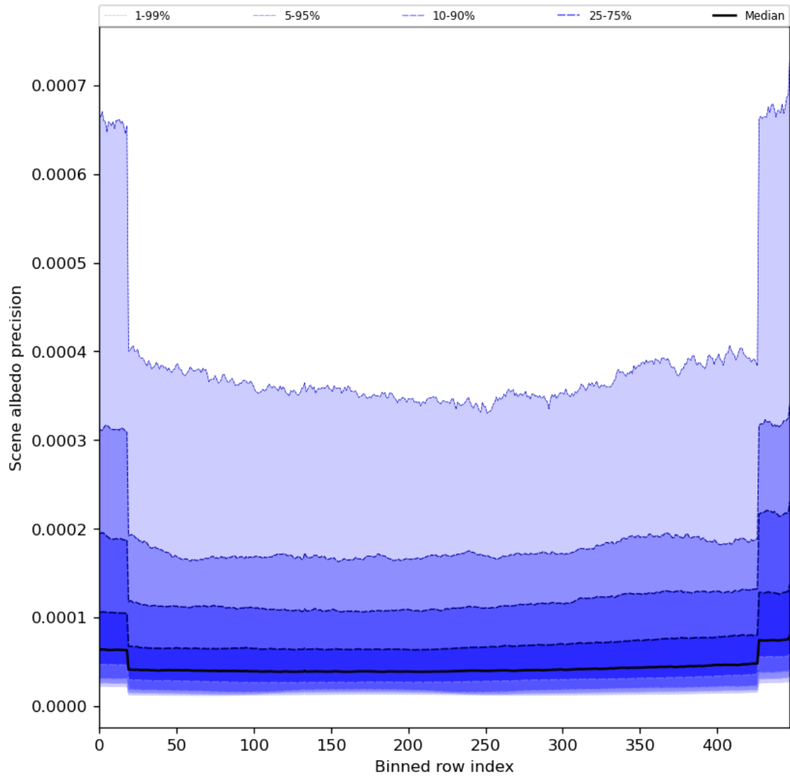
Figure 52: Along track statistics of “Scene albedo precision” for 2024-06-25 to 2024-06-27
