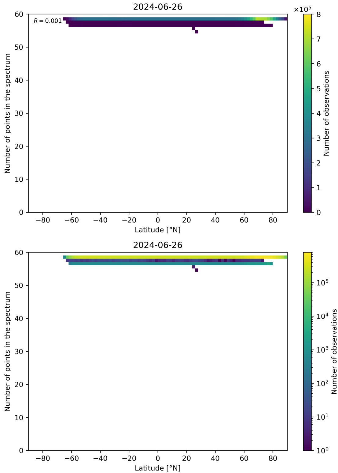
Figure 94: Scatter density plot of “Latitude” against “Number of points in the spectrum” for 2024-06-25 to 2024-06-27.
