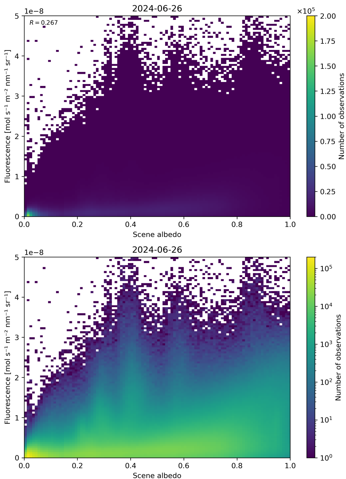
Figure 104: Scatter density plot of “Scene albedo” against “Fluorescence” for 2024-06-25 to 2024-06-27.
