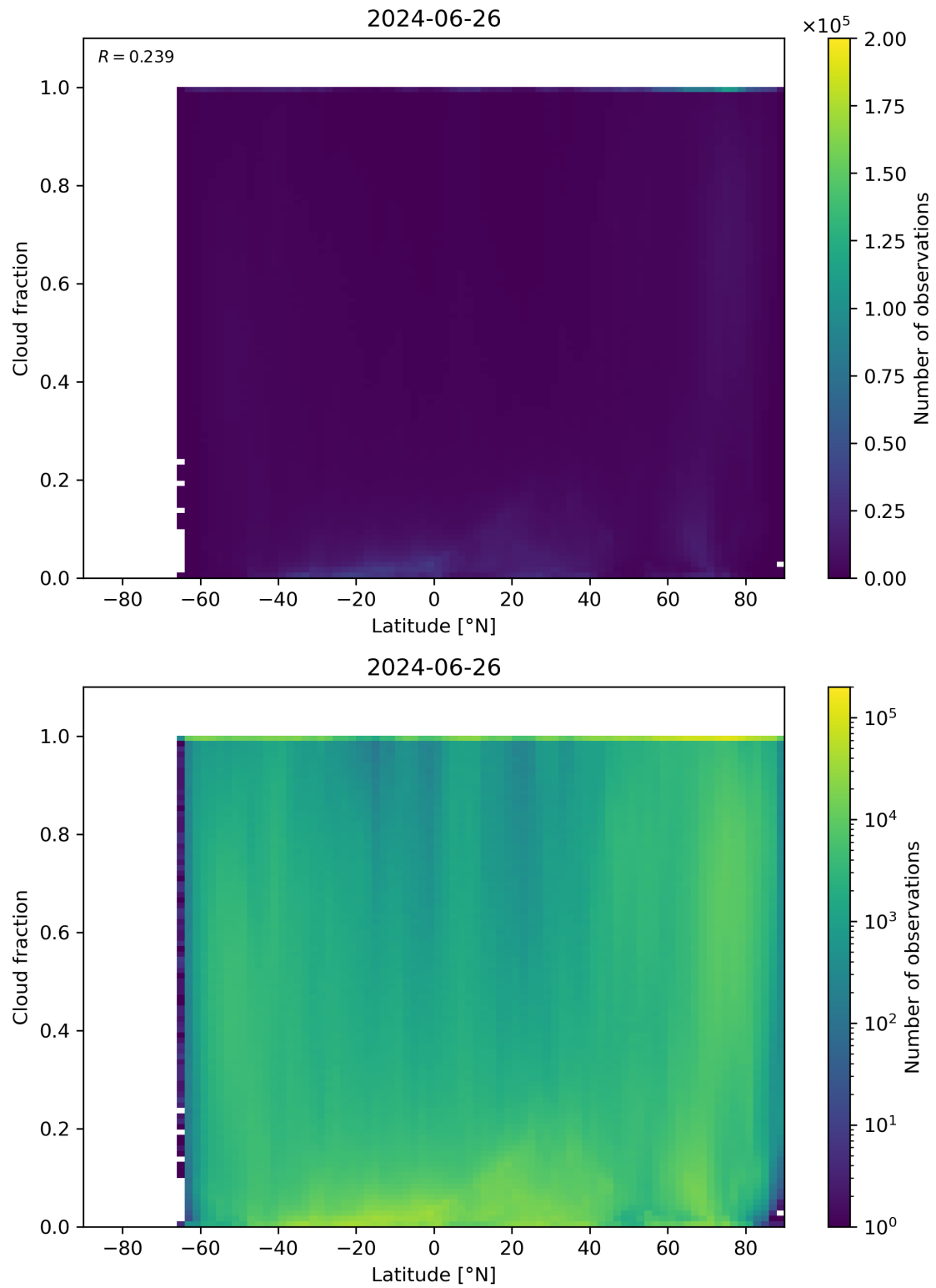
Figure 90: Scatter density plot of “Latitude” against “Cloud fraction” for 2024-06-25 to 2024-06-27.
