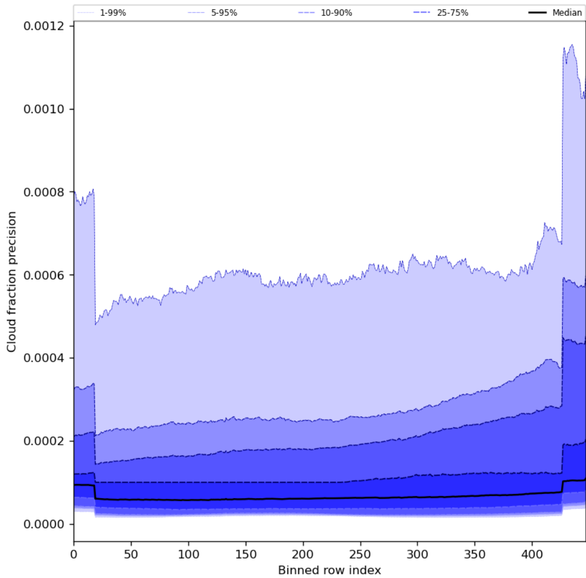
Figure 50: Along track statistics of “Cloud fraction precision” for 2024-06-25 to 2024-06-27
