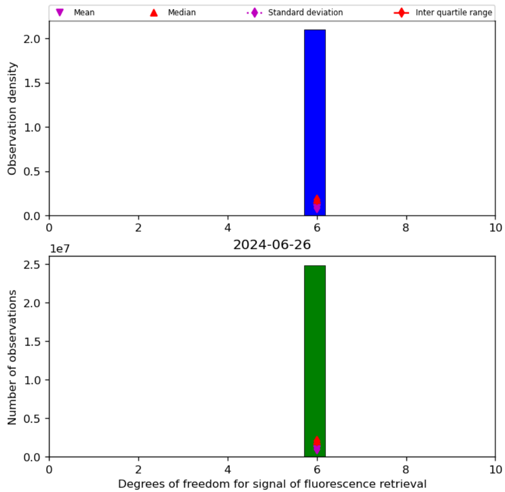
Figure 43: Histogram of “Degrees of freedom for signal of fluorescence retrieval” for 2024-06-25 to 2024-06-27
