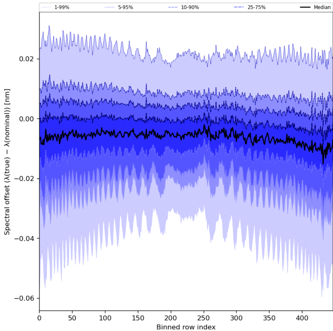
Figure 62: Along track statistics of “Spectral offset ( \lambda(\text{true}) - \lambda(\text{nominal}) )” for 2024-06-25 to 2024-06-27
