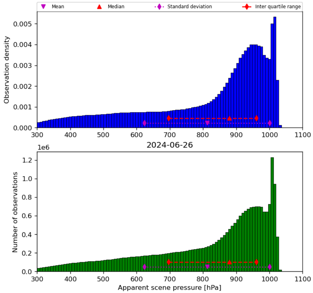
Figure 36: Histogram of “Apparent scene pressure” for 2024-06-25 to 2024-06-27
