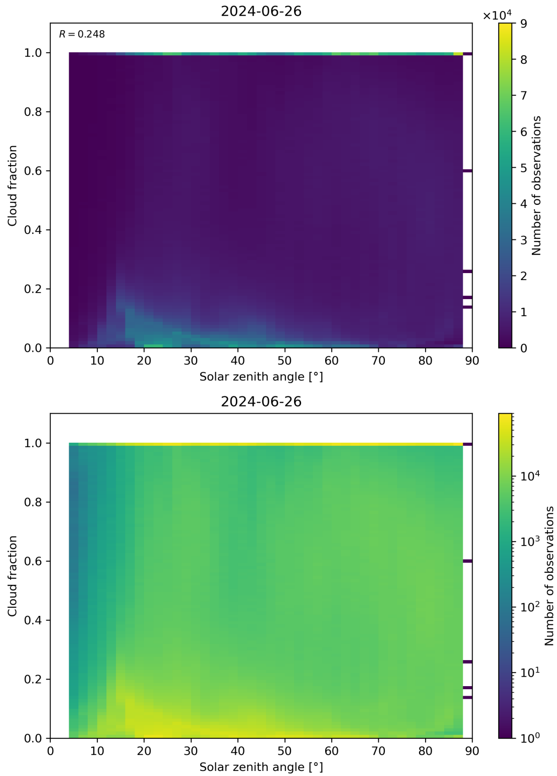
Figure 110: Scatter density plot of “Solar zenith angle” against “Cloud fraction” for 2024-06-25 to 2024-06-27.
