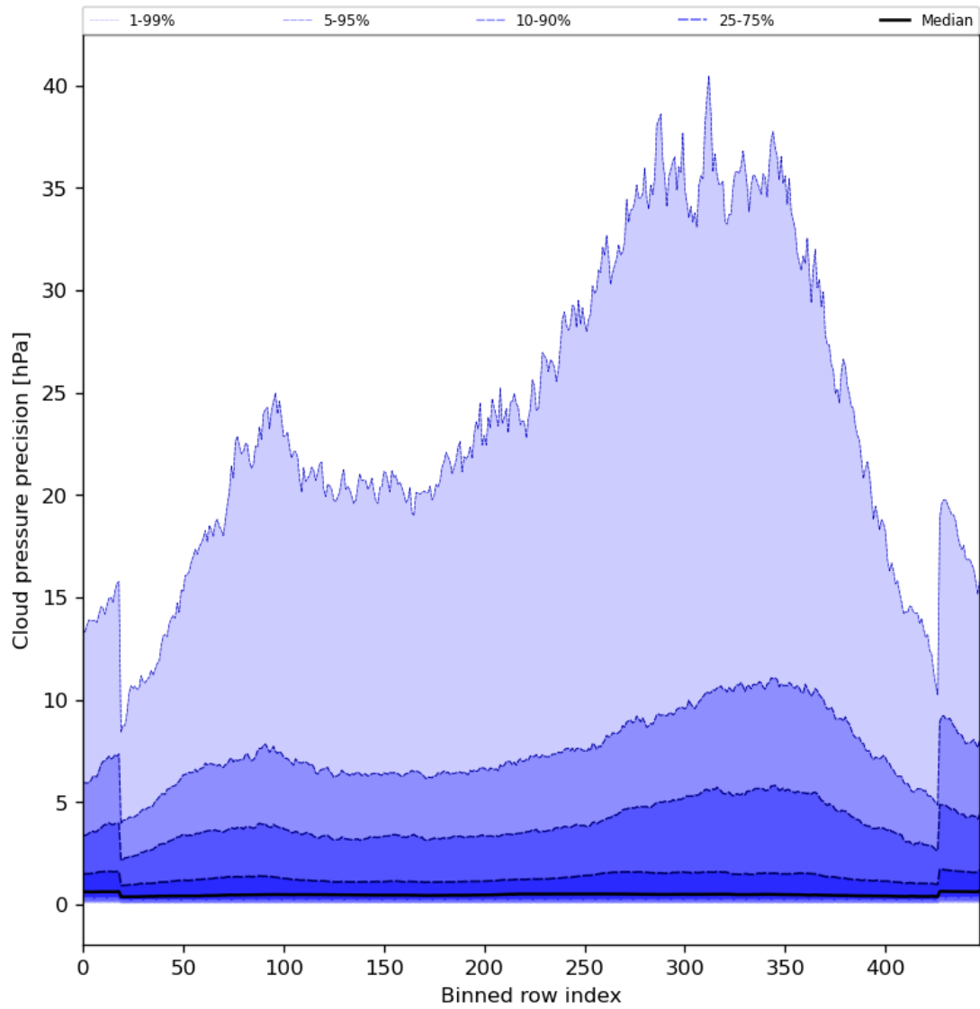
Figure 48: Along track statistics of “Cloud pressure precision” for 2024-06-25 to 2024-06-27
