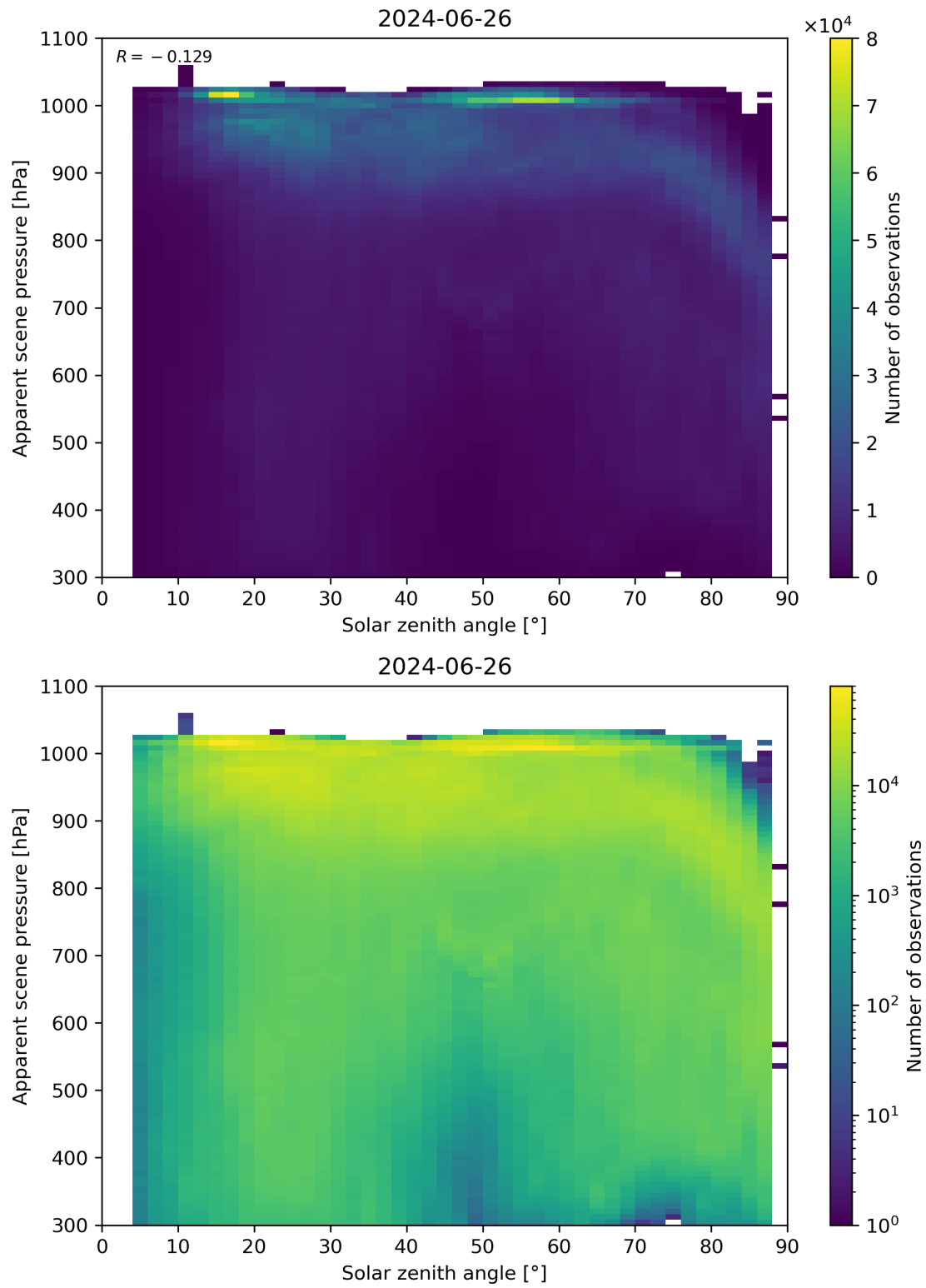
Figure 108: Scatter density plot of “Solar zenith angle” against “Apparent scene pressure” for 2024-06-25 to 2024-06-27.
