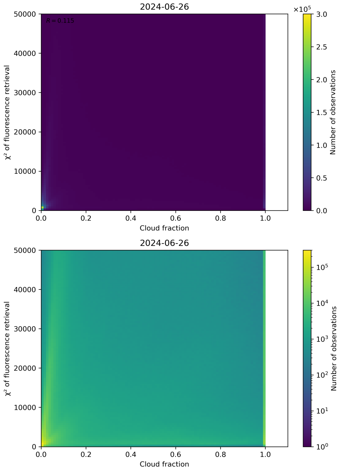
Figure 71: Scatter density plot of “Cloud fraction” against “ \chi^2 of fluorescence retrieval” for 2024-06-25 to 2024-06-27.
