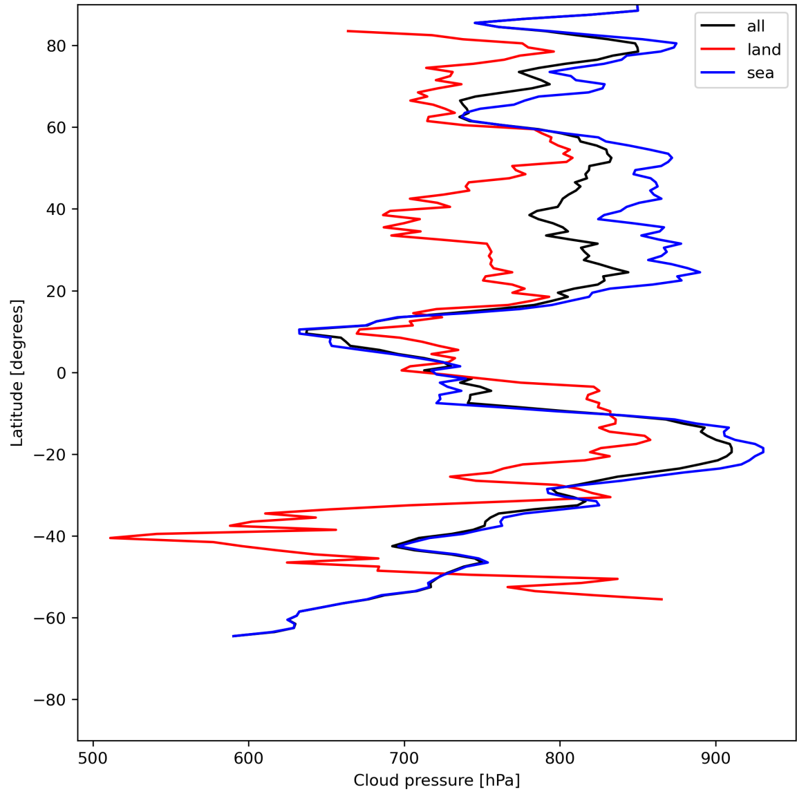
Figure 13: Zonal average of “Cloud pressure” for 2024-06-25 to 2024-06-27.
