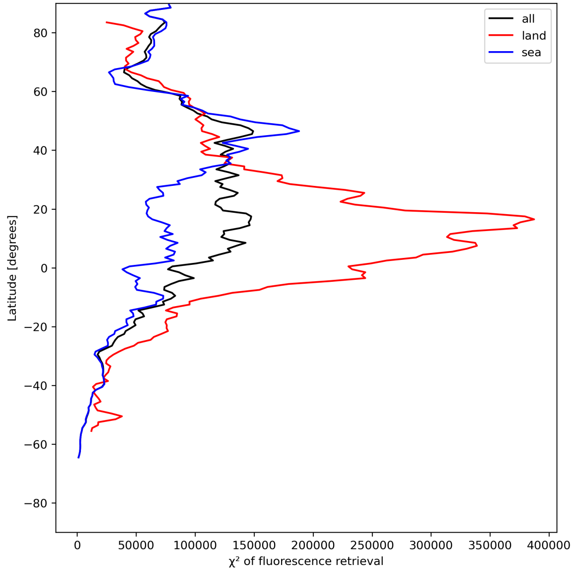
Figure 25: Zonal average of “ \chi^2 of fluorescence retrieval” for 2024-06-25 to 2024-06-27.
