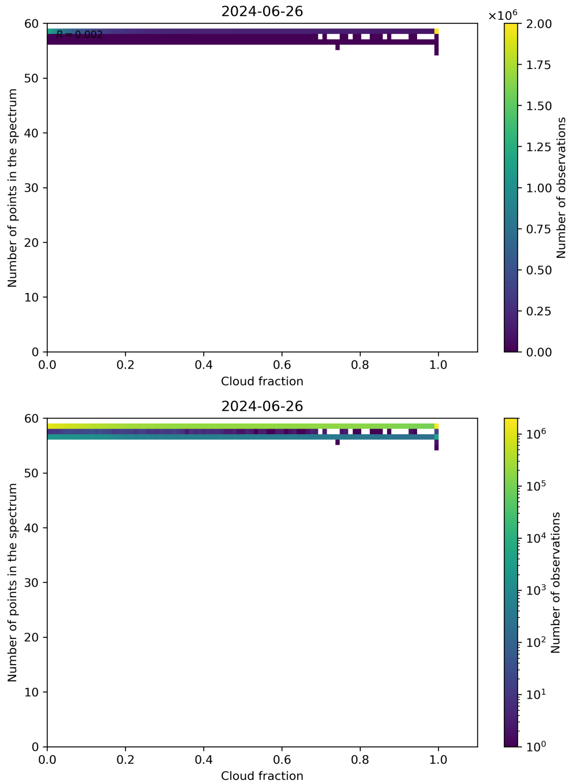
Figure 74: Scatter density plot of “Cloud fraction” against “Number of points in the spectrum” for 2024-06-25 to 2024-06-27.
