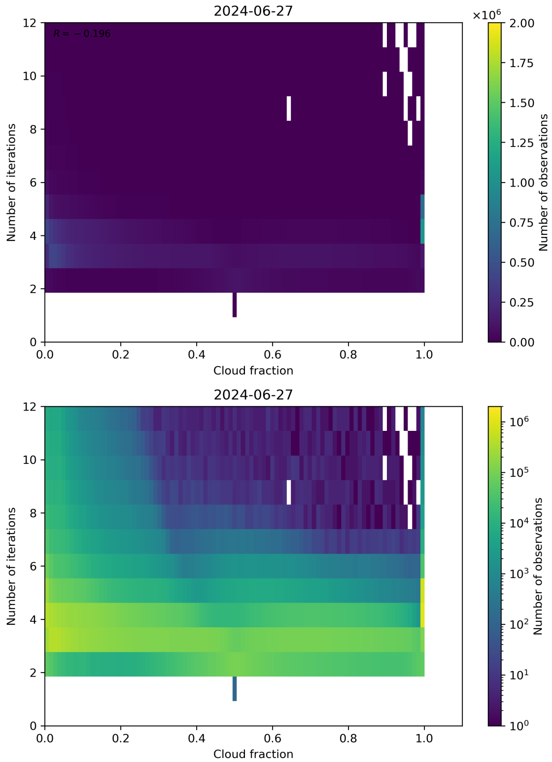
Figure 73: Scatter density plot of “Cloud fraction” against “Number of iterations” for 2024-06-26 to 2024-06-28.
