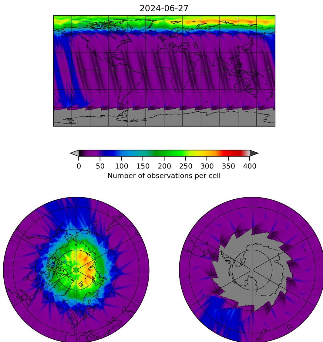
Figure 11: Map of the number of observations for 2024-06-26 to 2024-06-28
