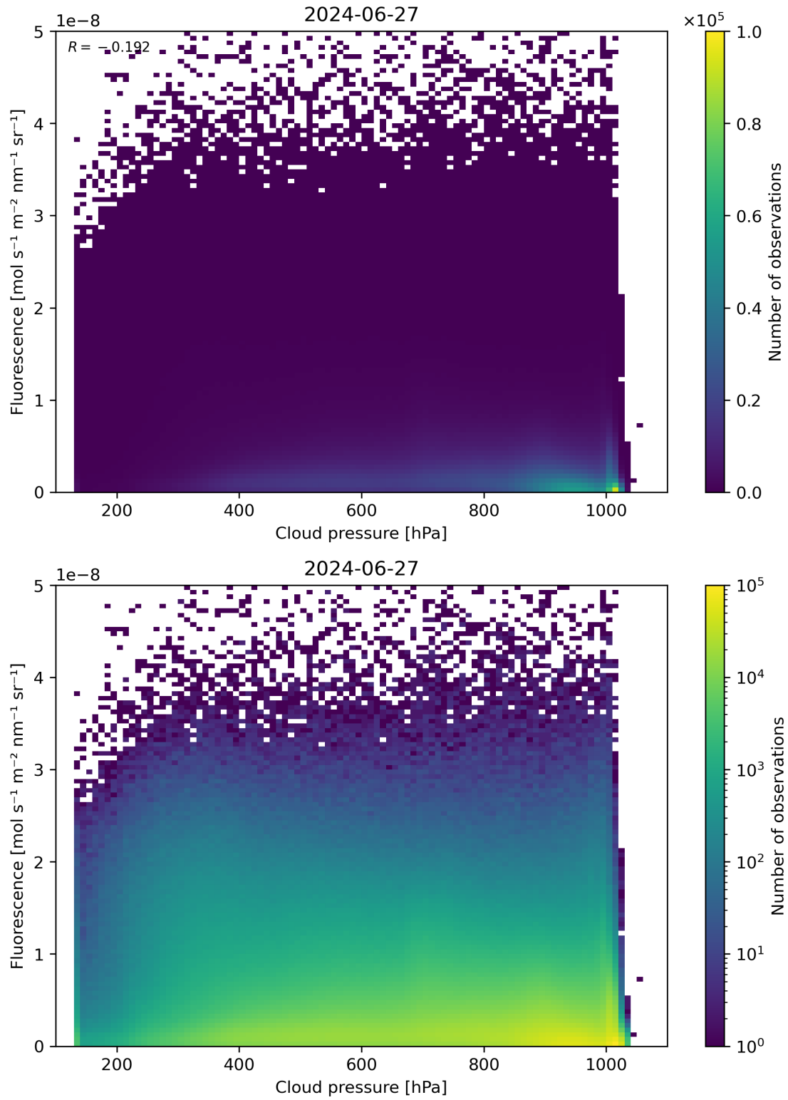
Figure 80: Scatter density plot of “Cloud pressure” against “Fluorescence” for 2024-06-26 to 2024-06-28.
