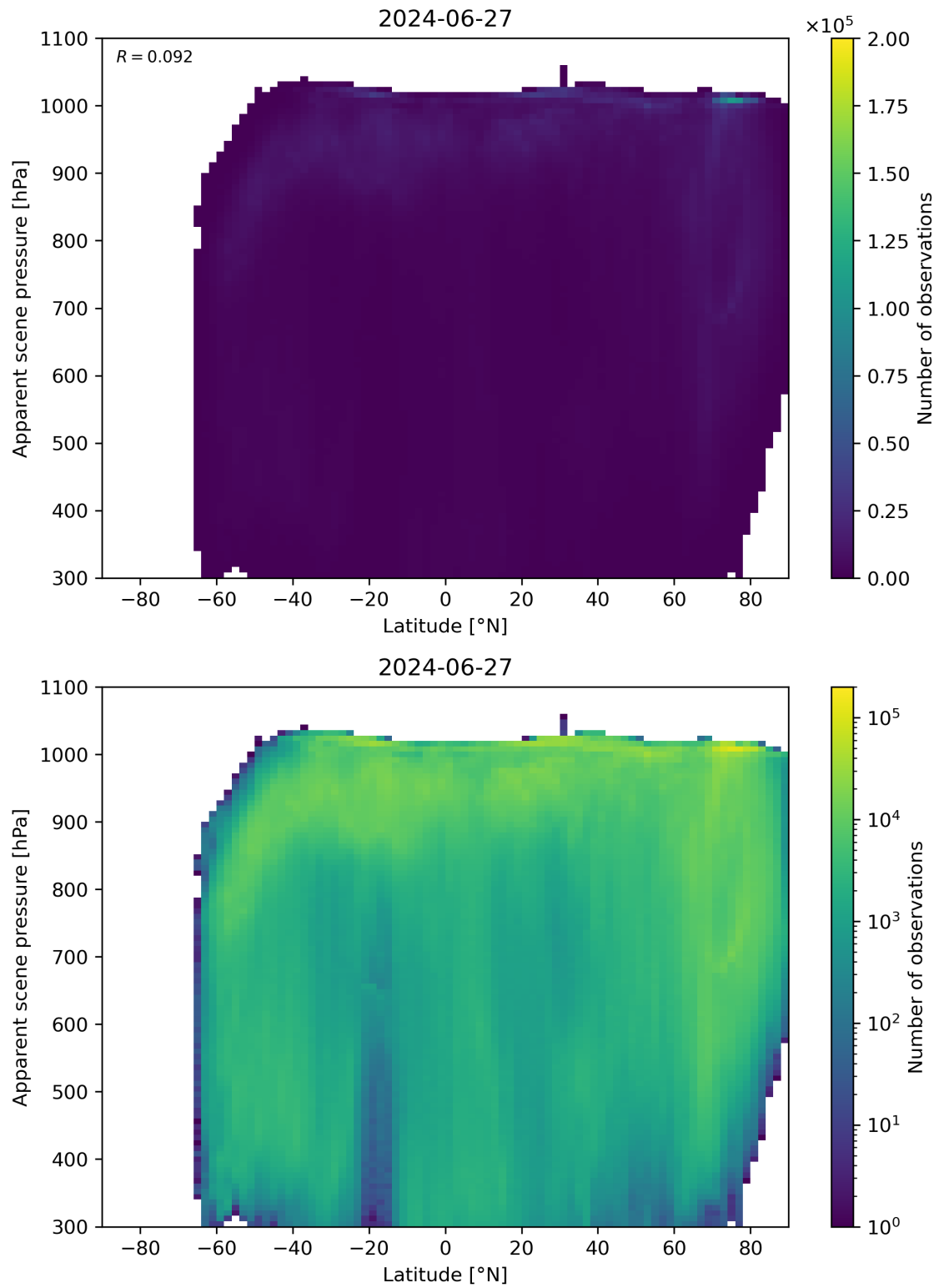
Figure 88: Scatter density plot of “Latitude” against “Apparent scene pressure” for 2024-06-26 to 2024-06-28.
