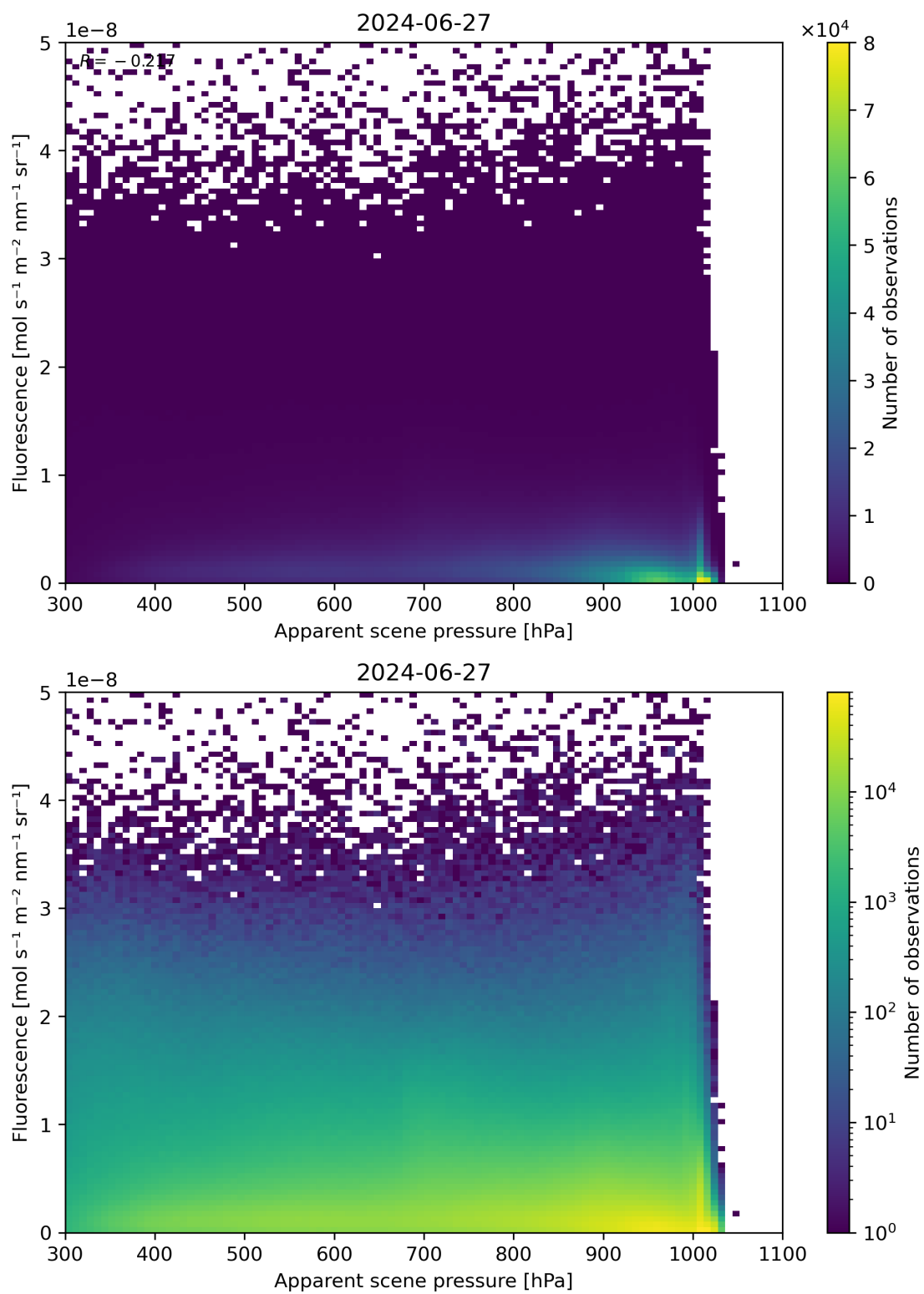
Figure 64: Scatter density plot of “Apparent scene pressure” against “Fluorescence” for 2024-06-26 to 2024-06-28.
