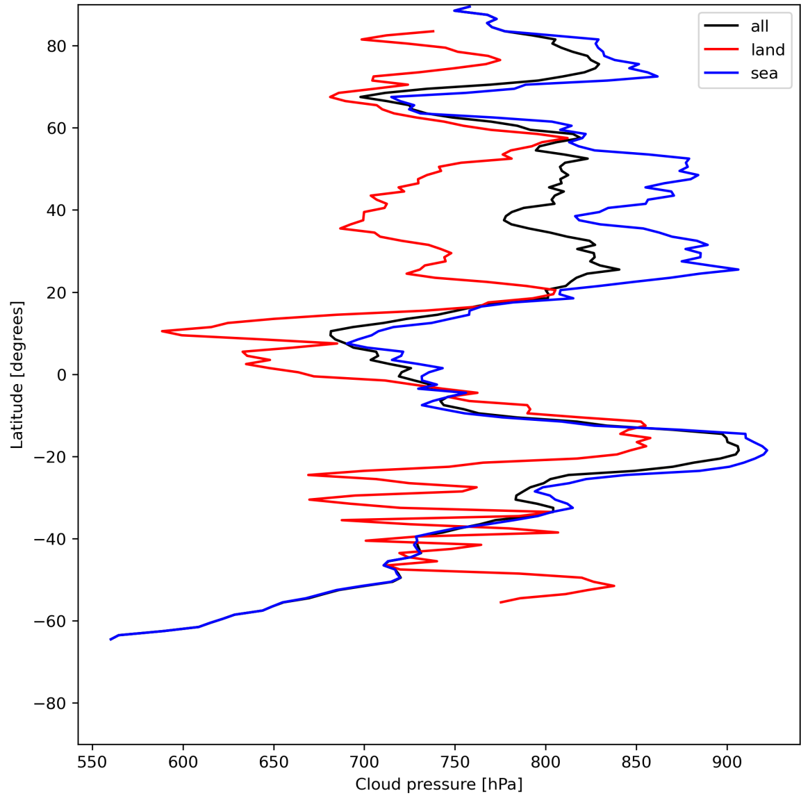
Figure 13: Zonal average of “Cloud pressure” for 2024-06-26 to 2024-06-28.
