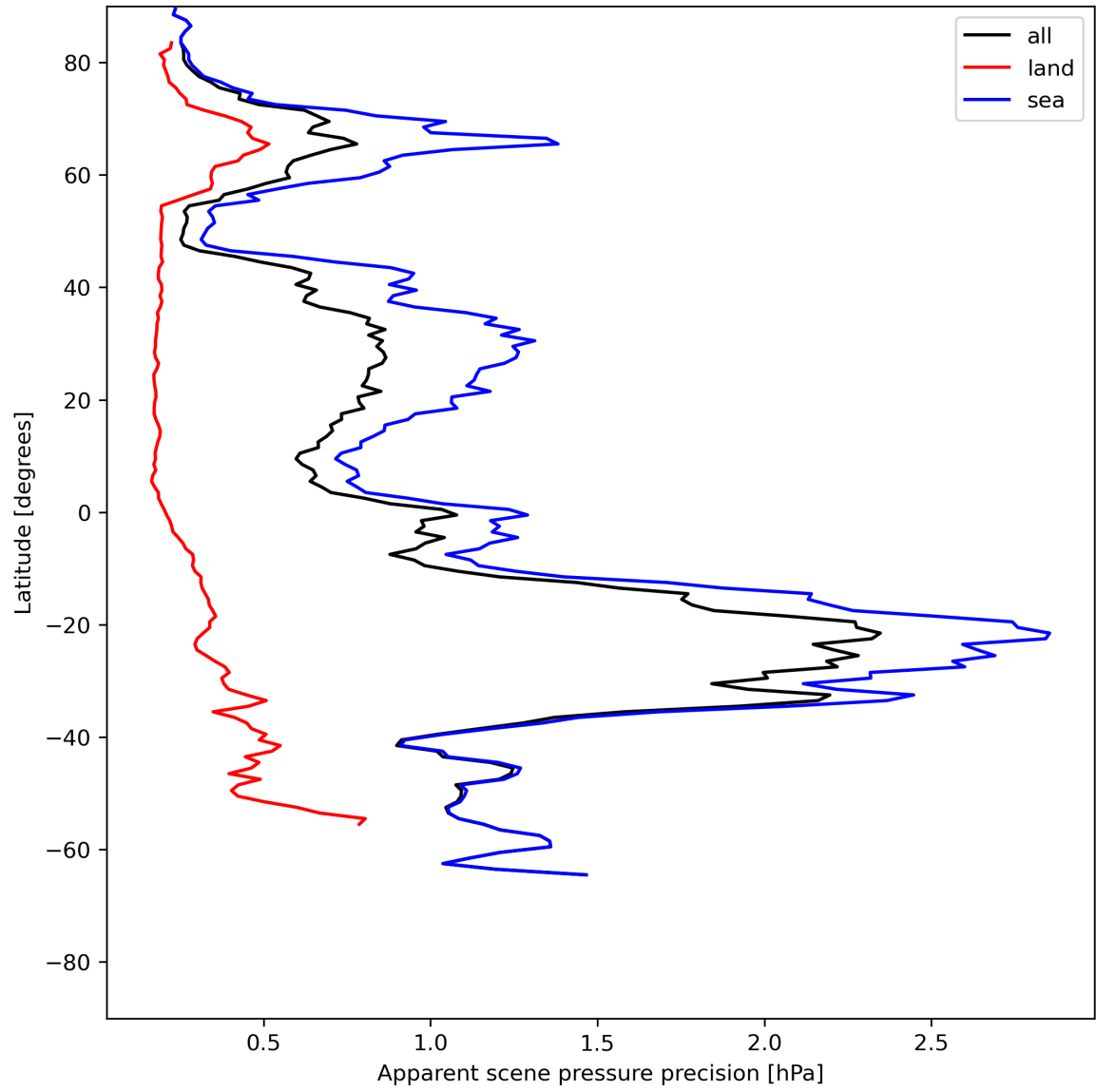
Figure 20: Zonal average of “Apparent scene pressure precision” for 2024-06-26 to 2024-06-28.
