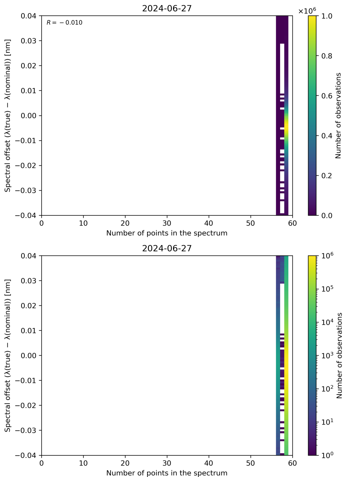
Figure 101: Scatter density plot of “Number of points in the spectrum” against “Spectral offset ( \lambda(\text{true}) - \lambda(\text{nominal}) )” for 2024-06-26 to 2024-06-28.
