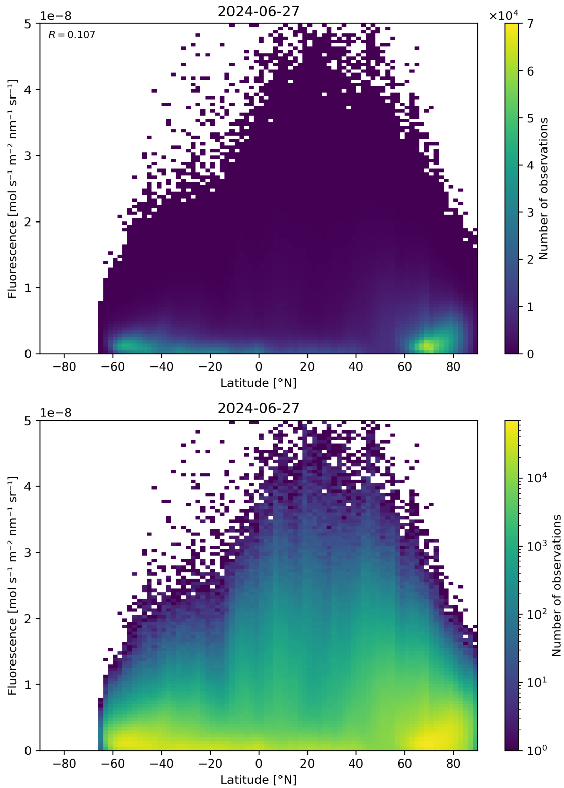
Figure 92: Scatter density plot of “Latitude” against “Fluorescence” for 2024-06-26 to 2024-06-28.
