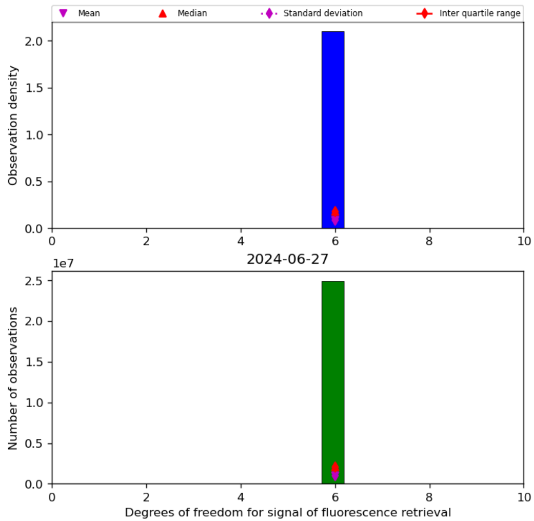
Figure 43: Histogram of “Degrees of freedom for signal of fluorescence retrieval” for 2024-06-26 to 2024-06-28
