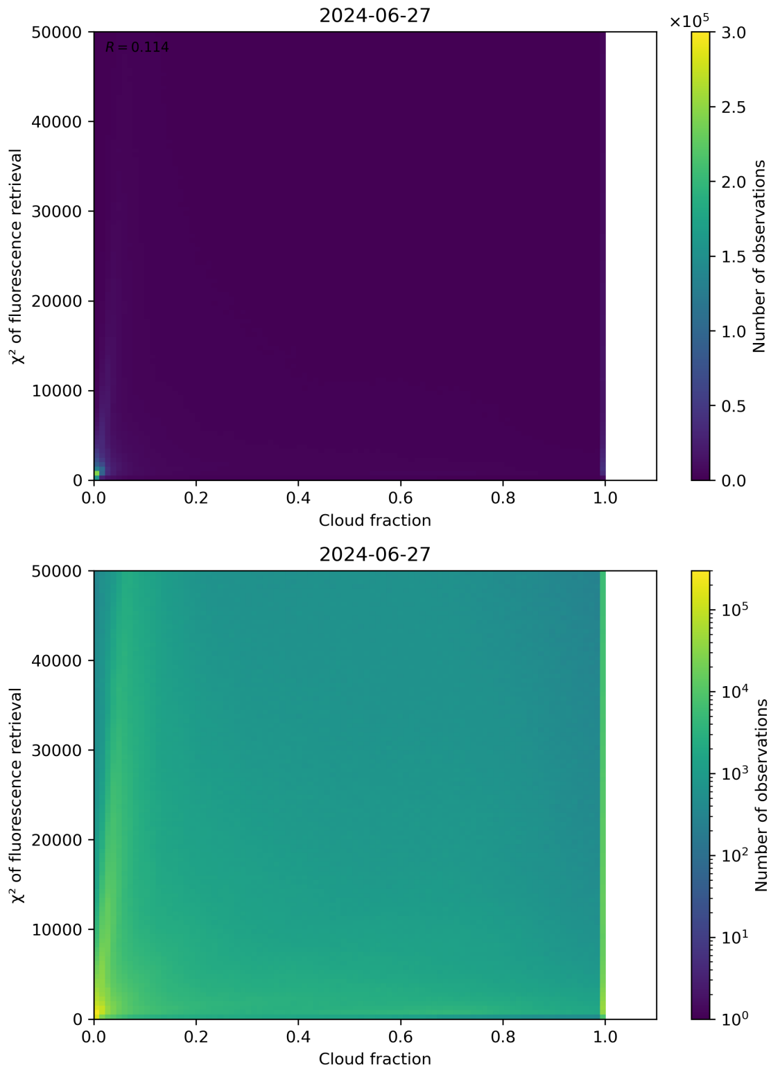
Figure 71: Scatter density plot of “Cloud fraction” against “ \chi^2 of fluorescence retrieval” for 2024-06-26 to 2024-06-28.
