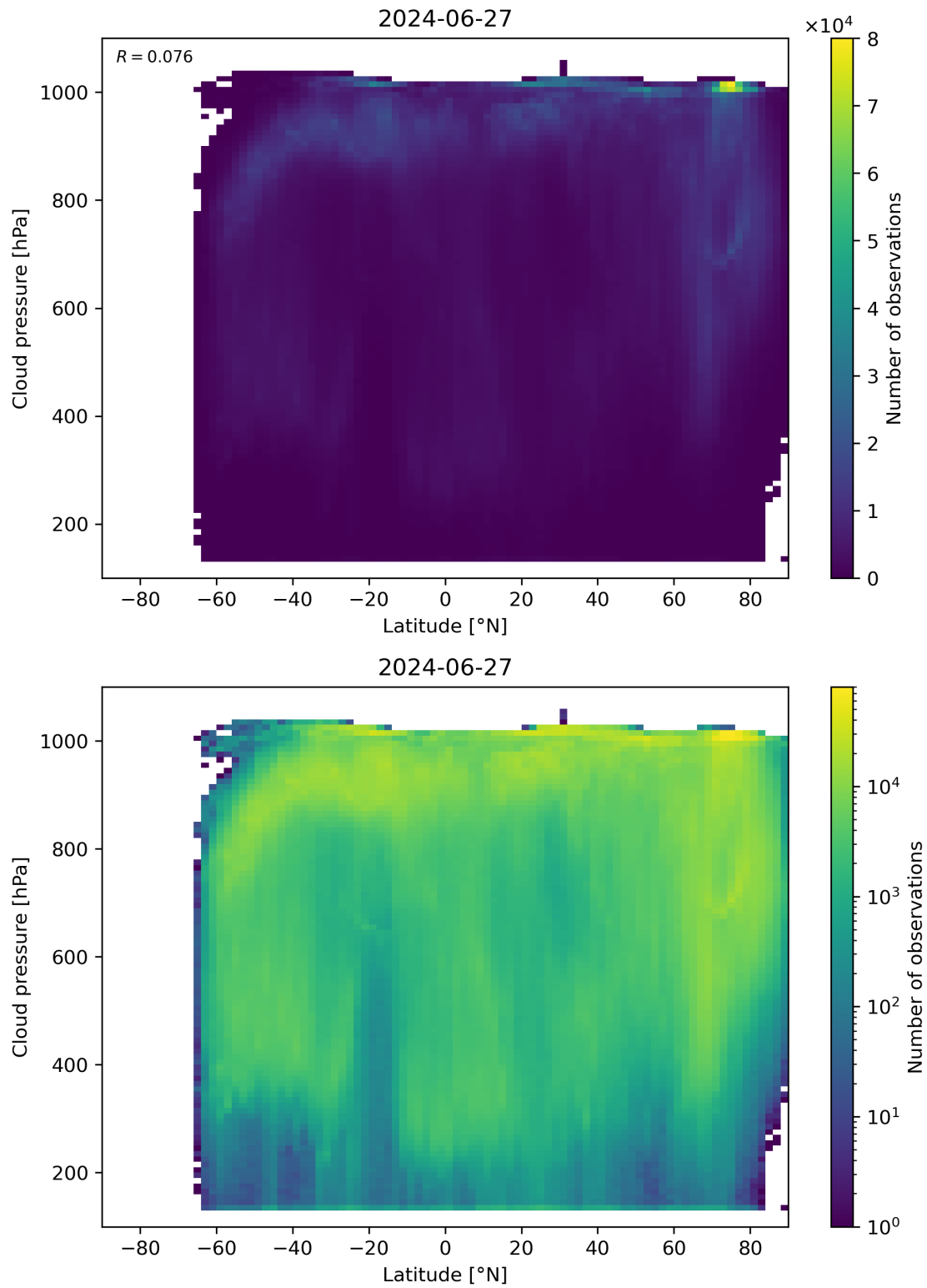
Figure 91: Scatter density plot of “Latitude” against “Cloud pressure” for 2024-06-26 to 2024-06-28.
