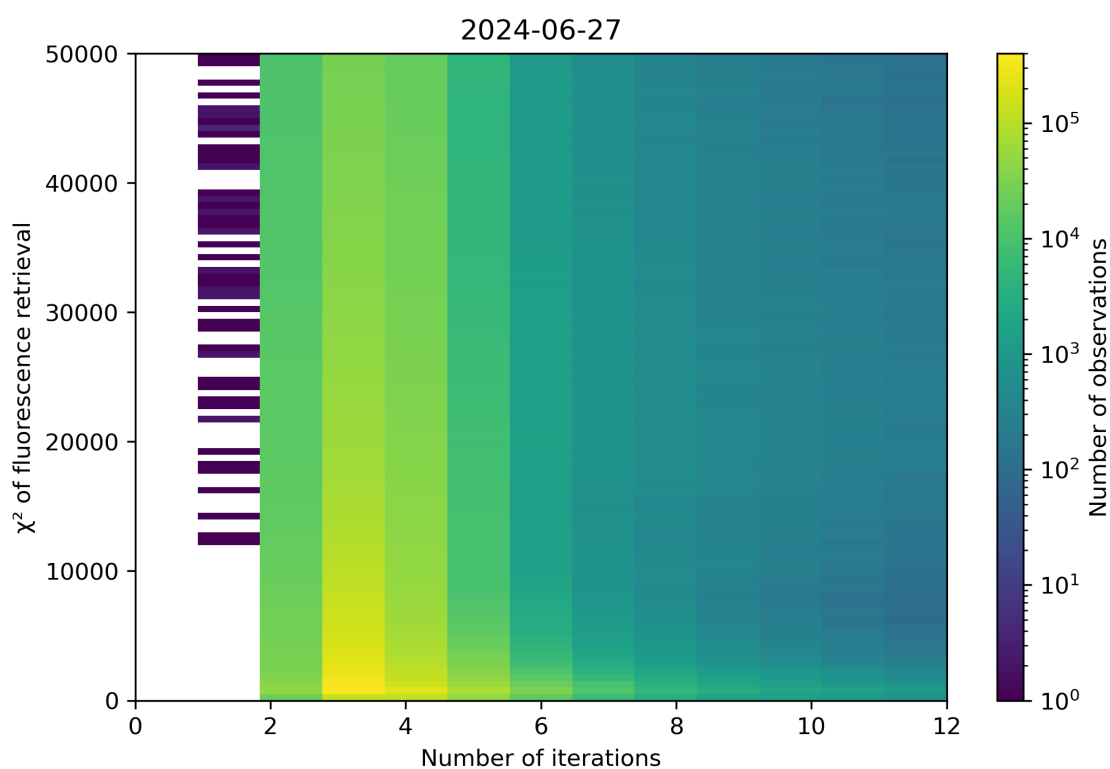
Figure 97: Scatter density plot of “Number of iterations” against “ \chi^2 of fluorescence retrieval” for 2024-06-26 to 2024-06-28.
