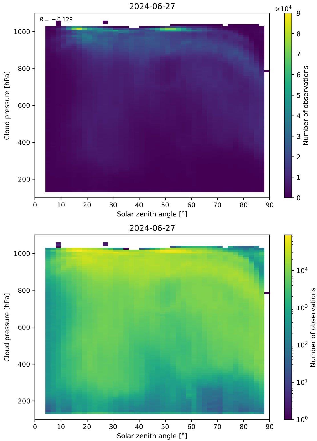
Figure 111: Scatter density plot of “Solar zenith angle” against “Cloud pressure” for 2024-06-26 to 2024-06-28.
