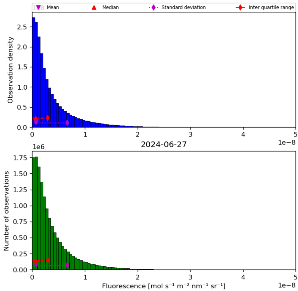
Figure 40: Histogram of “Fluorescence” for 2024-06-26 to 2024-06-28
