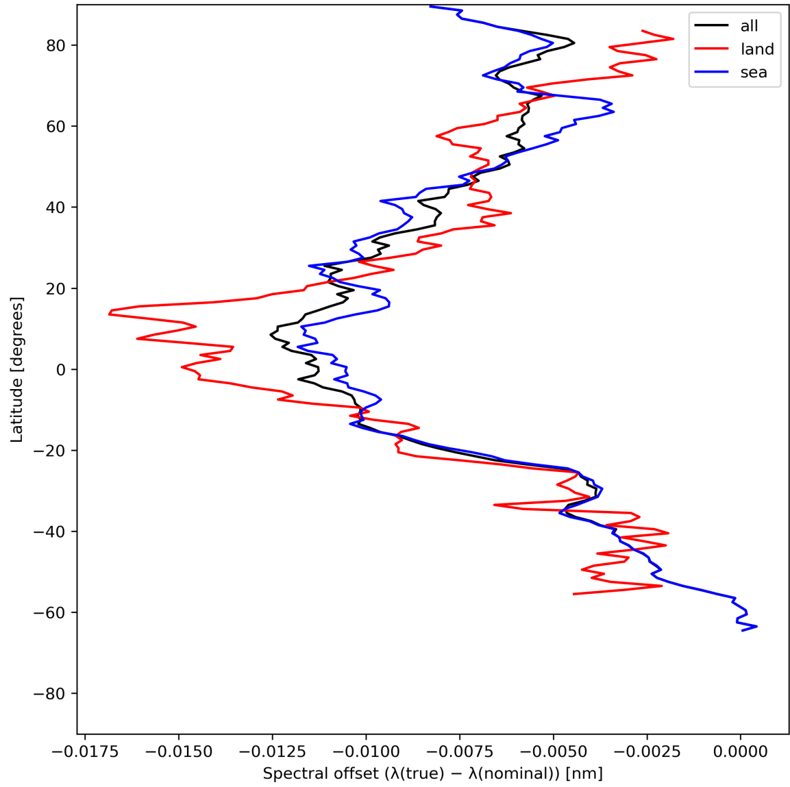
Figure 28: Zonal average of “Spectral offset ( \lambda(\text{true}) - \lambda(\text{nominal}) )” for 2024-06-26 to 2024-06-28.
