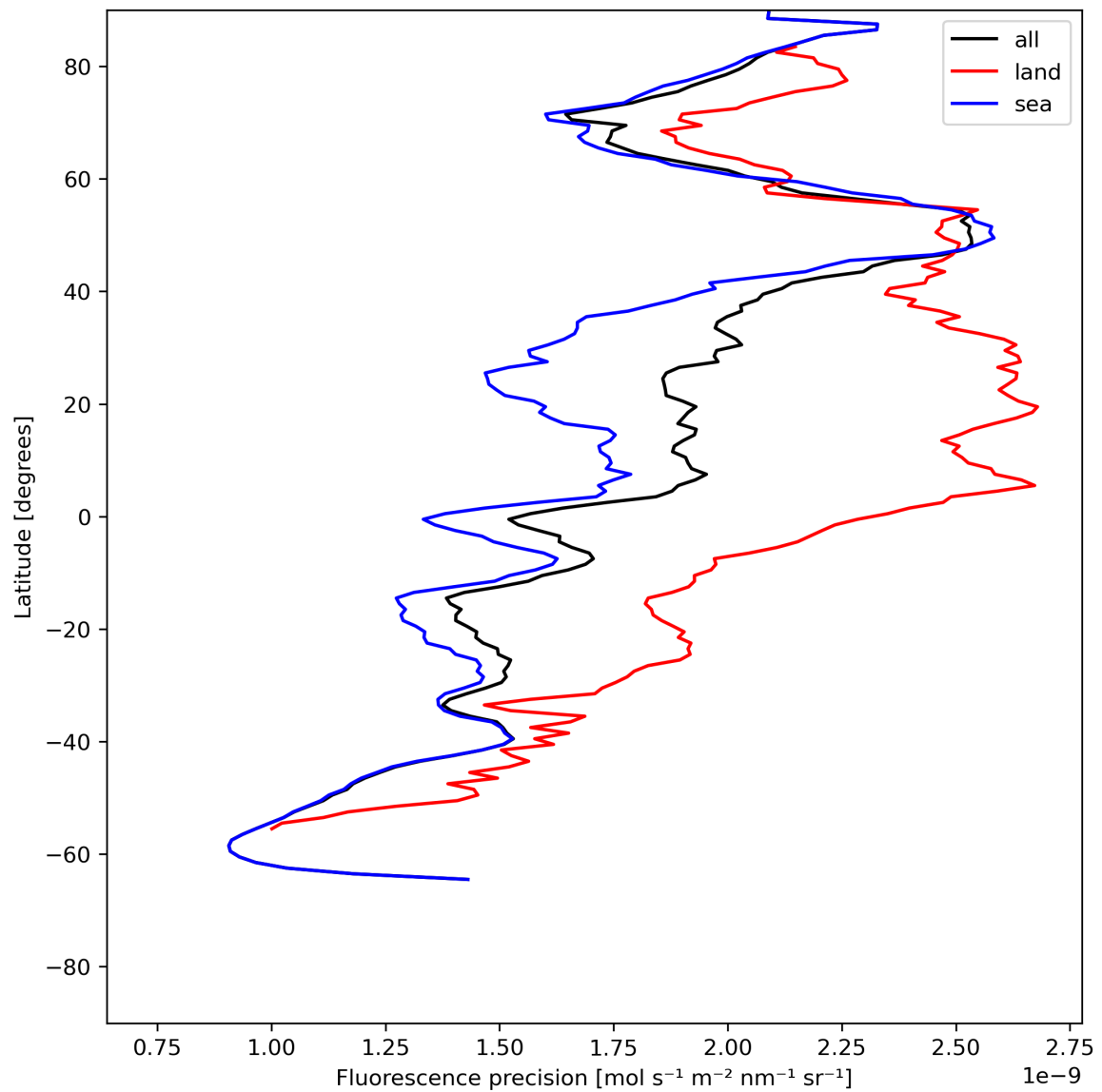
Figure 24: Zonal average of “Fluorescence precision” for 2024-06-26 to 2024-06-28.
