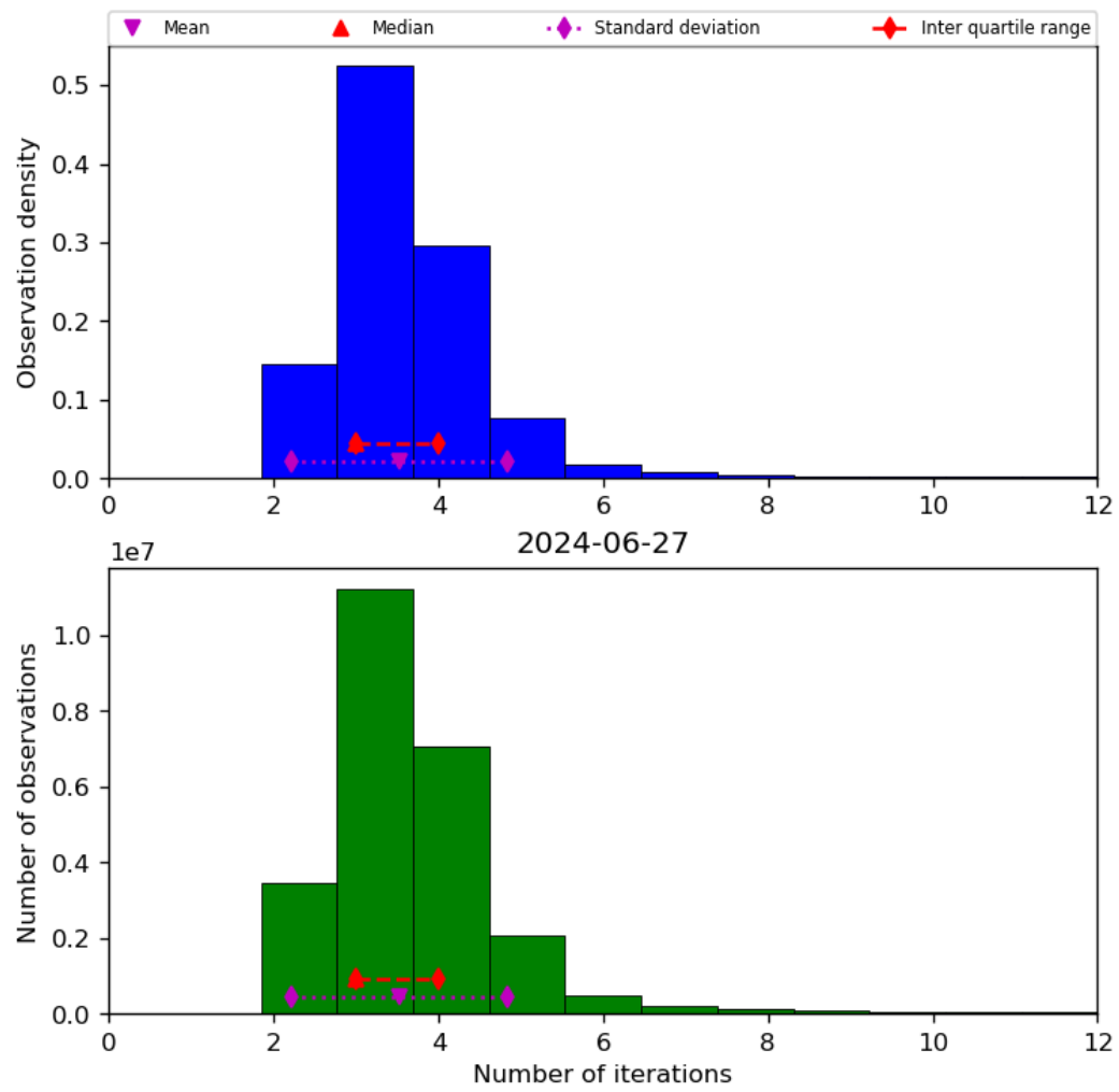
Figure 39: Histogram of “Number of iterations” for 2024-06-26 to 2024-06-28
