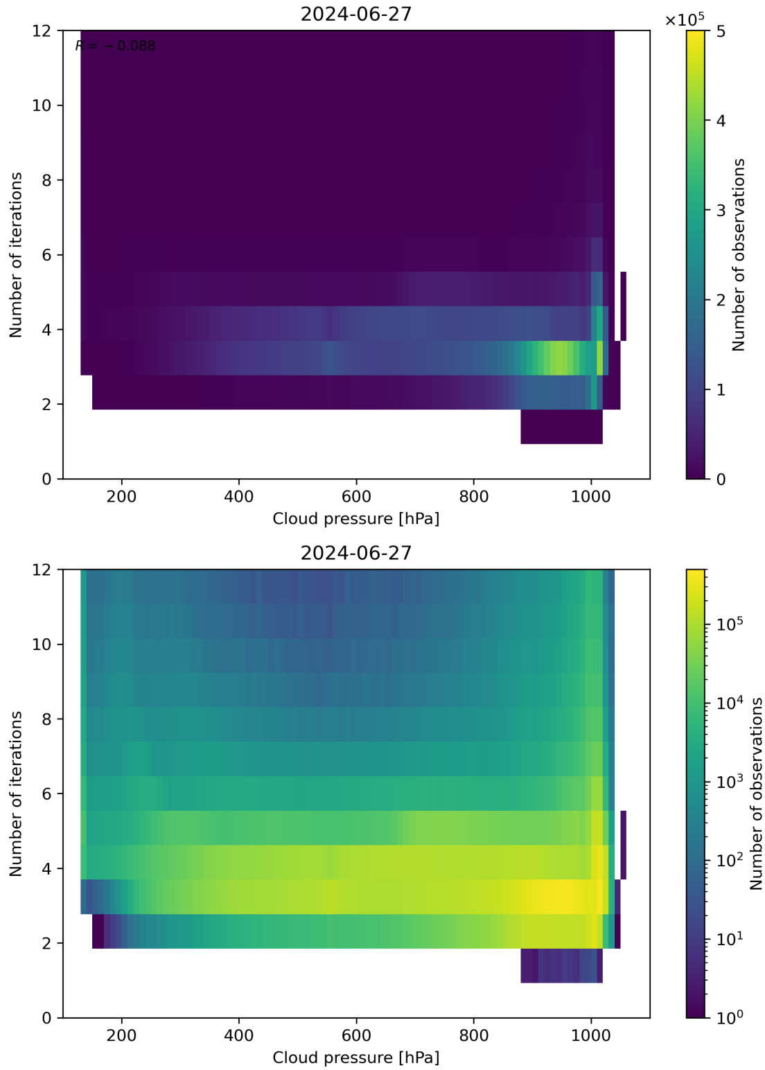
Figure 81: Scatter density plot of “Cloud pressure” against “Number of iterations” for 2024-06-26 to 2024-06-28.
