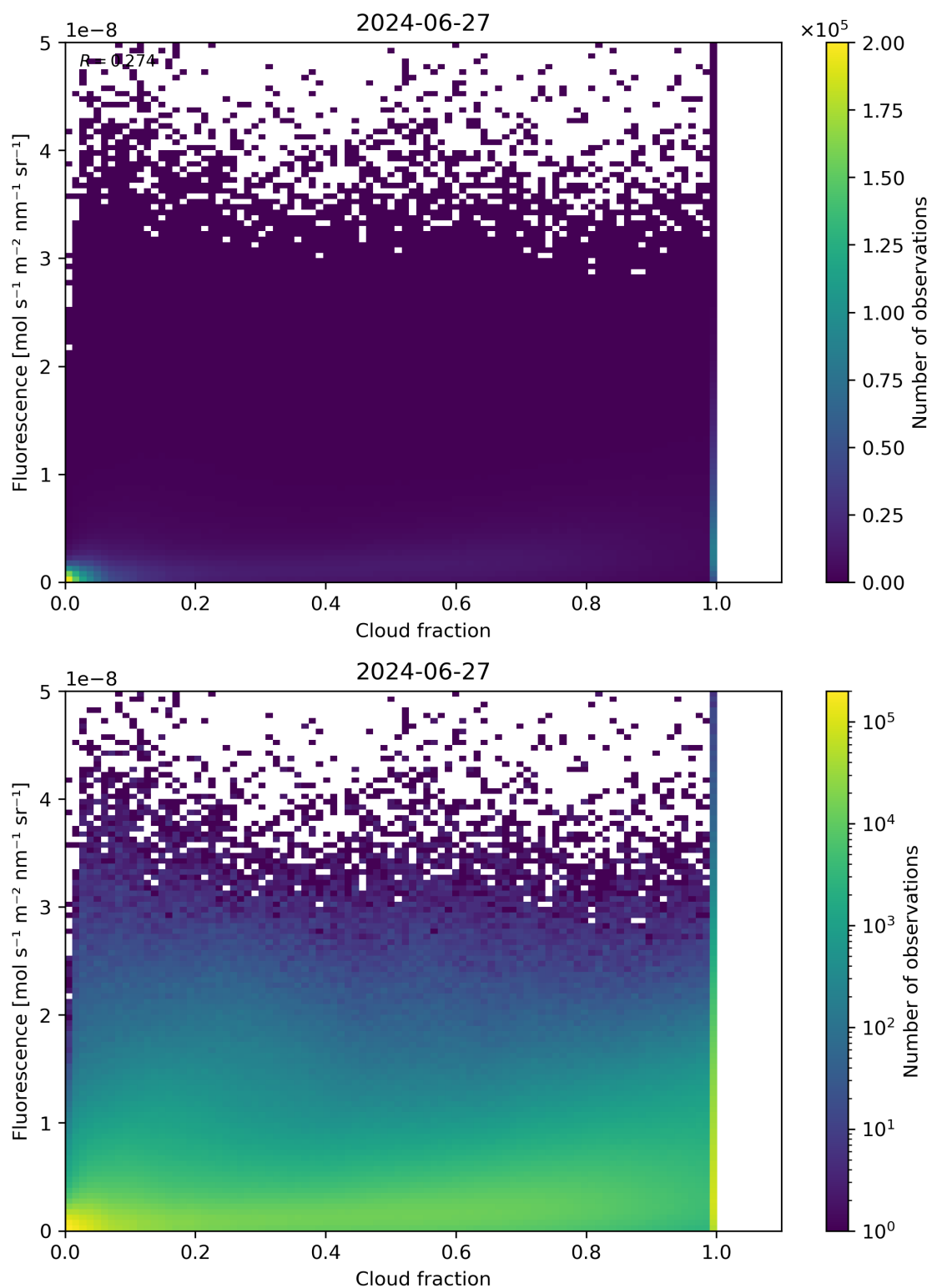
Figure 72: Scatter density plot of “Cloud fraction” against “Fluorescence” for 2024-06-26 to 2024-06-28.
