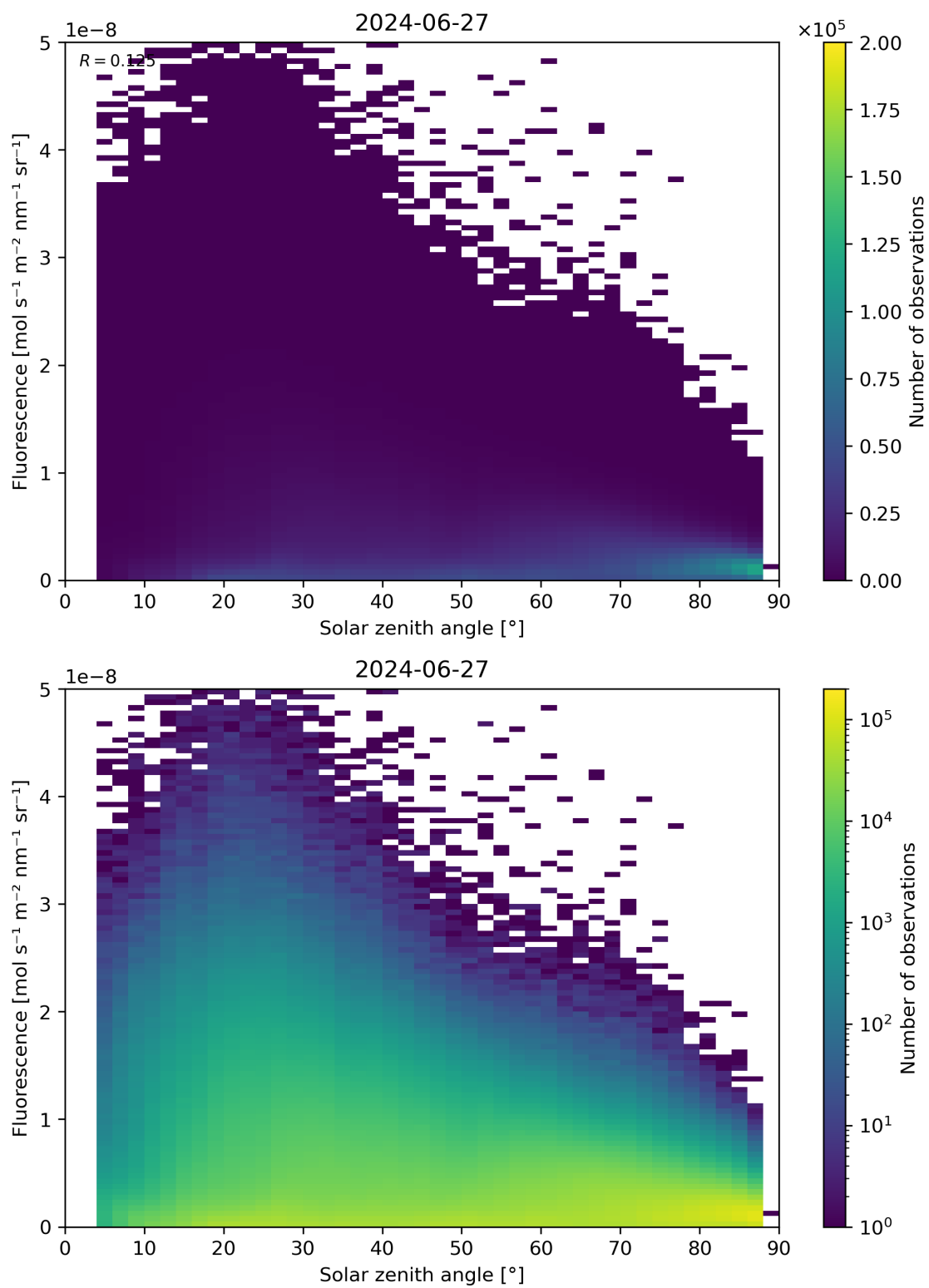
Figure 112: Scatter density plot of “Solar zenith angle” against “Fluorescence” for 2024-06-26 to 2024-06-28.
