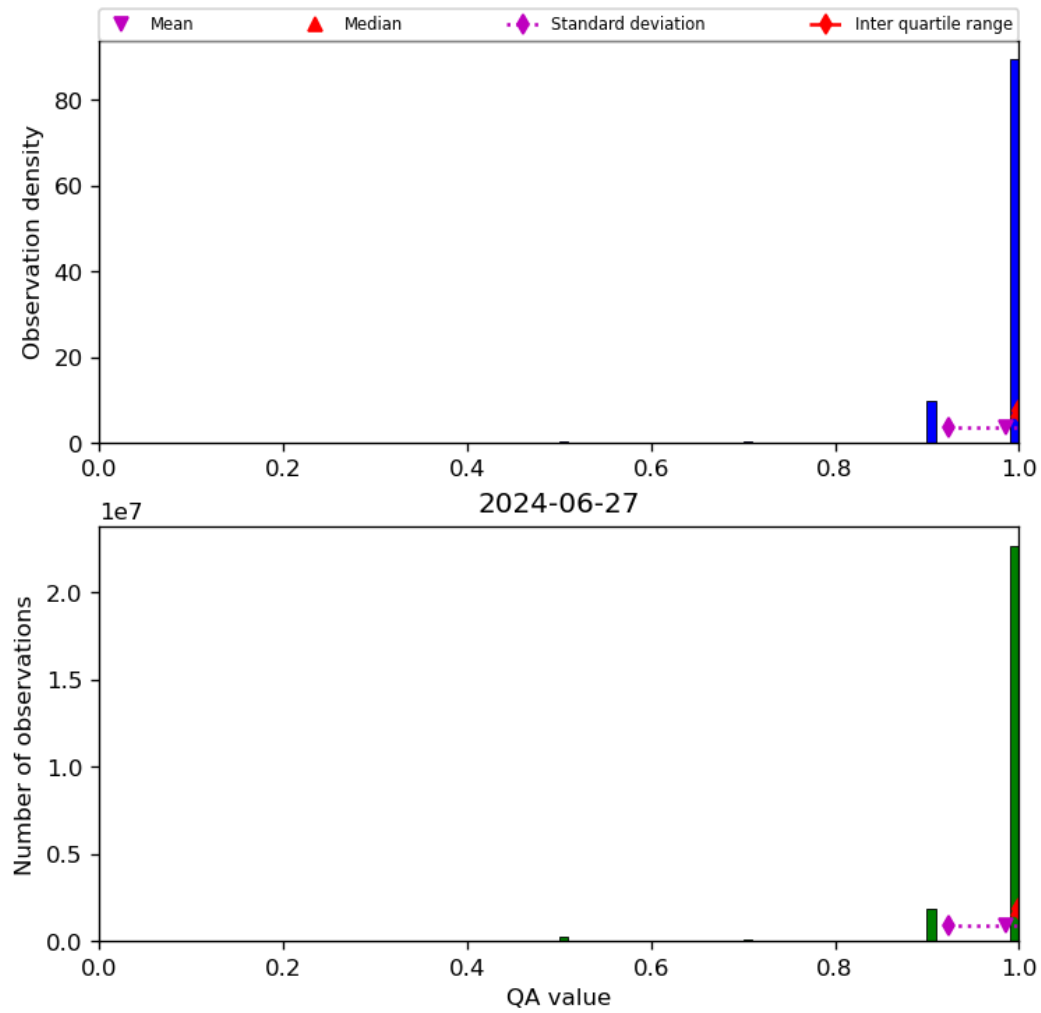
Figure 29: Histogram of “QA value” for 2024-06-26 to 2024-06-28
