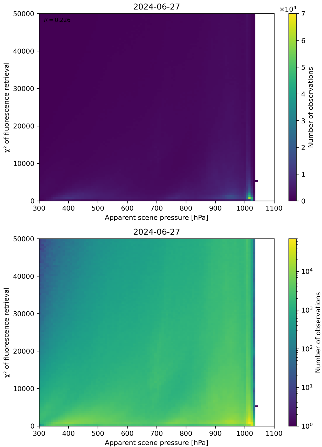
Figure 63: Scatter density plot of “Apparent scene pressure” against “ \chi^2 of fluorescence retrieval” for 2024-06-26 to 2024-06-28.
