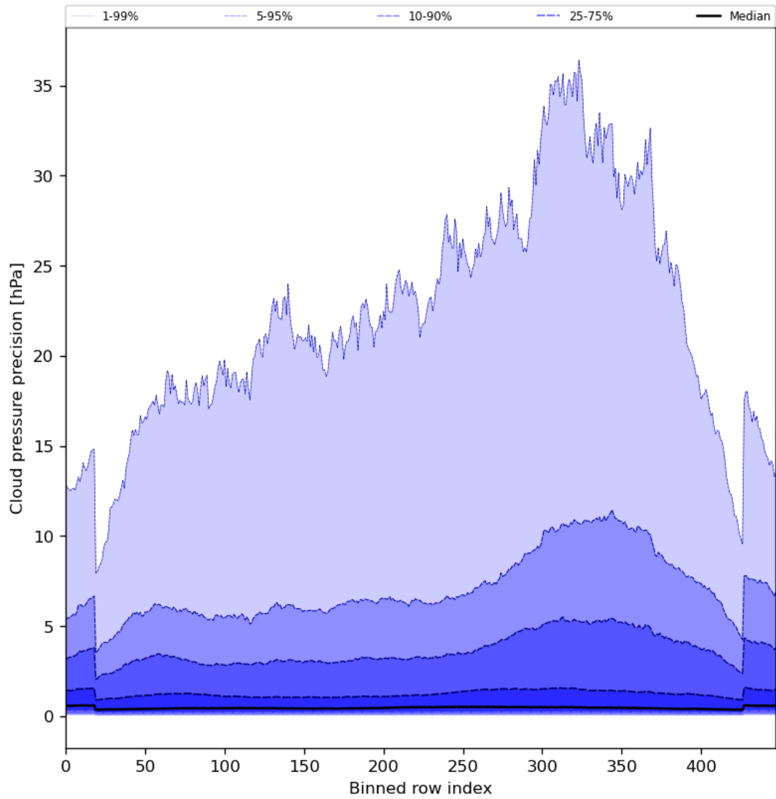
Figure 48: Along track statistics of “Cloud pressure precision” for 2024-06-26 to 2024-06-28
