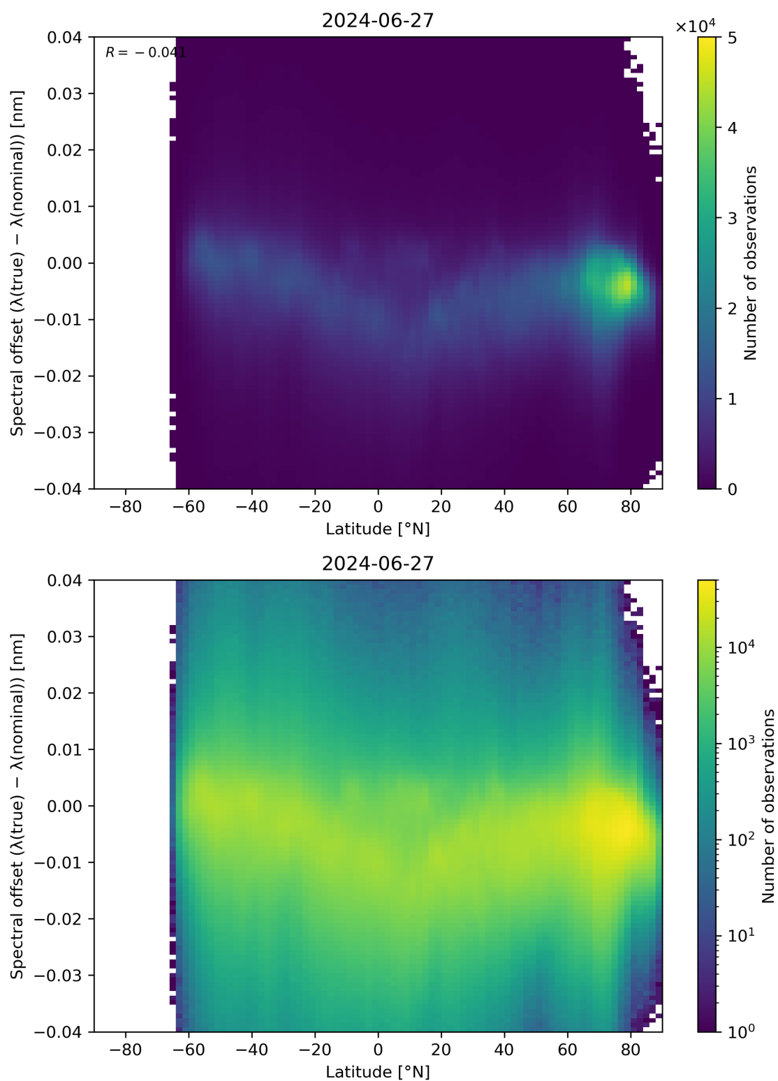
Figure 96: Scatter density plot of “Latitude” against “Spectral offset ( \lambda(\text{true}) - \lambda(\text{nominal}) )” for 2024-06-26 to 2024-06-28.
