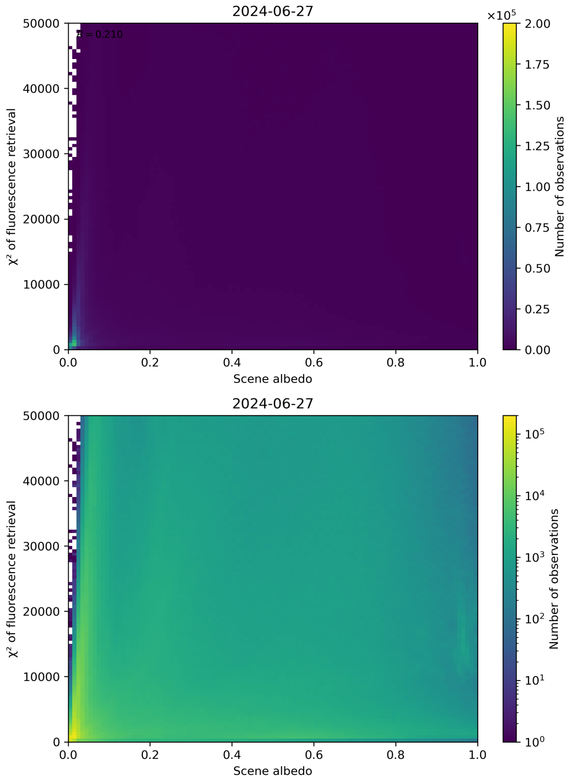
Figure 103: Scatter density plot of “Scene albedo” against “ \chi^2 of fluorescence retrieval” for 2024-06-26 to 2024-06-28.
