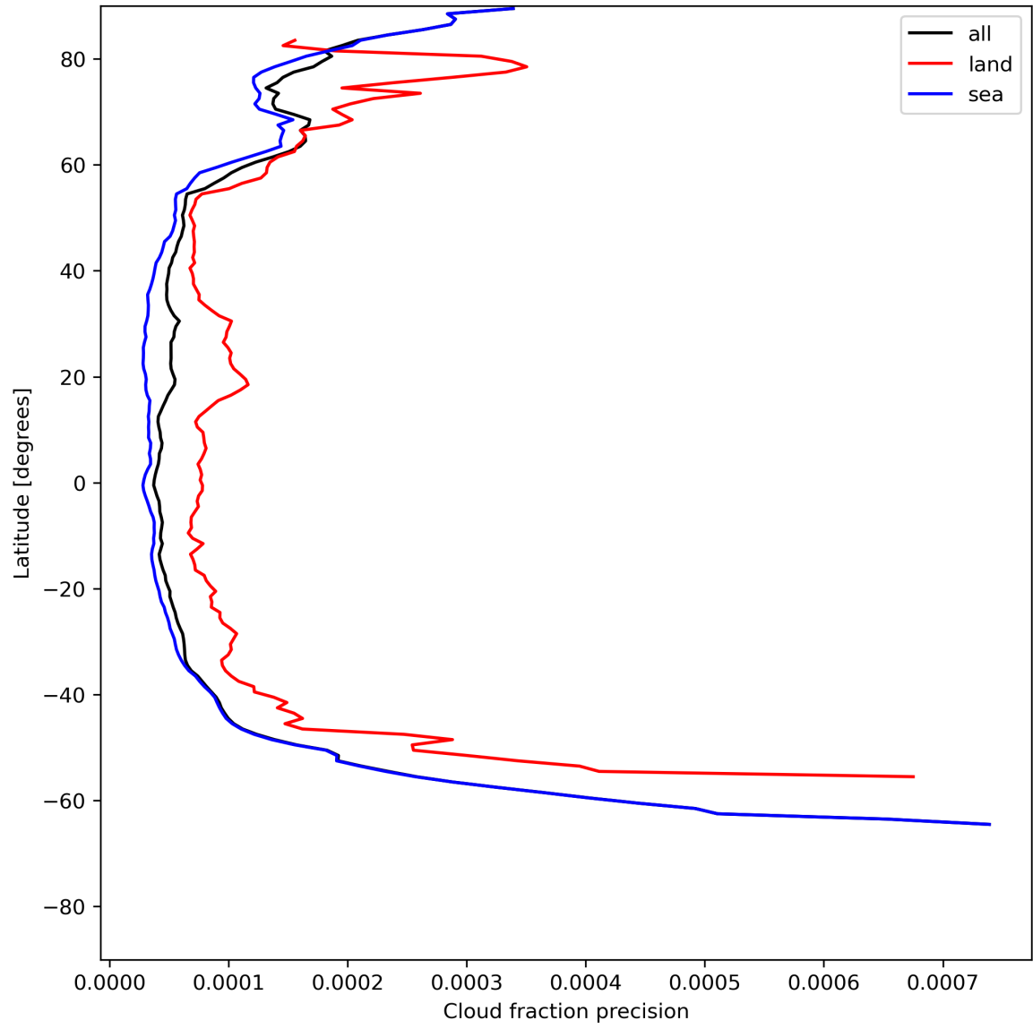
Figure 16: Zonal average of “Cloud fraction precision” for 2024-06-26 to 2024-06-28.
