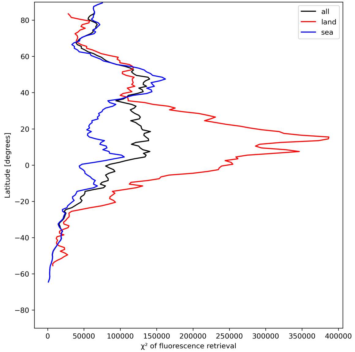
Figure 25: Zonal average of “ \chi^2 of fluorescence retrieval” for 2024-06-26 to 2024-06-28.
