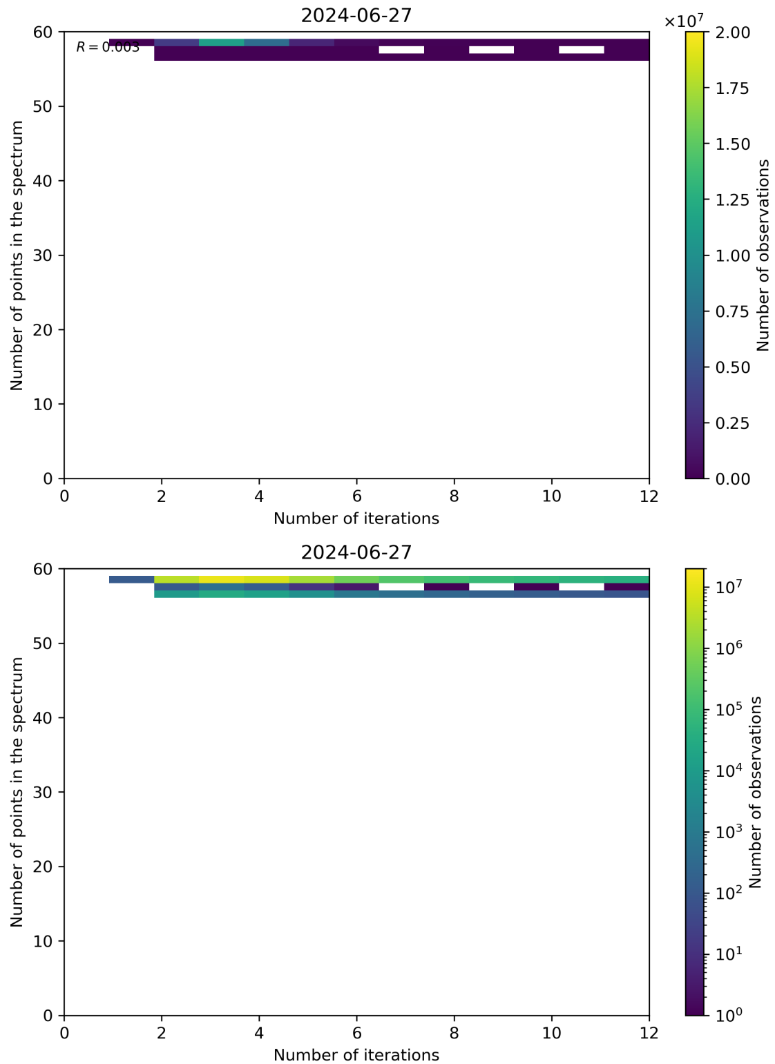
Figure 99: Scatter density plot of “Number of iterations” against “Number of points in the spectrum” for 2024-06-26 to 2024-06-28.
