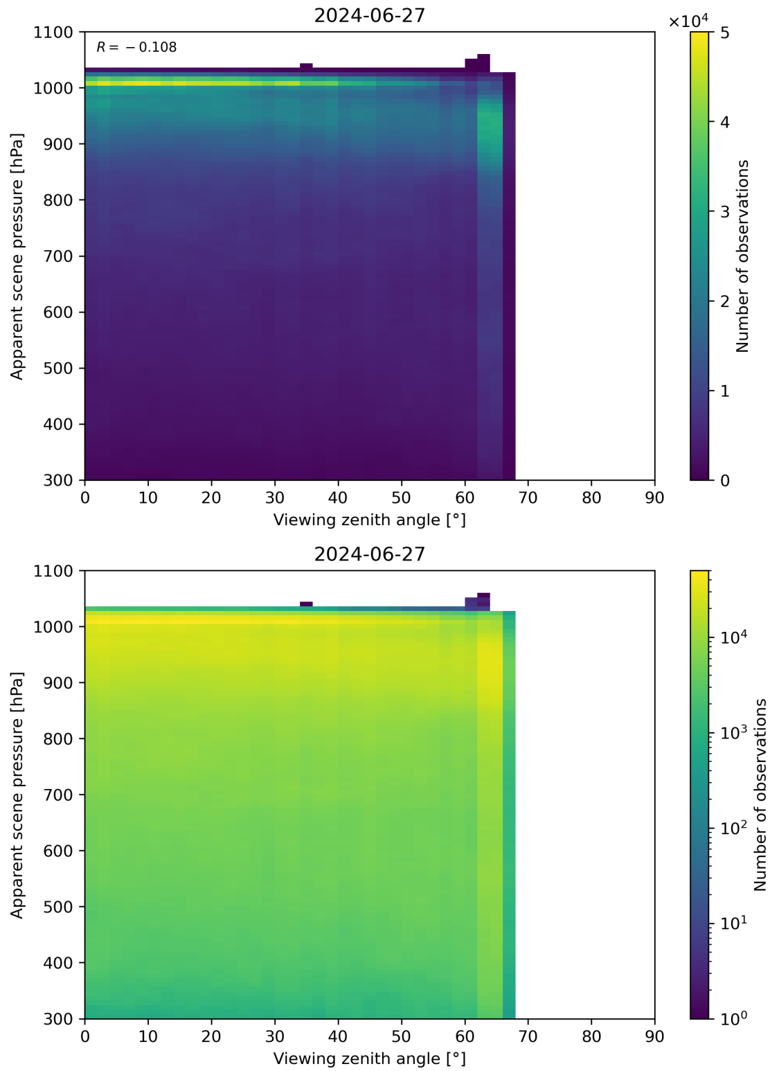
Figure 118: Scatter density plot of “Viewing zenith angle” against “Apparent scene pressure” for 2024-06-26 to 2024-06-28.
