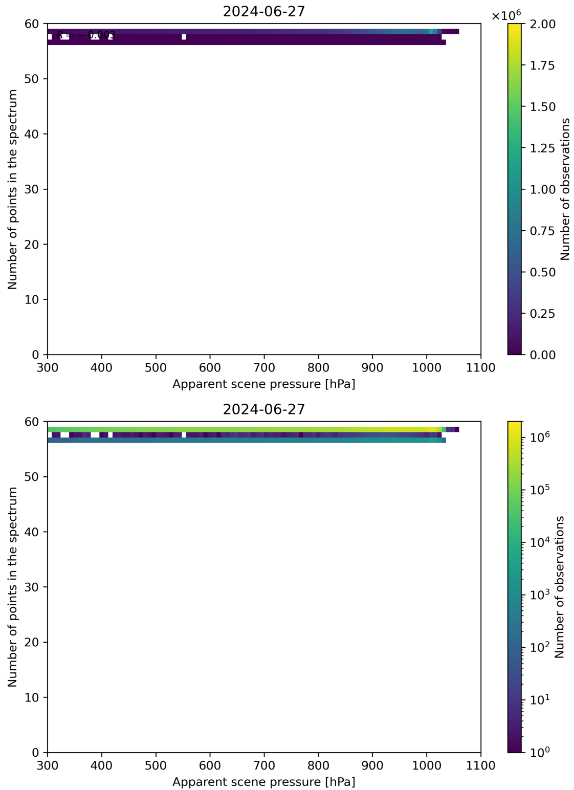
Figure 66: Scatter density plot of “Apparent scene pressure” against “Number of points in the spectrum” for 2024-06-26 to 2024-06-28.
