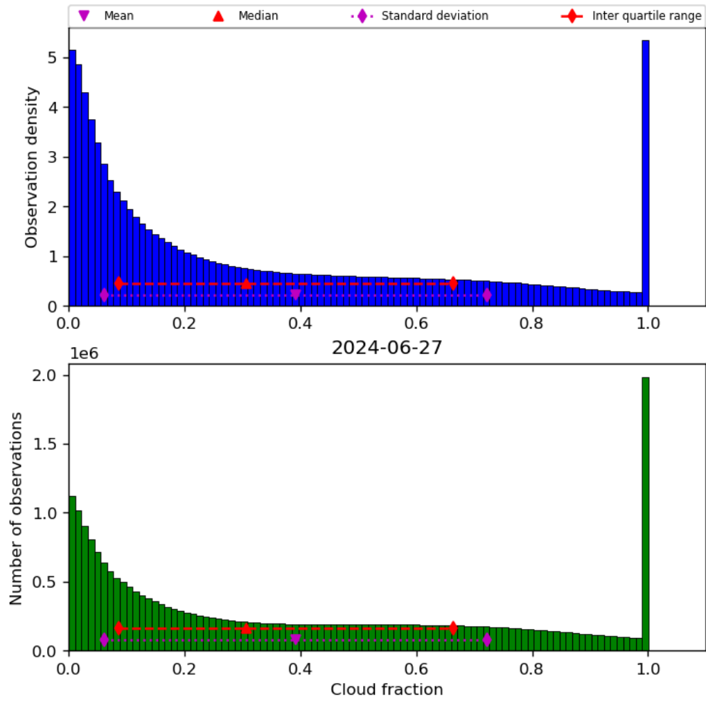
Figure 32: Histogram of “Cloud fraction” for 2024-06-26 to 2024-06-28
