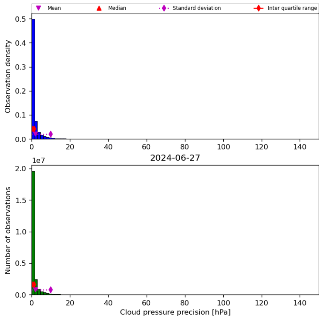
Figure 31: Histogram of “Cloud pressure precision” for 2024-06-26 to 2024-06-28
