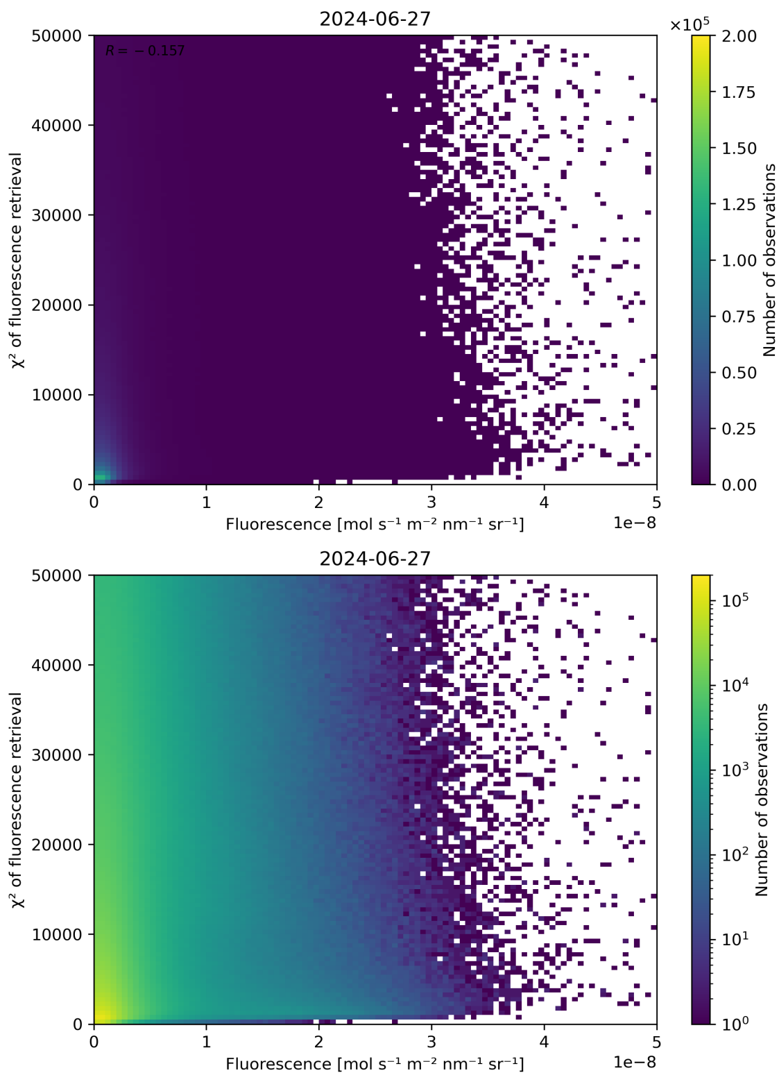
Figure 85: Scatter density plot of “Fluorescence” against “ \chi^2 of fluorescence retrieval” for 2024-06-26 to 2024-06-28.
