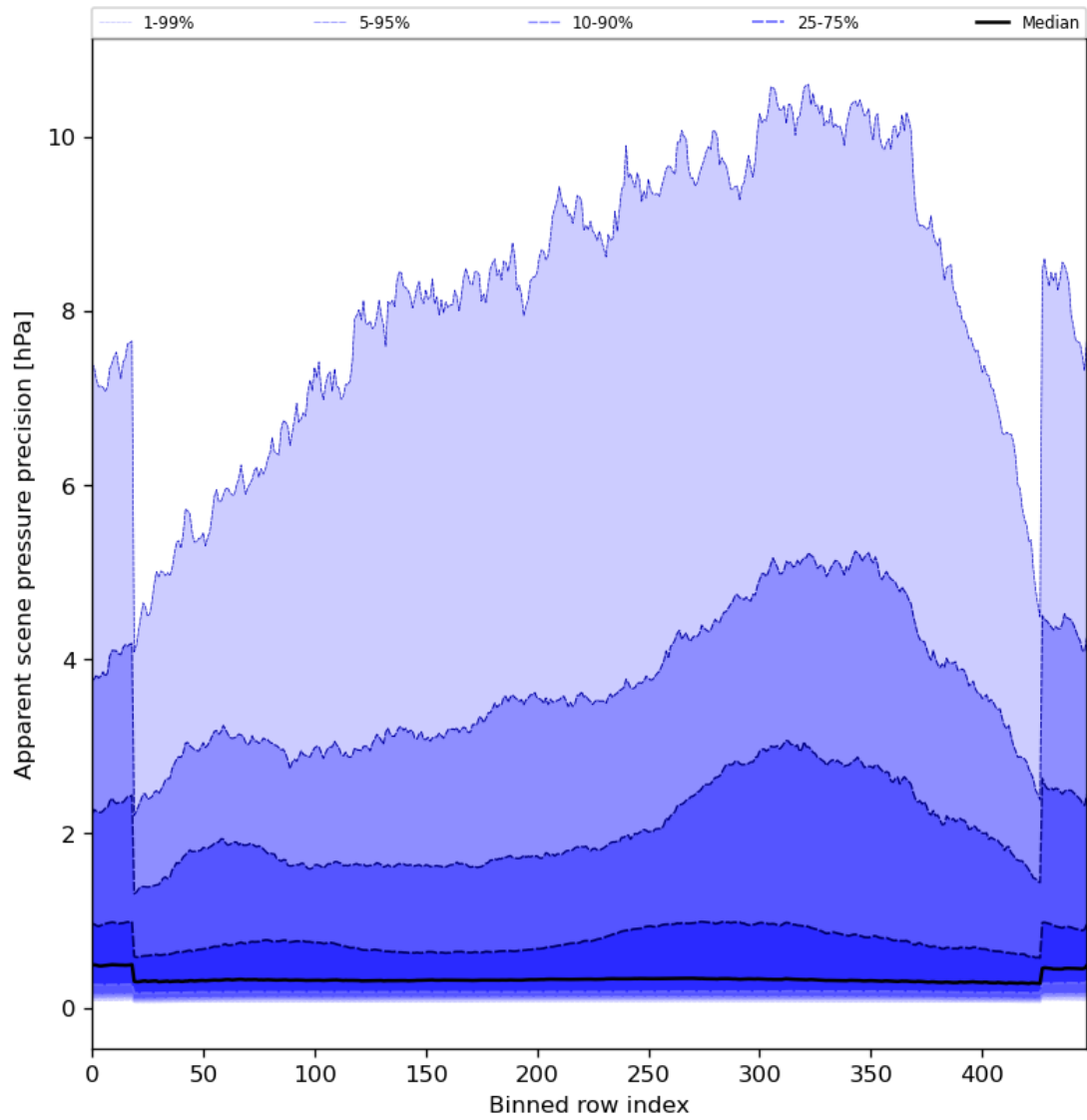
Figure 54: Along track statistics of “Apparent scene pressure precision” for 2024-06-26 to 2024-06-28
