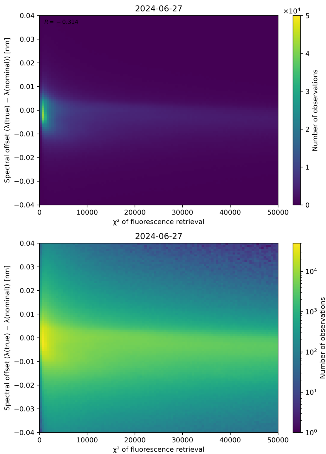
Figure 69: Scatter density plot of " \chi^2 of fluorescence retrieval" against "Spectral offset ( \lambda(\text{true}) - \lambda(\text{nominal})) " for 2024-06-26 to 2024-06-28.
