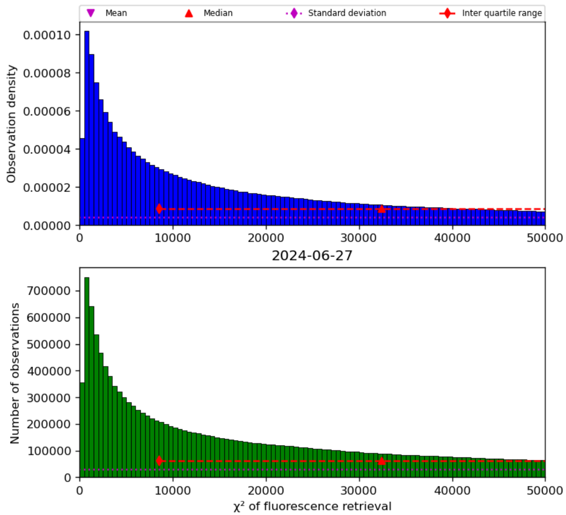
Figure 42: Histogram of “ \chi^2 of fluorescence retrieval” for 2024-06-26 to 2024-06-28
