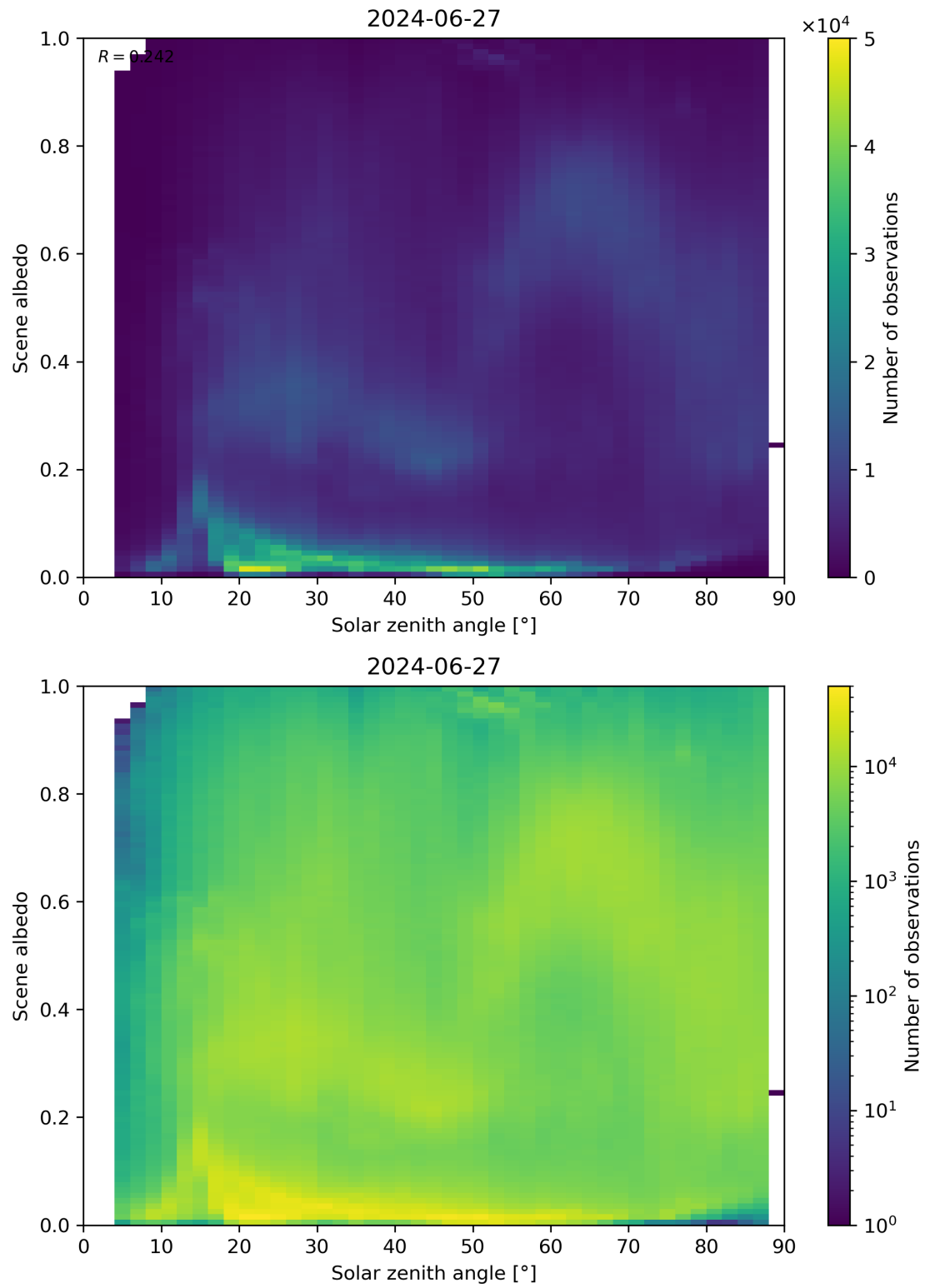
Figure 116: Scatter density plot of “Solar zenith angle” against “Scene albedo” for 2024-06-26 to 2024-06-28.
