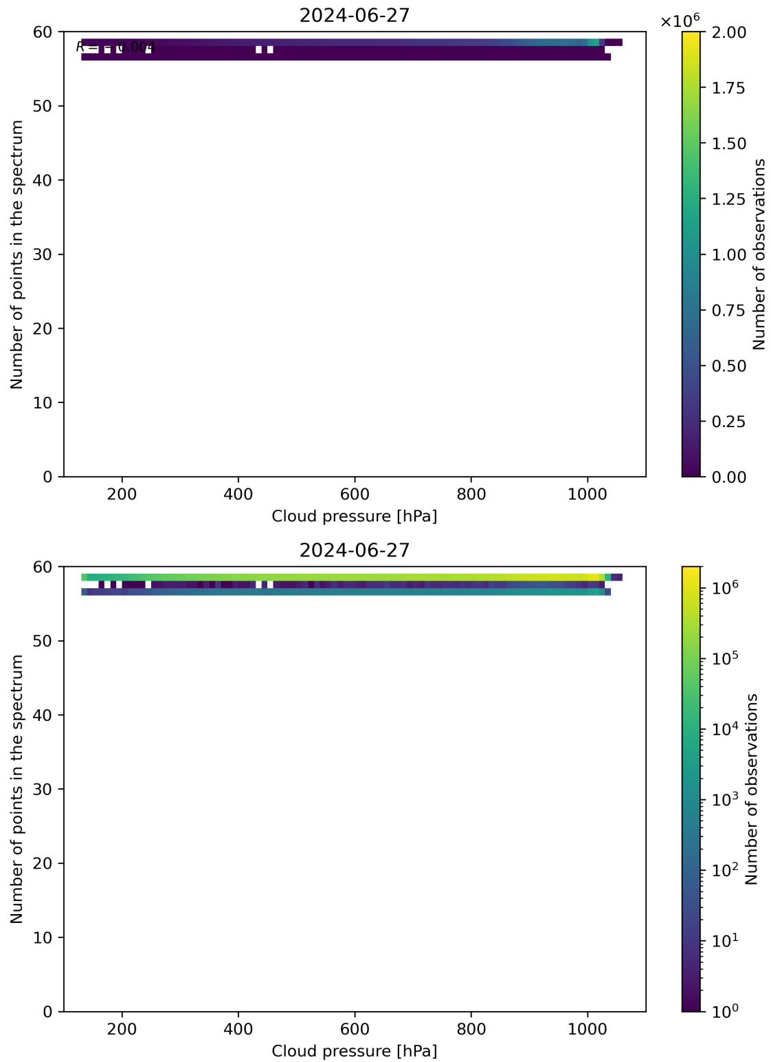
Figure 82: Scatter density plot of “Cloud pressure” against “Number of points in the spectrum” for 2024-06-26 to 2024-06-28.
