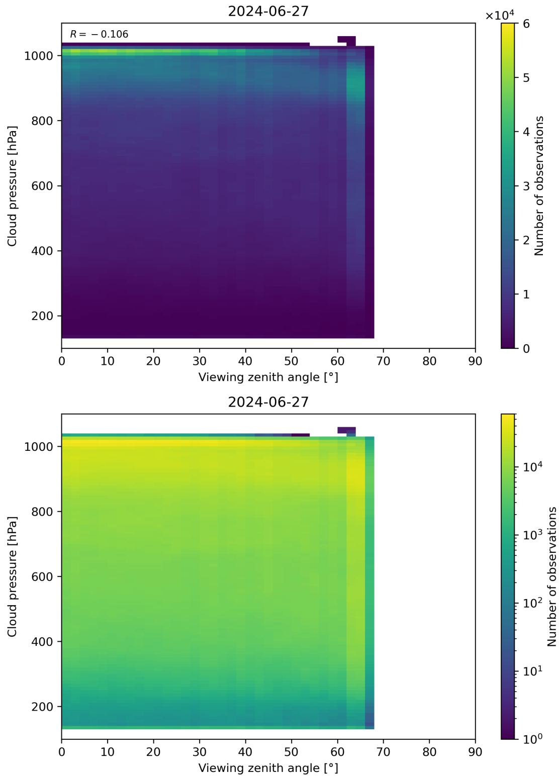
Figure 121: Scatter density plot of “Viewing zenith angle” against “Cloud pressure” for 2024-06-26 to 2024-06-28.
