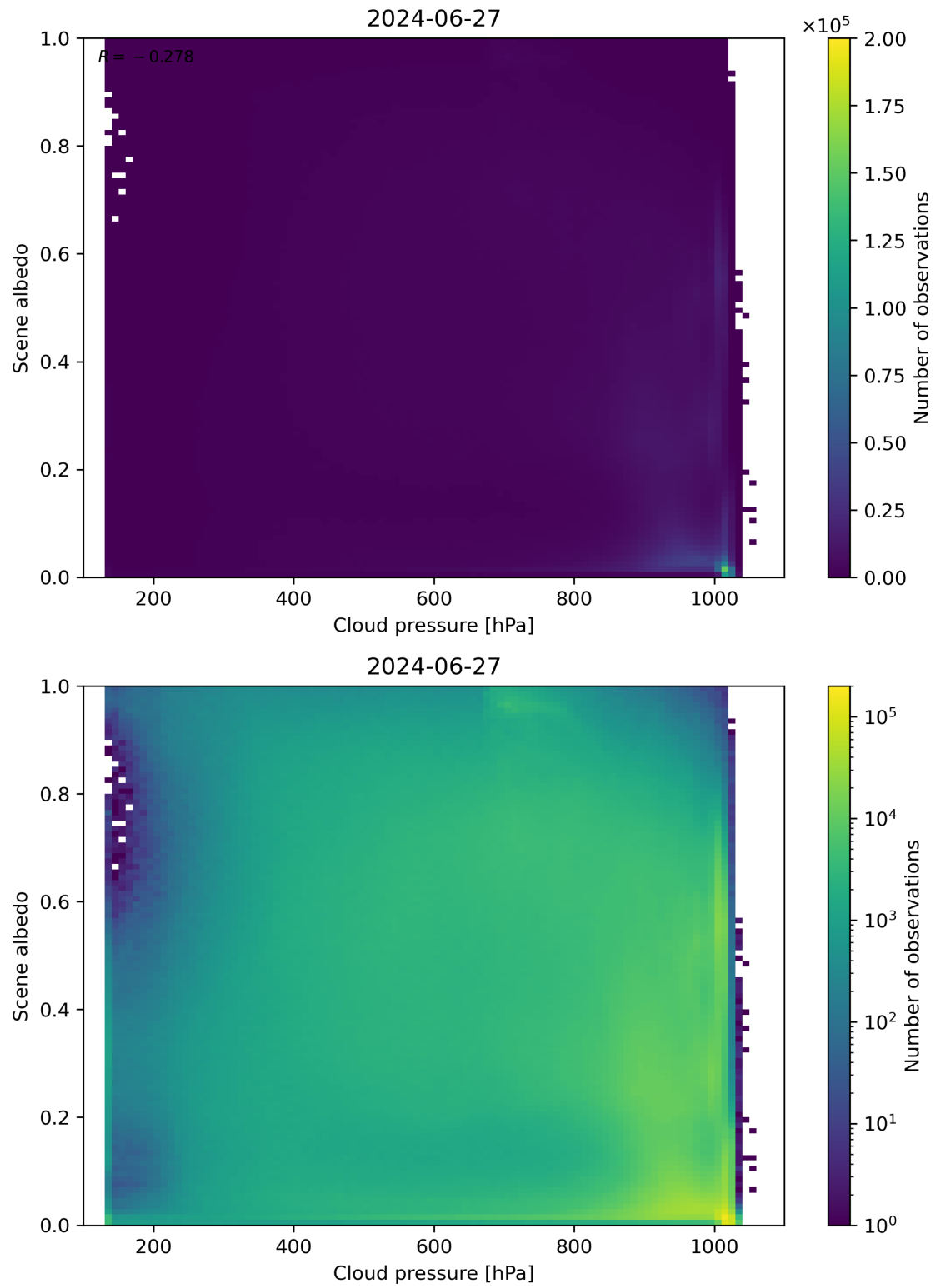
Figure 83: Scatter density plot of “Cloud pressure” against “Scene albedo” for 2024-06-26 to 2024-06-28.
