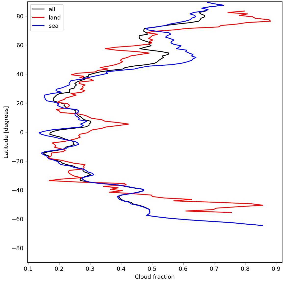
Figure 15: Zonal average of “Cloud fraction” for 2024-06-26 to 2024-06-28.
