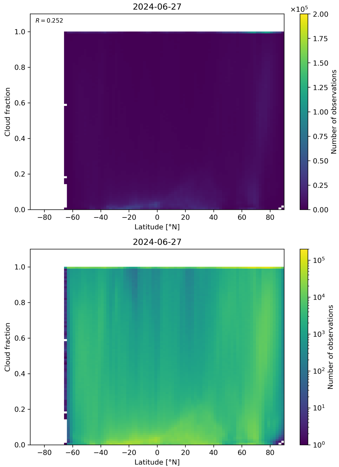
Figure 90: Scatter density plot of “Latitude” against “Cloud fraction” for 2024-06-26 to 2024-06-28.
