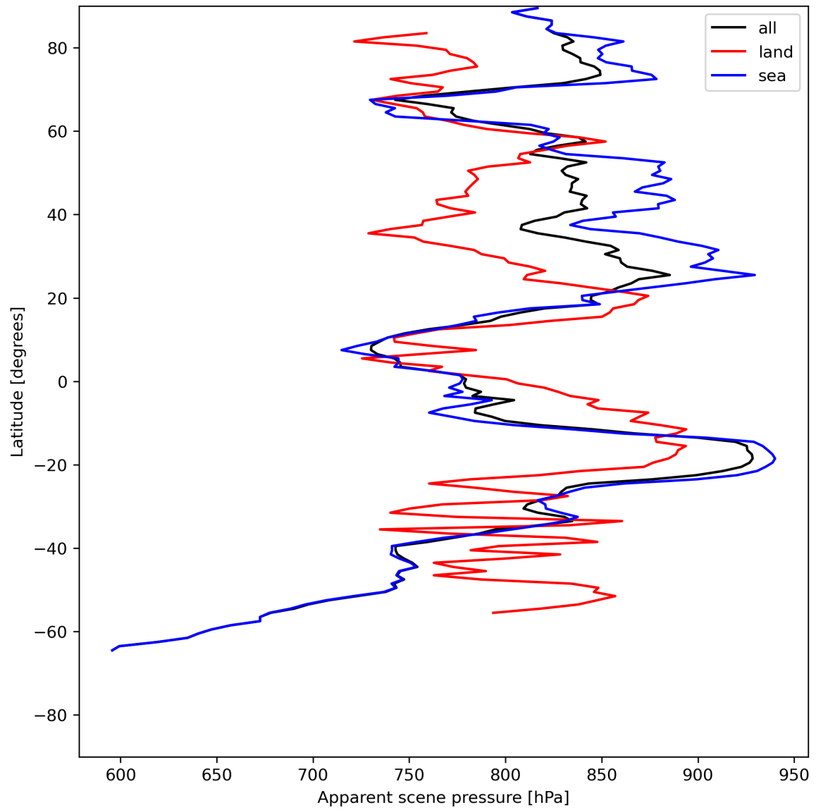
Figure 19: Zonal average of “Apparent scene pressure” for 2024-06-26 to 2024-06-28.
