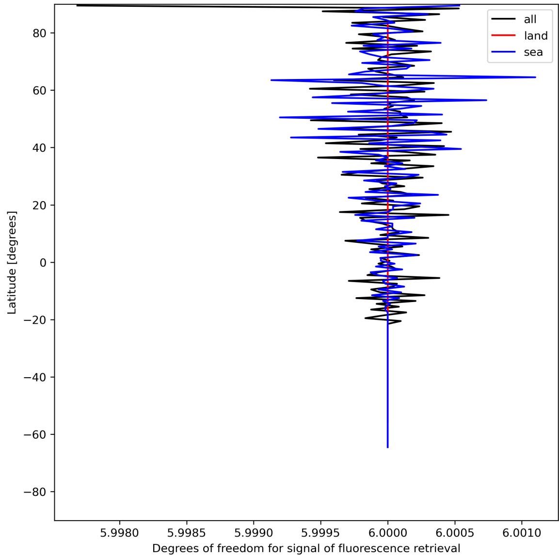
Figure 26: Zonal average of “Degrees of freedom for signal of fluorescence retrieval” for 2024-06-26 to 2024-06-28.
