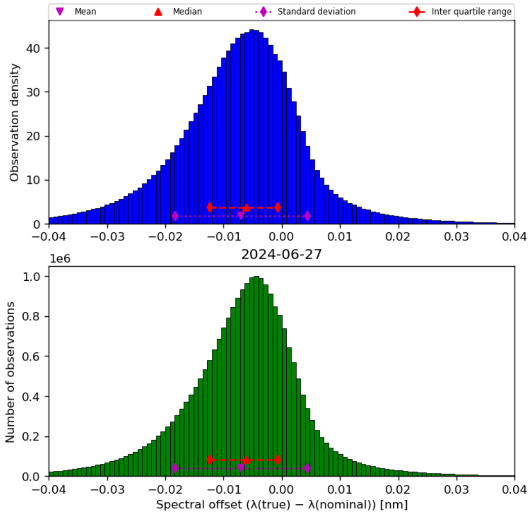
Figure 45: Histogram of “Spectral offset ( \lambda(\text{true}) - \lambda(\text{nominal}) )” for 2024-06-26 to 2024-06-28
