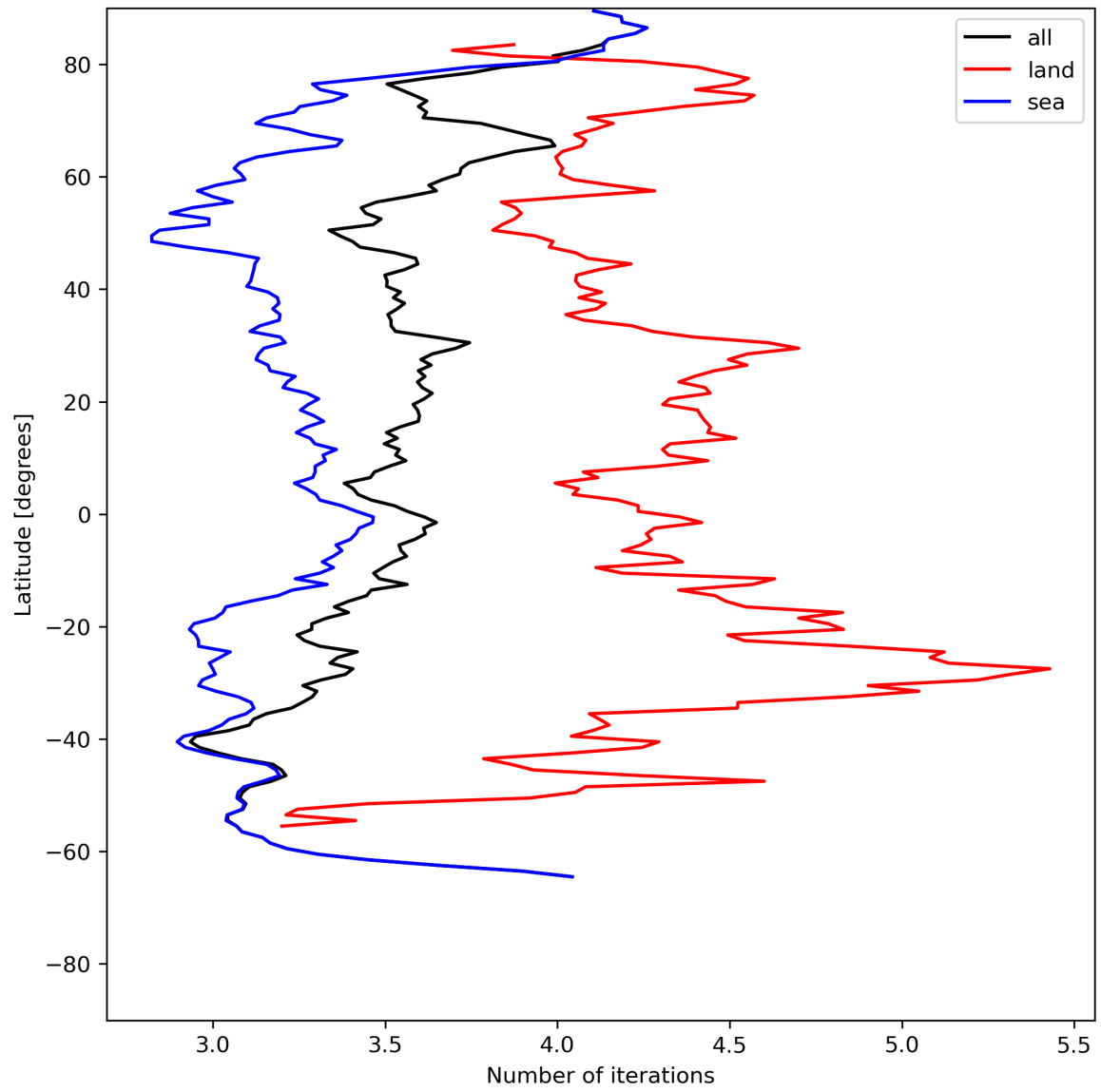
Figure 22: Zonal average of “Number of iterations” for 2024-06-26 to 2024-06-28.
