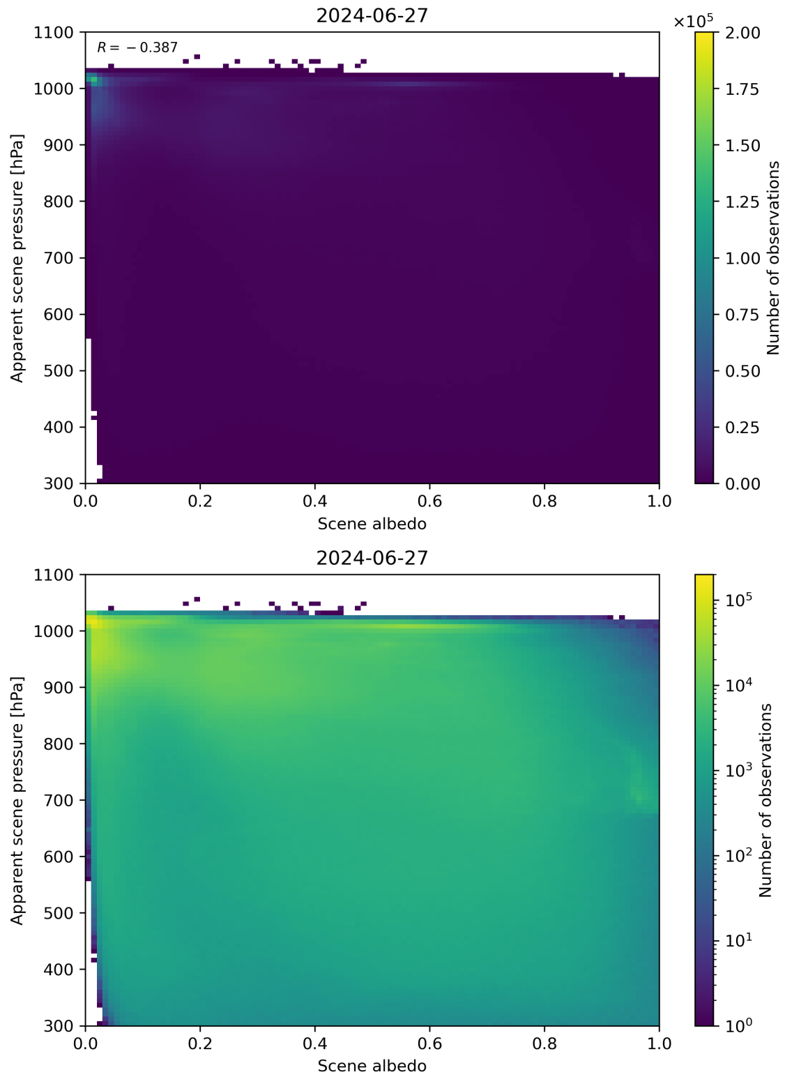
Figure 102: Scatter density plot of “Scene albedo” against “Apparent scene pressure” for 2024-06-26 to 2024-06-28.
