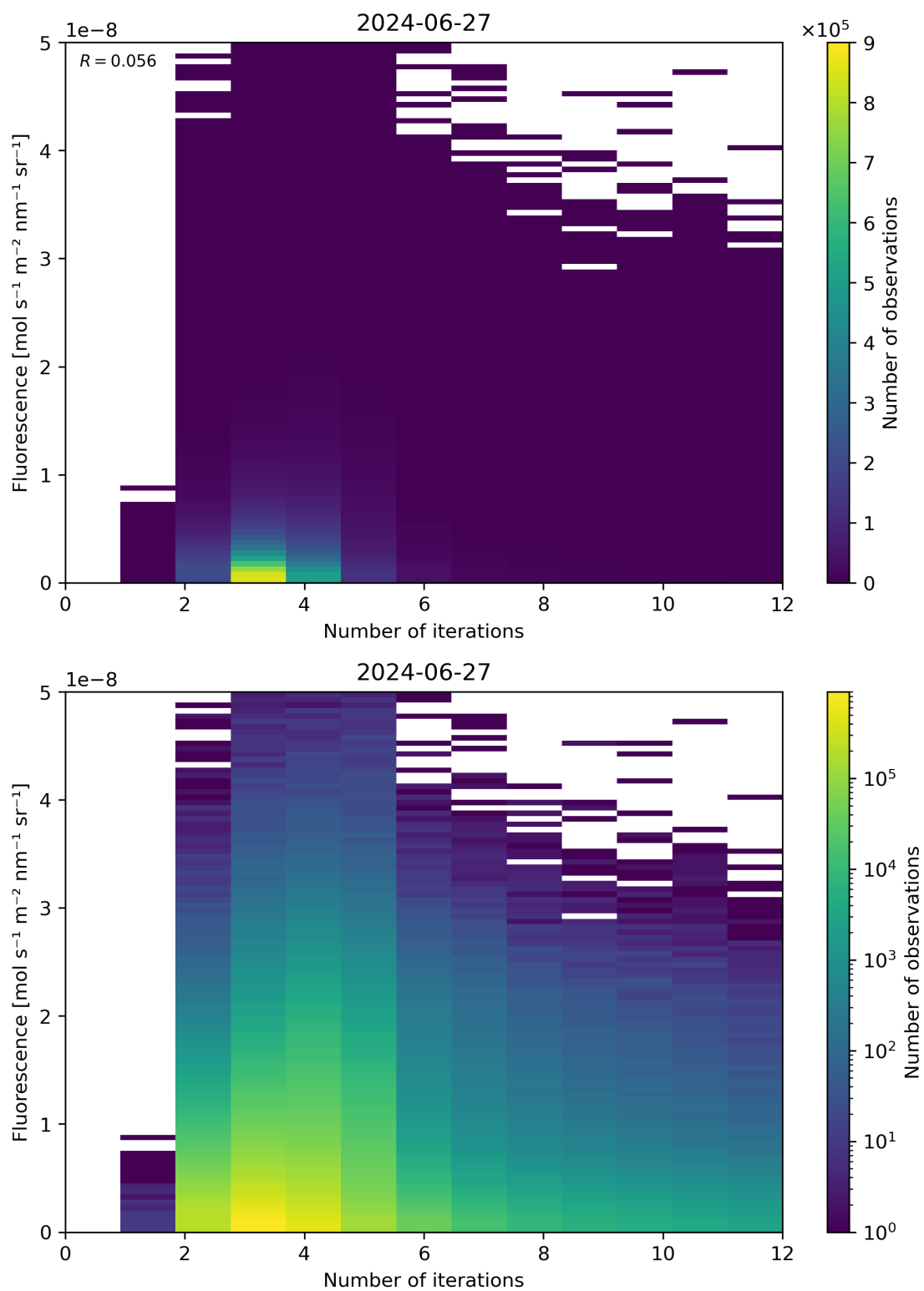
Figure 98: Scatter density plot of “Number of iterations” against “Fluorescence” for 2024-06-26 to 2024-06-28.
