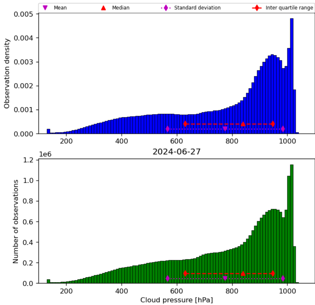
Figure 30: Histogram of “Cloud pressure” for 2024-06-26 to 2024-06-28
