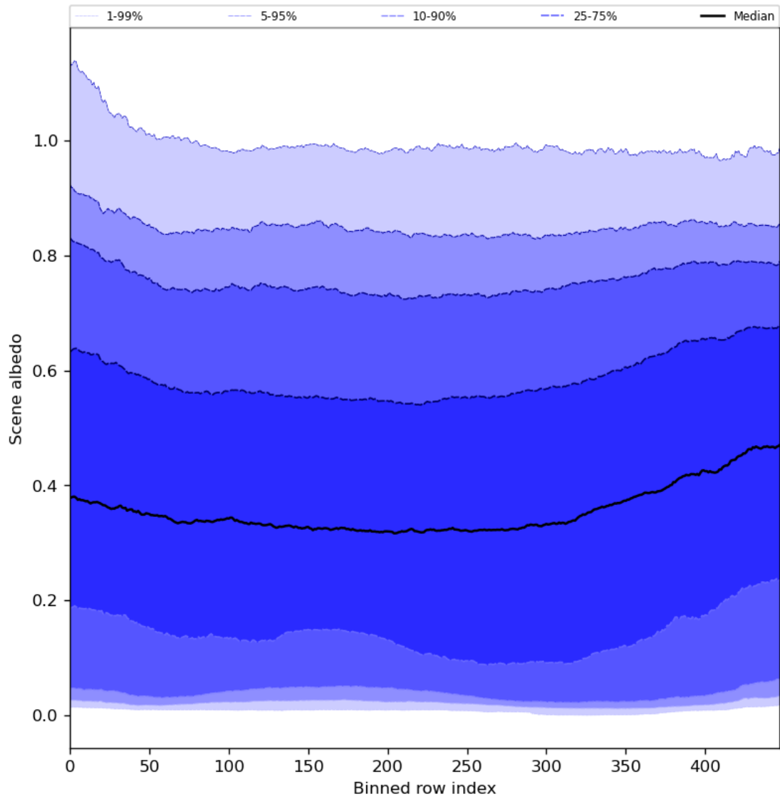
Figure 51: Along track statistics of “Scene albedo” for 2024-06-26 to 2024-06-28
