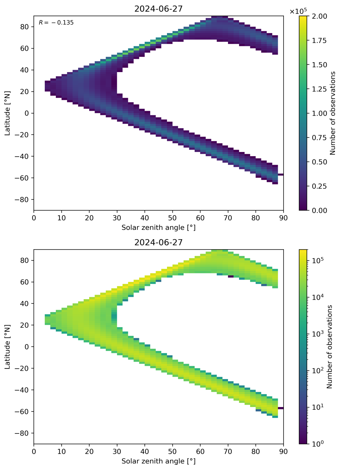
Figure 113: Scatter density plot of “Solar zenith angle” against “Latitude” for 2024-06-26 to 2024-06-28.
