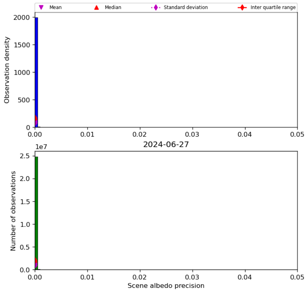
Figure 35: Histogram of “Scene albedo precision” for 2024-06-26 to 2024-06-28
