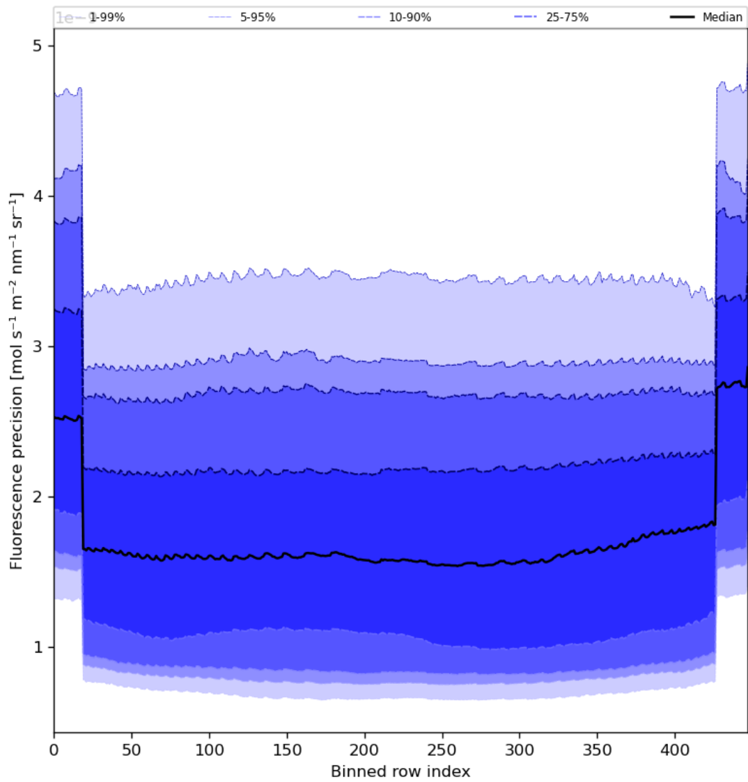
Figure 58: Along track statistics of “Fluorescence precision” for 2024-06-26 to 2024-06-28
