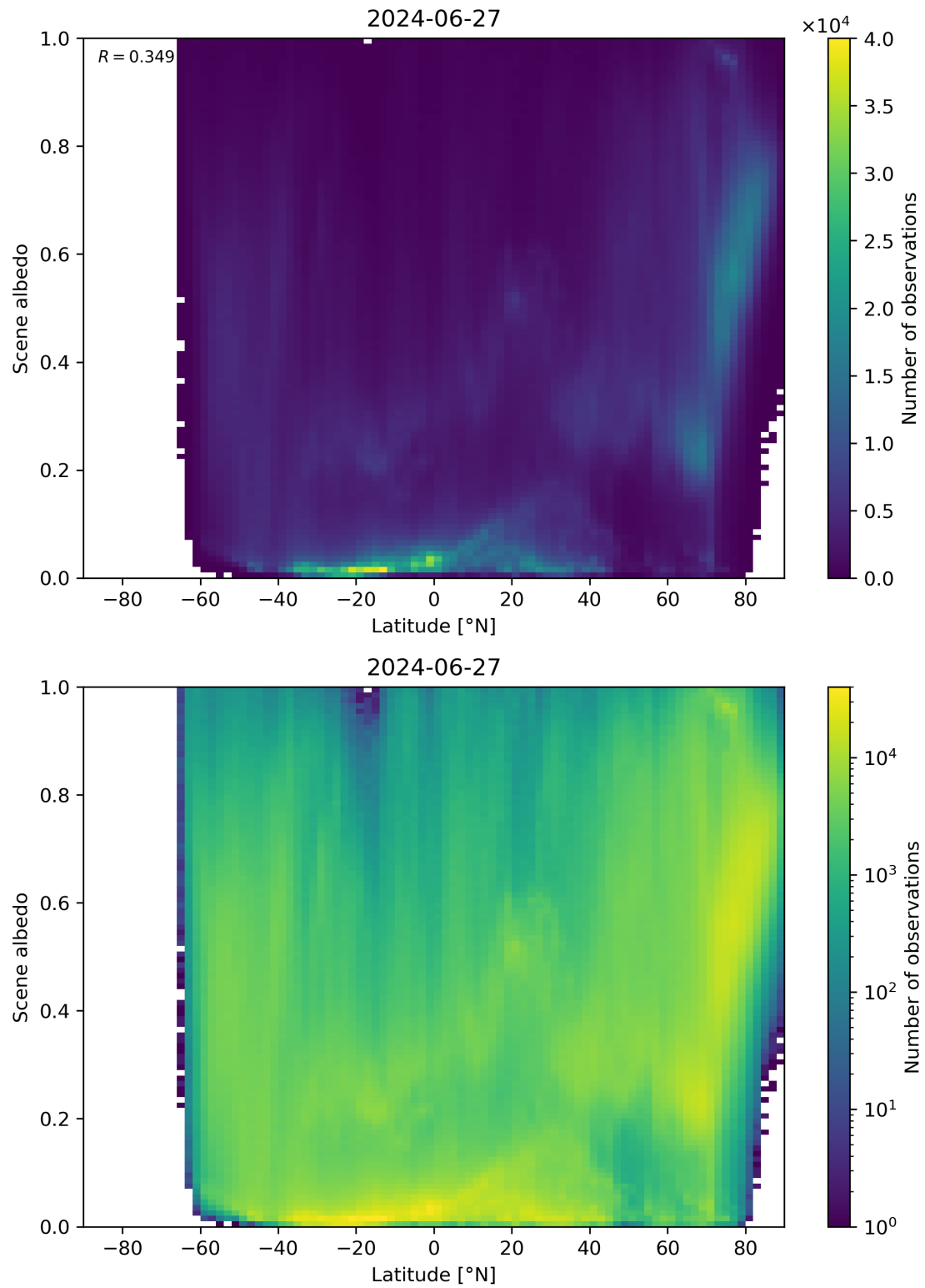
Figure 95: Scatter density plot of “Latitude” against “Scene albedo” for 2024-06-26 to 2024-06-28.
