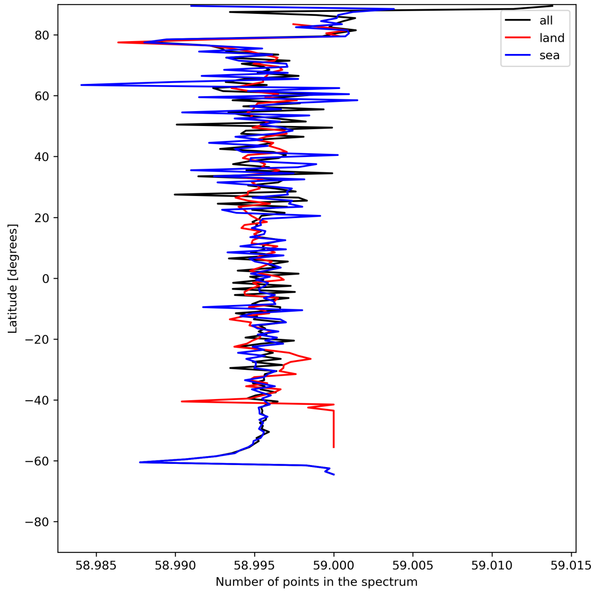
Figure 27: Zonal average of “Number of points in the spectrum” for 2024-06-26 to 2024-06-28.
