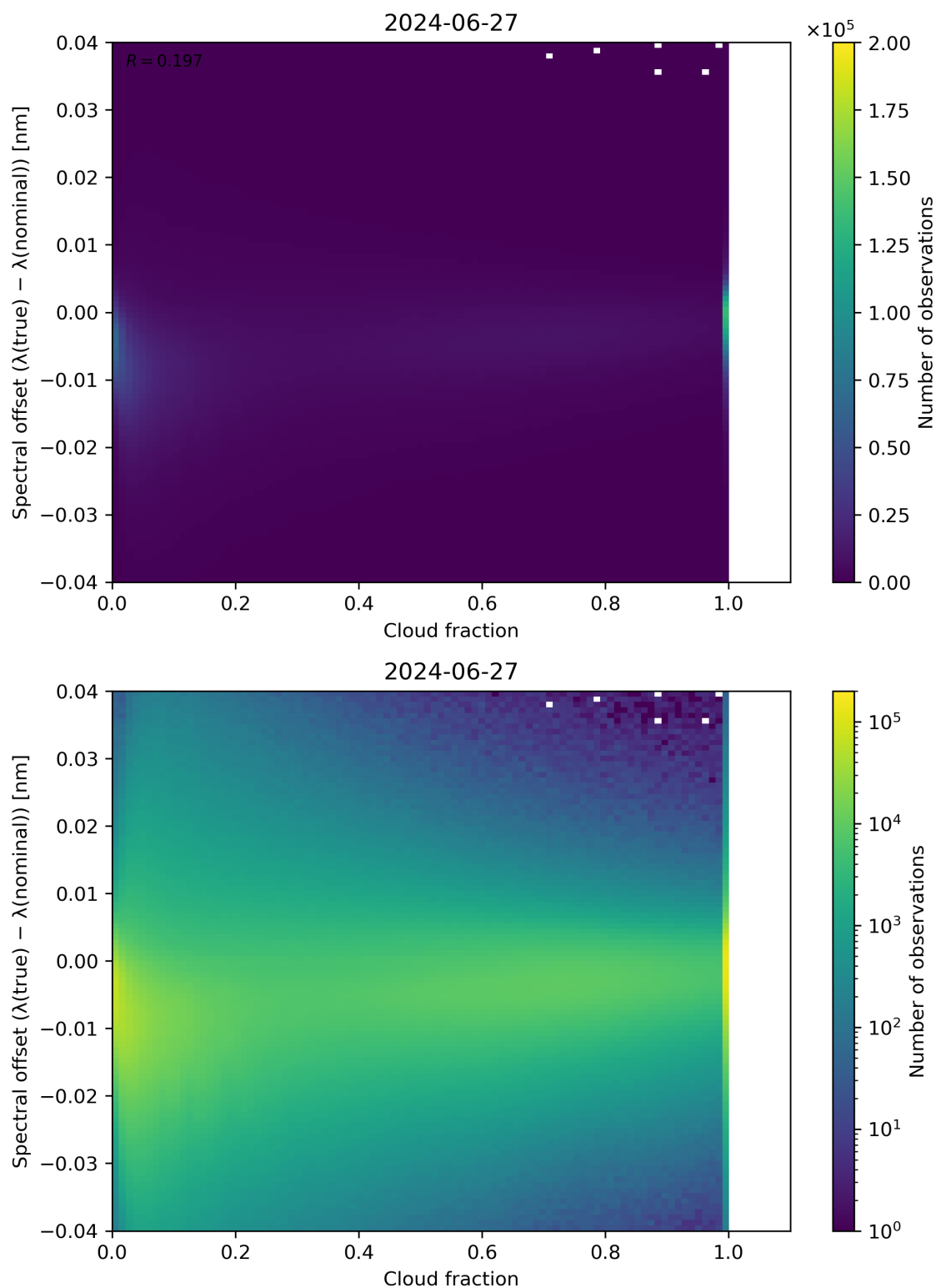
Figure 76: Scatter density plot of “Cloud fraction” against “Spectral offset ( \lambda(\text{true}) - \lambda(\text{nominal}) )” for 2024-06-26 to 2024-06-28.
