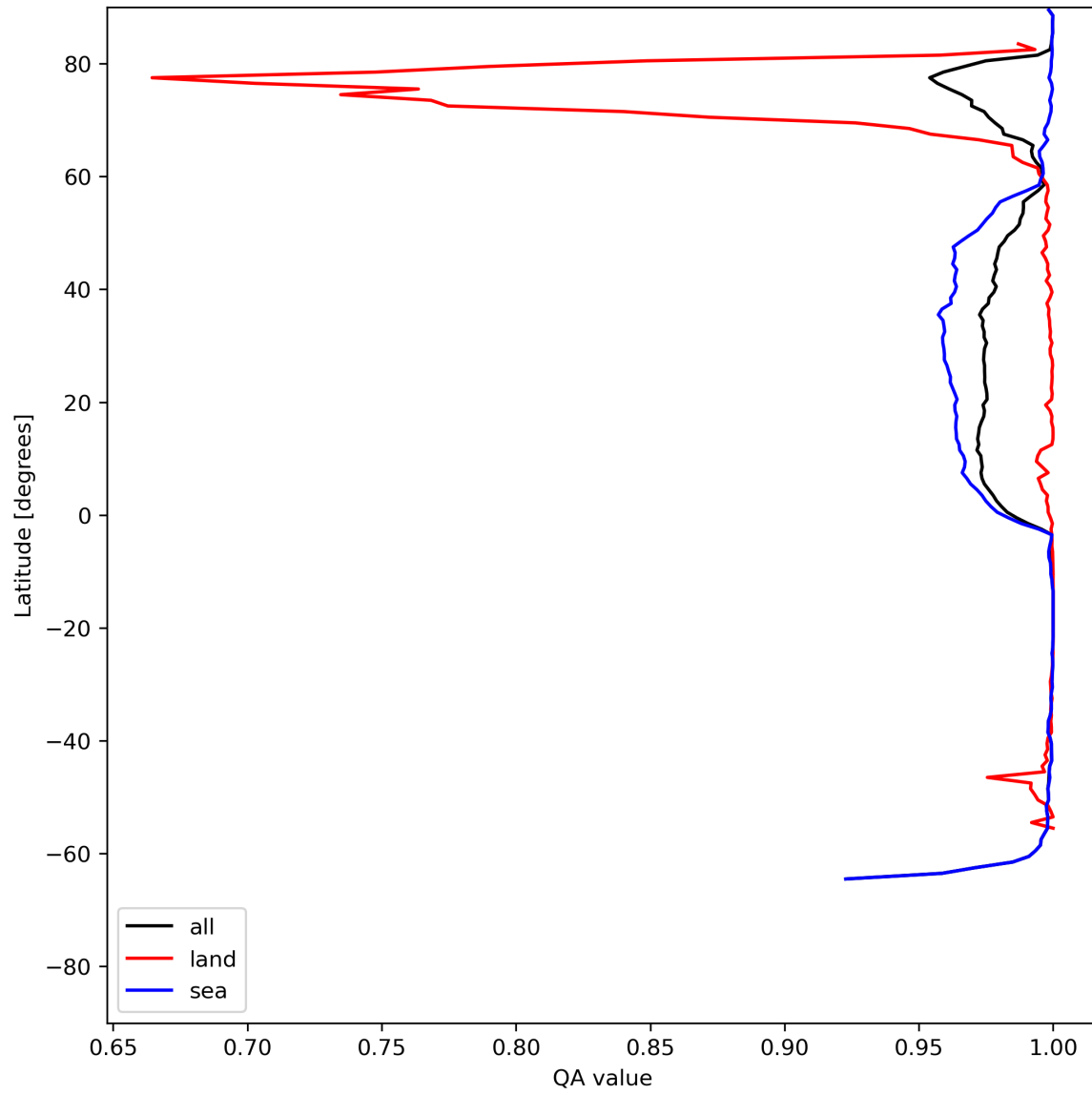
Figure 12: Zonal average of “QA value” for 2024-06-26 to 2024-06-28.
