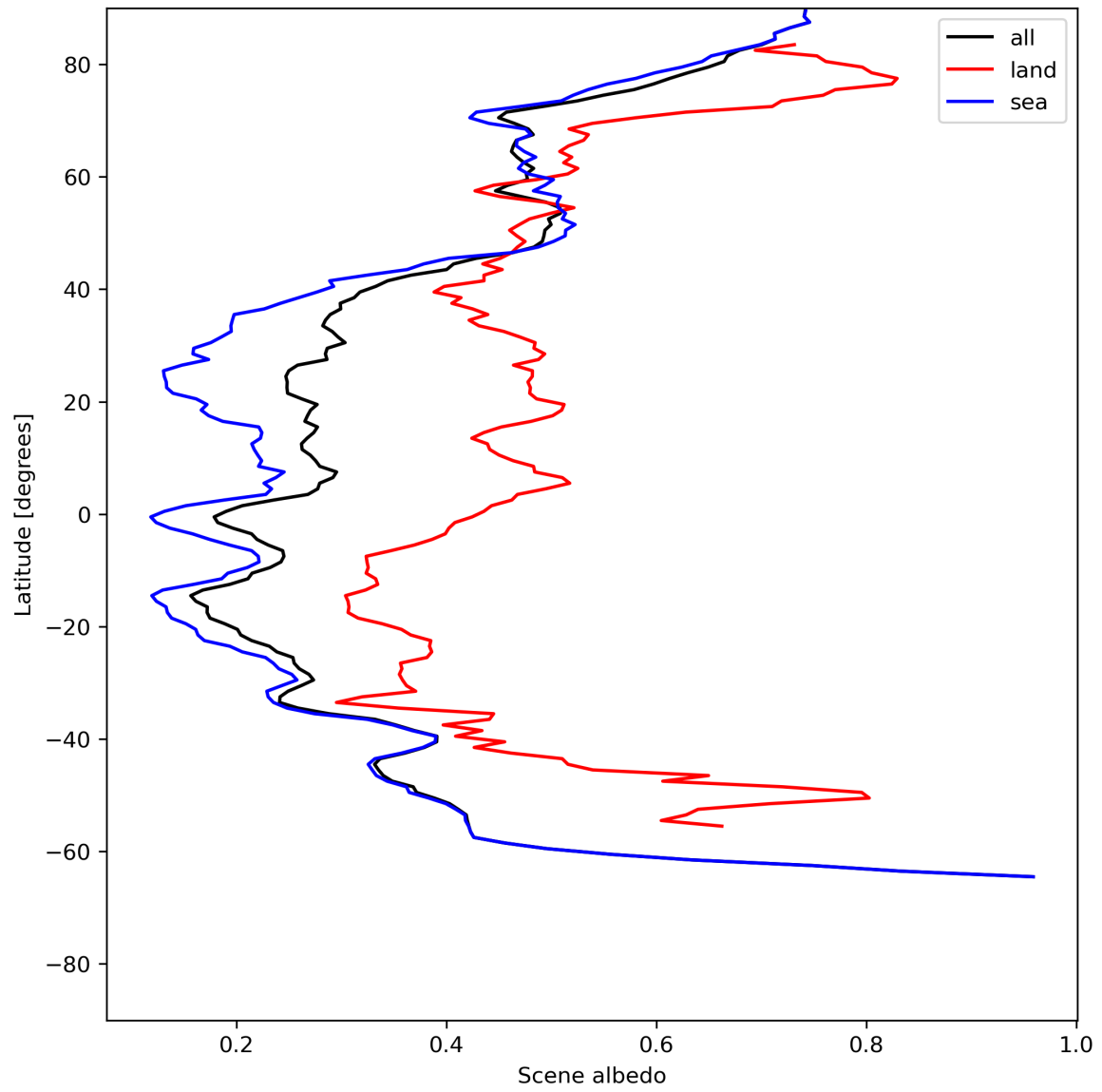
Figure 17: Zonal average of “Scene albedo” for 2024-06-26 to 2024-06-28.
