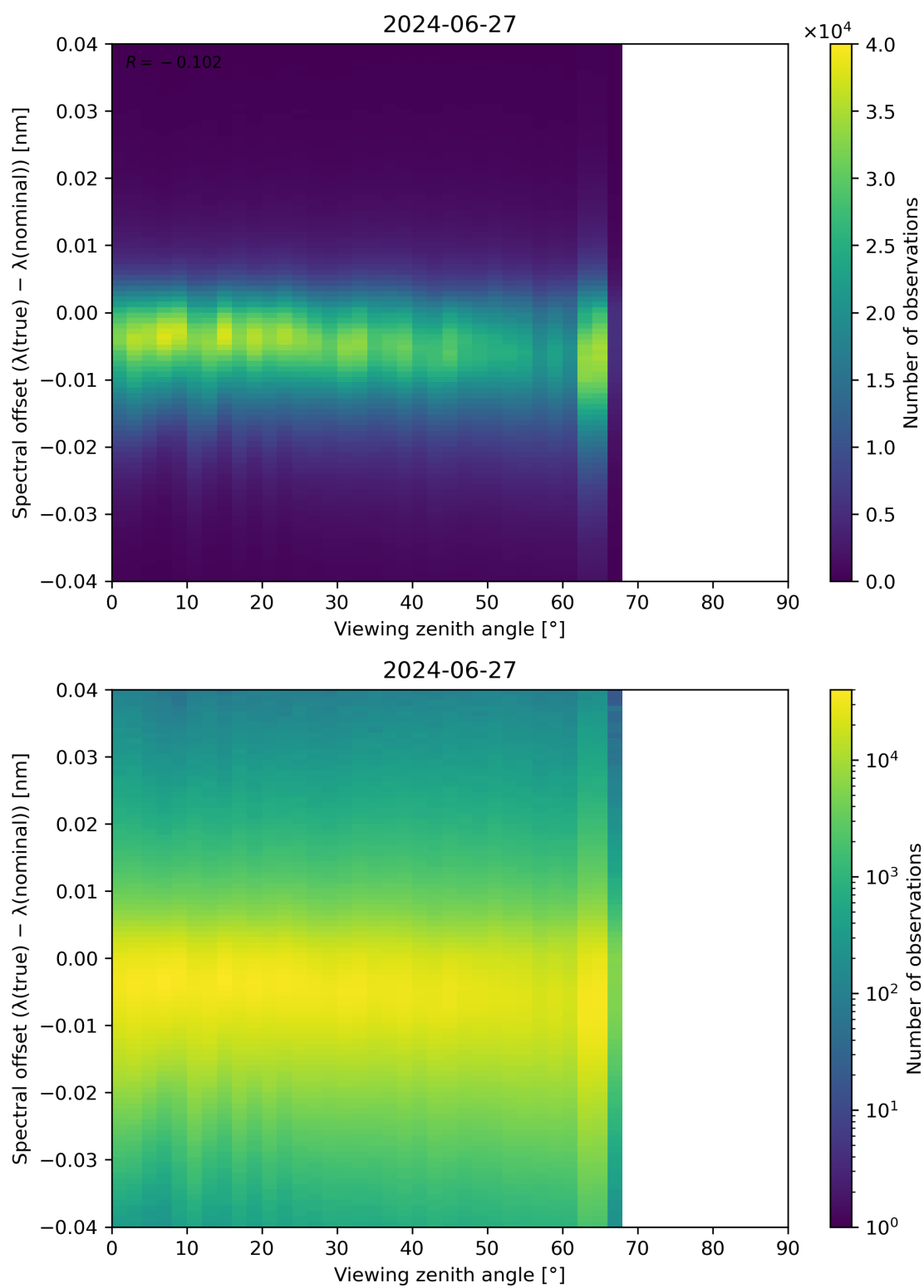
Figure 128: Scatter density plot of “Viewing zenith angle” against “Spectral offset ( \lambda(\text{true}) - \lambda(\text{nominal}) )” for 2024-06-26 to 2024-06-28.
