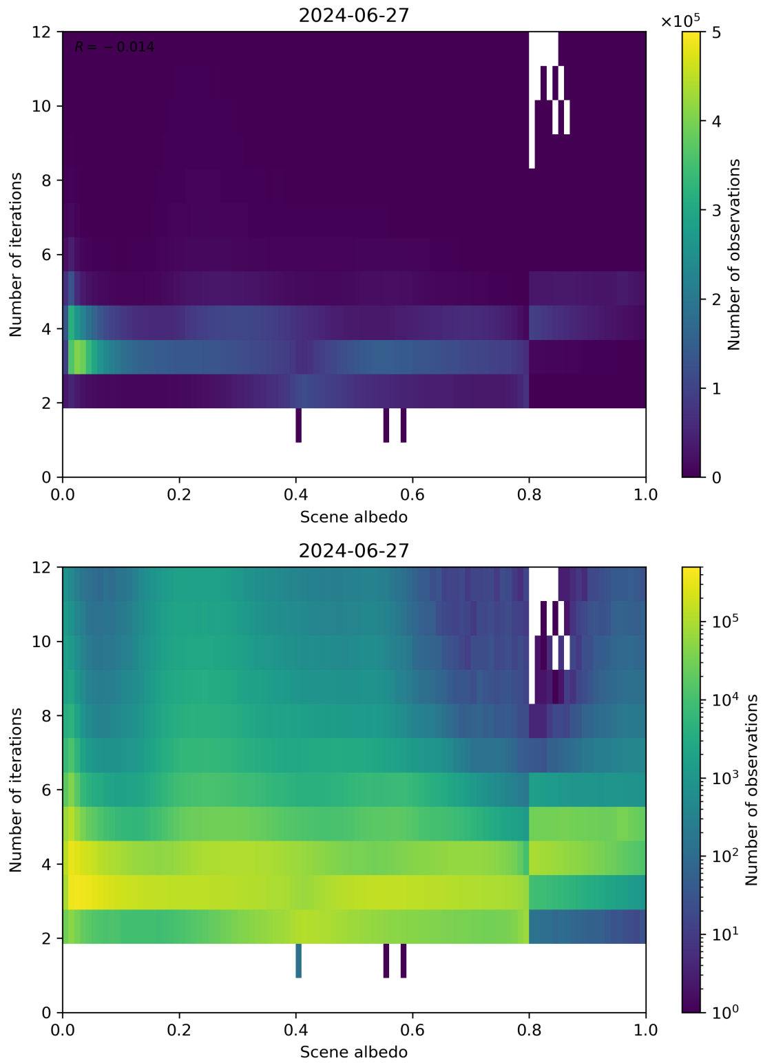
Figure 105: Scatter density plot of “Scene albedo” against “Number of iterations” for 2024-06-26 to 2024-06-28.
