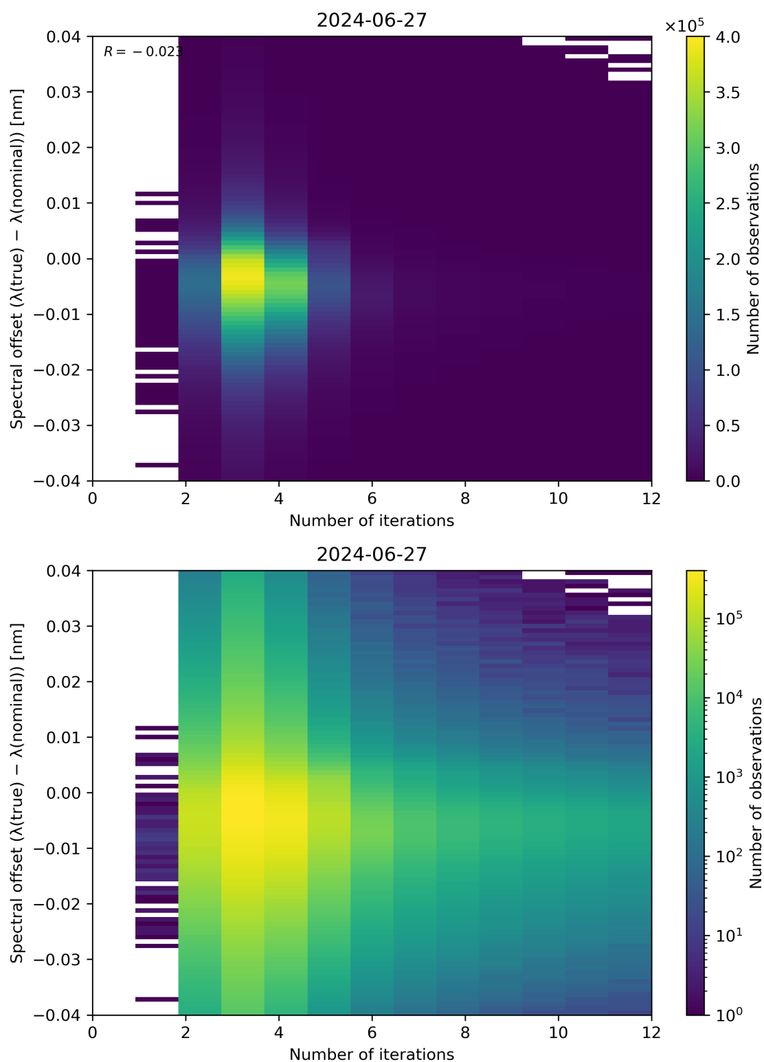
Figure 100: Scatter density plot of “Number of iterations” against “Spectral offset ( \lambda(\text{true}) - \lambda(\text{nominal}) )” for 2024-06-26 to 2024-06-28.
