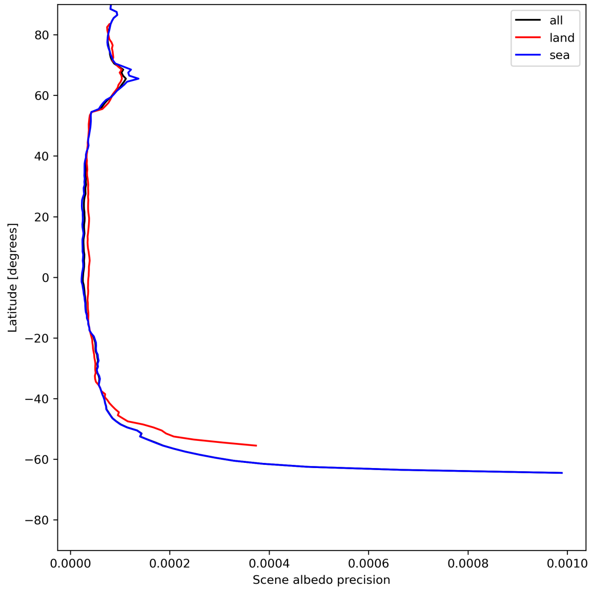
Figure 18: Zonal average of “Scene albedo precision” for 2024-06-26 to 2024-06-28.
