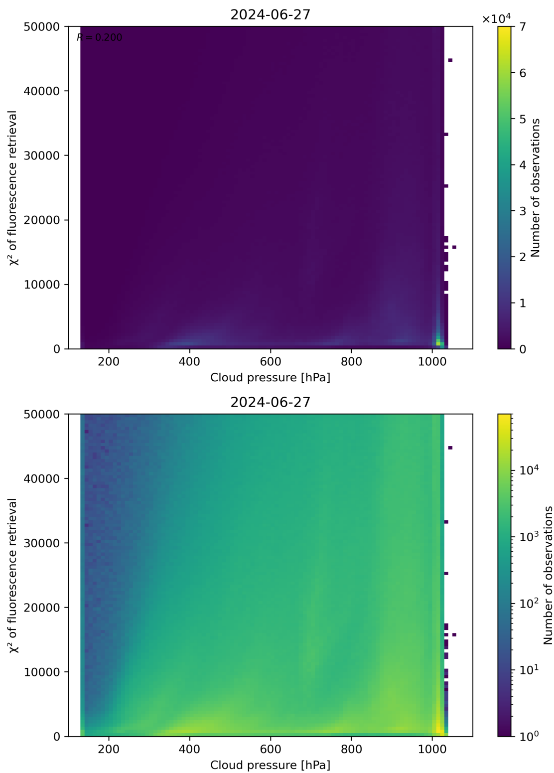
Figure 78: Scatter density plot of “Cloud pressure” against “ \chi^2 of fluorescence retrieval” for 2024-06-26 to 2024-06-28.
