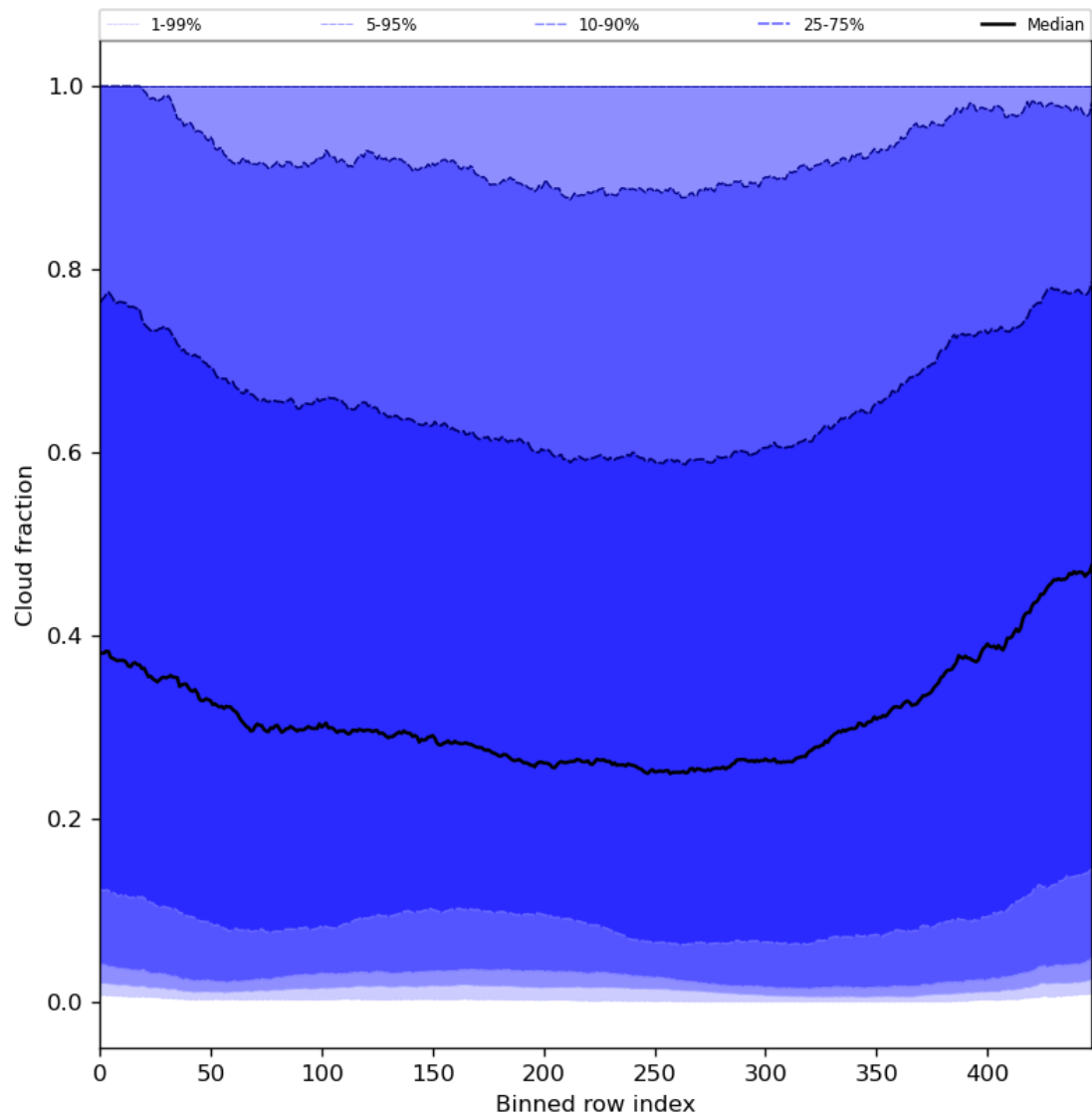
Figure 49: Along track statistics of “Cloud fraction” for 2024-06-26 to 2024-06-28
