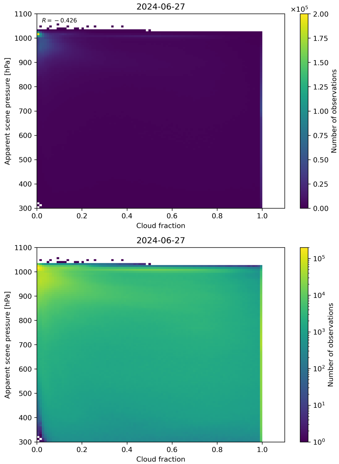
Figure 70: Scatter density plot of “Cloud fraction” against “Apparent scene pressure” for 2024-06-26 to 2024-06-28.
