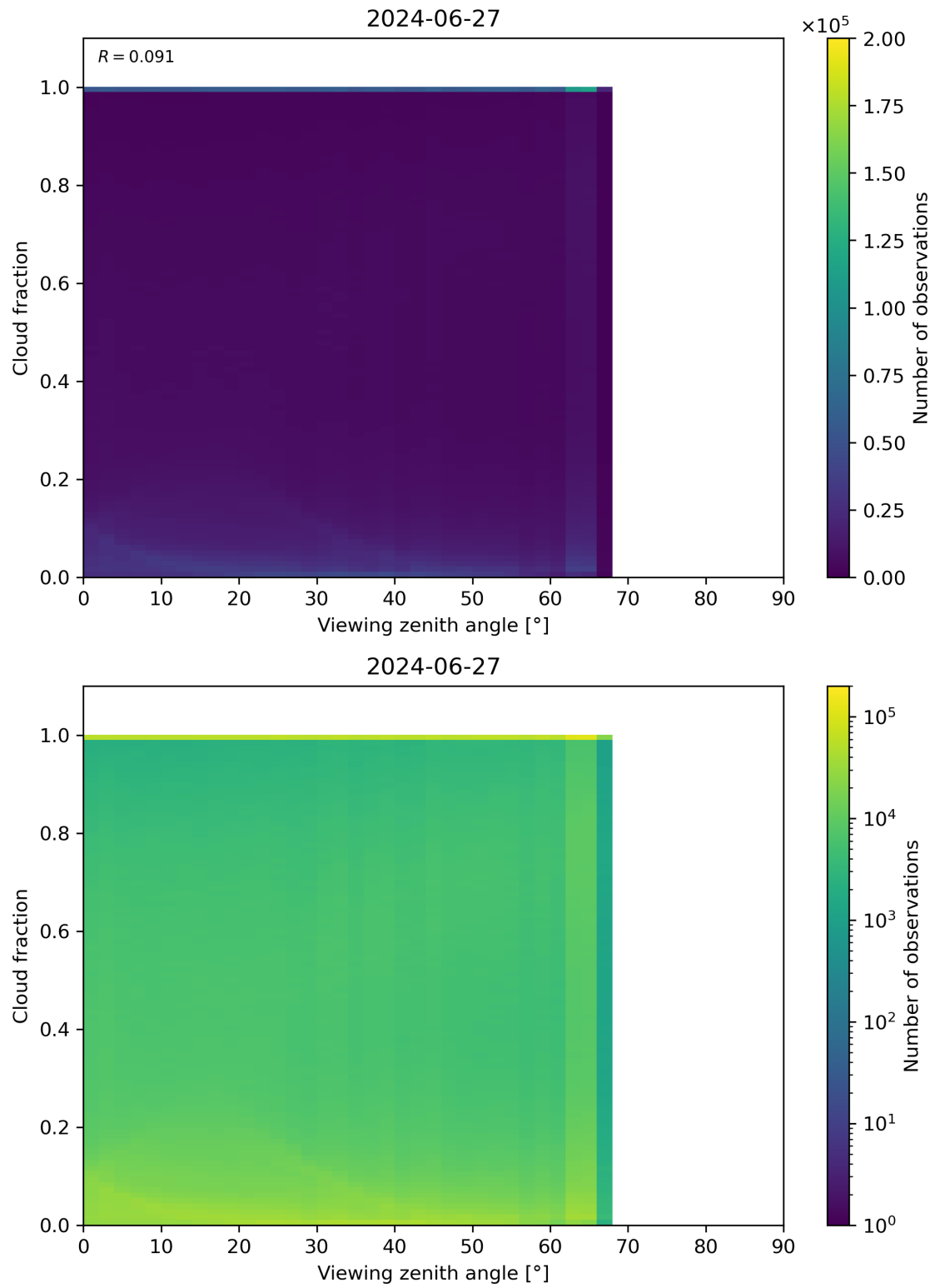
Figure 120: Scatter density plot of “Viewing zenith angle” against “Cloud fraction” for 2024-06-26 to 2024-06-28.
