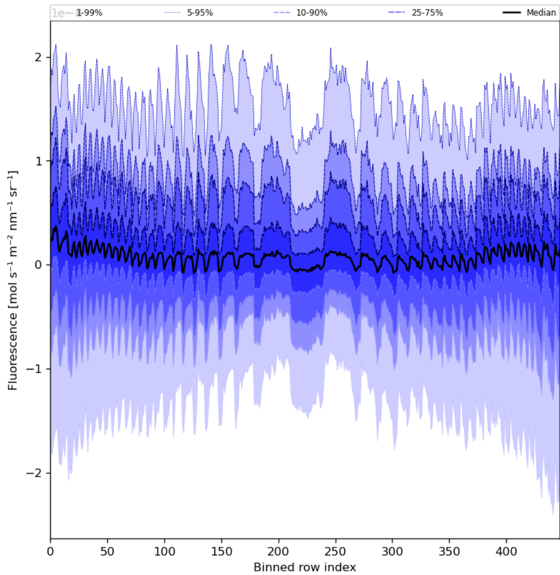
Figure 57: Along track statistics of “Fluorescence” for 2024-06-26 to 2024-06-28
