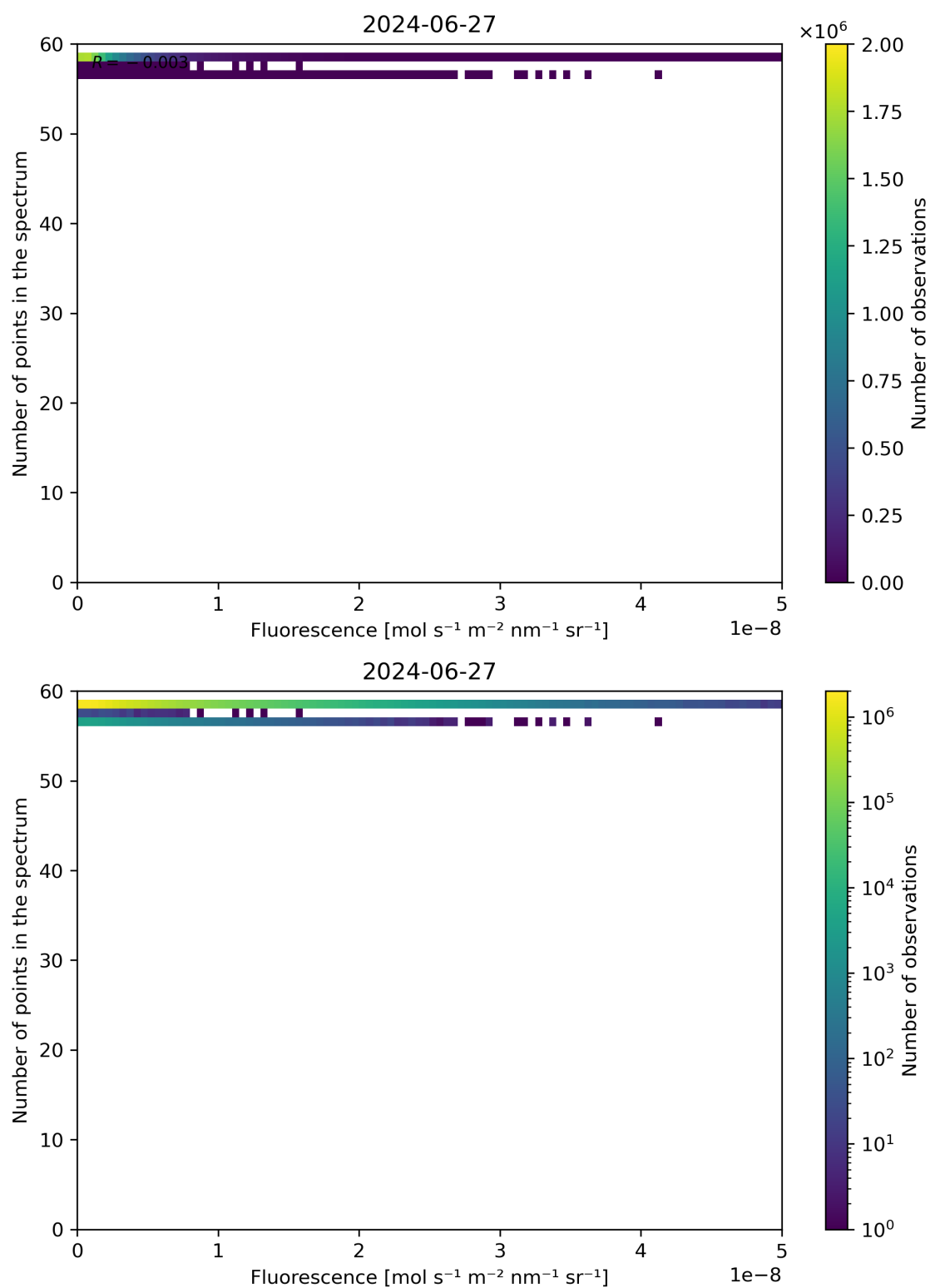
Figure 86: Scatter density plot of “Fluorescence” against “Number of points in the spectrum” for 2024-06-26 to 2024-06-28.
