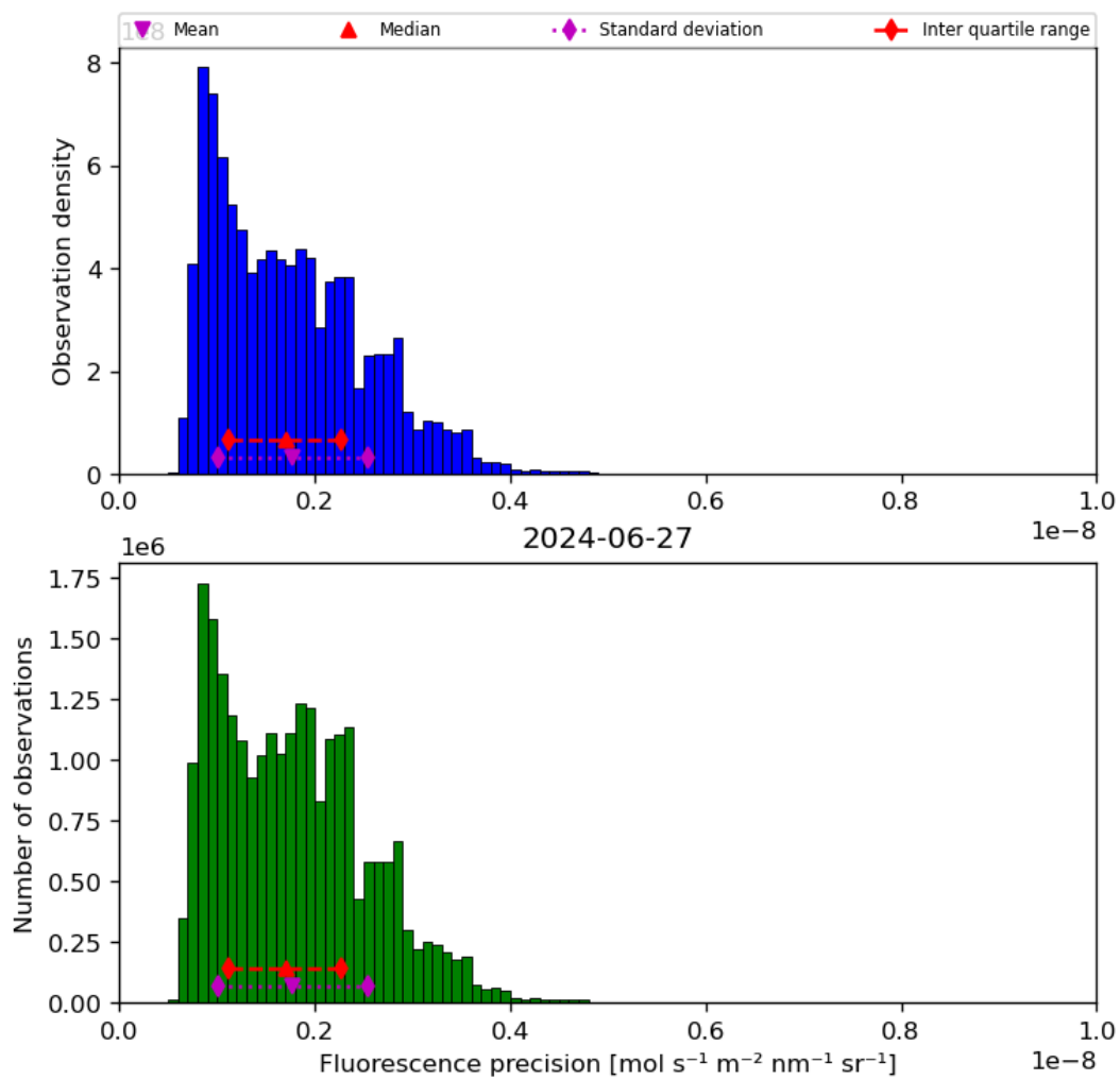
Figure 41: Histogram of “Fluorescence precision” for 2024-06-26 to 2024-06-28
