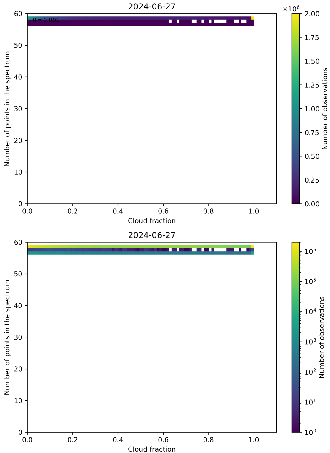
Figure 74: Scatter density plot of “Cloud fraction” against “Number of points in the spectrum” for 2024-06-26 to 2024-06-28.
