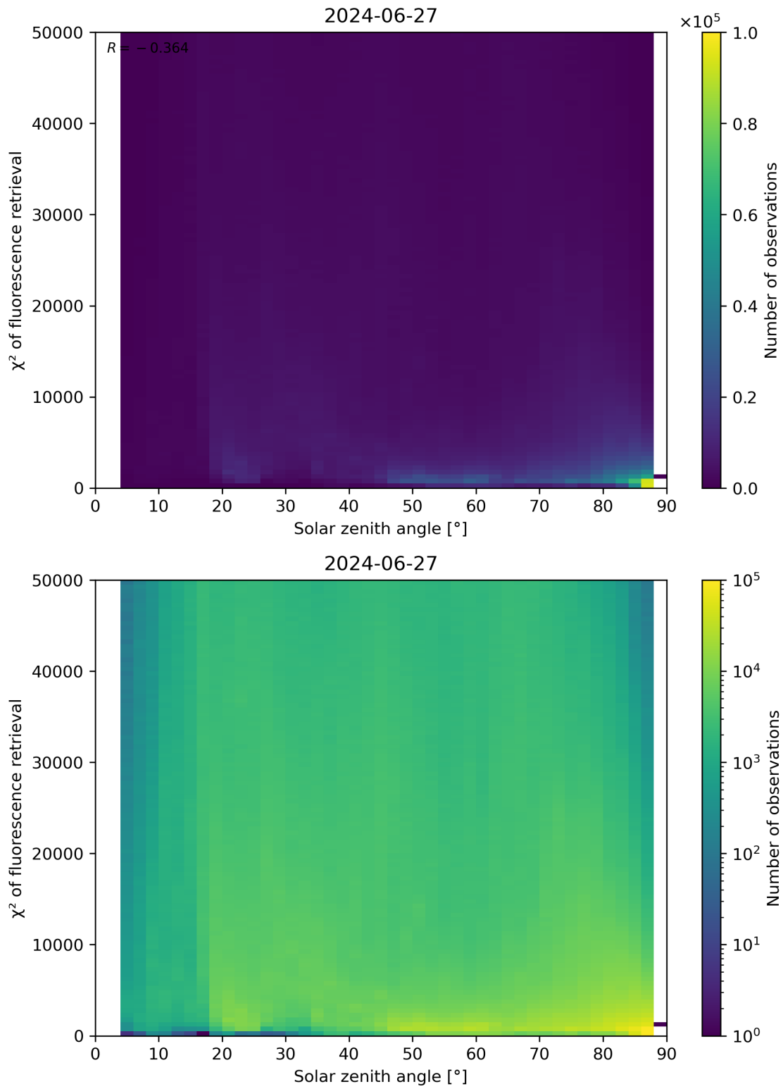
Figure 109: Scatter density plot of “Solar zenith angle” against “ \chi^2 of fluorescence retrieval” for 2024-06-26 to 2024-06-28.
