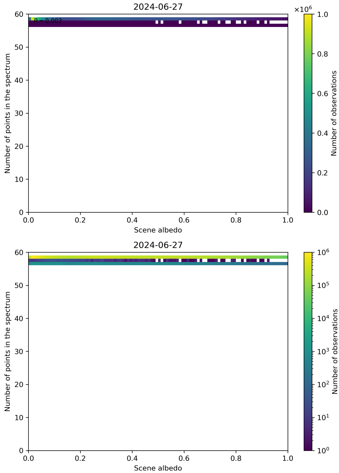
Figure 106: Scatter density plot of “Scene albedo” against “Number of points in the spectrum” for 2024-06-26 to 2024-06-28.
