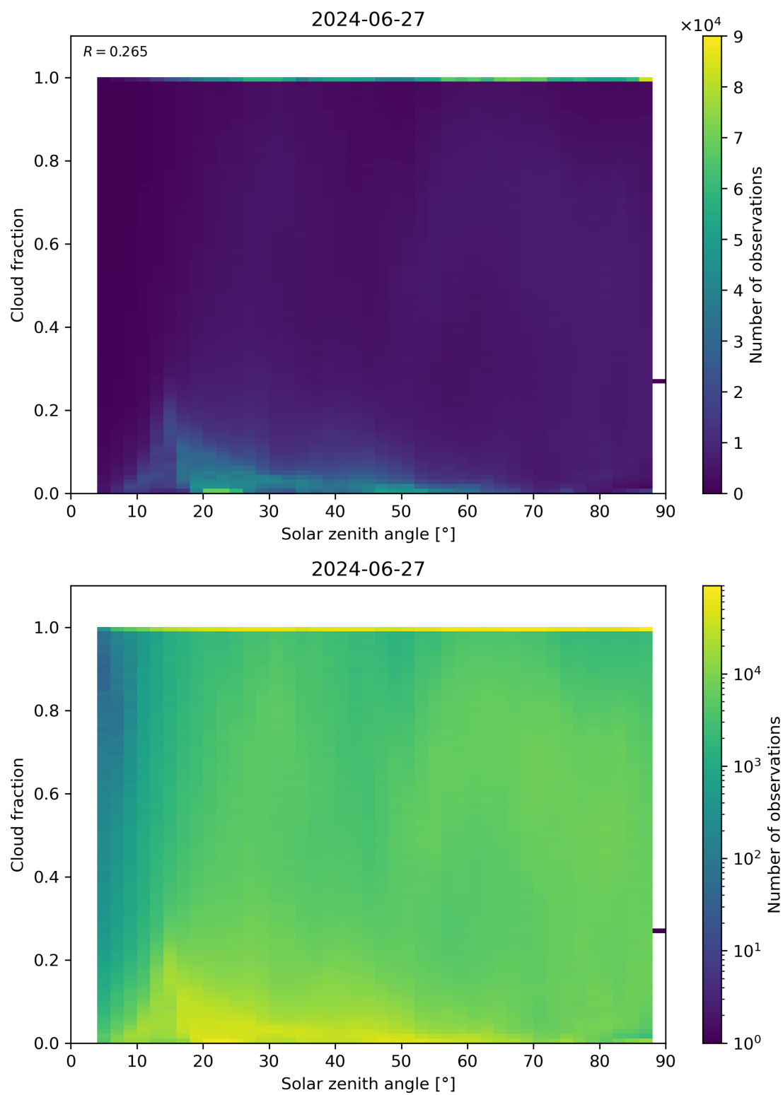
Figure 110: Scatter density plot of “Solar zenith angle” against “Cloud fraction” for 2024-06-26 to 2024-06-28.
