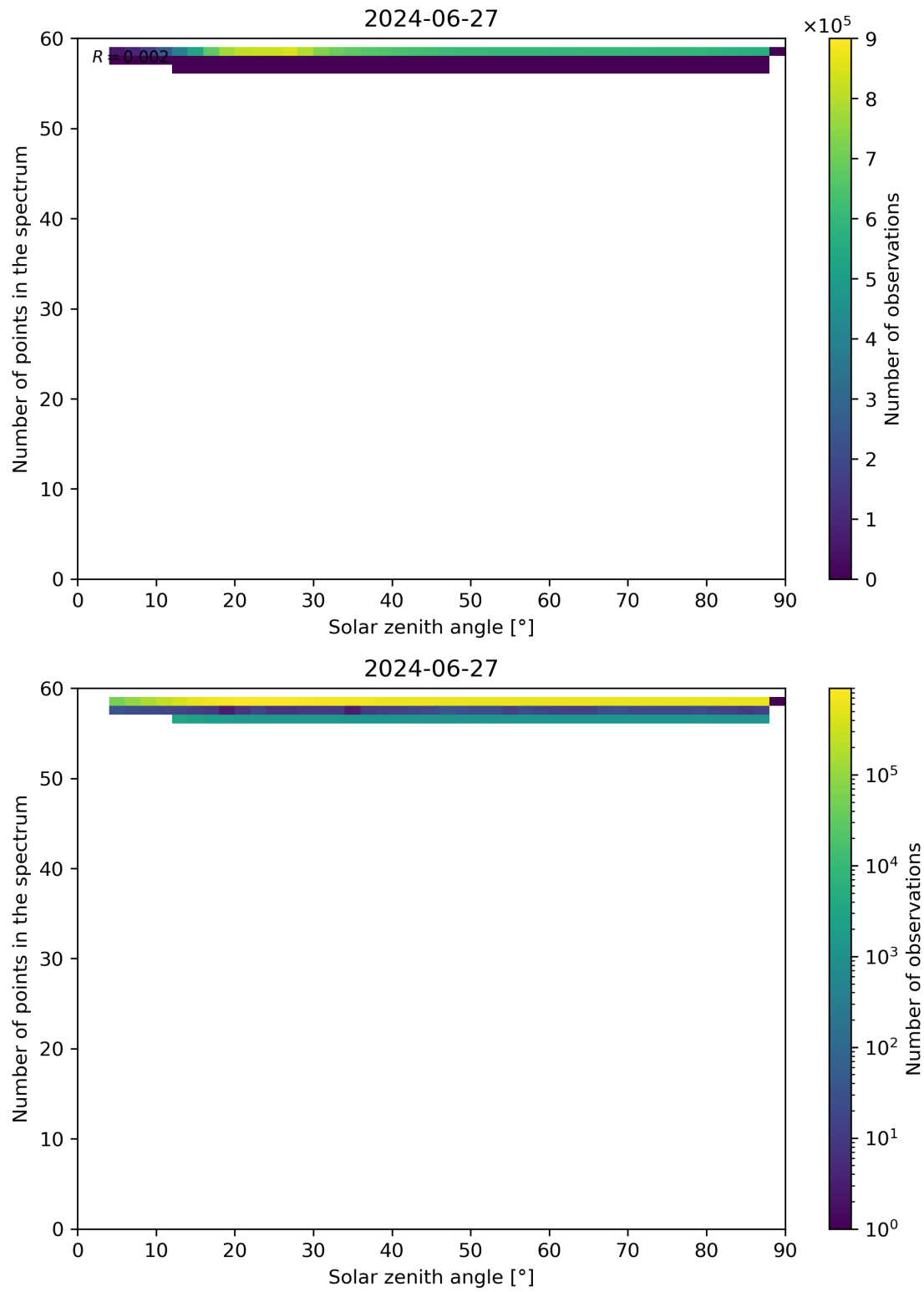
Figure 115: Scatter density plot of “Solar zenith angle” against “Number of points in the spectrum” for 2024-06-26 to 2024-06-28.
