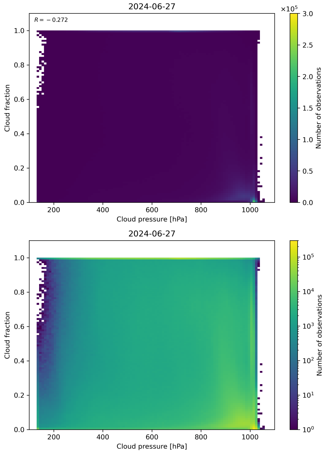
Figure 79: Scatter density plot of “Cloud pressure” against “Cloud fraction” for 2024-06-26 to 2024-06-28.
