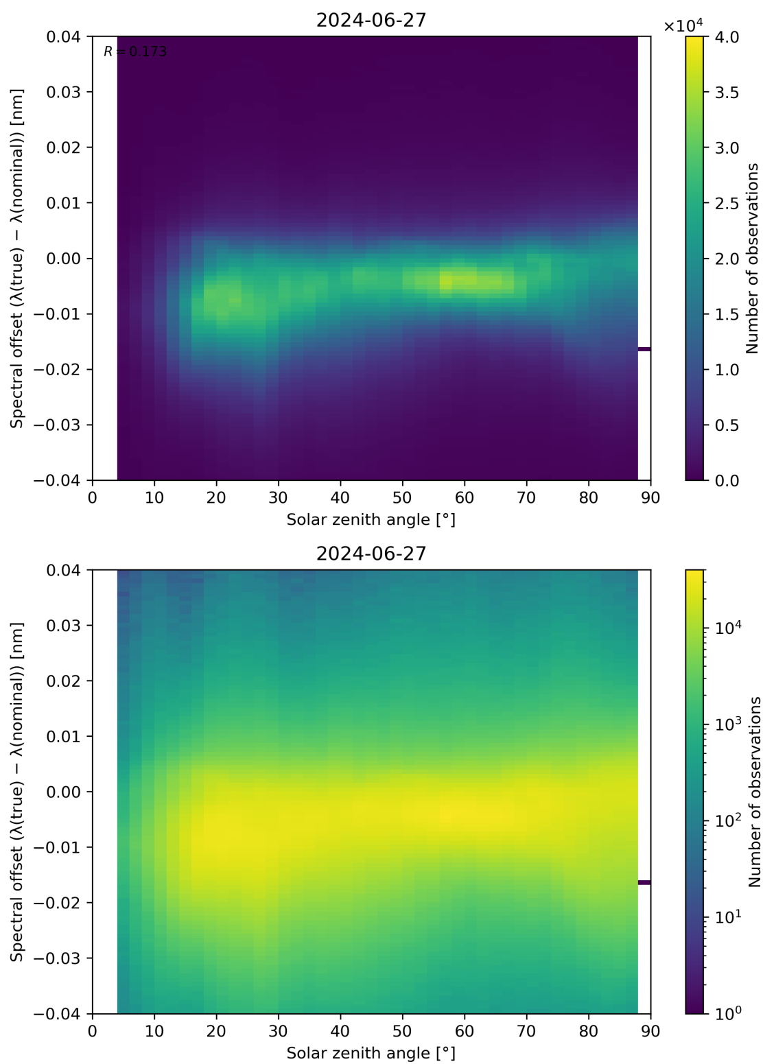
Figure 117: Scatter density plot of “Solar zenith angle” against “Spectral offset ( \lambda(\text{true}) - \lambda(\text{nominal}) )” for 2024-06-26 to 2024-06-28.
