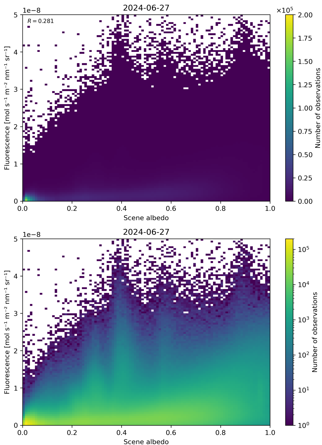
Figure 104: Scatter density plot of “Scene albedo” against “Fluorescence” for 2024-06-26 to 2024-06-28.
