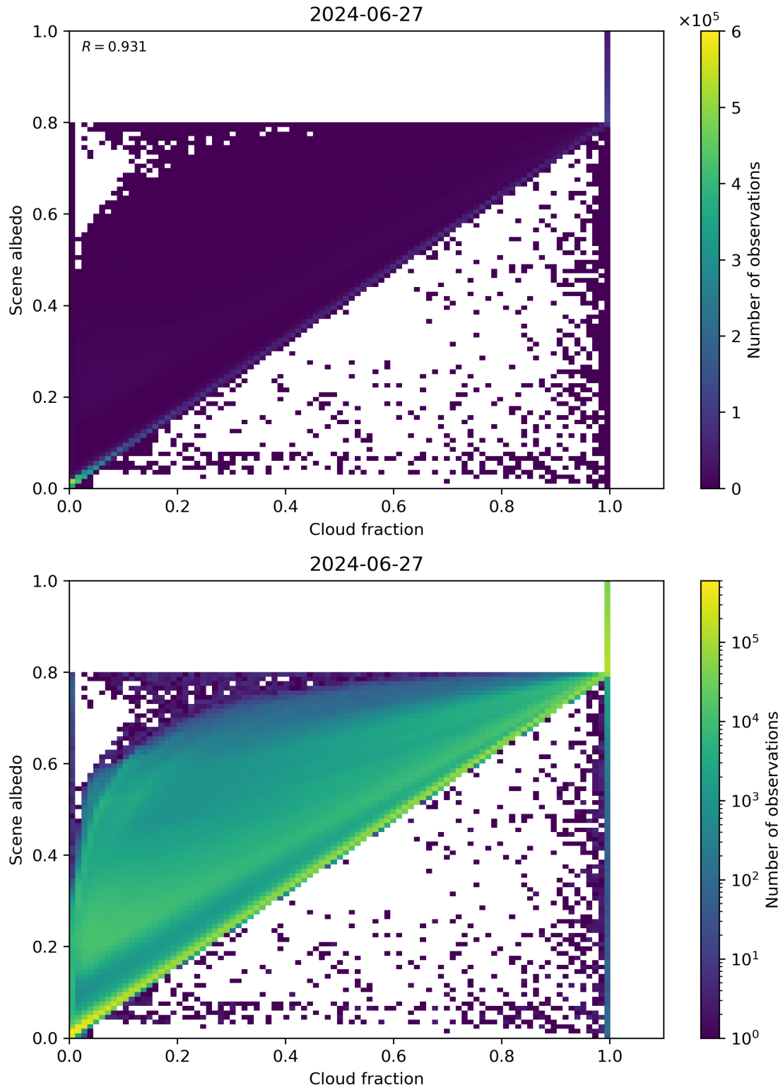
Figure 75: Scatter density plot of “Cloud fraction” against “Scene albedo” for 2024-06-26 to 2024-06-28.
