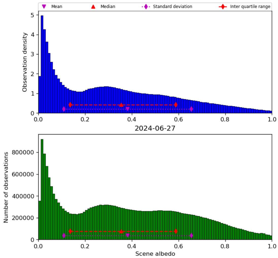
Figure 34: Histogram of “Scene albedo” for 2024-06-26 to 2024-06-28
