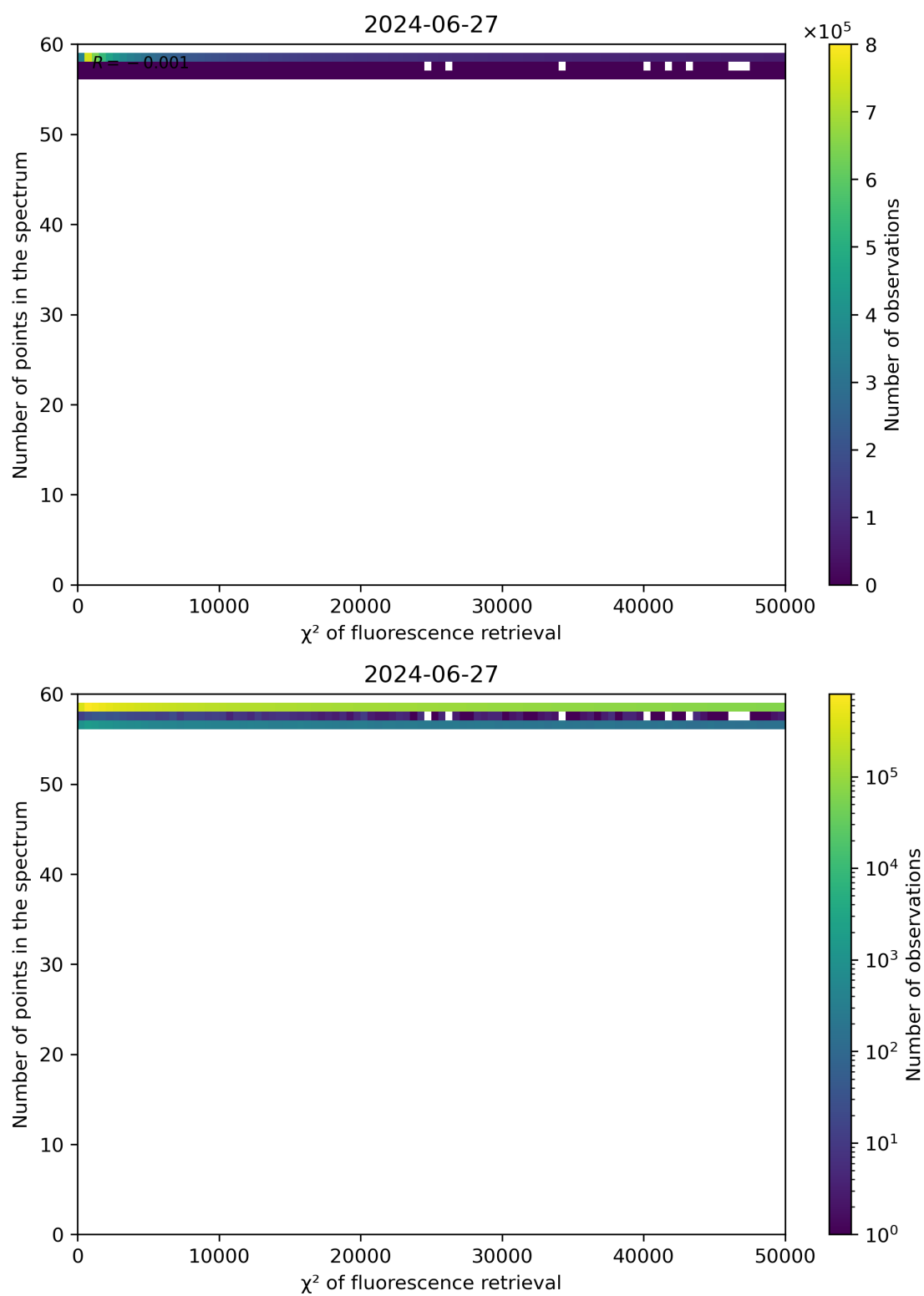
Figure 68: Scatter density plot of " \chi^2 of fluorescence retrieval" against "Number of points in the spectrum" for 2024-06-26 to 2024-06-28.
