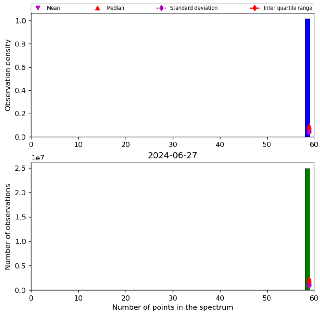
Figure 44: Histogram of “Number of points in the spectrum” for 2024-06-26 to 2024-06-28
