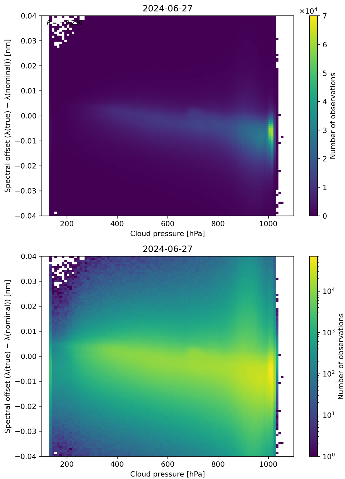
Figure 84: Scatter density plot of “Cloud pressure” against “Spectral offset ( \lambda(\text{true}) - \lambda(\text{nominal}) )” for 2024-06-26 to 2024-06-28.
