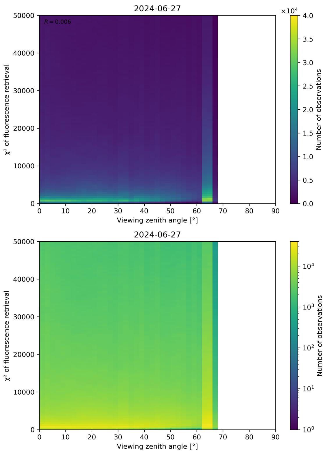
Figure 119: Scatter density plot of “Viewing zenith angle” against “ \chi^2 of fluorescence retrieval” for 2024-06-26 to 2024-06-28.
