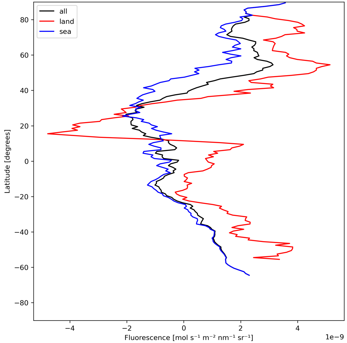
Figure 23: Zonal average of “Fluorescence” for 2024-06-26 to 2024-06-28.
