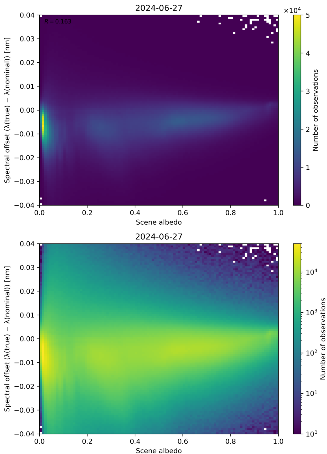
Figure 107: Scatter density plot of “Scene albedo” against “Spectral offset ( \lambda(\text{true}) - \lambda(\text{nominal}) )” for 2024-06-26 to 2024-06-28.
