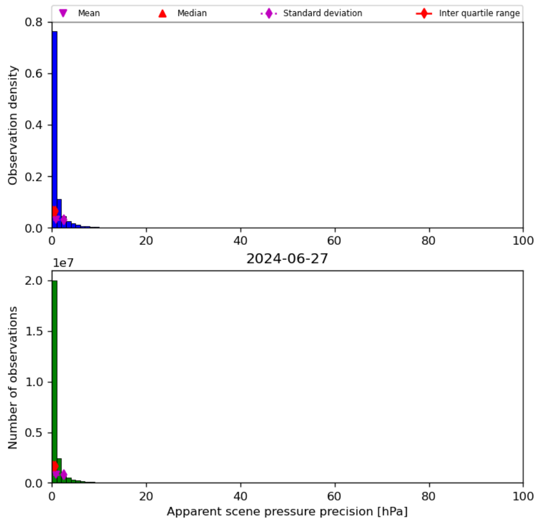
Figure 37: Histogram of “Apparent scene pressure precision” for 2024-06-26 to 2024-06-28
