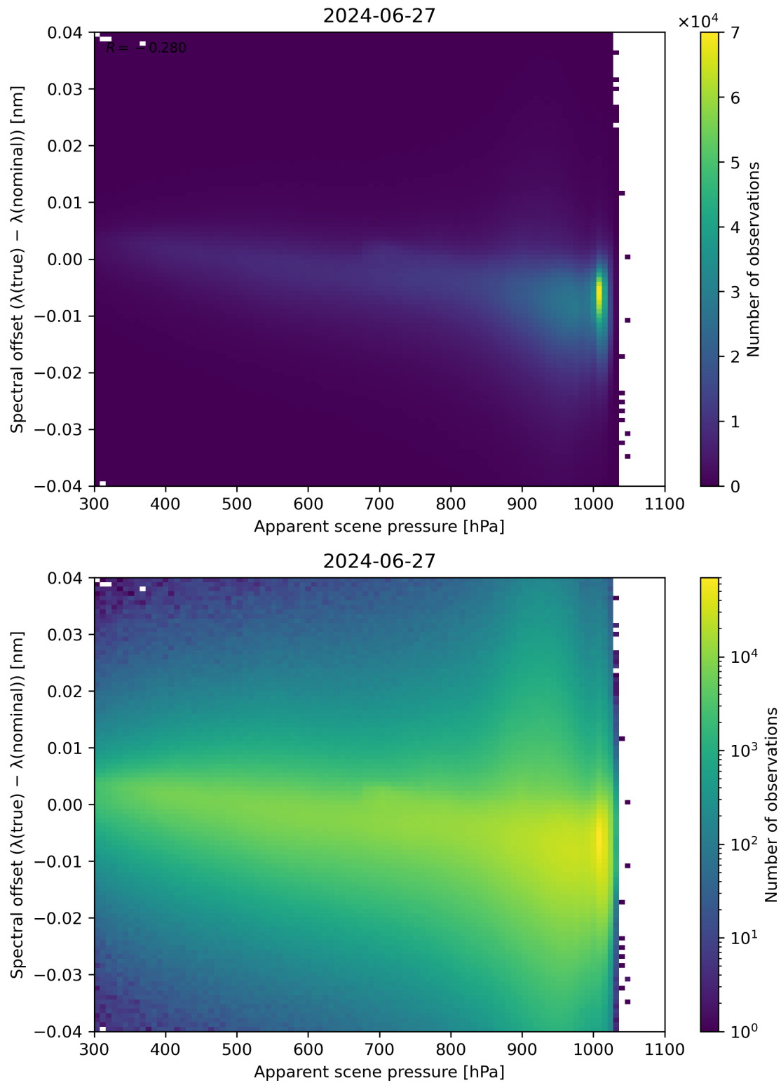
Figure 67: Scatter density plot of “Apparent scene pressure” against “Spectral offset ( \lambda(\text{true}) - \lambda(\text{nominal}) )” for 2024-06-26 to 2024-06-28.
