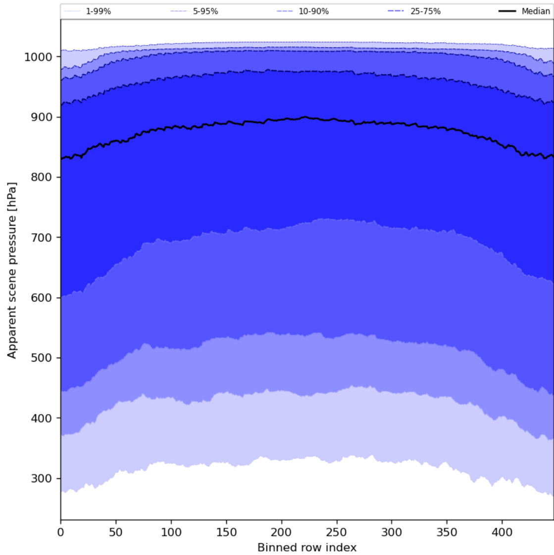
Figure 53: Along track statistics of “Apparent scene pressure” for 2024-06-26 to 2024-06-28
