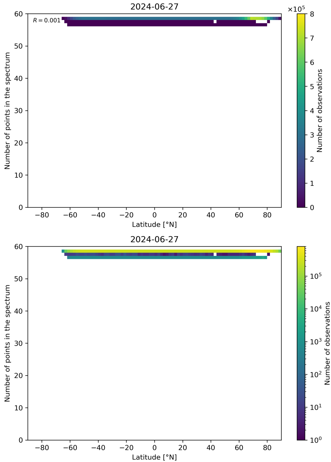
Figure 94: Scatter density plot of “Latitude” against “Number of points in the spectrum” for 2024-06-26 to 2024-06-28.
