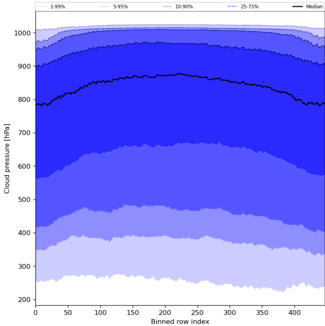
Figure 47: Along track statistics of “Cloud pressure” for 2024-06-26 to 2024-06-28
