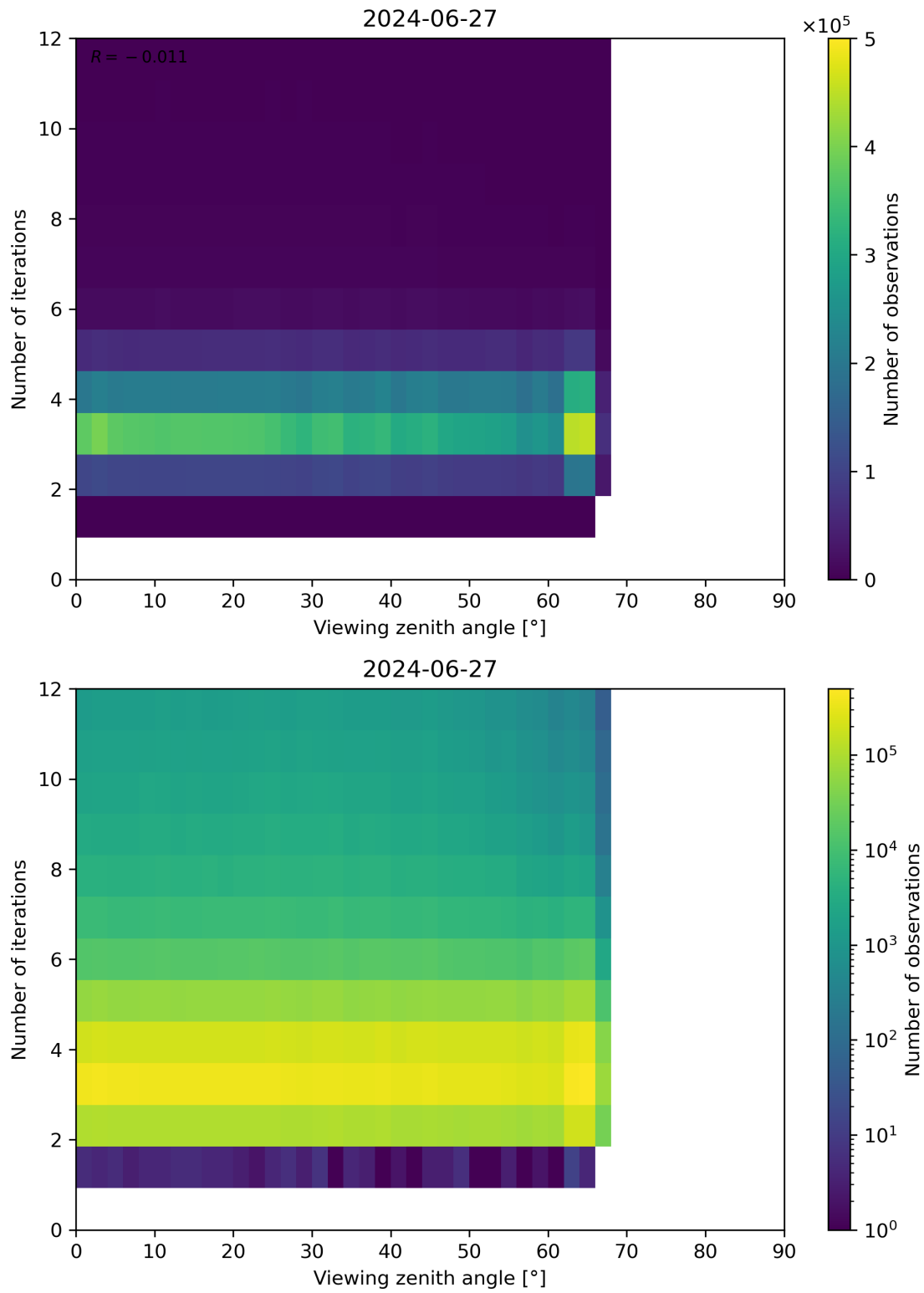
Figure 124: Scatter density plot of “Viewing zenith angle” against “Number of iterations” for 2024-06-26 to 2024-06-28.
