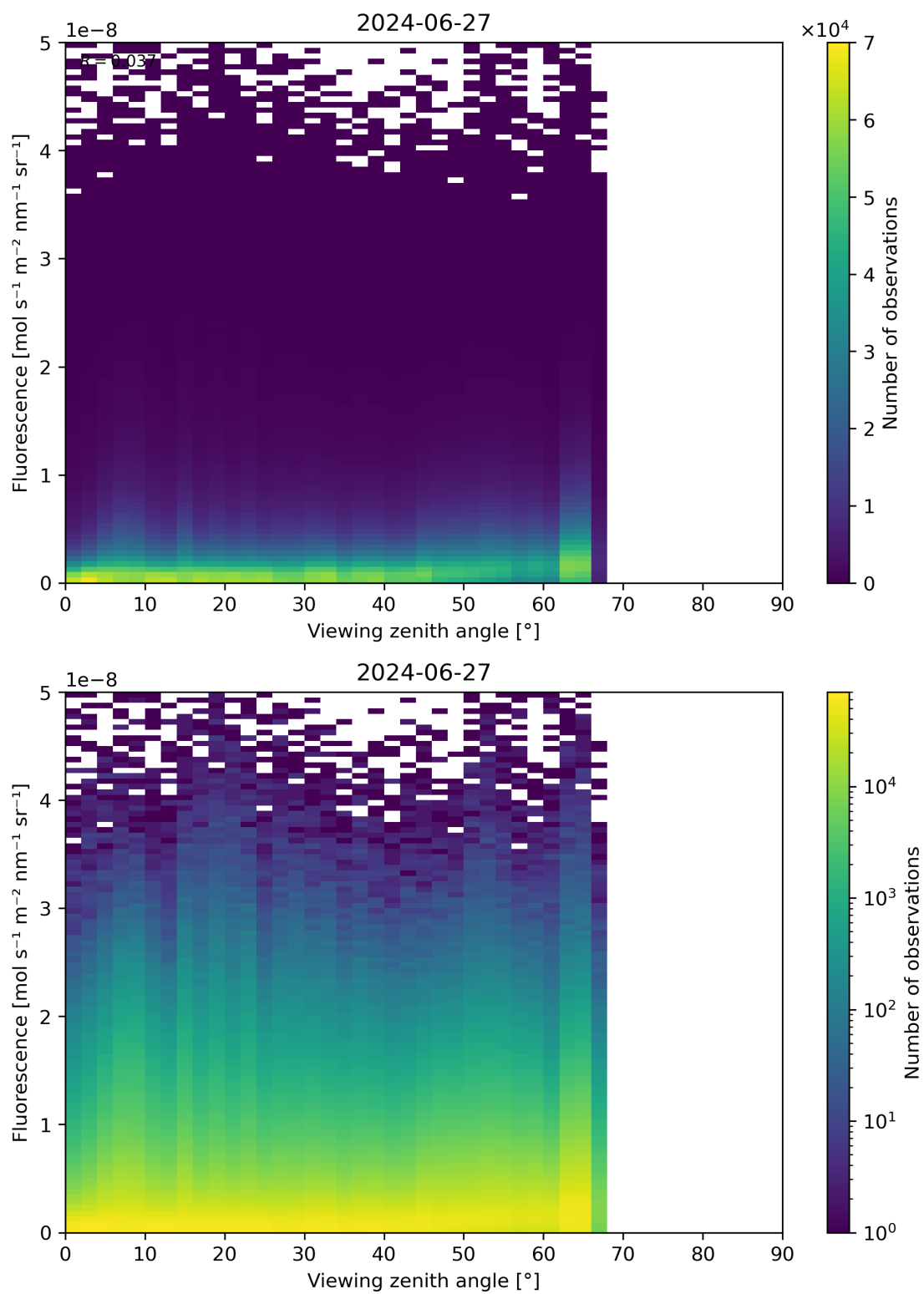
Figure 122: Scatter density plot of “Viewing zenith angle” against “Fluorescence” for 2024-06-26 to 2024-06-28.
