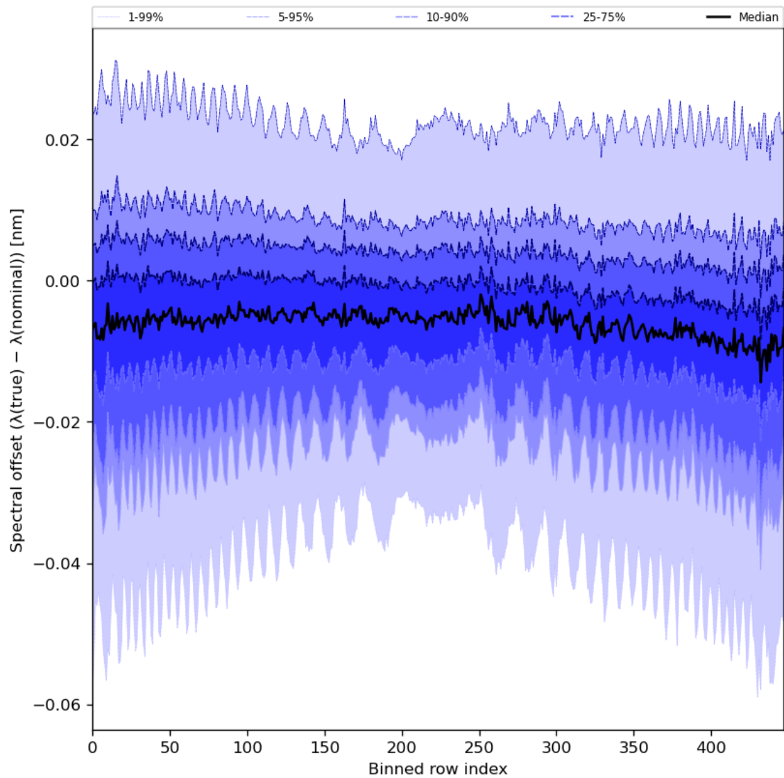
Figure 62: Along track statistics of “Spectral offset ( \lambda(\text{true}) - \lambda(\text{nominal}) )” for 2024-06-26 to 2024-06-28
