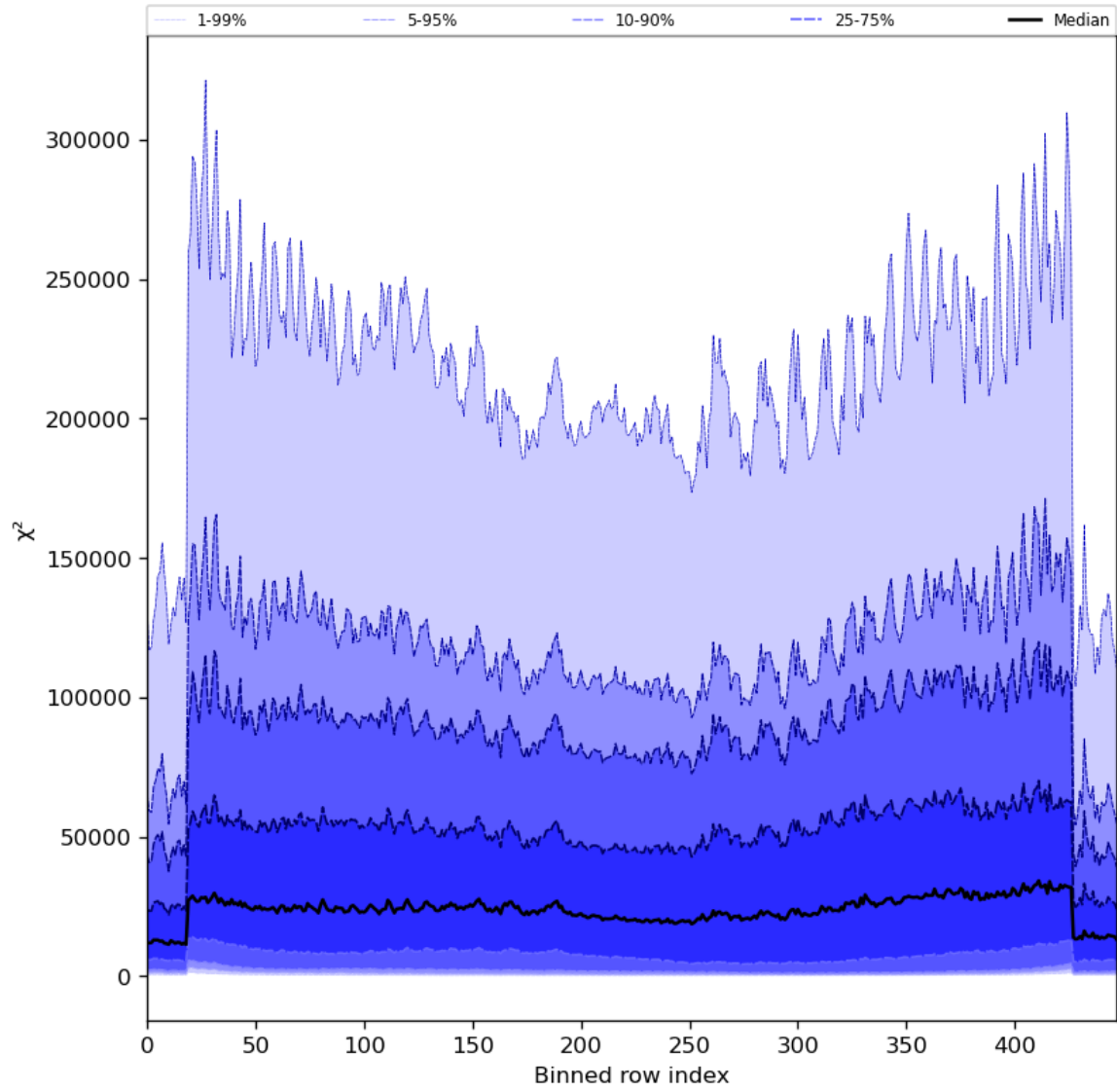
Figure 55: Along track statistics of “ \chi^2 ” for 2024-06-26 to 2024-06-28
