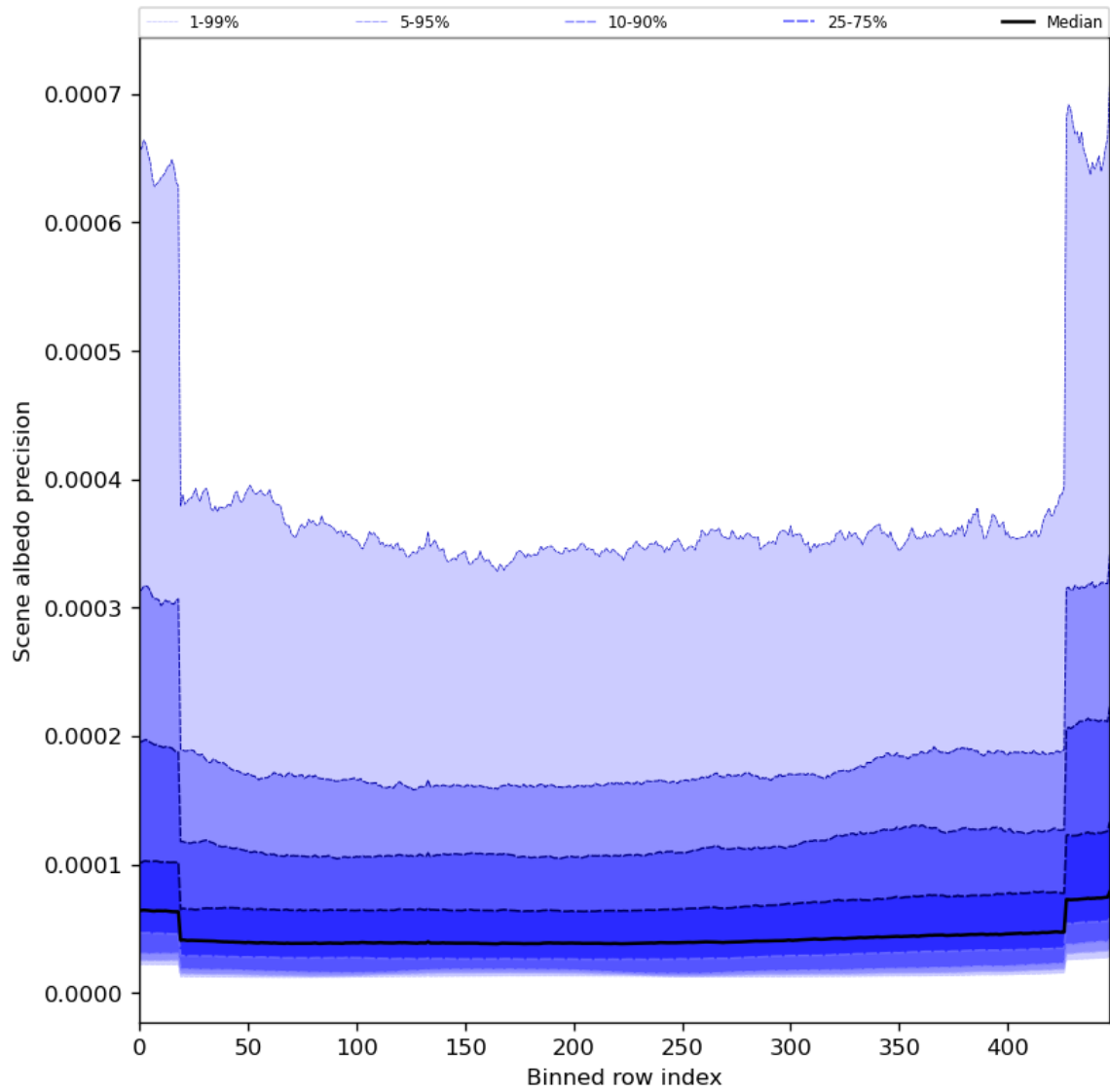
Figure 52: Along track statistics of “Scene albedo precision” for 2024-06-26 to 2024-06-28
