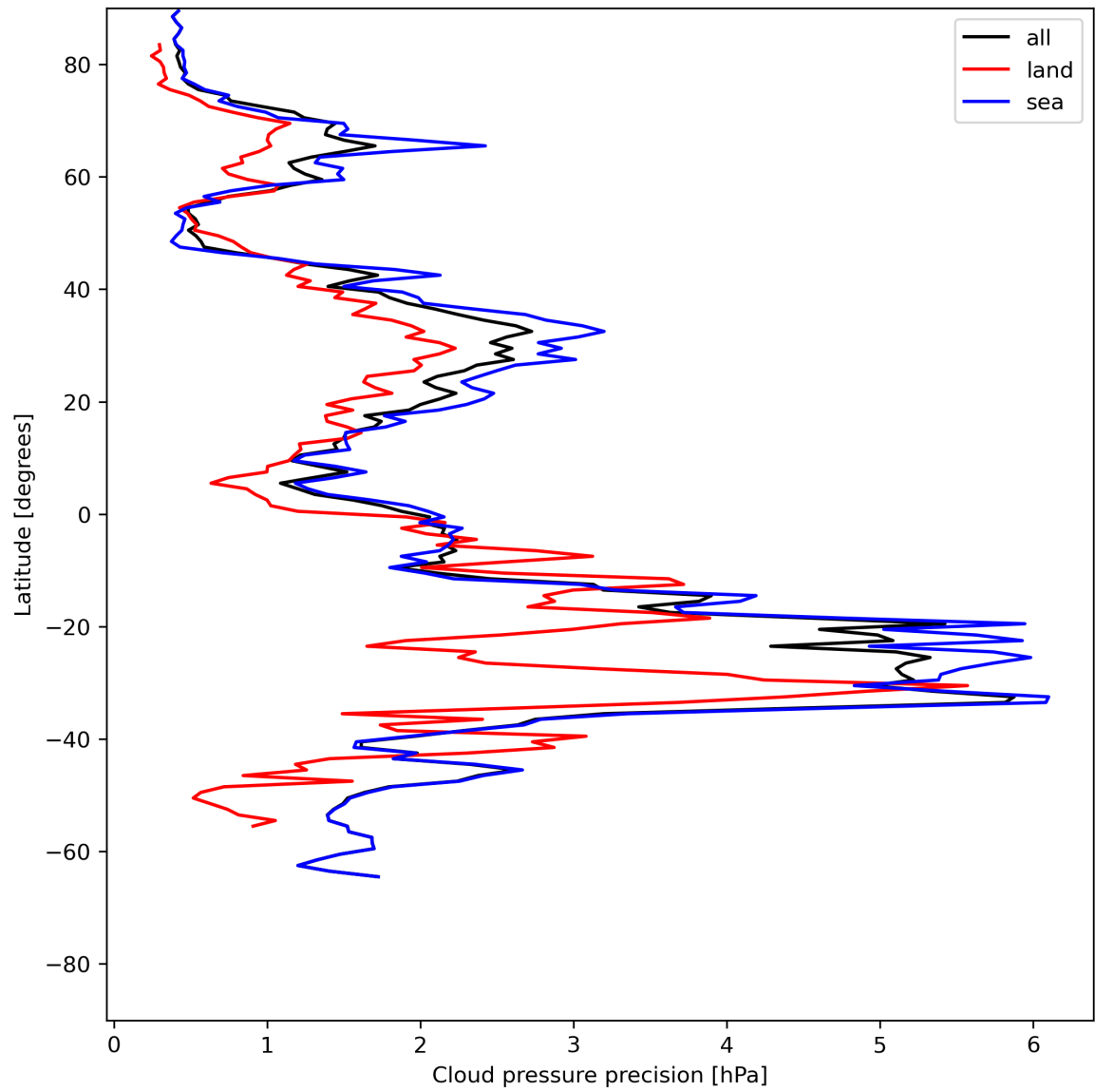
Figure 14: Zonal average of “Cloud pressure precision” for 2024-06-26 to 2024-06-28.
