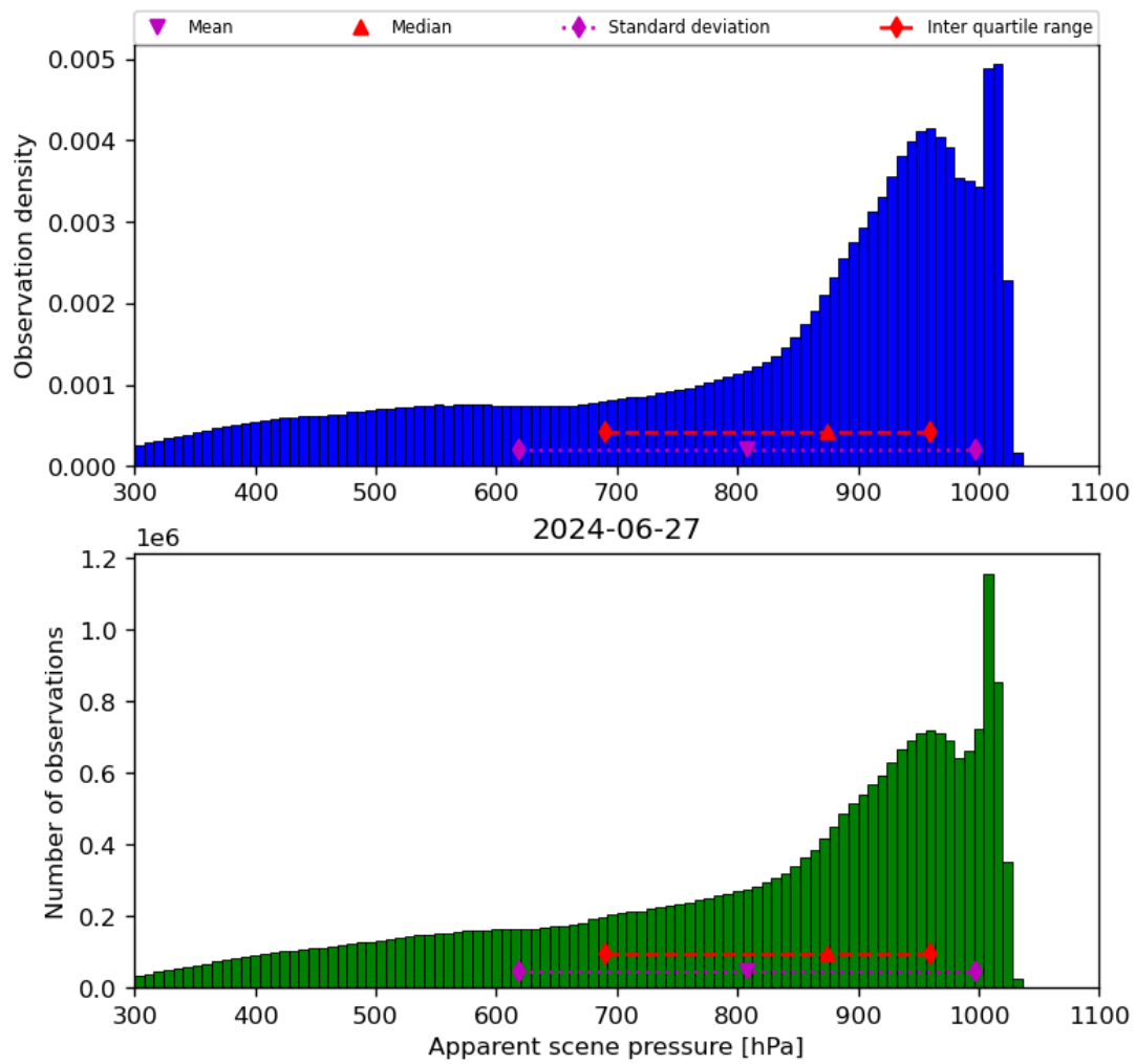
Figure 36: Histogram of “Apparent scene pressure” for 2024-06-26 to 2024-06-28
