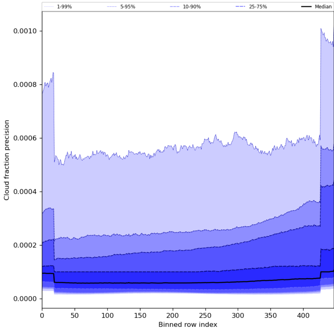
Figure 50: Along track statistics of “Cloud fraction precision” for 2024-06-26 to 2024-06-28
