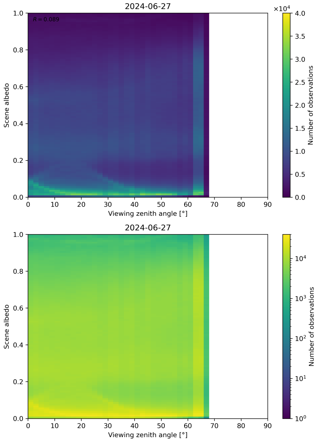
Figure 126: Scatter density plot of “Viewing zenith angle” against “Scene albedo” for 2024-06-26 to 2024-06-28.
