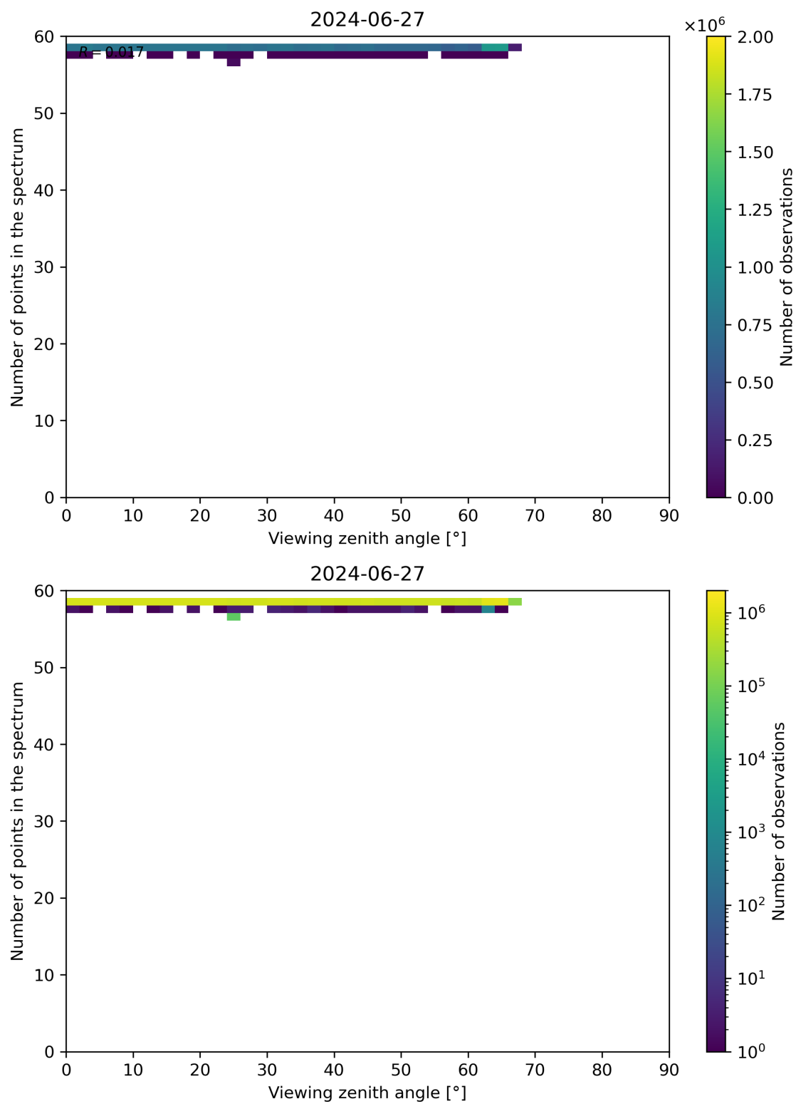
Figure 125: Scatter density plot of “Viewing zenith angle” against “Number of points in the spectrum” for 2024-06-26 to 2024-06-28.
