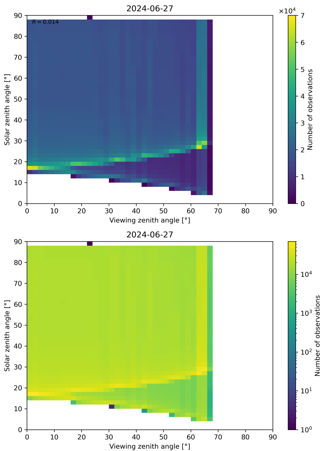
Figure 127: Scatter density plot of “Viewing zenith angle” against “Solar zenith angle” for 2024-06-26 to 2024-06-28.
