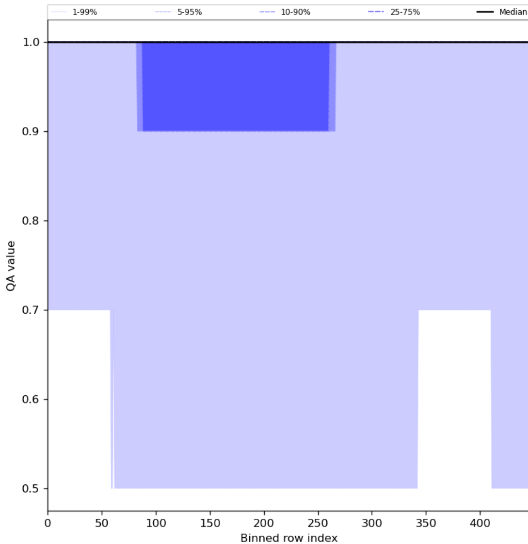
Figure 46: Along track statistics of “QA value” for 2024-06-26 to 2024-06-28
