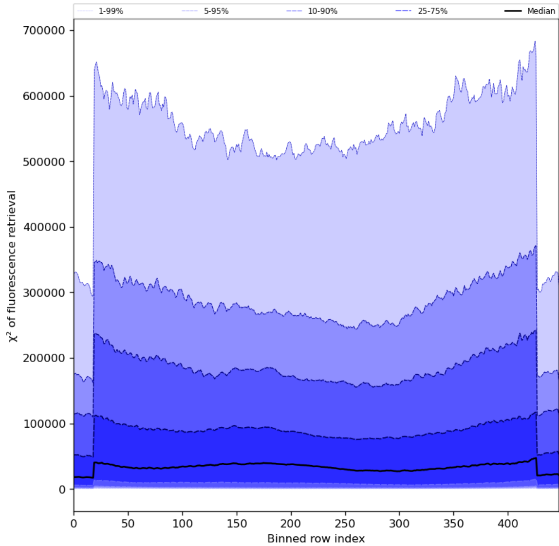
Figure 59: Along track statistics of “ \chi^2 of fluorescence retrieval” for 2024-06-26 to 2024-06-28
