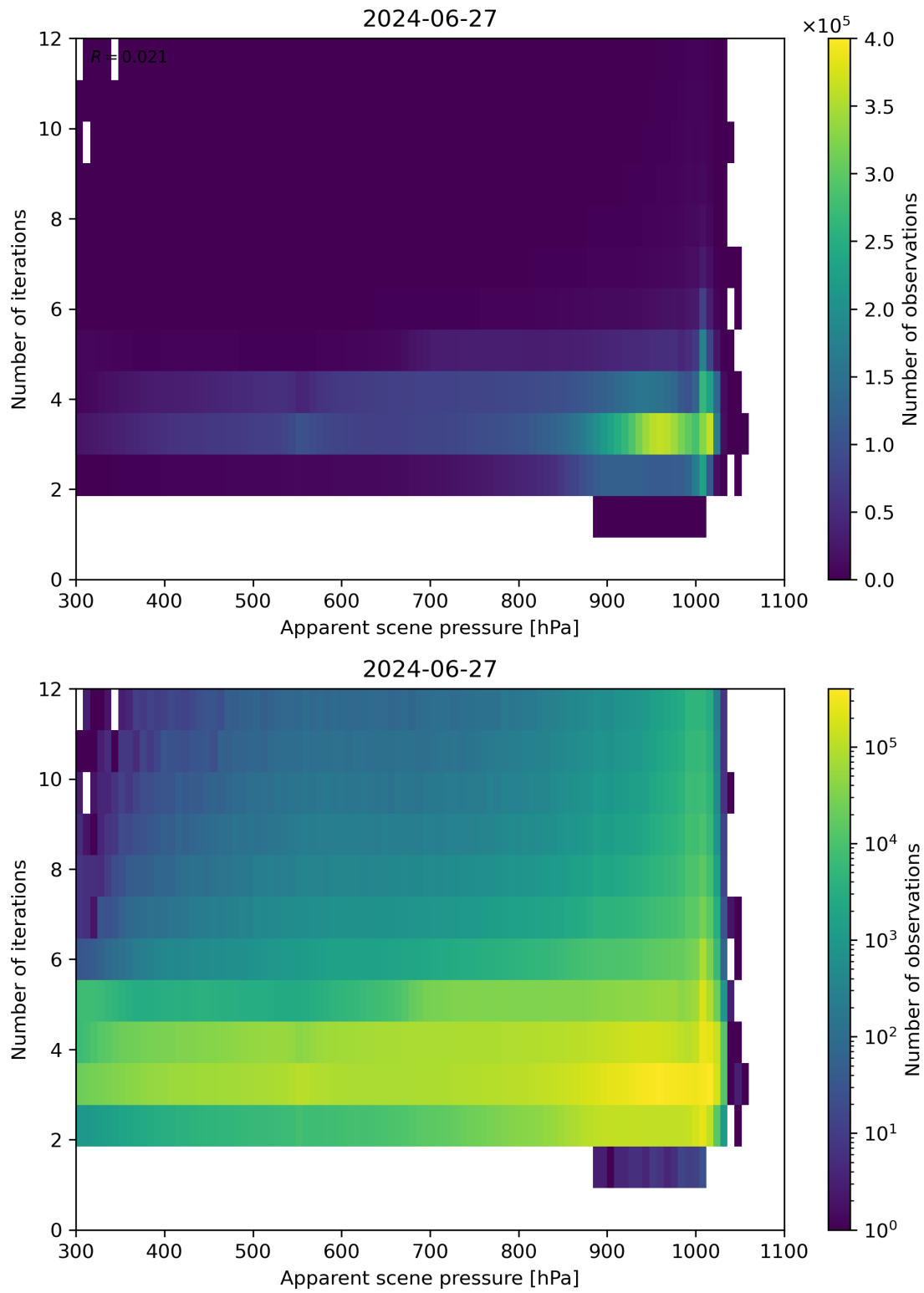
Figure 65: Scatter density plot of “Apparent scene pressure” against “Number of iterations” for 2024-06-26 to 2024-06-28.
