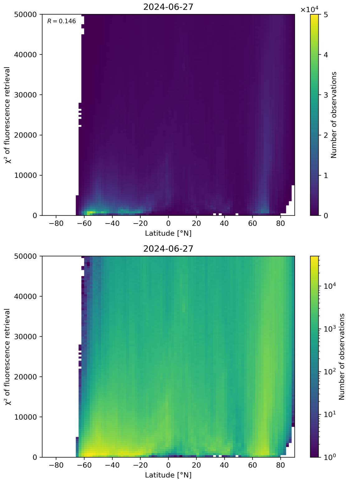
Figure 89: Scatter density plot of “Latitude” against “ \chi^2 of fluorescence retrieval” for 2024-06-26 to 2024-06-28.
