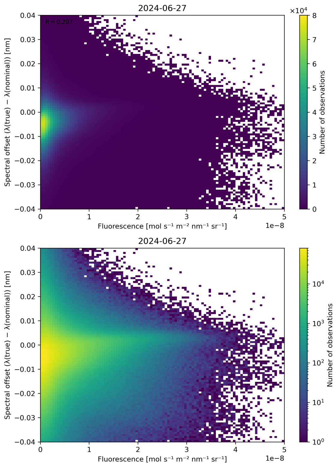
Figure 87: Scatter density plot of “Fluorescence” against “Spectral offset ( \lambda(\text{true}) - \lambda(\text{nominal}) )” for 2024-06-26 to 2024-06-28.
