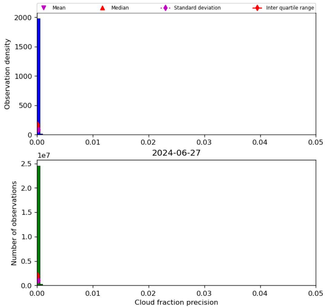
Figure 33: Histogram of “Cloud fraction precision” for 2024-06-26 to 2024-06-28
