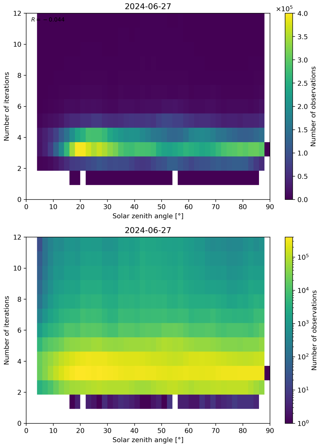
Figure 114: Scatter density plot of “Solar zenith angle” against “Number of iterations” for 2024-06-26 to 2024-06-28.
