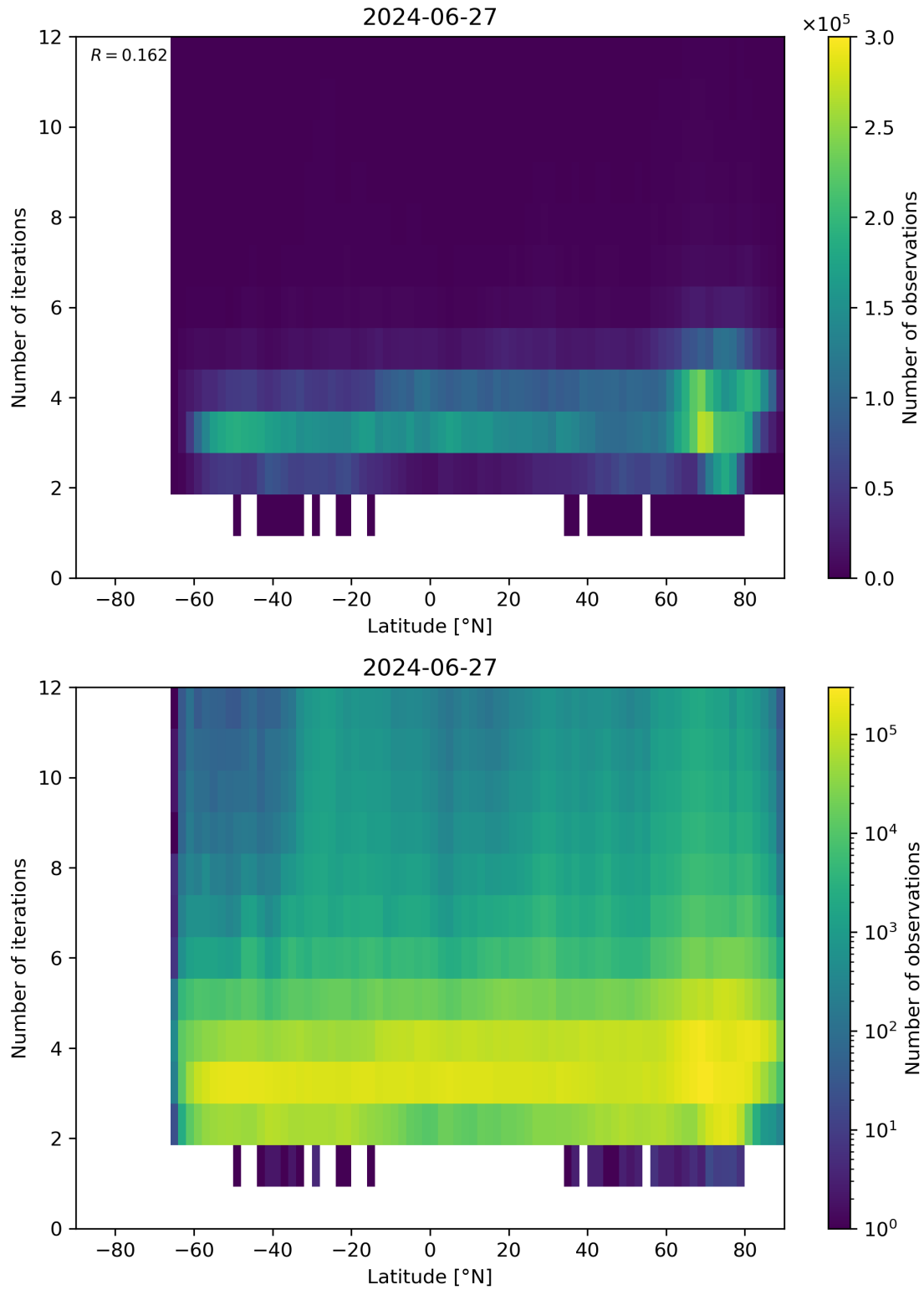
Figure 93: Scatter density plot of “Latitude” against “Number of iterations” for 2024-06-26 to 2024-06-28.
