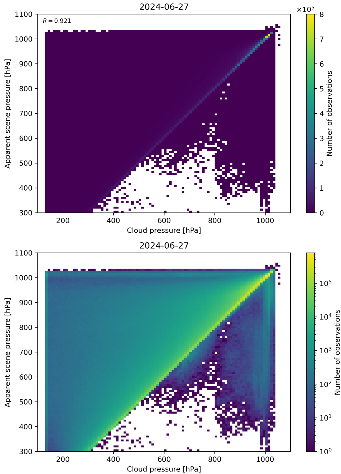
Figure 77: Scatter density plot of “Cloud pressure” against “Apparent scene pressure” for 2024-06-26 to 2024-06-28.
