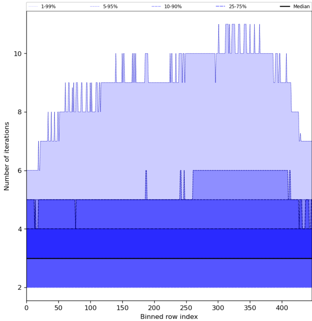
Figure 56: Along track statistics of “Number of iterations” for 2024-06-26 to 2024-06-28
