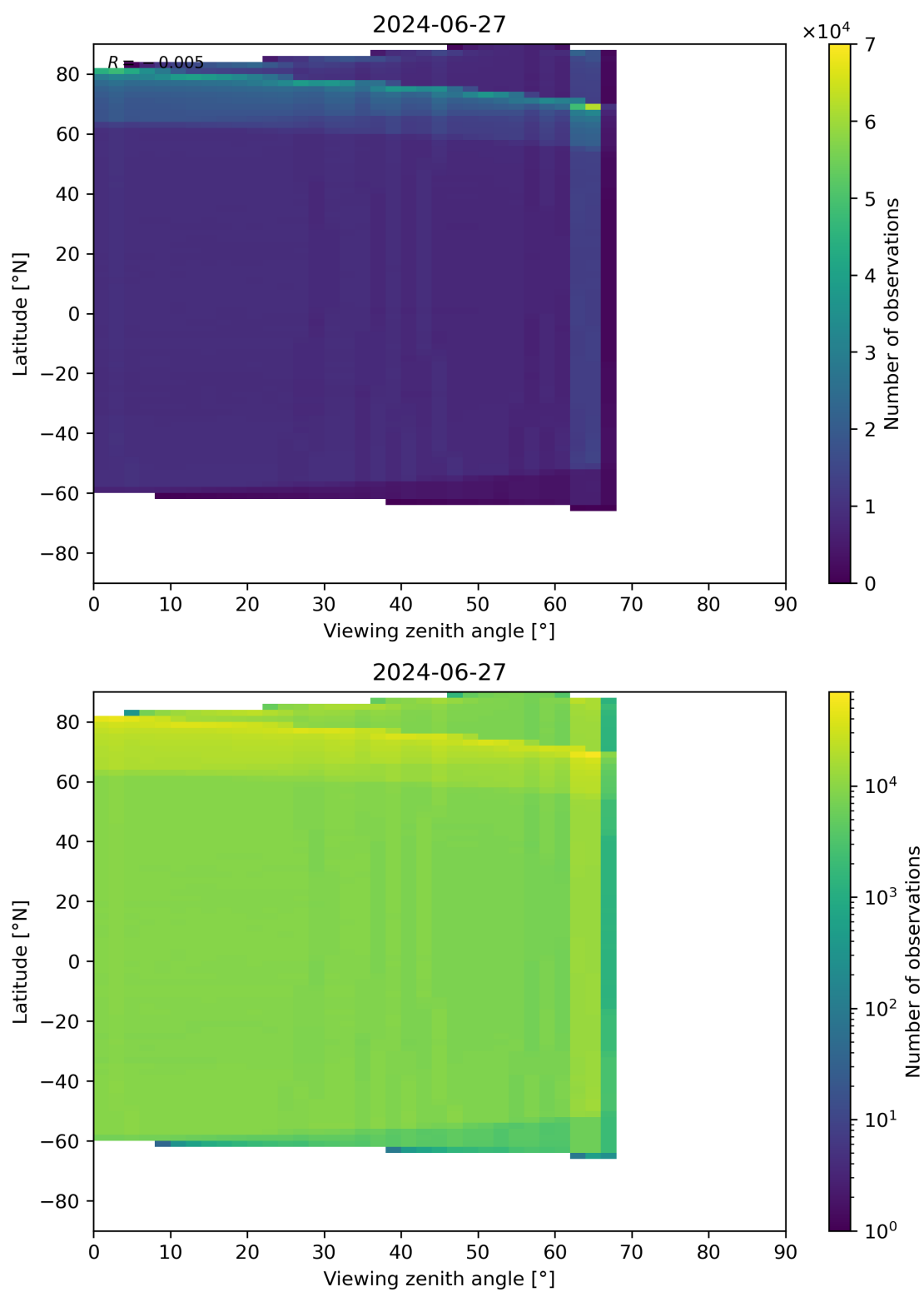
Figure 123: Scatter density plot of “Viewing zenith angle” against “Latitude” for 2024-06-26 to 2024-06-28.
