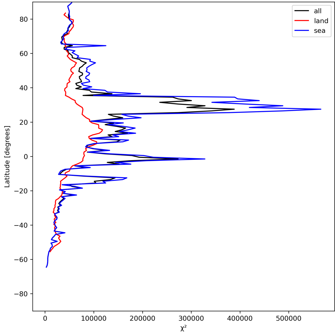
Figure 21: Zonal average of “ \chi^2 ” for 2024-06-26 to 2024-06-28.
