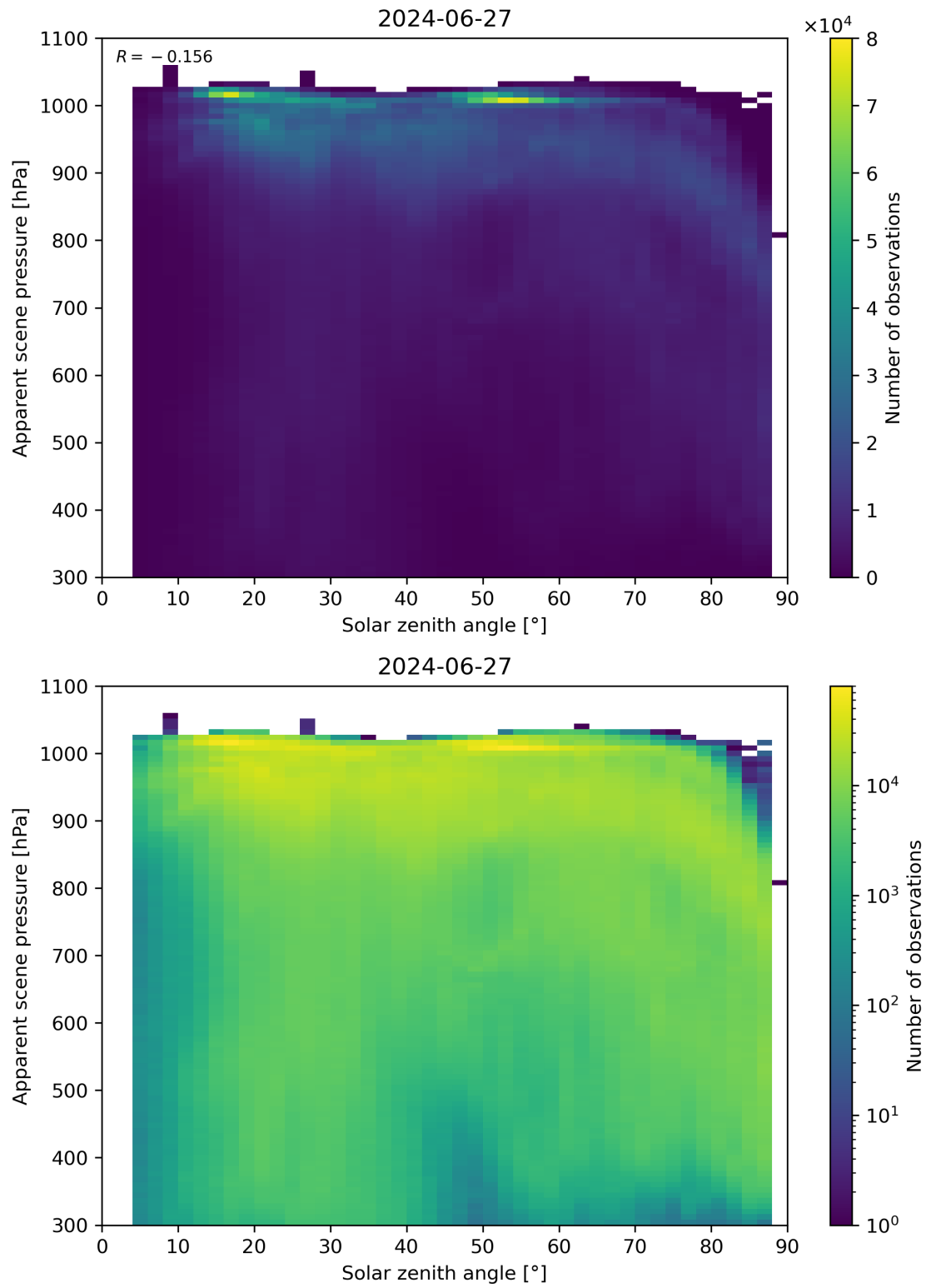
Figure 108: Scatter density plot of “Solar zenith angle” against “Apparent scene pressure” for 2024-06-26 to 2024-06-28.
