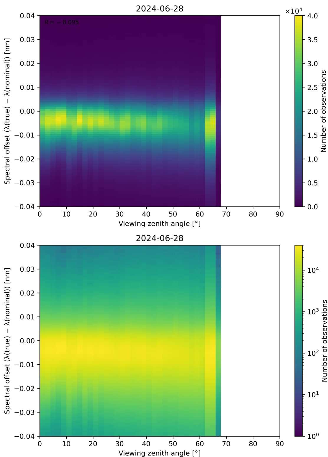
Figure 128: Scatter density plot of “Viewing zenith angle” against “Spectral offset ( \lambda(\text{true}) - \lambda(\text{nominal}) )” for 2024-06-27 to 2024-06-29.
