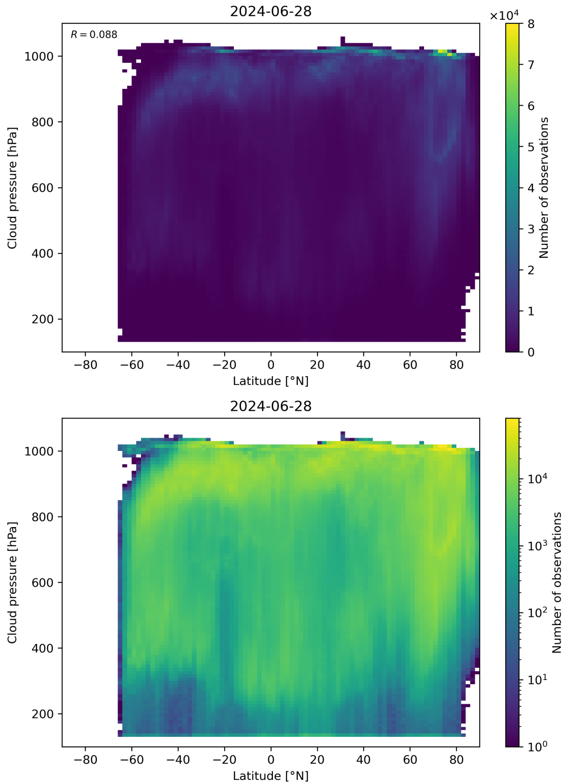
Figure 91: Scatter density plot of “Latitude” against “Cloud pressure” for 2024-06-27 to 2024-06-29.
