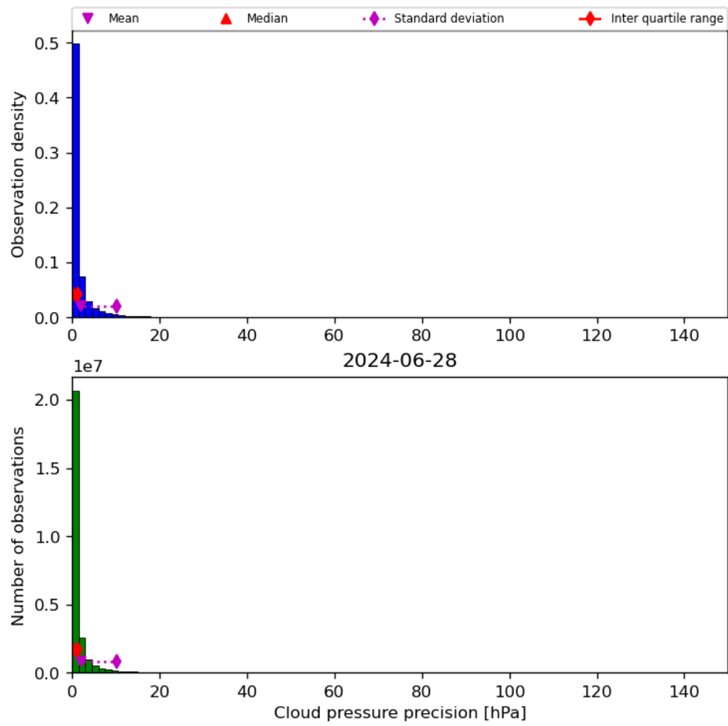
Figure 31: Histogram of “Cloud pressure precision” for 2024-06-27 to 2024-06-29
