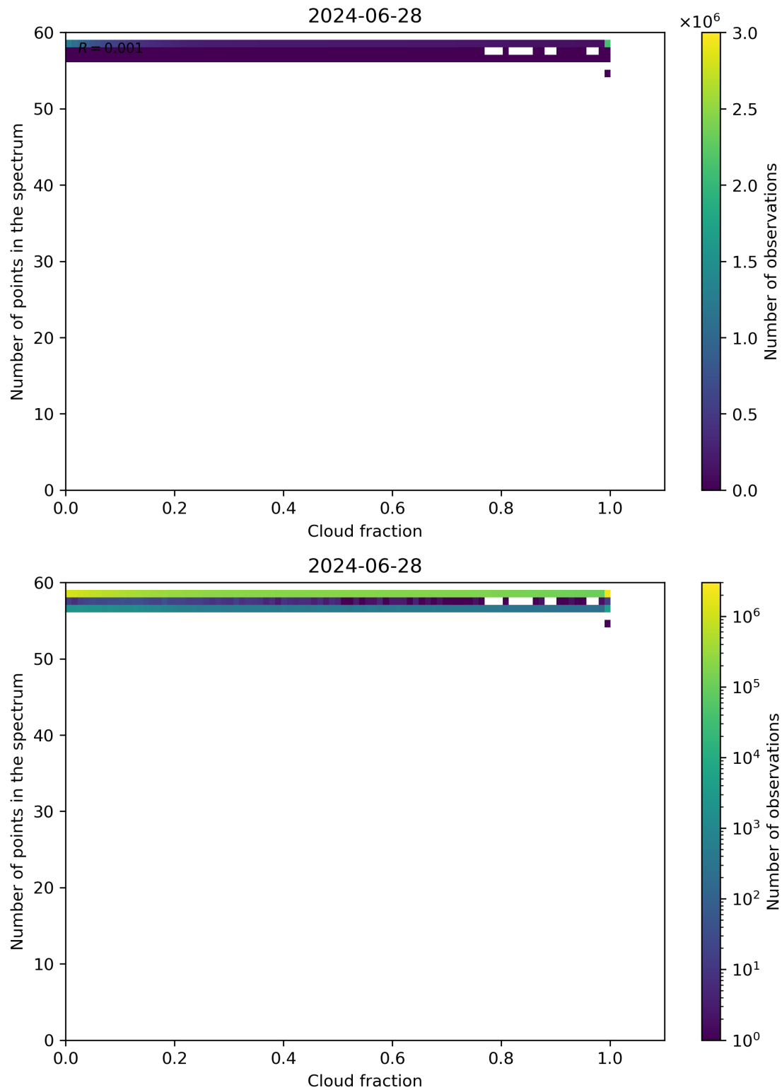
Figure 74: Scatter density plot of “Cloud fraction” against “Number of points in the spectrum” for 2024-06-27 to 2024-06-29.
