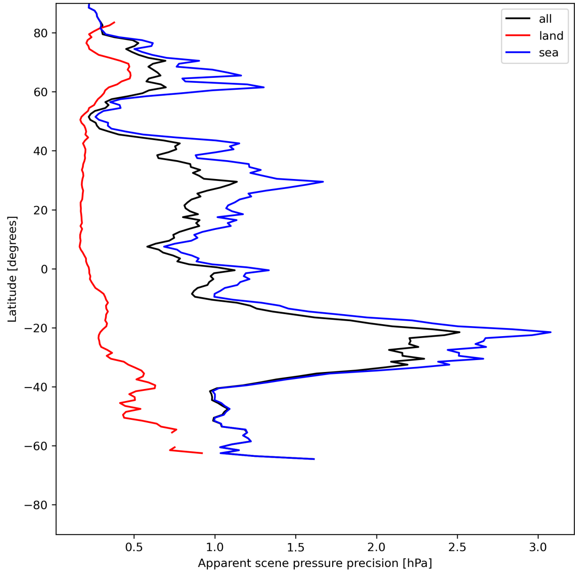
Figure 20: Zonal average of “Apparent scene pressure precision” for 2024-06-27 to 2024-06-29.
