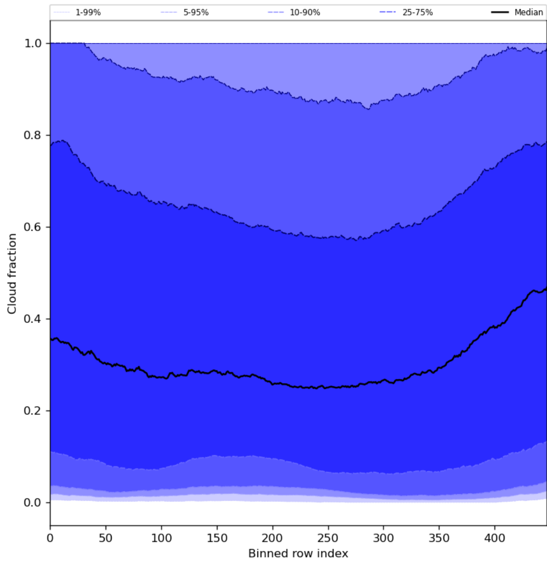
Figure 49: Along track statistics of “Cloud fraction” for 2024-06-27 to 2024-06-29
