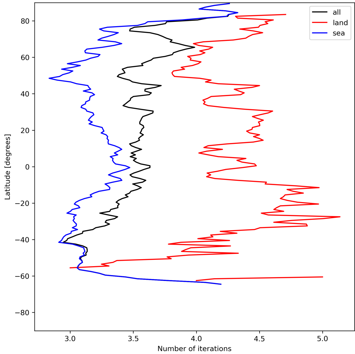
Figure 22: Zonal average of “Number of iterations” for 2024-06-27 to 2024-06-29.
