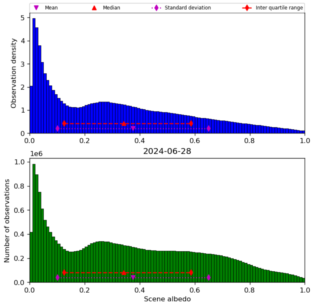
Figure 34: Histogram of “Scene albedo” for 2024-06-27 to 2024-06-29
