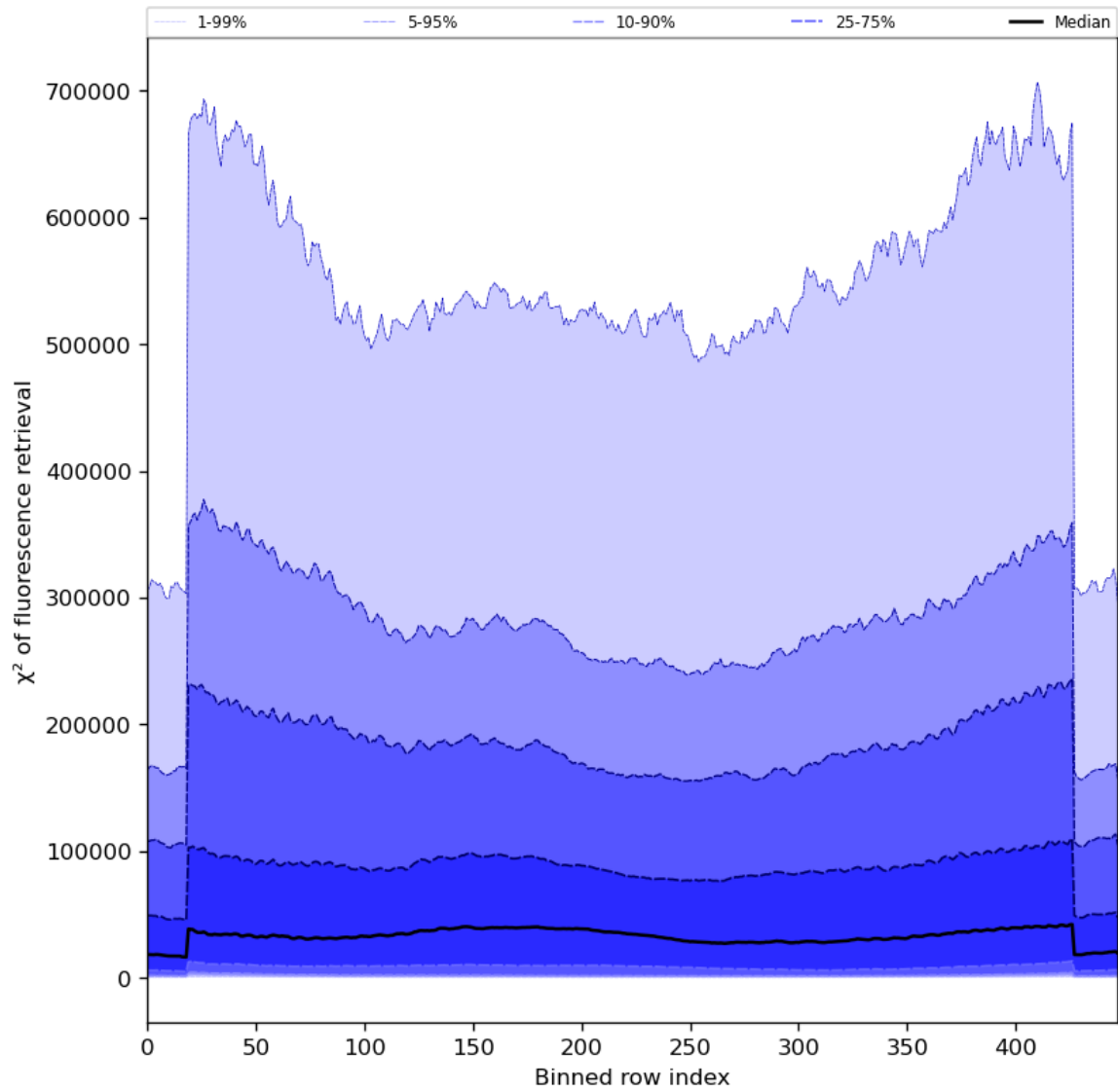
Figure 59: Along track statistics of “ \chi^2 of fluorescence retrieval” for 2024-06-27 to 2024-06-29
