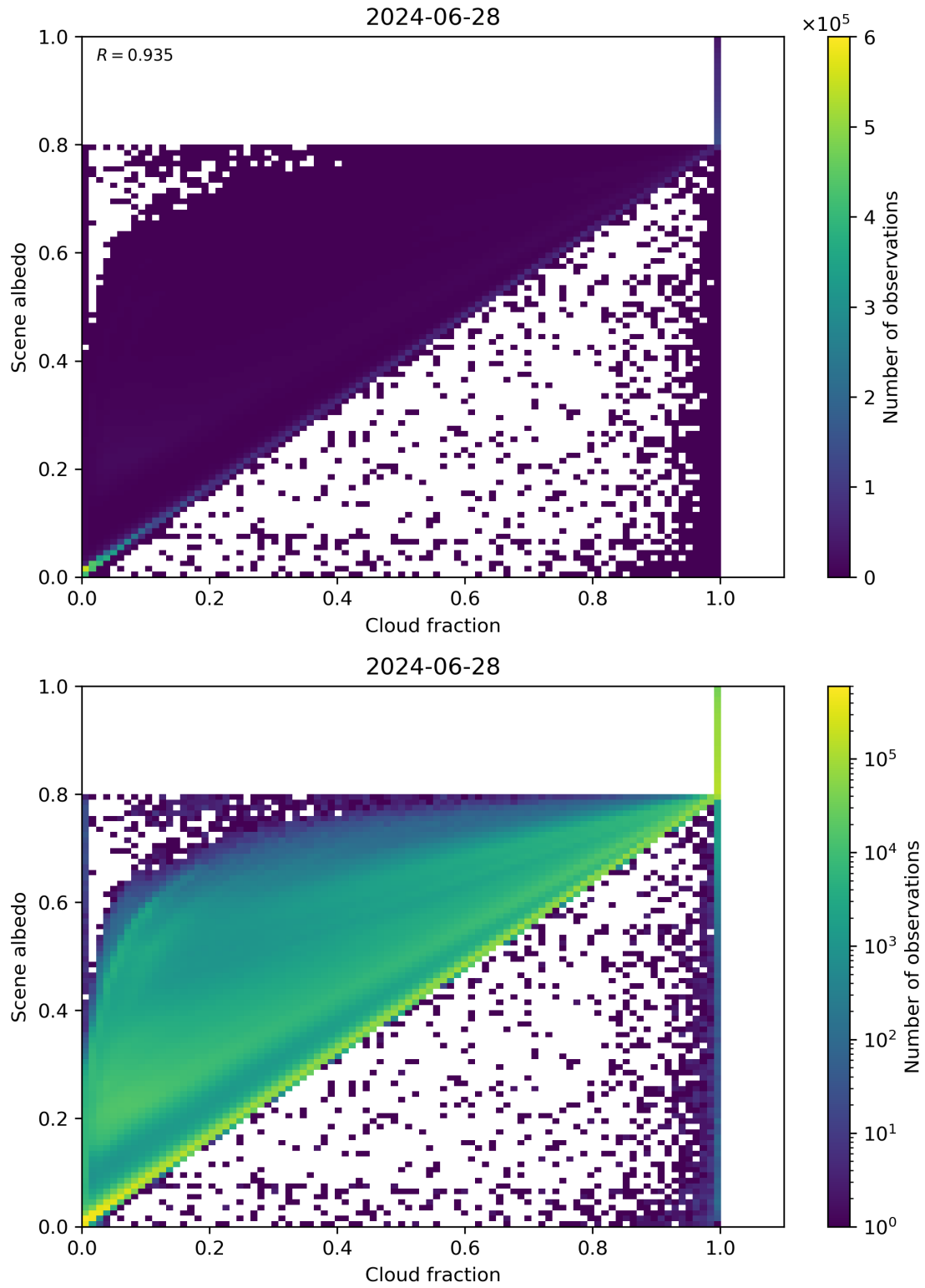
Figure 75: Scatter density plot of “Cloud fraction” against “Scene albedo” for 2024-06-27 to 2024-06-29.
