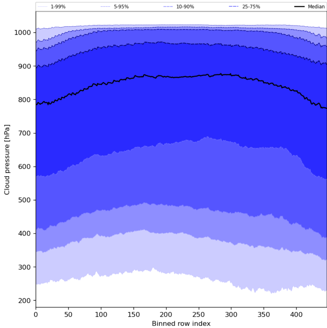
Figure 47: Along track statistics of “Cloud pressure” for 2024-06-27 to 2024-06-29
