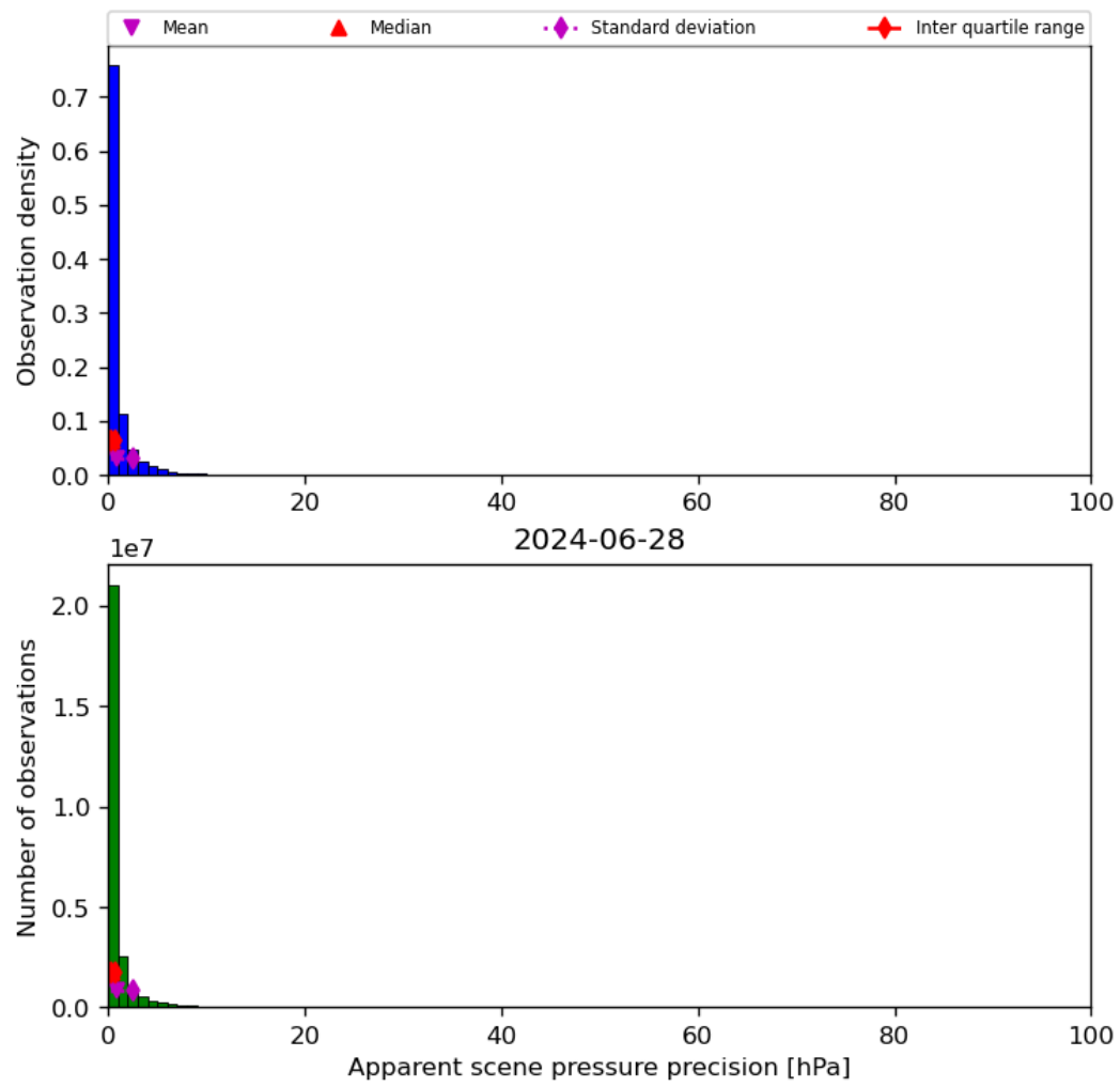
Figure 37: Histogram of “Apparent scene pressure precision” for 2024-06-27 to 2024-06-29
