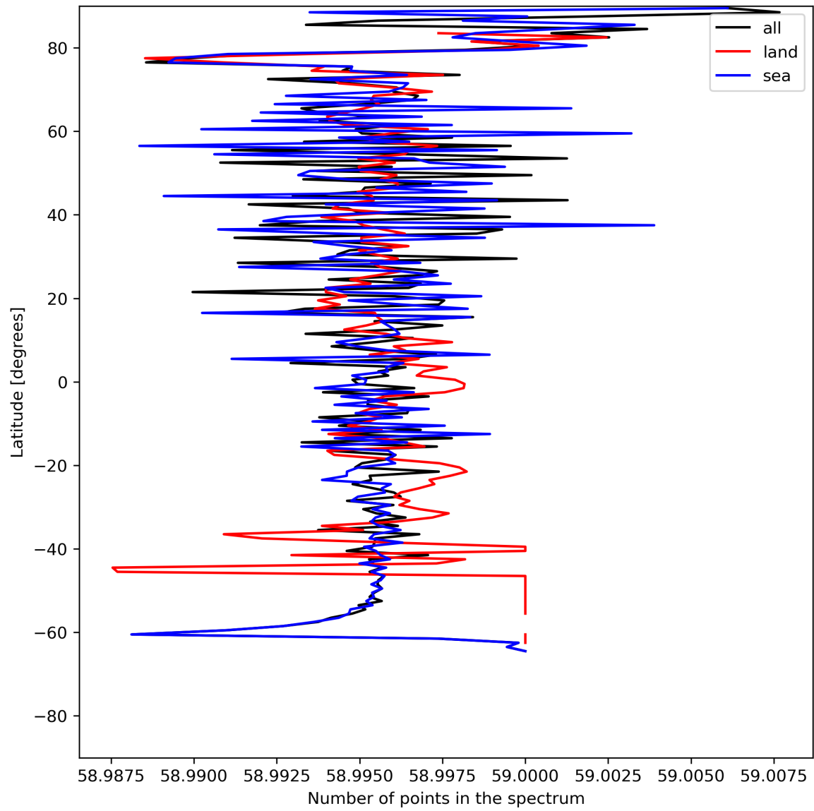
Figure 27: Zonal average of “Number of points in the spectrum” for 2024-06-27 to 2024-06-29.
