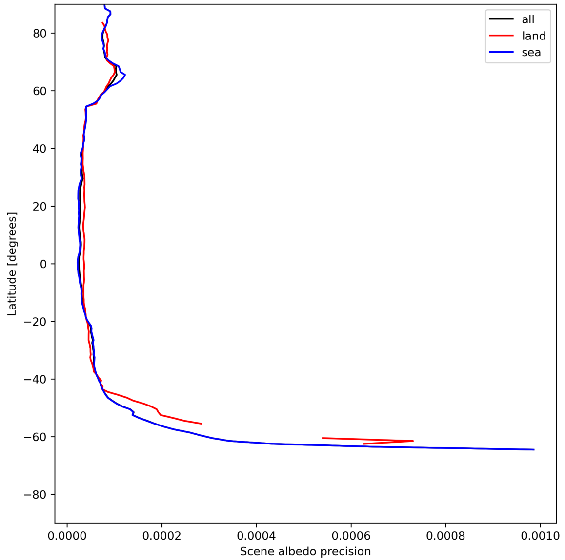
Figure 18: Zonal average of “Scene albedo precision” for 2024-06-27 to 2024-06-29.
