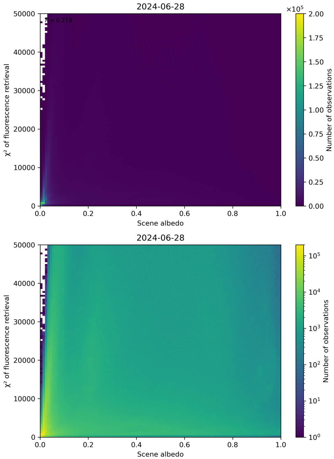
Figure 103: Scatter density plot of “Scene albedo” against “ \chi^2 of fluorescence retrieval” for 2024-06-27 to 2024-06-29.
