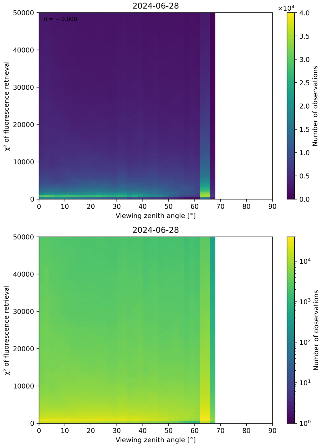
Figure 119: Scatter density plot of “Viewing zenith angle” against “ \chi^2 of fluorescence retrieval” for 2024-06-27 to 2024-06-29.
