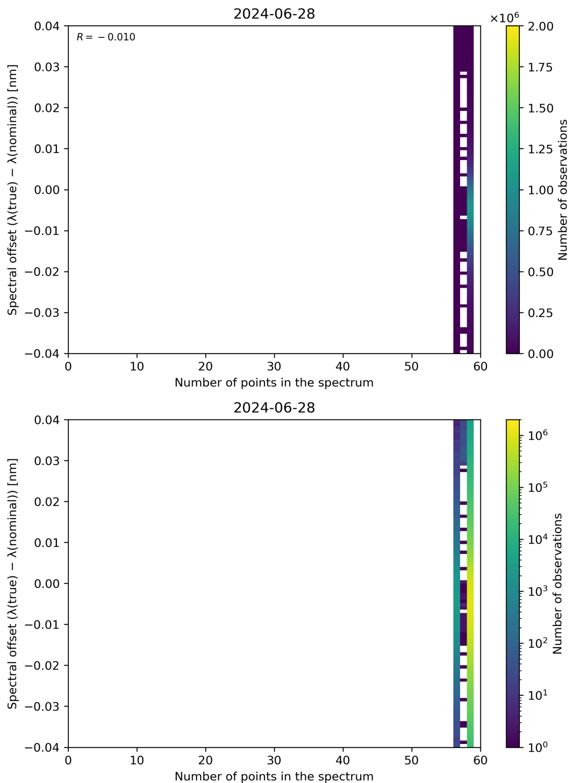
Figure 101: Scatter density plot of “Number of points in the spectrum” against “Spectral offset ( \lambda(\text{true}) - \lambda(\text{nominal}) )” for 2024-06-27 to 2024-06-29.
