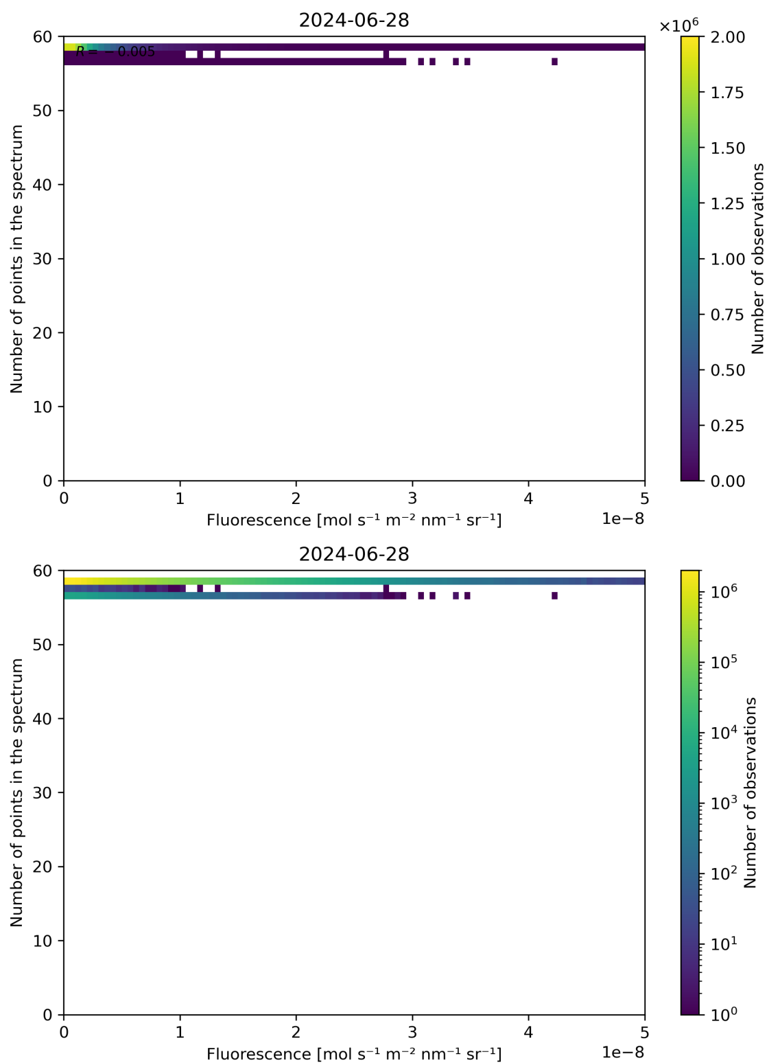
Figure 86: Scatter density plot of “Fluorescence” against “Number of points in the spectrum” for 2024-06-27 to 2024-06-29.
