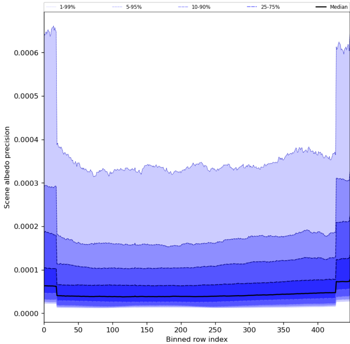
Figure 52: Along track statistics of “Scene albedo precision” for 2024-06-27 to 2024-06-29
