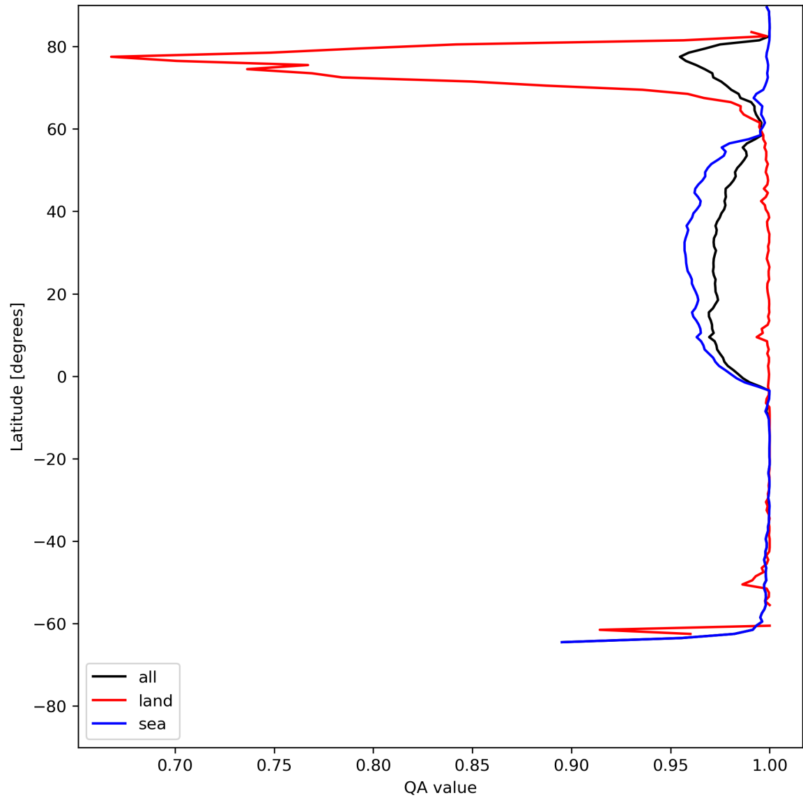
Figure 12: Zonal average of “QA value” for 2024-06-27 to 2024-06-29.
