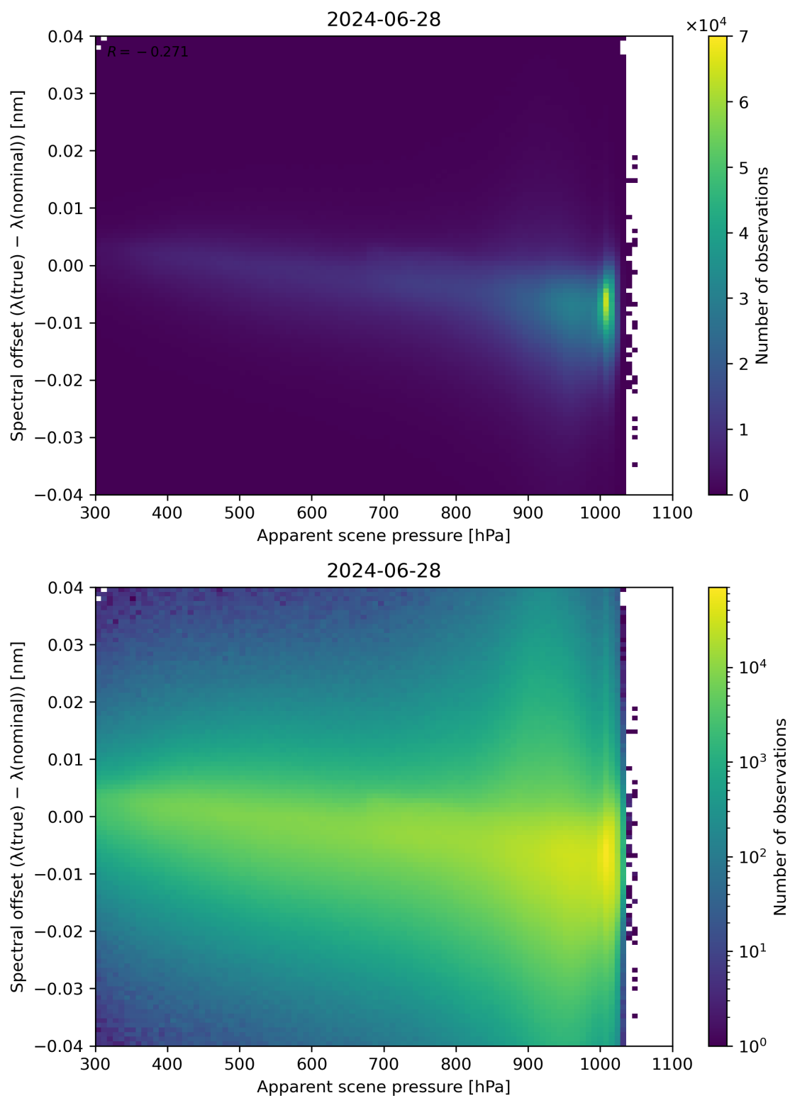
Figure 67: Scatter density plot of “Apparent scene pressure” against “Spectral offset ( \lambda(\text{true}) - \lambda(\text{nominal}) )” for 2024-06-27 to 2024-06-29.
