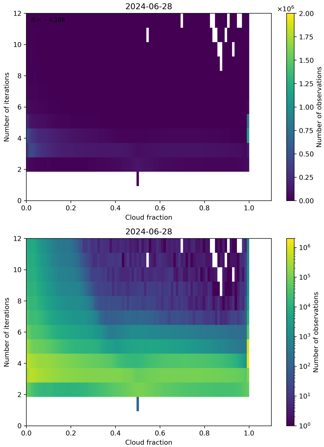
Figure 73: Scatter density plot of “Cloud fraction” against “Number of iterations” for 2024-06-27 to 2024-06-29.
