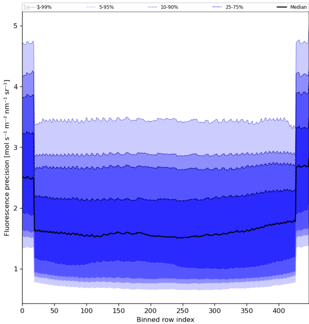
Figure 58: Along track statistics of “Fluorescence precision” for 2024-06-27 to 2024-06-29
