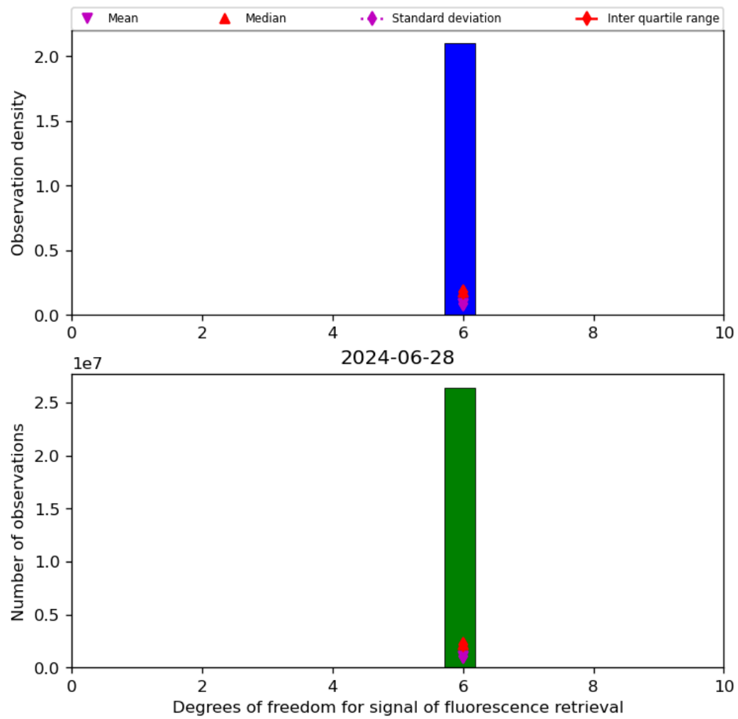
Figure 43: Histogram of “Degrees of freedom for signal of fluorescence retrieval” for 2024-06-27 to 2024-06-29
