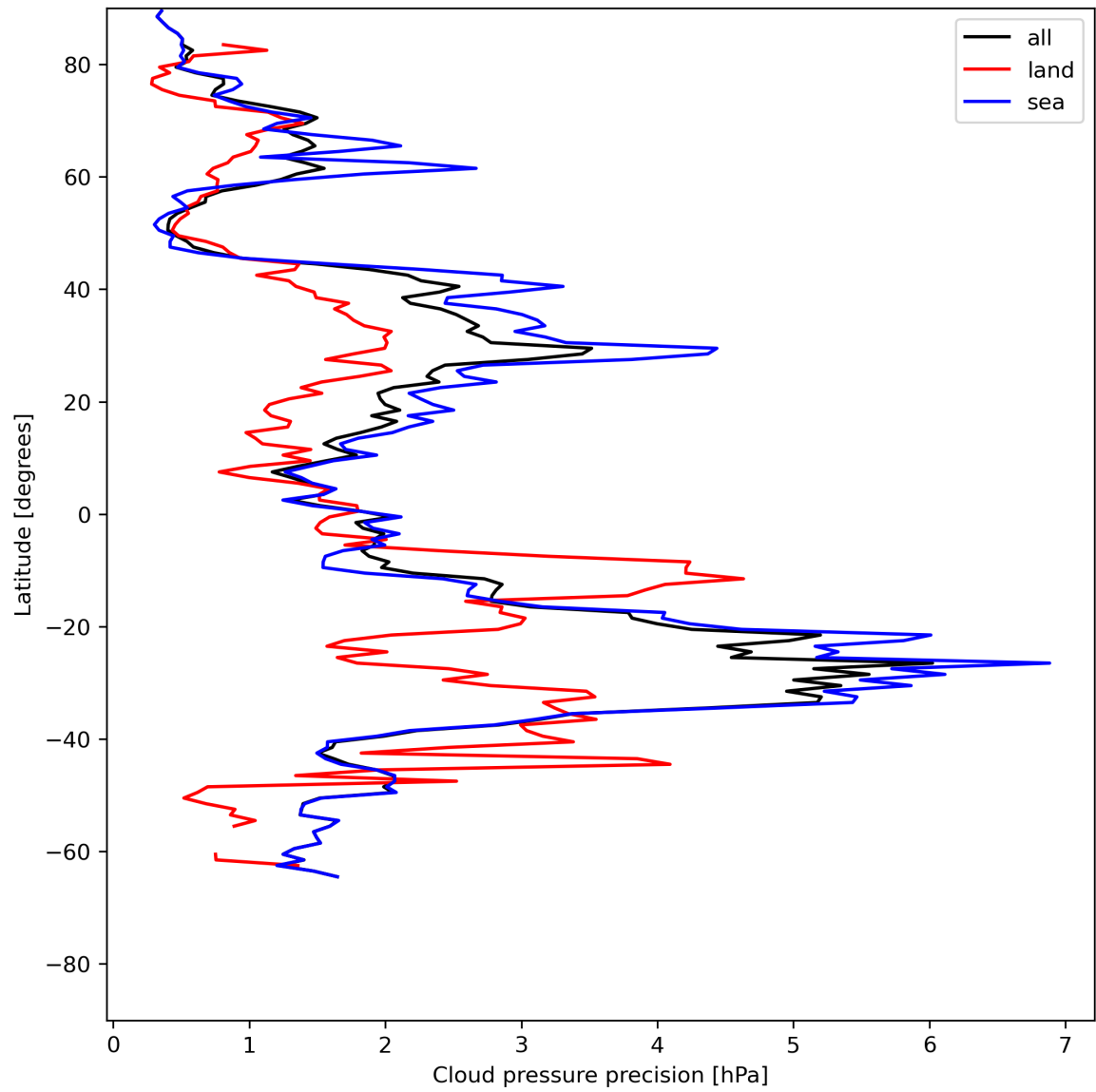
Figure 14: Zonal average of “Cloud pressure precision” for 2024-06-27 to 2024-06-29.
