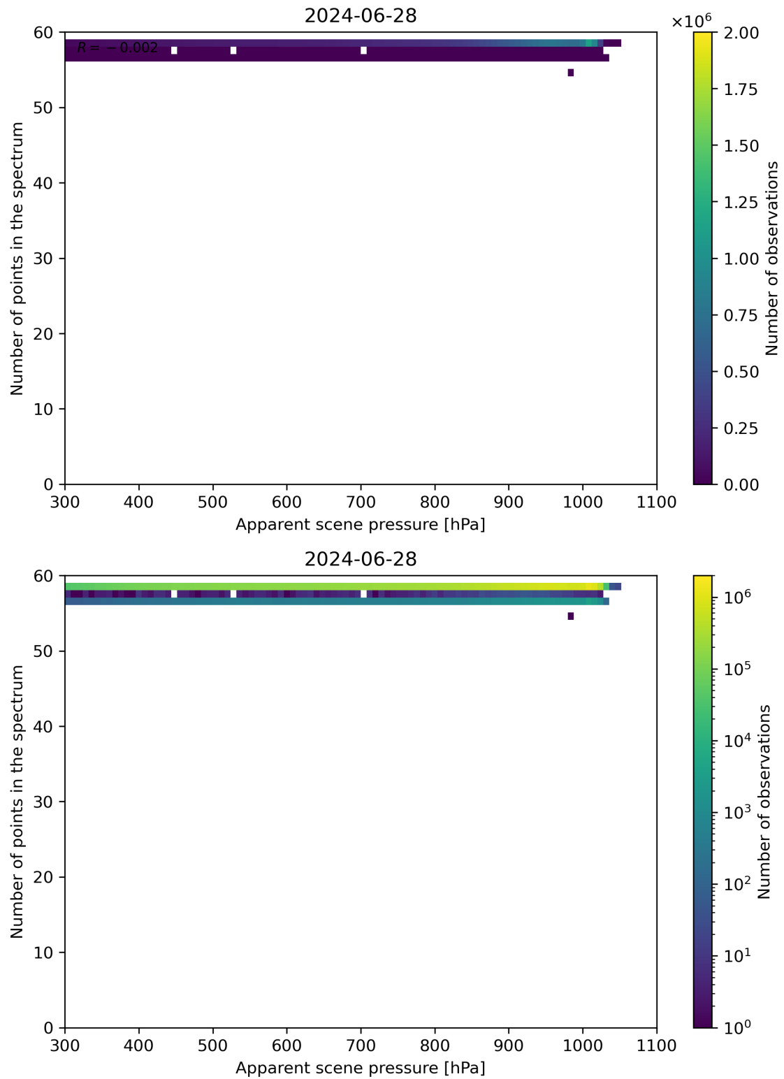
Figure 66: Scatter density plot of “Apparent scene pressure” against “Number of points in the spectrum” for 2024-06-27 to 2024-06-29.
