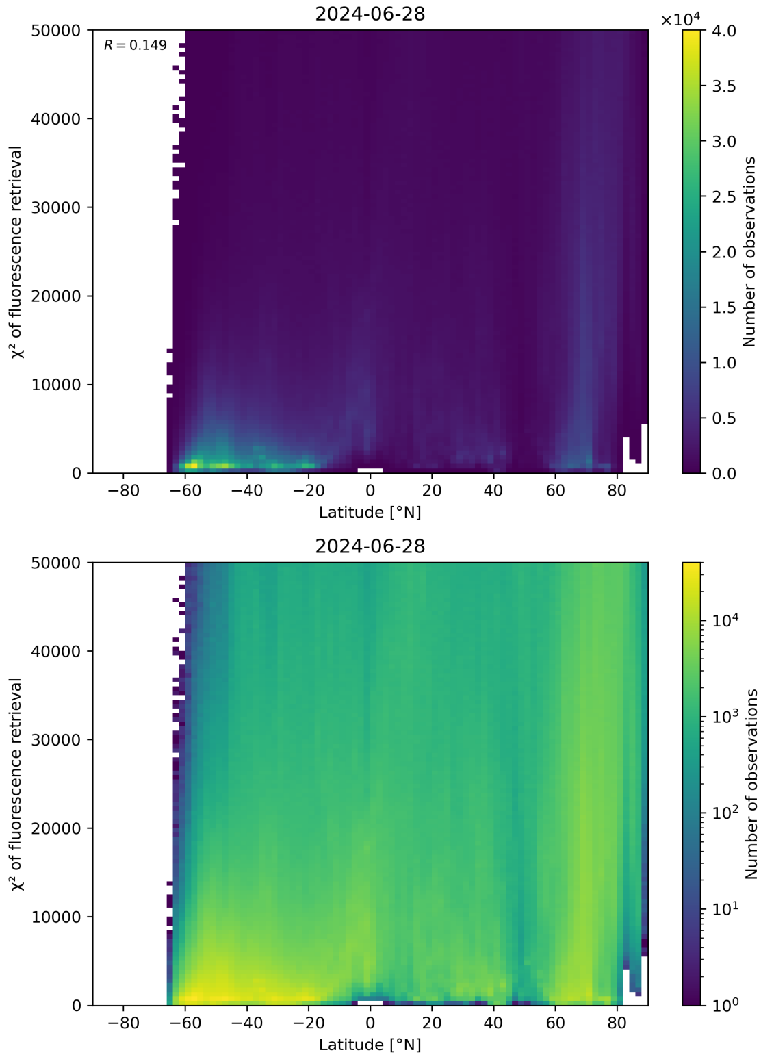
Figure 89: Scatter density plot of “Latitude” against “ \chi^2 of fluorescence retrieval” for 2024-06-27 to 2024-06-29.
