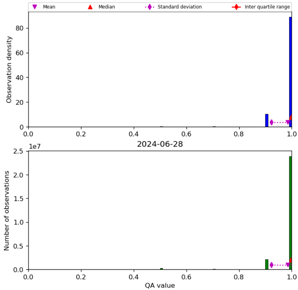
Figure 29: Histogram of “QA value” for 2024-06-27 to 2024-06-29
