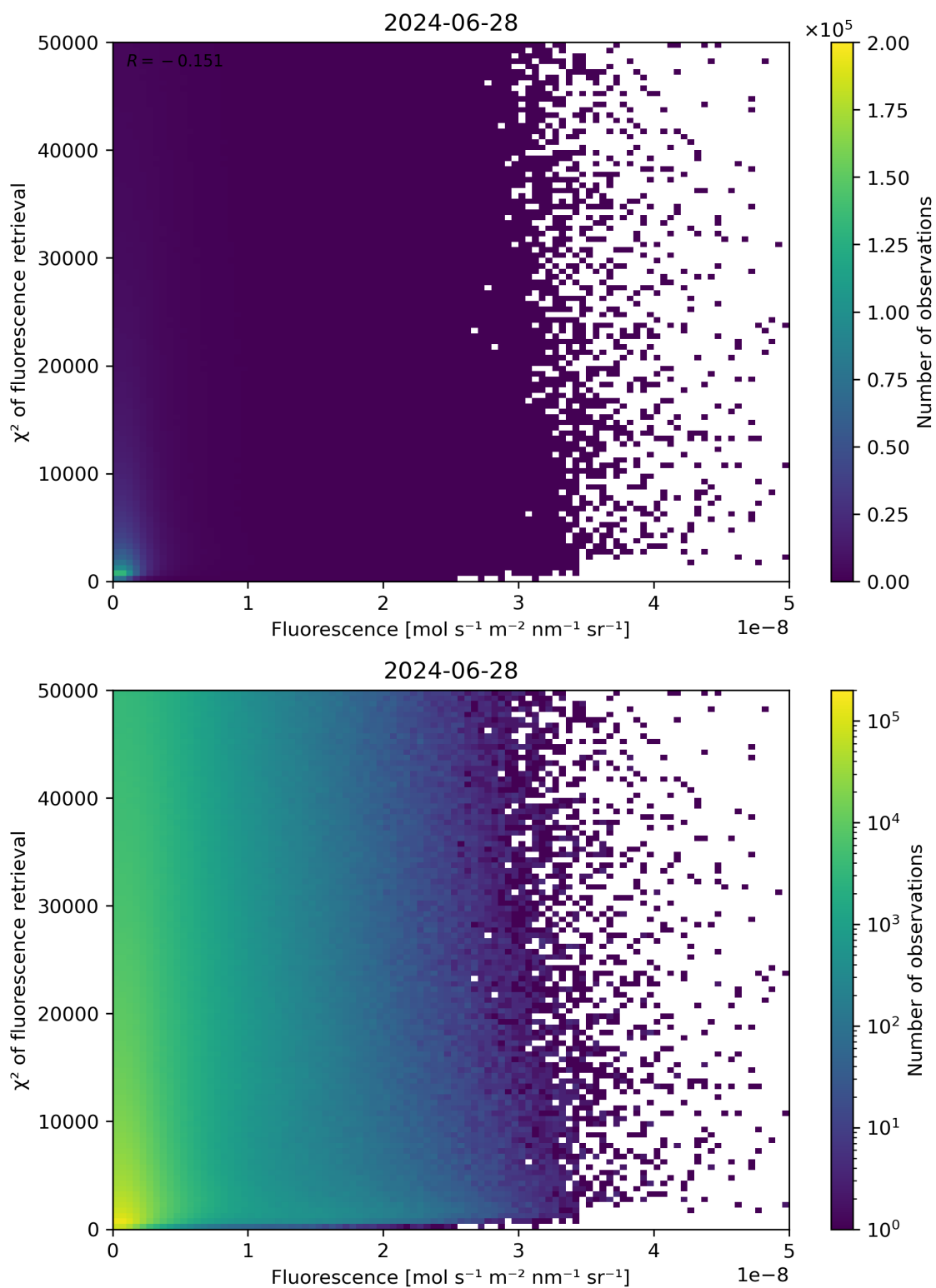
Figure 85: Scatter density plot of “Fluorescence” against “ \chi^2 of fluorescence retrieval” for 2024-06-27 to 2024-06-29.
