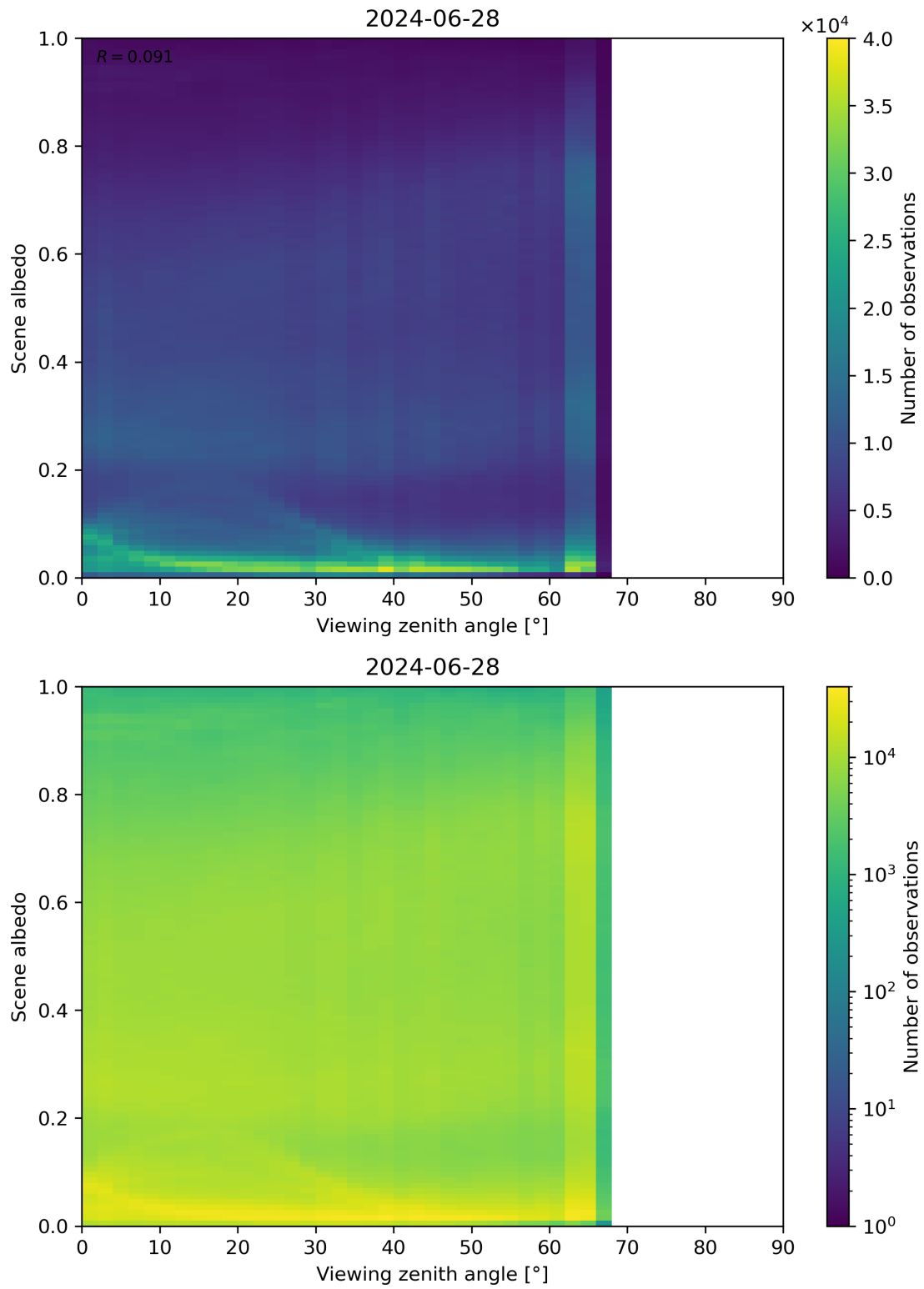
Figure 126: Scatter density plot of “Viewing zenith angle” against “Scene albedo” for 2024-06-27 to 2024-06-29.
