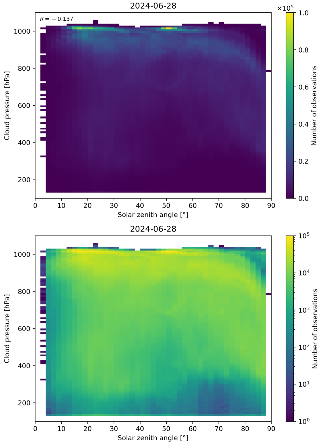
Figure 111: Scatter density plot of “Solar zenith angle” against “Cloud pressure” for 2024-06-27 to 2024-06-29.
