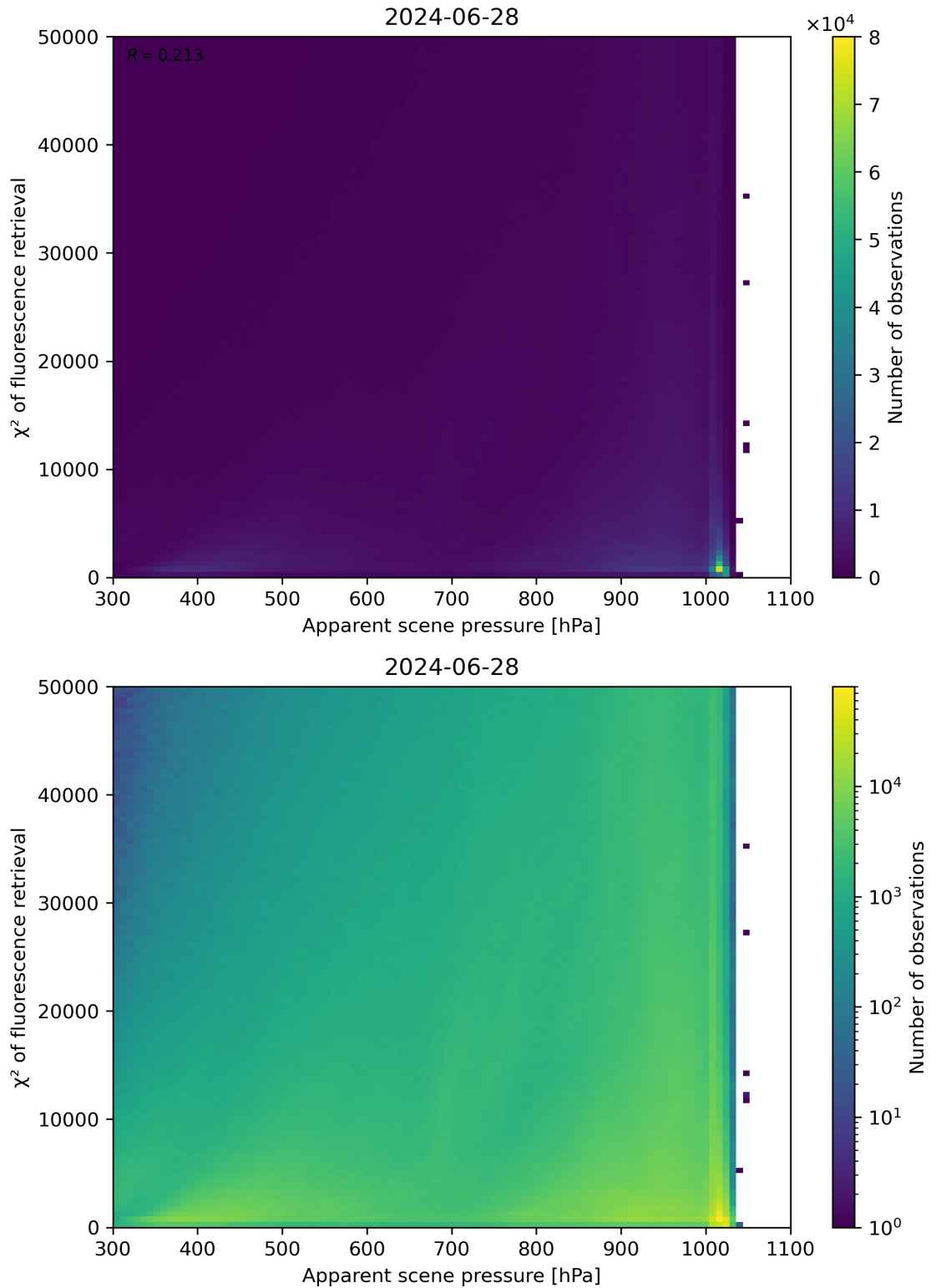
Figure 63: Scatter density plot of “Apparent scene pressure” against “ \chi^2 of fluorescence retrieval” for 2024-06-27 to 2024-06-29.
