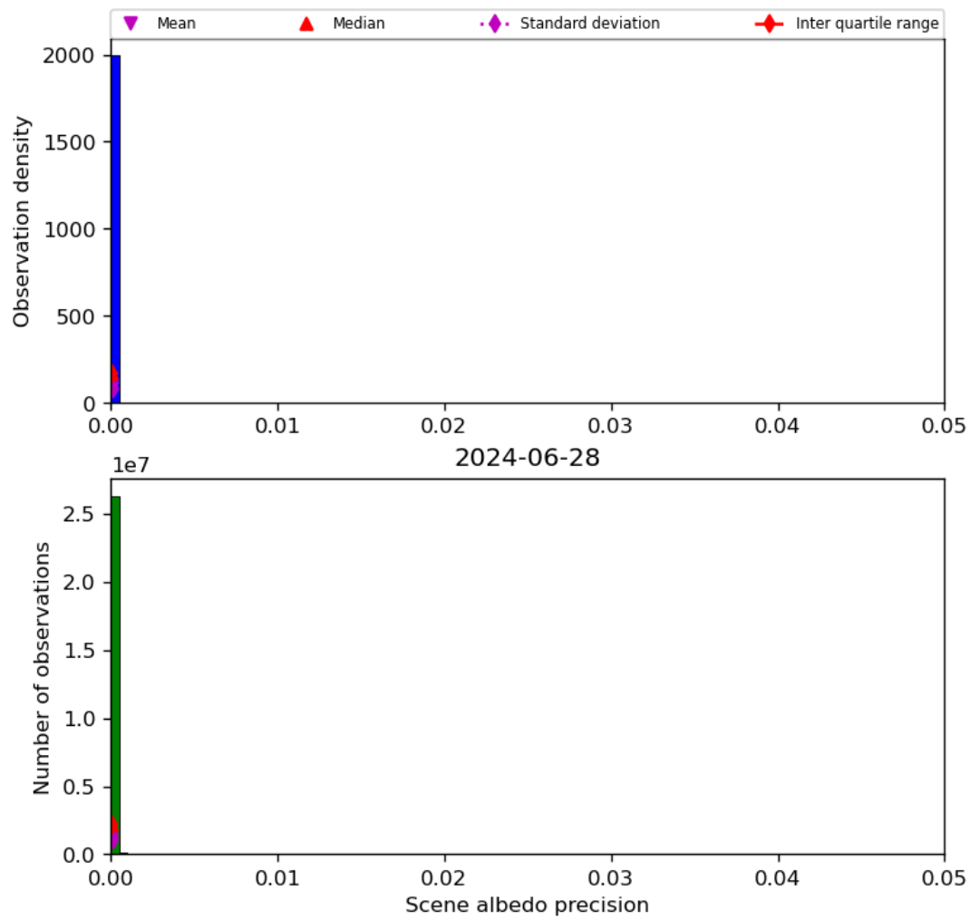
Figure 35: Histogram of “Scene albedo precision” for 2024-06-27 to 2024-06-29
