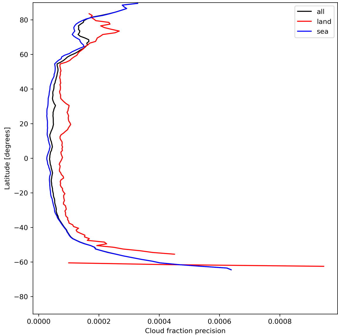
Figure 16: Zonal average of “Cloud fraction precision” for 2024-06-27 to 2024-06-29.
