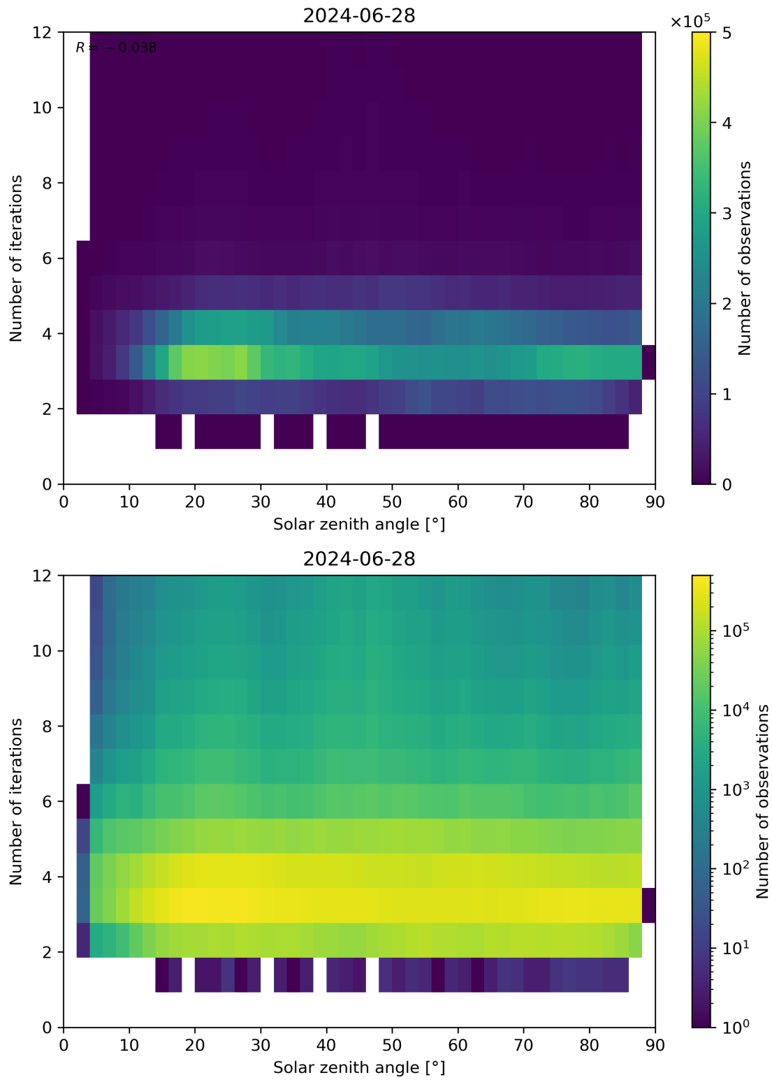
Figure 114: Scatter density plot of “Solar zenith angle” against “Number of iterations” for 2024-06-27 to 2024-06-29.
