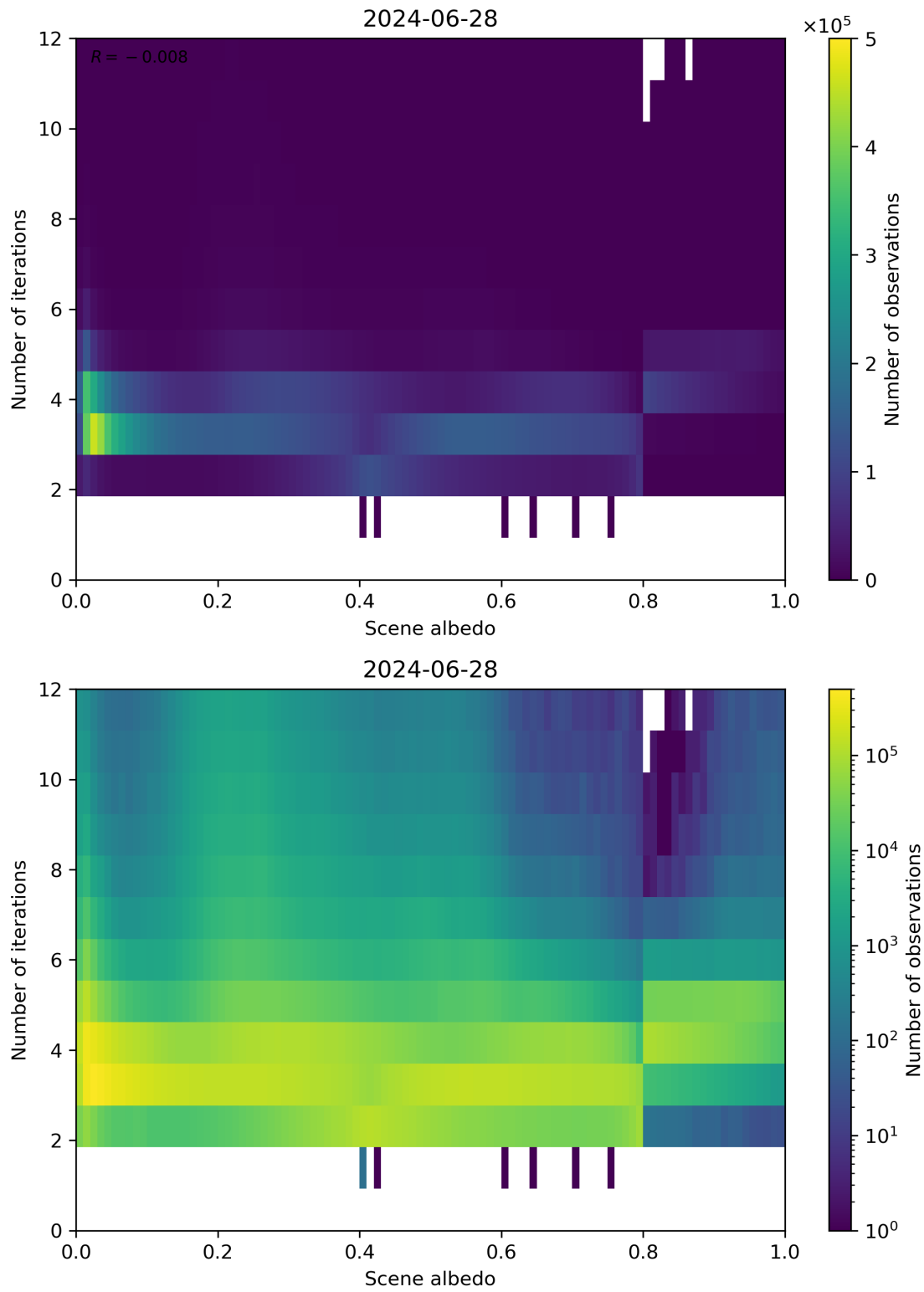
Figure 105: Scatter density plot of “Scene albedo” against “Number of iterations” for 2024-06-27 to 2024-06-29.
