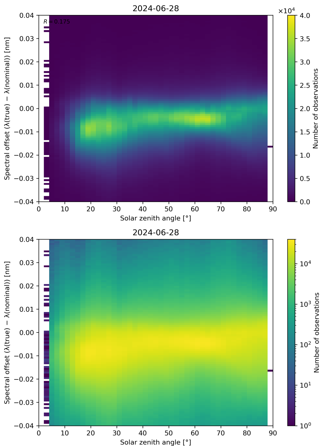
Figure 117: Scatter density plot of “Solar zenith angle” against “Spectral offset ( \lambda(\text{true}) - \lambda(\text{nominal}) )” for 2024-06-27 to 2024-06-29.
