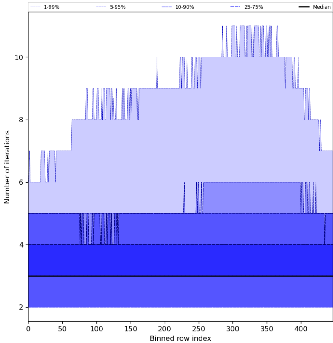
Figure 56: Along track statistics of “Number of iterations” for 2024-06-27 to 2024-06-29
