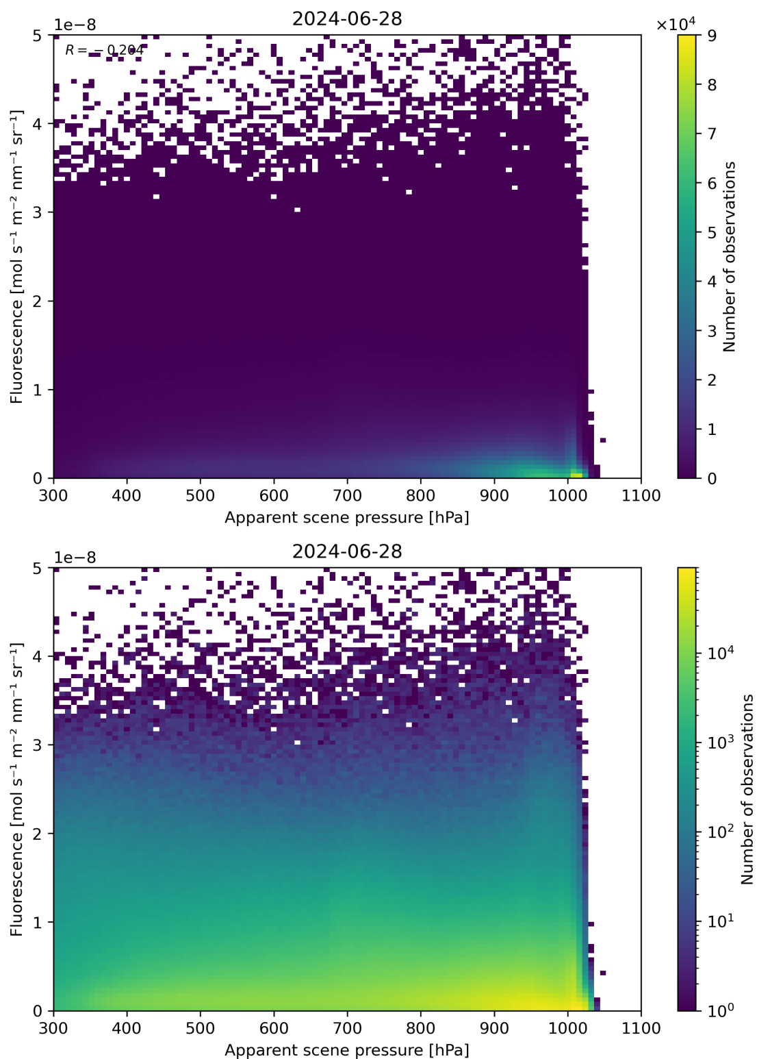
Figure 64: Scatter density plot of “Apparent scene pressure” against “Fluorescence” for 2024-06-27 to 2024-06-29.
