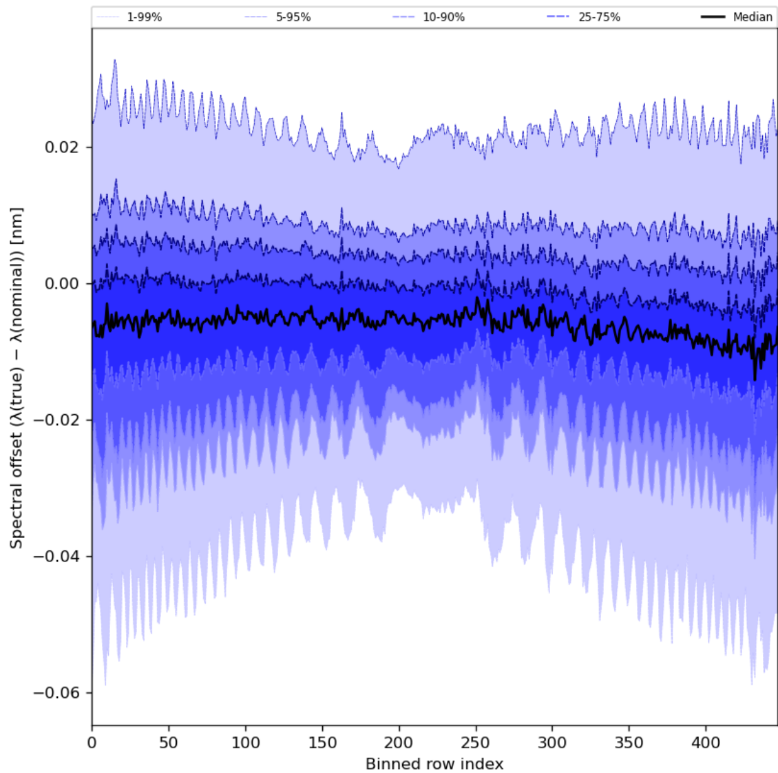
Figure 62: Along track statistics of “Spectral offset ( \lambda(\text{true}) - \lambda(\text{nominal}) )” for 2024-06-27 to 2024-06-29
