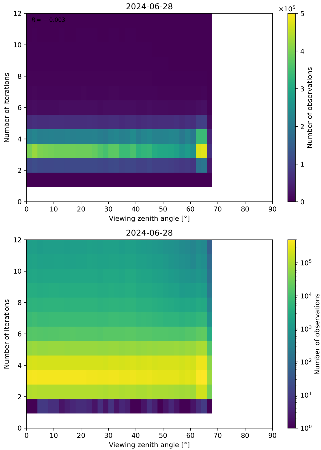
Figure 124: Scatter density plot of “Viewing zenith angle” against “Number of iterations” for 2024-06-27 to 2024-06-29.
