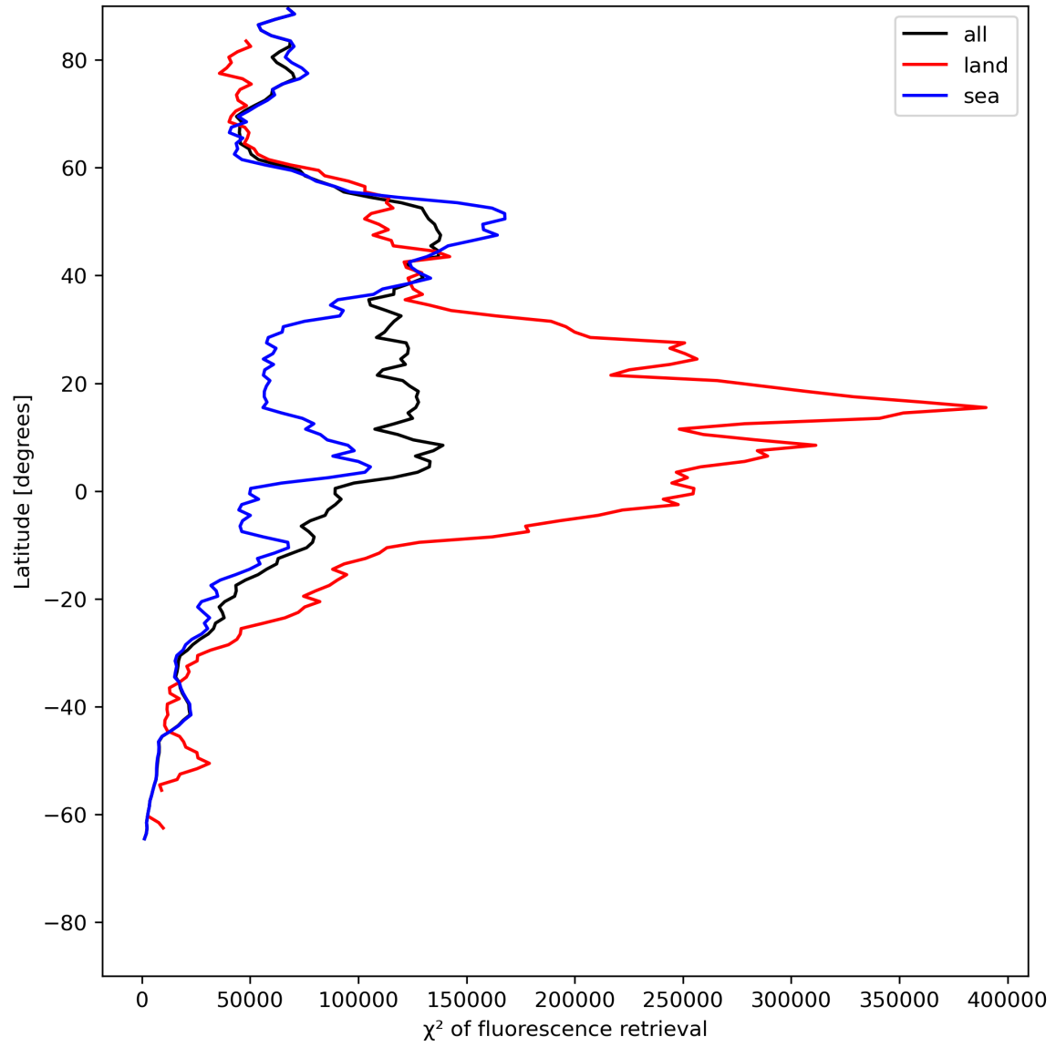
Figure 25: Zonal average of “ \chi^2 of fluorescence retrieval” for 2024-06-27 to 2024-06-29.
