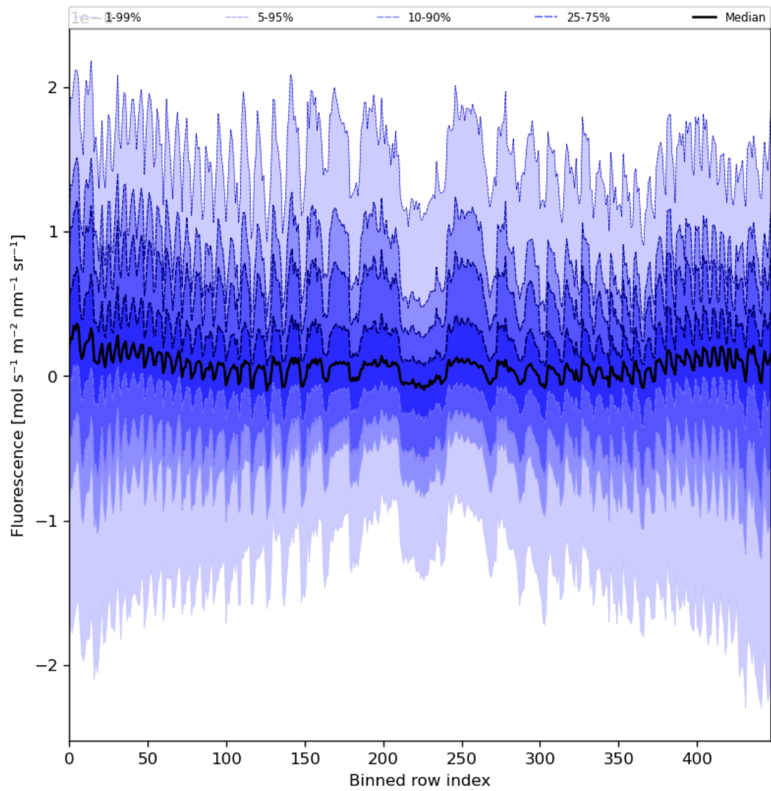
Figure 57: Along track statistics of “Fluorescence” for 2024-06-27 to 2024-06-29
