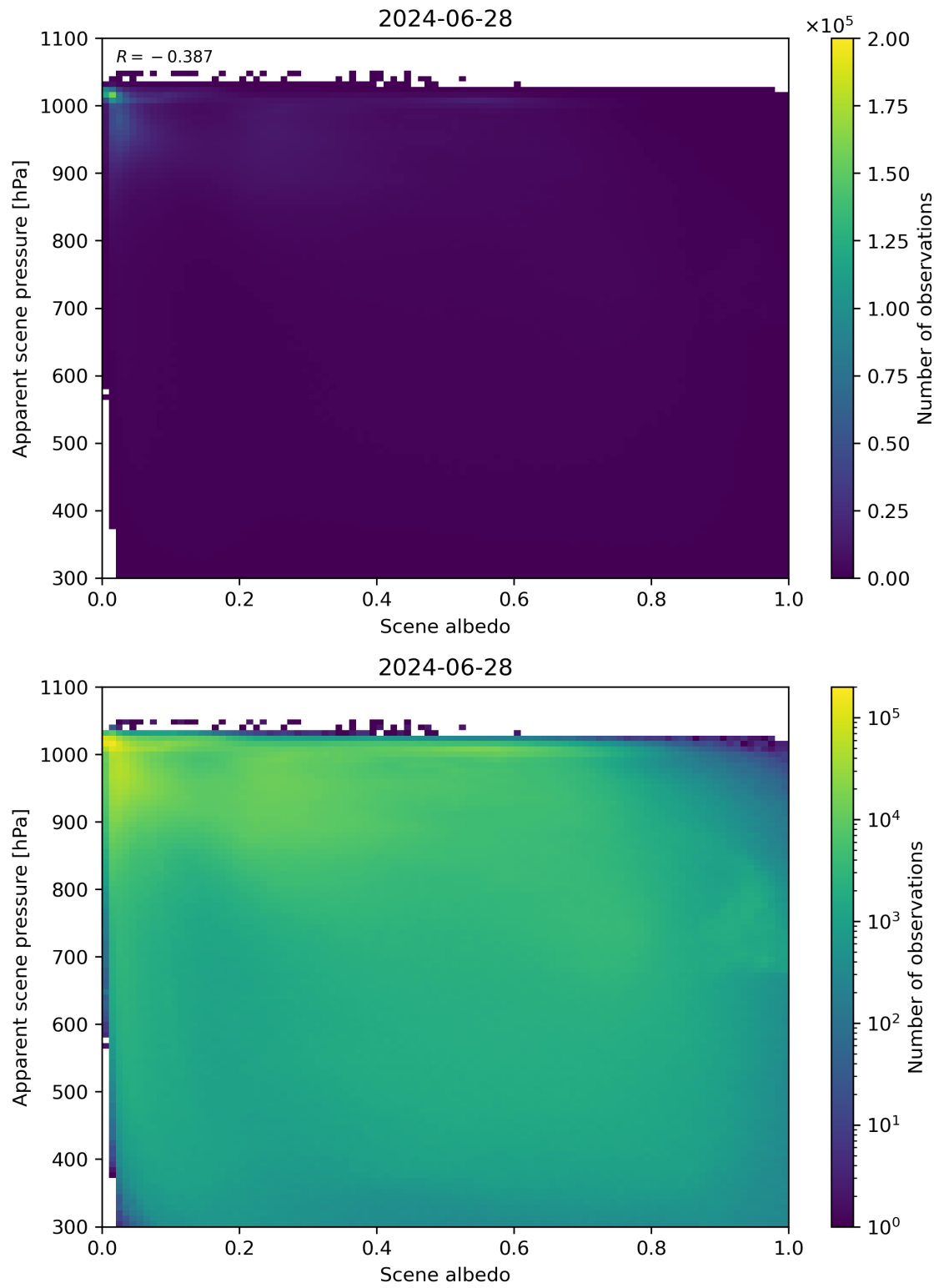
Figure 102: Scatter density plot of “Scene albedo” against “Apparent scene pressure” for 2024-06-27 to 2024-06-29.
