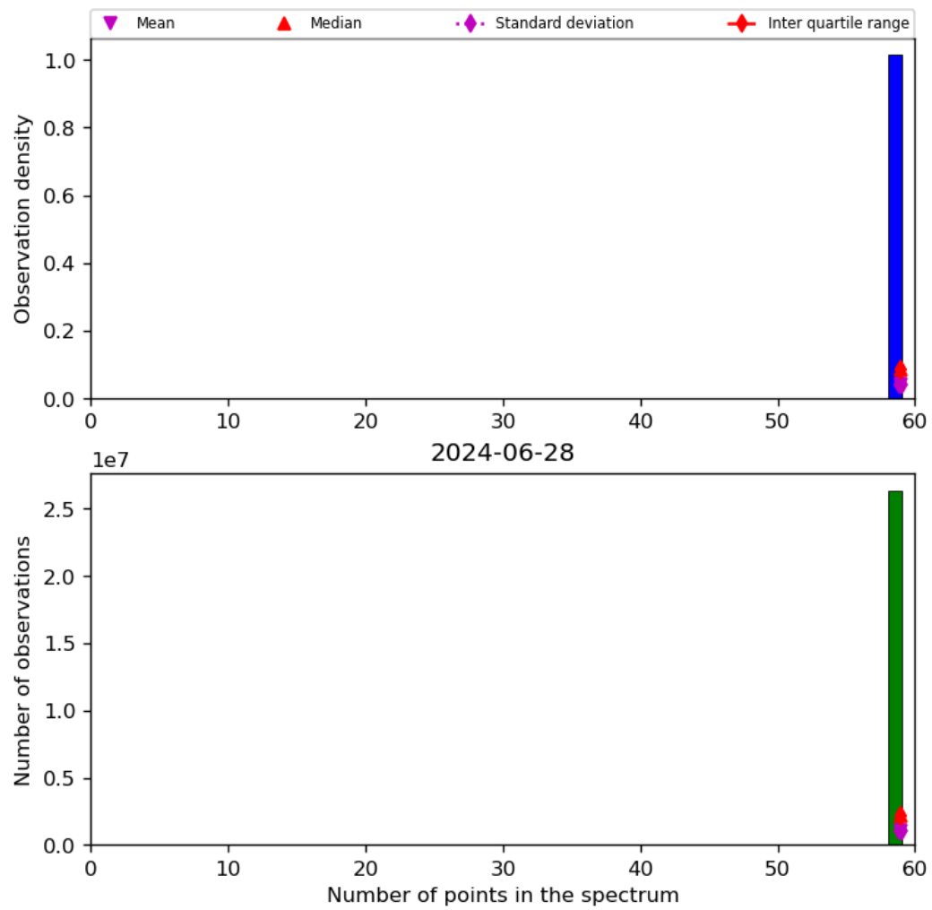
Figure 44: Histogram of “Number of points in the spectrum” for 2024-06-27 to 2024-06-29
