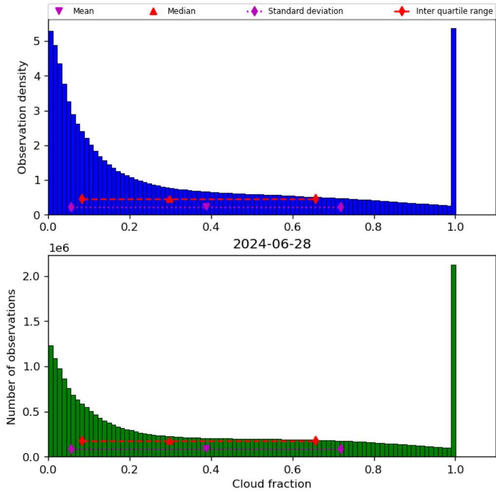
Figure 32: Histogram of “Cloud fraction” for 2024-06-27 to 2024-06-29
