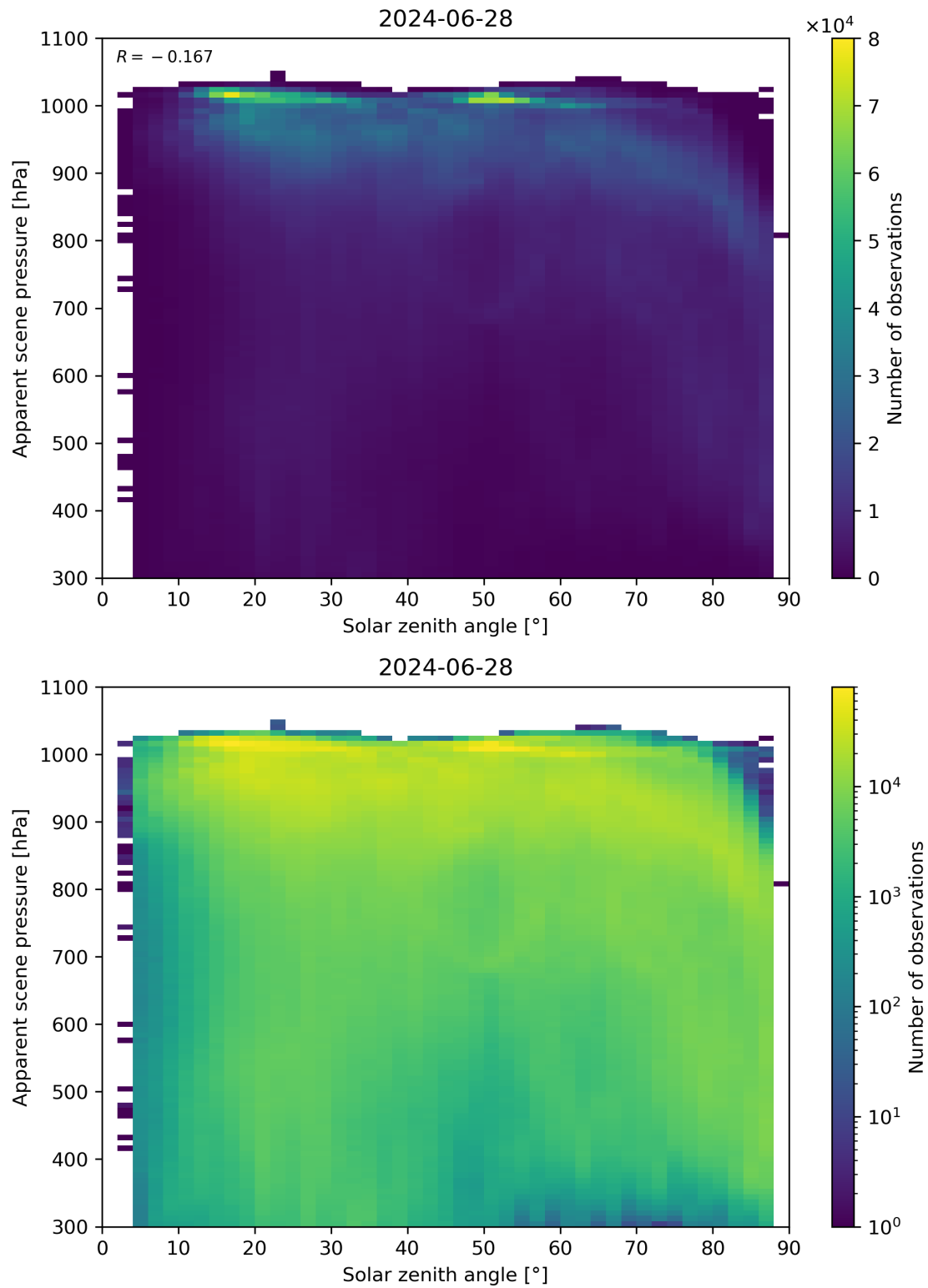
Figure 108: Scatter density plot of “Solar zenith angle” against “Apparent scene pressure” for 2024-06-27 to 2024-06-29.
