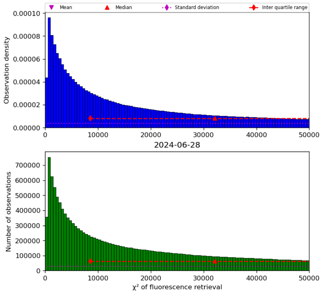
Figure 42: Histogram of “ \chi^2 of fluorescence retrieval” for 2024-06-27 to 2024-06-29
