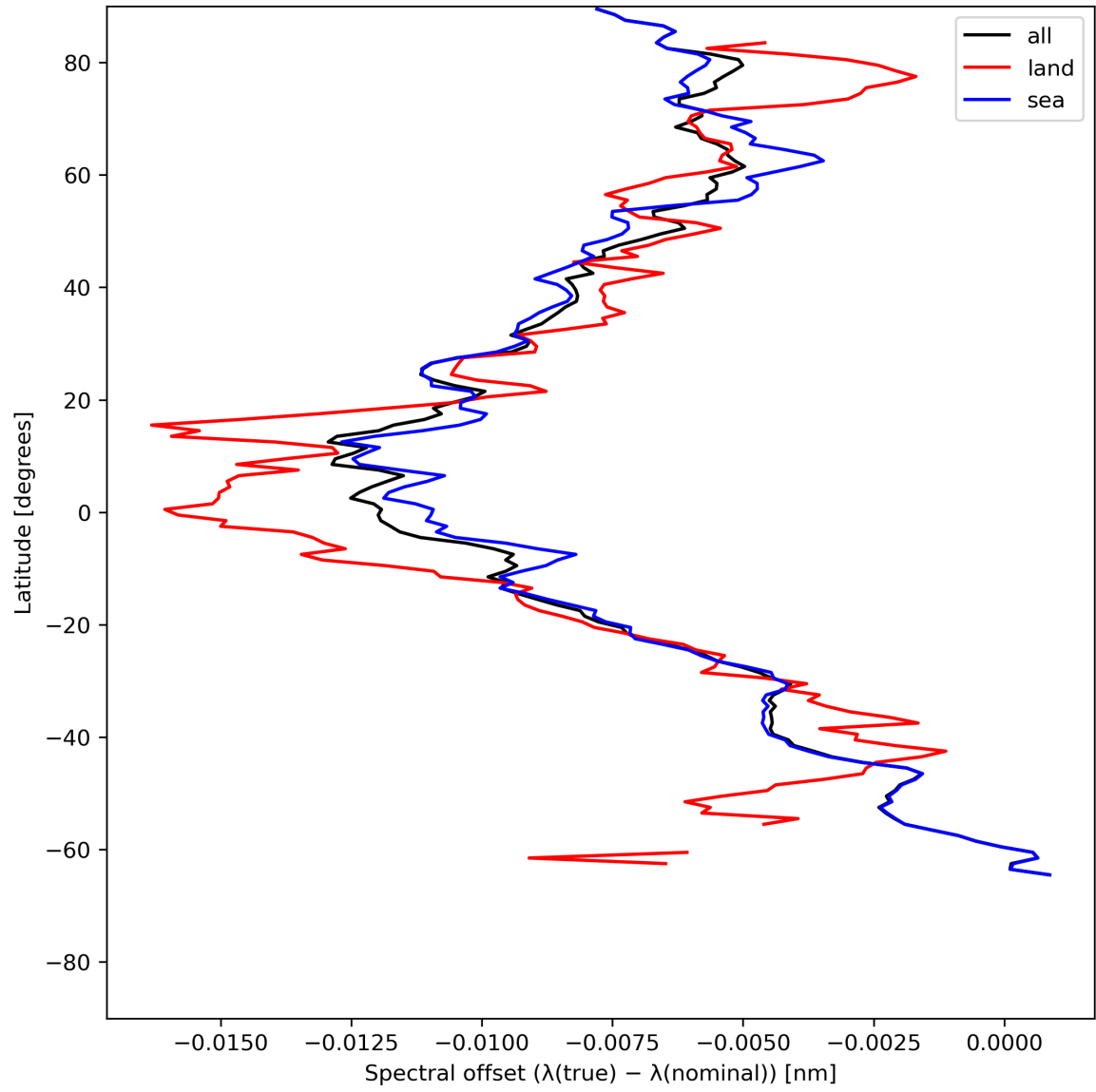
Figure 28: Zonal average of “Spectral offset ( \lambda(\text{true}) - \lambda(\text{nominal}) )” for 2024-06-27 to 2024-06-29.
