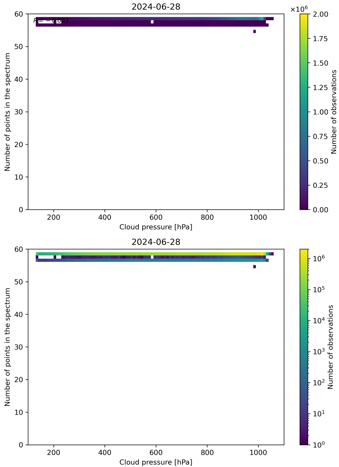
Figure 82: Scatter density plot of “Cloud pressure” against “Number of points in the spectrum” for 2024-06-27 to 2024-06-29.
