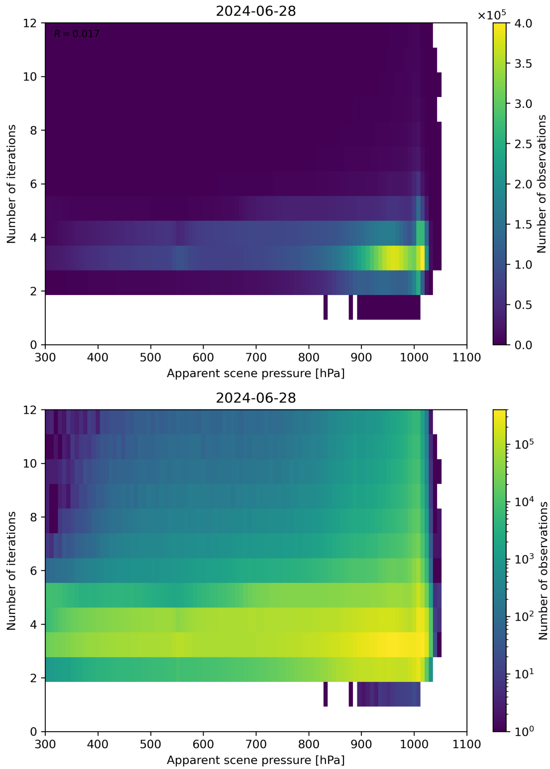
Figure 65: Scatter density plot of “Apparent scene pressure” against “Number of iterations” for 2024-06-27 to 2024-06-29.
