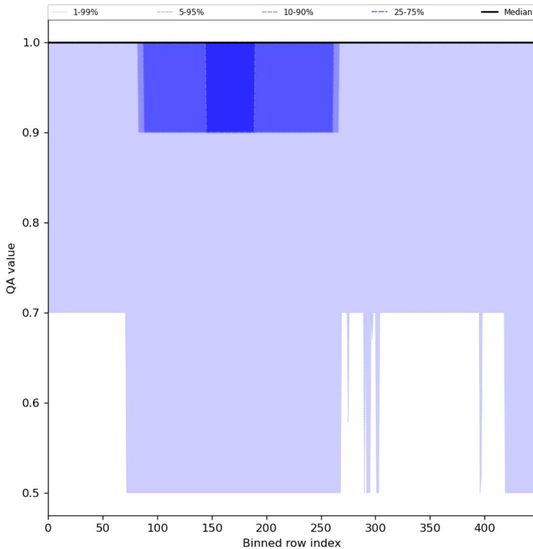
Figure 46: Along track statistics of “QA value” for 2024-06-27 to 2024-06-29
