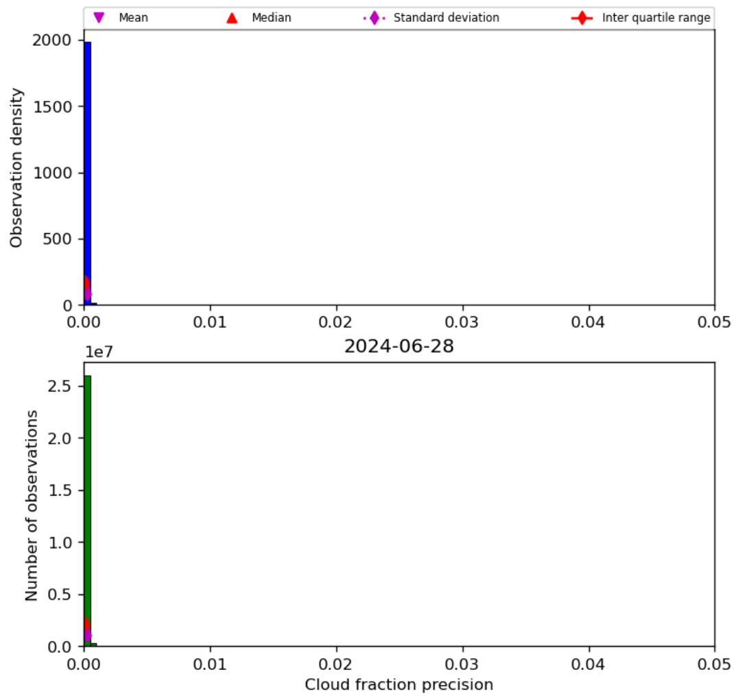
Figure 33: Histogram of “Cloud fraction precision” for 2024-06-27 to 2024-06-29
