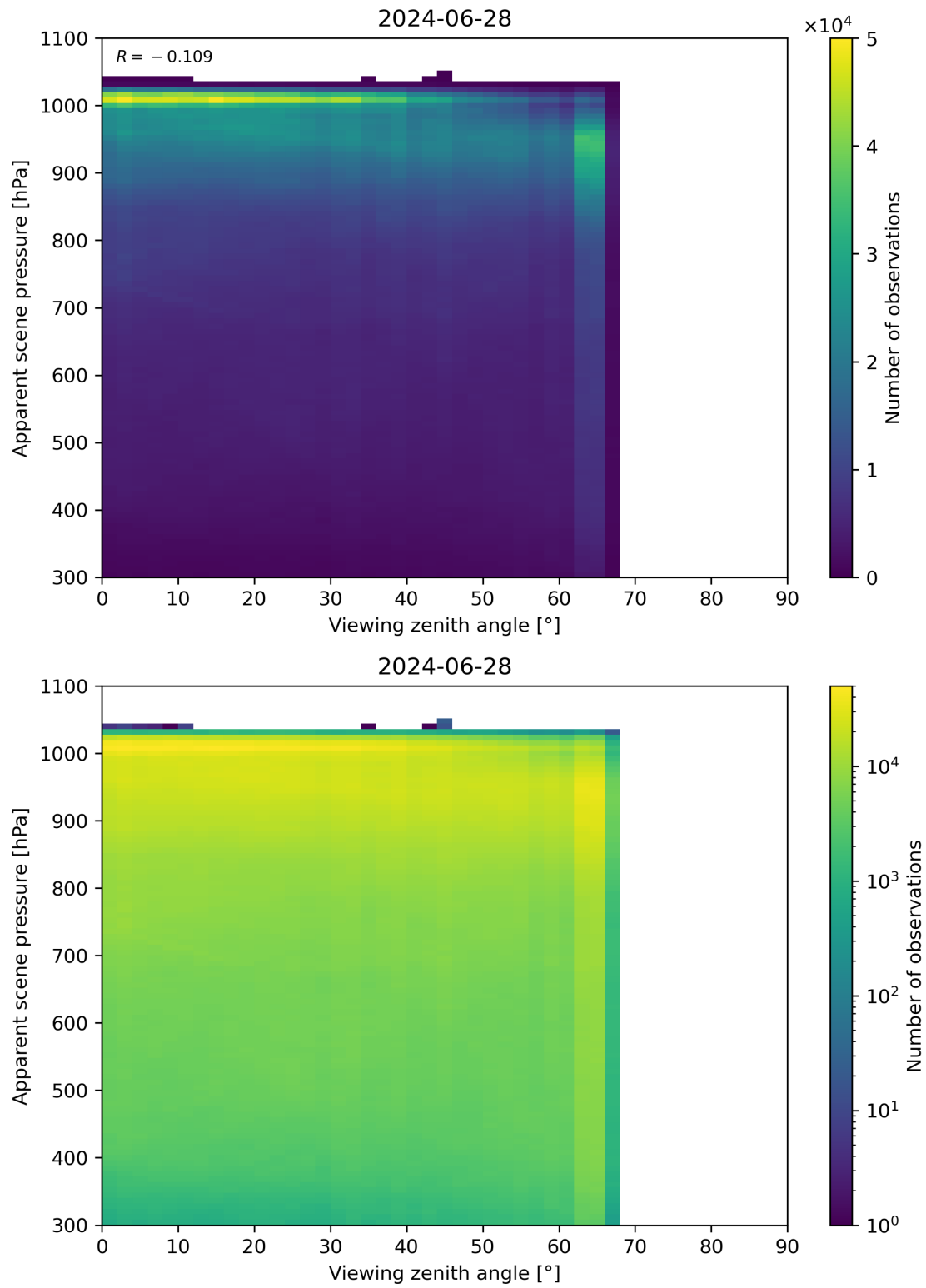
Figure 118: Scatter density plot of “Viewing zenith angle” against “Apparent scene pressure” for 2024-06-27 to 2024-06-29.
