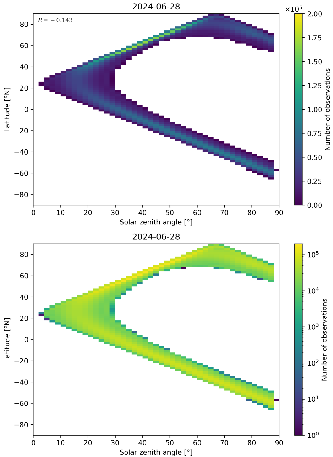
Figure 113: Scatter density plot of “Solar zenith angle” against “Latitude” for 2024-06-27 to 2024-06-29.
