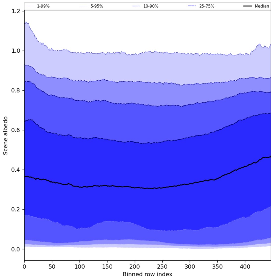
Figure 51: Along track statistics of “Scene albedo” for 2024-06-27 to 2024-06-29
