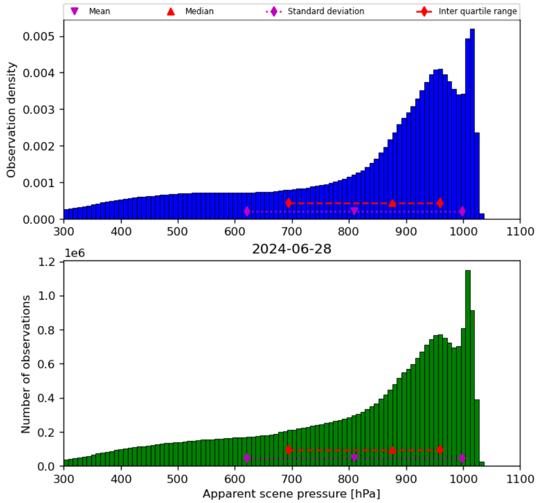
Figure 36: Histogram of “Apparent scene pressure” for 2024-06-27 to 2024-06-29
