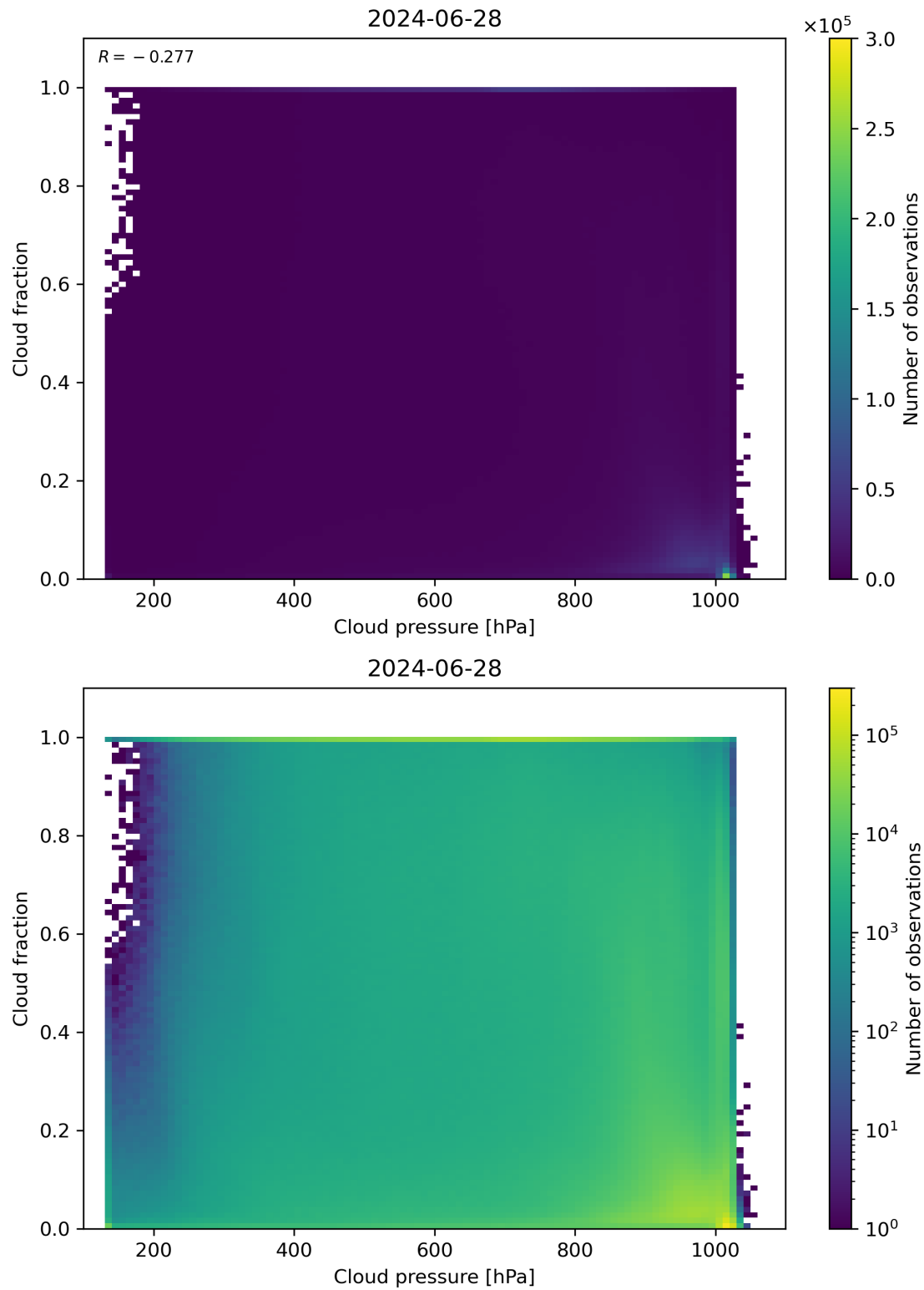
Figure 79: Scatter density plot of “Cloud pressure” against “Cloud fraction” for 2024-06-27 to 2024-06-29.
