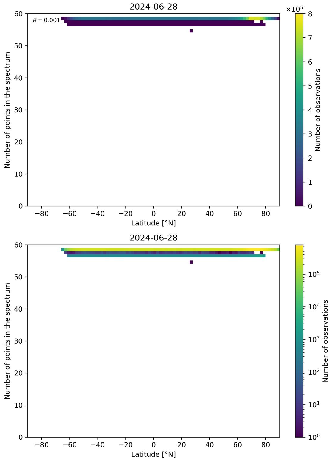
Figure 94: Scatter density plot of “Latitude” against “Number of points in the spectrum” for 2024-06-27 to 2024-06-29.
