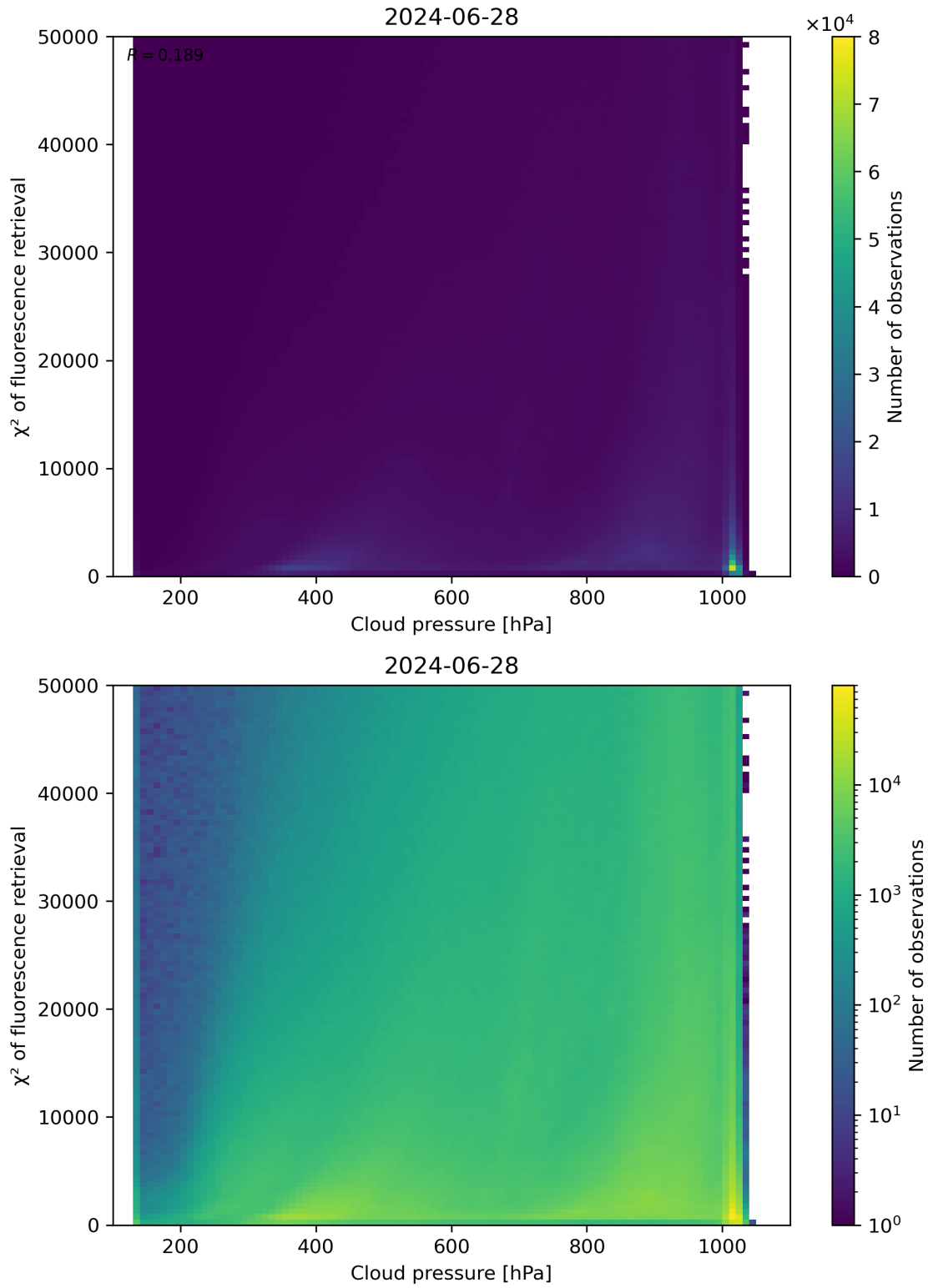
Figure 78: Scatter density plot of “Cloud pressure” against “ \chi^2 of fluorescence retrieval” for 2024-06-27 to 2024-06-29.
