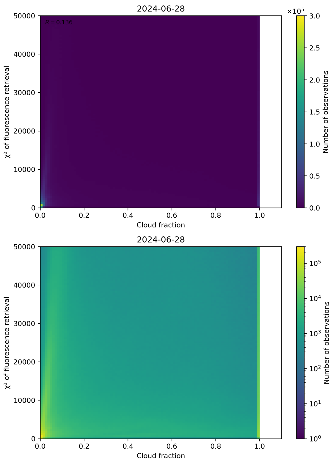
Figure 71: Scatter density plot of “Cloud fraction” against “ \chi^2 of fluorescence retrieval” for 2024-06-27 to 2024-06-29.
