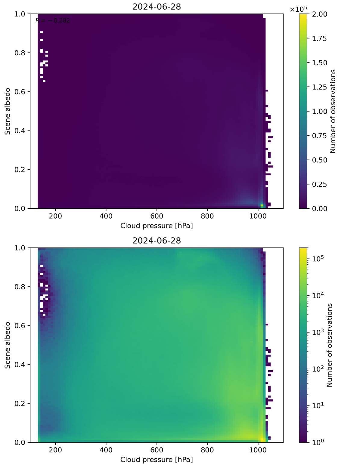
Figure 83: Scatter density plot of “Cloud pressure” against “Scene albedo” for 2024-06-27 to 2024-06-29.
