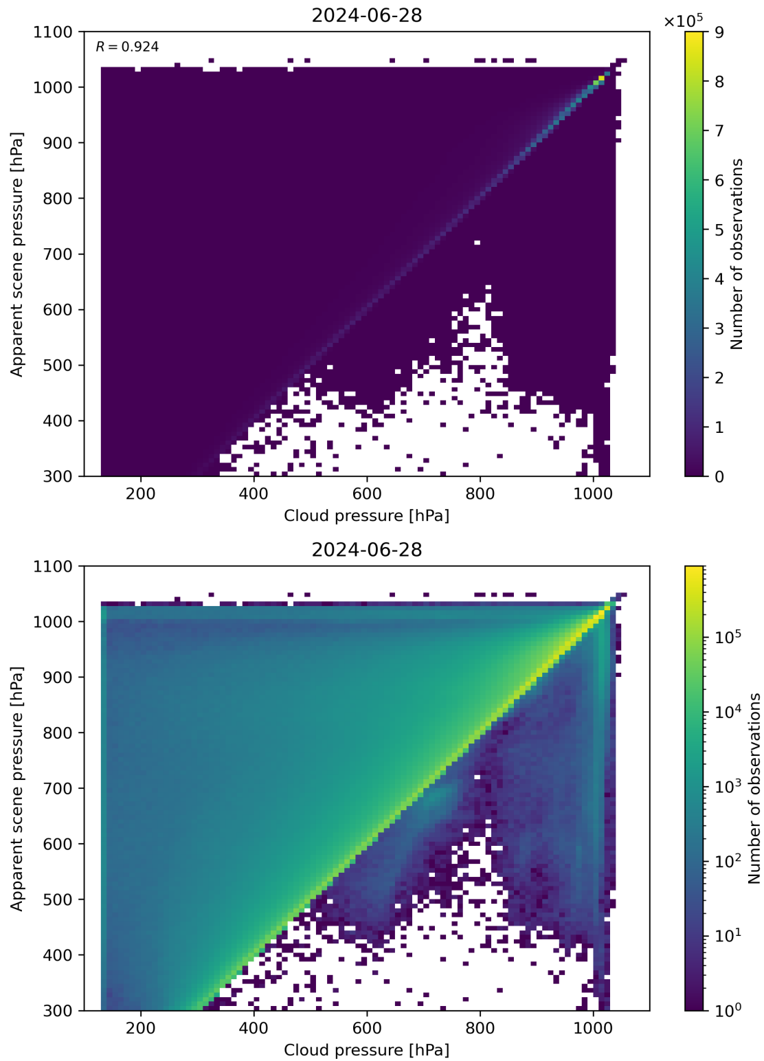
Figure 77: Scatter density plot of “Cloud pressure” against “Apparent scene pressure” for 2024-06-27 to 2024-06-29.
