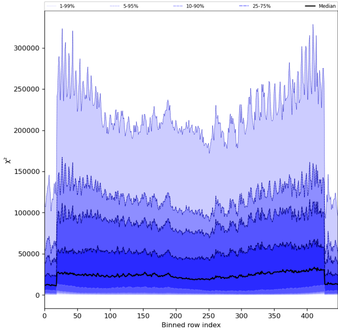
Figure 55: Along track statistics of “ \chi^2 ” for 2024-06-27 to 2024-06-29
