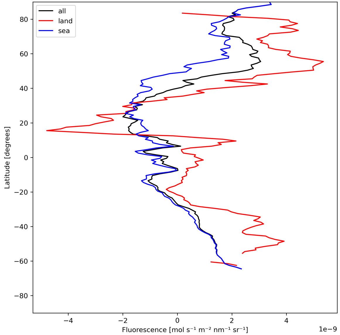
Figure 23: Zonal average of “Fluorescence” for 2024-06-27 to 2024-06-29.
