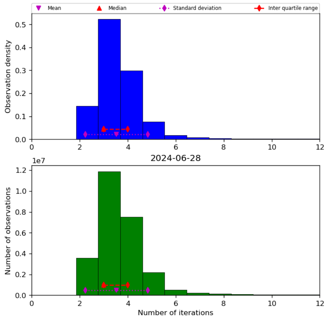
Figure 39: Histogram of “Number of iterations” for 2024-06-27 to 2024-06-29
