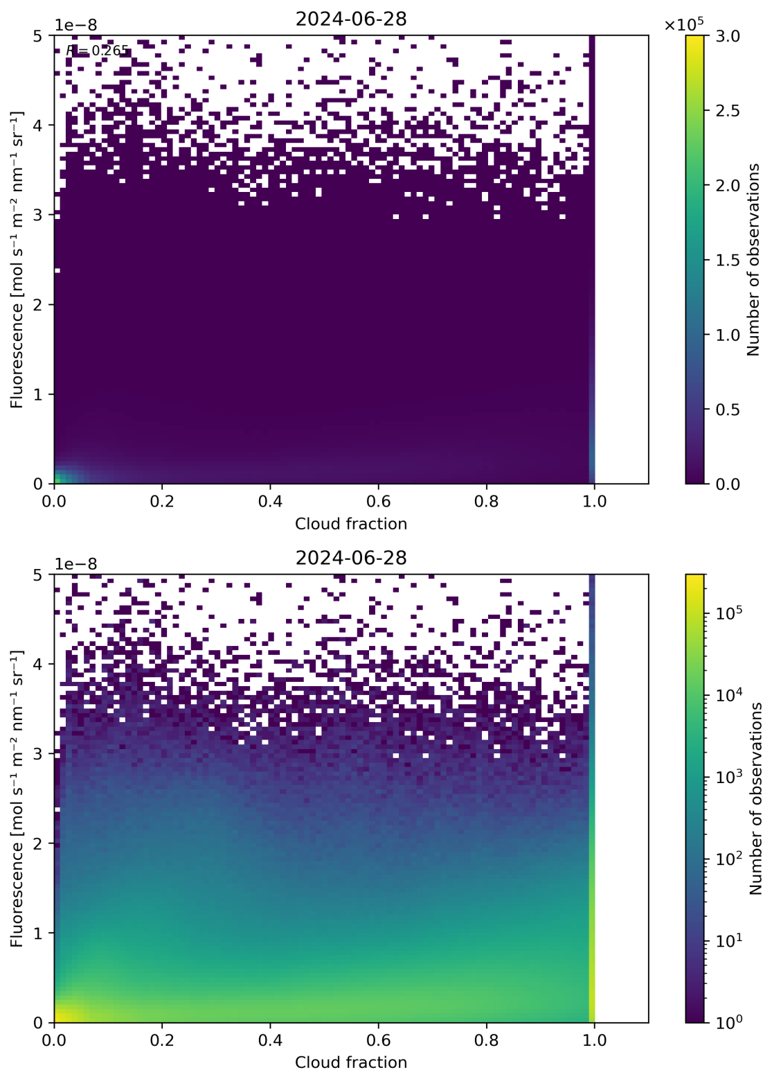
Figure 72: Scatter density plot of “Cloud fraction” against “Fluorescence” for 2024-06-27 to 2024-06-29.
