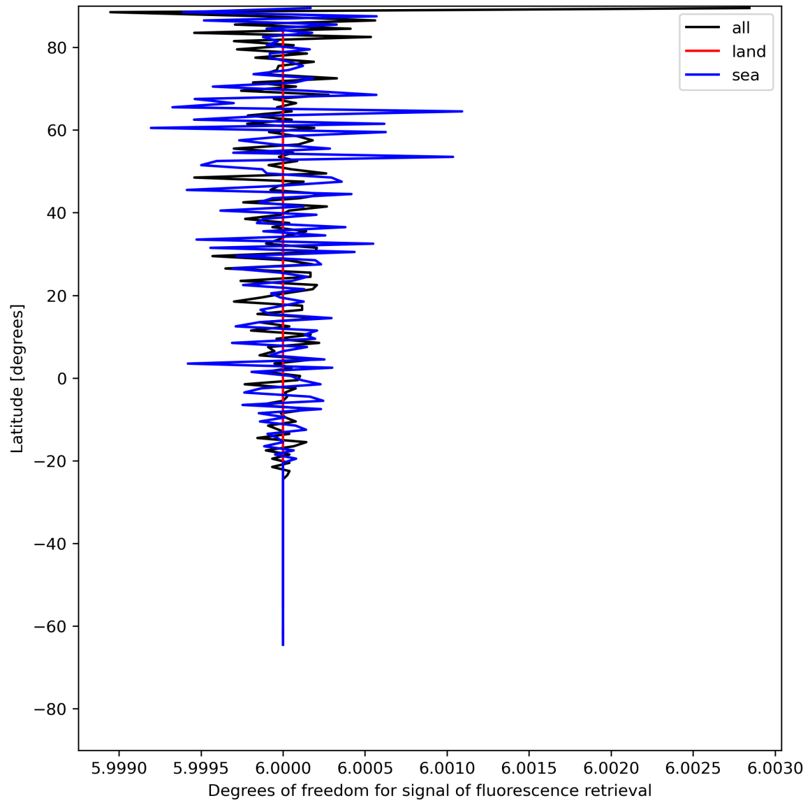
Figure 26: Zonal average of “Degrees of freedom for signal of fluorescence retrieval” for 2024-06-27 to 2024-06-29.
