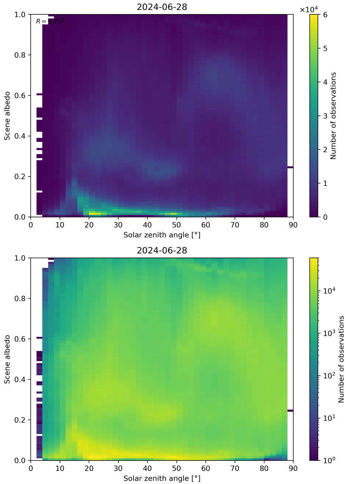
Figure 116: Scatter density plot of “Solar zenith angle” against “Scene albedo” for 2024-06-27 to 2024-06-29.
