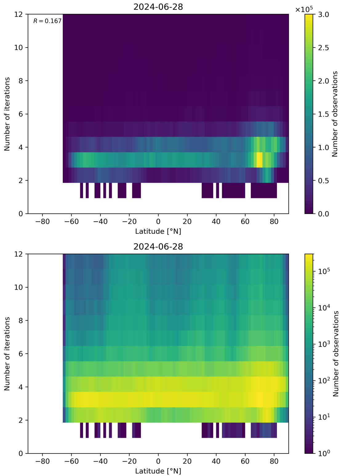
Figure 93: Scatter density plot of “Latitude” against “Number of iterations” for 2024-06-27 to 2024-06-29.
