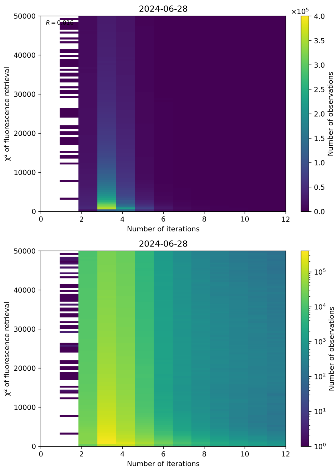
Figure 97: Scatter density plot of “Number of iterations” against “ \chi^2 of fluorescence retrieval” for 2024-06-27 to 2024-06-29.
