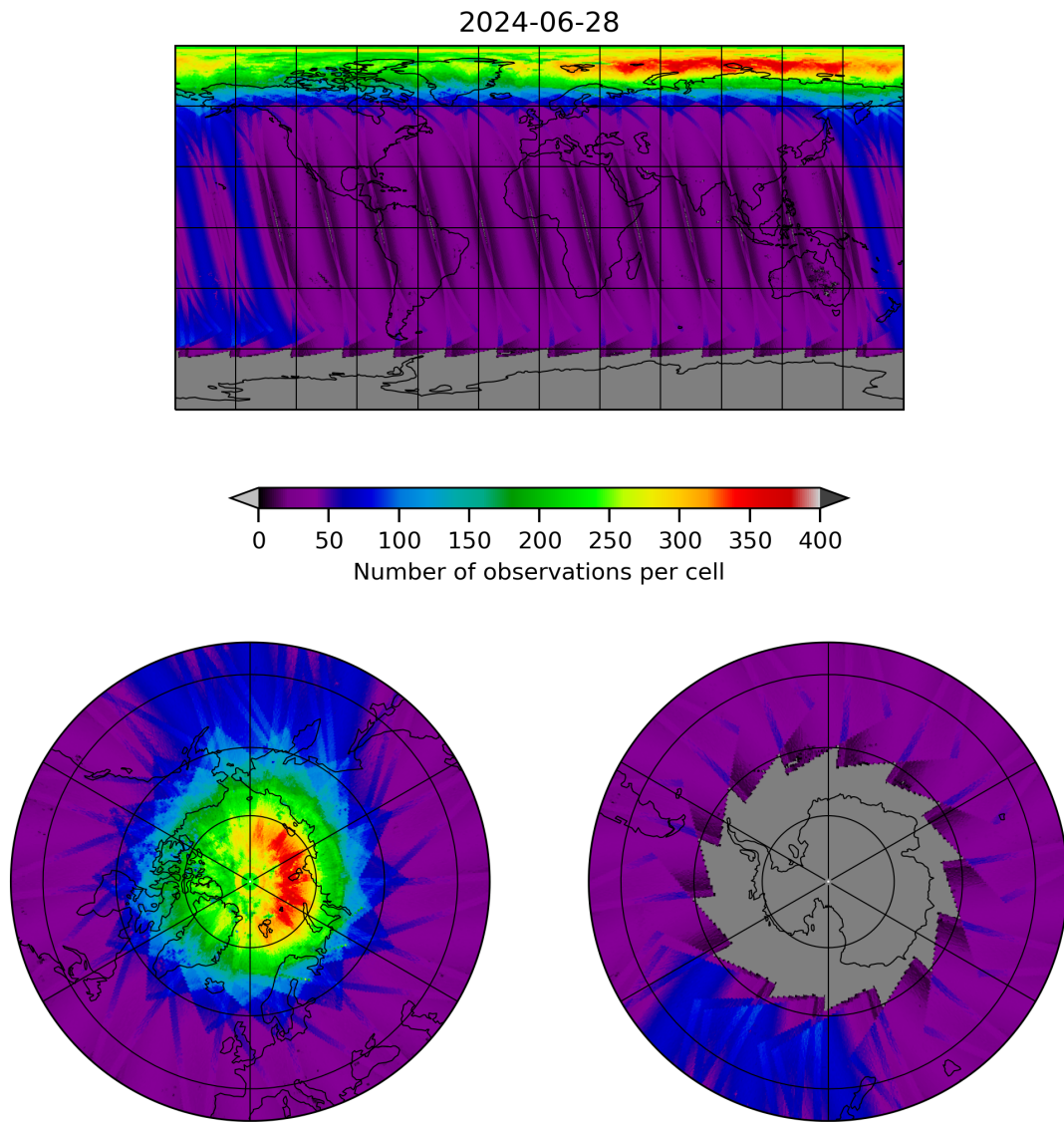
Figure 11: Map of the number of observations for 2024-06-27 to 2024-06-29
