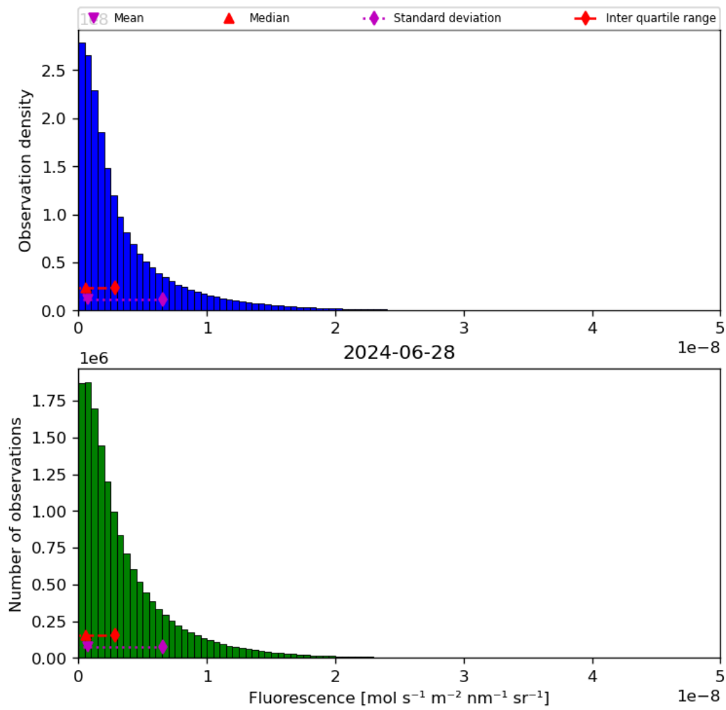
Figure 40: Histogram of “Fluorescence” for 2024-06-27 to 2024-06-29
