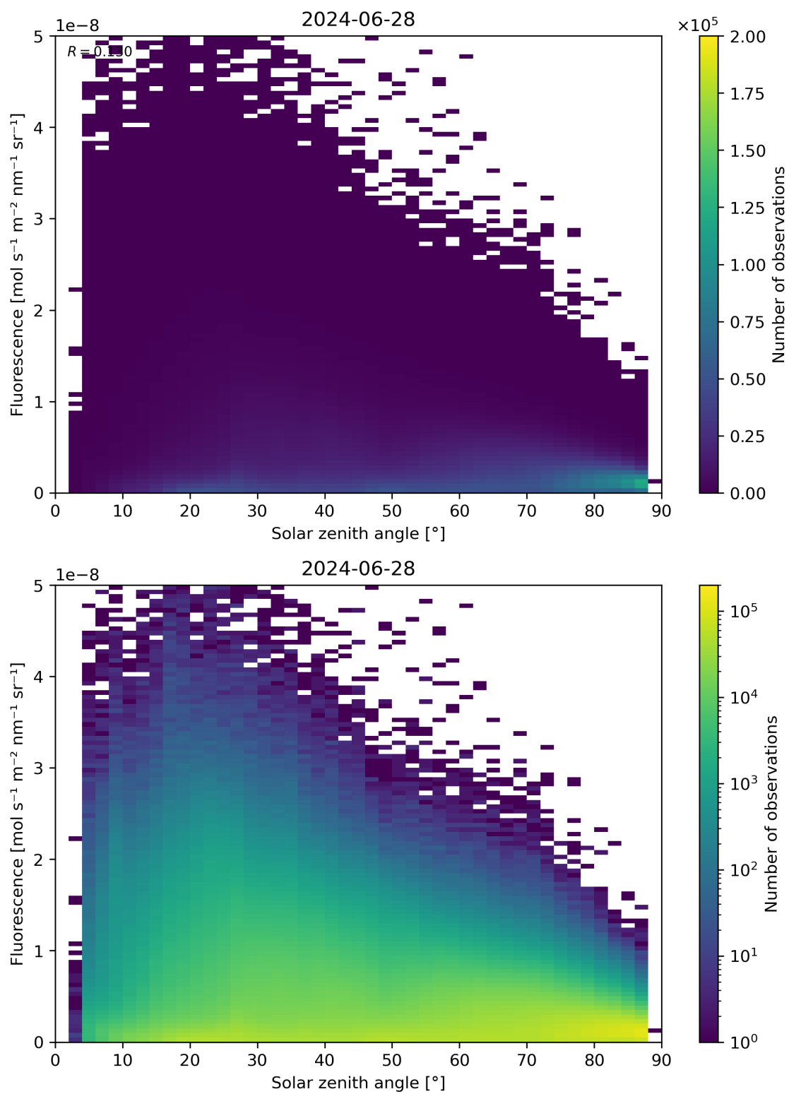
Figure 112: Scatter density plot of “Solar zenith angle” against “Fluorescence” for 2024-06-27 to 2024-06-29.
