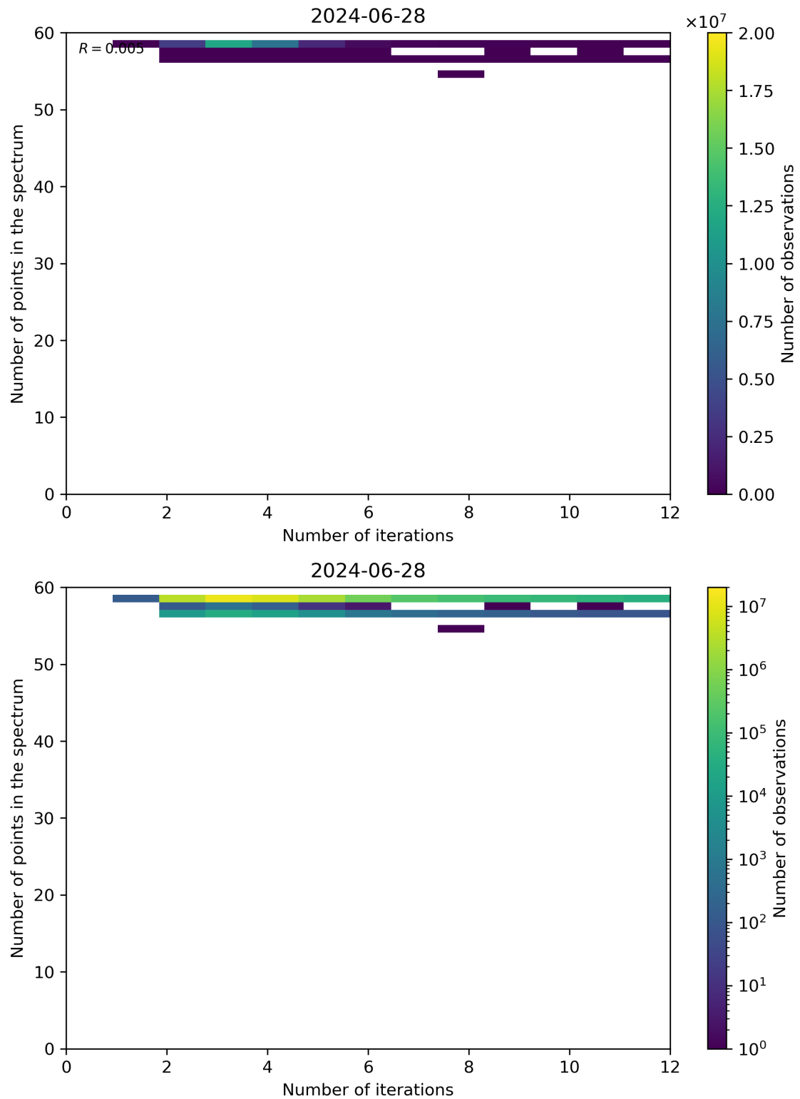
Figure 99: Scatter density plot of “Number of iterations” against “Number of points in the spectrum” for 2024-06-27 to 2024-06-29.
