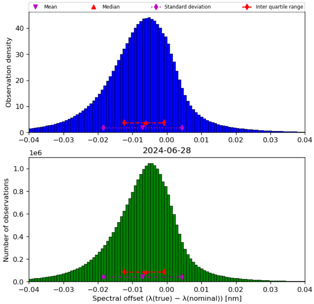
Figure 45: Histogram of “Spectral offset ( \lambda(\text{true}) - \lambda(\text{nominal}) )” for 2024-06-27 to 2024-06-29
