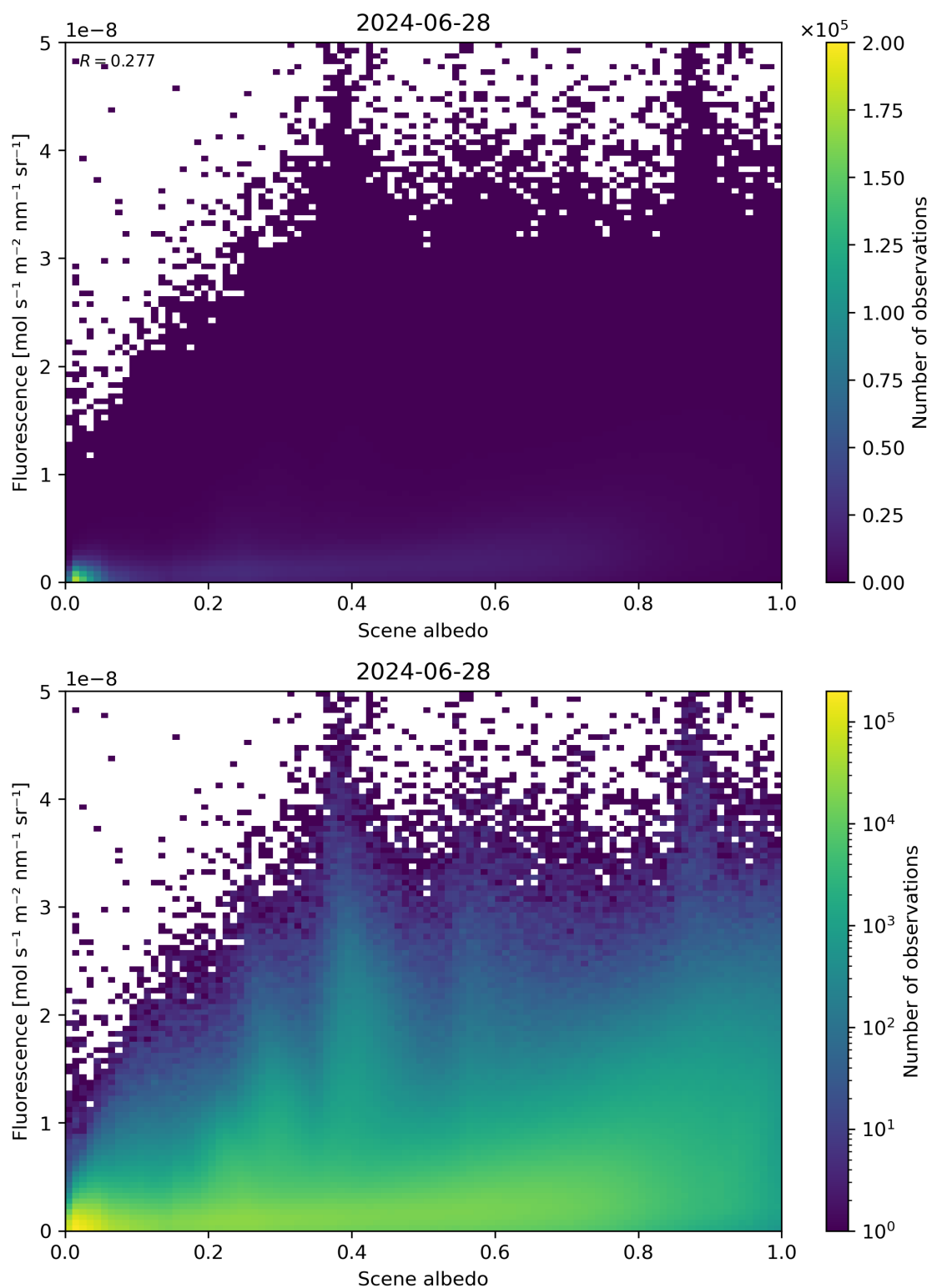
Figure 104: Scatter density plot of “Scene albedo” against “Fluorescence” for 2024-06-27 to 2024-06-29.
