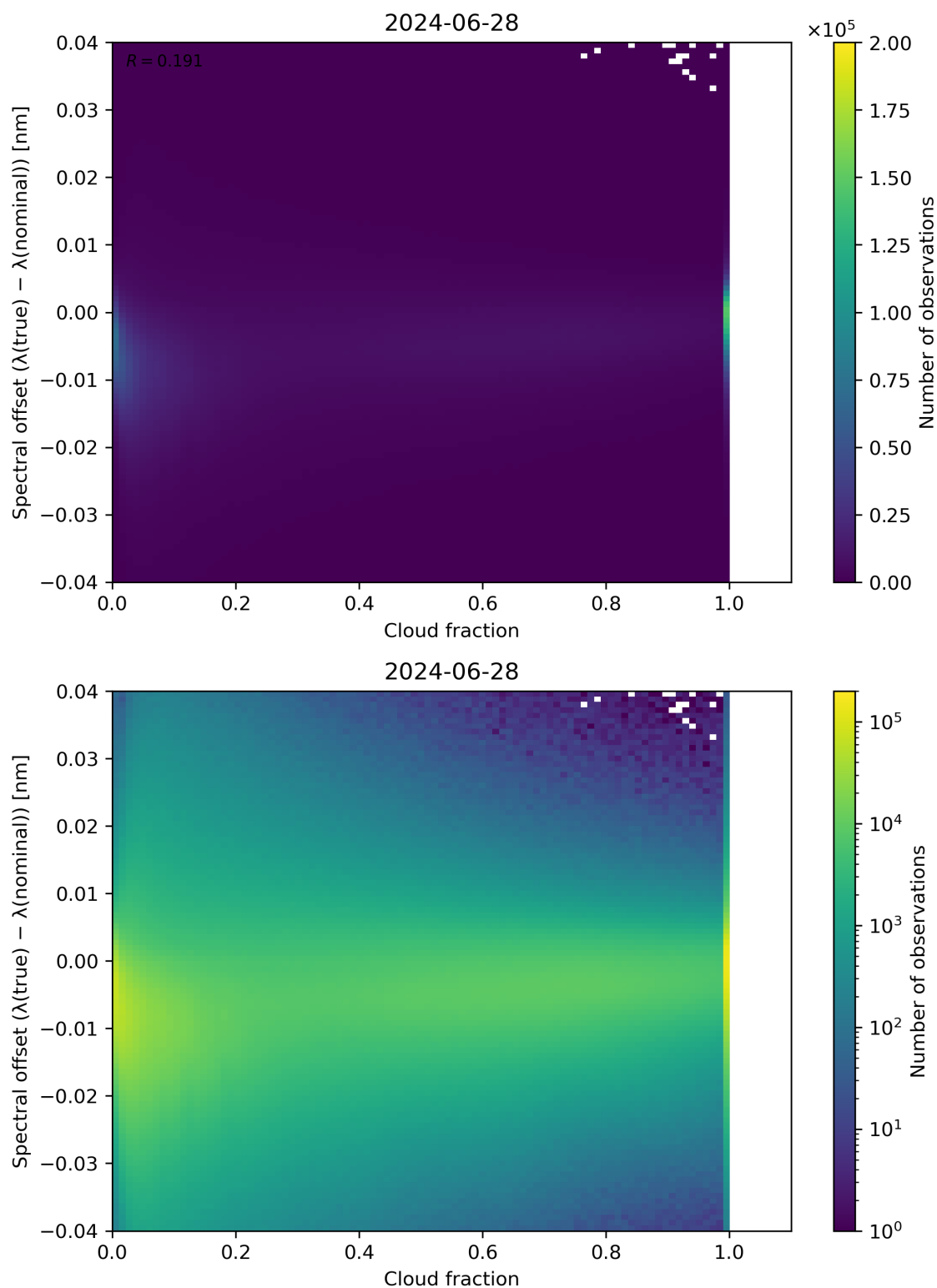
Figure 76: Scatter density plot of “Cloud fraction” against “Spectral offset ( \lambda(\text{true}) - \lambda(\text{nominal}) )” for 2024-06-27 to 2024-06-29.
