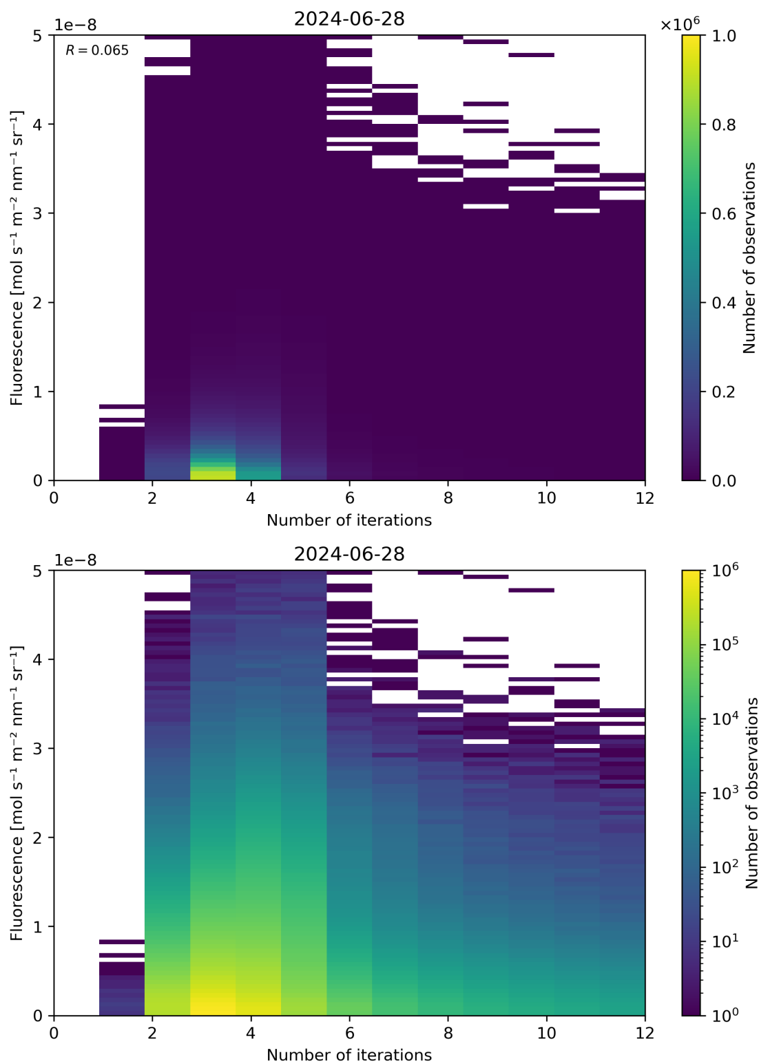
Figure 98: Scatter density plot of “Number of iterations” against “Fluorescence” for 2024-06-27 to 2024-06-29.
