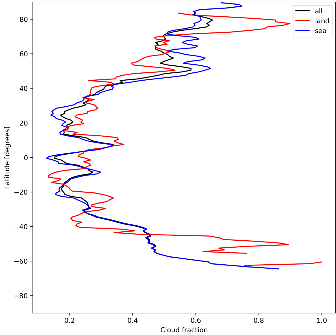
Figure 15: Zonal average of “Cloud fraction” for 2024-06-27 to 2024-06-29.
