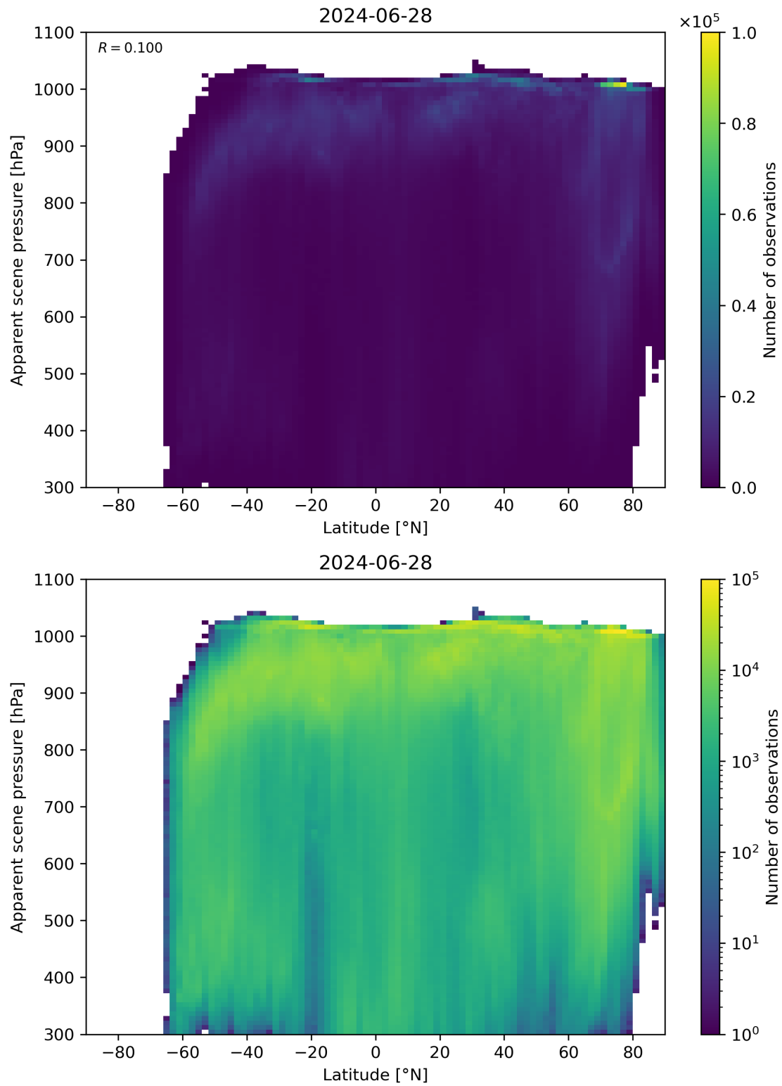
Figure 88: Scatter density plot of “Latitude” against “Apparent scene pressure” for 2024-06-27 to 2024-06-29.
