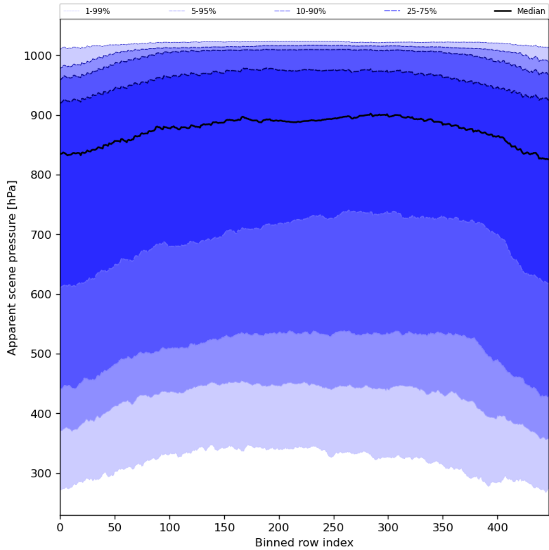
Figure 53: Along track statistics of “Apparent scene pressure” for 2024-06-27 to 2024-06-29
