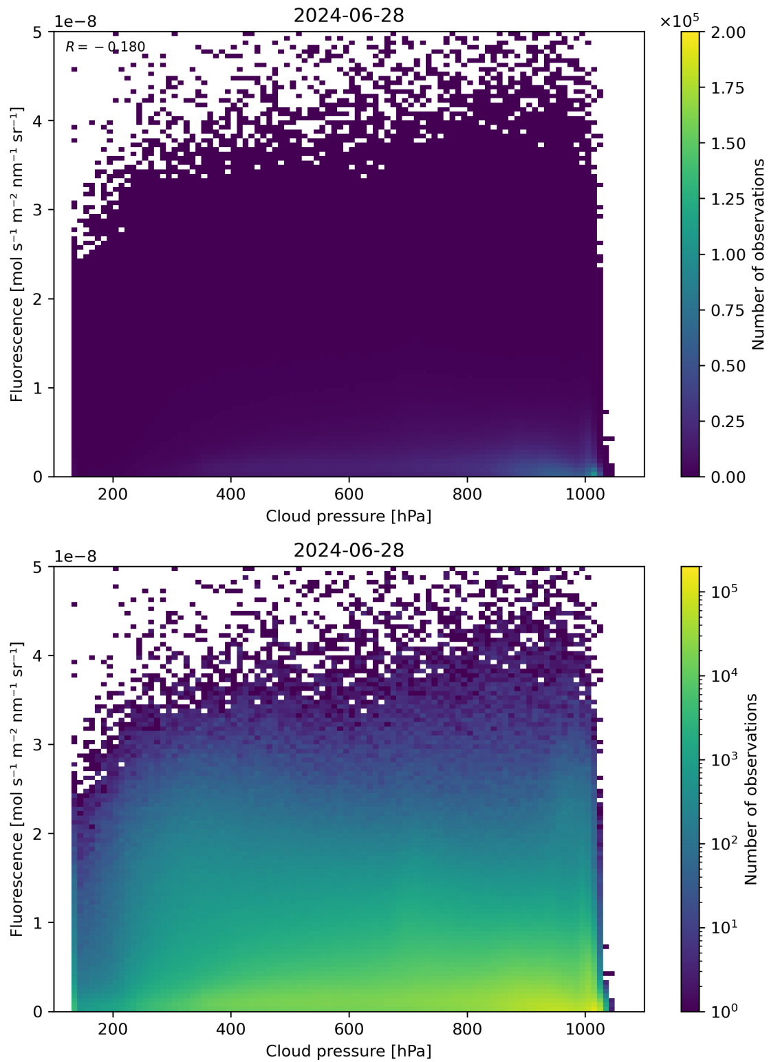
Figure 80: Scatter density plot of “Cloud pressure” against “Fluorescence” for 2024-06-27 to 2024-06-29.
