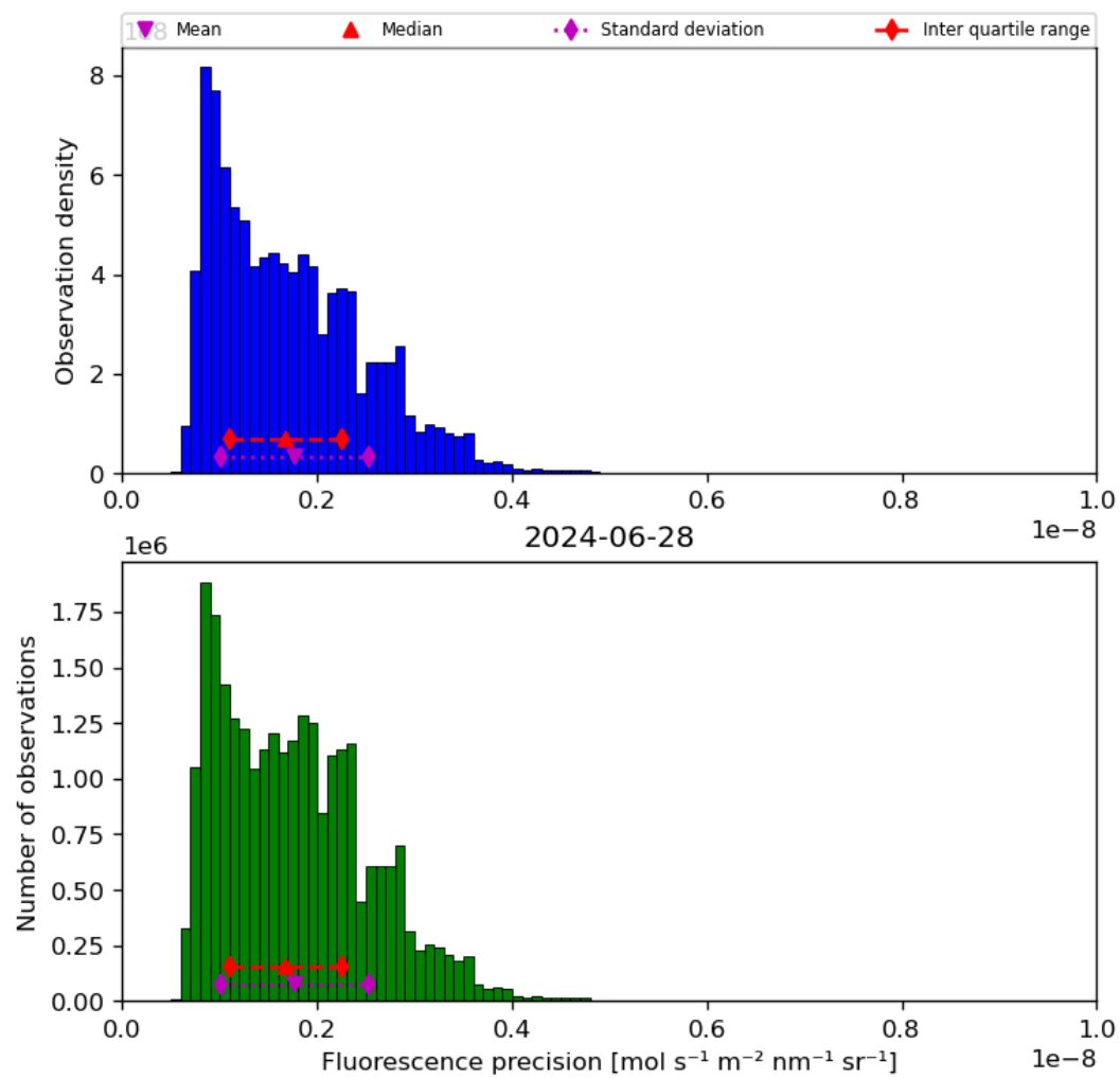
Figure 41: Histogram of “Fluorescence precision” for 2024-06-27 to 2024-06-29
