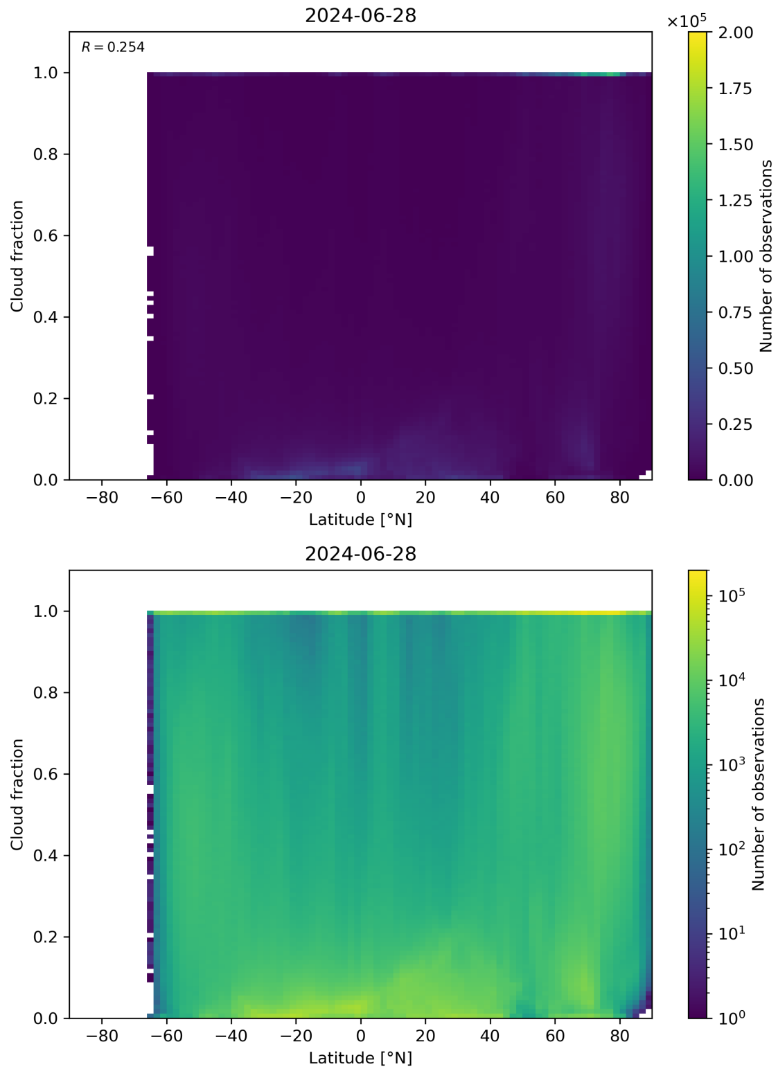
Figure 90: Scatter density plot of “Latitude” against “Cloud fraction” for 2024-06-27 to 2024-06-29.
