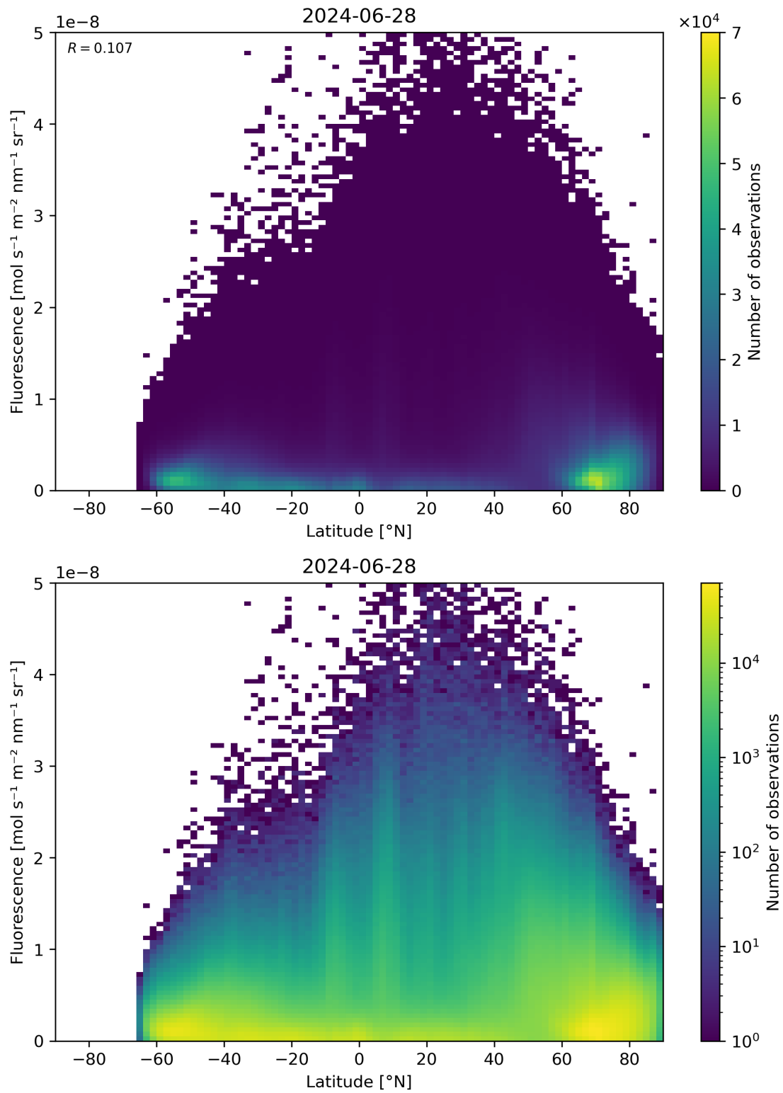
Figure 92: Scatter density plot of “Latitude” against “Fluorescence” for 2024-06-27 to 2024-06-29.
