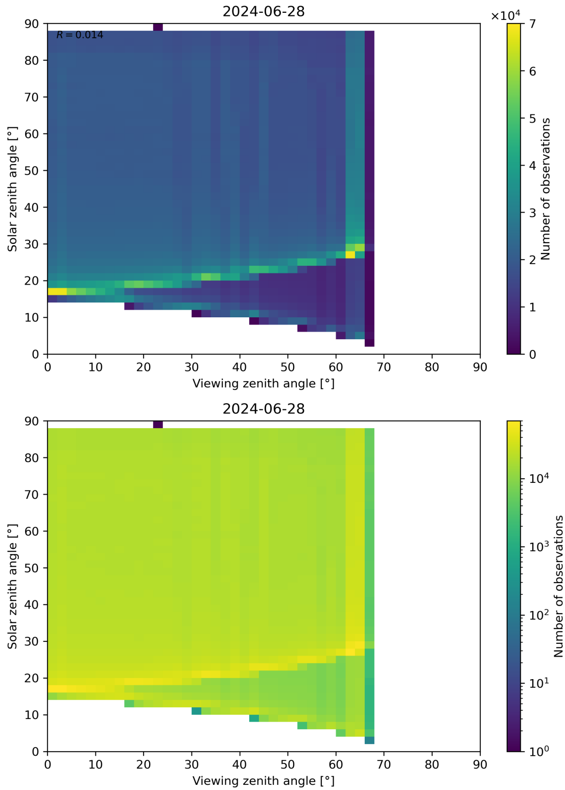
Figure 127: Scatter density plot of “Viewing zenith angle” against “Solar zenith angle” for 2024-06-27 to 2024-06-29.
