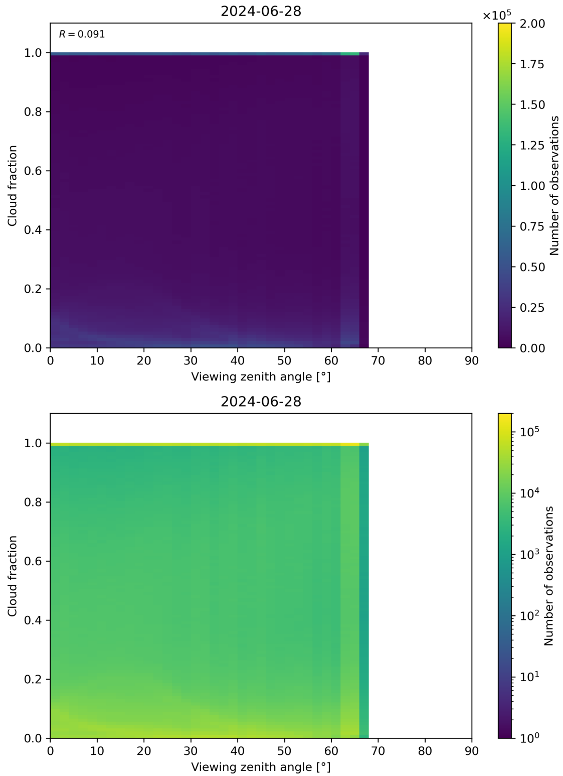
Figure 120: Scatter density plot of “Viewing zenith angle” against “Cloud fraction” for 2024-06-27 to 2024-06-29.
