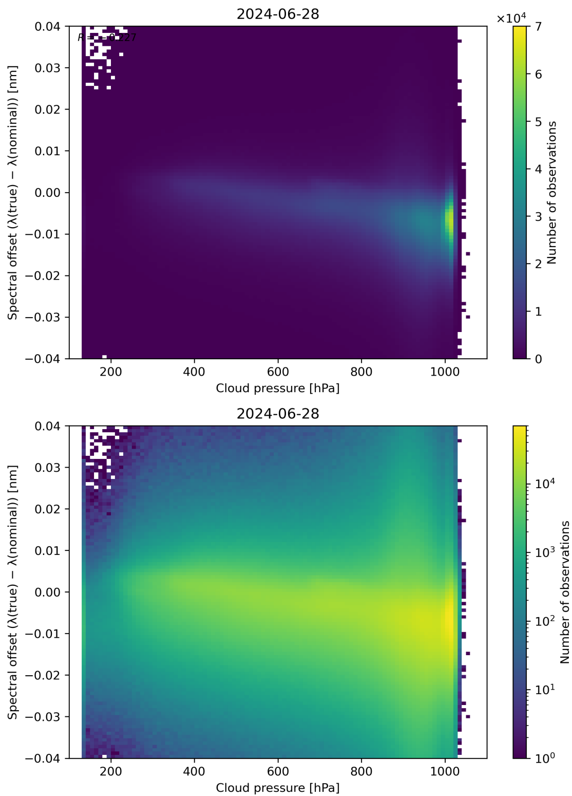
Figure 84: Scatter density plot of “Cloud pressure” against “Spectral offset ( \lambda(\text{true}) - \lambda(\text{nominal}) )” for 2024-06-27 to 2024-06-29.
