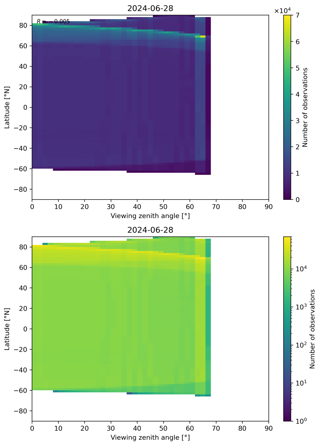
Figure 123: Scatter density plot of “Viewing zenith angle” against “Latitude” for 2024-06-27 to 2024-06-29.
