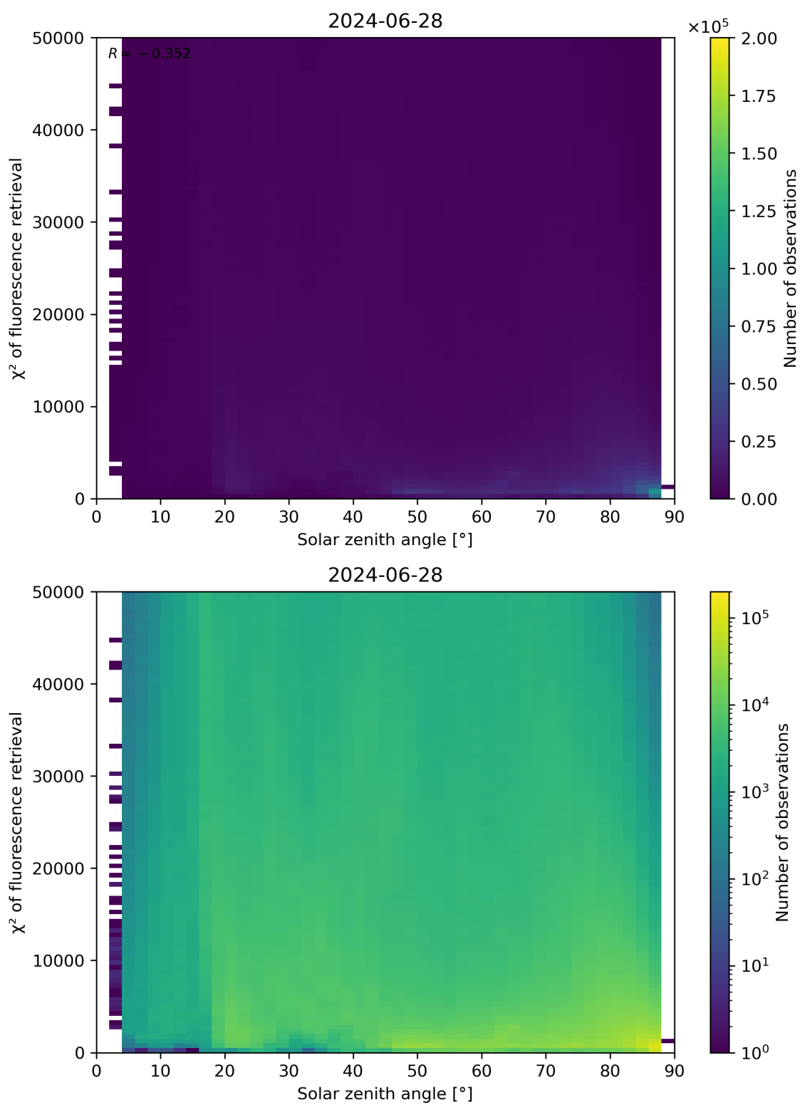
Figure 109: Scatter density plot of “Solar zenith angle” against “ \chi^2 of fluorescence retrieval” for 2024-06-27 to 2024-06-29.
