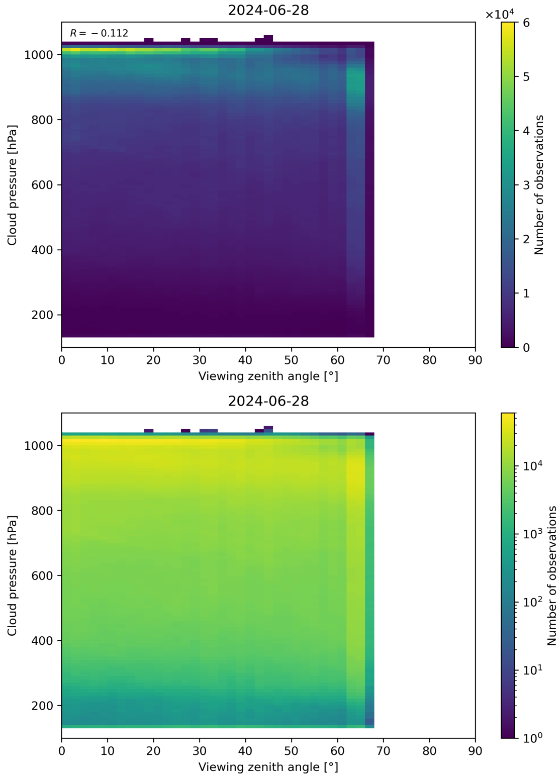
Figure 121: Scatter density plot of “Viewing zenith angle” against “Cloud pressure” for 2024-06-27 to 2024-06-29.
