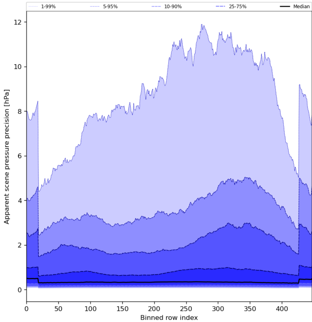
Figure 54: Along track statistics of “Apparent scene pressure precision” for 2024-06-27 to 2024-06-29
