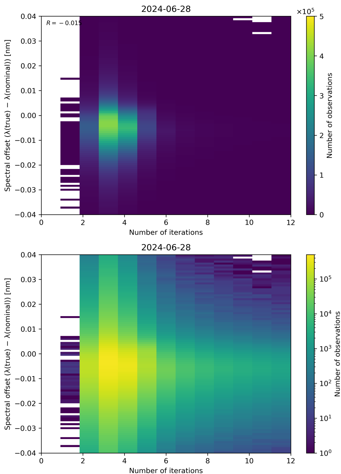
Figure 100: Scatter density plot of “Number of iterations” against “Spectral offset ( \lambda(\text{true}) - \lambda(\text{nominal}) )” for 2024-06-27 to 2024-06-29.
