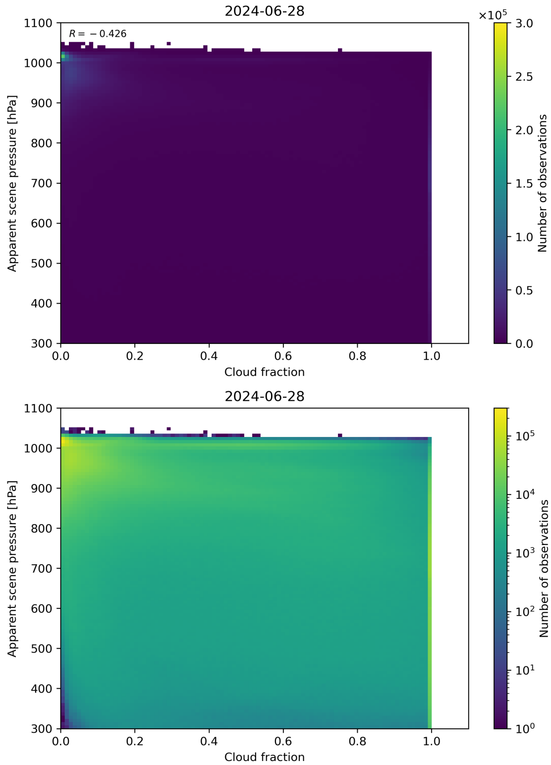
Figure 70: Scatter density plot of “Cloud fraction” against “Apparent scene pressure” for 2024-06-27 to 2024-06-29.
