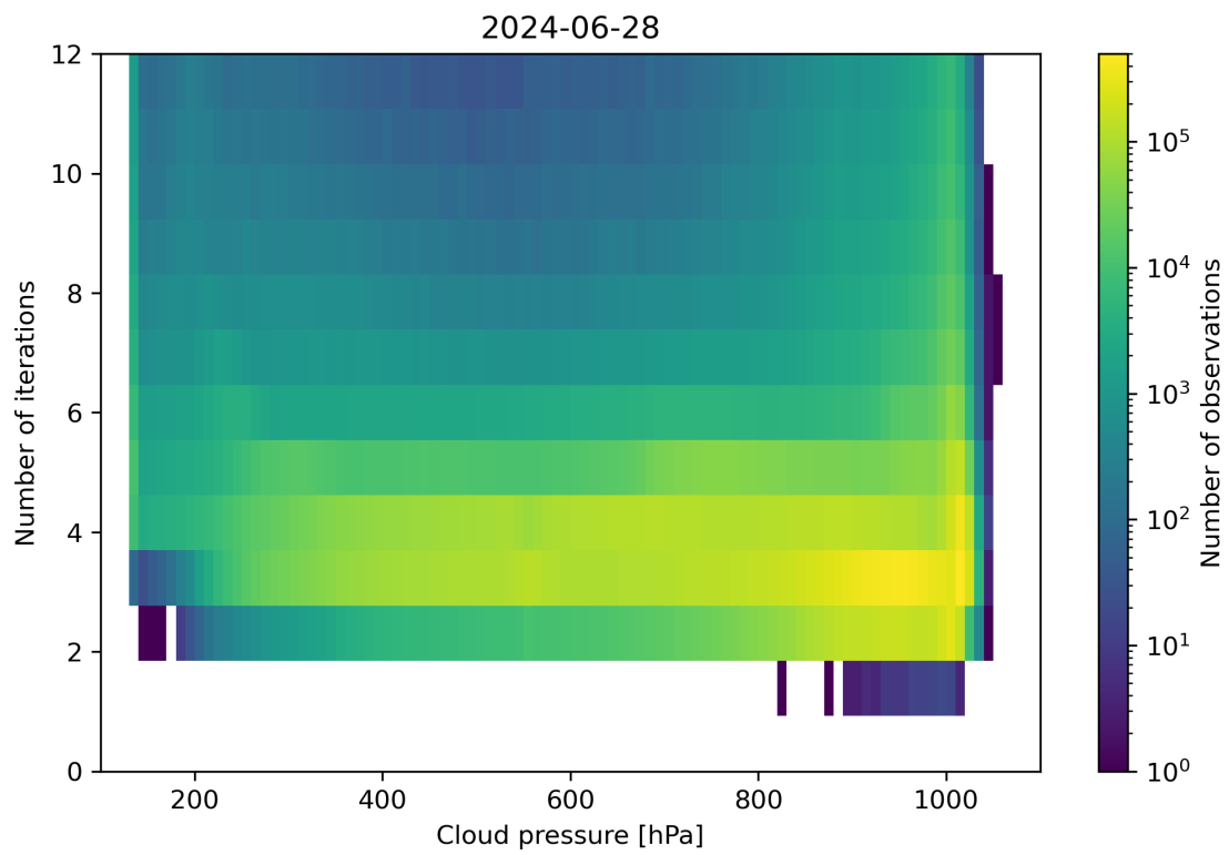
Figure 81: Scatter density plot of “Cloud pressure” against “Number of iterations” for 2024-06-27 to 2024-06-29.
