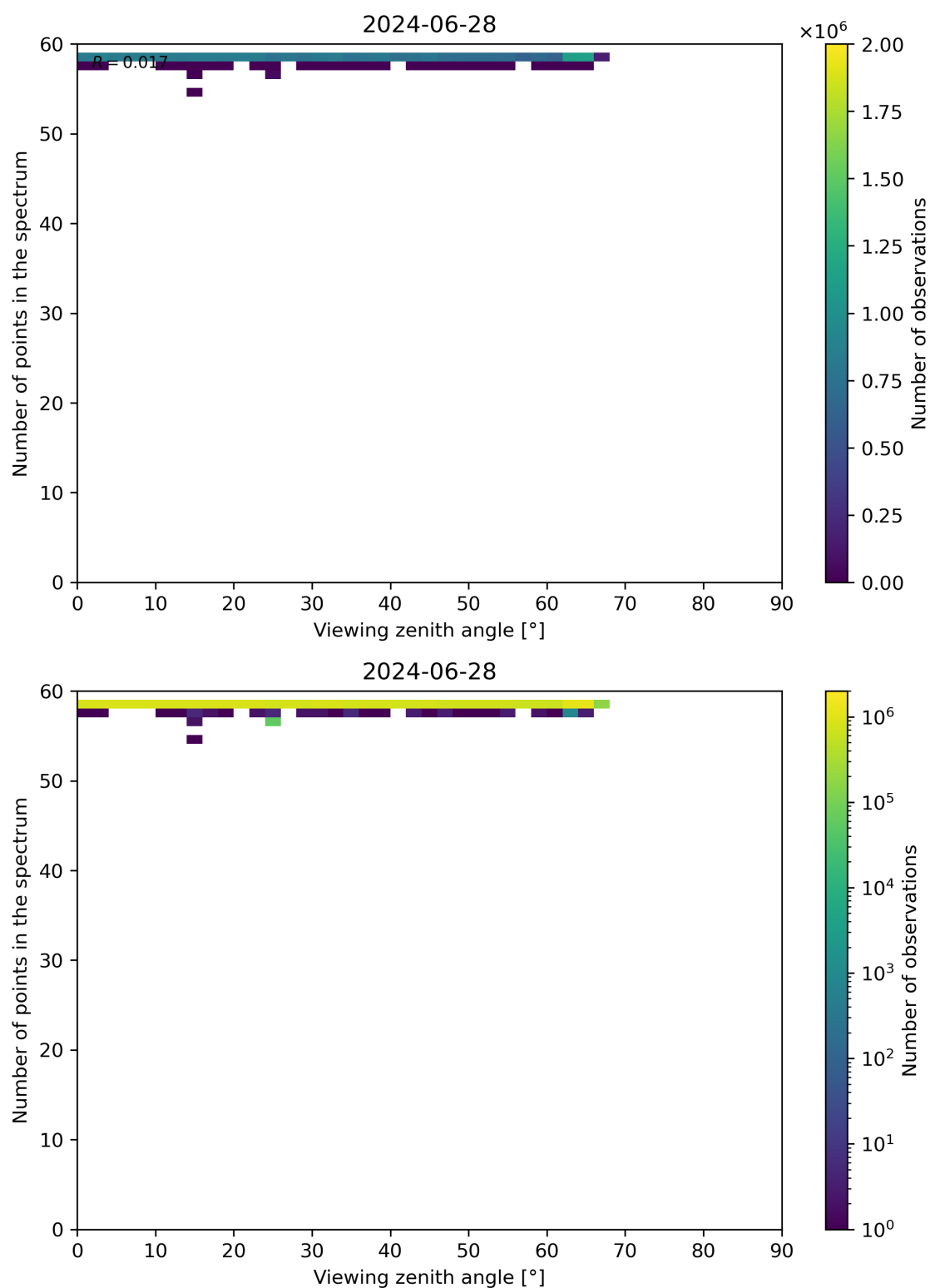
Figure 125: Scatter density plot of “Viewing zenith angle” against “Number of points in the spectrum” for 2024-06-27 to 2024-06-29.
