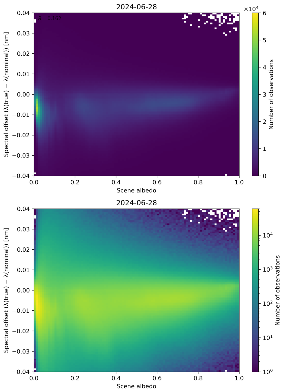
Figure 107: Scatter density plot of “Scene albedo” against “Spectral offset ( \lambda(\text{true}) - \lambda(\text{nominal}) )” for 2024-06-27 to 2024-06-29.
