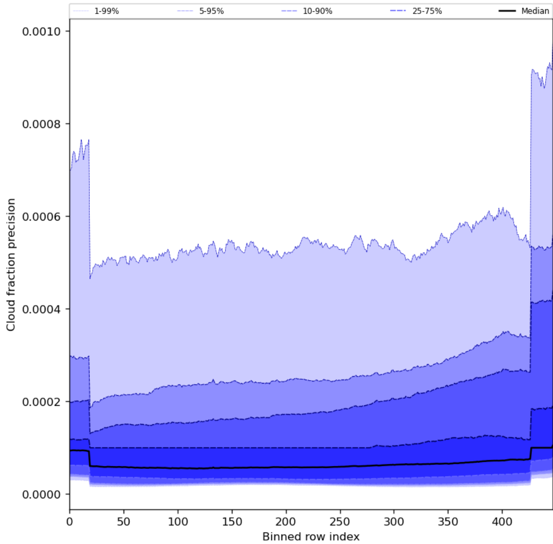
Figure 50: Along track statistics of “Cloud fraction precision” for 2024-06-27 to 2024-06-29
