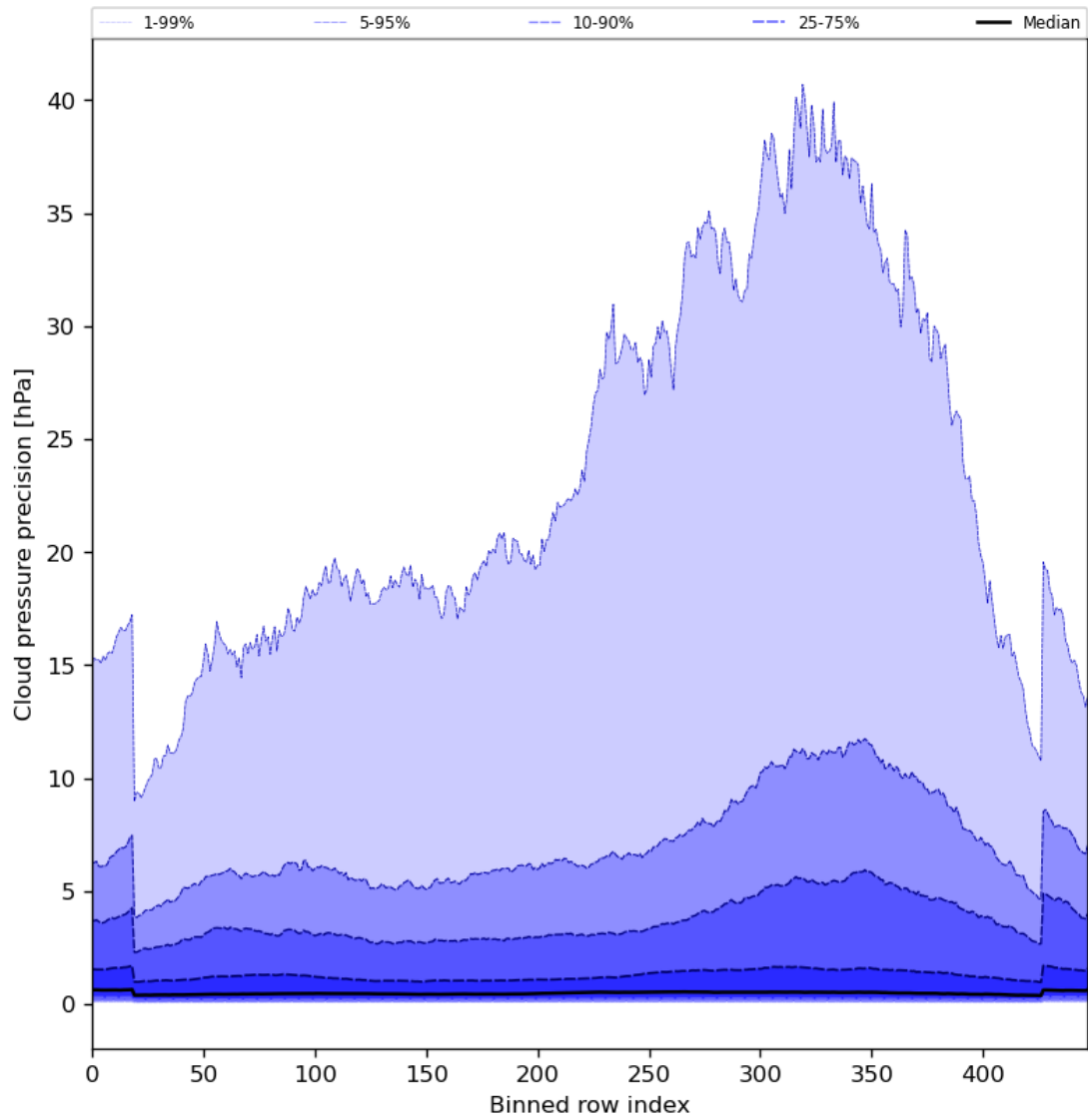
Figure 48: Along track statistics of “Cloud pressure precision” for 2024-06-27 to 2024-06-29
