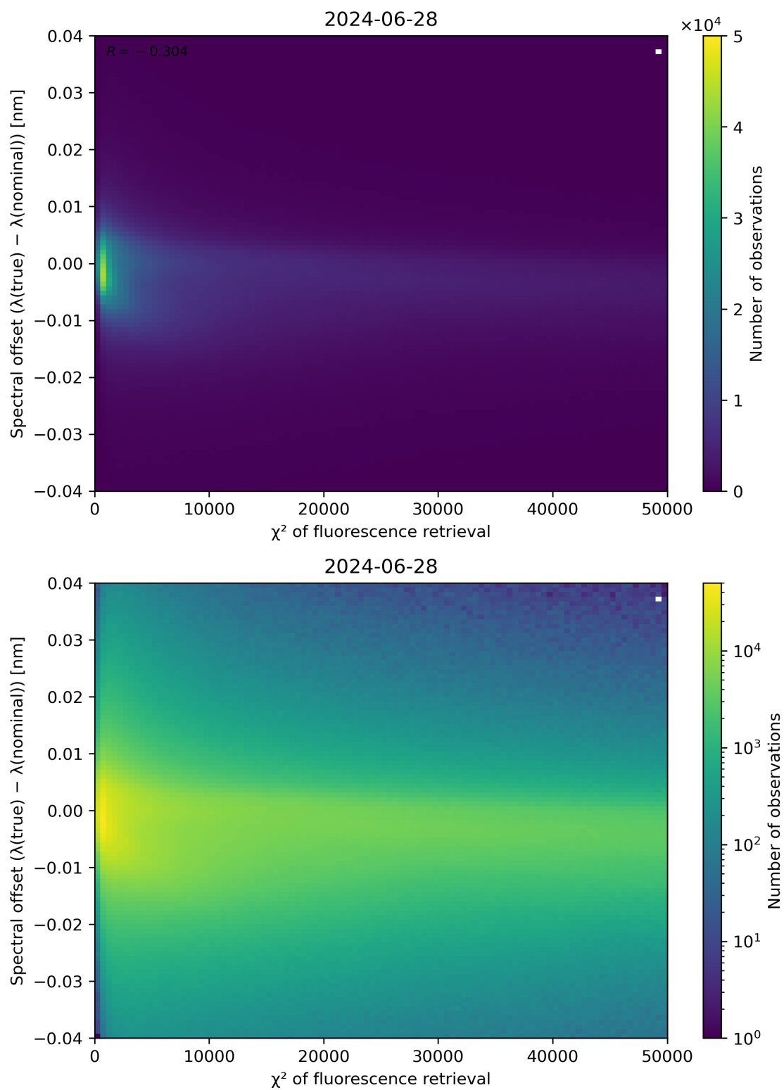
Figure 69: Scatter density plot of “ \chi^2 of fluorescence retrieval” against “Spectral offset ( \lambda(\text{true}) - \lambda(\text{nominal}) )” for 2024-06-27 to 2024-06-29.
