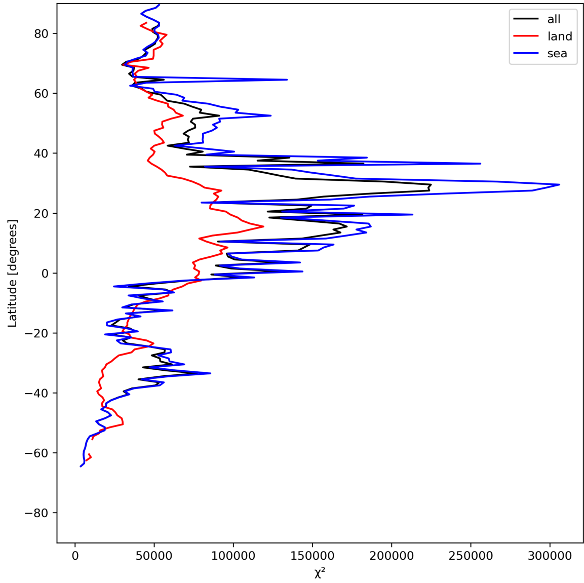
Figure 21: Zonal average of “ \chi^2 ” for 2024-06-27 to 2024-06-29.
