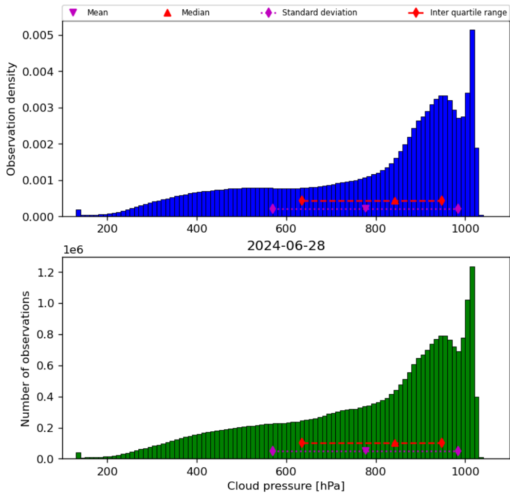
Figure 30: Histogram of “Cloud pressure” for 2024-06-27 to 2024-06-29
