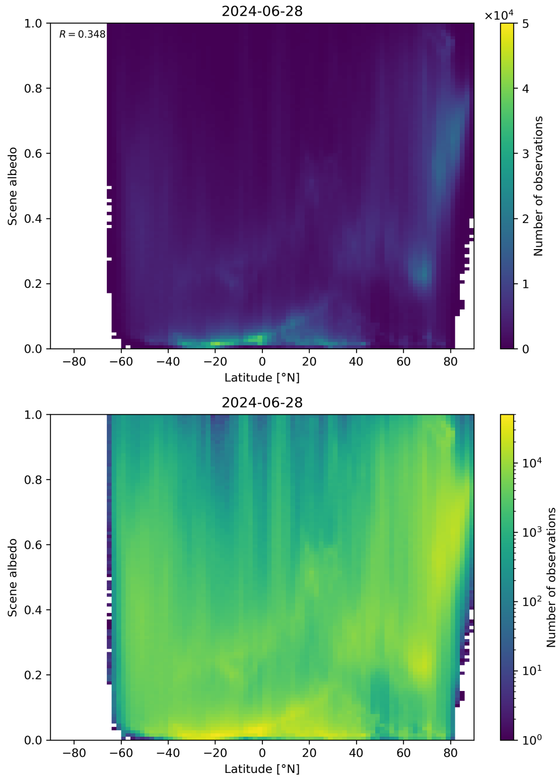
Figure 95: Scatter density plot of “Latitude” against “Scene albedo” for 2024-06-27 to 2024-06-29.
