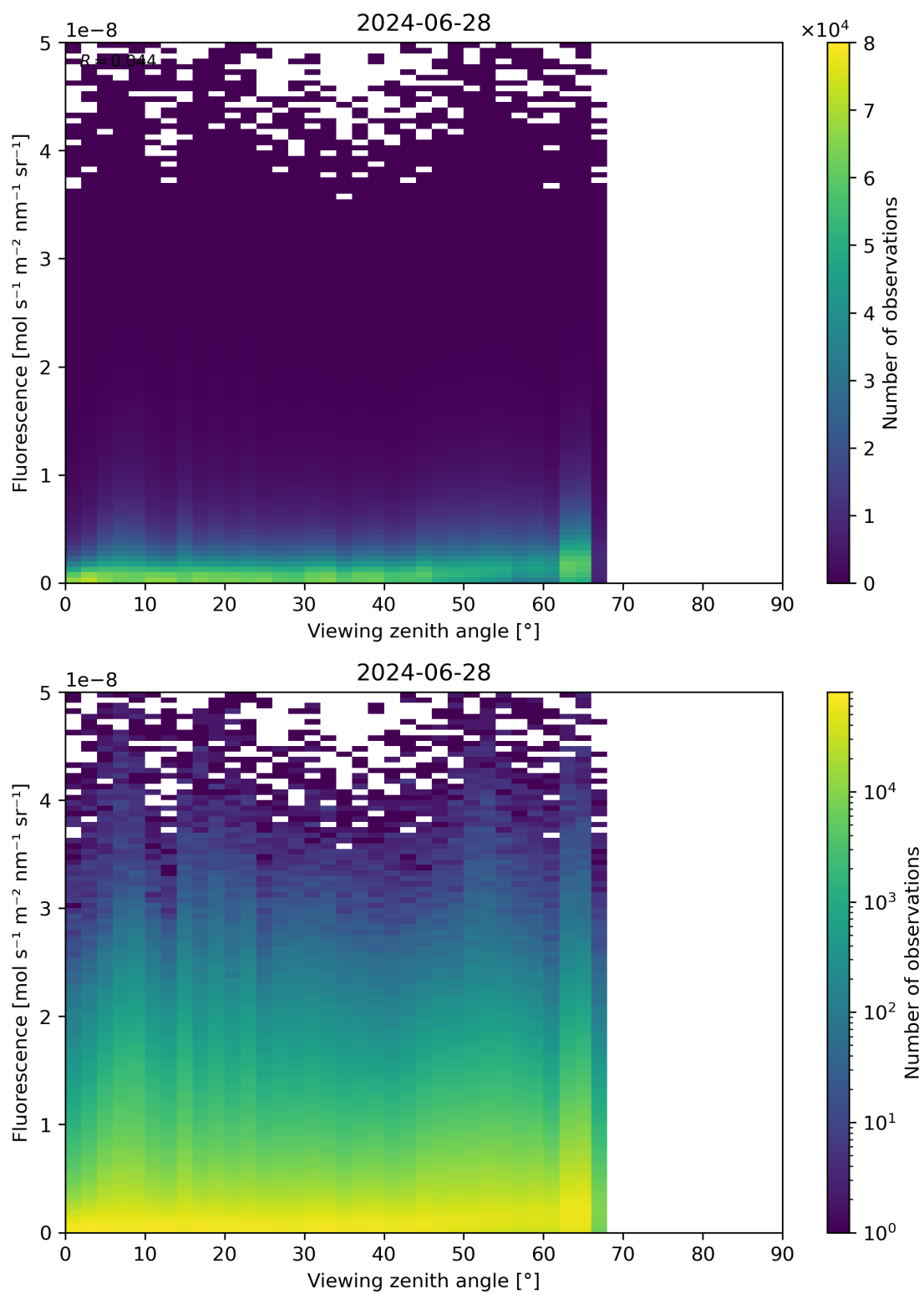
Figure 122: Scatter density plot of “Viewing zenith angle” against “Fluorescence” for 2024-06-27 to 2024-06-29.
