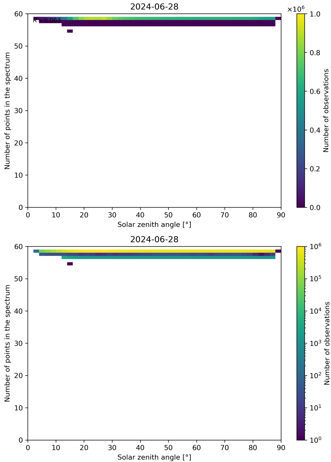
Figure 115: Scatter density plot of “Solar zenith angle” against “Number of points in the spectrum” for 2024-06-27 to 2024-06-29.
