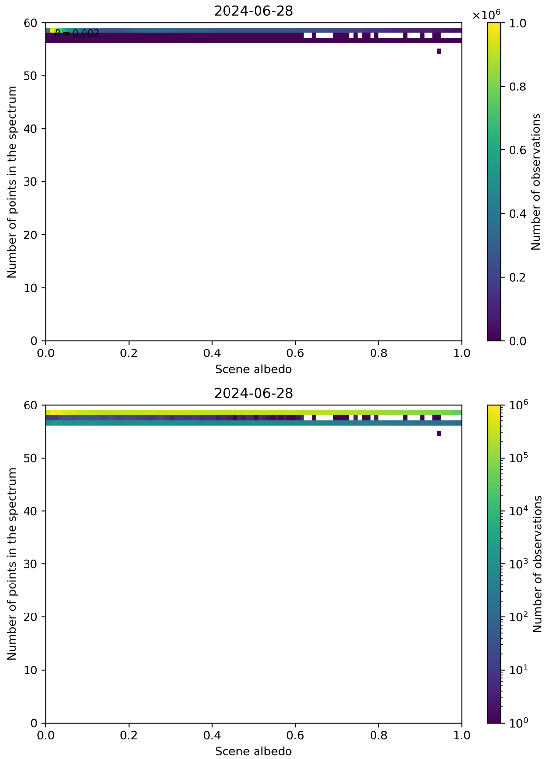
Figure 106: Scatter density plot of “Scene albedo” against “Number of points in the spectrum” for 2024-06-27 to 2024-06-29.
