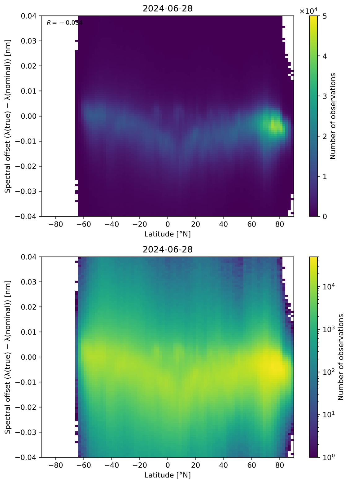
Figure 96: Scatter density plot of “Latitude” against “Spectral offset ( \lambda(\text{true}) - \lambda(\text{nominal}) )” for 2024-06-27 to 2024-06-29.
