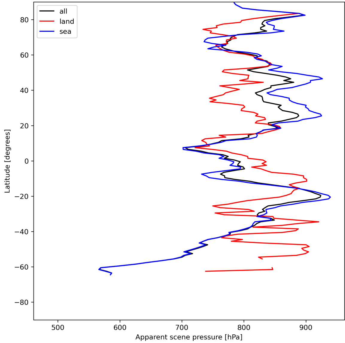
Figure 19: Zonal average of “Apparent scene pressure” for 2024-06-27 to 2024-06-29.
