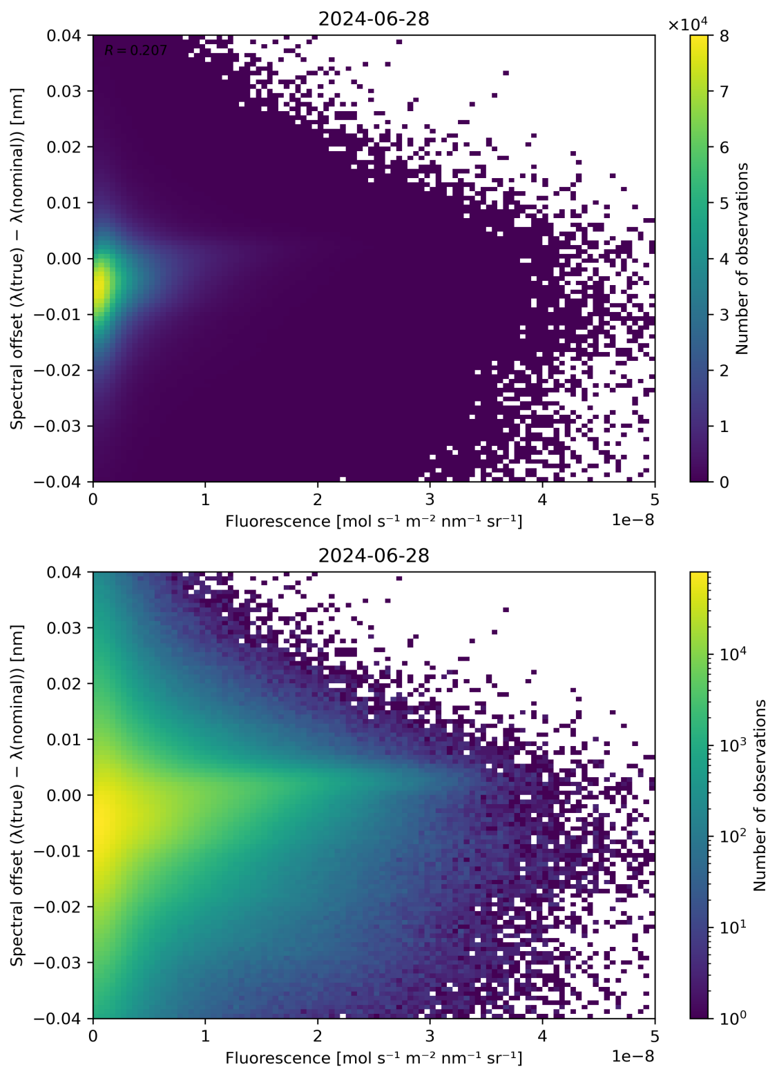
Figure 87: Scatter density plot of “Fluorescence” against “Spectral offset ( \lambda(\text{true}) - \lambda(\text{nominal}) )” for 2024-06-27 to 2024-06-29.
