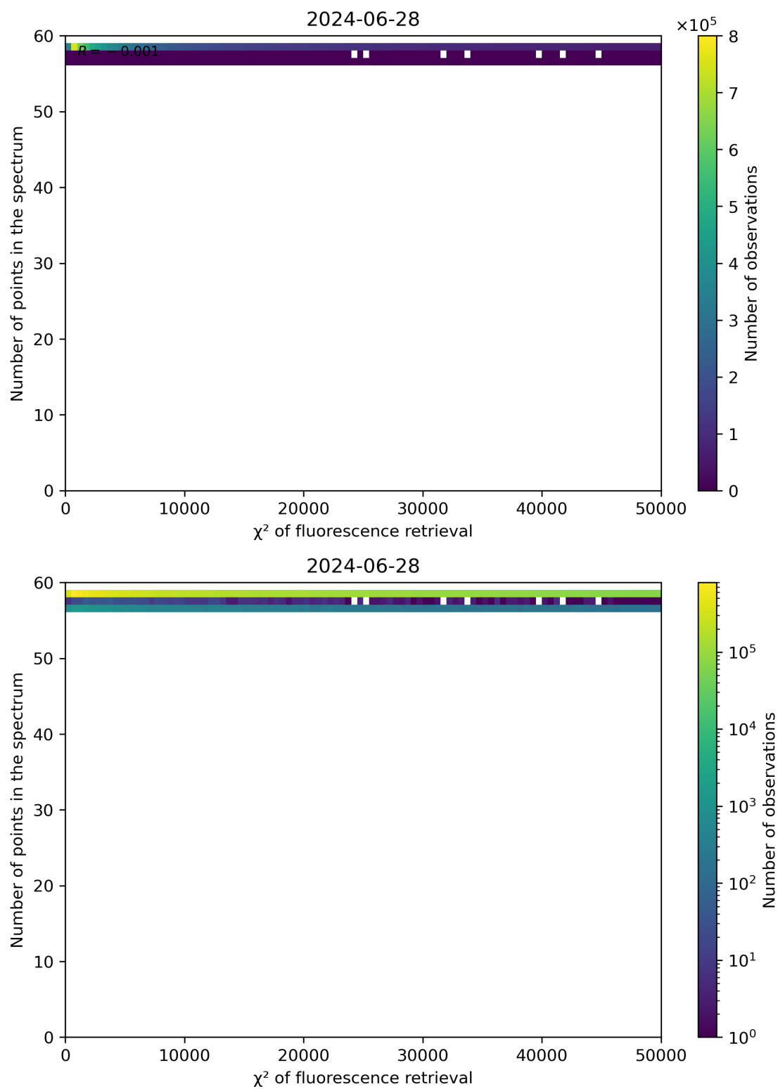
Figure 68: Scatter density plot of " \chi^2 of fluorescence retrieval" against "Number of points in the spectrum" for 2024-06-27 to 2024-06-29.
