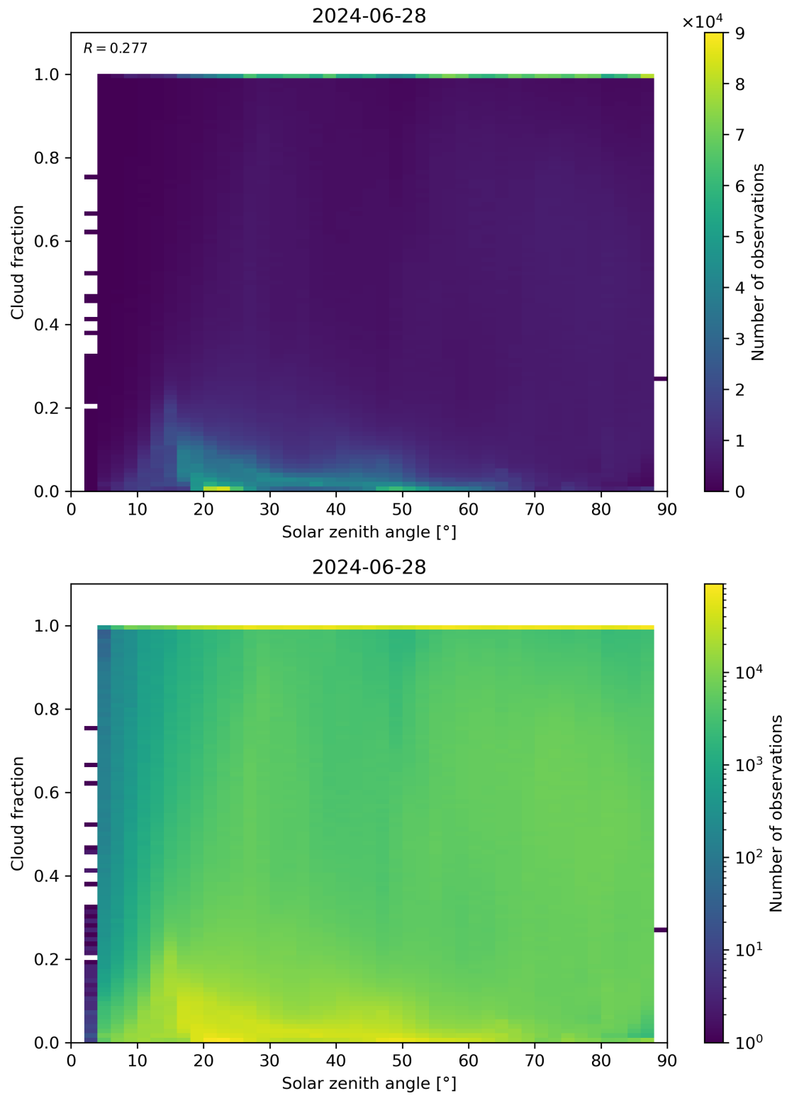
Figure 110: Scatter density plot of “Solar zenith angle” against “Cloud fraction” for 2024-06-27 to 2024-06-29.
