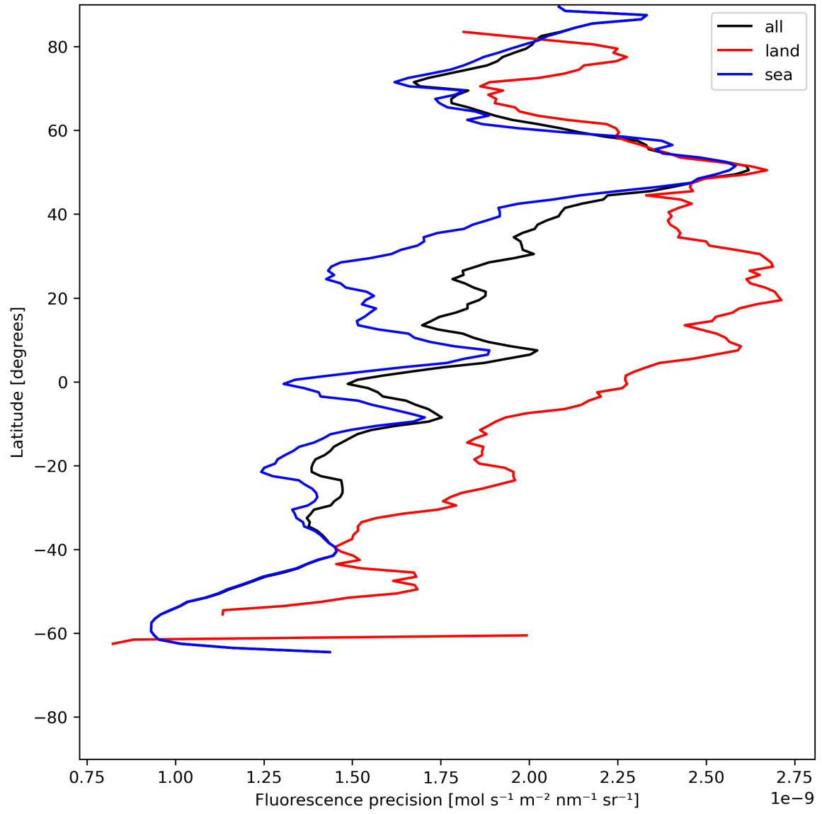
Figure 24: Zonal average of “Fluorescence precision” for 2024-06-27 to 2024-06-29.
