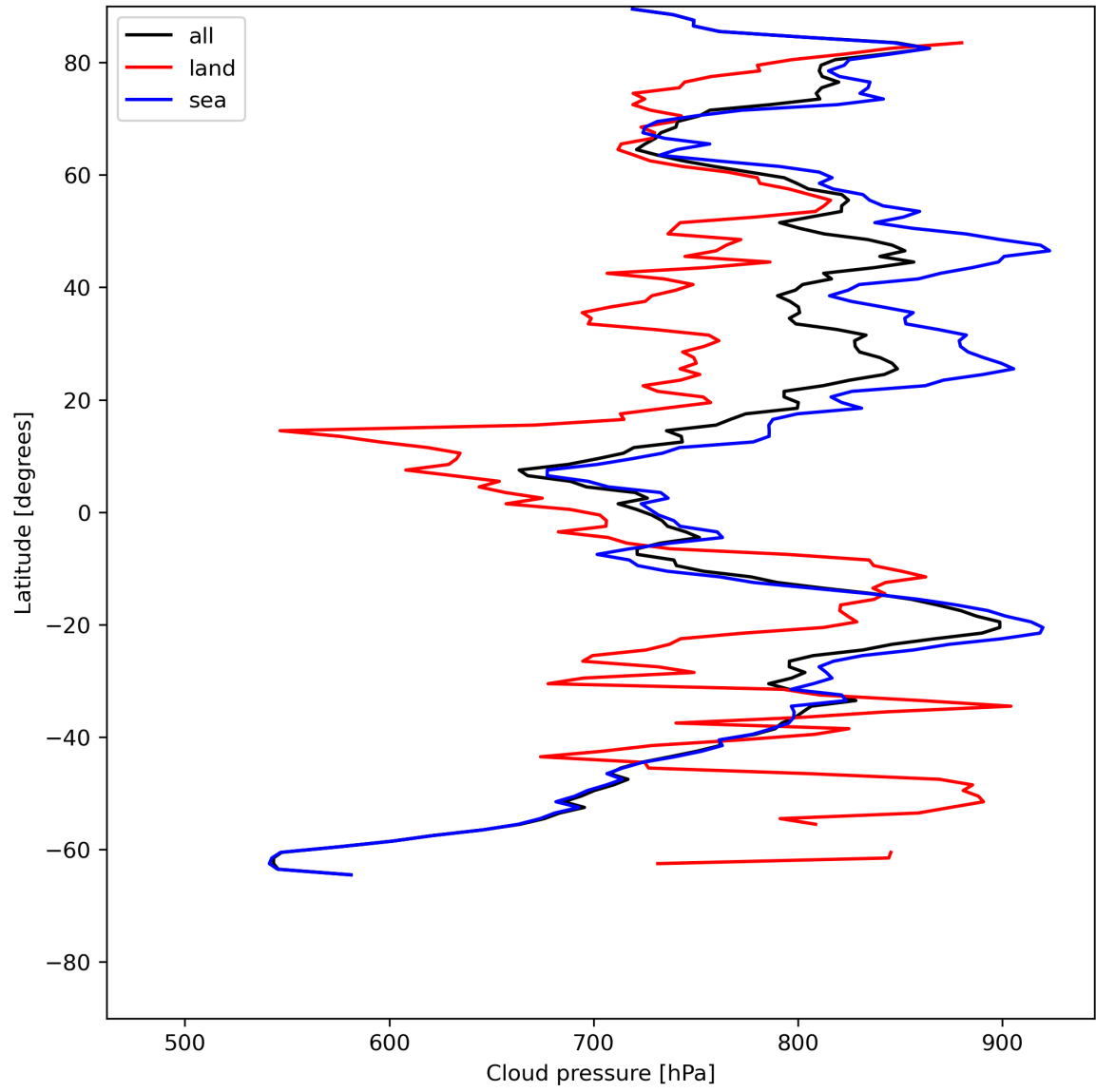
Figure 13: Zonal average of “Cloud pressure” for 2024-06-27 to 2024-06-29.
