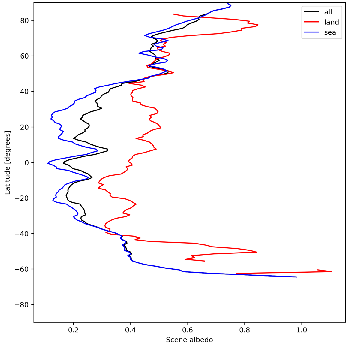
Figure 17: Zonal average of “Scene albedo” for 2024-06-27 to 2024-06-29.
