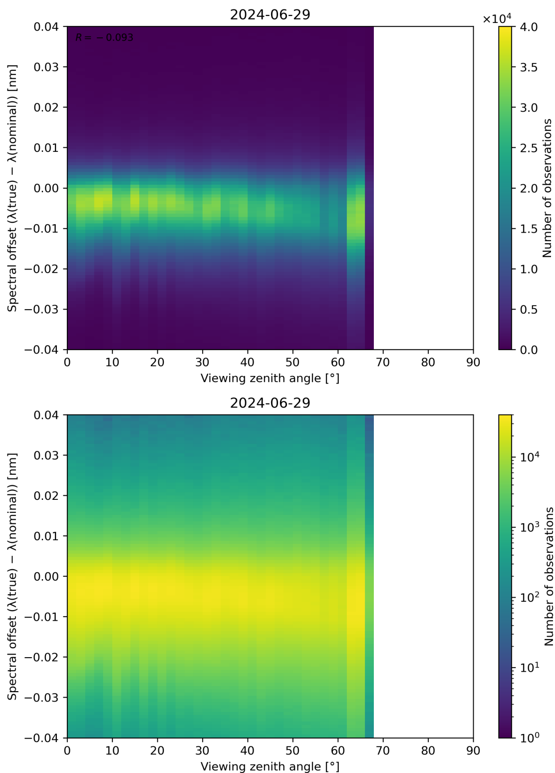
Figure 128: Scatter density plot of “Viewing zenith angle” against “Spectral offset ( \lambda(\text{true}) - \lambda(\text{nominal}) )” for 2024-06-29 to 2024-06-30.
