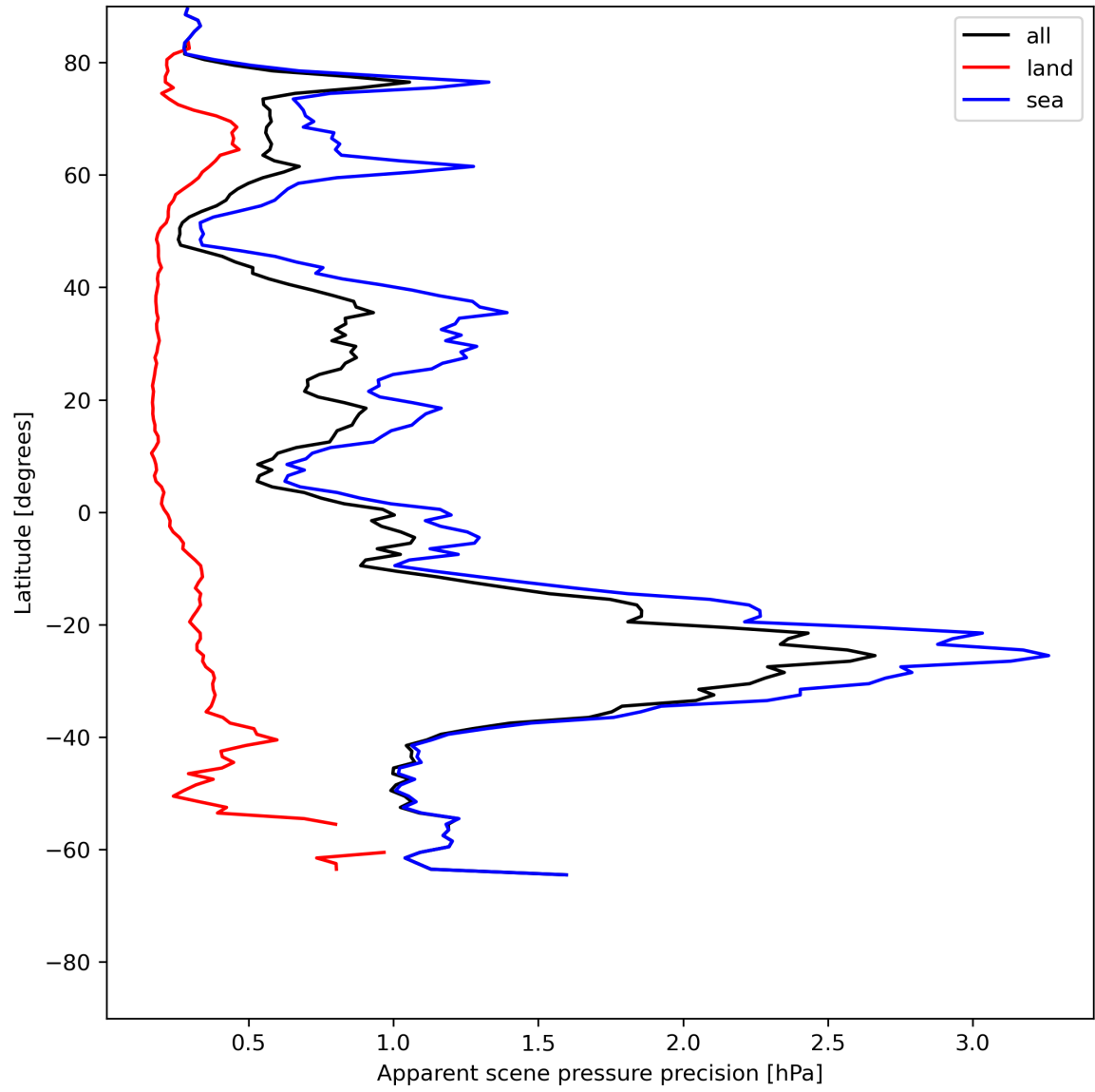
Figure 20: Zonal average of “Apparent scene pressure precision” for 2024-06-29 to 2024-06-30.
