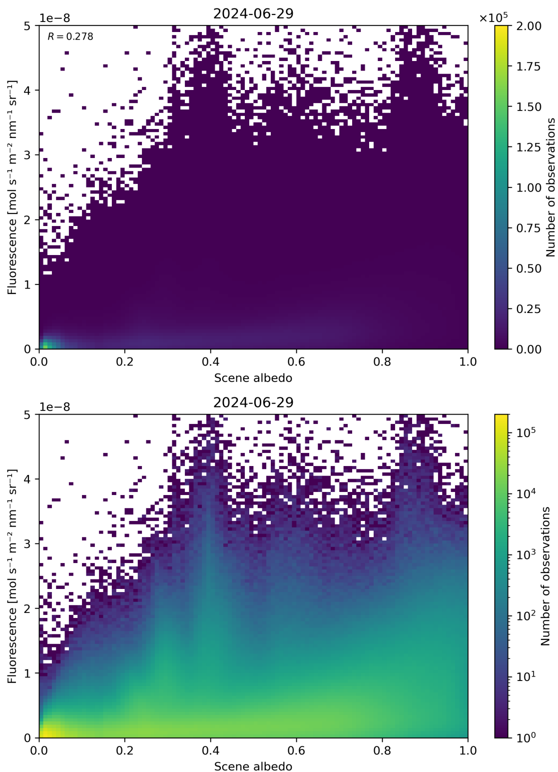
Figure 104: Scatter density plot of “Scene albedo” against “Fluorescence” for 2024-06-29 to 2024-06-30.
