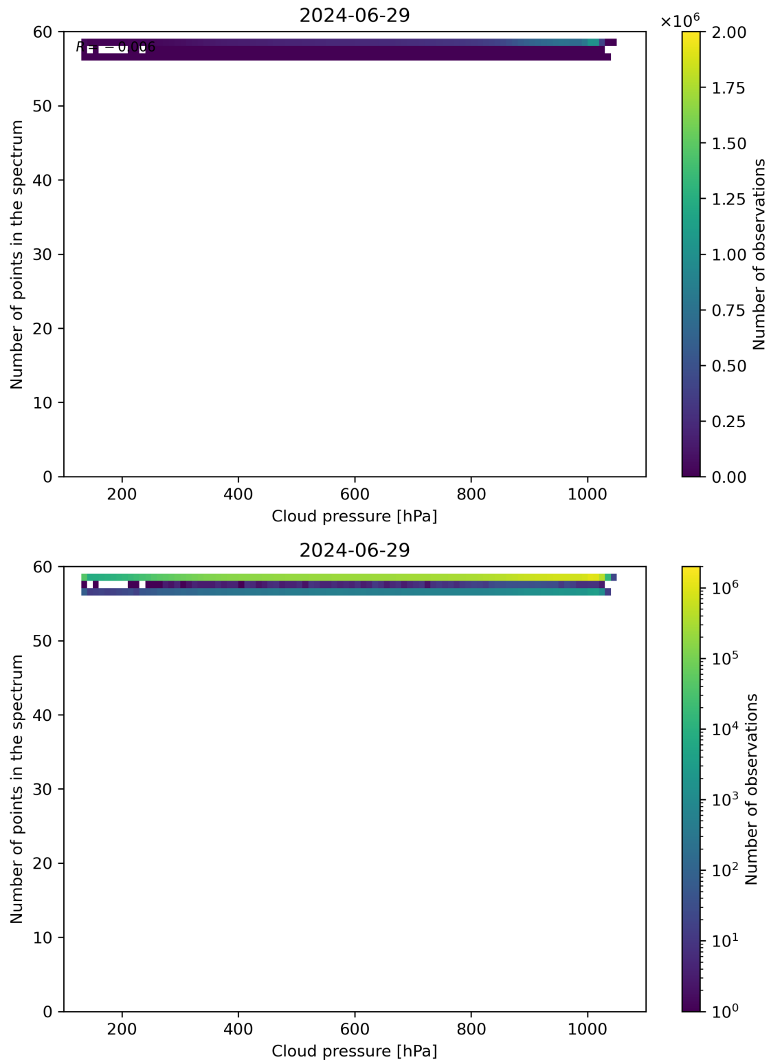
Figure 82: Scatter density plot of “Cloud pressure” against “Number of points in the spectrum” for 2024-06-29 to 2024-06-30.
