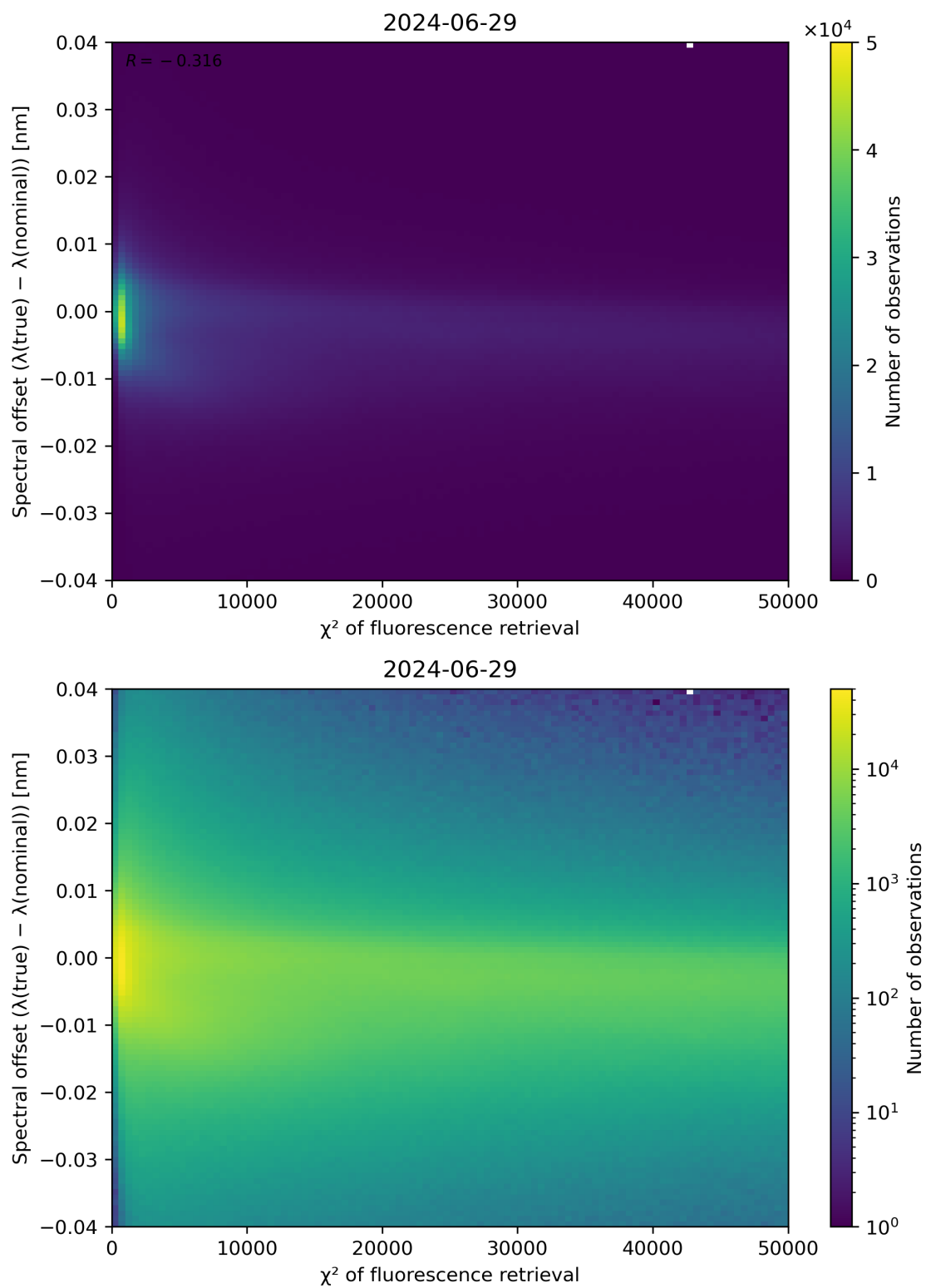
Figure 69: Scatter density plot of “ \chi^2 of fluorescence retrieval” against “Spectral offset ( \lambda(\text{true}) - \lambda(\text{nominal}) )” for 2024-06-29 to 2024-06-30.
