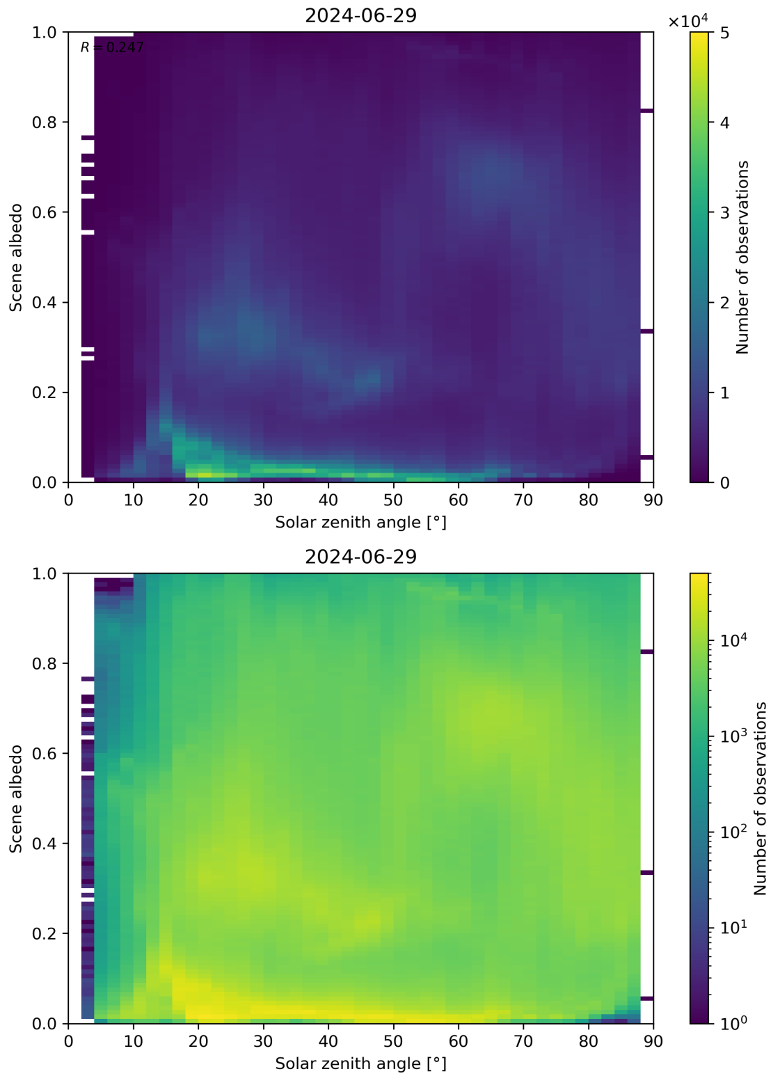
Figure 116: Scatter density plot of “Solar zenith angle” against “Scene albedo” for 2024-06-29 to 2024-06-30.
