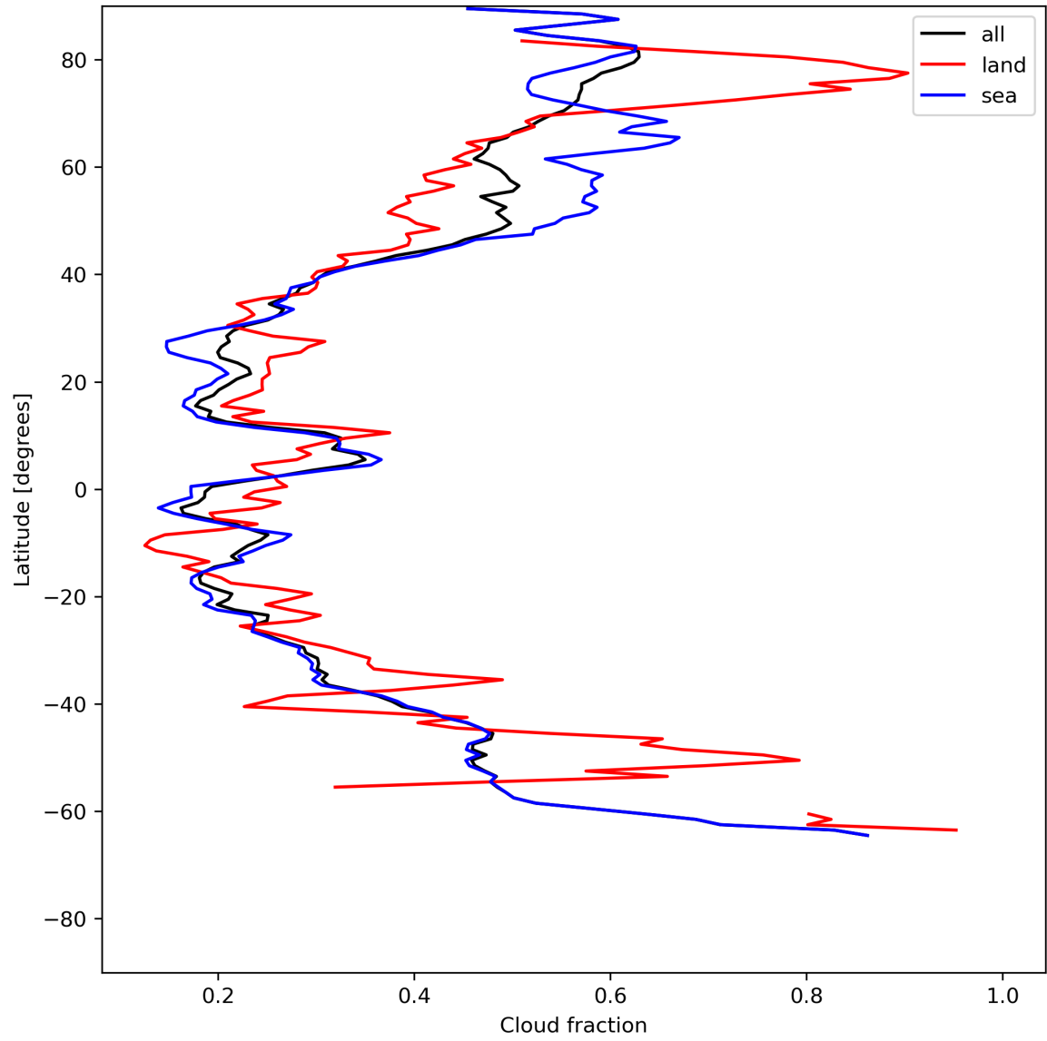
Figure 15: Zonal average of “Cloud fraction” for 2024-06-29 to 2024-06-30.
