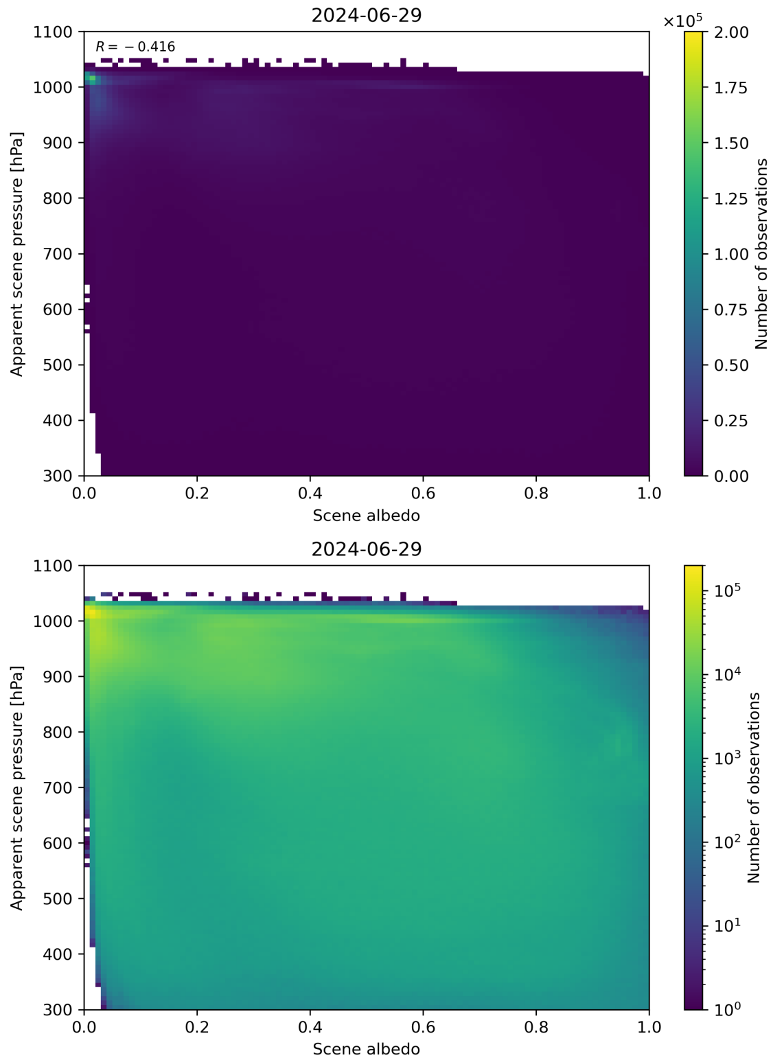
Figure 102: Scatter density plot of “Scene albedo” against “Apparent scene pressure” for 2024-06-29 to 2024-06-30.
