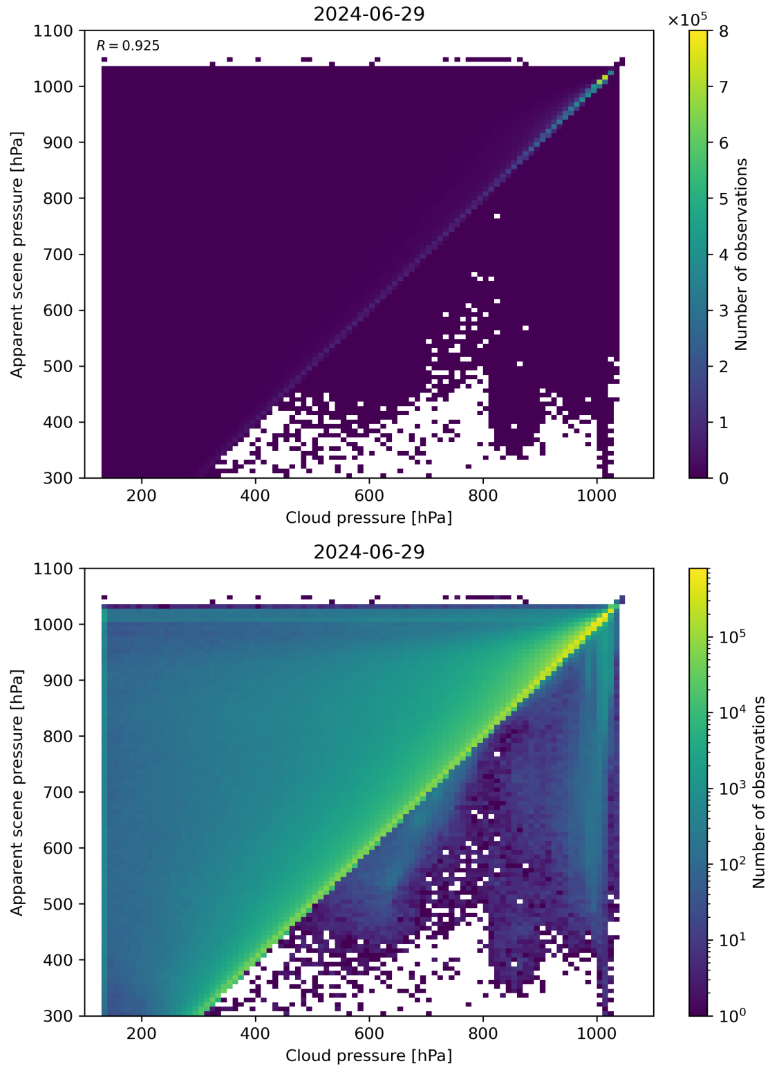
Figure 77: Scatter density plot of “Cloud pressure” against “Apparent scene pressure” for 2024-06-29 to 2024-06-30.
