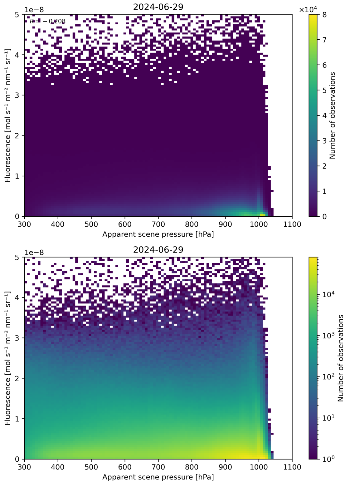
Figure 64: Scatter density plot of “Apparent scene pressure” against “Fluorescence” for 2024-06-29 to 2024-06-30.
