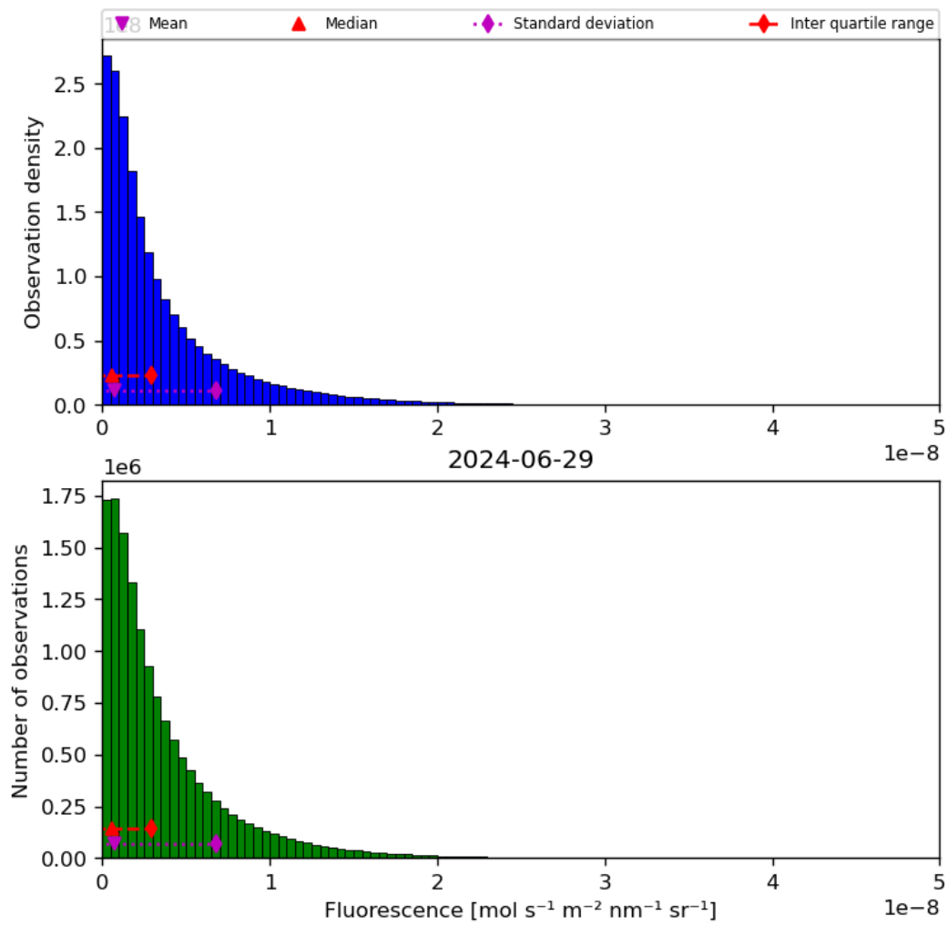
Figure 40: Histogram of “Fluorescence” for 2024-06-29 to 2024-06-30
