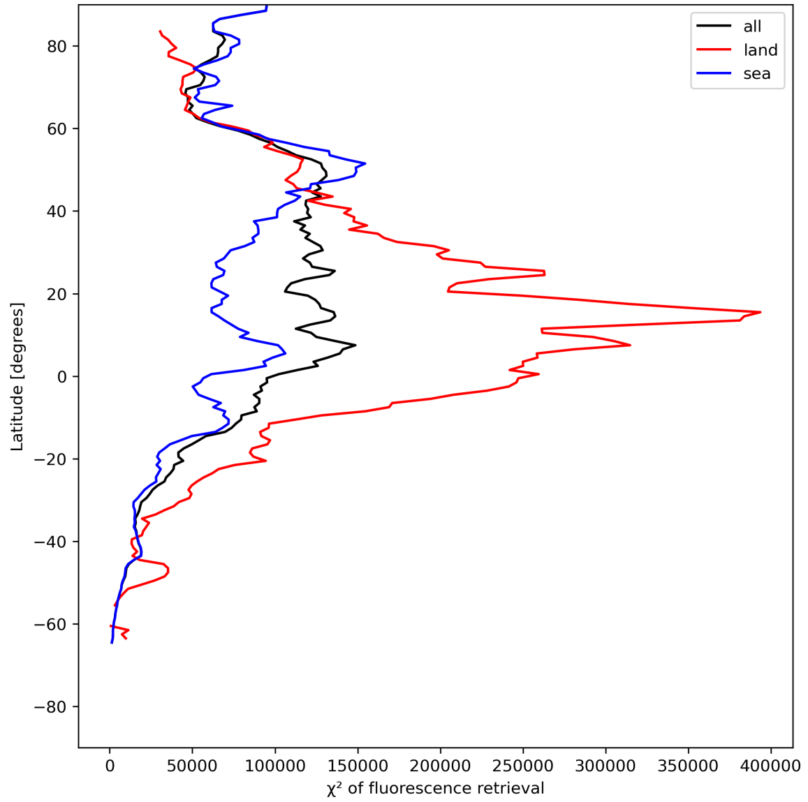
Figure 25: Zonal average of “ \chi^2 of fluorescence retrieval” for 2024-06-29 to 2024-06-30.
