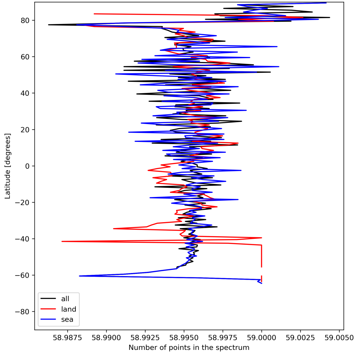
Figure 27: Zonal average of “Number of points in the spectrum” for 2024-06-29 to 2024-06-30.
