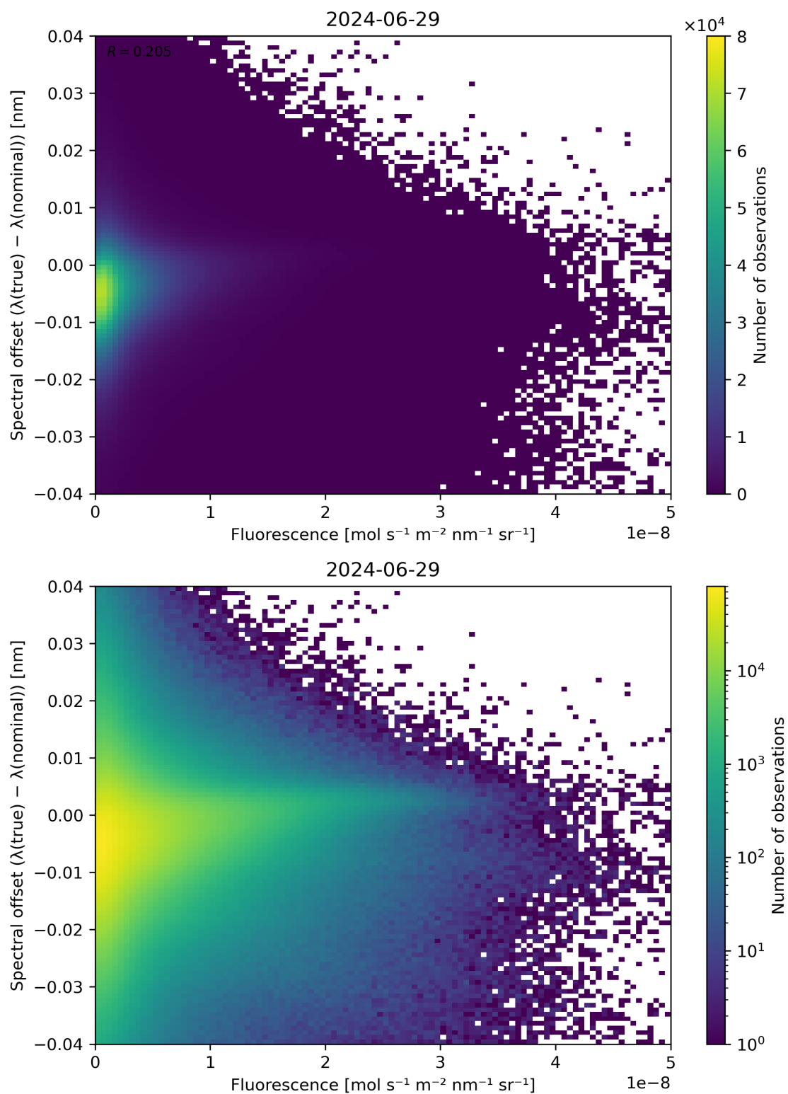
Figure 87: Scatter density plot of “Fluorescence” against “Spectral offset ( \lambda(\text{true}) - \lambda(\text{nominal}) )” for 2024-06-29 to 2024-06-30.
