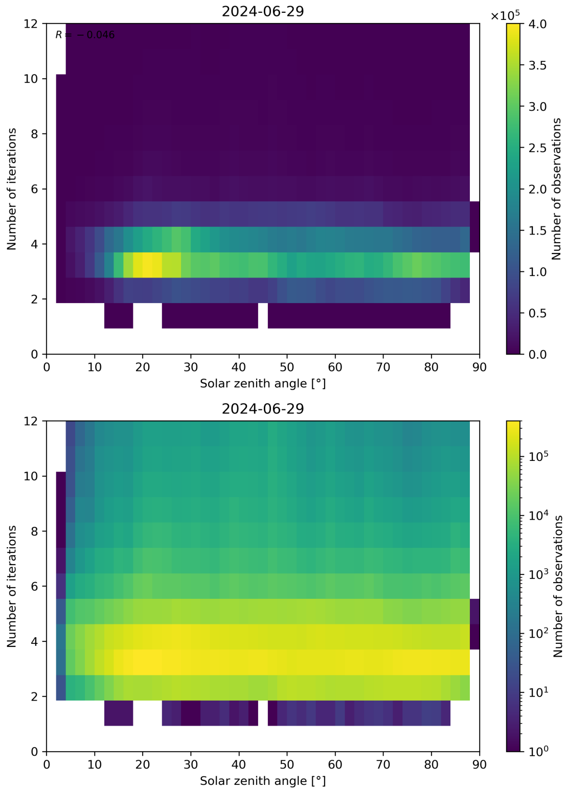
Figure 114: Scatter density plot of “Solar zenith angle” against “Number of iterations” for 2024-06-29 to 2024-06-30.
