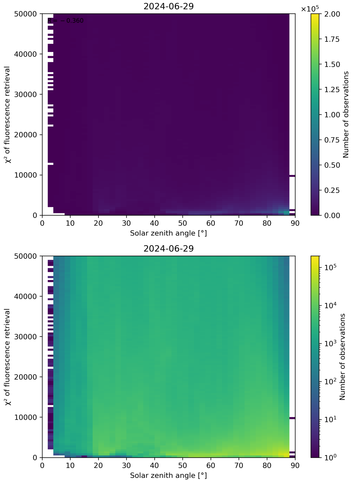
Figure 109: Scatter density plot of “Solar zenith angle” against “ \chi^2 of fluorescence retrieval” for 2024-06-29 to 2024-06-30.
