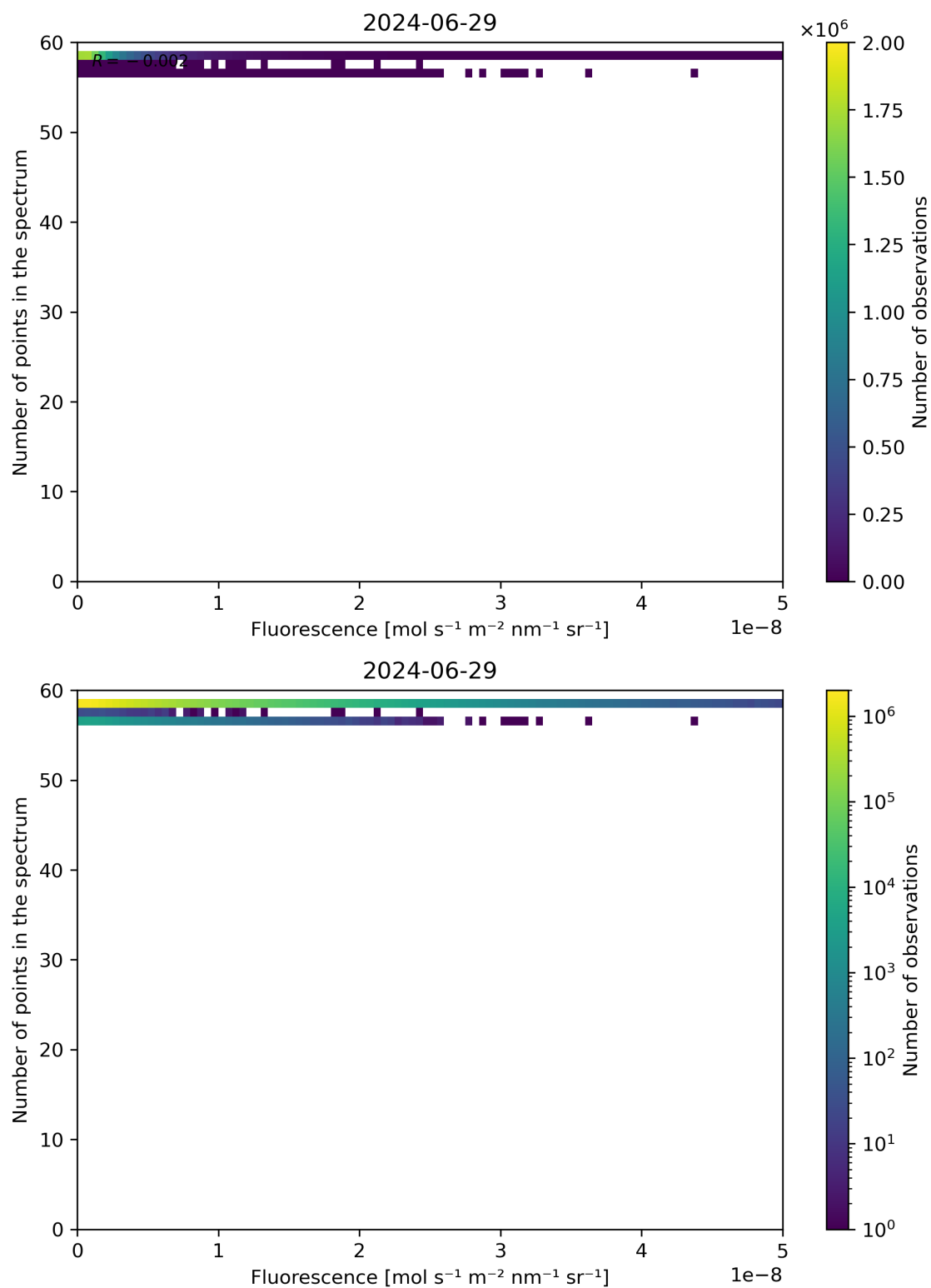
Figure 86: Scatter density plot of “Fluorescence” against “Number of points in the spectrum” for 2024-06-29 to 2024-06-30.
