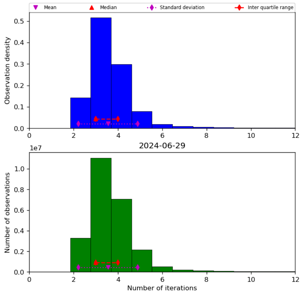
Figure 39: Histogram of “Number of iterations” for 2024-06-29 to 2024-06-30
