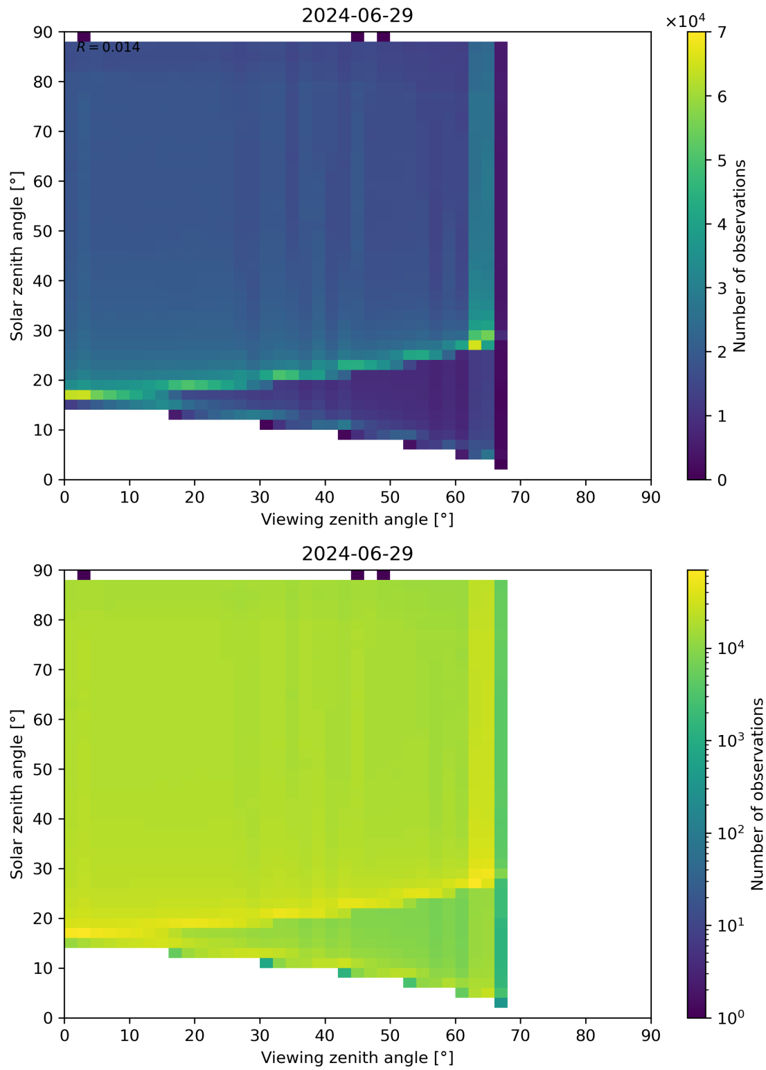
Figure 127: Scatter density plot of “Viewing zenith angle” against “Solar zenith angle” for 2024-06-29 to 2024-06-30.
