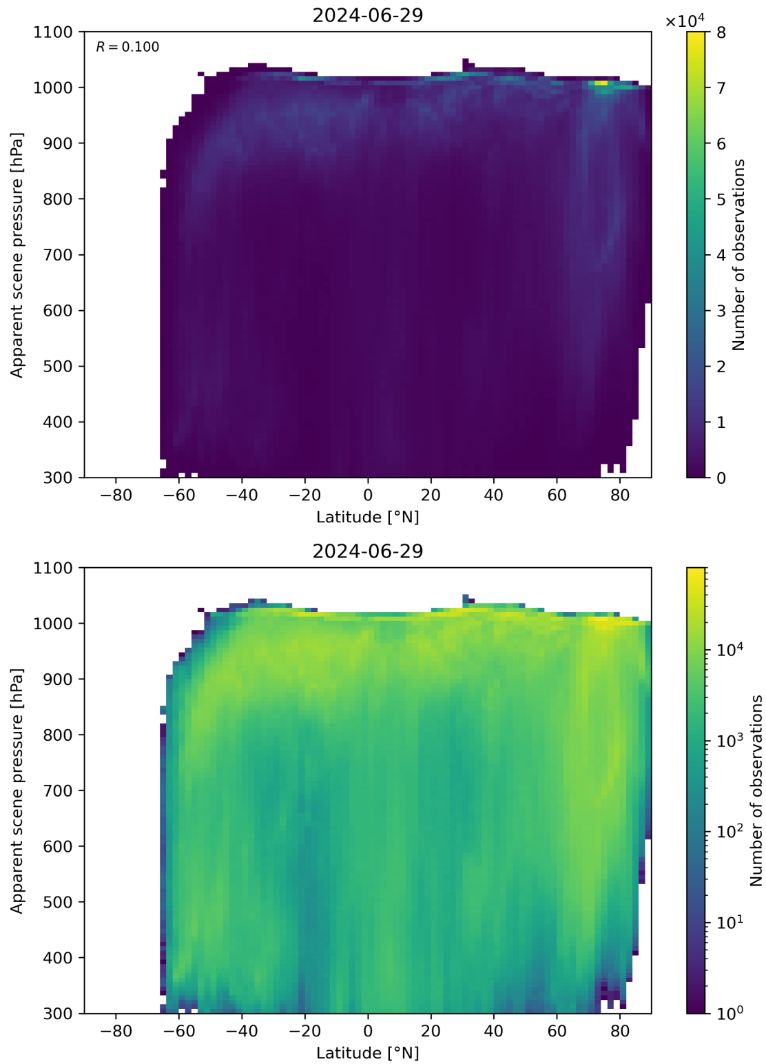
Figure 88: Scatter density plot of “Latitude” against “Apparent scene pressure” for 2024-06-29 to 2024-06-30.
