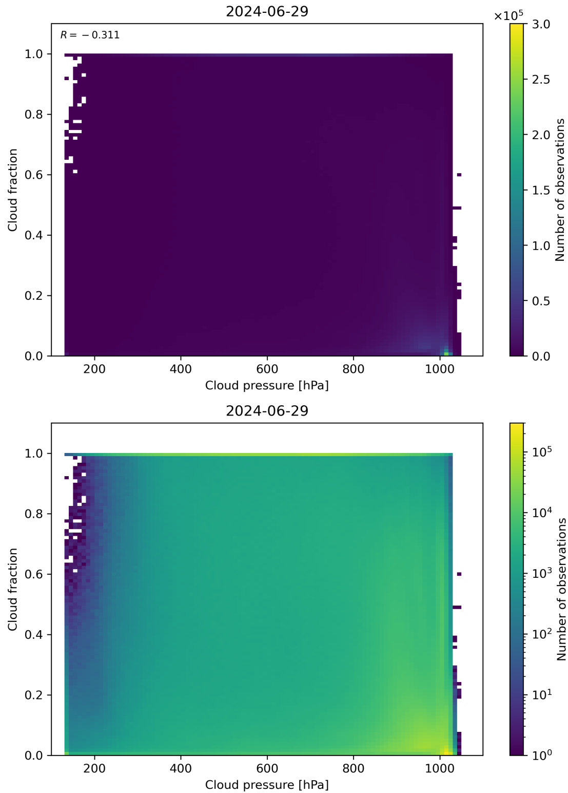
Figure 79: Scatter density plot of “Cloud pressure” against “Cloud fraction” for 2024-06-29 to 2024-06-30.
