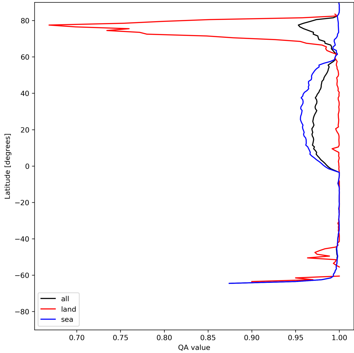
Figure 12: Zonal average of “QA value” for 2024-06-29 to 2024-06-30.
