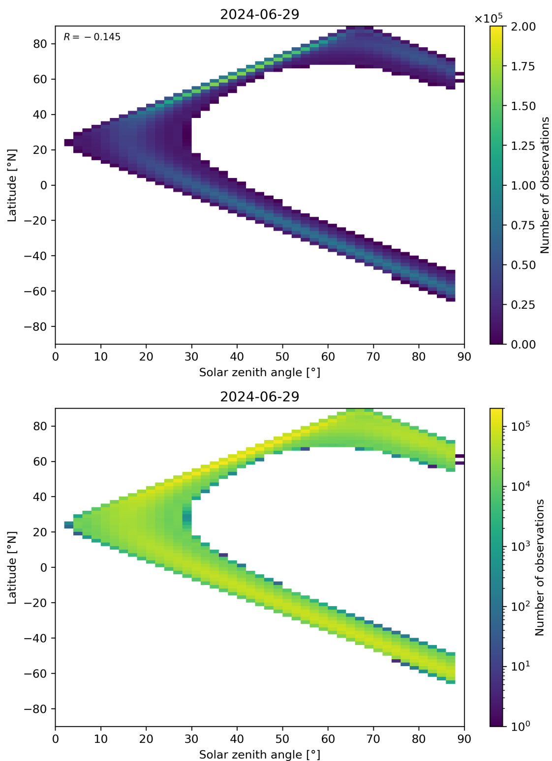
Figure 113: Scatter density plot of “Solar zenith angle” against “Latitude” for 2024-06-29 to 2024-06-30.
