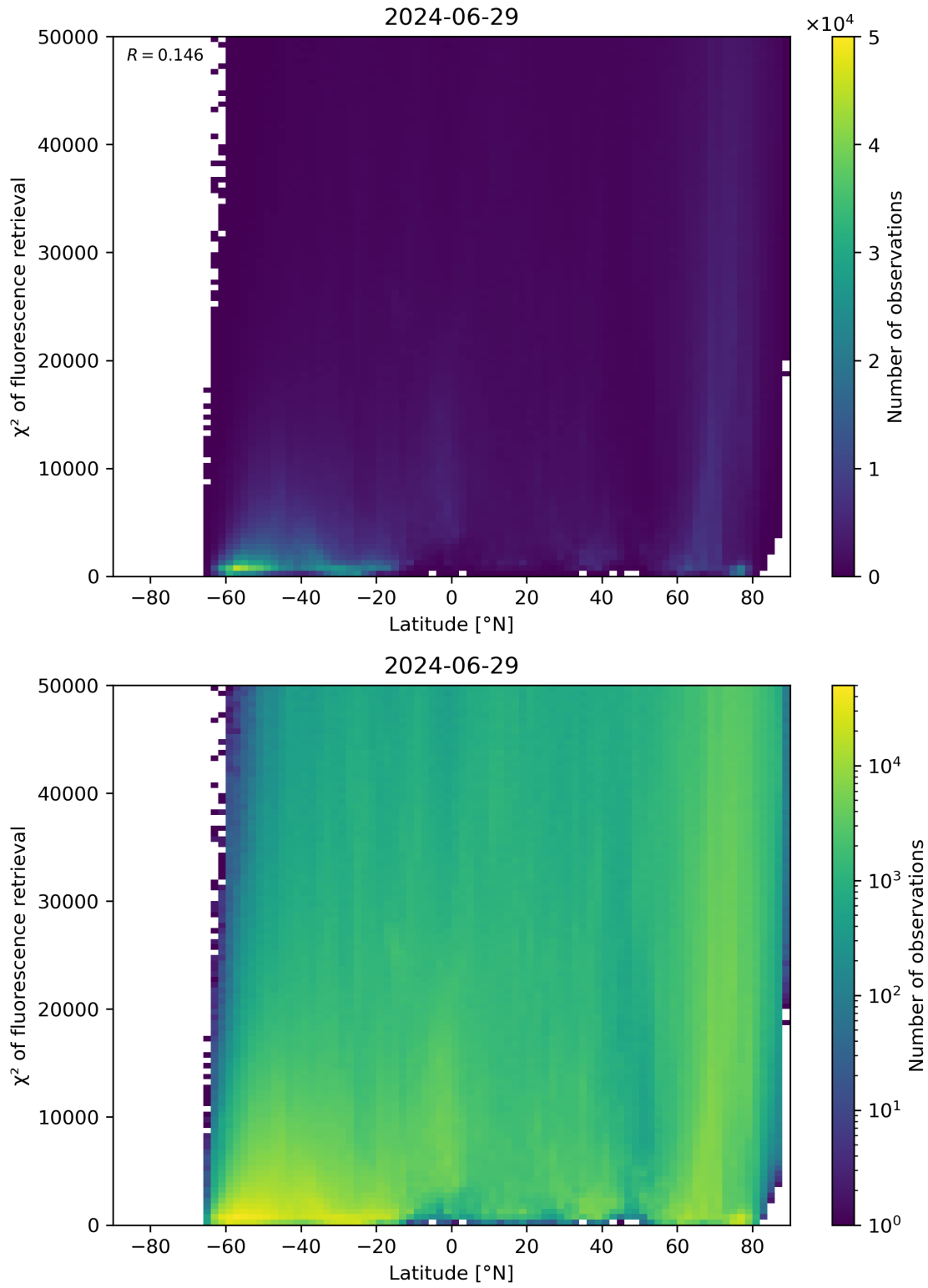
Figure 89: Scatter density plot of “Latitude” against “ \chi^2 of fluorescence retrieval” for 2024-06-29 to 2024-06-30.
