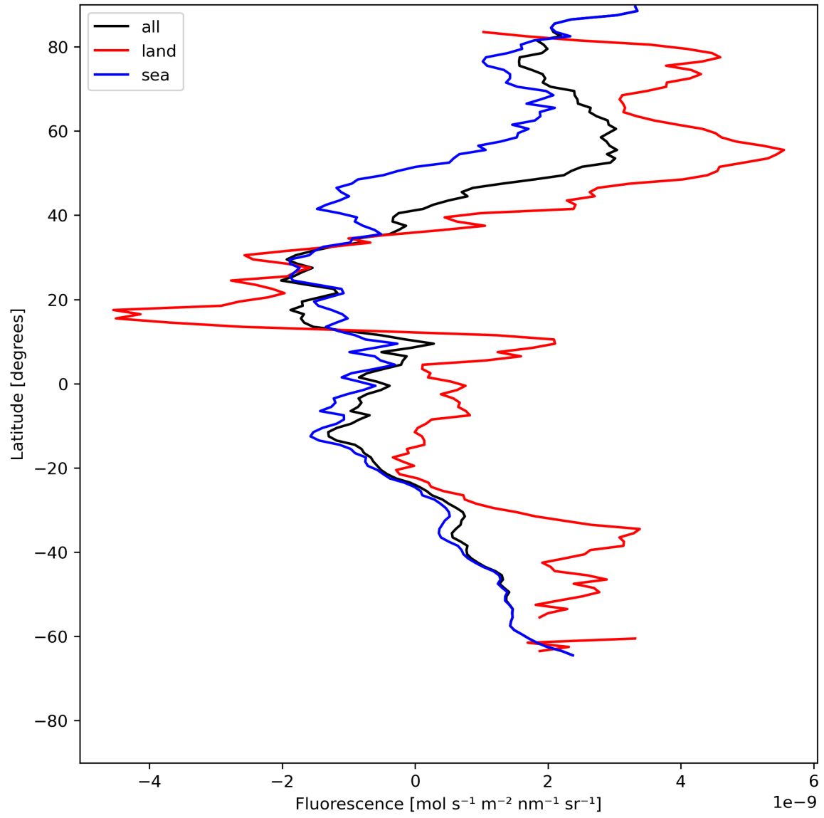
Figure 23: Zonal average of “Fluorescence” for 2024-06-29 to 2024-06-30.
