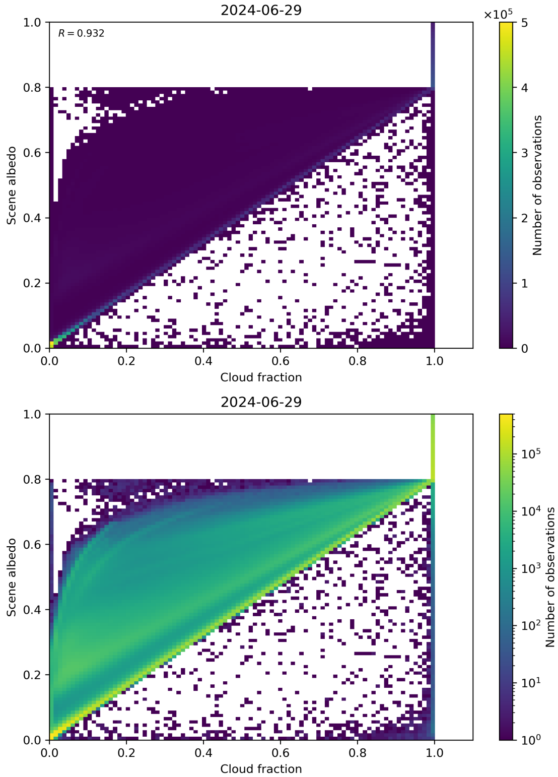
Figure 75: Scatter density plot of “Cloud fraction” against “Scene albedo” for 2024-06-29 to 2024-06-30.
