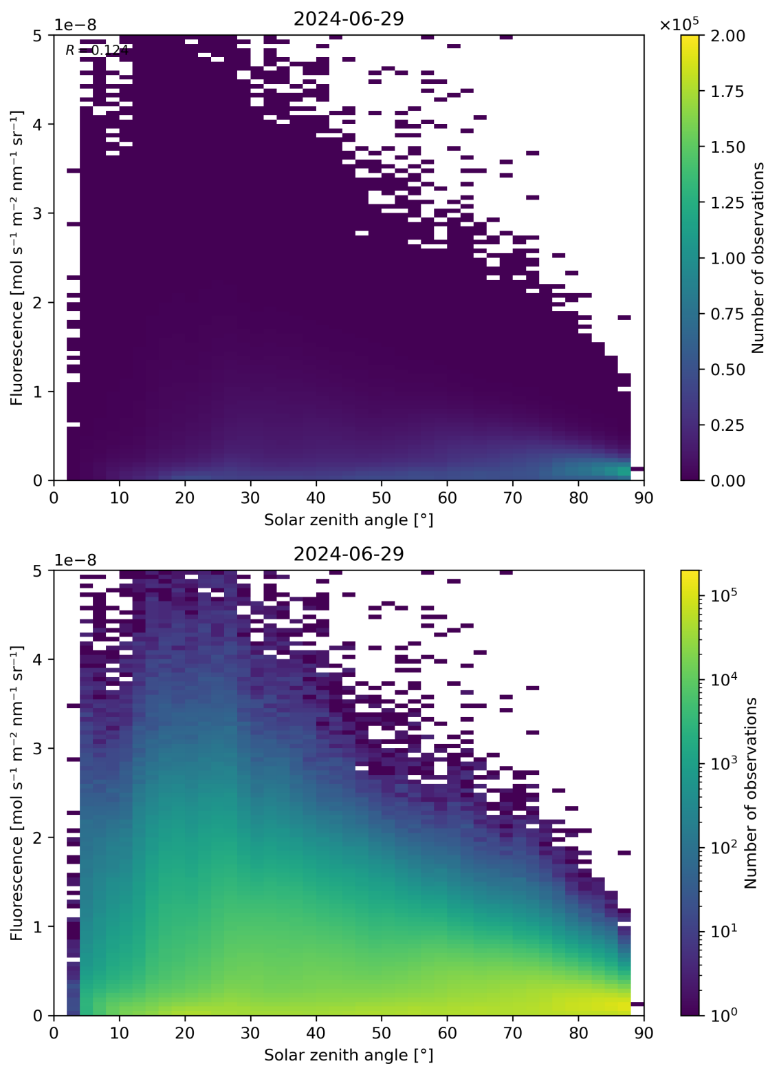
Figure 112: Scatter density plot of “Solar zenith angle” against “Fluorescence” for 2024-06-29 to 2024-06-30.
