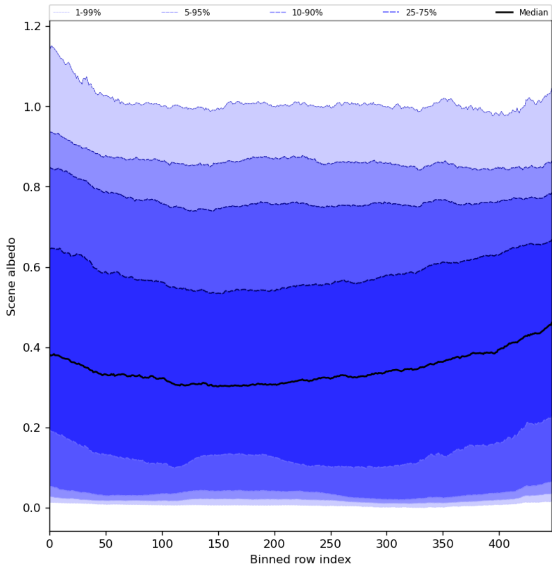
Figure 51: Along track statistics of “Scene albedo” for 2024-06-29 to 2024-06-30
