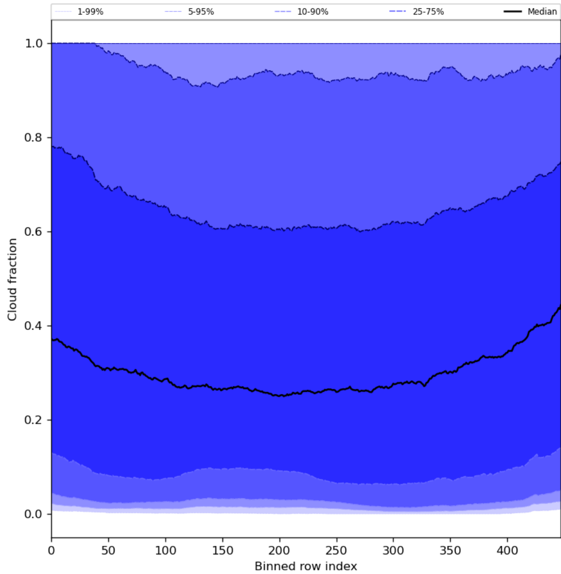
Figure 49: Along track statistics of “Cloud fraction” for 2024-06-29 to 2024-06-30
