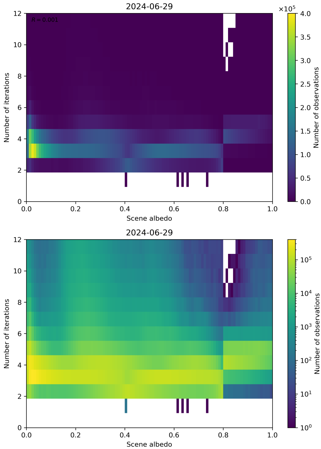
Figure 105: Scatter density plot of “Scene albedo” against “Number of iterations” for 2024-06-29 to 2024-06-30.
