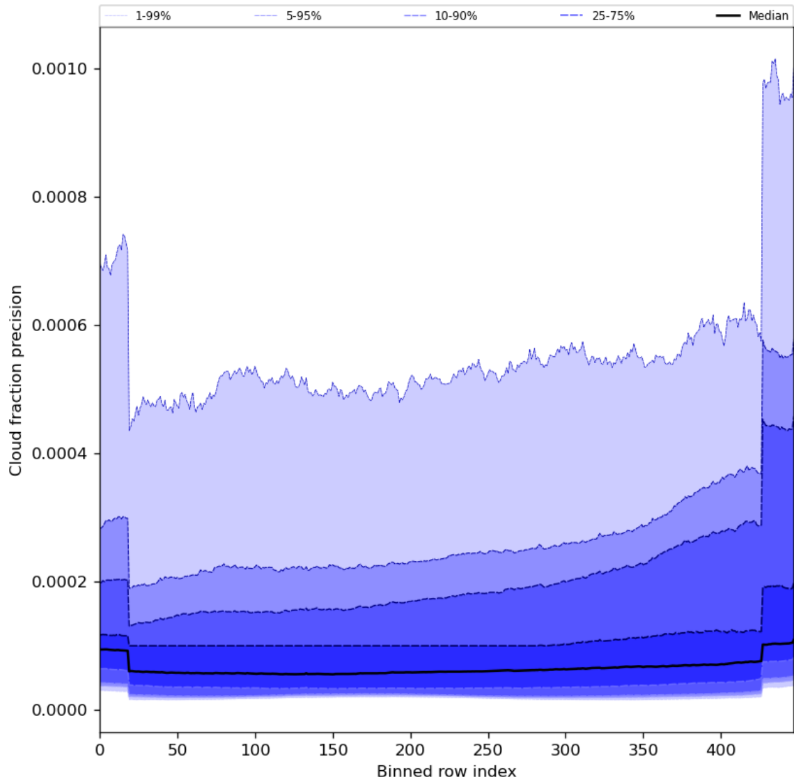
Figure 50: Along track statistics of “Cloud fraction precision” for 2024-06-29 to 2024-06-30
