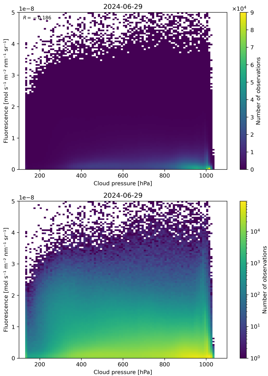
Figure 80: Scatter density plot of “Cloud pressure” against “Fluorescence” for 2024-06-29 to 2024-06-30.
