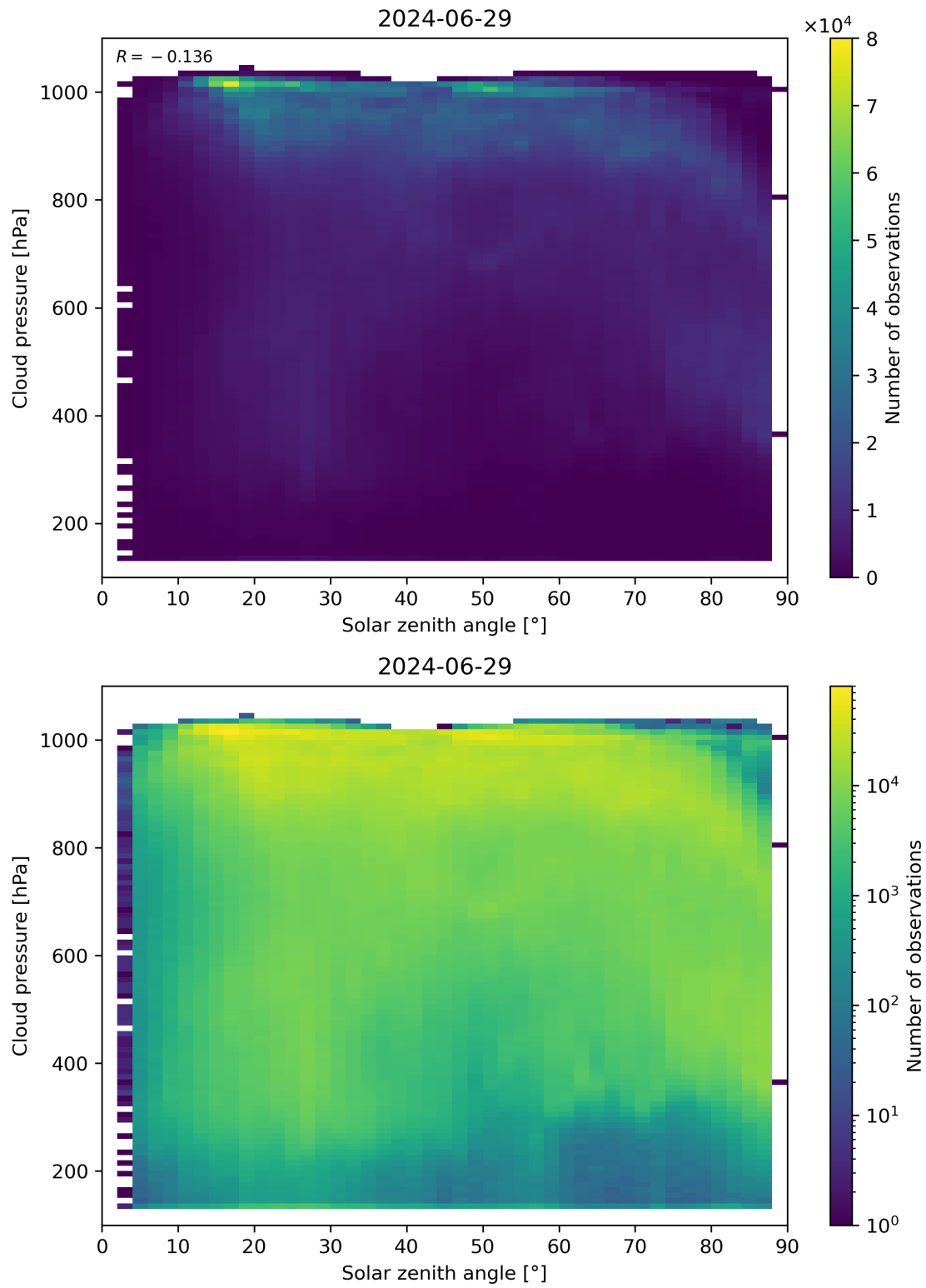
Figure 111: Scatter density plot of “Solar zenith angle” against “Cloud pressure” for 2024-06-29 to 2024-06-30.
