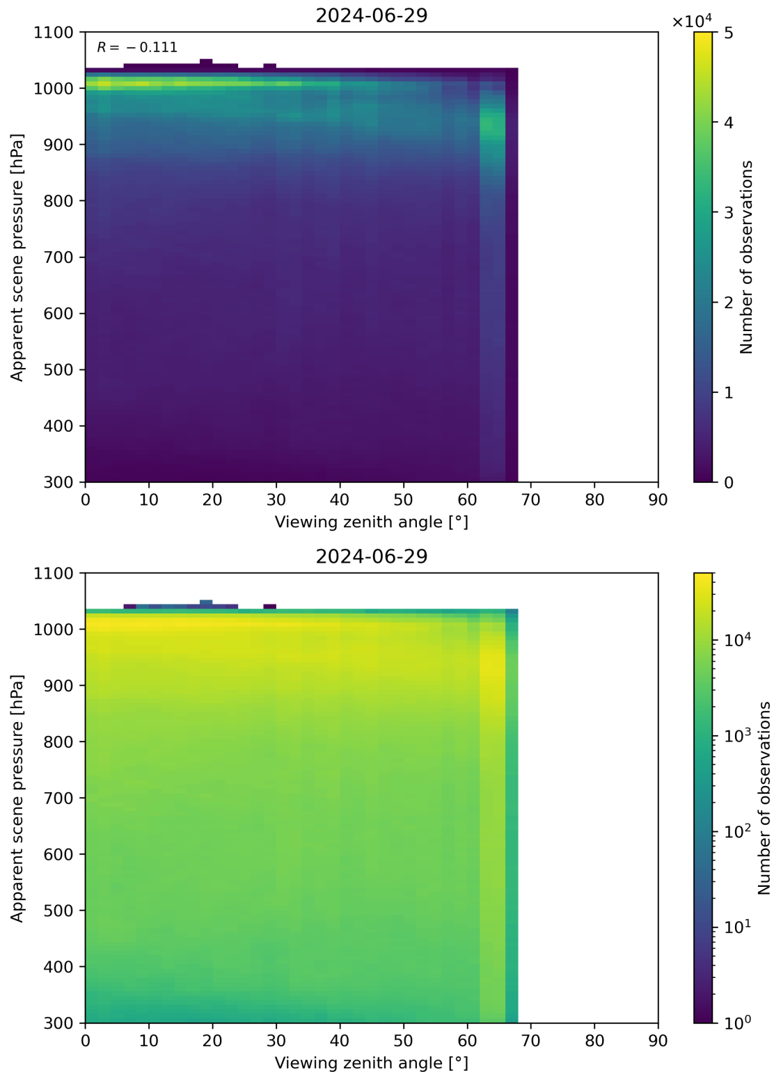
Figure 118: Scatter density plot of “Viewing zenith angle” against “Apparent scene pressure” for 2024-06-29 to 2024-06-30.
