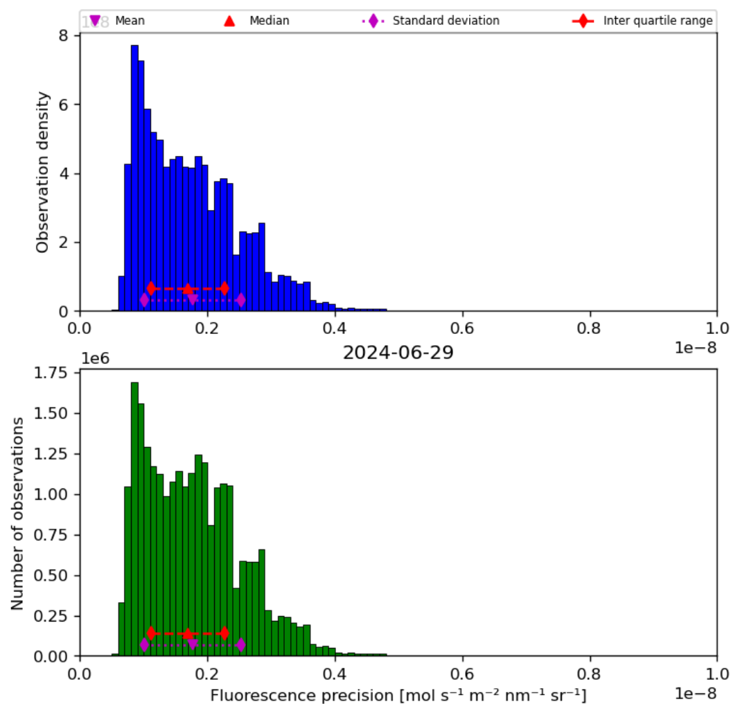
Figure 41: Histogram of “Fluorescence precision” for 2024-06-29 to 2024-06-30
