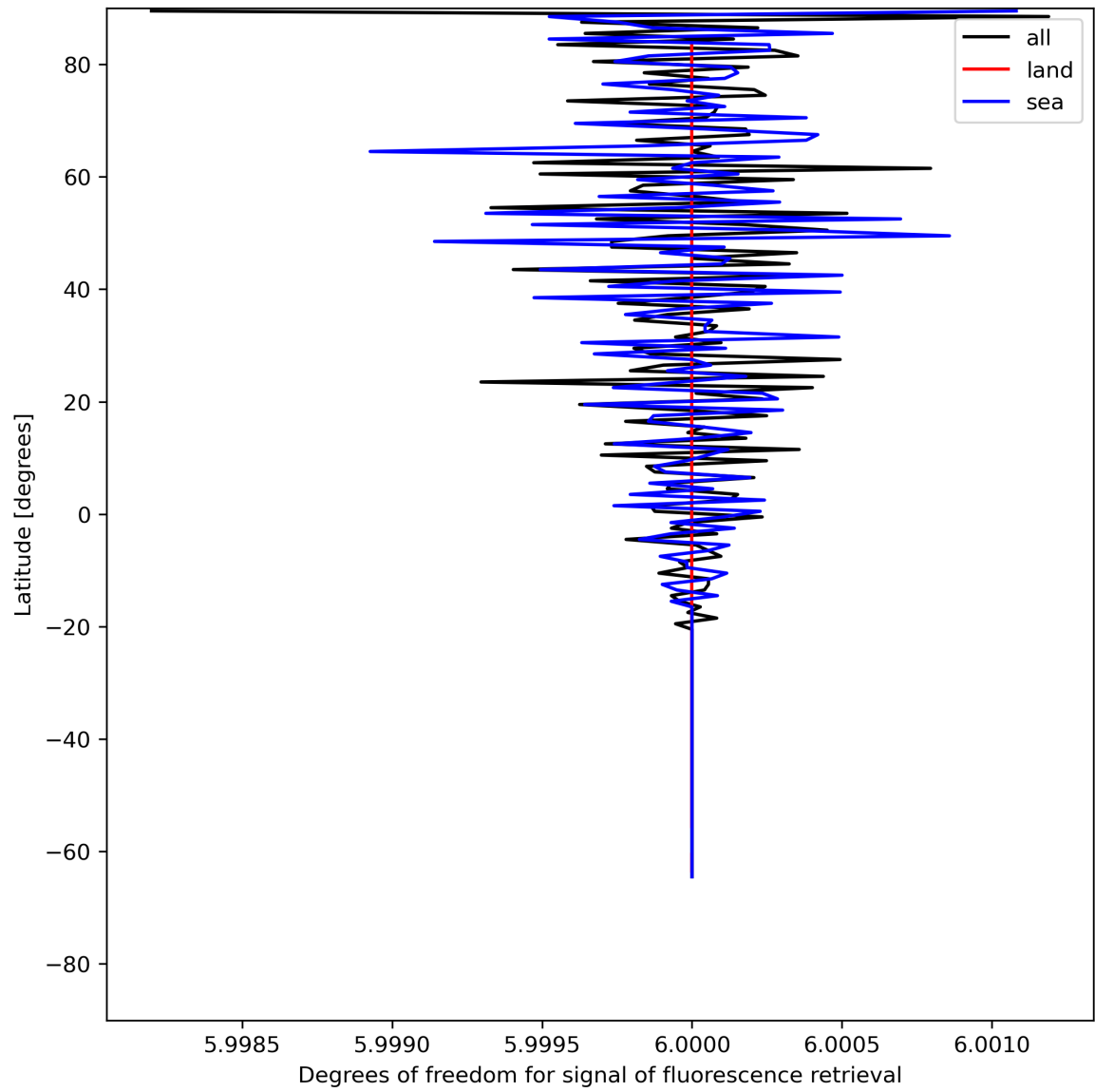
Figure 26: Zonal average of “Degrees of freedom for signal of fluorescence retrieval” for 2024-06-29 to 2024-06-30.
