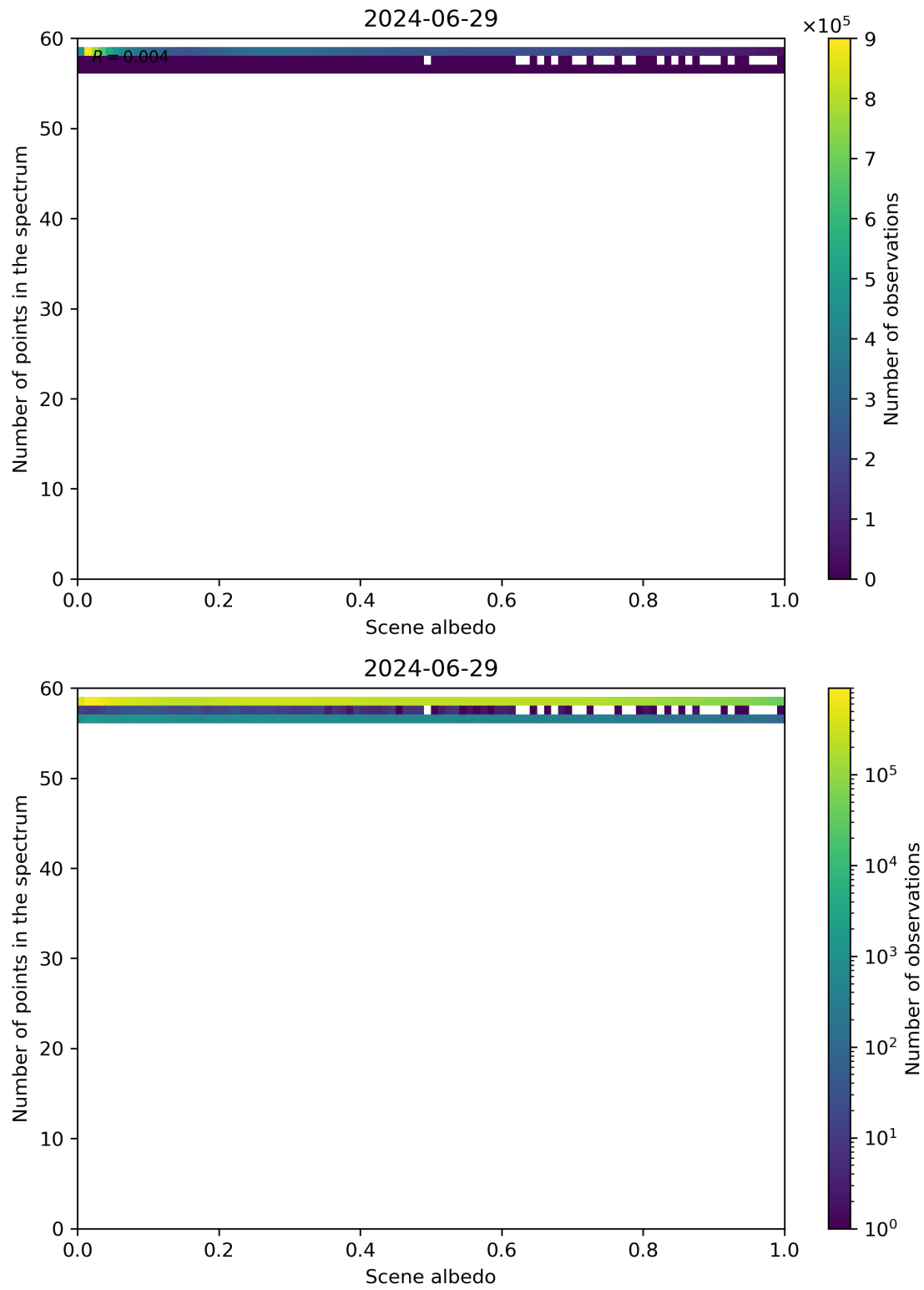
Figure 106: Scatter density plot of “Scene albedo” against “Number of points in the spectrum” for 2024-06-29 to 2024-06-30.
