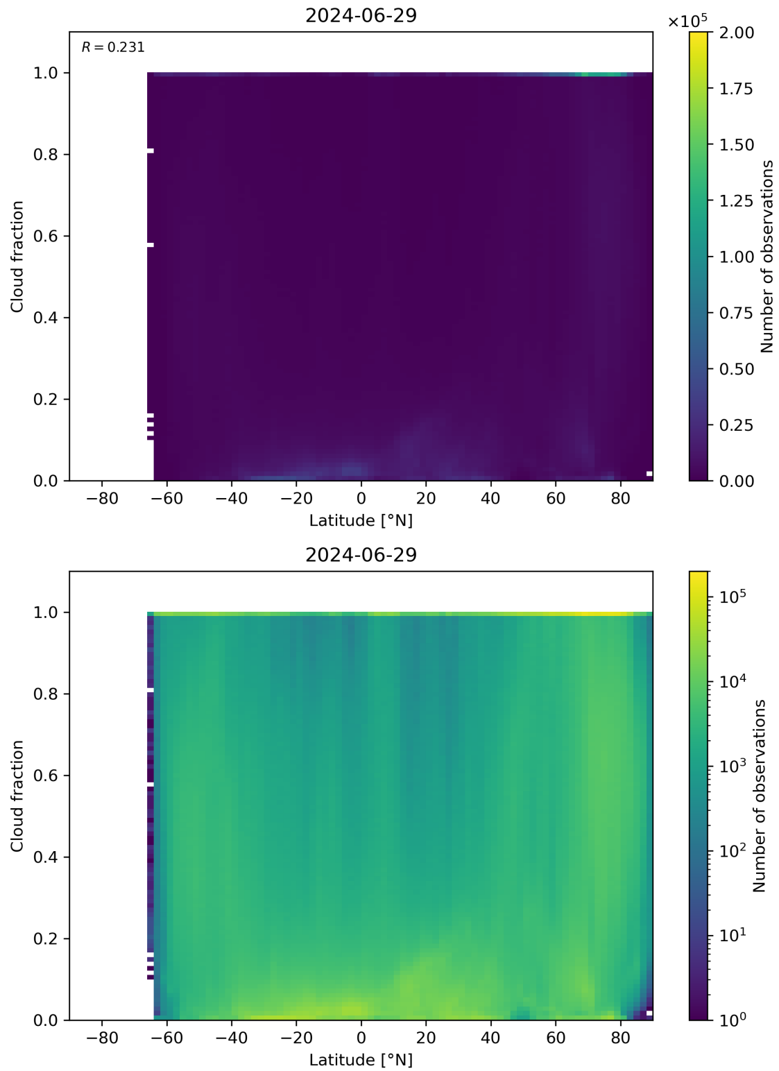
Figure 90: Scatter density plot of “Latitude” against “Cloud fraction” for 2024-06-29 to 2024-06-30.
