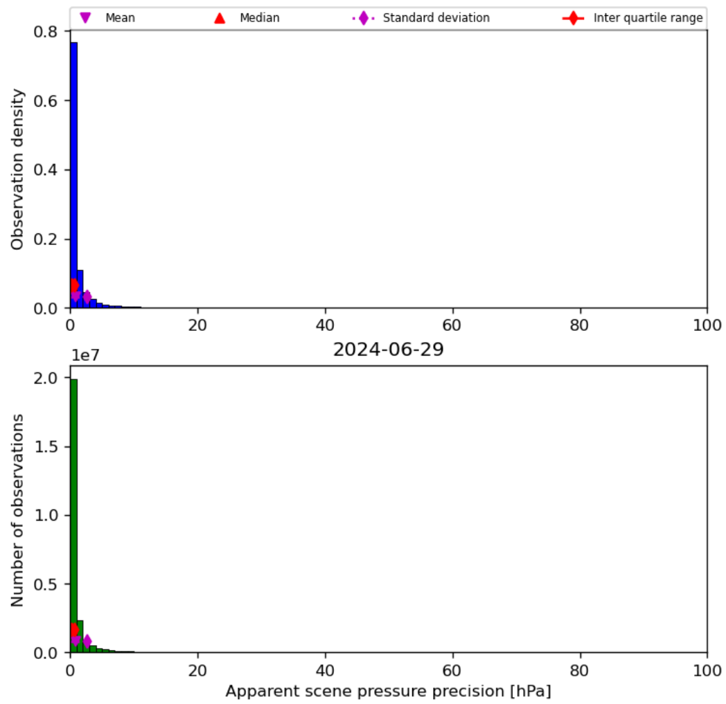
Figure 37: Histogram of “Apparent scene pressure precision” for 2024-06-29 to 2024-06-30
