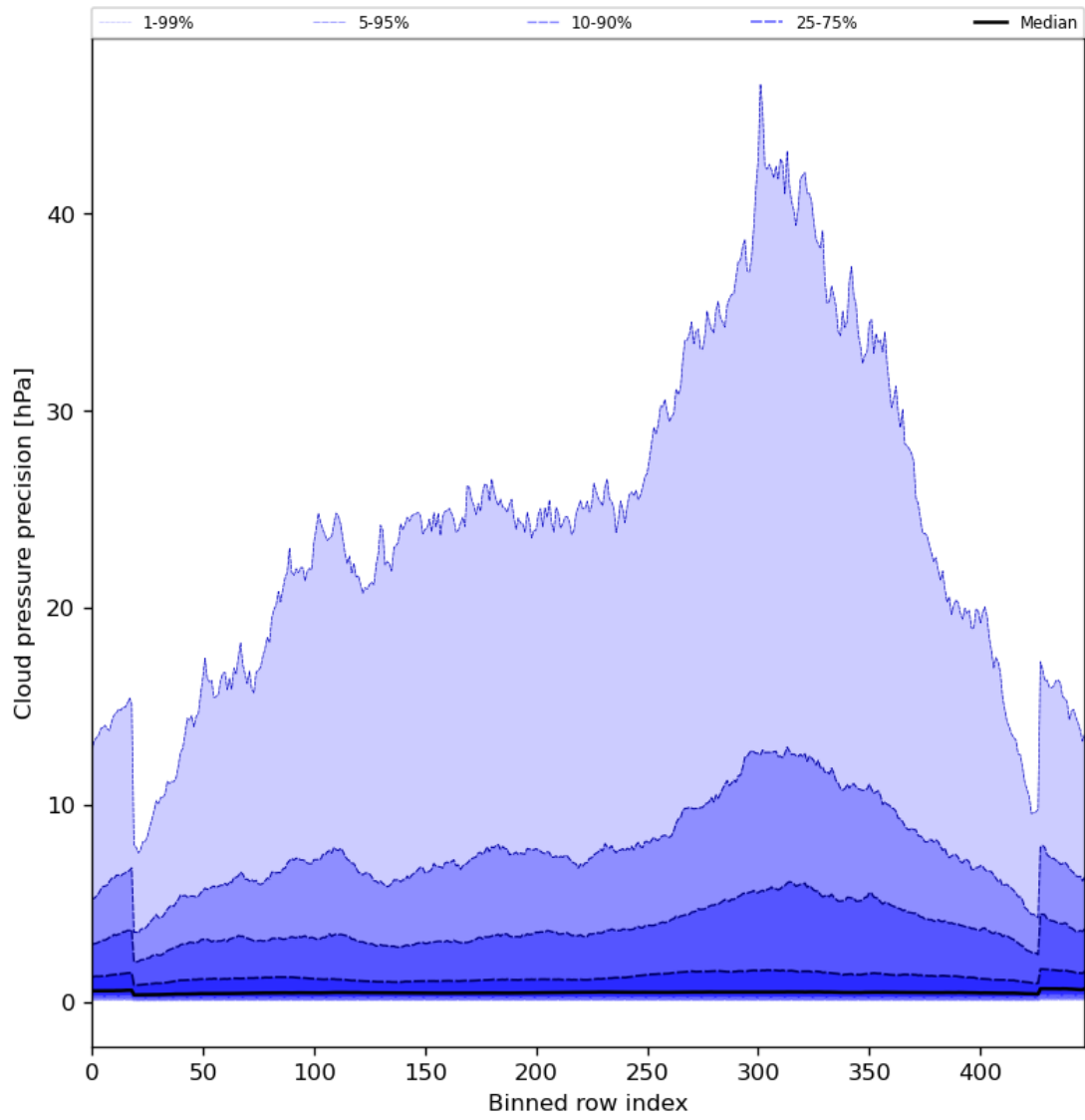
Figure 48: Along track statistics of “Cloud pressure precision” for 2024-06-29 to 2024-06-30
