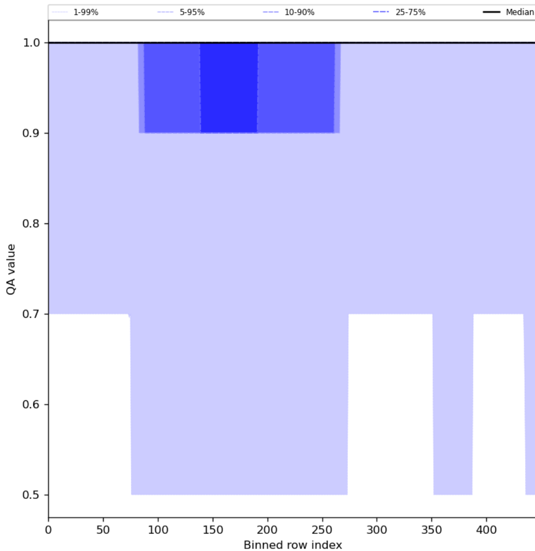
Figure 46: Along track statistics of “QA value” for 2024-06-29 to 2024-06-30
