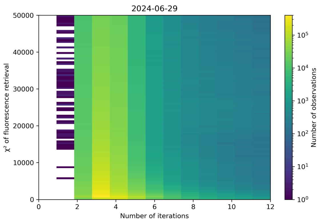
Figure 97: Scatter density plot of “Number of iterations” against “ \chi^2 of fluorescence retrieval” for 2024-06-29 to 2024-06-30.
