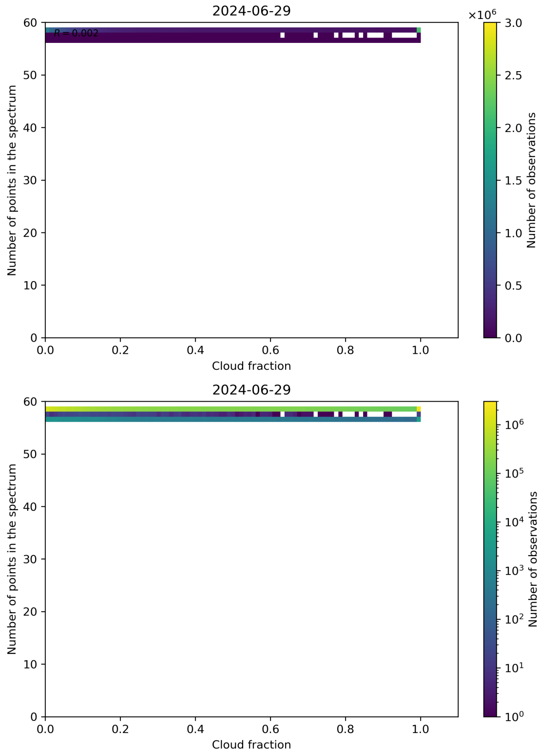
Figure 74: Scatter density plot of “Cloud fraction” against “Number of points in the spectrum” for 2024-06-29 to 2024-06-30.
