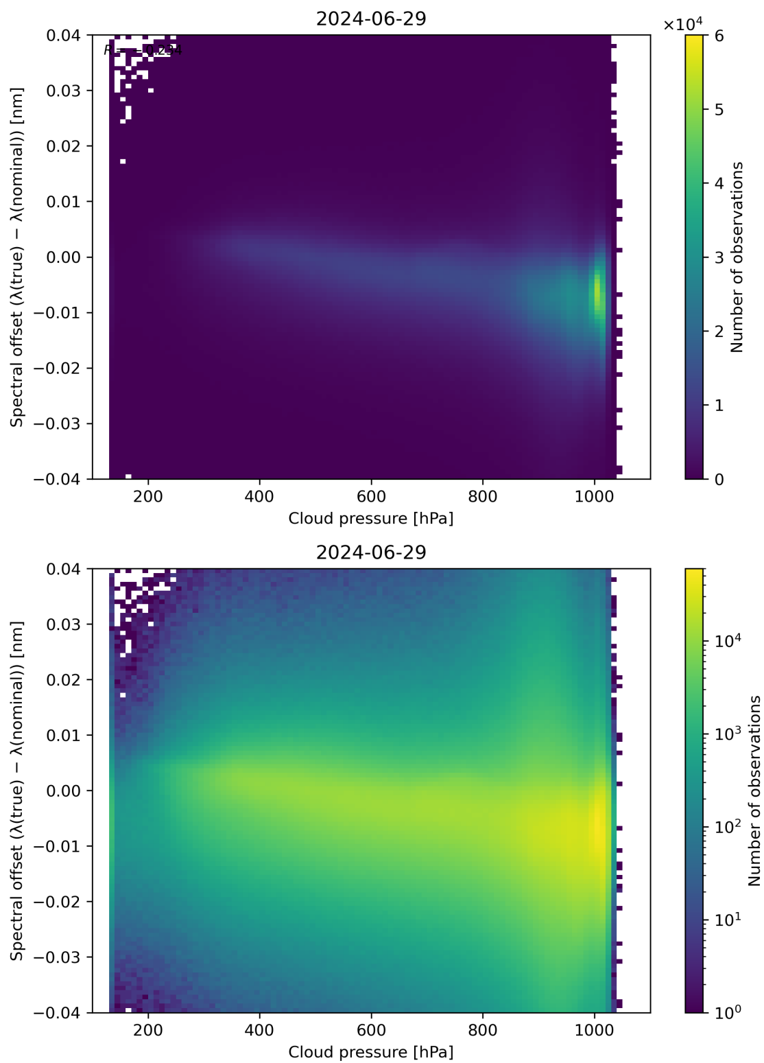
Figure 84: Scatter density plot of “Cloud pressure” against “Spectral offset ( \lambda(\text{true}) - \lambda(\text{nominal}) )” for 2024-06-29 to 2024-06-30.
