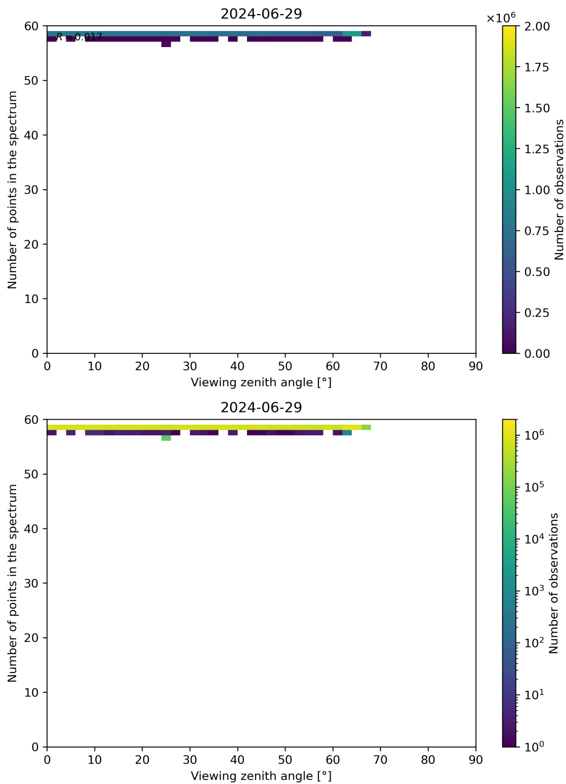
Figure 125: Scatter density plot of “Viewing zenith angle” against “Number of points in the spectrum” for 2024-06-29 to 2024-06-30.
