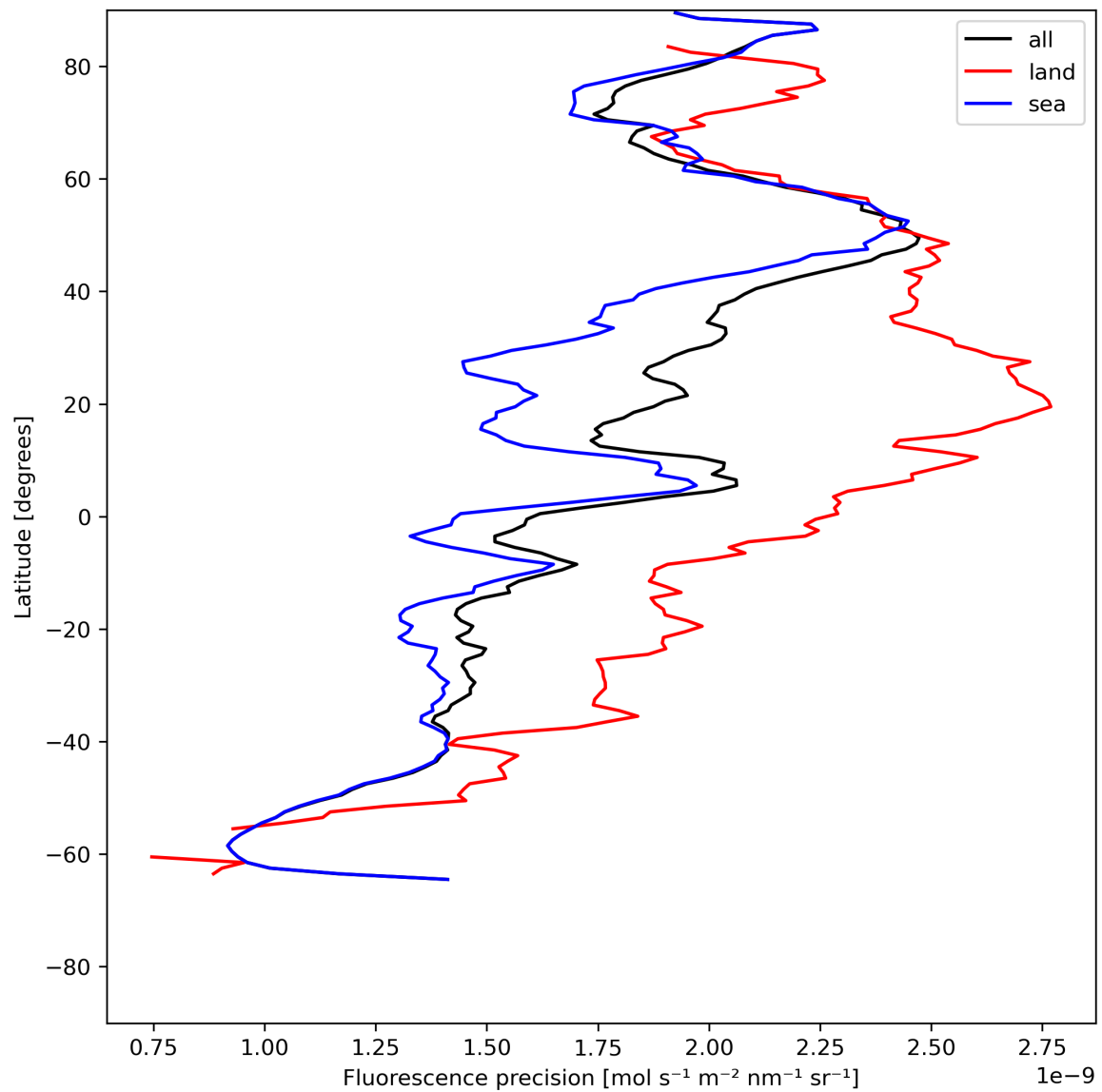
Figure 24: Zonal average of “Fluorescence precision” for 2024-06-29 to 2024-06-30.
