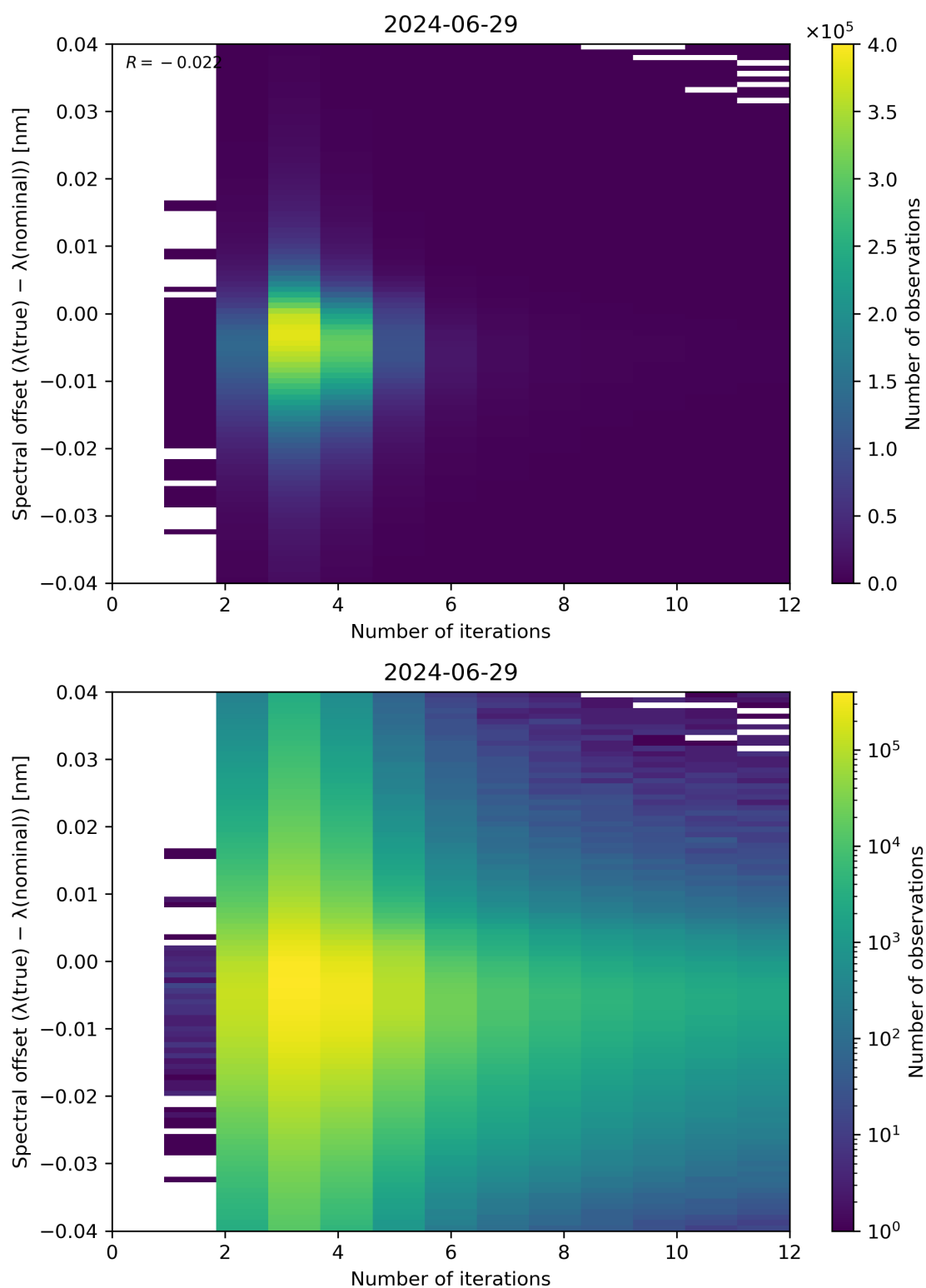
Figure 100: Scatter density plot of “Number of iterations” against “Spectral offset ( \lambda(\text{true}) - \lambda(\text{nominal}) )” for 2024-06-29 to 2024-06-30.
