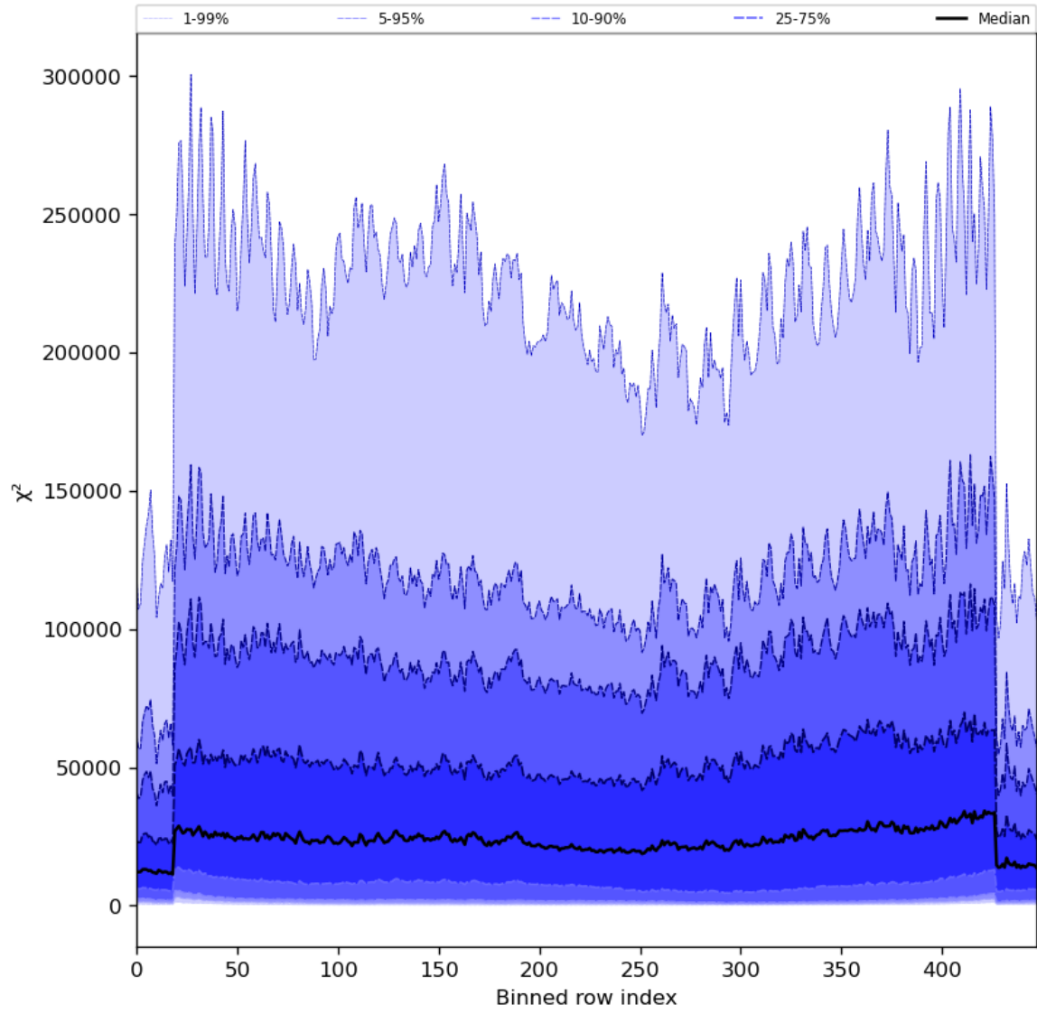
Figure 55: Along track statistics of “ \chi^2 ” for 2024-06-29 to 2024-06-30
