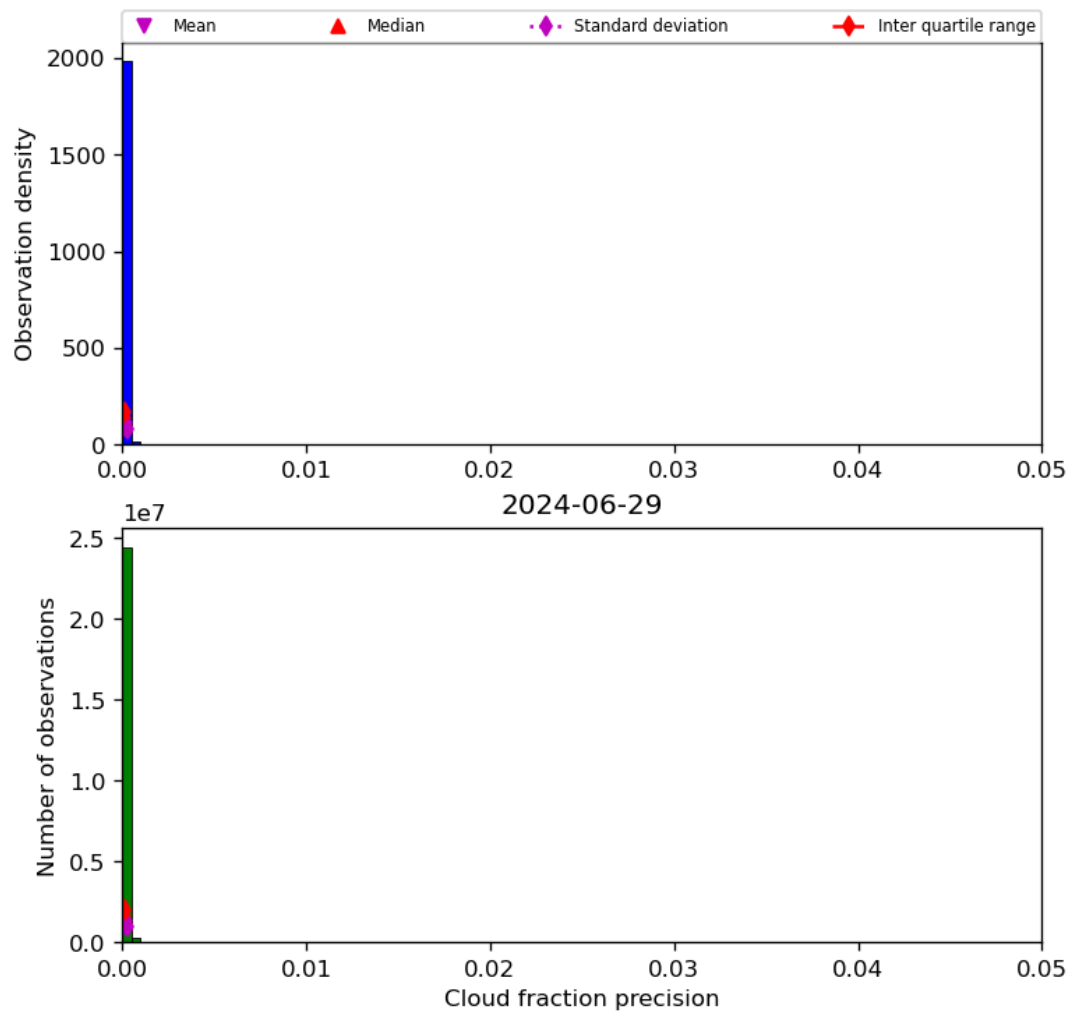
Figure 33: Histogram of “Cloud fraction precision” for 2024-06-29 to 2024-06-30
