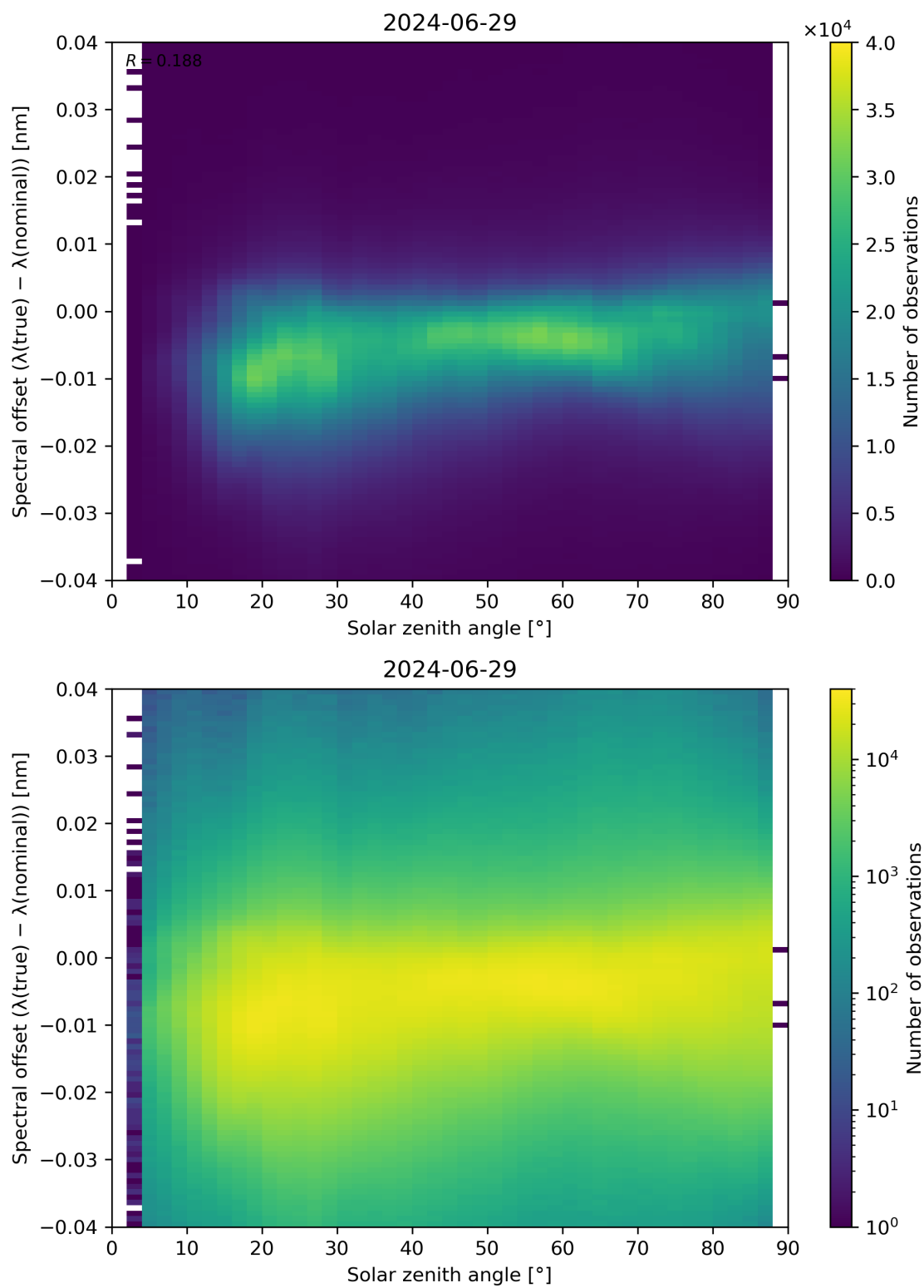
Figure 117: Scatter density plot of “Solar zenith angle” against “Spectral offset ( \lambda(\text{true}) - \lambda(\text{nominal}) )” for 2024-06-29 to 2024-06-30.
