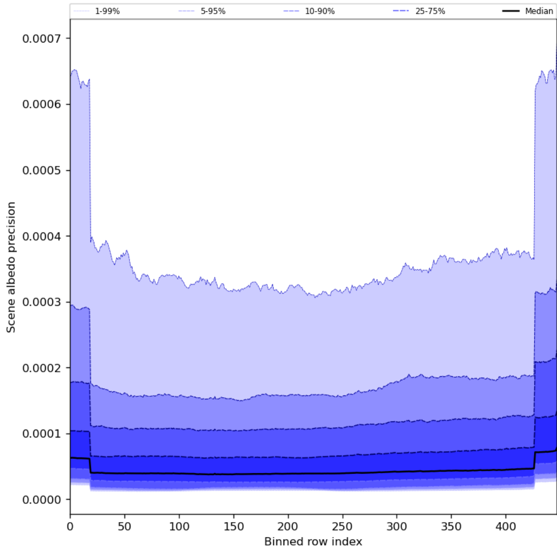
Figure 52: Along track statistics of “Scene albedo precision” for 2024-06-29 to 2024-06-30
