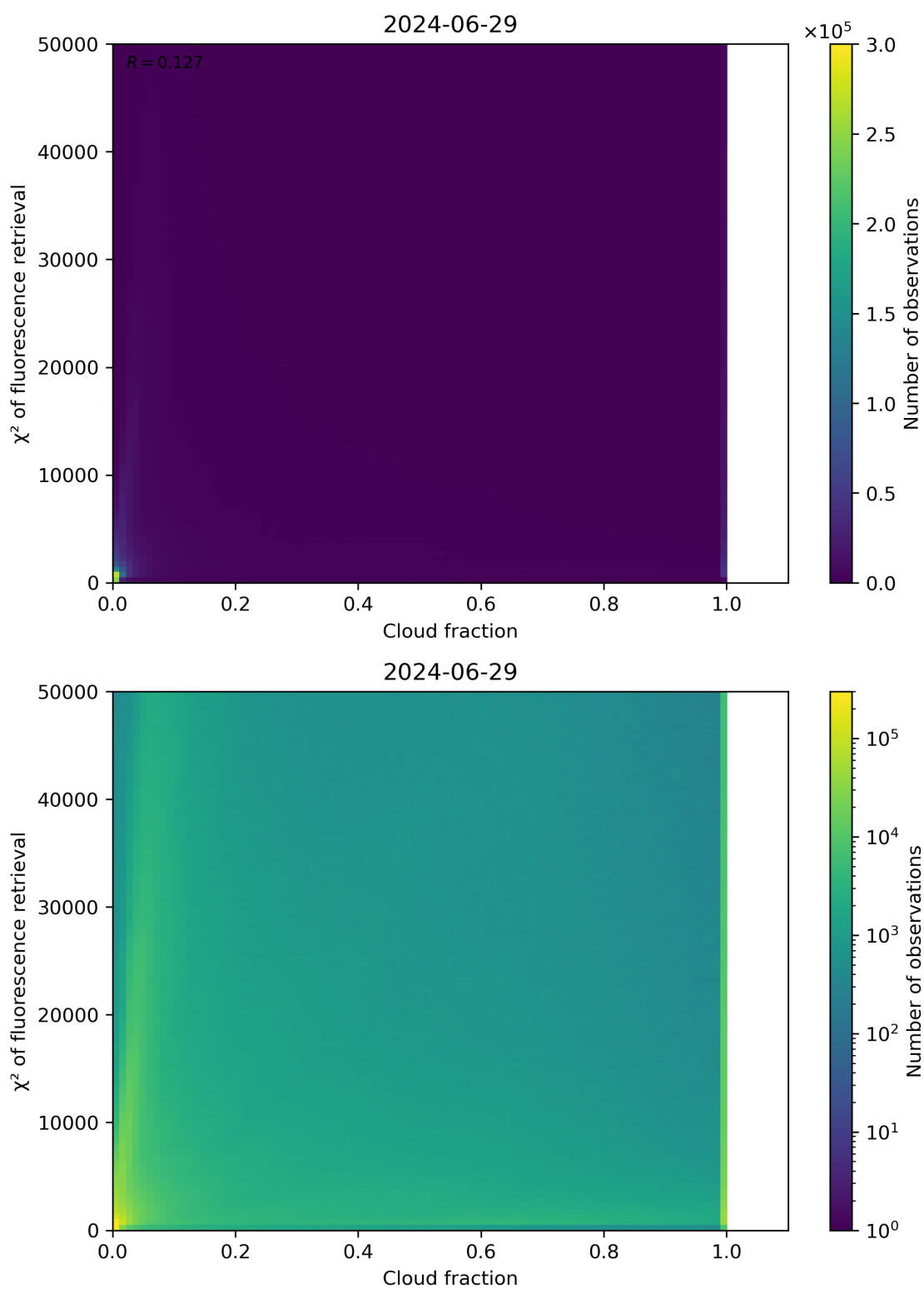
Figure 71: Scatter density plot of “Cloud fraction” against “ \chi^2 of fluorescence retrieval” for 2024-06-29 to 2024-06-30.
