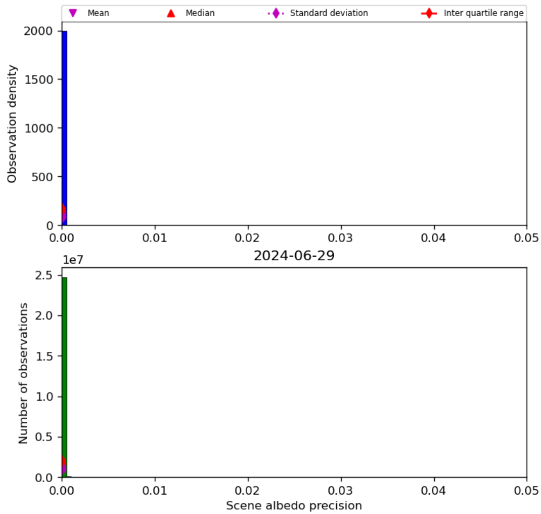
Figure 35: Histogram of “Scene albedo precision” for 2024-06-29 to 2024-06-30
