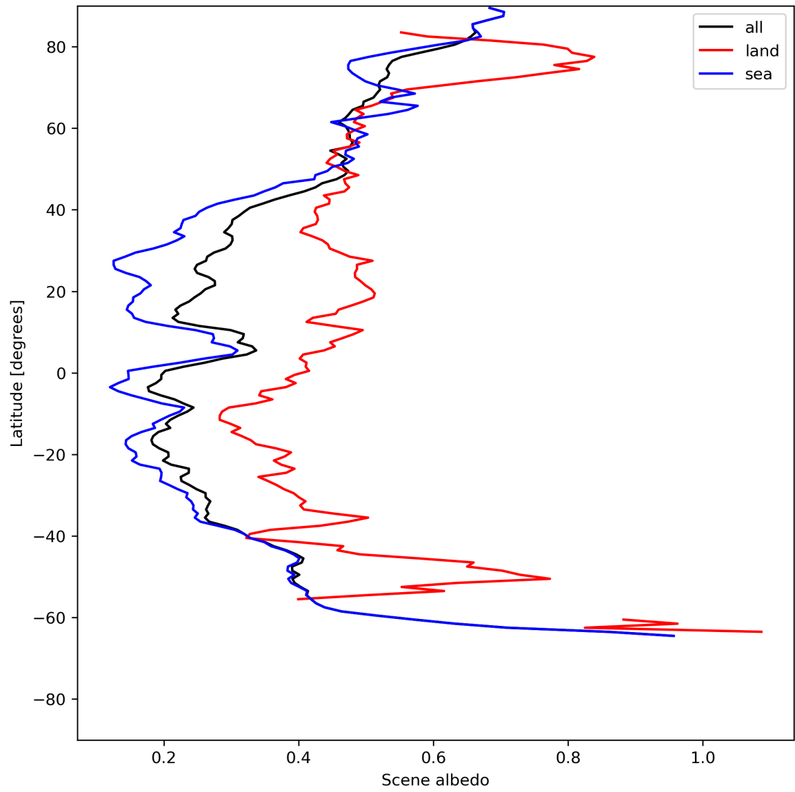
Figure 17: Zonal average of “Scene albedo” for 2024-06-29 to 2024-06-30.
