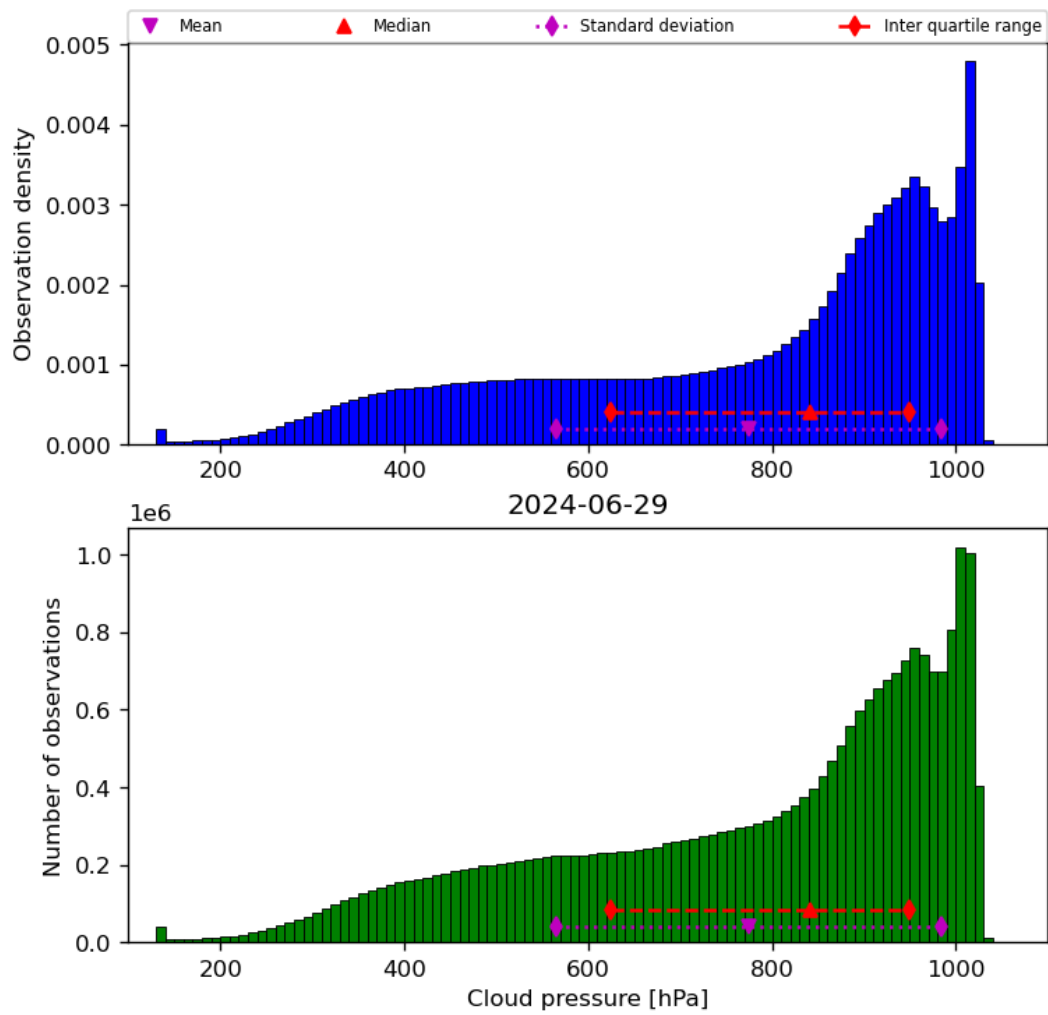
Figure 30: Histogram of “Cloud pressure” for 2024-06-29 to 2024-06-30
