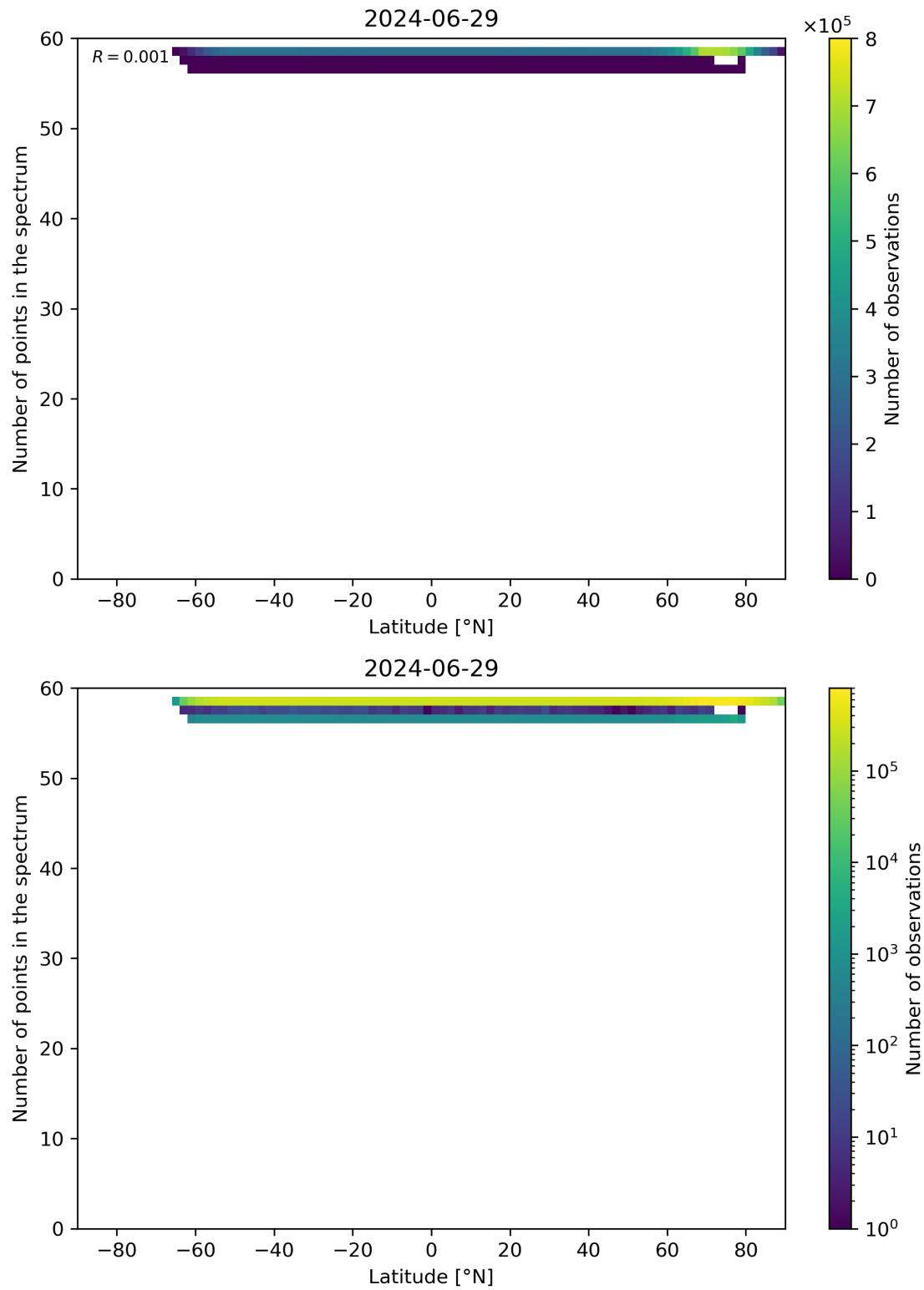
Figure 94: Scatter density plot of “Latitude” against “Number of points in the spectrum” for 2024-06-29 to 2024-06-30.
