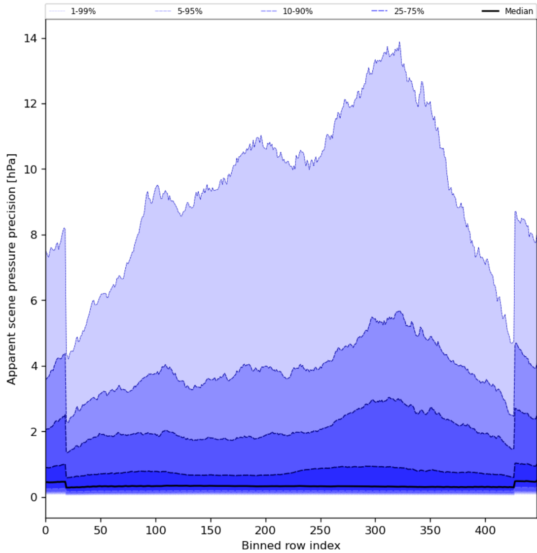
Figure 54: Along track statistics of “Apparent scene pressure precision” for 2024-06-29 to 2024-06-30
