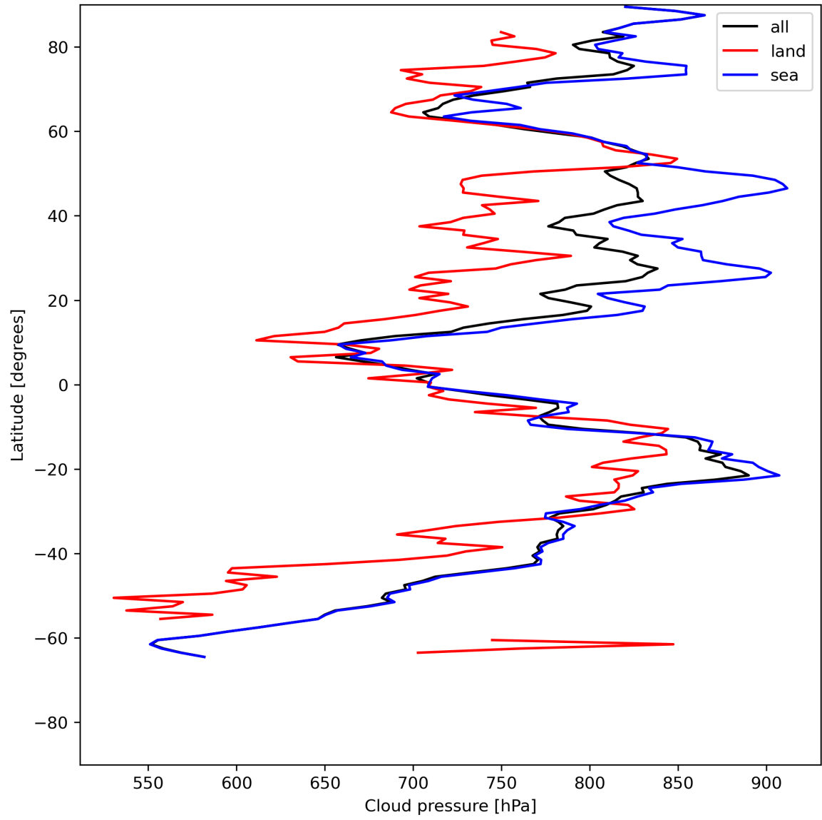
Figure 13: Zonal average of “Cloud pressure” for 2024-06-29 to 2024-06-30.
