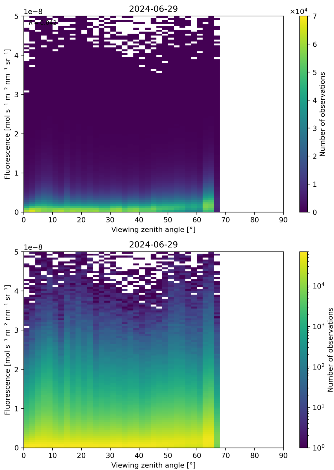
Figure 122: Scatter density plot of “Viewing zenith angle” against “Fluorescence” for 2024-06-29 to 2024-06-30.
