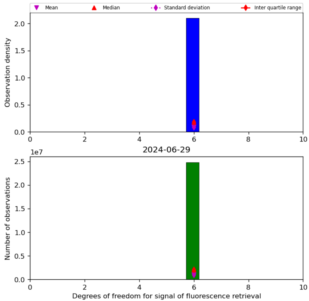
Figure 43: Histogram of “Degrees of freedom for signal of fluorescence retrieval” for 2024-06-29 to 2024-06-30
