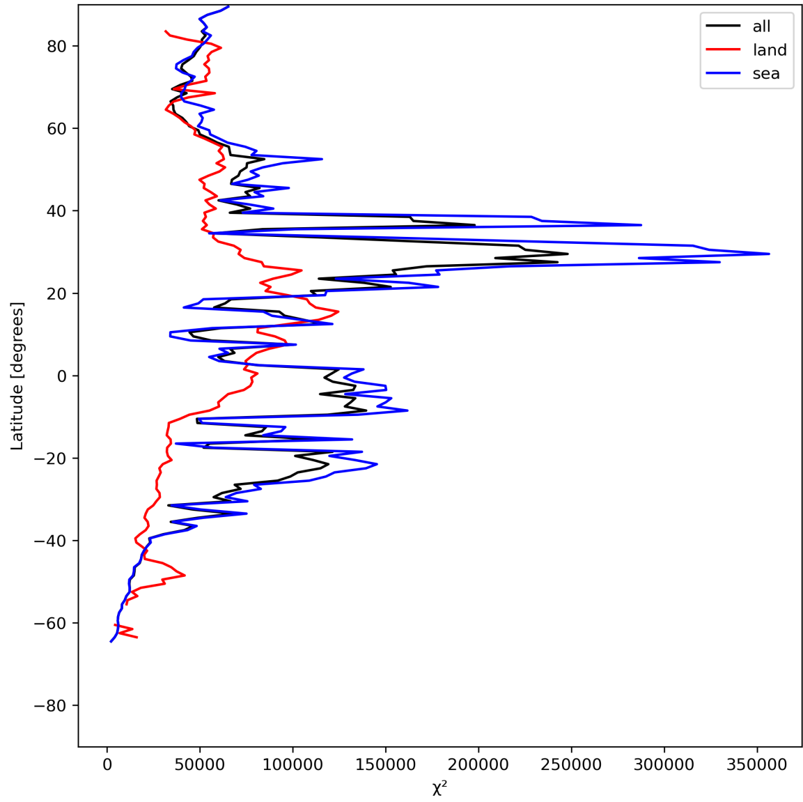
Figure 21: Zonal average of “ \chi^2 ” for 2024-06-29 to 2024-06-30.
