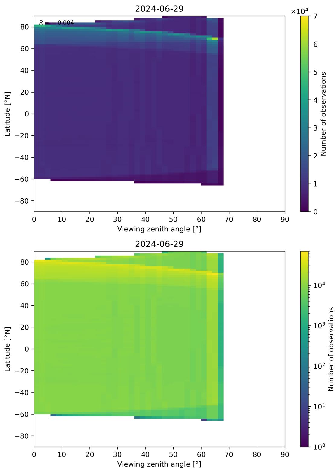
Figure 123: Scatter density plot of “Viewing zenith angle” against “Latitude” for 2024-06-29 to 2024-06-30.
