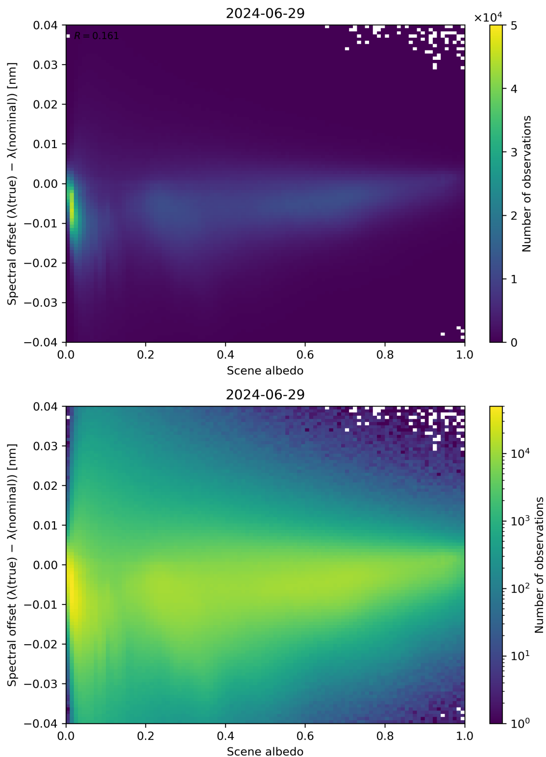
Figure 107: Scatter density plot of “Scene albedo” against “Spectral offset ( \lambda(\text{true}) - \lambda(\text{nominal}) )” for 2024-06-29 to 2024-06-30.
