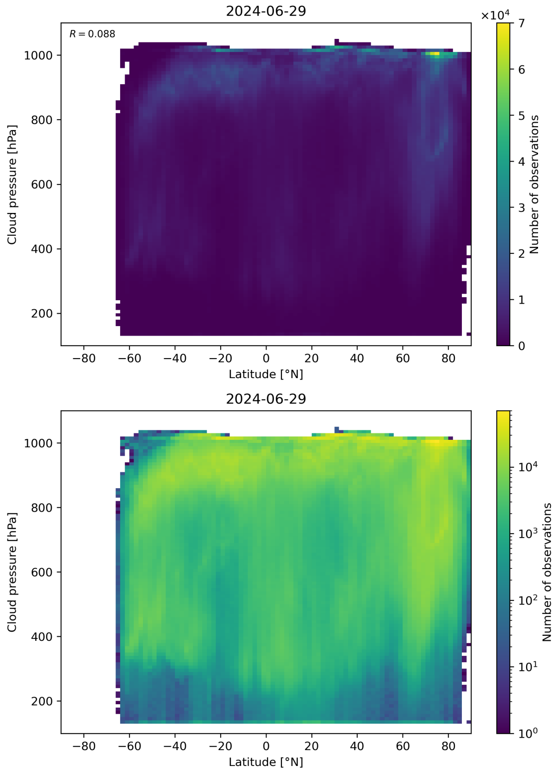
Figure 91: Scatter density plot of “Latitude” against “Cloud pressure” for 2024-06-29 to 2024-06-30.
