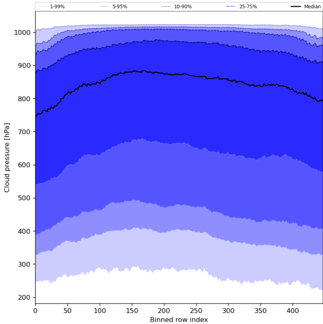
Figure 47: Along track statistics of “Cloud pressure” for 2024-06-29 to 2024-06-30
