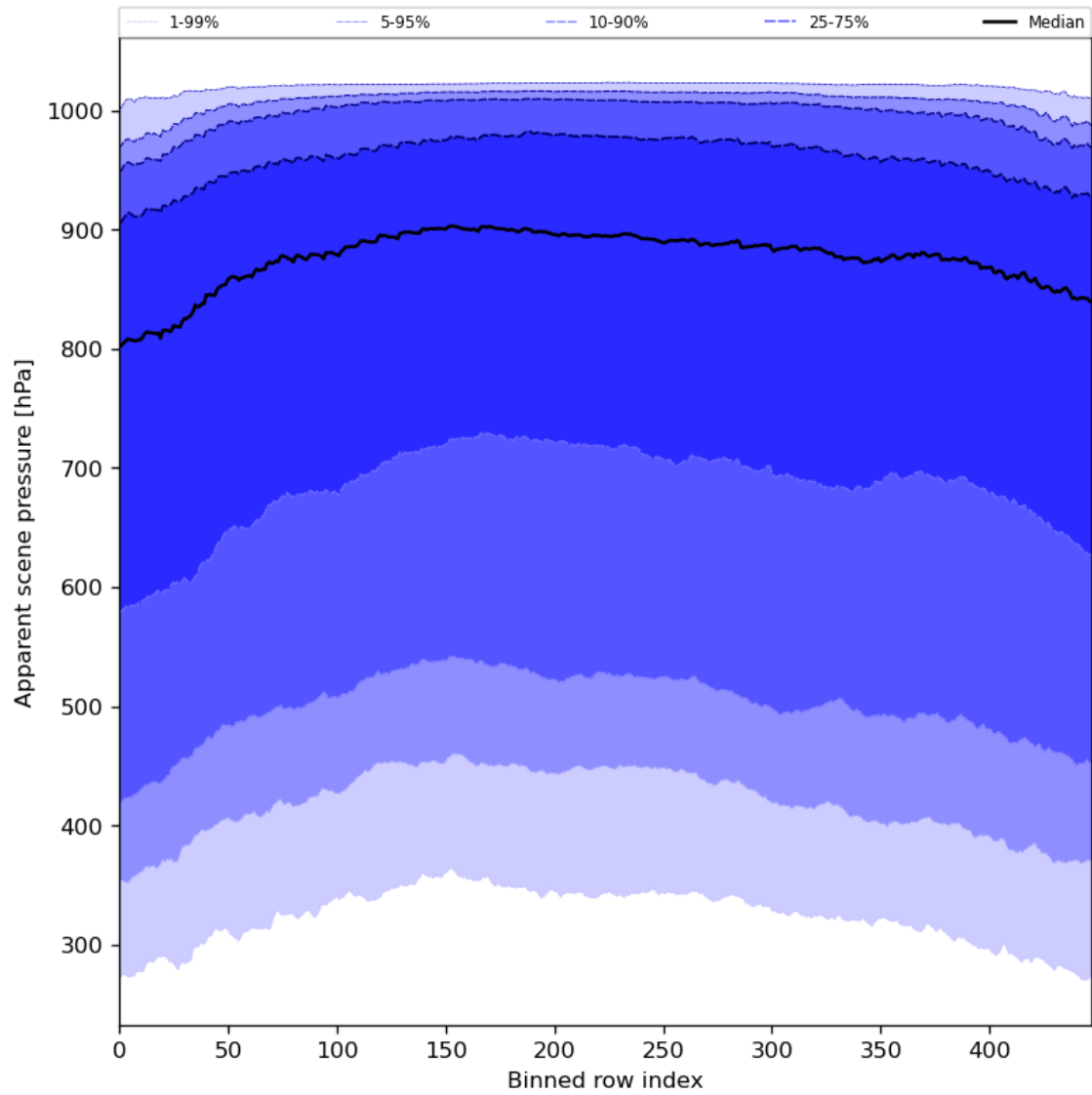
Figure 53: Along track statistics of “Apparent scene pressure” for 2024-06-29 to 2024-06-30
