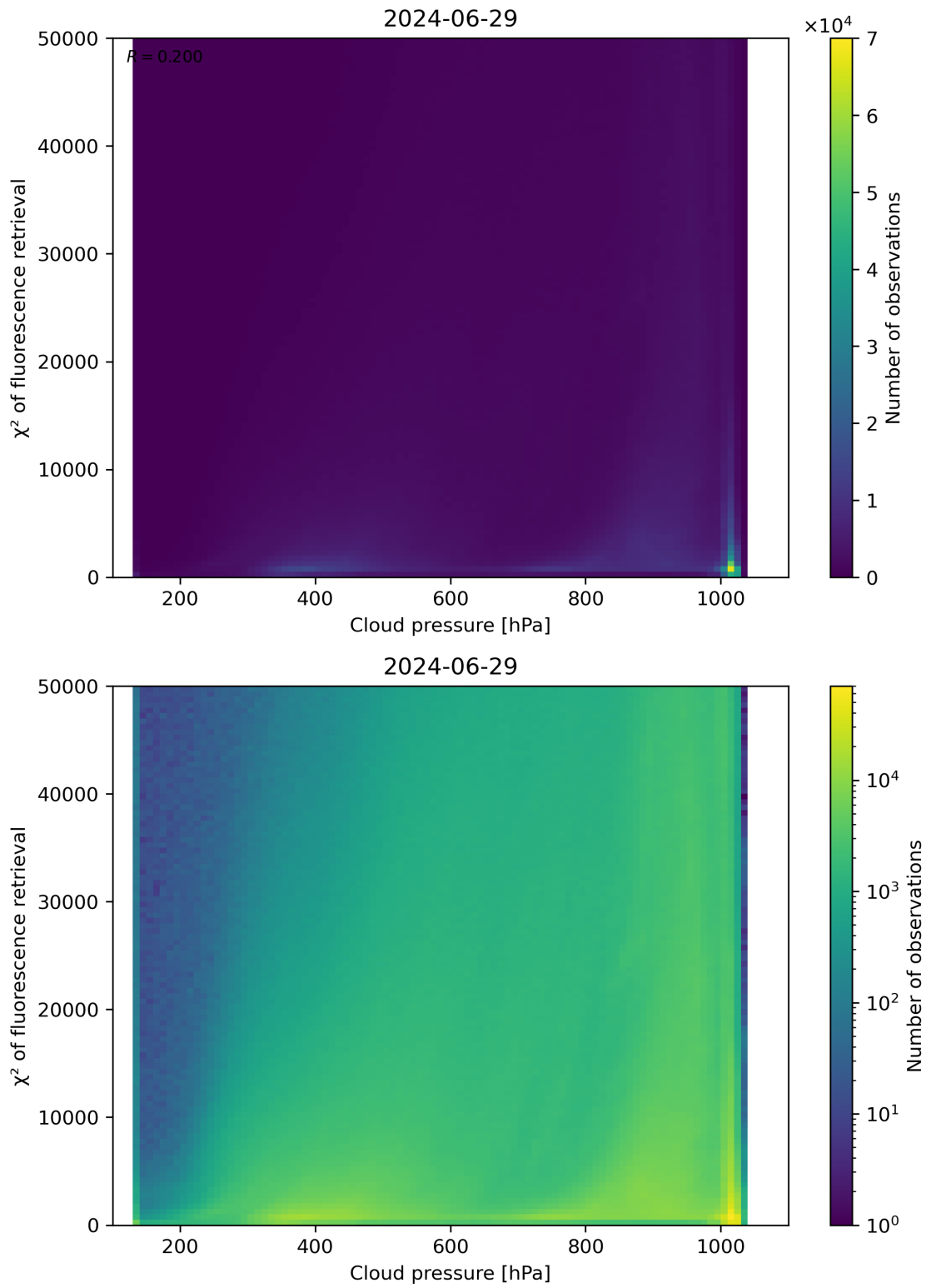
Figure 78: Scatter density plot of “Cloud pressure” against “ \chi^2 of fluorescence retrieval” for 2024-06-29 to 2024-06-30.
