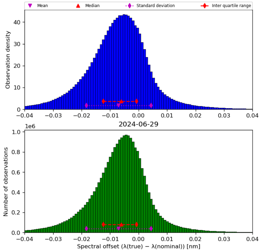
Figure 45: Histogram of “Spectral offset ( \lambda(\text{true}) - \lambda(\text{nominal}) )” for 2024-06-29 to 2024-06-30
