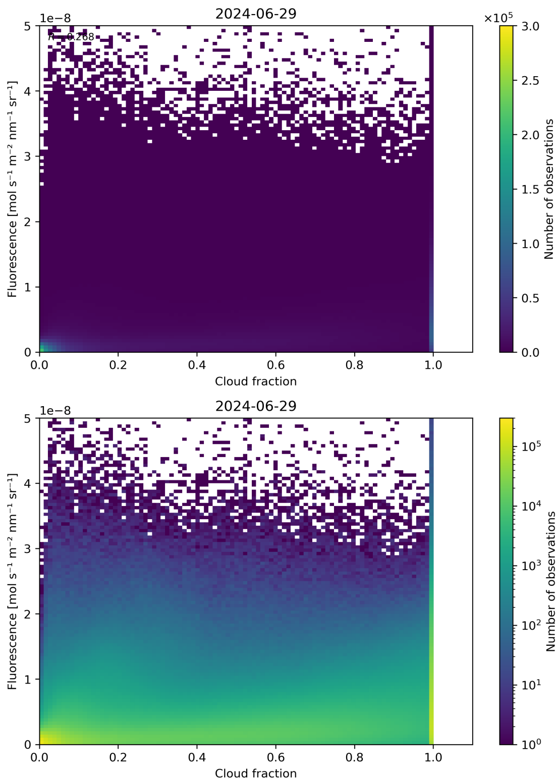
Figure 72: Scatter density plot of “Cloud fraction” against “Fluorescence” for 2024-06-29 to 2024-06-30.
