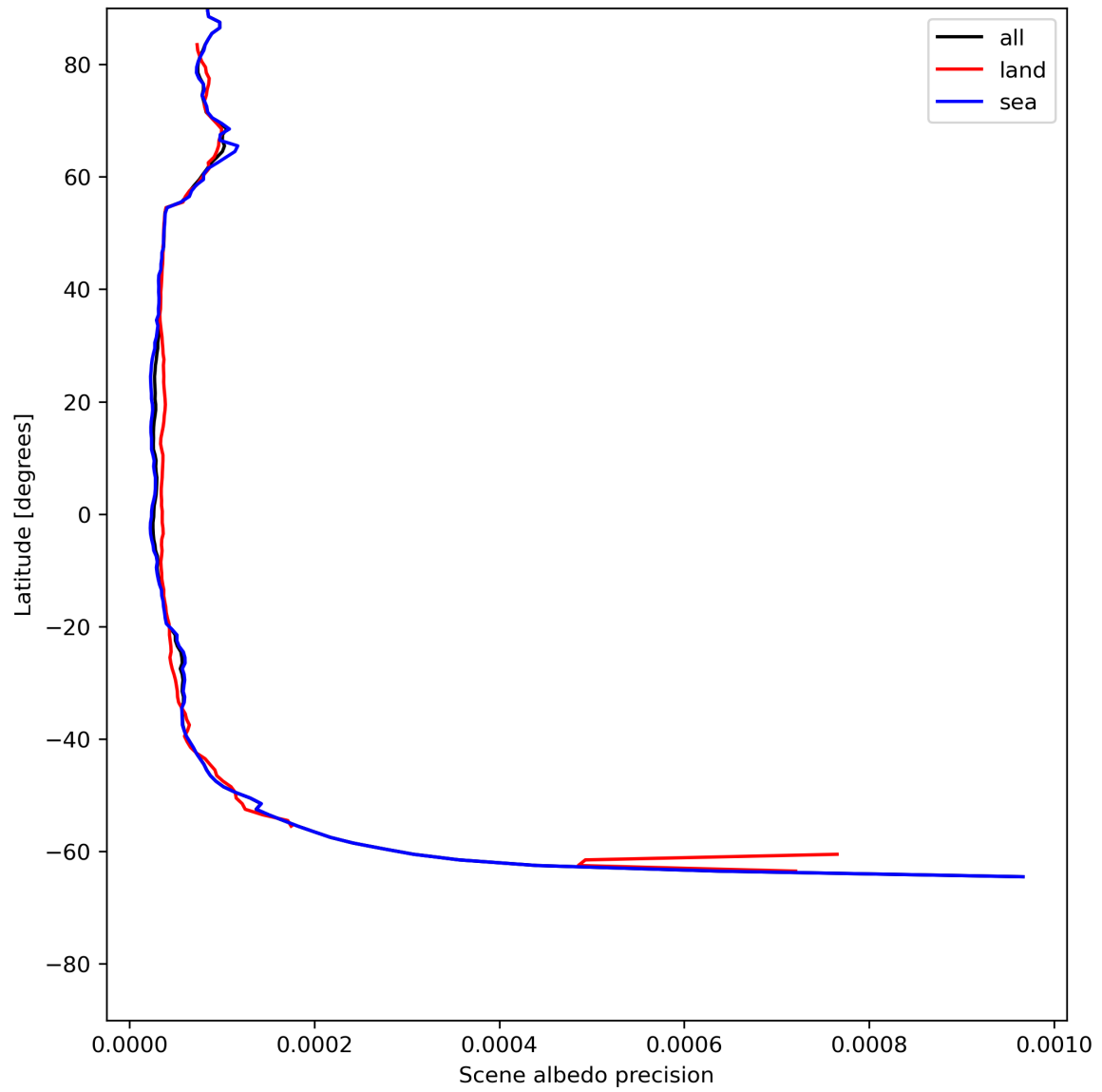
Figure 18: Zonal average of “Scene albedo precision” for 2024-06-29 to 2024-06-30.
