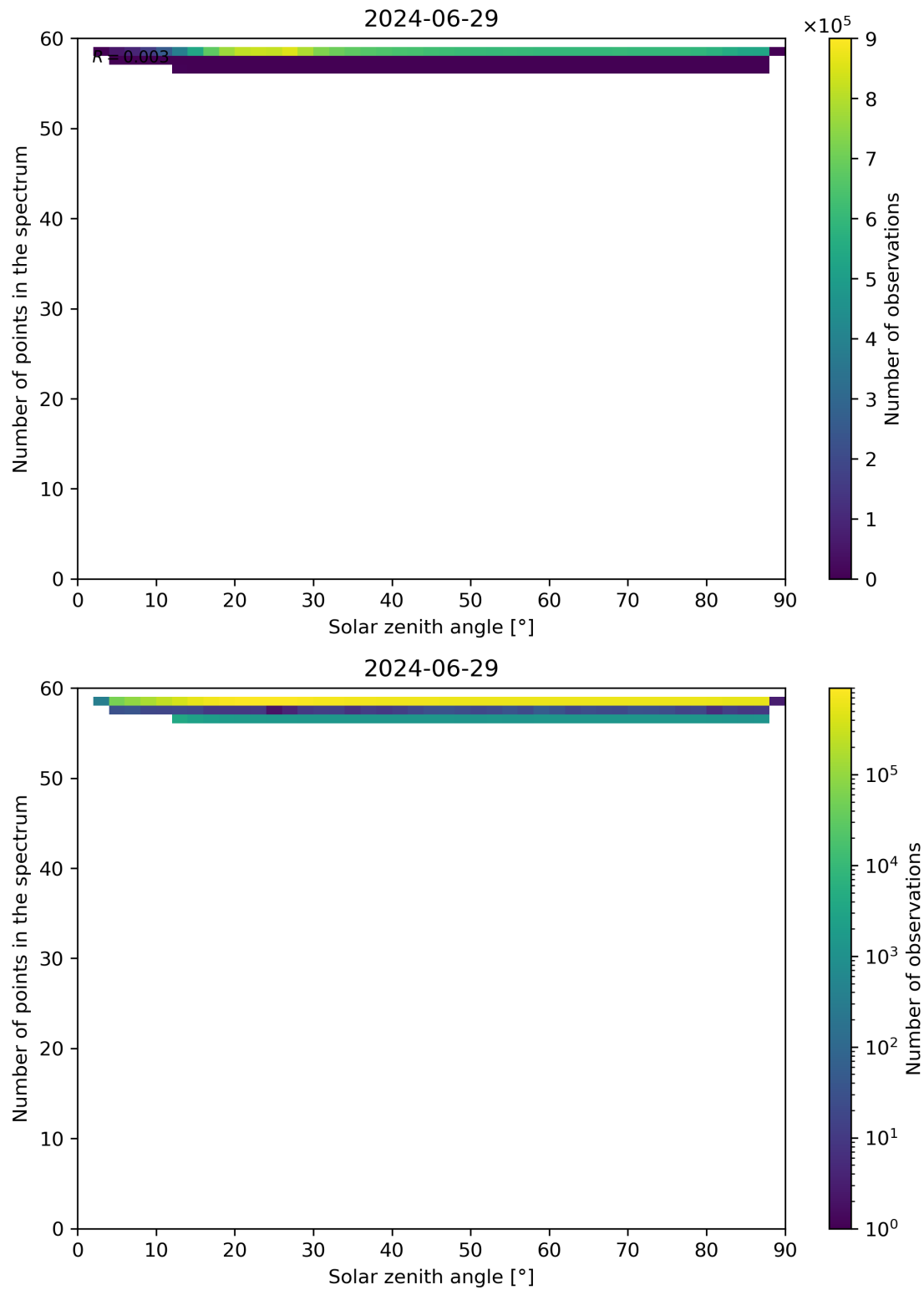
Figure 115: Scatter density plot of “Solar zenith angle” against “Number of points in the spectrum” for 2024-06-29 to 2024-06-30.
