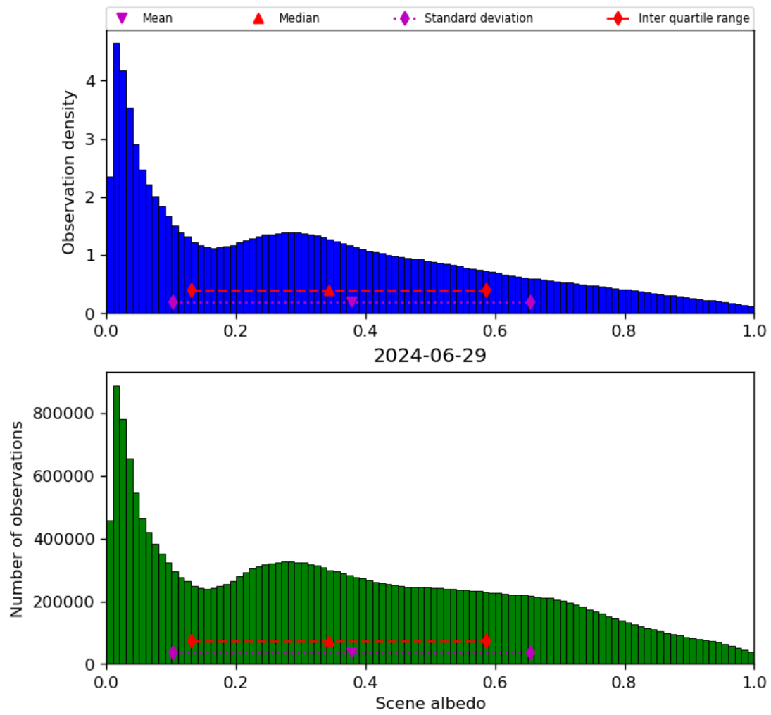
Figure 34: Histogram of “Scene albedo” for 2024-06-29 to 2024-06-30
