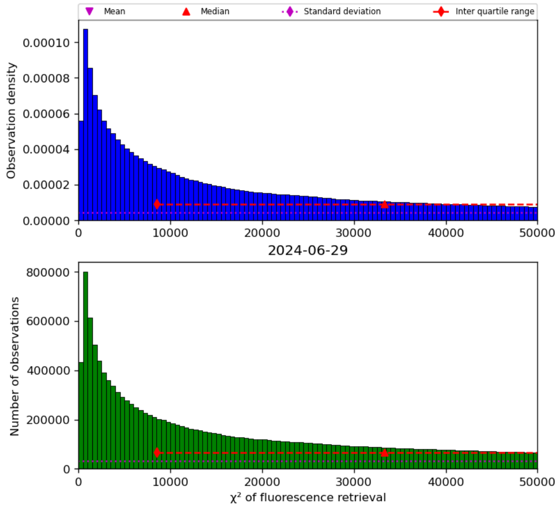
Figure 42: Histogram of “ \chi^2 of fluorescence retrieval” for 2024-06-29 to 2024-06-30
