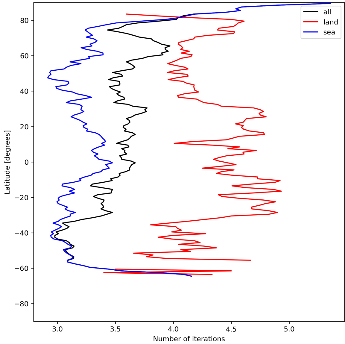
Figure 22: Zonal average of “Number of iterations” for 2024-06-29 to 2024-06-30.
