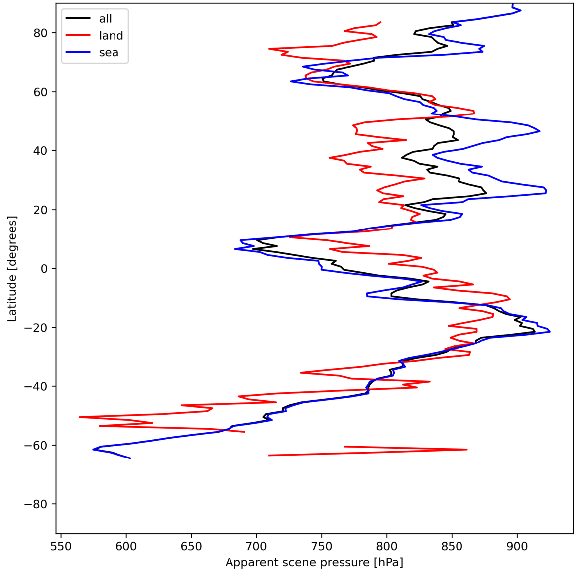
Figure 19: Zonal average of “Apparent scene pressure” for 2024-06-29 to 2024-06-30.
