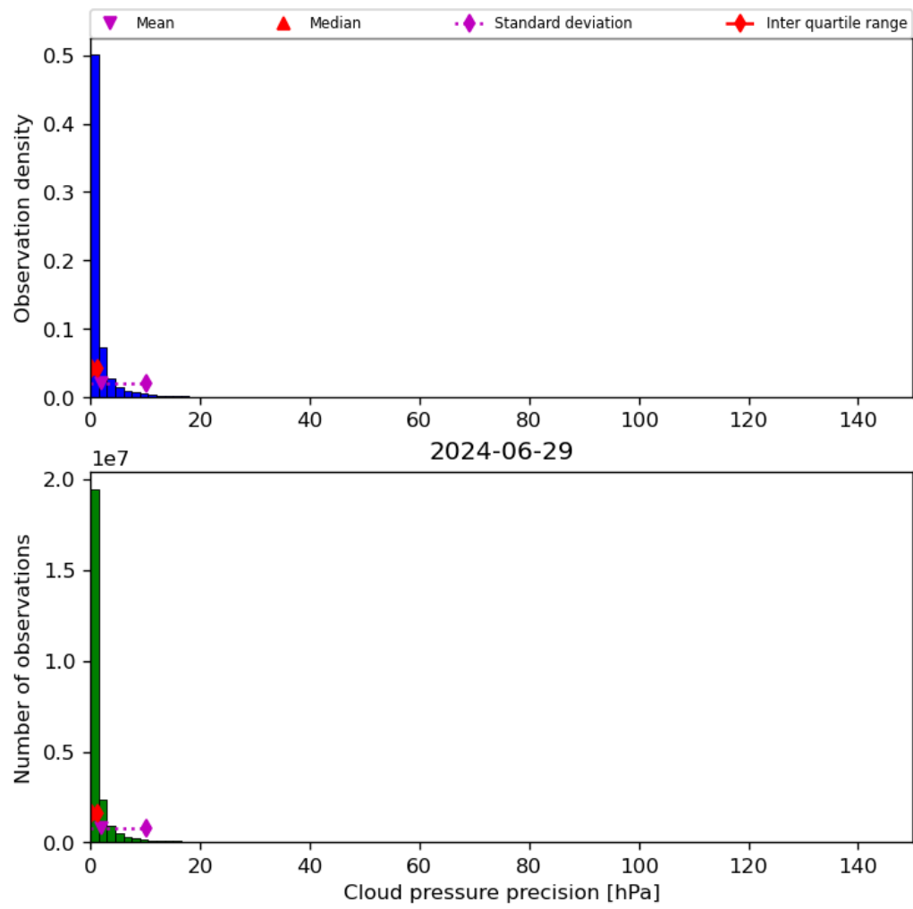
Figure 31: Histogram of “Cloud pressure precision” for 2024-06-29 to 2024-06-30
