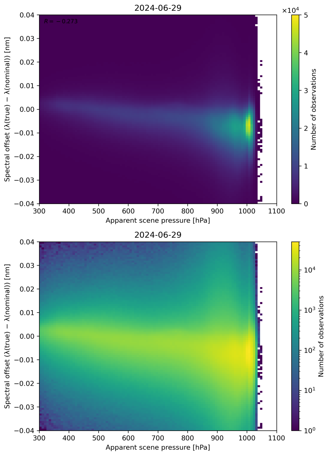
Figure 67: Scatter density plot of “Apparent scene pressure” against “Spectral offset ( \lambda(\text{true}) - \lambda(\text{nominal}) )” for 2024-06-29 to 2024-06-30.
