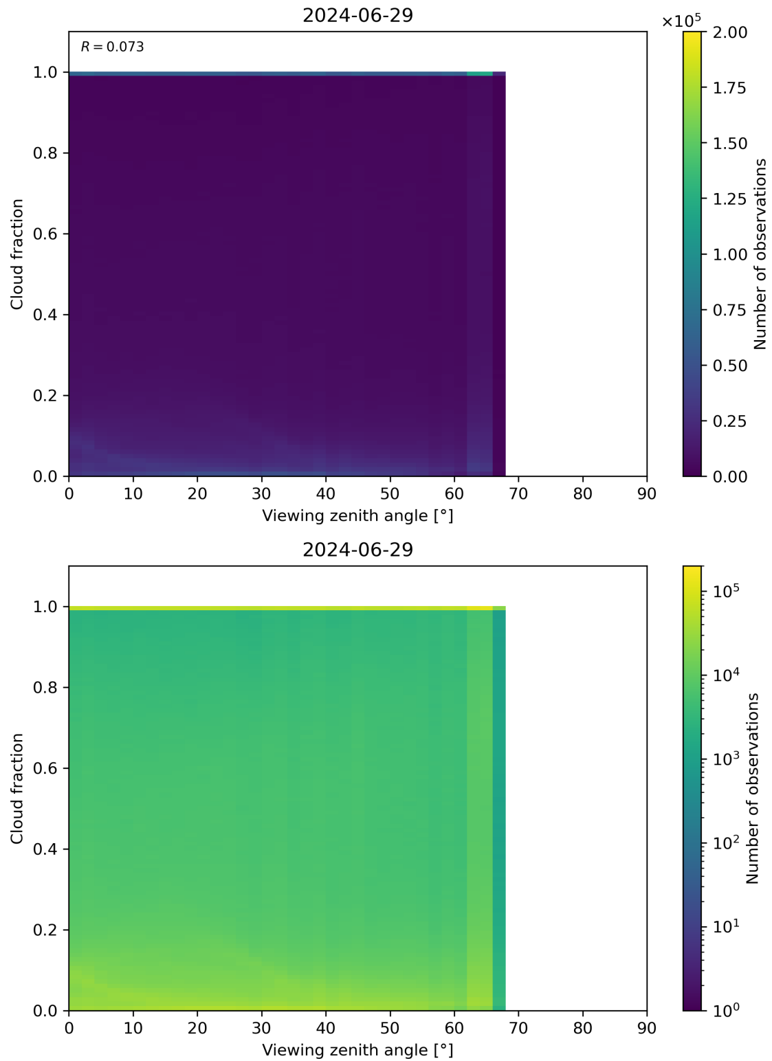
Figure 120: Scatter density plot of “Viewing zenith angle” against “Cloud fraction” for 2024-06-29 to 2024-06-30.
