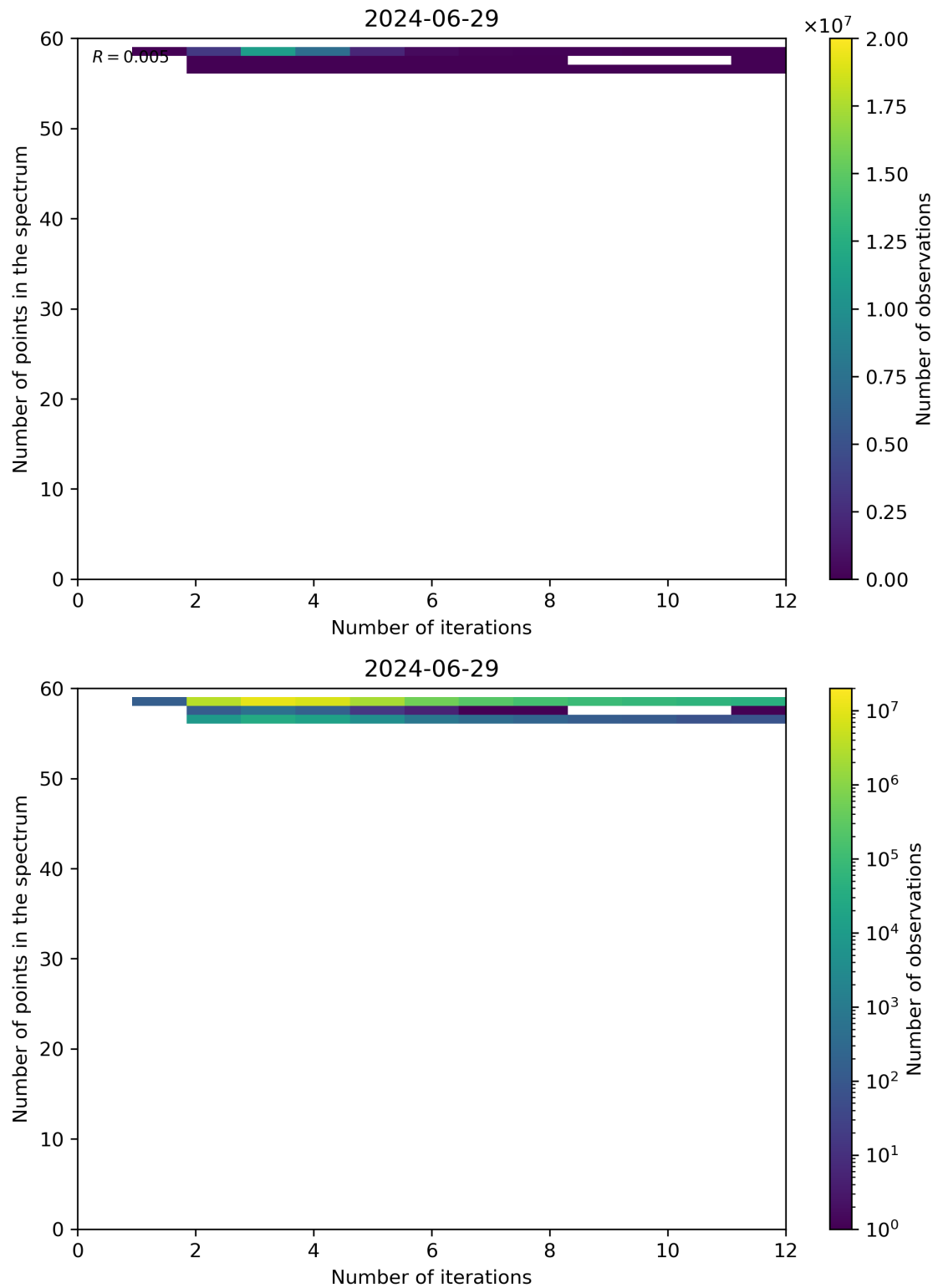
Figure 99: Scatter density plot of “Number of iterations” against “Number of points in the spectrum” for 2024-06-29 to 2024-06-30.
