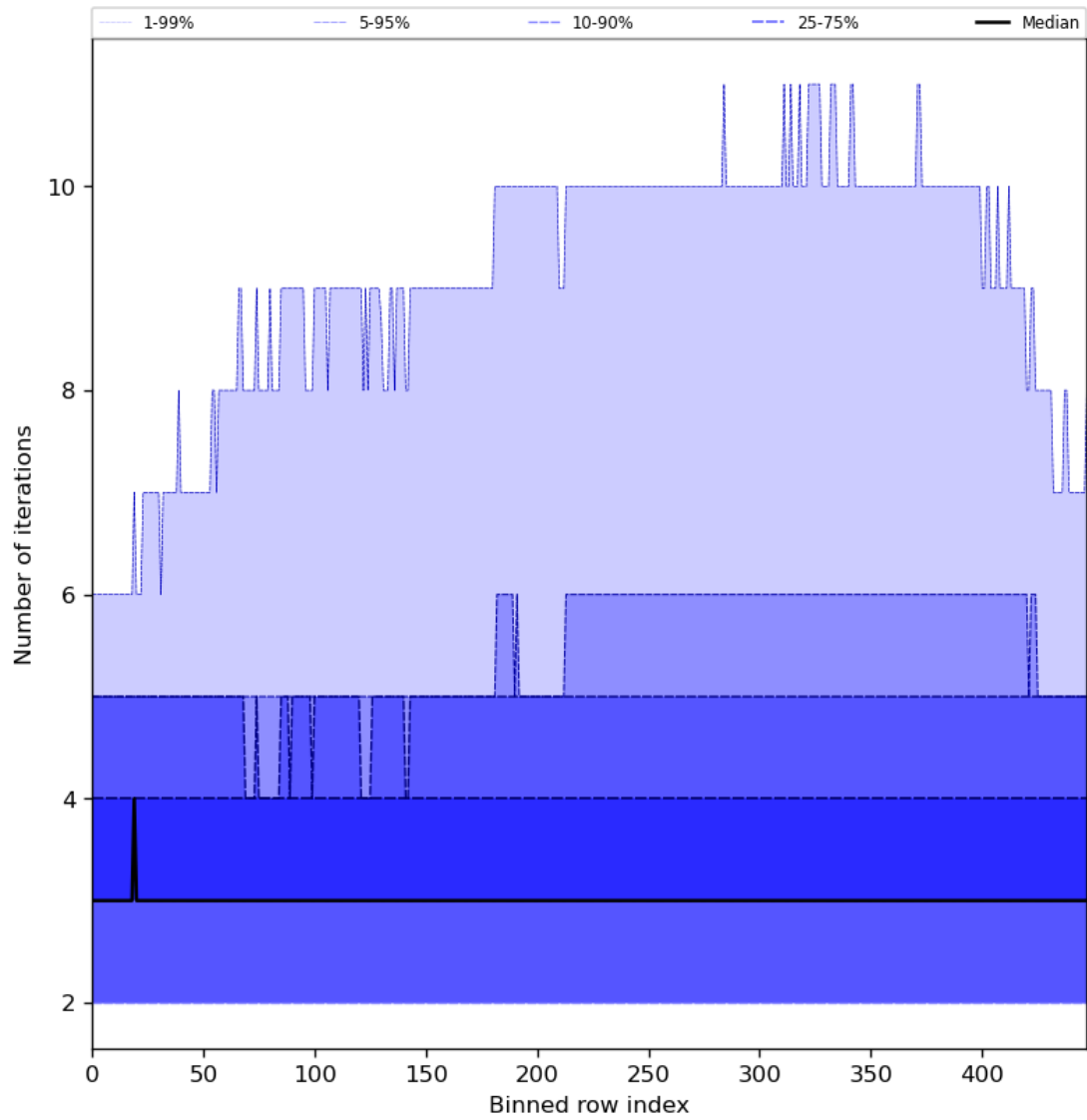
Figure 56: Along track statistics of “Number of iterations” for 2024-06-29 to 2024-06-30
