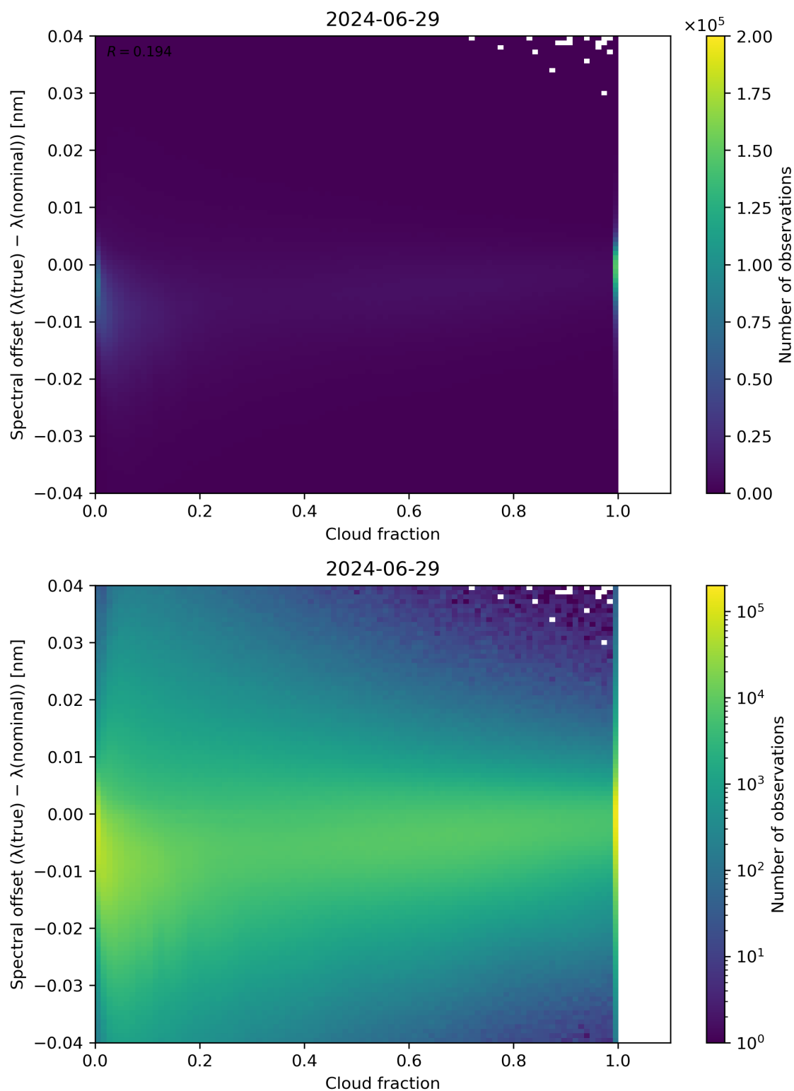
Figure 76: Scatter density plot of “Cloud fraction” against “Spectral offset ( \lambda(\text{true}) - \lambda(\text{nominal}) )” for 2024-06-29 to 2024-06-30.
