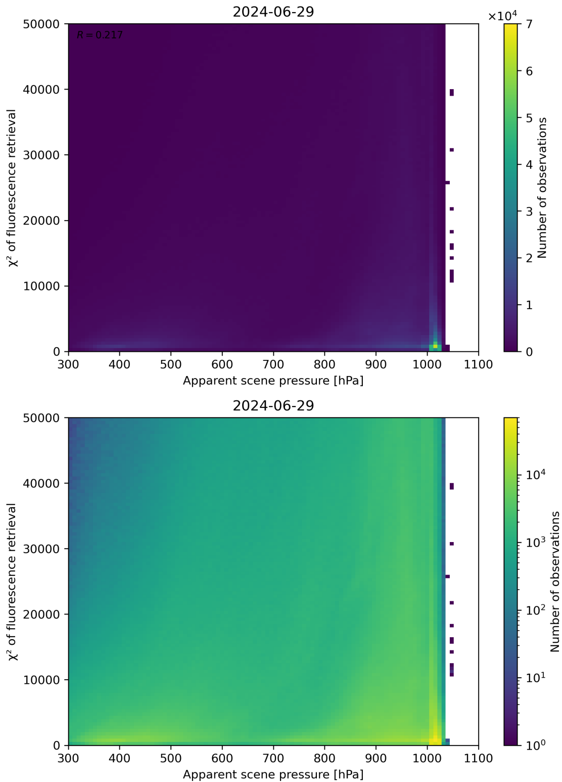
Figure 63: Scatter density plot of “Apparent scene pressure” against “ \chi^2 of fluorescence retrieval” for 2024-06-29 to 2024-06-30.
