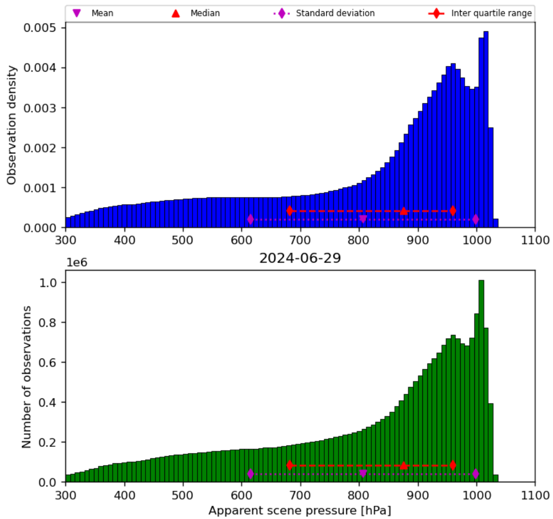
Figure 36: Histogram of “Apparent scene pressure” for 2024-06-29 to 2024-06-30
