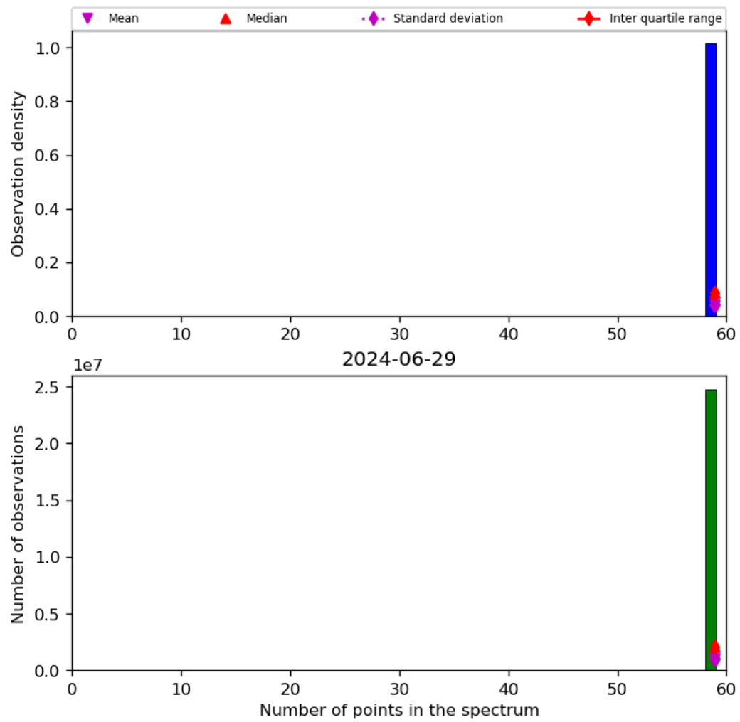
Figure 44: Histogram of “Number of points in the spectrum” for 2024-06-29 to 2024-06-30
