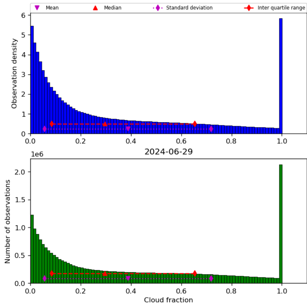
Figure 32: Histogram of “Cloud fraction” for 2024-06-29 to 2024-06-30
