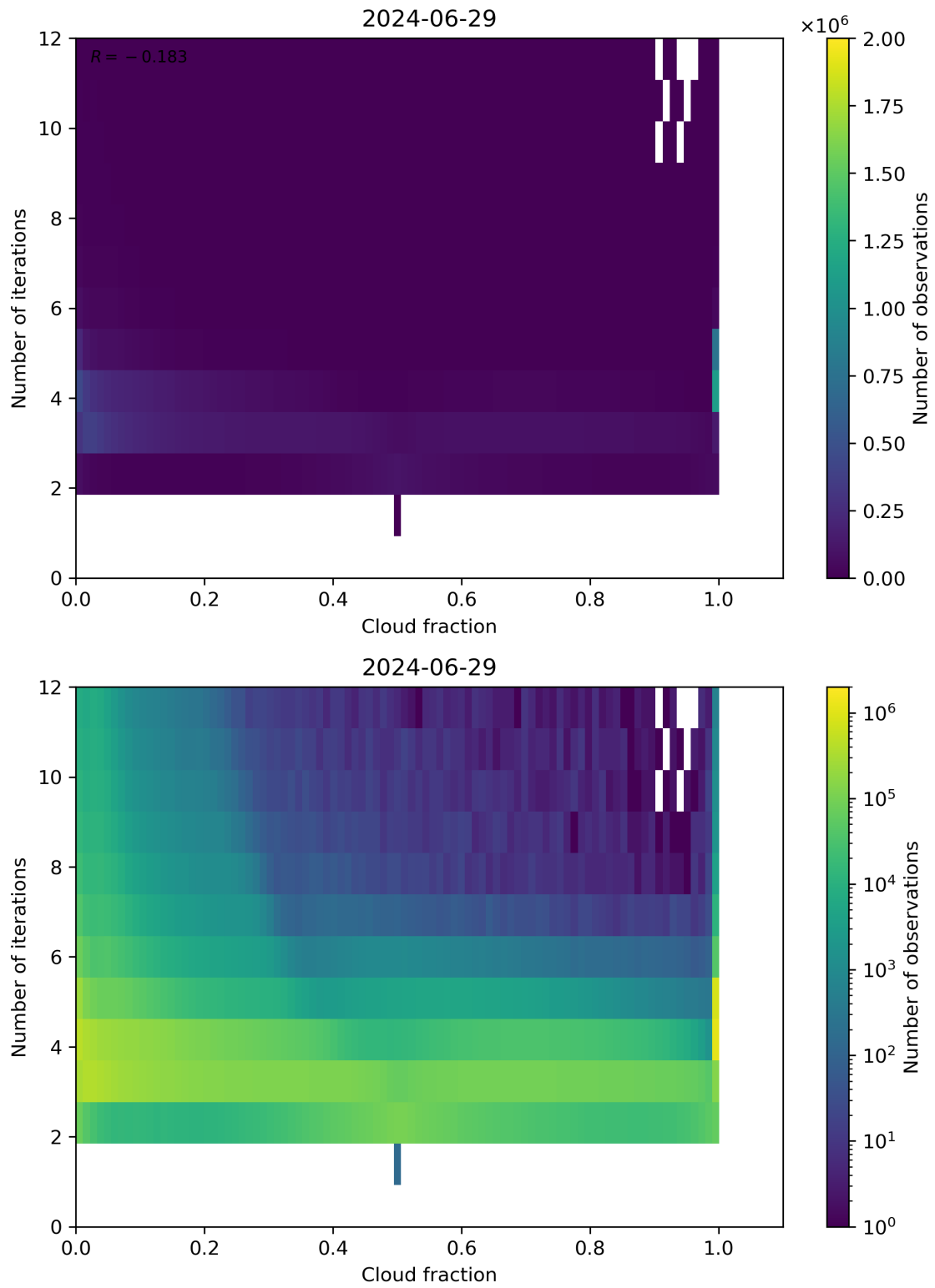
Figure 73: Scatter density plot of “Cloud fraction” against “Number of iterations” for 2024-06-29 to 2024-06-30.
