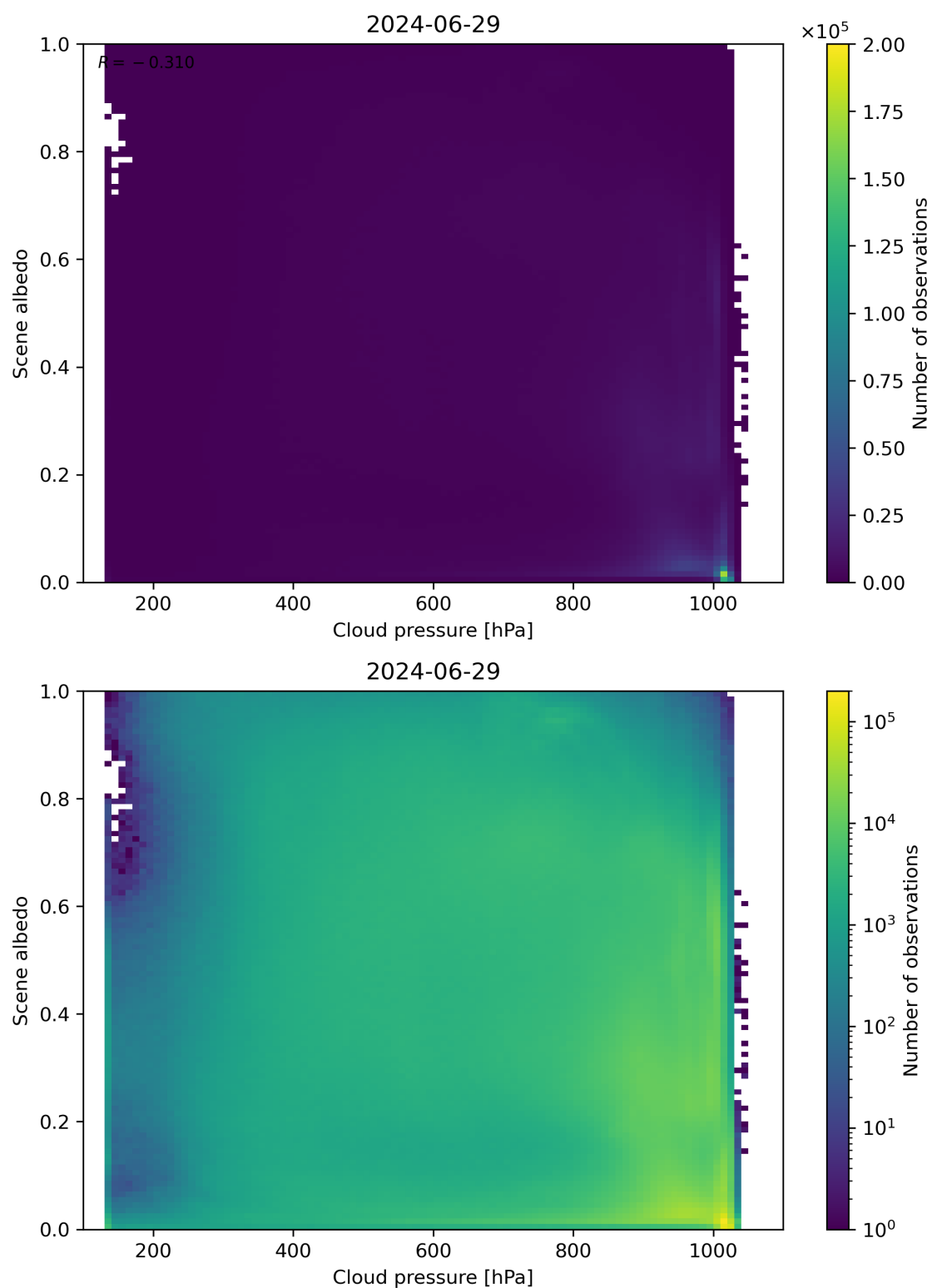
Figure 83: Scatter density plot of “Cloud pressure” against “Scene albedo” for 2024-06-29 to 2024-06-30.
