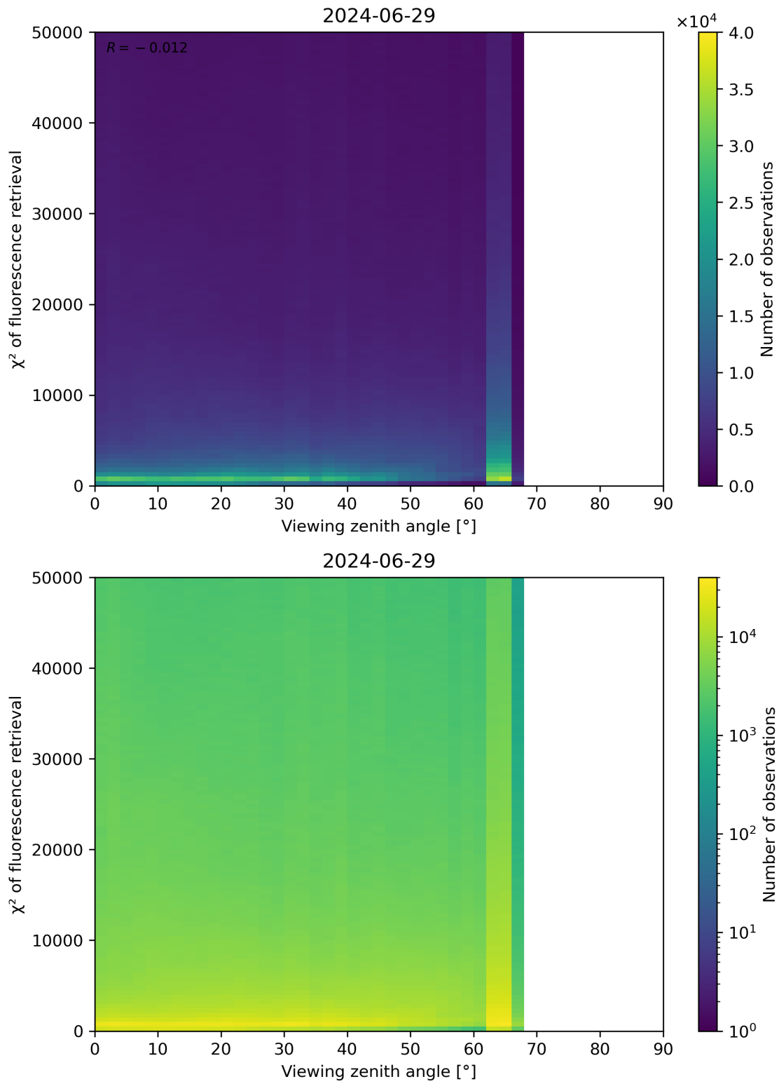
Figure 119: Scatter density plot of “Viewing zenith angle” against “ \chi^2 of fluorescence retrieval” for 2024-06-29 to 2024-06-30.
