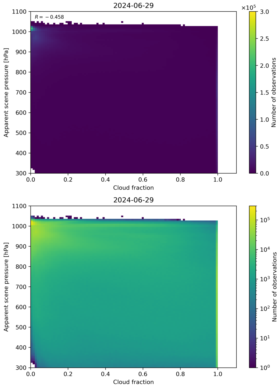
Figure 70: Scatter density plot of “Cloud fraction” against “Apparent scene pressure” for 2024-06-29 to 2024-06-30.
