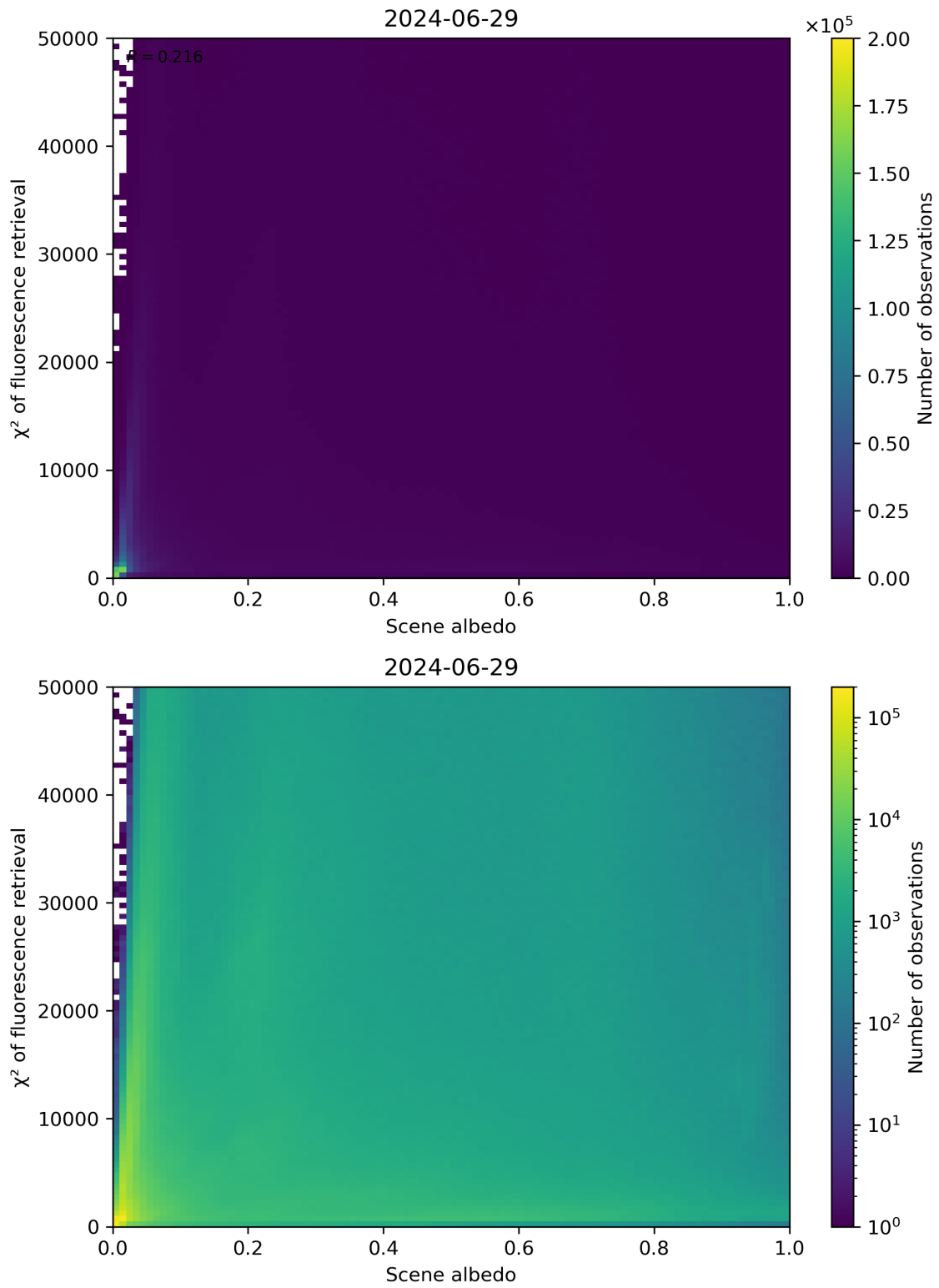
Figure 103: Scatter density plot of “Scene albedo” against “ \chi^2 of fluorescence retrieval” for 2024-06-29 to 2024-06-30.
