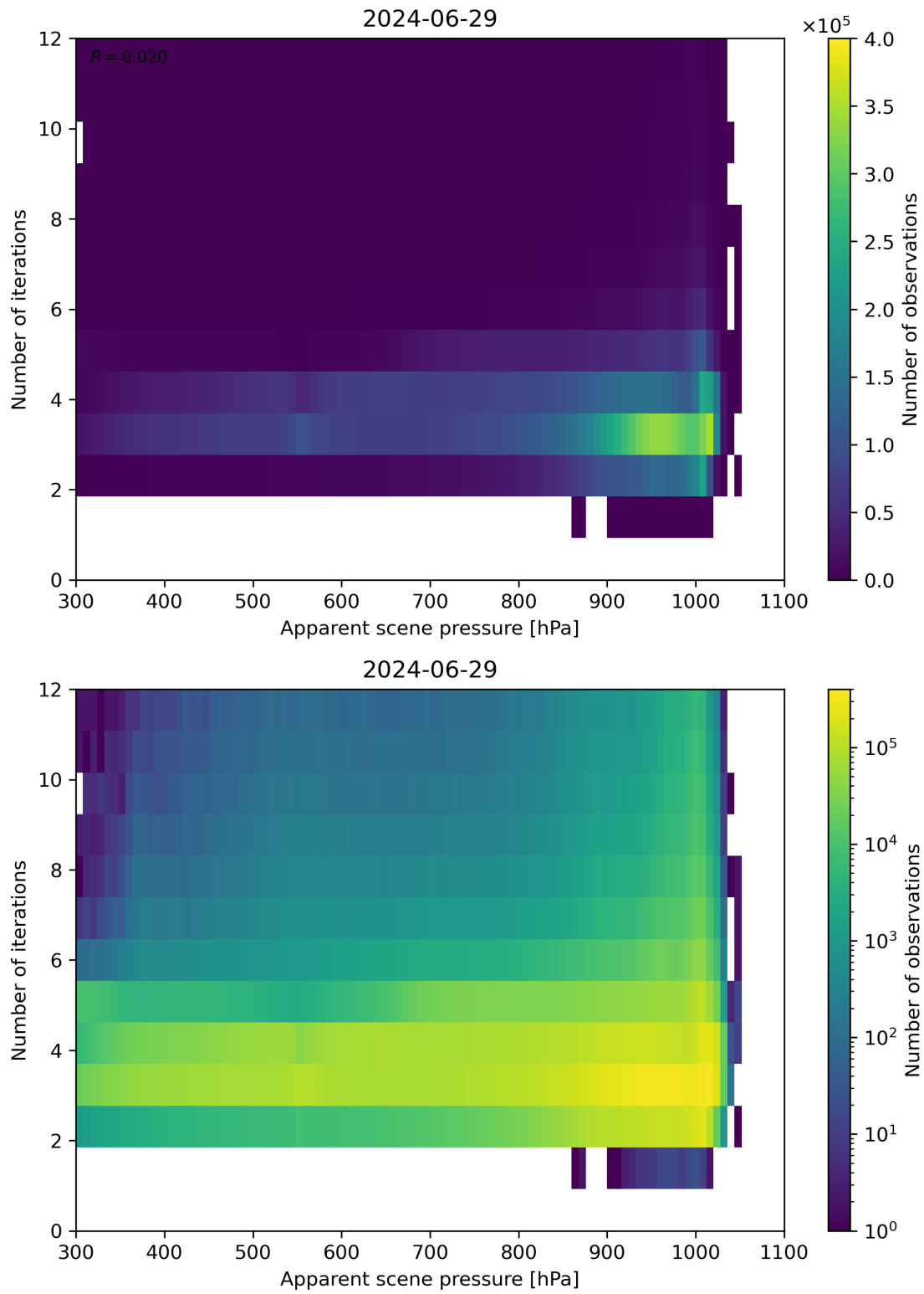
Figure 65: Scatter density plot of “Apparent scene pressure” against “Number of iterations” for 2024-06-29 to 2024-06-30.
