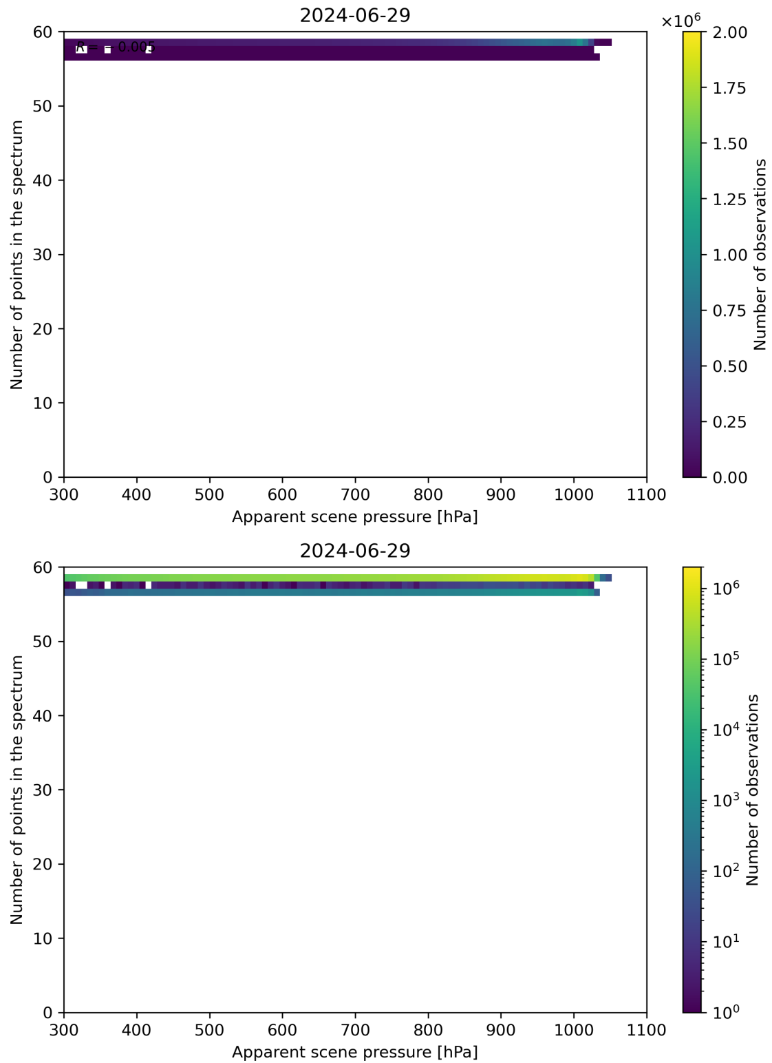
Figure 66: Scatter density plot of “Apparent scene pressure” against “Number of points in the spectrum” for 2024-06-29 to 2024-06-30.
