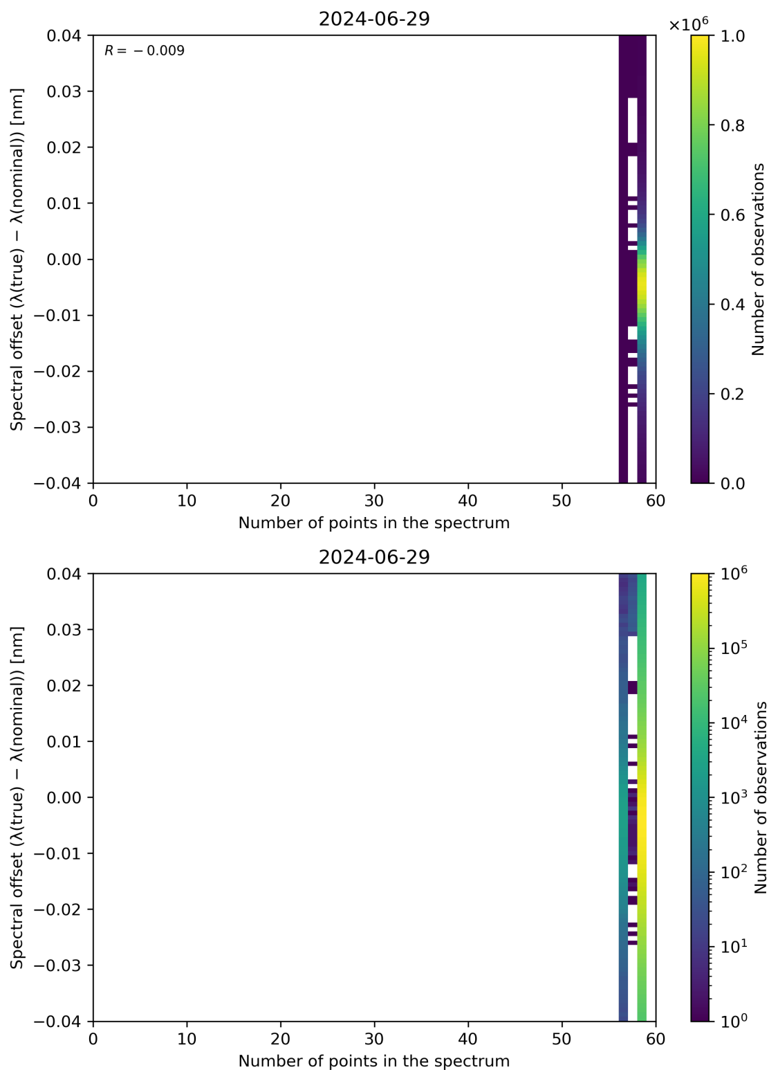
Figure 101: Scatter density plot of “Number of points in the spectrum” against “Spectral offset ( \lambda(\text{true}) - \lambda(\text{nominal}) )” for 2024-06-29 to 2024-06-30.
