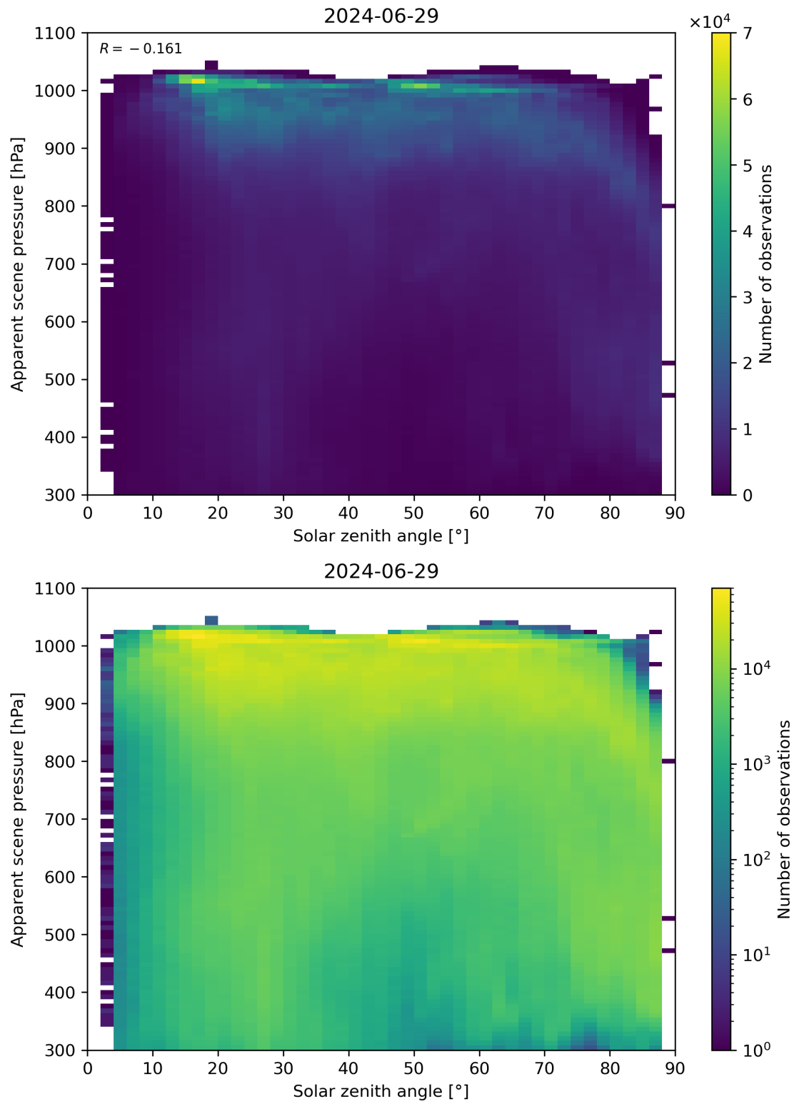
Figure 108: Scatter density plot of “Solar zenith angle” against “Apparent scene pressure” for 2024-06-29 to 2024-06-30.
