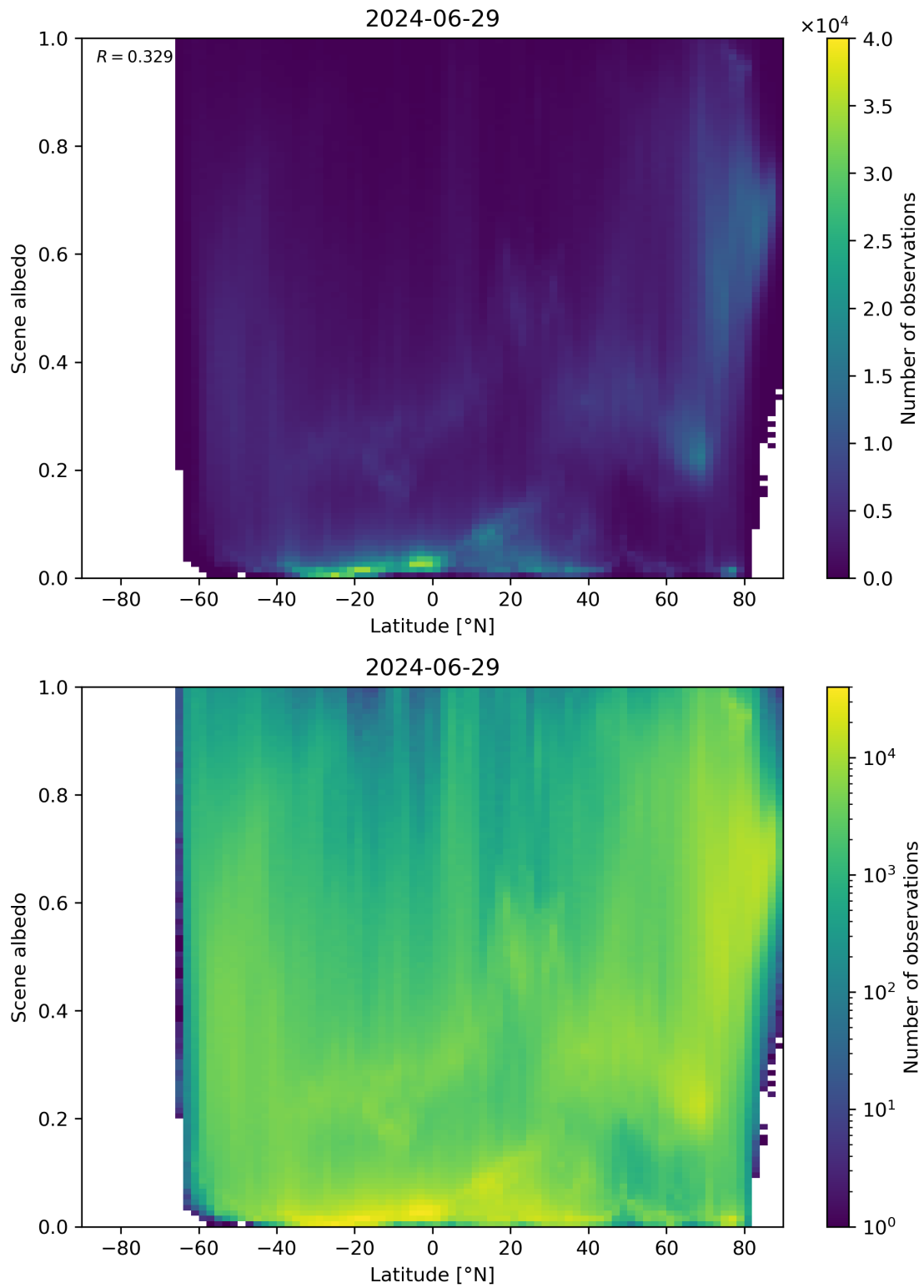
Figure 95: Scatter density plot of “Latitude” against “Scene albedo” for 2024-06-29 to 2024-06-30.
