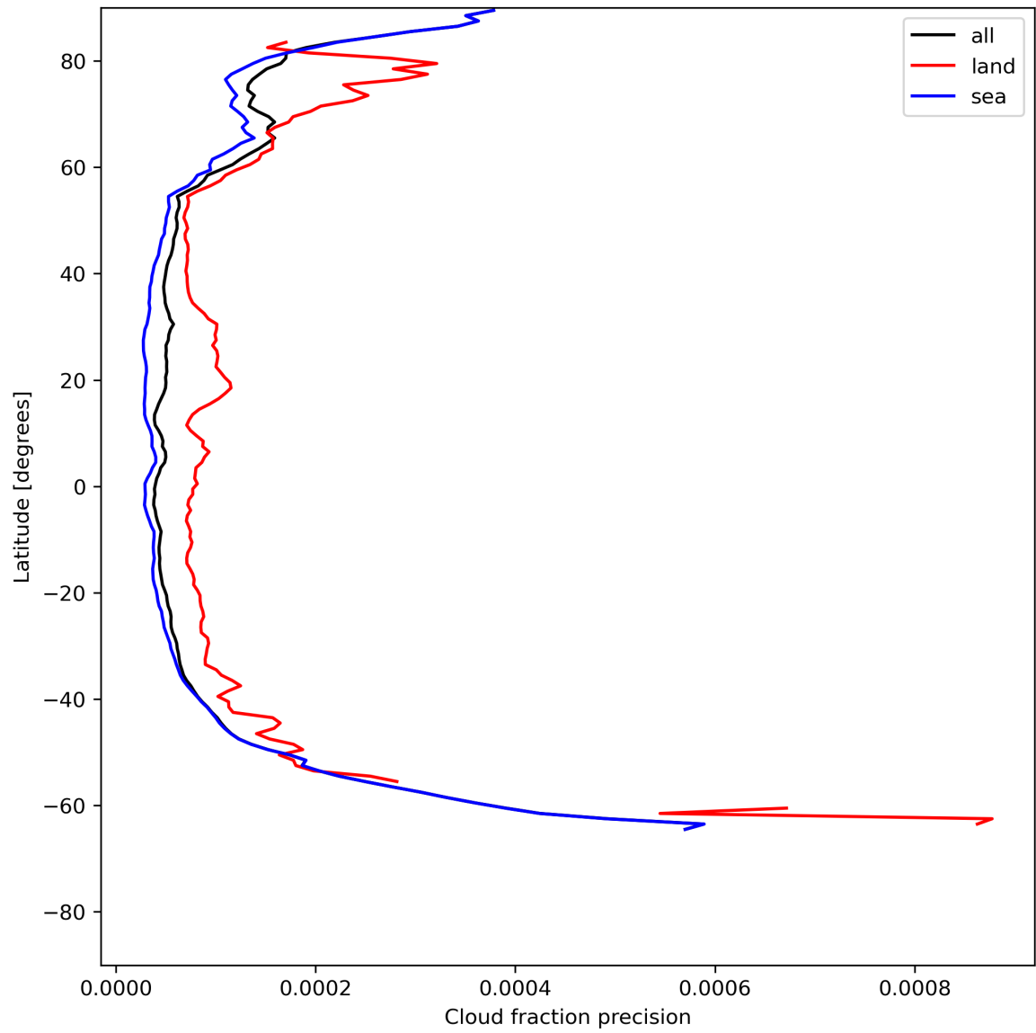
Figure 16: Zonal average of “Cloud fraction precision” for 2024-06-29 to 2024-06-30.
