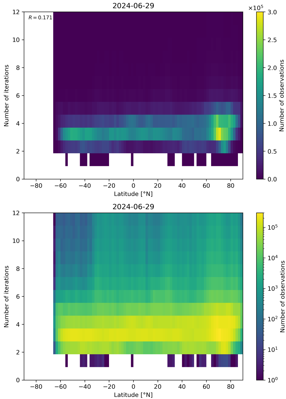
Figure 93: Scatter density plot of “Latitude” against “Number of iterations” for 2024-06-29 to 2024-06-30.
