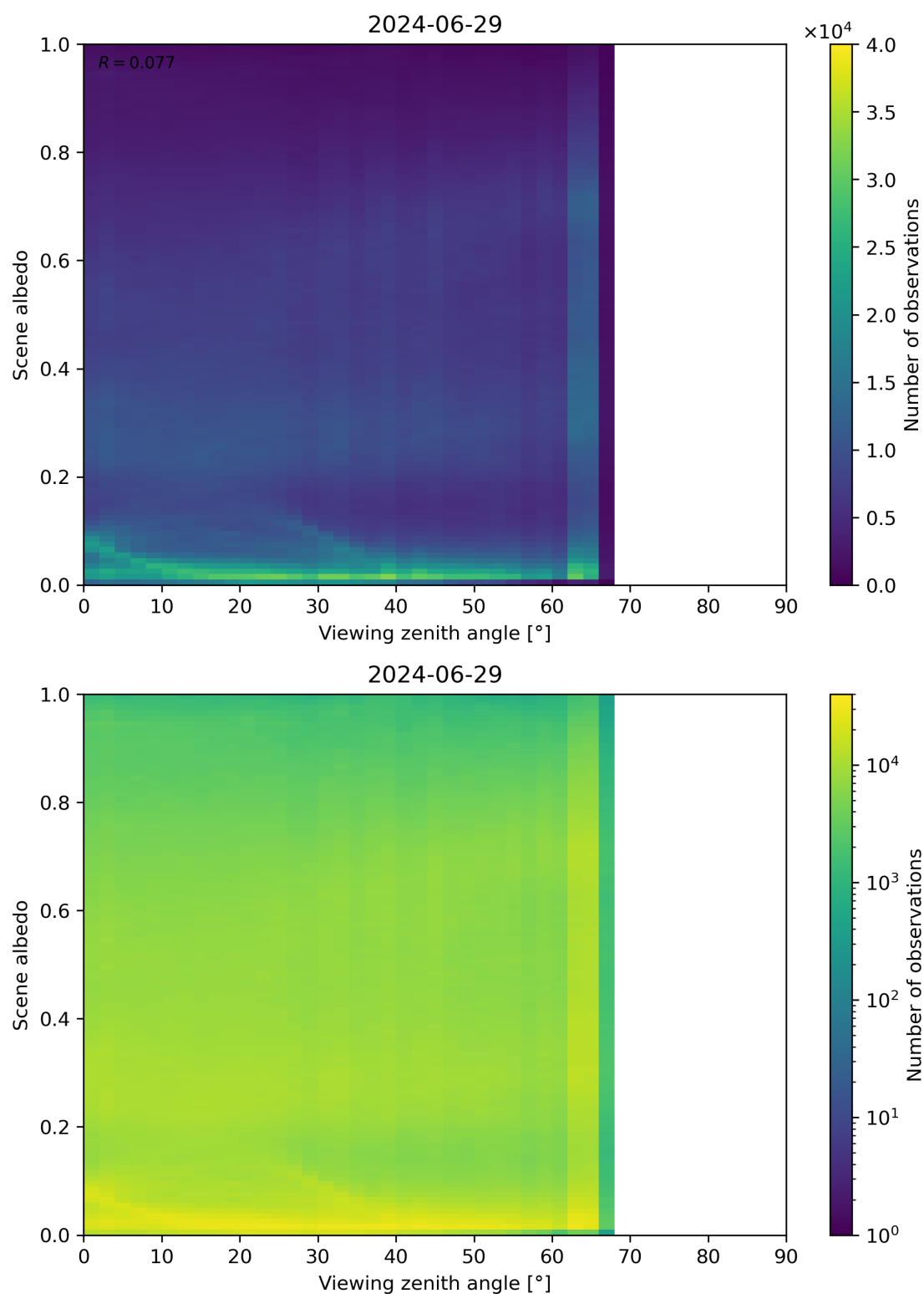
Figure 126: Scatter density plot of “Viewing zenith angle” against “Scene albedo” for 2024-06-29 to 2024-06-30.
