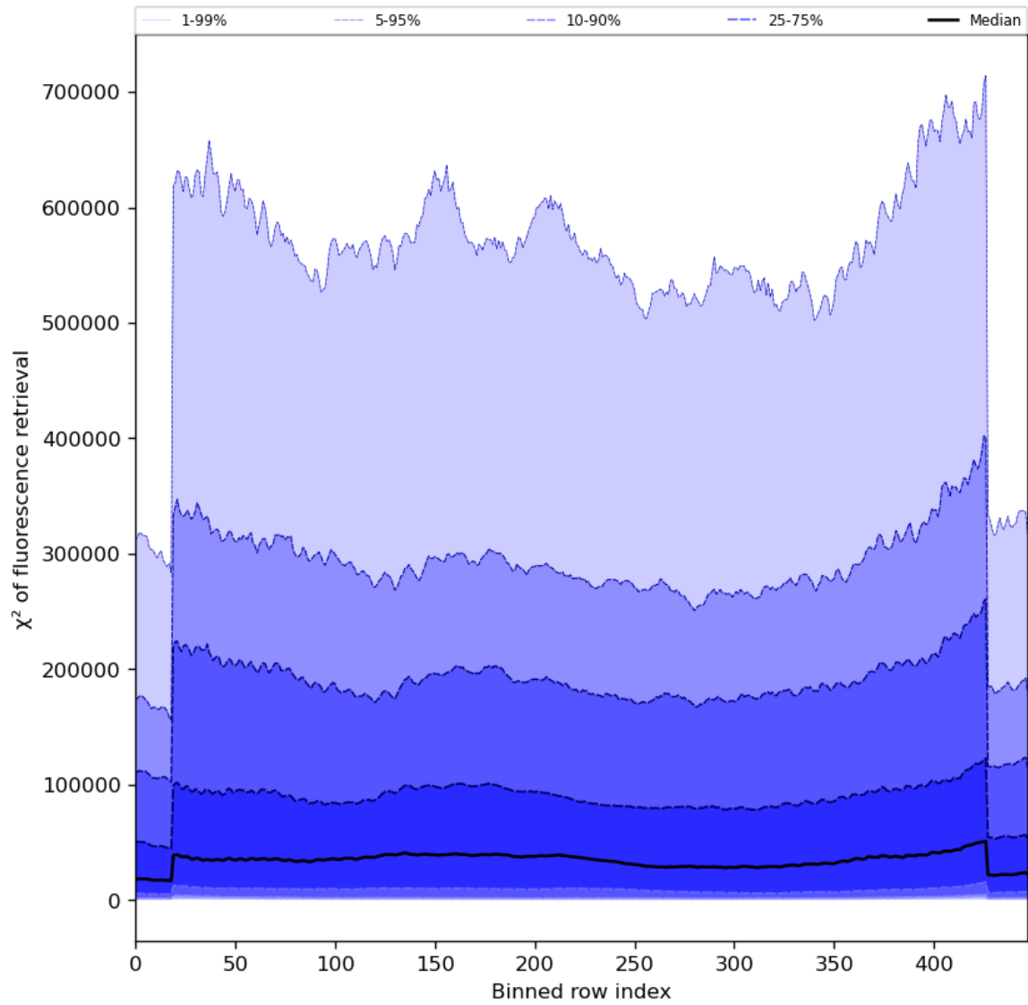
Figure 59: Along track statistics of “ \chi^2 of fluorescence retrieval” for 2024-06-29 to 2024-06-30
