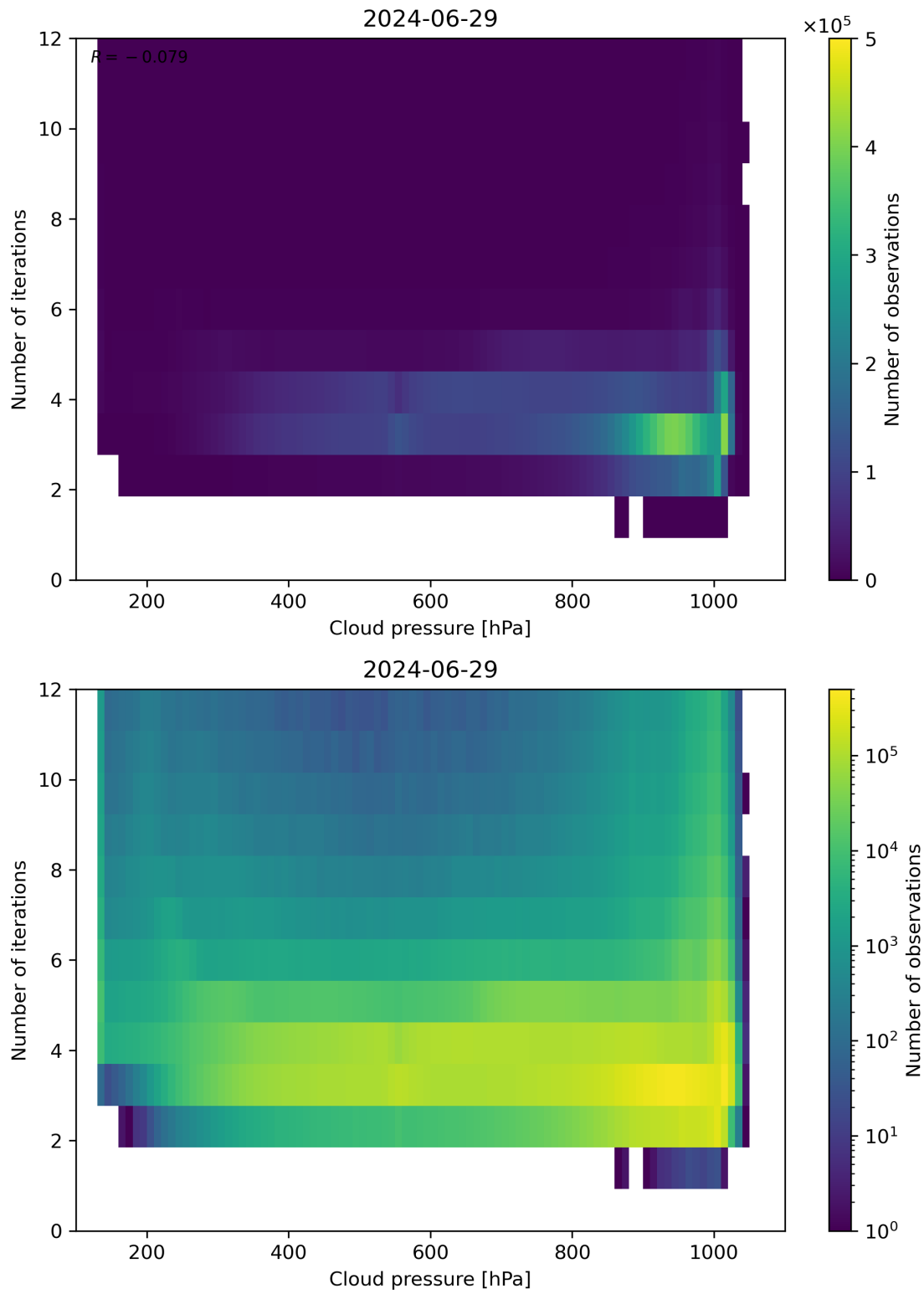
Figure 81: Scatter density plot of “Cloud pressure” against “Number of iterations” for 2024-06-29 to 2024-06-30.
