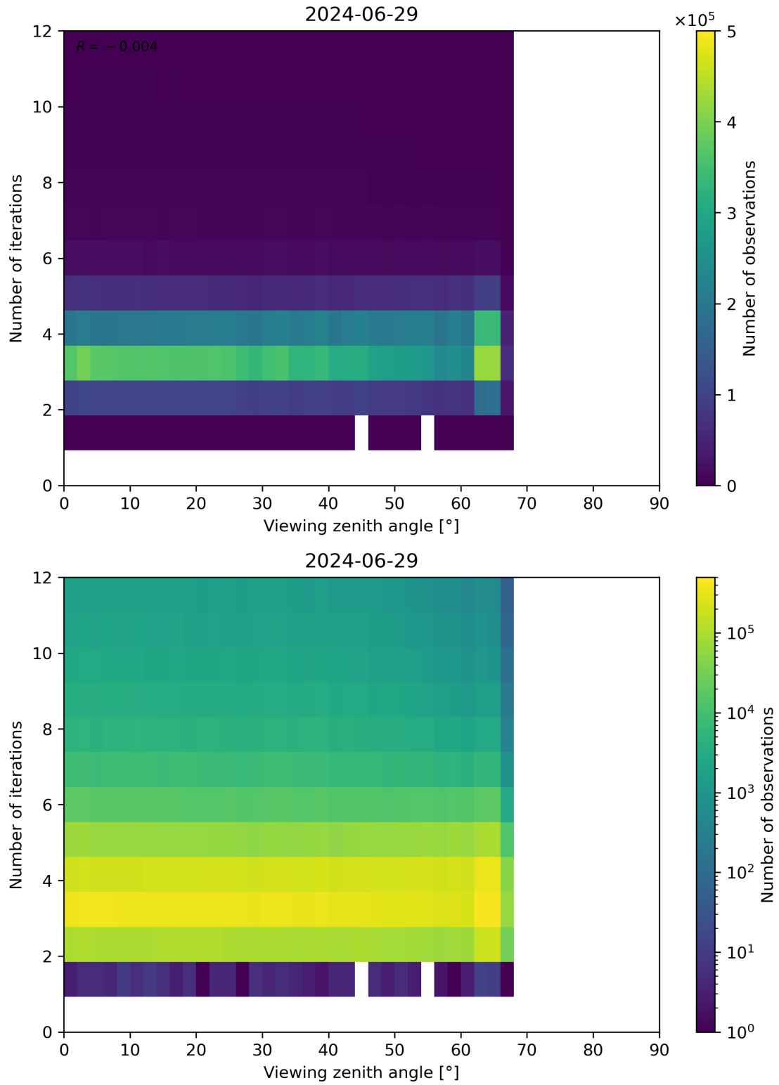
Figure 124: Scatter density plot of “Viewing zenith angle” against “Number of iterations” for 2024-06-29 to 2024-06-30.
