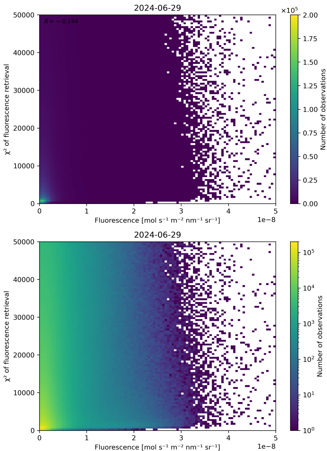
Figure 85: Scatter density plot of “Fluorescence” against “ \chi^2 of fluorescence retrieval” for 2024-06-29 to 2024-06-30.
