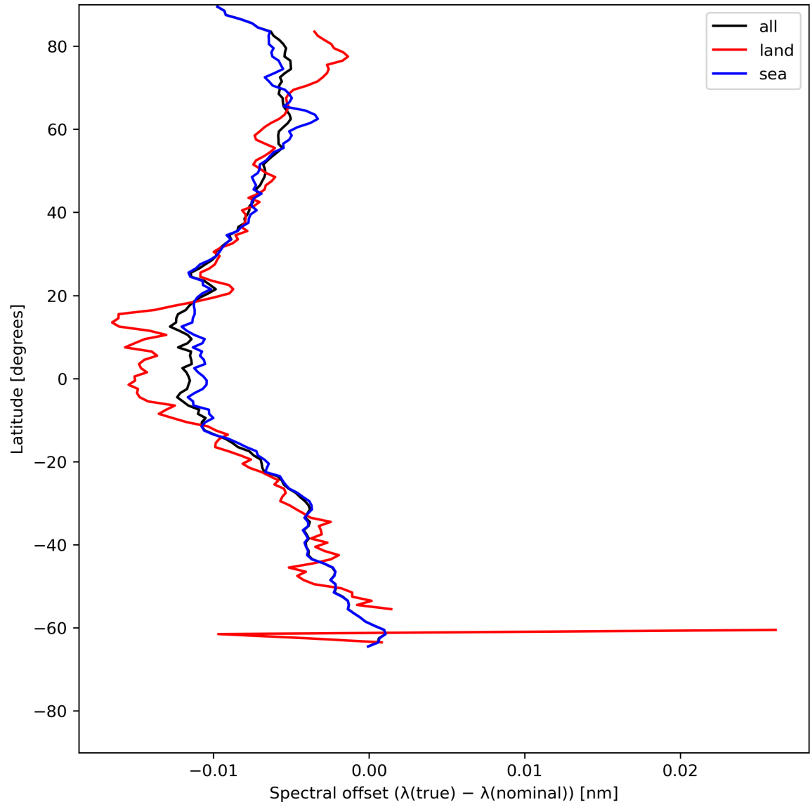
Figure 28: Zonal average of “Spectral offset ( \lambda(\text{true}) - \lambda(\text{nominal}) )” for 2024-06-29 to 2024-06-30.
