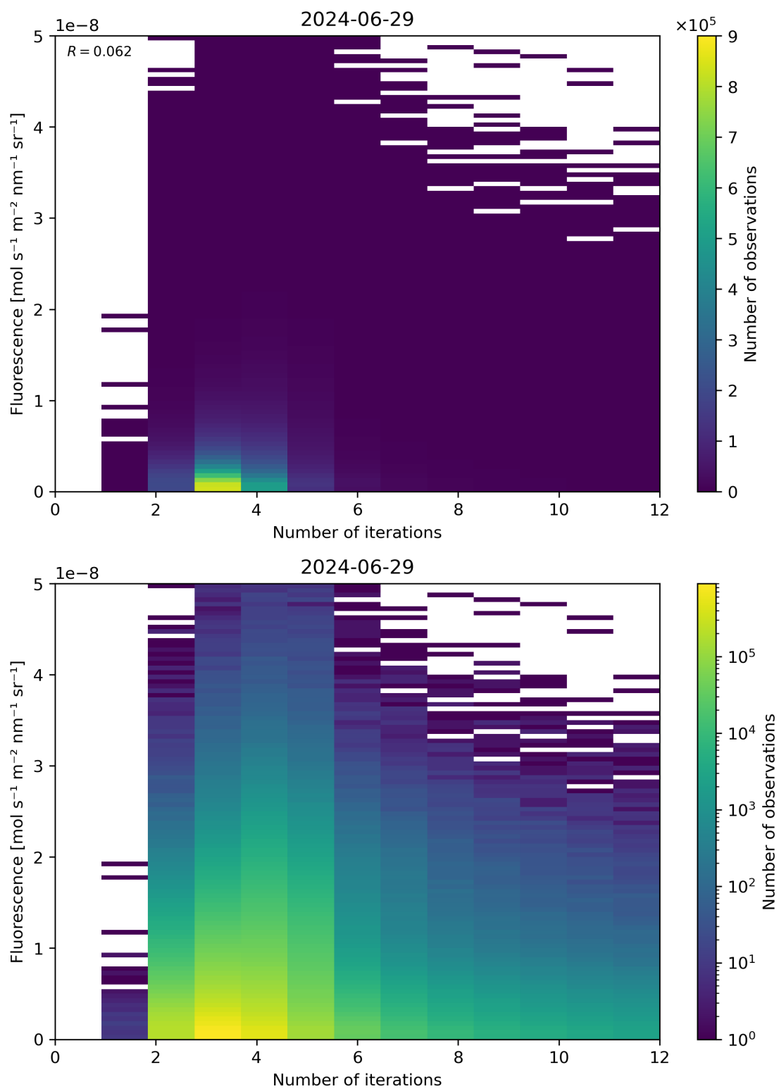
Figure 98: Scatter density plot of “Number of iterations” against “Fluorescence” for 2024-06-29 to 2024-06-30.
