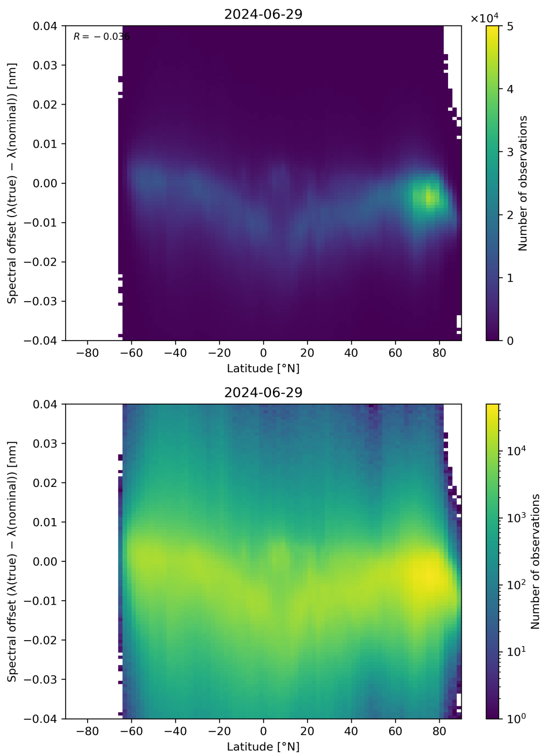
Figure 96: Scatter density plot of “Latitude” against “Spectral offset ( \lambda(\text{true}) - \lambda(\text{nominal}) )” for 2024-06-29 to 2024-06-30.
