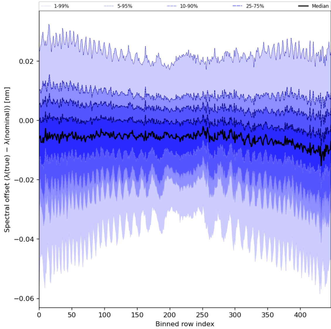
Figure 62: Along track statistics of “Spectral offset ( \lambda(\text{true}) - \lambda(\text{nominal}) )” for 2024-06-29 to 2024-06-30
