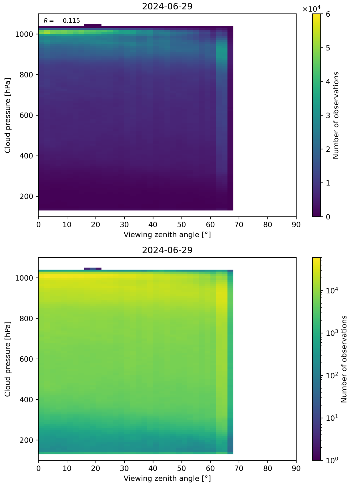
Figure 121: Scatter density plot of “Viewing zenith angle” against “Cloud pressure” for 2024-06-29 to 2024-06-30.
