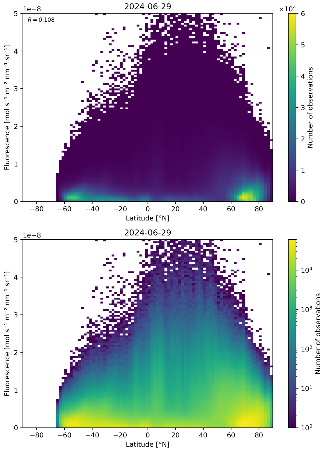
Figure 92: Scatter density plot of “Latitude” against “Fluorescence” for 2024-06-29 to 2024-06-30.
