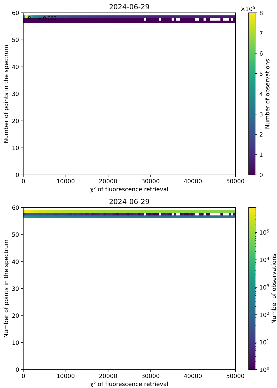
Figure 68: Scatter density plot of “ \chi^2 of fluorescence retrieval” against “Number of points in the spectrum” for 2024-06-29 to 2024-06-30.
