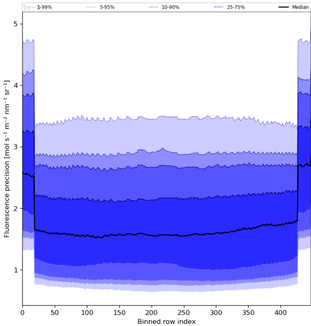
Figure 58: Along track statistics of “Fluorescence precision” for 2024-06-29 to 2024-06-30
