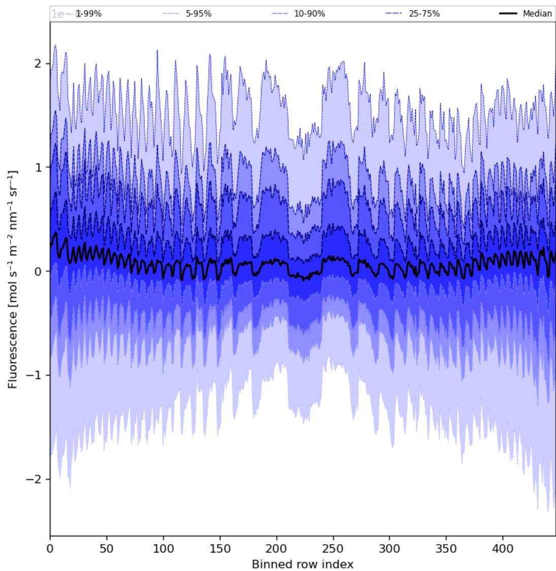
Figure 57: Along track statistics of “Fluorescence” for 2024-06-29 to 2024-06-30
