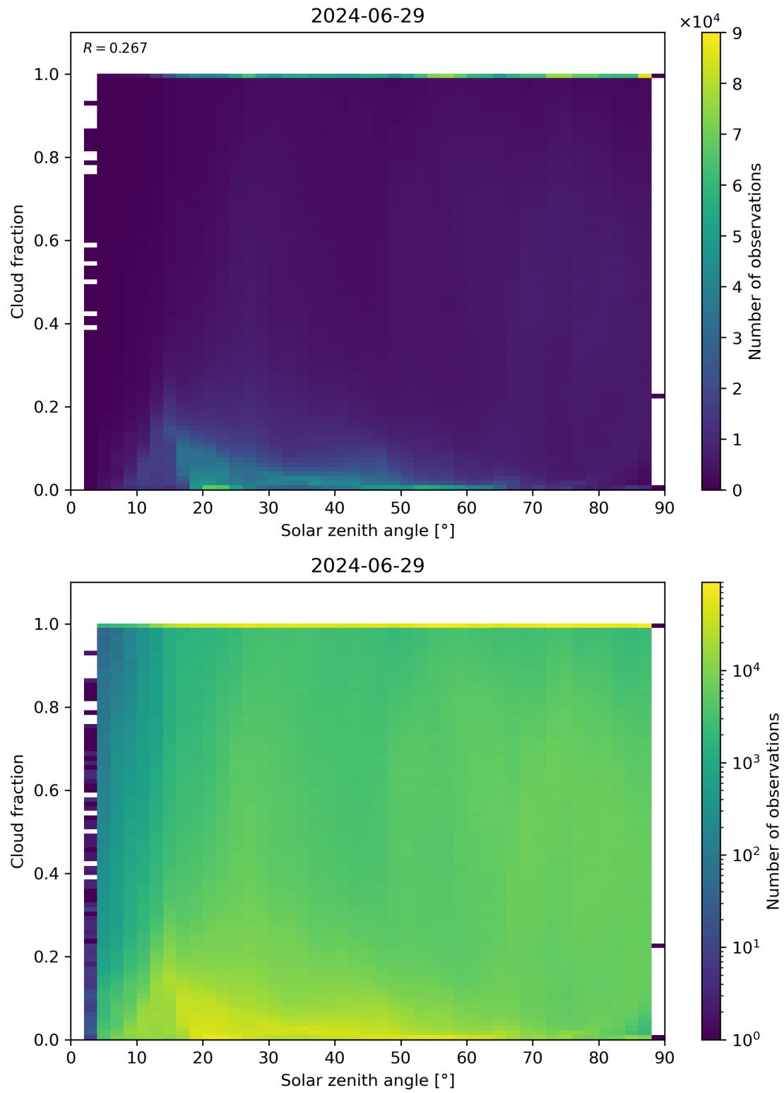
Figure 110: Scatter density plot of “Solar zenith angle” against “Cloud fraction” for 2024-06-29 to 2024-06-30.
