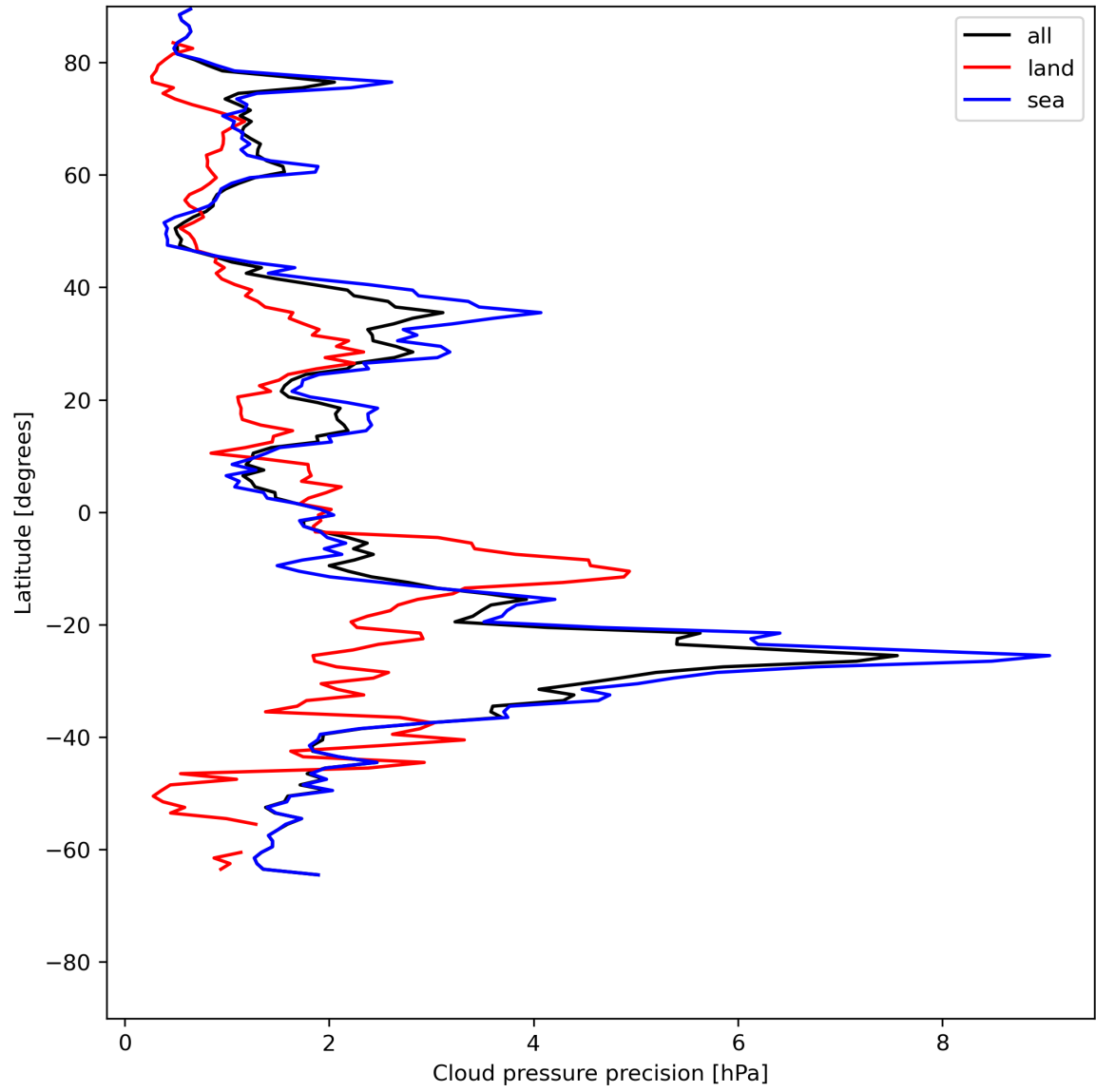
Figure 14: Zonal average of “Cloud pressure precision” for 2024-06-29 to 2024-06-30.
