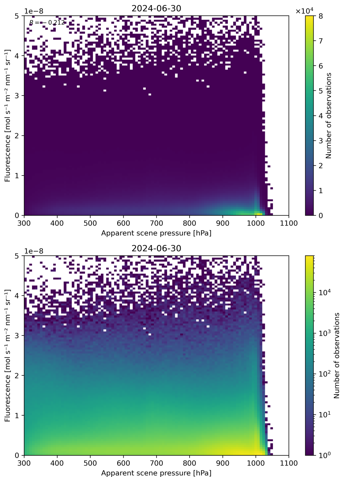
Figure 64: Scatter density plot of “Apparent scene pressure” against “Fluorescence” for 2024-06-29 to 2024-07-01.
