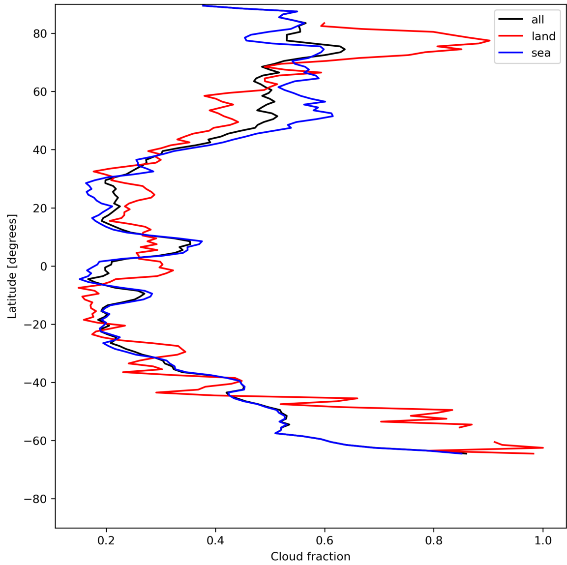
Figure 15: Zonal average of “Cloud fraction” for 2024-06-29 to 2024-07-01.
