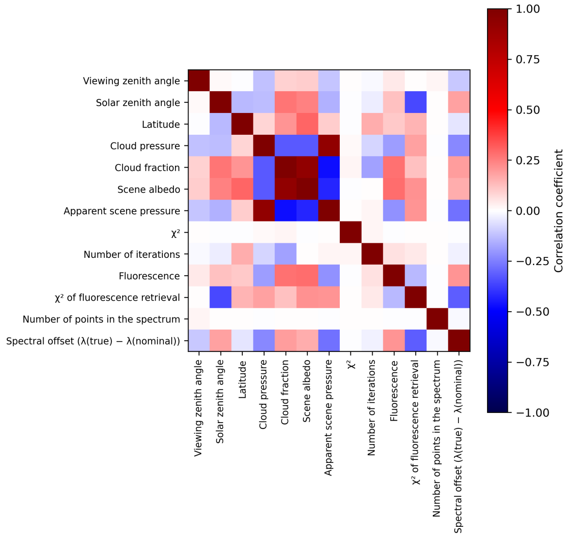
Figure 2: Map of correlation matrix for 2024-06-29 to 2024-07-01.
