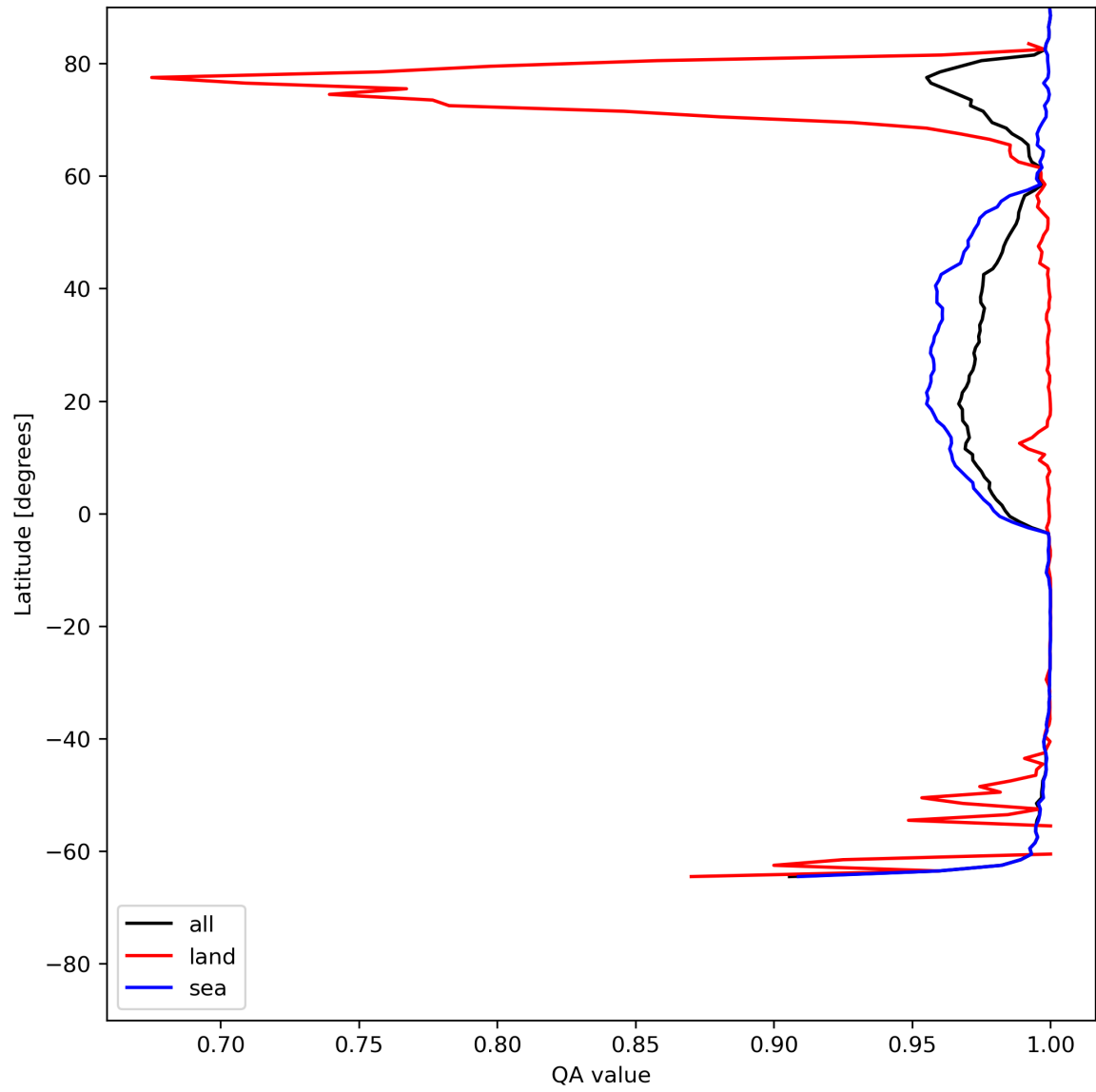
Figure 12: Zonal average of “QA value” for 2024-06-29 to 2024-07-01.
