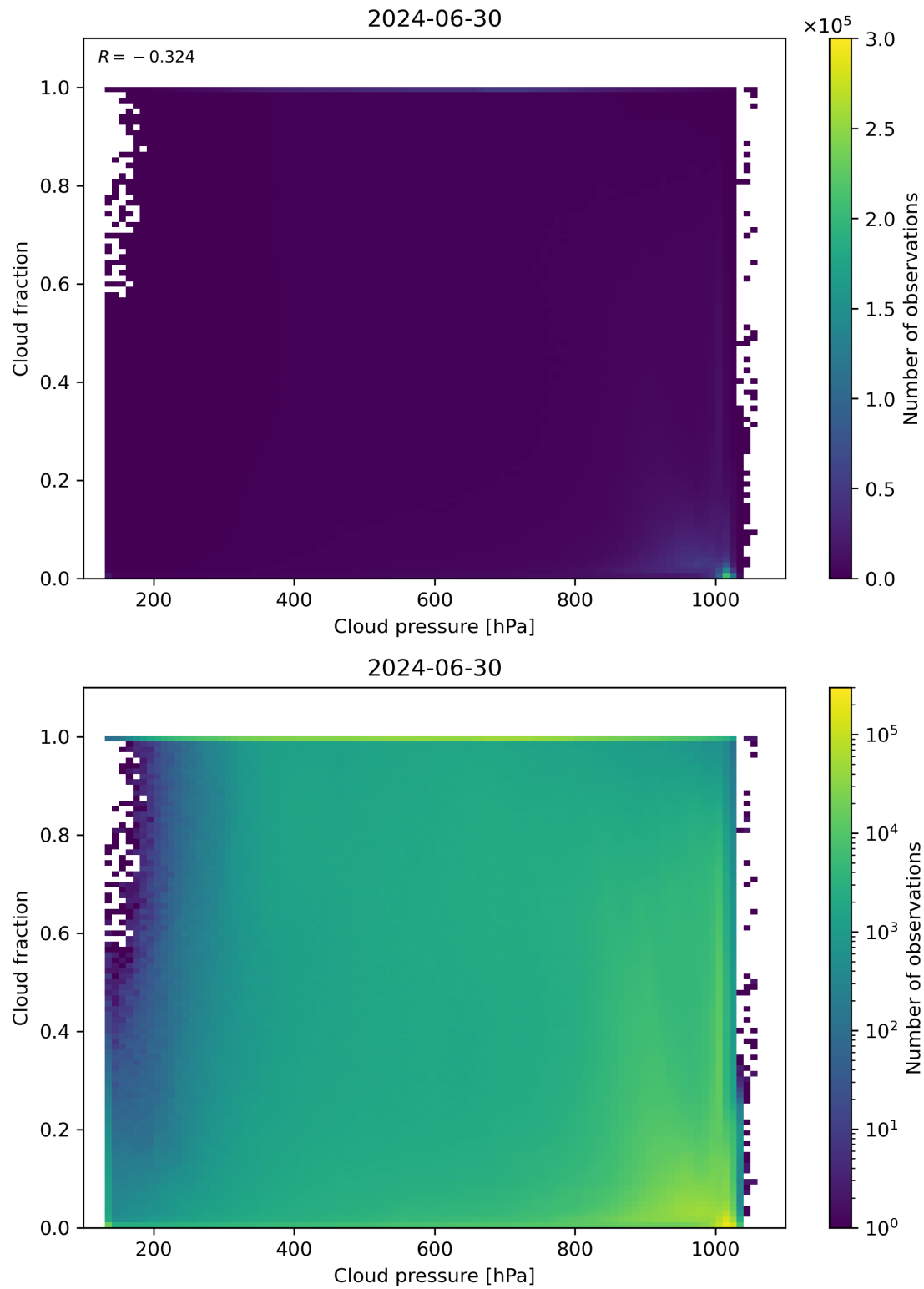
Figure 79: Scatter density plot of “Cloud pressure” against “Cloud fraction” for 2024-06-29 to 2024-07-01.
