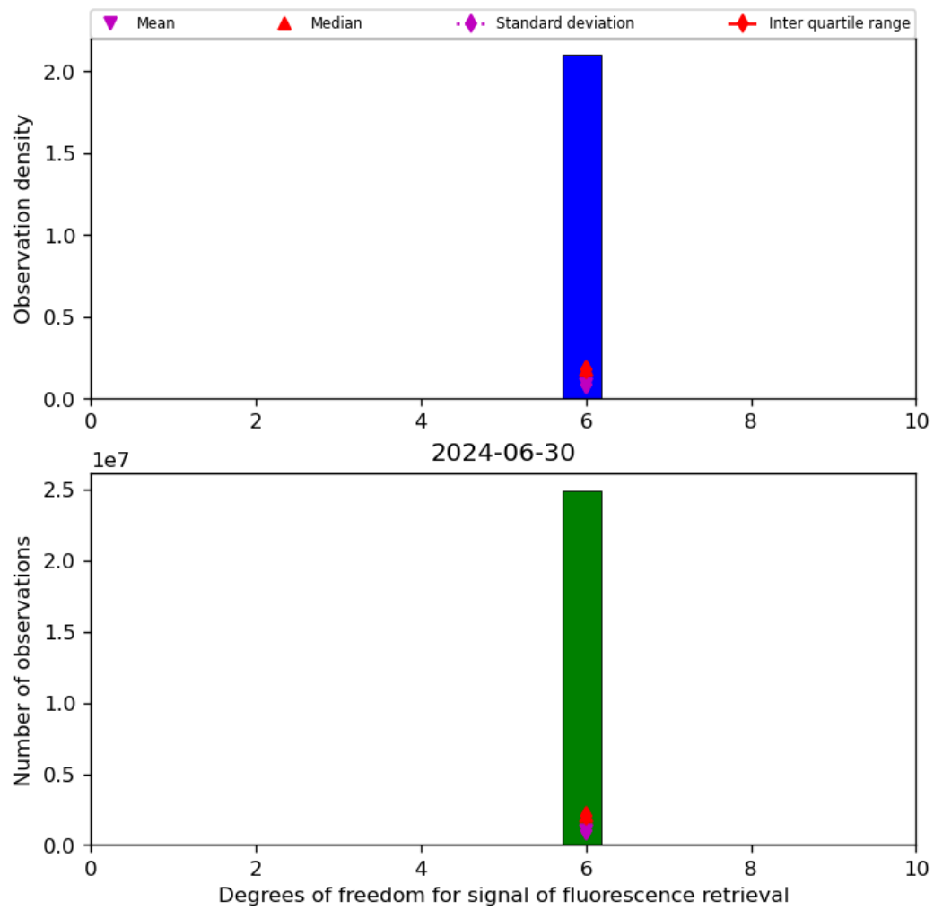
Figure 43: Histogram of “Degrees of freedom for signal of fluorescence retrieval” for 2024-06-29 to 2024-07-01
