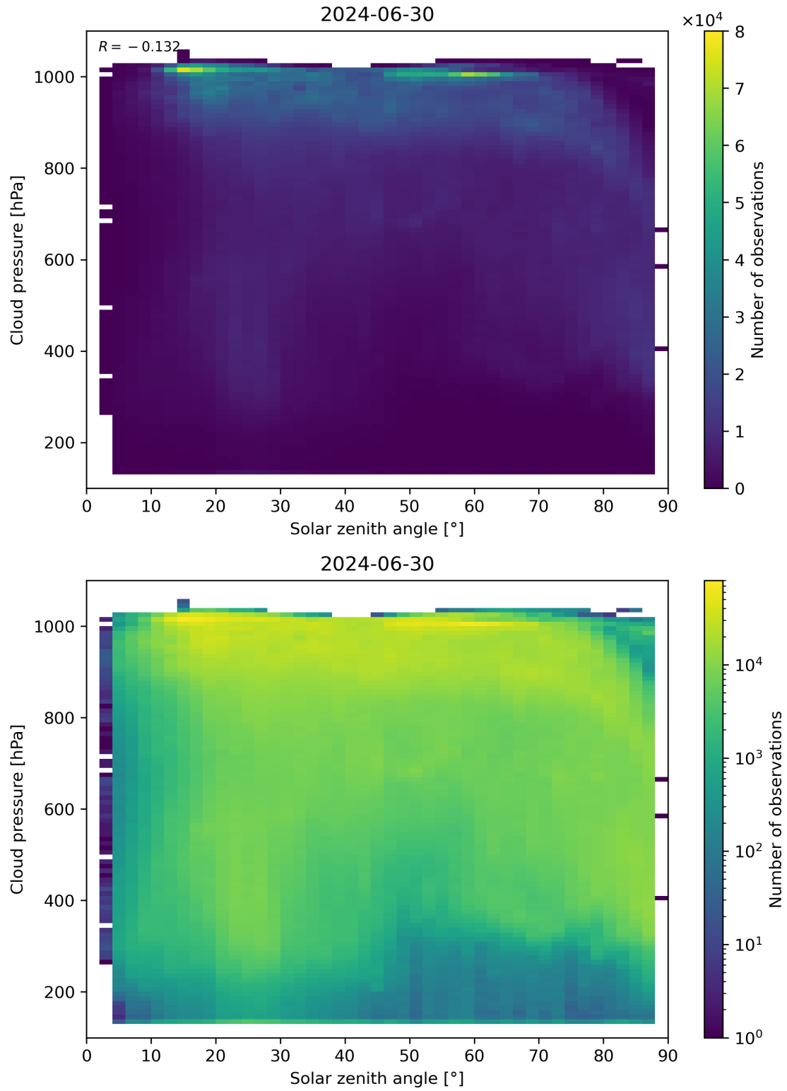
Figure 111: Scatter density plot of “Solar zenith angle” against “Cloud pressure” for 2024-06-29 to 2024-07-01.
