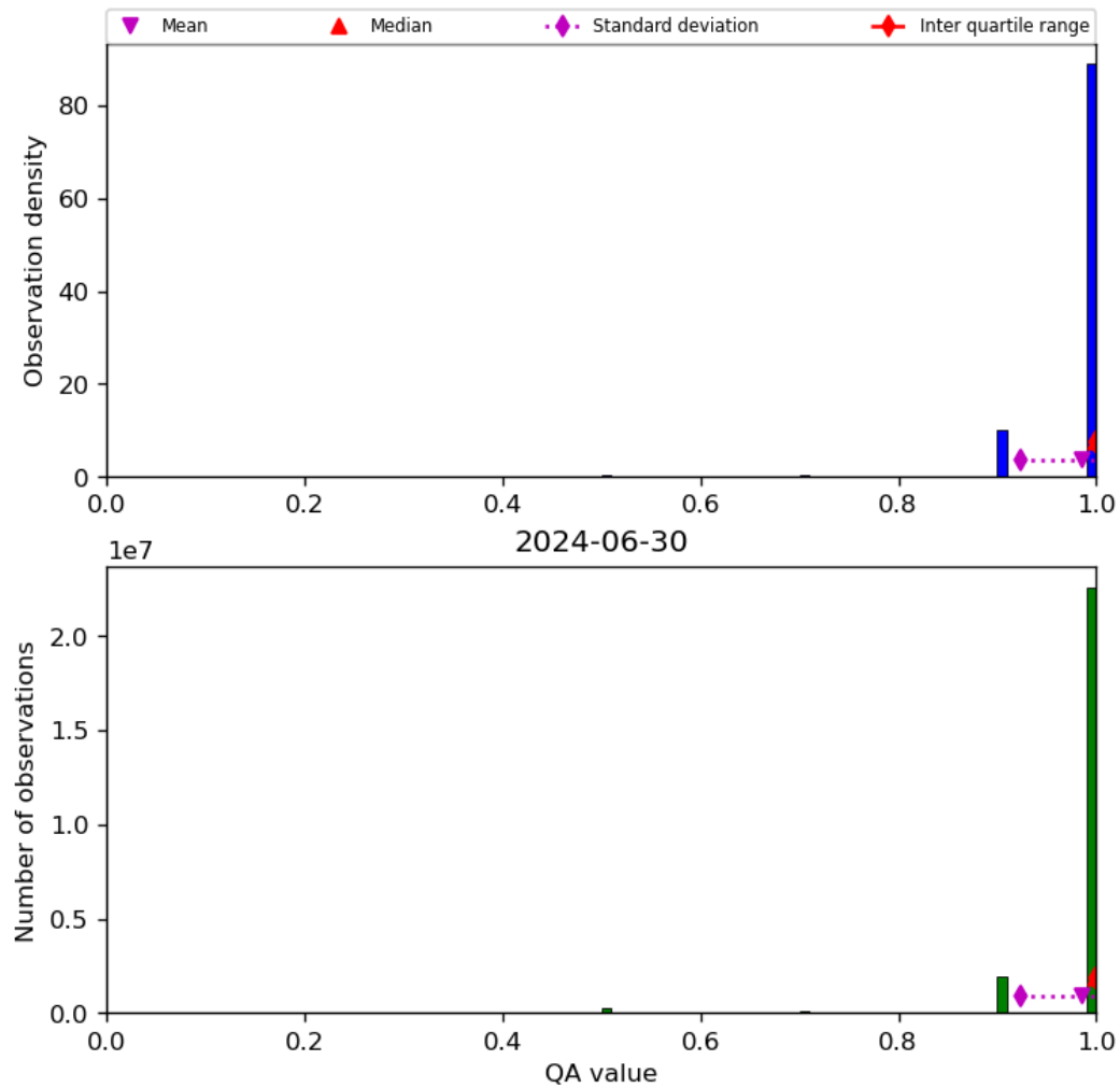
Figure 29: Histogram of “QA value” for 2024-06-29 to 2024-07-01
