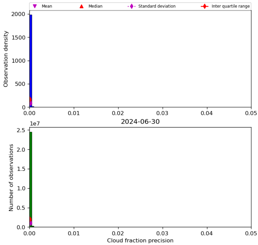
Figure 33: Histogram of “Cloud fraction precision” for 2024-06-29 to 2024-07-01
