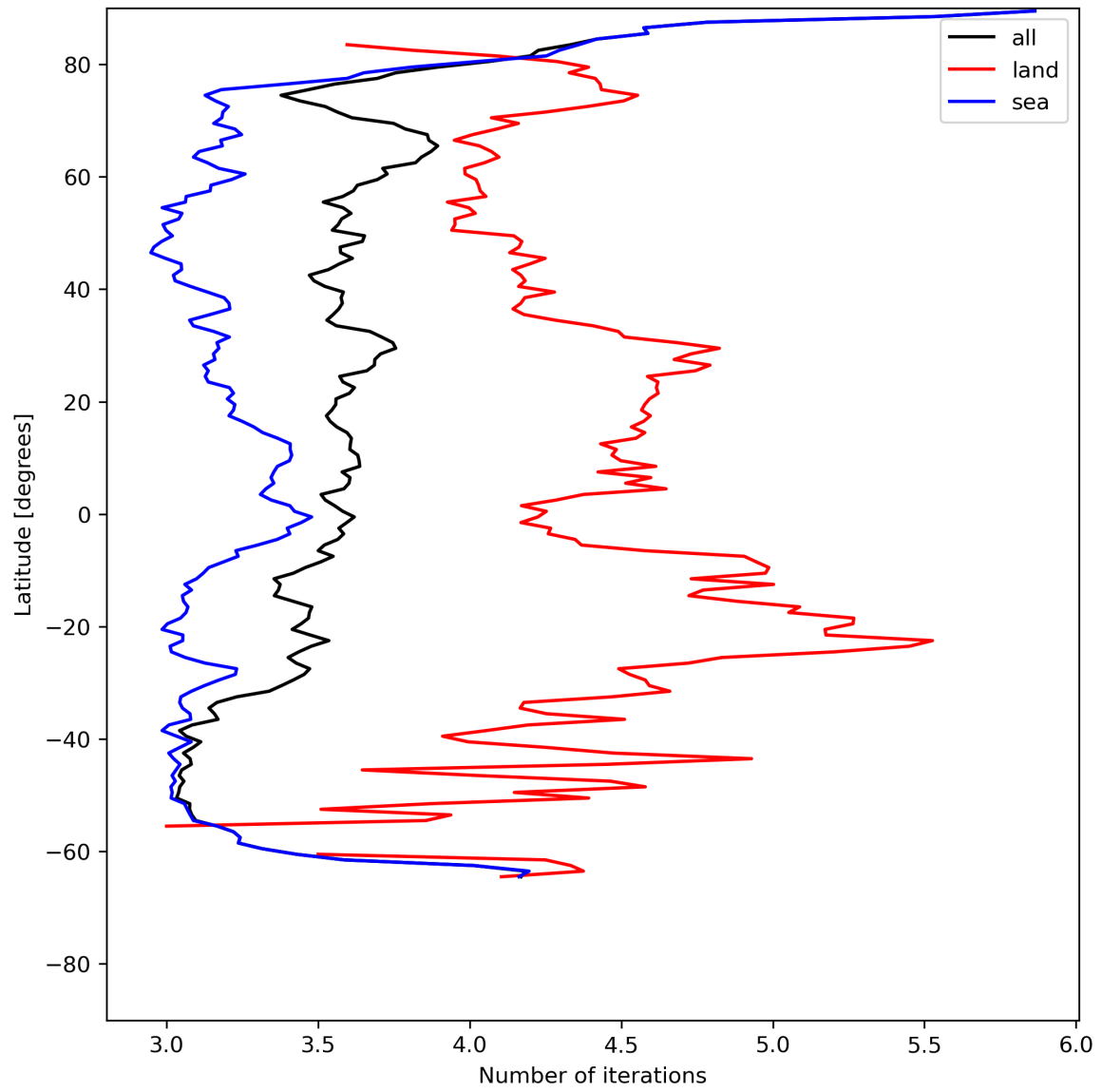
Figure 22: Zonal average of “Number of iterations” for 2024-06-29 to 2024-07-01.
