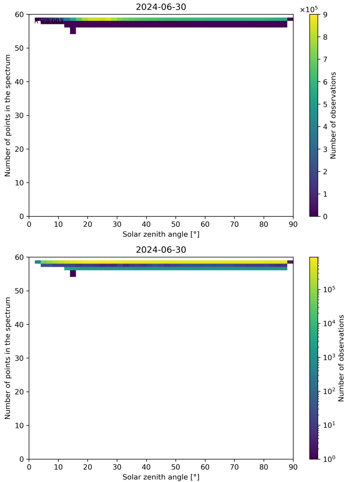
Figure 115: Scatter density plot of “Solar zenith angle” against “Number of points in the spectrum” for 2024-06-29 to 2024-07-01.
