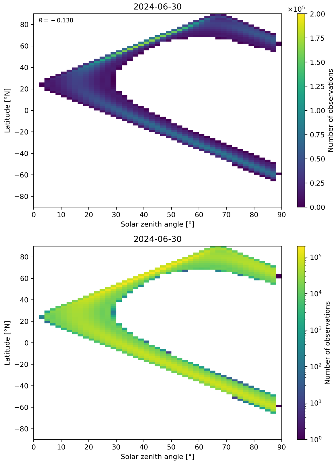
Figure 113: Scatter density plot of “Solar zenith angle” against “Latitude” for 2024-06-29 to 2024-07-01.
