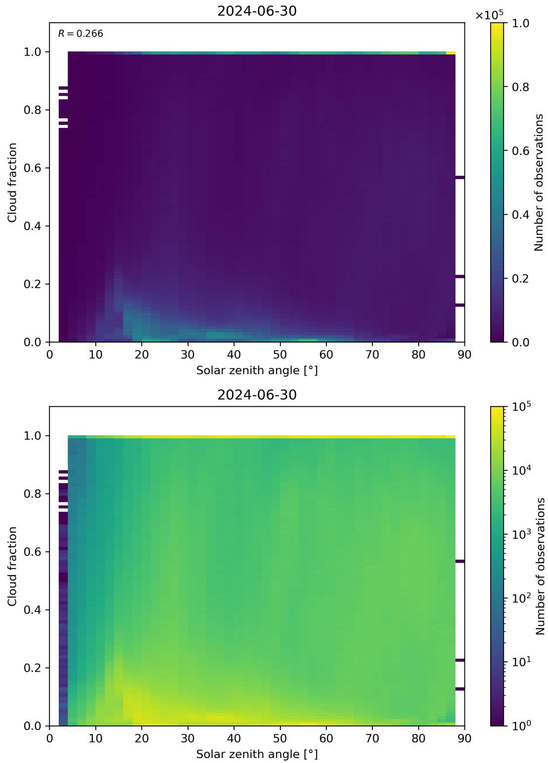
Figure 110: Scatter density plot of “Solar zenith angle” against “Cloud fraction” for 2024-06-29 to 2024-07-01.
