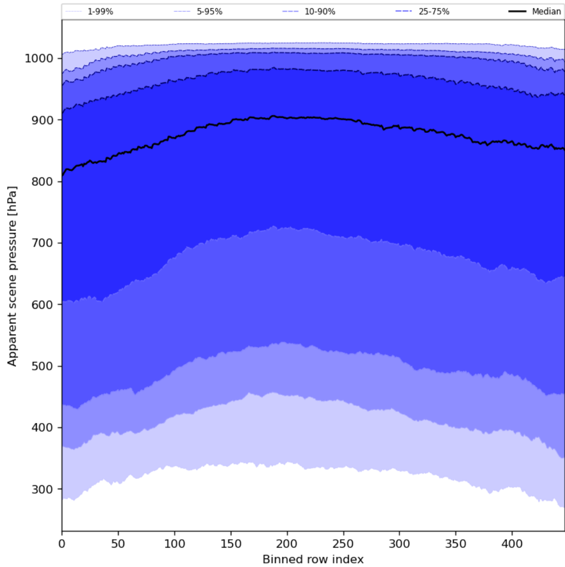
Figure 53: Along track statistics of “Apparent scene pressure” for 2024-06-29 to 2024-07-01
