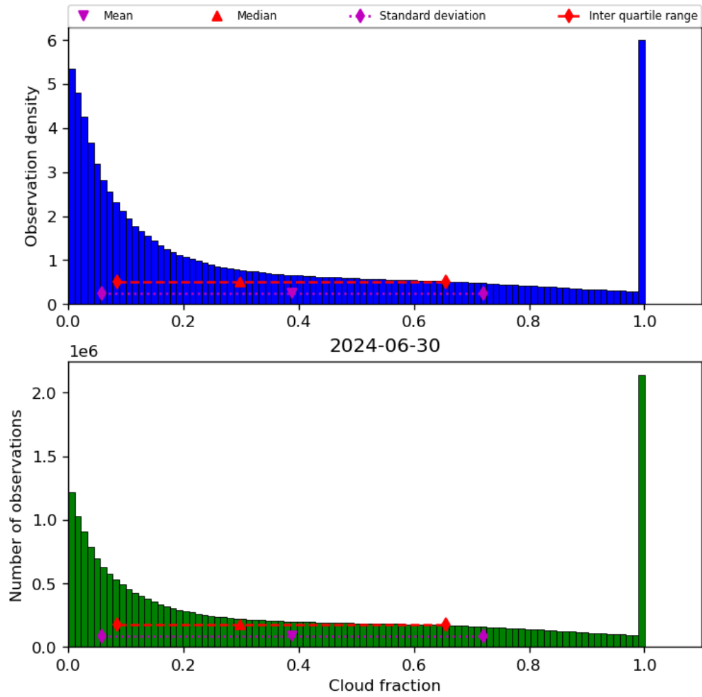
Figure 32: Histogram of “Cloud fraction” for 2024-06-29 to 2024-07-01
