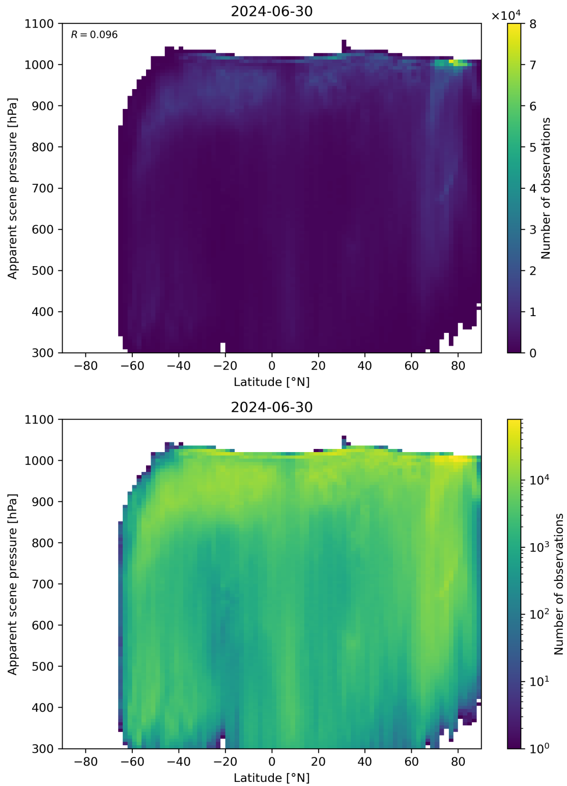
Figure 88: Scatter density plot of “Latitude” against “Apparent scene pressure” for 2024-06-29 to 2024-07-01.
