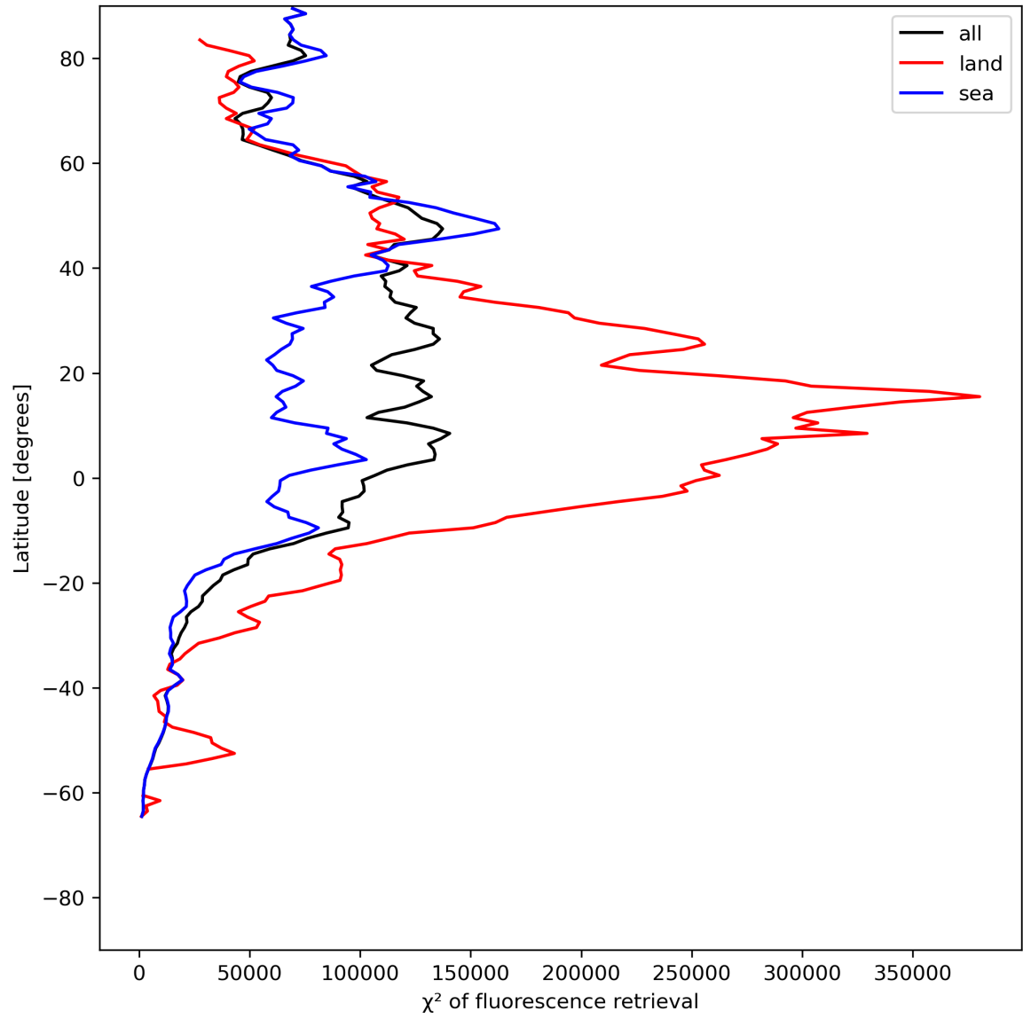
Figure 25: Zonal average of “ \chi^2 of fluorescence retrieval” for 2024-06-29 to 2024-07-01.
