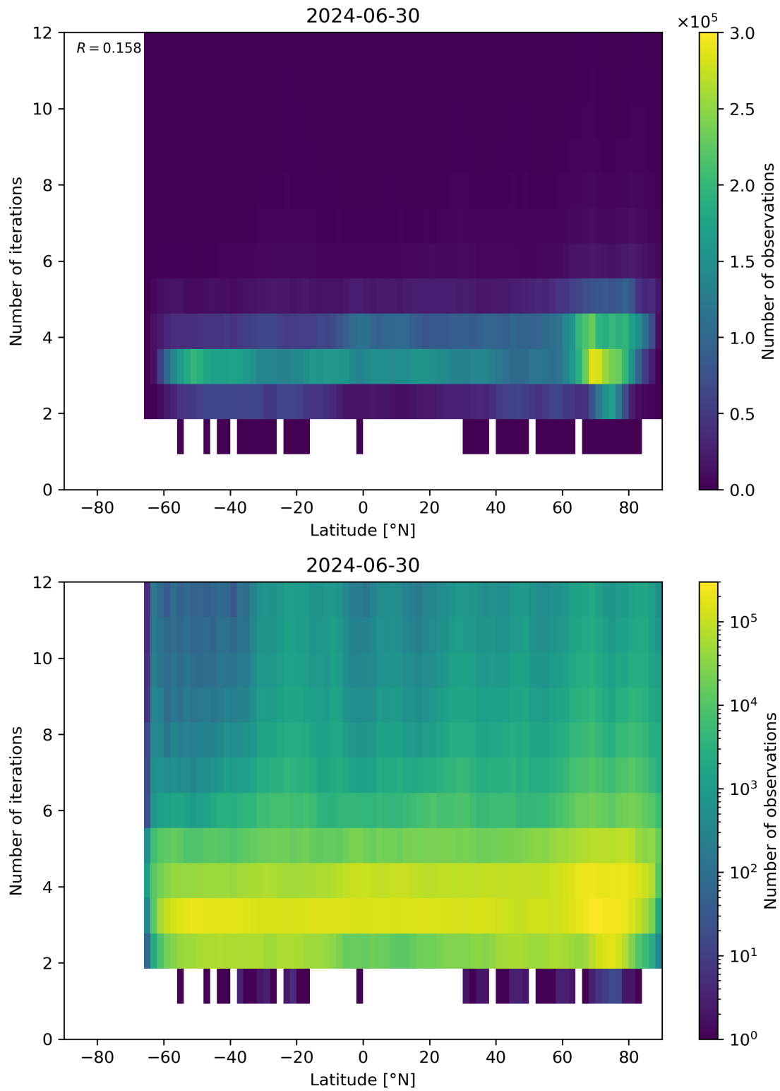
Figure 93: Scatter density plot of “Latitude” against “Number of iterations” for 2024-06-29 to 2024-07-01.
