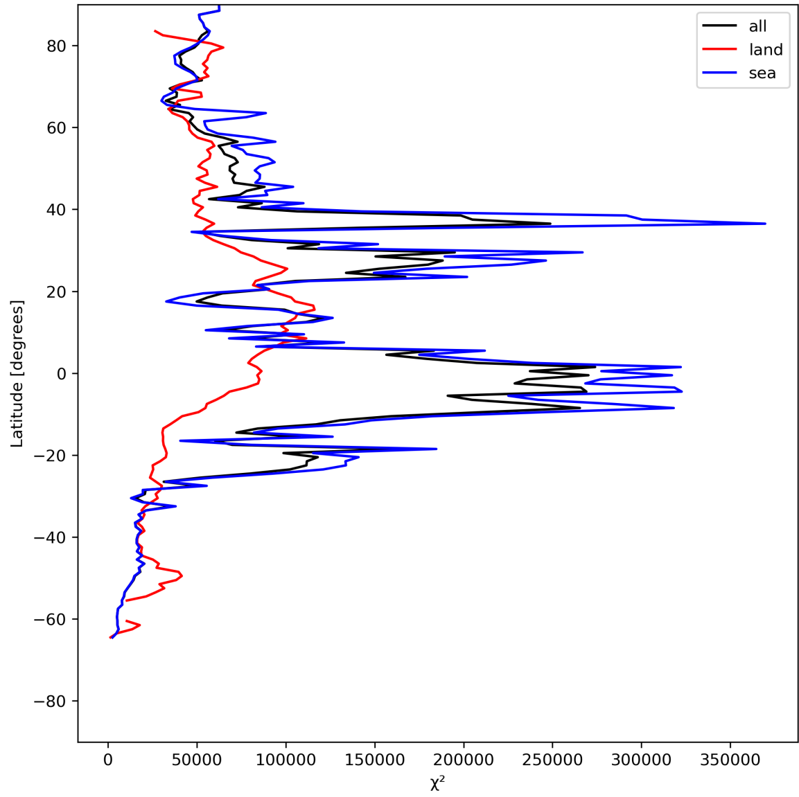
Figure 21: Zonal average of “ \chi^2 ” for 2024-06-29 to 2024-07-01.
