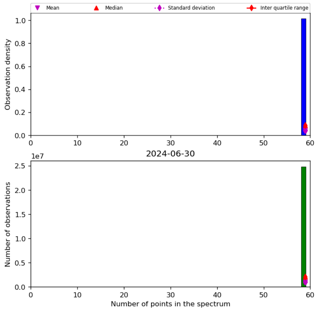
Figure 44: Histogram of “Number of points in the spectrum” for 2024-06-29 to 2024-07-01
