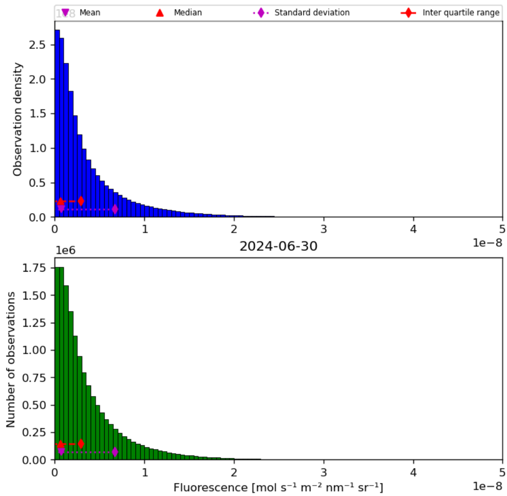
Figure 40: Histogram of “Fluorescence” for 2024-06-29 to 2024-07-01
