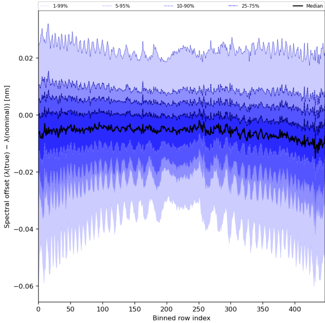
Figure 62: Along track statistics of “Spectral offset ( \lambda(\text{true}) - \lambda(\text{nominal}) )” for 2024-06-29 to 2024-07-01
