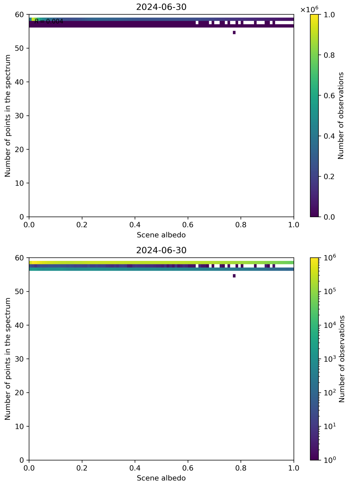
Figure 106: Scatter density plot of “Scene albedo” against “Number of points in the spectrum” for 2024-06-29 to 2024-07-01.
