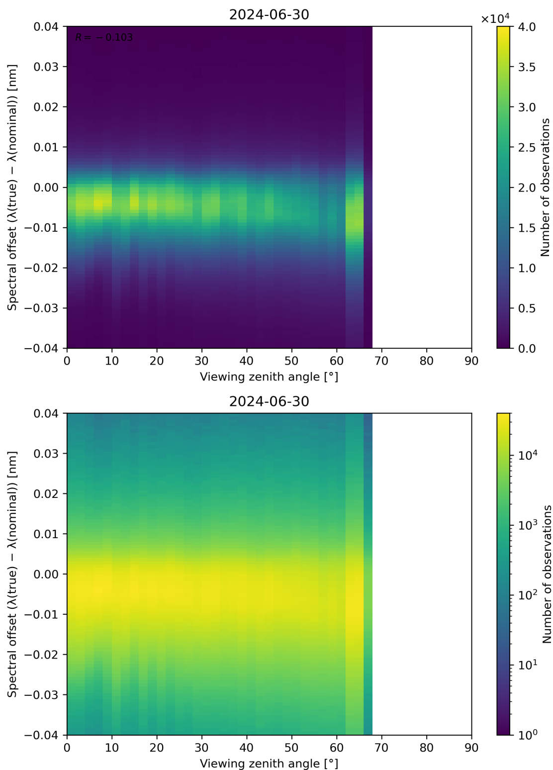
Figure 128: Scatter density plot of “Viewing zenith angle” against “Spectral offset ( \lambda(\text{true}) - \lambda(\text{nominal}) )” for 2024-06-29 to 2024-07-01.
