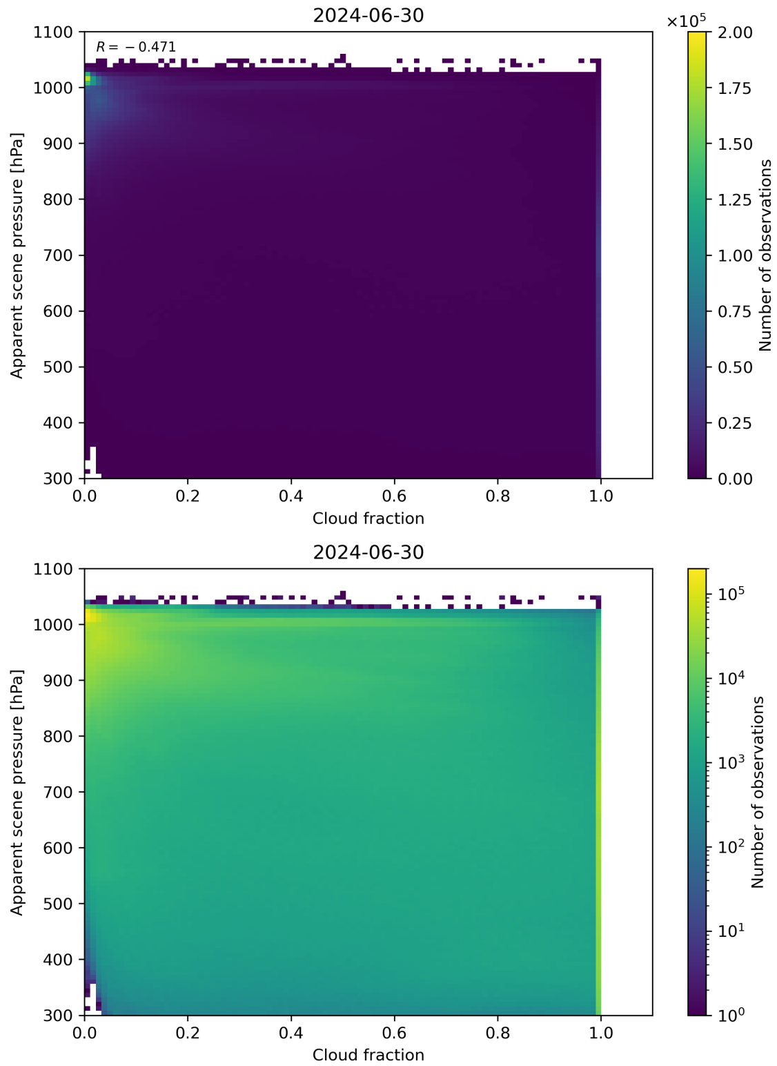
Figure 70: Scatter density plot of “Cloud fraction” against “Apparent scene pressure” for 2024-06-29 to 2024-07-01.
