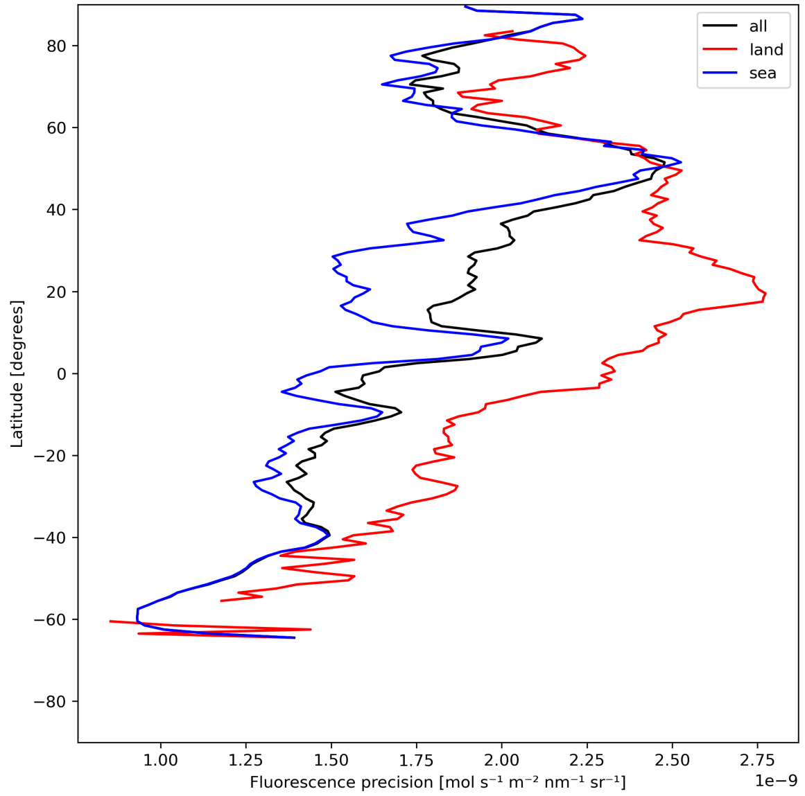
Figure 24: Zonal average of “Fluorescence precision” for 2024-06-29 to 2024-07-01.
