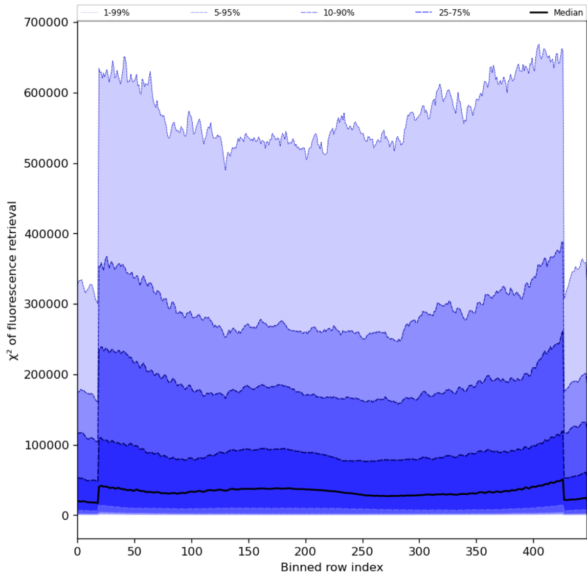
Figure 59: Along track statistics of “ \chi^2 of fluorescence retrieval” for 2024-06-29 to 2024-07-01
