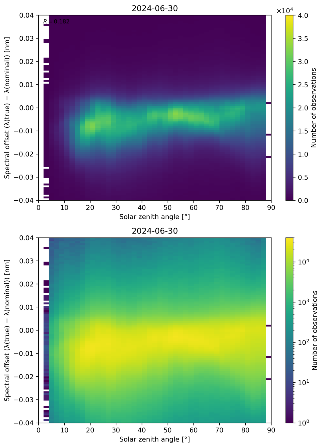
Figure 117: Scatter density plot of “Solar zenith angle” against “Spectral offset ( \lambda(\text{true}) - \lambda(\text{nominal}) )” for 2024-06-29 to 2024-07-01.
