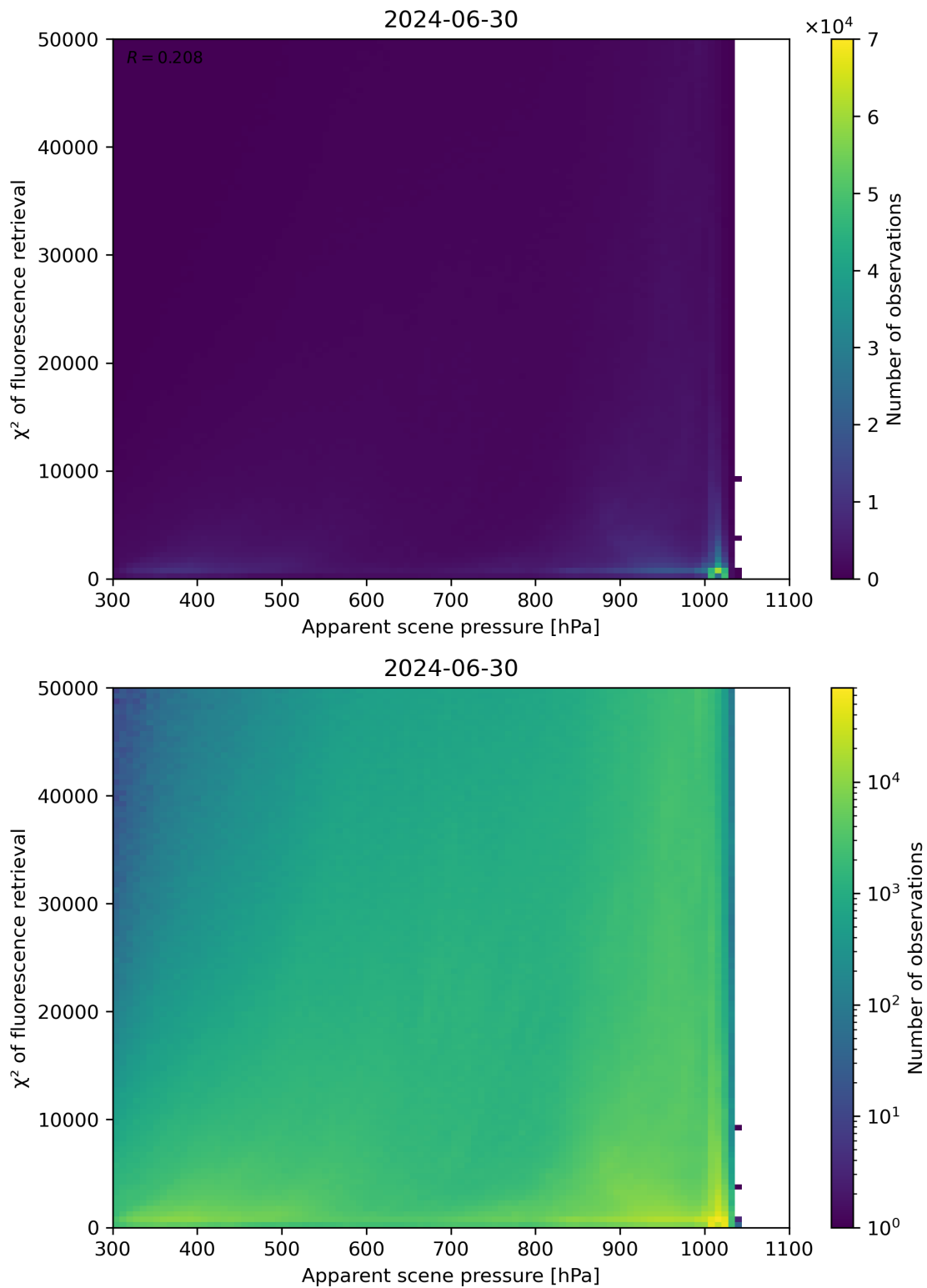
Figure 63: Scatter density plot of “Apparent scene pressure” against “ \chi^2 of fluorescence retrieval” for 2024-06-29 to 2024-07-01.
