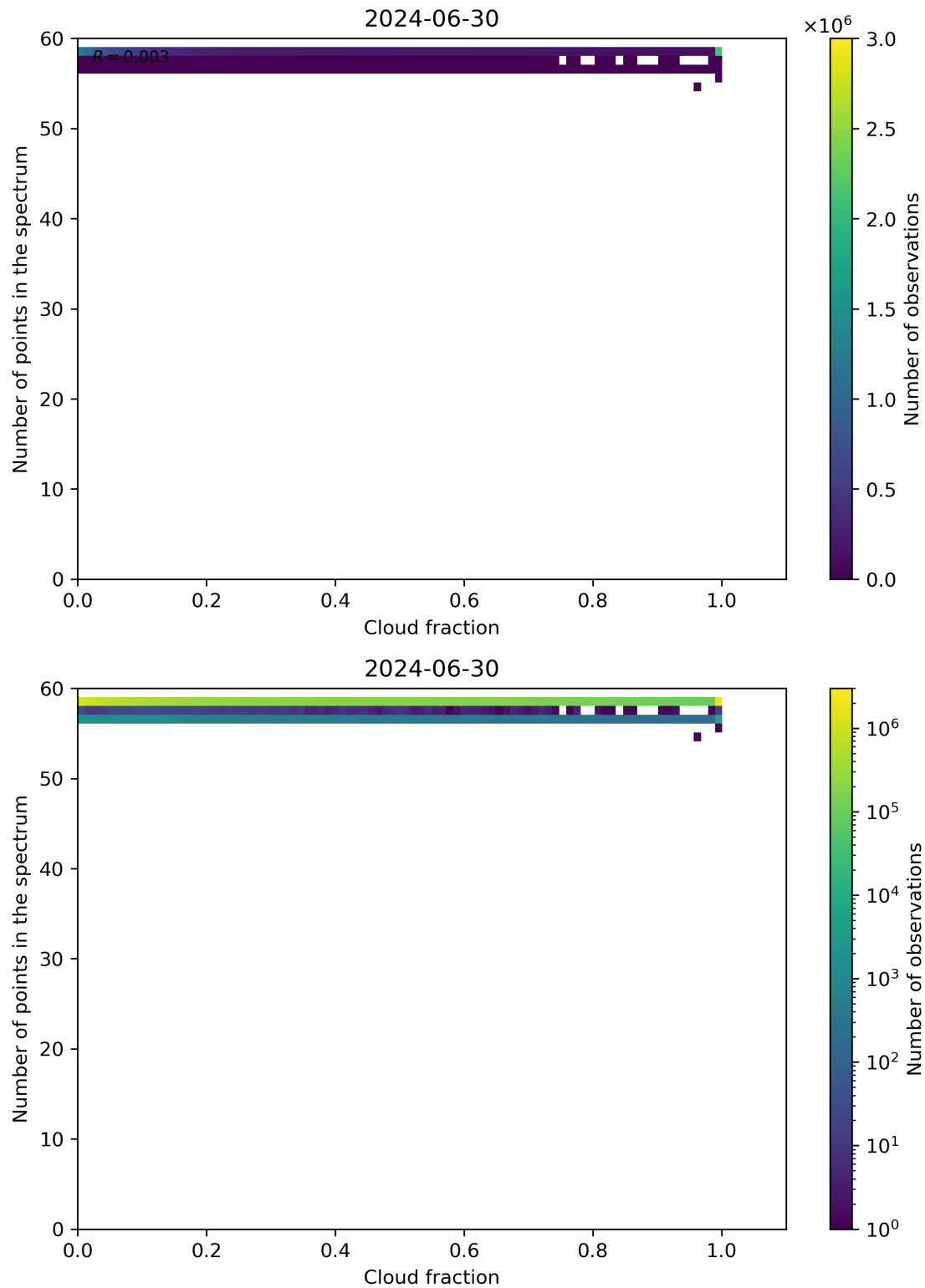
Figure 74: Scatter density plot of “Cloud fraction” against “Number of points in the spectrum” for 2024-06-29 to 2024-07-01.
