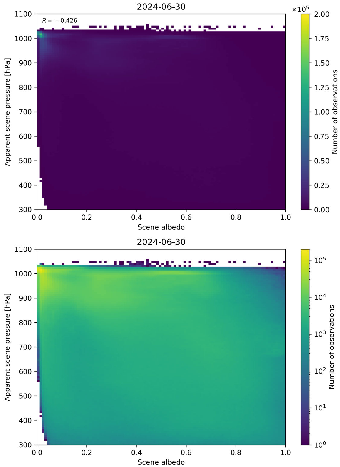
Figure 102: Scatter density plot of “Scene albedo” against “Apparent scene pressure” for 2024-06-29 to 2024-07-01.
