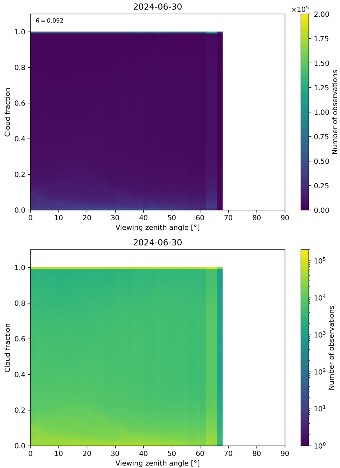
Figure 120: Scatter density plot of “Viewing zenith angle” against “Cloud fraction” for 2024-06-29 to 2024-07-01.
