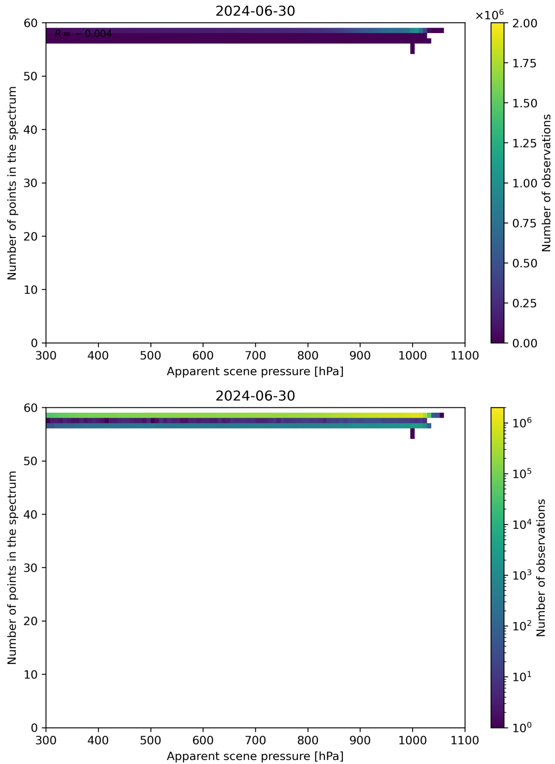
Figure 66: Scatter density plot of “Apparent scene pressure” against “Number of points in the spectrum” for 2024-06-29 to 2024-07-01.
