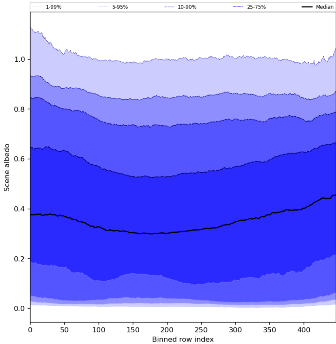
Figure 51: Along track statistics of “Scene albedo” for 2024-06-29 to 2024-07-01
