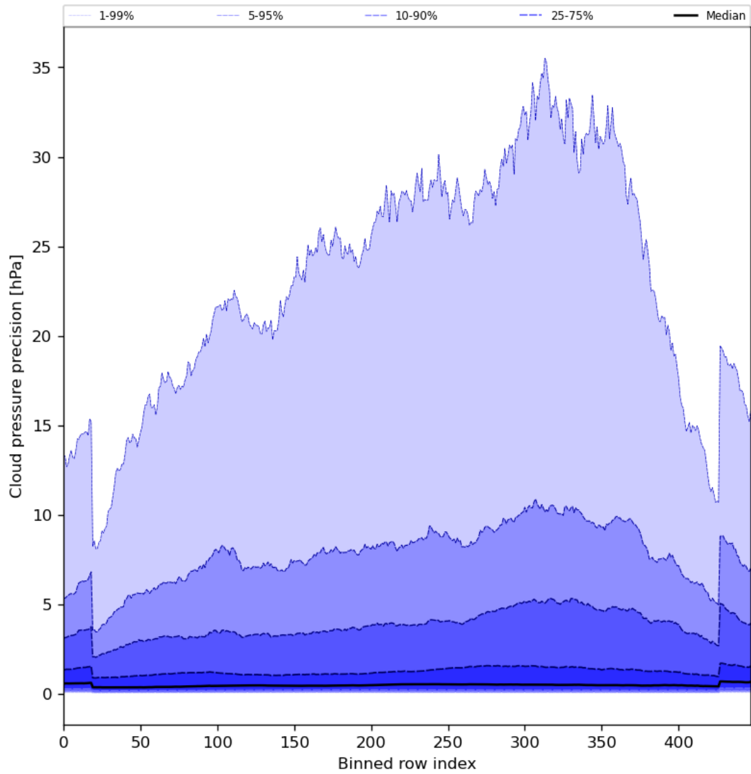
Figure 48: Along track statistics of “Cloud pressure precision” for 2024-06-29 to 2024-07-01
