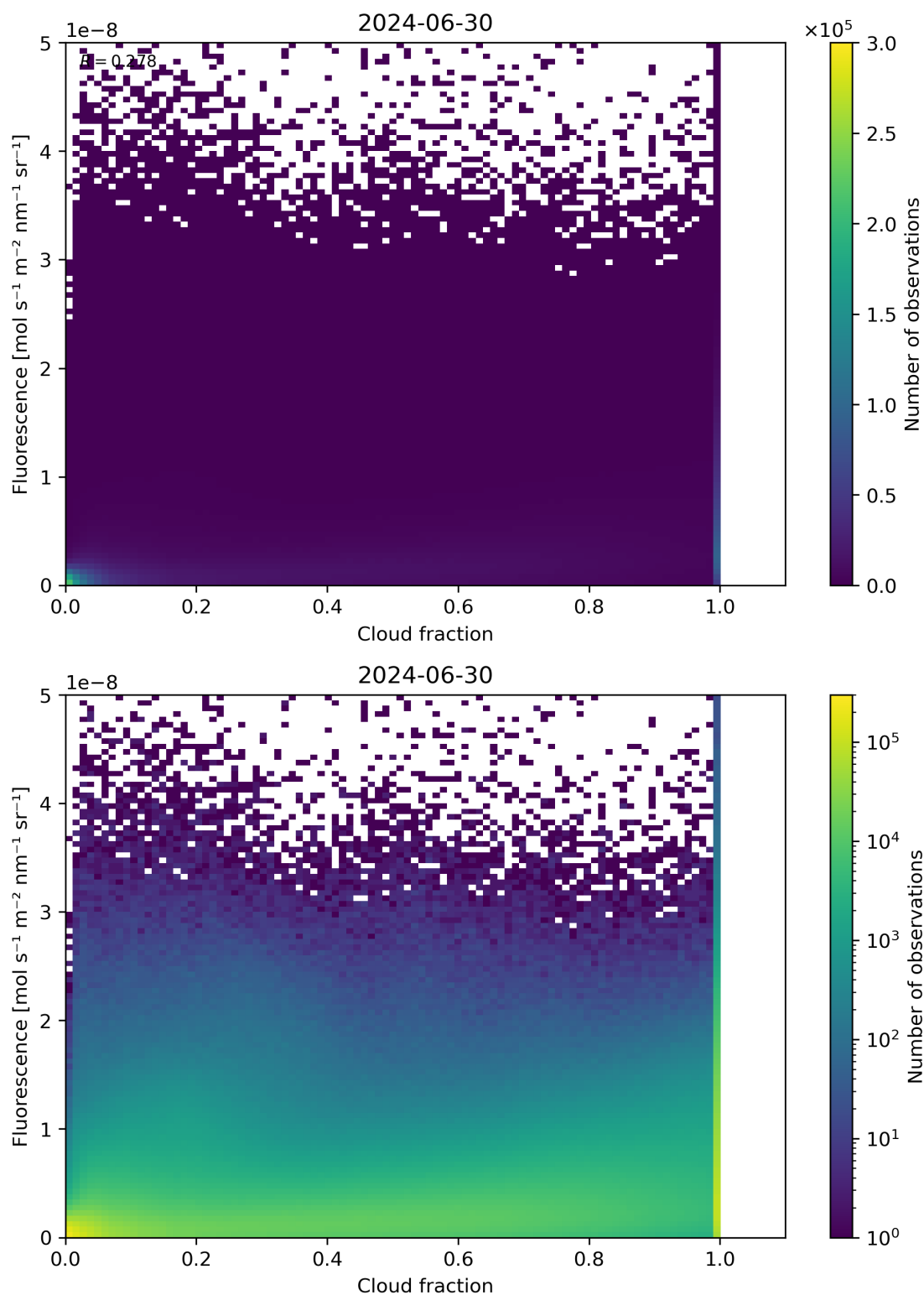
Figure 72: Scatter density plot of “Cloud fraction” against “Fluorescence” for 2024-06-29 to 2024-07-01.
