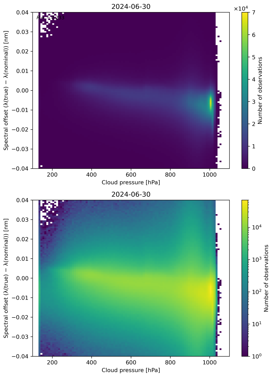
Figure 84: Scatter density plot of “Cloud pressure” against “Spectral offset ( \lambda(\text{true}) - \lambda(\text{nominal}) )” for 2024-06-29 to 2024-07-01.
