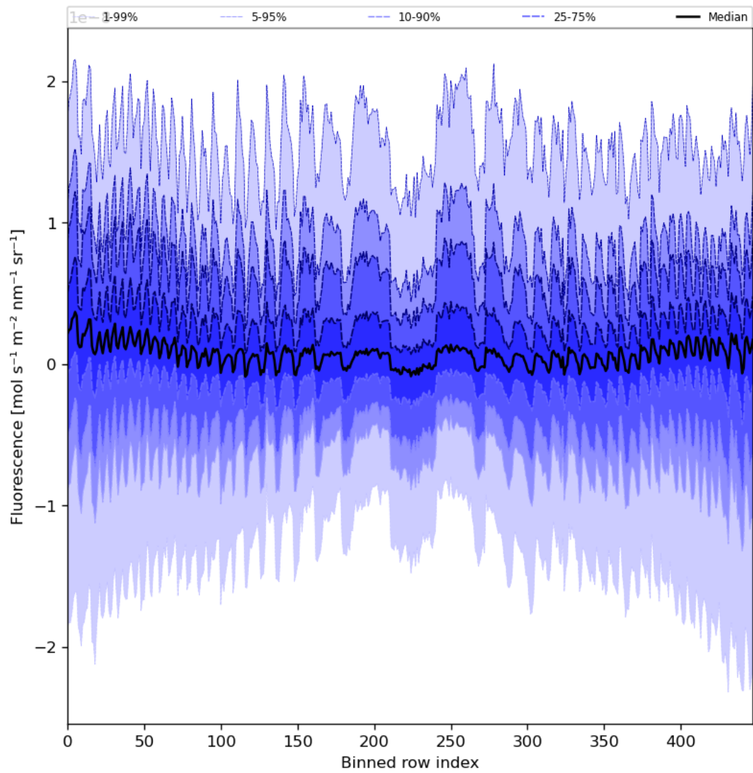
Figure 57: Along track statistics of "Fluorescence" for 2024-06-29 to 2024-07-01
