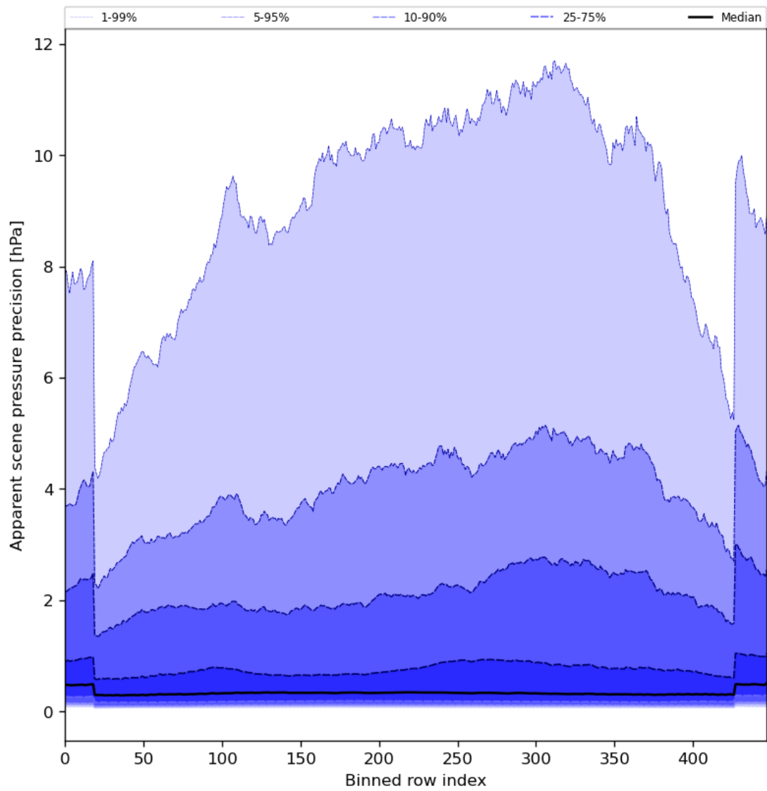
Figure 54: Along track statistics of “Apparent scene pressure precision” for 2024-06-29 to 2024-07-01
