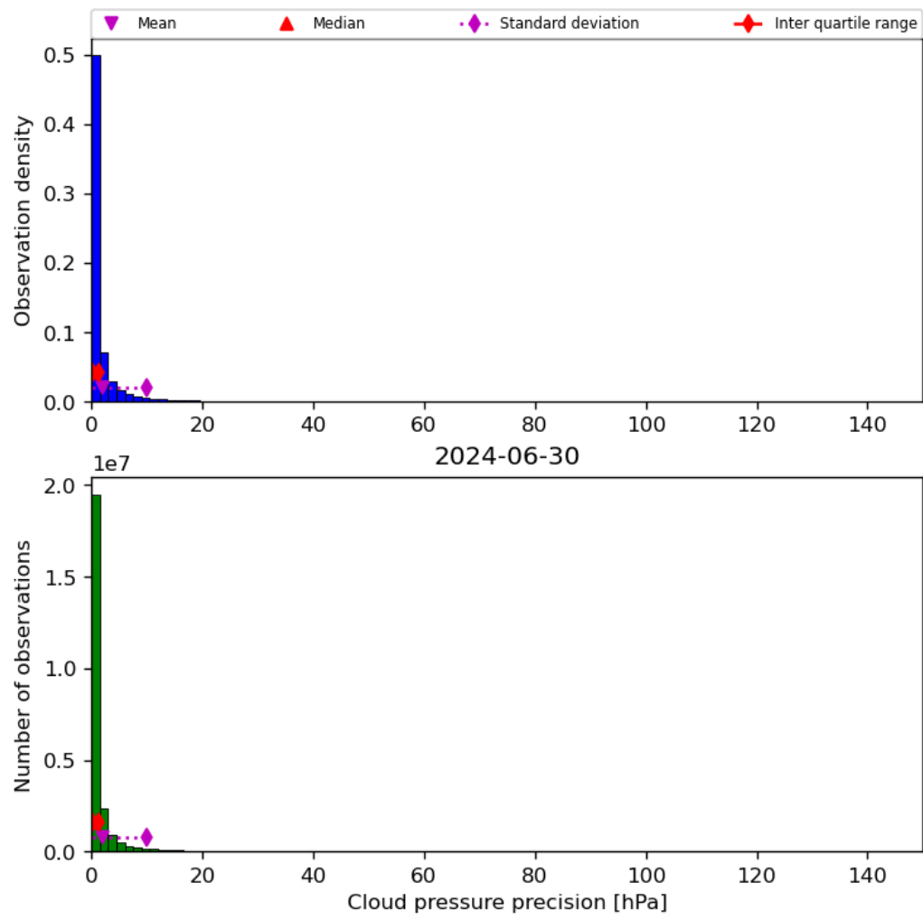
Figure 31: Histogram of “Cloud pressure precision” for 2024-06-29 to 2024-07-01
