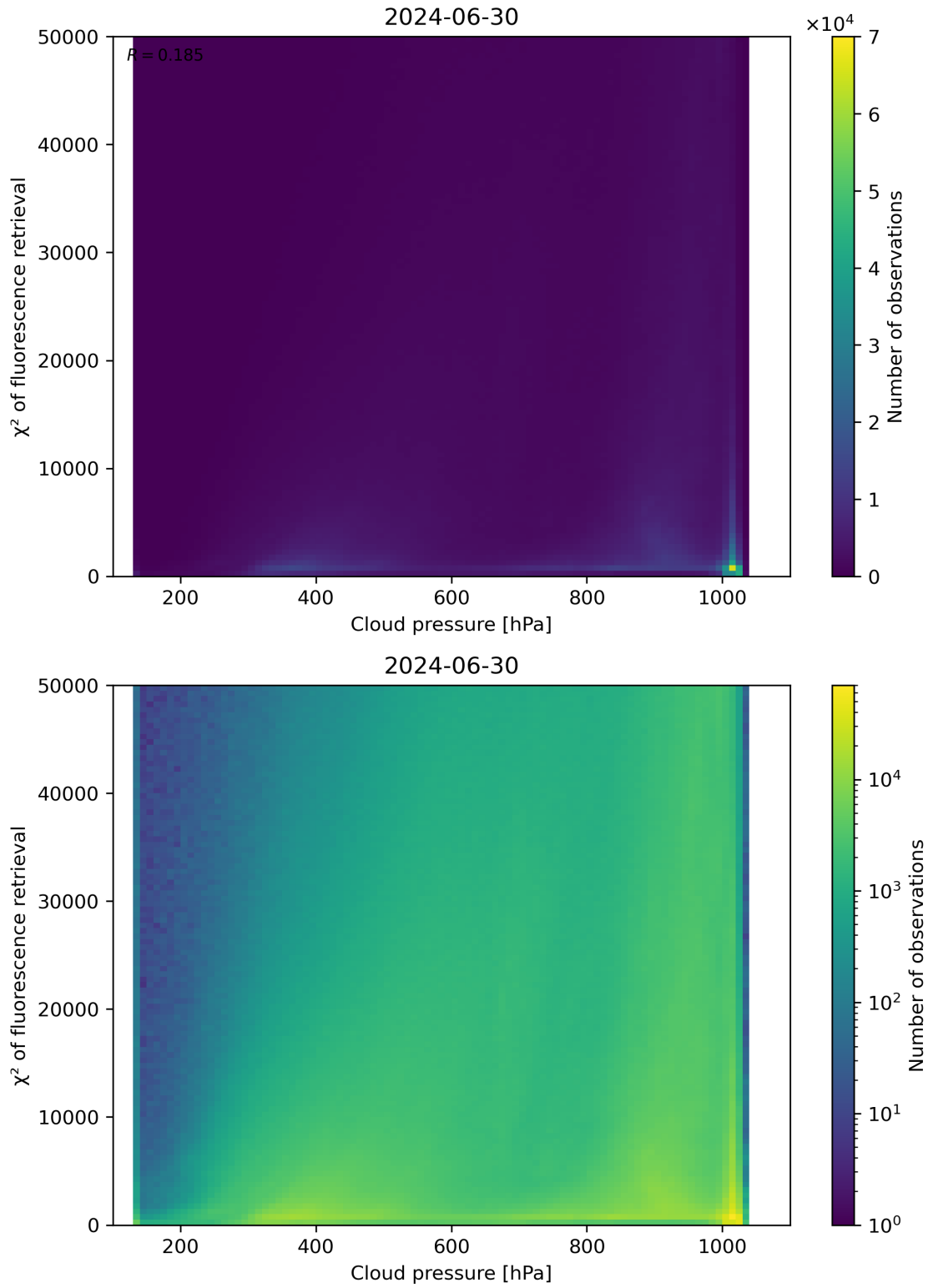
Figure 78: Scatter density plot of “Cloud pressure” against “ \chi^2 of fluorescence retrieval” for 2024-06-29 to 2024-07-01.
