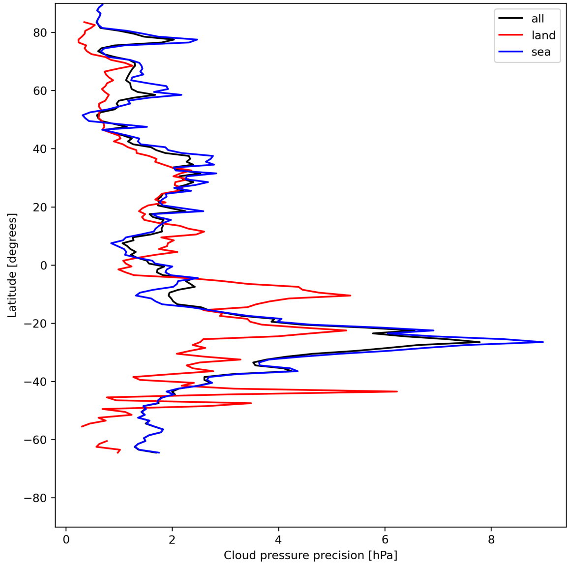
Figure 14: Zonal average of "Cloud pressure precision" for 2024-06-29 to 2024-07-01.
