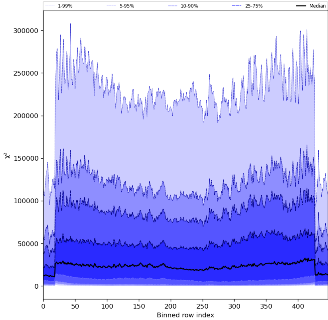
Figure 55: Along track statistics of “ \chi^2 ” for 2024-06-29 to 2024-07-01
