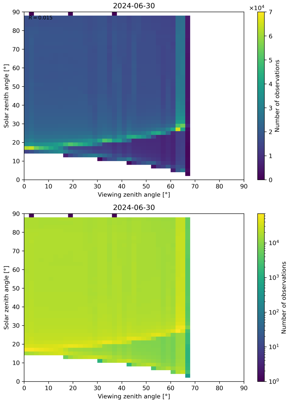
Figure 127: Scatter density plot of “Viewing zenith angle” against “Solar zenith angle” for 2024-06-29 to 2024-07-01.
