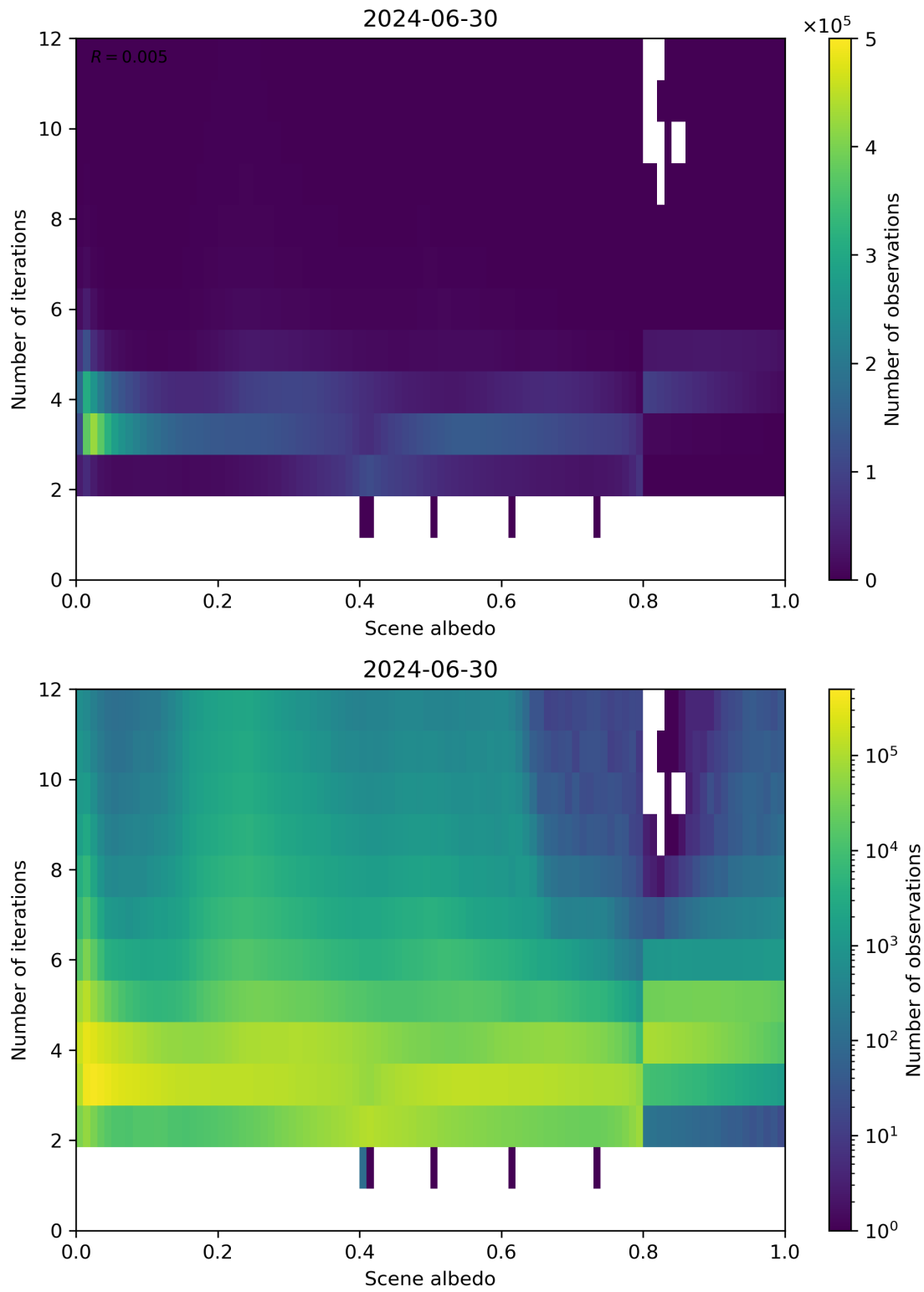
Figure 105: Scatter density plot of “Scene albedo” against “Number of iterations” for 2024-06-29 to 2024-07-01.
