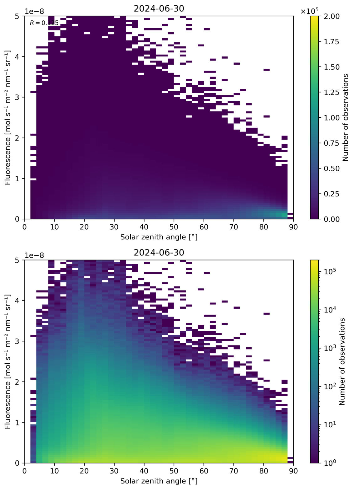
Figure 112: Scatter density plot of “Solar zenith angle” against “Fluorescence” for 2024-06-29 to 2024-07-01.
