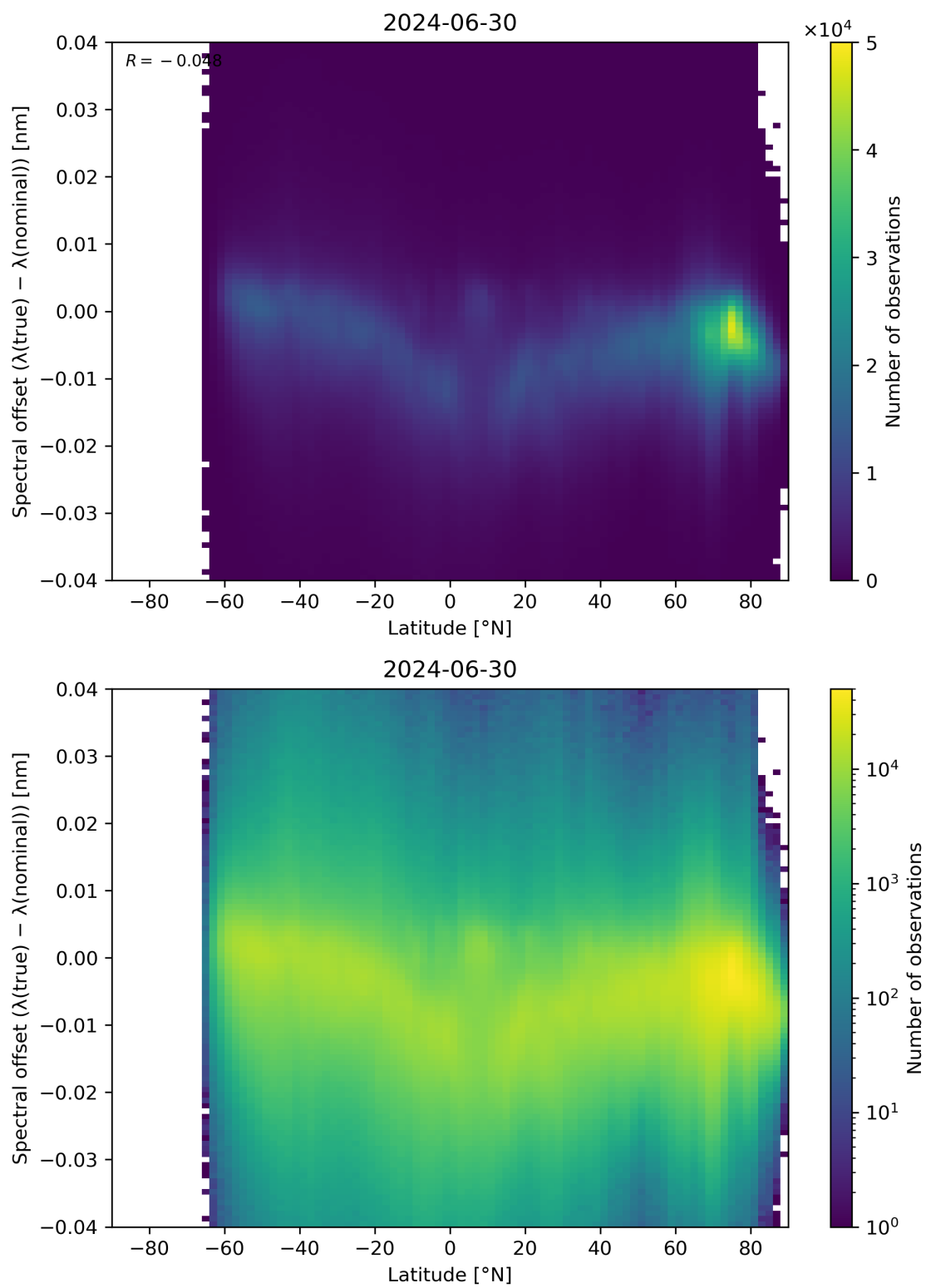
Figure 96: Scatter density plot of “Latitude” against “Spectral offset ( \lambda(\text{true}) - \lambda(\text{nominal}) )” for 2024-06-29 to 2024-07-01.
