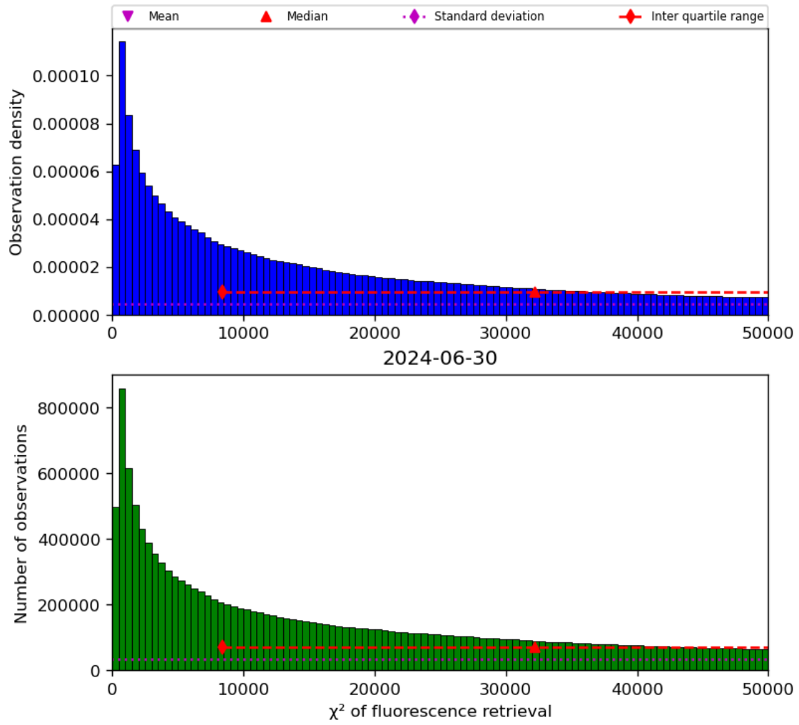
Figure 42: Histogram of “ \chi^2 of fluorescence retrieval” for 2024-06-29 to 2024-07-01
