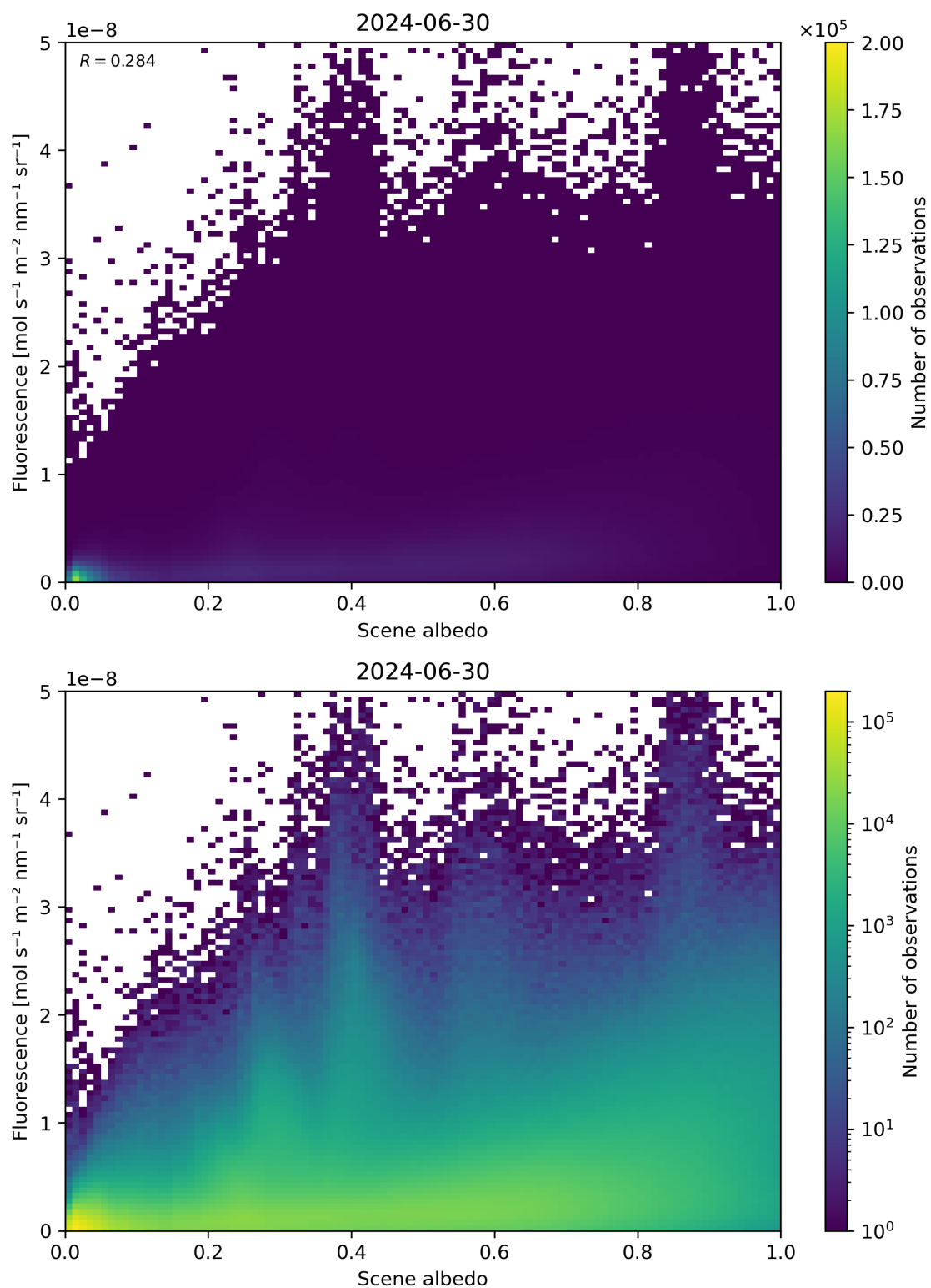
Figure 104: Scatter density plot of “Scene albedo” against “Fluorescence” for 2024-06-29 to 2024-07-01.
