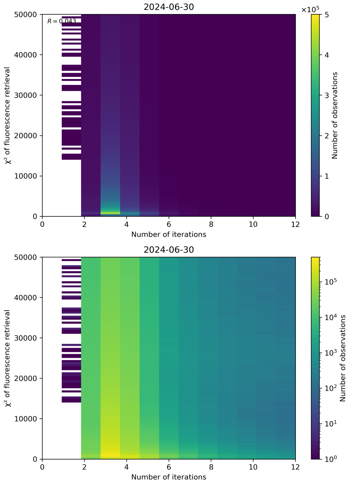
Figure 97: Scatter density plot of “Number of iterations” against “ \chi^2 of fluorescence retrieval” for 2024-06-29 to 2024-07-01.
