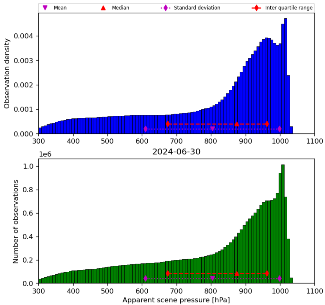
Figure 36: Histogram of “Apparent scene pressure” for 2024-06-29 to 2024-07-01
