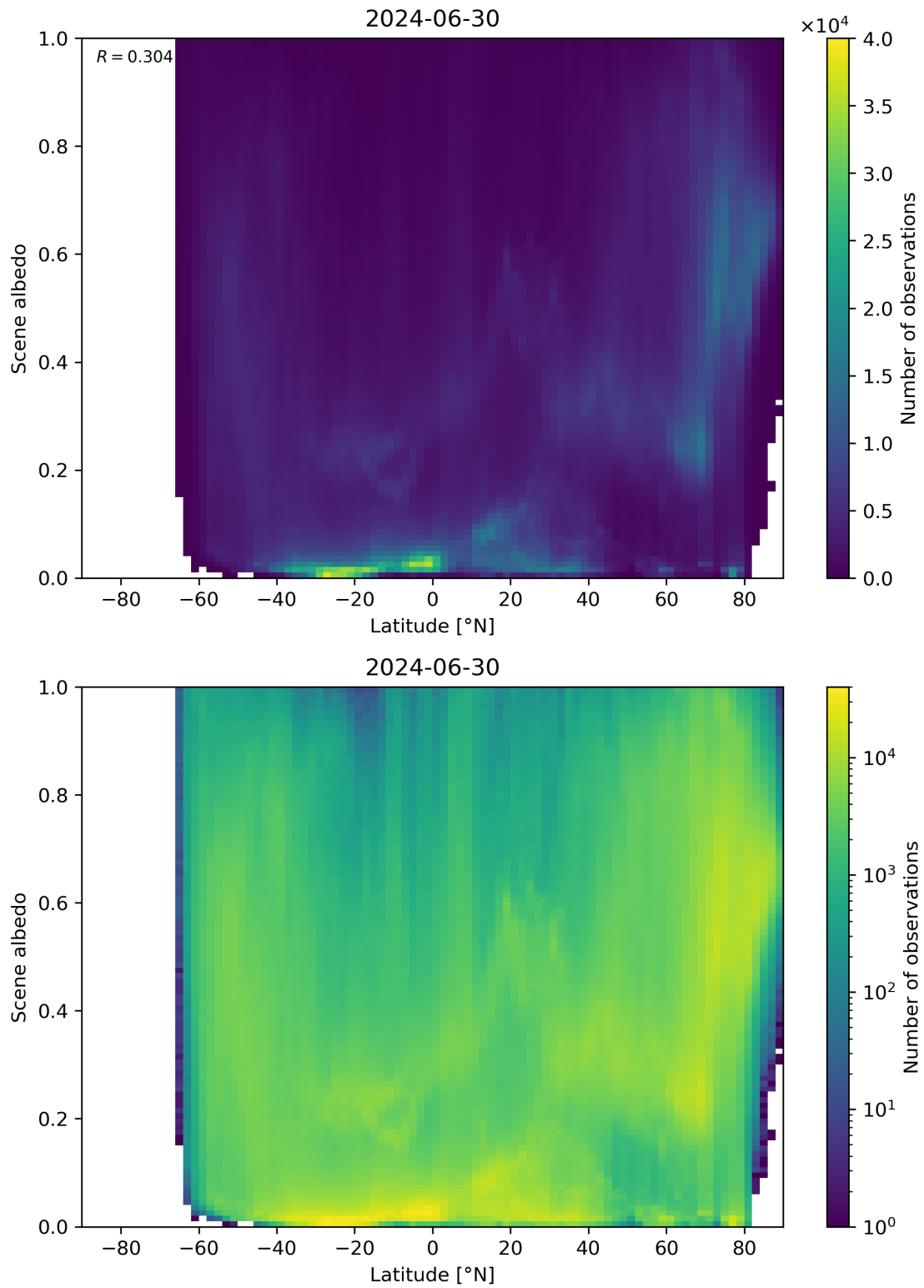
Figure 95: Scatter density plot of “Latitude” against “Scene albedo” for 2024-06-29 to 2024-07-01.
