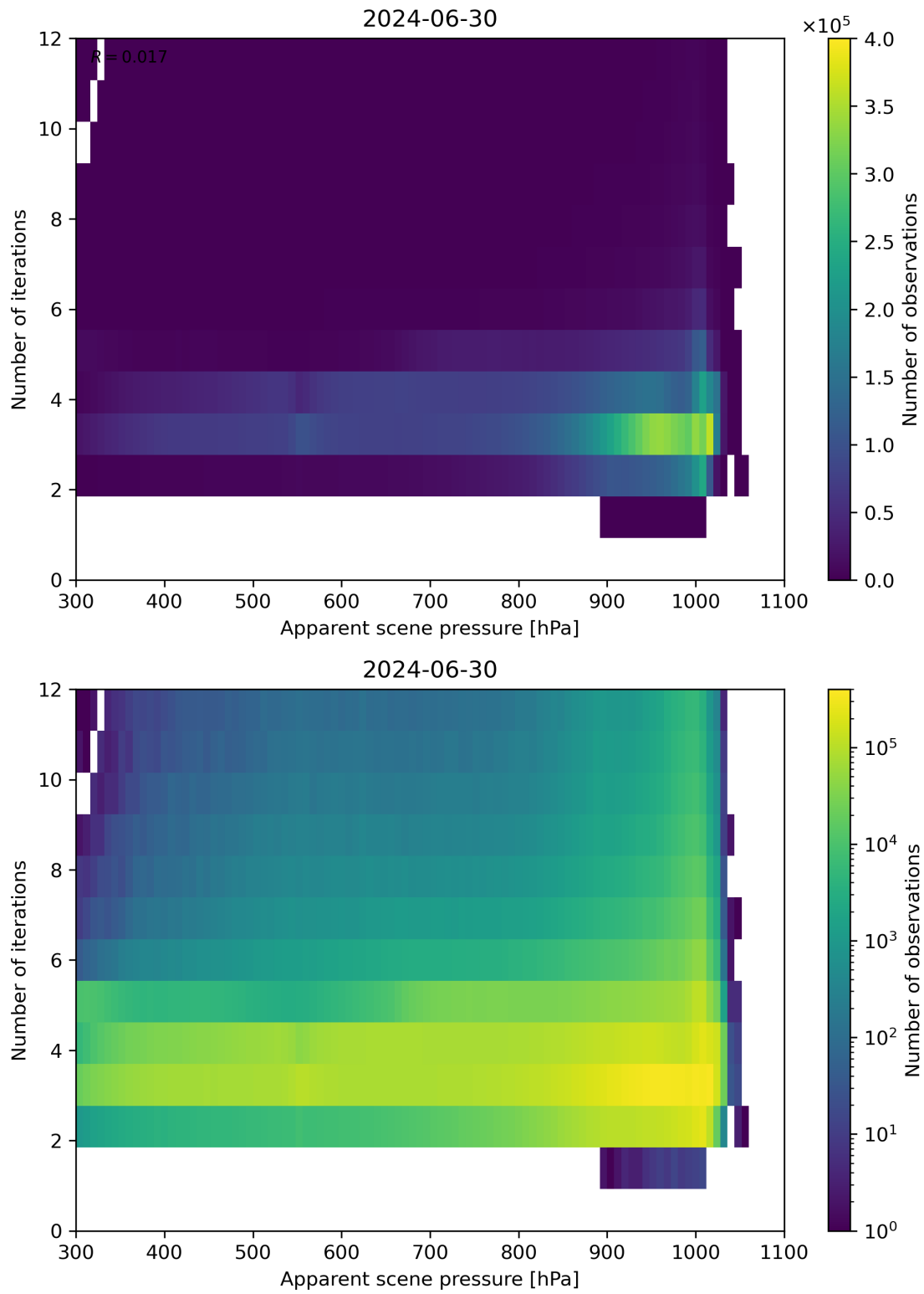
Figure 65: Scatter density plot of “Apparent scene pressure” against “Number of iterations” for 2024-06-29 to 2024-07-01.
