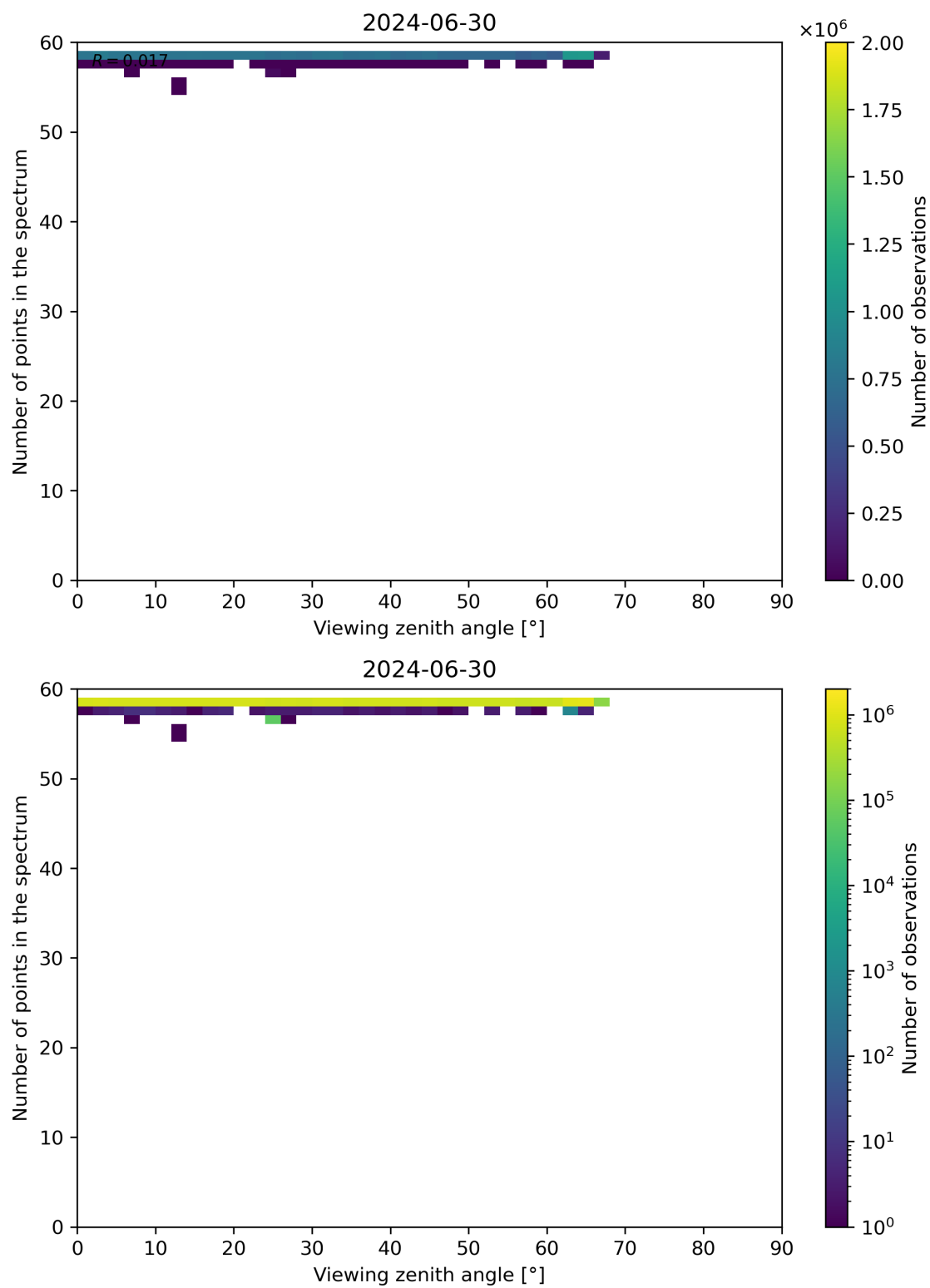
Figure 125: Scatter density plot of “Viewing zenith angle” against “Number of points in the spectrum” for 2024-06-29 to 2024-07-01.
