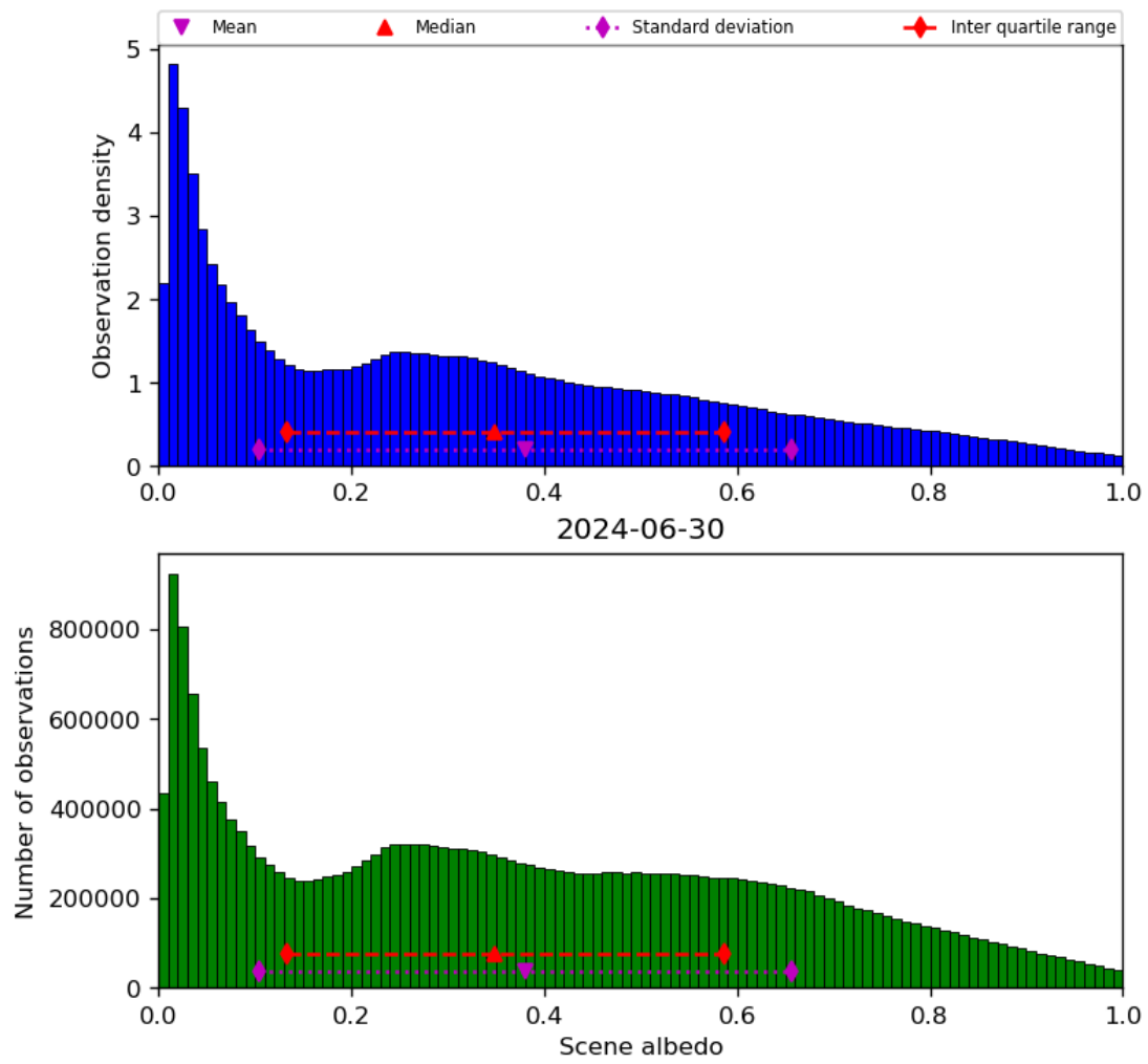
Figure 34: Histogram of “Scene albedo” for 2024-06-29 to 2024-07-01
