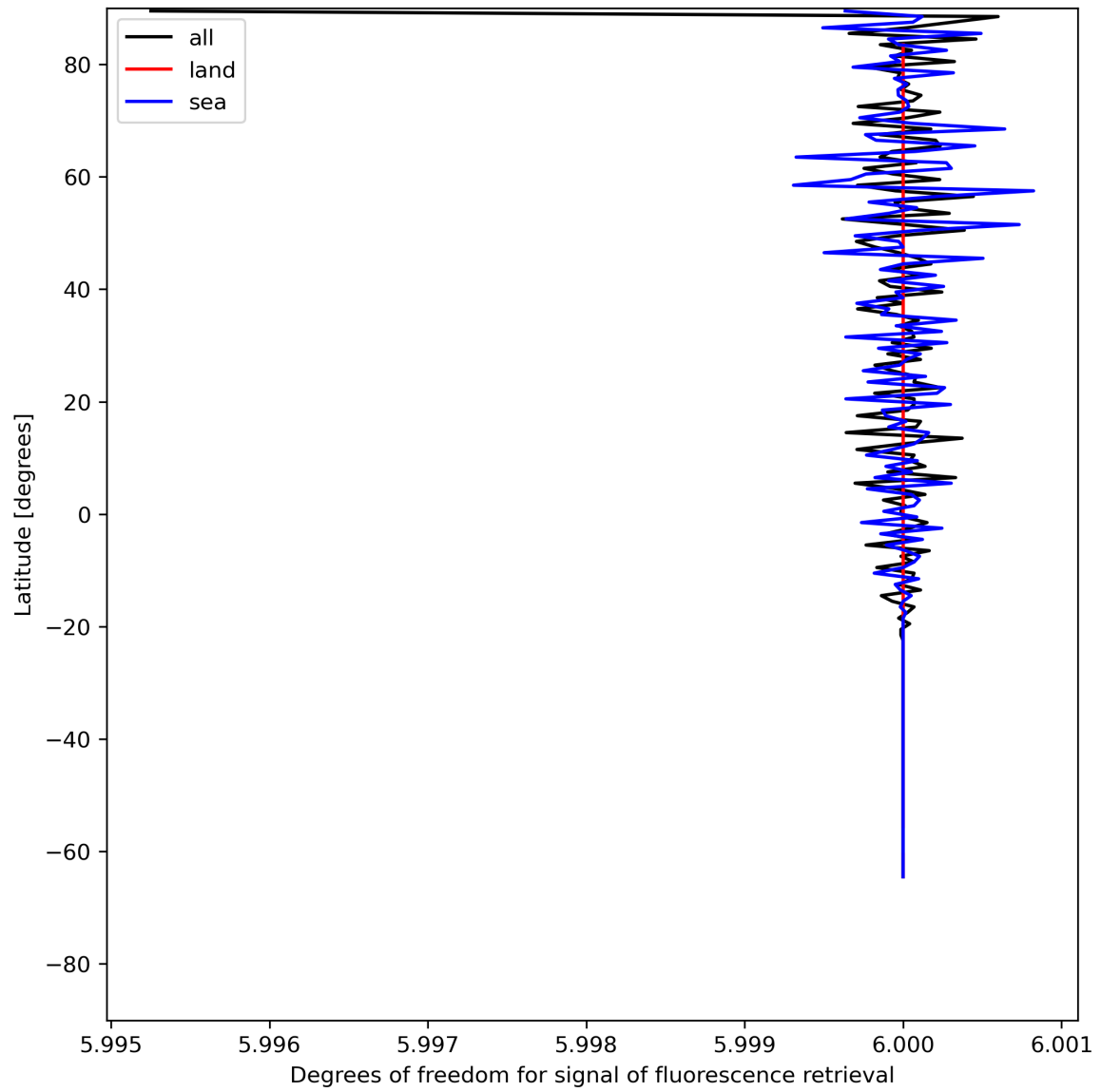
Figure 26: Zonal average of “Degrees of freedom for signal of fluorescence retrieval” for 2024-06-29 to 2024-07-01.
