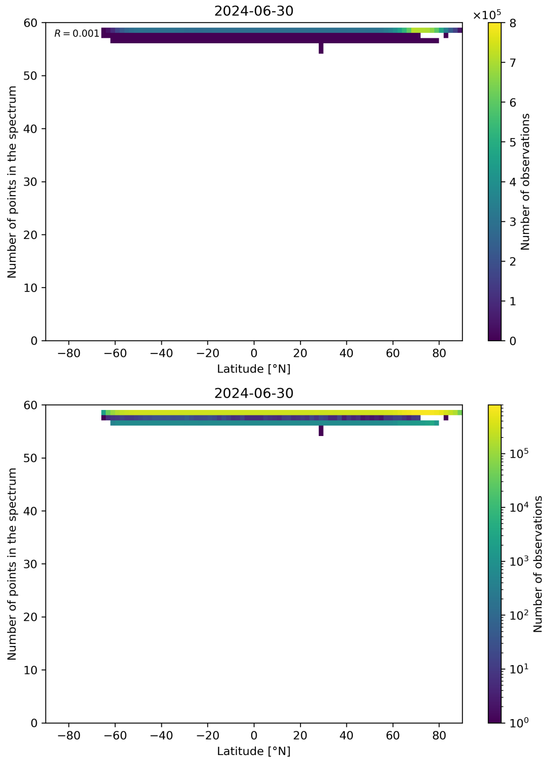
Figure 94: Scatter density plot of “Latitude” against “Number of points in the spectrum” for 2024-06-29 to 2024-07-01.
