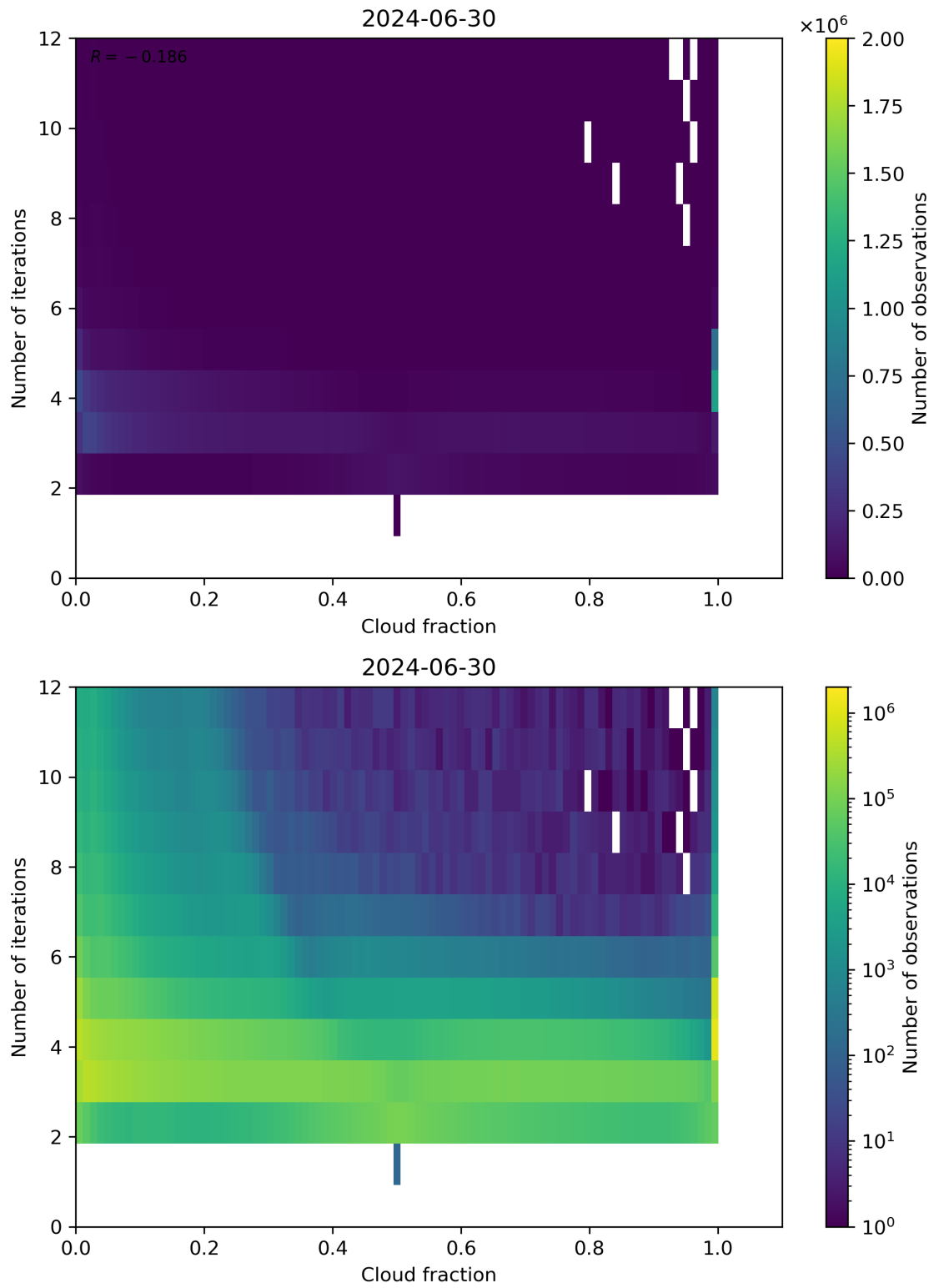
Figure 73: Scatter density plot of “Cloud fraction” against “Number of iterations” for 2024-06-29 to 2024-07-01.
