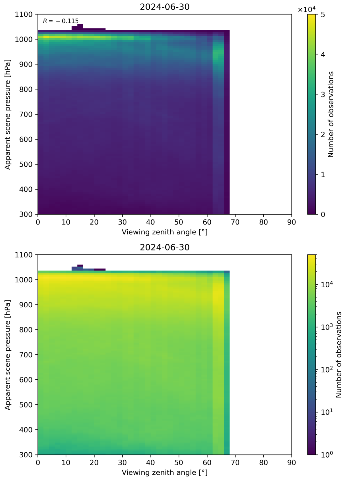
Figure 118: Scatter density plot of “Viewing zenith angle” against “Apparent scene pressure” for 2024-06-29 to 2024-07-01.
