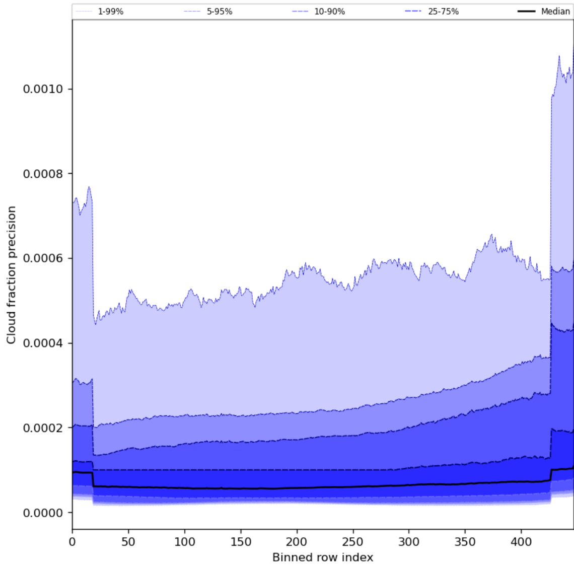
Figure 50: Along track statistics of “Cloud fraction precision” for 2024-06-29 to 2024-07-01
