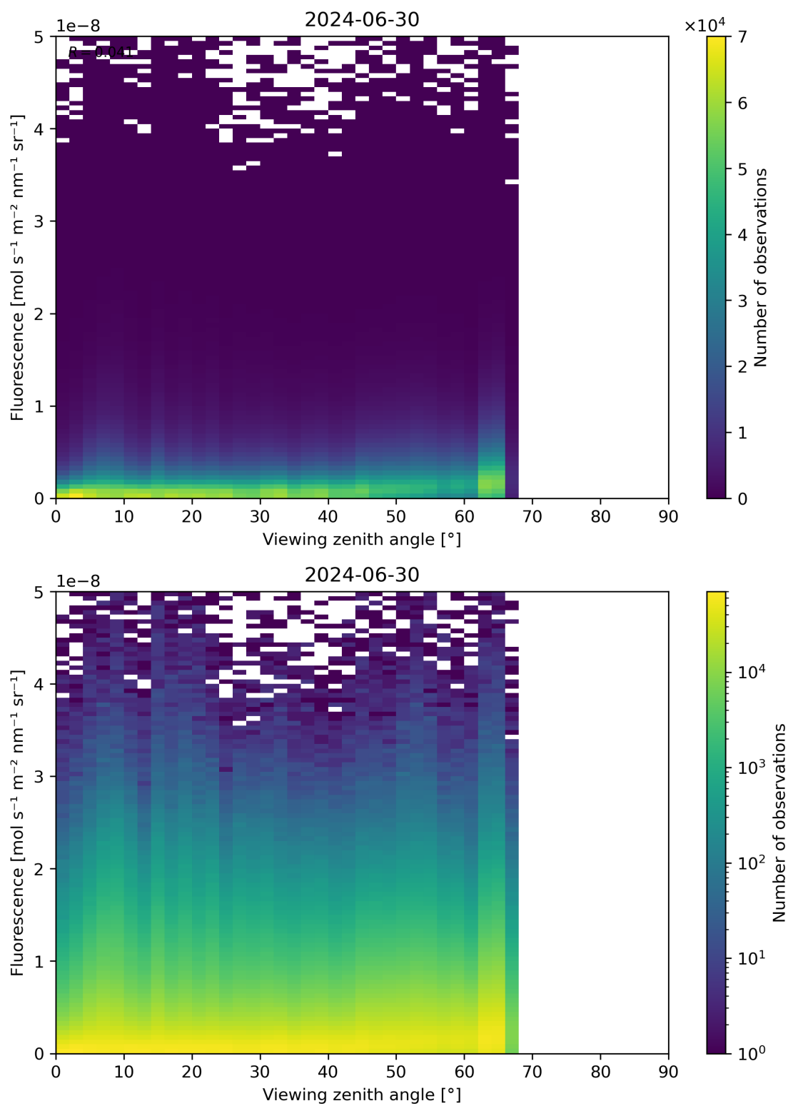
Figure 122: Scatter density plot of "Viewing zenith angle" against "Fluorescence" for 2024-06-29 to 2024-07-01.
