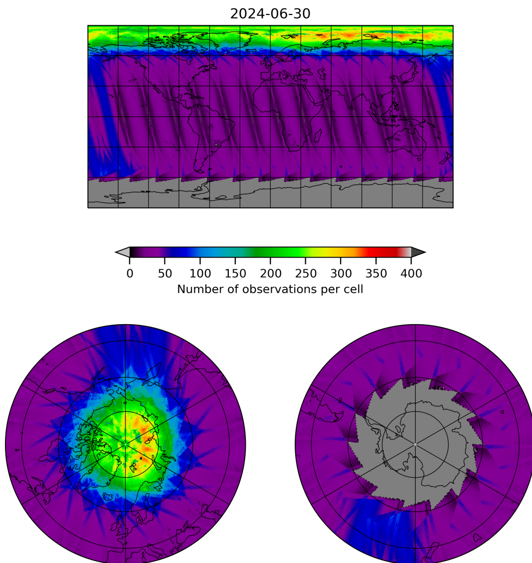
Figure 11: Map of the number of observations for 2024-06-29 to 2024-07-01
