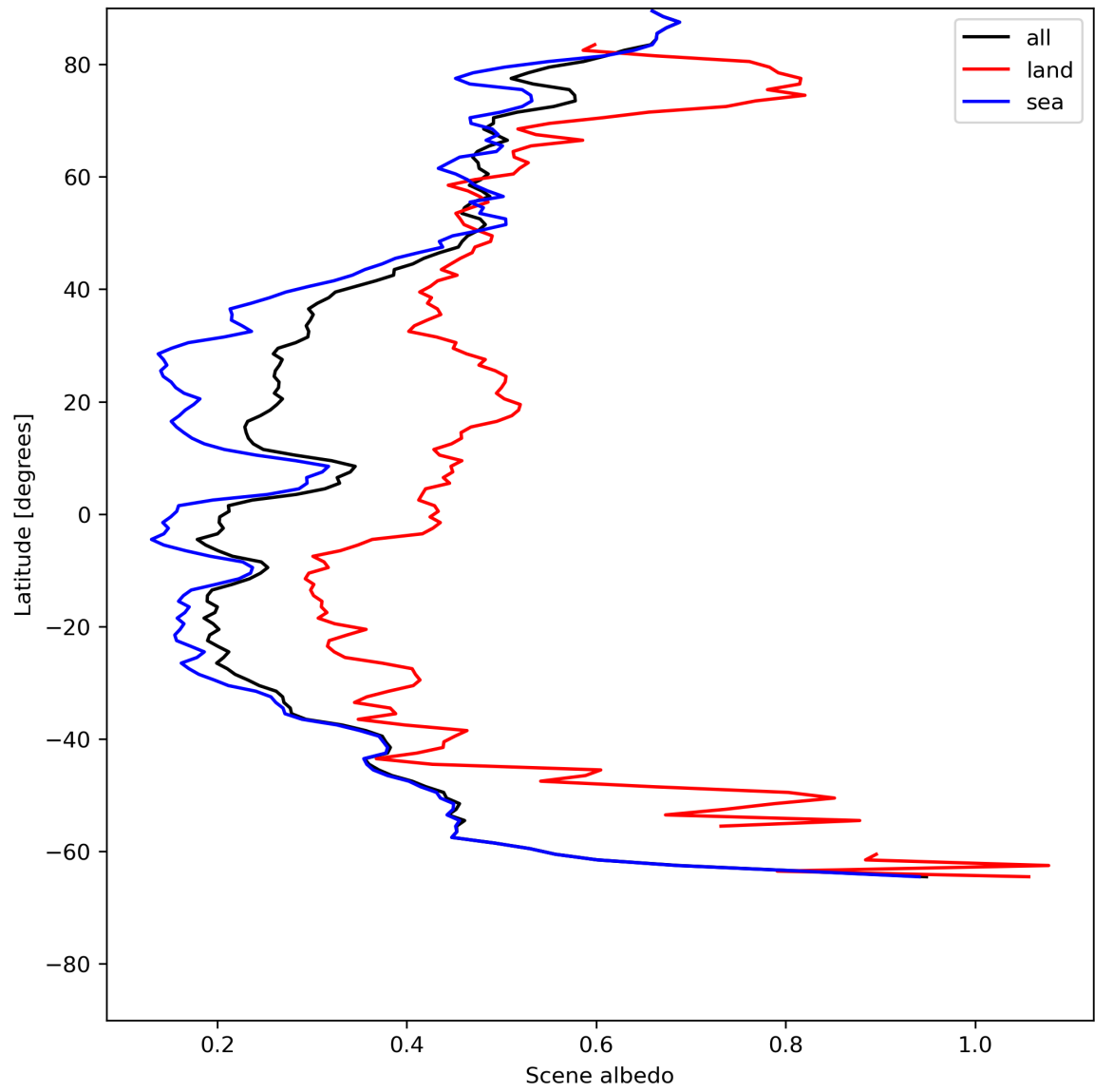
Figure 17: Zonal average of “Scene albedo” for 2024-06-29 to 2024-07-01.
