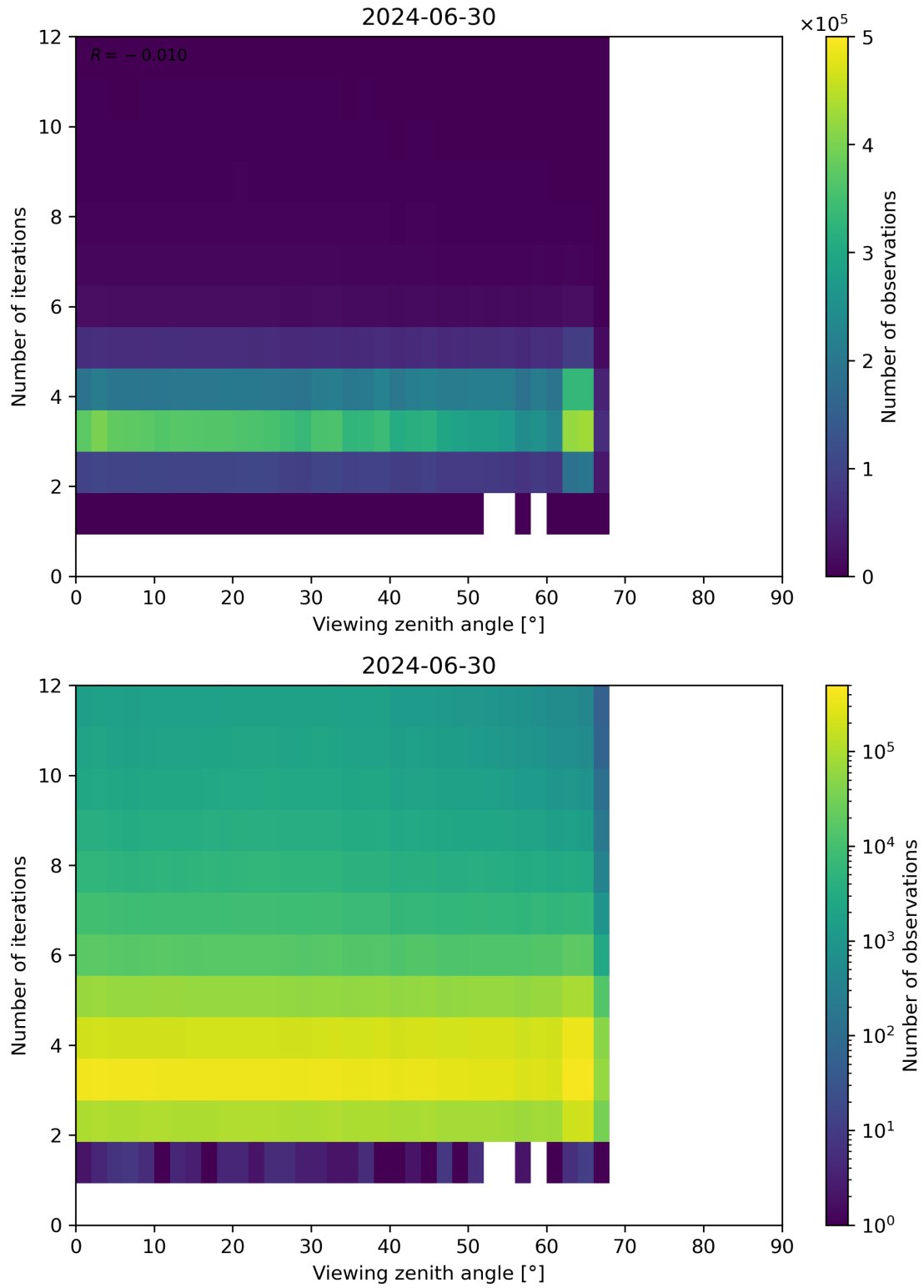
Figure 124: Scatter density plot of “Viewing zenith angle” against “Number of iterations” for 2024-06-29 to 2024-07-01.
