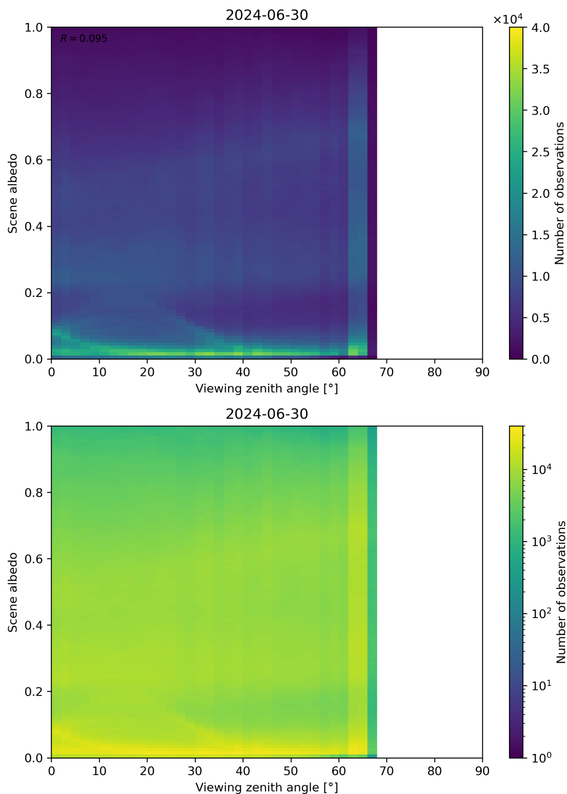
Figure 126: Scatter density plot of “Viewing zenith angle” against “Scene albedo” for 2024-06-29 to 2024-07-01.
