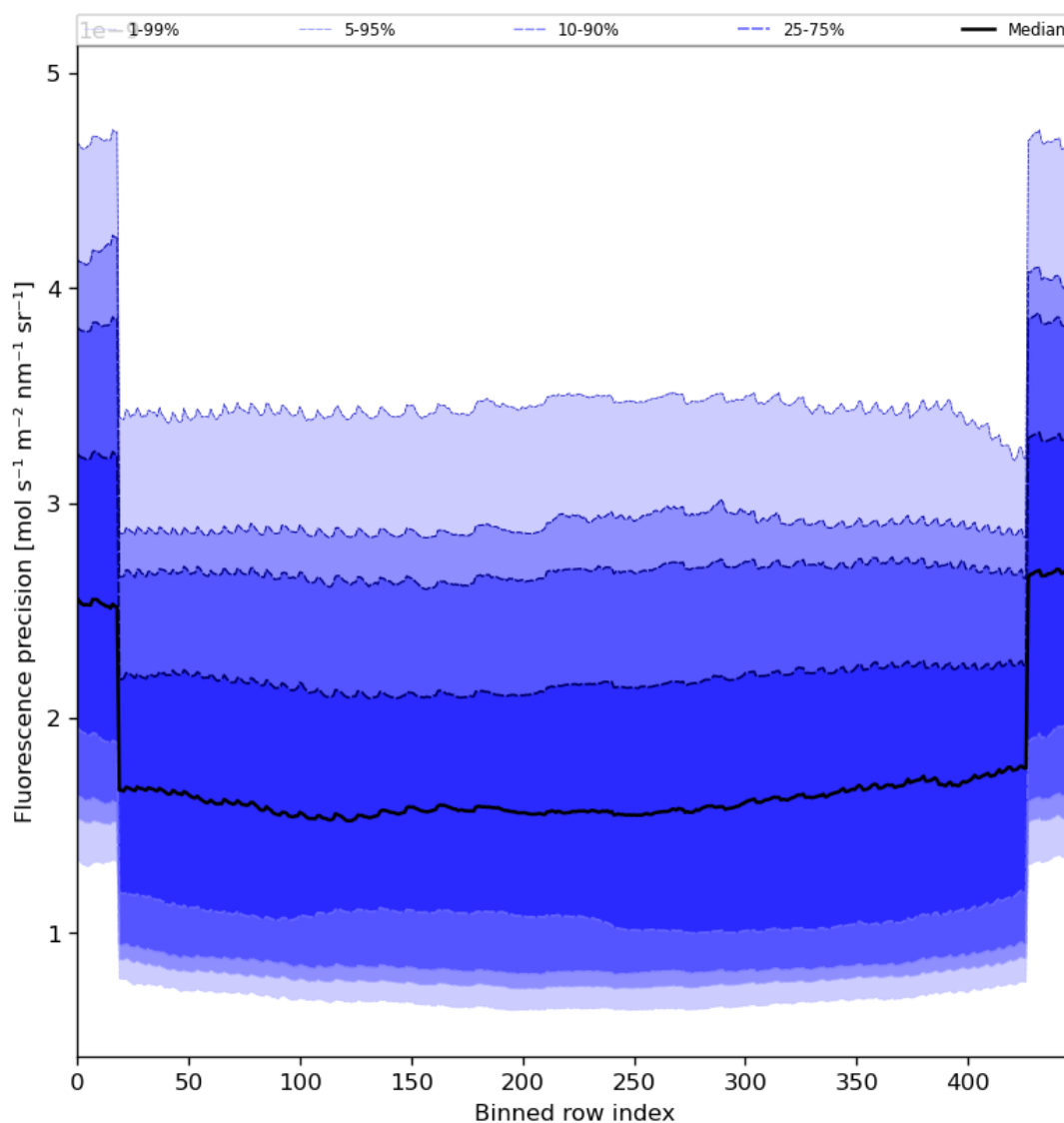
Figure 58: Along track statistics of “Fluorescence precision” for 2024-06-29 to 2024-07-01
