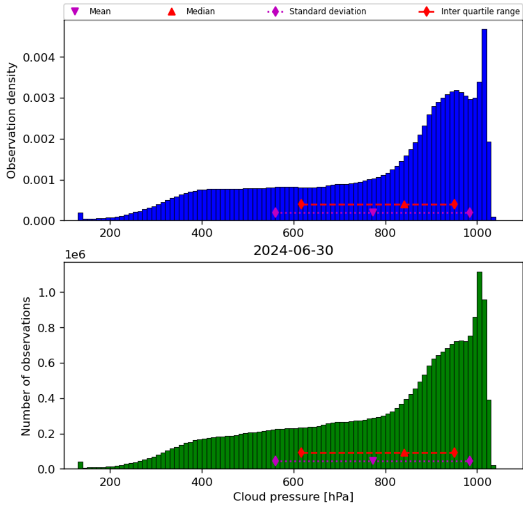
Figure 30: Histogram of “Cloud pressure” for 2024-06-29 to 2024-07-01
