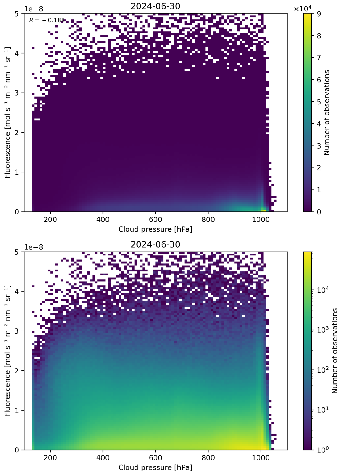
Figure 80: Scatter density plot of “Cloud pressure” against “Fluorescence” for 2024-06-29 to 2024-07-01.
