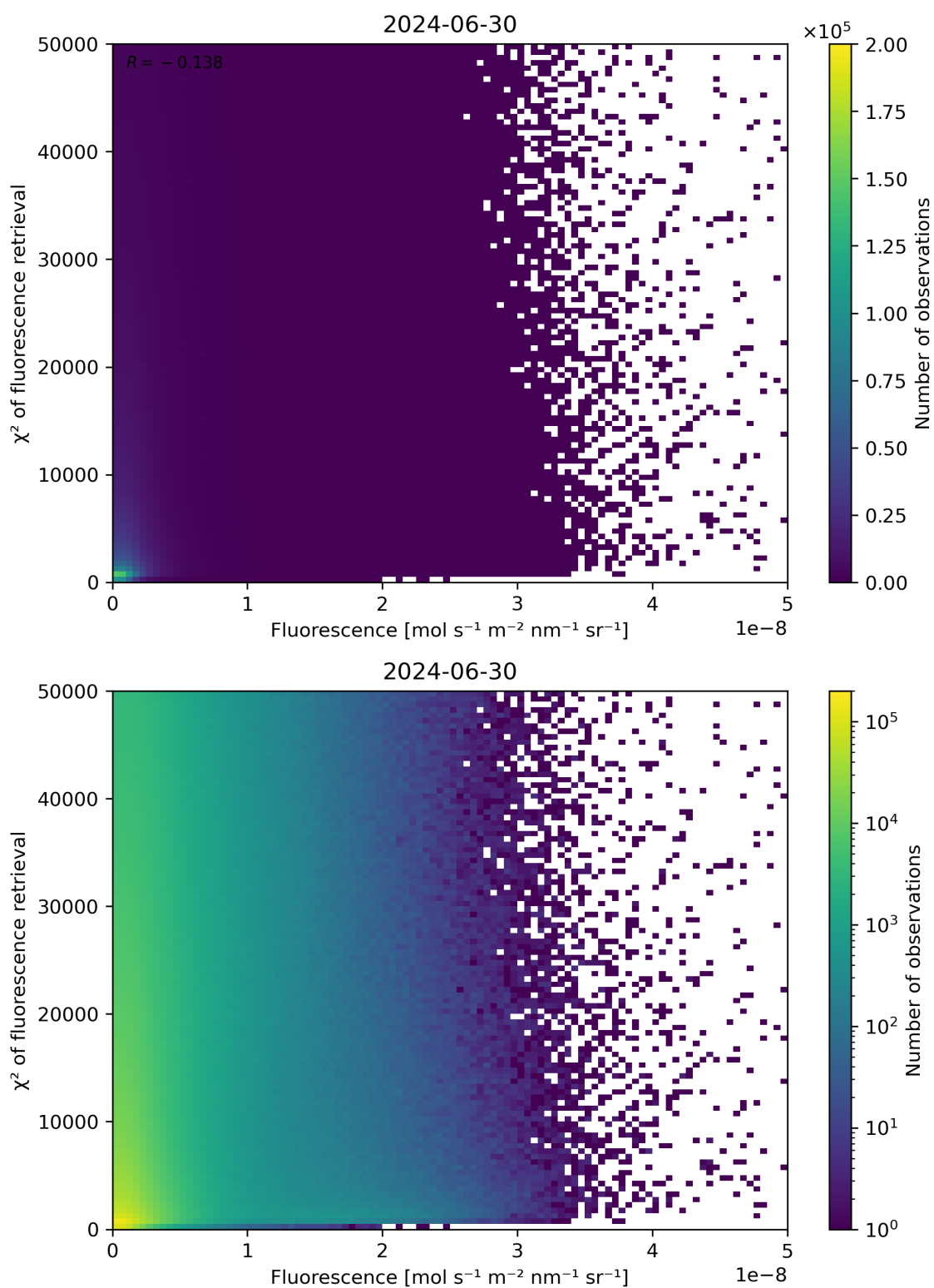
Figure 85: Scatter density plot of “Fluorescence” against “ \chi^2 of fluorescence retrieval” for 2024-06-29 to 2024-07-01.
