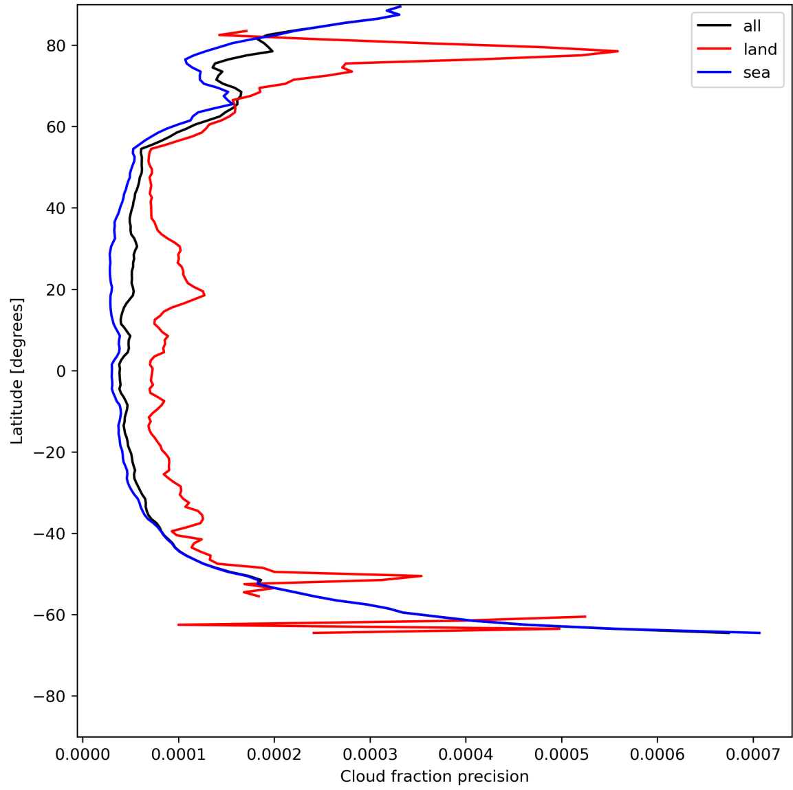
Figure 16: Zonal average of “Cloud fraction precision” for 2024-06-29 to 2024-07-01.
