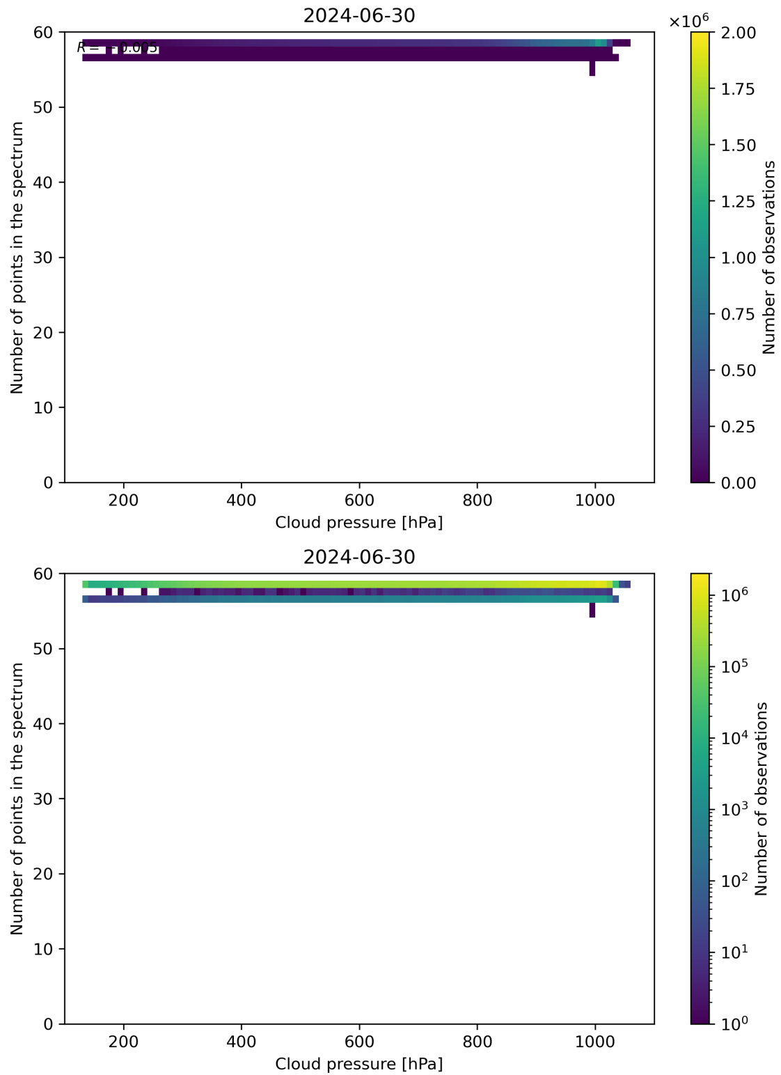
Figure 82: Scatter density plot of “Cloud pressure” against “Number of points in the spectrum” for 2024-06-29 to 2024-07-01.
