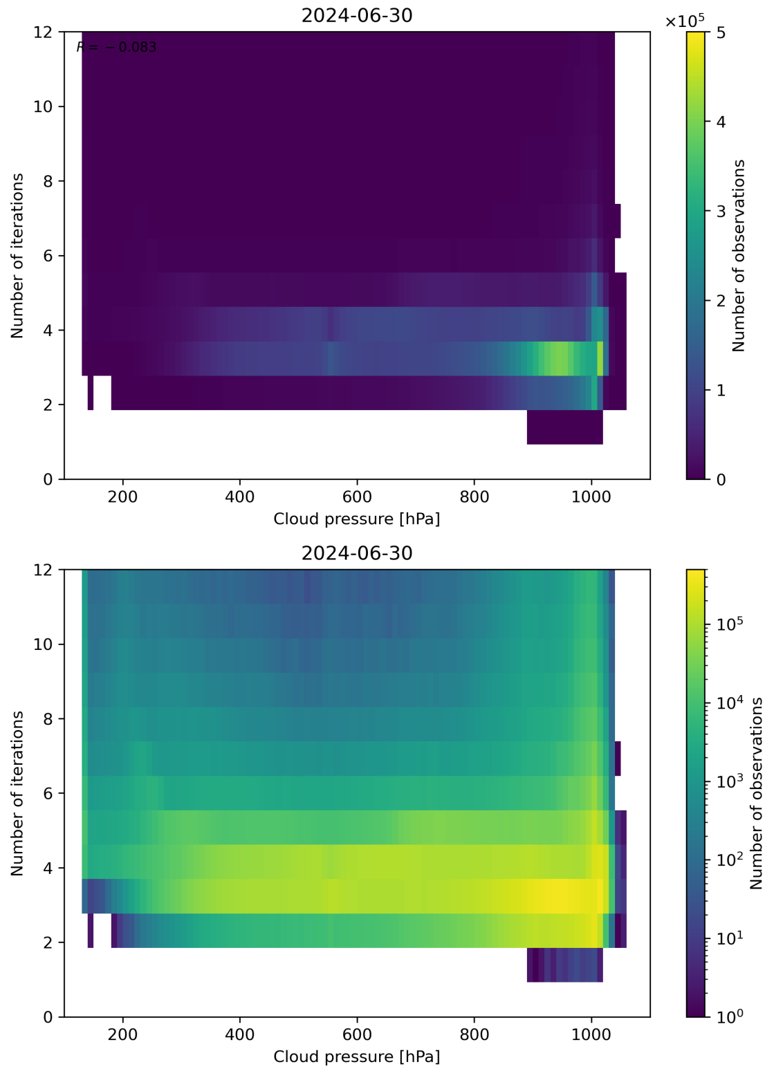
Figure 81: Scatter density plot of “Cloud pressure” against “Number of iterations” for 2024-06-29 to 2024-07-01.
