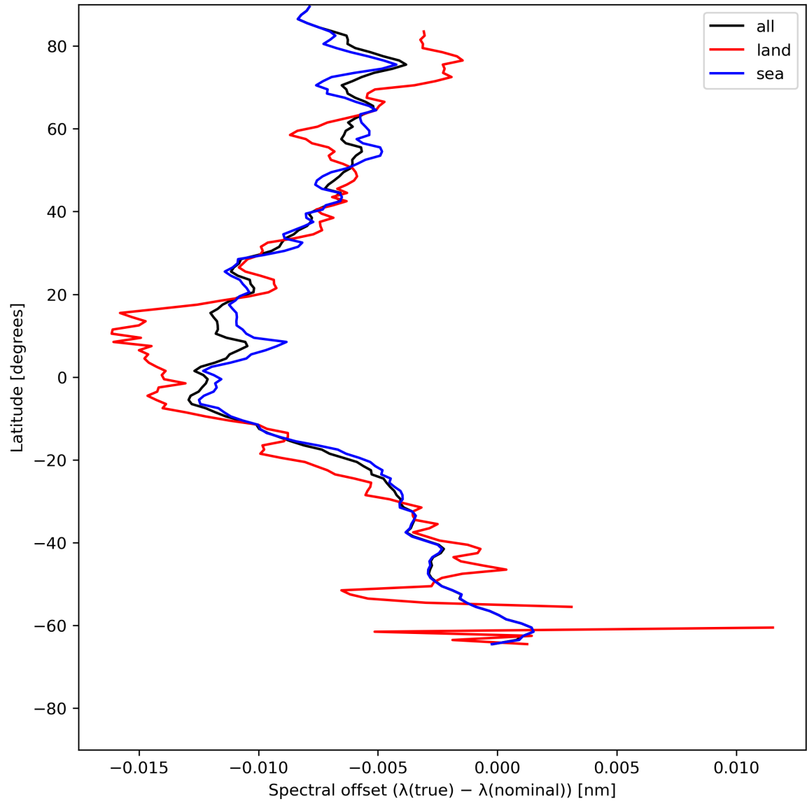
Figure 28: Zonal average of “Spectral offset ( \lambda(\text{true}) - \lambda(\text{nominal}) )” for 2024-06-29 to 2024-07-01.
