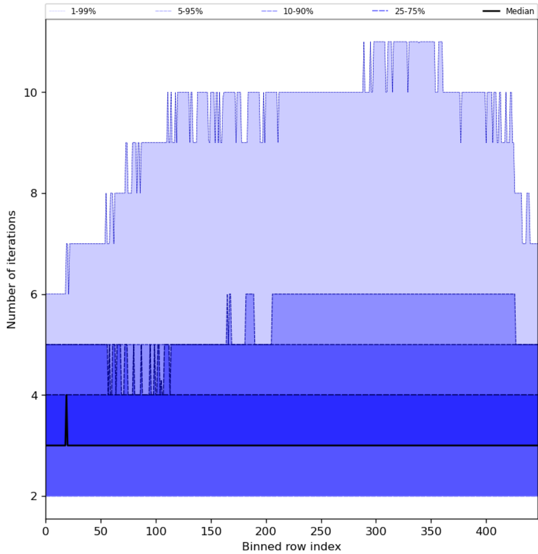
Figure 56: Along track statistics of “Number of iterations” for 2024-06-29 to 2024-07-01
