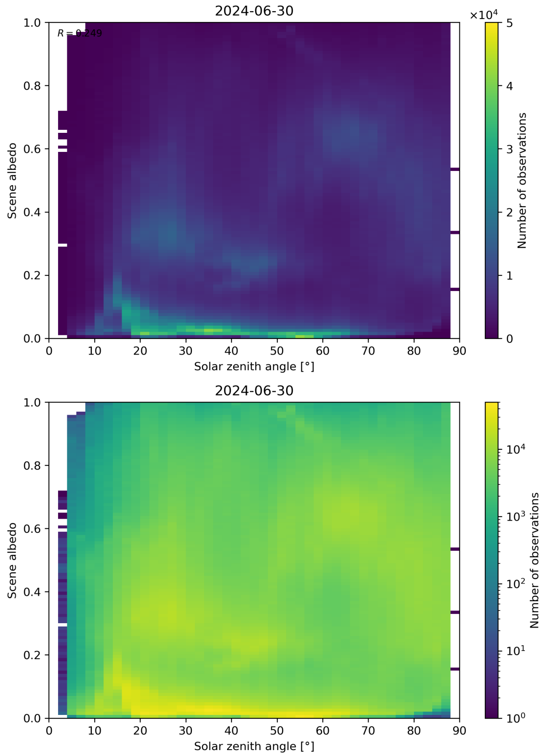
Figure 116: Scatter density plot of “Solar zenith angle” against “Scene albedo” for 2024-06-29 to 2024-07-01.
