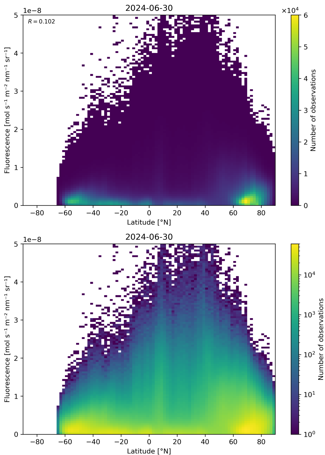
Figure 92: Scatter density plot of “Latitude” against “Fluorescence” for 2024-06-29 to 2024-07-01.
