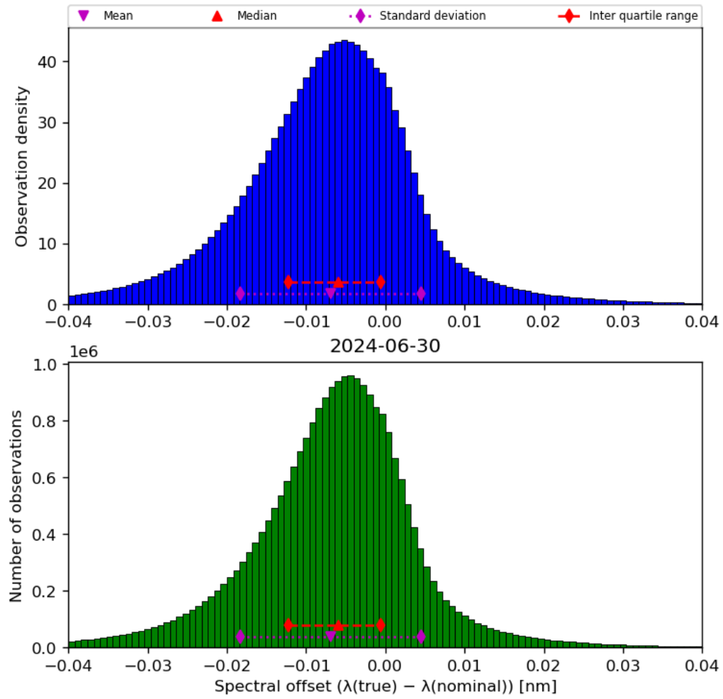
Figure 45: Histogram of “Spectral offset ( \lambda(\text{true}) - \lambda(\text{nominal}) )” for 2024-06-29 to 2024-07-01
