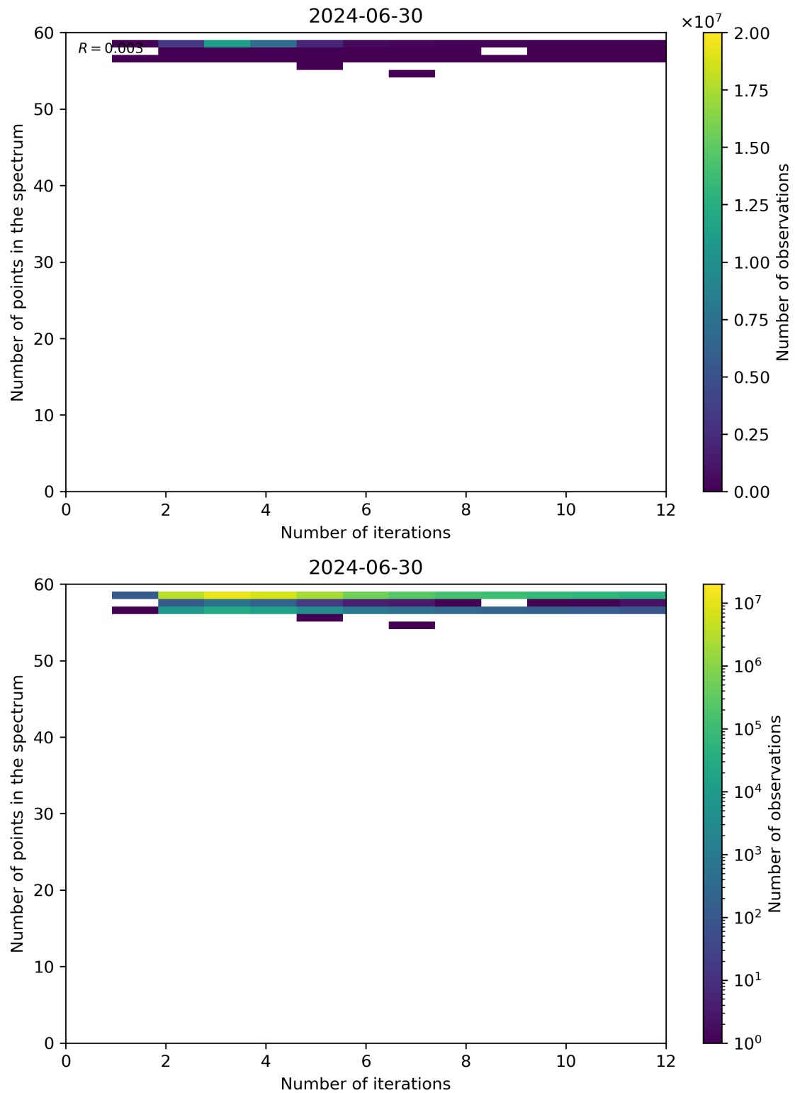
Figure 99: Scatter density plot of “Number of iterations” against “Number of points in the spectrum” for 2024-06-29 to 2024-07-01.
