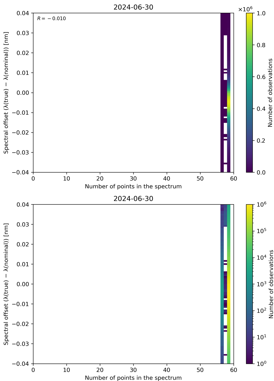
Figure 101: Scatter density plot of “Number of points in the spectrum” against “Spectral offset ( \lambda(\text{true}) - \lambda(\text{nominal}) )” for 2024-06-29 to 2024-07-01.
