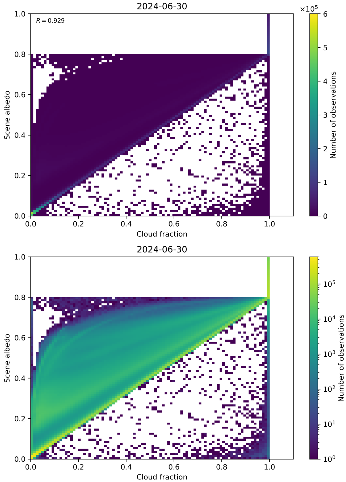
Figure 75: Scatter density plot of “Cloud fraction” against “Scene albedo” for 2024-06-29 to 2024-07-01.
