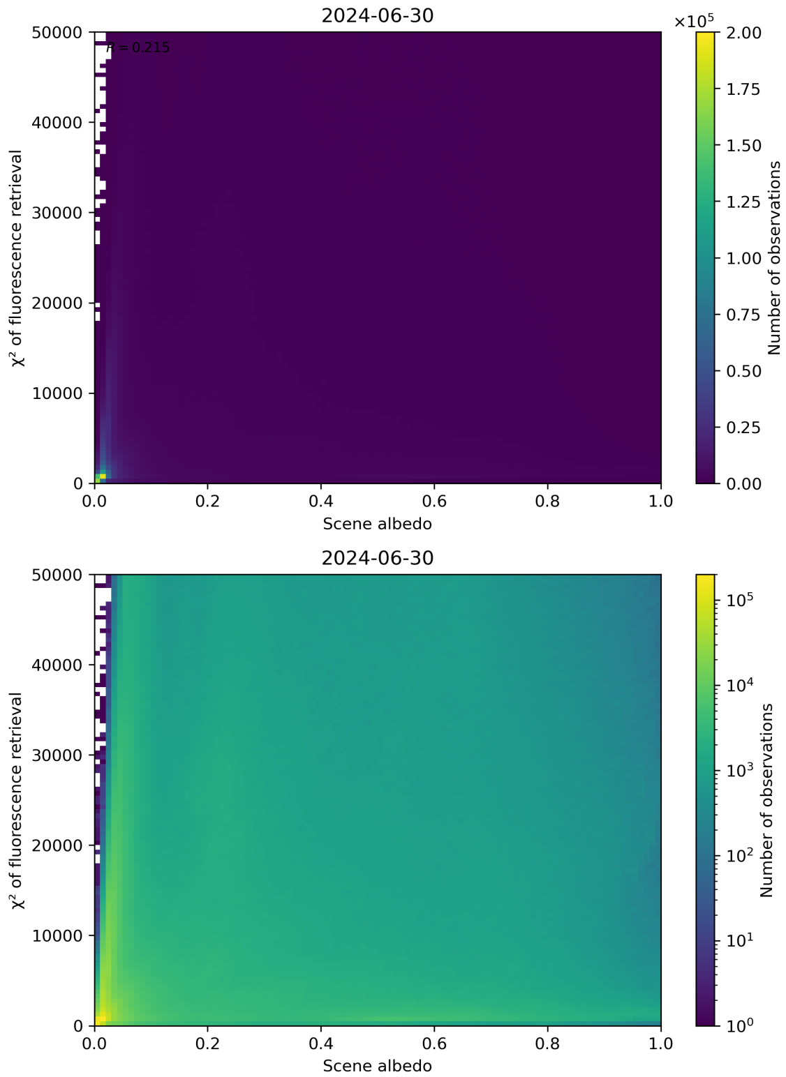
Figure 103: Scatter density plot of “Scene albedo” against “ \chi^2 of fluorescence retrieval” for 2024-06-29 to 2024-07-01.
