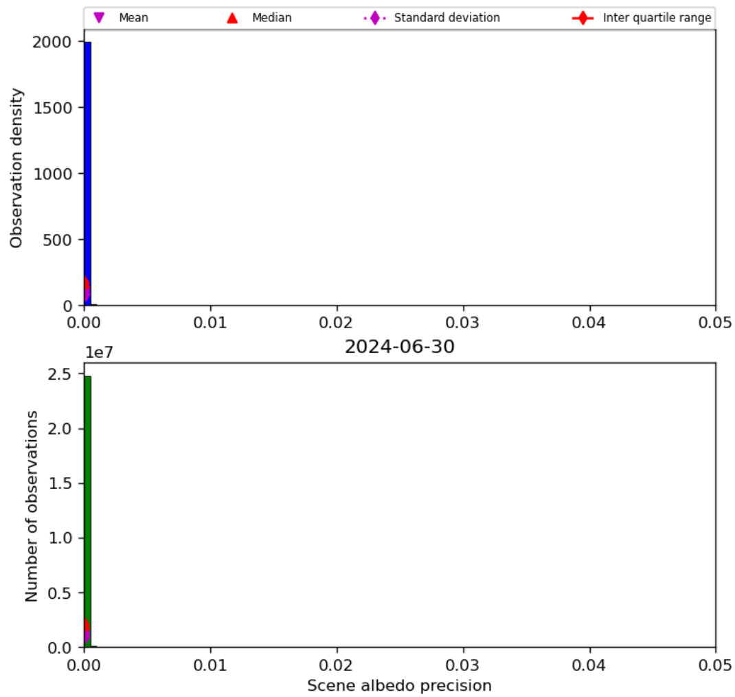
Figure 35: Histogram of “Scene albedo precision” for 2024-06-29 to 2024-07-01
