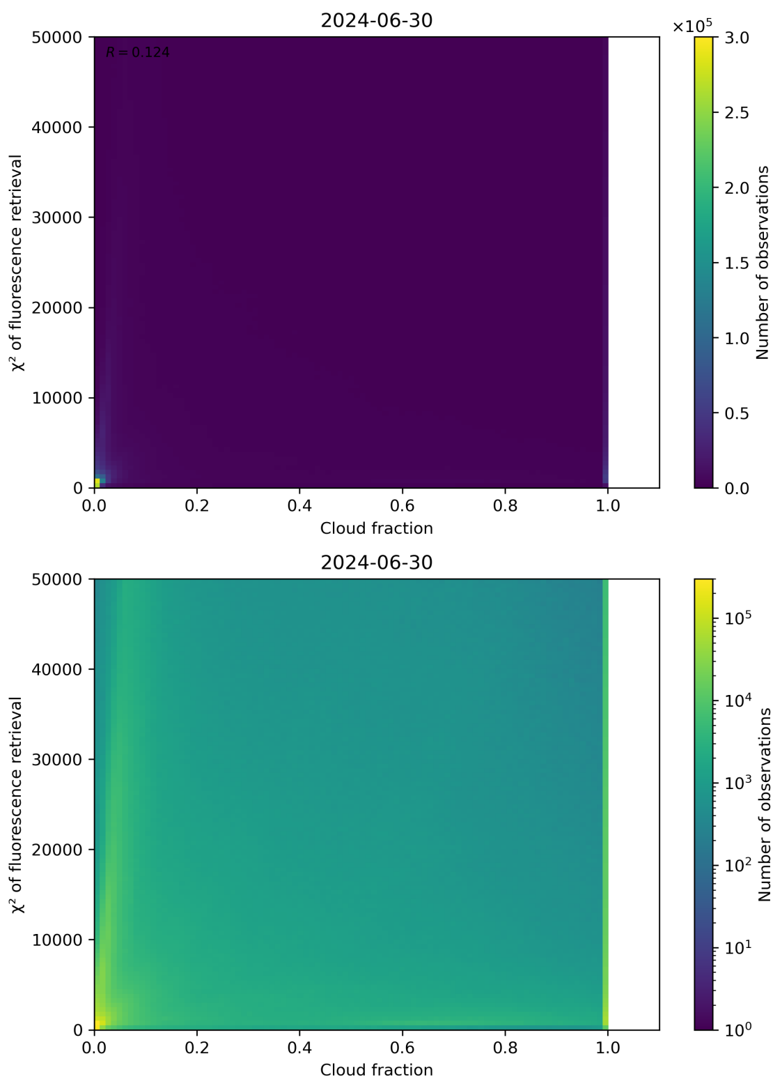
Figure 71: Scatter density plot of “Cloud fraction” against “ \chi^2 of fluorescence retrieval” for 2024-06-29 to 2024-07-01.
