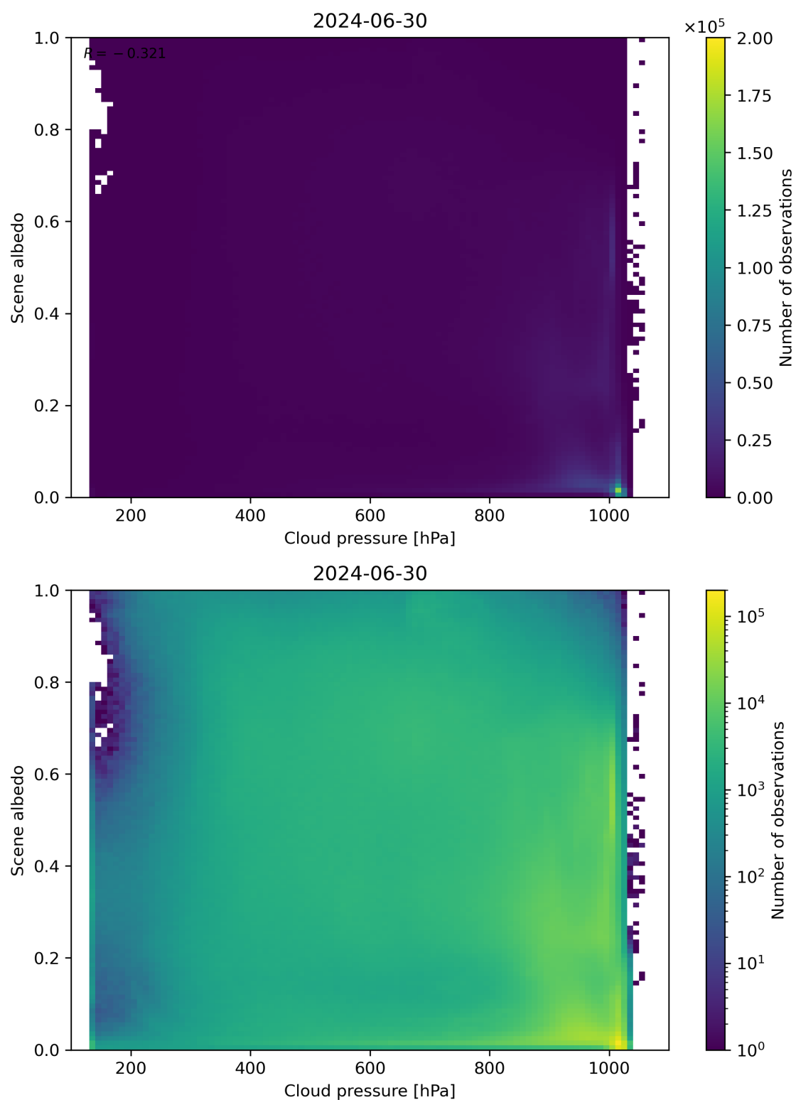
Figure 83: Scatter density plot of “Cloud pressure” against “Scene albedo” for 2024-06-29 to 2024-07-01.
