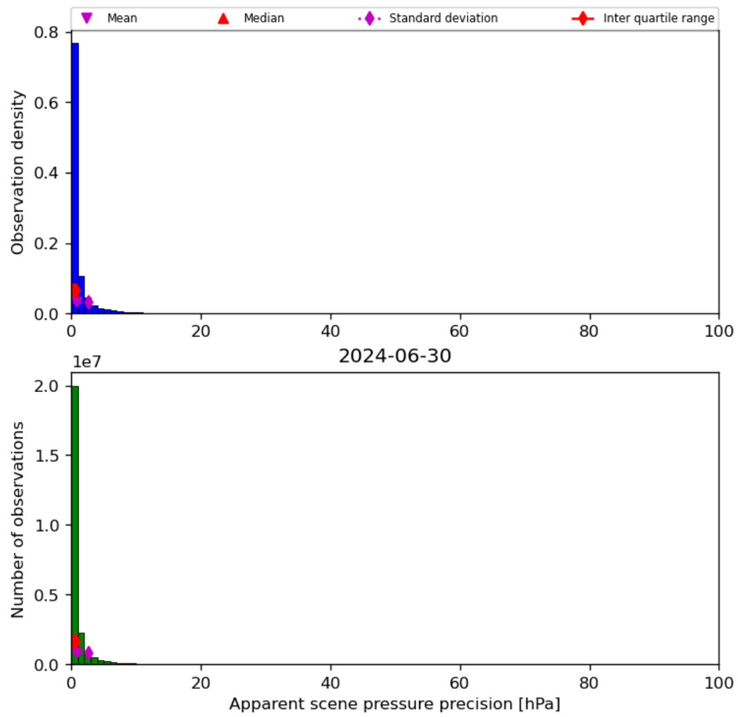
Figure 37: Histogram of “Apparent scene pressure precision” for 2024-06-29 to 2024-07-01
