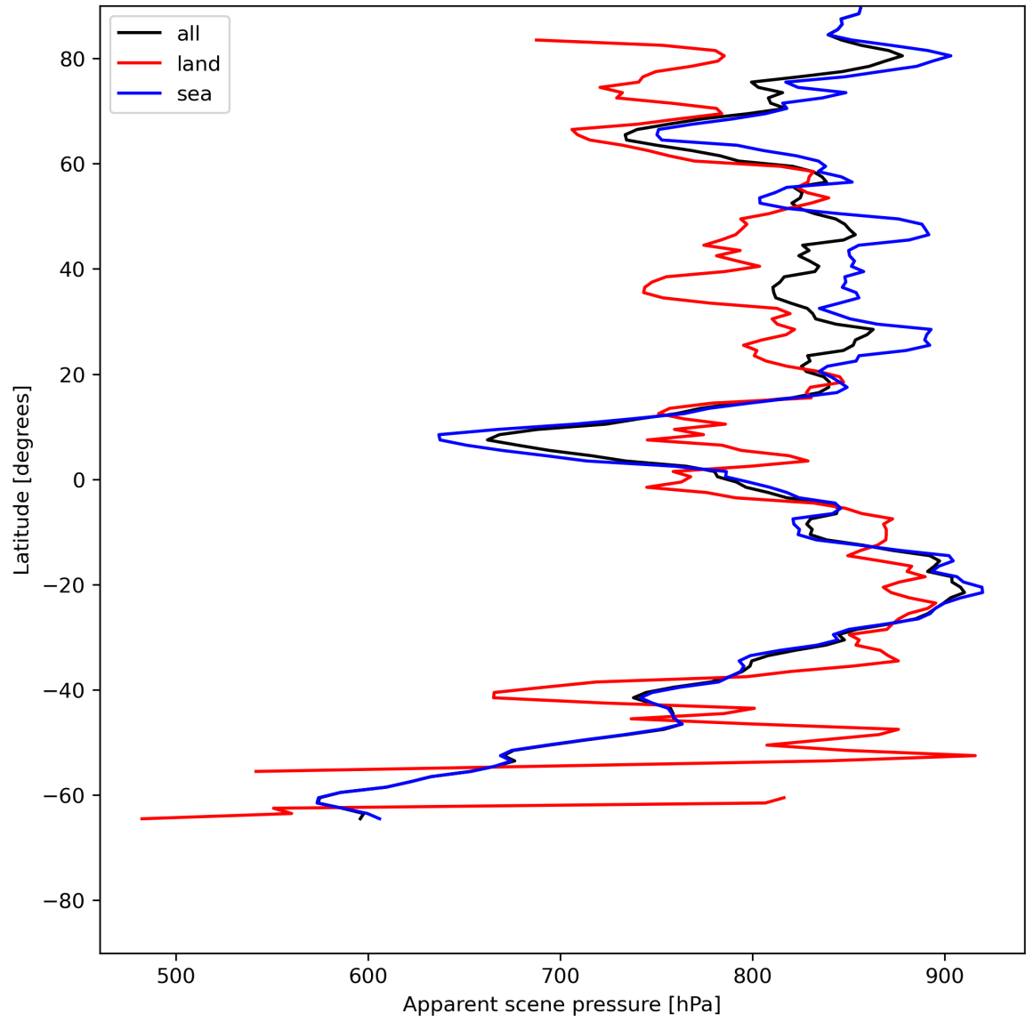
Figure 19: Zonal average of “Apparent scene pressure” for 2024-06-29 to 2024-07-01.
