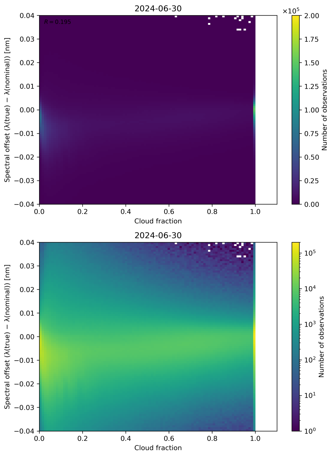
Figure 76: Scatter density plot of “Cloud fraction” against “Spectral offset ( \lambda(\text{true}) - \lambda(\text{nominal}) )” for 2024-06-29 to 2024-07-01.
