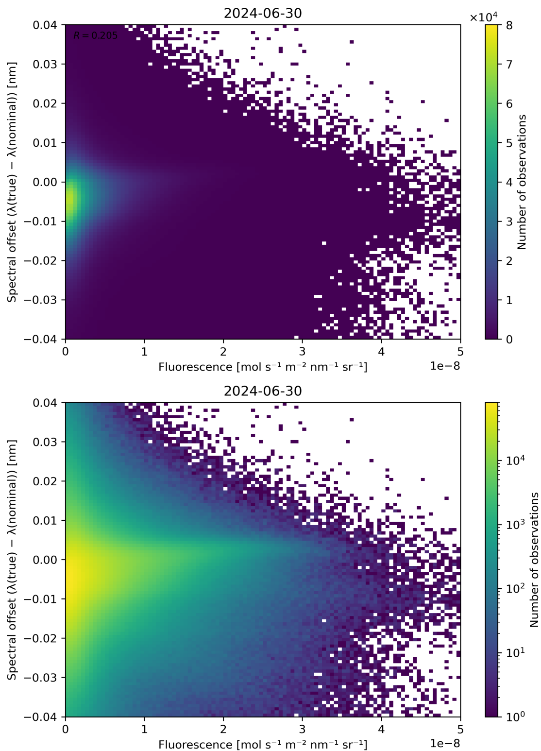
Figure 87: Scatter density plot of “Fluorescence” against “Spectral offset ( \lambda(\text{true}) - \lambda(\text{nominal}) )” for 2024-06-29 to 2024-07-01.
