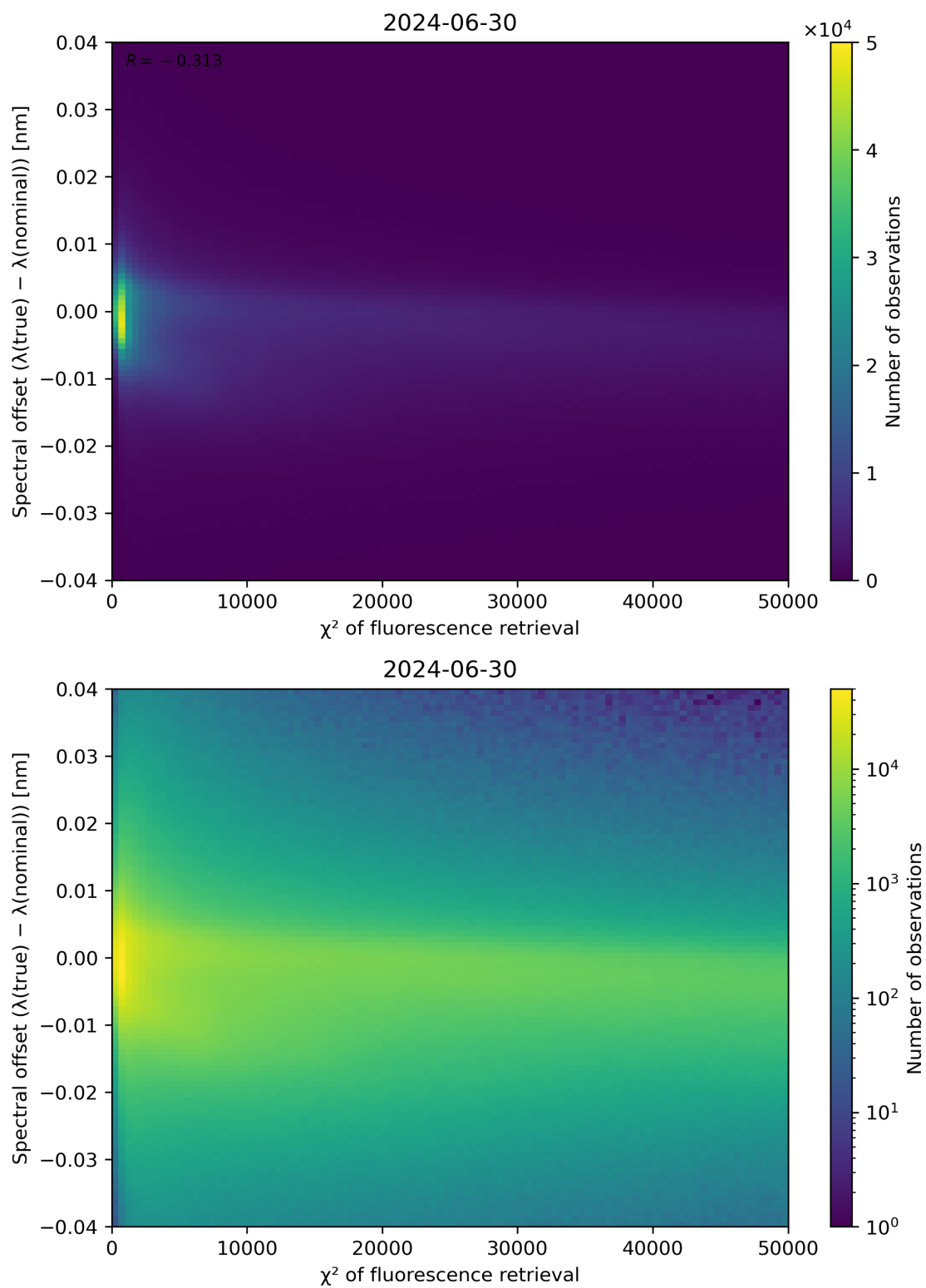
Figure 69: Scatter density plot of " \chi^2 of fluorescence retrieval" against "Spectral offset ( \lambda(\text{true}) - \lambda(\text{nominal}) )" for 2024-06-29 to 2024-07-01.
