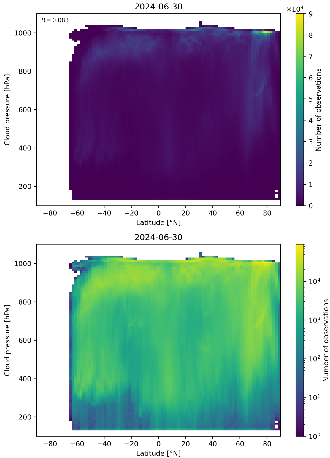
Figure 91: Scatter density plot of “Latitude” against “Cloud pressure” for 2024-06-29 to 2024-07-01.
