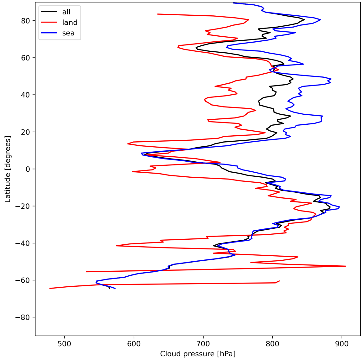
Figure 13: Zonal average of “Cloud pressure” for 2024-06-29 to 2024-07-01.
