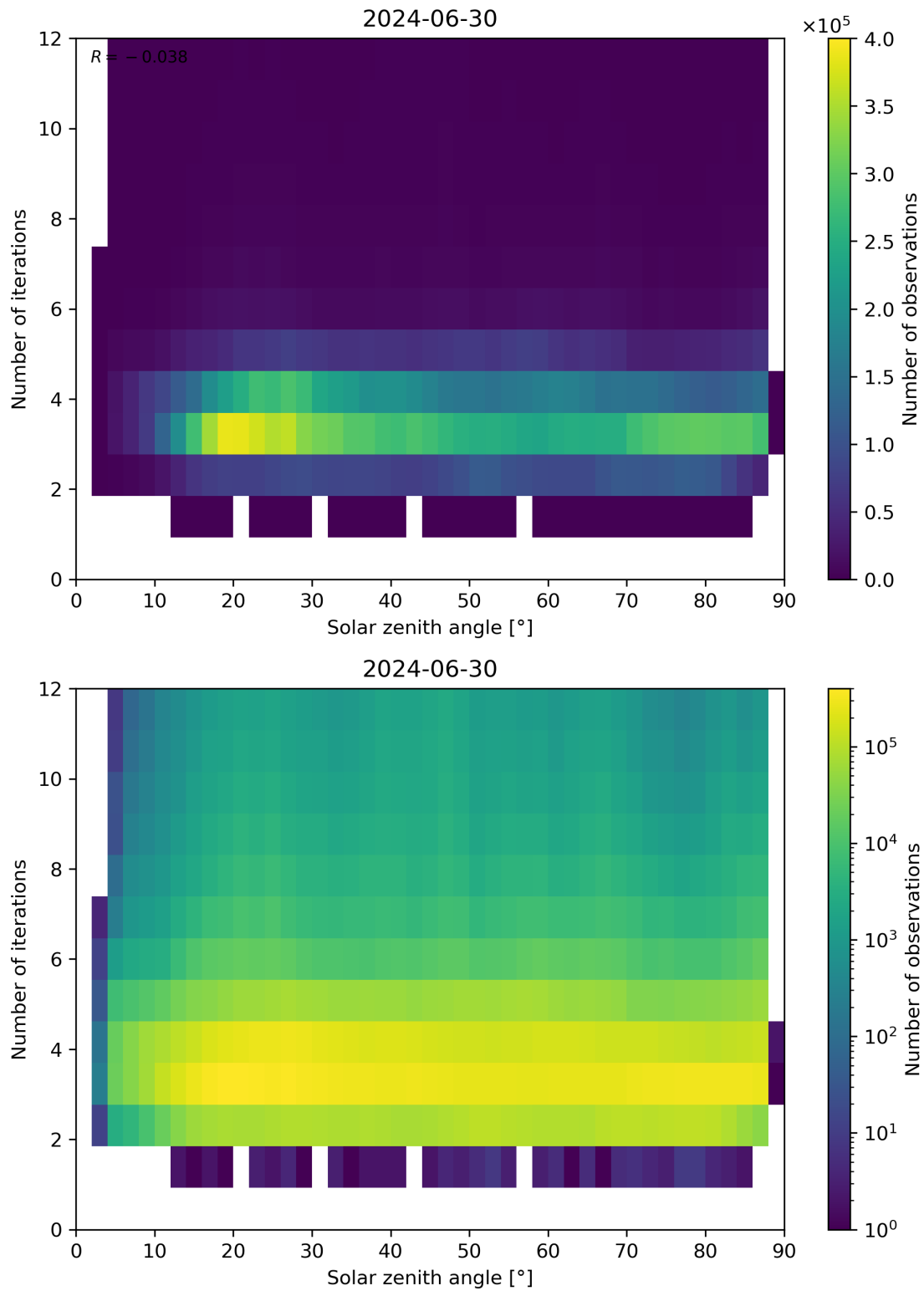
Figure 114: Scatter density plot of “Solar zenith angle” against “Number of iterations” for 2024-06-29 to 2024-07-01.
