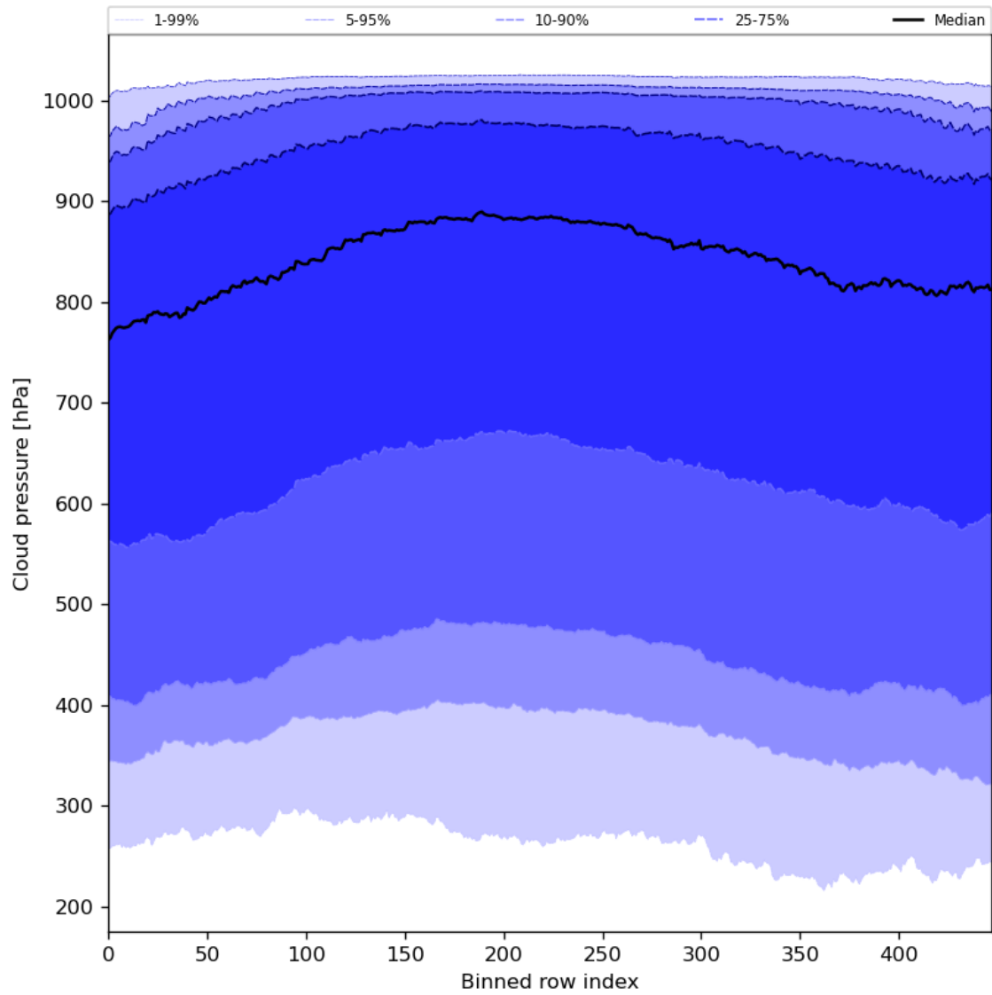
Figure 47: Along track statistics of “Cloud pressure” for 2024-06-29 to 2024-07-01
