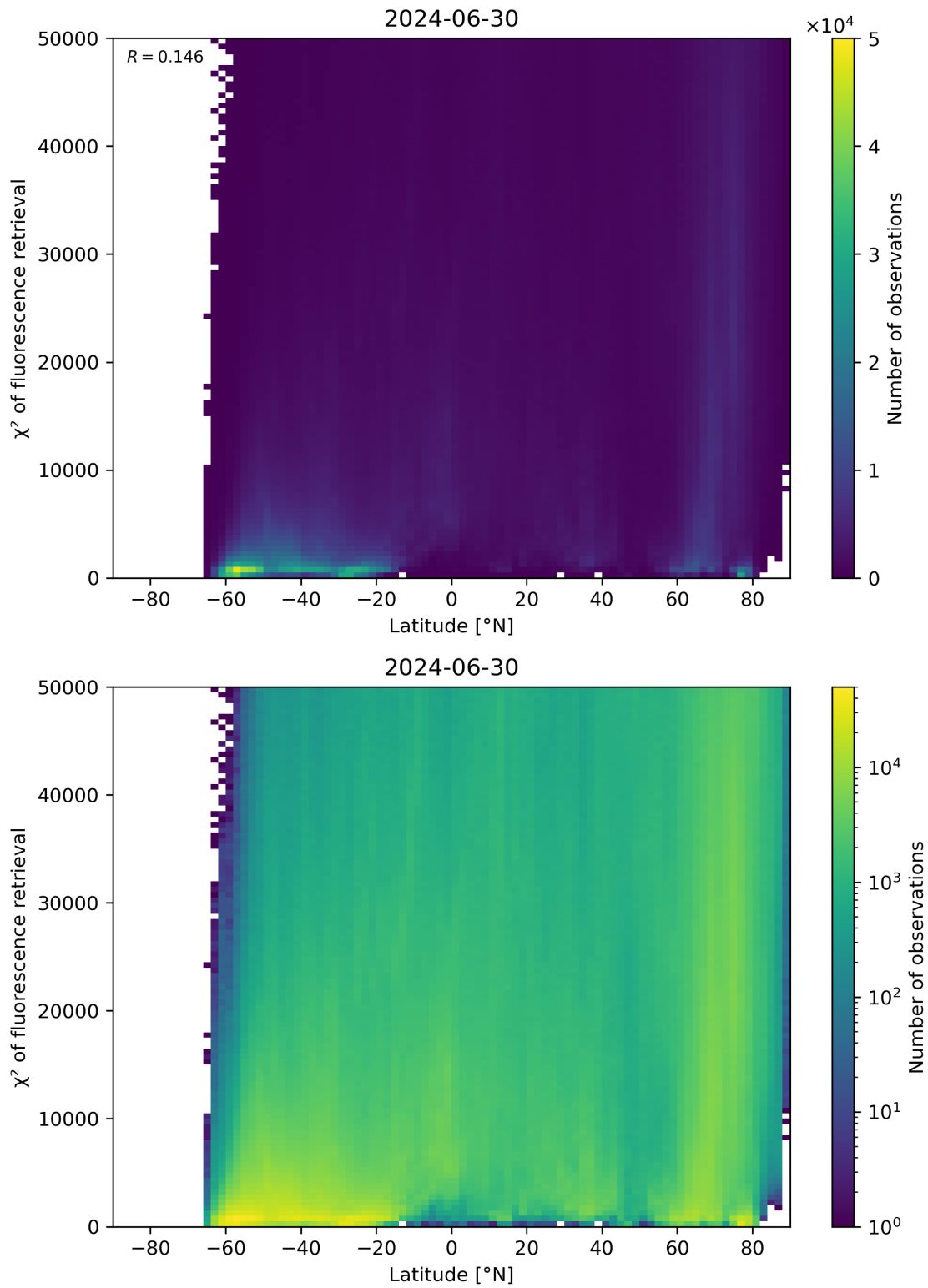
Figure 89: Scatter density plot of “Latitude” against “ \chi^2 of fluorescence retrieval” for 2024-06-29 to 2024-07-01.
