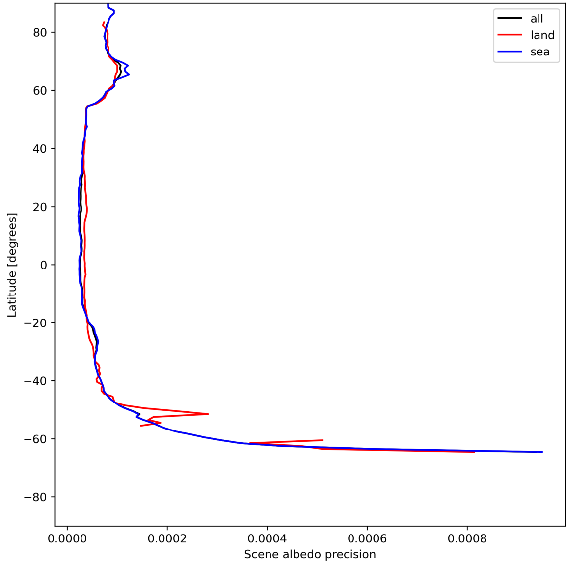
Figure 18: Zonal average of “Scene albedo precision” for 2024-06-29 to 2024-07-01.
