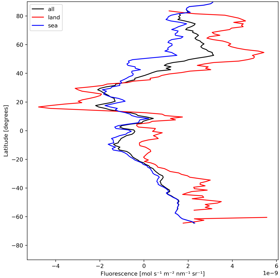
Figure 23: Zonal average of “Fluorescence” for 2024-06-29 to 2024-07-01.
