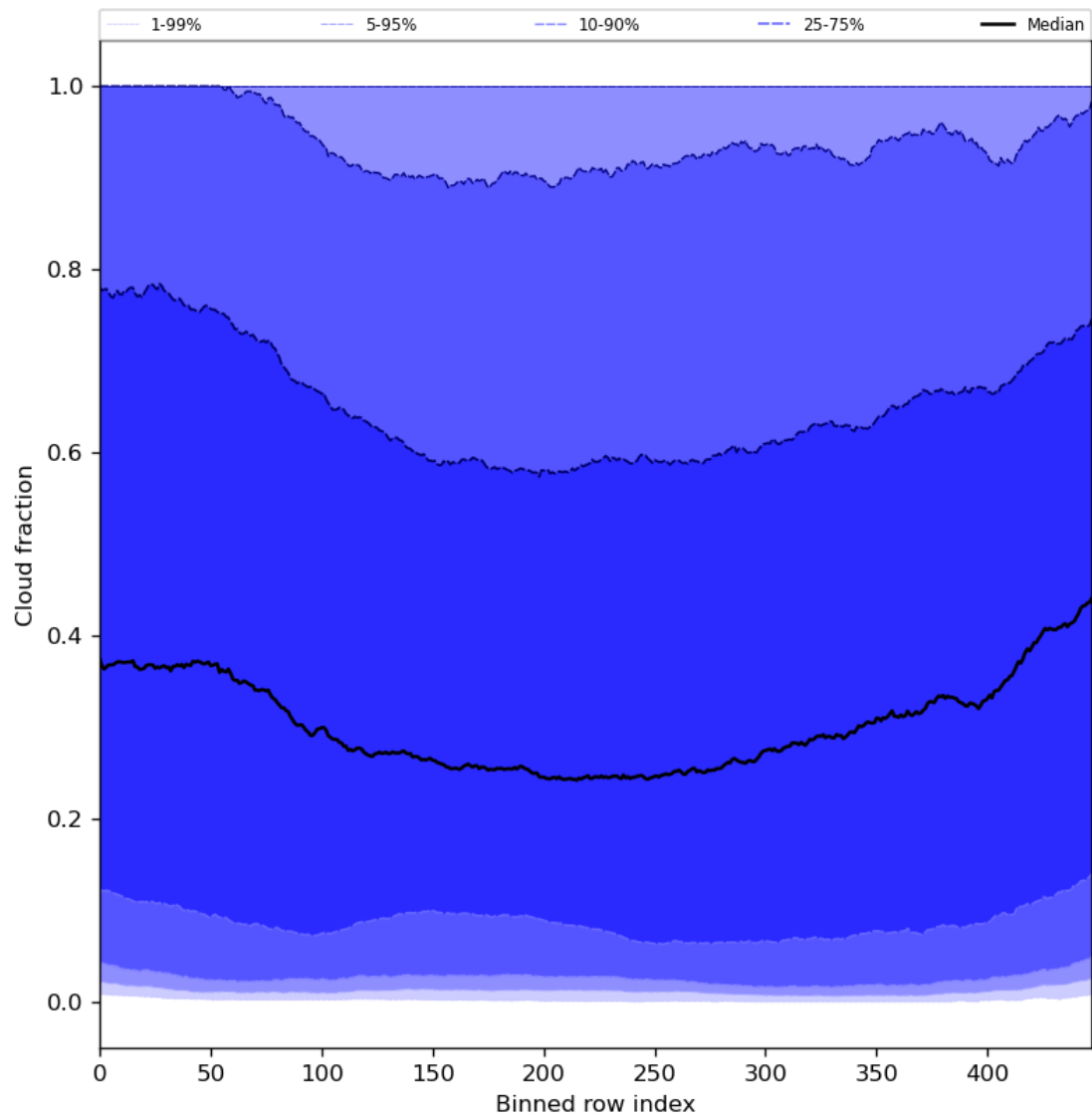
Figure 49: Along track statistics of “Cloud fraction” for 2024-06-29 to 2024-07-01
