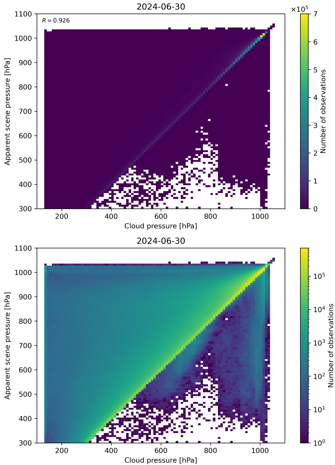
Figure 77: Scatter density plot of “Cloud pressure” against “Apparent scene pressure” for 2024-06-29 to 2024-07-01.
