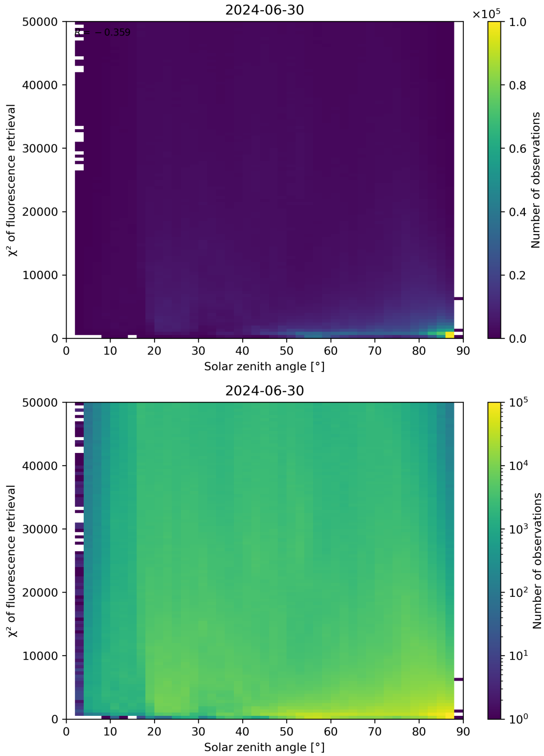
Figure 109: Scatter density plot of “Solar zenith angle” against “ \chi^2 of fluorescence retrieval” for 2024-06-29 to 2024-07-01.
