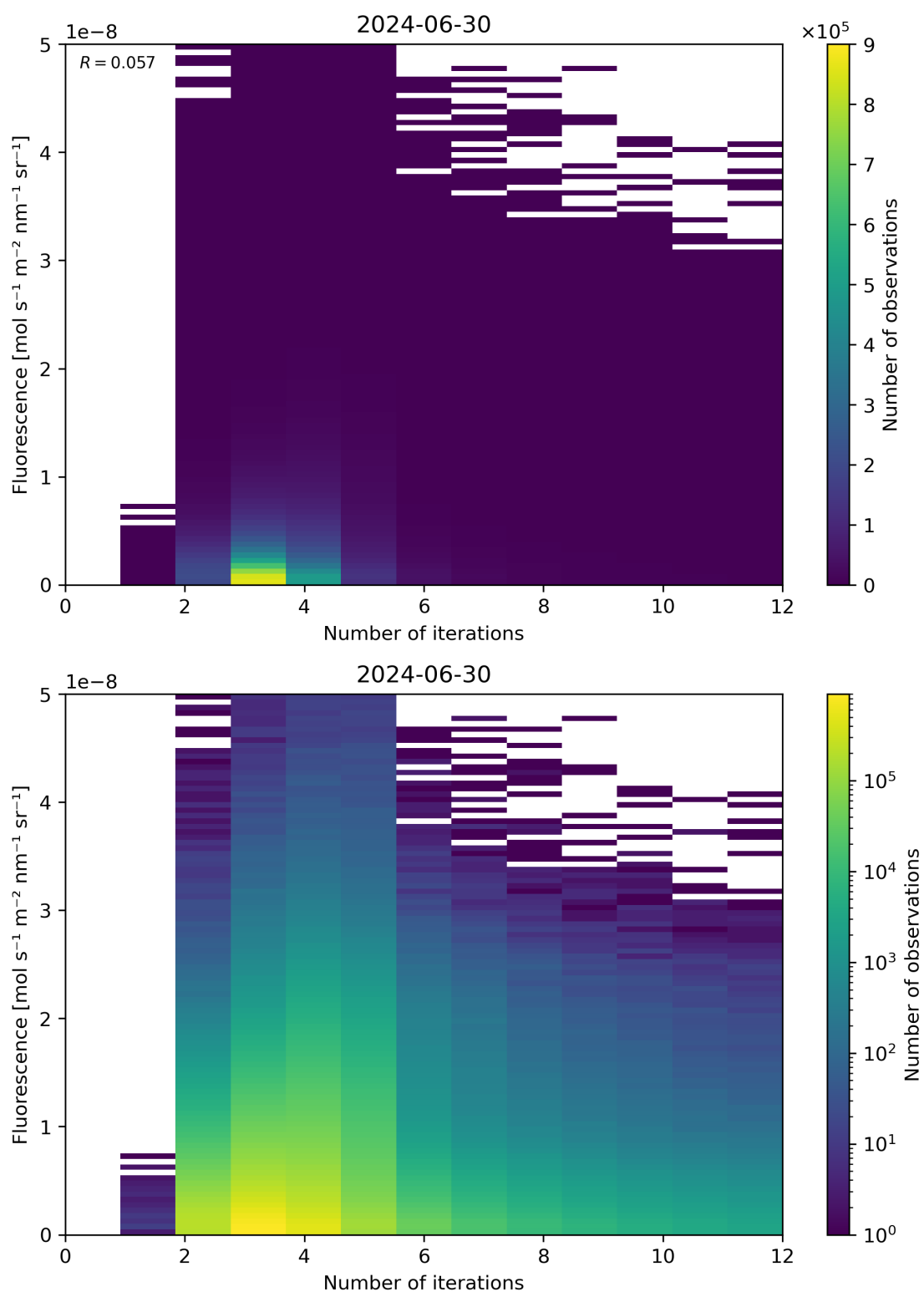
Figure 98: Scatter density plot of “Number of iterations” against “Fluorescence” for 2024-06-29 to 2024-07-01.
