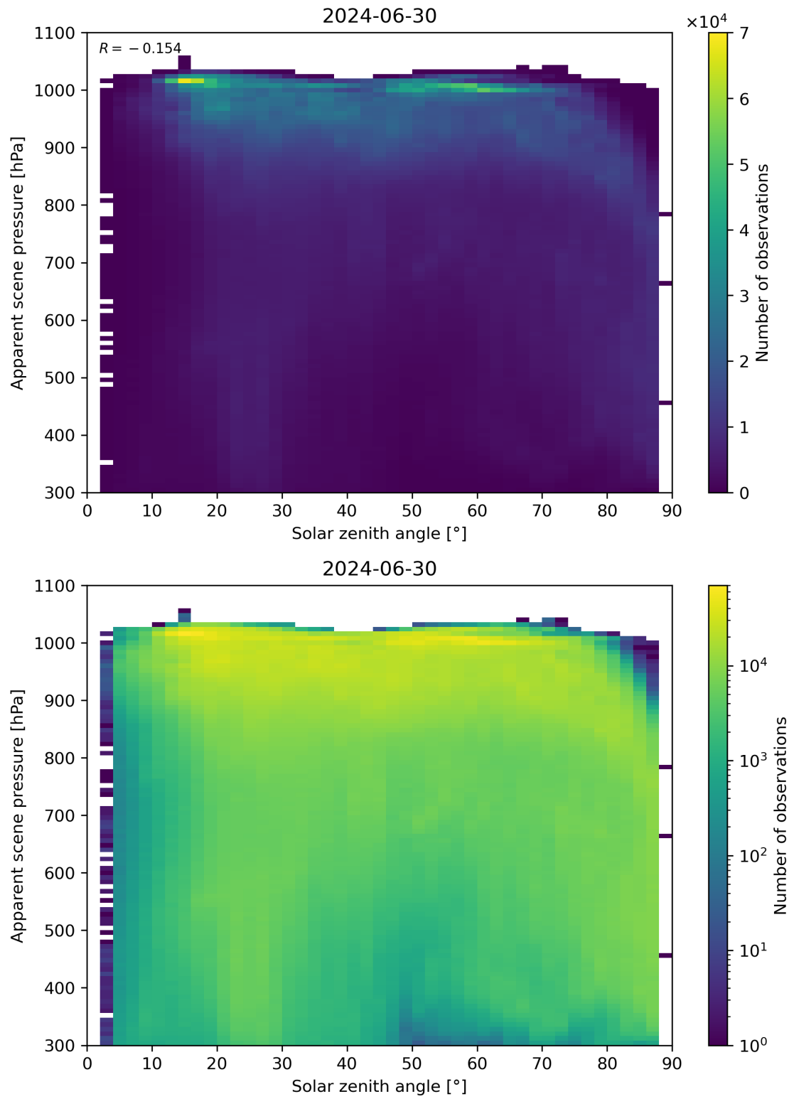
Figure 108: Scatter density plot of “Solar zenith angle” against “Apparent scene pressure” for 2024-06-29 to 2024-07-01.
