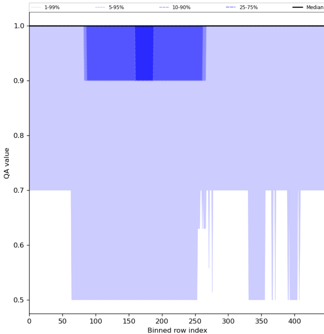
Figure 46: Along track statistics of “QA value” for 2024-06-29 to 2024-07-01
