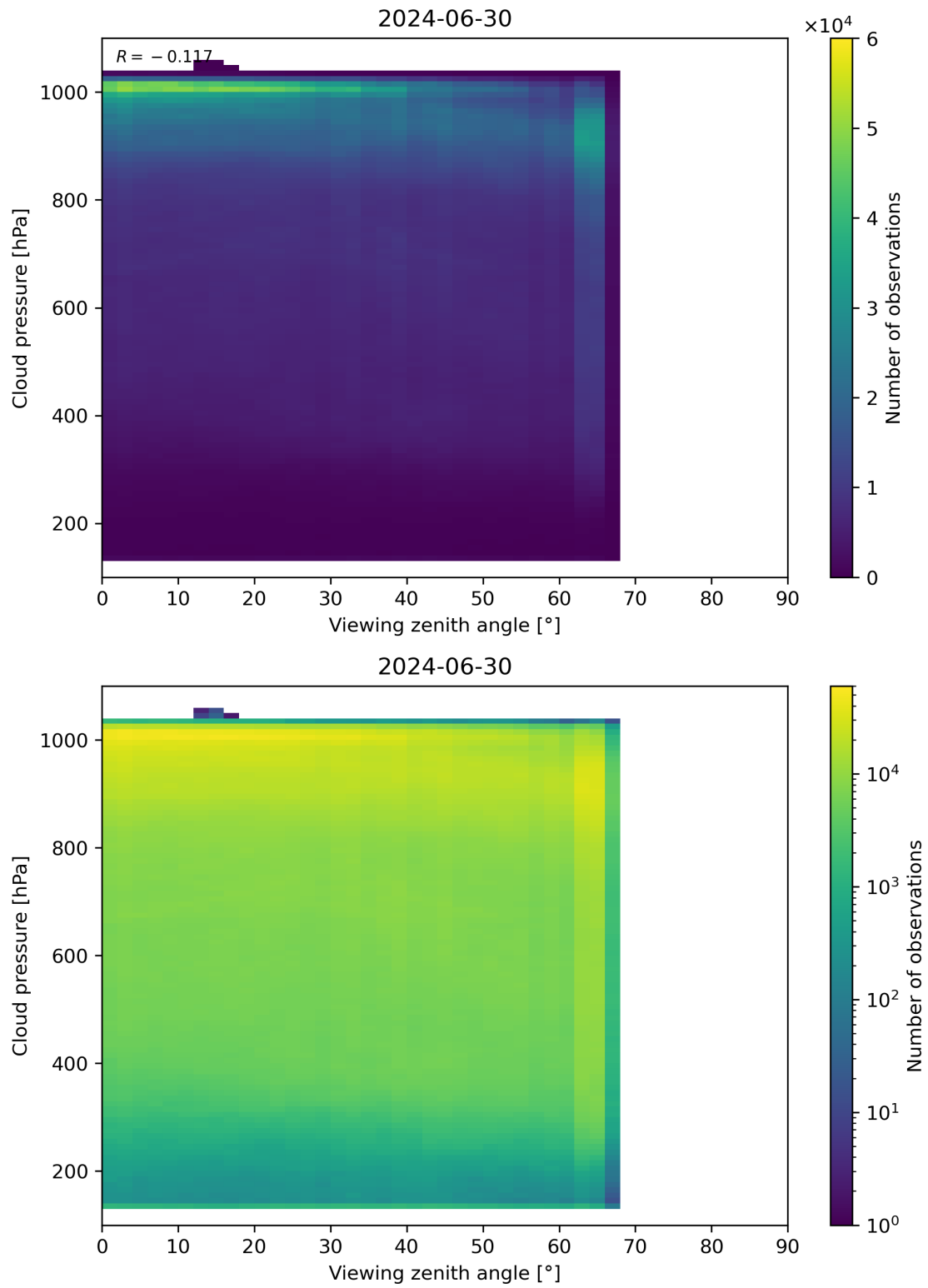
Figure 121: Scatter density plot of “Viewing zenith angle” against “Cloud pressure” for 2024-06-29 to 2024-07-01.
