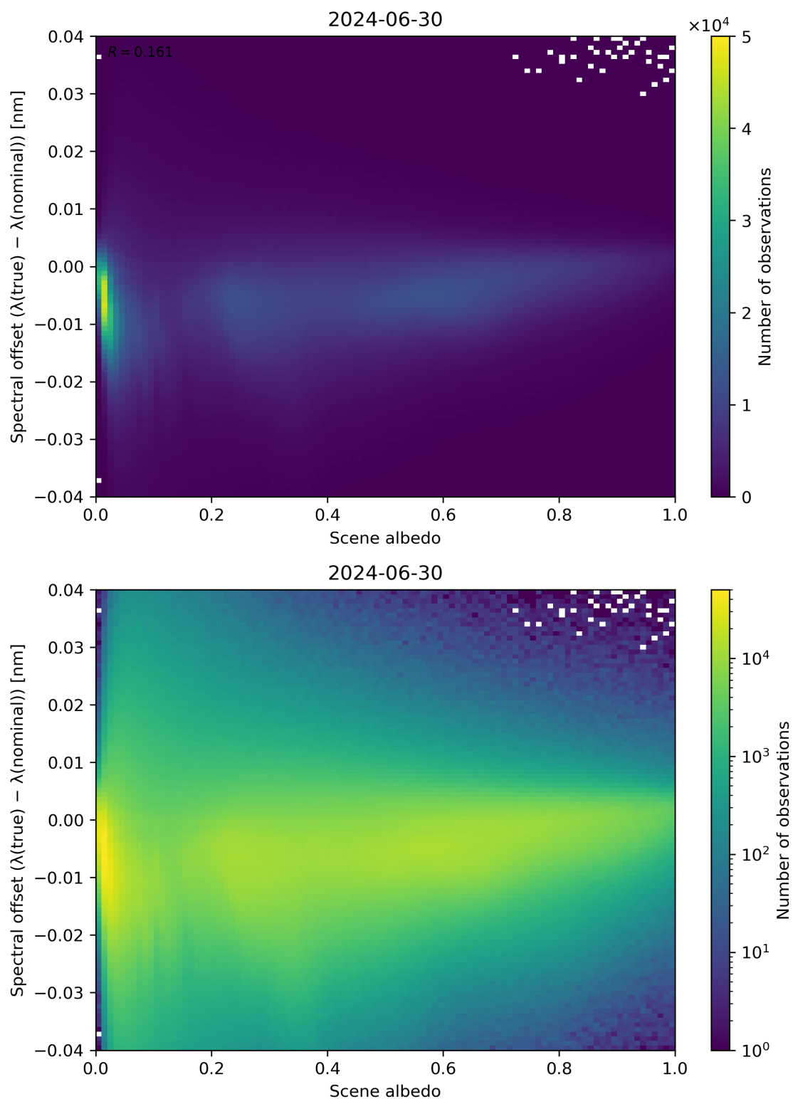
Figure 107: Scatter density plot of “Scene albedo” against “Spectral offset ( \lambda(\text{true}) - \lambda(\text{nominal}) )” for 2024-06-29 to 2024-07-01.
