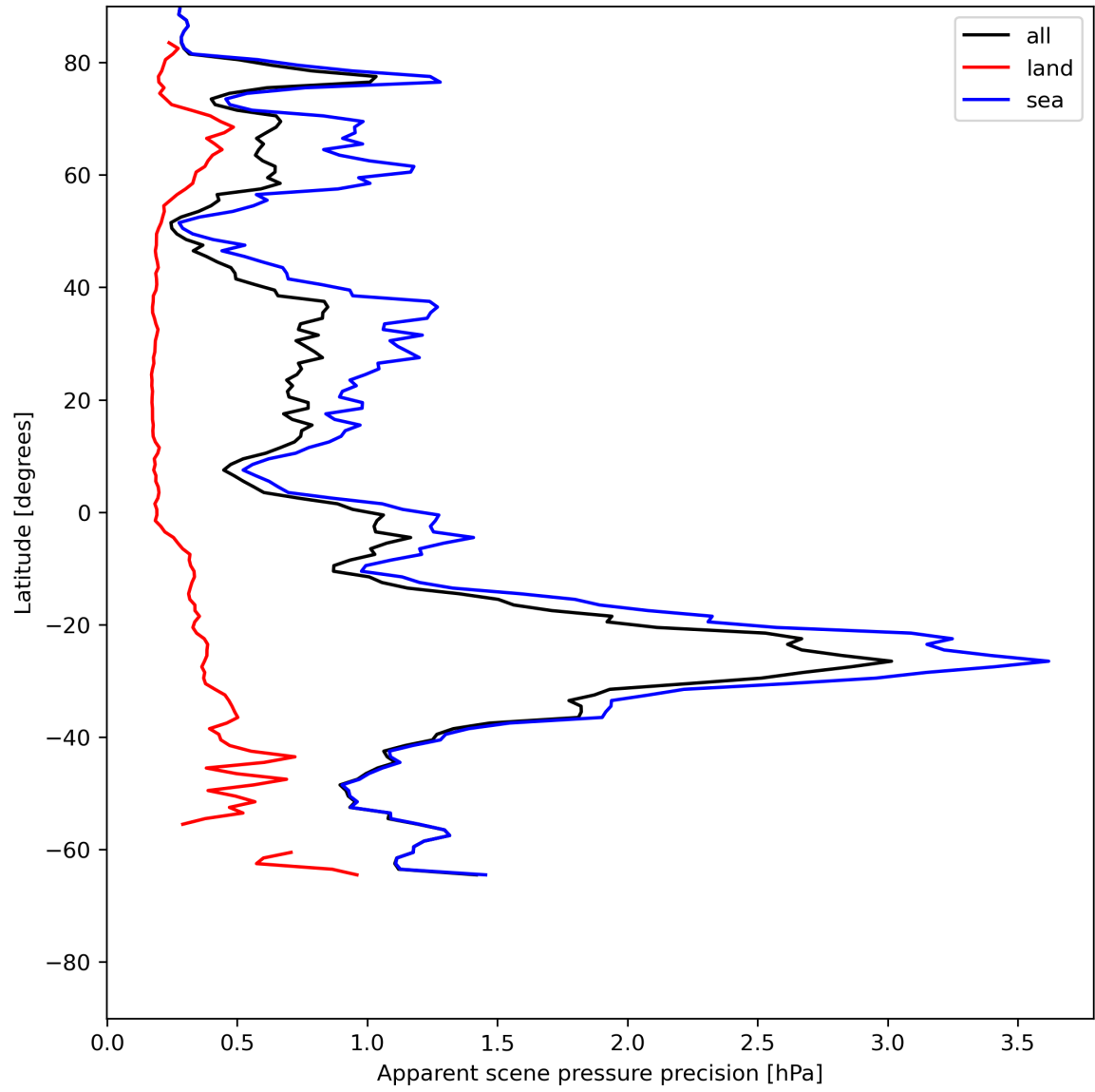
Figure 20: Zonal average of “Apparent scene pressure precision” for 2024-06-29 to 2024-07-01.
