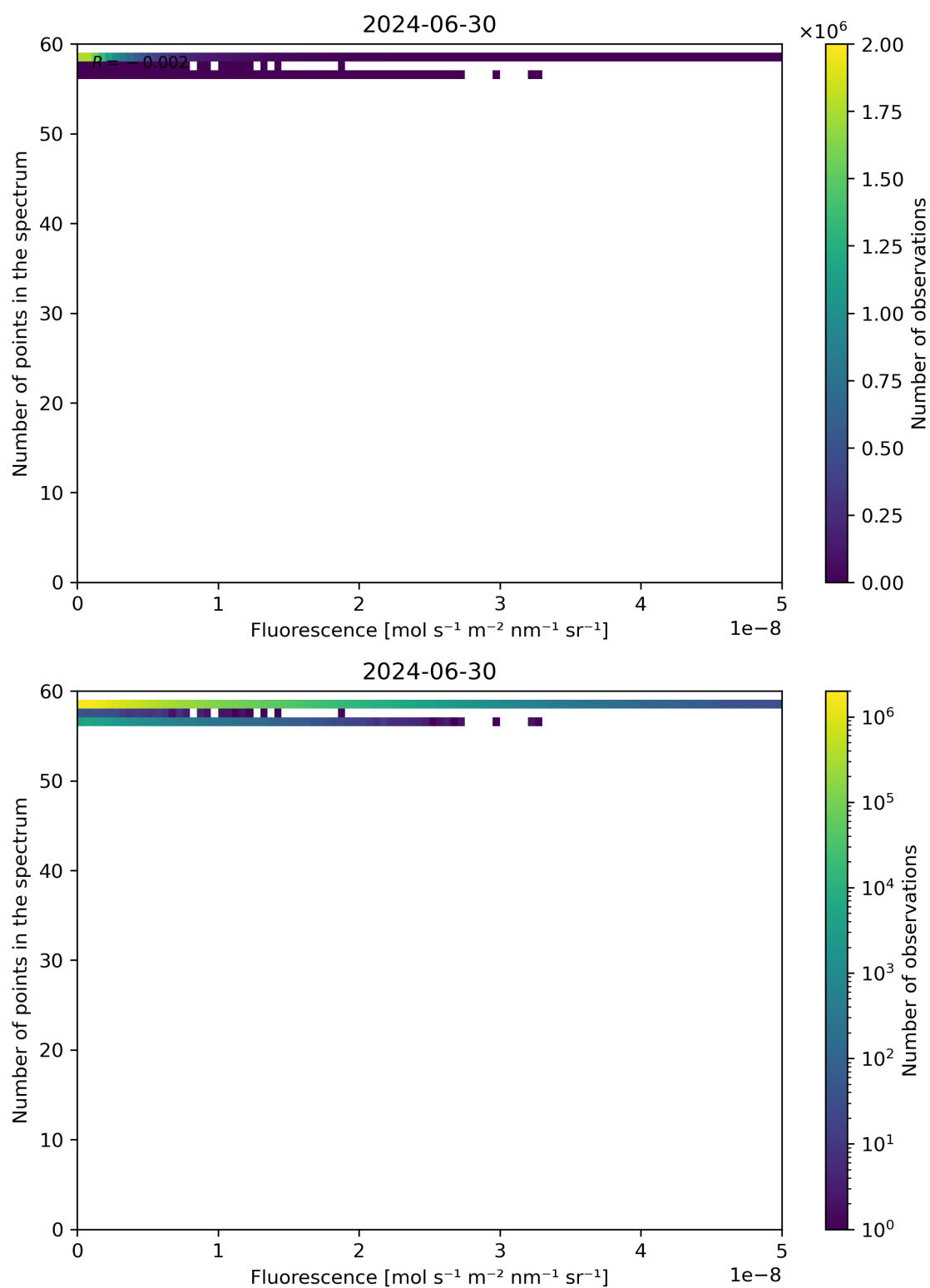
Figure 86: Scatter density plot of “Fluorescence” against “Number of points in the spectrum” for 2024-06-29 to 2024-07-01.
