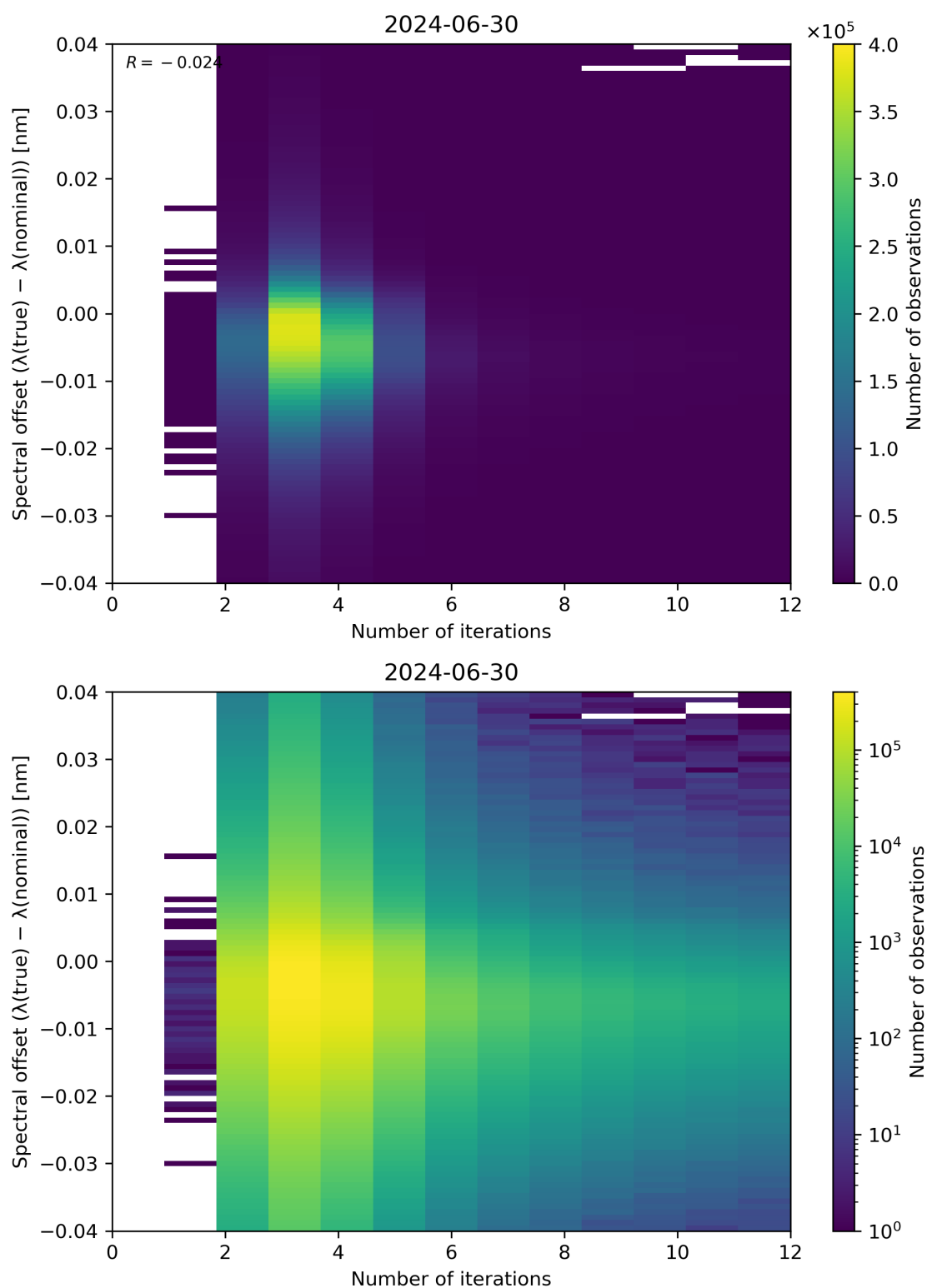
Figure 100: Scatter density plot of “Number of iterations” against “Spectral offset ( \lambda(\text{true}) - \lambda(\text{nominal}) )” for 2024-06-29 to 2024-07-01.
