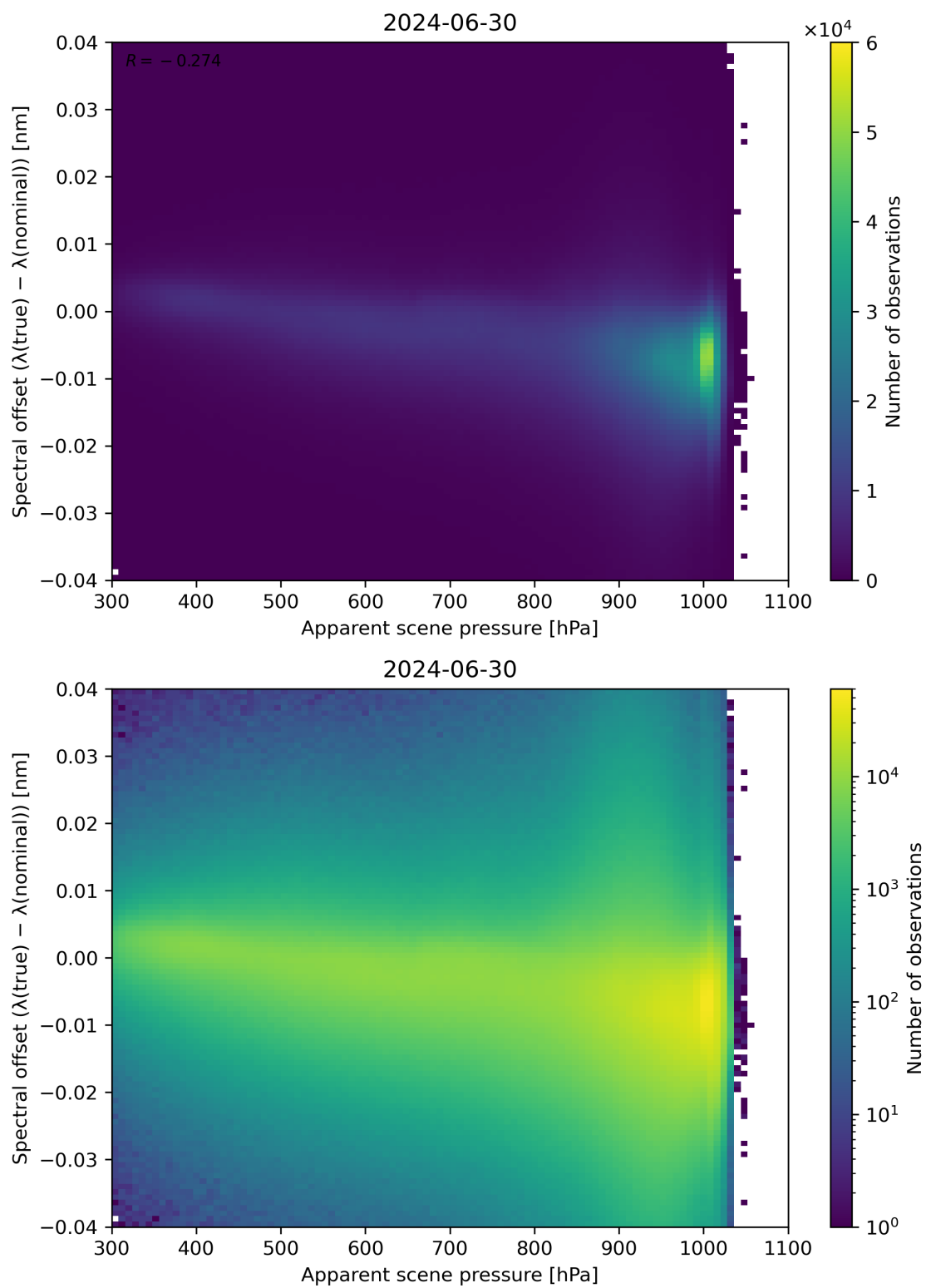
Figure 67: Scatter density plot of “Apparent scene pressure” against “Spectral offset ( \lambda(\text{true}) - \lambda(\text{nominal}) )” for 2024-06-29 to 2024-07-01.
