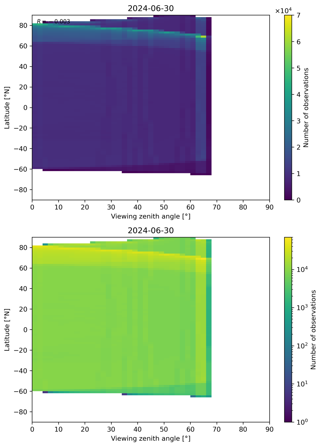
Figure 123: Scatter density plot of “Viewing zenith angle” against “Latitude” for 2024-06-29 to 2024-07-01.
