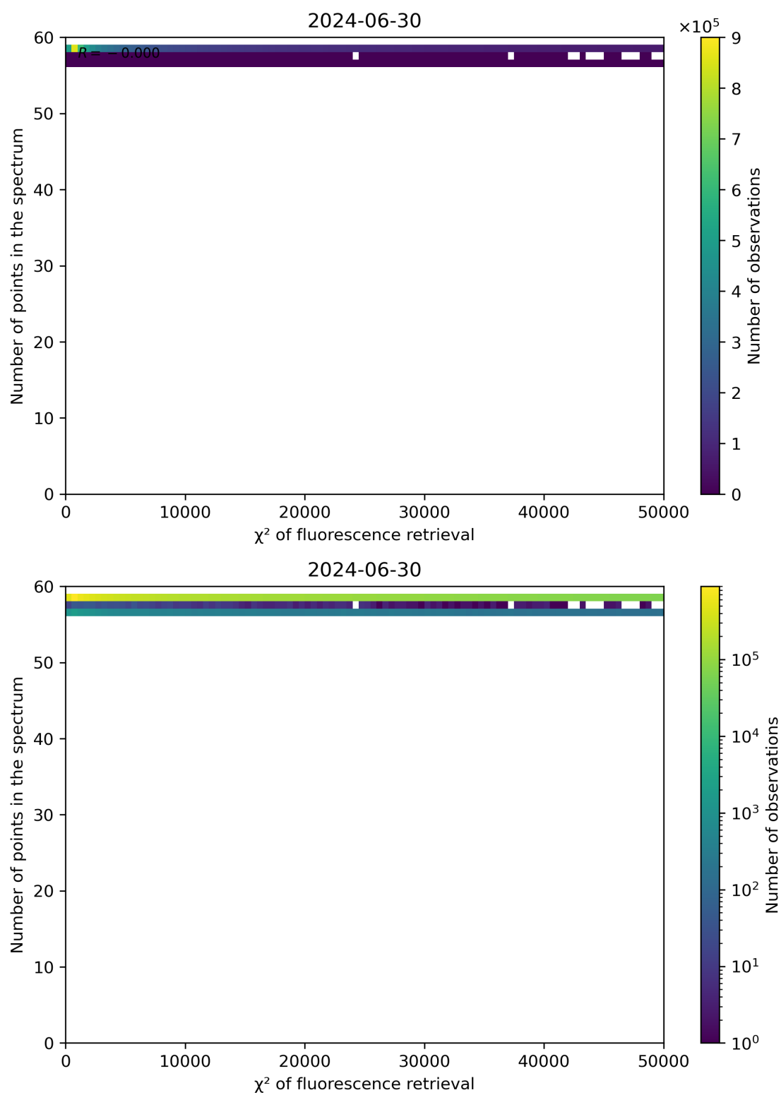
Figure 68: Scatter density plot of " \chi^2 of fluorescence retrieval" against "Number of points in the spectrum" for 2024-06-29 to 2024-07-01.
