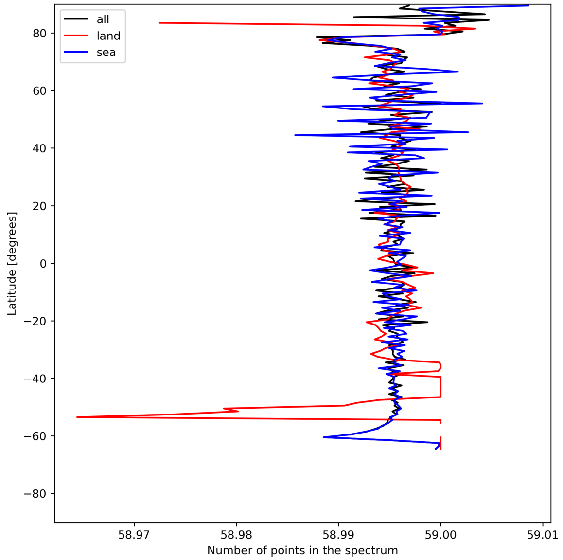
Figure 27: Zonal average of “Number of points in the spectrum” for 2024-06-29 to 2024-07-01.
