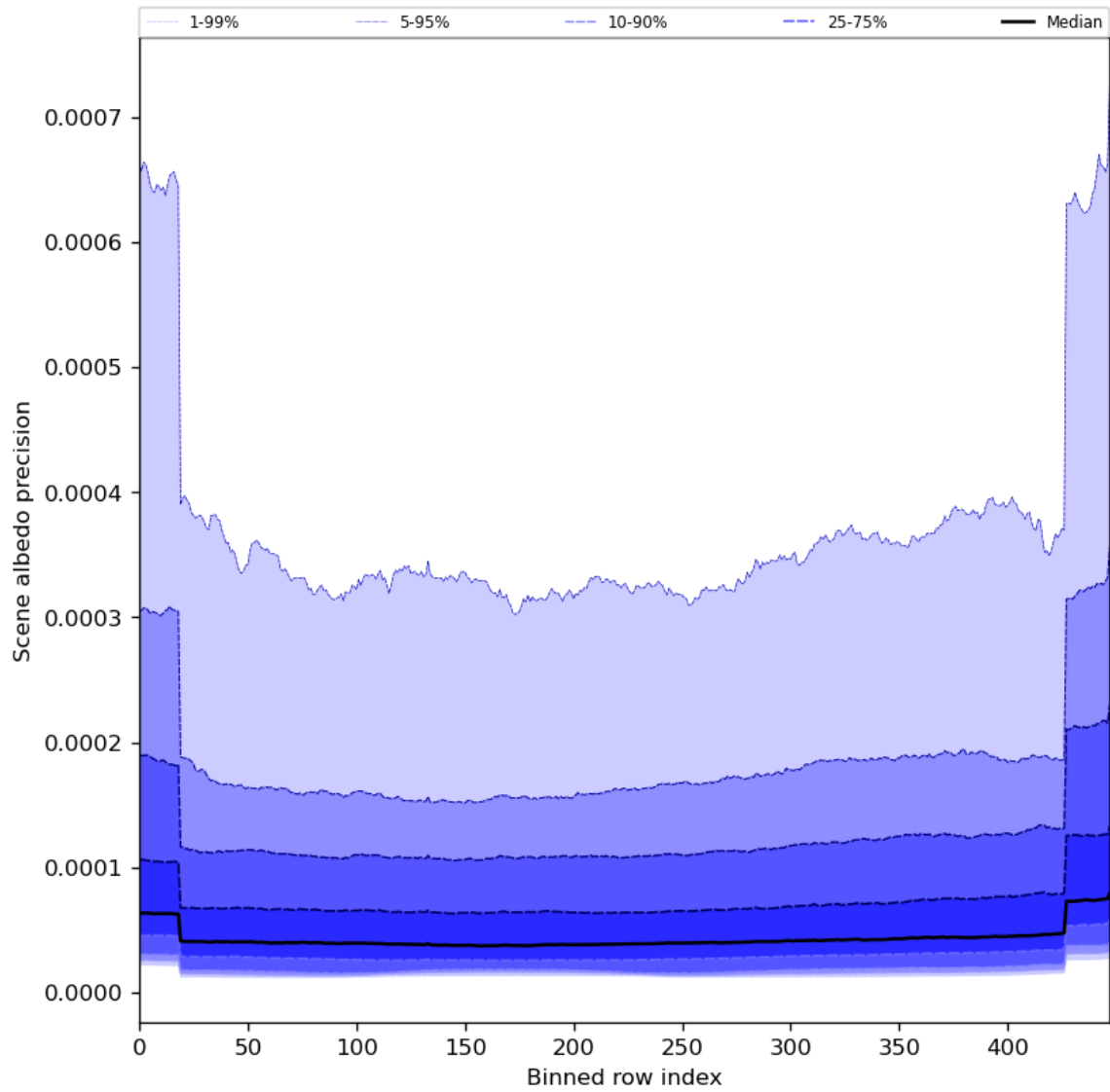
Figure 52: Along track statistics of “Scene albedo precision” for 2024-06-29 to 2024-07-01
