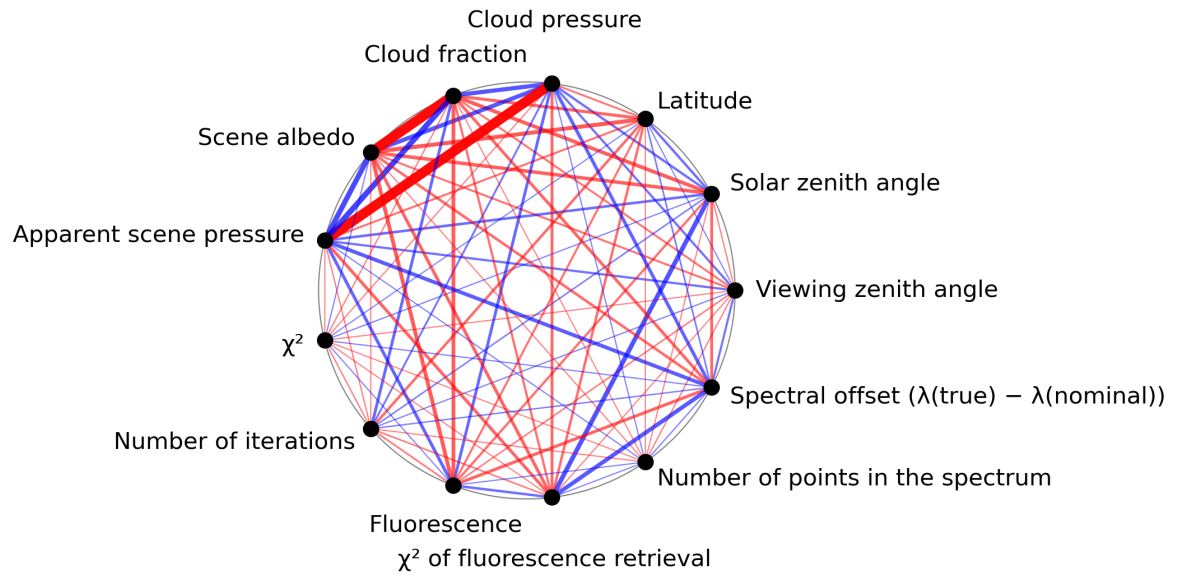
Figure 1: Map of correlation graph for 2024-06-29 to 2024-07-01.
