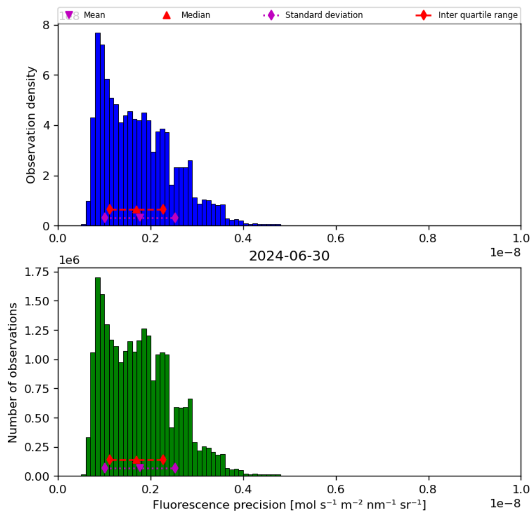
Figure 41: Histogram of “Fluorescence precision” for 2024-06-29 to 2024-07-01
