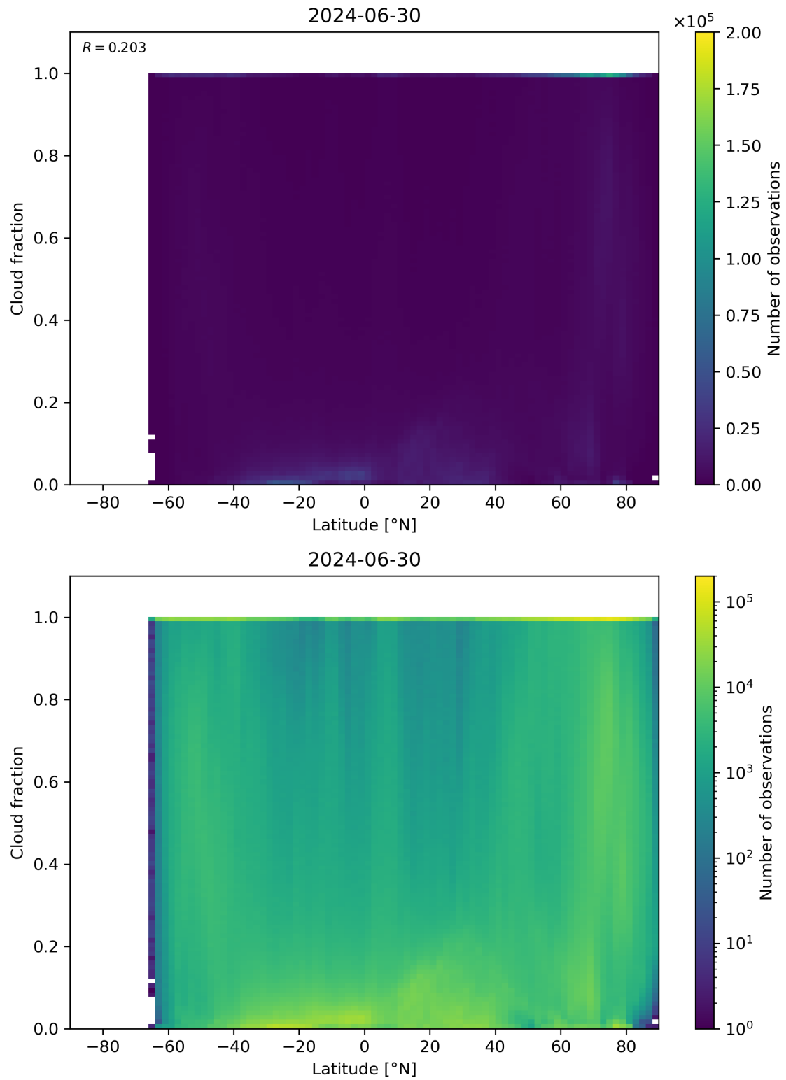
Figure 90: Scatter density plot of “Latitude” against “Cloud fraction” for 2024-06-29 to 2024-07-01.
