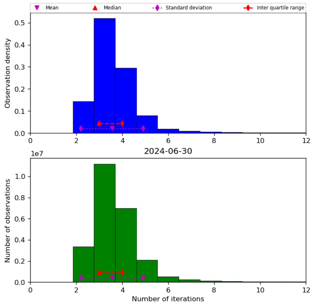
Figure 39: Histogram of “Number of iterations” for 2024-06-29 to 2024-07-01
