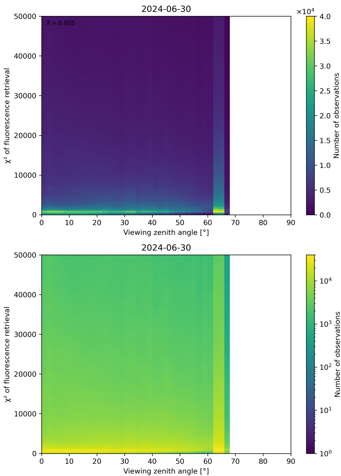
Figure 119: Scatter density plot of “Viewing zenith angle” against “ \chi^2 of fluorescence retrieval” for 2024-06-29 to 2024-07-01.
