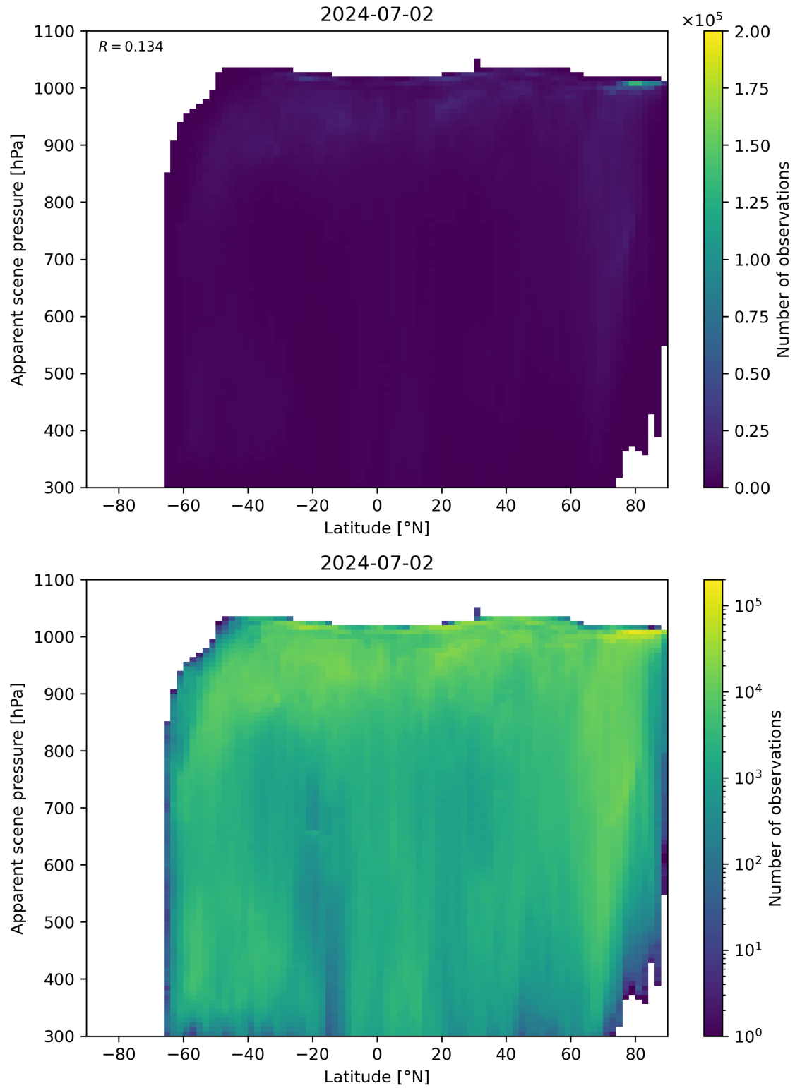
Figure 88: Scatter density plot of “Latitude” against “Apparent scene pressure” for 2024-07-01 to 2024-07-03.
