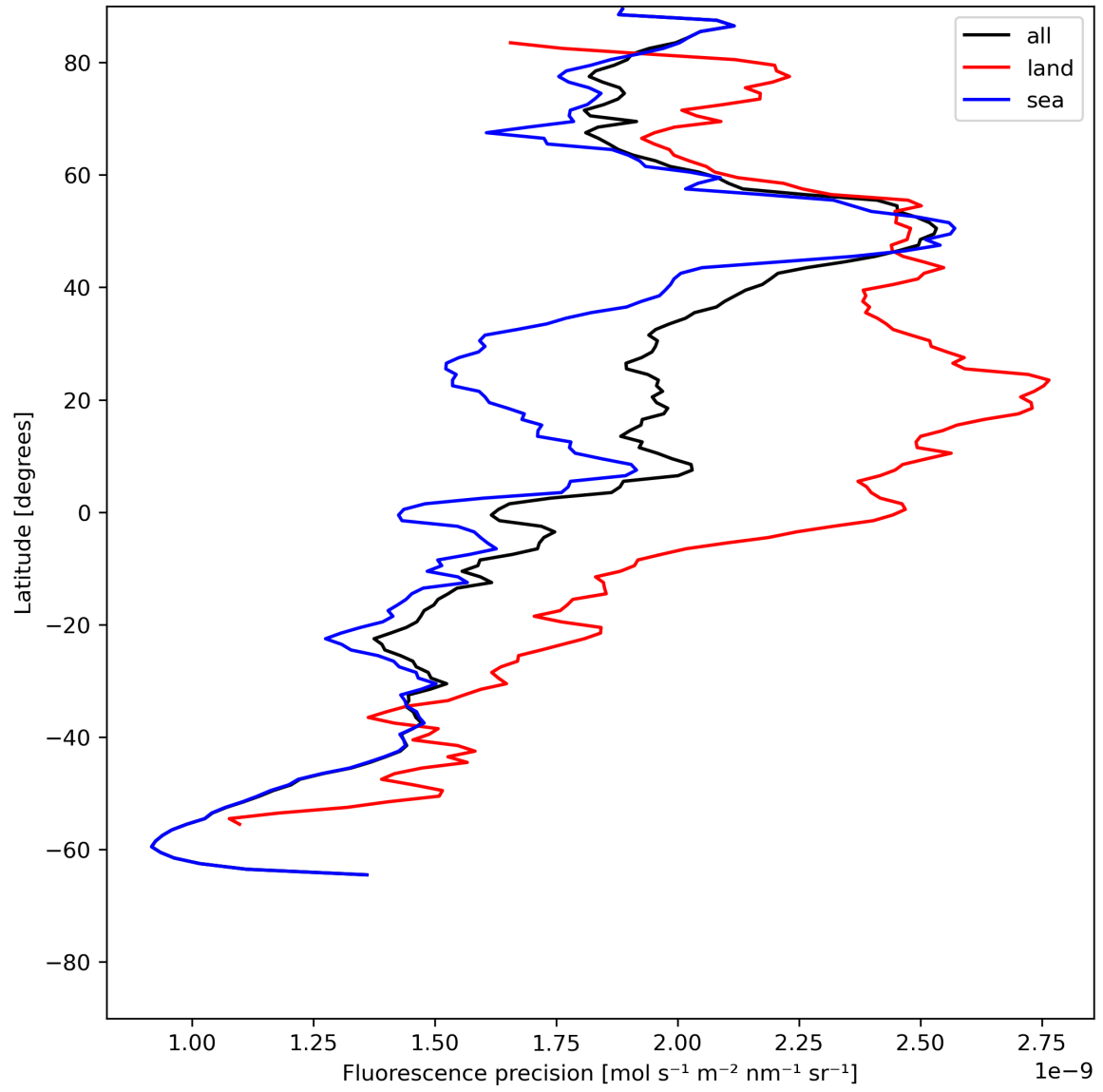
Figure 24: Zonal average of “Fluorescence precision” for 2024-07-01 to 2024-07-03.
