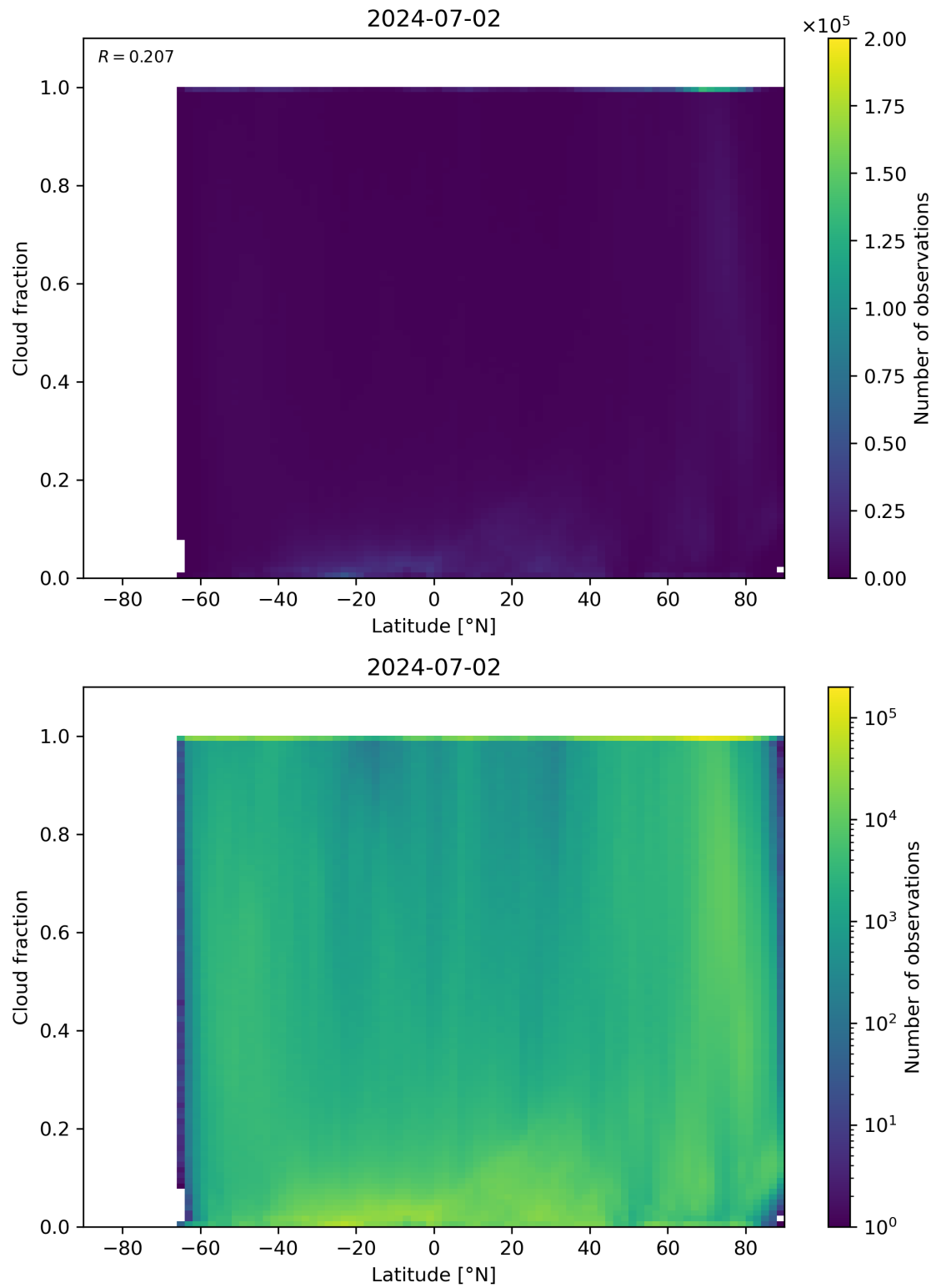
Figure 90: Scatter density plot of “Latitude” against “Cloud fraction” for 2024-07-01 to 2024-07-03.
