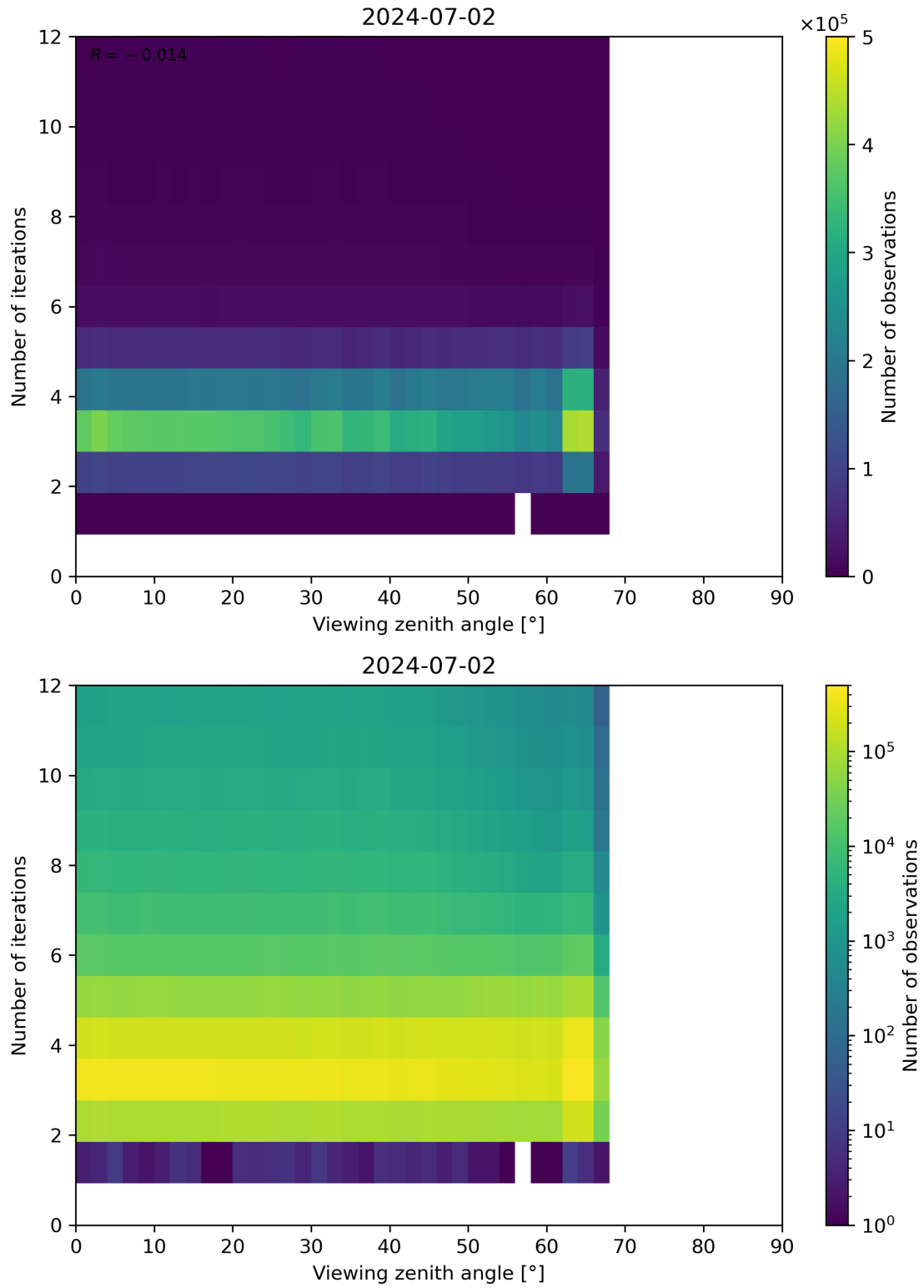
Figure 124: Scatter density plot of “Viewing zenith angle” against “Number of iterations” for 2024-07-01 to 2024-07-03.
