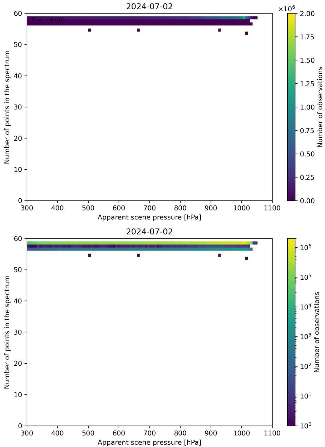
Figure 66: Scatter density plot of “Apparent scene pressure” against “Number of points in the spectrum” for 2024-07-01 to 2024-07-03.
