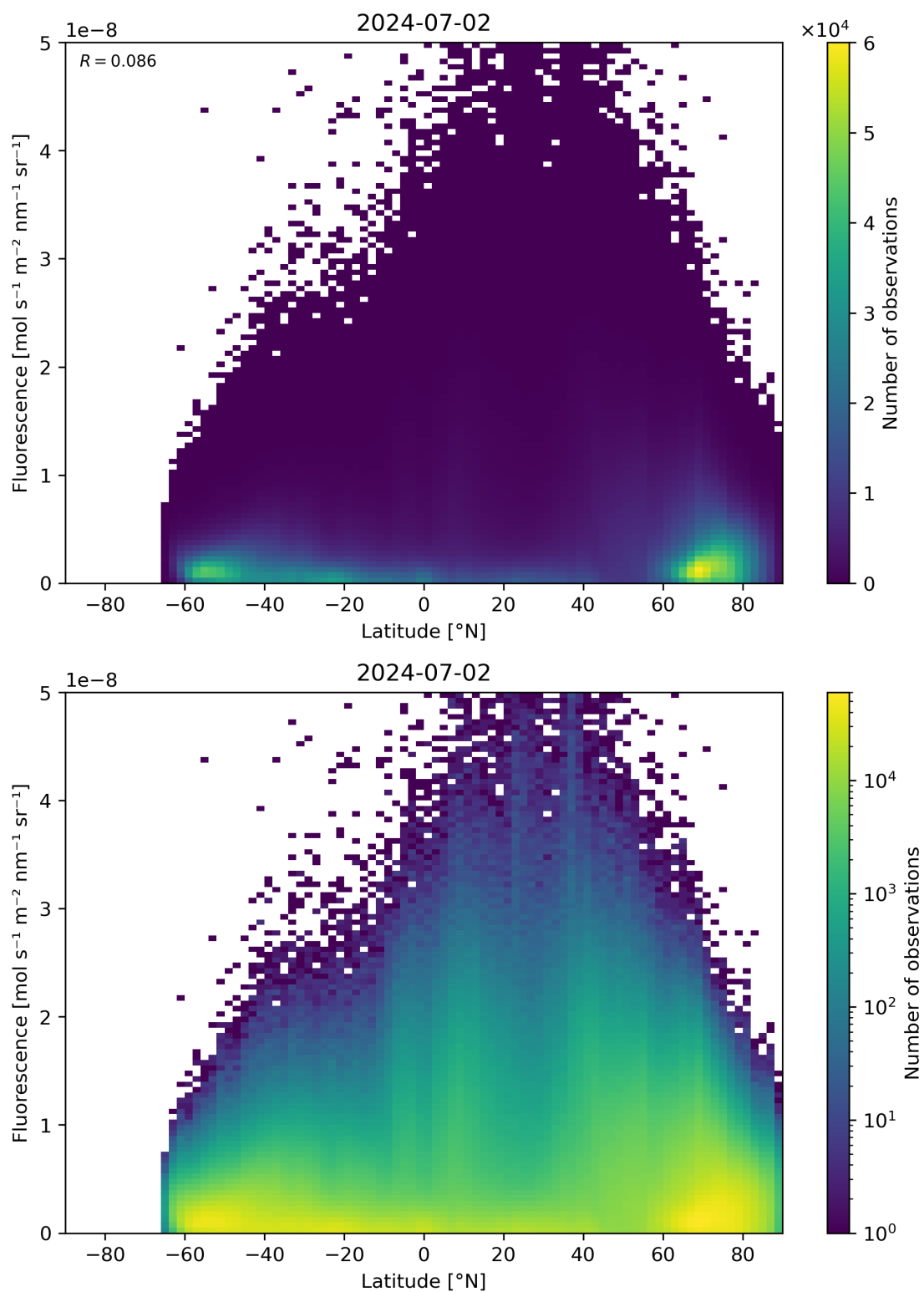
Figure 92: Scatter density plot of “Latitude” against “Fluorescence” for 2024-07-01 to 2024-07-03.
