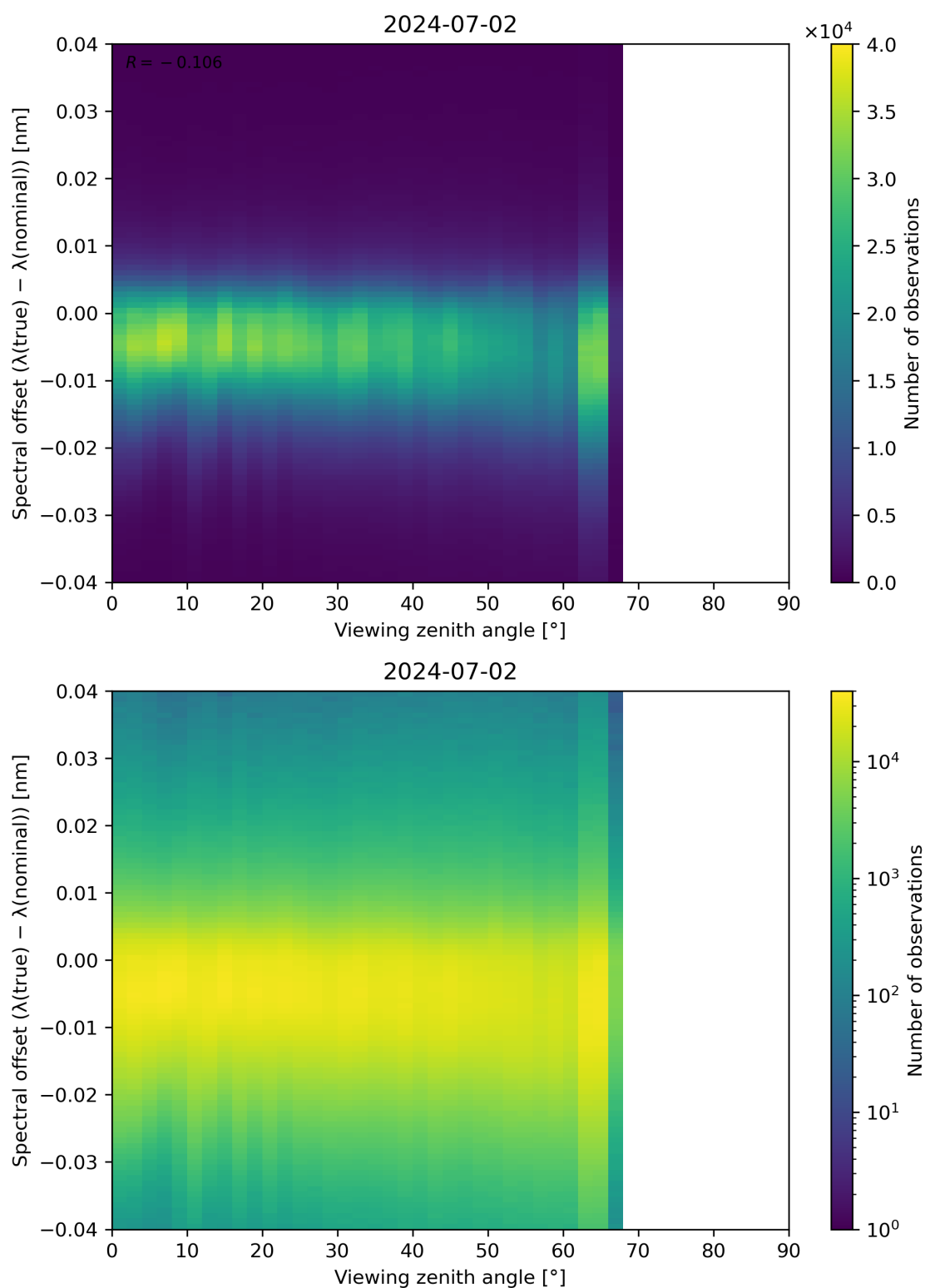
Figure 128: Scatter density plot of “Viewing zenith angle” against “Spectral offset ( \lambda(\text{true}) - \lambda(\text{nominal}) )” for 2024-07-01 to 2024-07-03.
