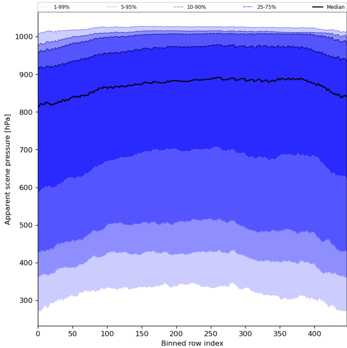
Figure 53: Along track statistics of “Apparent scene pressure” for 2024-07-01 to 2024-07-03
