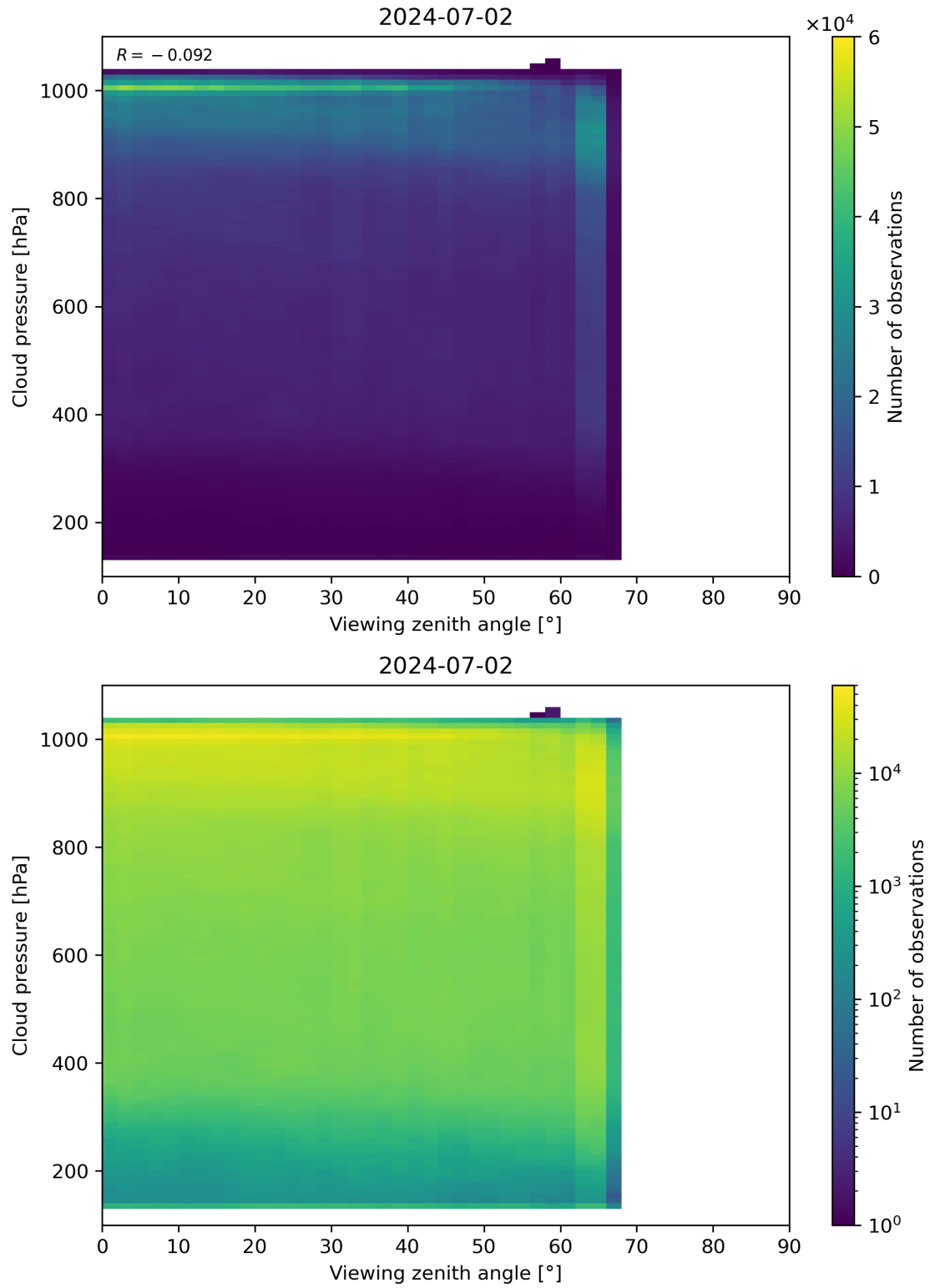
Figure 121: Scatter density plot of “Viewing zenith angle” against “Cloud pressure” for 2024-07-01 to 2024-07-03.
