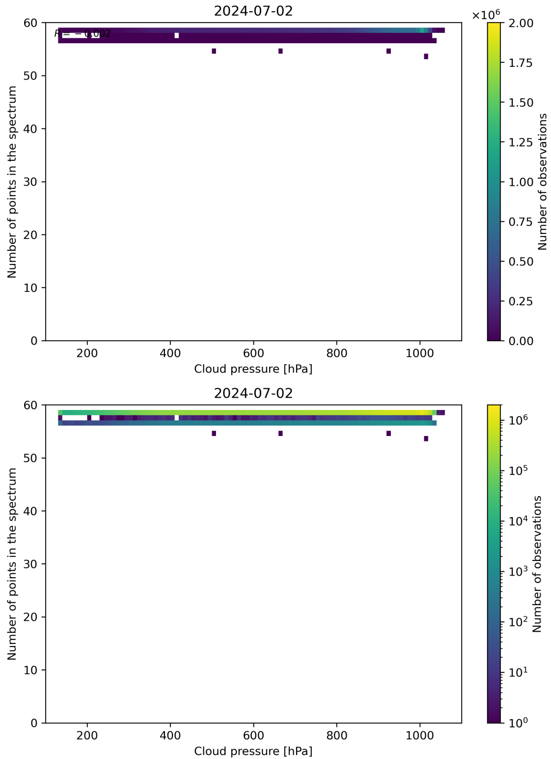
Figure 82: Scatter density plot of “Cloud pressure” against “Number of points in the spectrum” for 2024-07-01 to 2024-07-03.
