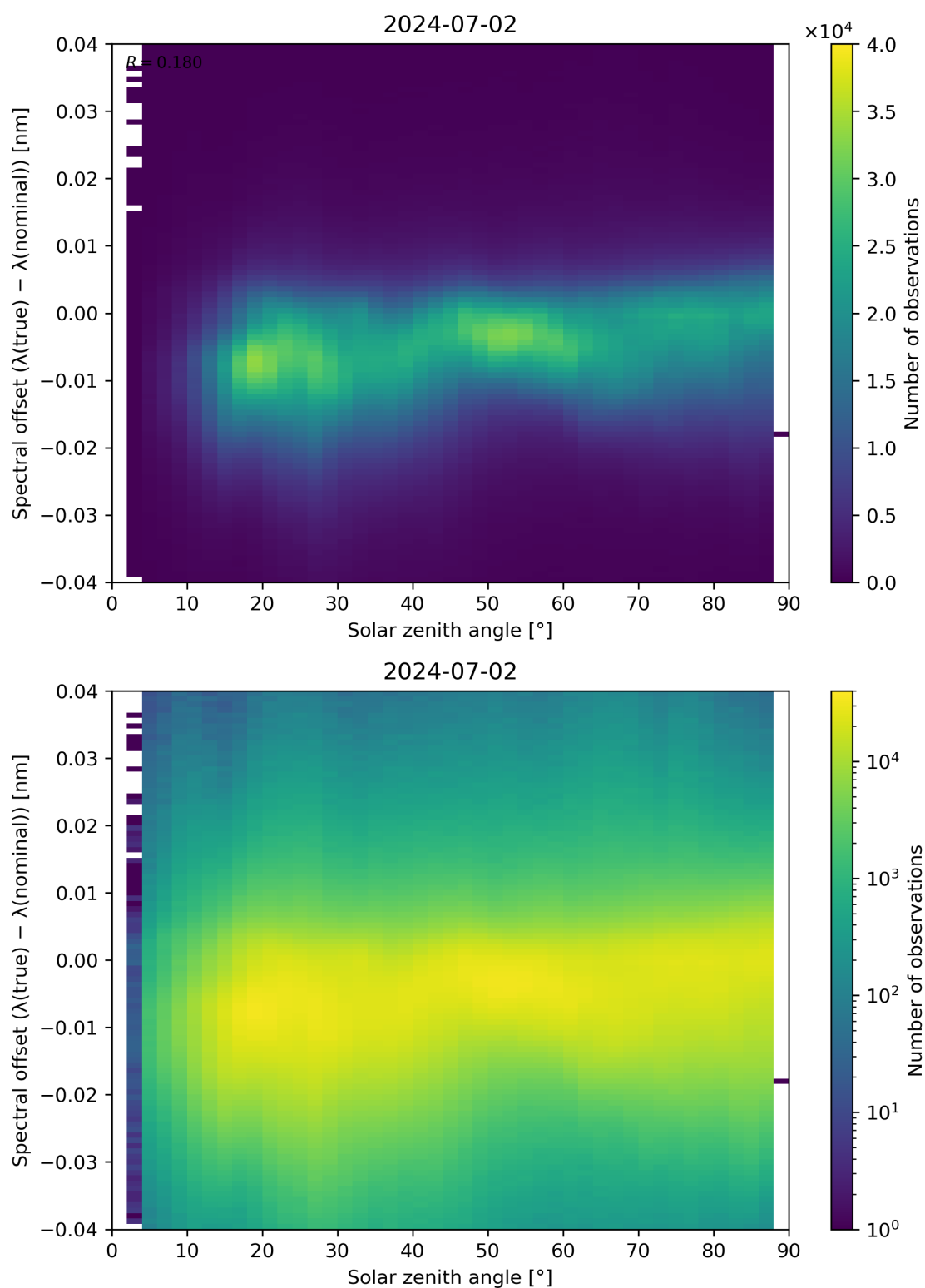
Figure 117: Scatter density plot of “Solar zenith angle” against “Spectral offset ( \lambda(\text{true}) - \lambda(\text{nominal}) )” for 2024-07-01 to 2024-07-03.
