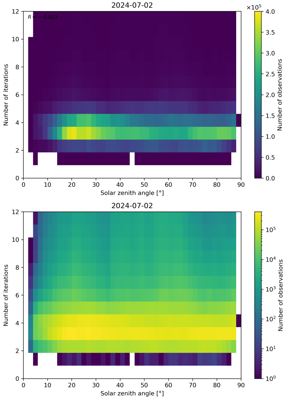
Figure 114: Scatter density plot of “Solar zenith angle” against “Number of iterations” for 2024-07-01 to 2024-07-03.
