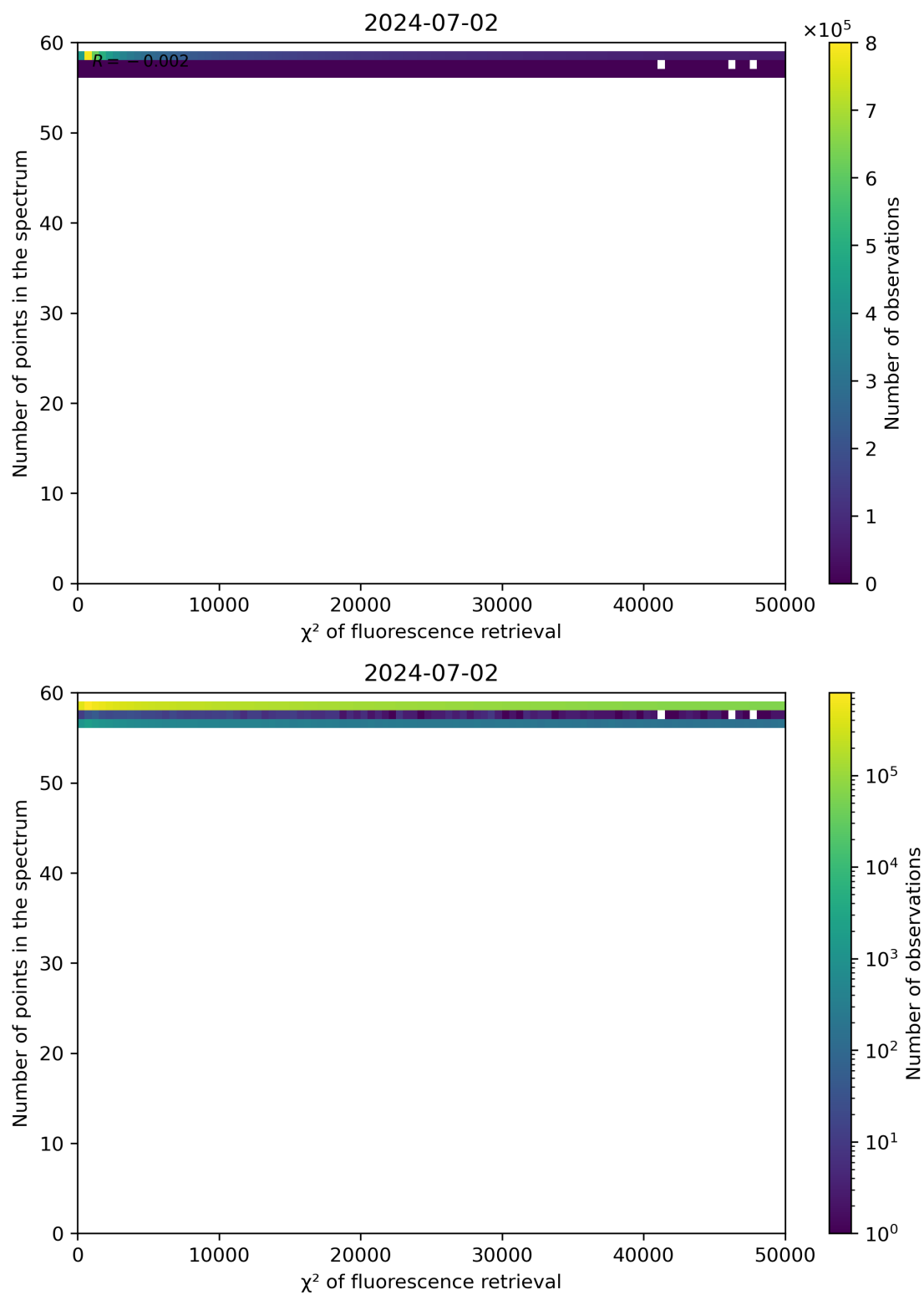
Figure 68: Scatter density plot of " \chi^2 of fluorescence retrieval" against "Number of points in the spectrum" for 2024-07-01 to 2024-07-03.
