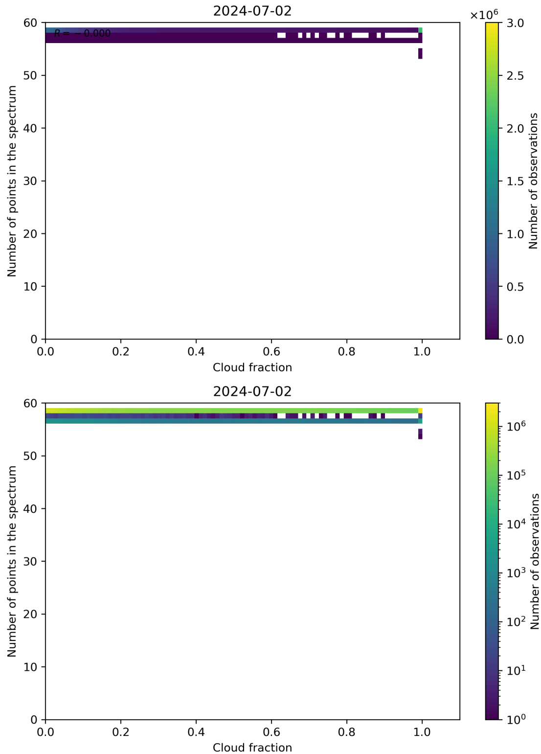
Figure 74: Scatter density plot of “Cloud fraction” against “Number of points in the spectrum” for 2024-07-01 to 2024-07-03.
