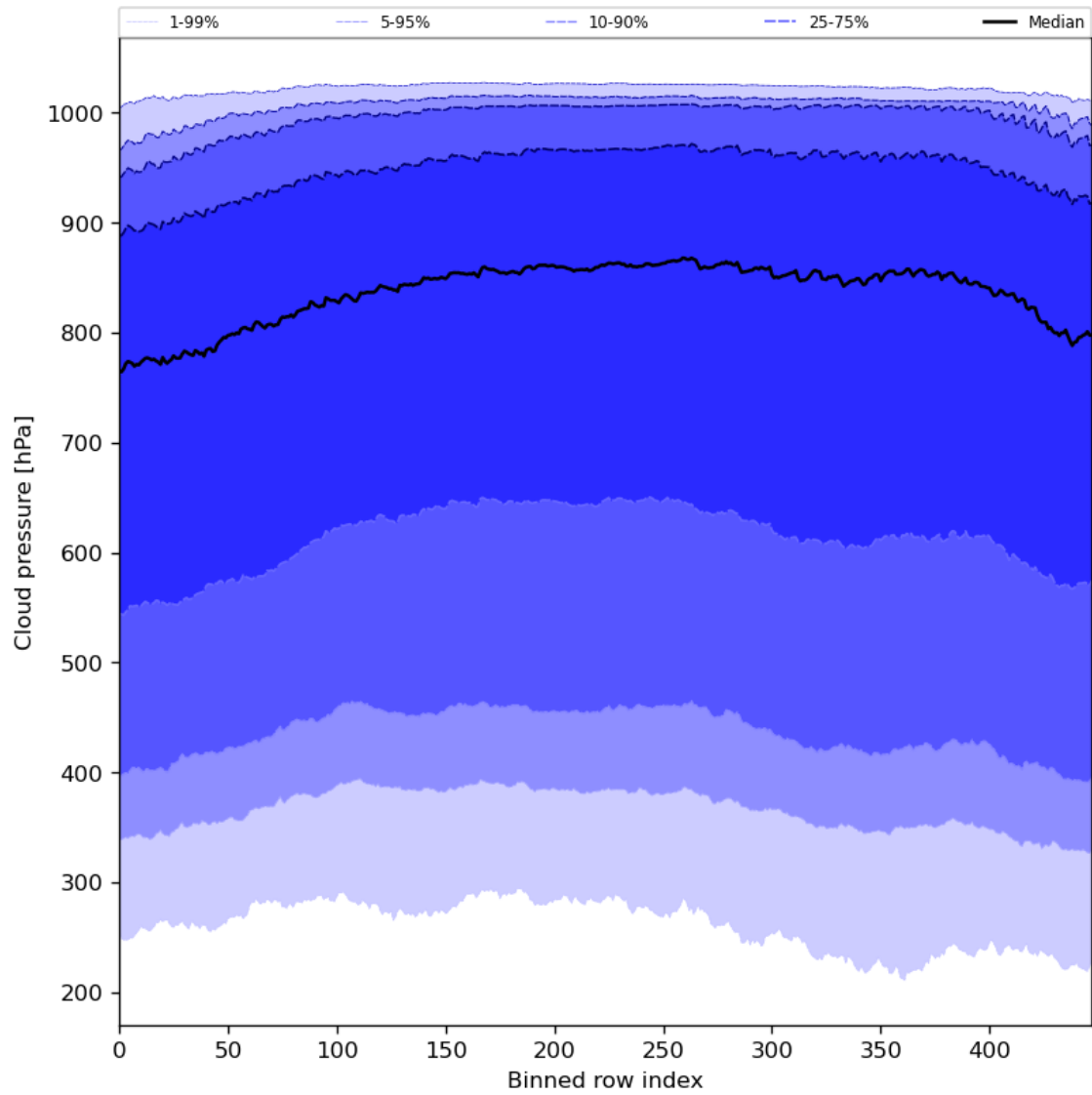
Figure 47: Along track statistics of “Cloud pressure” for 2024-07-01 to 2024-07-03
