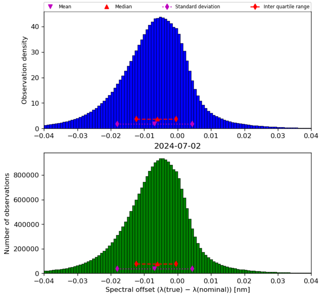
Figure 45: Histogram of “Spectral offset ( \lambda(\text{true}) - \lambda(\text{nominal}) )” for 2024-07-01 to 2024-07-03
