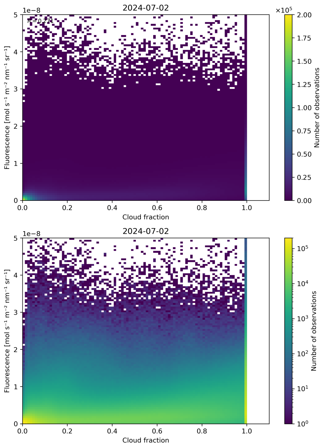
Figure 72: Scatter density plot of “Cloud fraction” against “Fluorescence” for 2024-07-01 to 2024-07-03.
