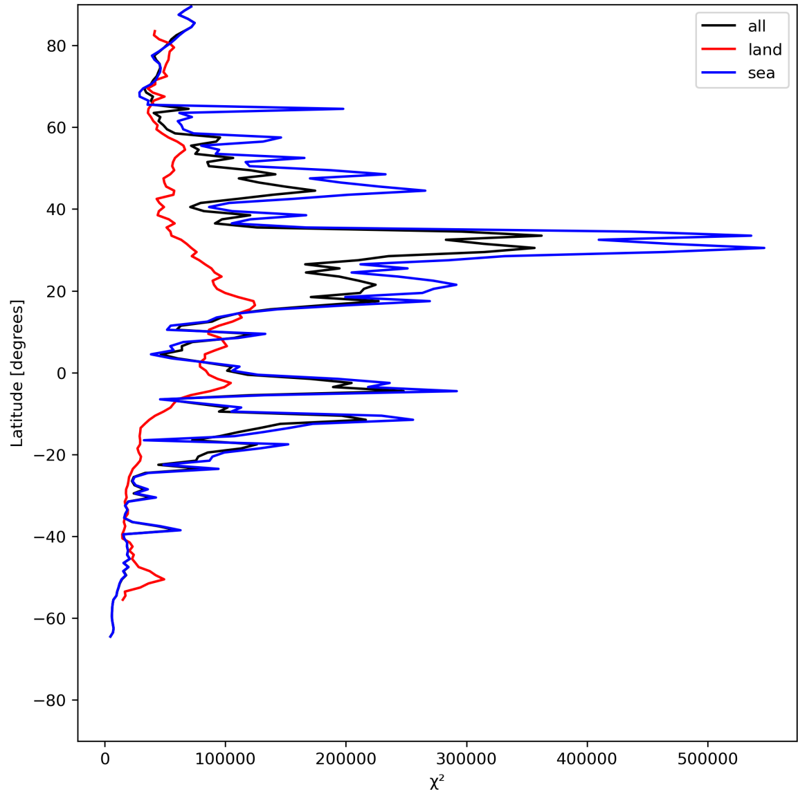
Figure 21: Zonal average of “ \chi^2 ” for 2024-07-01 to 2024-07-03.
