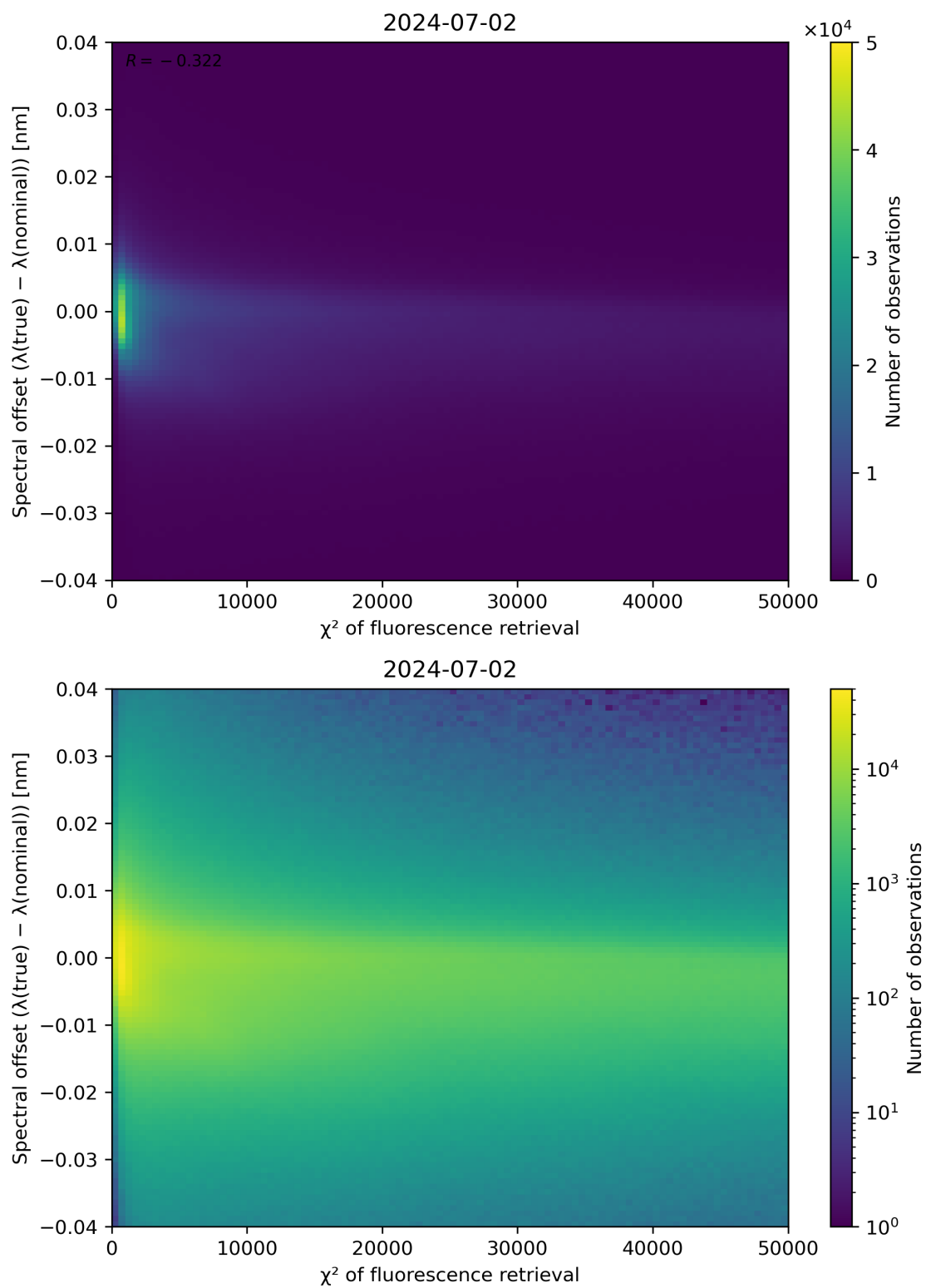
Figure 69: Scatter density plot of " \chi^2 of fluorescence retrieval" against "Spectral offset ( \lambda(\text{true}) - \lambda(\text{nominal})) " for 2024-07-01 to 2024-07-03.
