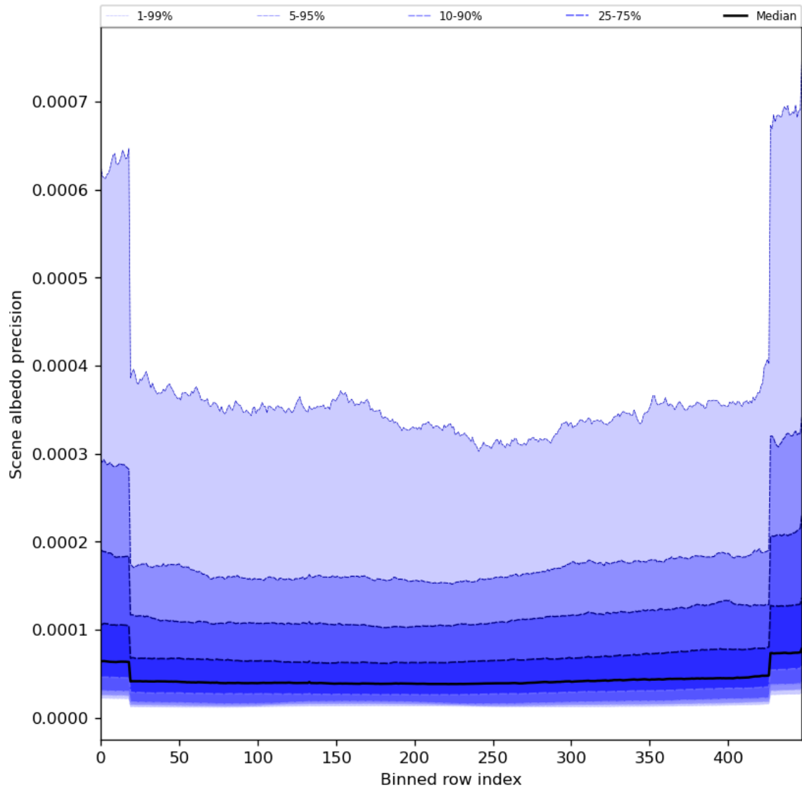
Figure 52: Along track statistics of “Scene albedo precision” for 2024-07-01 to 2024-07-03
