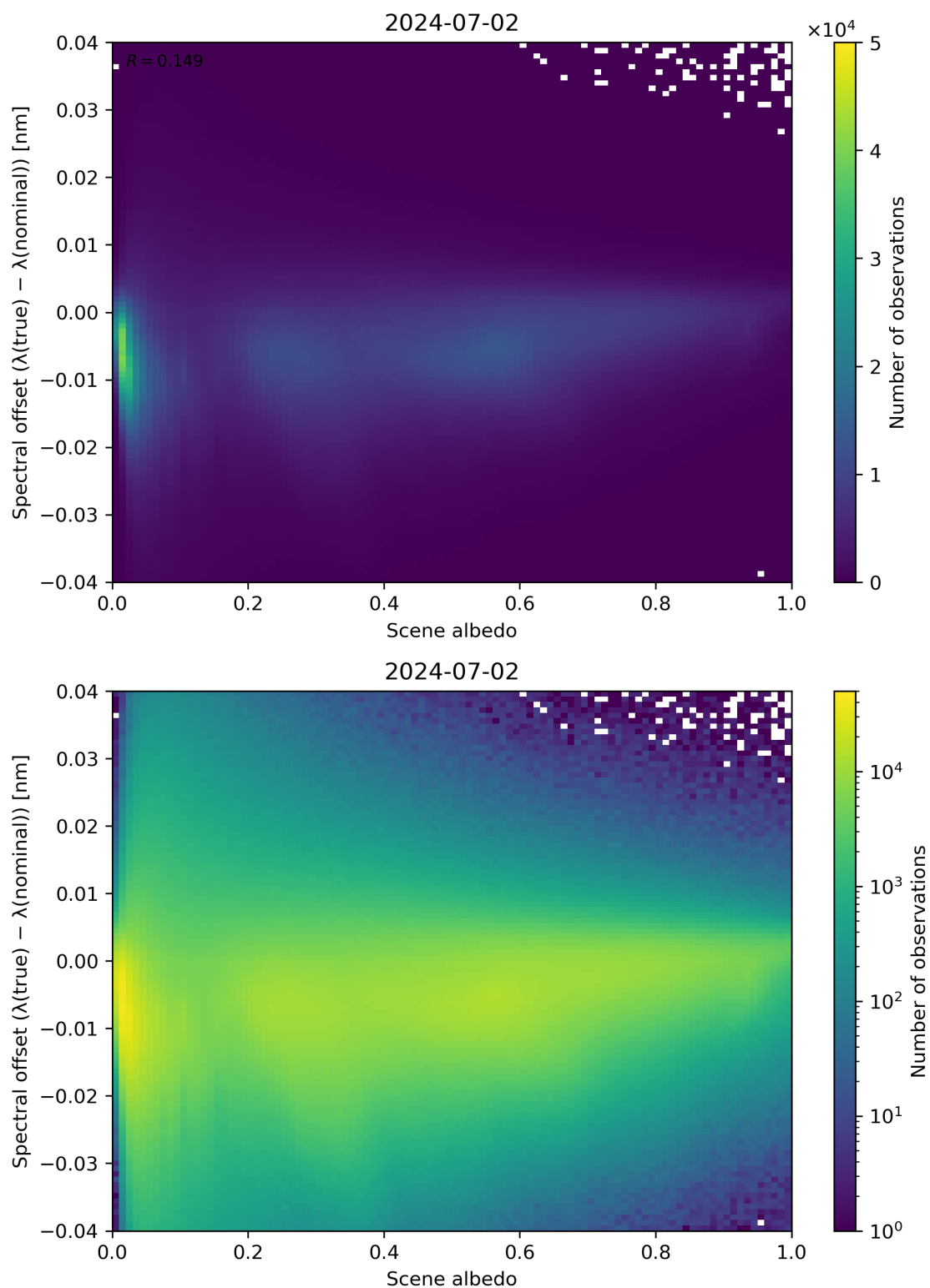
Figure 107: Scatter density plot of “Scene albedo” against “Spectral offset ( \lambda(\text{true}) - \lambda(\text{nominal}) )” for 2024-07-01 to 2024-07-03.
