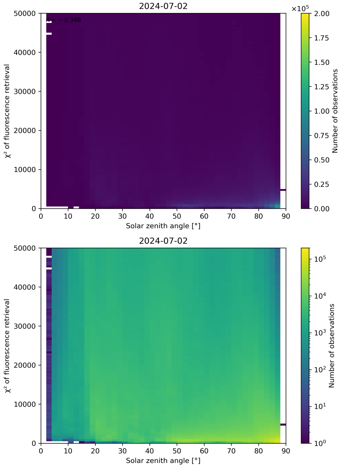
Figure 109: Scatter density plot of “Solar zenith angle” against “ \chi^2 of fluorescence retrieval” for 2024-07-01 to 2024-07-03.
