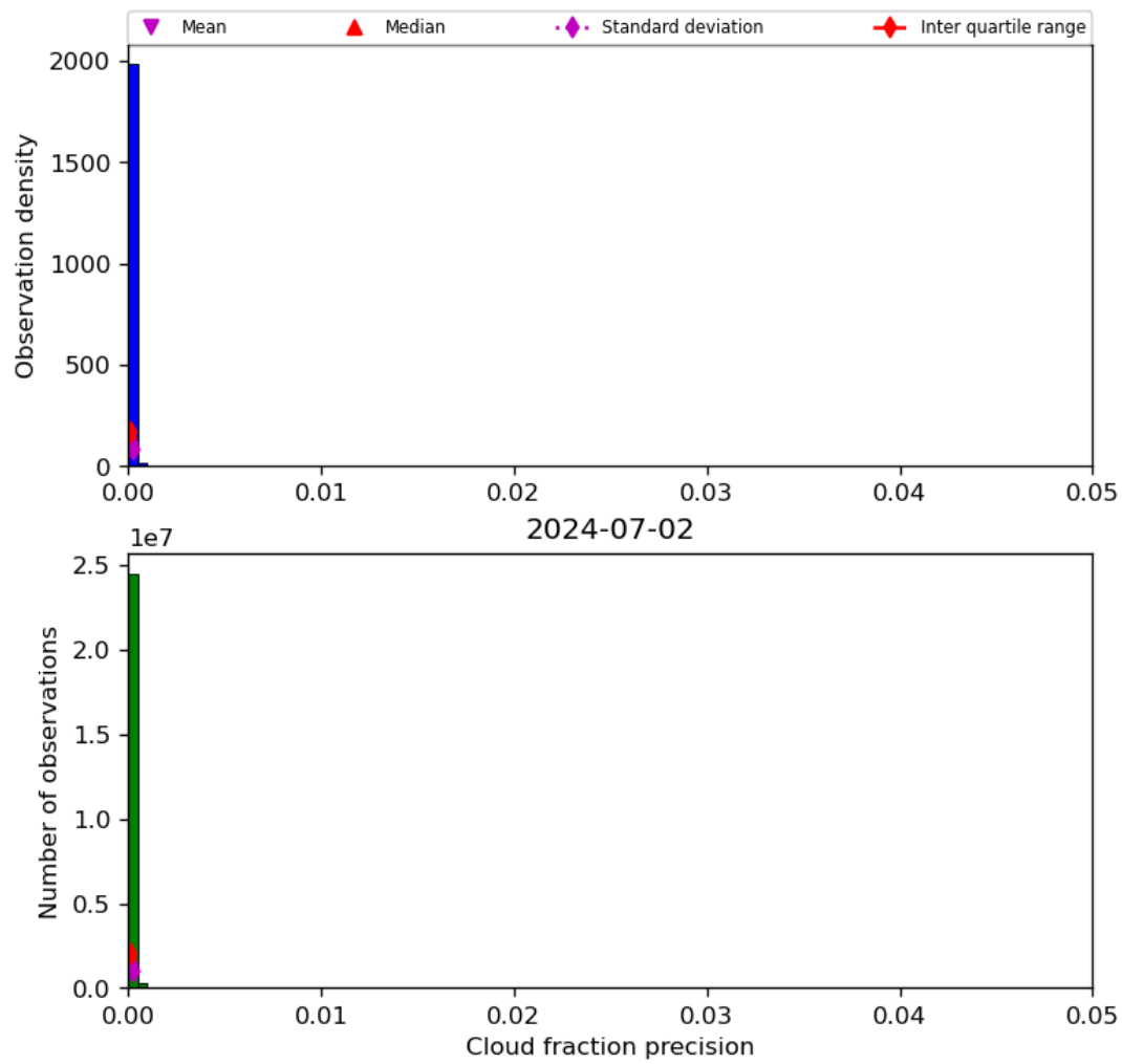
Figure 33: Histogram of “Cloud fraction precision” for 2024-07-01 to 2024-07-03
