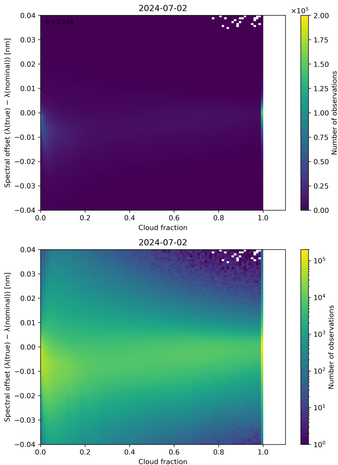
Figure 76: Scatter density plot of “Cloud fraction” against “Spectral offset ( \lambda(\text{true}) - \lambda(\text{nominal}) )” for 2024-07-01 to 2024-07-03.
