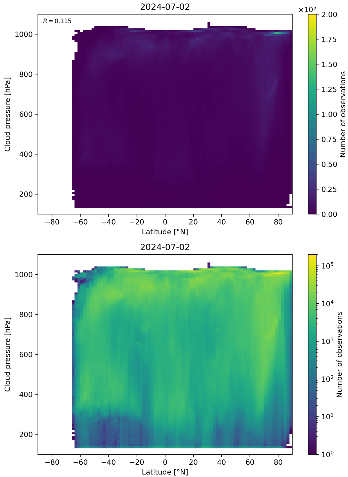
Figure 91: Scatter density plot of “Latitude” against “Cloud pressure” for 2024-07-01 to 2024-07-03.
