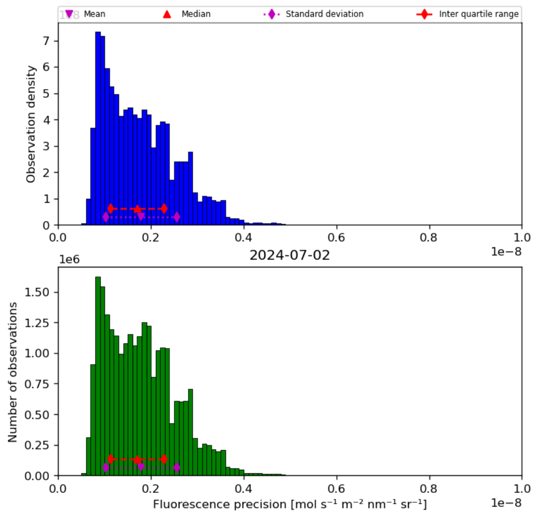
Figure 41: Histogram of “Fluorescence precision” for 2024-07-01 to 2024-07-03
