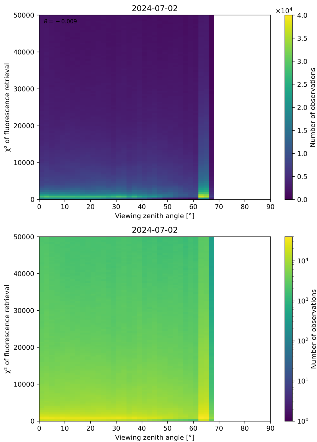
Figure 119: Scatter density plot of “Viewing zenith angle” against “ \chi^2 of fluorescence retrieval” for 2024-07-01 to 2024-07-03.
