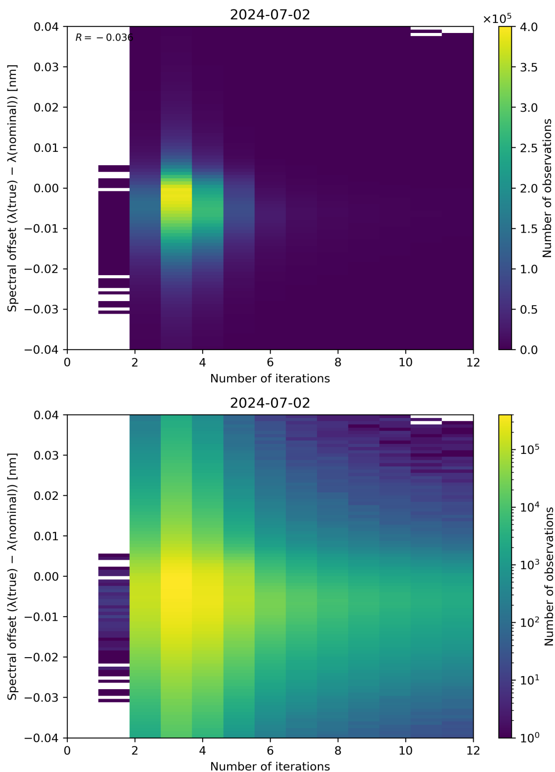
Figure 100: Scatter density plot of “Number of iterations” against “Spectral offset ( \lambda(\text{true}) - \lambda(\text{nominal}) )” for 2024-07-01 to 2024-07-03.
