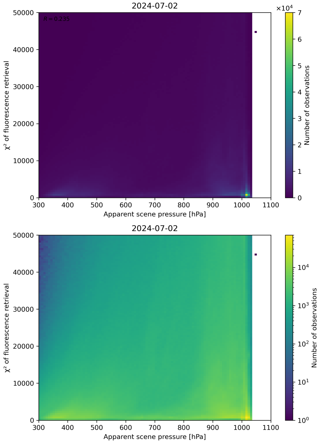
Figure 63: Scatter density plot of “Apparent scene pressure” against “ \chi^2 of fluorescence retrieval” for 2024-07-01 to 2024-07-03.
