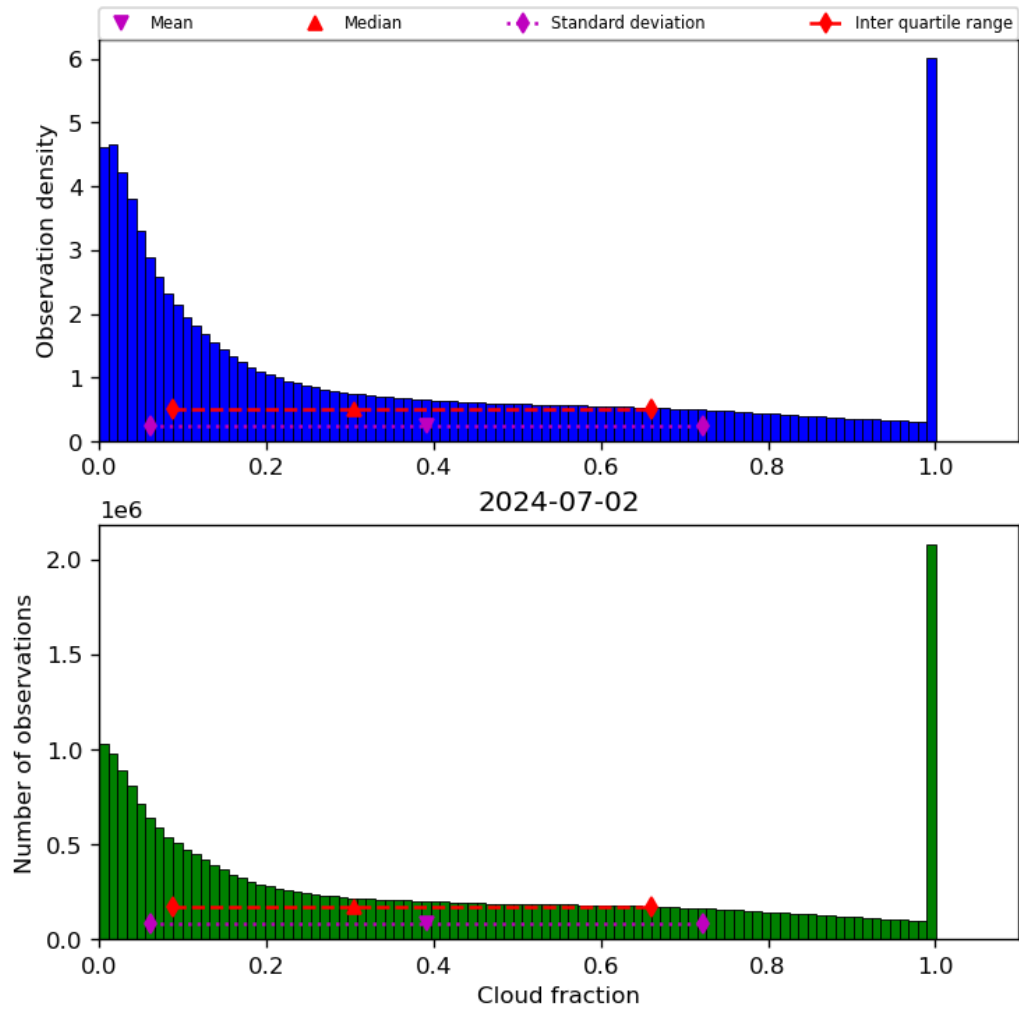
Figure 32: Histogram of “Cloud fraction” for 2024-07-01 to 2024-07-03
