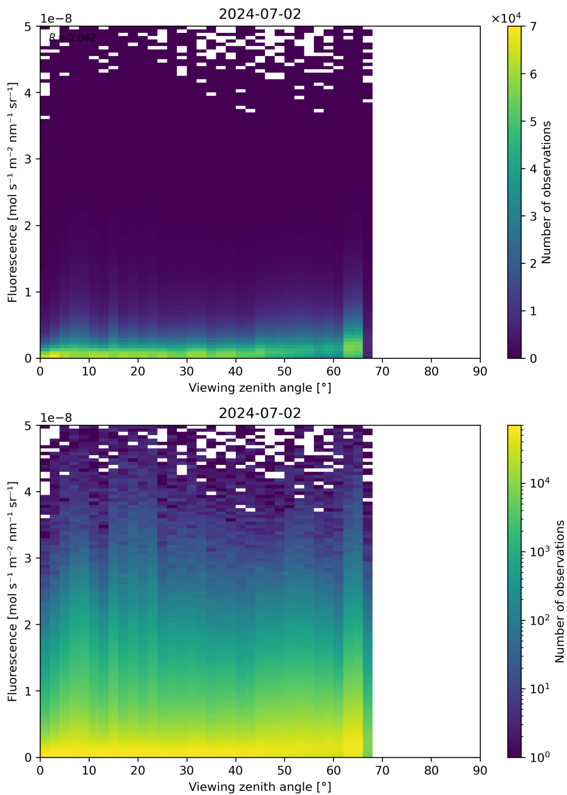
Figure 122: Scatter density plot of “Viewing zenith angle” against “Fluorescence” for 2024-07-01 to 2024-07-03.
