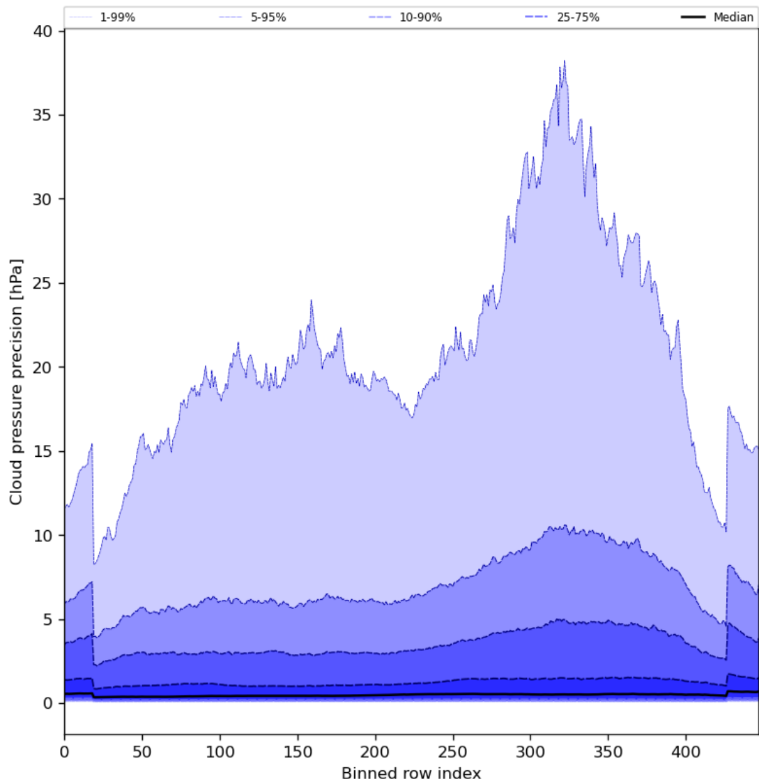
Figure 48: Along track statistics of “Cloud pressure precision” for 2024-07-01 to 2024-07-03
