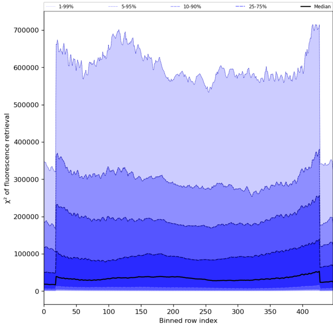
Figure 59: Along track statistics of “ \chi^2 of fluorescence retrieval” for 2024-07-01 to 2024-07-03
