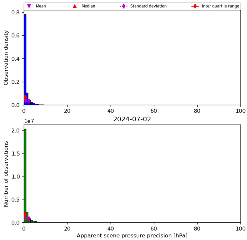
Figure 37: Histogram of “Apparent scene pressure precision” for 2024-07-01 to 2024-07-03
