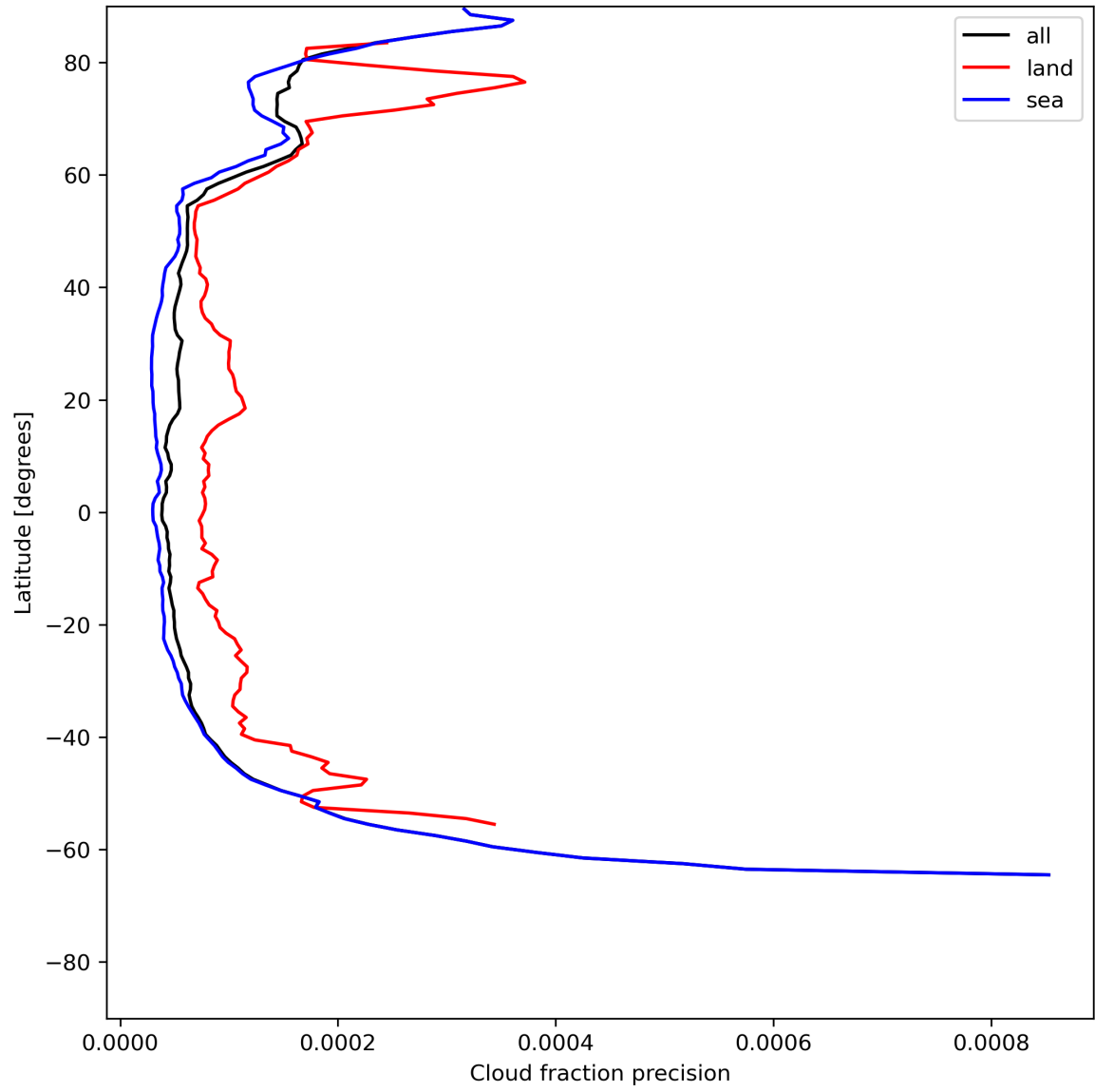
Figure 16: Zonal average of “Cloud fraction precision” for 2024-07-01 to 2024-07-03.
