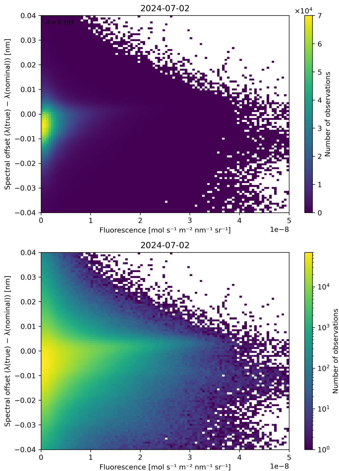
Figure 87: Scatter density plot of “Fluorescence” against “Spectral offset ( \lambda(\text{true}) - \lambda(\text{nominal}) )” for 2024-07-01 to 2024-07-03.
