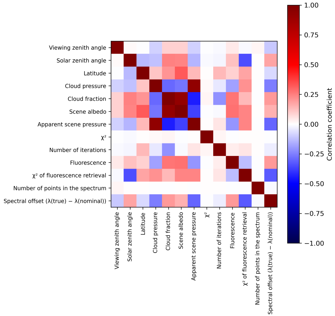
Figure 2: Map of correlation matrix for 2024-07-01 to 2024-07-03.
