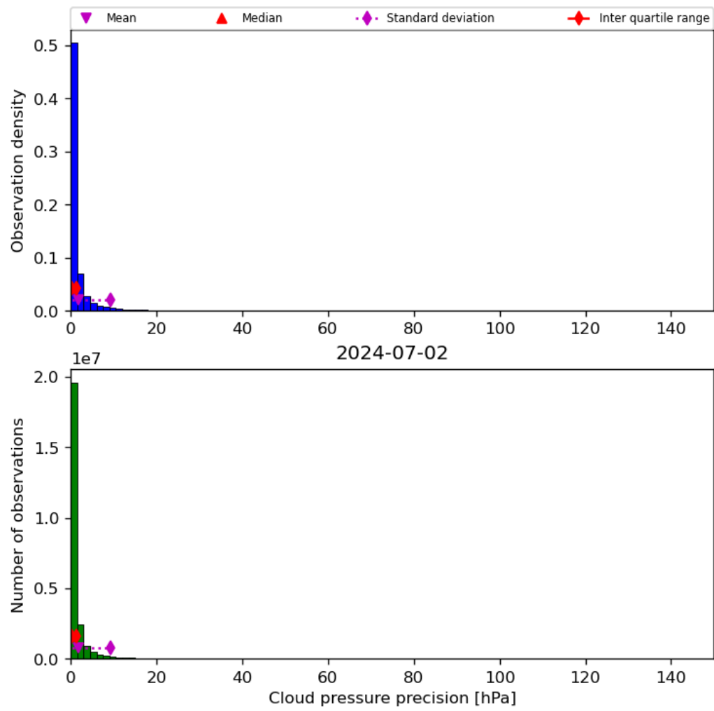
Figure 31: Histogram of “Cloud pressure precision” for 2024-07-01 to 2024-07-03
