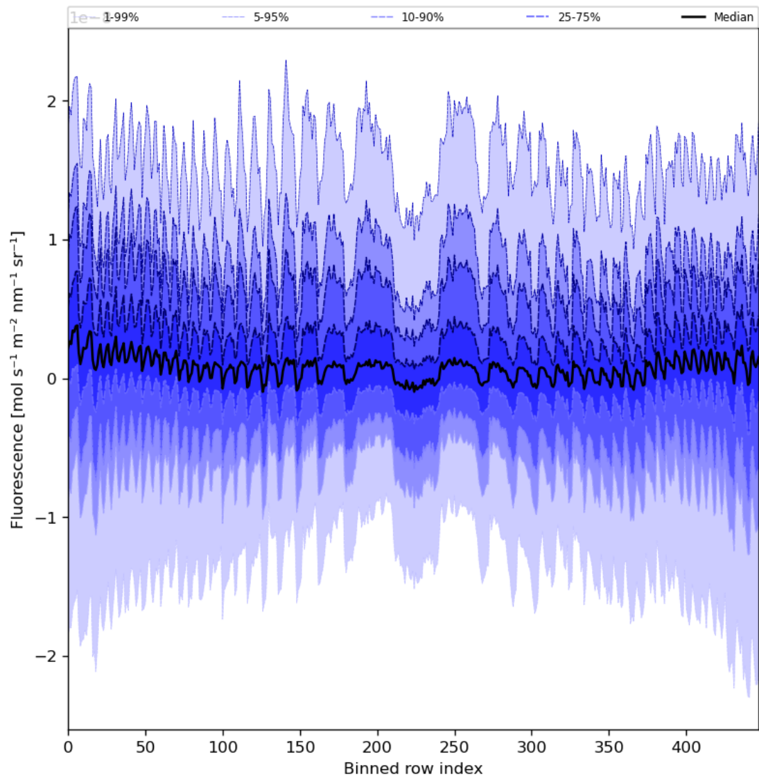
Figure 57: Along track statistics of “Fluorescence” for 2024-07-01 to 2024-07-03
