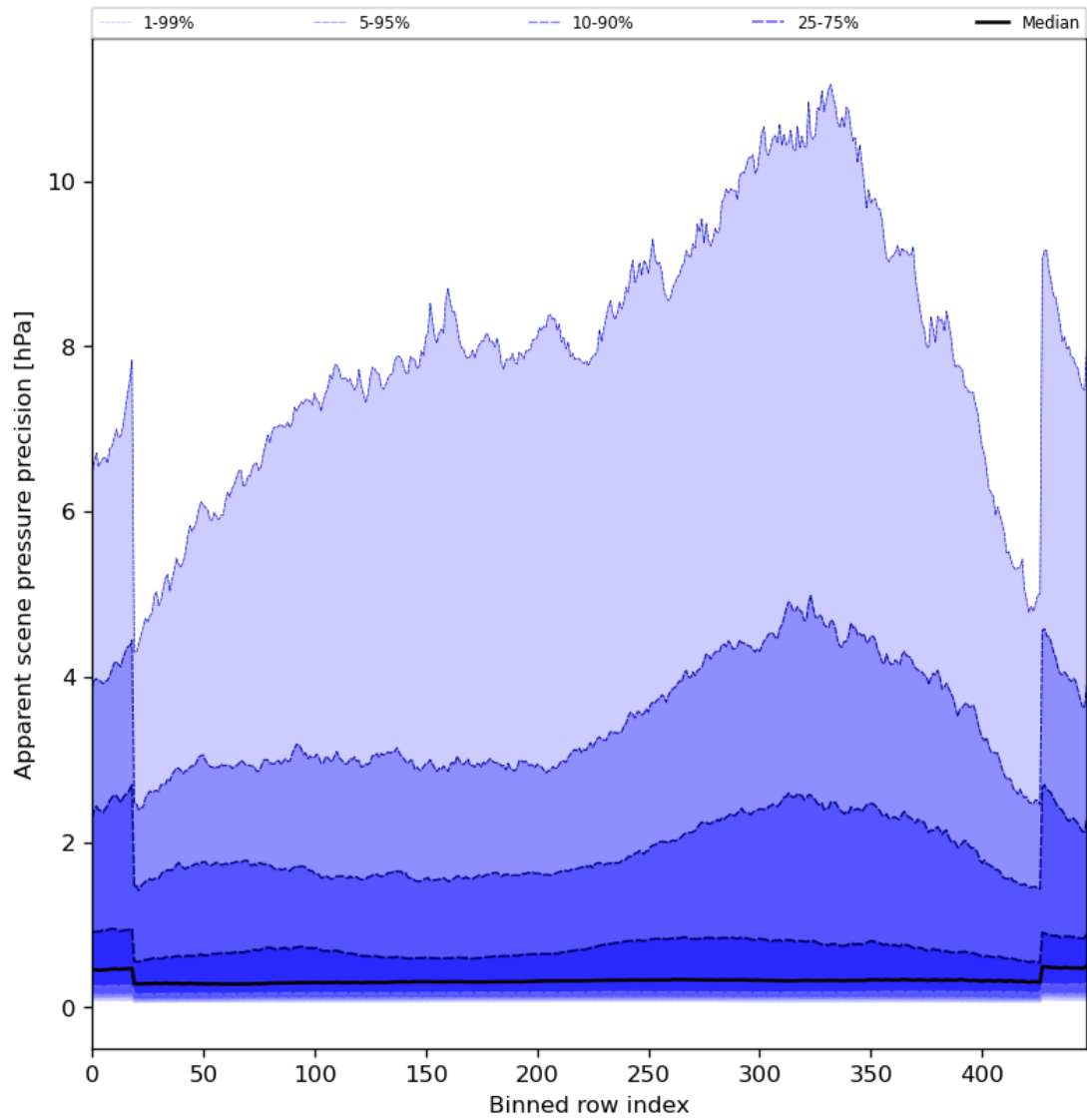
Figure 54: Along track statistics of “Apparent scene pressure precision” for 2024-07-01 to 2024-07-03
