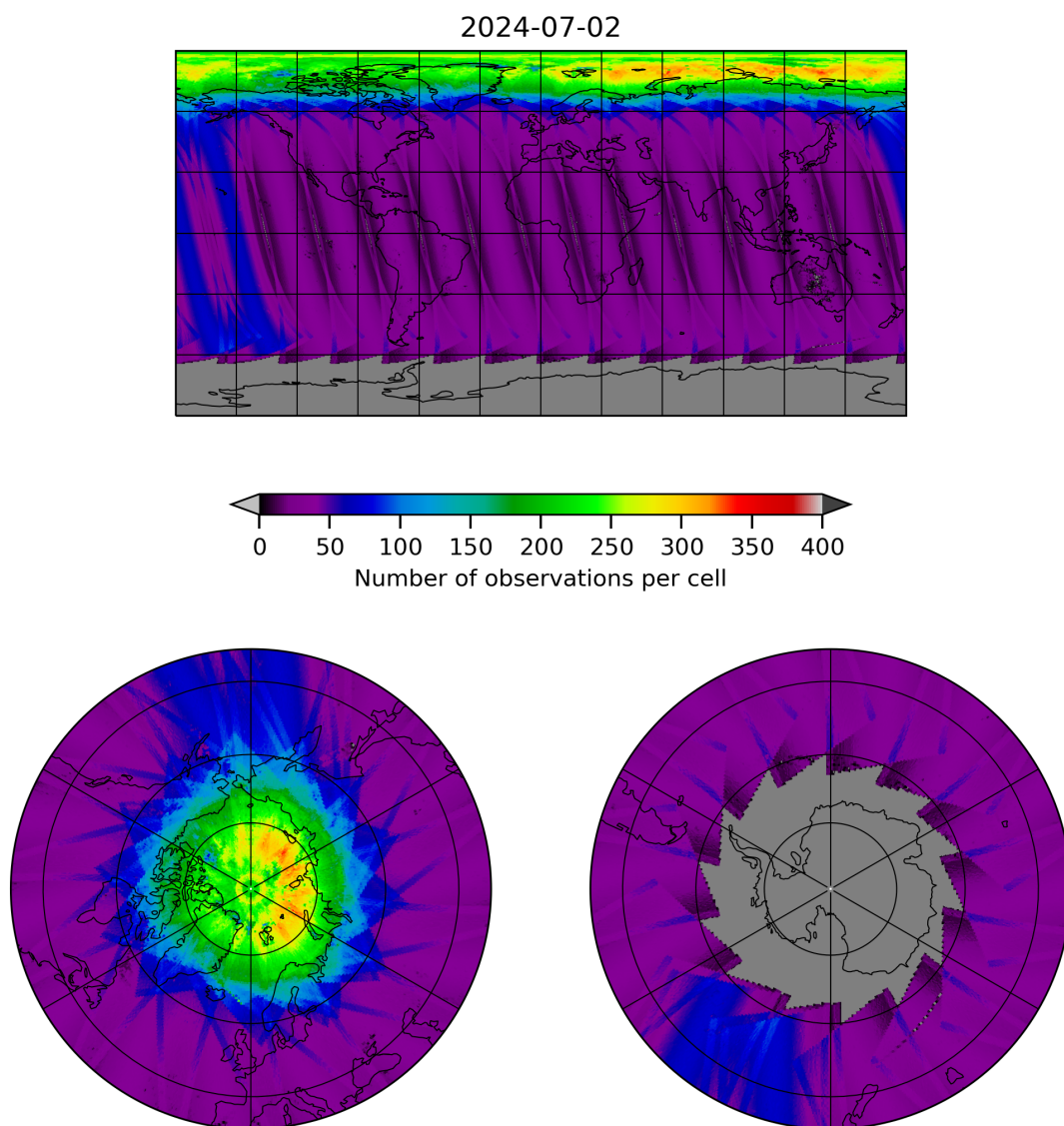
Figure 11: Map of the number of observations for 2024-07-01 to 2024-07-03
