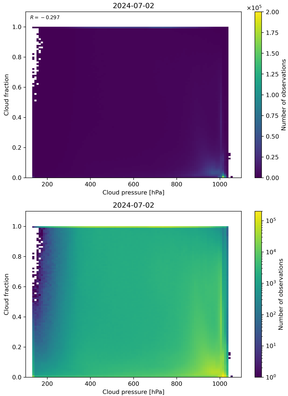
Figure 79: Scatter density plot of “Cloud pressure” against “Cloud fraction” for 2024-07-01 to 2024-07-03.
