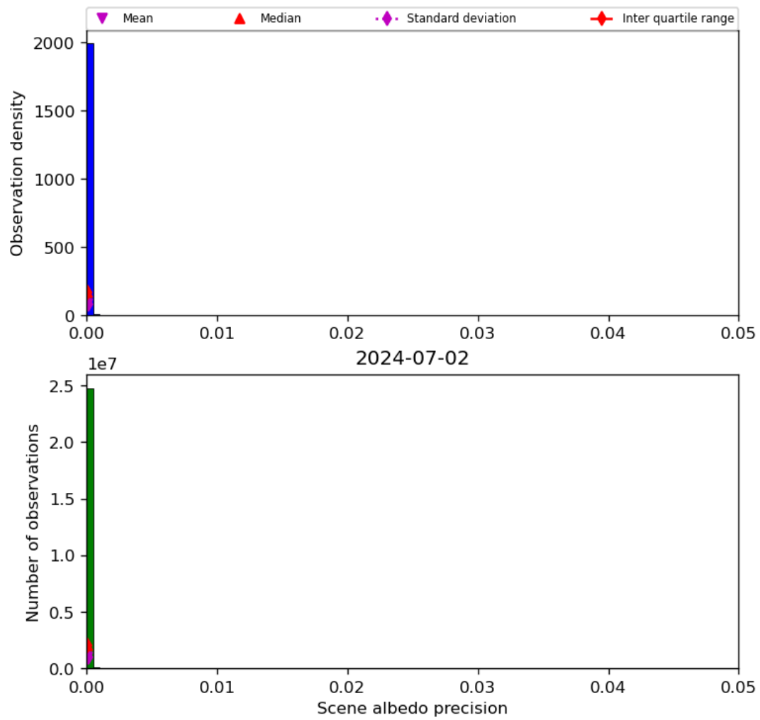
Figure 35: Histogram of “Scene albedo precision” for 2024-07-01 to 2024-07-03
