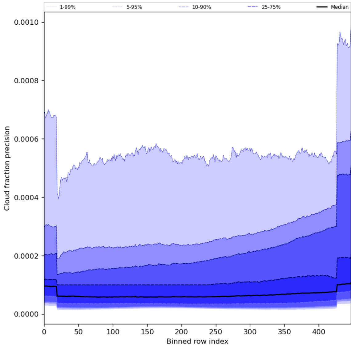
Figure 50: Along track statistics of “Cloud fraction precision” for 2024-07-01 to 2024-07-03
