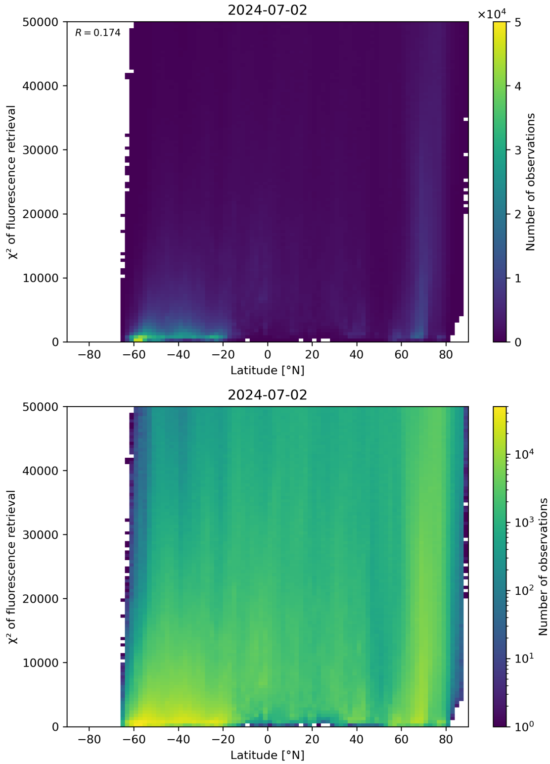
Figure 89: Scatter density plot of “Latitude” against “ \chi^2 of fluorescence retrieval” for 2024-07-01 to 2024-07-03.
