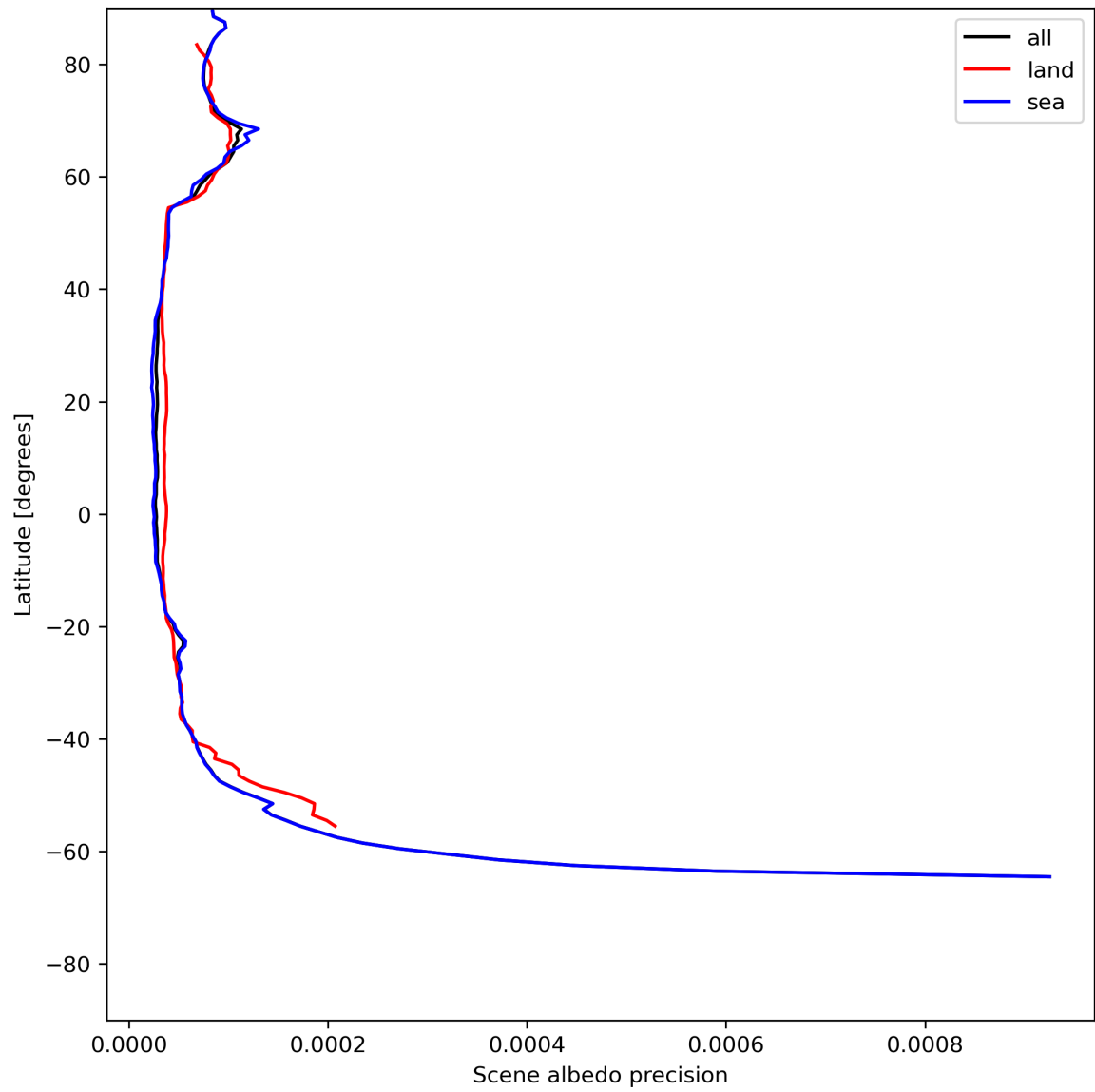
Figure 18: Zonal average of “Scene albedo precision” for 2024-07-01 to 2024-07-03.
