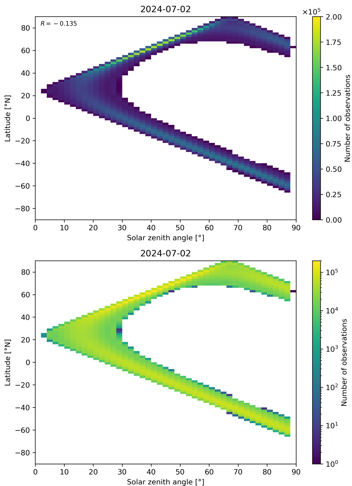
Figure 113: Scatter density plot of “Solar zenith angle” against “Latitude” for 2024-07-01 to 2024-07-03.
