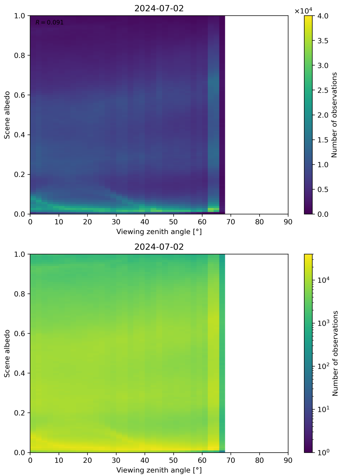
Figure 126: Scatter density plot of “Viewing zenith angle” against “Scene albedo” for 2024-07-01 to 2024-07-03.
