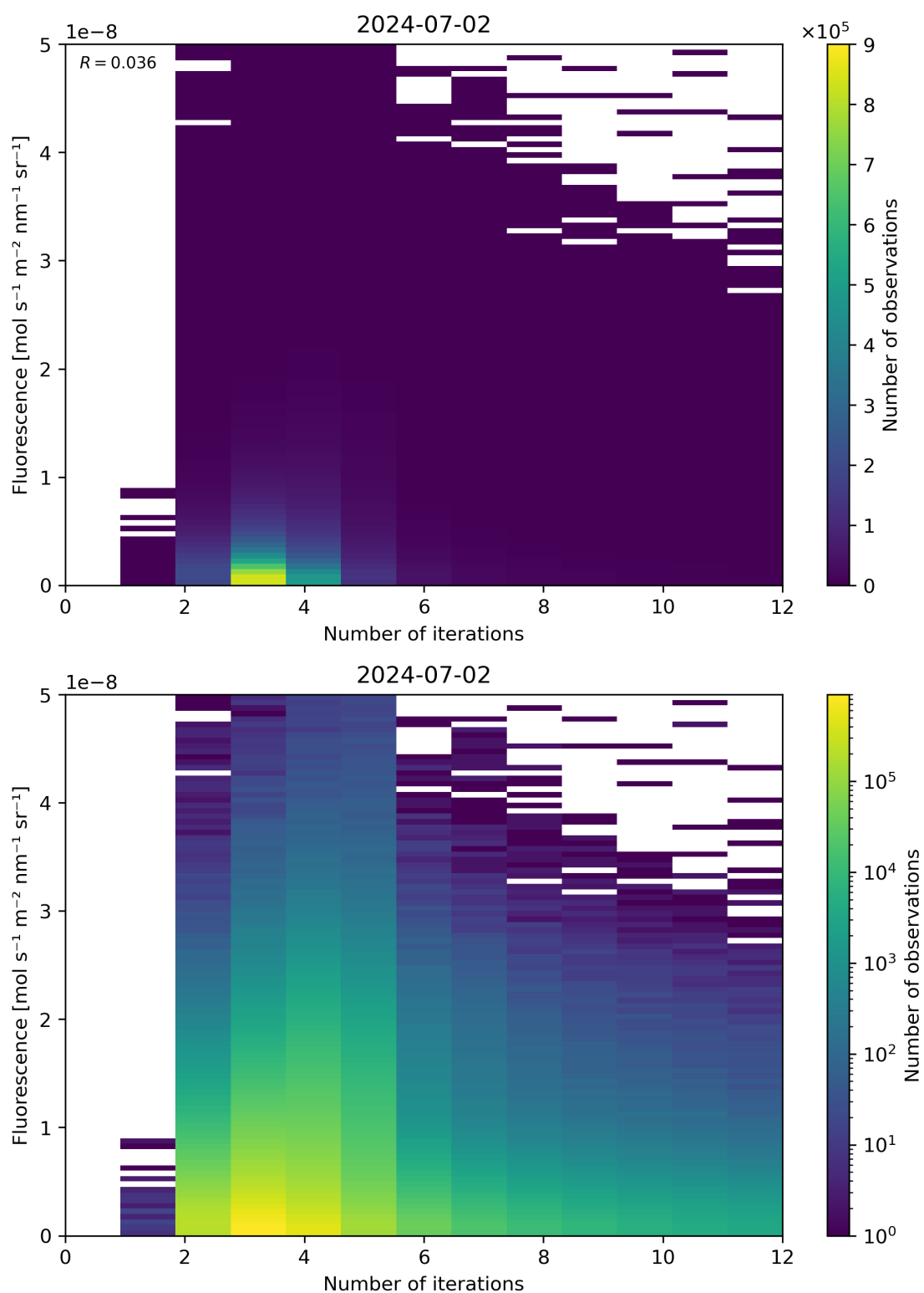
Figure 98: Scatter density plot of “Number of iterations” against “Fluorescence” for 2024-07-01 to 2024-07-03.
