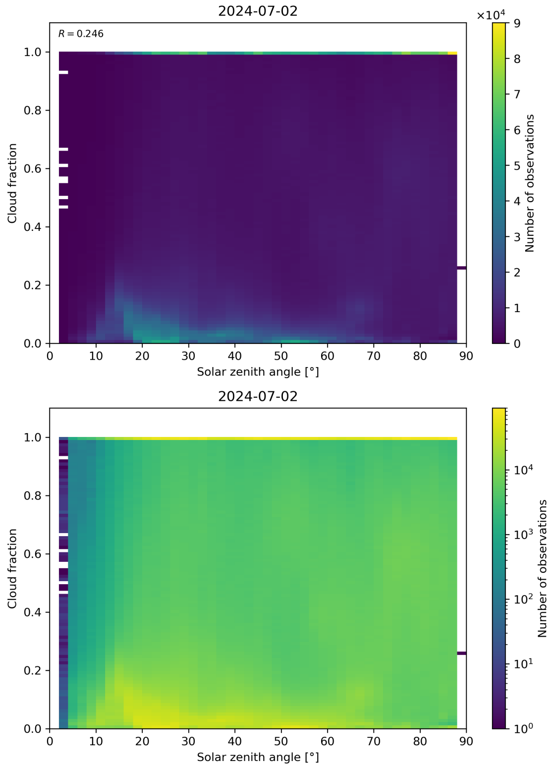
Figure 110: Scatter density plot of “Solar zenith angle” against “Cloud fraction” for 2024-07-01 to 2024-07-03.
