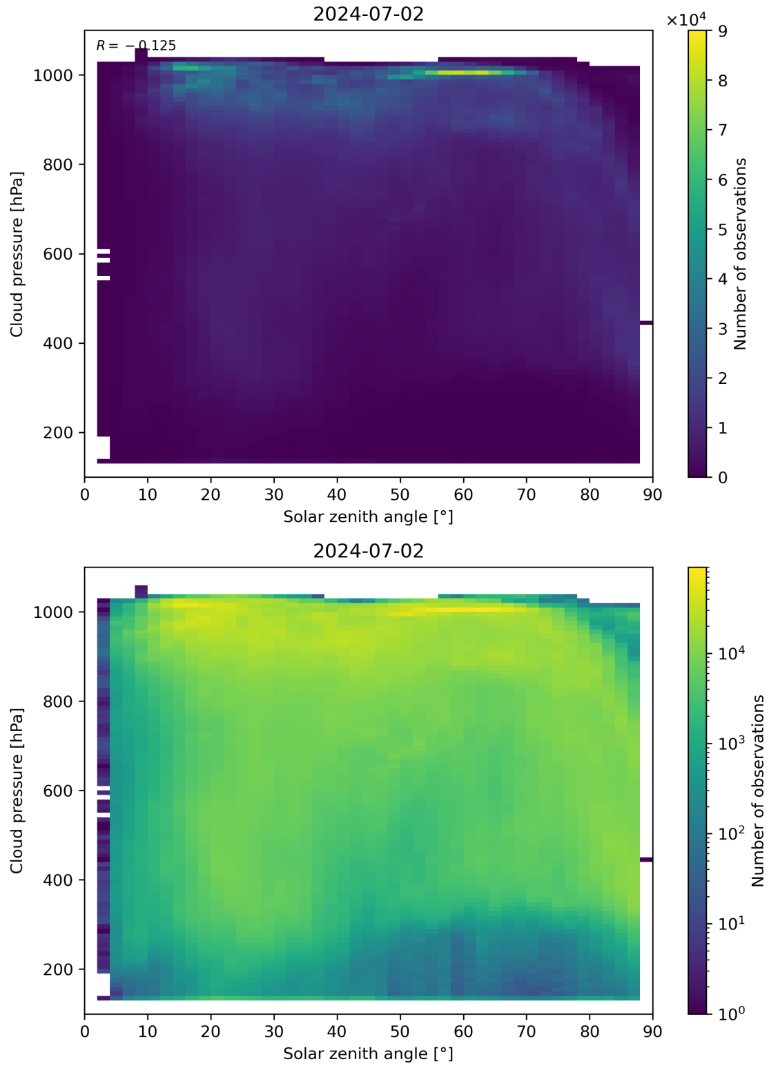
Figure 111: Scatter density plot of “Solar zenith angle” against “Cloud pressure” for 2024-07-01 to 2024-07-03.
