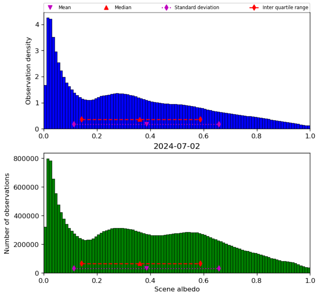
Figure 34: Histogram of “Scene albedo” for 2024-07-01 to 2024-07-03
