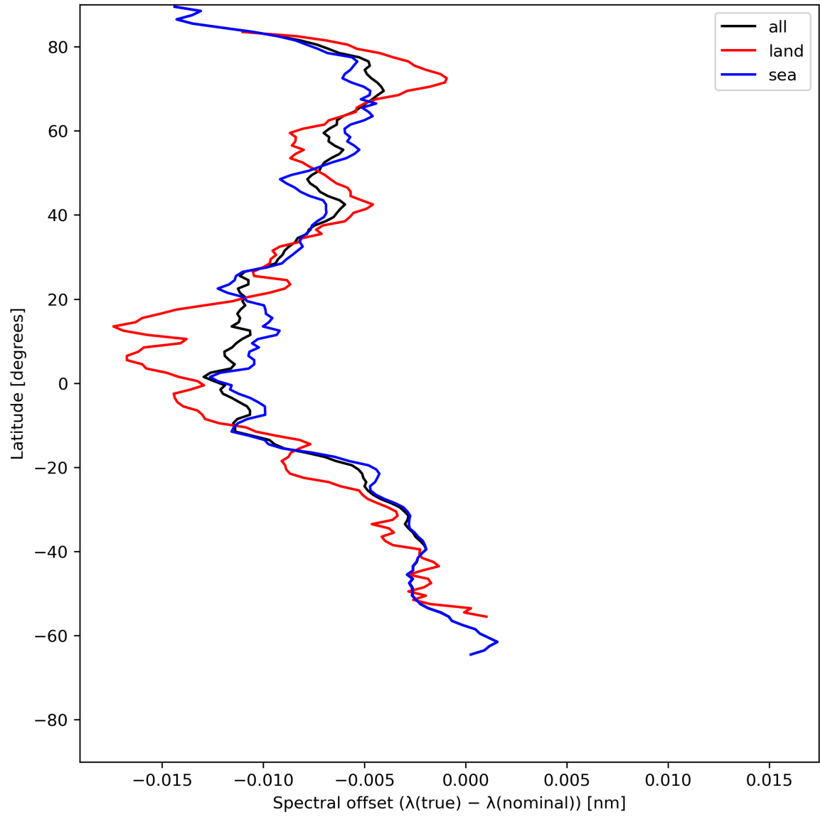
Figure 28: Zonal average of “Spectral offset ( \lambda(\text{true}) - \lambda(\text{nominal}) )” for 2024-07-01 to 2024-07-03.
