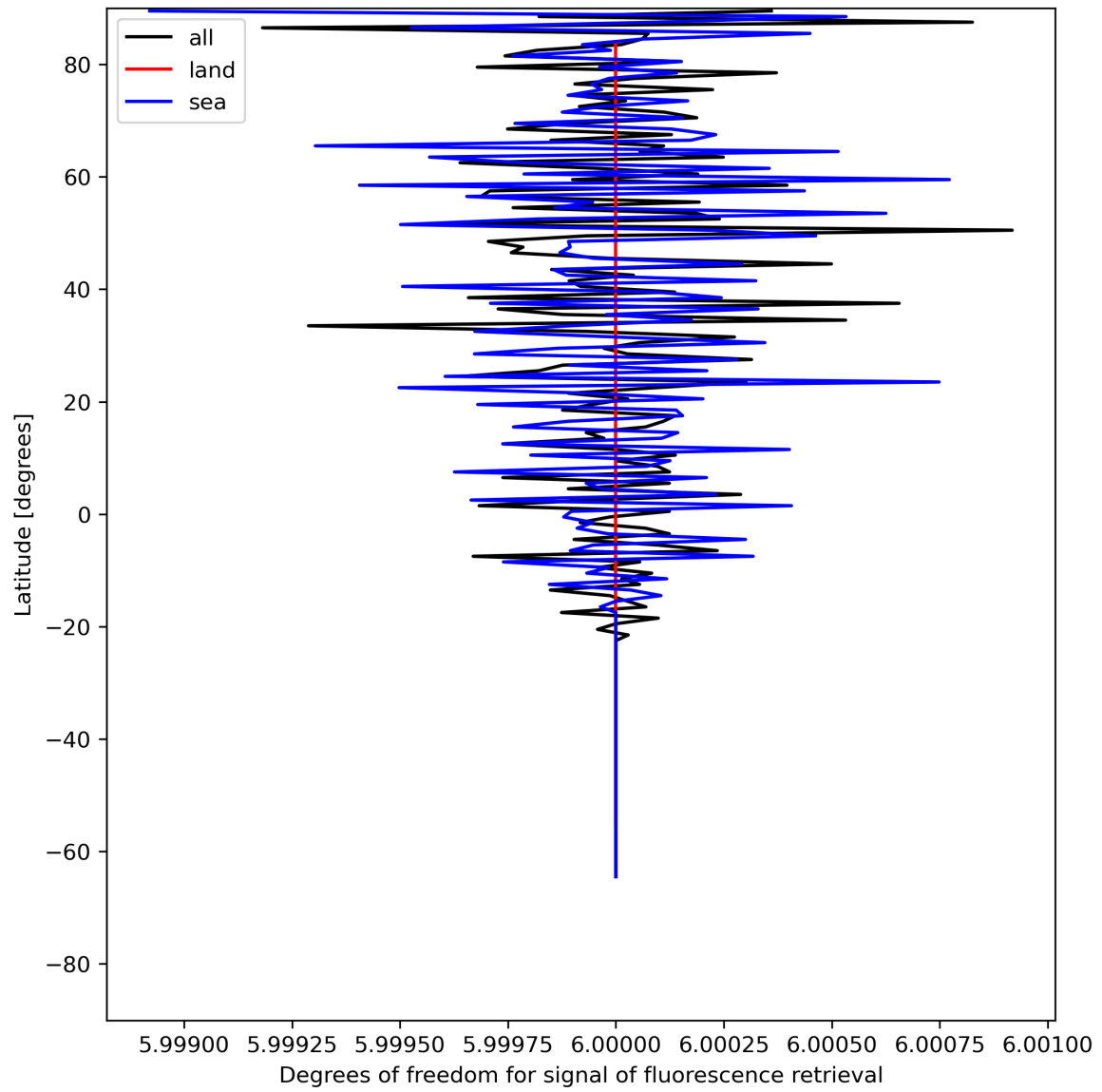
Figure 26: Zonal average of “Degrees of freedom for signal of fluorescence retrieval” for 2024-07-01 to 2024-07-03.
