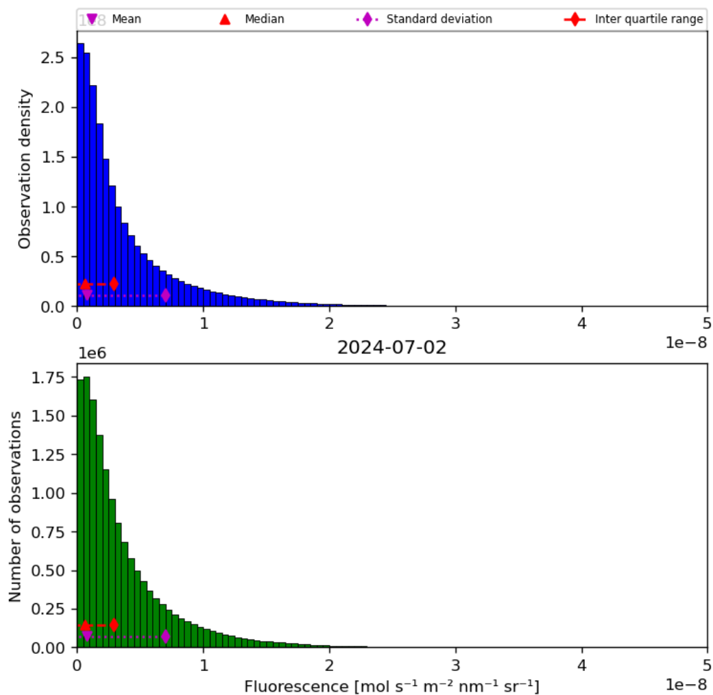
Figure 40: Histogram of “Fluorescence” for 2024-07-01 to 2024-07-03
