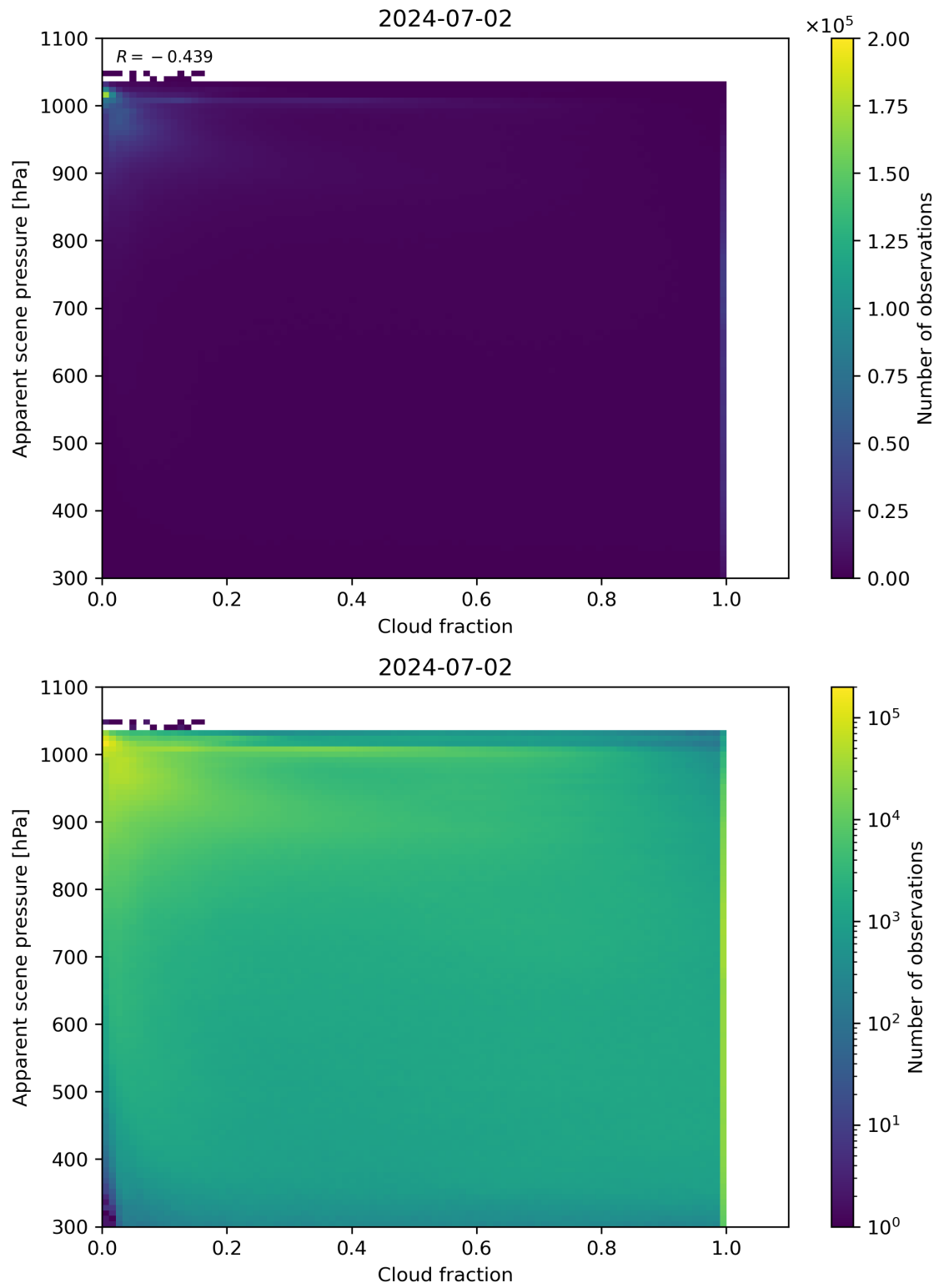
Figure 70: Scatter density plot of “Cloud fraction” against “Apparent scene pressure” for 2024-07-01 to 2024-07-03.
