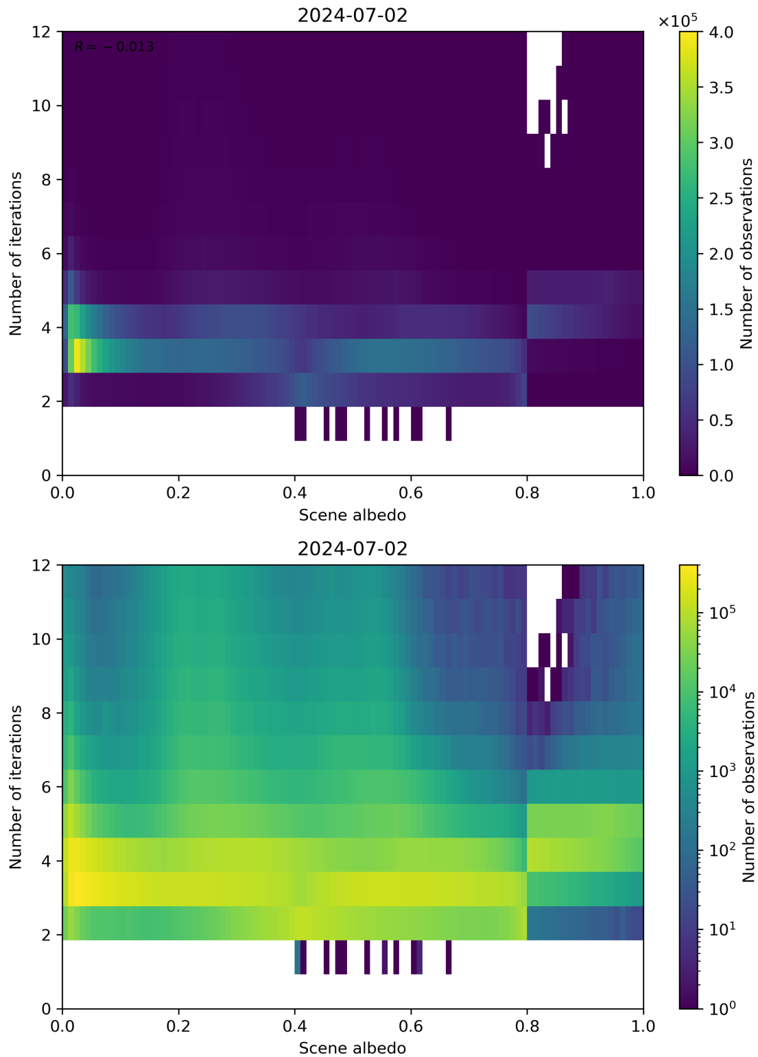
Figure 105: Scatter density plot of “Scene albedo” against “Number of iterations” for 2024-07-01 to 2024-07-03.
