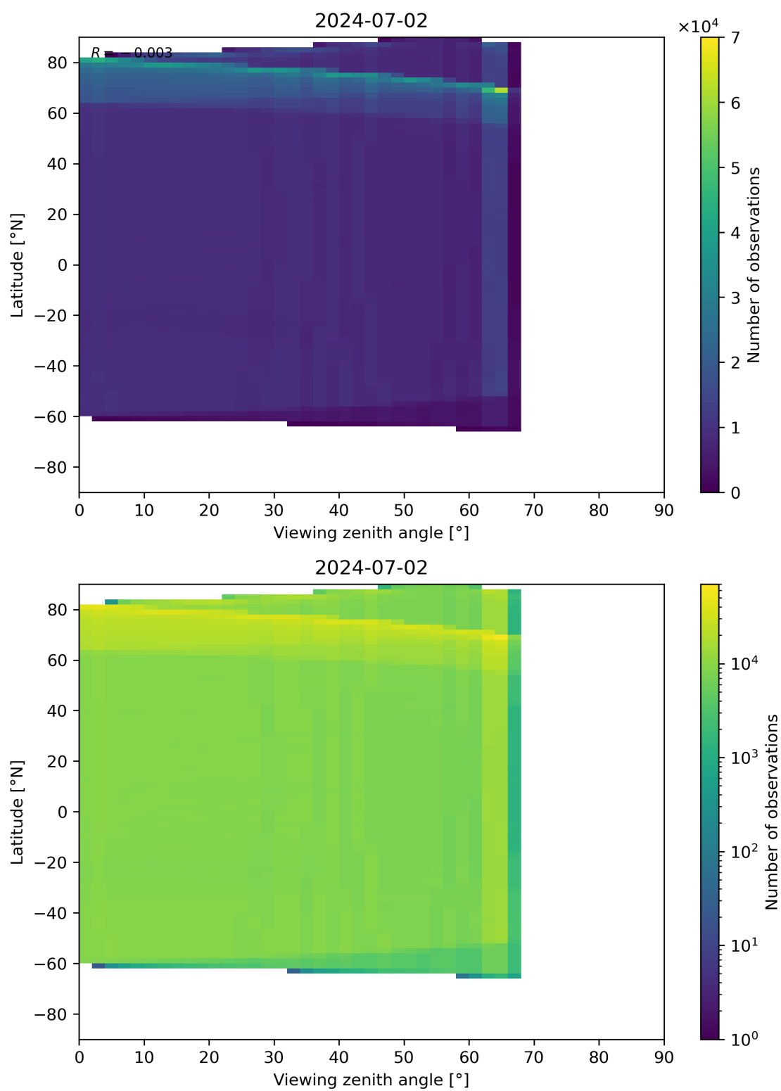
Figure 123: Scatter density plot of “Viewing zenith angle” against “Latitude” for 2024-07-01 to 2024-07-03.
