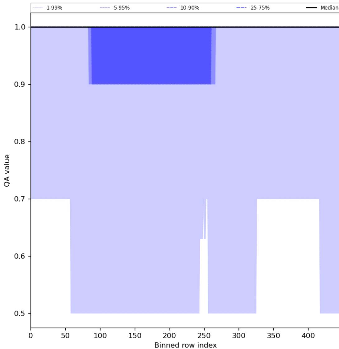
Figure 46: Along track statistics of “QA value” for 2024-07-01 to 2024-07-03
