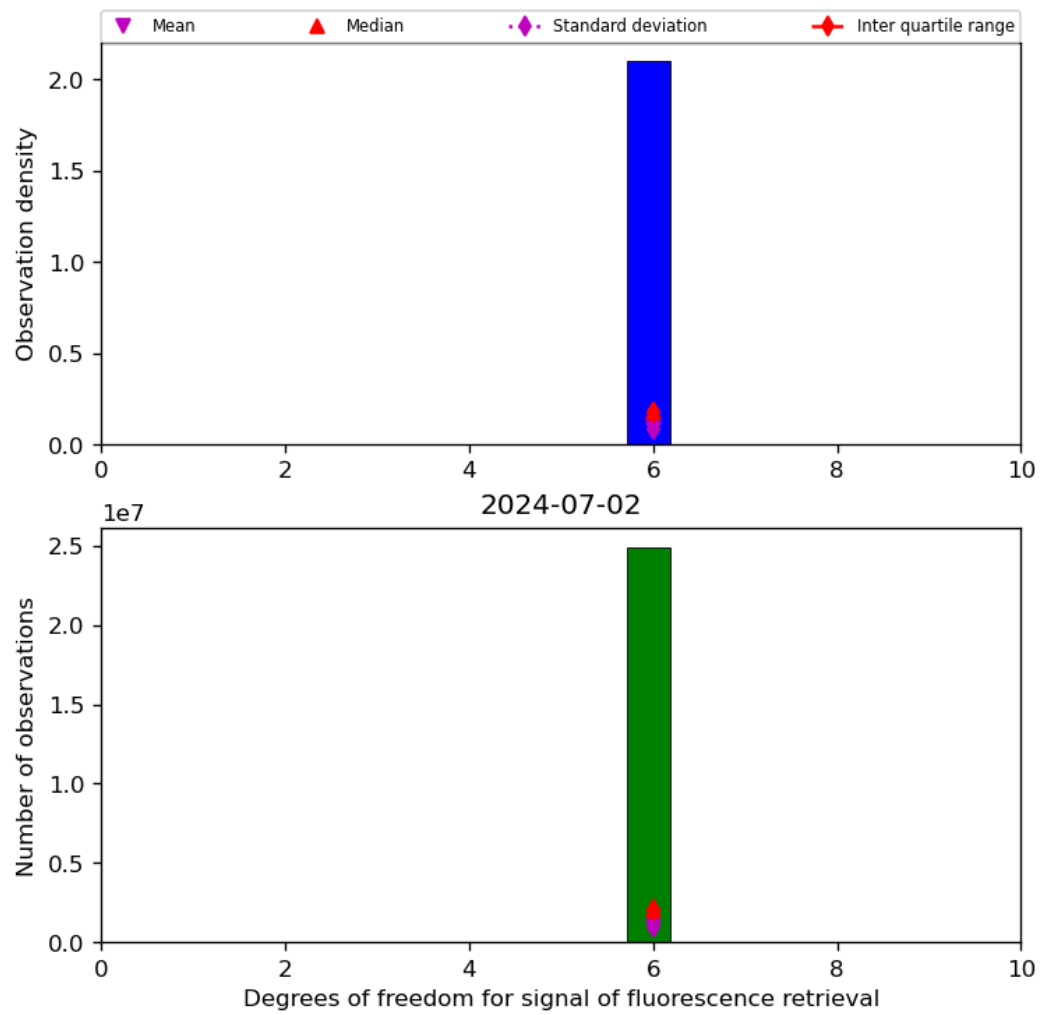
Figure 43: Histogram of “Degrees of freedom for signal of fluorescence retrieval” for 2024-07-01 to 2024-07-03
