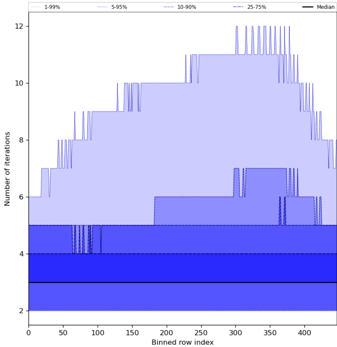
Figure 56: Along track statistics of “Number of iterations” for 2024-07-01 to 2024-07-03
