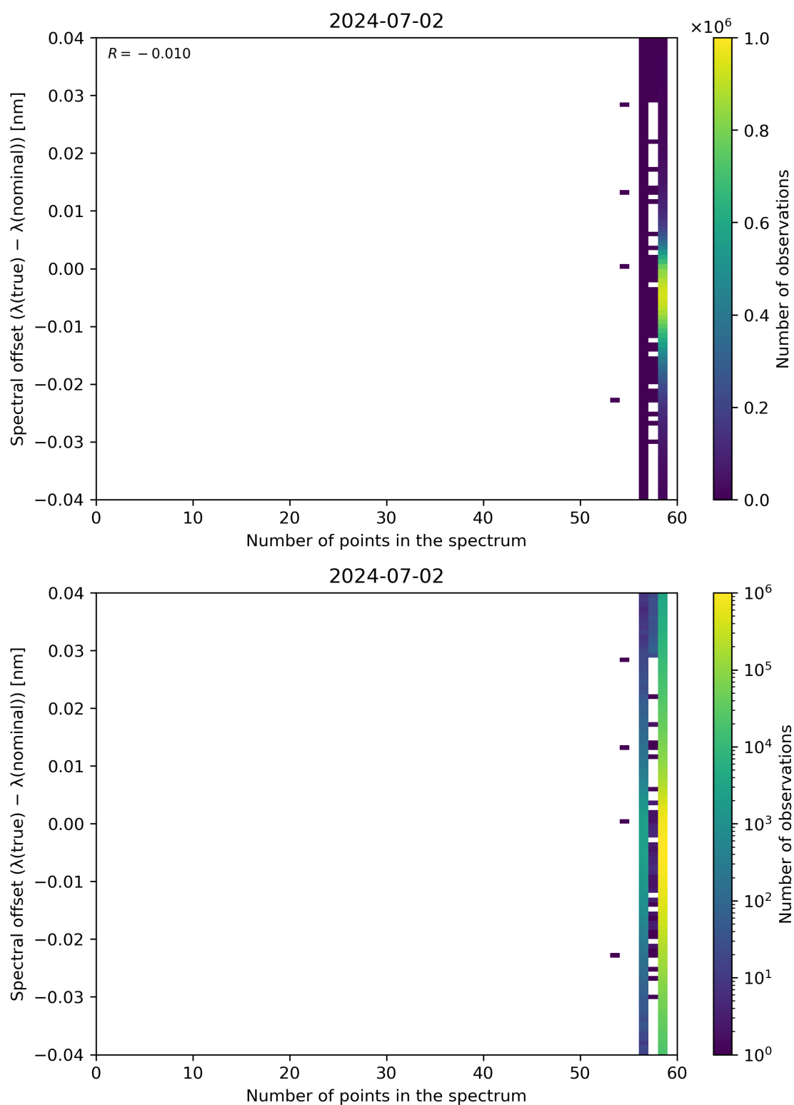
Figure 101: Scatter density plot of “Number of points in the spectrum” against “Spectral offset ( \lambda(\text{true}) - \lambda(\text{nominal}) )” for 2024-07-01 to 2024-07-03.
