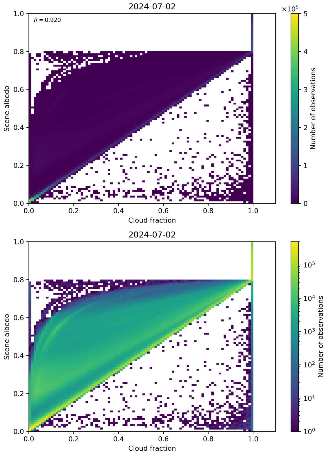
Figure 75: Scatter density plot of “Cloud fraction” against “Scene albedo” for 2024-07-01 to 2024-07-03.
