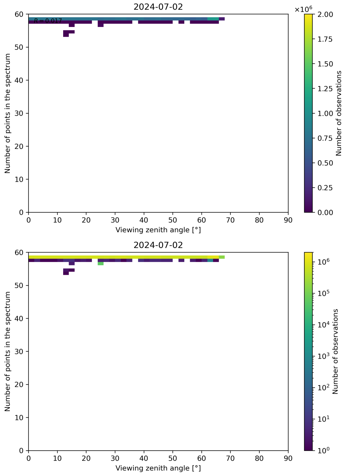
Figure 125: Scatter density plot of “Viewing zenith angle” against “Number of points in the spectrum” for 2024-07-01 to 2024-07-03.
