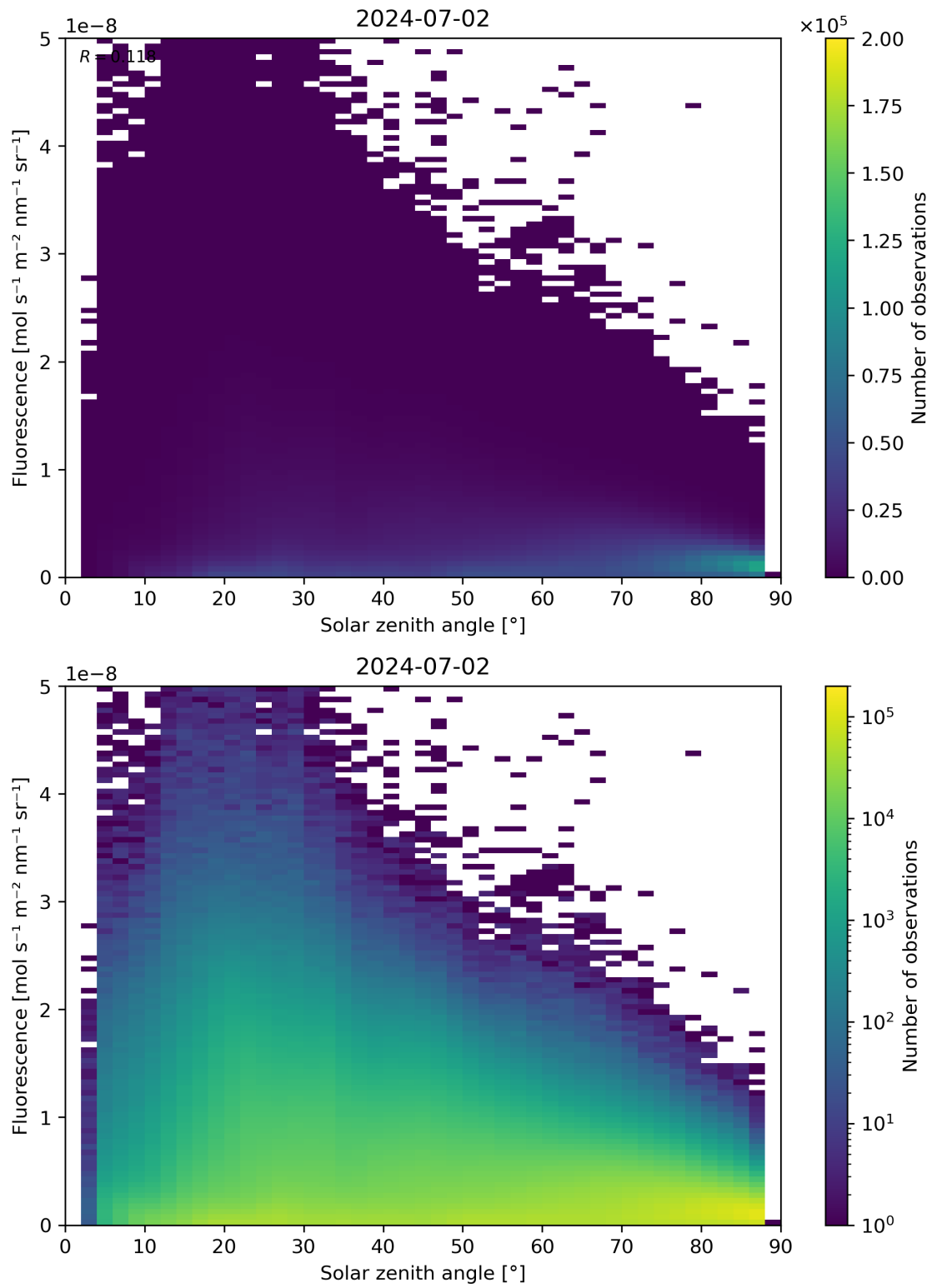
Figure 112: Scatter density plot of “Solar zenith angle” against “Fluorescence” for 2024-07-01 to 2024-07-03.
