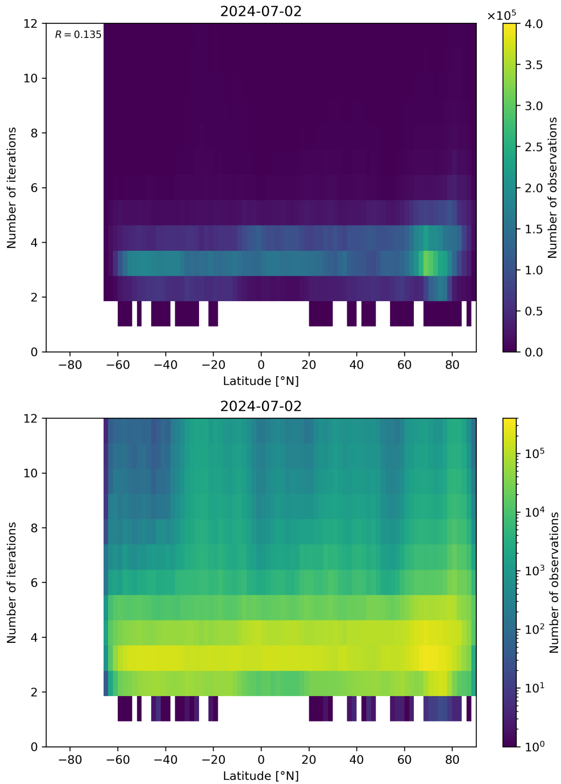
Figure 93: Scatter density plot of “Latitude” against “Number of iterations” for 2024-07-01 to 2024-07-03.
