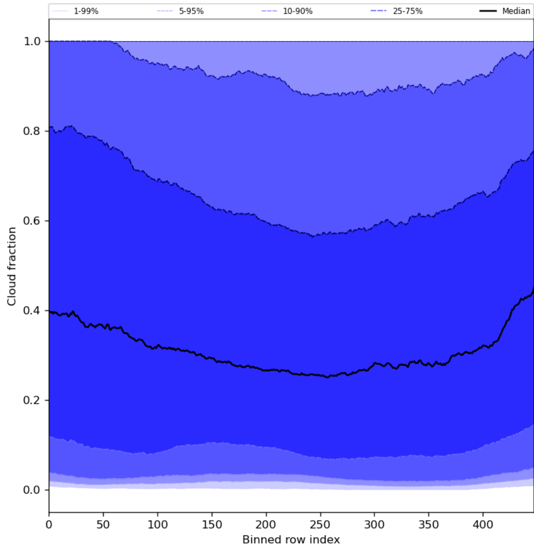
Figure 49: Along track statistics of “Cloud fraction” for 2024-07-01 to 2024-07-03
