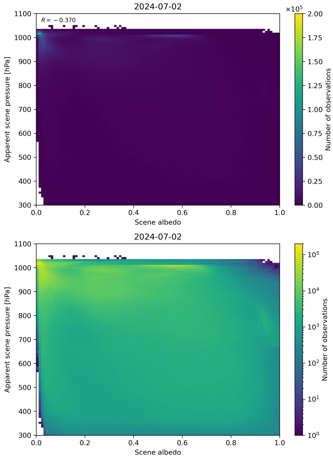
Figure 102: Scatter density plot of “Scene albedo” against “Apparent scene pressure” for 2024-07-01 to 2024-07-03.
