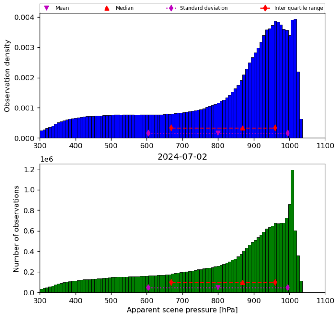
Figure 36: Histogram of “Apparent scene pressure” for 2024-07-01 to 2024-07-03
