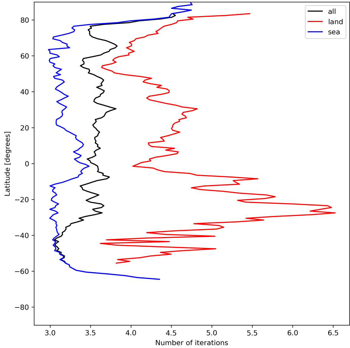
Figure 22: Zonal average of “Number of iterations” for 2024-07-01 to 2024-07-03.
