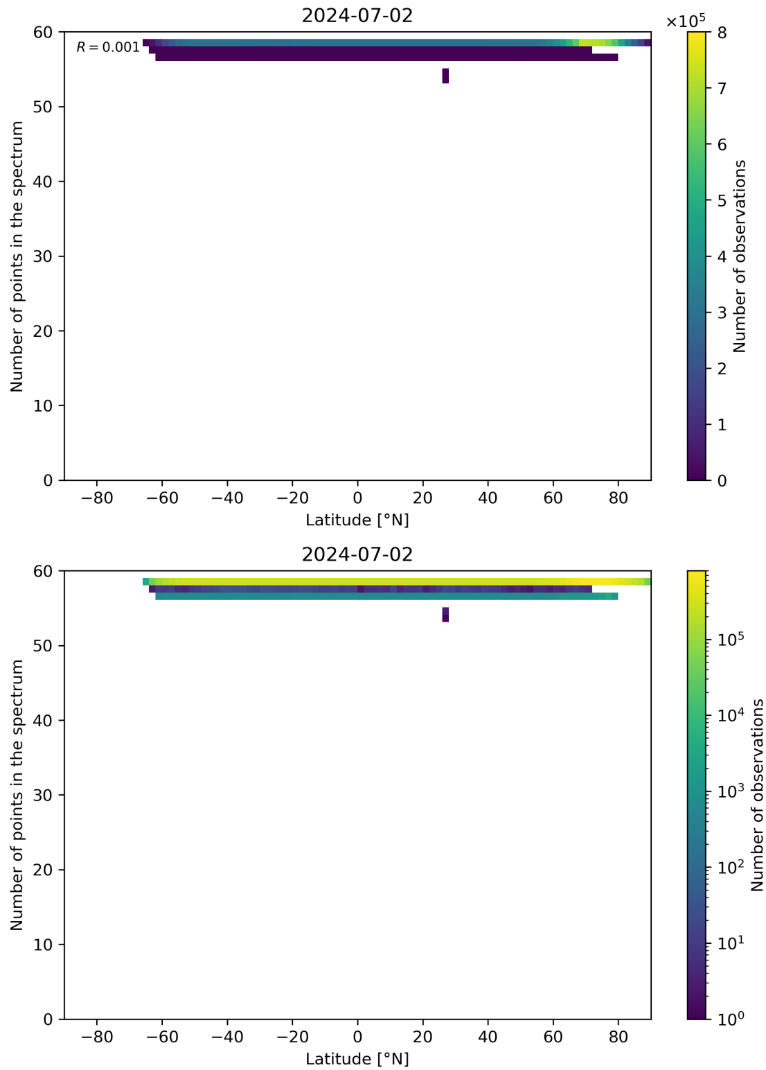
Figure 94: Scatter density plot of “Latitude” against “Number of points in the spectrum” for 2024-07-01 to 2024-07-03.
