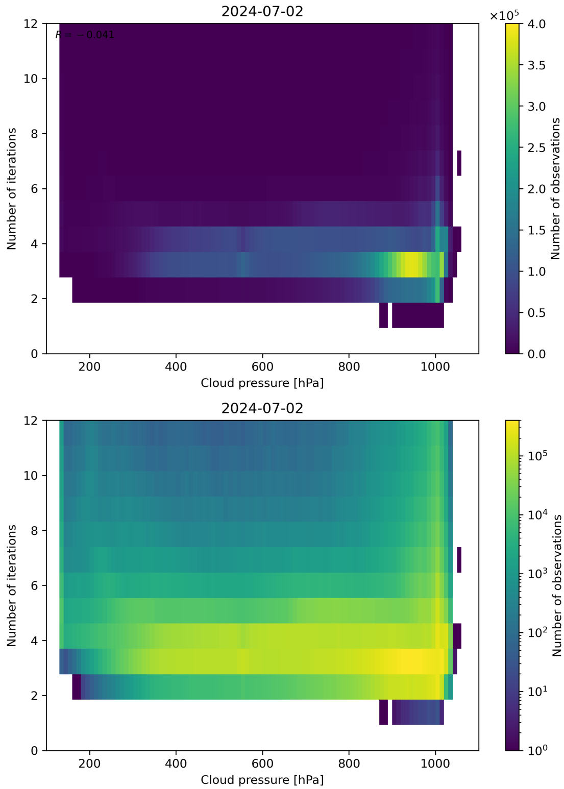
Figure 81: Scatter density plot of “Cloud pressure” against “Number of iterations” for 2024-07-01 to 2024-07-03.
