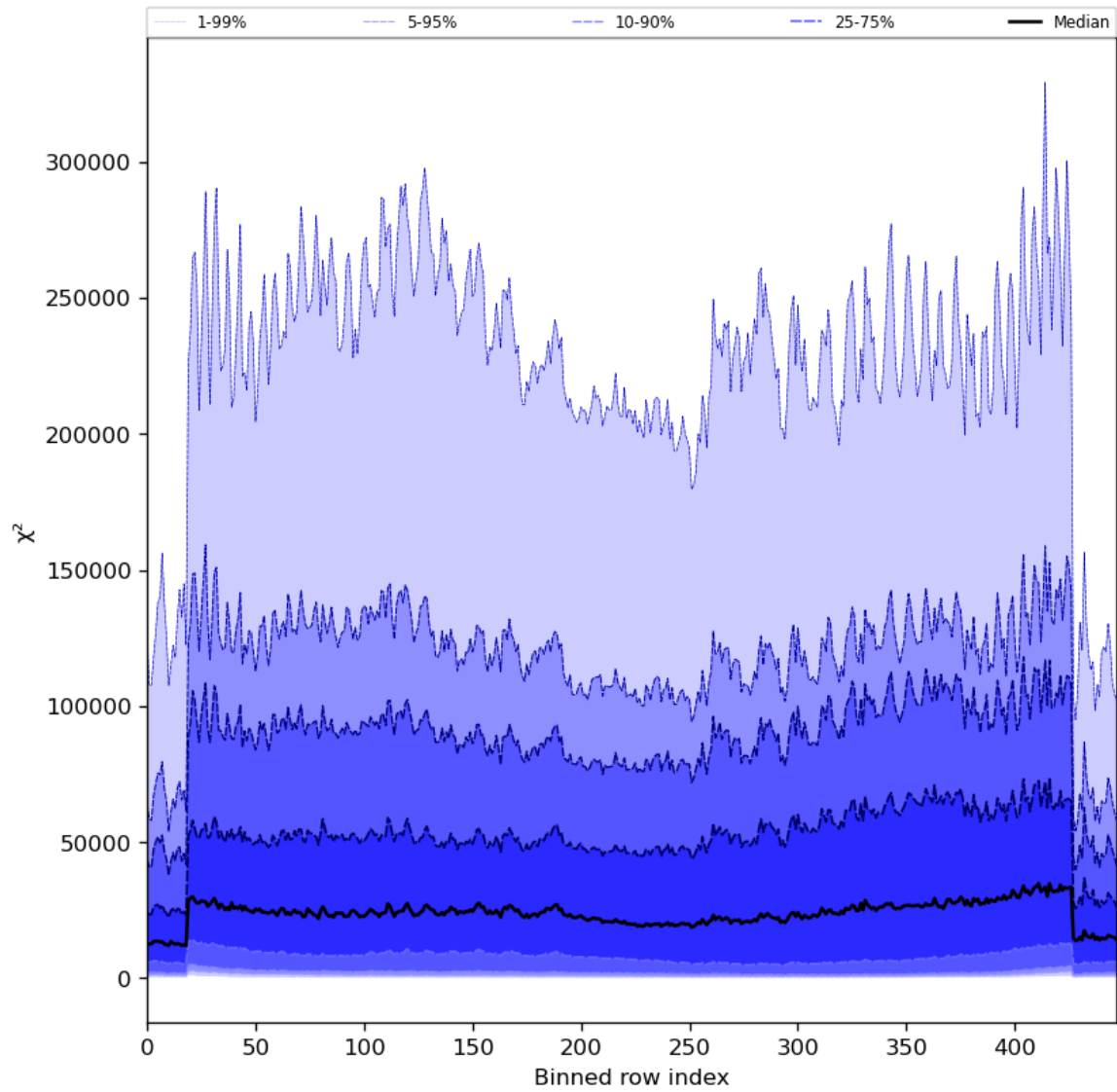
Figure 55: Along track statistics of “ \chi^2 ” for 2024-07-01 to 2024-07-03
