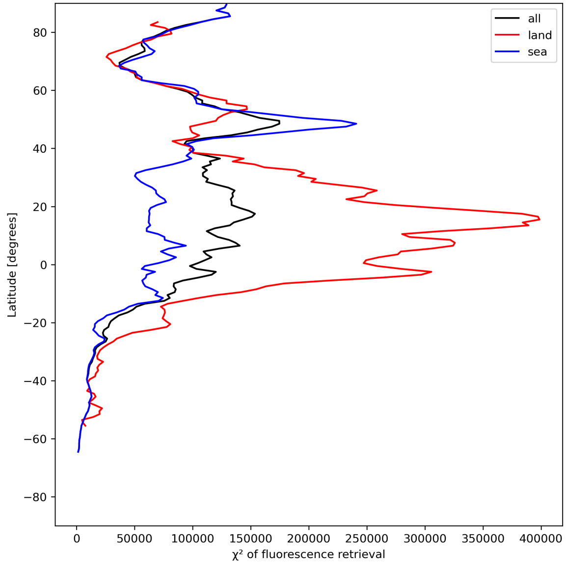
Figure 25: Zonal average of “ \chi^2 of fluorescence retrieval” for 2024-07-01 to 2024-07-03.
