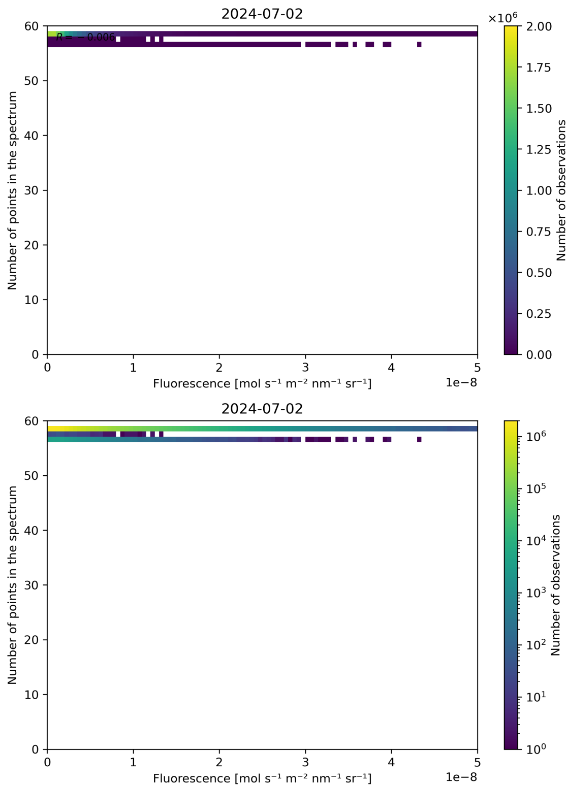
Figure 86: Scatter density plot of “Fluorescence” against “Number of points in the spectrum” for 2024-07-01 to 2024-07-03.
