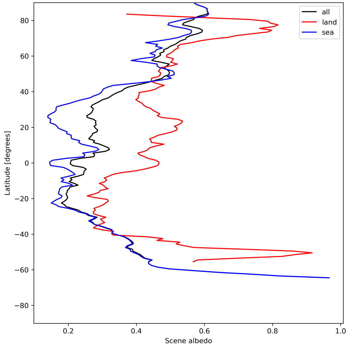
Figure 17: Zonal average of “Scene albedo” for 2024-07-01 to 2024-07-03.
