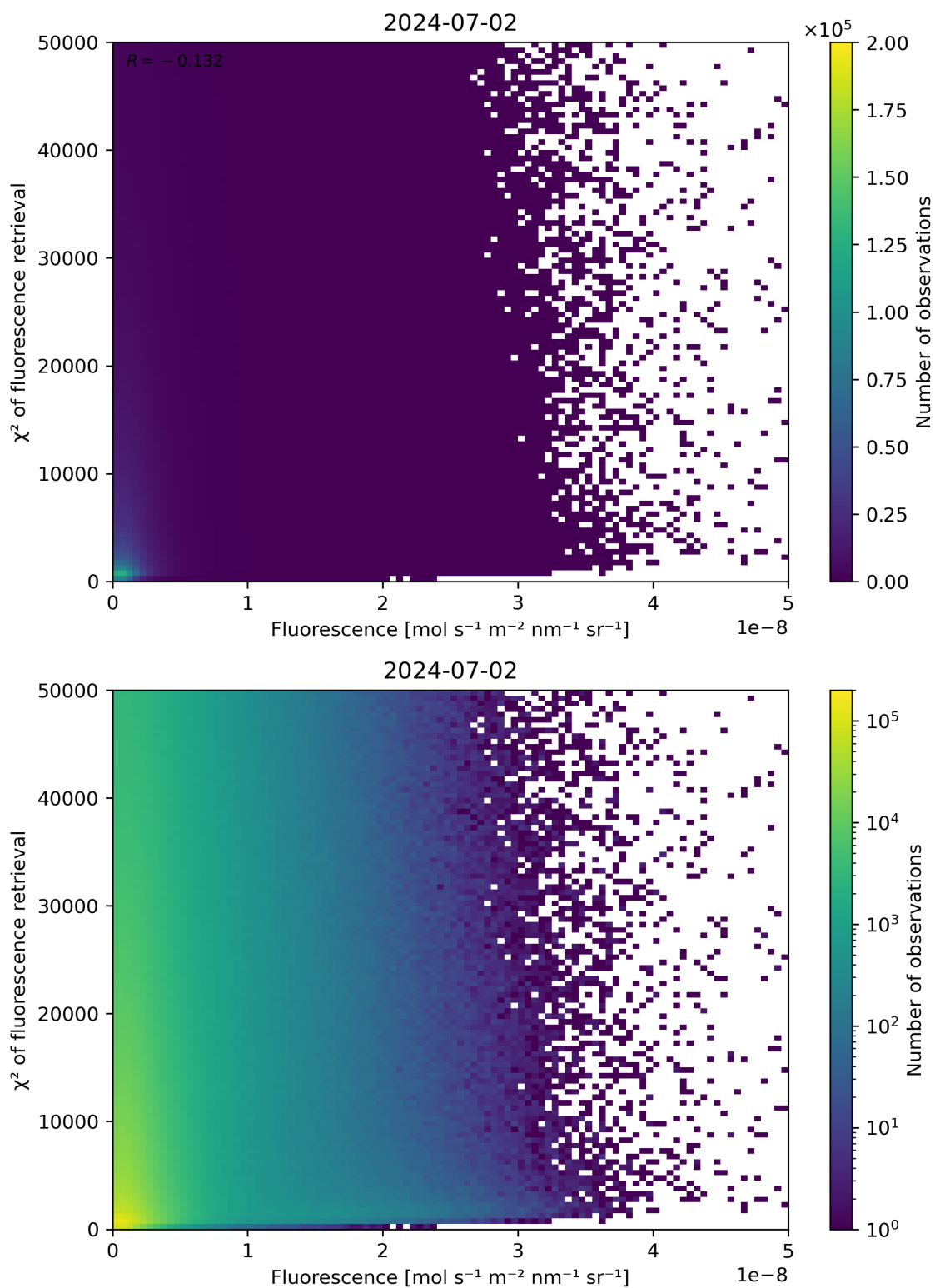
Figure 85: Scatter density plot of “Fluorescence” against “ \chi^2 of fluorescence retrieval” for 2024-07-01 to 2024-07-03.
