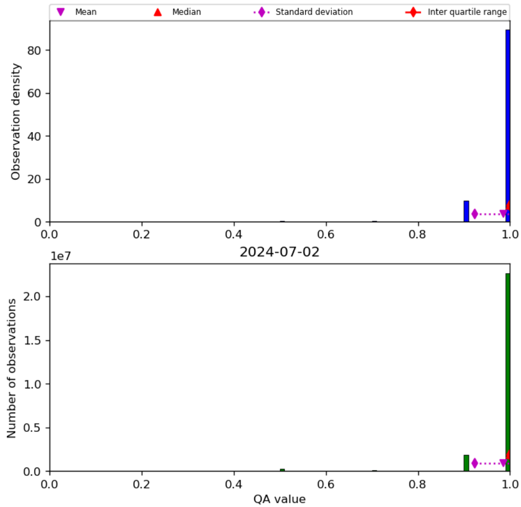
Figure 29: Histogram of “QA value” for 2024-07-01 to 2024-07-03
