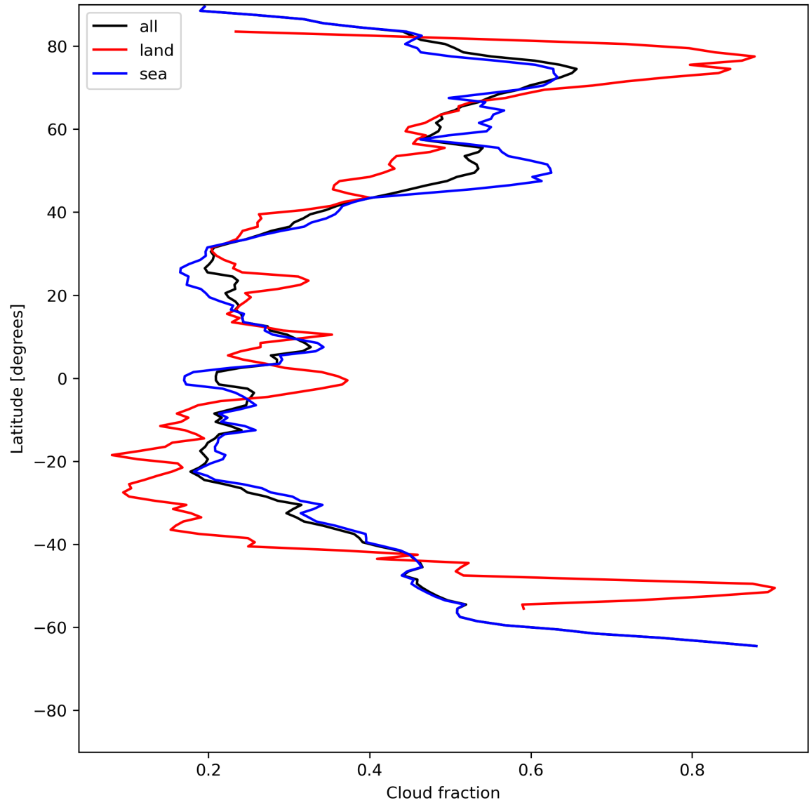
Figure 15: Zonal average of “Cloud fraction” for 2024-07-01 to 2024-07-03.
