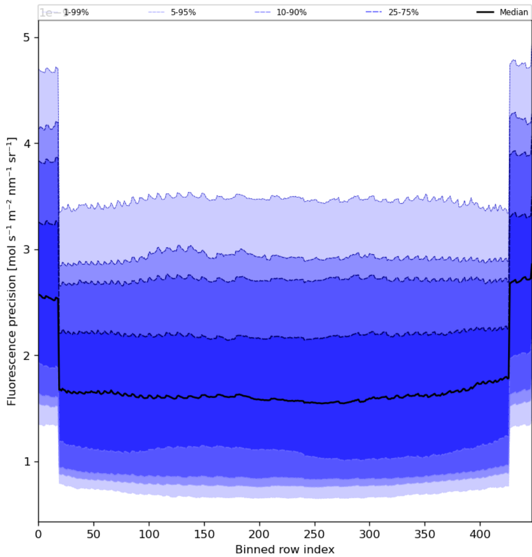
Figure 58: Along track statistics of “Fluorescence precision” for 2024-07-01 to 2024-07-03
