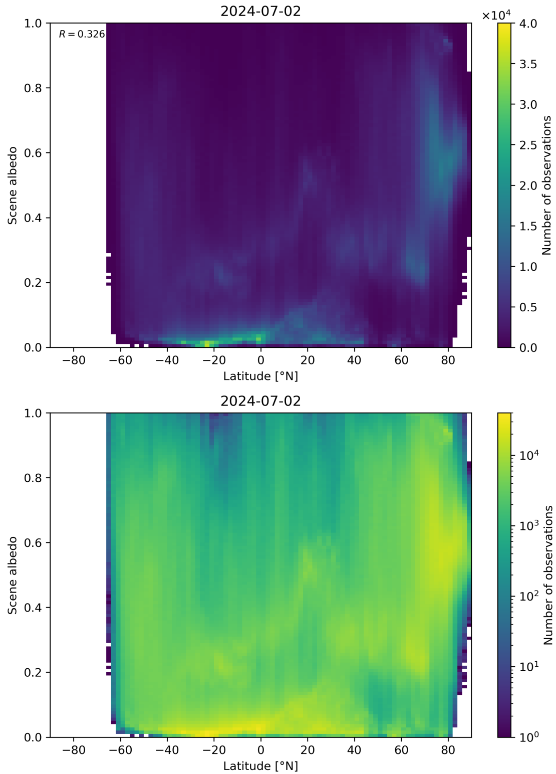
Figure 95: Scatter density plot of “Latitude” against “Scene albedo” for 2024-07-01 to 2024-07-03.
