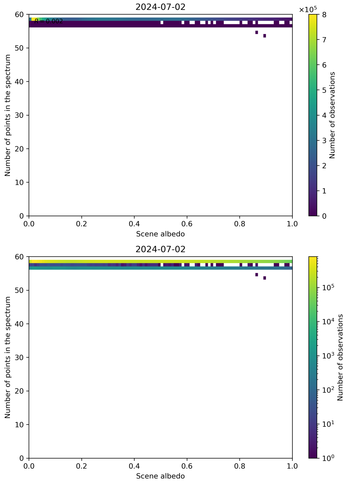
Figure 106: Scatter density plot of “Scene albedo” against “Number of points in the spectrum” for 2024-07-01 to 2024-07-03.
