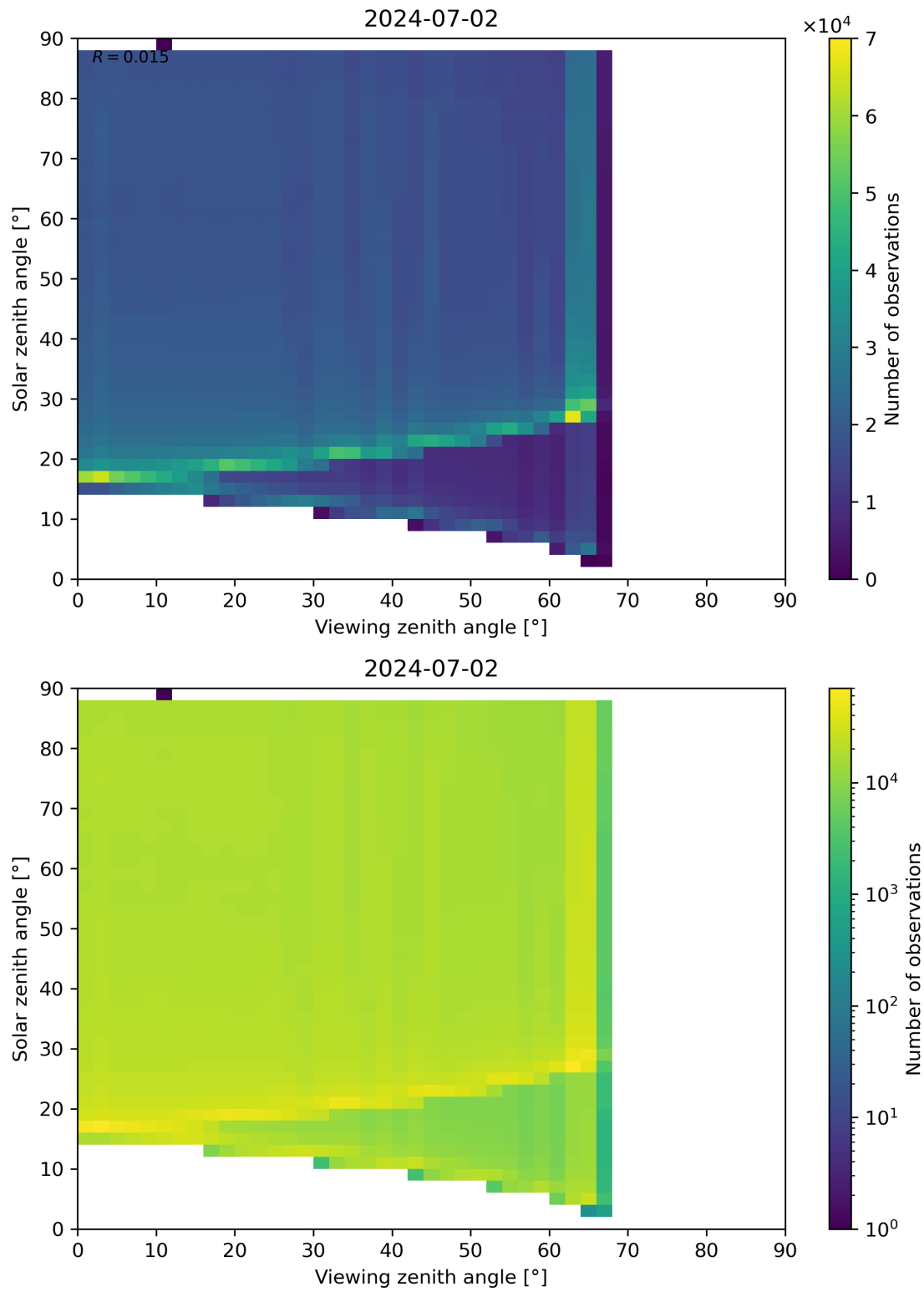
Figure 127: Scatter density plot of “Viewing zenith angle” against “Solar zenith angle” for 2024-07-01 to 2024-07-03.
