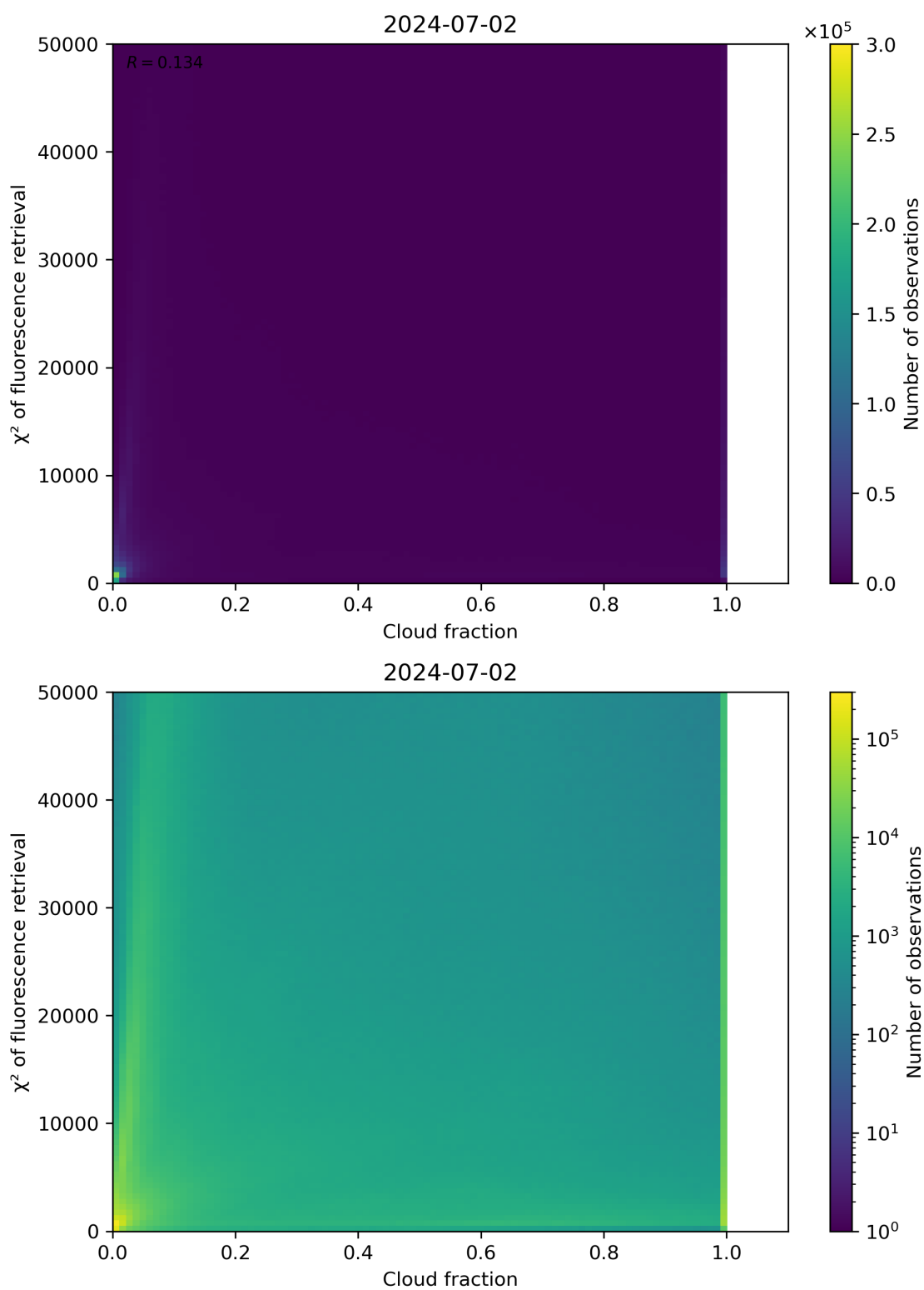
Figure 71: Scatter density plot of “Cloud fraction” against “ \chi^2 of fluorescence retrieval” for 2024-07-01 to 2024-07-03.
