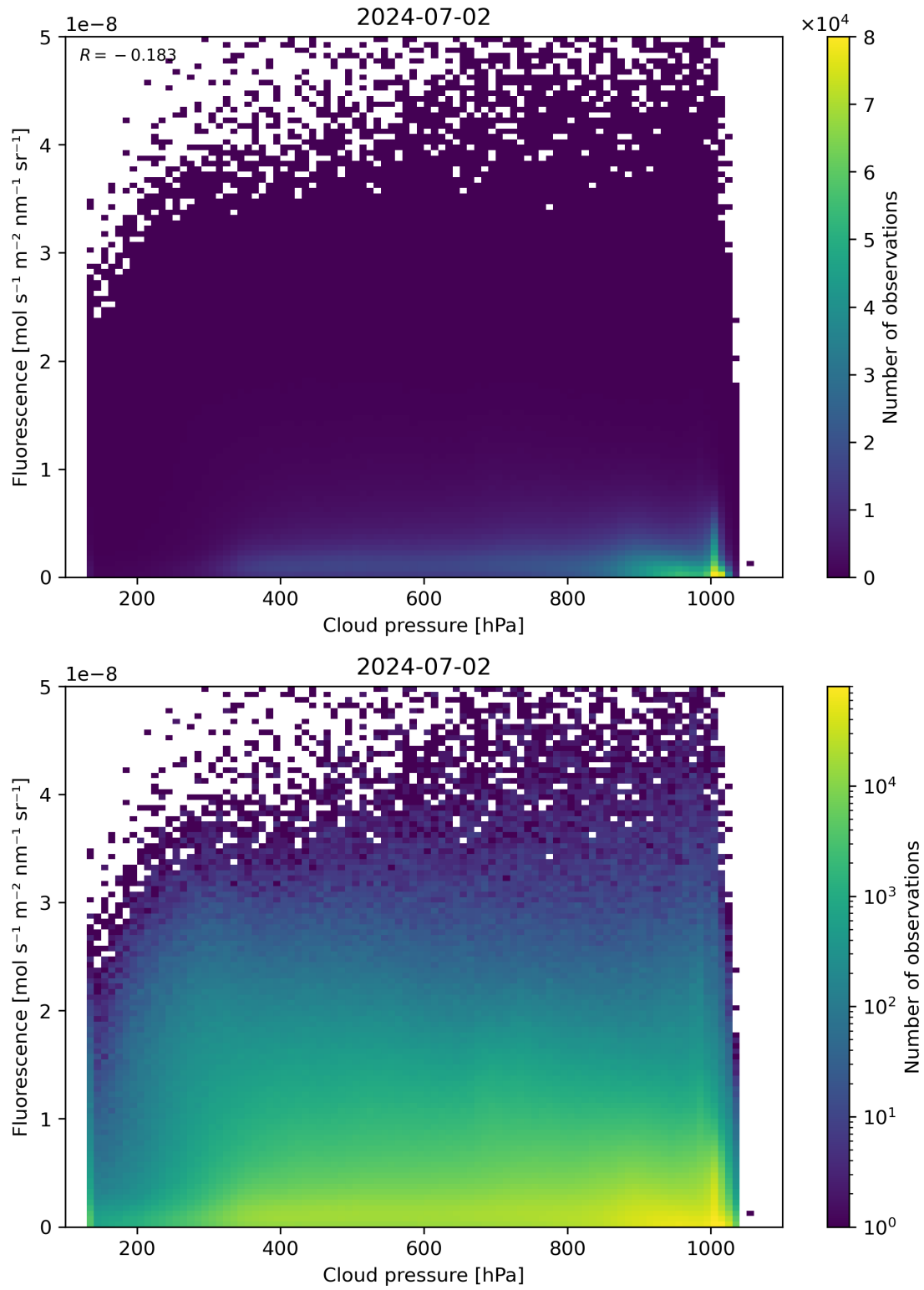
Figure 80: Scatter density plot of “Cloud pressure” against “Fluorescence” for 2024-07-01 to 2024-07-03.
