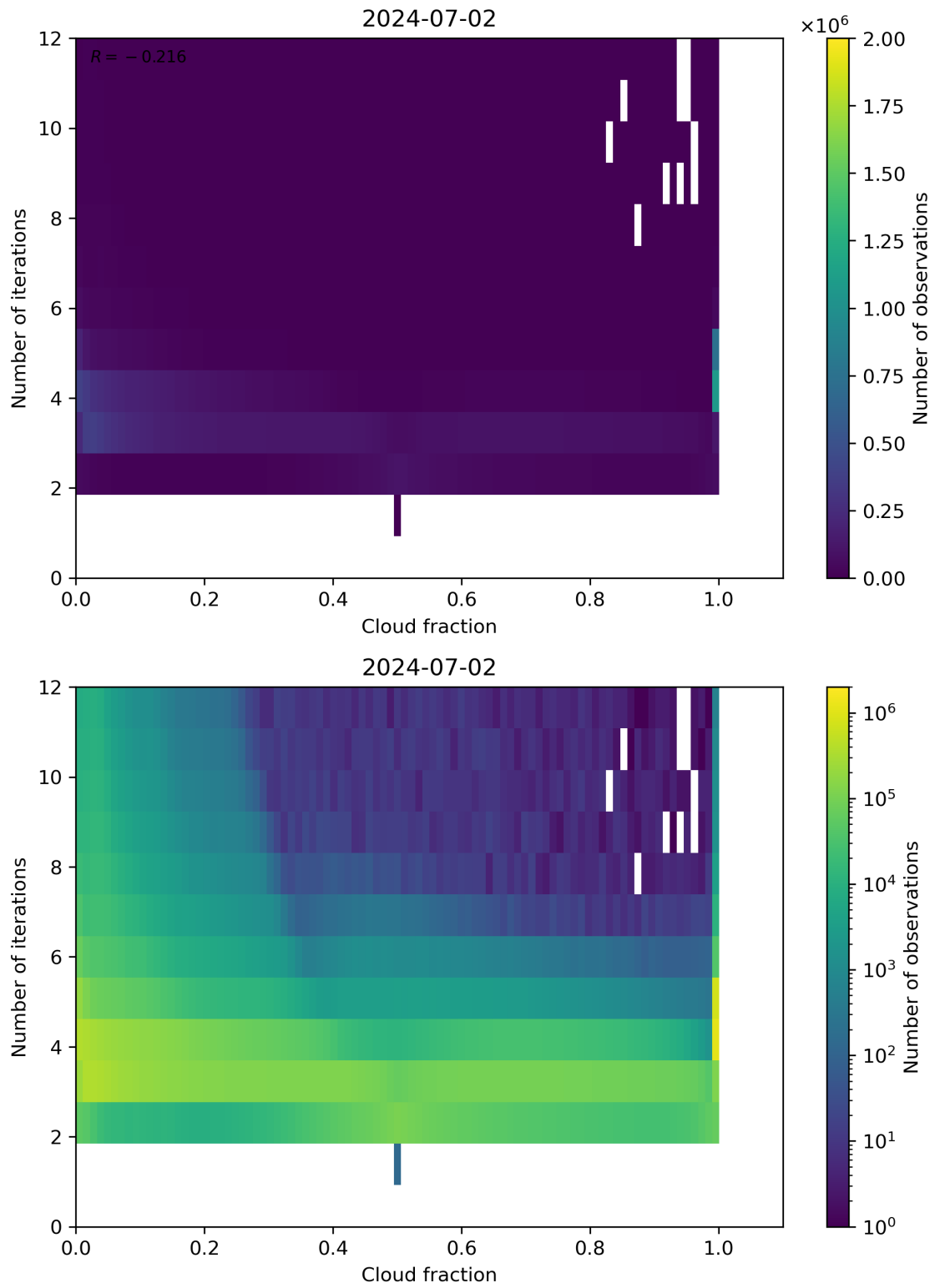
Figure 73: Scatter density plot of “Cloud fraction” against “Number of iterations” for 2024-07-01 to 2024-07-03.
