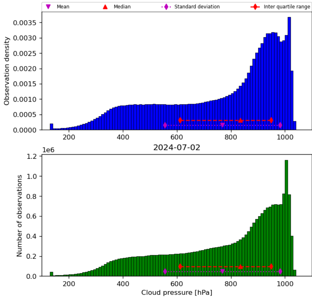
Figure 30: Histogram of “Cloud pressure” for 2024-07-01 to 2024-07-03
