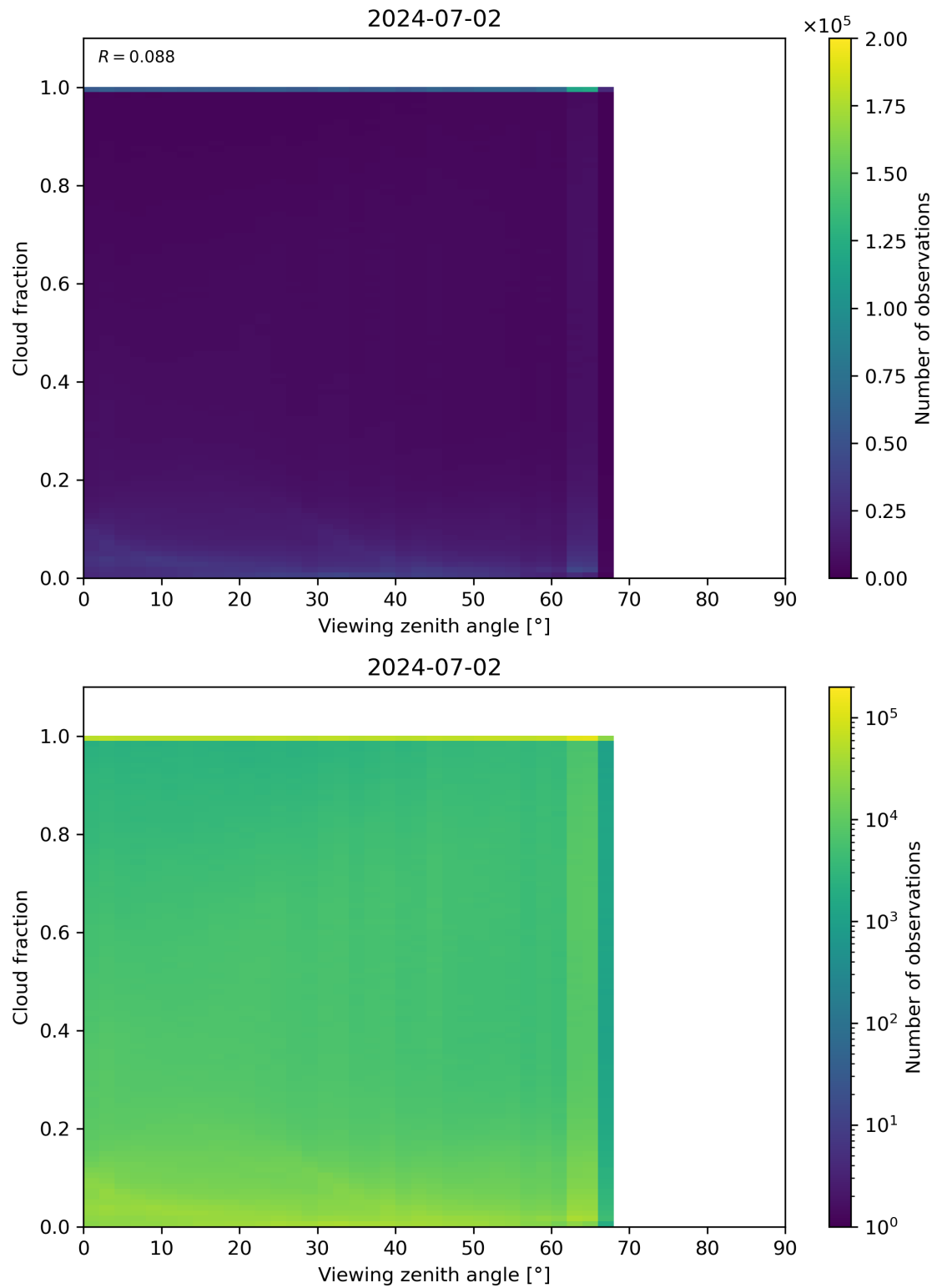
Figure 120: Scatter density plot of “Viewing zenith angle” against “Cloud fraction” for 2024-07-01 to 2024-07-03.
