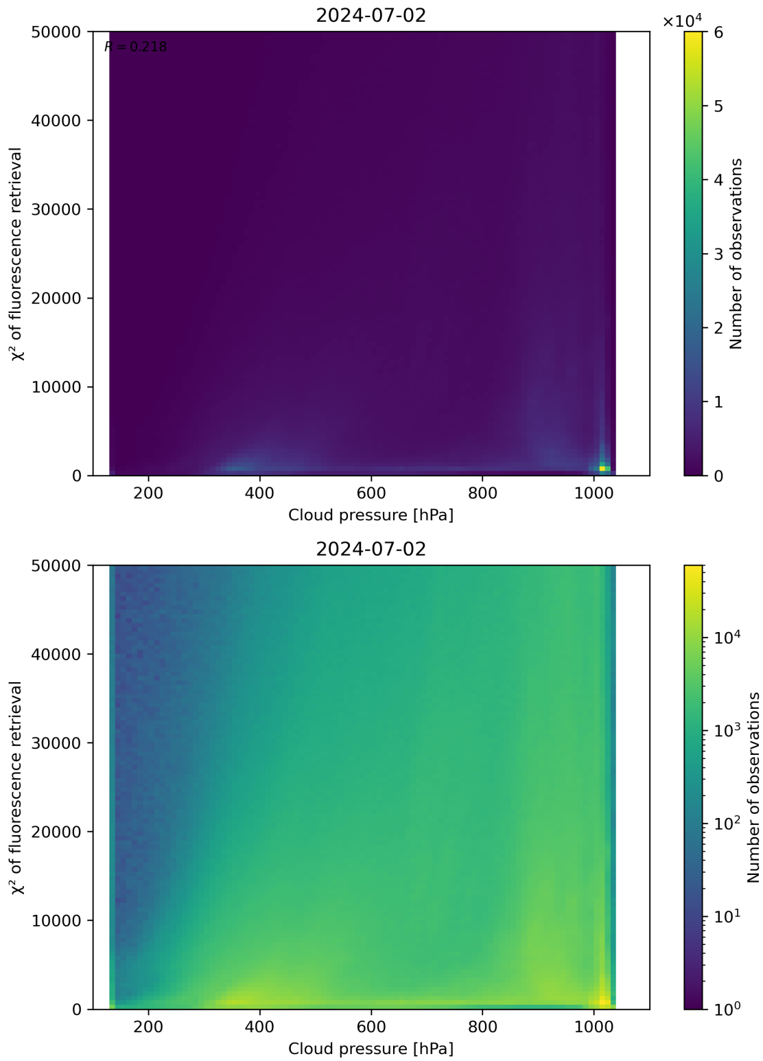
Figure 78: Scatter density plot of “Cloud pressure” against “ \chi^2 of fluorescence retrieval” for 2024-07-01 to 2024-07-03.
