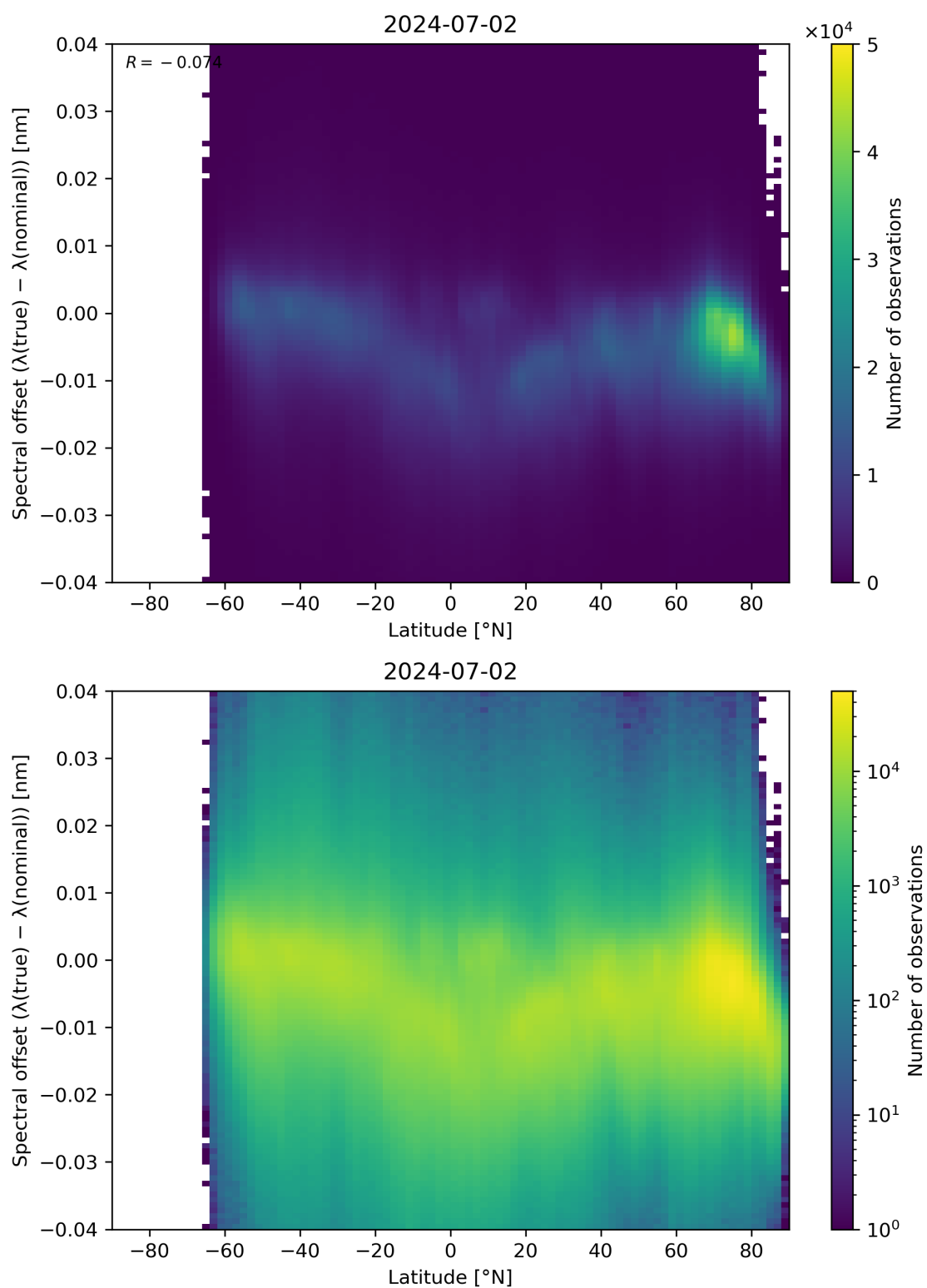
Figure 96: Scatter density plot of “Latitude” against “Spectral offset ( \lambda(\text{true}) - \lambda(\text{nominal}) )” for 2024-07-01 to 2024-07-03.
