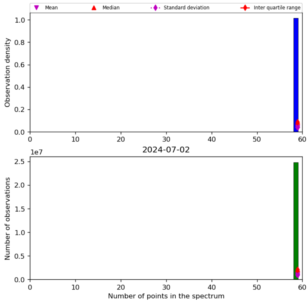
Figure 44: Histogram of “Number of points in the spectrum” for 2024-07-01 to 2024-07-03
