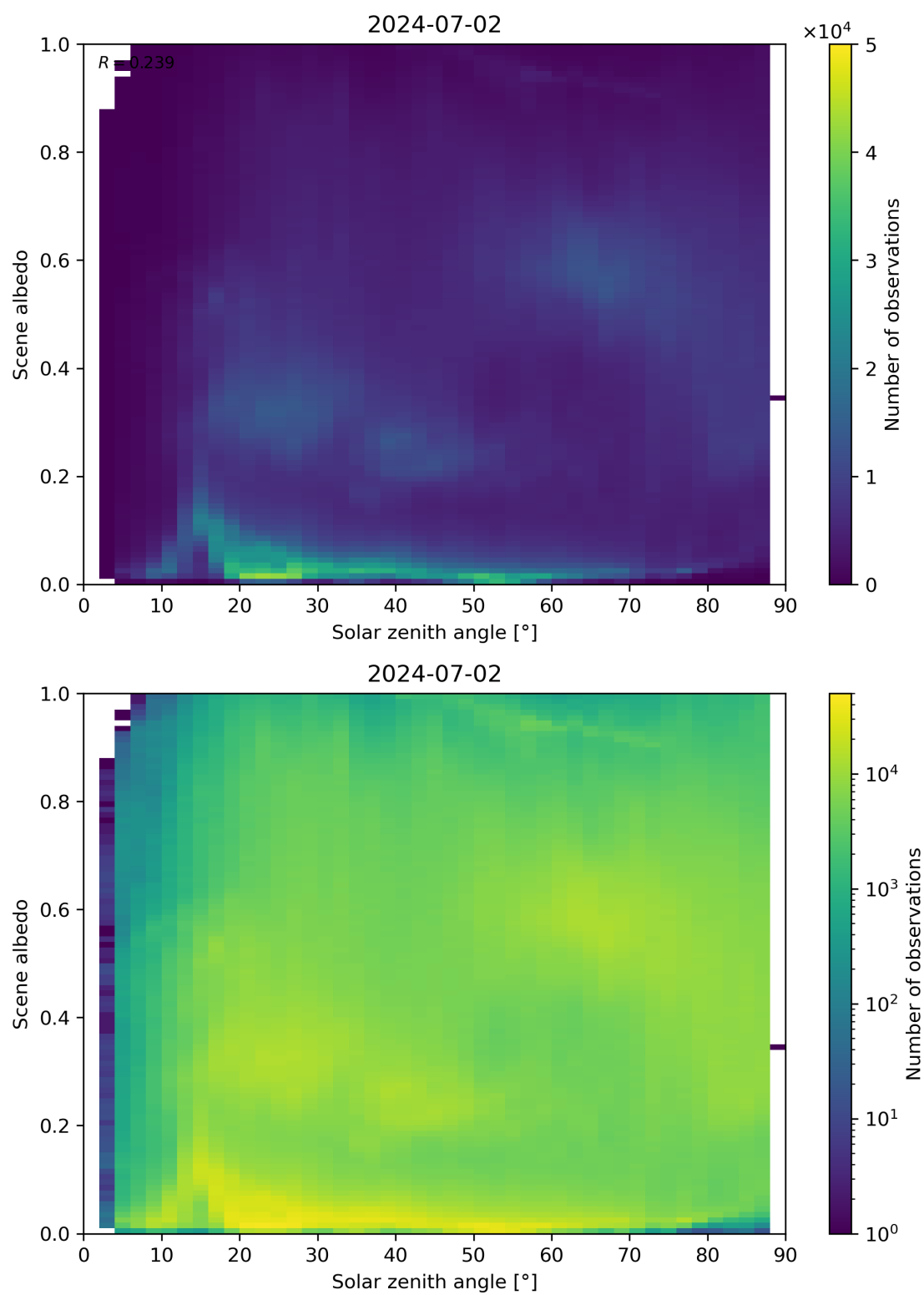
Figure 116: Scatter density plot of “Solar zenith angle” against “Scene albedo” for 2024-07-01 to 2024-07-03.
