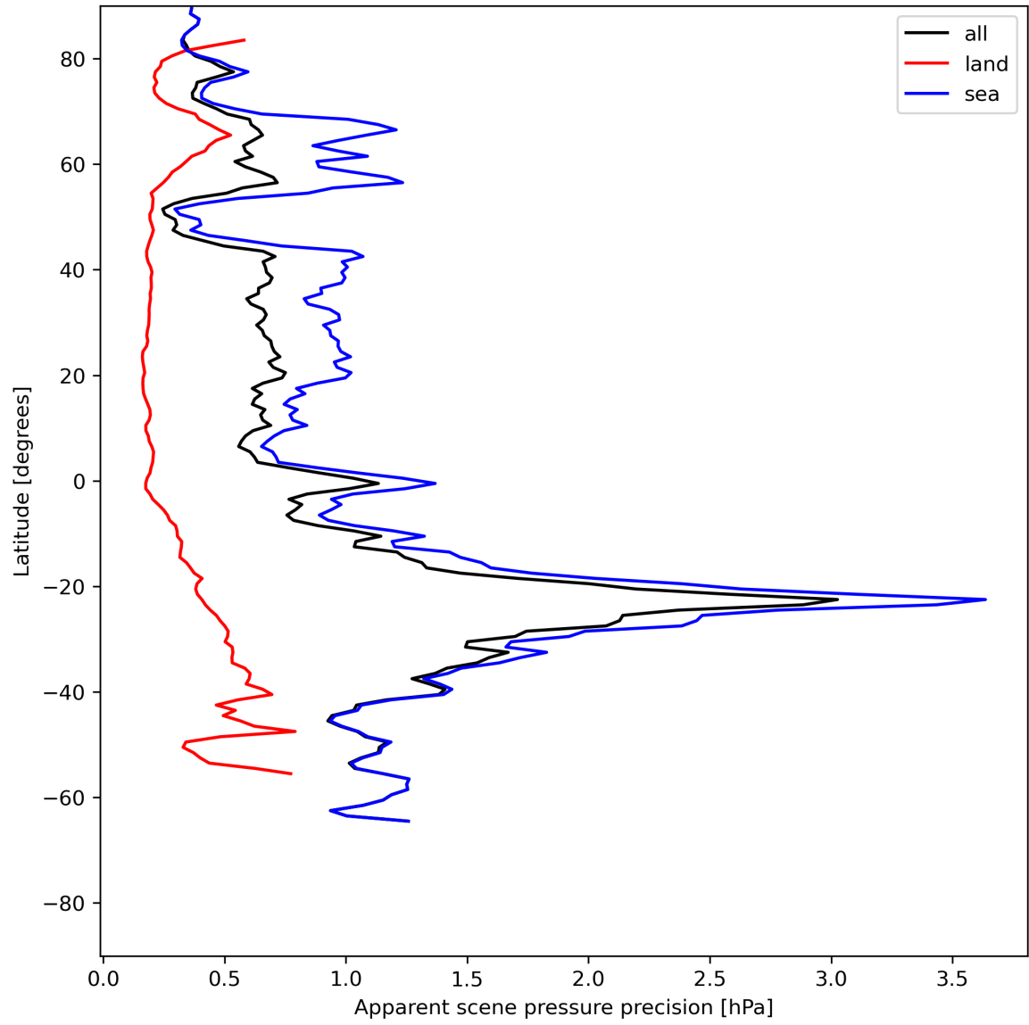
Figure 20: Zonal average of “Apparent scene pressure precision” for 2024-07-01 to 2024-07-03.
