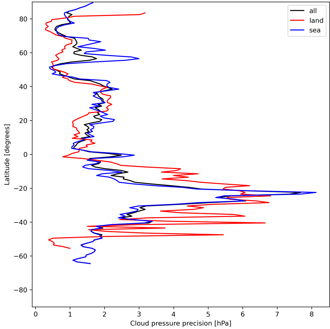
Figure 14: Zonal average of “Cloud pressure precision” for 2024-07-01 to 2024-07-03.
