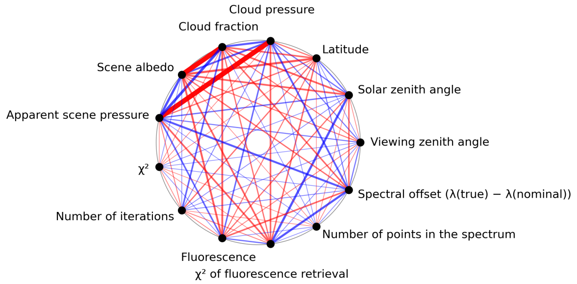
Figure 1: Map of correlation graph for 2024-07-01 to 2024-07-03.
