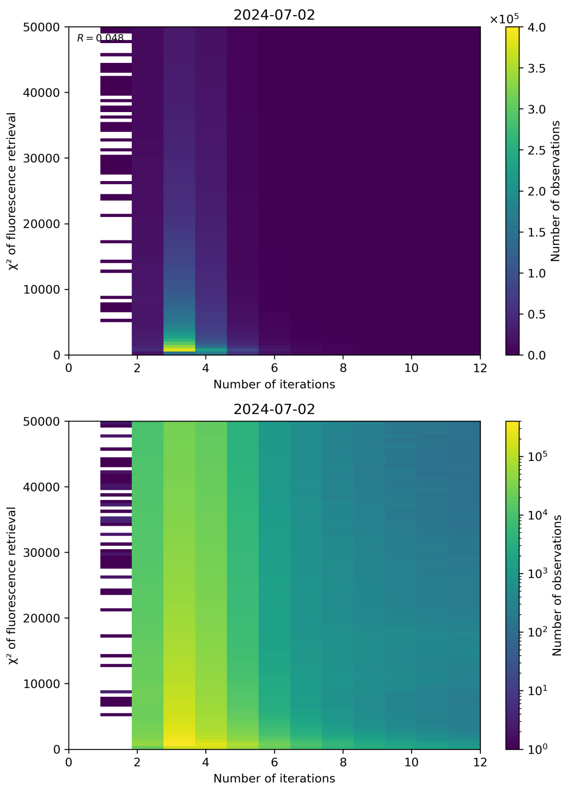
Figure 97: Scatter density plot of “Number of iterations” against “ \chi^2 of fluorescence retrieval” for 2024-07-01 to 2024-07-03.
