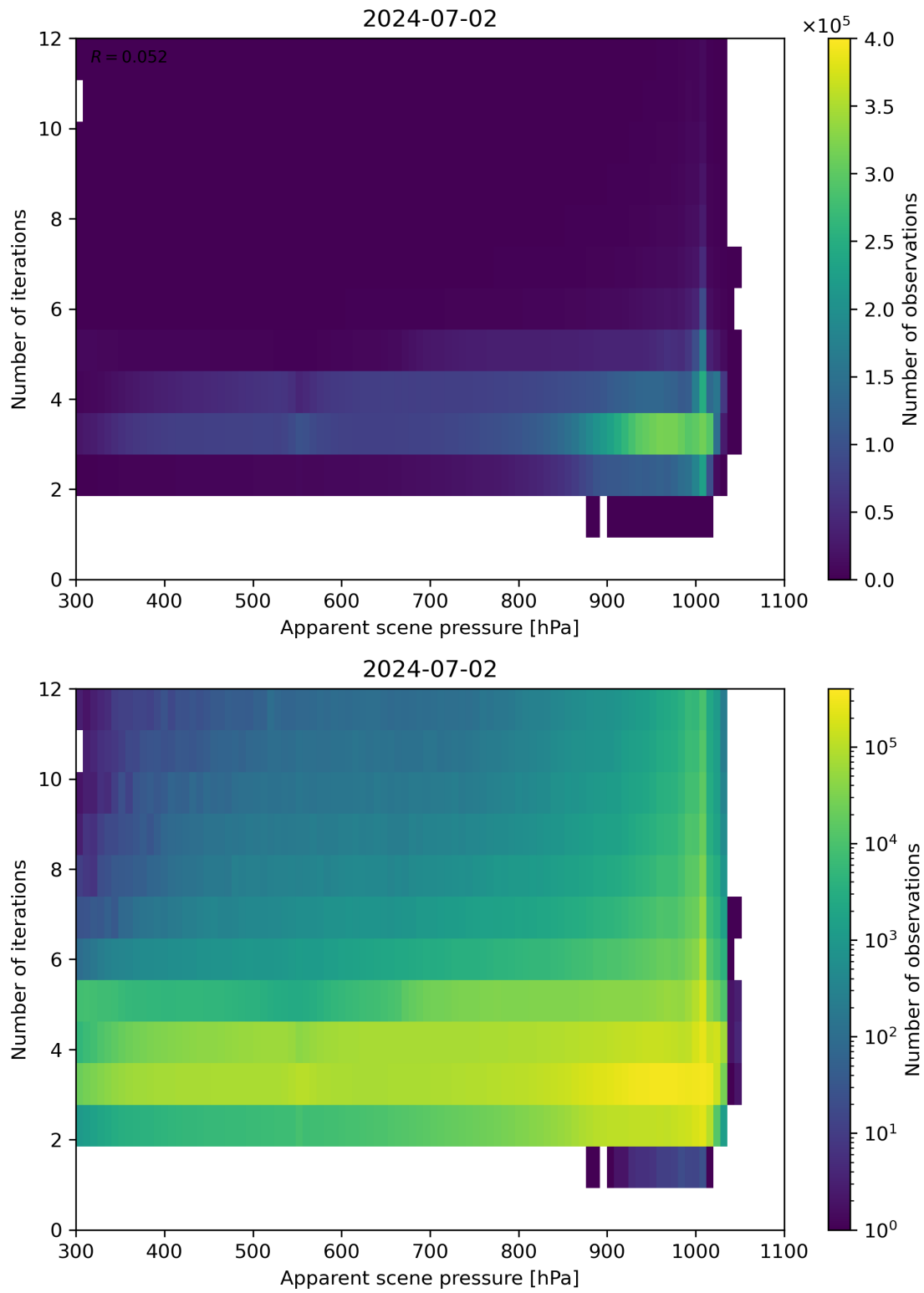
Figure 65: Scatter density plot of “Apparent scene pressure” against “Number of iterations” for 2024-07-01 to 2024-07-03.
