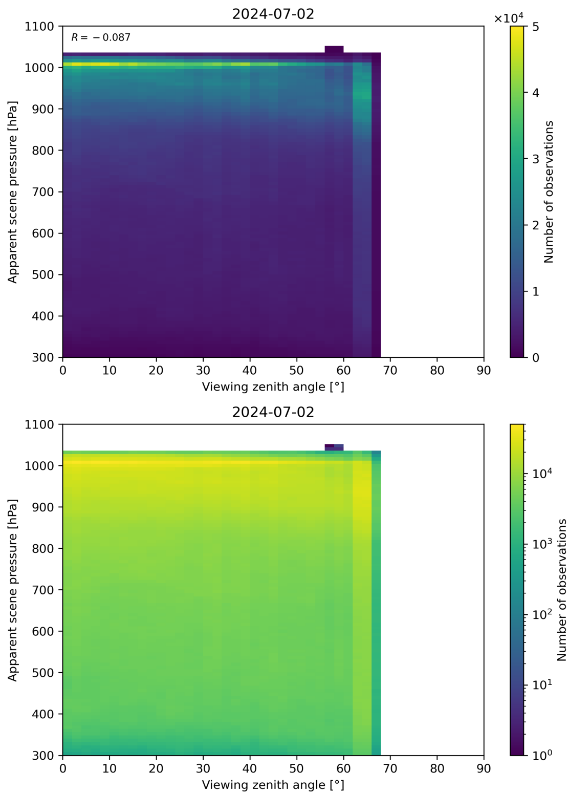
Figure 118: Scatter density plot of “Viewing zenith angle” against “Apparent scene pressure” for 2024-07-01 to 2024-07-03.
