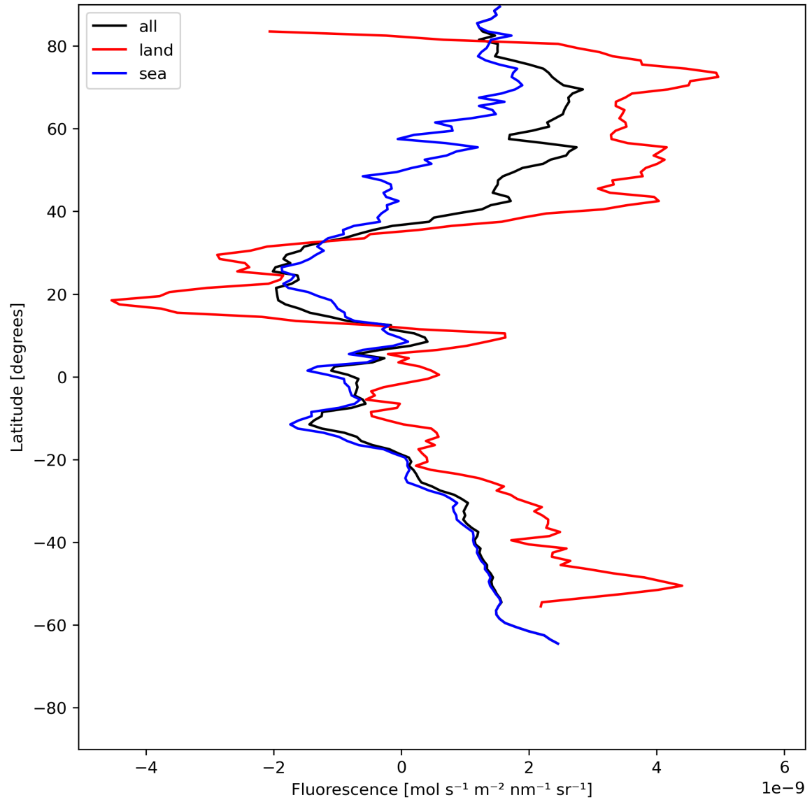
Figure 23: Zonal average of “Fluorescence” for 2024-07-01 to 2024-07-03.
