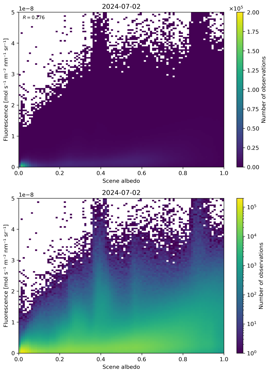
Figure 104: Scatter density plot of “Scene albedo” against “Fluorescence” for 2024-07-01 to 2024-07-03.
