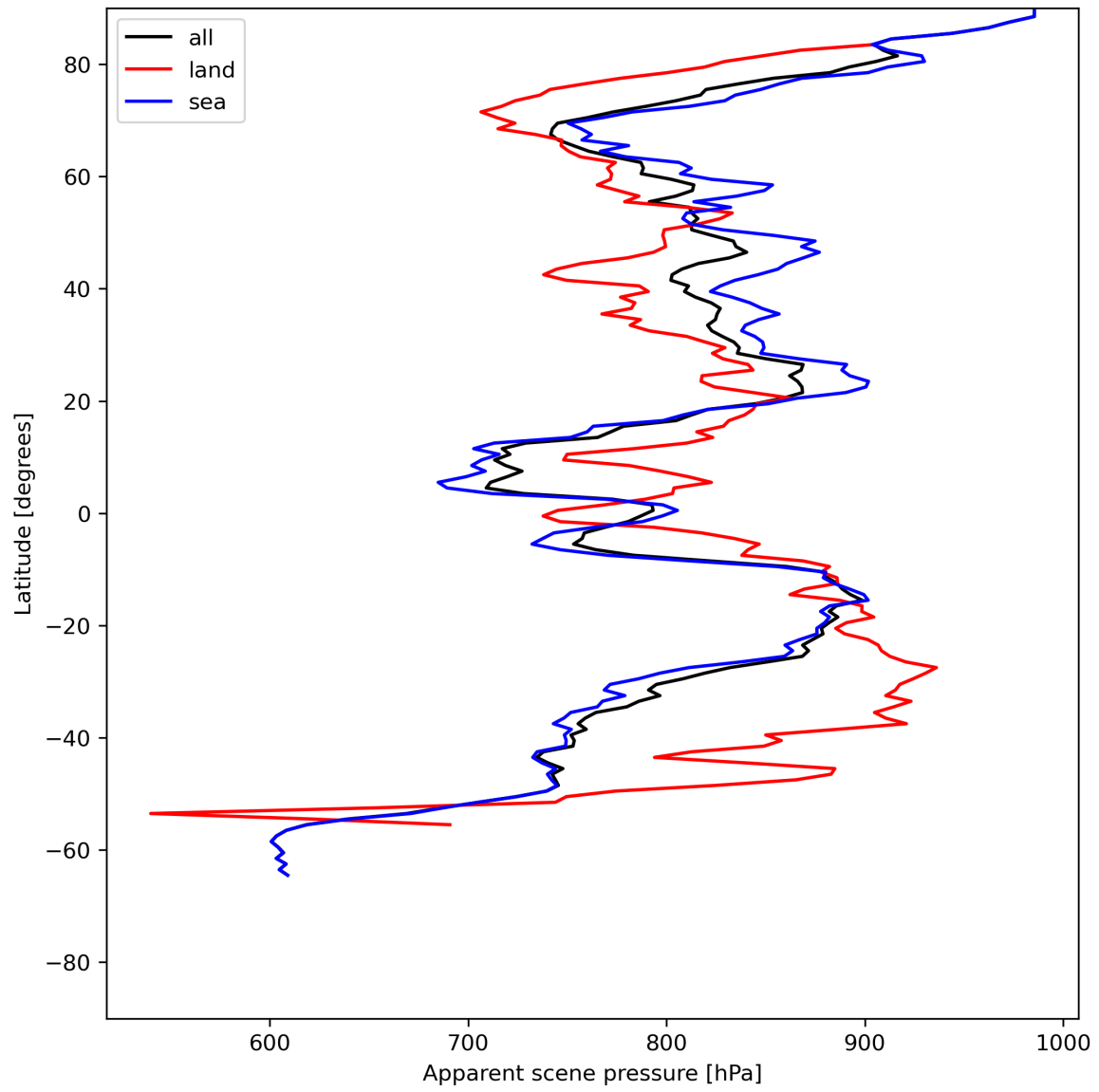
Figure 19: Zonal average of “Apparent scene pressure” for 2024-07-01 to 2024-07-03.
