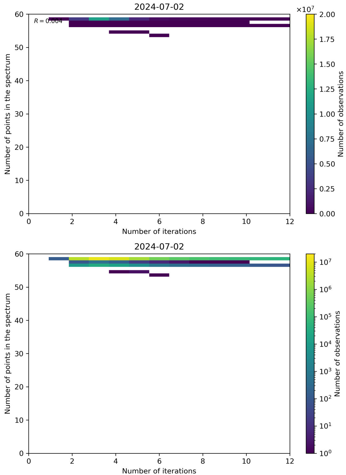
Figure 99: Scatter density plot of “Number of iterations” against “Number of points in the spectrum” for 2024-07-01 to 2024-07-03.
