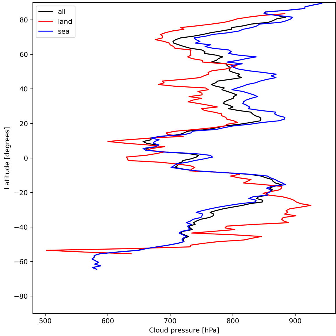
Figure 13: Zonal average of “Cloud pressure” for 2024-07-01 to 2024-07-03.
