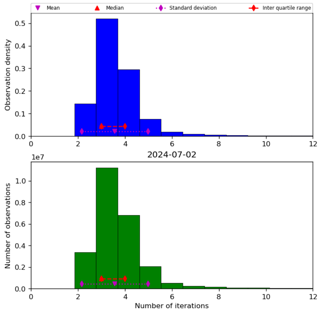
Figure 39: Histogram of “Number of iterations” for 2024-07-01 to 2024-07-03
