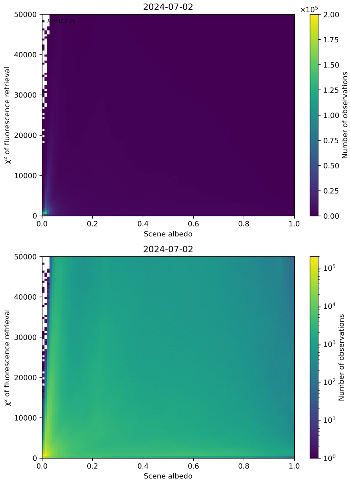
Figure 103: Scatter density plot of “Scene albedo” against “ \chi^2 of fluorescence retrieval” for 2024-07-01 to 2024-07-03.
