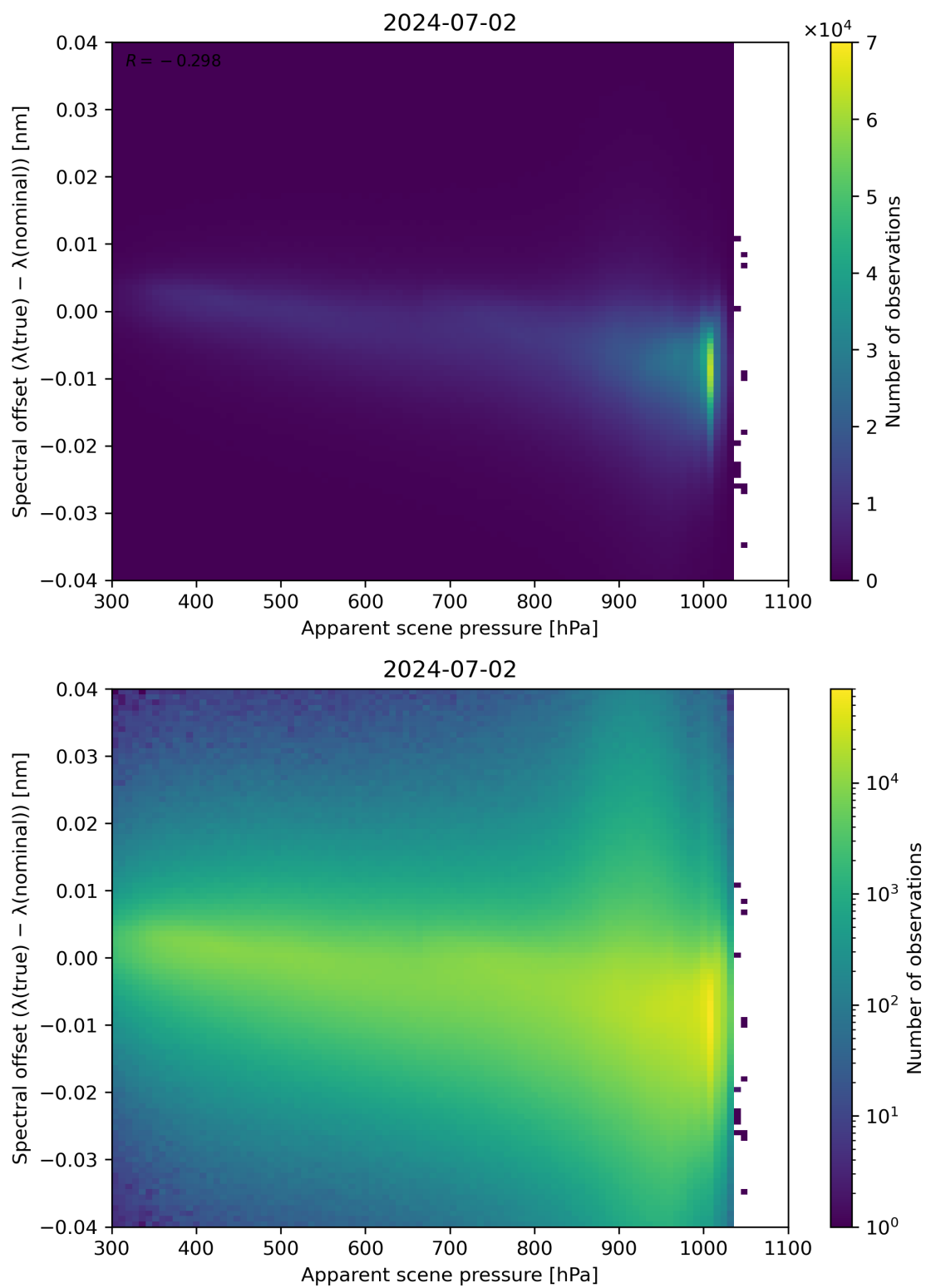
Figure 67: Scatter density plot of “Apparent scene pressure” against “Spectral offset ( \lambda(\text{true}) - \lambda(\text{nominal}) )” for 2024-07-01 to 2024-07-03.
