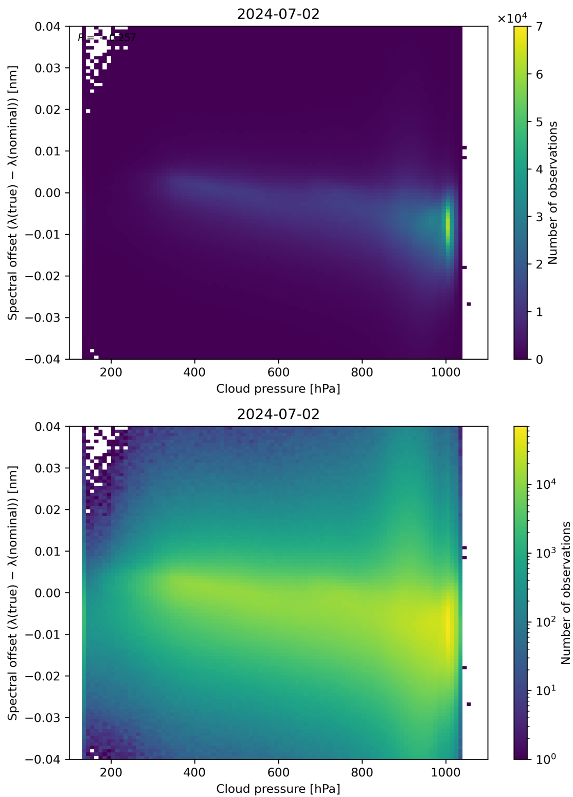
Figure 84: Scatter density plot of “Cloud pressure” against “Spectral offset ( \lambda(\text{true}) - \lambda(\text{nominal}) )” for 2024-07-01 to 2024-07-03.
