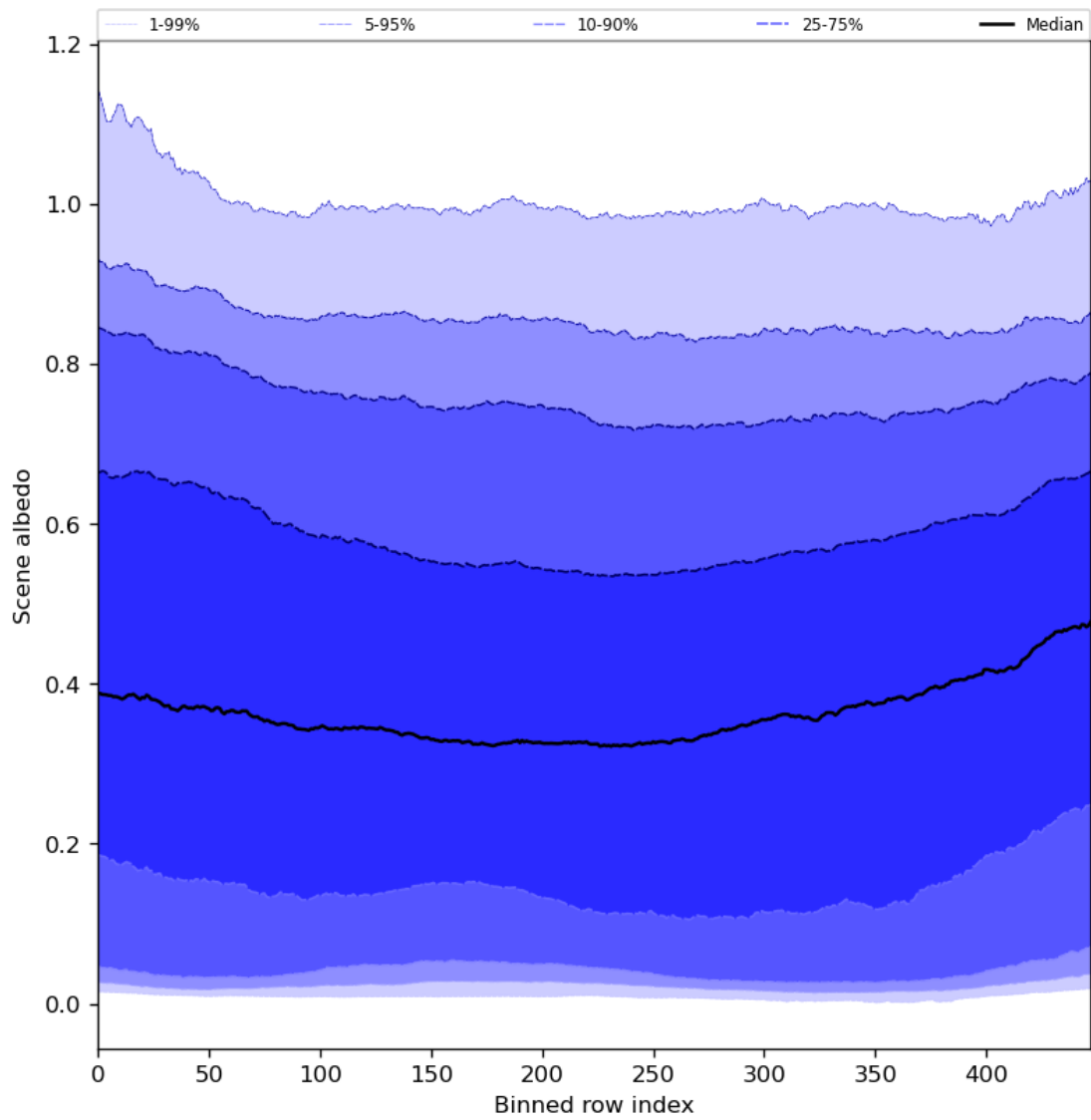
Figure 51: Along track statistics of “Scene albedo” for 2024-07-01 to 2024-07-03
