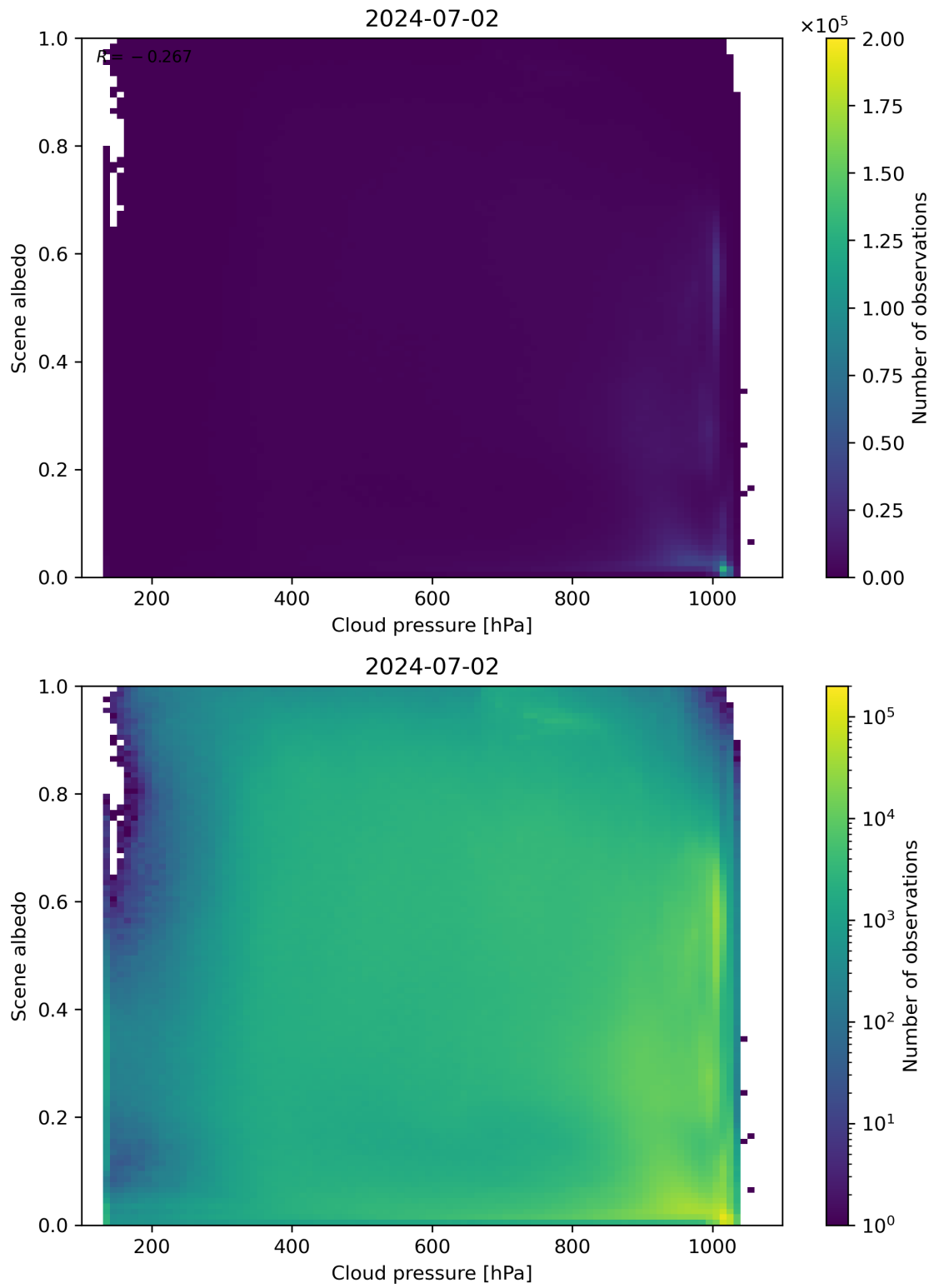
Figure 83: Scatter density plot of “Cloud pressure” against “Scene albedo” for 2024-07-01 to 2024-07-03.
