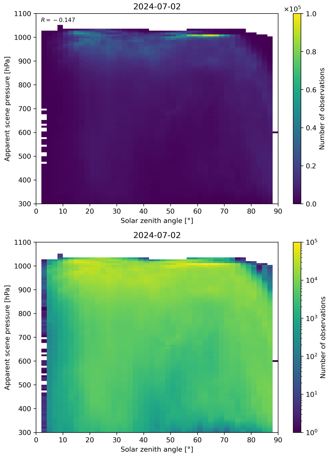
Figure 108: Scatter density plot of “Solar zenith angle” against “Apparent scene pressure” for 2024-07-01 to 2024-07-03.
