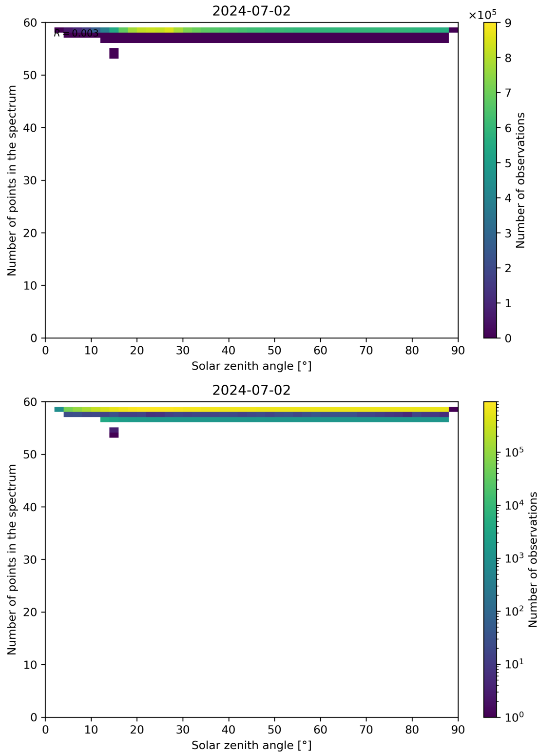
Figure 115: Scatter density plot of “Solar zenith angle” against “Number of points in the spectrum” for 2024-07-01 to 2024-07-03.
