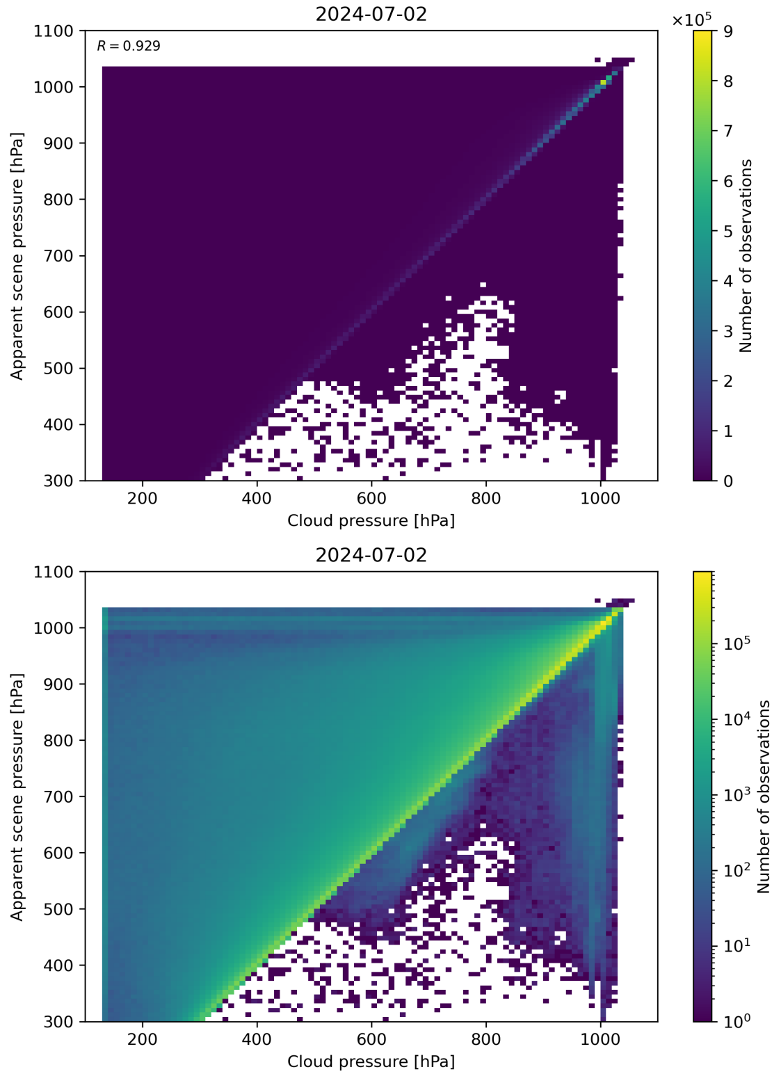
Figure 77: Scatter density plot of “Cloud pressure” against “Apparent scene pressure” for 2024-07-01 to 2024-07-03.
