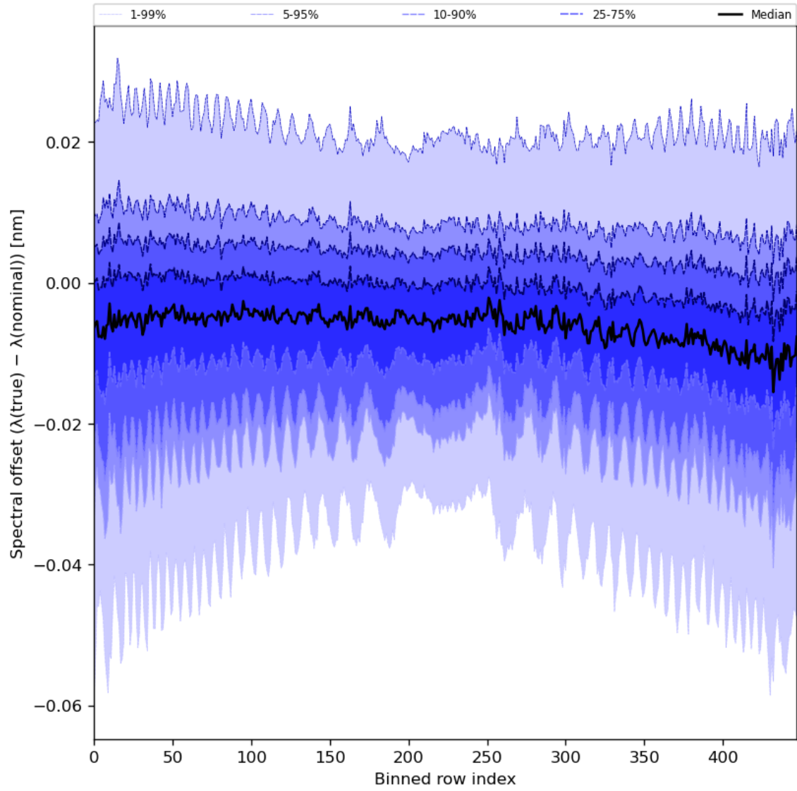
Figure 62: Along track statistics of “Spectral offset ( \lambda(\text{true}) - \lambda(\text{nominal}) )” for 2024-07-01 to 2024-07-03
