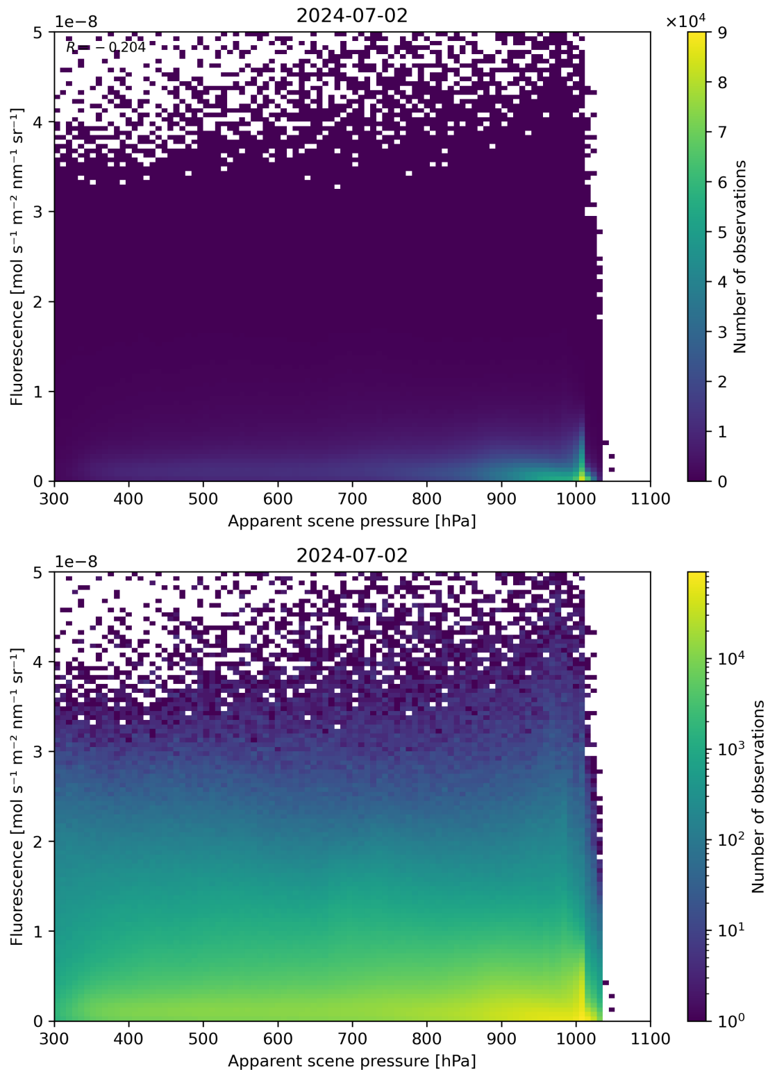
Figure 64: Scatter density plot of “Apparent scene pressure” against “Fluorescence” for 2024-07-01 to 2024-07-03.
