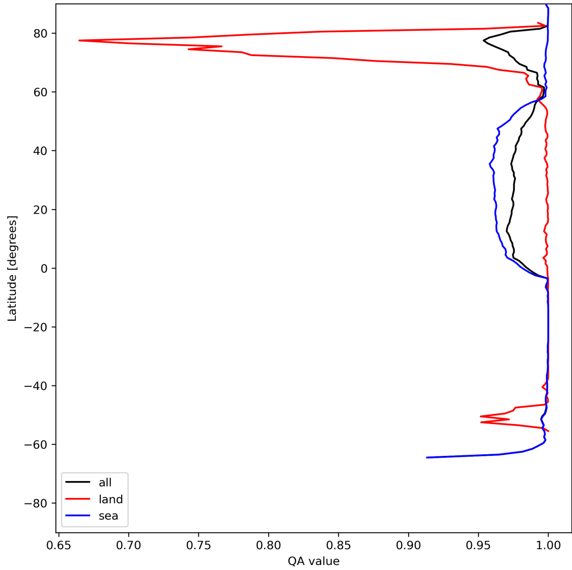
Figure 12: Zonal average of “QA value” for 2024-07-01 to 2024-07-03.
