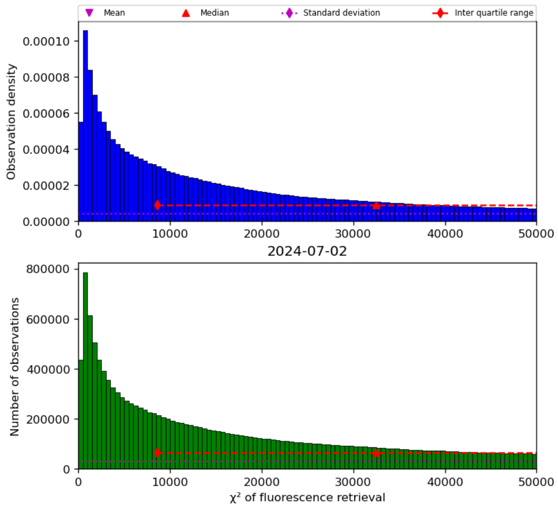
Figure 42: Histogram of “ \chi^2 of fluorescence retrieval” for 2024-07-01 to 2024-07-03
