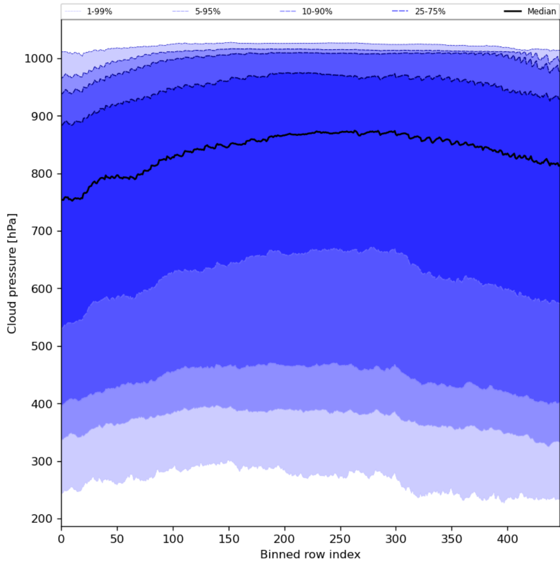
Figure 47: Along track statistics of “Cloud pressure” for 2024-07-02 to 2024-07-04
