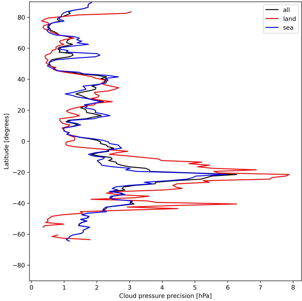
Figure 14: Zonal average of “Cloud pressure precision” for 2024-07-02 to 2024-07-04.
