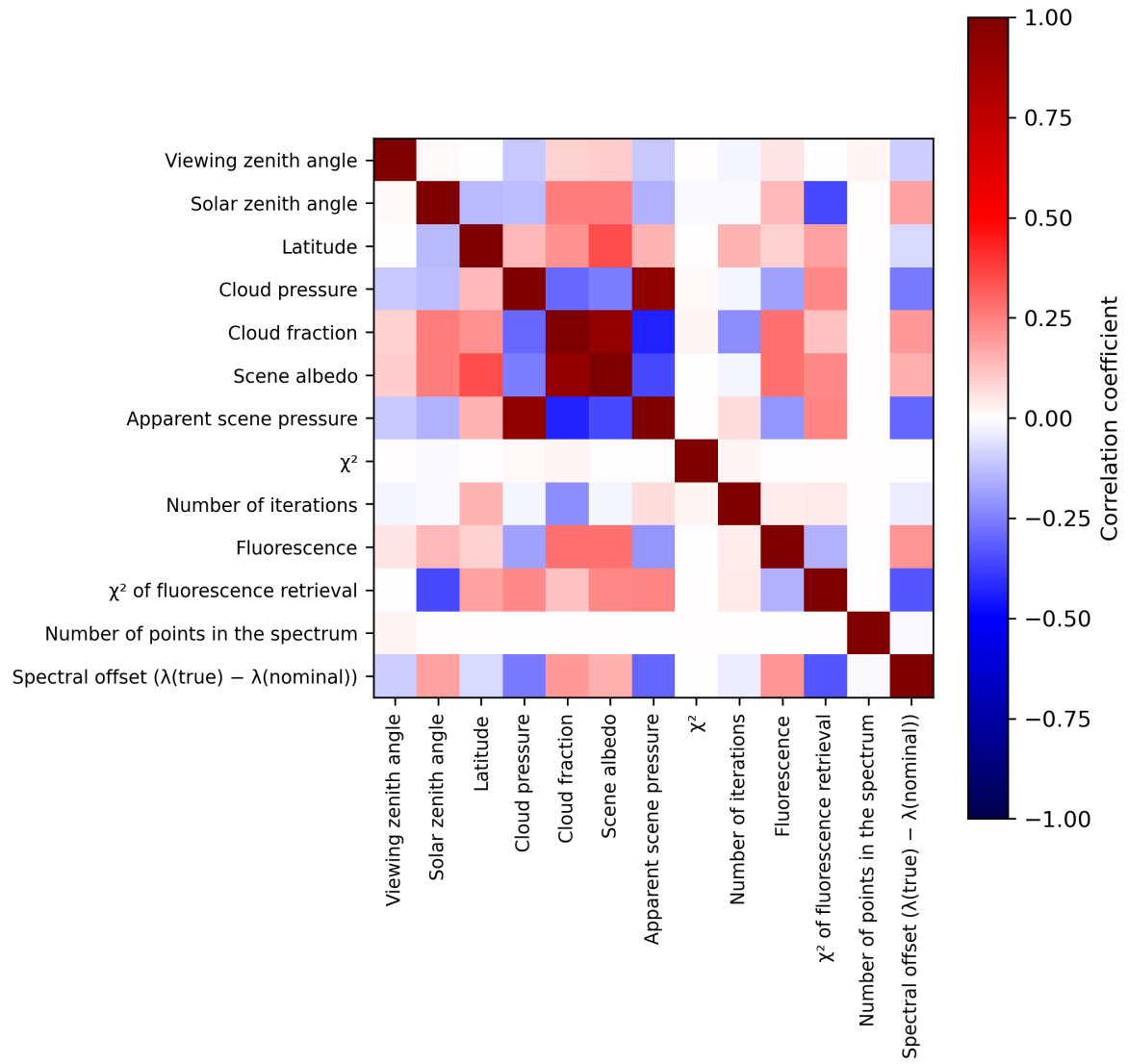
Figure 2: Map of correlation matrix for 2024-07-02 to 2024-07-04.
