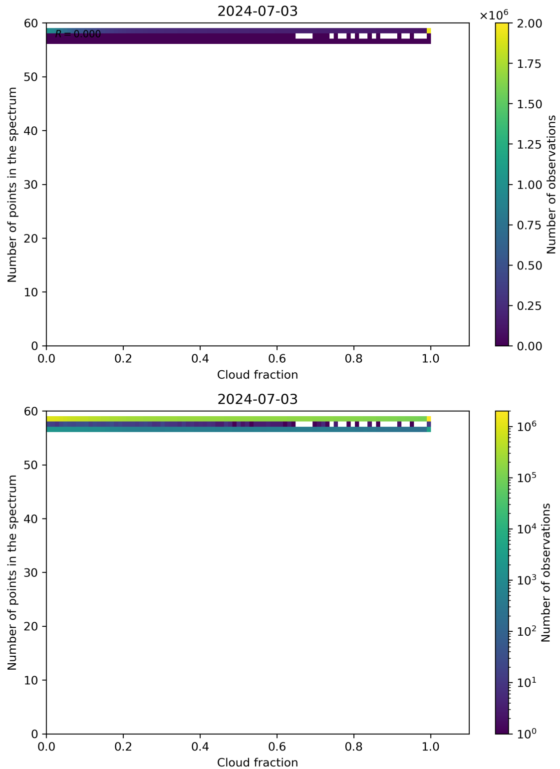
Figure 74: Scatter density plot of “Cloud fraction” against “Number of points in the spectrum” for 2024-07-02 to 2024-07-04.
