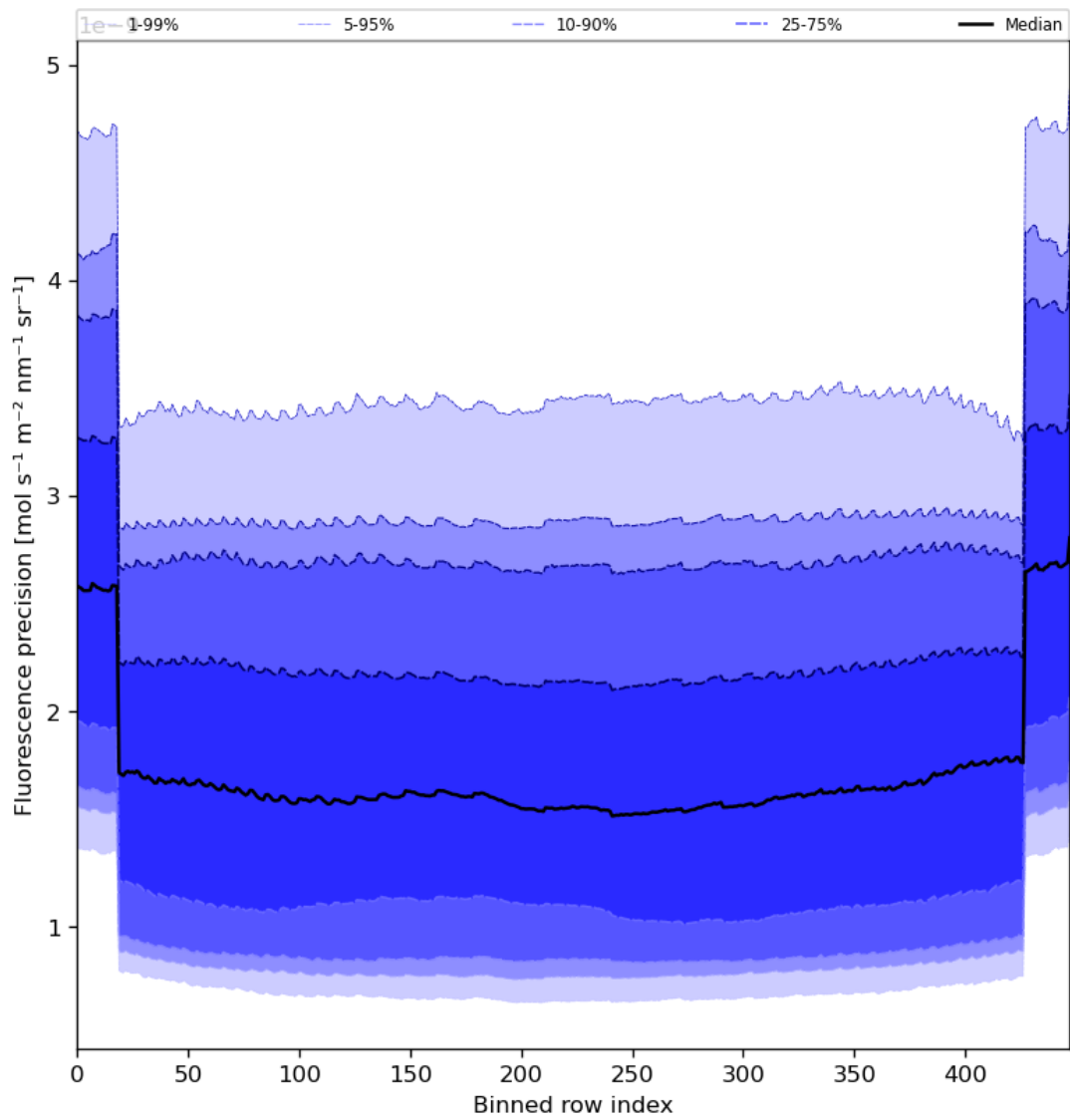
Figure 58: Along track statistics of “Fluorescence precision” for 2024-07-02 to 2024-07-04
