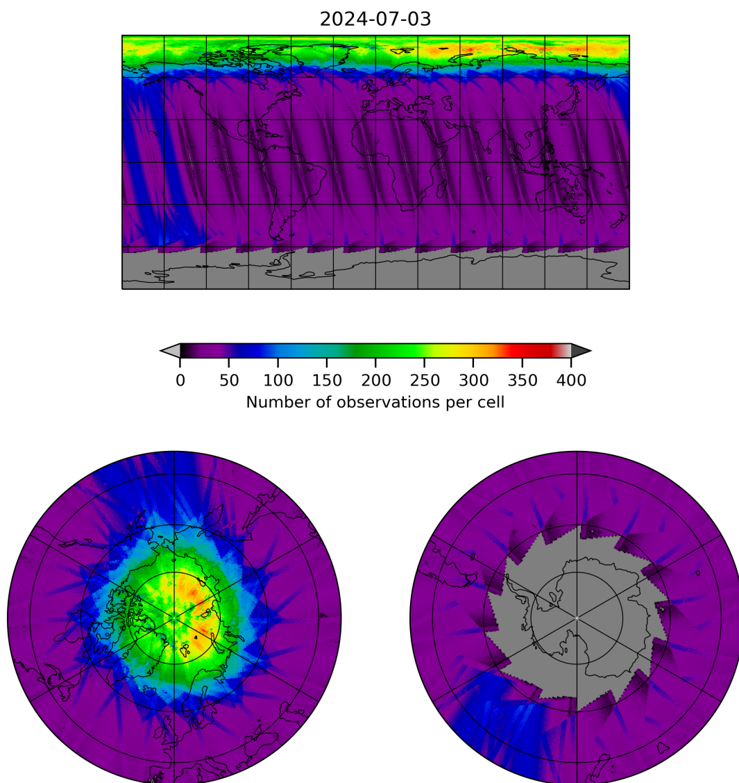
Figure 11: Map of the number of observations for 2024-07-02 to 2024-07-04
