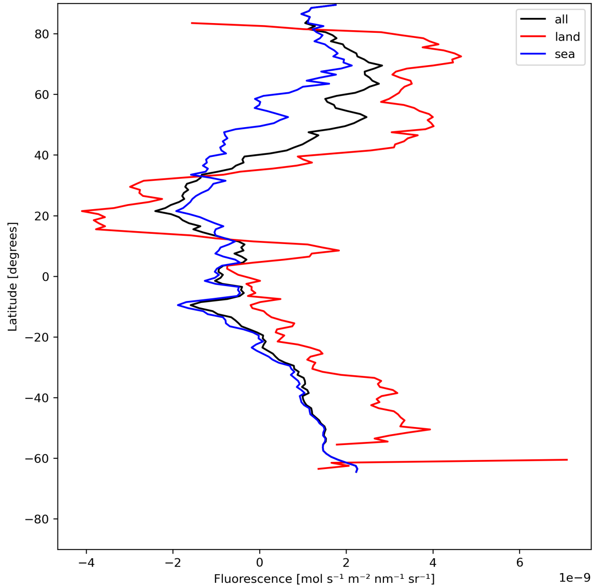
Figure 23: Zonal average of “Fluorescence” for 2024-07-02 to 2024-07-04.
