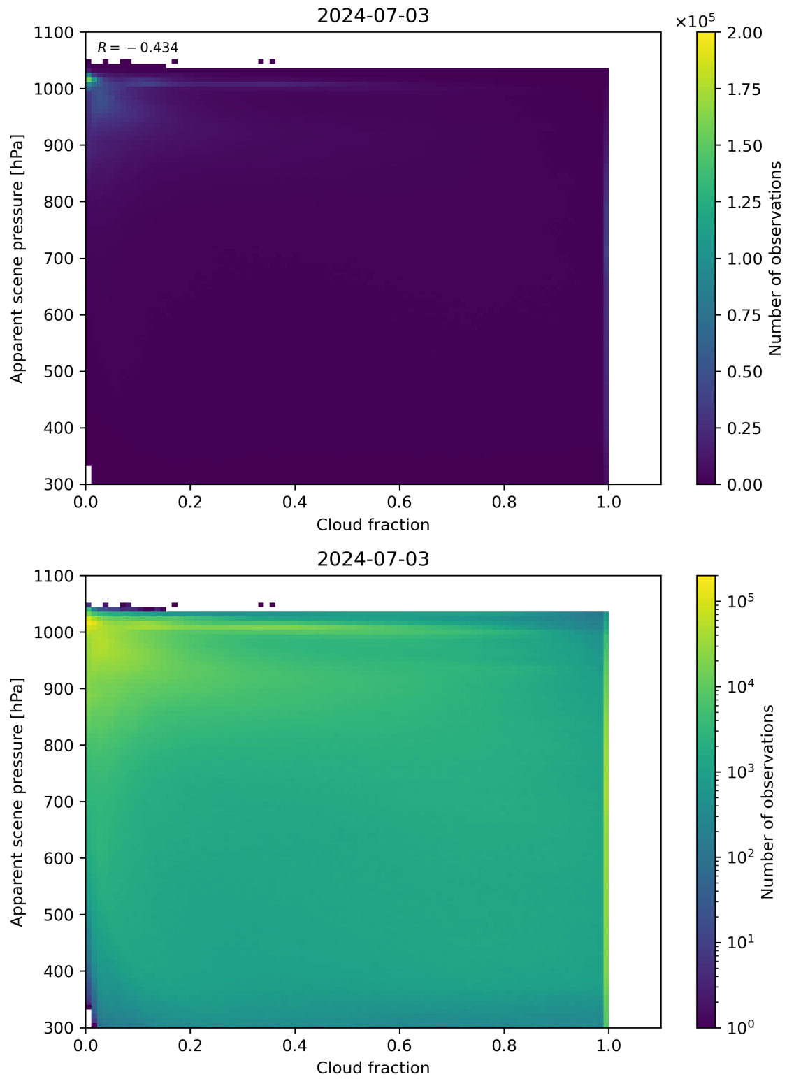
Figure 70: Scatter density plot of “Cloud fraction” against “Apparent scene pressure” for 2024-07-02 to 2024-07-04.
