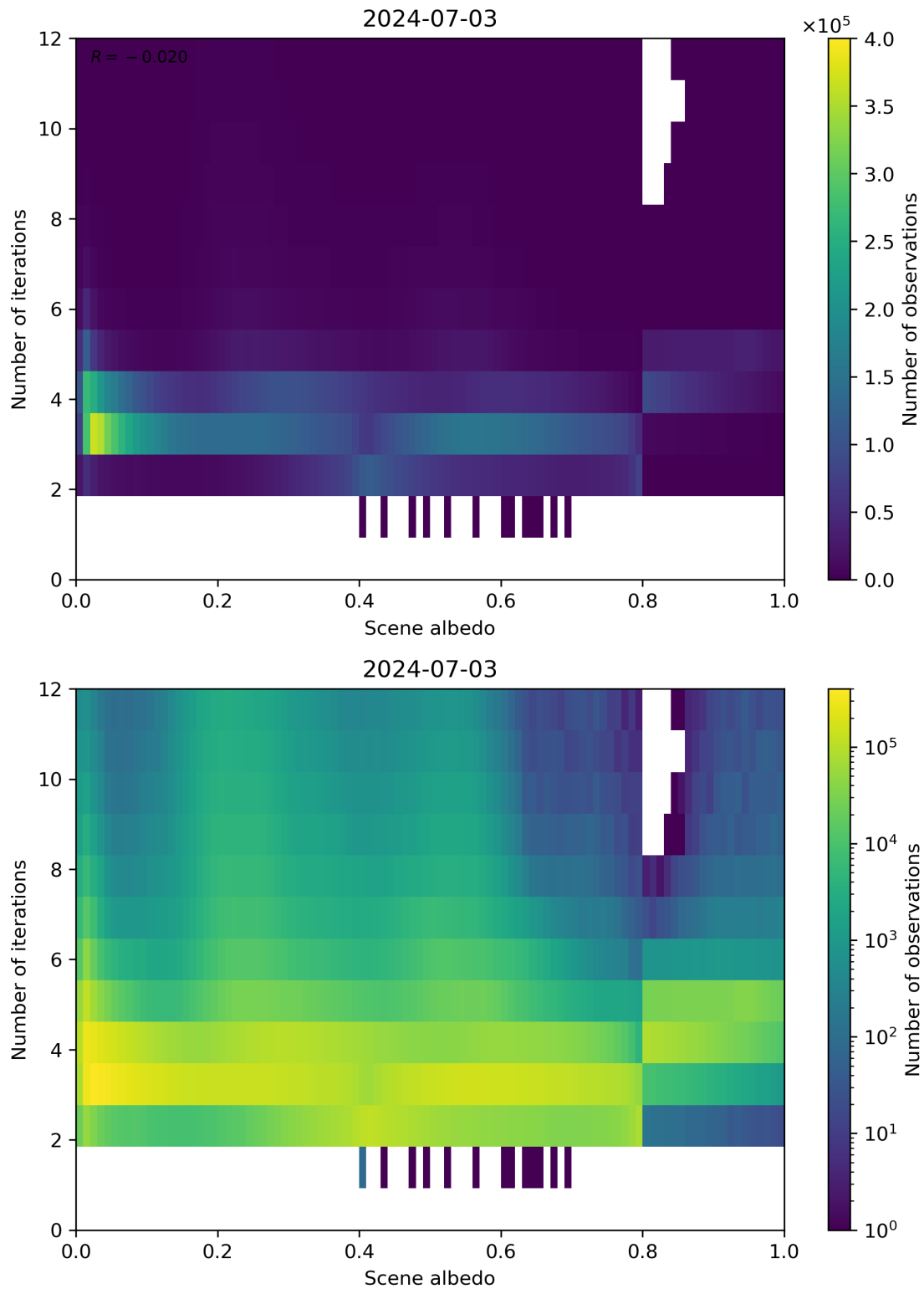
Figure 105: Scatter density plot of “Scene albedo” against “Number of iterations” for 2024-07-02 to 2024-07-04.
