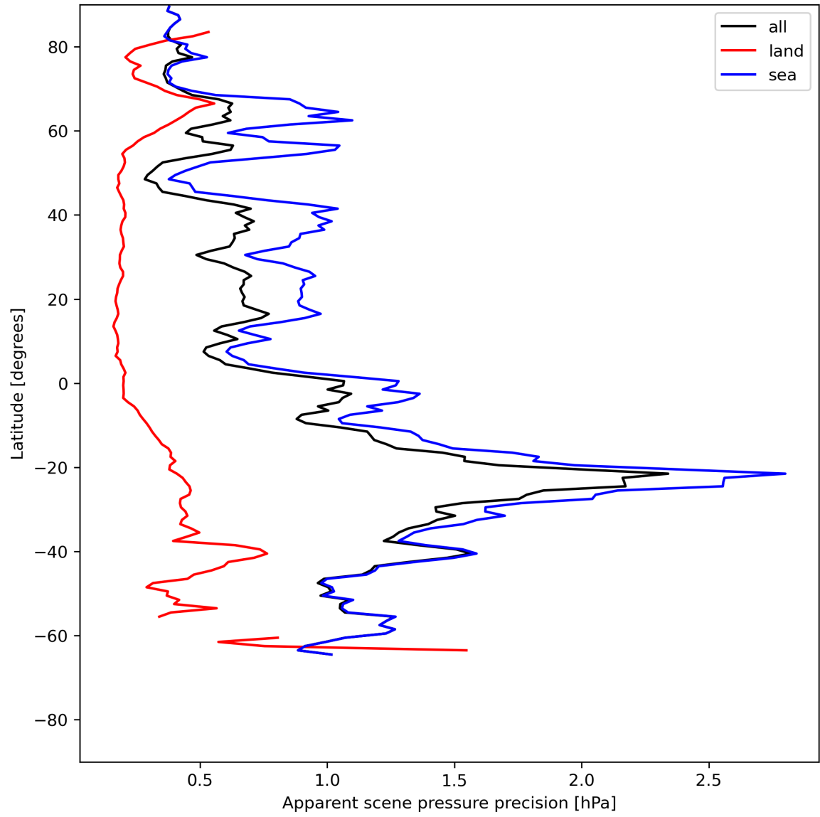
Figure 20: Zonal average of “Apparent scene pressure precision” for 2024-07-02 to 2024-07-04.
