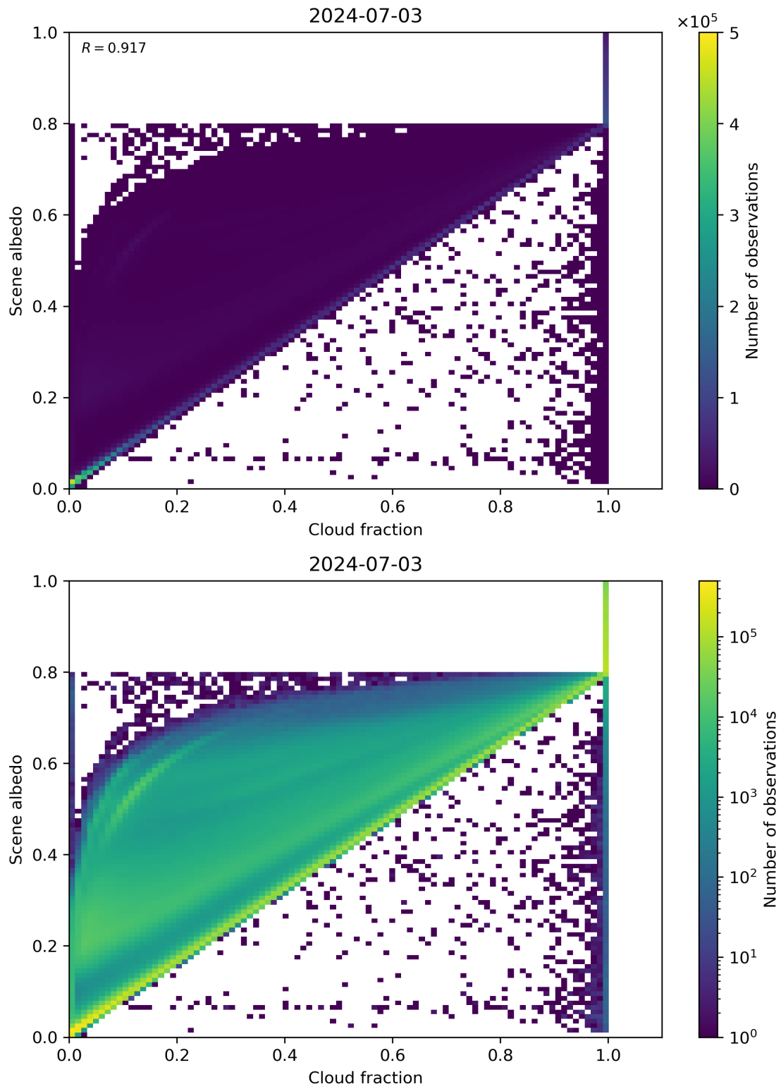
Figure 75: Scatter density plot of “Cloud fraction” against “Scene albedo” for 2024-07-02 to 2024-07-04.
