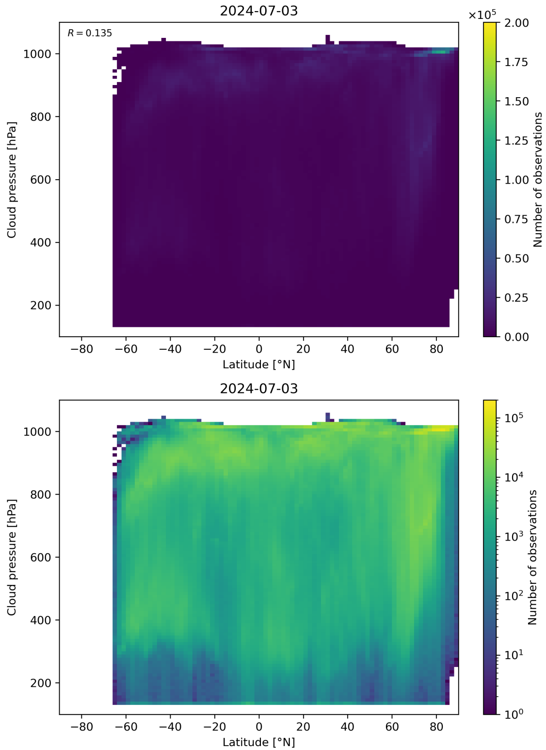
Figure 91: Scatter density plot of “Latitude” against “Cloud pressure” for 2024-07-02 to 2024-07-04.
