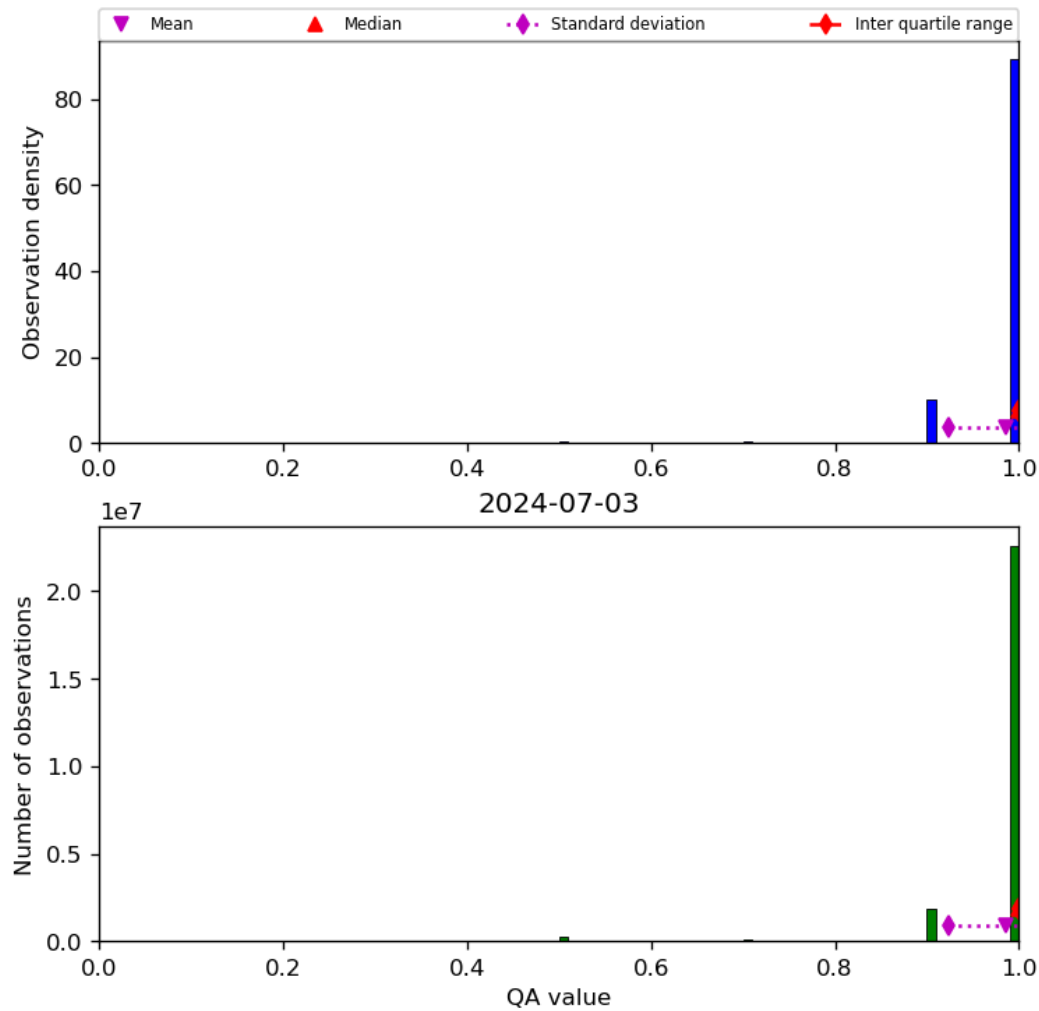
Figure 29: Histogram of “QA value” for 2024-07-02 to 2024-07-04
