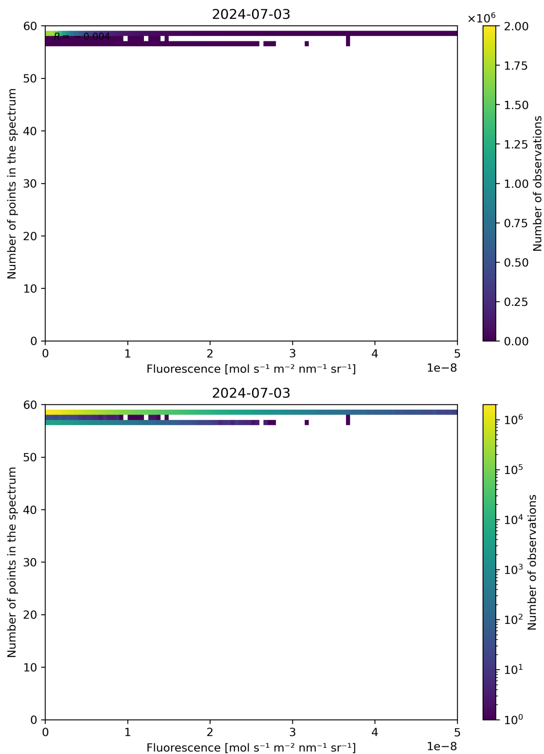
Figure 86: Scatter density plot of “Fluorescence” against “Number of points in the spectrum” for 2024-07-02 to 2024-07-04.
