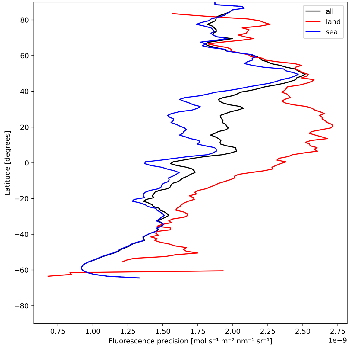
Figure 24: Zonal average of “Fluorescence precision” for 2024-07-02 to 2024-07-04.
