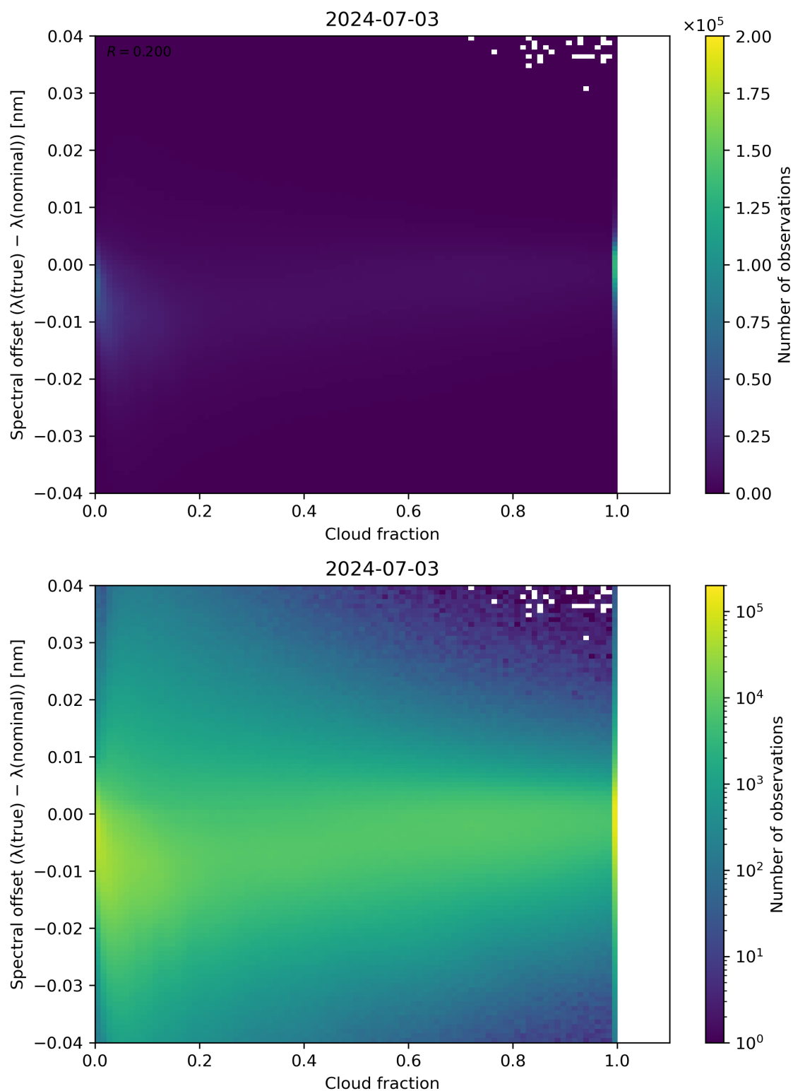
Figure 76: Scatter density plot of “Cloud fraction” against “Spectral offset ( \lambda(\text{true}) - \lambda(\text{nominal}) )” for 2024-07-02 to 2024-07-04.
