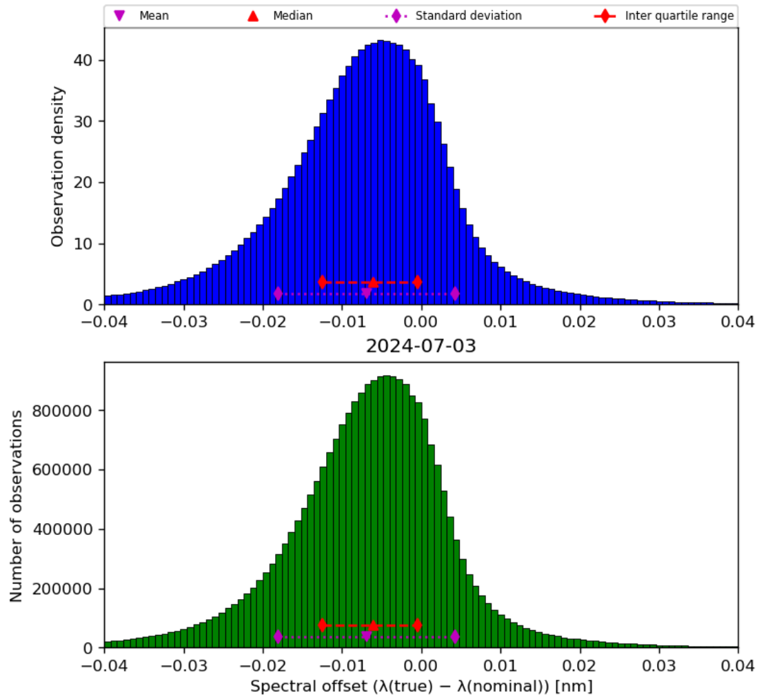
Figure 45: Histogram of “Spectral offset ( \lambda(\text{true}) - \lambda(\text{nominal}) )” for 2024-07-02 to 2024-07-04
