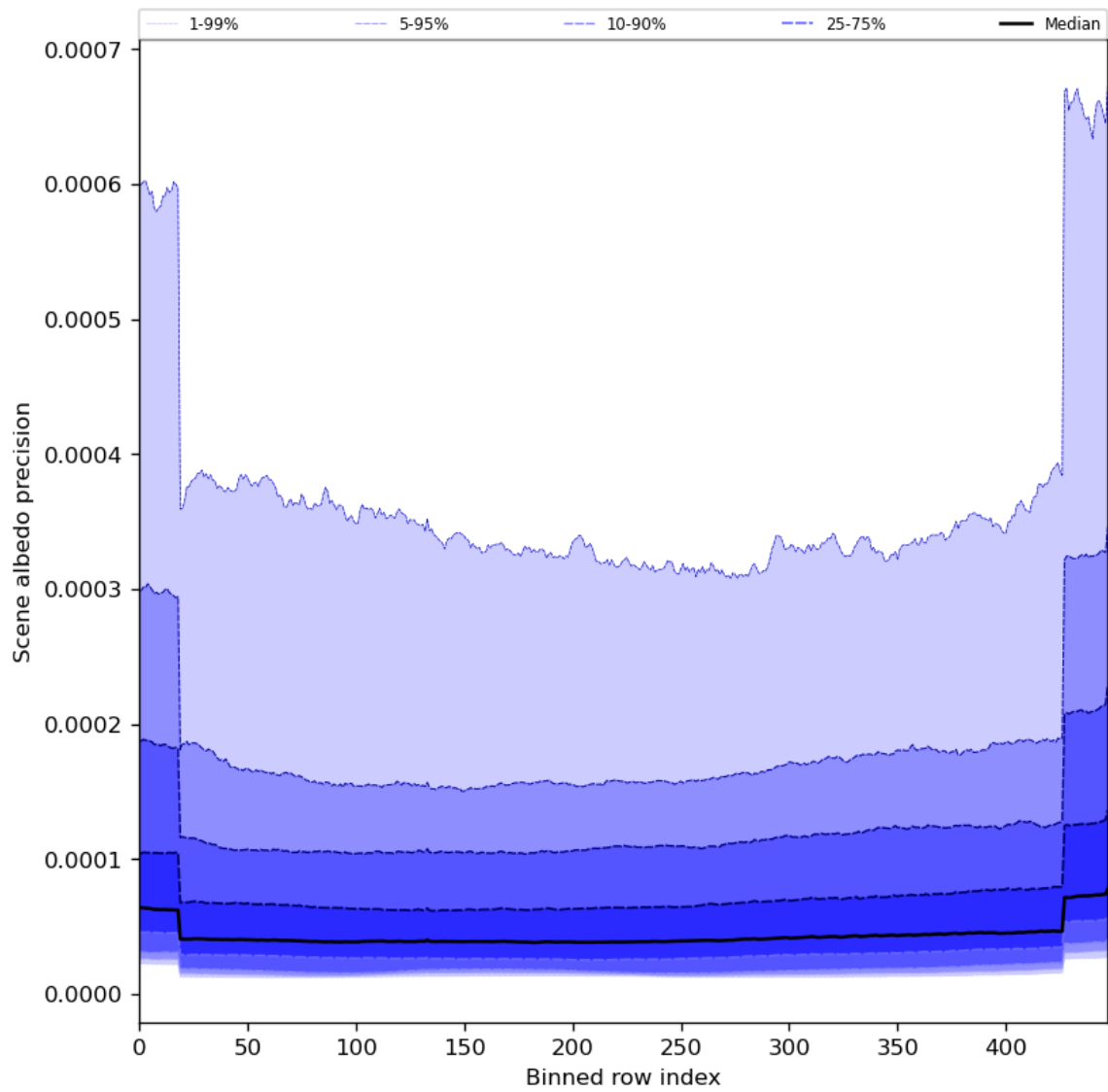
Figure 52: Along track statistics of “Scene albedo precision” for 2024-07-02 to 2024-07-04
