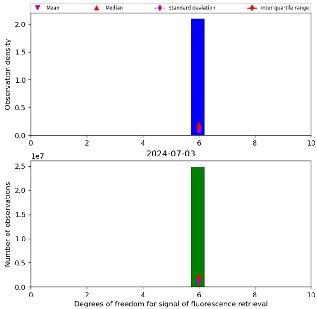
Figure 43: Histogram of “Degrees of freedom for signal of fluorescence retrieval” for 2024-07-02 to 2024-07-04
