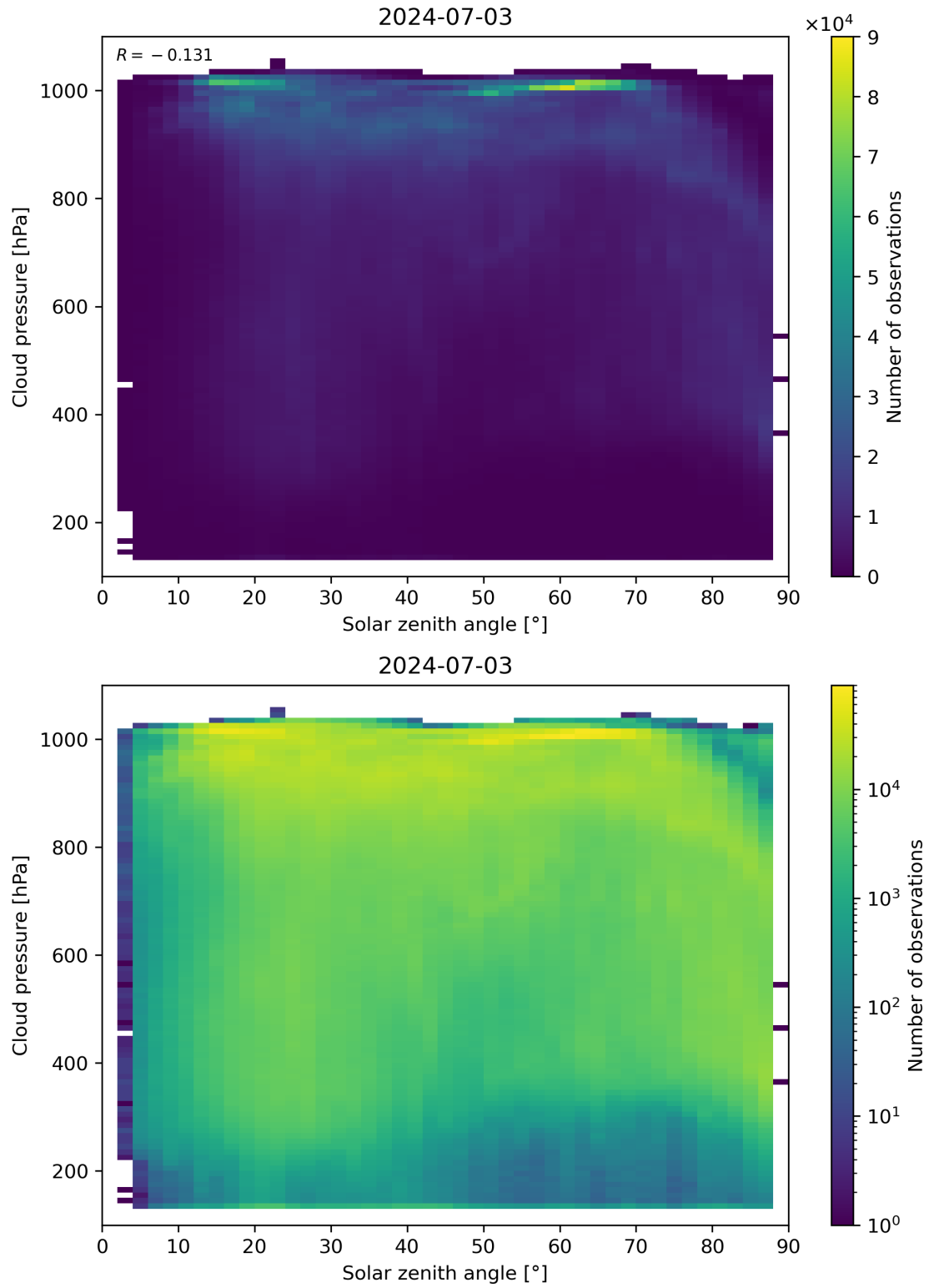
Figure 111: Scatter density plot of “Solar zenith angle” against “Cloud pressure” for 2024-07-02 to 2024-07-04.
