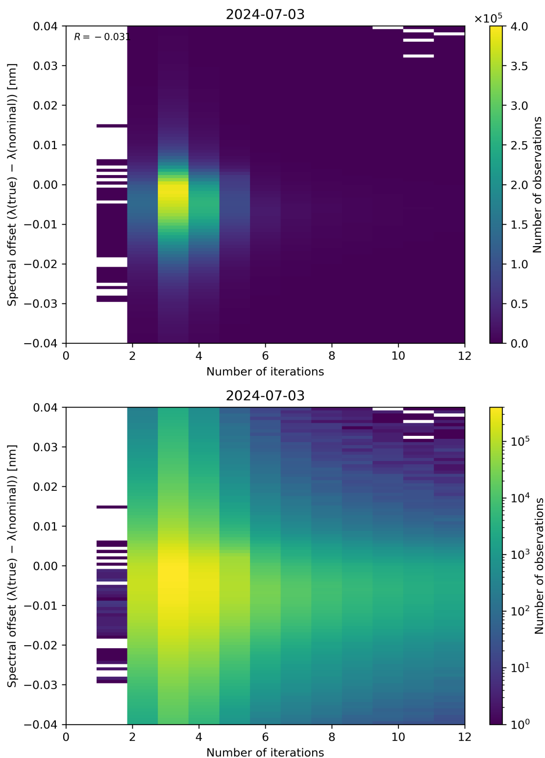
Figure 100: Scatter density plot of “Number of iterations” against “Spectral offset ( \lambda(\text{true}) - \lambda(\text{nominal}) )” for 2024-07-02 to 2024-07-04.
