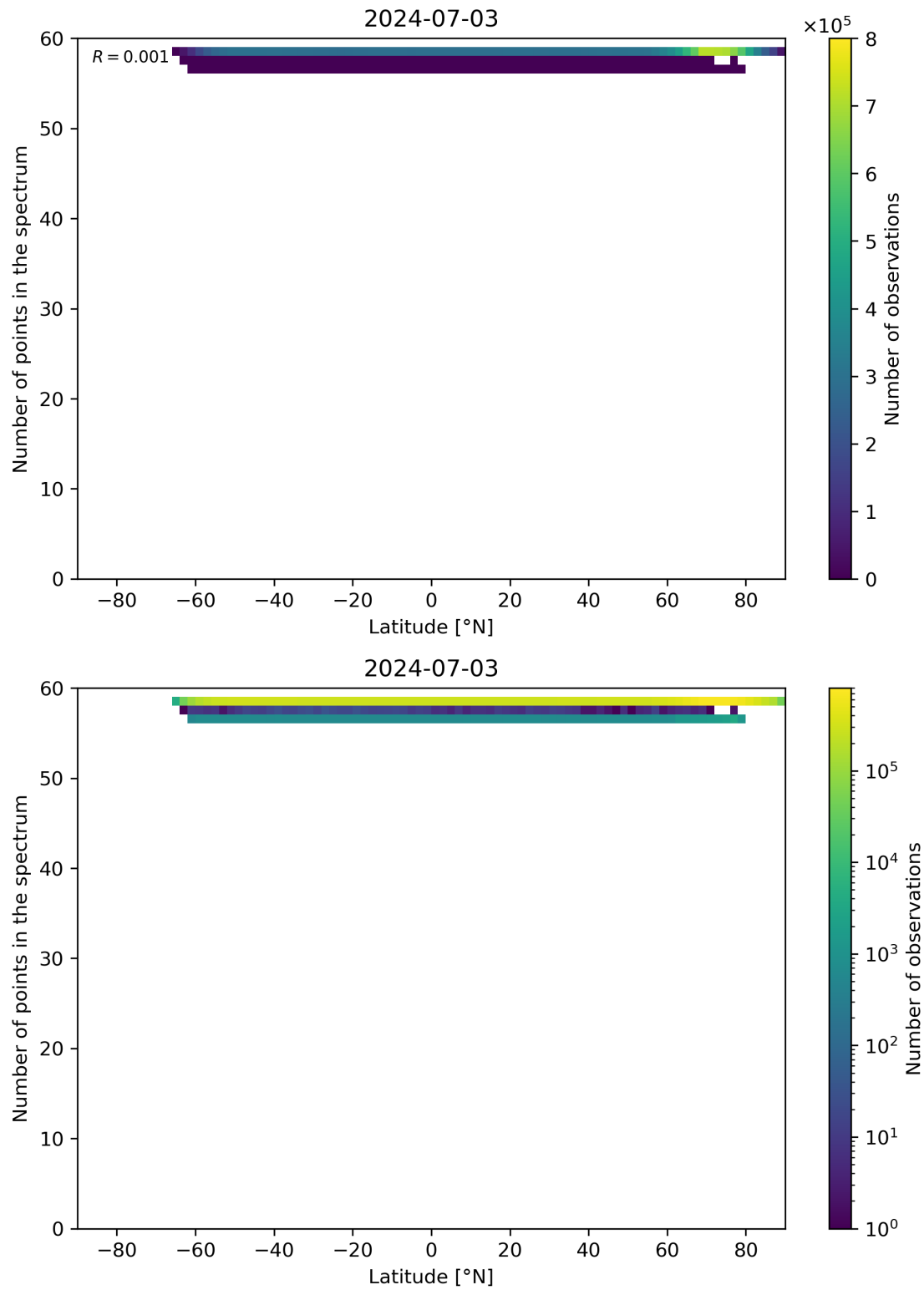
Figure 94: Scatter density plot of “Latitude” against “Number of points in the spectrum” for 2024-07-02 to 2024-07-04.
