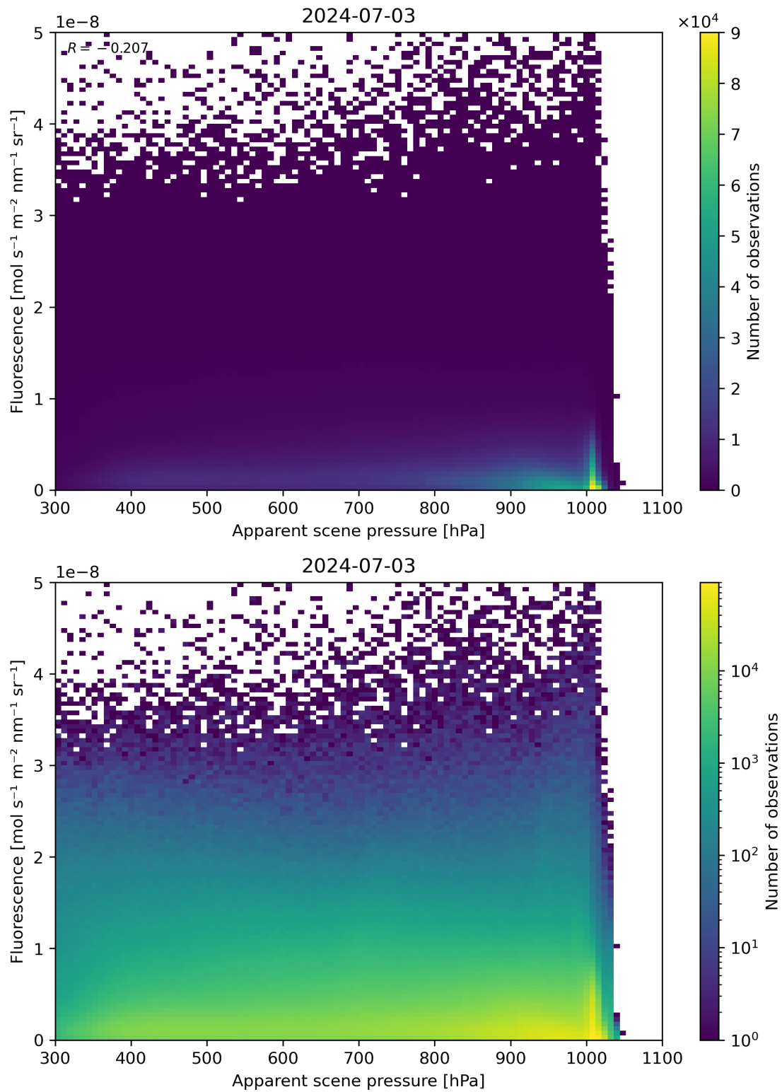
Figure 64: Scatter density plot of “Apparent scene pressure” against “Fluorescence” for 2024-07-02 to 2024-07-04.
