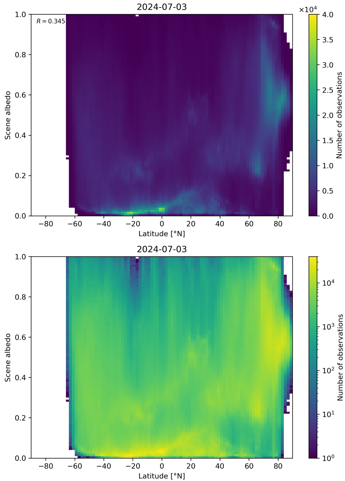
Figure 95: Scatter density plot of “Latitude” against “Scene albedo” for 2024-07-02 to 2024-07-04.
