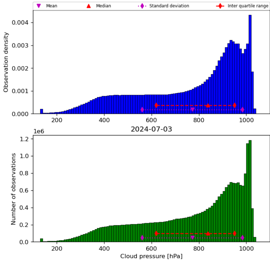
Figure 30: Histogram of “Cloud pressure” for 2024-07-02 to 2024-07-04
