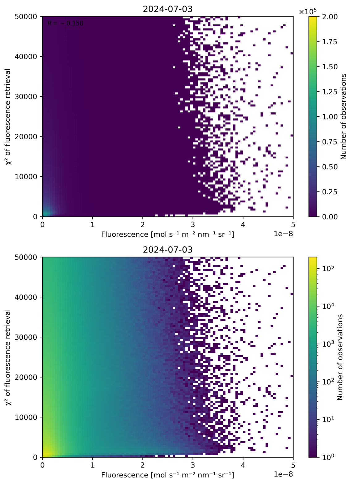
Figure 85: Scatter density plot of “Fluorescence” against “ \chi^2 of fluorescence retrieval” for 2024-07-02 to 2024-07-04.
