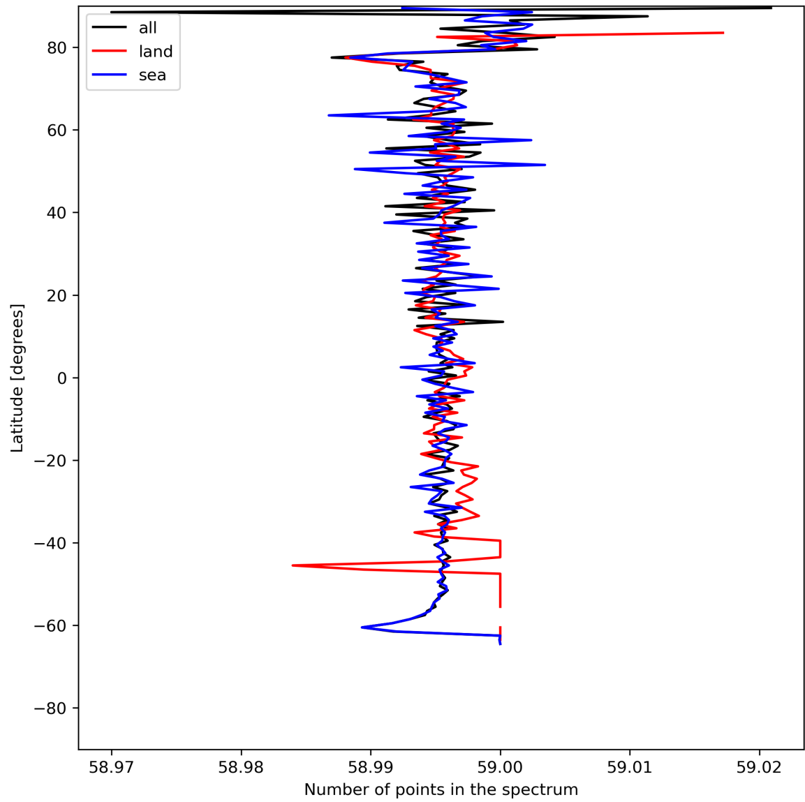
Figure 27: Zonal average of “Number of points in the spectrum” for 2024-07-02 to 2024-07-04.
