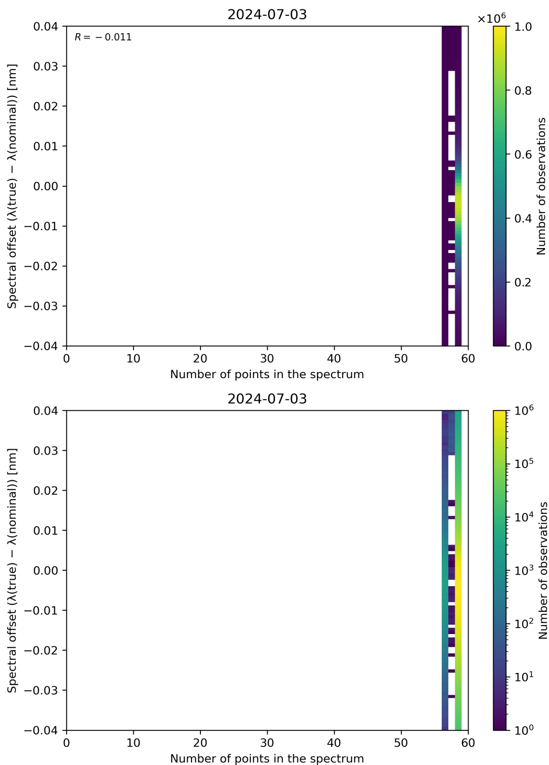
Figure 101: Scatter density plot of “Number of points in the spectrum” against “Spectral offset ( \lambda(\text{true}) - \lambda(\text{nominal}) )” for 2024-07-02 to 2024-07-04.
