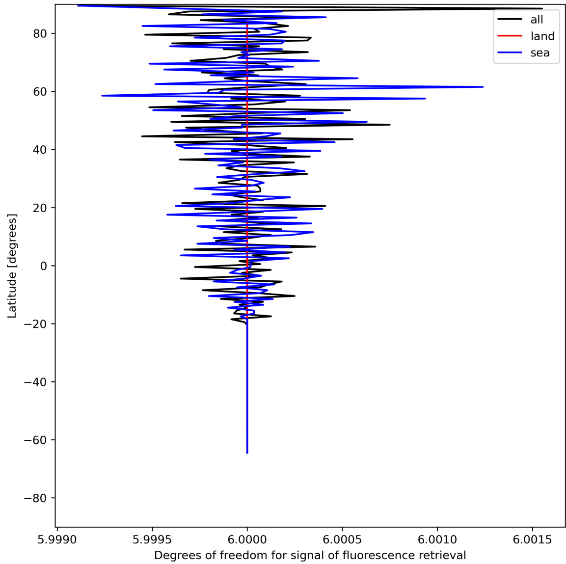
Figure 26: Zonal average of “Degrees of freedom for signal of fluorescence retrieval” for 2024-07-02 to 2024-07-04.
