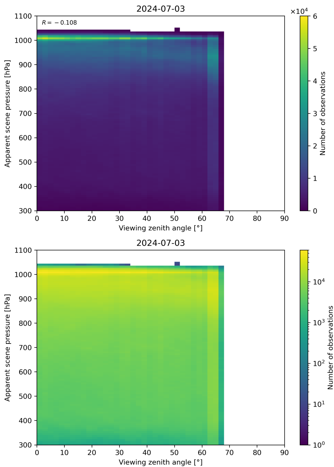
Figure 118: Scatter density plot of “Viewing zenith angle” against “Apparent scene pressure” for 2024-07-02 to 2024-07-04.
