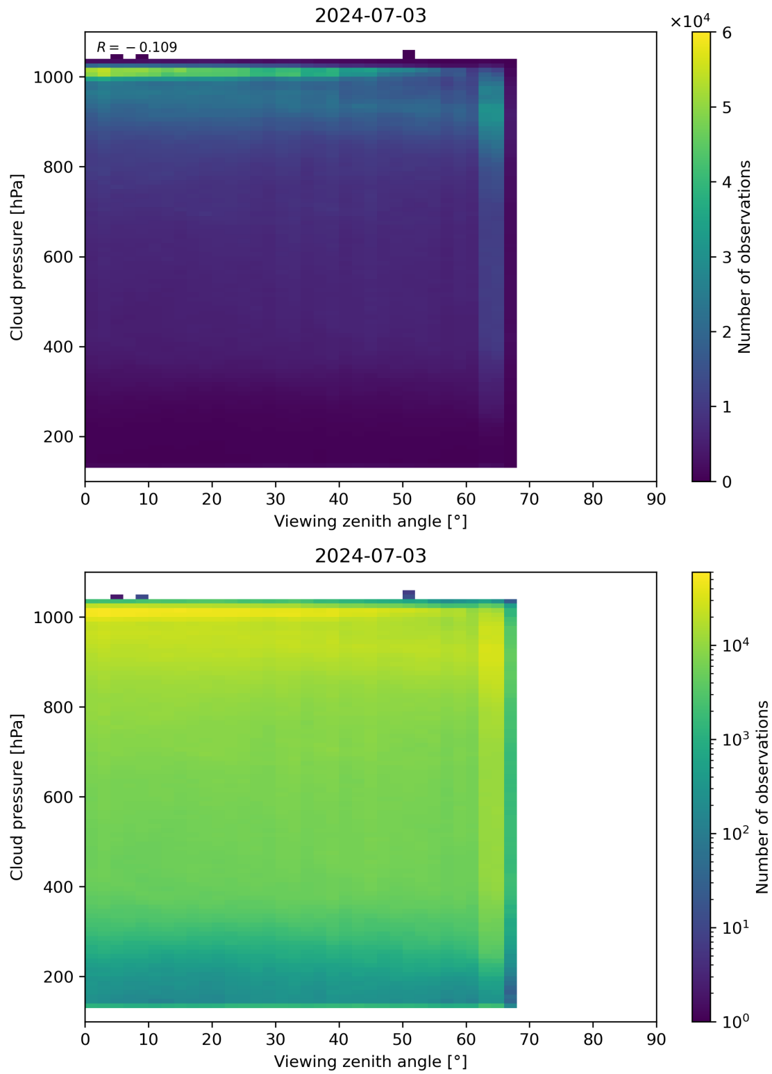
Figure 121: Scatter density plot of “Viewing zenith angle” against “Cloud pressure” for 2024-07-02 to 2024-07-04.
