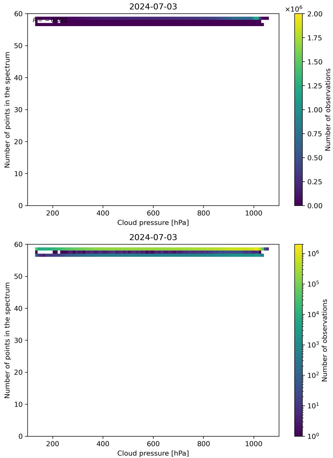
Figure 82: Scatter density plot of “Cloud pressure” against “Number of points in the spectrum” for 2024-07-02 to 2024-07-04.
