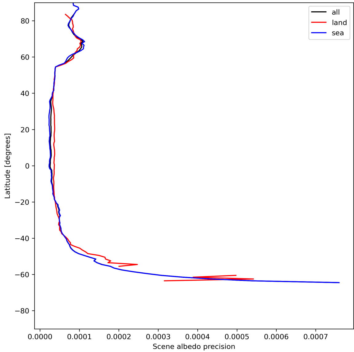
Figure 18: Zonal average of “Scene albedo precision” for 2024-07-02 to 2024-07-04.
