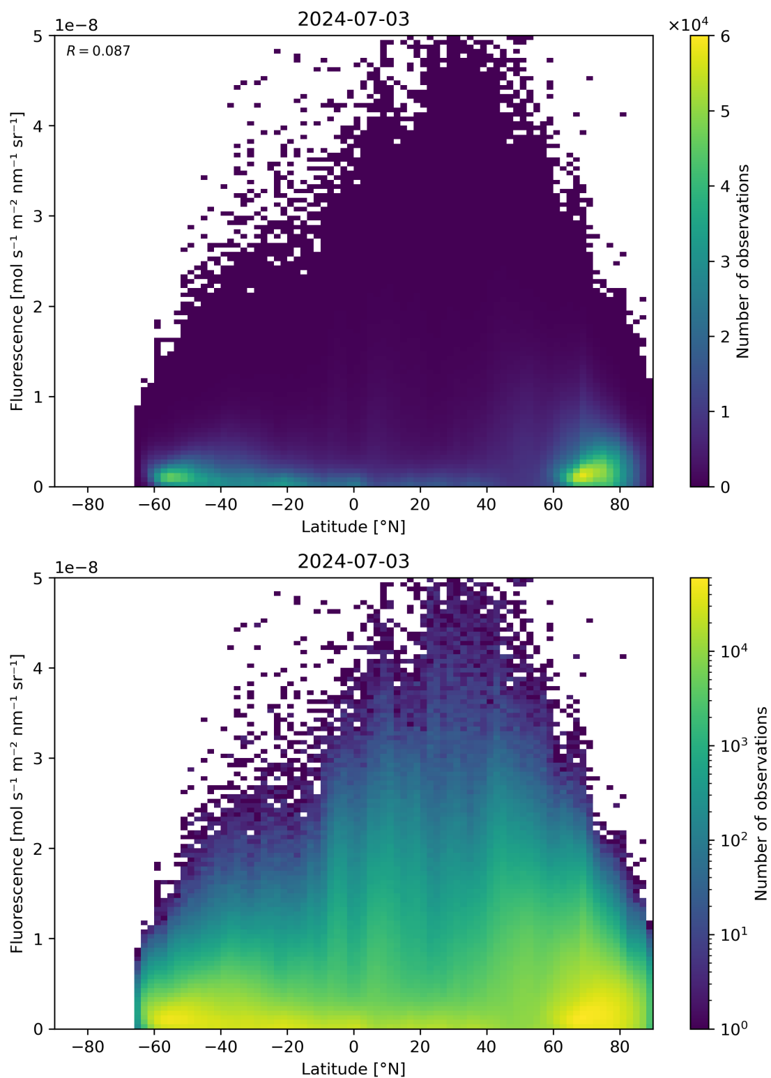
Figure 92: Scatter density plot of “Latitude” against “Fluorescence” for 2024-07-02 to 2024-07-04.
