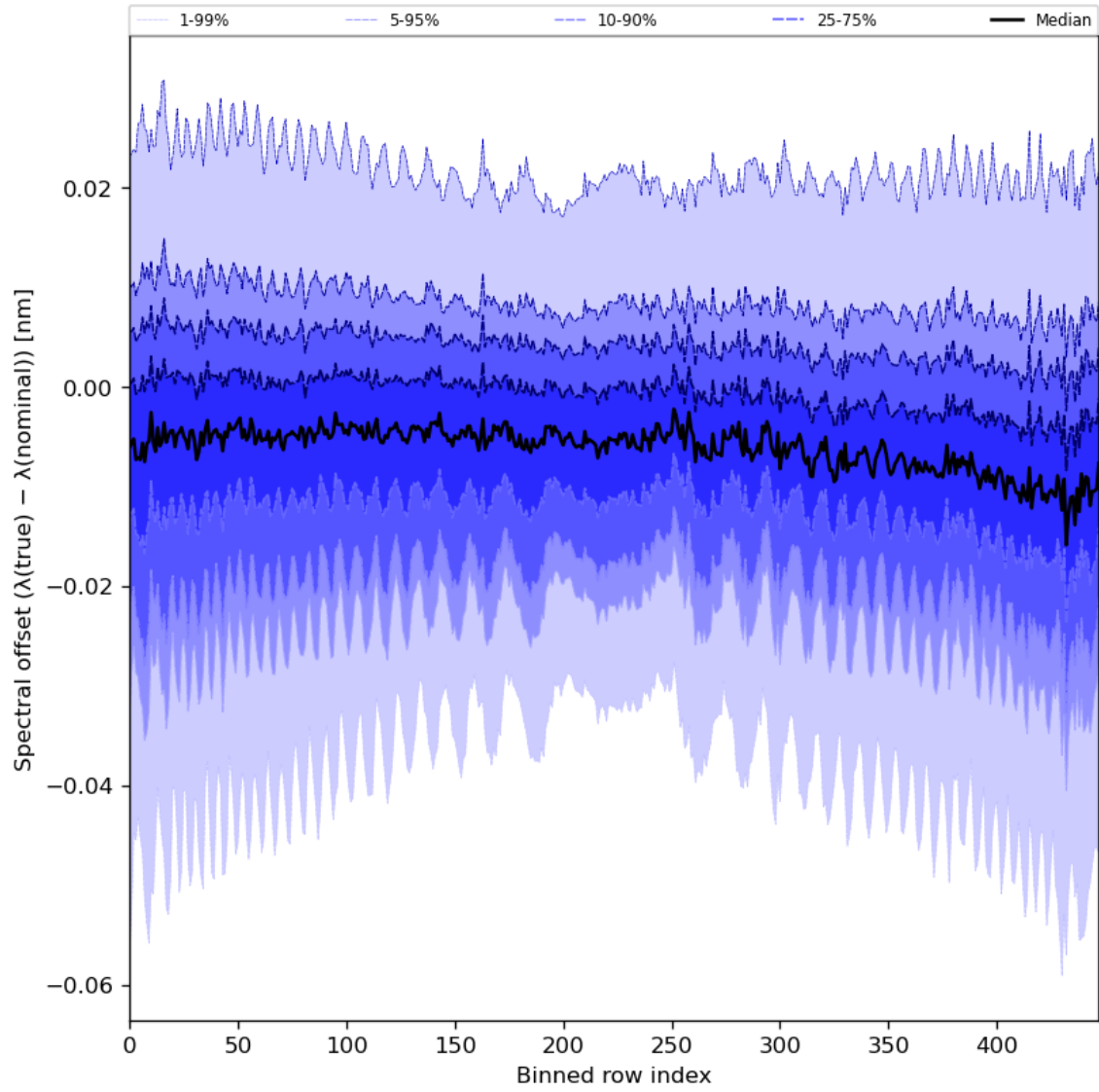
Figure 62: Along track statistics of “Spectral offset ( \lambda(\text{true}) - \lambda(\text{nominal}) )” for 2024-07-02 to 2024-07-04
