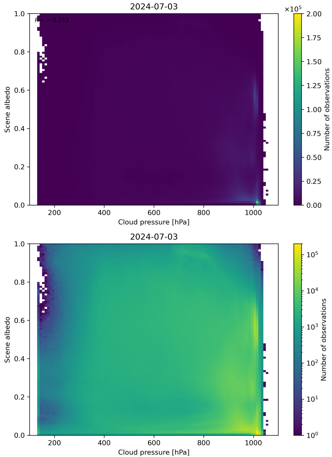
Figure 83: Scatter density plot of “Cloud pressure” against “Scene albedo” for 2024-07-02 to 2024-07-04.
