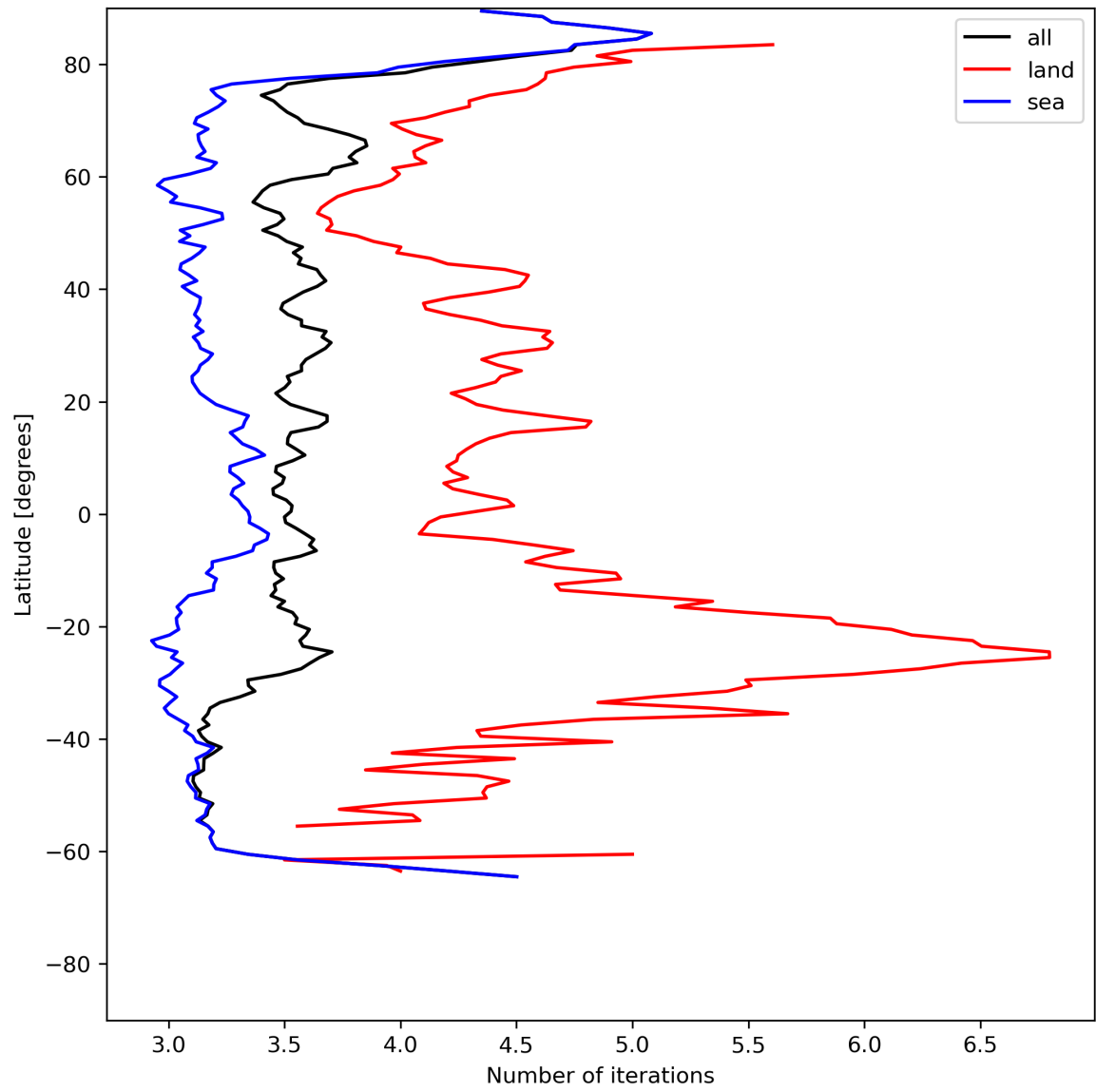
Figure 22: Zonal average of “Number of iterations” for 2024-07-02 to 2024-07-04.
