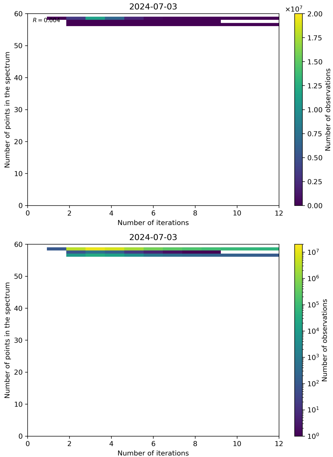
Figure 99: Scatter density plot of “Number of iterations” against “Number of points in the spectrum” for 2024-07-02 to 2024-07-04.
