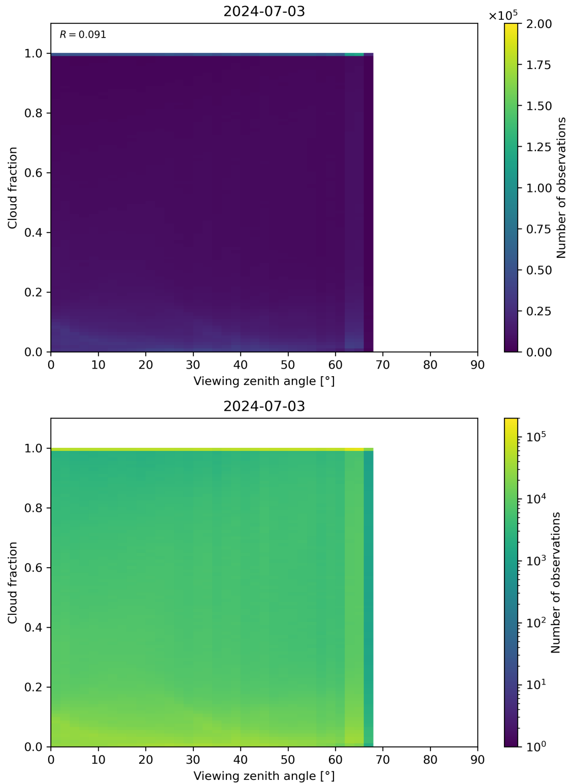
Figure 120: Scatter density plot of “Viewing zenith angle” against “Cloud fraction” for 2024-07-02 to 2024-07-04.
