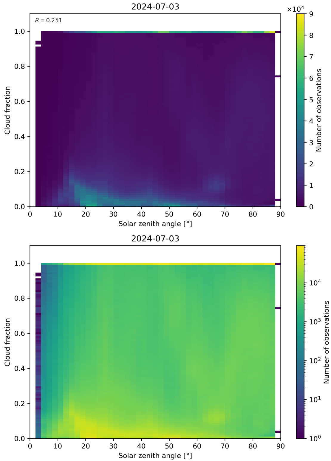
Figure 110: Scatter density plot of “Solar zenith angle” against “Cloud fraction” for 2024-07-02 to 2024-07-04.
