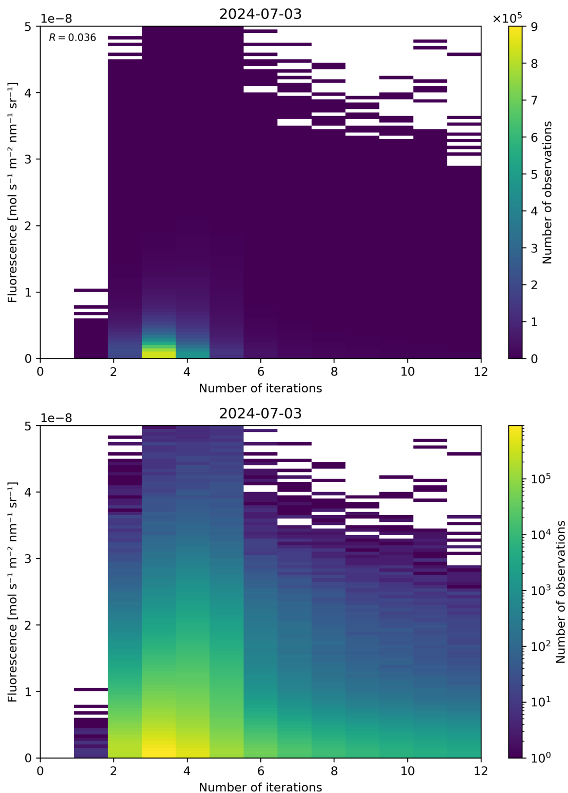
Figure 98: Scatter density plot of “Number of iterations” against “Fluorescence” for 2024-07-02 to 2024-07-04.
