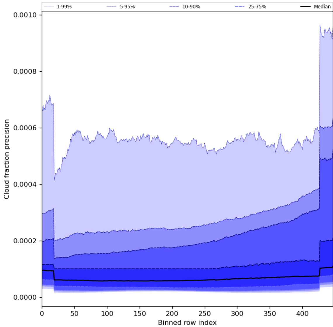
Figure 50: Along track statistics of “Cloud fraction precision” for 2024-07-02 to 2024-07-04
