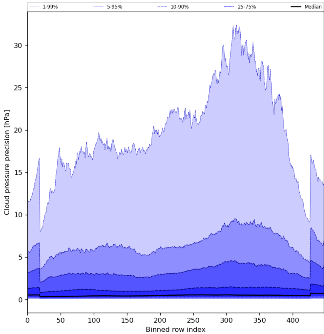
Figure 48: Along track statistics of “Cloud pressure precision” for 2024-07-02 to 2024-07-04
