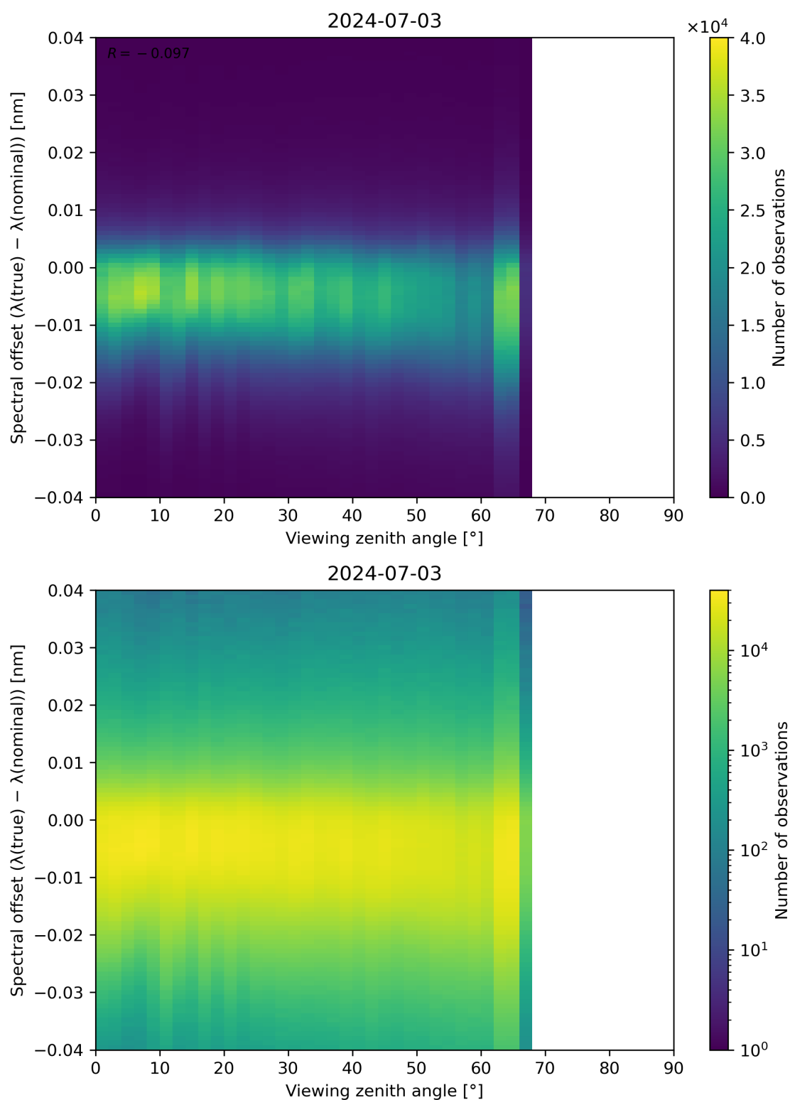
Figure 128: Scatter density plot of “Viewing zenith angle” against “Spectral offset ( \lambda(\text{true}) - \lambda(\text{nominal}) )” for 2024-07-02 to 2024-07-04.
