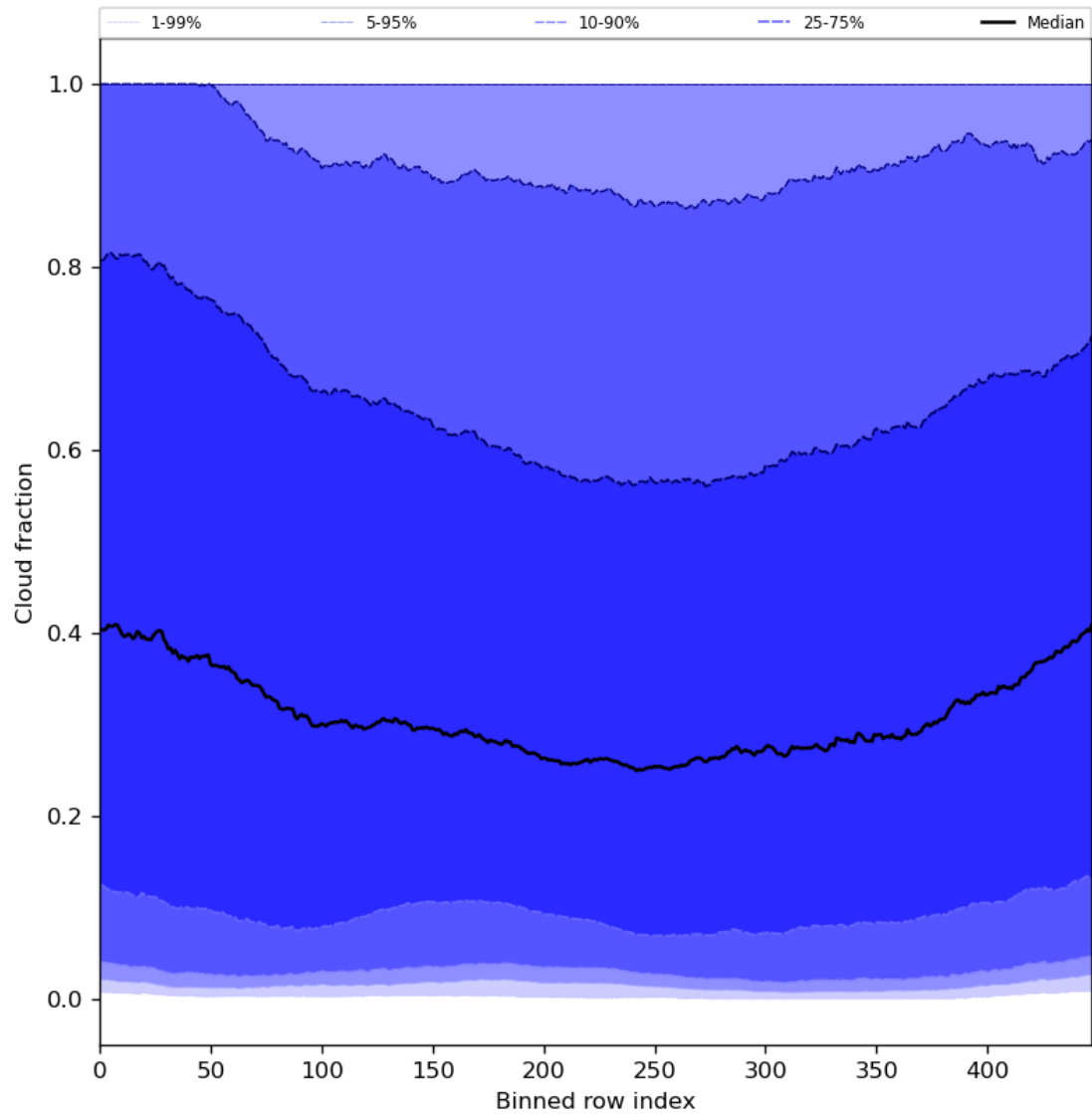
Figure 49: Along track statistics of “Cloud fraction” for 2024-07-02 to 2024-07-04
