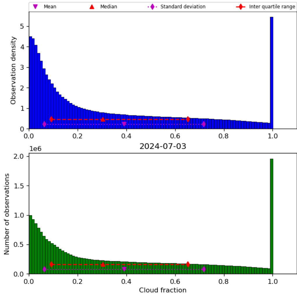
Figure 32: Histogram of “Cloud fraction” for 2024-07-02 to 2024-07-04
