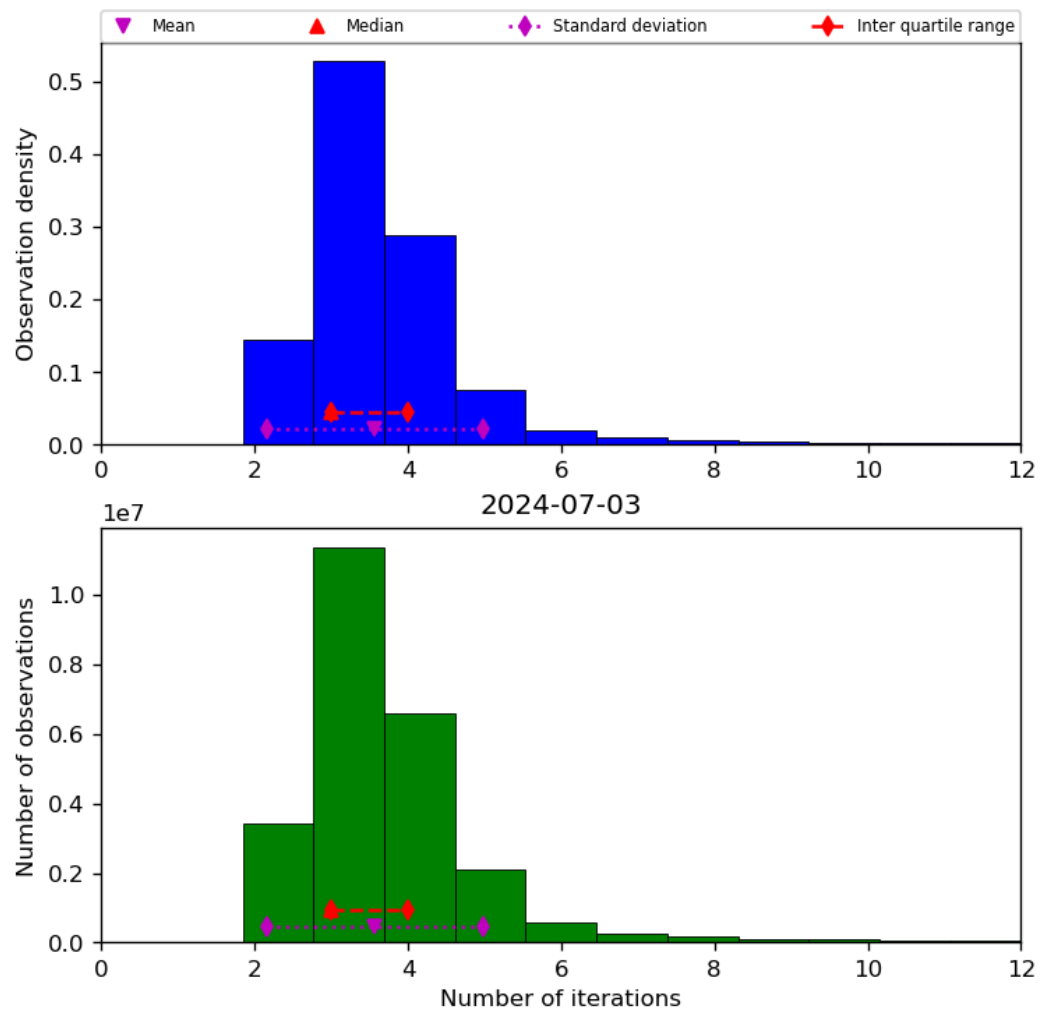
Figure 39: Histogram of “Number of iterations” for 2024-07-02 to 2024-07-04
