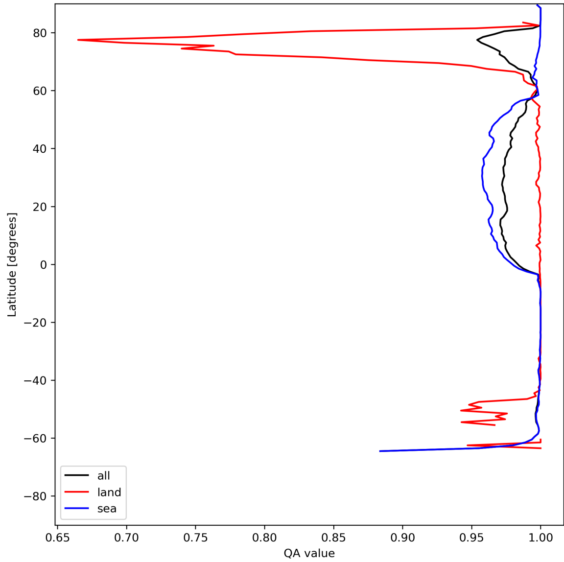
Figure 12: Zonal average of “QA value” for 2024-07-02 to 2024-07-04.
