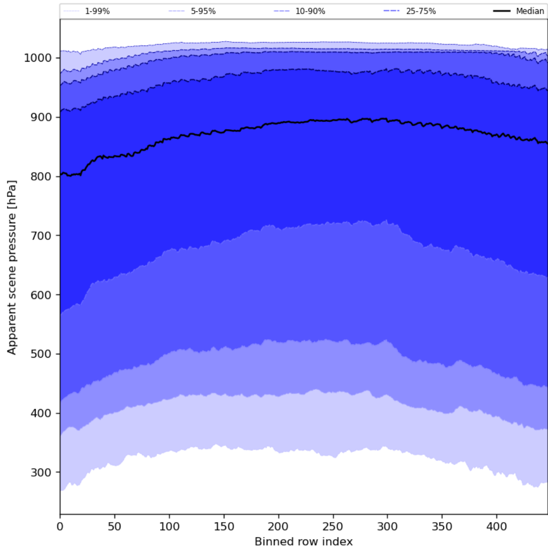
Figure 53: Along track statistics of “Apparent scene pressure” for 2024-07-02 to 2024-07-04
