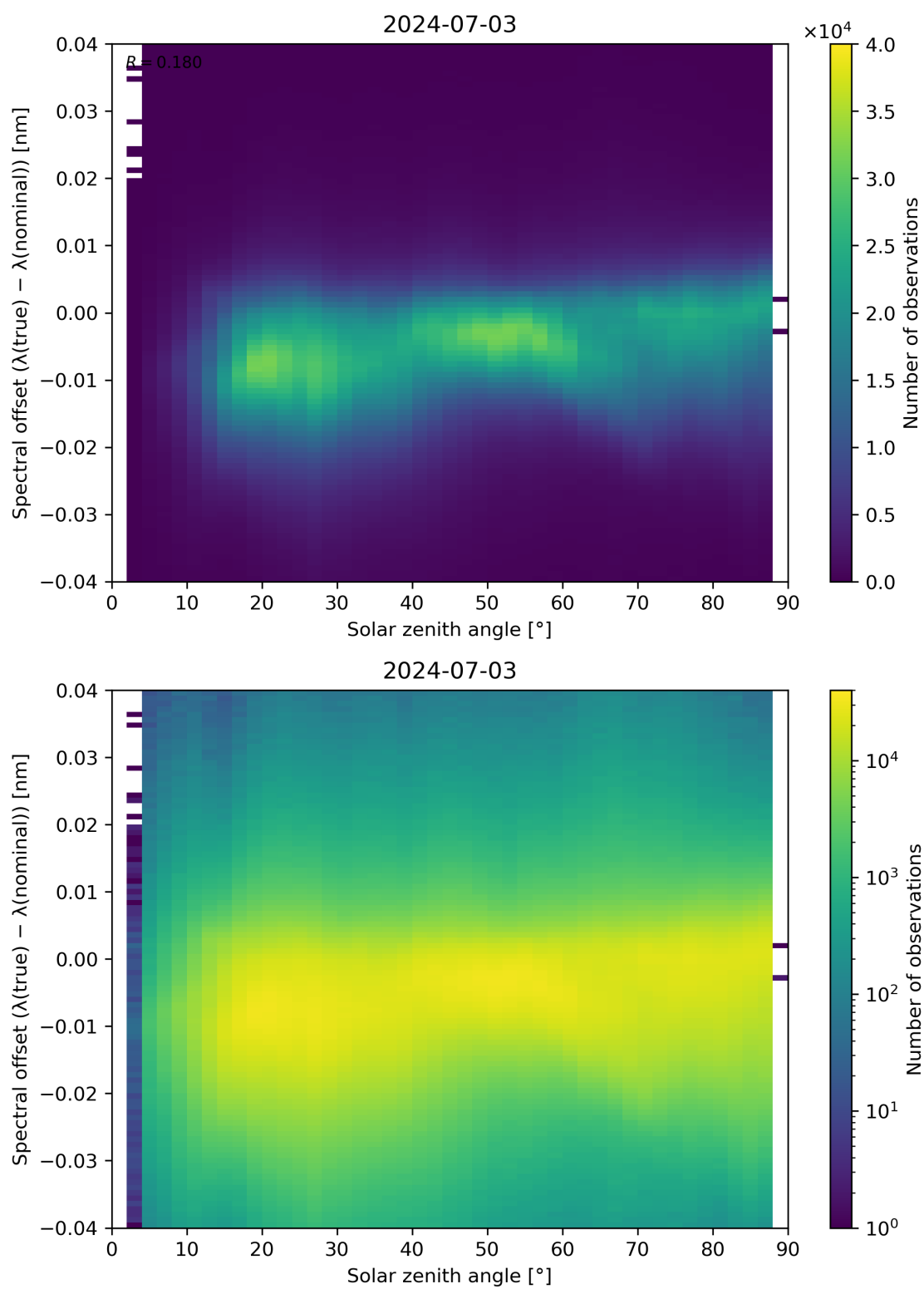
Figure 117: Scatter density plot of “Solar zenith angle” against “Spectral offset ( \lambda(\text{true}) - \lambda(\text{nominal}) )” for 2024-07-02 to 2024-07-04.
