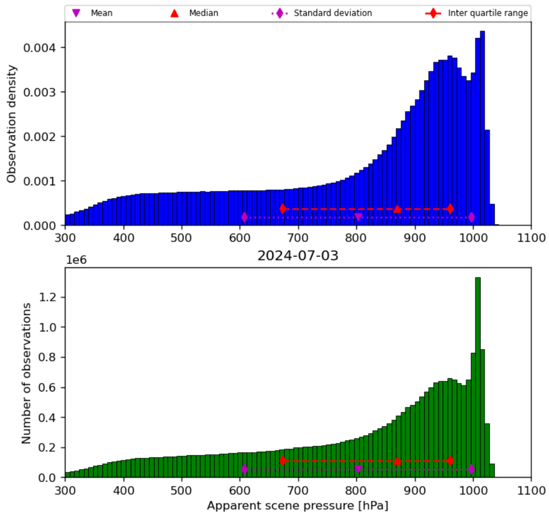
Figure 36: Histogram of “Apparent scene pressure” for 2024-07-02 to 2024-07-04
