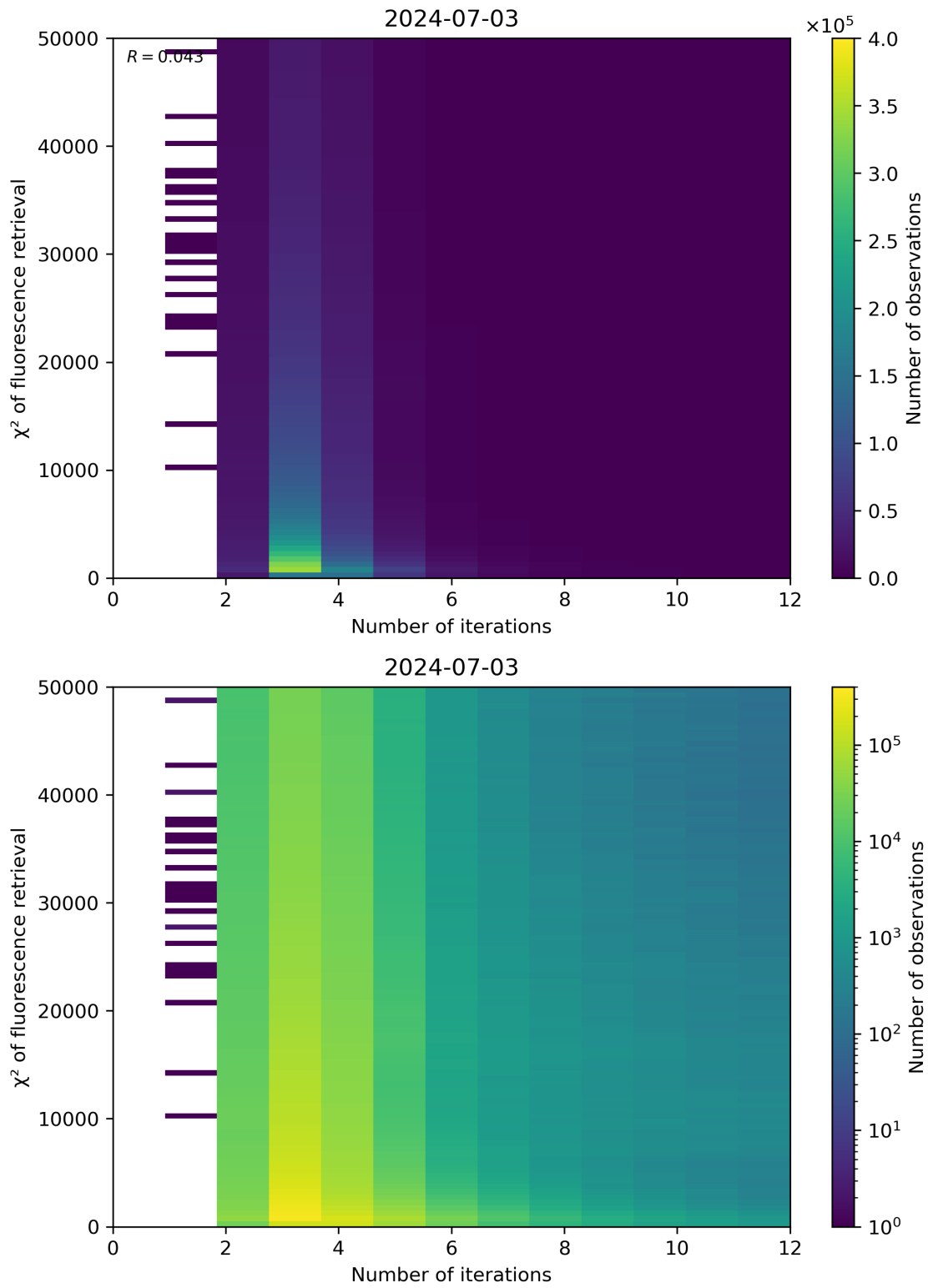
Figure 97: Scatter density plot of “Number of iterations” against “ \chi^2 of fluorescence retrieval” for 2024-07-02 to 2024-07-04.
