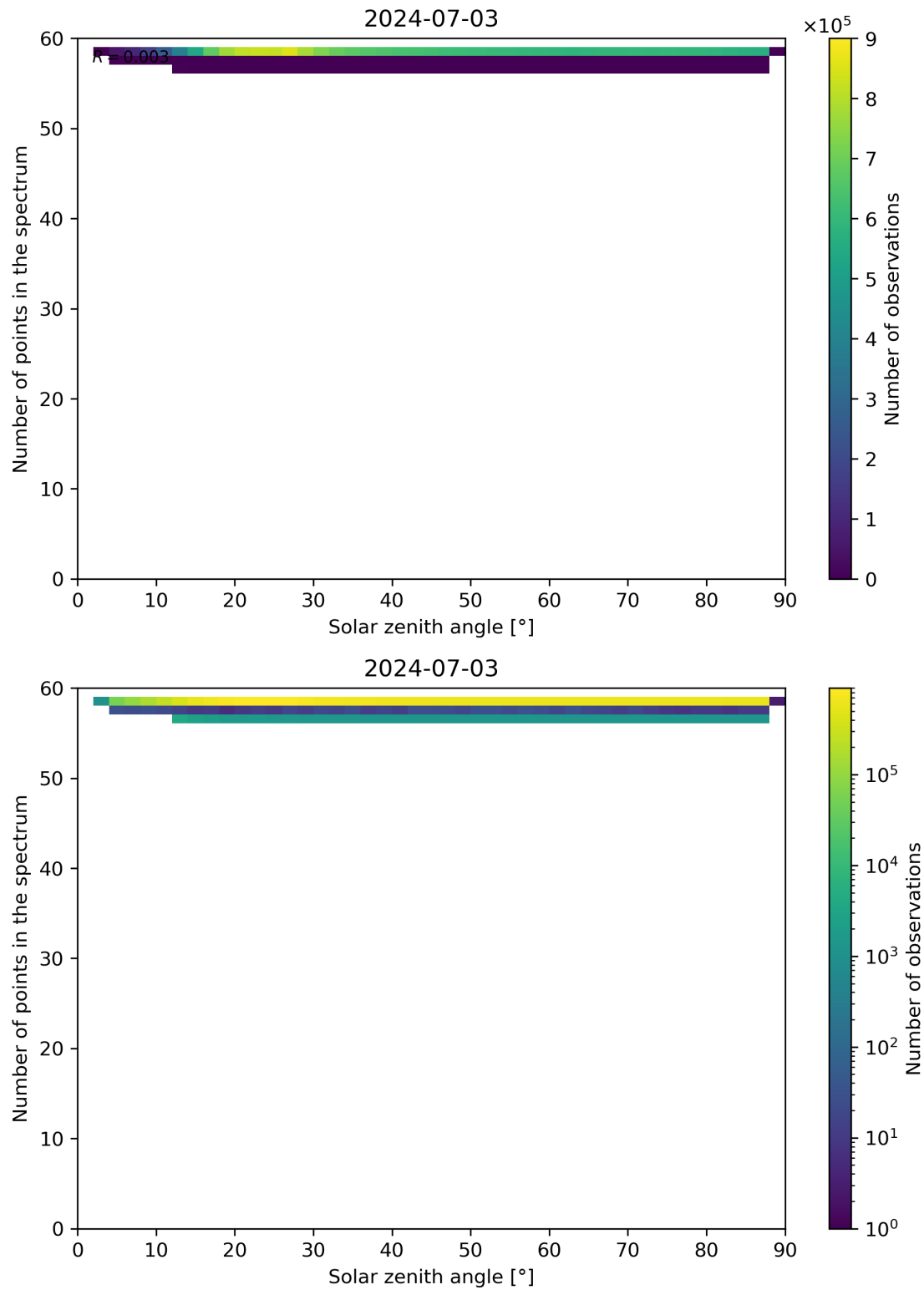
Figure 115: Scatter density plot of “Solar zenith angle” against “Number of points in the spectrum” for 2024-07-02 to 2024-07-04.
