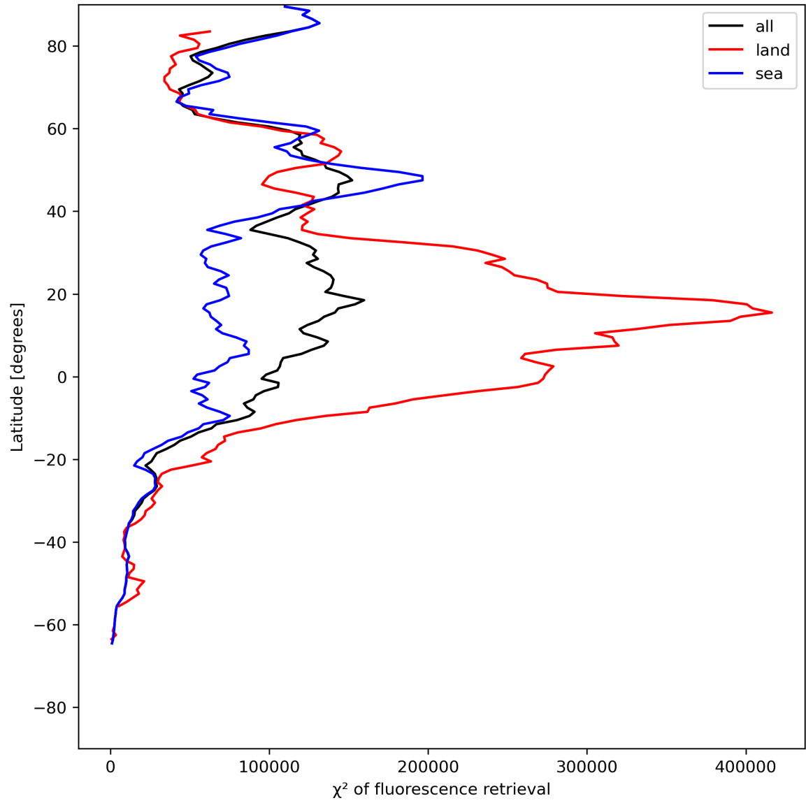
Figure 25: Zonal average of “ \chi^2 of fluorescence retrieval” for 2024-07-02 to 2024-07-04.
