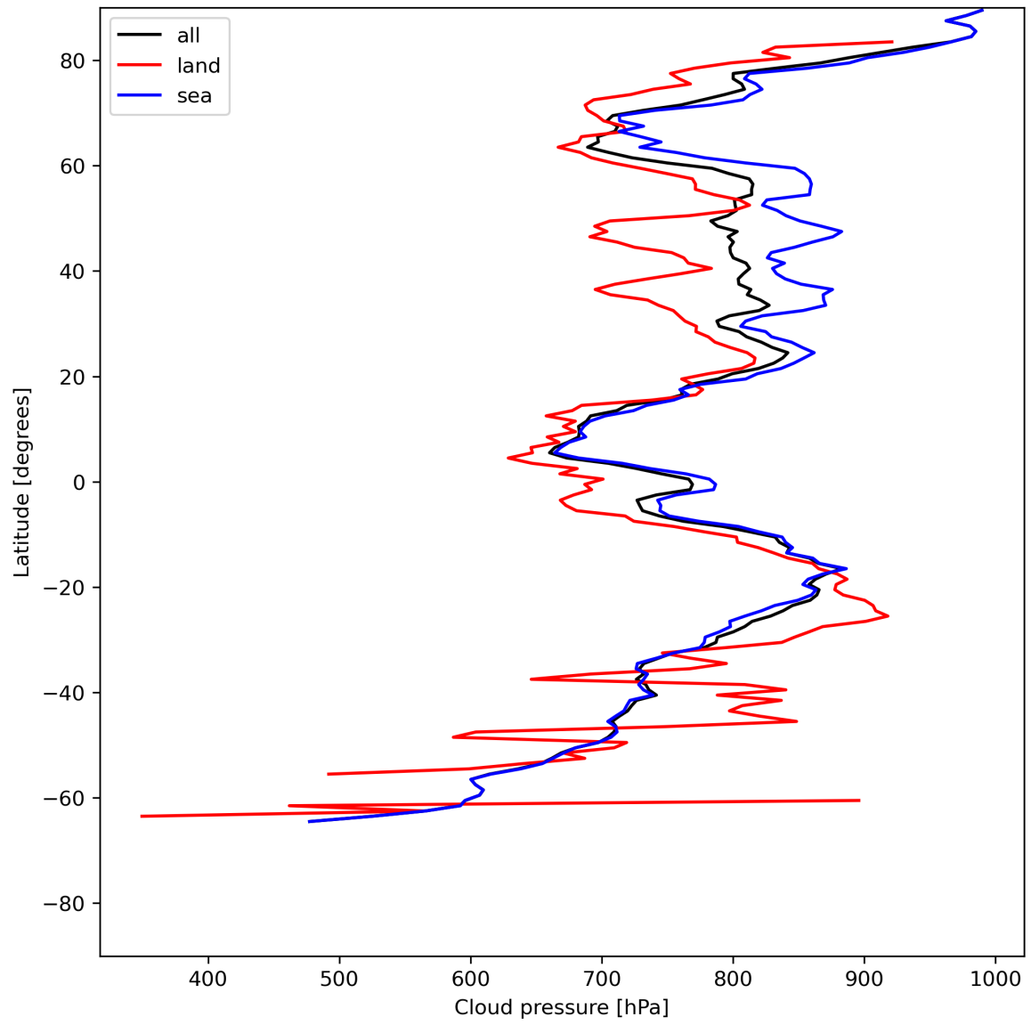
Figure 13: Zonal average of “Cloud pressure” for 2024-07-02 to 2024-07-04.
