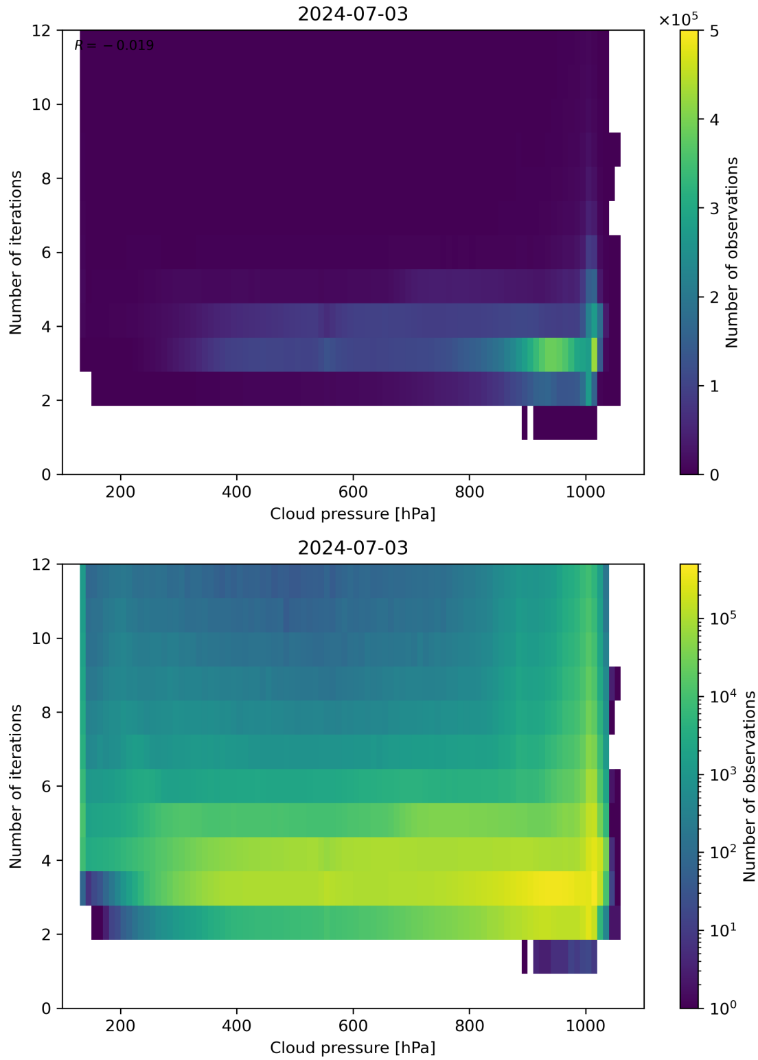
Figure 81: Scatter density plot of “Cloud pressure” against “Number of iterations” for 2024-07-02 to 2024-07-04.
