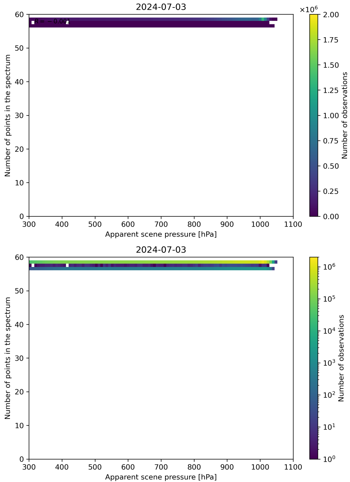
Figure 66: Scatter density plot of “Apparent scene pressure” against “Number of points in the spectrum” for 2024-07-02 to 2024-07-04.
