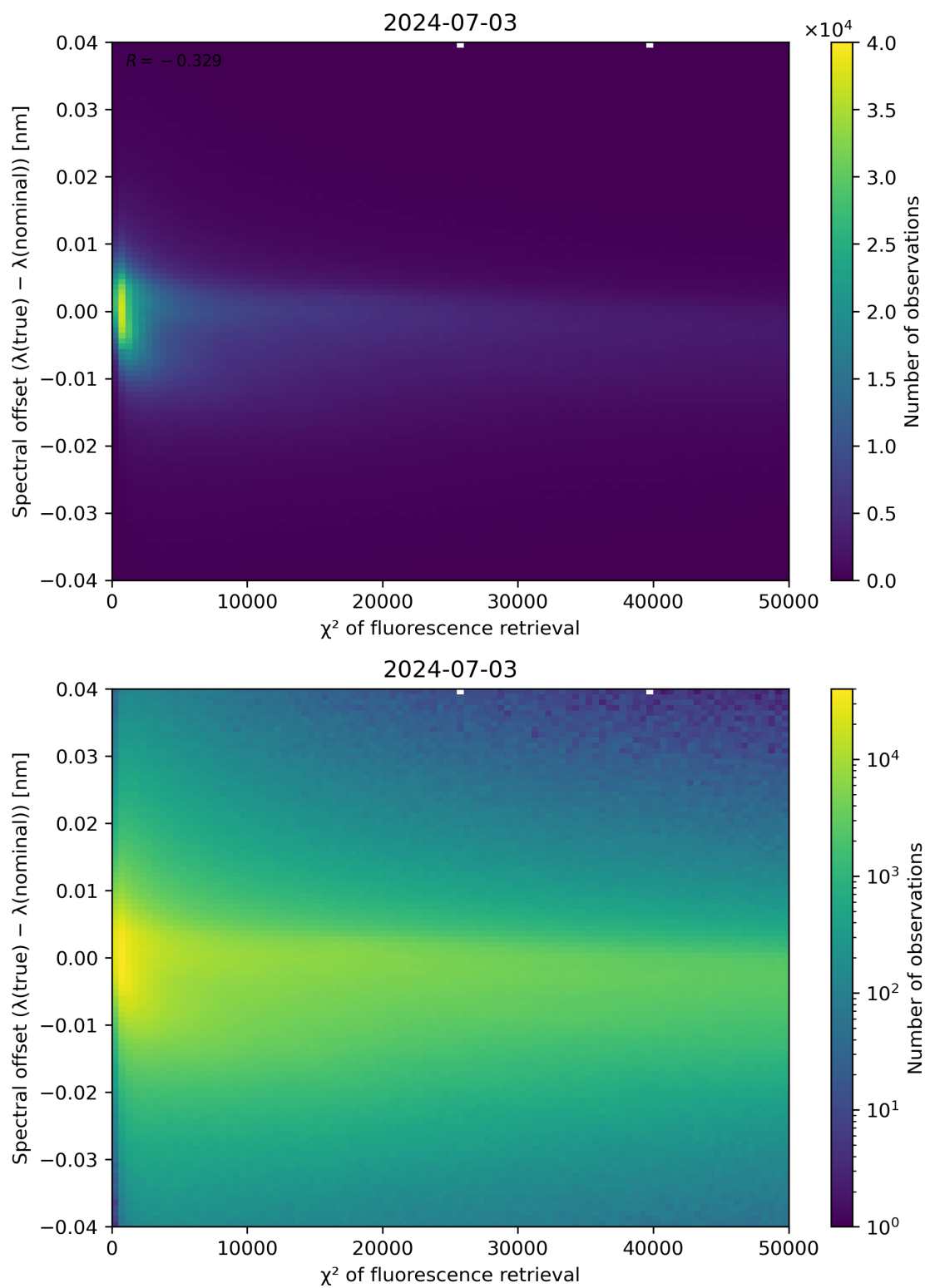
Figure 69: Scatter density plot of " \chi^2 of fluorescence retrieval" against "Spectral offset ( \lambda(\text{true}) - \lambda(\text{nominal})) " for 2024-07-02 to 2024-07-04.
