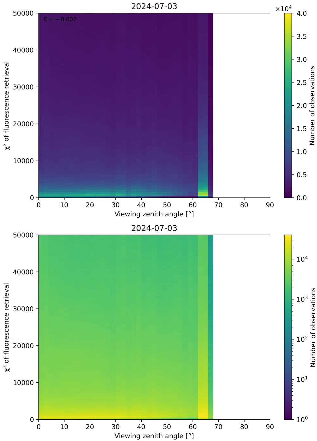
Figure 119: Scatter density plot of “Viewing zenith angle” against “ \chi^2 of fluorescence retrieval” for 2024-07-02 to 2024-07-04.
