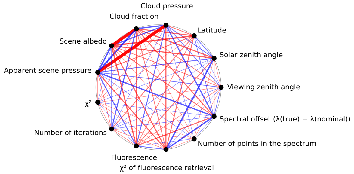
Figure 1: Map of correlation graph for 2024-07-02 to 2024-07-04.
