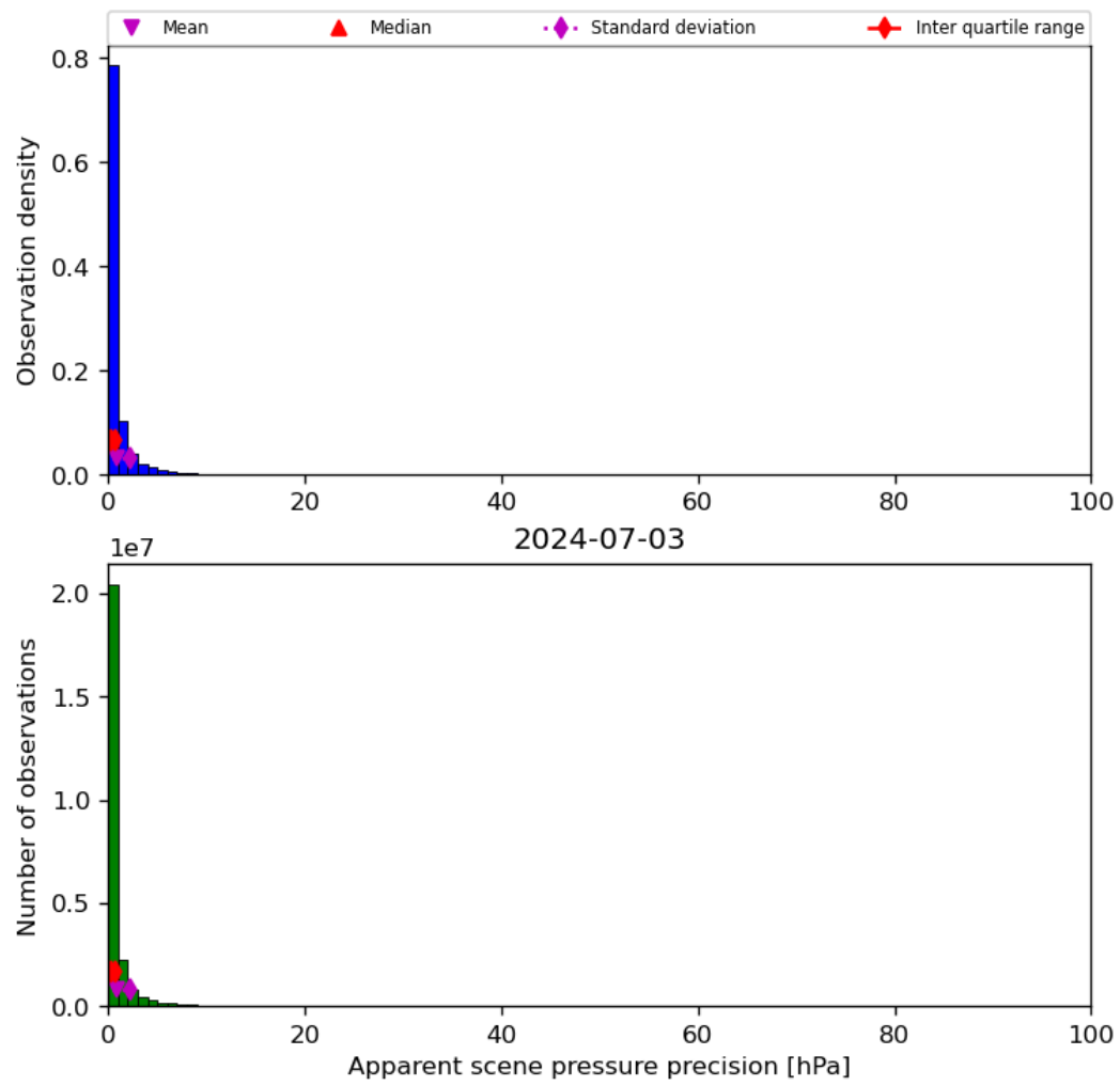
Figure 37: Histogram of “Apparent scene pressure precision” for 2024-07-02 to 2024-07-04
