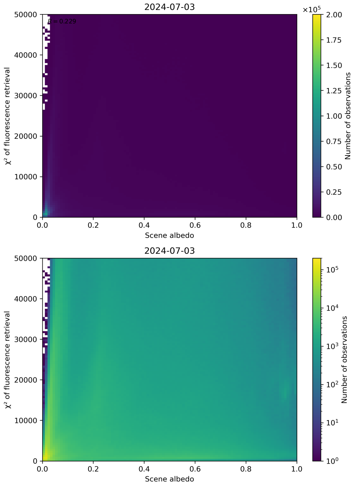
Figure 103: Scatter density plot of “Scene albedo” against “ \chi^2 of fluorescence retrieval” for 2024-07-02 to 2024-07-04.
