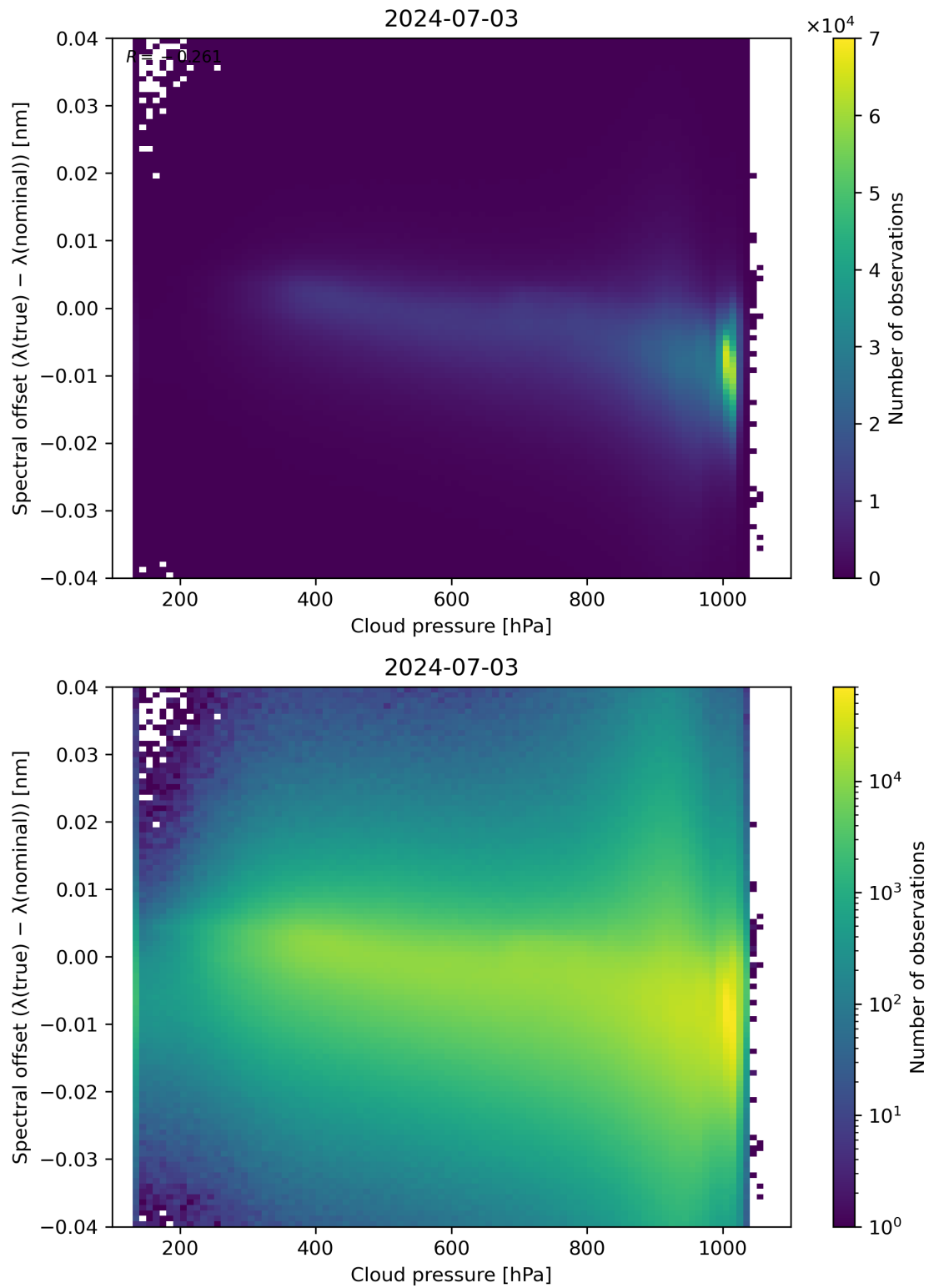
Figure 84: Scatter density plot of “Cloud pressure” against “Spectral offset ( \lambda(\text{true}) - \lambda(\text{nominal}) )” for 2024-07-02 to 2024-07-04.
