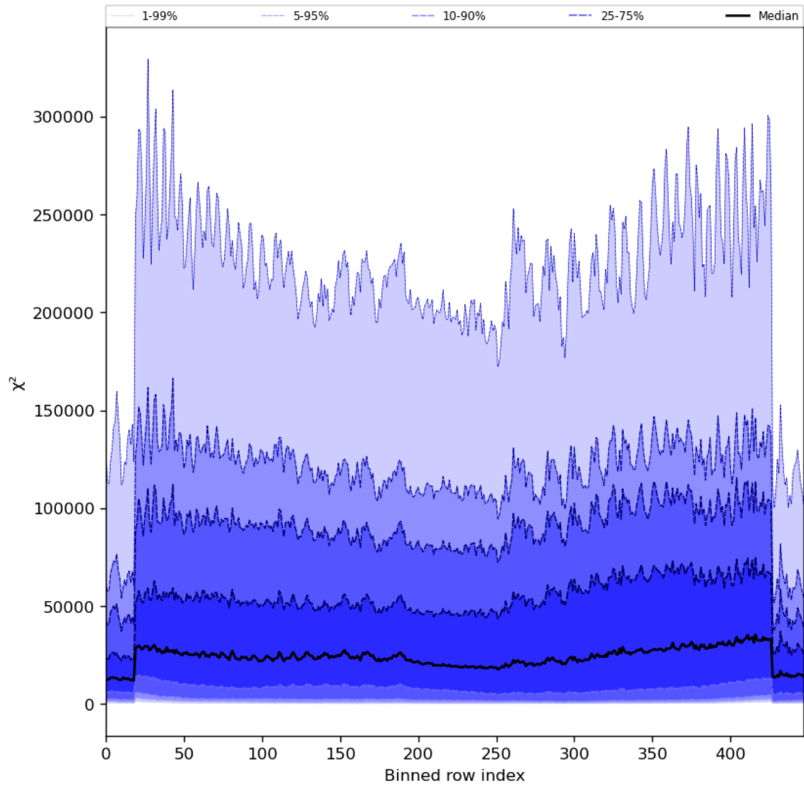
Figure 55: Along track statistics of “ \chi^2 ” for 2024-07-02 to 2024-07-04
