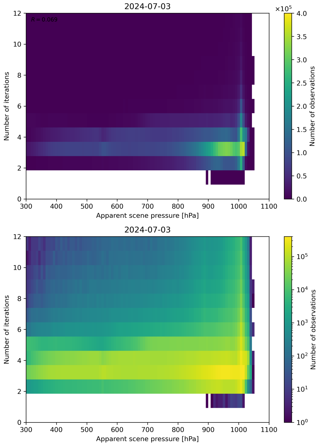
Figure 65: Scatter density plot of “Apparent scene pressure” against “Number of iterations” for 2024-07-02 to 2024-07-04.
