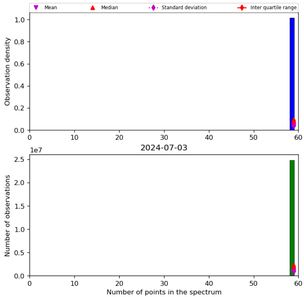
Figure 44: Histogram of “Number of points in the spectrum” for 2024-07-02 to 2024-07-04
