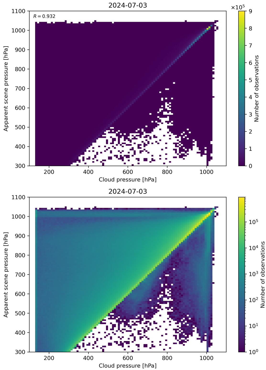
Figure 77: Scatter density plot of “Cloud pressure” against “Apparent scene pressure” for 2024-07-02 to 2024-07-04.
