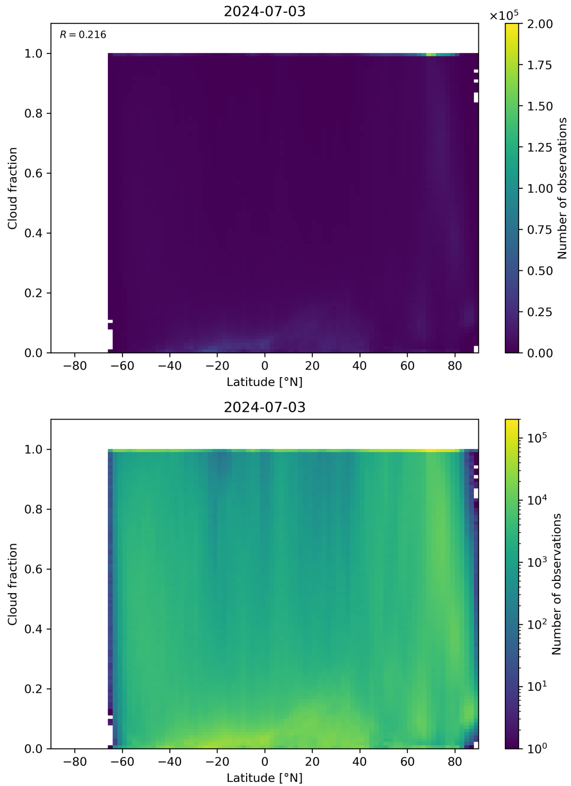
Figure 90: Scatter density plot of “Latitude” against “Cloud fraction” for 2024-07-02 to 2024-07-04.
