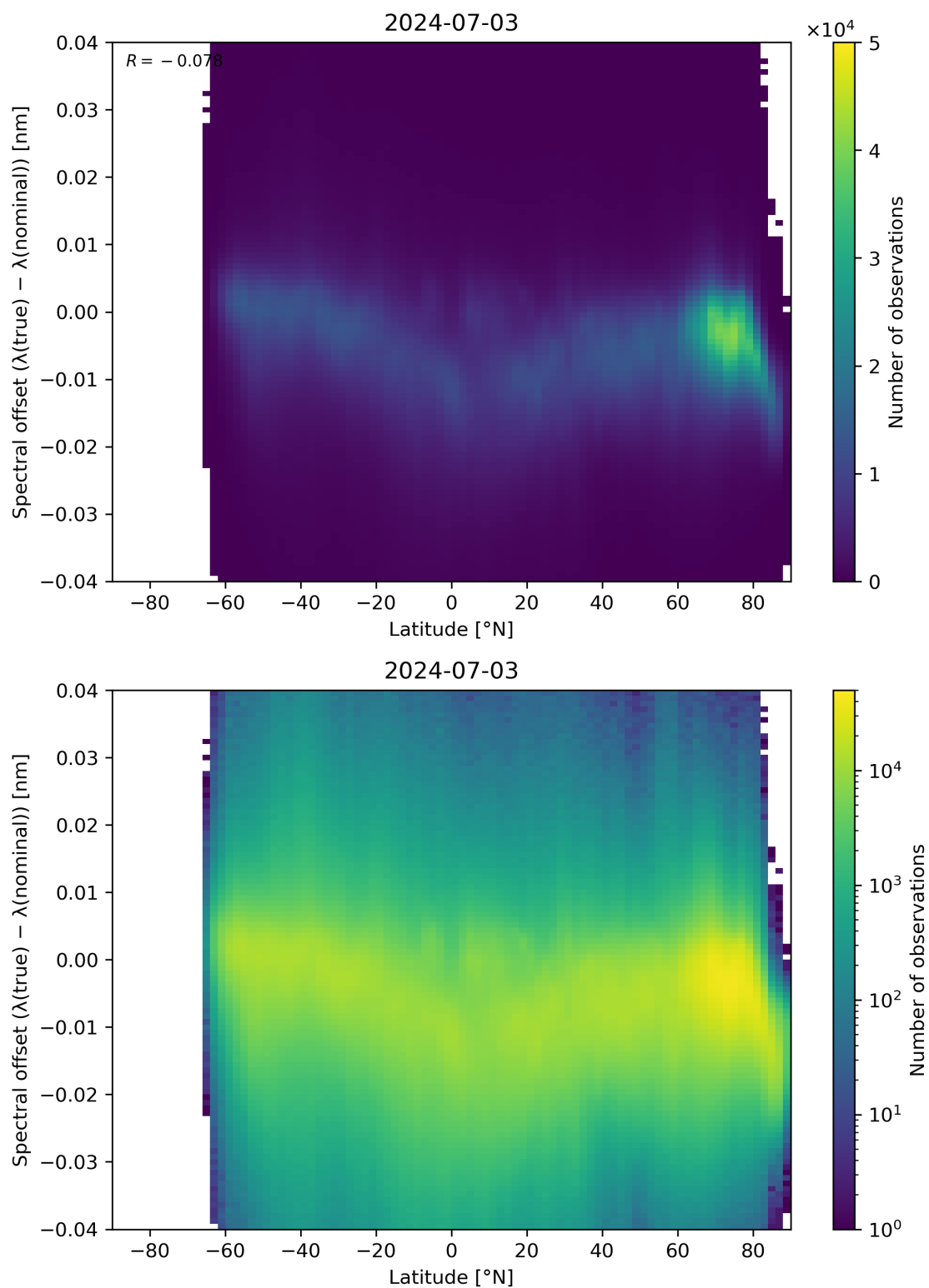
Figure 96: Scatter density plot of “Latitude” against “Spectral offset ( \lambda(\text{true}) - \lambda(\text{nominal}) )” for 2024-07-02 to 2024-07-04.
