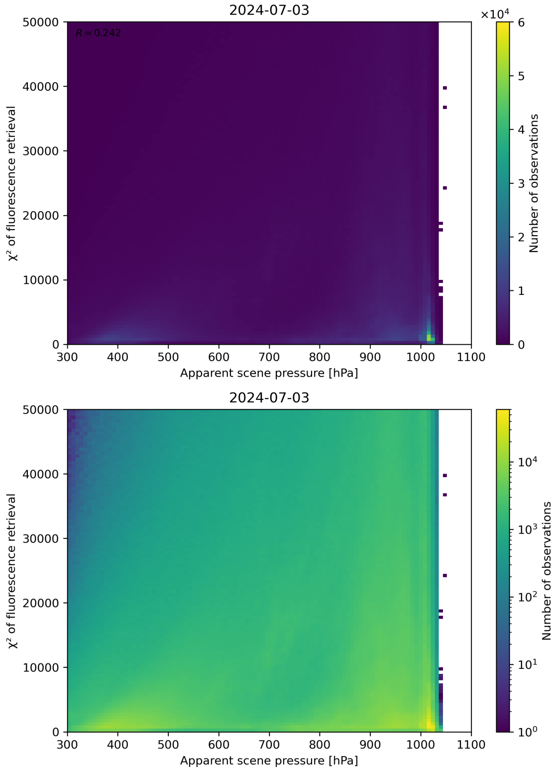
Figure 63: Scatter density plot of “Apparent scene pressure” against “ \chi^2 of fluorescence retrieval” for 2024-07-02 to 2024-07-04.
