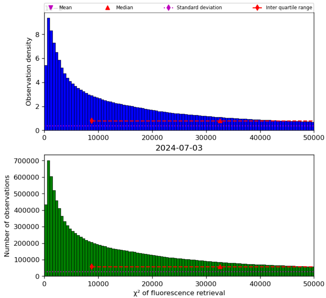
Figure 42: Histogram of “ \chi^2 of fluorescence retrieval” for 2024-07-02 to 2024-07-04
