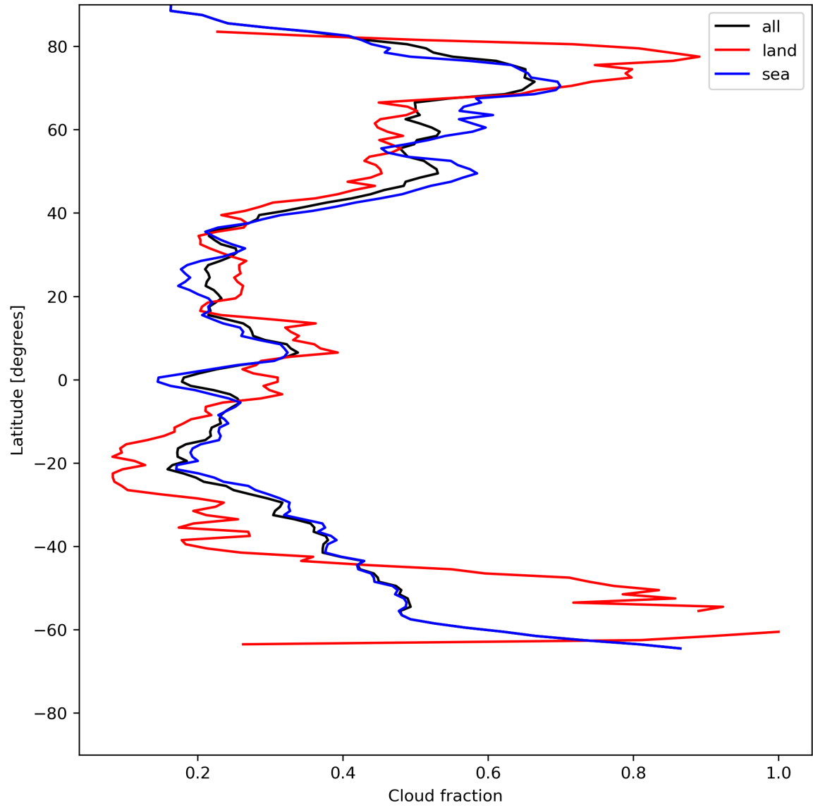
Figure 15: Zonal average of “Cloud fraction” for 2024-07-02 to 2024-07-04.
