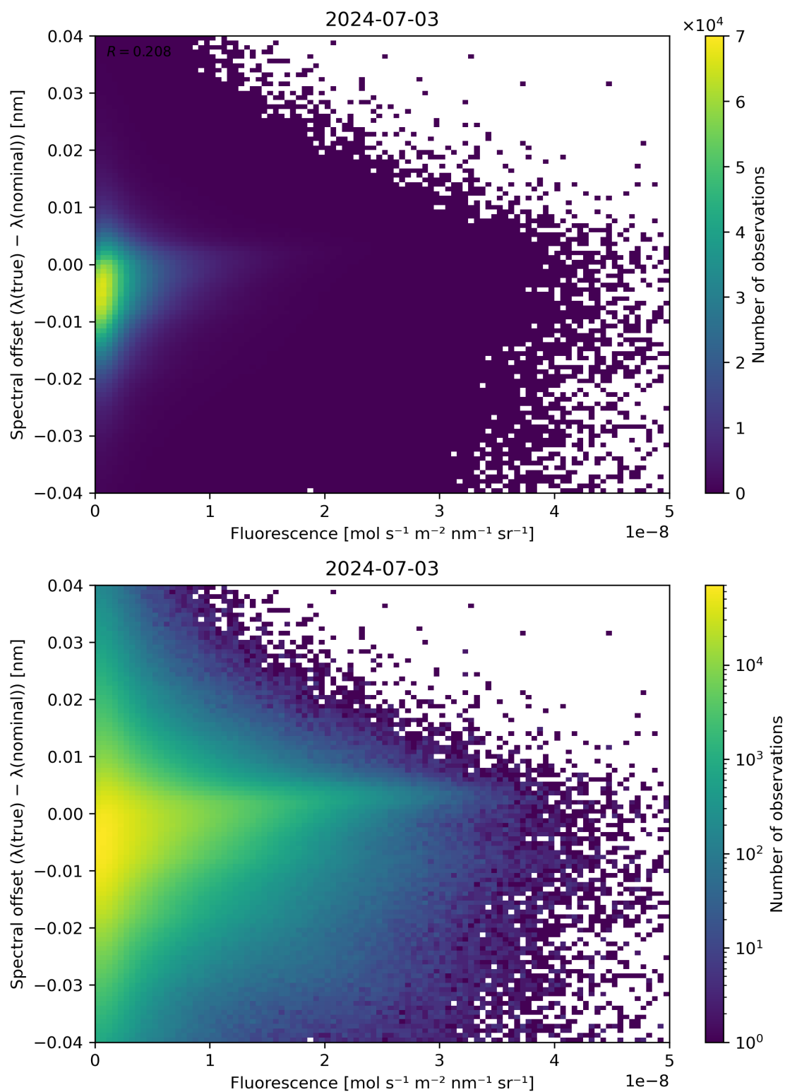
Figure 87: Scatter density plot of “Fluorescence” against “Spectral offset ( \lambda(\text{true}) - \lambda(\text{nominal}) )” for 2024-07-02 to 2024-07-04.
