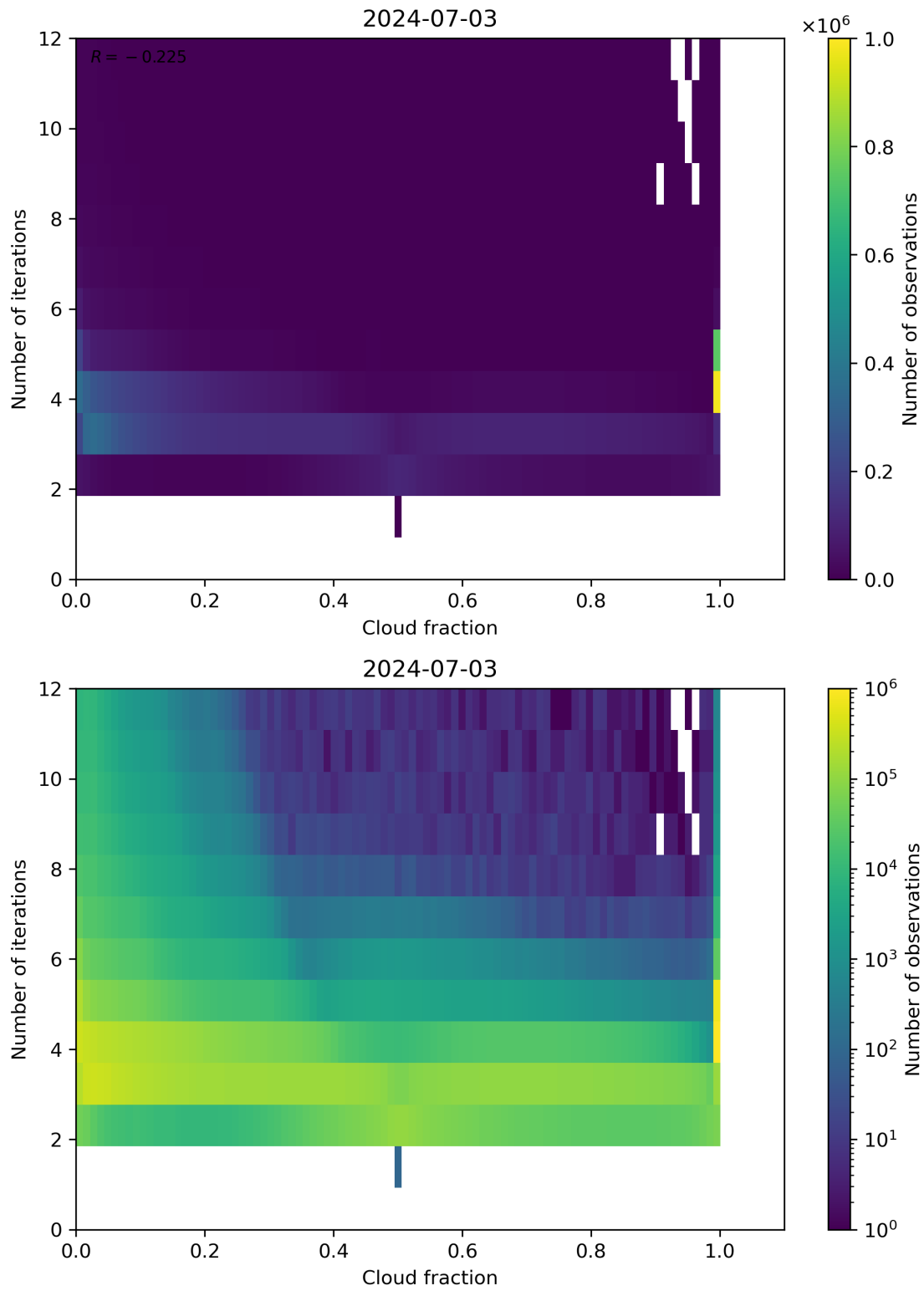
Figure 73: Scatter density plot of “Cloud fraction” against “Number of iterations” for 2024-07-02 to 2024-07-04.
