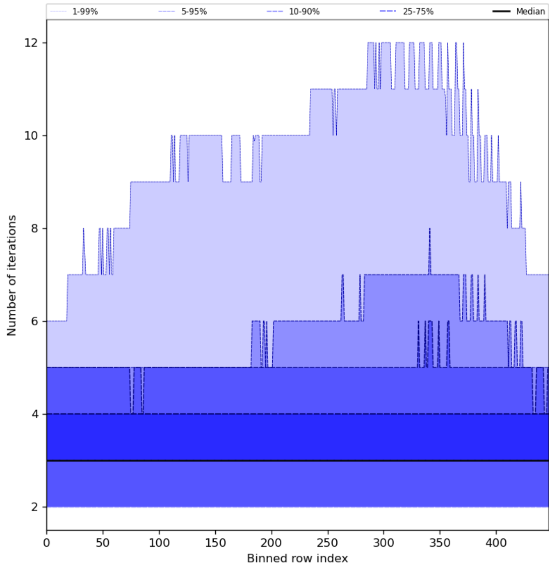
Figure 56: Along track statistics of “Number of iterations” for 2024-07-02 to 2024-07-04
