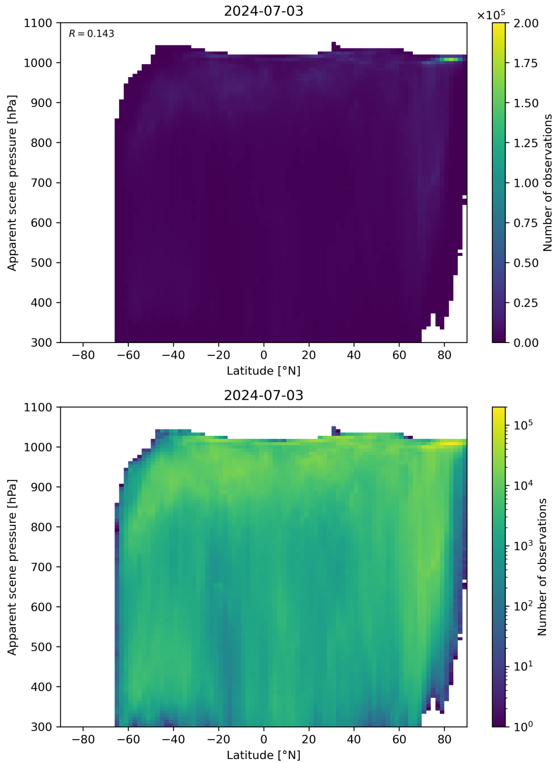
Figure 88: Scatter density plot of “Latitude” against “Apparent scene pressure” for 2024-07-02 to 2024-07-04.
