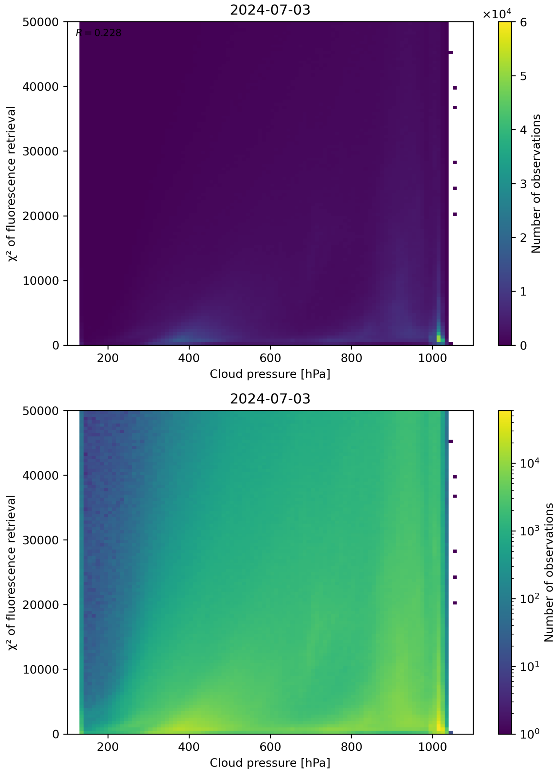
Figure 78: Scatter density plot of “Cloud pressure” against “ \chi^2 of fluorescence retrieval” for 2024-07-02 to 2024-07-04.
