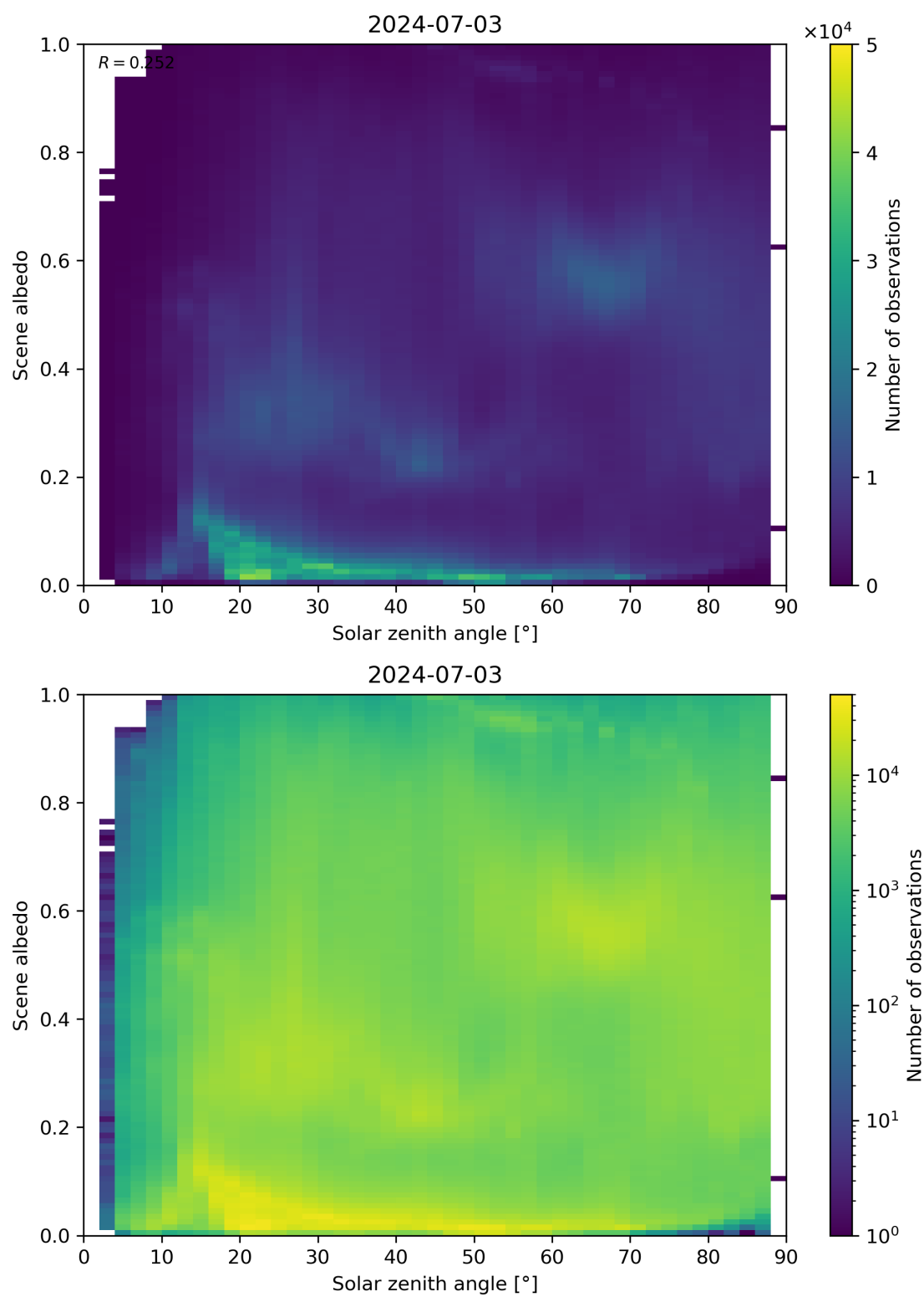
Figure 116: Scatter density plot of “Solar zenith angle” against “Scene albedo” for 2024-07-02 to 2024-07-04.
