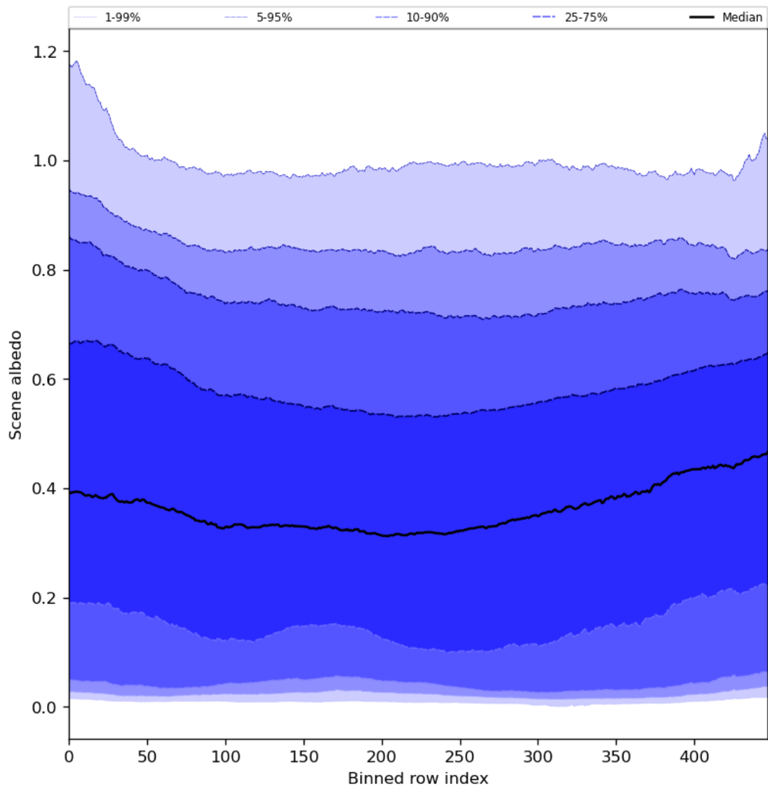
Figure 51: Along track statistics of “Scene albedo” for 2024-07-02 to 2024-07-04
