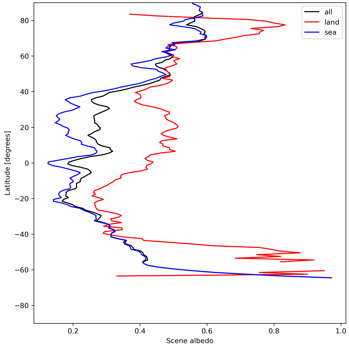
Figure 17: Zonal average of “Scene albedo” for 2024-07-02 to 2024-07-04.
