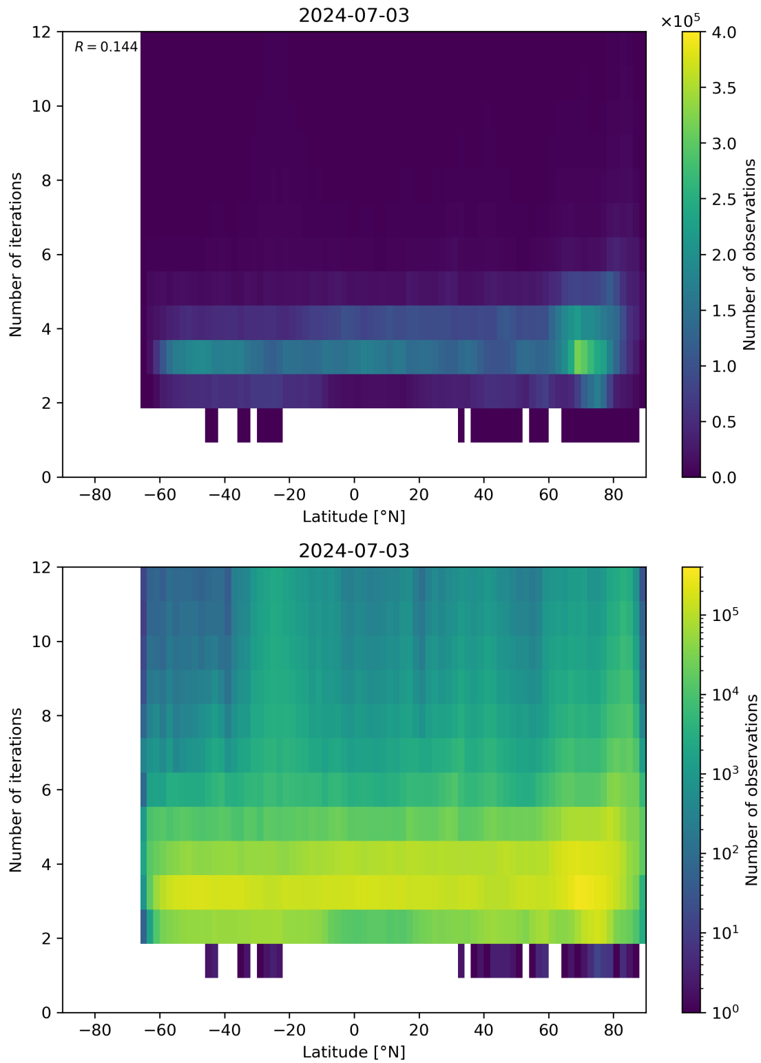
Figure 93: Scatter density plot of “Latitude” against “Number of iterations” for 2024-07-02 to 2024-07-04.
