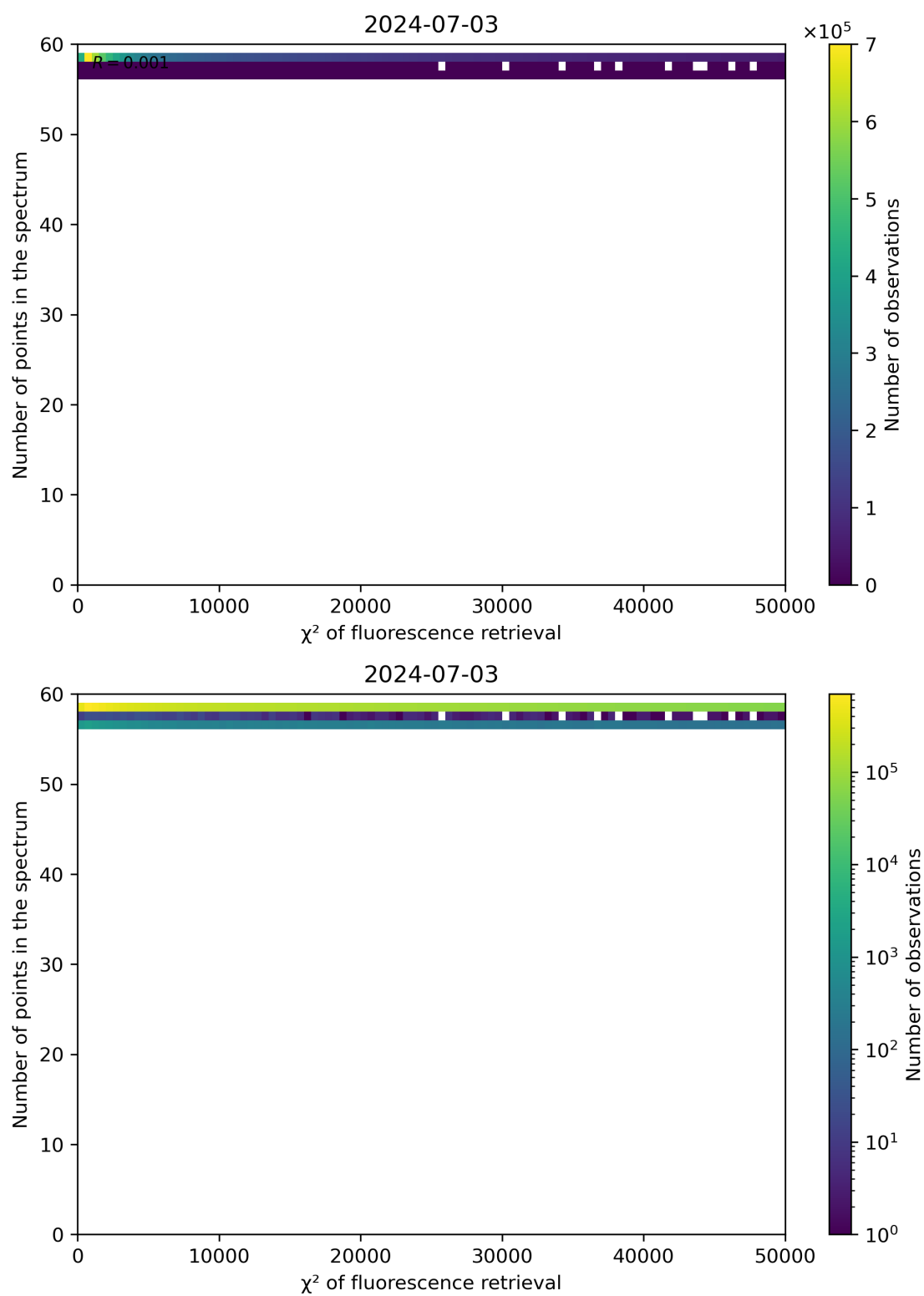
Figure 68: Scatter density plot of " \chi^2 of fluorescence retrieval" against "Number of points in the spectrum" for 2024-07-02 to 2024-07-04.
