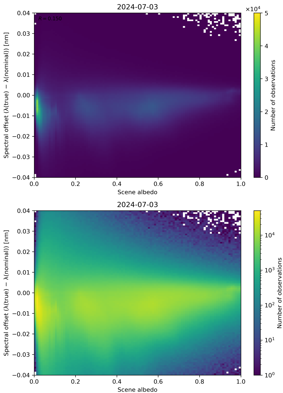
Figure 107: Scatter density plot of “Scene albedo” against “Spectral offset ( \lambda(\text{true}) - \lambda(\text{nominal}) )” for 2024-07-02 to 2024-07-04.
