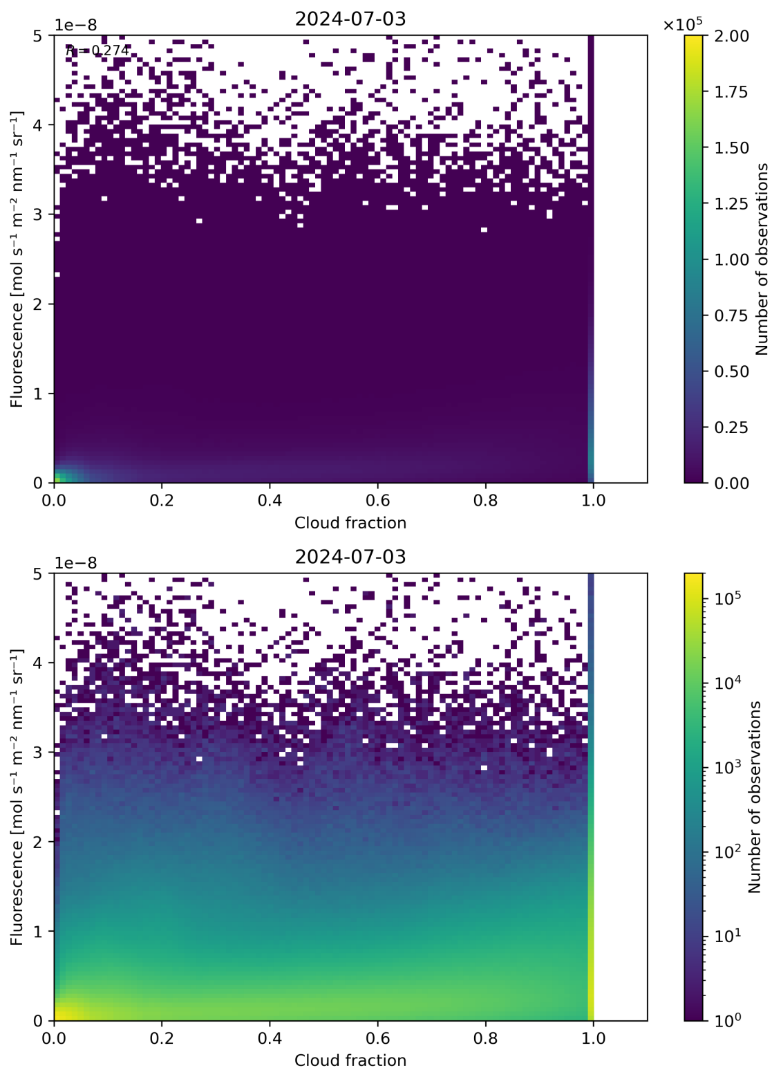
Figure 72: Scatter density plot of “Cloud fraction” against “Fluorescence” for 2024-07-02 to 2024-07-04.
