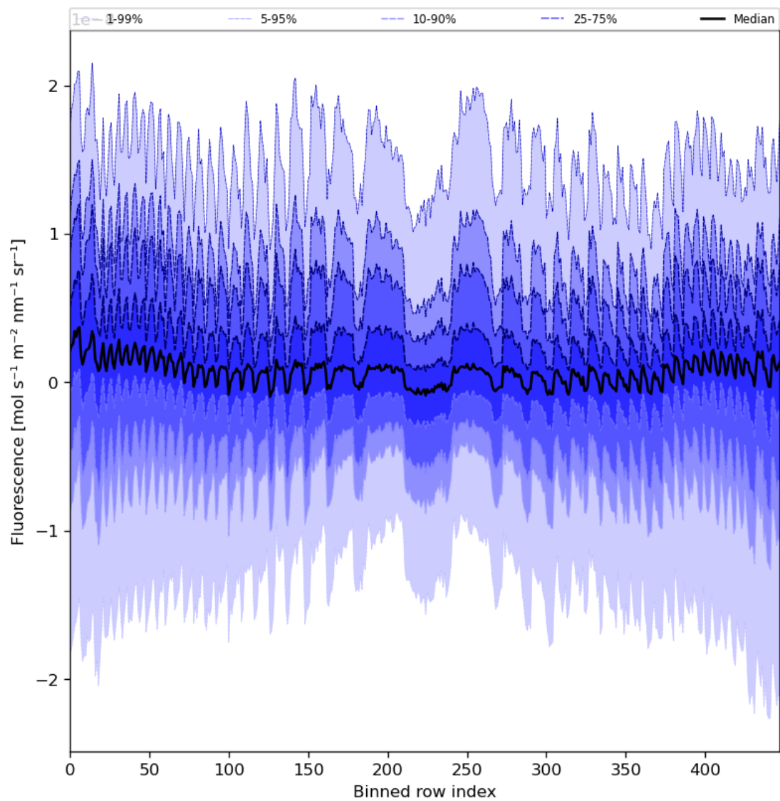
Figure 57: Along track statistics of “Fluorescence” for 2024-07-02 to 2024-07-04
