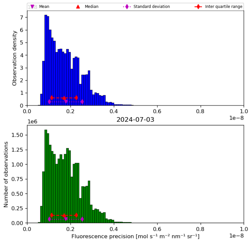
Figure 41: Histogram of “Fluorescence precision” for 2024-07-02 to 2024-07-04
