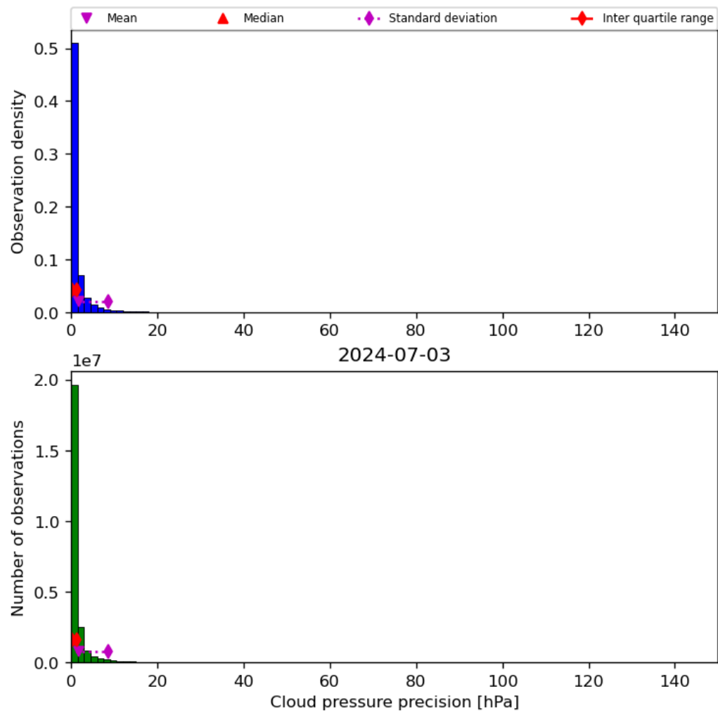
Figure 31: Histogram of “Cloud pressure precision” for 2024-07-02 to 2024-07-04
