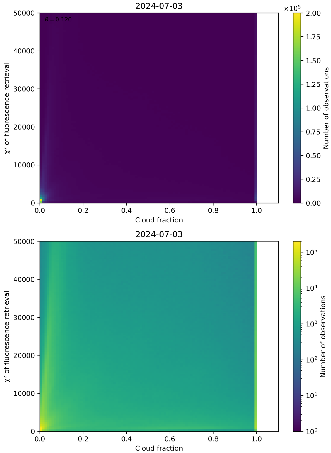
Figure 71: Scatter density plot of “Cloud fraction” against “ \chi^2 of fluorescence retrieval” for 2024-07-02 to 2024-07-04.
