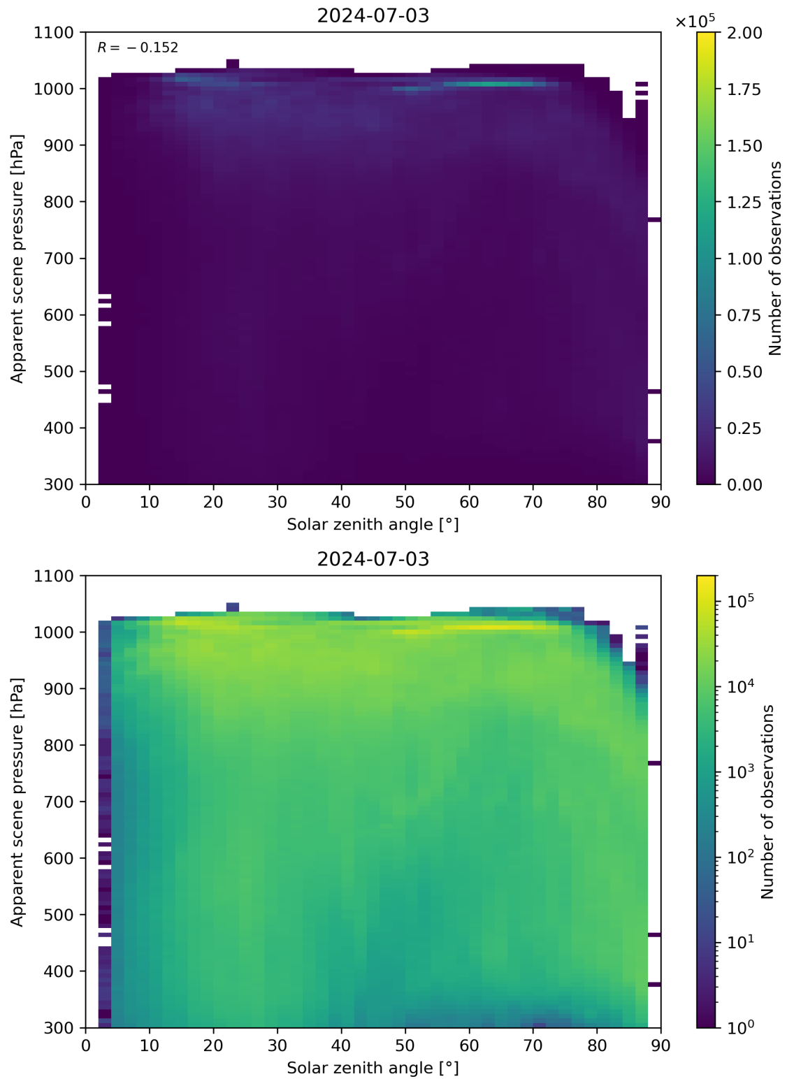
Figure 108: Scatter density plot of “Solar zenith angle” against “Apparent scene pressure” for 2024-07-02 to 2024-07-04.
