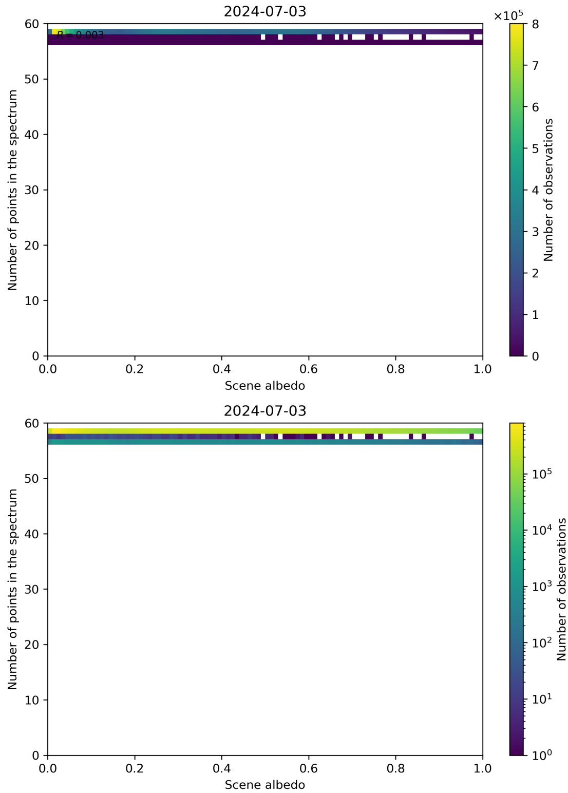
Figure 106: Scatter density plot of “Scene albedo” against “Number of points in the spectrum” for 2024-07-02 to 2024-07-04.
