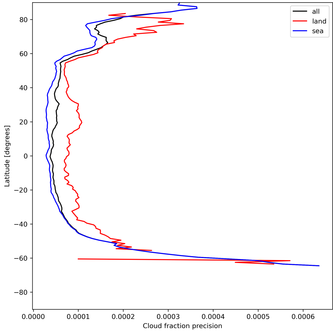
Figure 16: Zonal average of “Cloud fraction precision” for 2024-07-02 to 2024-07-04.
