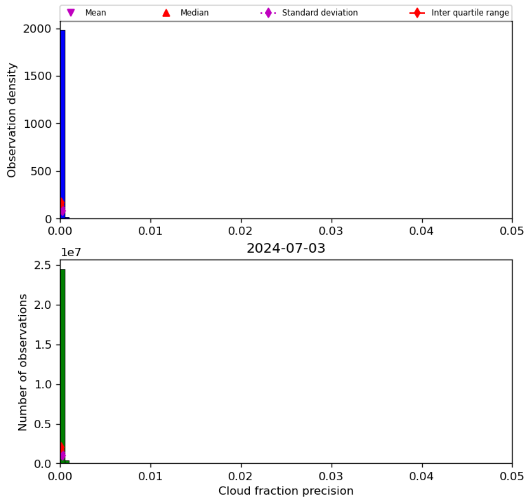
Figure 33: Histogram of “Cloud fraction precision” for 2024-07-02 to 2024-07-04
