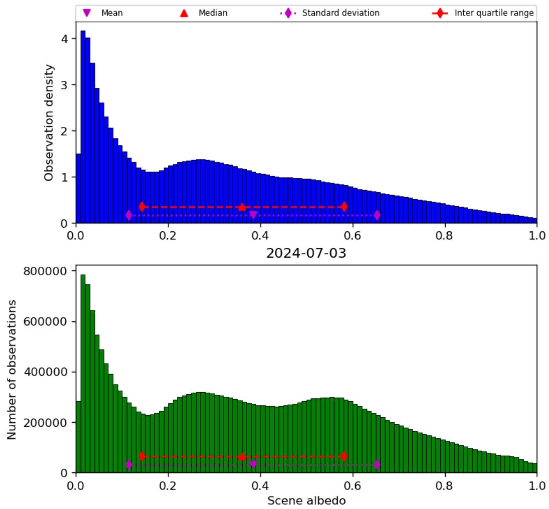
Figure 34: Histogram of “Scene albedo” for 2024-07-02 to 2024-07-04
