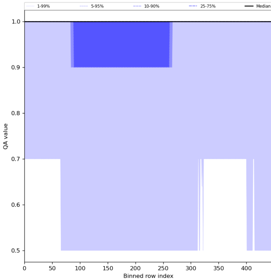
Figure 46: Along track statistics of “QA value” for 2024-07-02 to 2024-07-04
