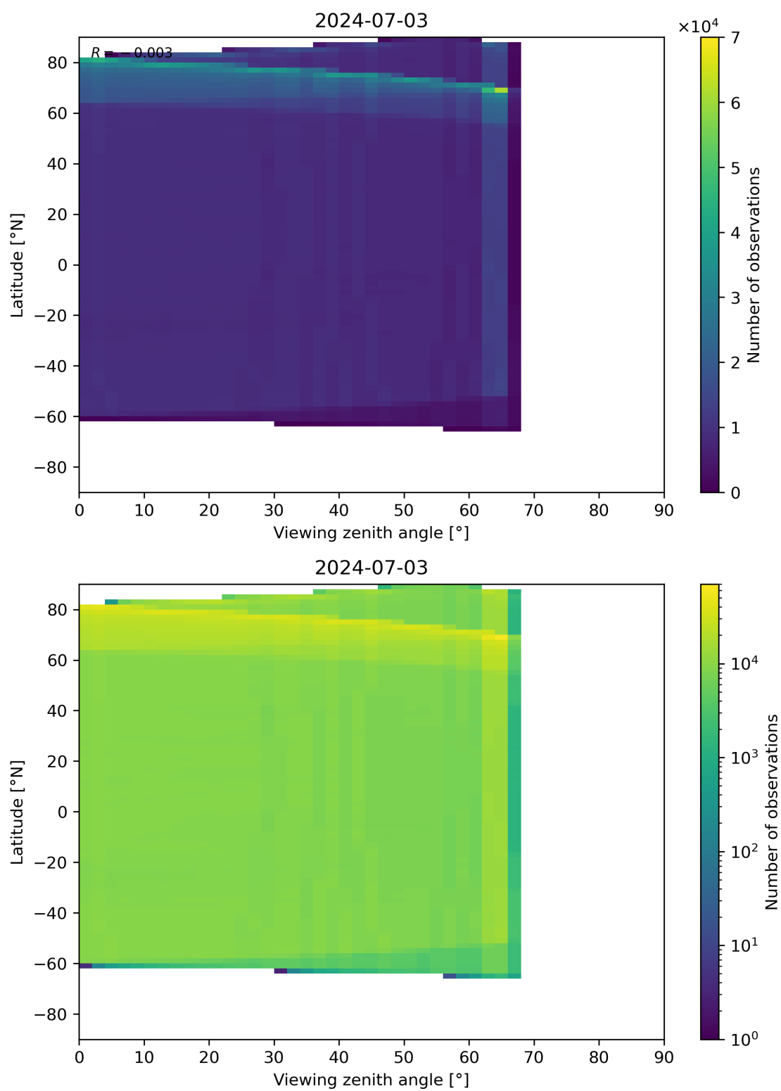
Figure 123: Scatter density plot of “Viewing zenith angle” against “Latitude” for 2024-07-02 to 2024-07-04.
