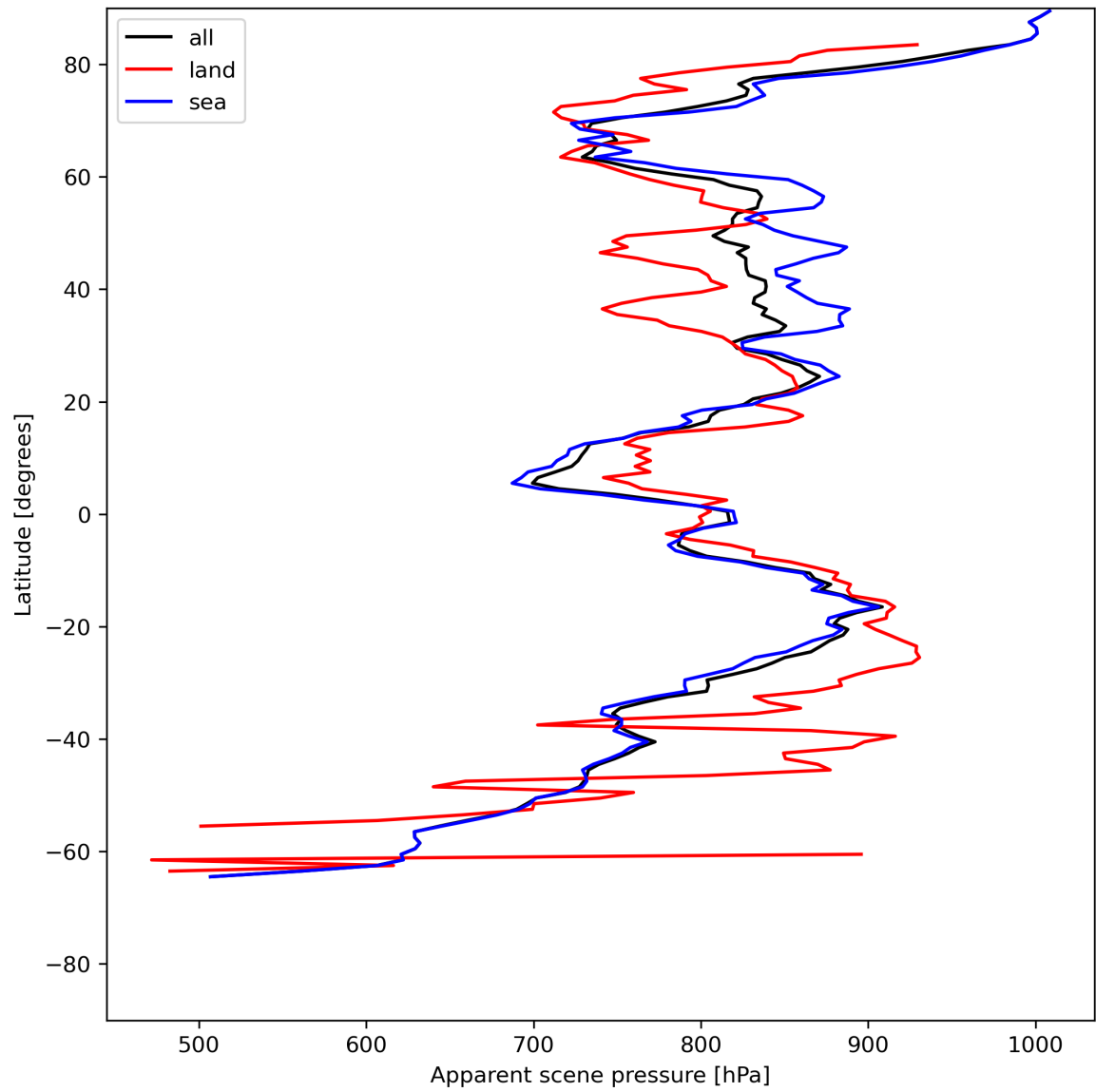
Figure 19: Zonal average of “Apparent scene pressure” for 2024-07-02 to 2024-07-04.
