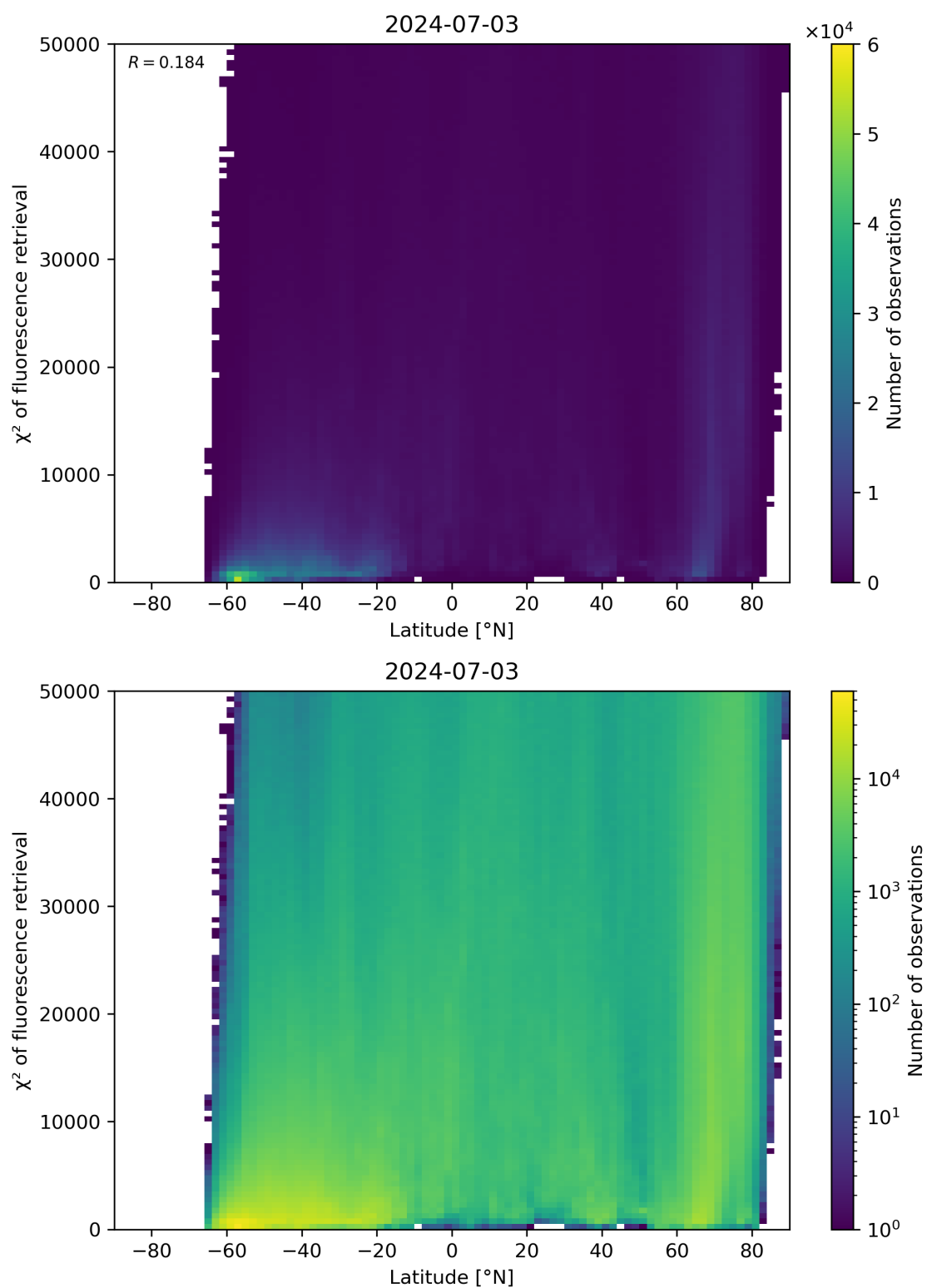
Figure 89: Scatter density plot of “Latitude” against “ \chi^2 of fluorescence retrieval” for 2024-07-02 to 2024-07-04.
