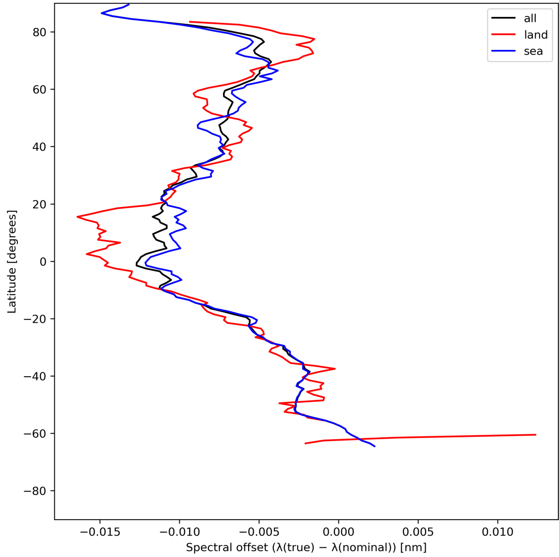
Figure 28: Zonal average of “Spectral offset ( \lambda(\text{true}) - \lambda(\text{nominal}) )” for 2024-07-02 to 2024-07-04.
