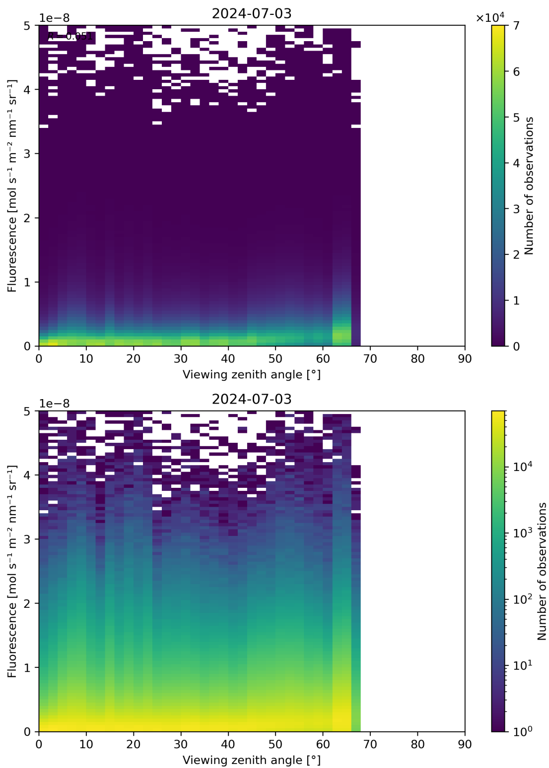
Figure 122: Scatter density plot of “Viewing zenith angle” against “Fluorescence” for 2024-07-02 to 2024-07-04.
