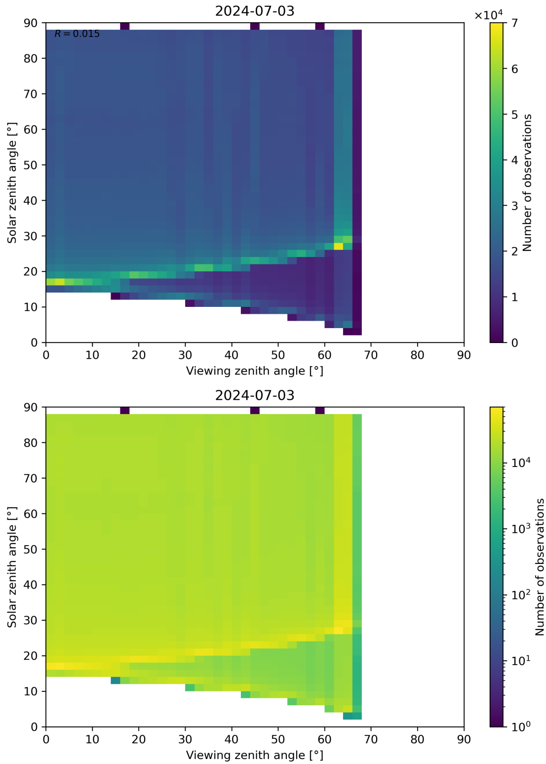
Figure 127: Scatter density plot of “Viewing zenith angle” against “Solar zenith angle” for 2024-07-02 to 2024-07-04.
