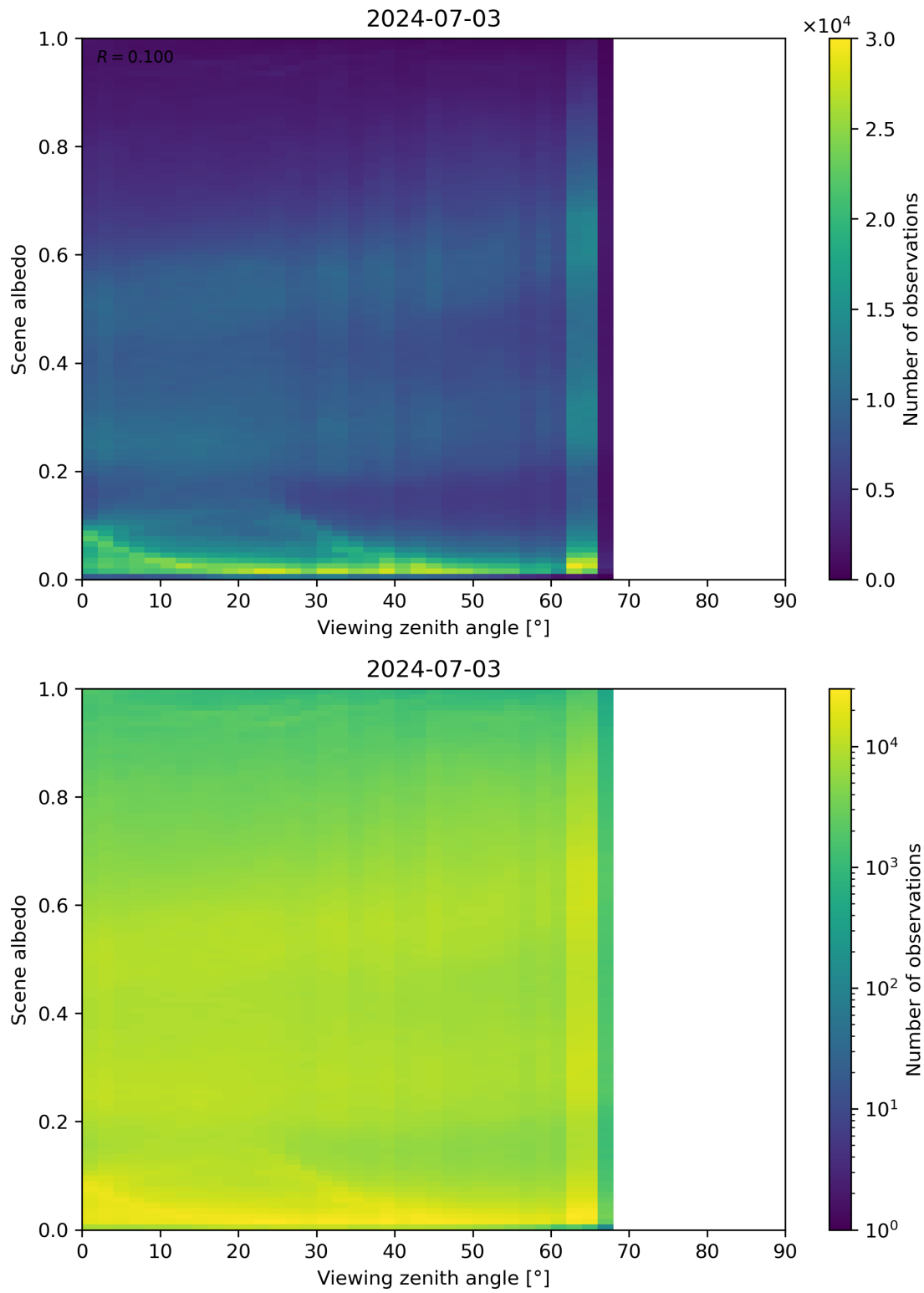
Figure 126: Scatter density plot of “Viewing zenith angle” against “Scene albedo” for 2024-07-02 to 2024-07-04.
