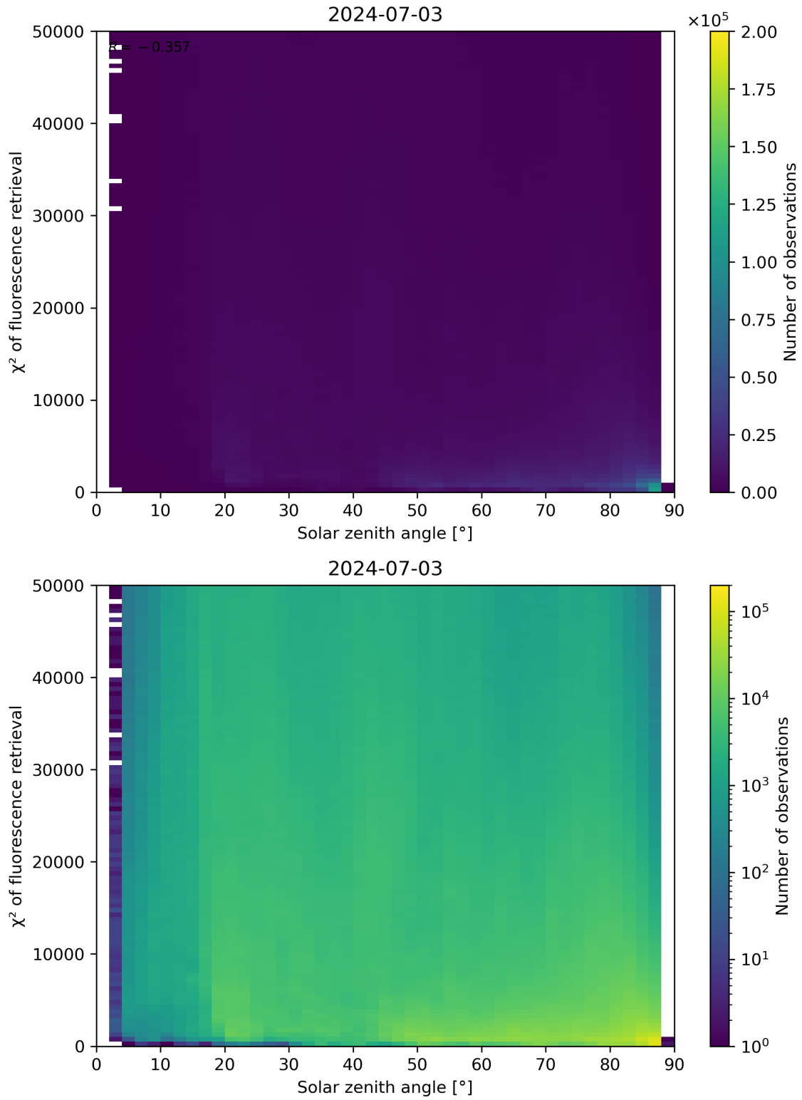
Figure 109: Scatter density plot of “Solar zenith angle” against “ \chi^2 of fluorescence retrieval” for 2024-07-02 to 2024-07-04.
