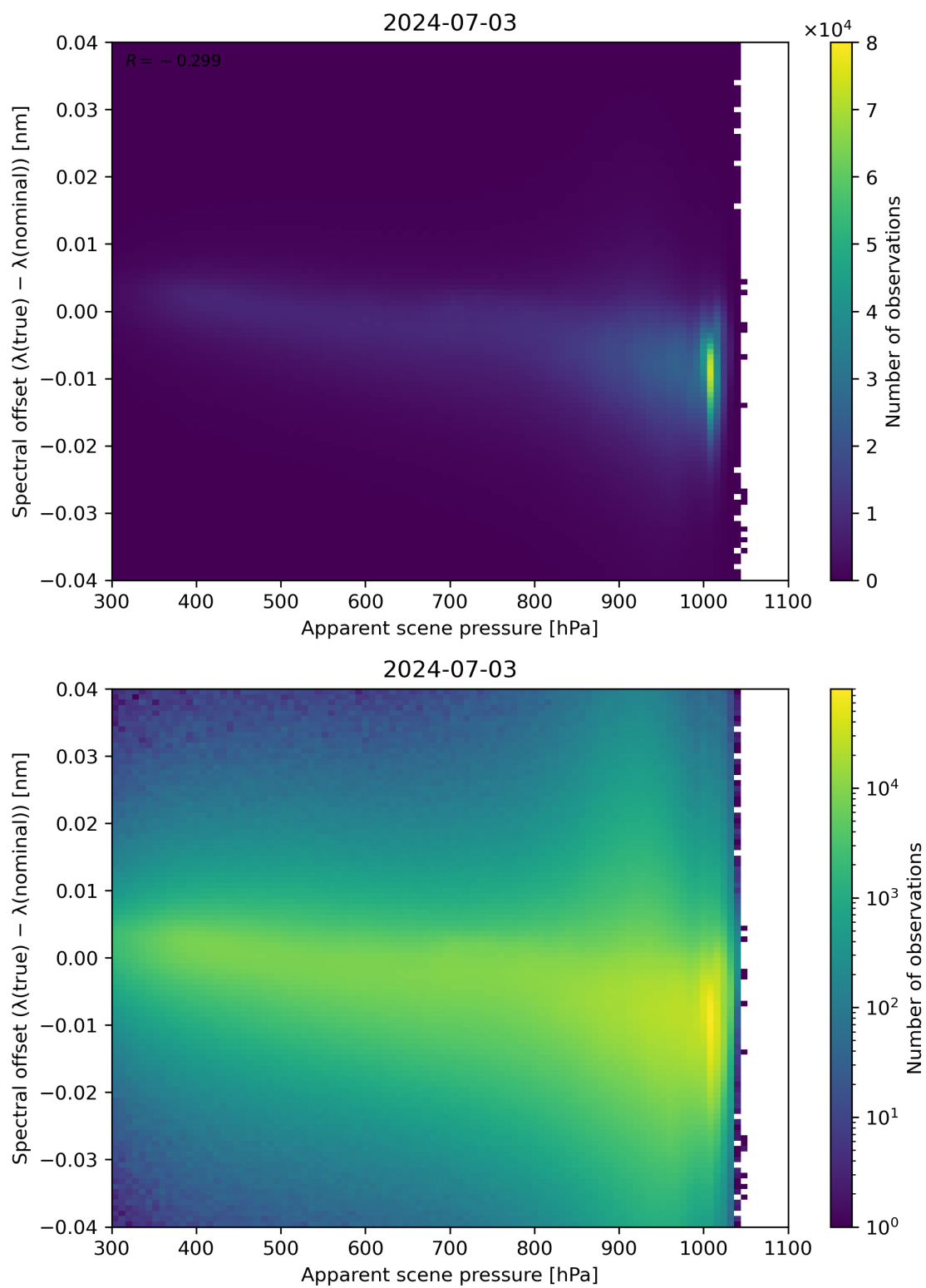
Figure 67: Scatter density plot of “Apparent scene pressure” against “Spectral offset ( \lambda(\text{true}) - \lambda(\text{nominal}) )” for 2024-07-02 to 2024-07-04.
