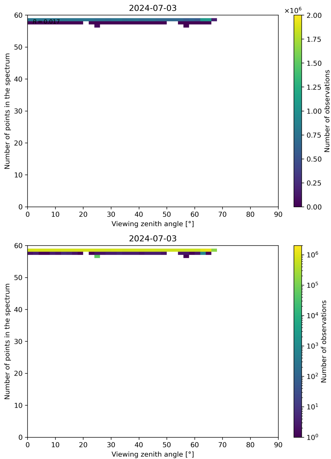
Figure 125: Scatter density plot of “Viewing zenith angle” against “Number of points in the spectrum” for 2024-07-02 to 2024-07-04.
