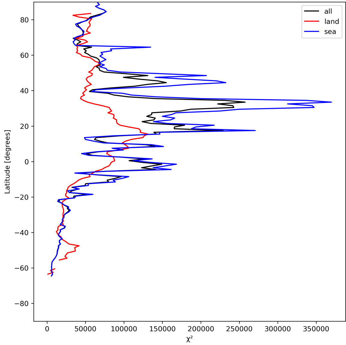
Figure 21: Zonal average of “ \chi^2 ” for 2024-07-02 to 2024-07-04.
