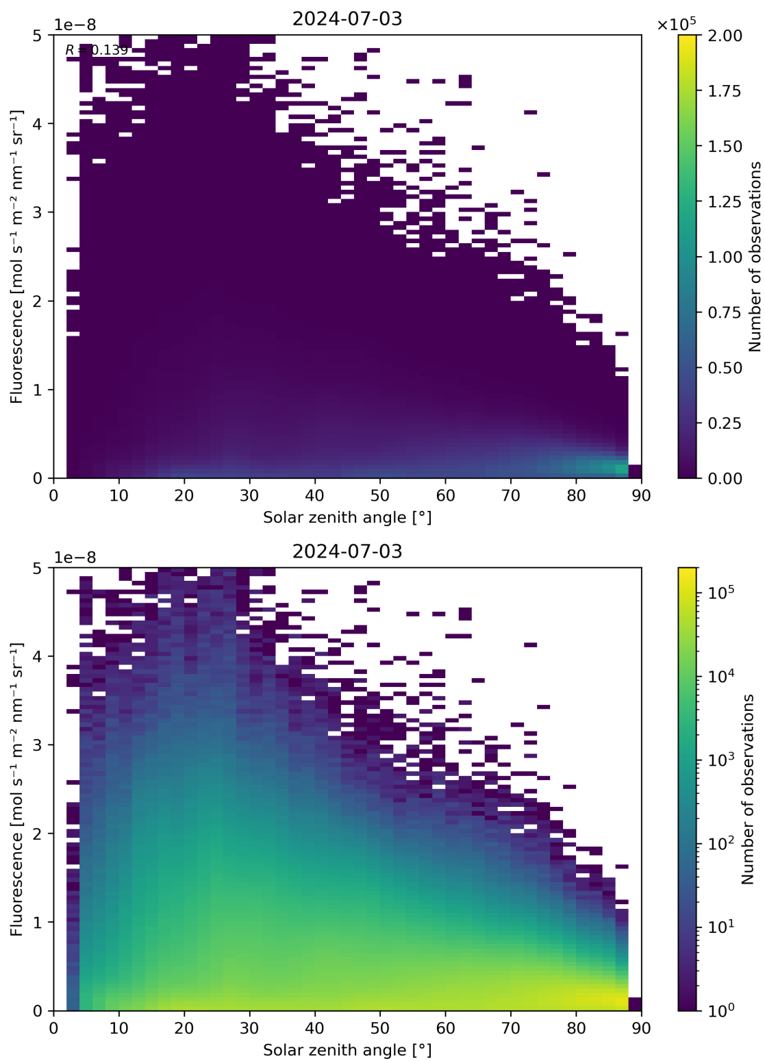
Figure 112: Scatter density plot of “Solar zenith angle” against “Fluorescence” for 2024-07-02 to 2024-07-04.
