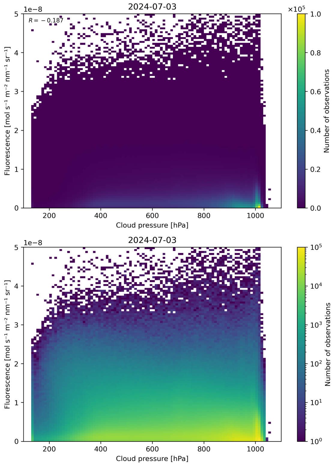
Figure 80: Scatter density plot of “Cloud pressure” against “Fluorescence” for 2024-07-02 to 2024-07-04.
