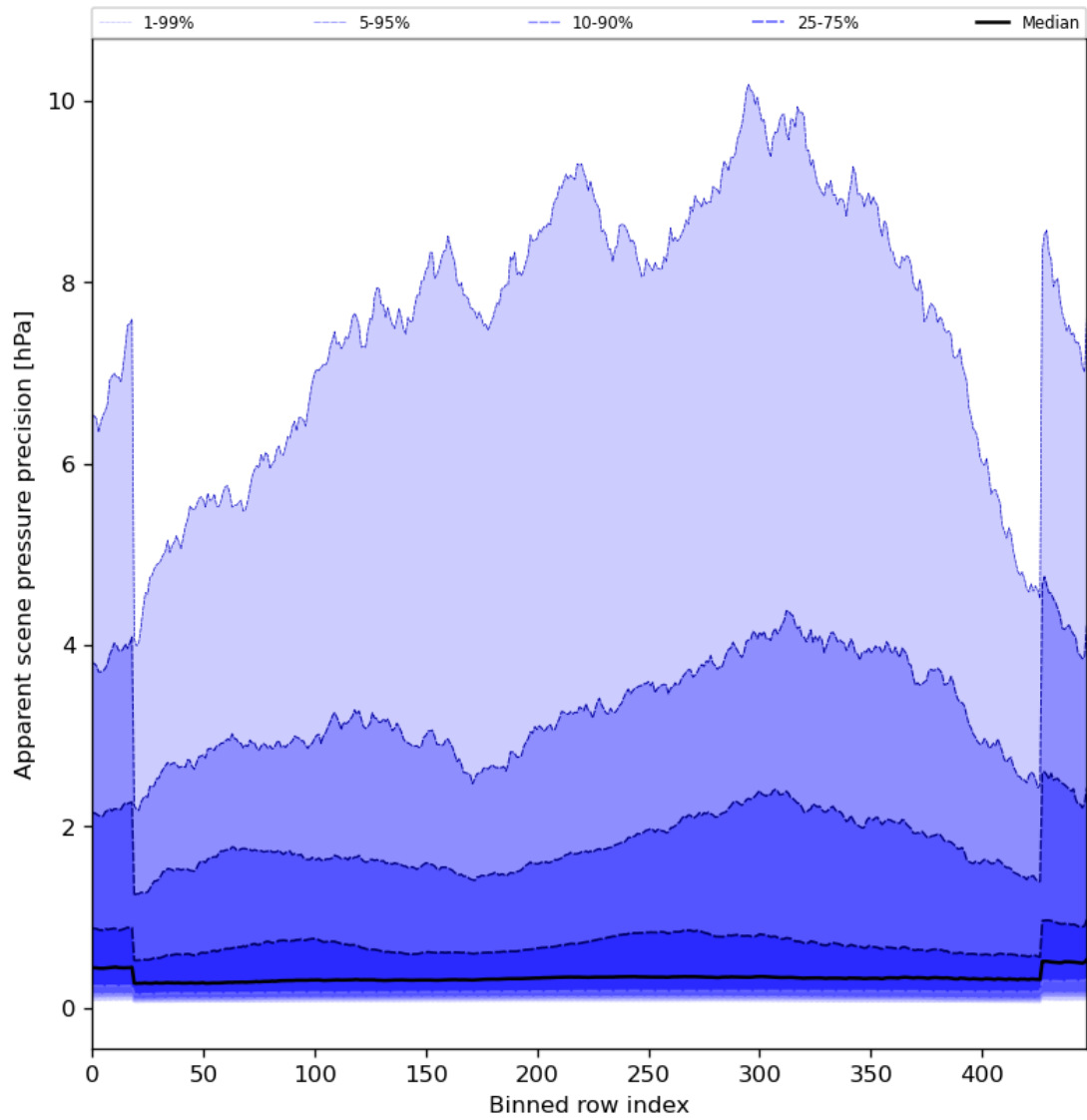
Figure 54: Along track statistics of “Apparent scene pressure precision” for 2024-07-02 to 2024-07-04
