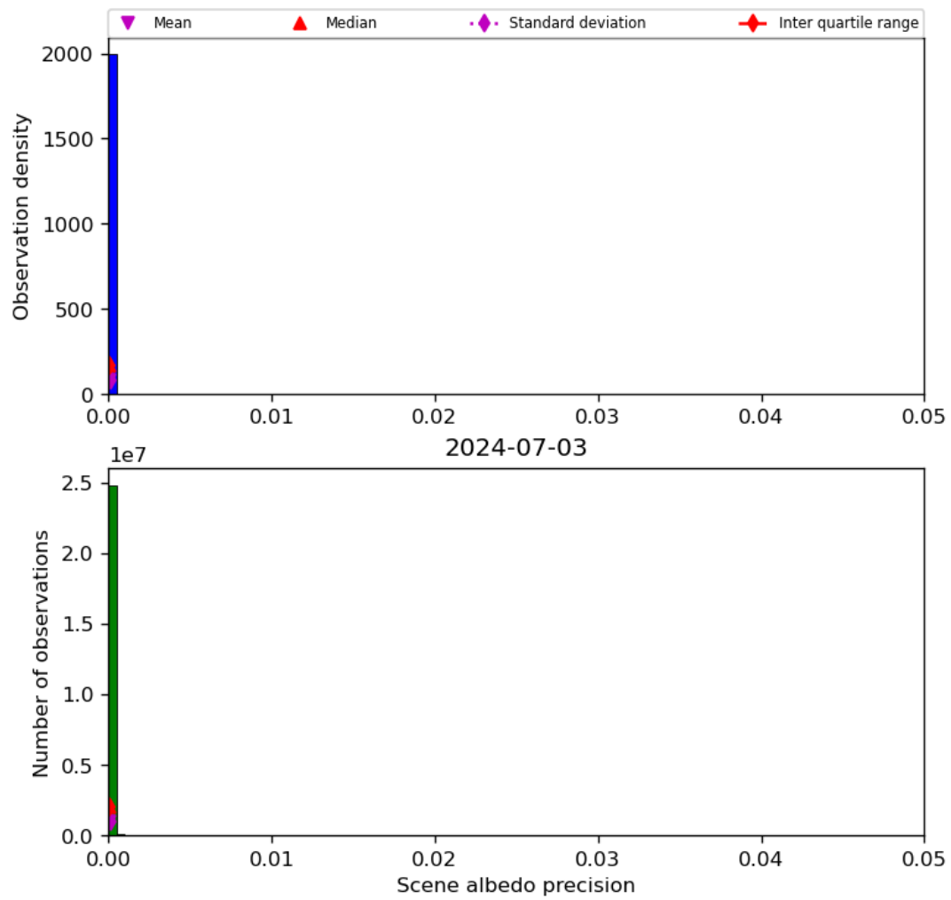
Figure 35: Histogram of “Scene albedo precision” for 2024-07-02 to 2024-07-04
