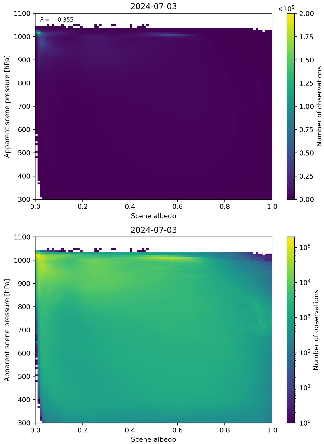
Figure 102: Scatter density plot of “Scene albedo” against “Apparent scene pressure” for 2024-07-02 to 2024-07-04.
