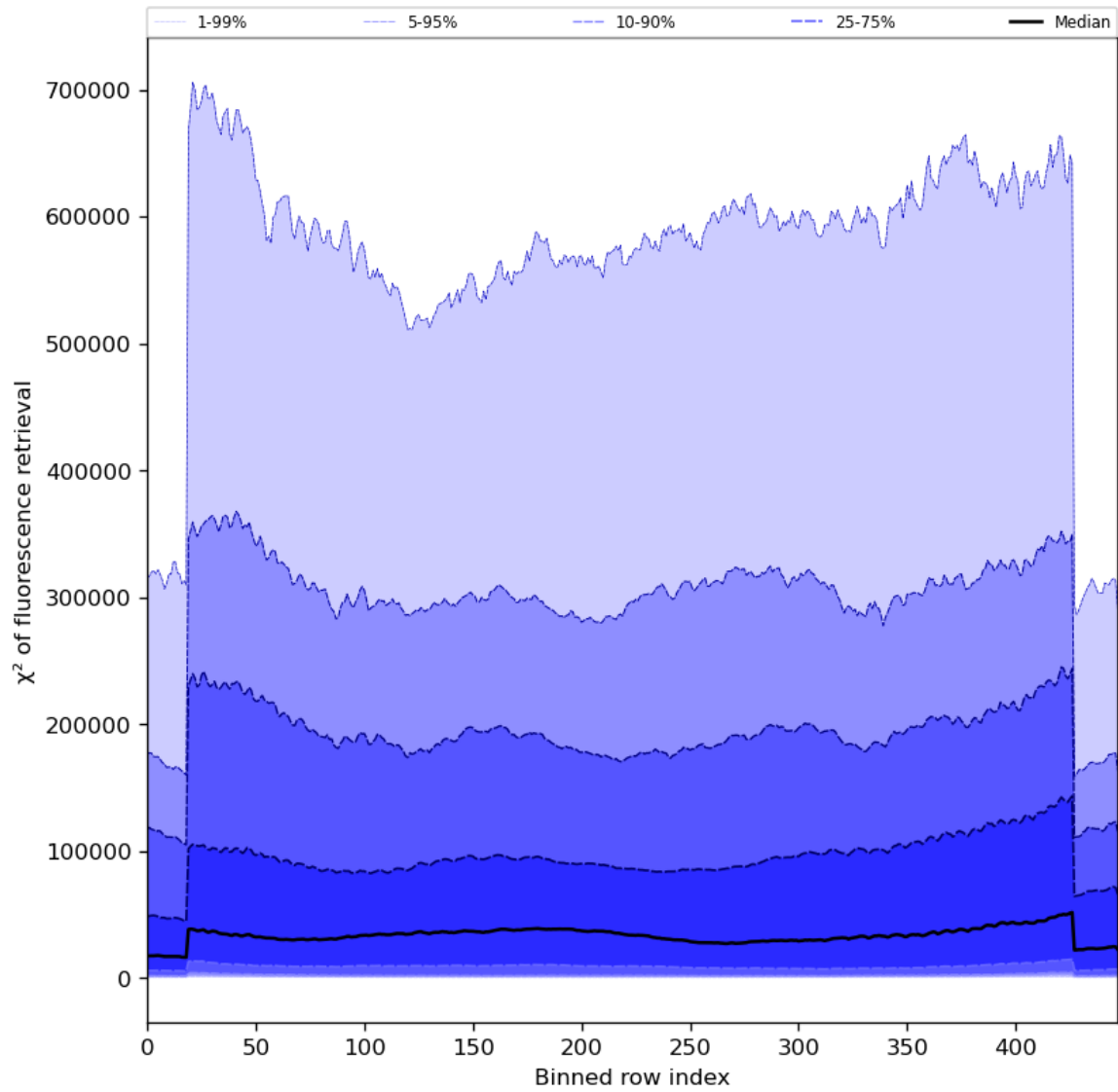
Figure 59: Along track statistics of “ \chi^2 of fluorescence retrieval” for 2024-07-02 to 2024-07-04
