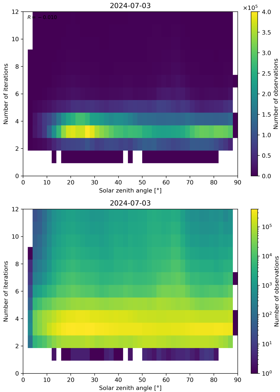
Figure 114: Scatter density plot of “Solar zenith angle” against “Number of iterations” for 2024-07-02 to 2024-07-04.
