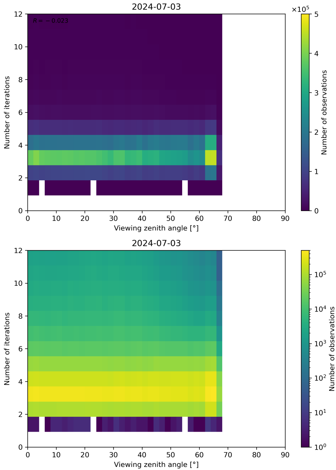
Figure 124: Scatter density plot of “Viewing zenith angle” against “Number of iterations” for 2024-07-02 to 2024-07-04.
