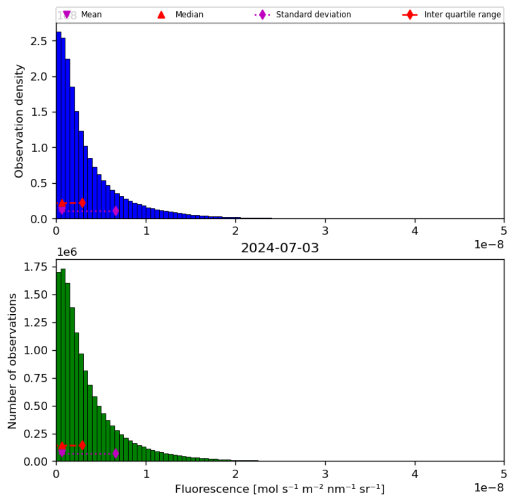
Figure 40: Histogram of “Fluorescence” for 2024-07-02 to 2024-07-04
