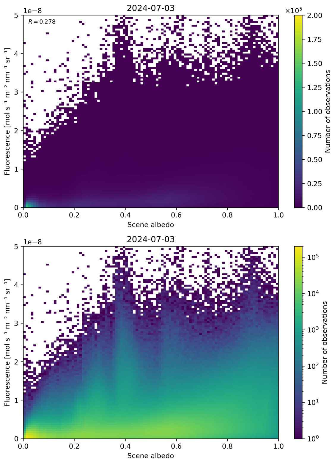
Figure 104: Scatter density plot of “Scene albedo” against “Fluorescence” for 2024-07-02 to 2024-07-04.
