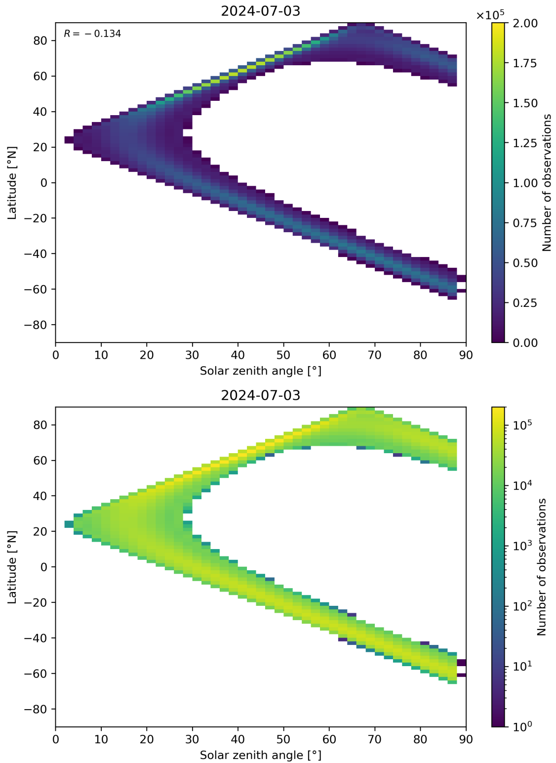
Figure 113: Scatter density plot of “Solar zenith angle” against “Latitude” for 2024-07-02 to 2024-07-04.
