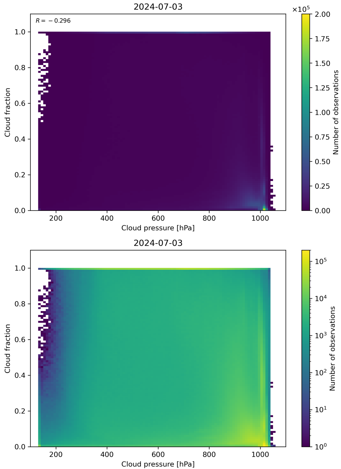
Figure 79: Scatter density plot of “Cloud pressure” against “Cloud fraction” for 2024-07-02 to 2024-07-04.
