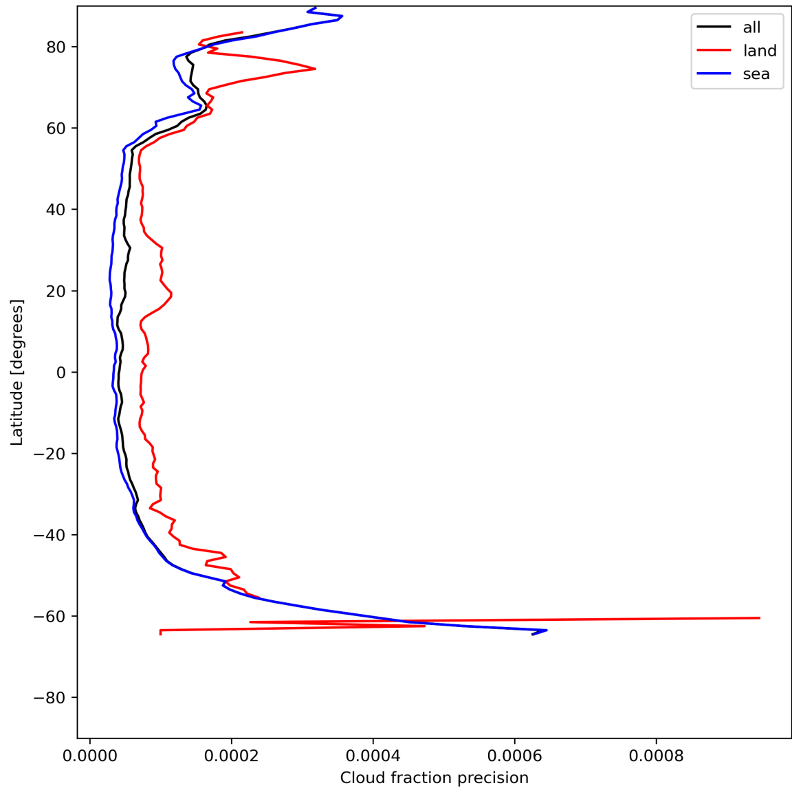
Figure 16: Zonal average of “Cloud fraction precision” for 2024-07-03 to 2024-07-05.
