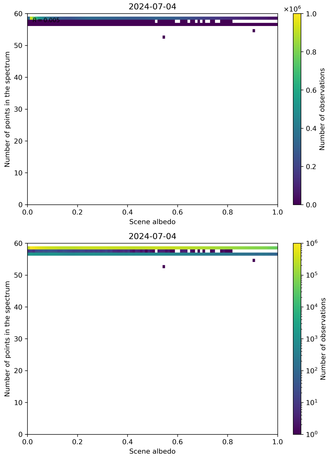
Figure 106: Scatter density plot of “Scene albedo” against “Number of points in the spectrum” for 2024-07-03 to 2024-07-05.
