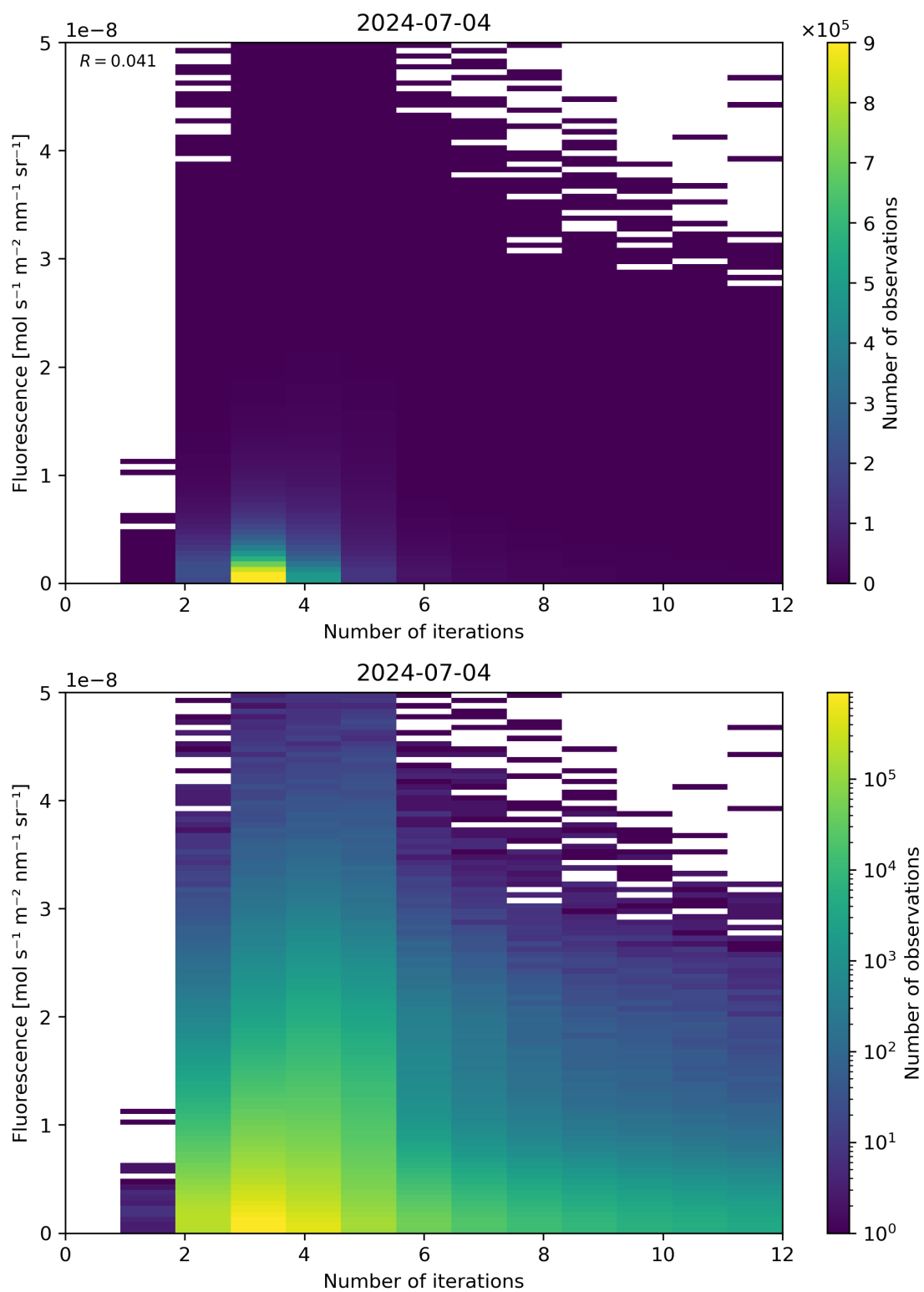
Figure 98: Scatter density plot of “Number of iterations” against “Fluorescence” for 2024-07-03 to 2024-07-05.
