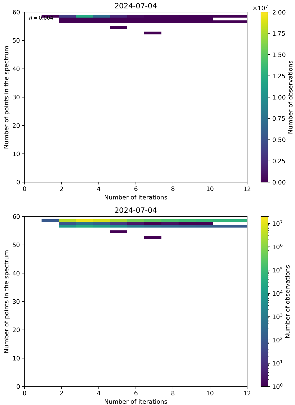
Figure 99: Scatter density plot of “Number of iterations” against “Number of points in the spectrum” for 2024-07-03 to 2024-07-05.
