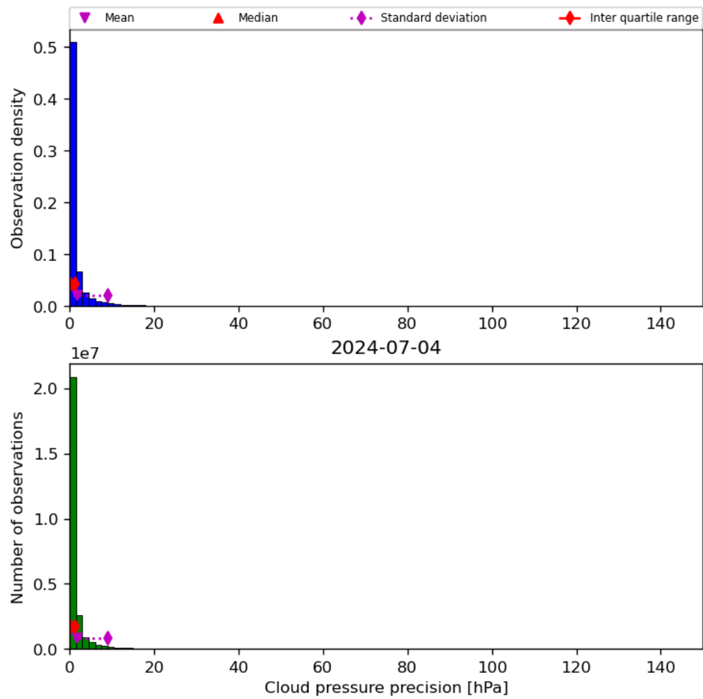
Figure 31: Histogram of “Cloud pressure precision” for 2024-07-03 to 2024-07-05
