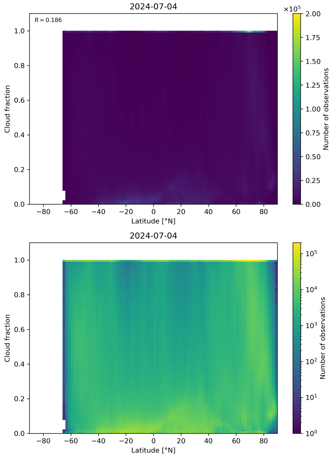
Figure 90: Scatter density plot of “Latitude” against “Cloud fraction” for 2024-07-03 to 2024-07-05.
