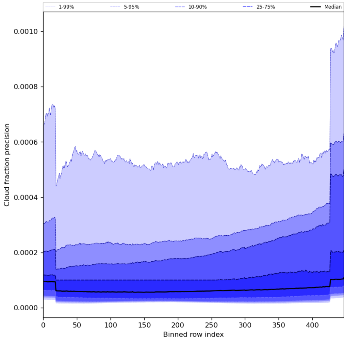
Figure 50: Along track statistics of “Cloud fraction precision” for 2024-07-03 to 2024-07-05
