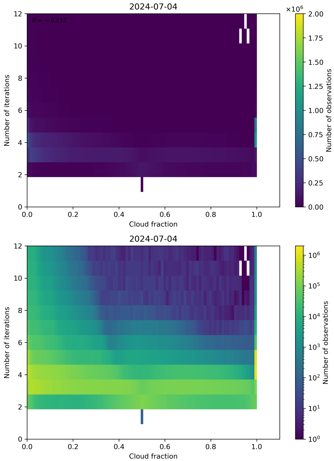
Figure 73: Scatter density plot of “Cloud fraction” against “Number of iterations” for 2024-07-03 to 2024-07-05.
