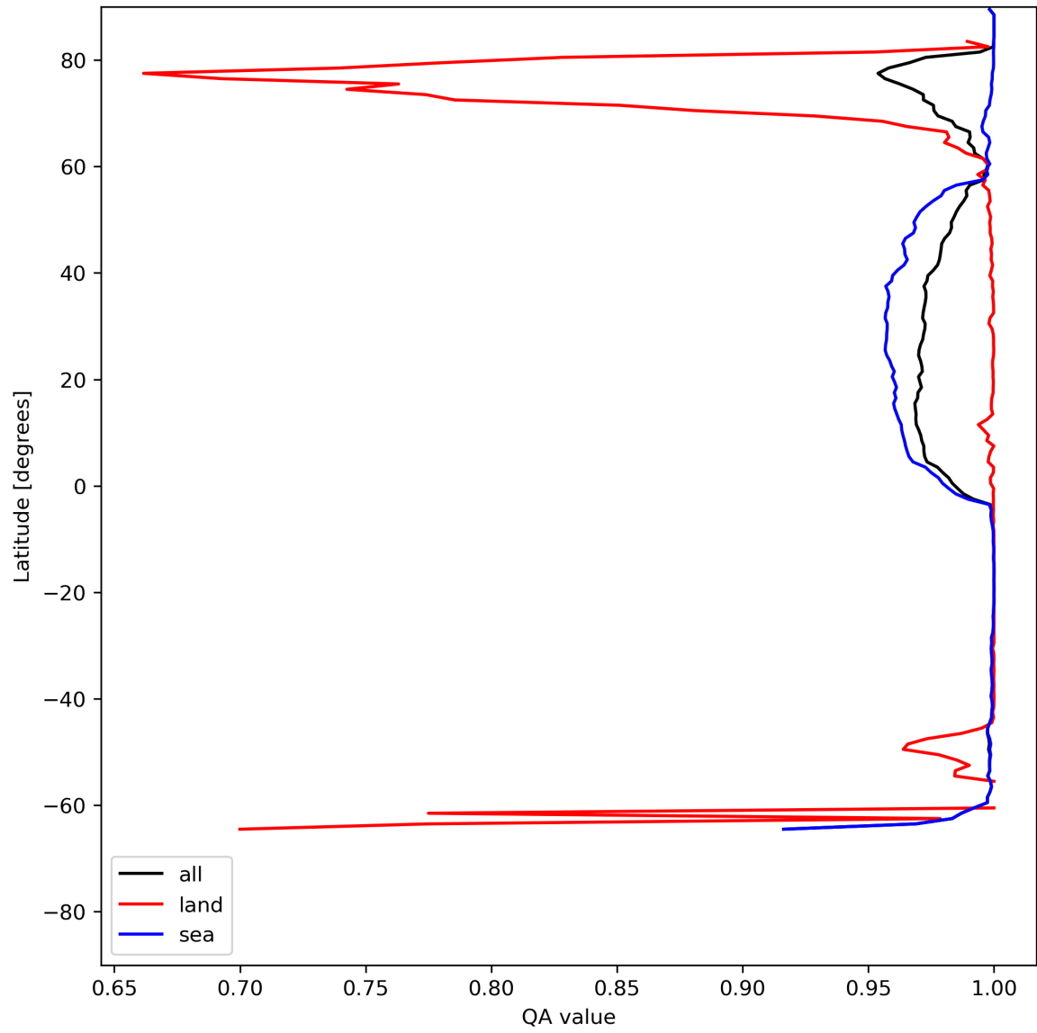
Figure 12: Zonal average of “QA value” for 2024-07-03 to 2024-07-05.
