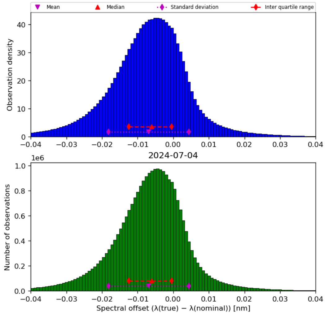
Figure 45: Histogram of “Spectral offset ( \lambda(\text{true}) - \lambda(\text{nominal}) )” for 2024-07-03 to 2024-07-05
