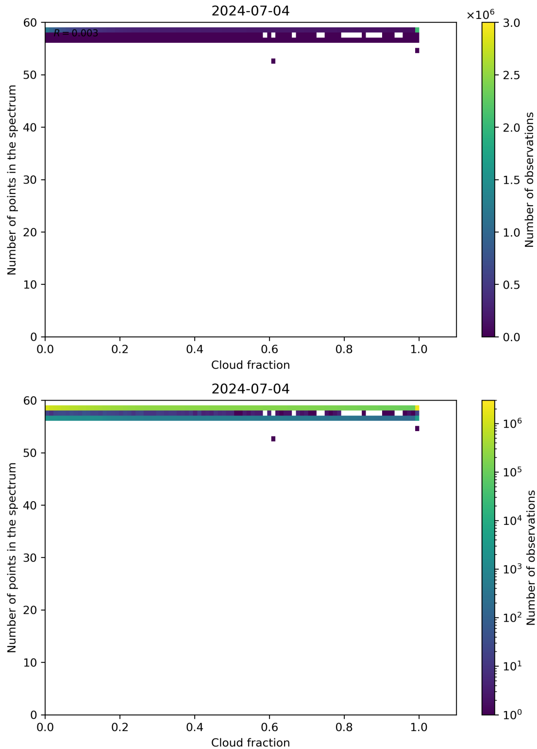
Figure 74: Scatter density plot of “Cloud fraction” against “Number of points in the spectrum” for 2024-07-03 to 2024-07-05.
