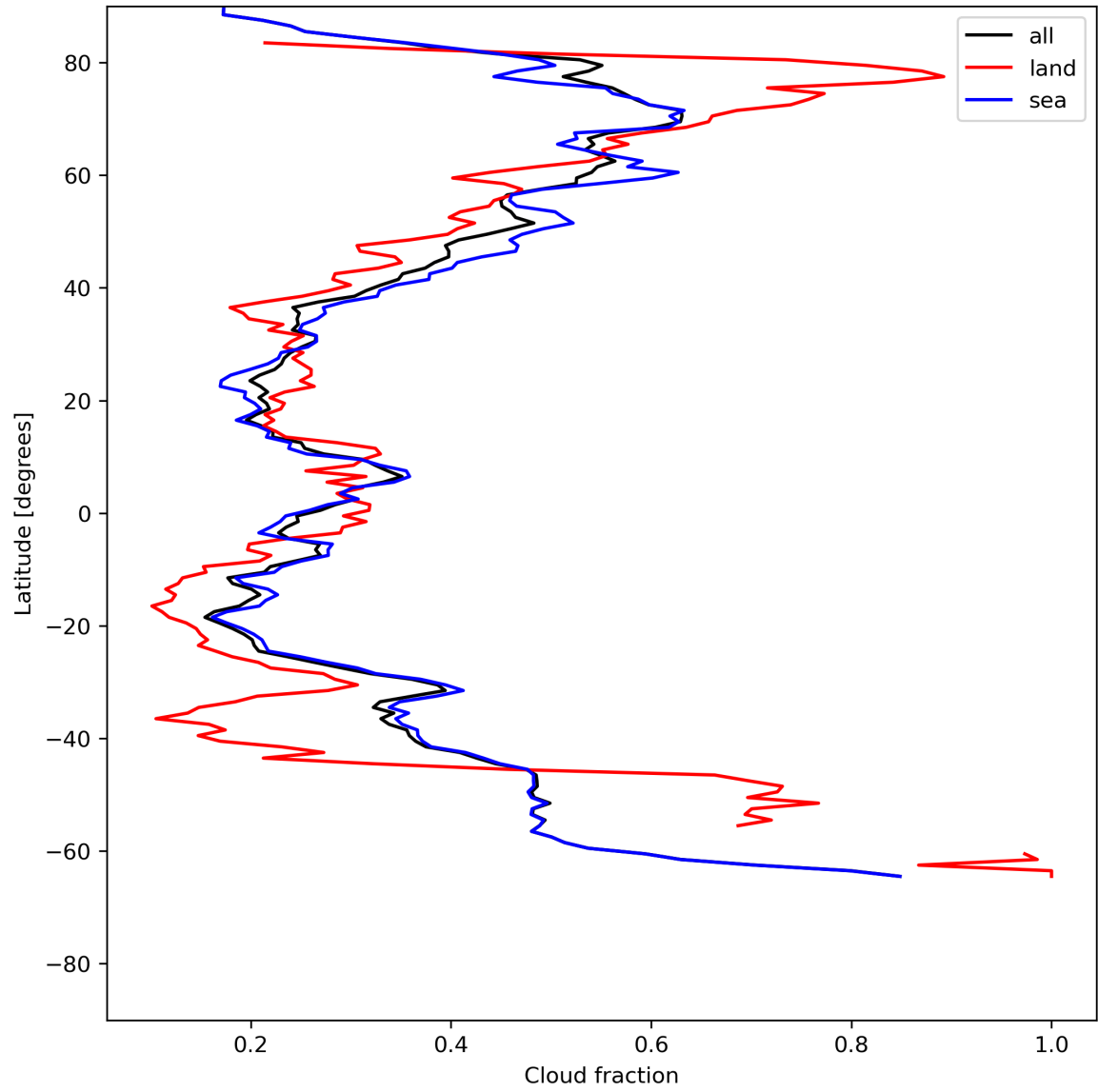
Figure 15: Zonal average of “Cloud fraction” for 2024-07-03 to 2024-07-05.
