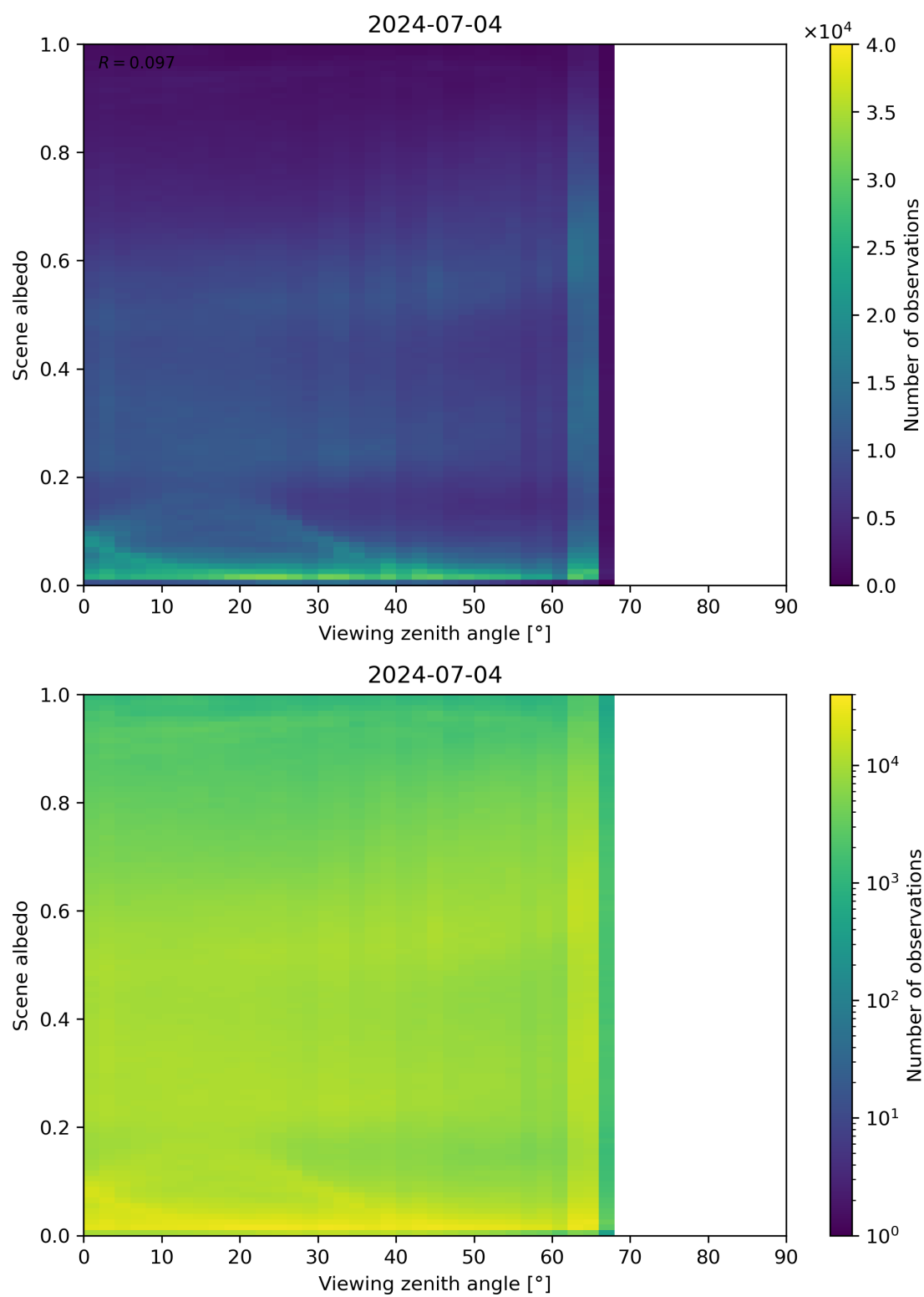
Figure 126: Scatter density plot of “Viewing zenith angle” against “Scene albedo” for 2024-07-03 to 2024-07-05.
