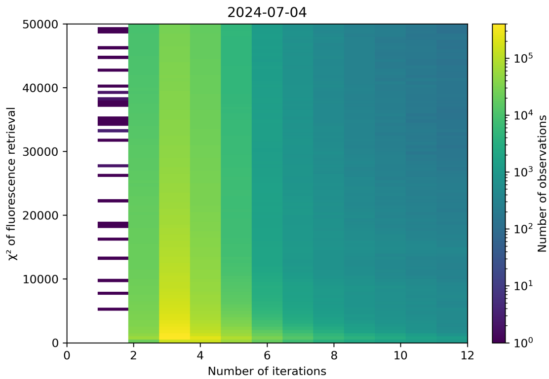
Figure 97: Scatter density plot of “Number of iterations” against “ \chi^2 of fluorescence retrieval” for 2024-07-03 to 2024-07-05.
