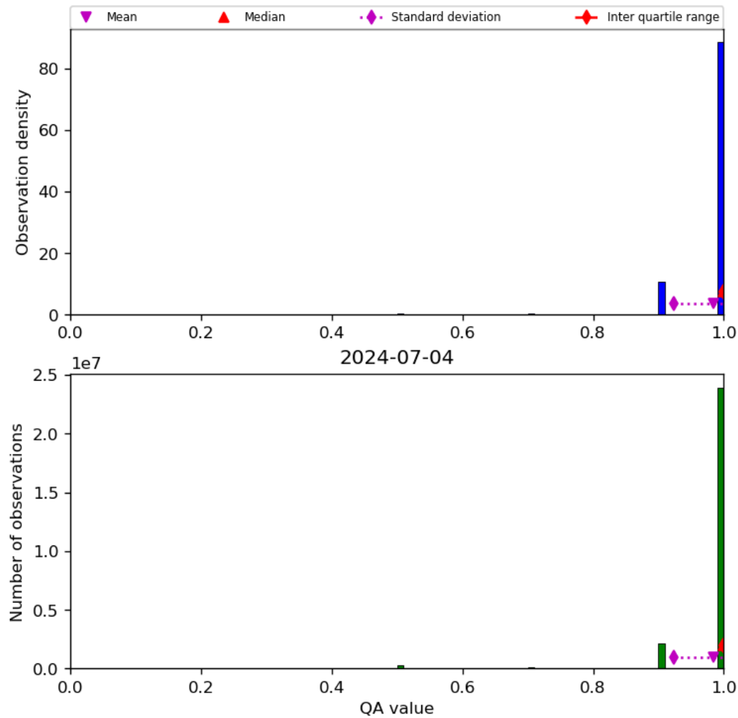
Figure 29: Histogram of “QA value” for 2024-07-03 to 2024-07-05
