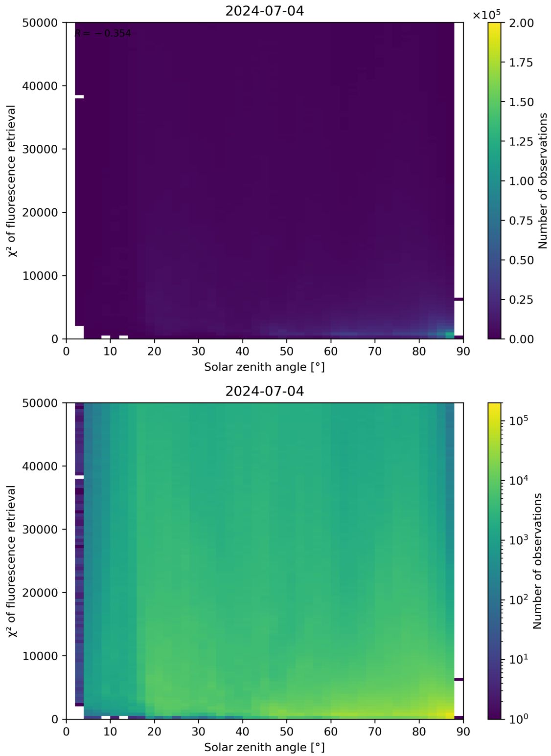
Figure 109: Scatter density plot of “Solar zenith angle” against “ \chi^2 of fluorescence retrieval” for 2024-07-03 to 2024-07-05.
