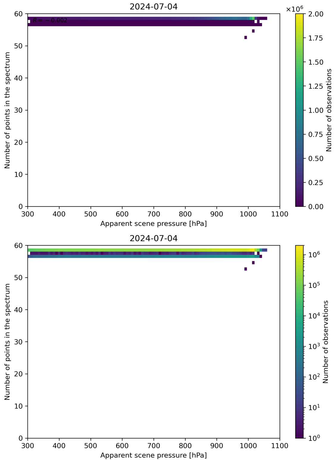
Figure 66: Scatter density plot of “Apparent scene pressure” against “Number of points in the spectrum” for 2024-07-03 to 2024-07-05.
