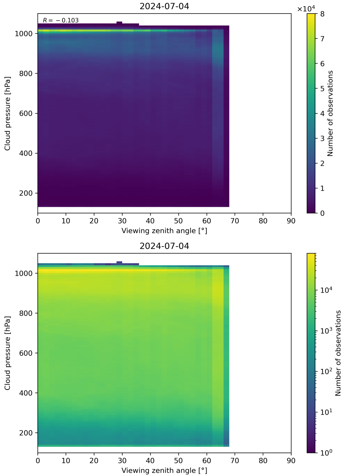
Figure 121: Scatter density plot of “Viewing zenith angle” against “Cloud pressure” for 2024-07-03 to 2024-07-05.
