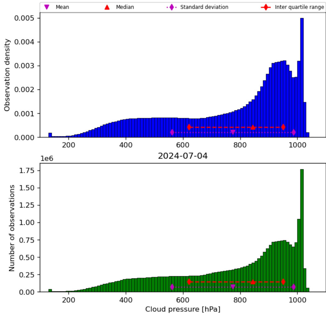
Figure 30: Histogram of “Cloud pressure” for 2024-07-03 to 2024-07-05
