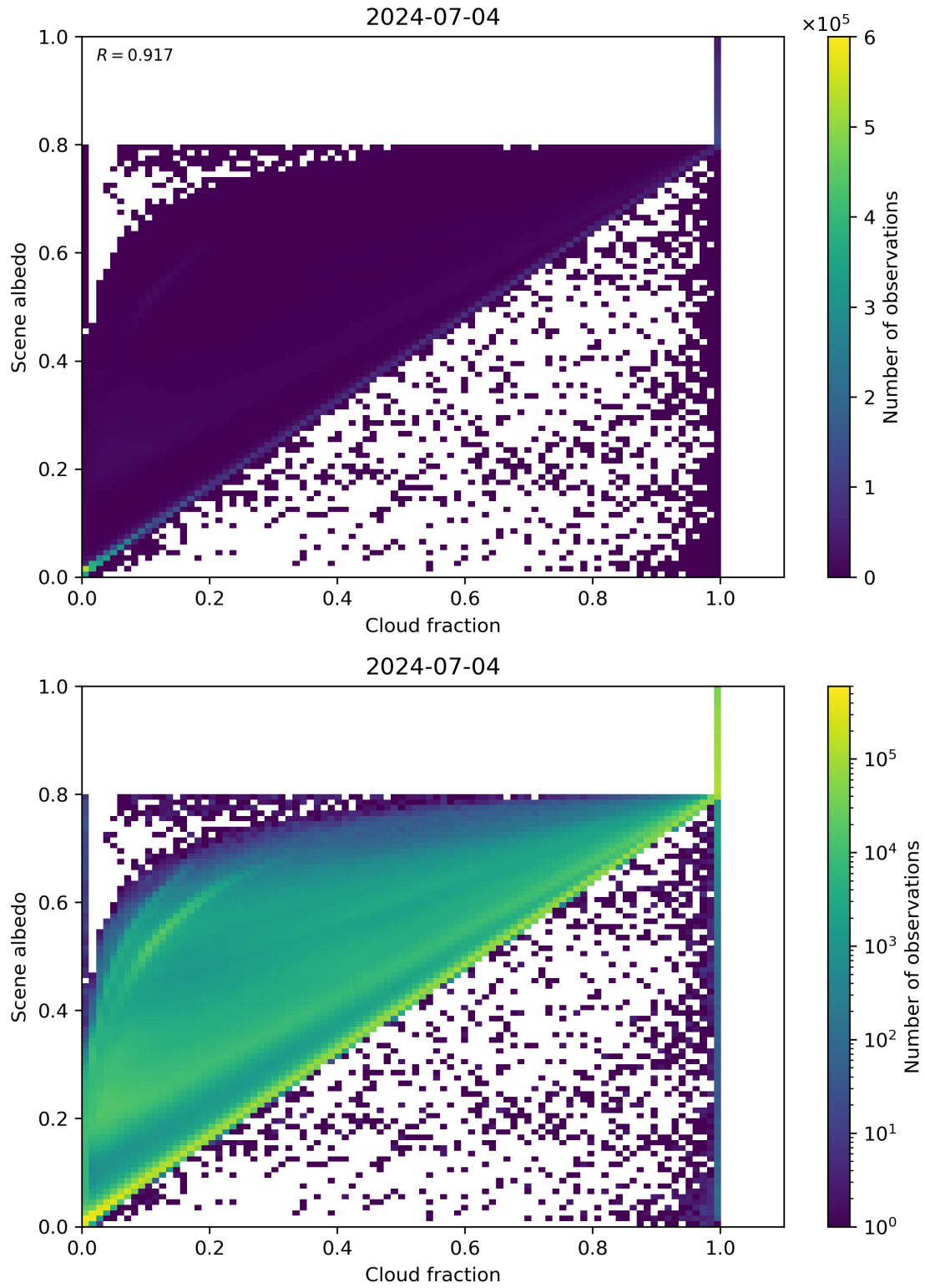
Figure 75: Scatter density plot of “Cloud fraction” against “Scene albedo” for 2024-07-03 to 2024-07-05.
