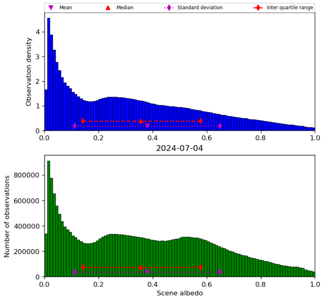
Figure 34: Histogram of “Scene albedo” for 2024-07-03 to 2024-07-05
