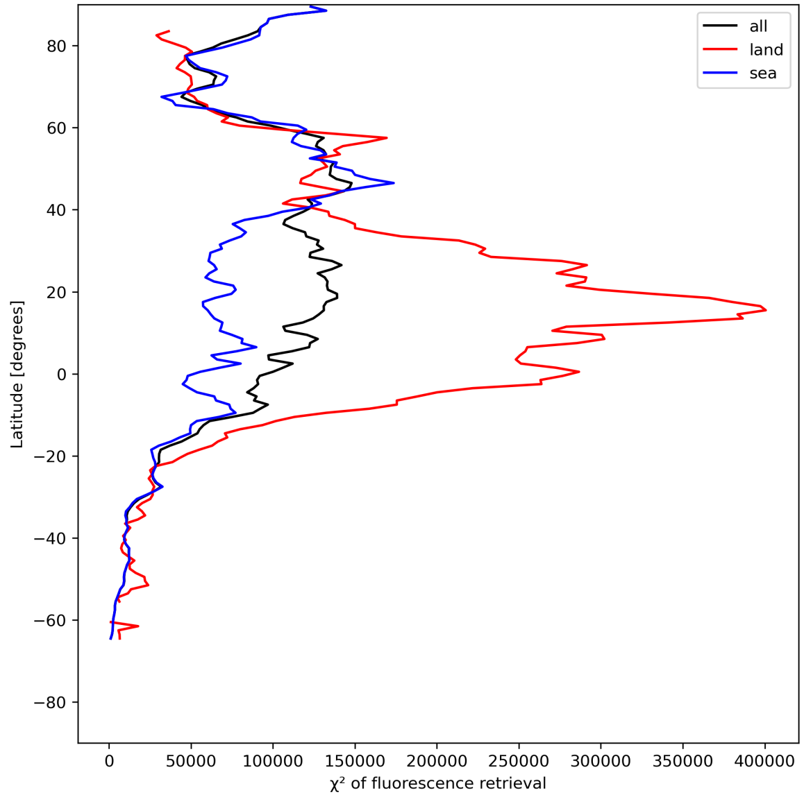
Figure 25: Zonal average of “ \chi^2 of fluorescence retrieval” for 2024-07-03 to 2024-07-05.
