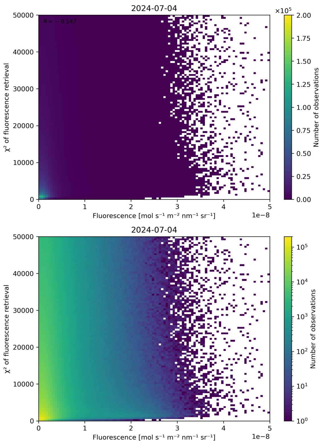
Figure 85: Scatter density plot of “Fluorescence” against “ \chi^2 of fluorescence retrieval” for 2024-07-03 to 2024-07-05.
