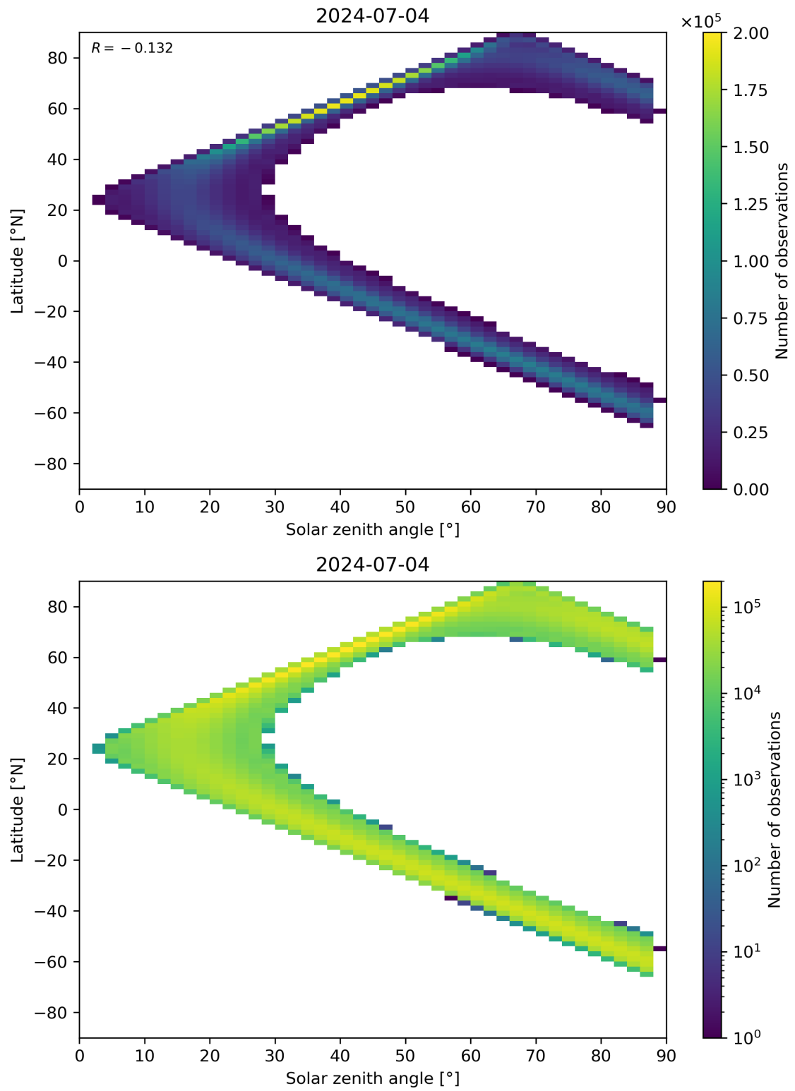
Figure 113: Scatter density plot of “Solar zenith angle” against “Latitude” for 2024-07-03 to 2024-07-05.
