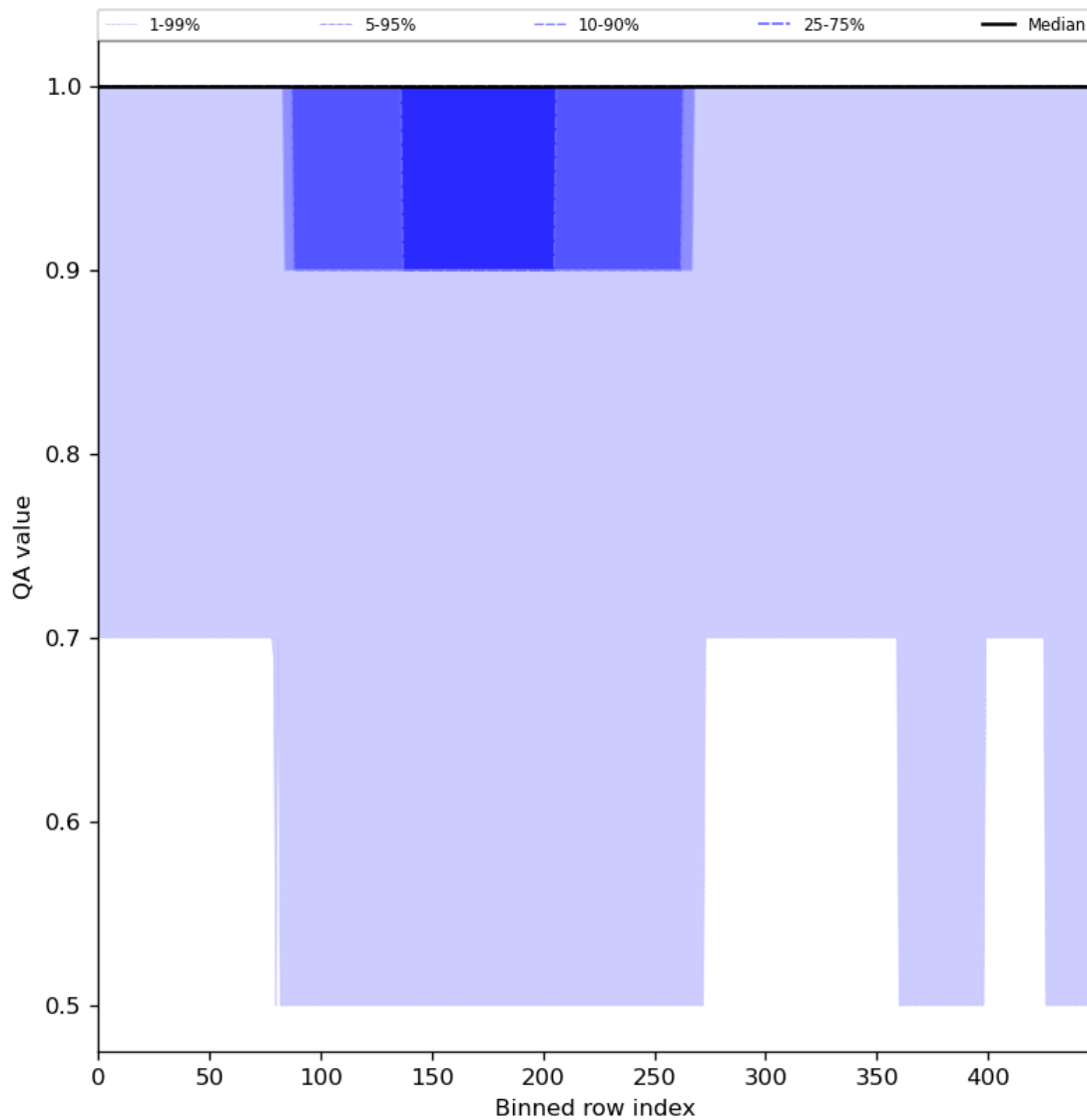
Figure 46: Along track statistics of “QA value” for 2024-07-03 to 2024-07-05
