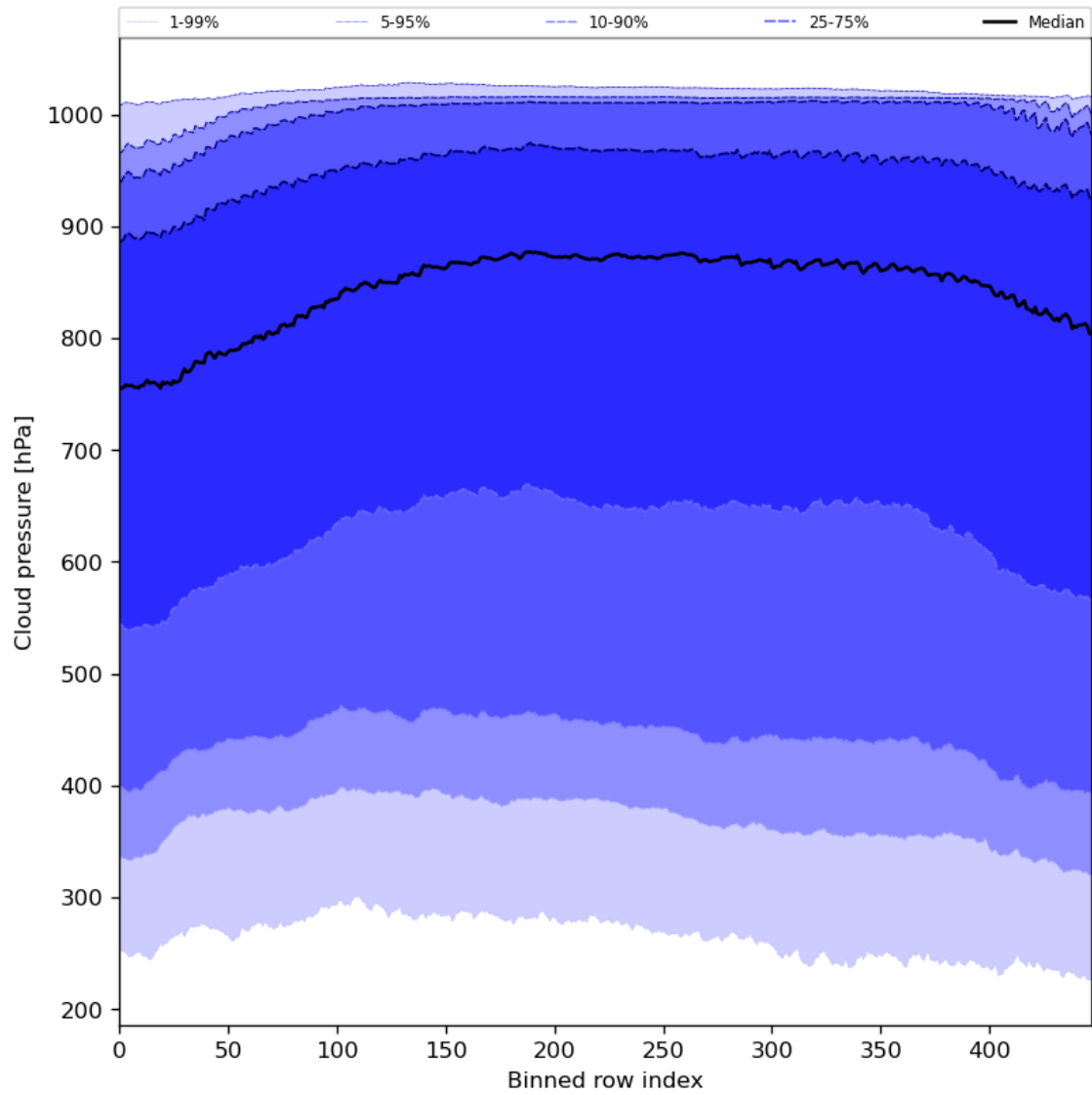
Figure 47: Along track statistics of “Cloud pressure” for 2024-07-03 to 2024-07-05
