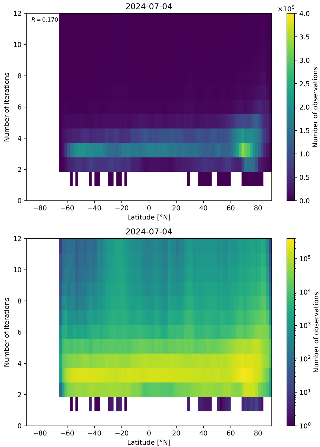
Figure 93: Scatter density plot of “Latitude” against “Number of iterations” for 2024-07-03 to 2024-07-05.
