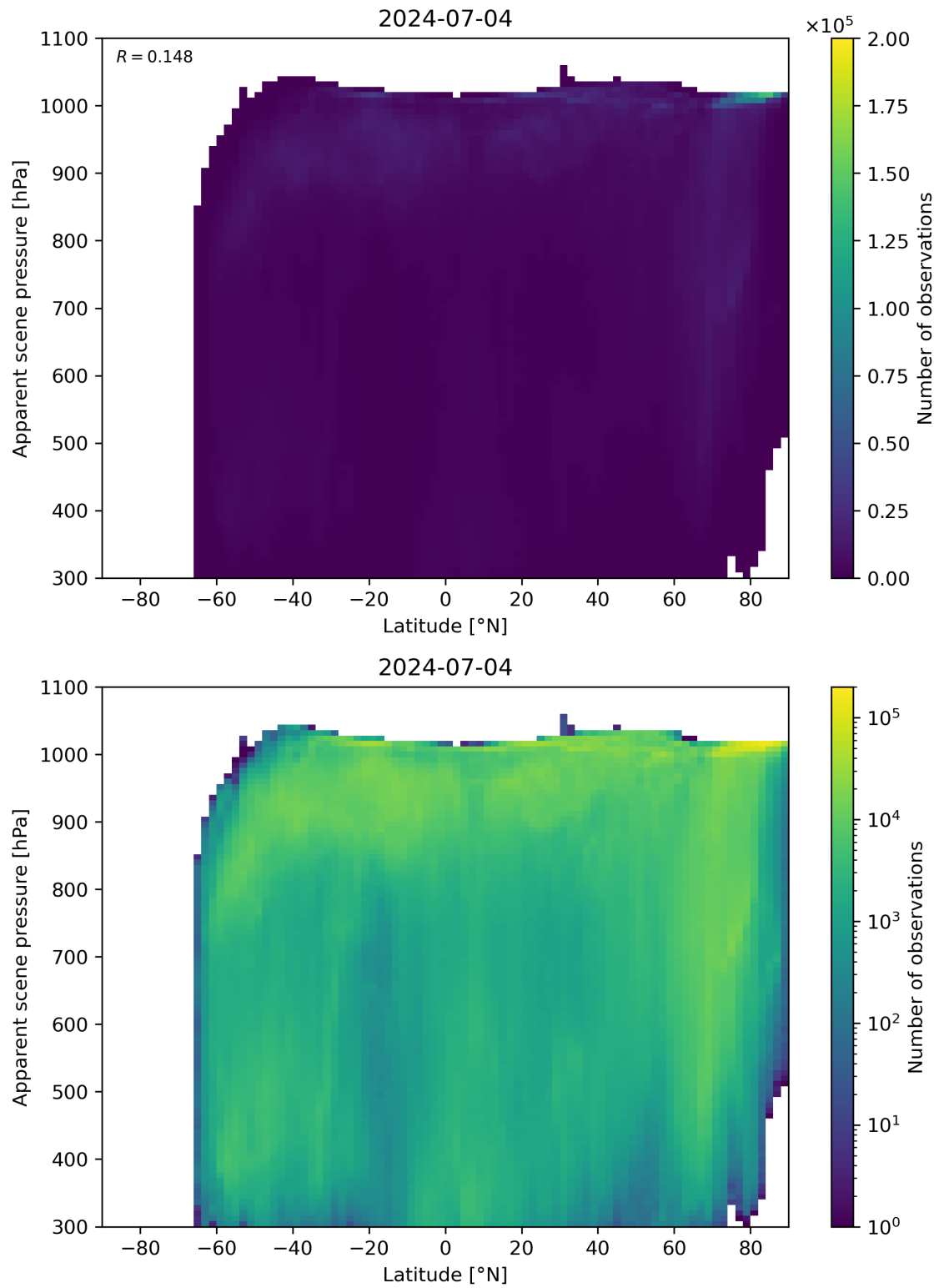
Figure 88: Scatter density plot of “Latitude” against “Apparent scene pressure” for 2024-07-03 to 2024-07-05.
