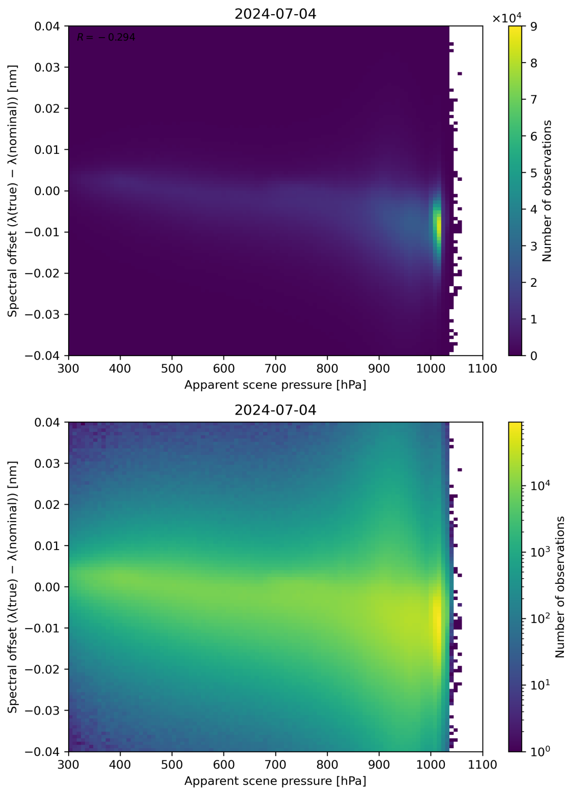
Figure 67: Scatter density plot of “Apparent scene pressure” against “Spectral offset ( \lambda(\text{true}) - \lambda(\text{nominal}) )” for 2024-07-03 to 2024-07-05.
