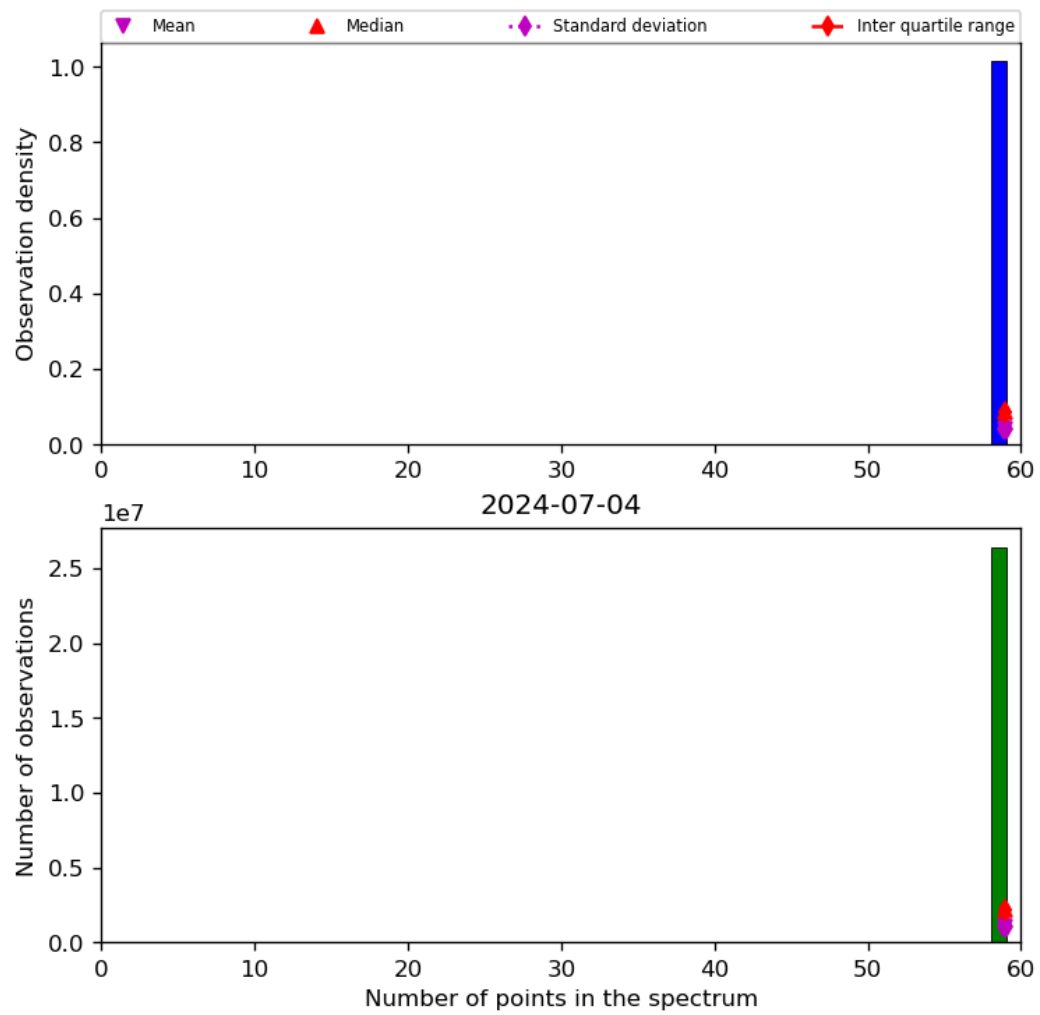
Figure 44: Histogram of “Number of points in the spectrum” for 2024-07-03 to 2024-07-05
