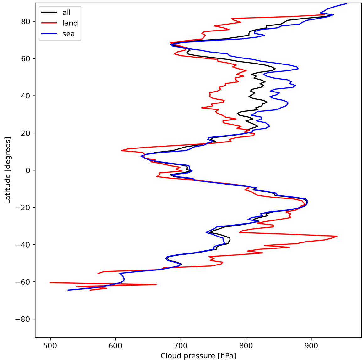
Figure 13: Zonal average of “Cloud pressure” for 2024-07-03 to 2024-07-05.
