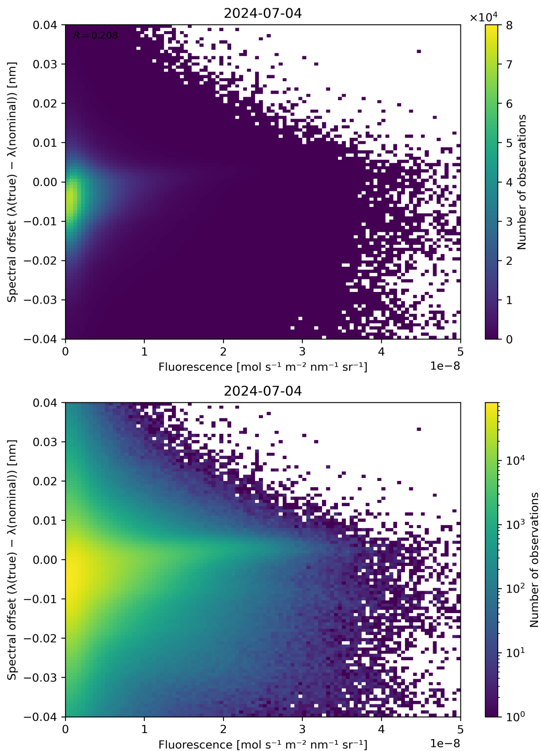
Figure 87: Scatter density plot of “Fluorescence” against “Spectral offset ( \lambda(\text{true}) - \lambda(\text{nominal}) )” for 2024-07-03 to 2024-07-05.
