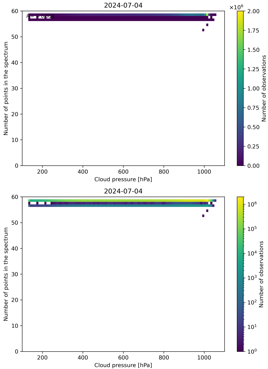
Figure 82: Scatter density plot of “Cloud pressure” against “Number of points in the spectrum” for 2024-07-03 to 2024-07-05.
