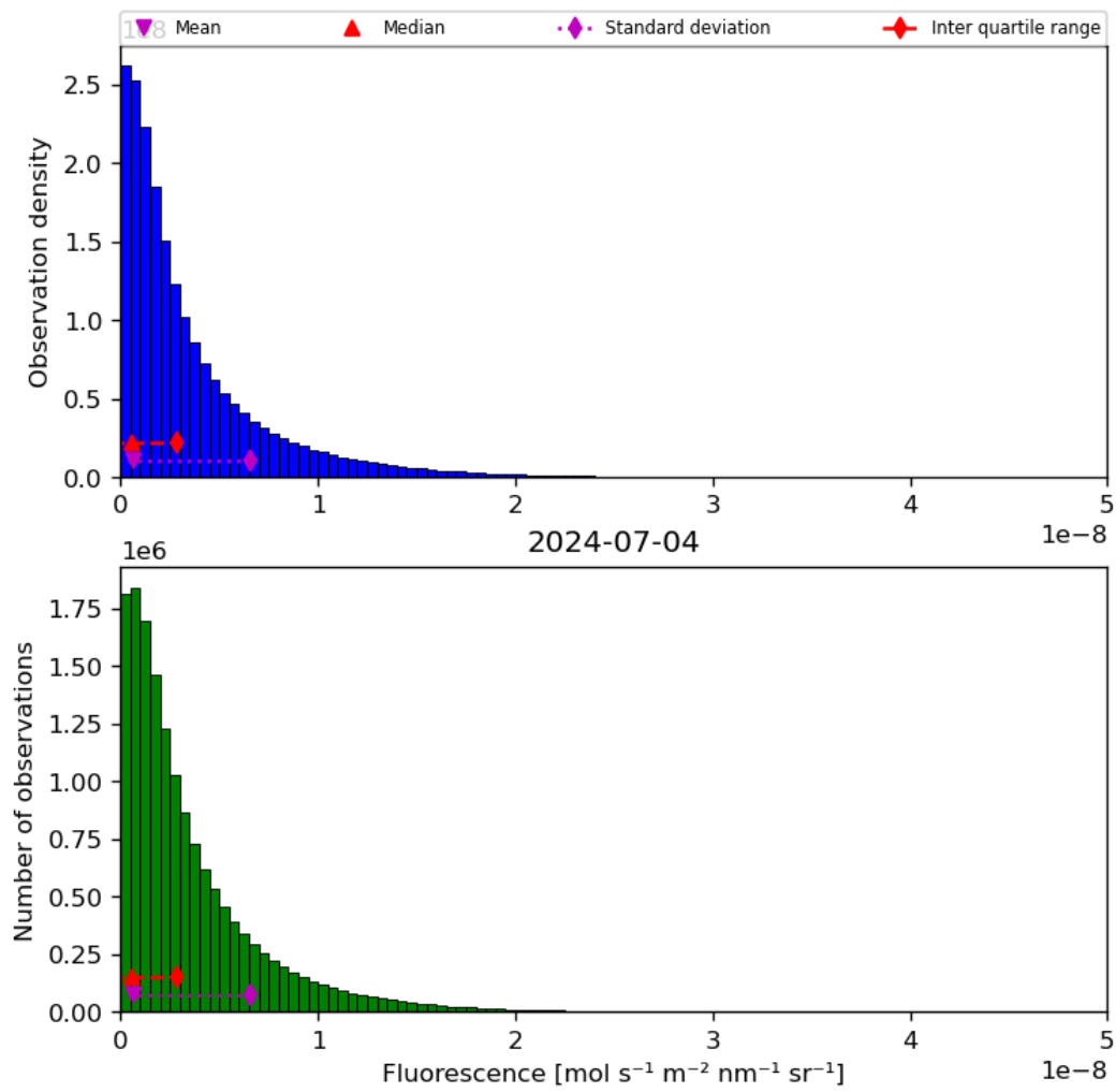
Figure 40: Histogram of “Fluorescence” for 2024-07-03 to 2024-07-05
