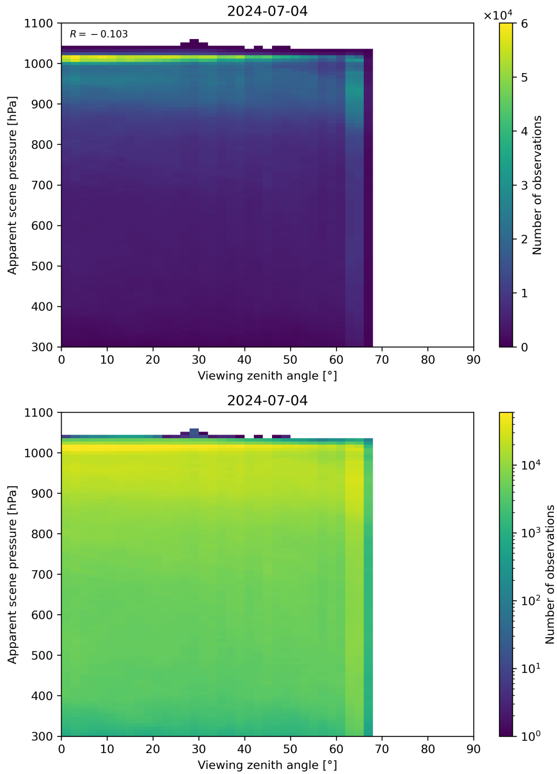
Figure 118: Scatter density plot of “Viewing zenith angle” against “Apparent scene pressure” for 2024-07-03 to 2024-07-05.
