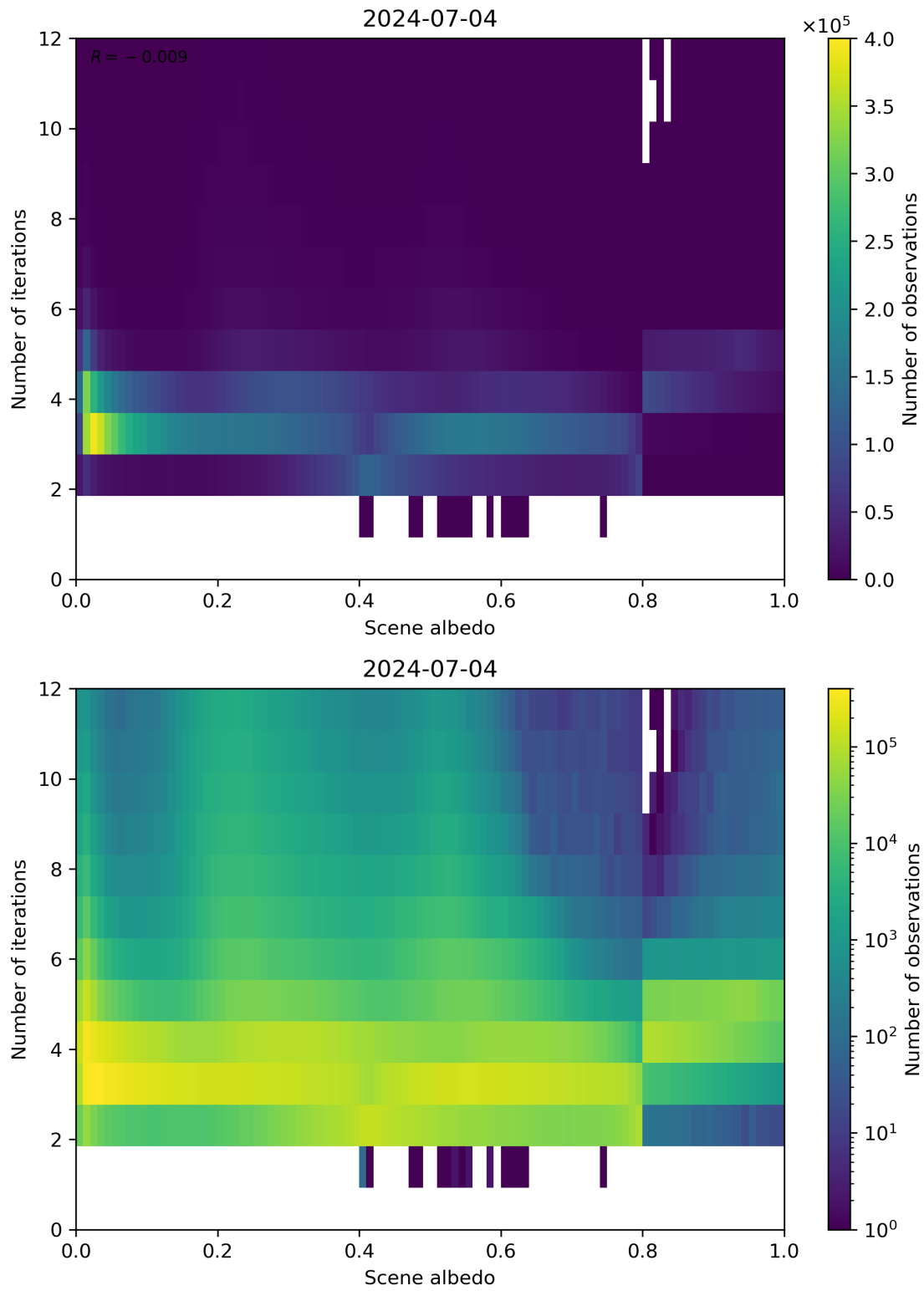
Figure 105: Scatter density plot of “Scene albedo” against “Number of iterations” for 2024-07-03 to 2024-07-05.
