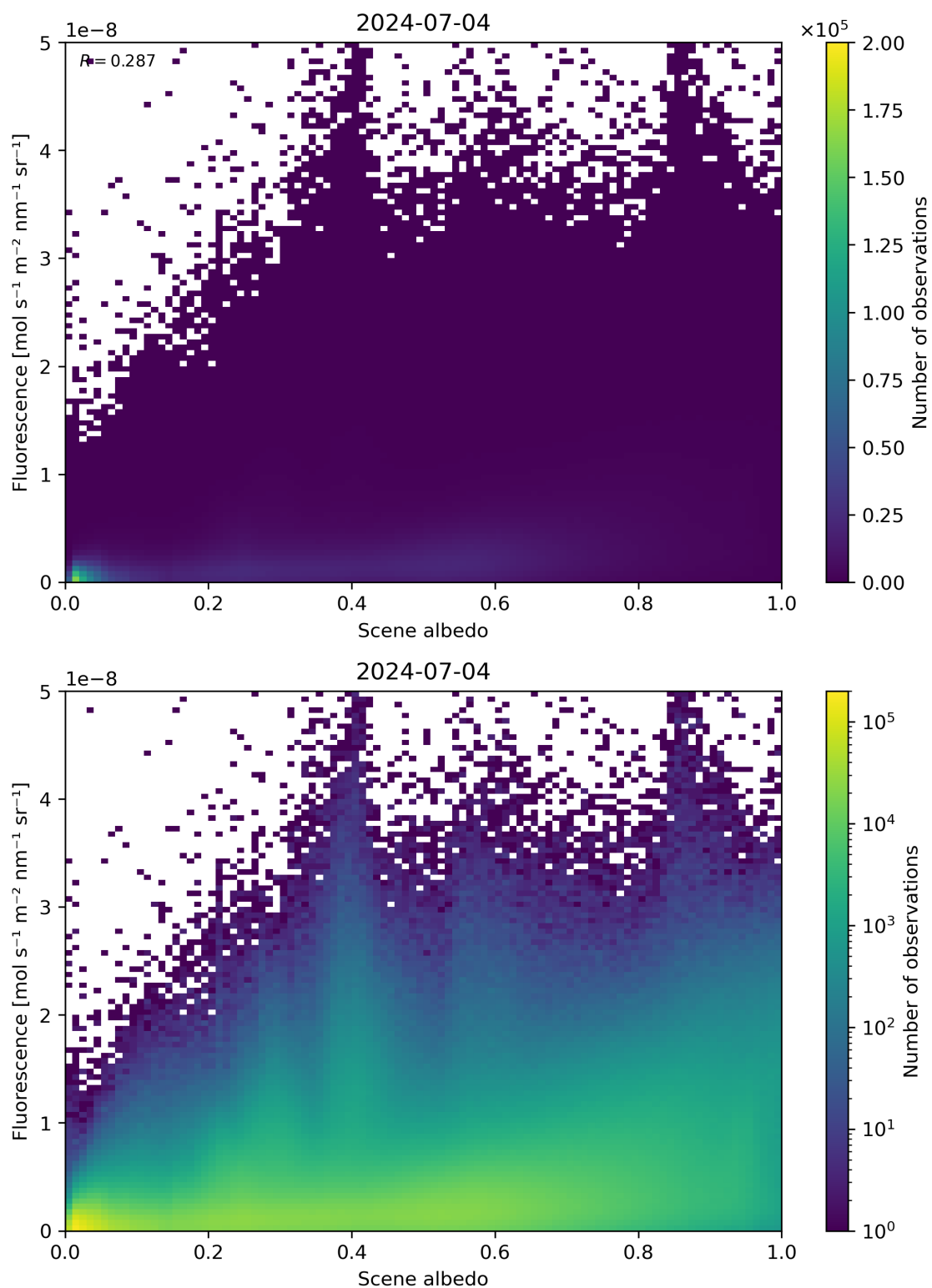
Figure 104: Scatter density plot of “Scene albedo” against “Fluorescence” for 2024-07-03 to 2024-07-05.
