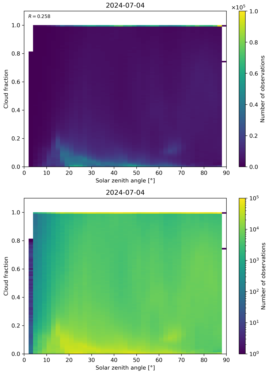
Figure 110: Scatter density plot of “Solar zenith angle” against “Cloud fraction” for 2024-07-03 to 2024-07-05.
