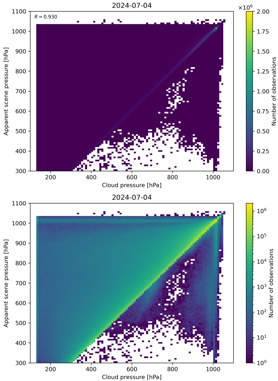
Figure 77: Scatter density plot of “Cloud pressure” against “Apparent scene pressure” for 2024-07-03 to 2024-07-05.
