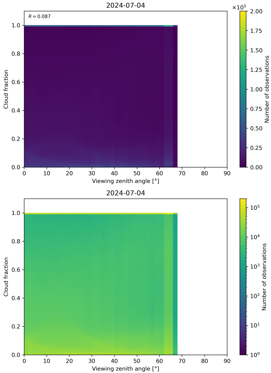
Figure 120: Scatter density plot of “Viewing zenith angle” against “Cloud fraction” for 2024-07-03 to 2024-07-05.
