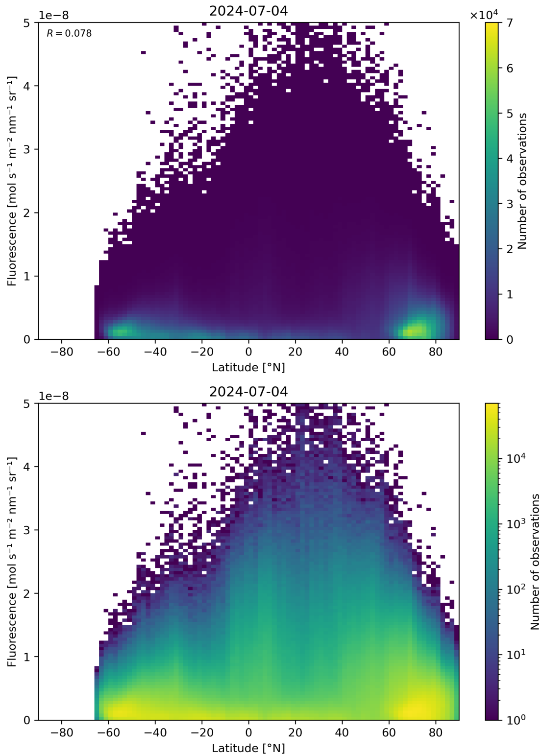
Figure 92: Scatter density plot of “Latitude” against “Fluorescence” for 2024-07-03 to 2024-07-05.
