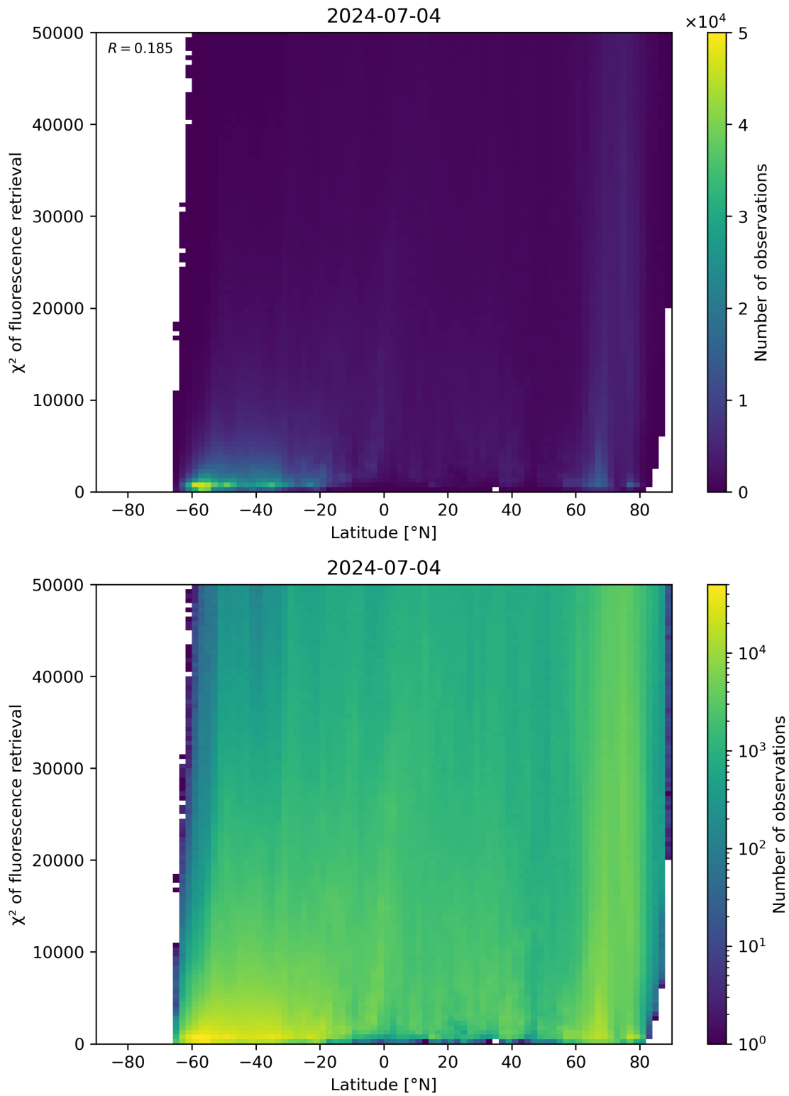
Figure 89: Scatter density plot of “Latitude” against “ \chi^2 of fluorescence retrieval” for 2024-07-03 to 2024-07-05.
