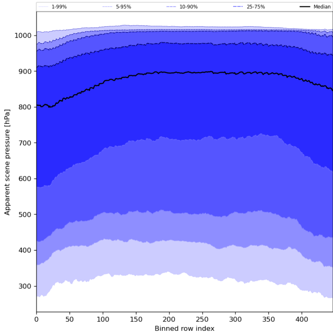
Figure 53: Along track statistics of “Apparent scene pressure” for 2024-07-03 to 2024-07-05
