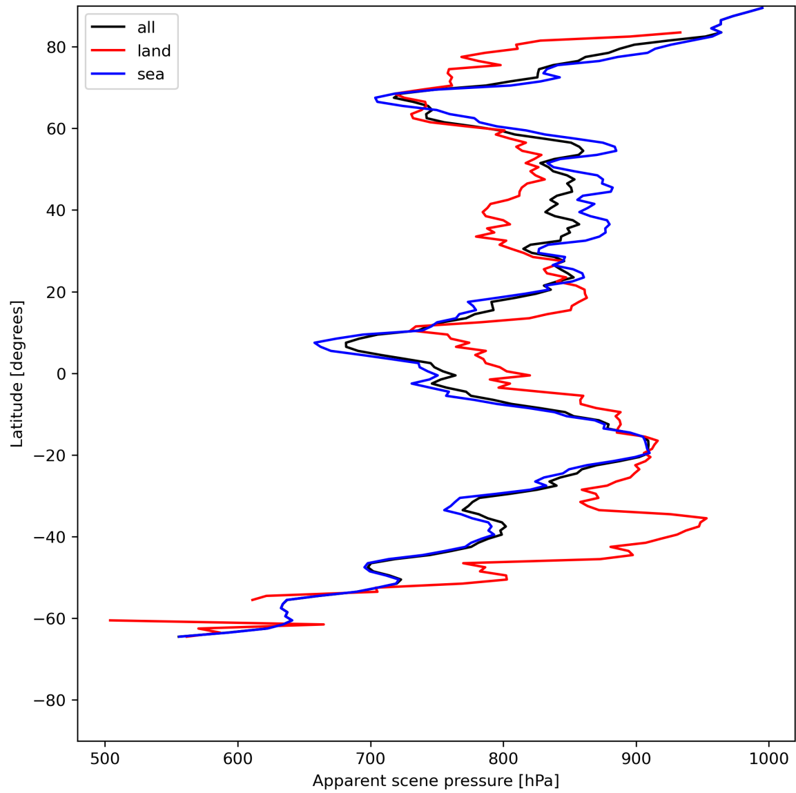
Figure 19: Zonal average of “Apparent scene pressure” for 2024-07-03 to 2024-07-05.
