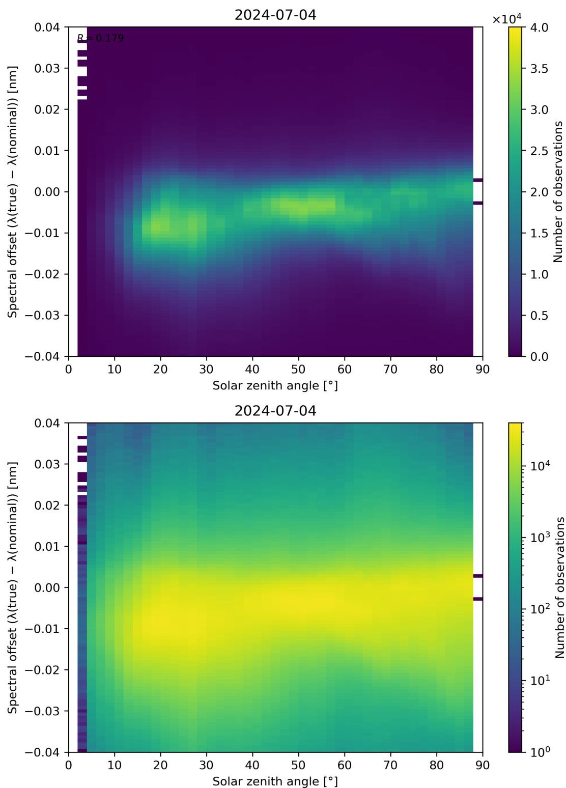
Figure 117: Scatter density plot of “Solar zenith angle” against “Spectral offset ( \lambda(\text{true}) - \lambda(\text{nominal}) )” for 2024-07-03 to 2024-07-05.
