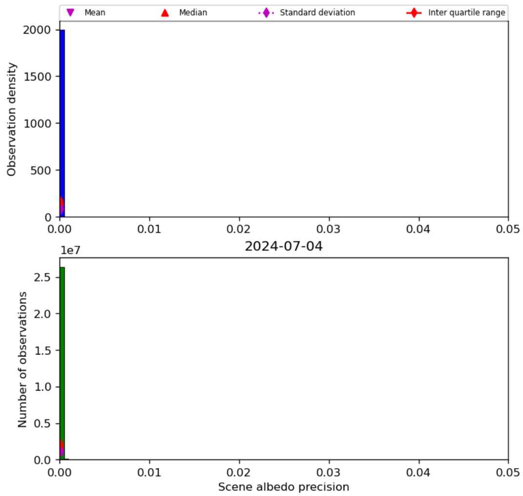
Figure 35: Histogram of “Scene albedo precision” for 2024-07-03 to 2024-07-05
