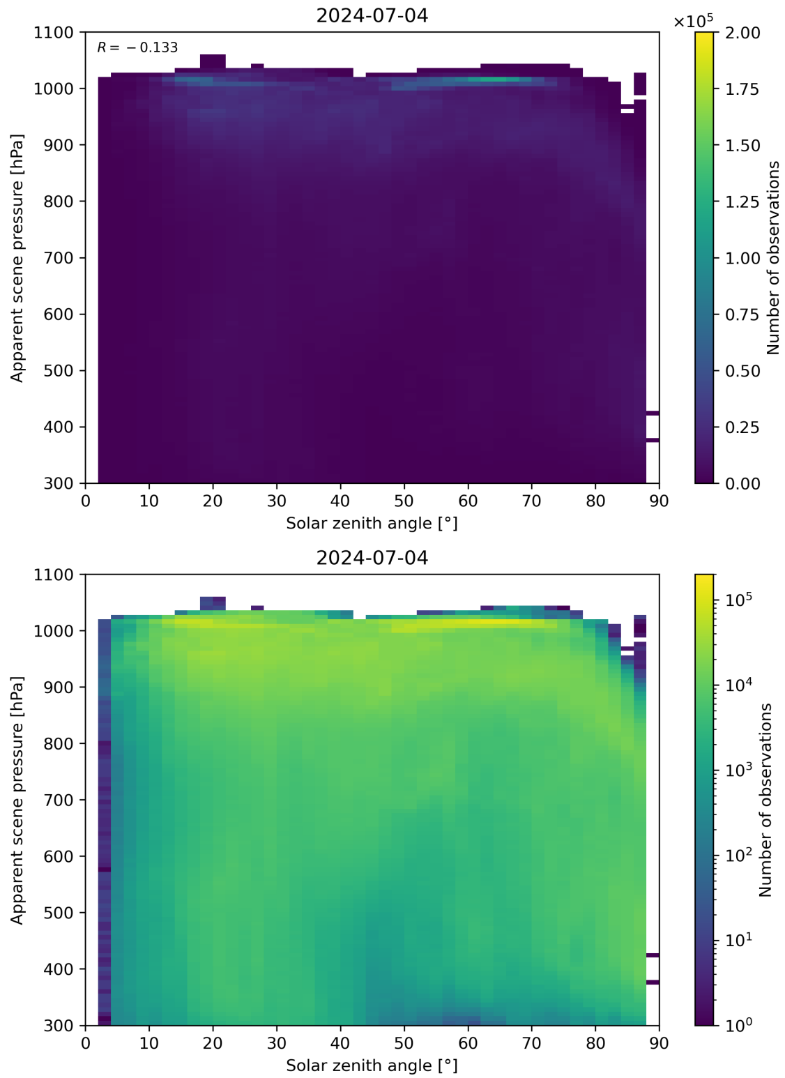
Figure 108: Scatter density plot of “Solar zenith angle” against “Apparent scene pressure” for 2024-07-03 to 2024-07-05.
