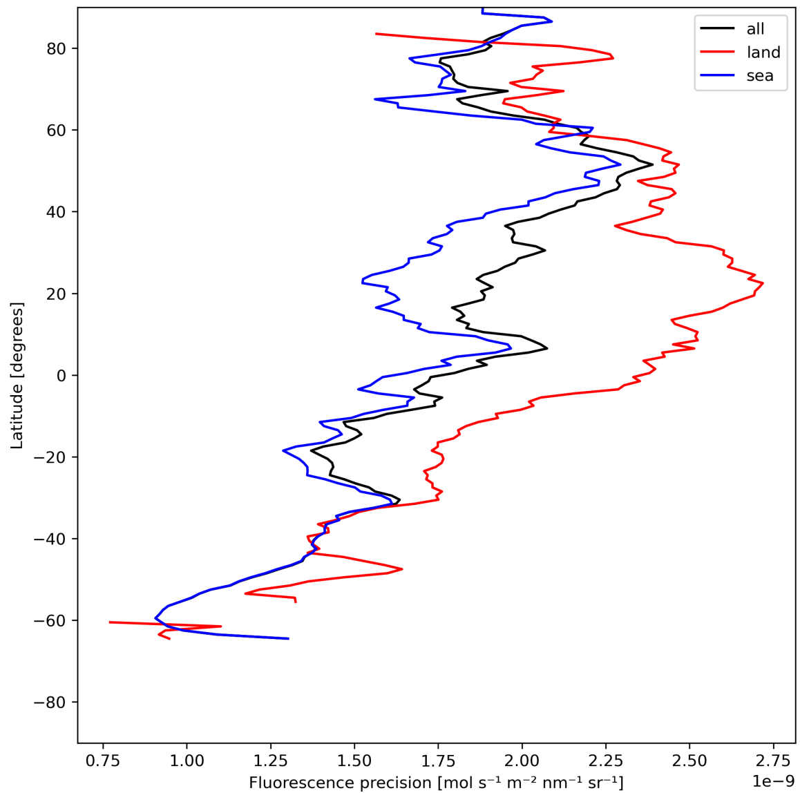
Figure 24: Zonal average of “Fluorescence precision” for 2024-07-03 to 2024-07-05.
