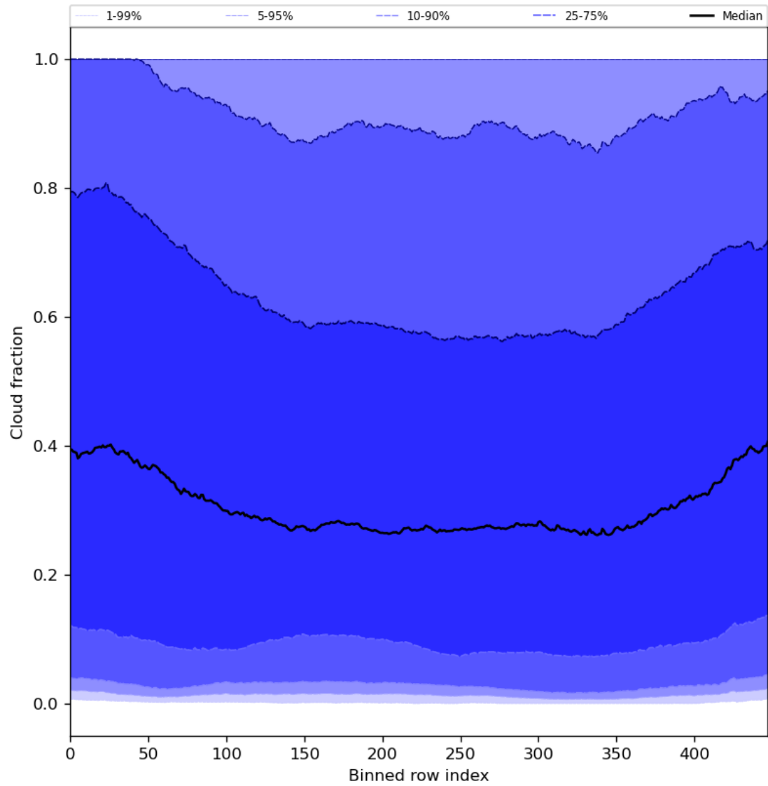
Figure 49: Along track statistics of “Cloud fraction” for 2024-07-03 to 2024-07-05
