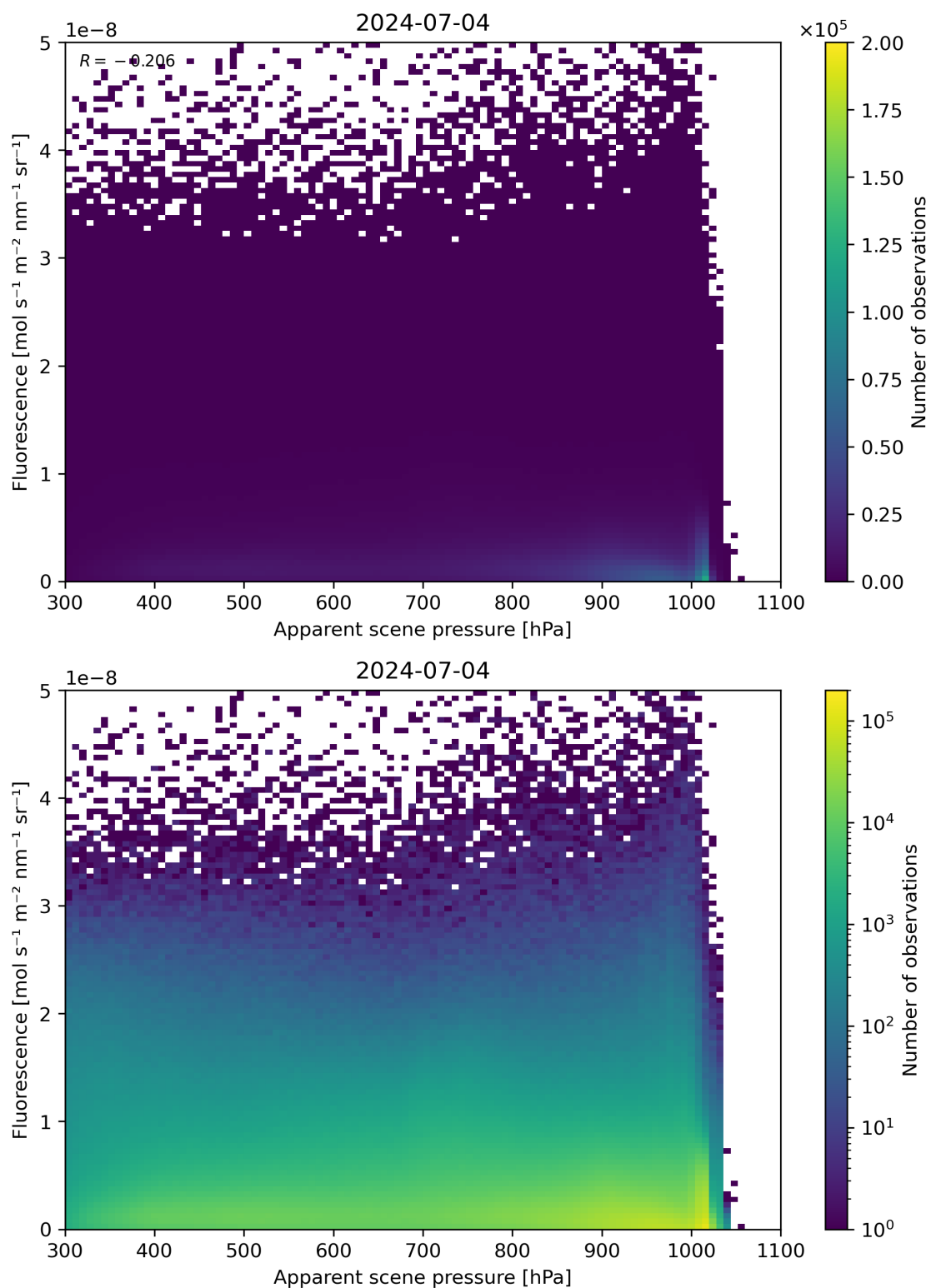
Figure 64: Scatter density plot of “Apparent scene pressure” against “Fluorescence” for 2024-07-03 to 2024-07-05.
