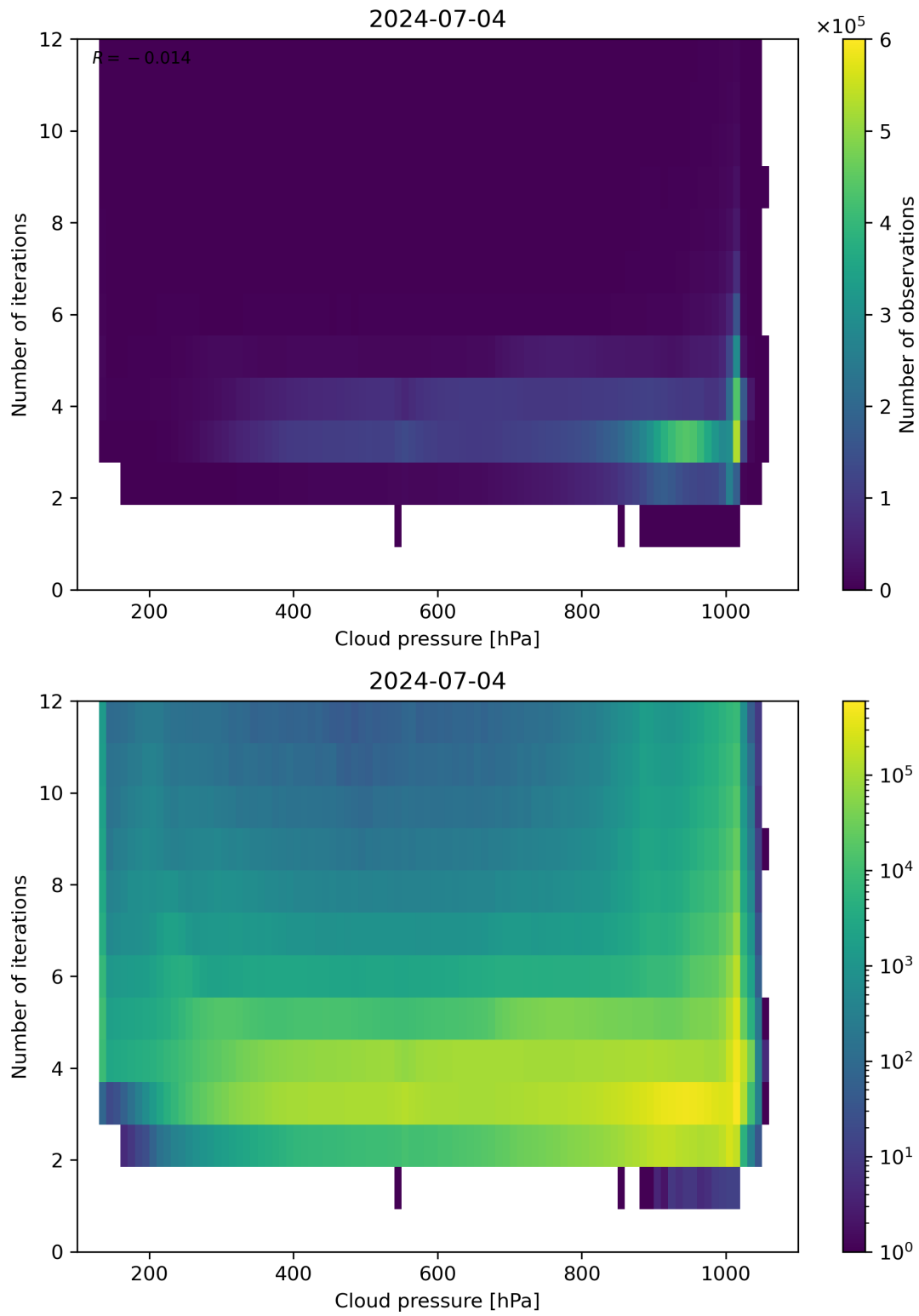
Figure 81: Scatter density plot of “Cloud pressure” against “Number of iterations” for 2024-07-03 to 2024-07-05.
