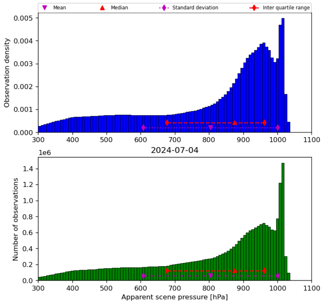
Figure 36: Histogram of “Apparent scene pressure” for 2024-07-03 to 2024-07-05
