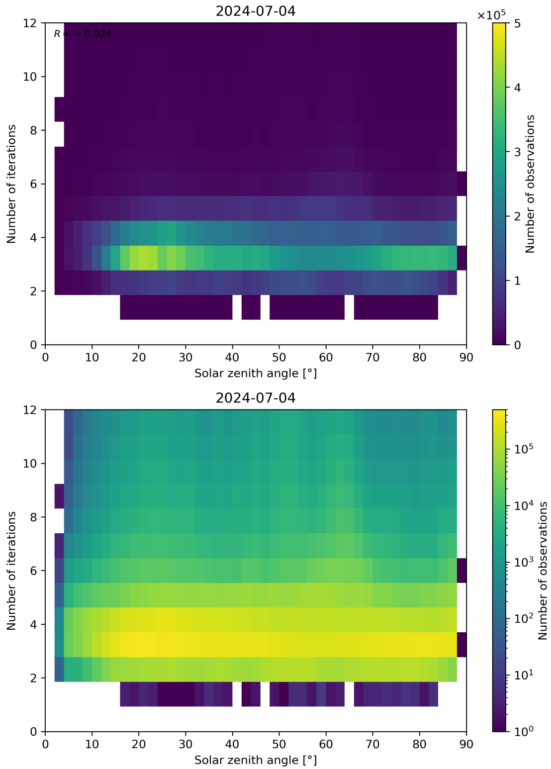
Figure 114: Scatter density plot of “Solar zenith angle” against “Number of iterations” for 2024-07-03 to 2024-07-05.
