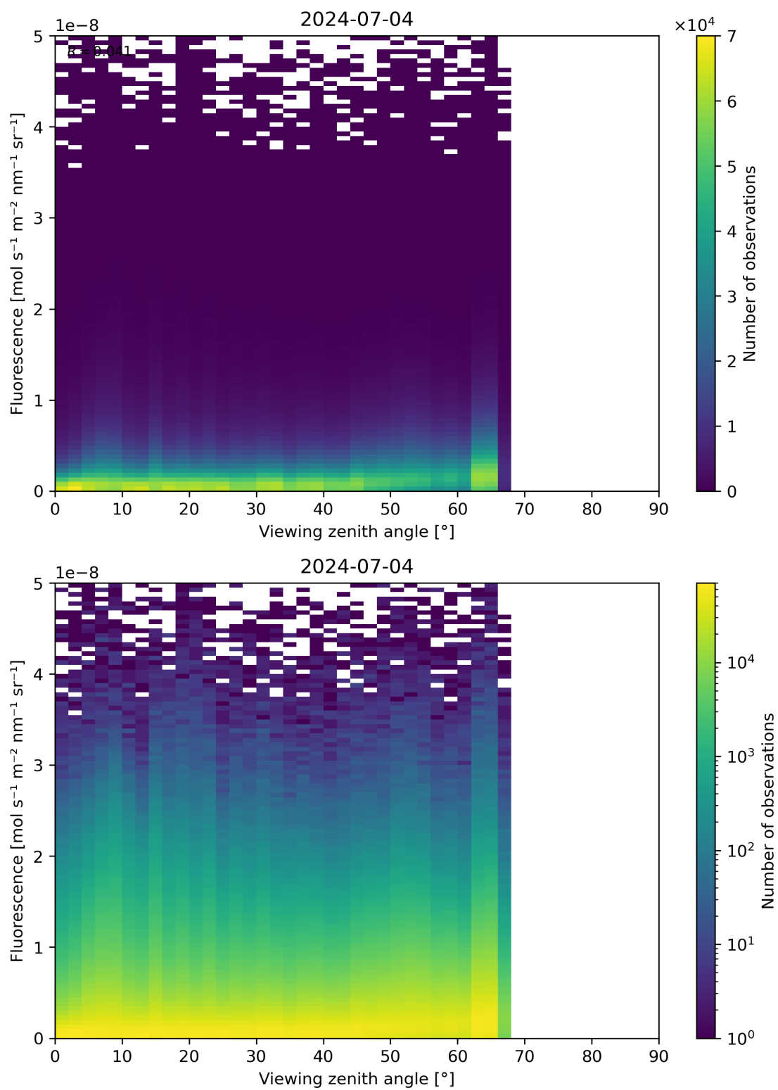
Figure 122: Scatter density plot of “Viewing zenith angle” against “Fluorescence” for 2024-07-03 to 2024-07-05.
