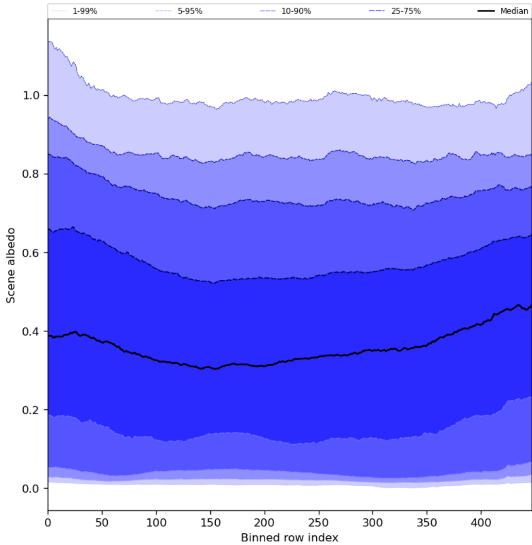
Figure 51: Along track statistics of “Scene albedo” for 2024-07-03 to 2024-07-05
