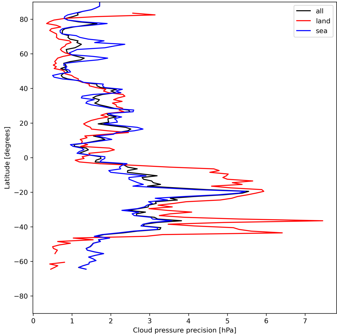
Figure 14: Zonal average of “Cloud pressure precision” for 2024-07-03 to 2024-07-05.
