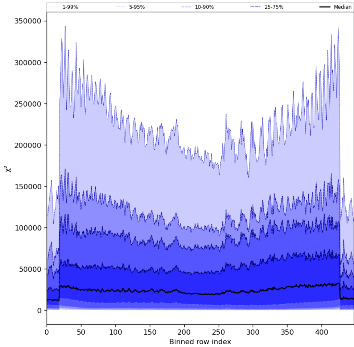
Figure 55: Along track statistics of “ \chi^2 ” for 2024-07-03 to 2024-07-05
