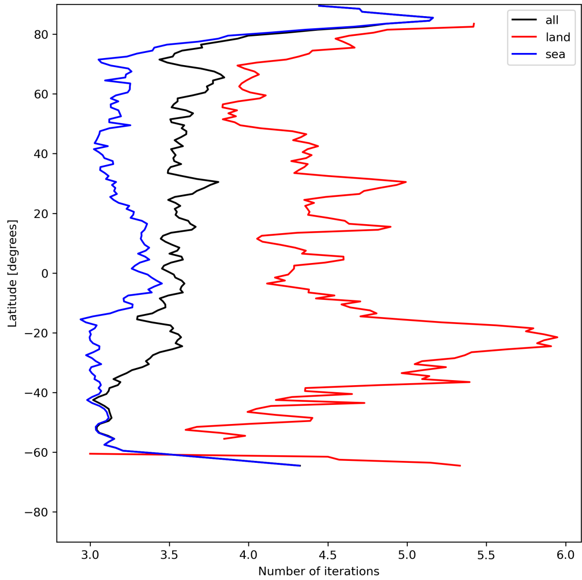
Figure 22: Zonal average of “Number of iterations” for 2024-07-03 to 2024-07-05.
