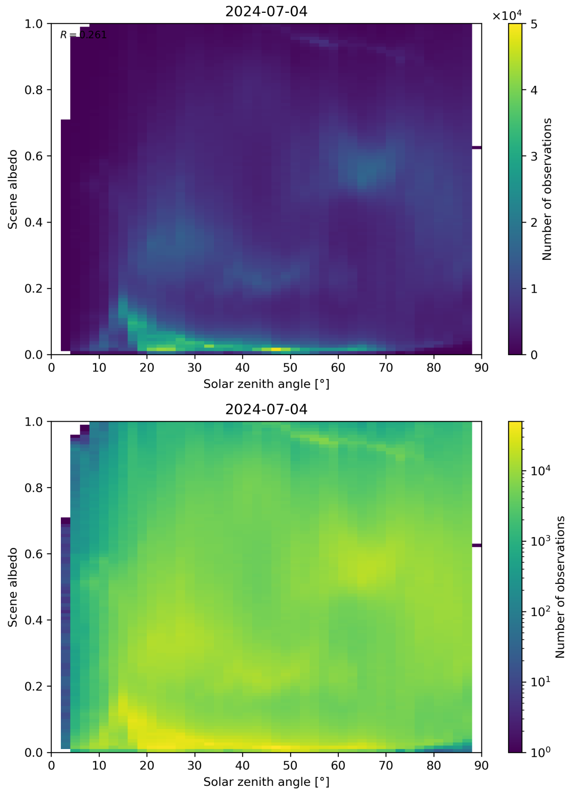
Figure 116: Scatter density plot of “Solar zenith angle” against “Scene albedo” for 2024-07-03 to 2024-07-05.
