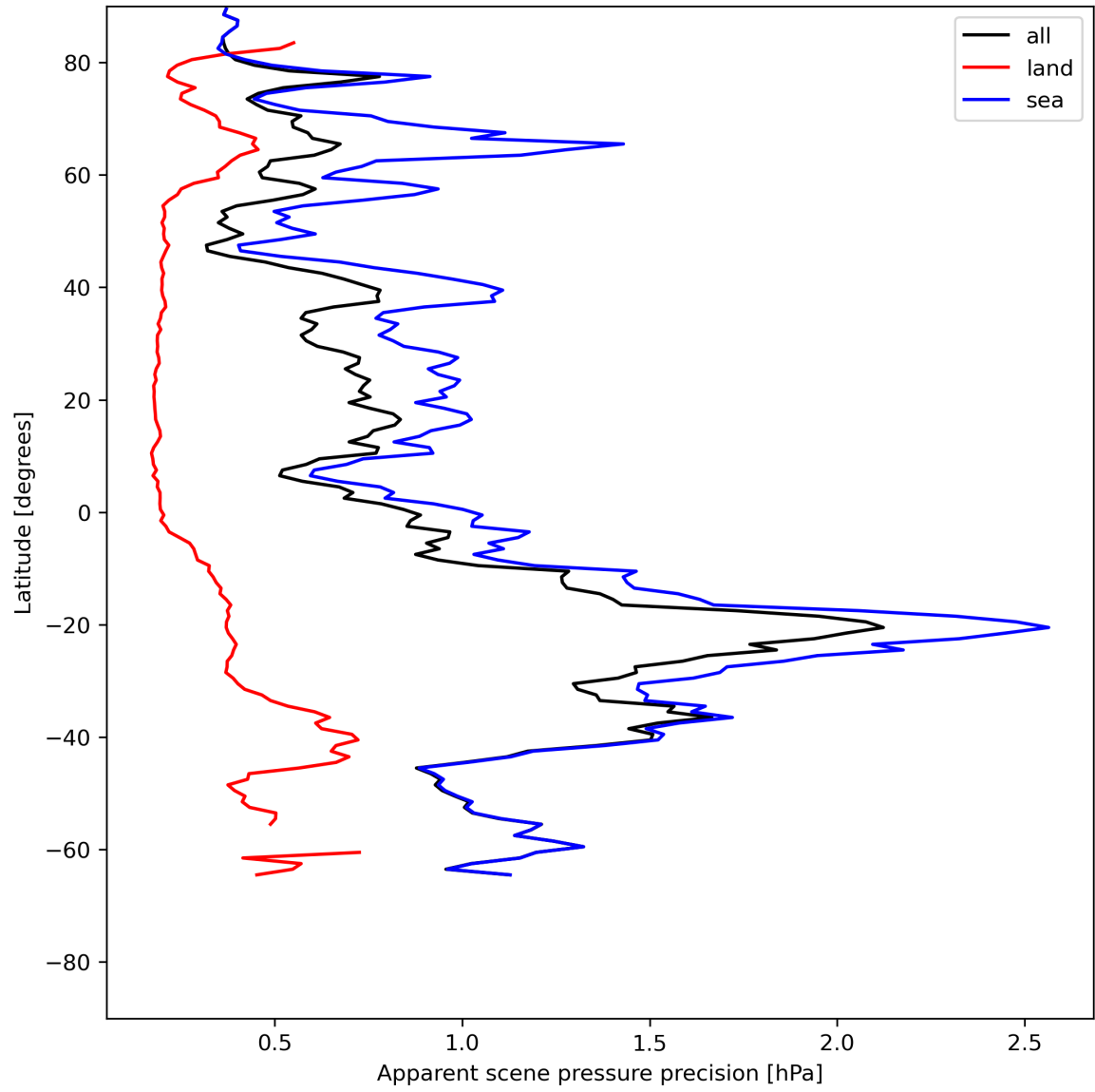
Figure 20: Zonal average of “Apparent scene pressure precision” for 2024-07-03 to 2024-07-05.
