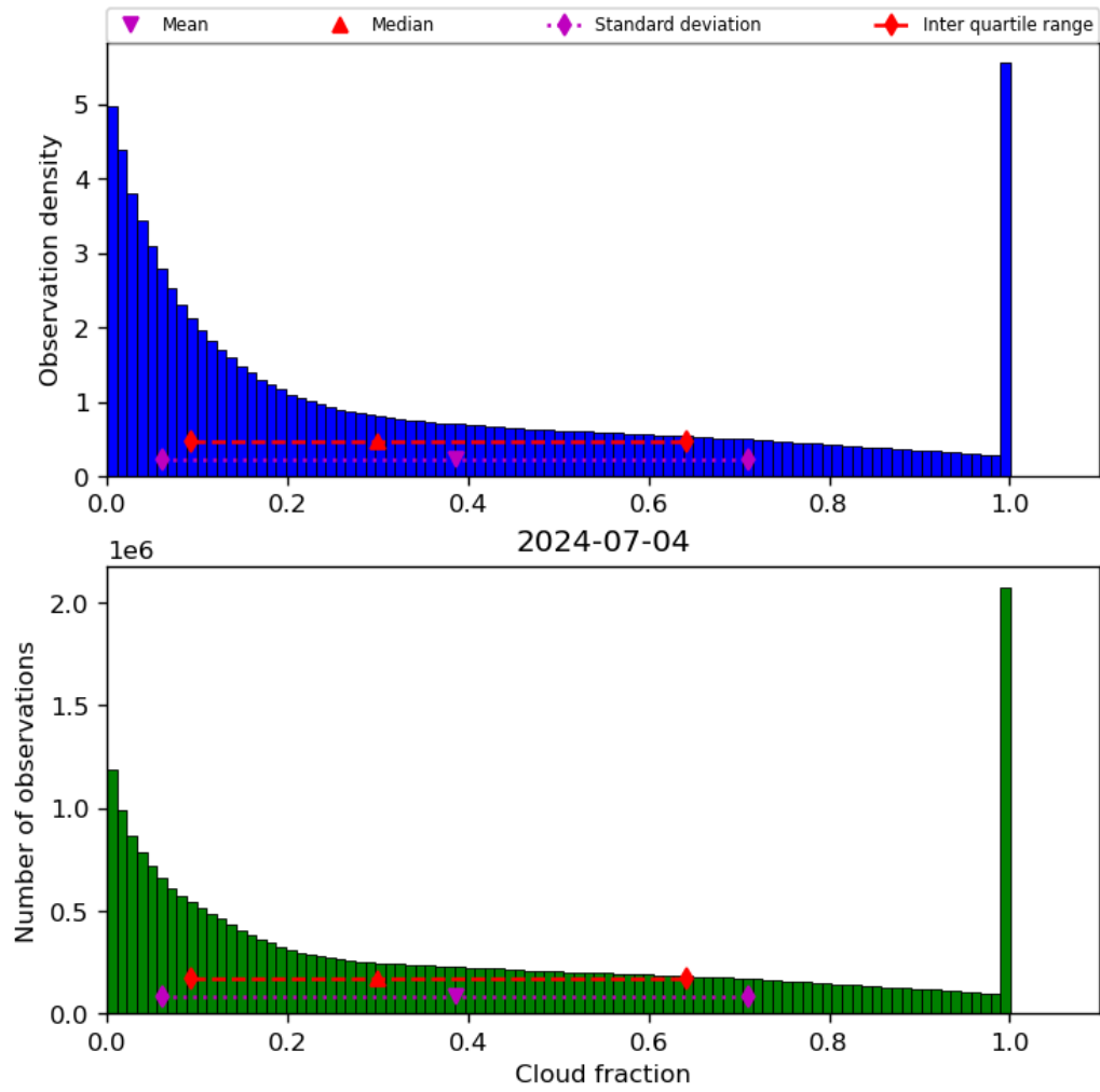
Figure 32: Histogram of “Cloud fraction” for 2024-07-03 to 2024-07-05
