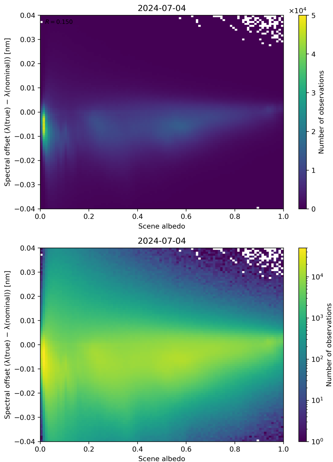
Figure 107: Scatter density plot of “Scene albedo” against “Spectral offset ( \lambda(\text{true}) - \lambda(\text{nominal}) )” for 2024-07-03 to 2024-07-05.
