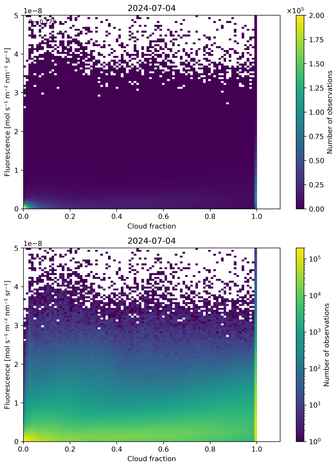
Figure 72: Scatter density plot of “Cloud fraction” against “Fluorescence” for 2024-07-03 to 2024-07-05.
