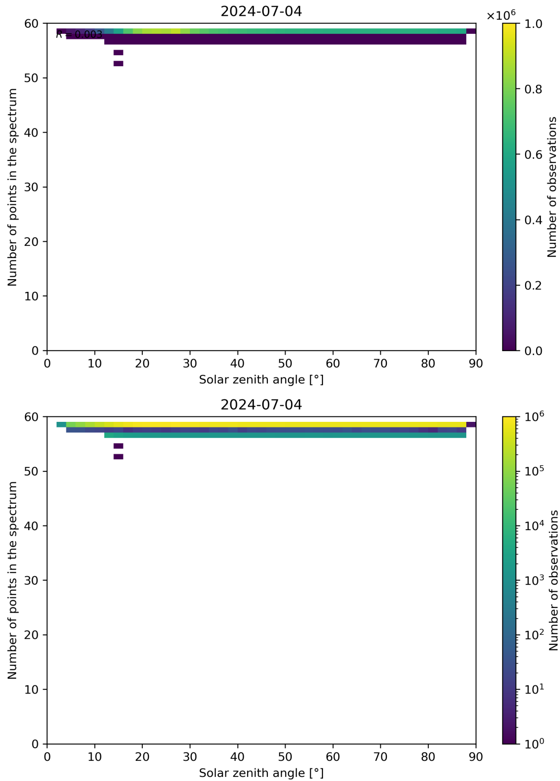
Figure 115: Scatter density plot of “Solar zenith angle” against “Number of points in the spectrum” for 2024-07-03 to 2024-07-05.
