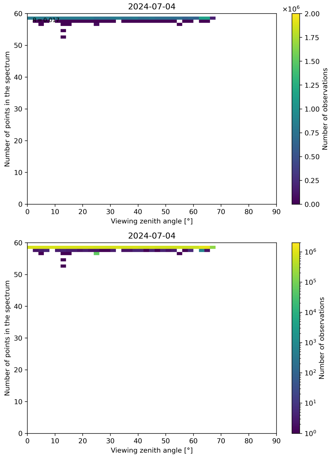
Figure 125: Scatter density plot of “Viewing zenith angle” against “Number of points in the spectrum” for 2024-07-03 to 2024-07-05.
