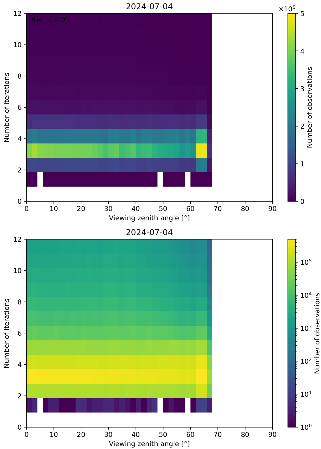
Figure 124: Scatter density plot of “Viewing zenith angle” against “Number of iterations” for 2024-07-03 to 2024-07-05.
