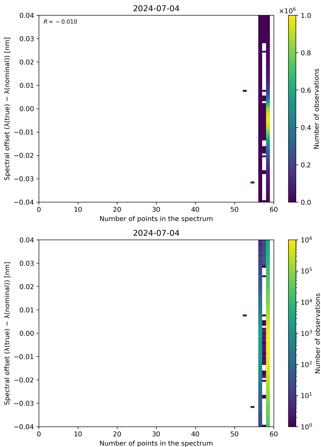
Figure 101: Scatter density plot of “Number of points in the spectrum” against “Spectral offset ( \lambda(\text{true}) - \lambda(\text{nominal}) )” for 2024-07-03 to 2024-07-05.
