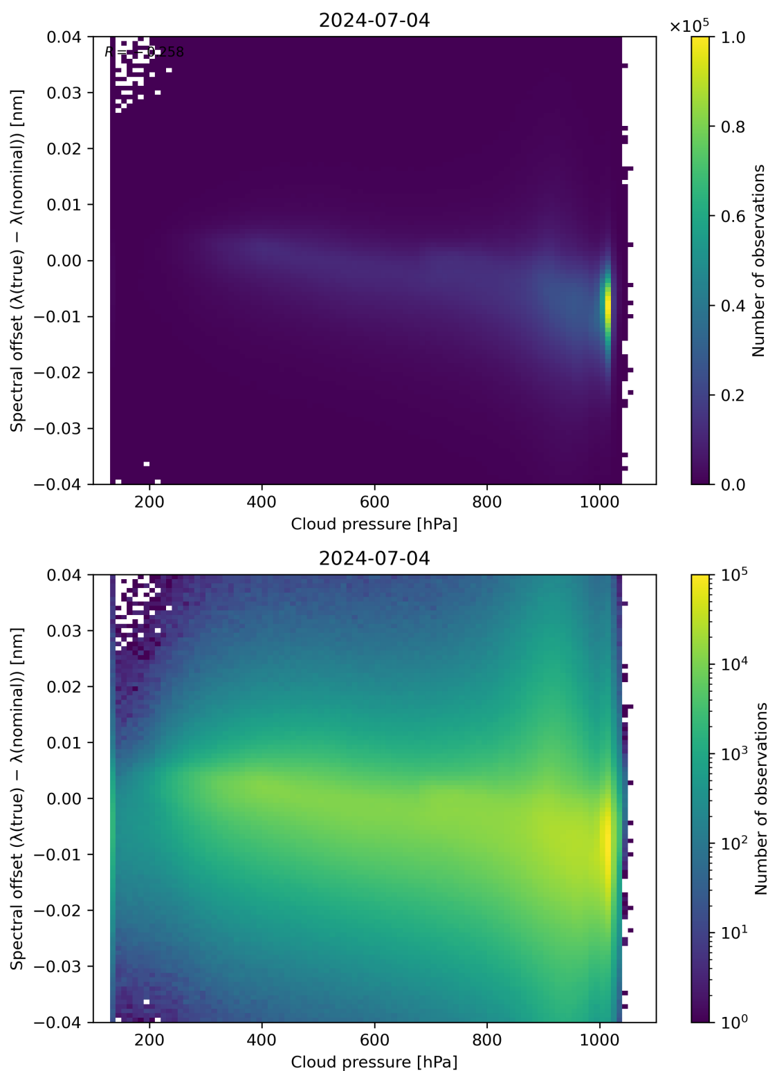
Figure 84: Scatter density plot of “Cloud pressure” against “Spectral offset ( \lambda(\text{true}) - \lambda(\text{nominal}) )” for 2024-07-03 to 2024-07-05.
