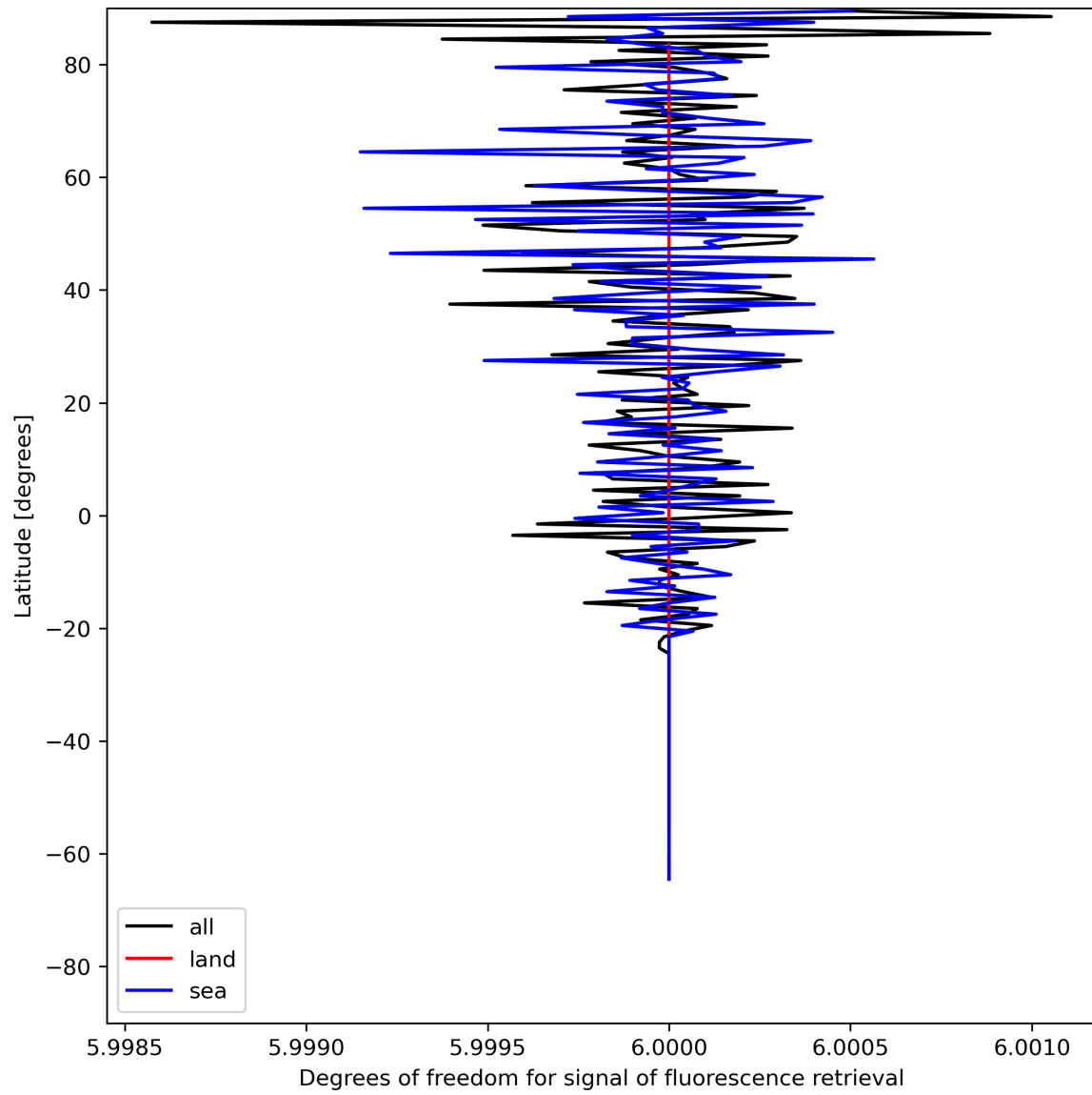
Figure 26: Zonal average of “Degrees of freedom for signal of fluorescence retrieval” for 2024-07-03 to 2024-07-05.
