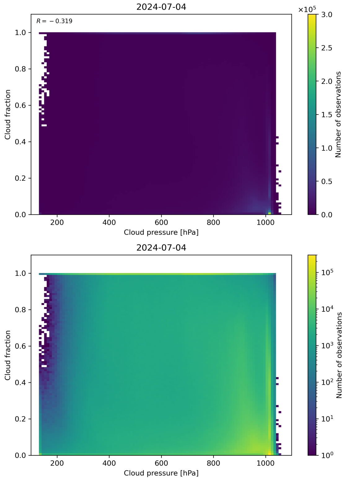
Figure 79: Scatter density plot of “Cloud pressure” against “Cloud fraction” for 2024-07-03 to 2024-07-05.
