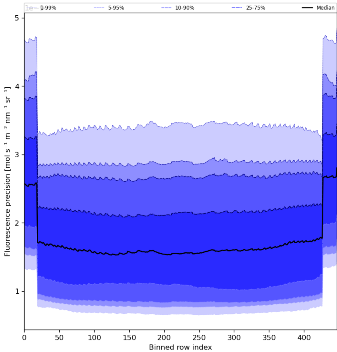
Figure 58: Along track statistics of “Fluorescence precision” for 2024-07-03 to 2024-07-05
