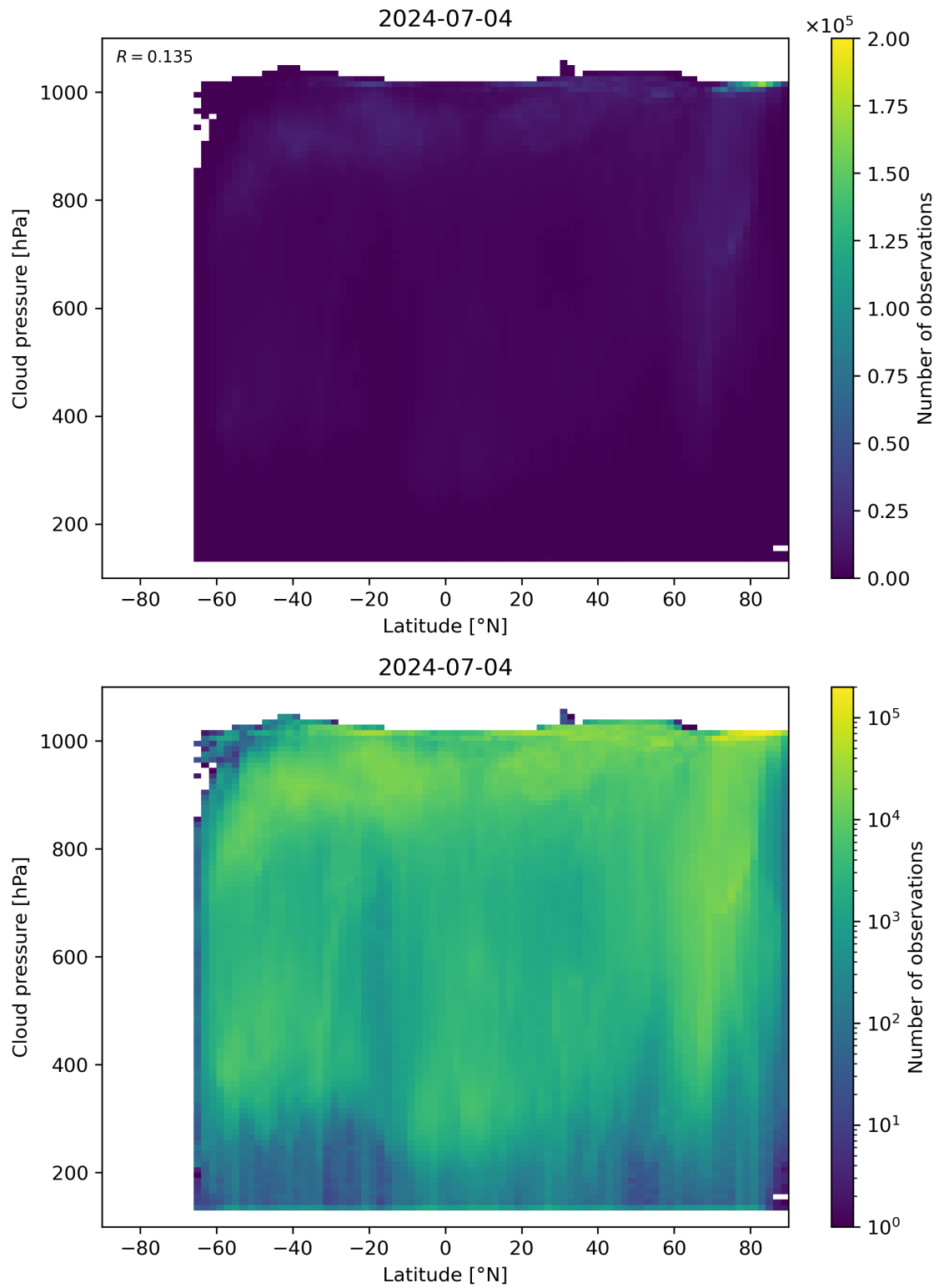
Figure 91: Scatter density plot of “Latitude” against “Cloud pressure” for 2024-07-03 to 2024-07-05.
