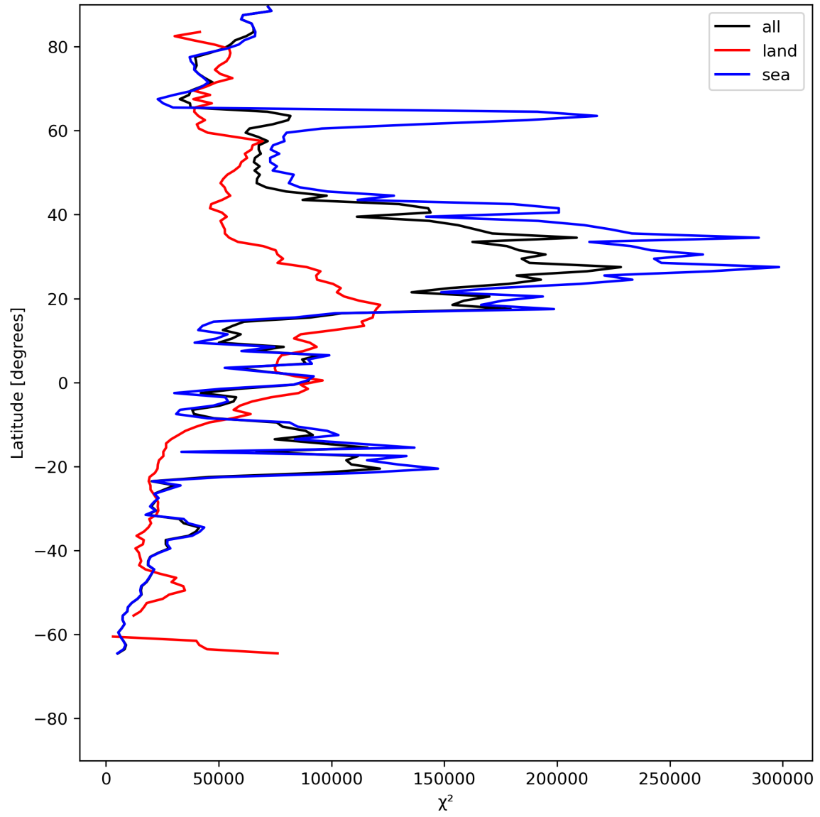
Figure 21: Zonal average of “ \chi^2 ” for 2024-07-03 to 2024-07-05.
