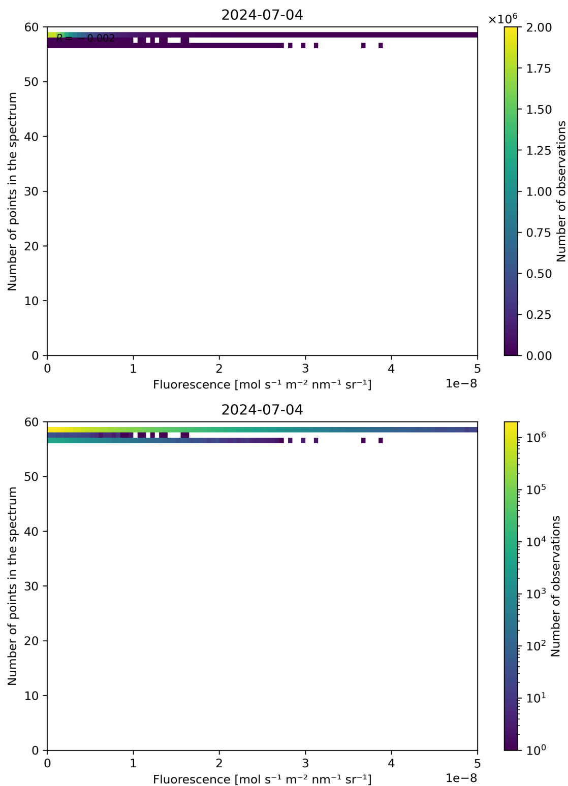
Figure 86: Scatter density plot of “Fluorescence” against “Number of points in the spectrum” for 2024-07-03 to 2024-07-05.
