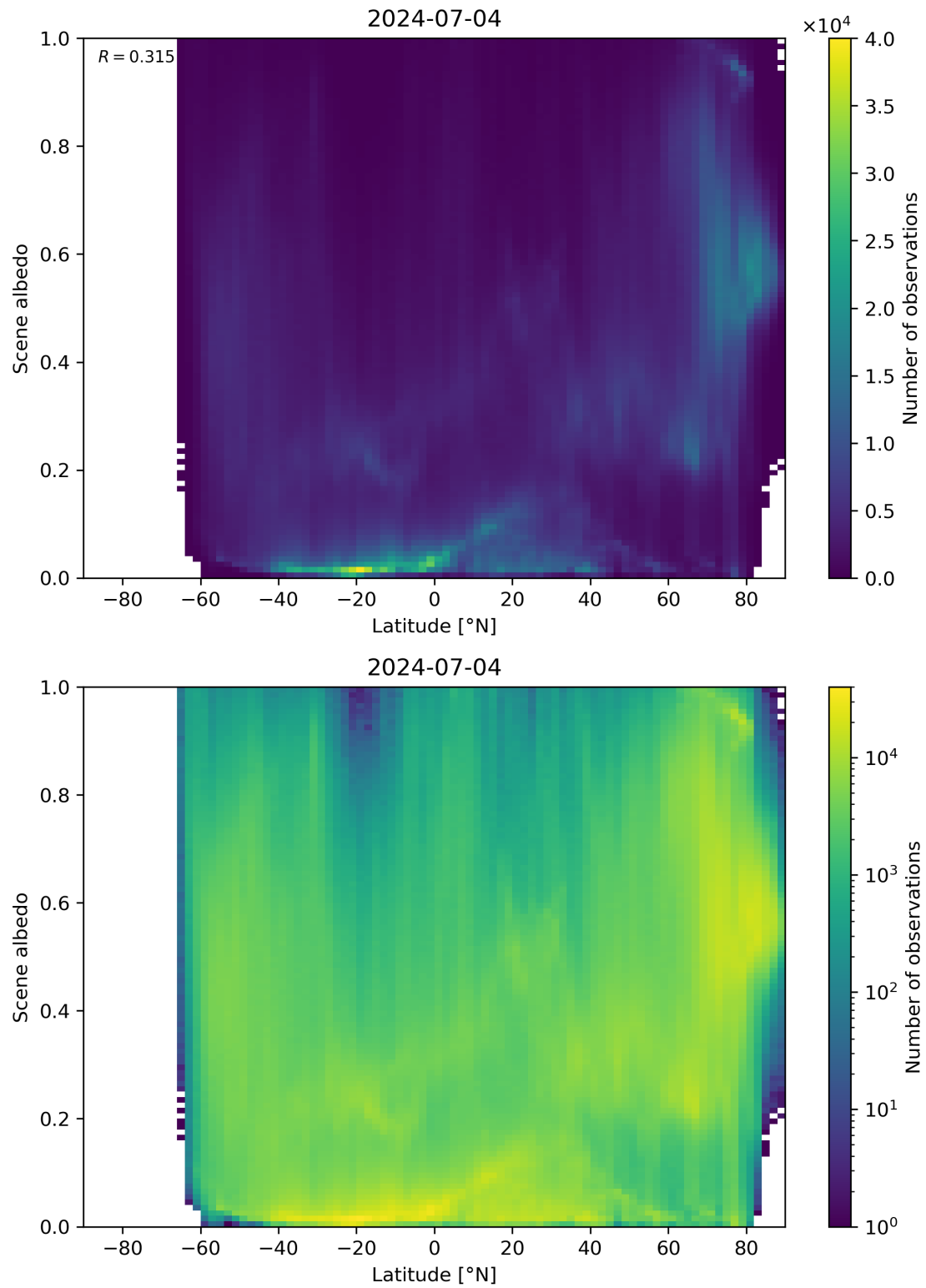
Figure 95: Scatter density plot of “Latitude” against “Scene albedo” for 2024-07-03 to 2024-07-05.
