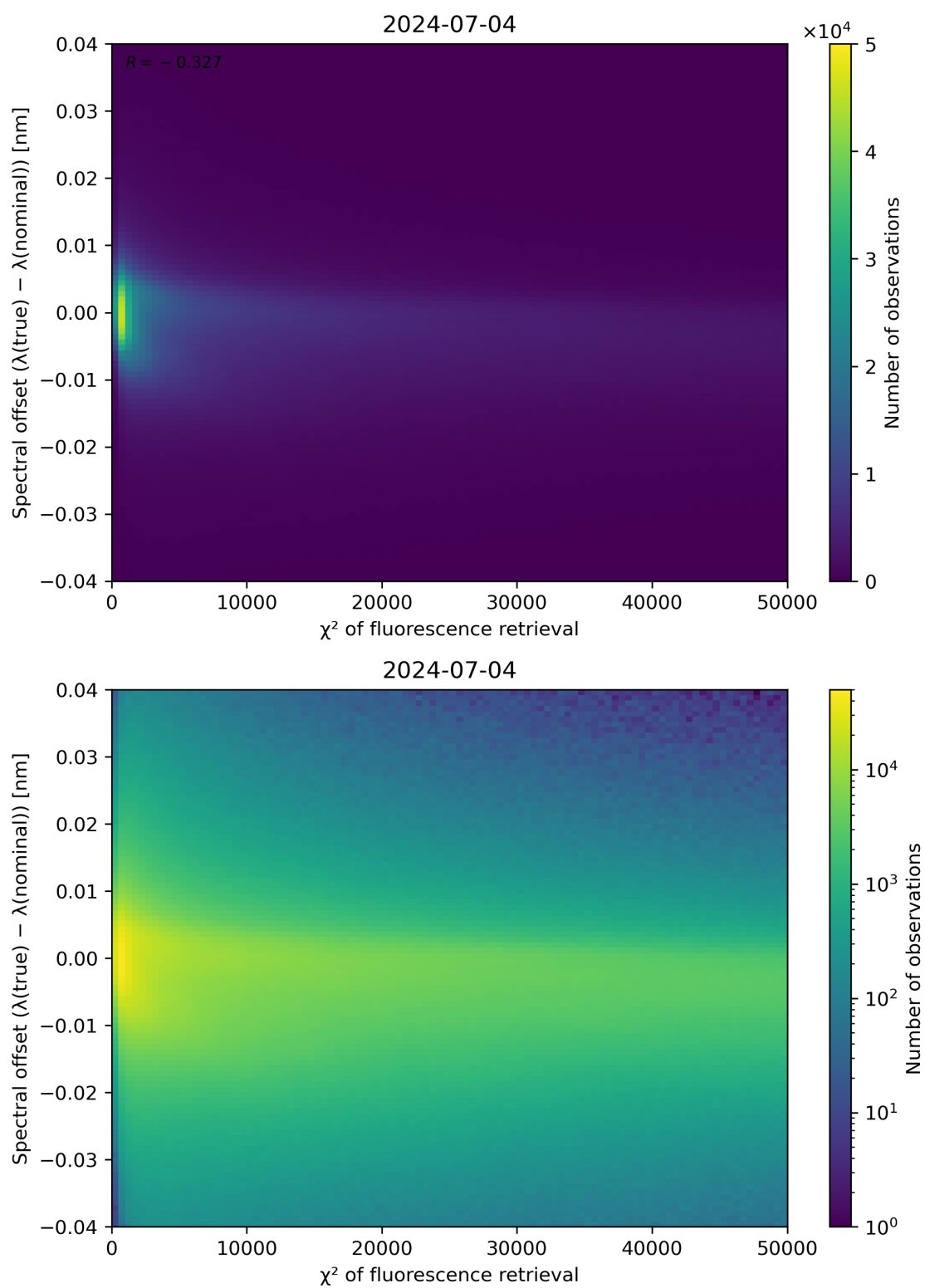
Figure 69: Scatter density plot of “ \chi^2 of fluorescence retrieval” against “Spectral offset ( \lambda(\text{true}) - \lambda(\text{nominal})) ” for 2024-07-03 to 2024-07-05.
