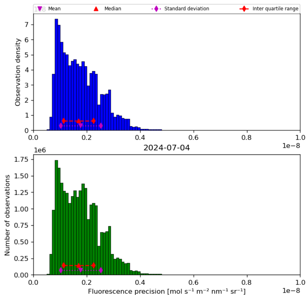
Figure 41: Histogram of “Fluorescence precision” for 2024-07-03 to 2024-07-05
