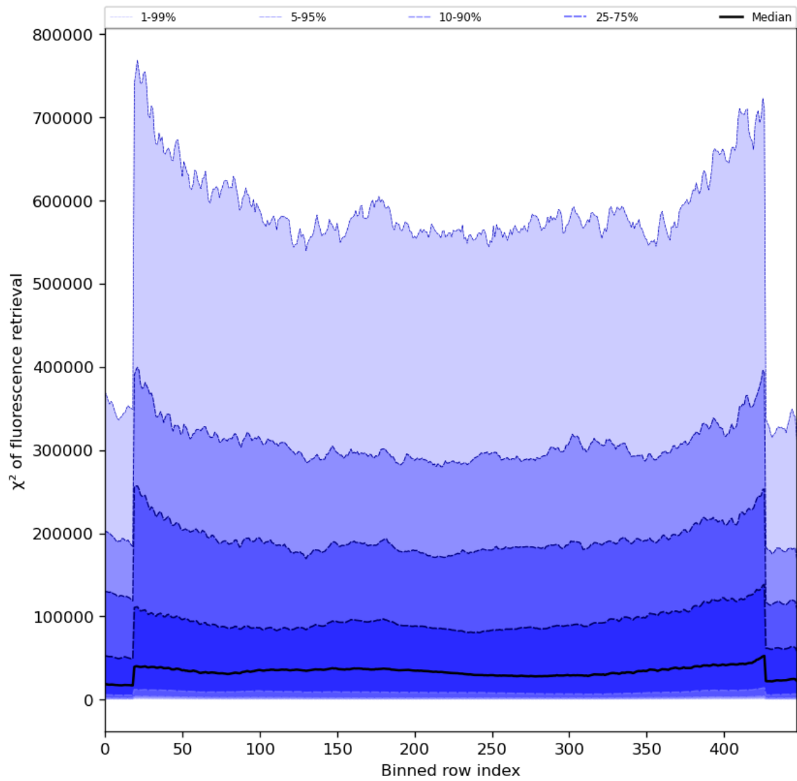
Figure 59: Along track statistics of “ \chi^2 of fluorescence retrieval” for 2024-07-03 to 2024-07-05
