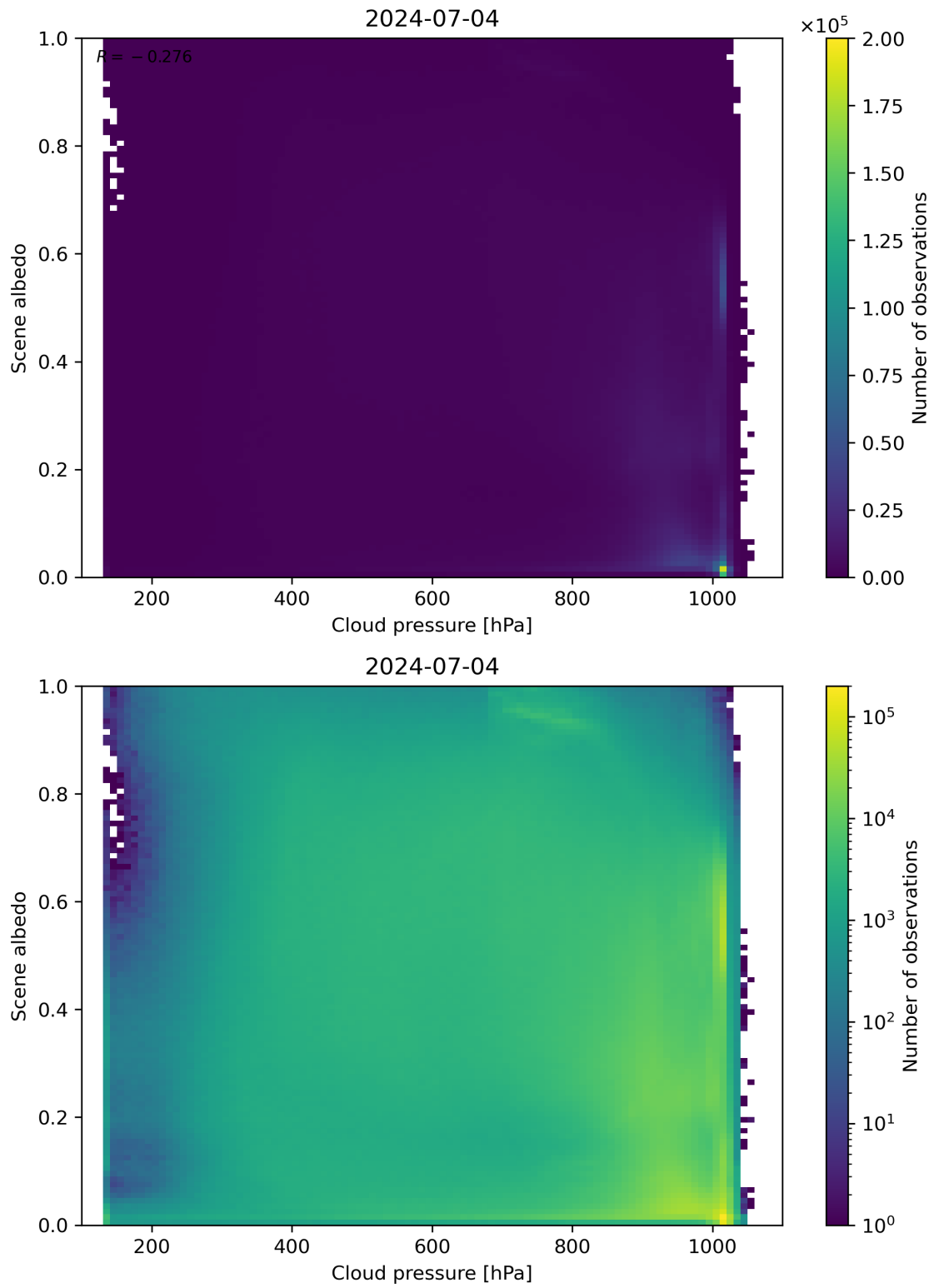
Figure 83: Scatter density plot of “Cloud pressure” against “Scene albedo” for 2024-07-03 to 2024-07-05.
