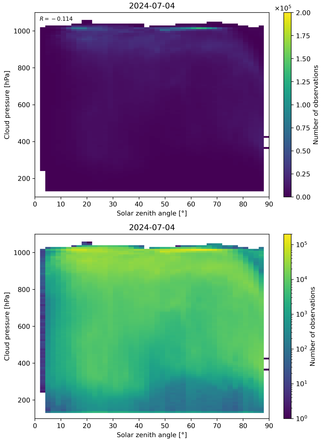
Figure 111: Scatter density plot of “Solar zenith angle” against “Cloud pressure” for 2024-07-03 to 2024-07-05.
