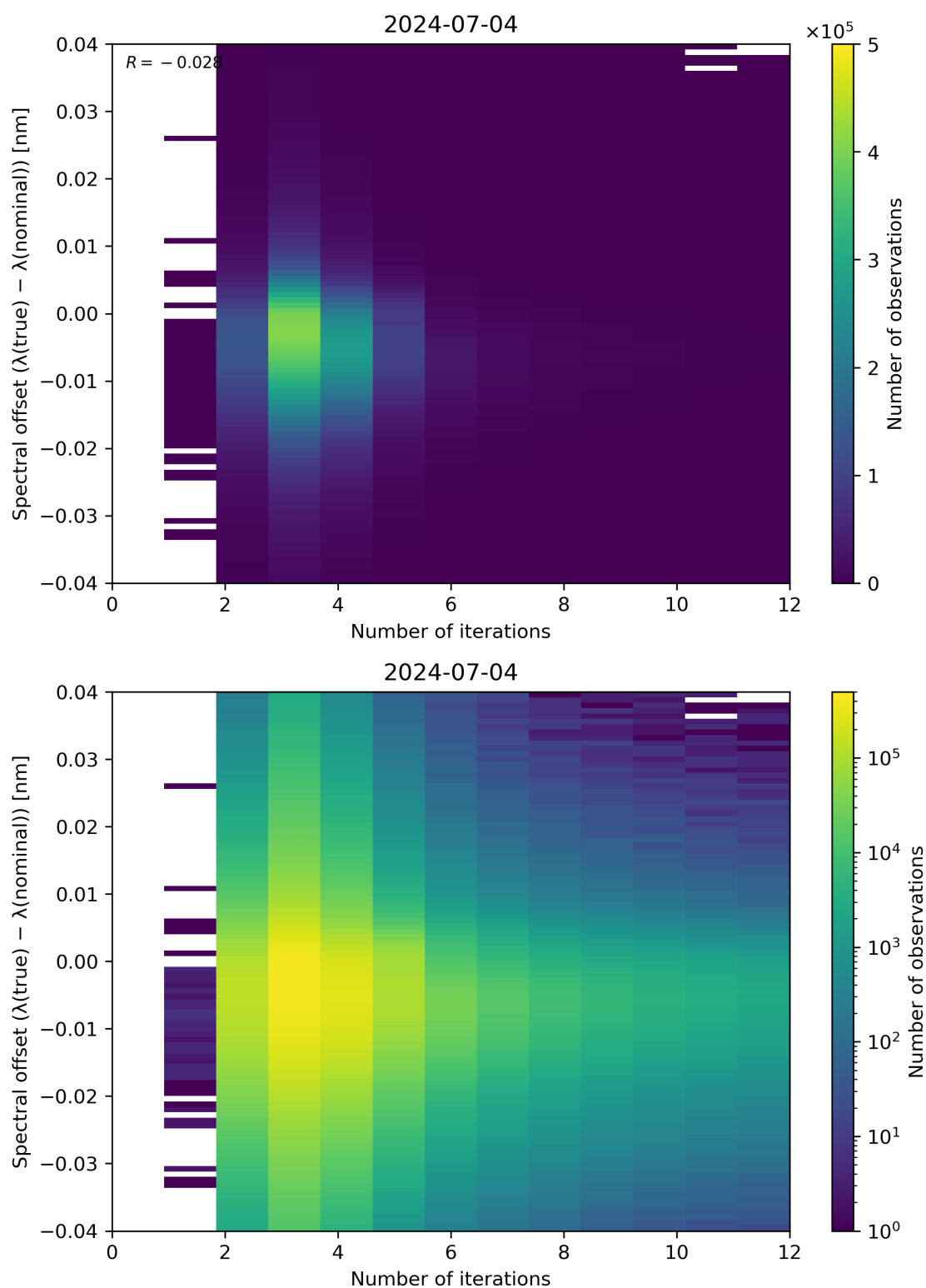
Figure 100: Scatter density plot of “Number of iterations” against “Spectral offset ( \lambda(\text{true}) - \lambda(\text{nominal}) )” for 2024-07-03 to 2024-07-05.
