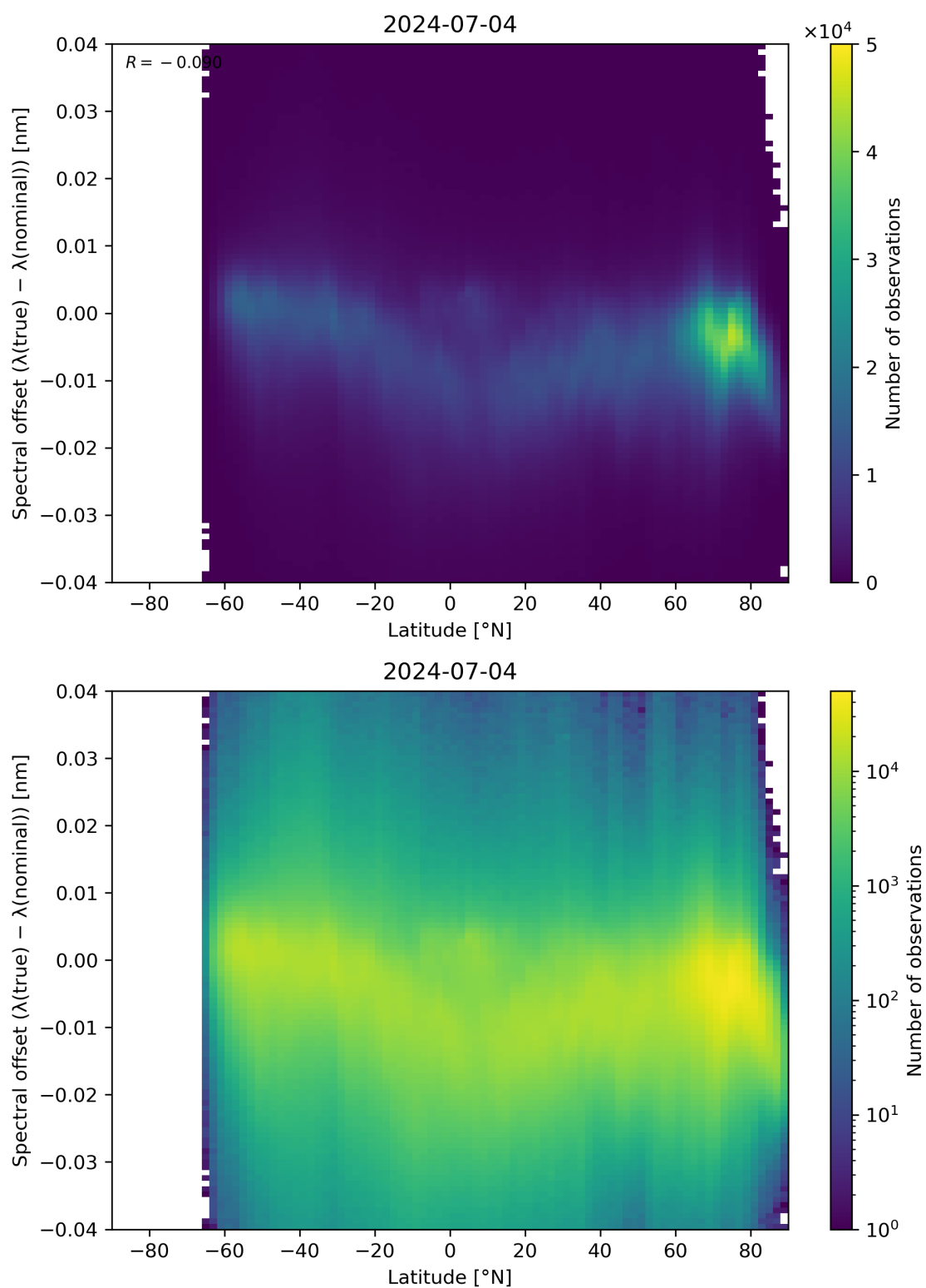
Figure 96: Scatter density plot of “Latitude” against “Spectral offset ( \lambda(\text{true}) - \lambda(\text{nominal}) )” for 2024-07-03 to 2024-07-05.
