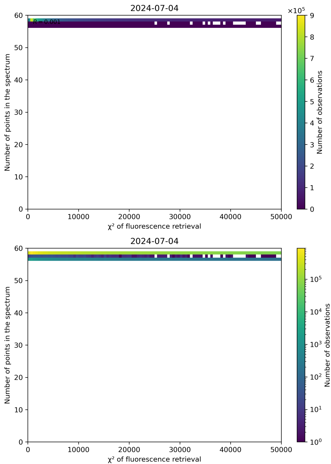
Figure 68: Scatter density plot of " \chi^2 of fluorescence retrieval" against "Number of points in the spectrum" for 2024-07-03 to 2024-07-05.
