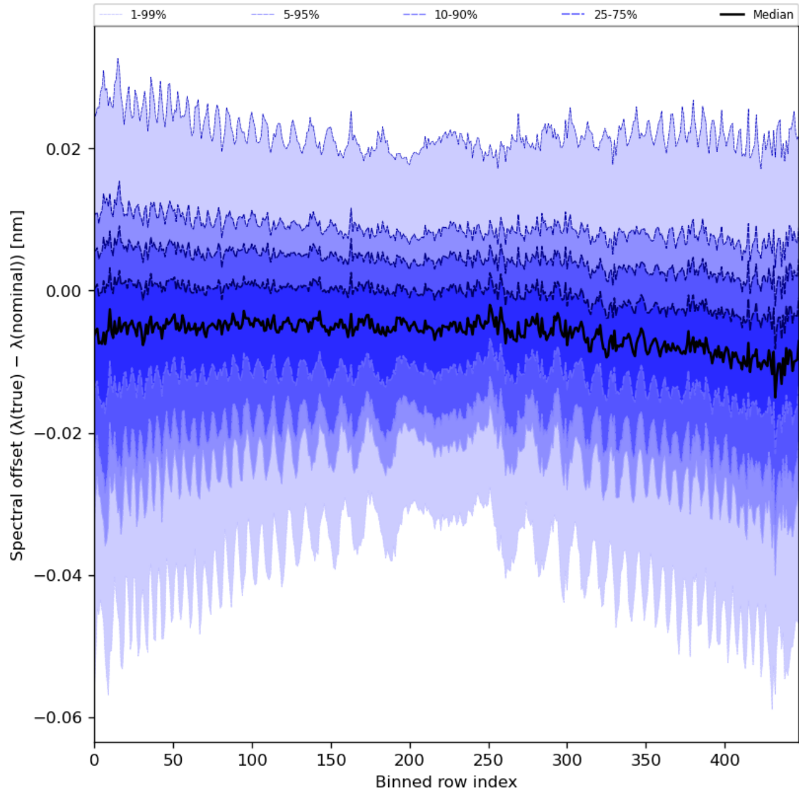
Figure 62: Along track statistics of “Spectral offset ( \lambda(\text{true}) - \lambda(\text{nominal}) )” for 2024-07-03 to 2024-07-05
