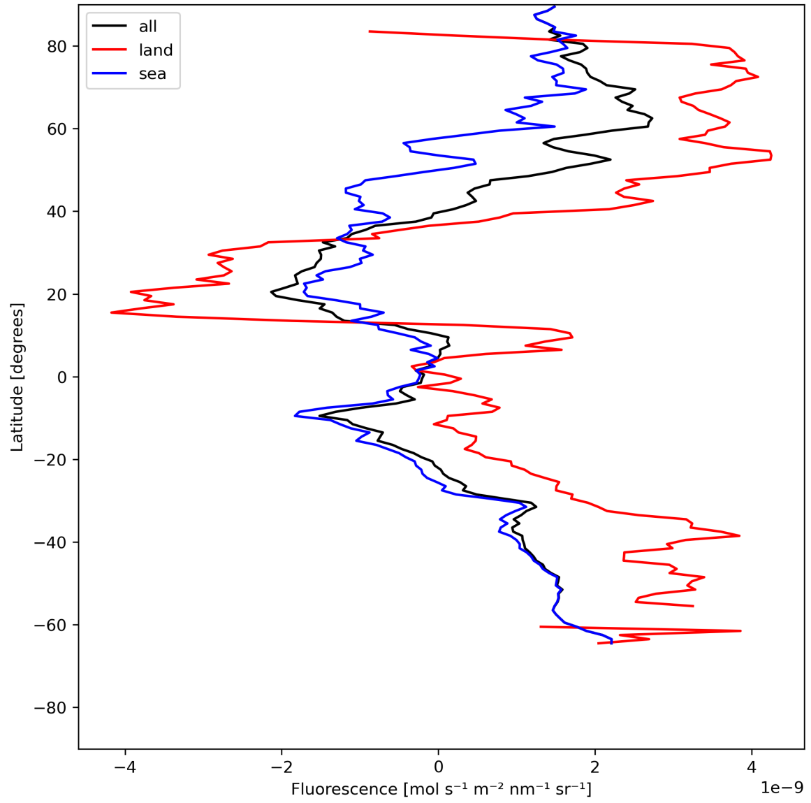
Figure 23: Zonal average of “Fluorescence” for 2024-07-03 to 2024-07-05.
