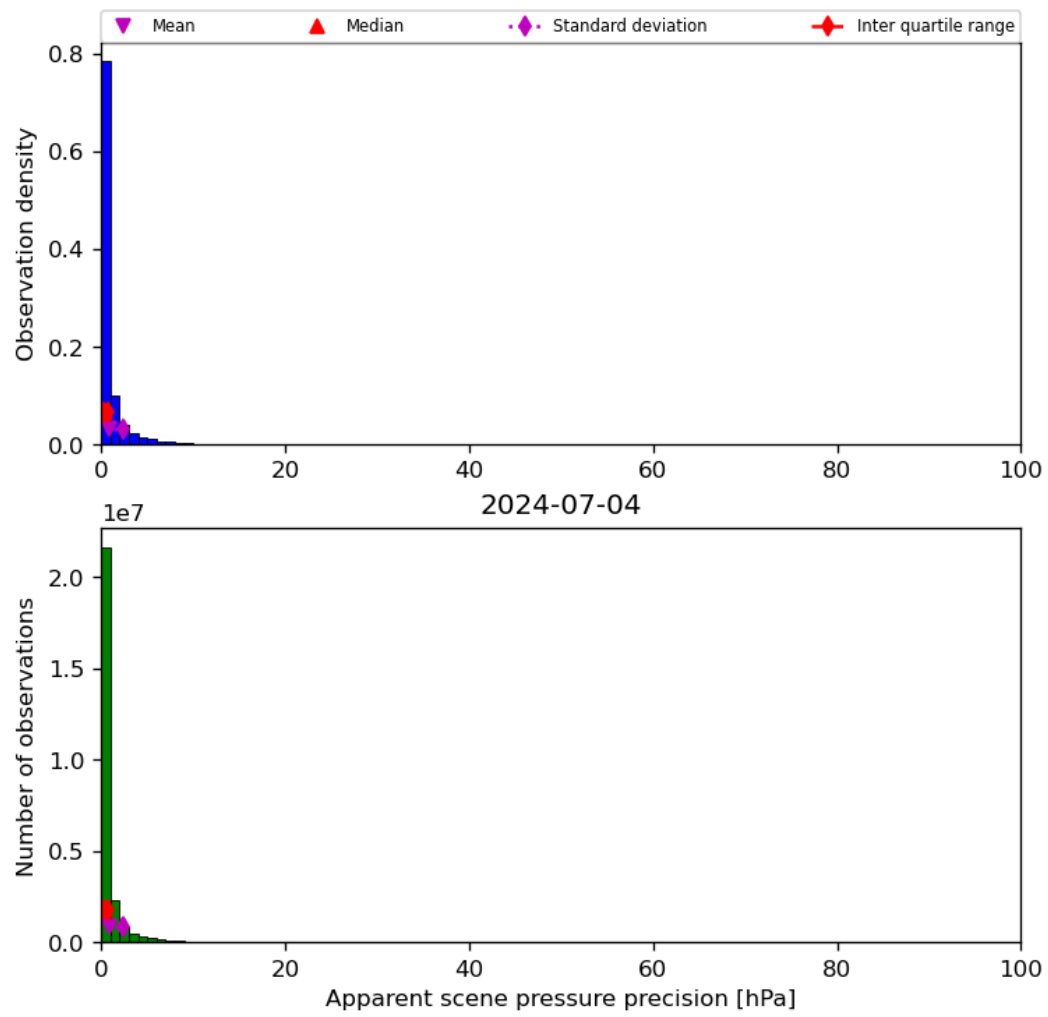
Figure 37: Histogram of “Apparent scene pressure precision” for 2024-07-03 to 2024-07-05
