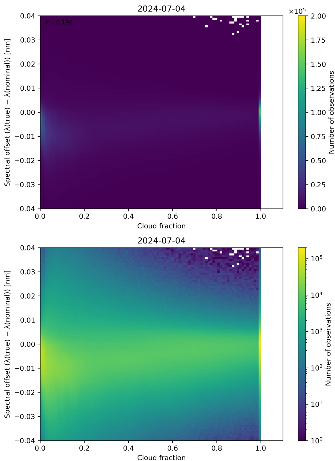
Figure 76: Scatter density plot of “Cloud fraction” against “Spectral offset ( \lambda(\text{true}) - \lambda(\text{nominal}) )” for 2024-07-03 to 2024-07-05.
