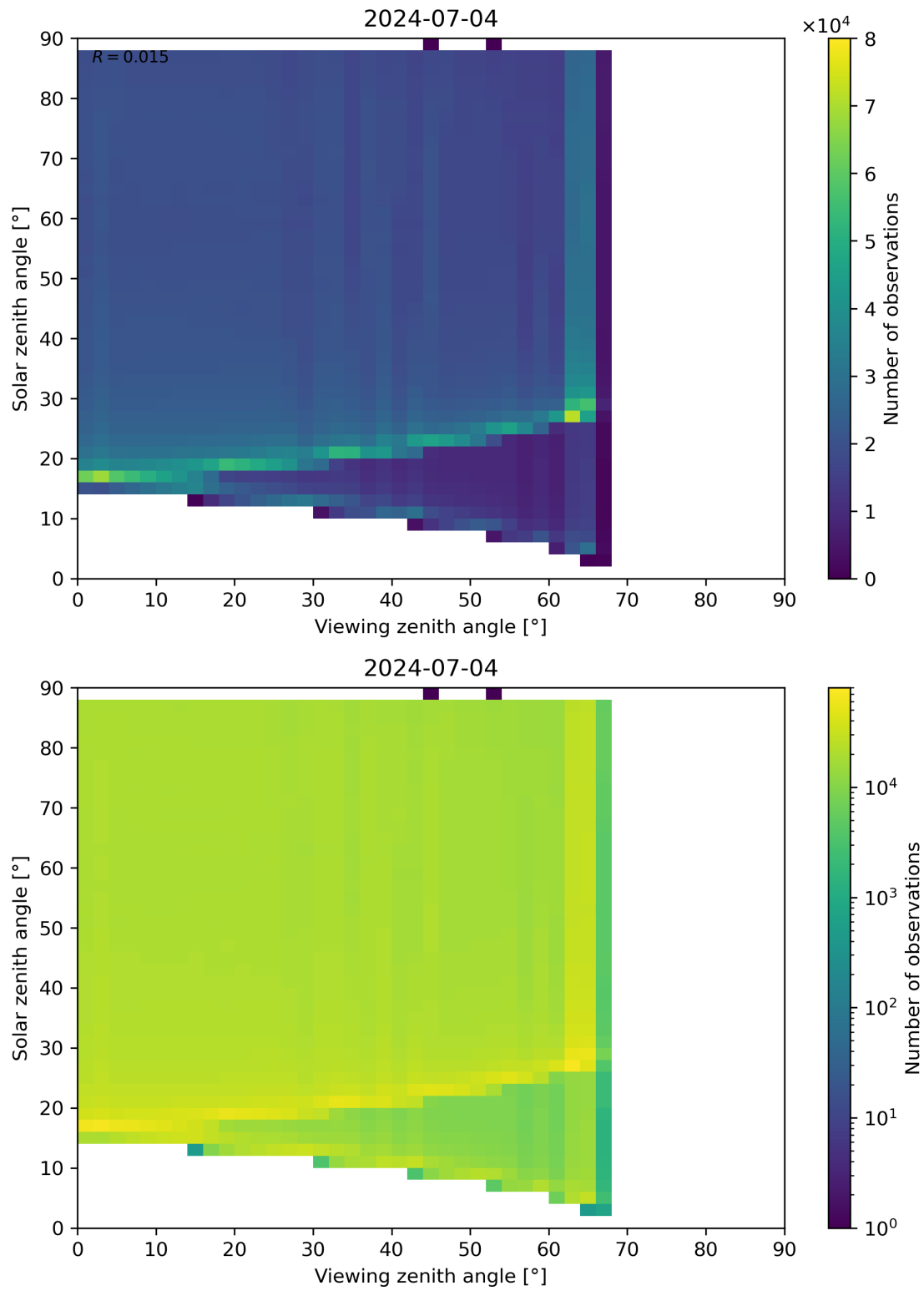
Figure 127: Scatter density plot of “Viewing zenith angle” against “Solar zenith angle” for 2024-07-03 to 2024-07-05.
