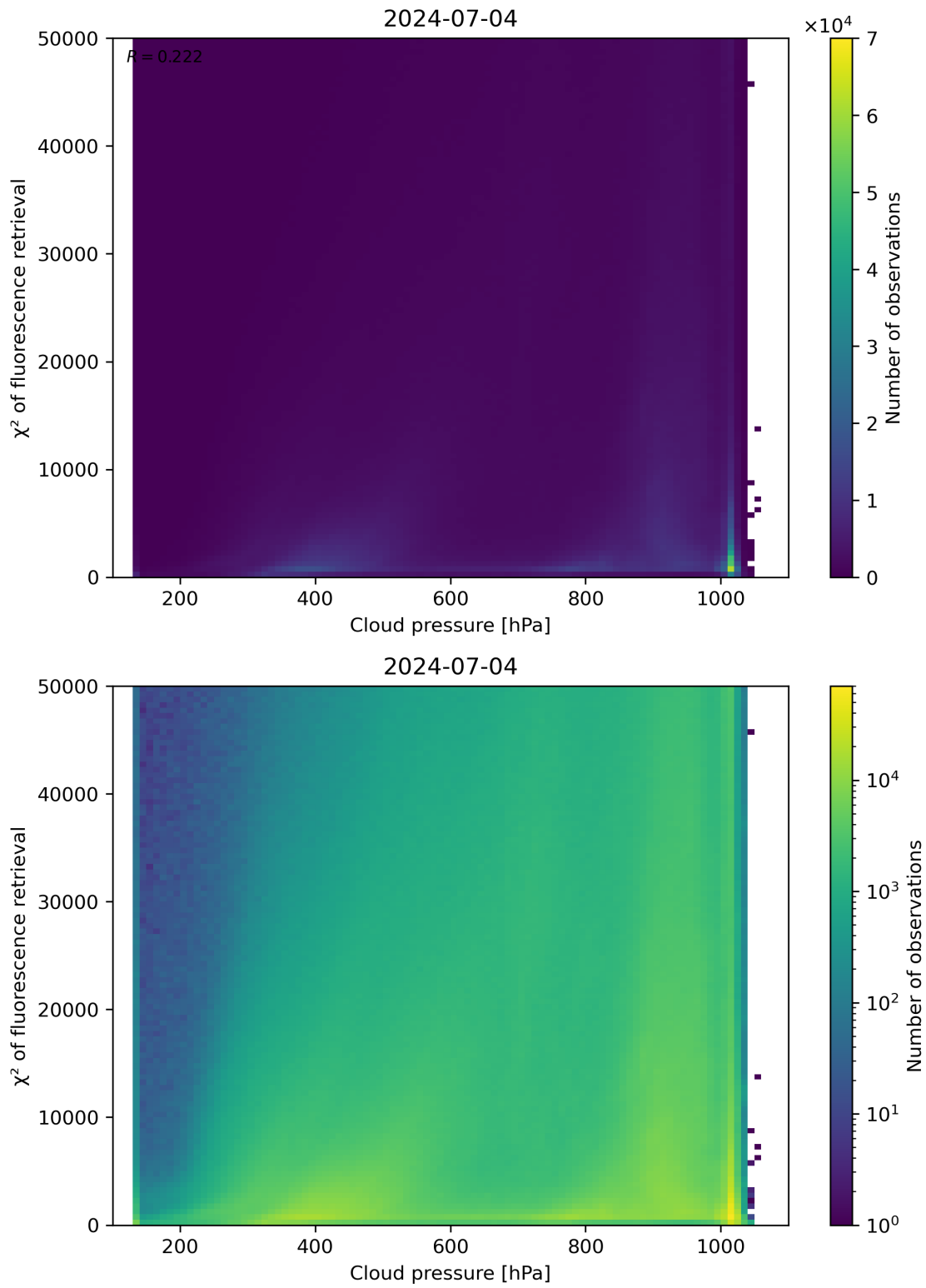
Figure 78: Scatter density plot of “Cloud pressure” against “ \chi^2 of fluorescence retrieval” for 2024-07-03 to 2024-07-05.
