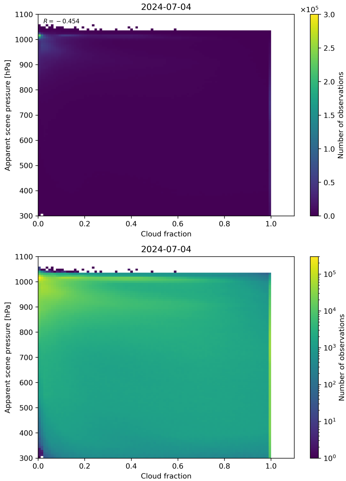
Figure 70: Scatter density plot of “Cloud fraction” against “Apparent scene pressure” for 2024-07-03 to 2024-07-05.
