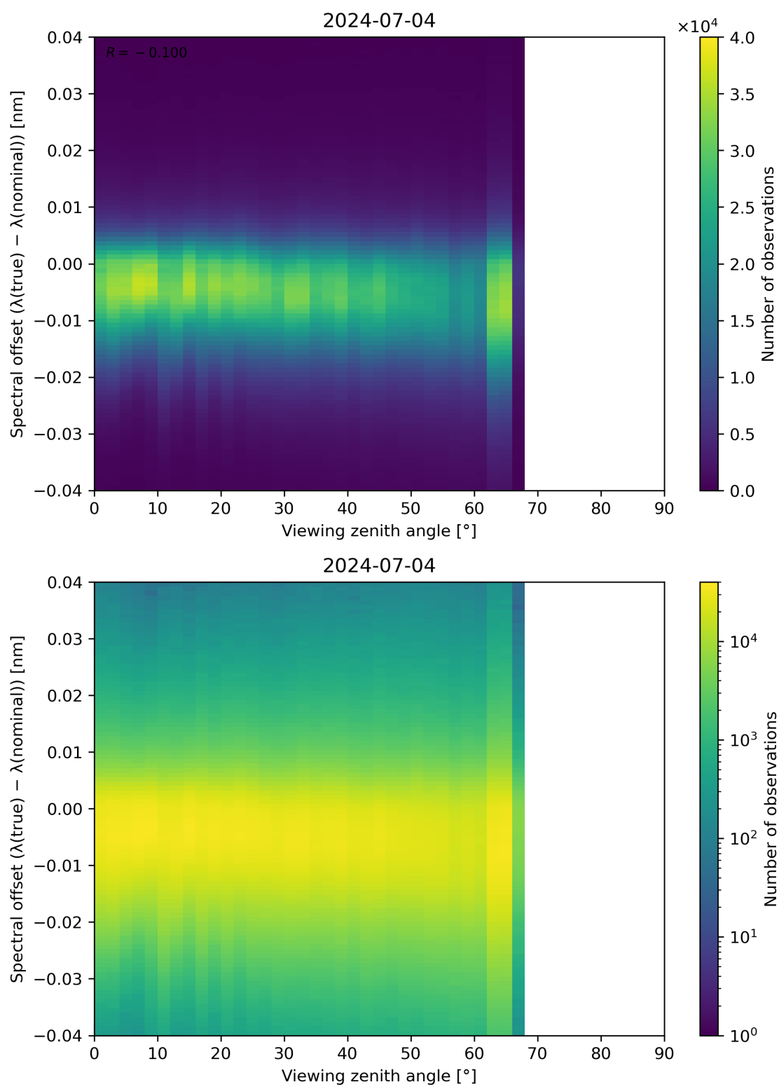
Figure 128: Scatter density plot of “Viewing zenith angle” against “Spectral offset ( \lambda(\text{true}) - \lambda(\text{nominal}) )” for 2024-07-03 to 2024-07-05.
