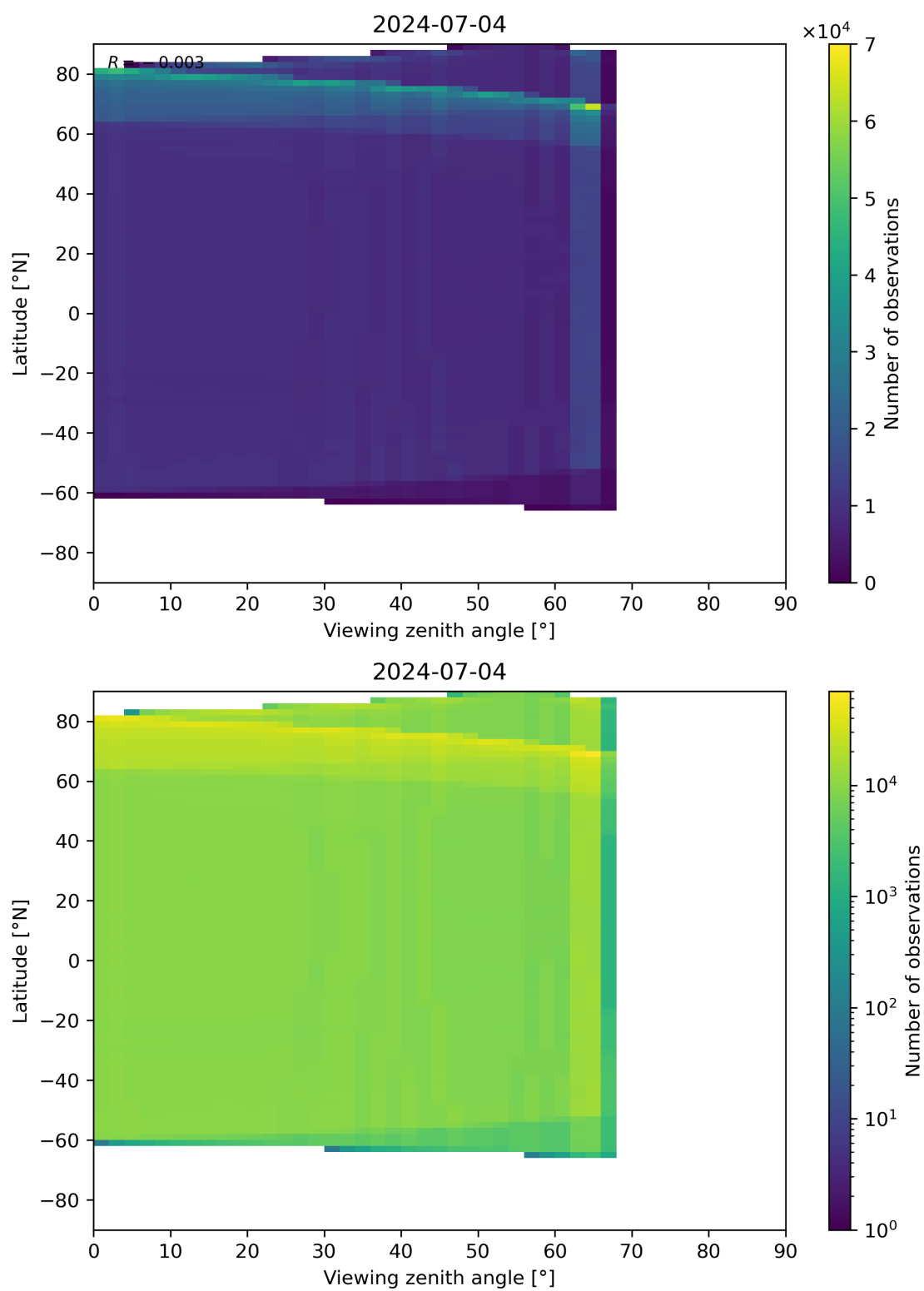
Figure 123: Scatter density plot of “Viewing zenith angle” against “Latitude” for 2024-07-03 to 2024-07-05.
