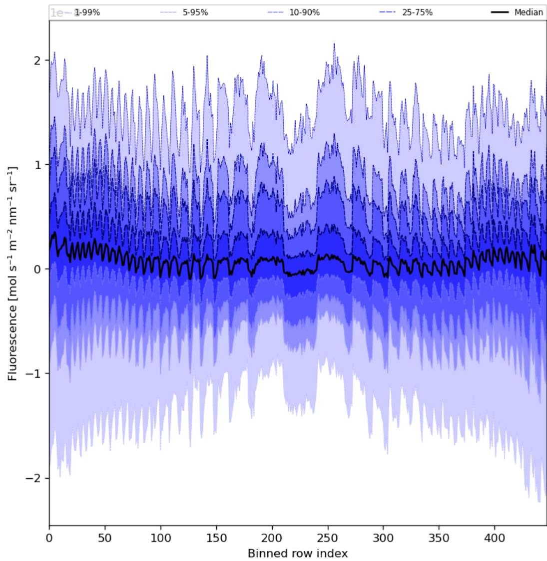
Figure 57: Along track statistics of “Fluorescence” for 2024-07-03 to 2024-07-05
