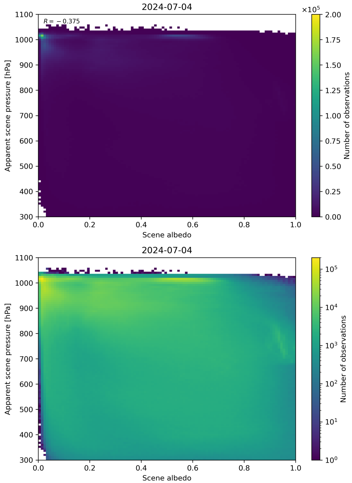
Figure 102: Scatter density plot of “Scene albedo” against “Apparent scene pressure” for 2024-07-03 to 2024-07-05.
