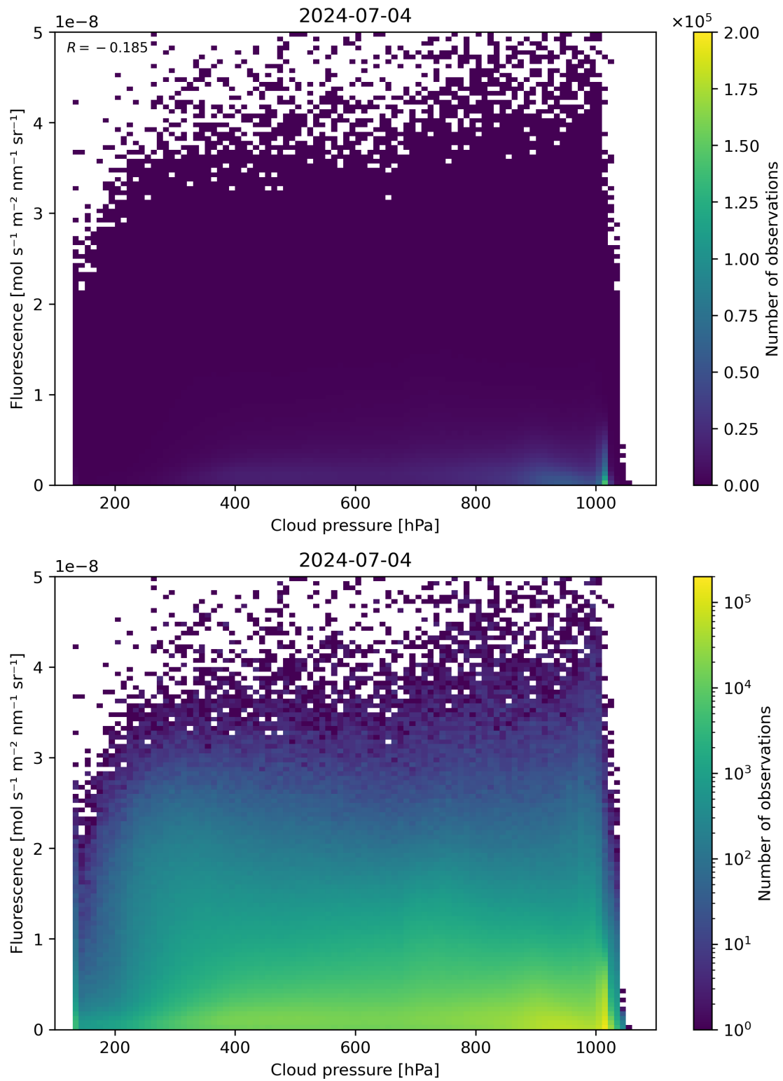
Figure 80: Scatter density plot of “Cloud pressure” against “Fluorescence” for 2024-07-03 to 2024-07-05.
