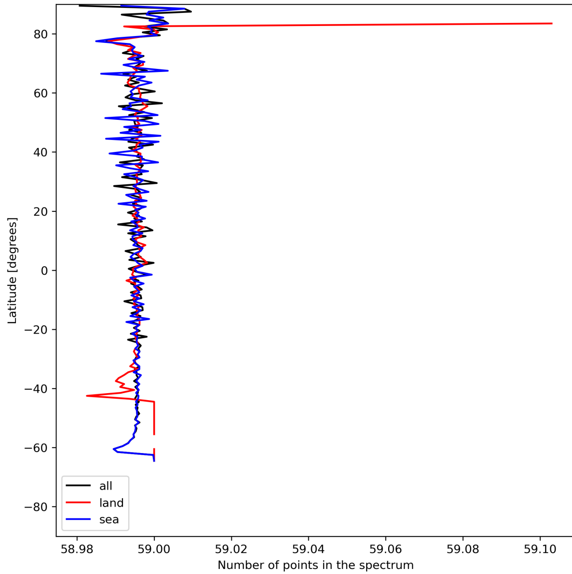
Figure 27: Zonal average of “Number of points in the spectrum” for 2024-07-03 to 2024-07-05.
