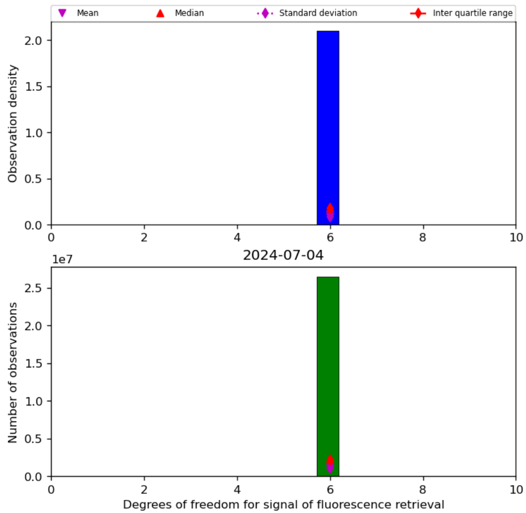
Figure 43: Histogram of “Degrees of freedom for signal of fluorescence retrieval” for 2024-07-03 to 2024-07-05
