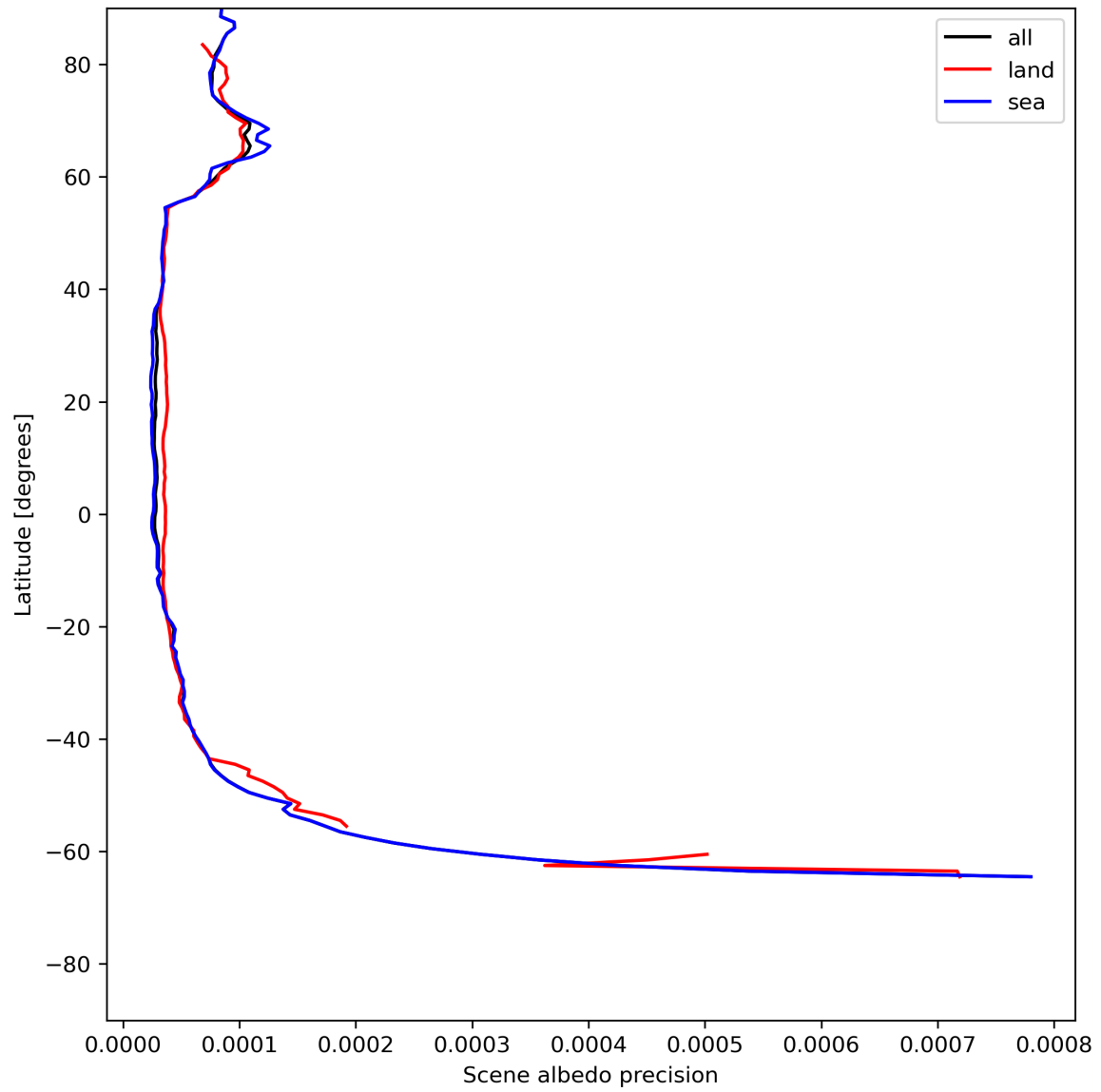
Figure 18: Zonal average of “Scene albedo precision” for 2024-07-03 to 2024-07-05.
