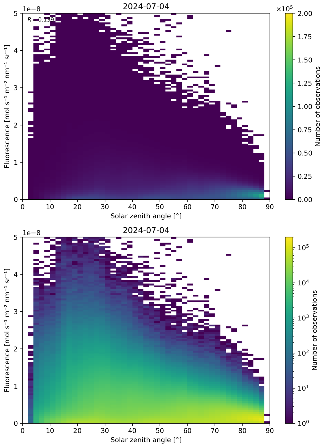
Figure 112: Scatter density plot of “Solar zenith angle” against “Fluorescence” for 2024-07-03 to 2024-07-05.
