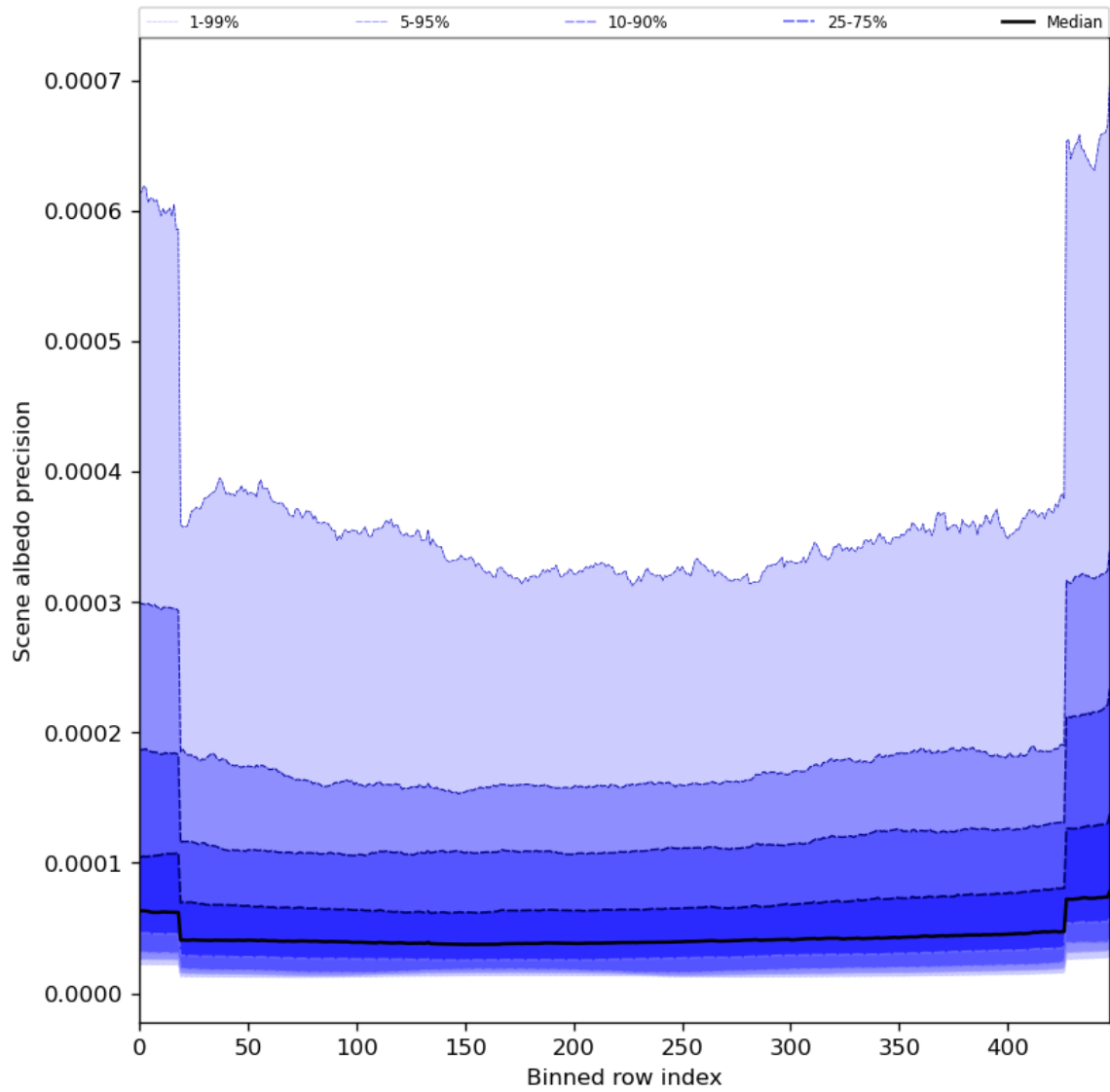
Figure 52: Along track statistics of “Scene albedo precision” for 2024-07-03 to 2024-07-05
