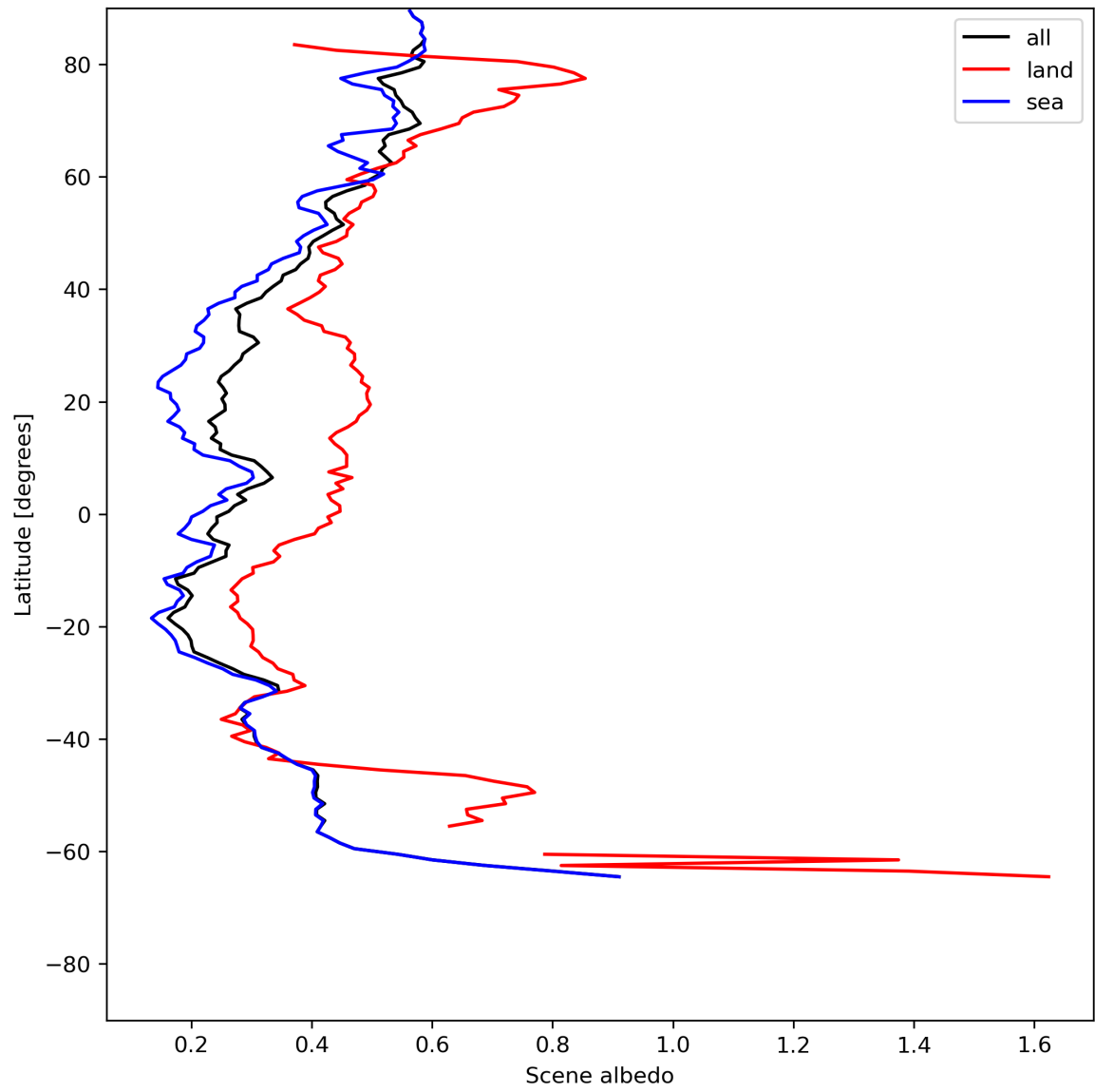
Figure 17: Zonal average of “Scene albedo” for 2024-07-03 to 2024-07-05.
