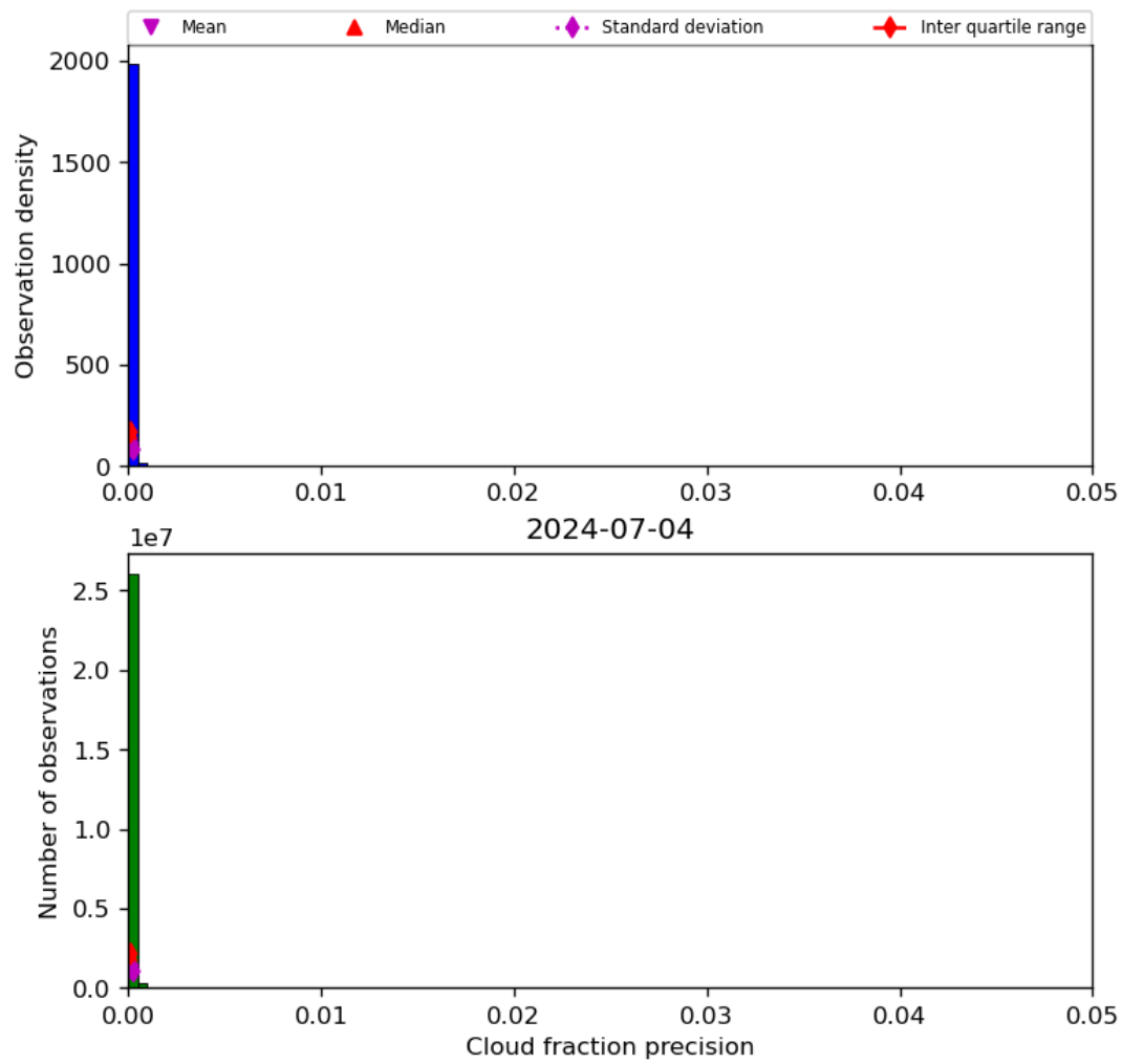
Figure 33: Histogram of “Cloud fraction precision” for 2024-07-03 to 2024-07-05
