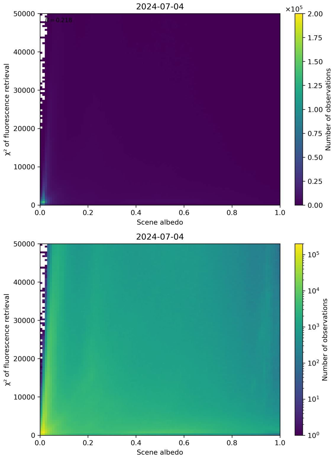
Figure 103: Scatter density plot of “Scene albedo” against “ \chi^2 of fluorescence retrieval” for 2024-07-03 to 2024-07-05.
