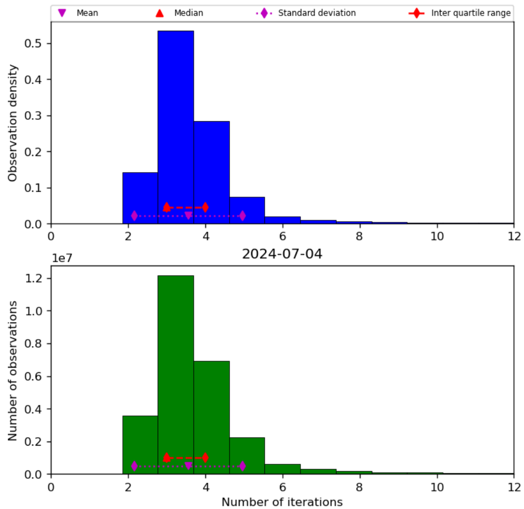
Figure 39: Histogram of “Number of iterations” for 2024-07-03 to 2024-07-05
