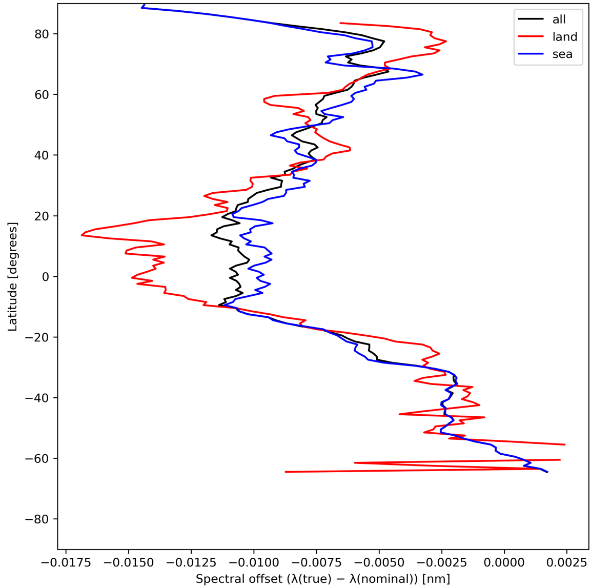
Figure 28: Zonal average of “Spectral offset ( \lambda(\text{true}) - \lambda(\text{nominal}) )” for 2024-07-03 to 2024-07-05.
