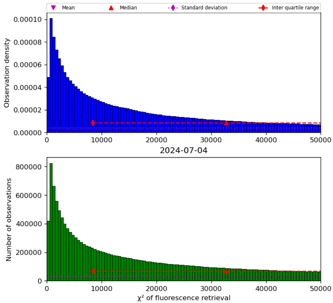
Figure 42: Histogram of “ \chi^2 of fluorescence retrieval” for 2024-07-03 to 2024-07-05
