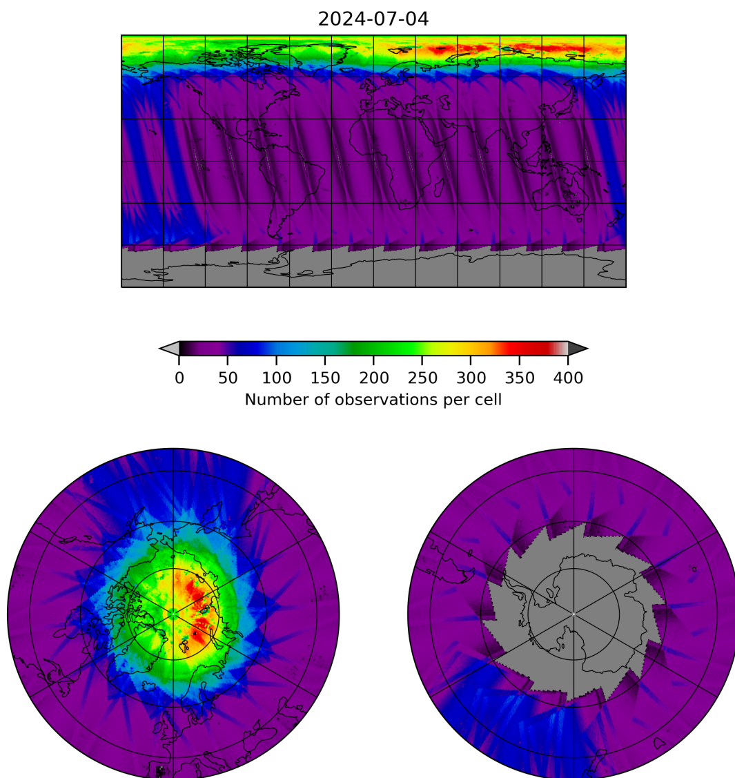
Figure 11: Map of the number of observations for 2024-07-03 to 2024-07-05
