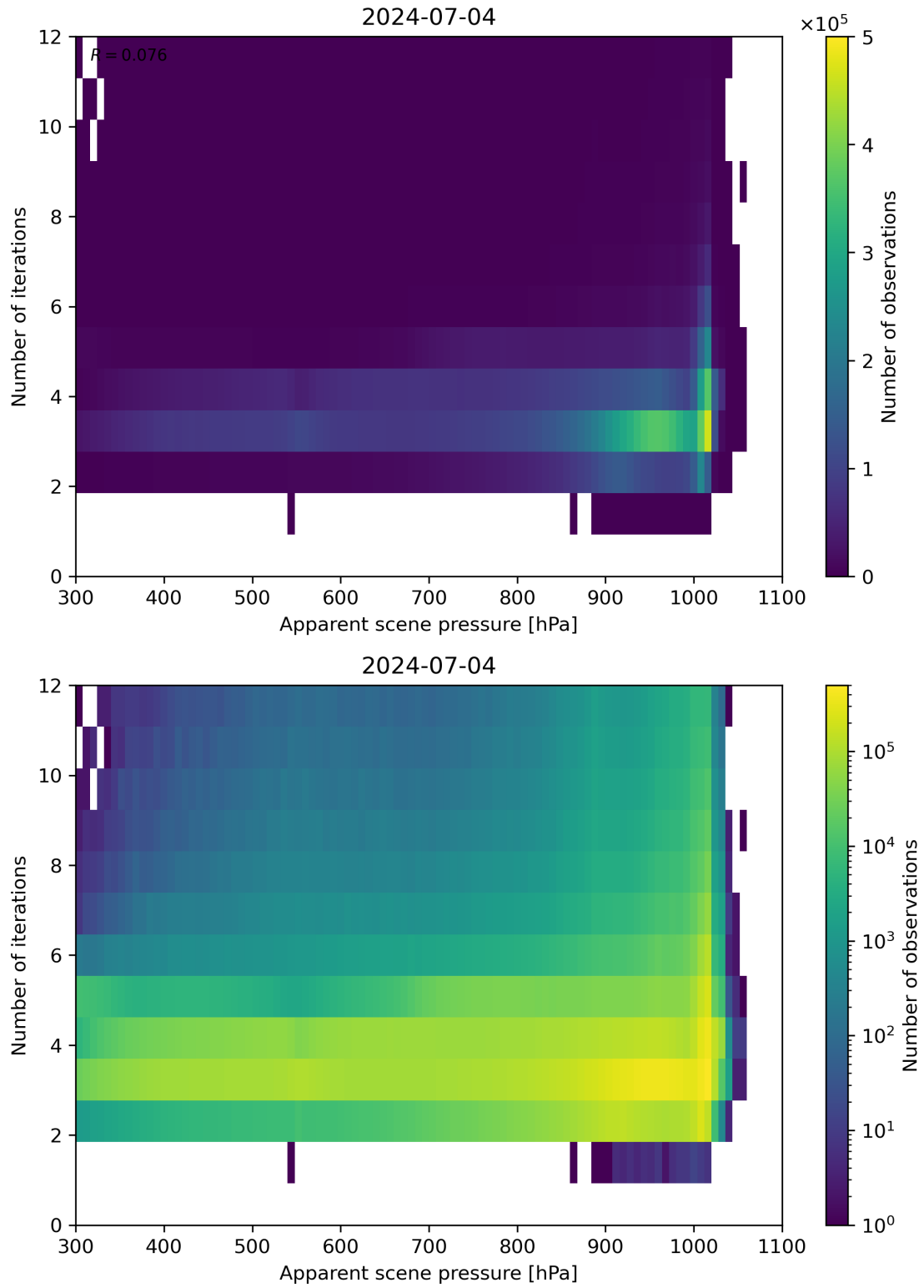
Figure 65: Scatter density plot of “Apparent scene pressure” against “Number of iterations” for 2024-07-03 to 2024-07-05.
