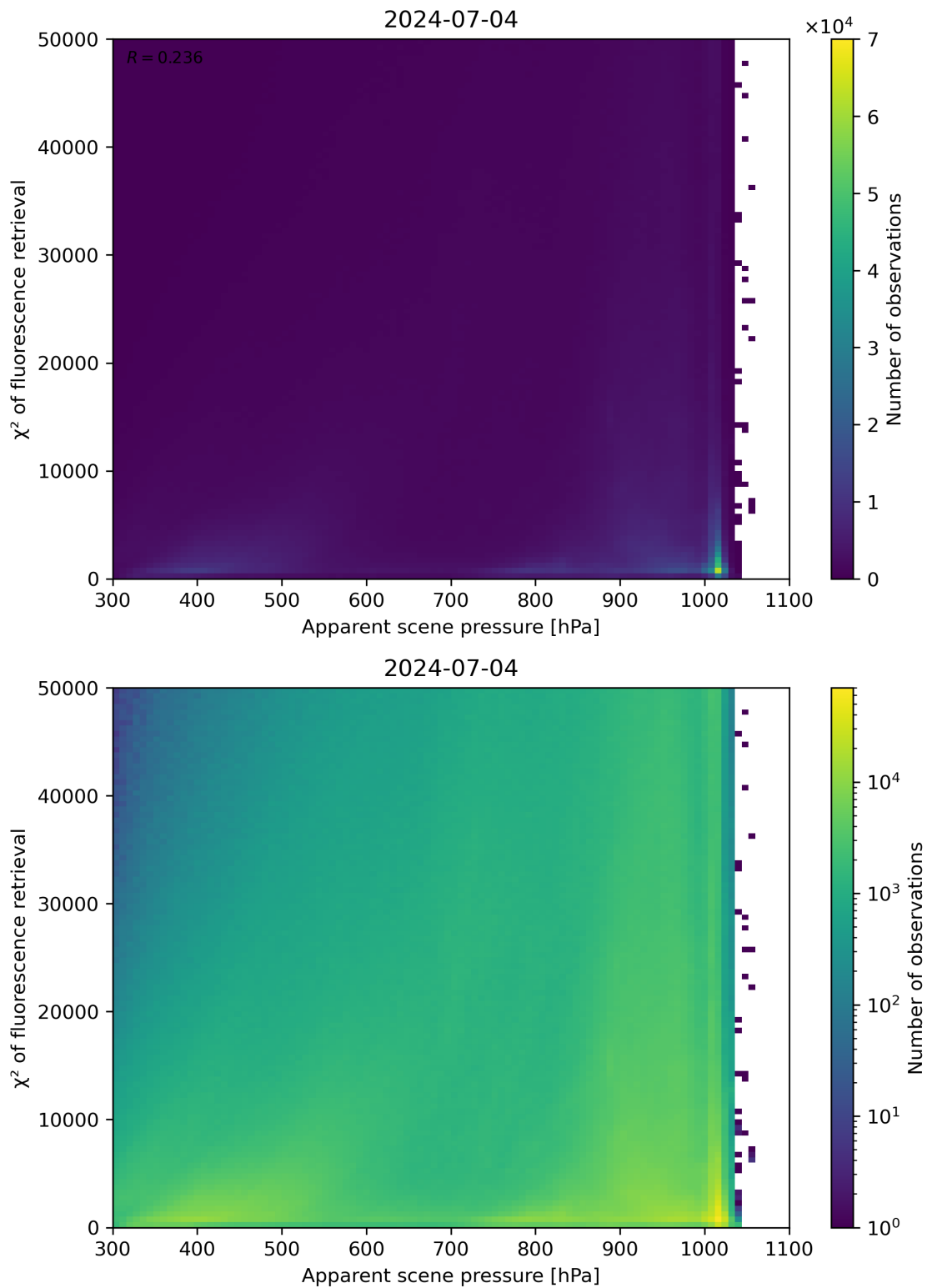
Figure 63: Scatter density plot of “Apparent scene pressure” against “ \chi^2 of fluorescence retrieval” for 2024-07-03 to 2024-07-05.
