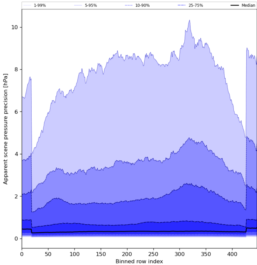
Figure 54: Along track statistics of “Apparent scene pressure precision” for 2024-07-03 to 2024-07-05
