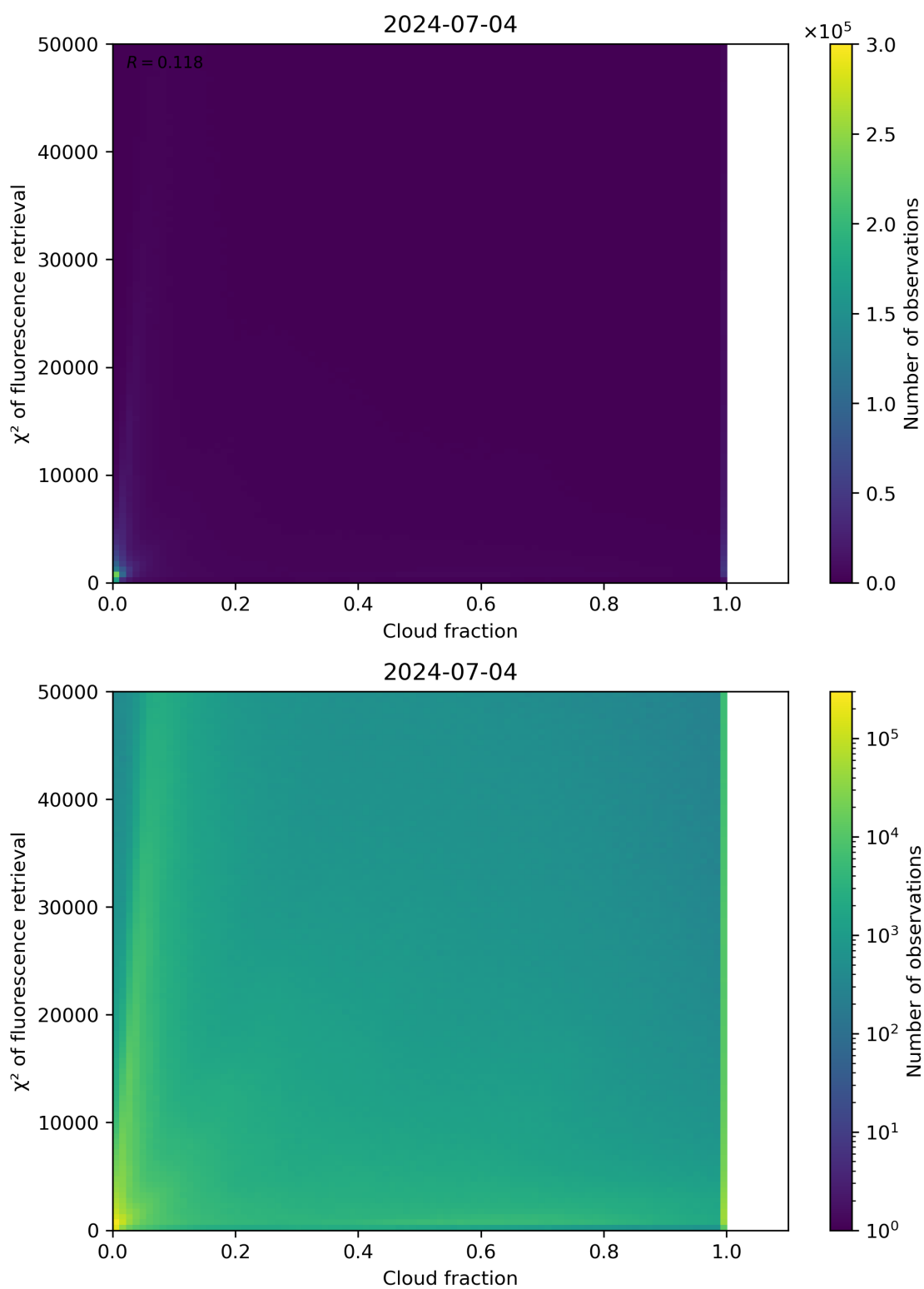
Figure 71: Scatter density plot of “Cloud fraction” against “ \chi^2 of fluorescence retrieval” for 2024-07-03 to 2024-07-05.
