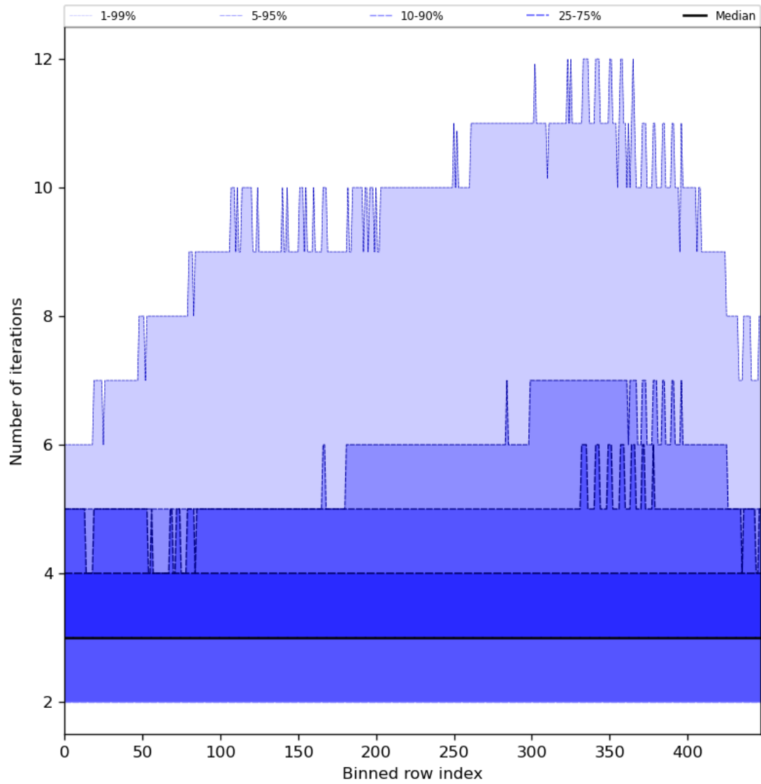
Figure 56: Along track statistics of “Number of iterations” for 2024-07-03 to 2024-07-05
