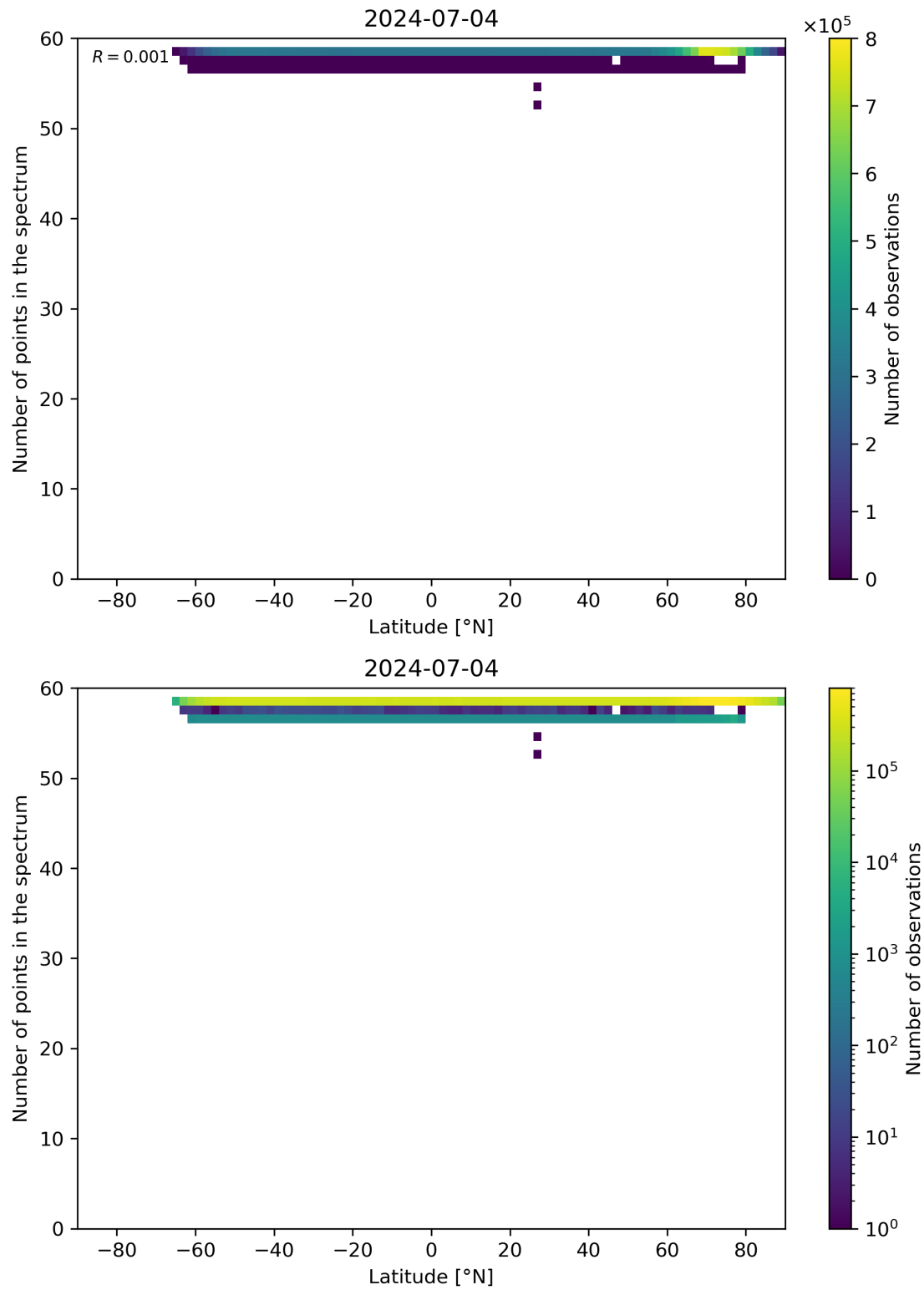
Figure 94: Scatter density plot of “Latitude” against “Number of points in the spectrum” for 2024-07-03 to 2024-07-05.
