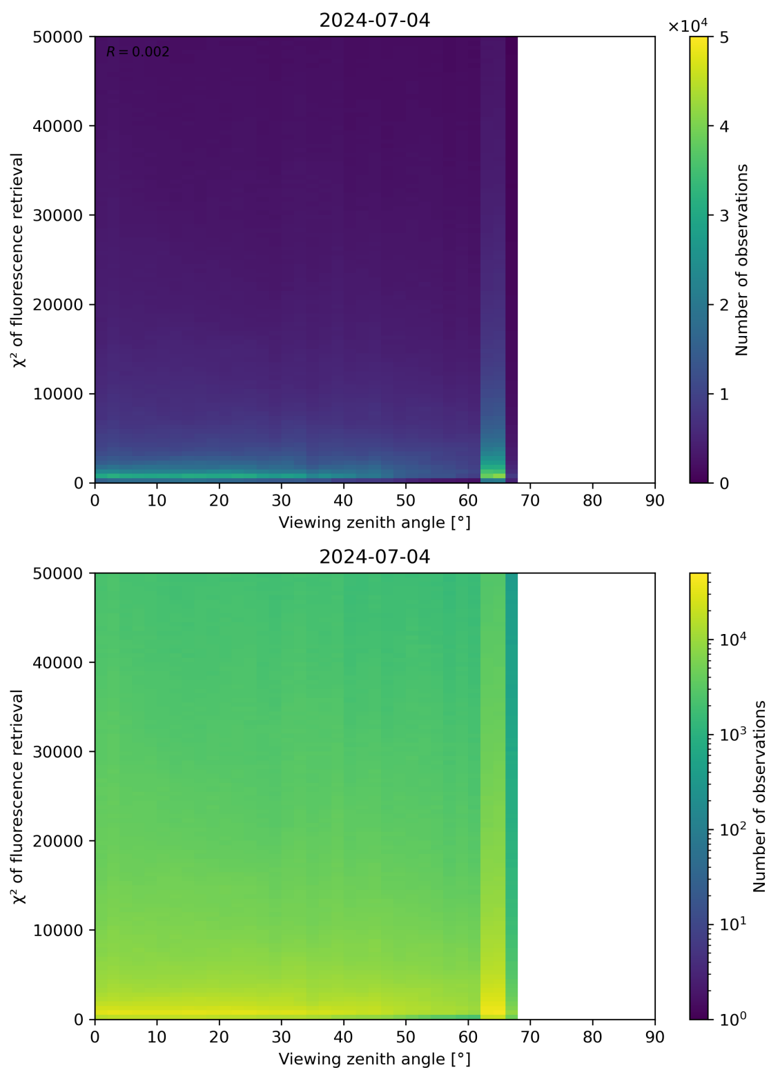
Figure 119: Scatter density plot of “Viewing zenith angle” against “ \chi^2 of fluorescence retrieval” for 2024-07-03 to 2024-07-05.
