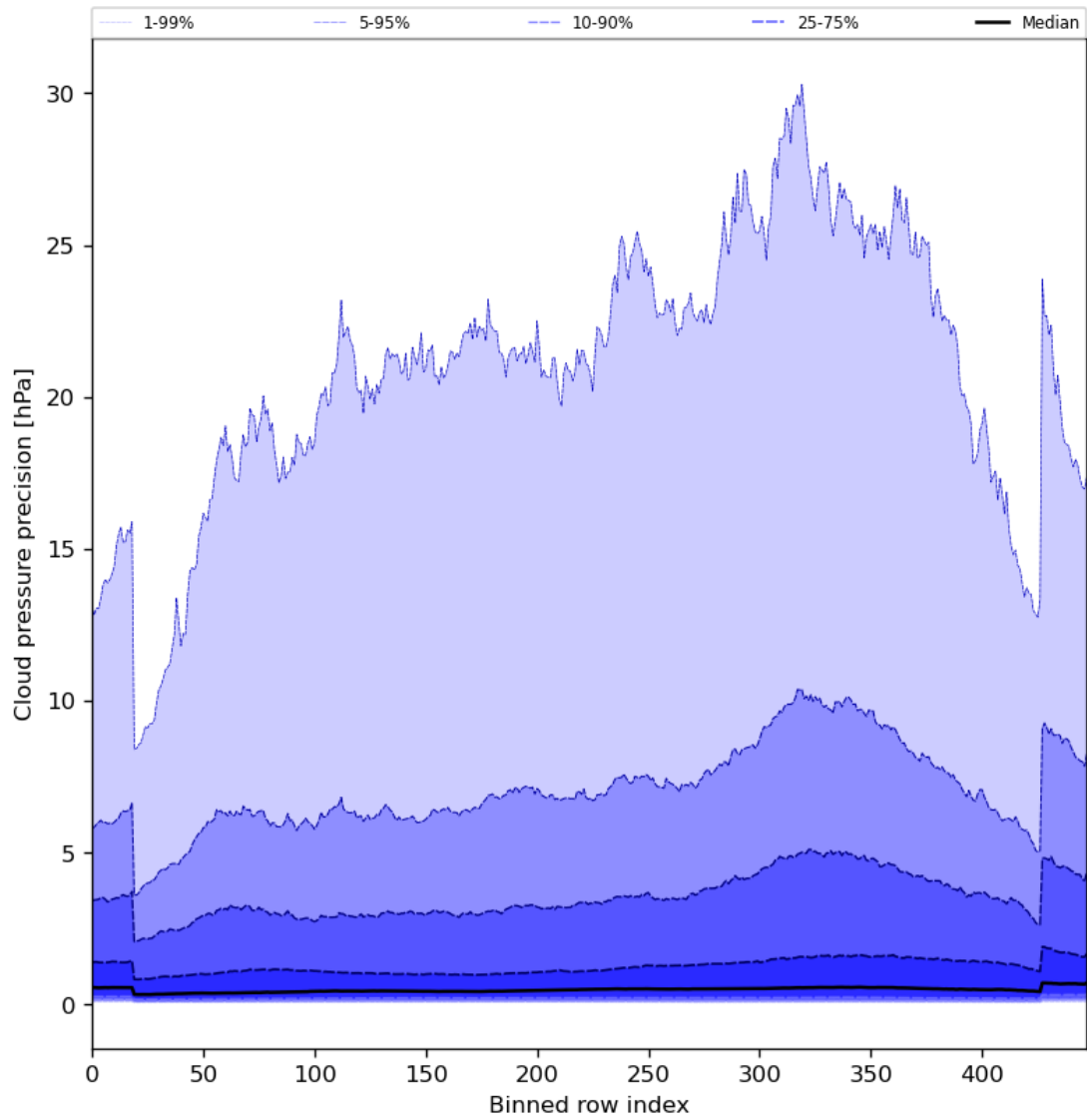
Figure 48: Along track statistics of “Cloud pressure precision” for 2024-07-03 to 2024-07-05
